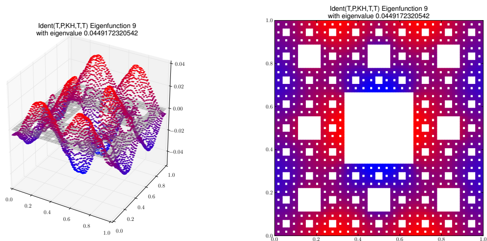
Eigenfunction 9 with eigenvalue 0.0449172320542
