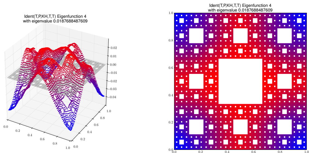
Eigenfunction 4 with eigenvalue 0.0187688487609
