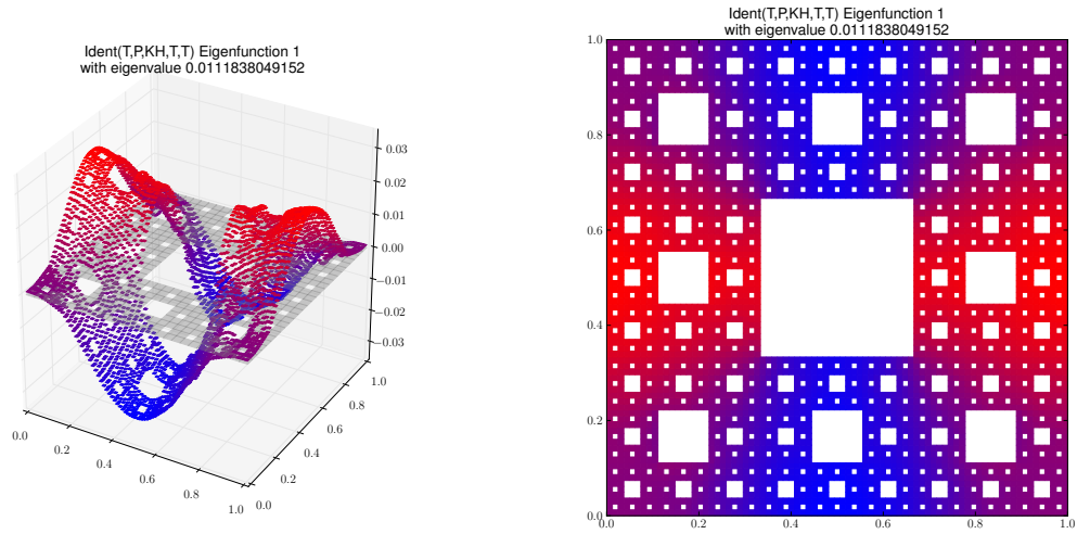
Eigenfunction 1 with eigenvalue 0.0111838049152
