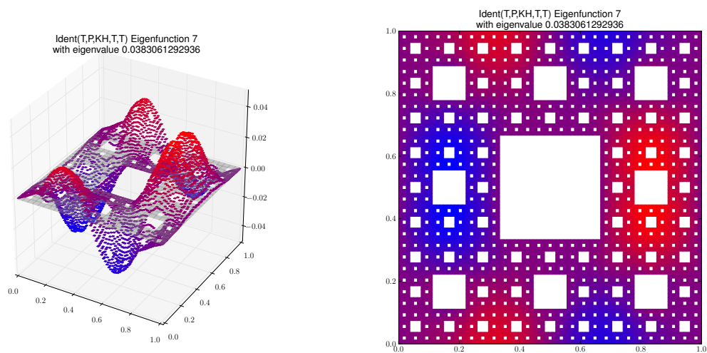
Eigenfunction 7 with eigenvalue 0.0383061292936
