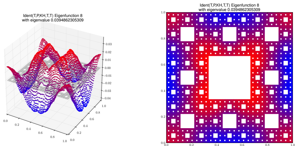
Eigenfunction 8 with eigenvalue 0.0394862305309
