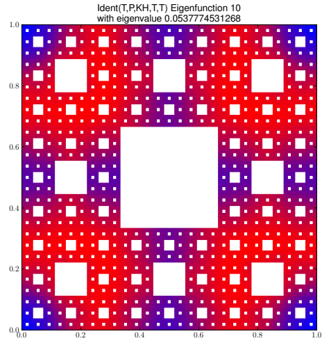
Eigenfunction 10 with eigenvalue 0.0537774531268
