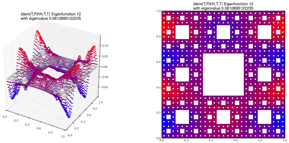
Eigenfunction 12 with eigenvalue 0.0610895122235
