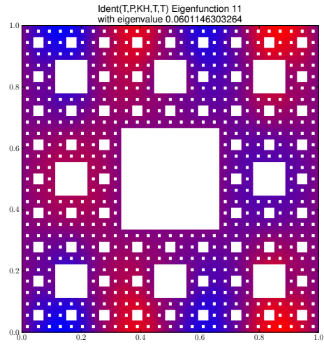
Eigenfunction 11 with eigenvalue 0.0601146303264
