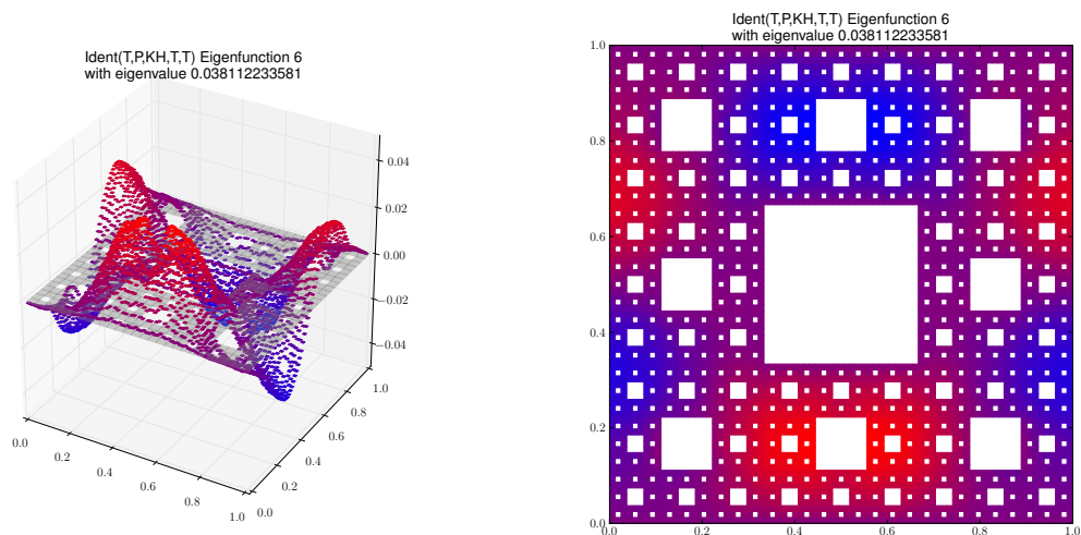
Eigenfunction 6 with eigenvalue 0.038112233581
