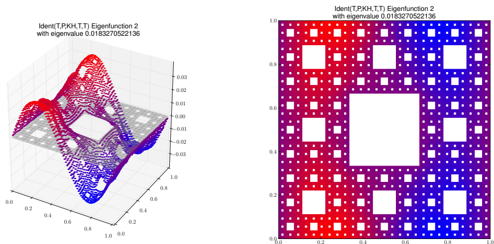
Eigenfunction 2 with eigenvalue 0.0183270522136
