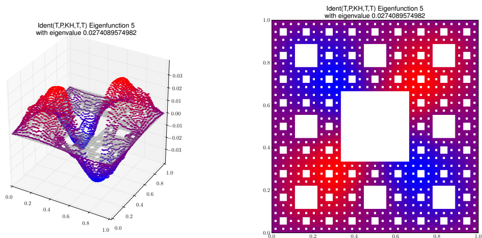
Eigenfunction 5 with eigenvalue 0.0274089574982
