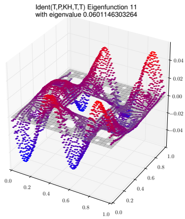
Eigenfunction 11 with eigenvalue 0.0601146303264
