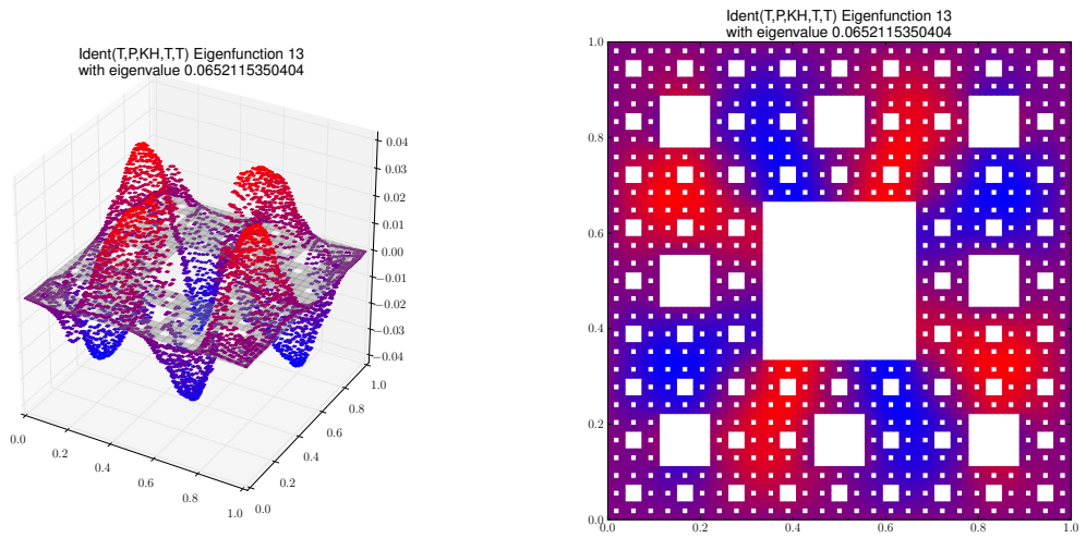
Eigenfunction 13 with eigenvalue 0.0652115350404
