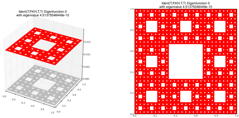
Eigenfunction 0 with eigenvalue 4.51375048449e-15
