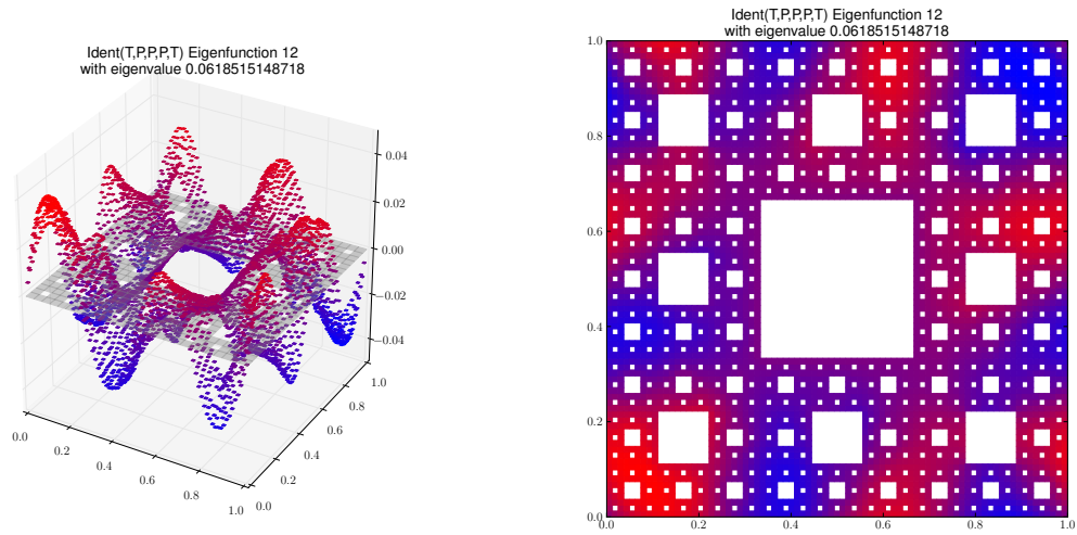
Eigenfunction 12 with eigenvalue 0.0618515148718
