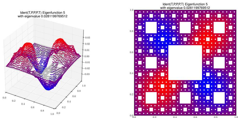
Eigenfunction 5 with eigenvalue 0.0281199769512
