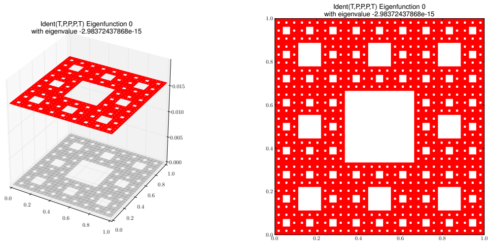
Eigenfunction 0 with eigenvalue -2.98372437868e-15
