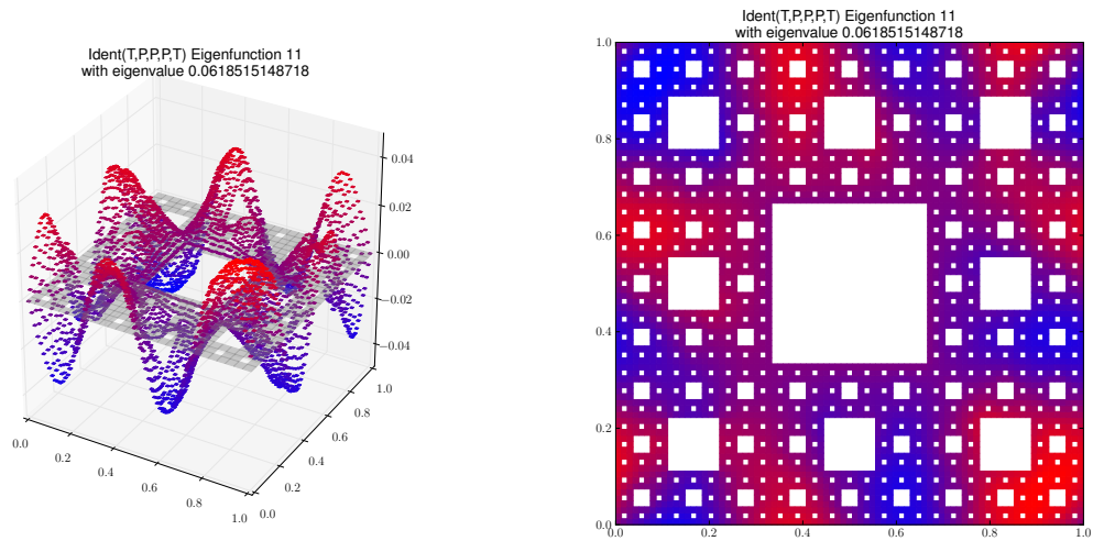
Eigenfunction 11 with eigenvalue 0.0618515148718
