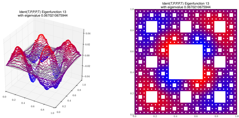
Eigenfunction 13 with eigenvalue 0.0670210675944
