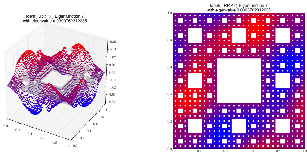
Eigenfunction 7 with eigenvalue 0.0390762312235
