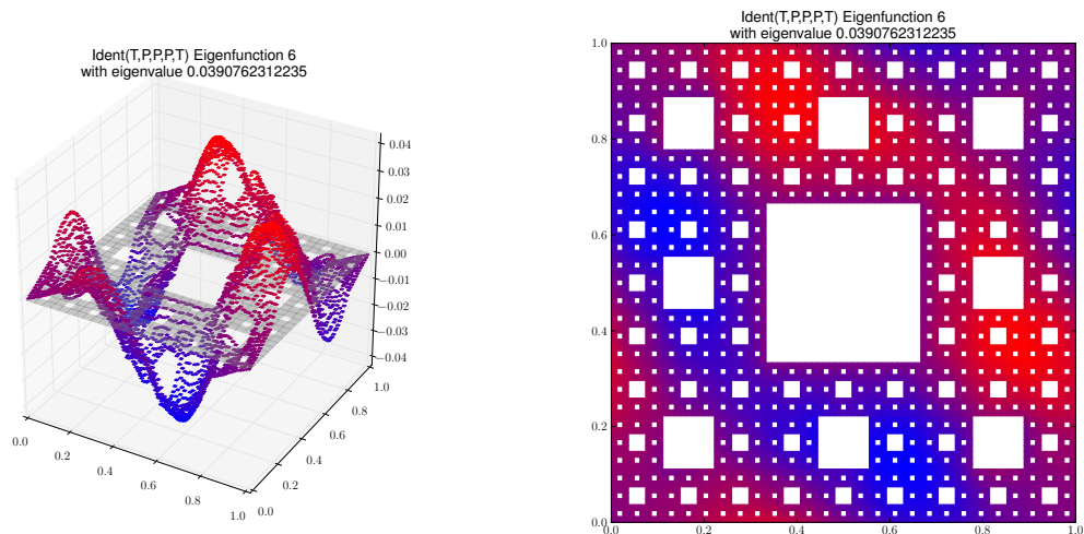
Eigenfunction 6 with eigenvalue 0.0390762312235
