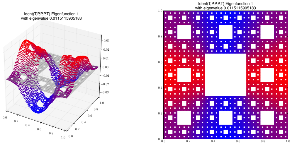
Eigenfunction 1 with eigenvalue 0.0115115905183
