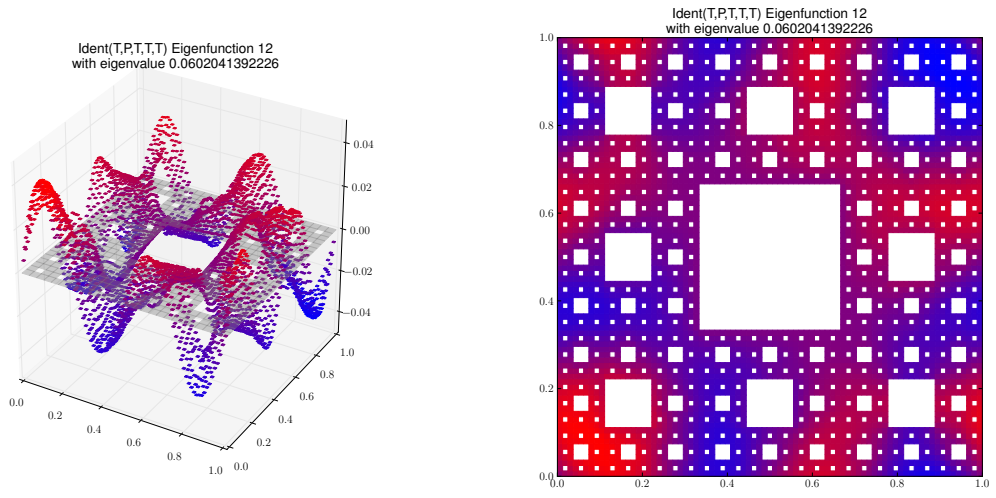
Eigenfunction 12 with eigenvalue 0.0602041392226
