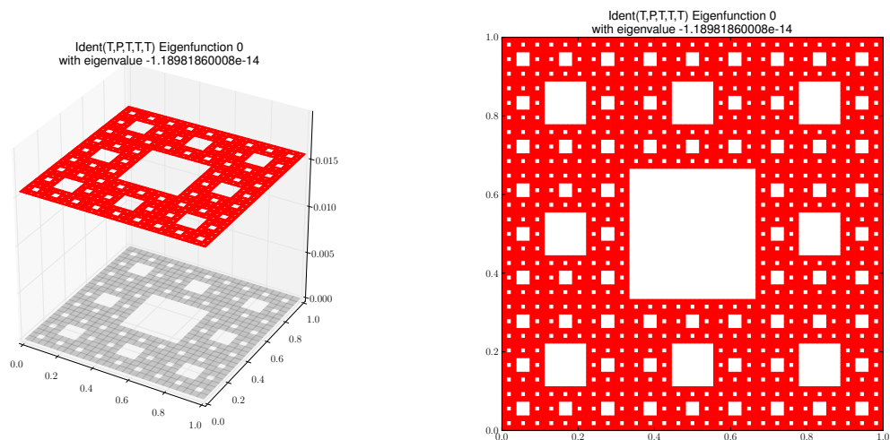
Eigenfunction 0 with eigenvalue -1.18981860008e-14
