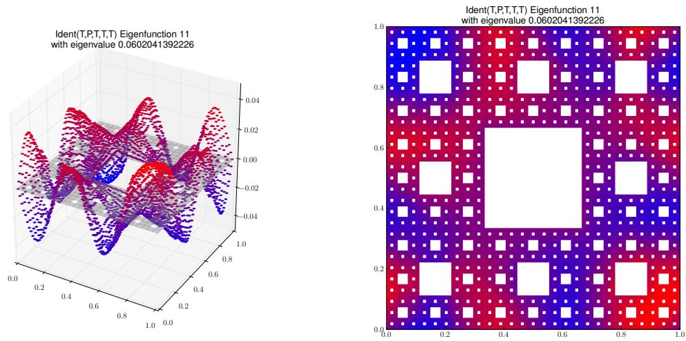
Eigenfunction 11 with eigenvalue 0.0602041392226
