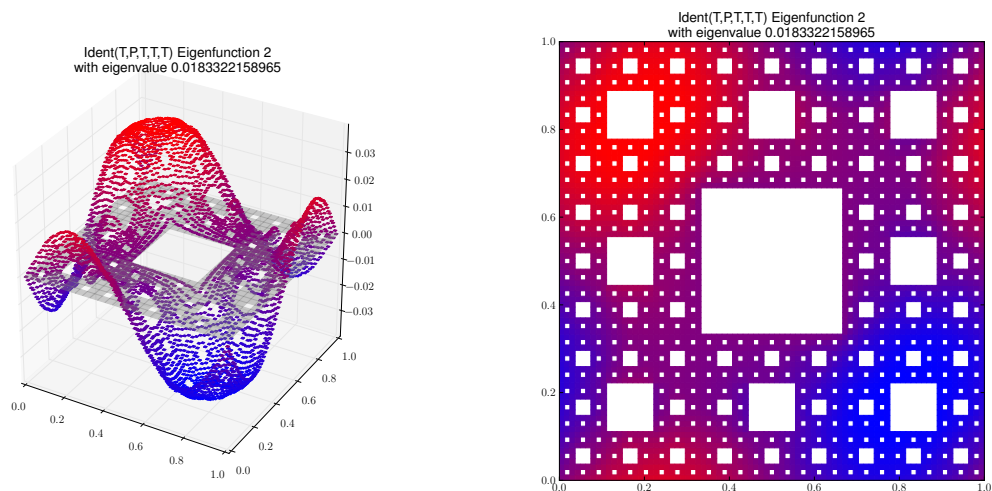
Eigenfunction 2 with eigenvalue 0.0183322158965
