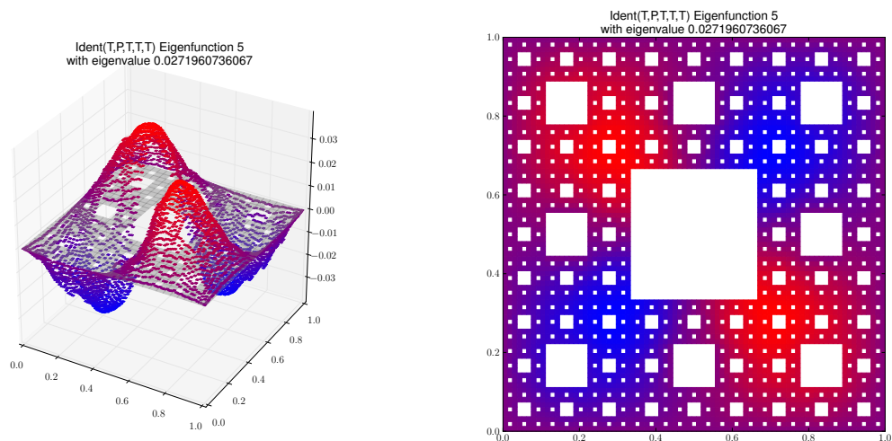
Eigenfunction 5 with eigenvalue 0.0271960736067
