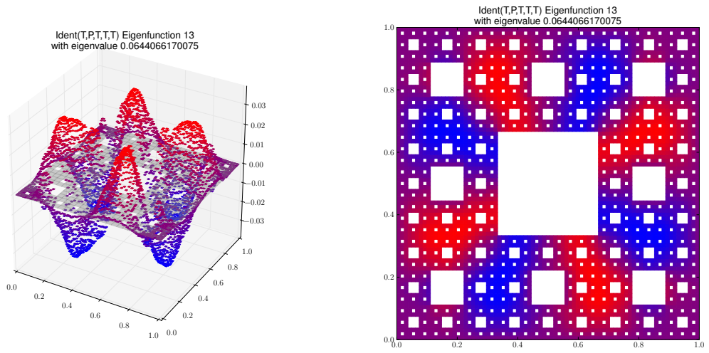
Eigenfunction 13 with eigenvalue 0.0644066170075
