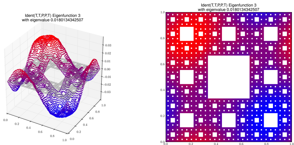
Eigenfunction 3 with eigenvalue 0.0180134342507
