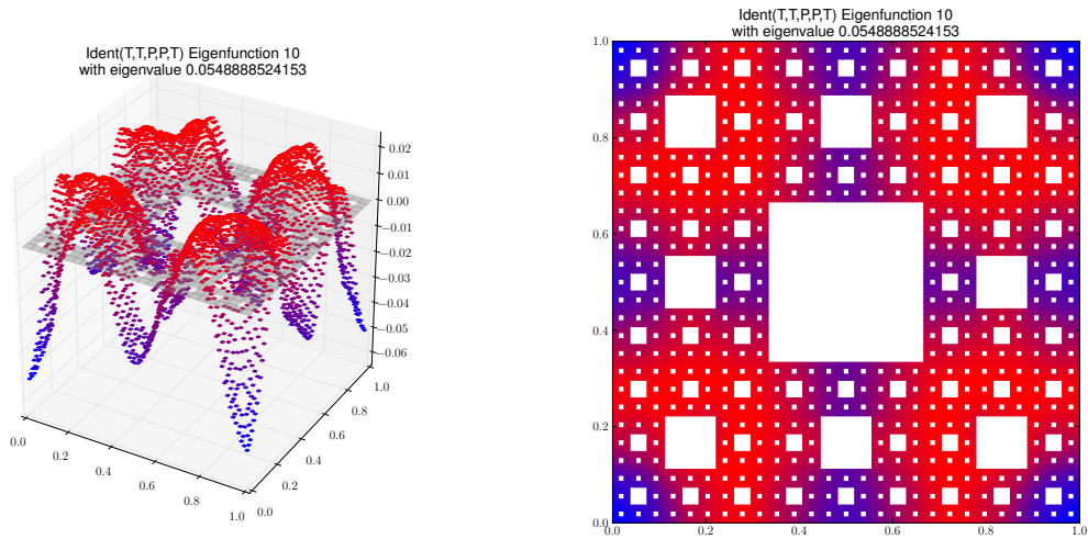
Eigenfunction 10 with eigenvalue 0.0548888524153
