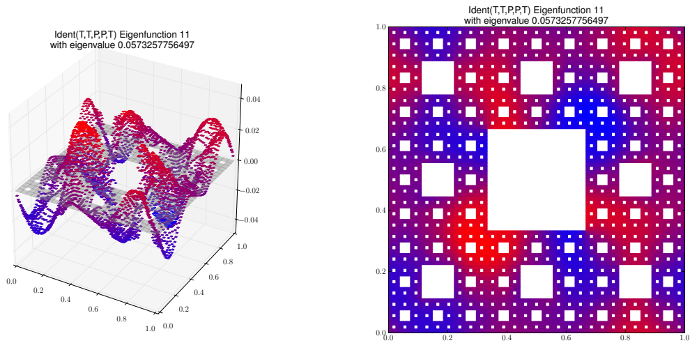
Eigenfunction 11 with eigenvalue 0.0573257756497
