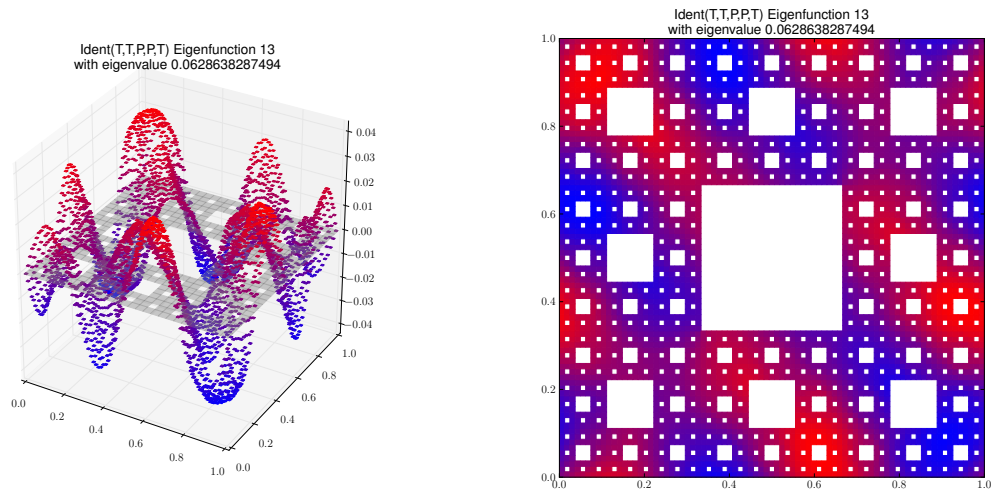
Eigenfunction 13 with eigenvalue 0.0628638287494
