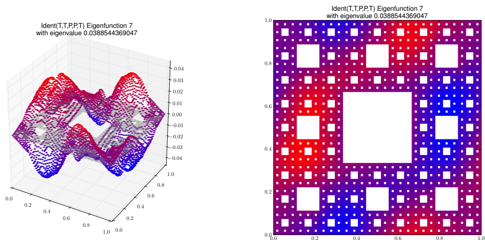
Eigenfunction 7 with eigenvalue 0.0388544369047
