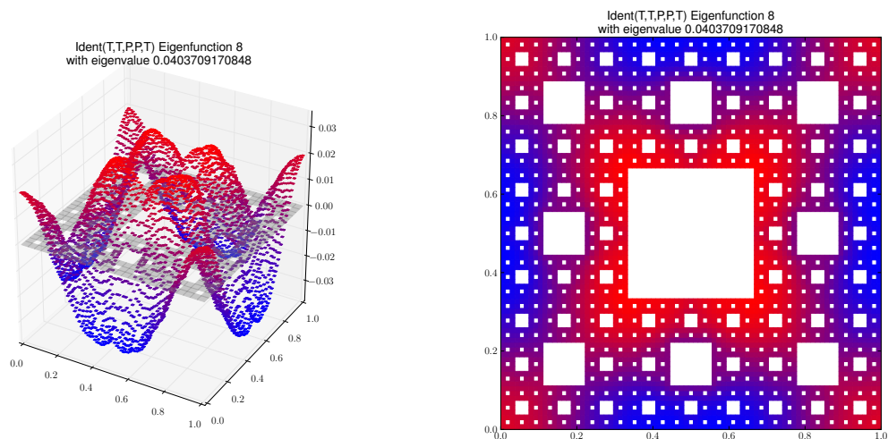
Eigenfunction 8 with eigenvalue 0.0403709170848
