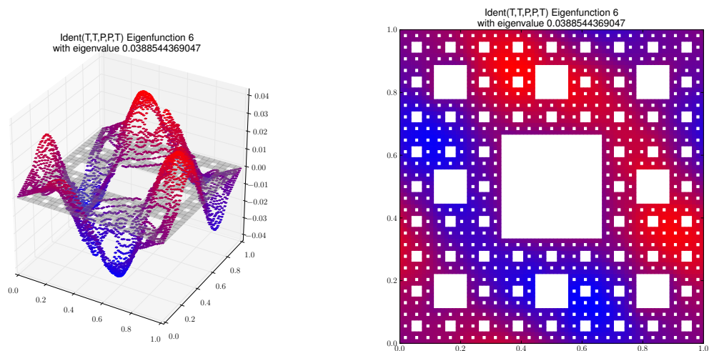
Eigenfunction 6 with eigenvalue 0.0388544369047
