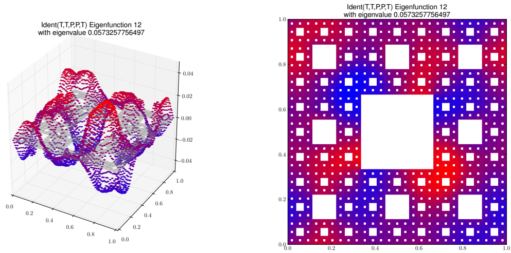
Eigenfunction 12 with eigenvalue 0.0573257756497
