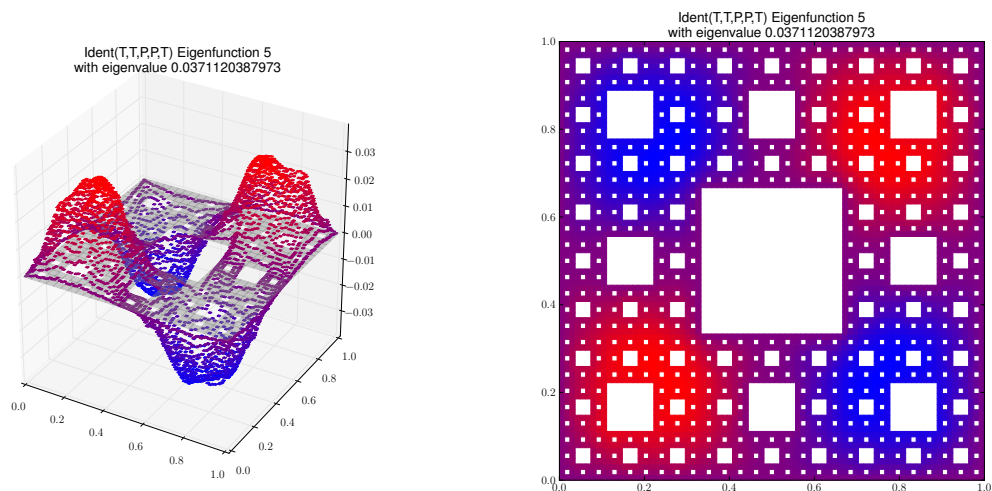
Eigenfunction 5 with eigenvalue 0.0371120387973
