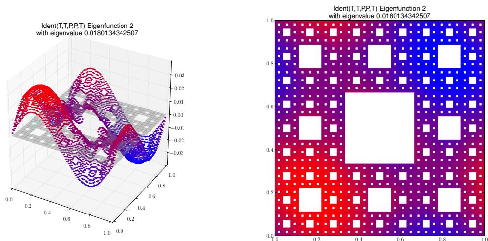
Eigenfunction 2 with eigenvalue 0.0180134342507
