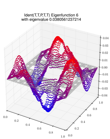
Eigenfunction 6 with eigenvalue 0.0380561237214
