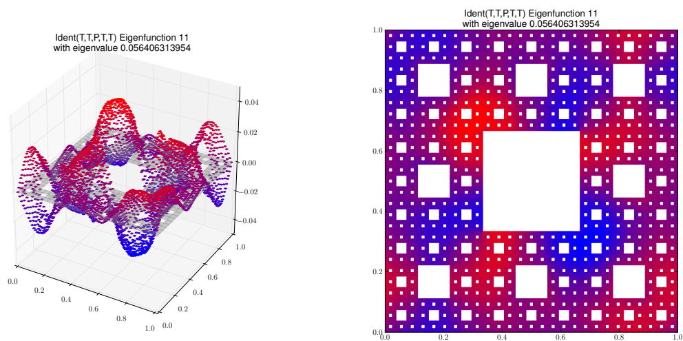
Eigenfunction 11 with eigenvalue 0.056406313954
