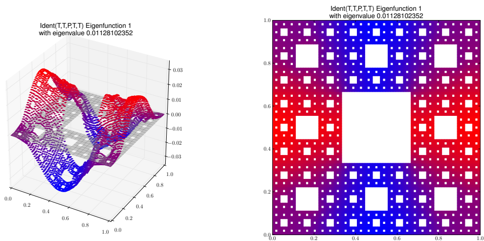
Eigenfunction 1 with eigenvalue 0.01128102352
