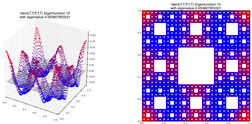
Eigenfunction 10 with eigenvalue 0.053807953321
