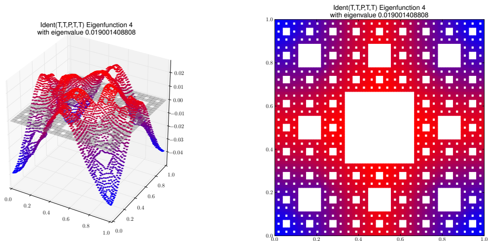
Eigenfunction 4 with eigenvalue 0.019001408808
