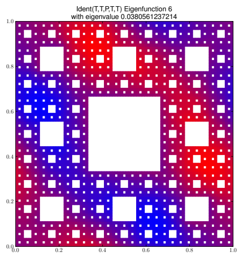
Eigenfunction 6 with eigenvalue 0.0380561237214
