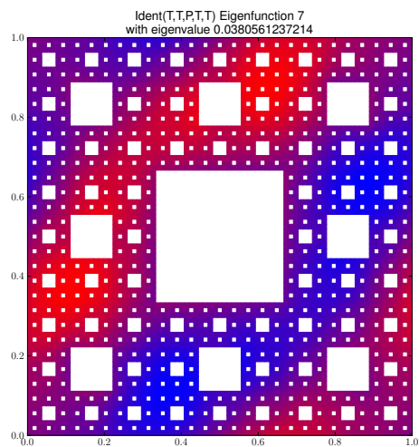
Eigenfunction 7 with eigenvalue 0.0380561237214
