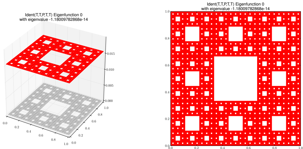
Eigenfunction 0 with eigenvalue -1.18009782868e-14
