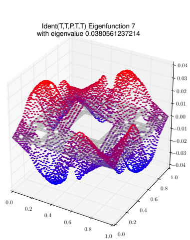
Eigenfunction 7 with eigenvalue 0.0380561237214
