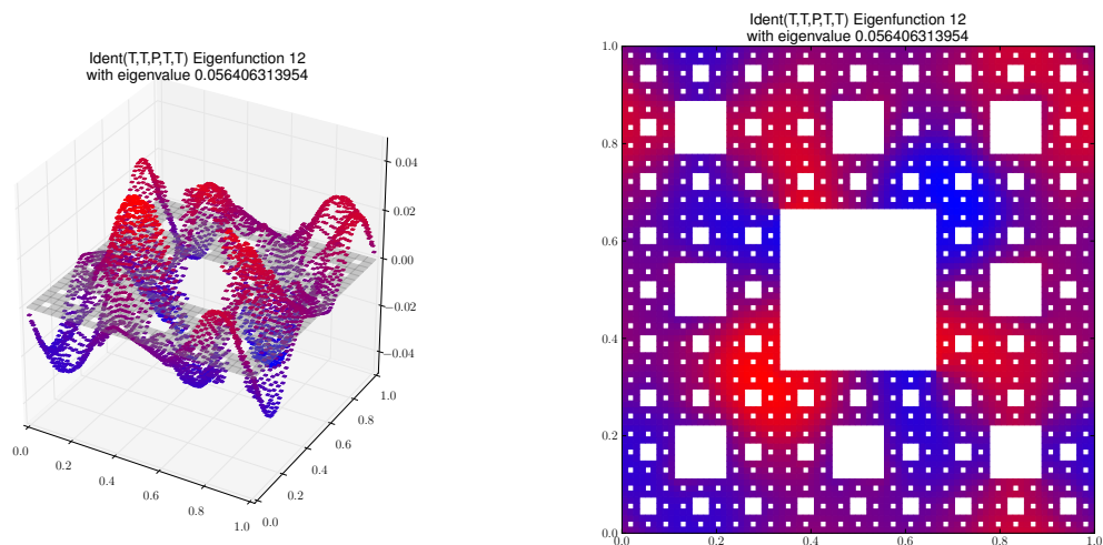
Eigenfunction 12 with eigenvalue 0.056406313954
