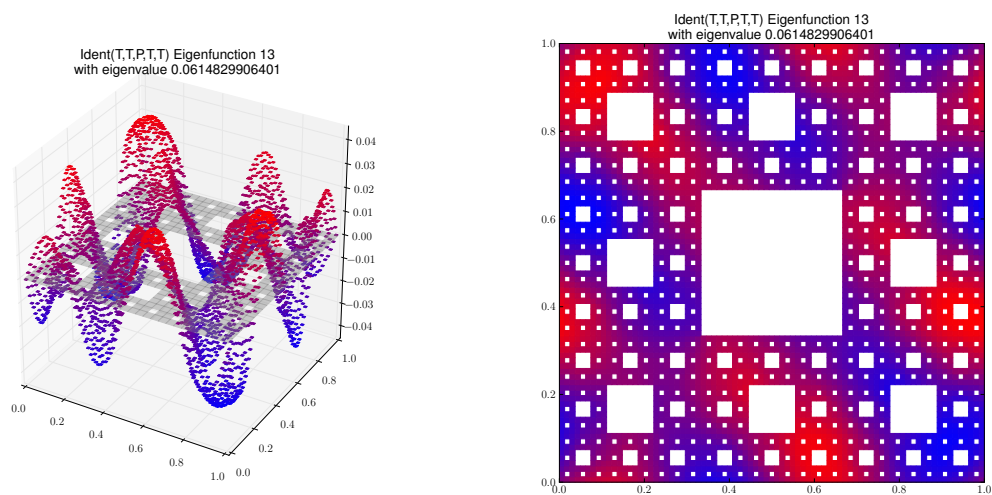
Eigenfunction 13 with eigenvalue 0.0614829906401
