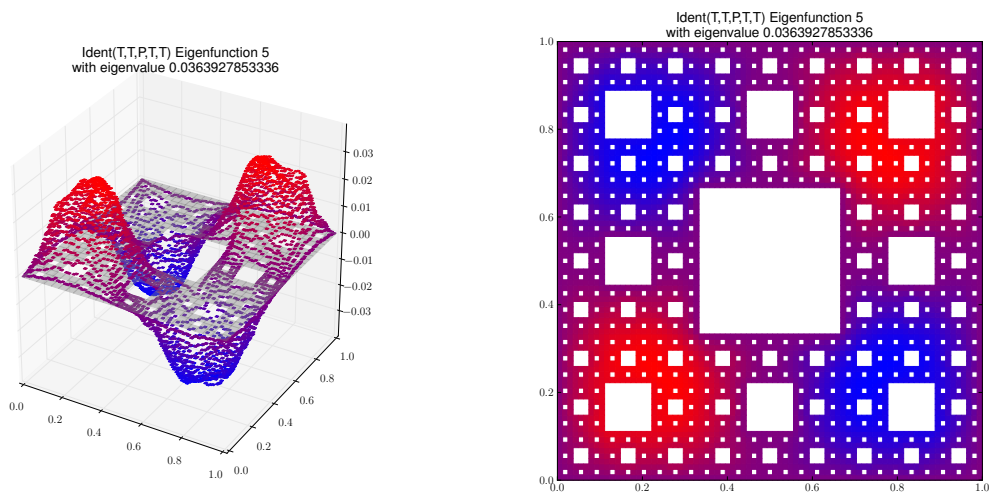
Eigenfunction 5 with eigenvalue 0.0363927853336
