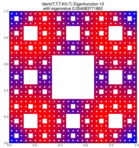
Eigenfunction 10 with eigenvalue 0.054083771862
