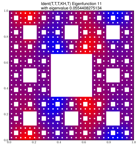
Eigenfunction 11 with eigenvalue 0.0554408275134
