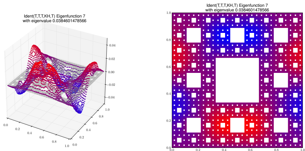
Eigenfunction 7 with eigenvalue 0.0384601478566
