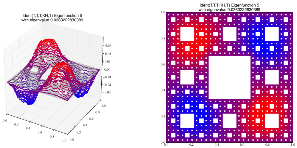
Eigenfunction 5 with eigenvalue 0.0363222830389
