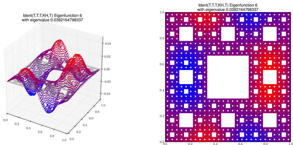
Eigenfunction 6 with eigenvalue 0.0382164798337
