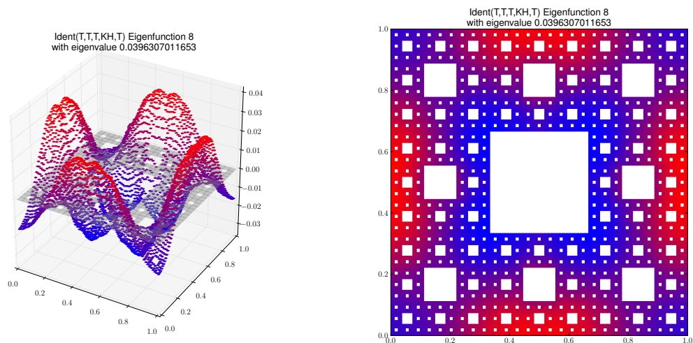
Eigenfunction 8 with eigenvalue 0.0396307011653
