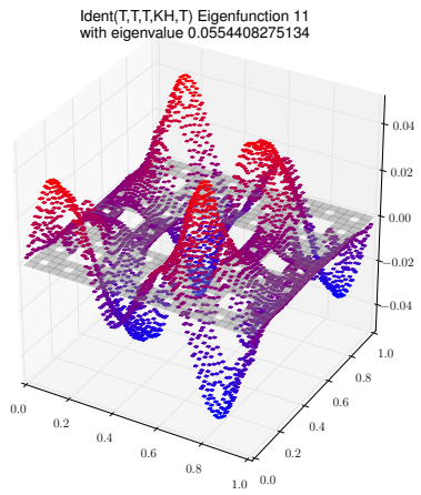
Eigenfunction 11 with eigenvalue 0.0554408275134
