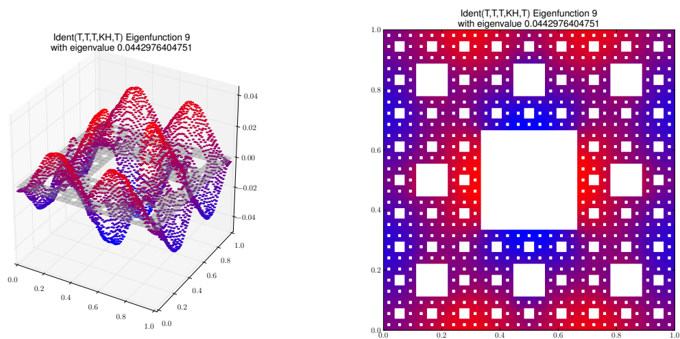
Eigenfunction 9 with eigenvalue 0.0442976404751
