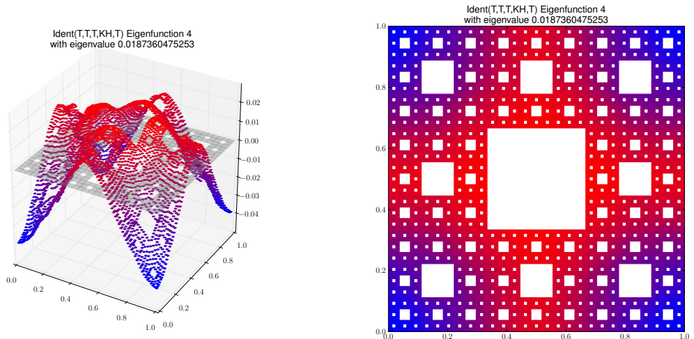
Eigenfunction 4 with eigenvalue 0.0187360475253
