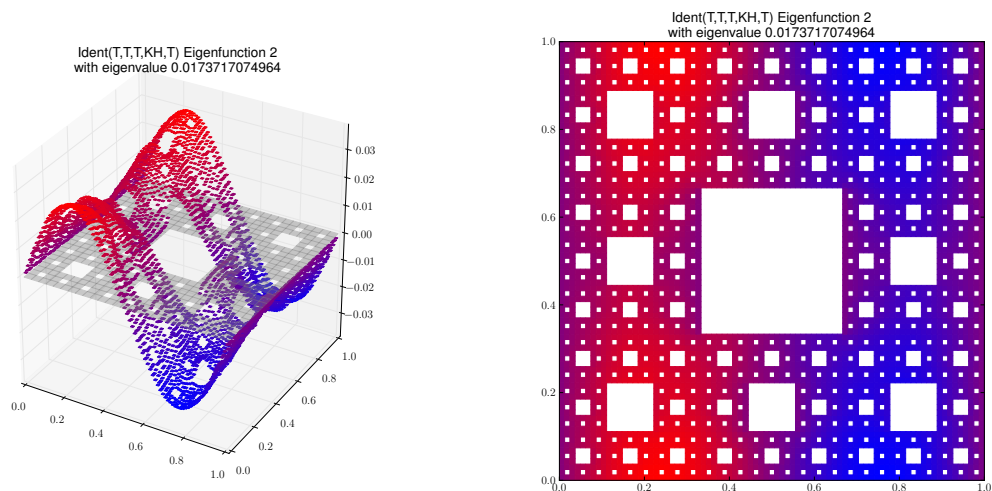
Eigenfunction 2 with eigenvalue 0.0173717074964
