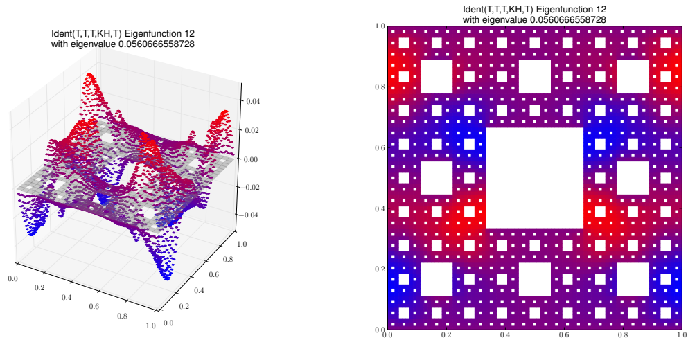
Eigenfunction 12 with eigenvalue 0.0560666558728
