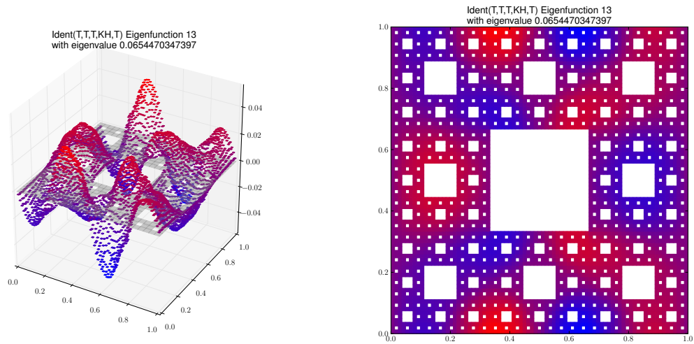
Eigenfunction 13 with eigenvalue 0.0654470347397
