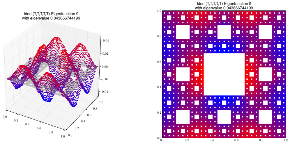
Eigenfunction 9 with eigenvalue 0.043866744199
