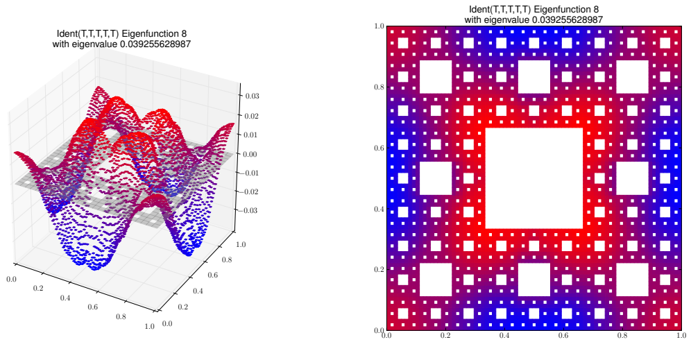
Eigenfunction 8 with eigenvalue 0.039255628987
