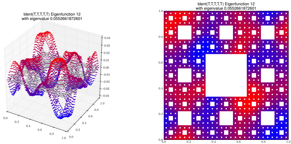
Eigenfunction 12 with eigenvalue 0.0552661872601
