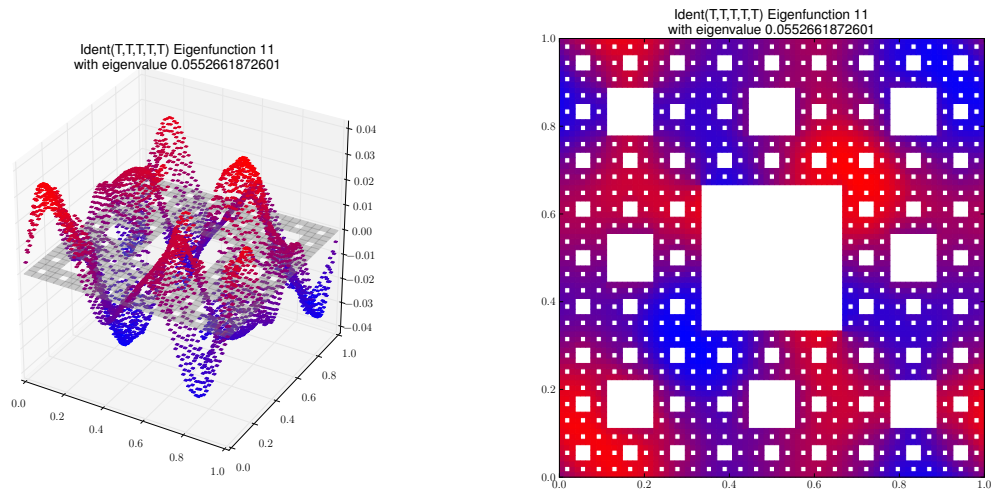
Eigenfunction 11 with eigenvalue 0.0552661872601
