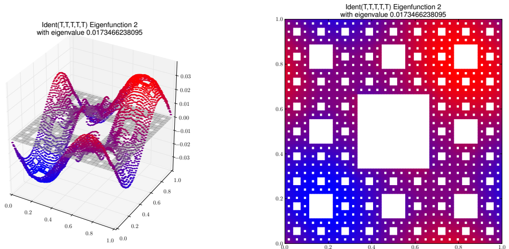
Eigenfunction 2 with eigenvalue 0.0173466238095
