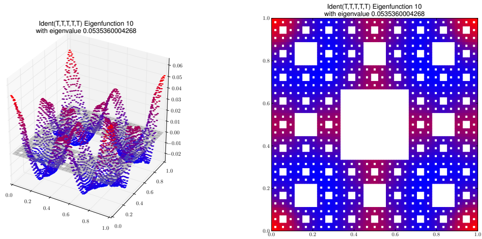
Eigenfunction 10 with eigenvalue 0.0535360004268
