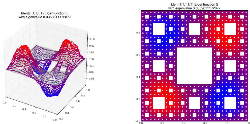
Eigenfunction 5 with eigenvalue 0.0359611172077
