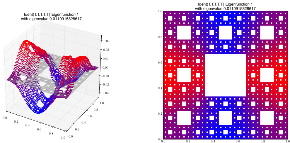
Eigenfunction 1 with eigenvalue 0.0110915828617
