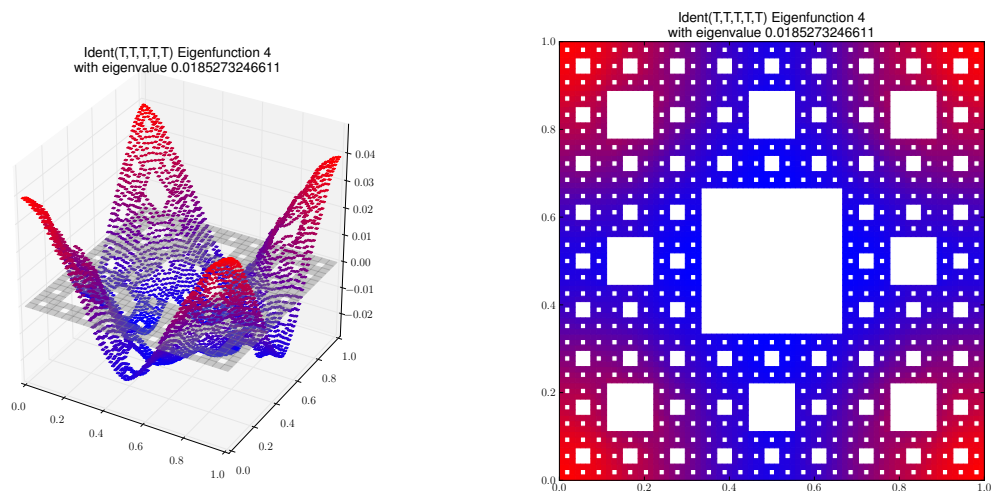
Eigenfunction 4 with eigenvalue 0.0185273246611
