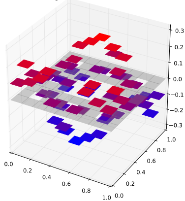
Klein Bottle Horizontal Glued Eigenfunction 19 with eigenvalue 2.98983225608
