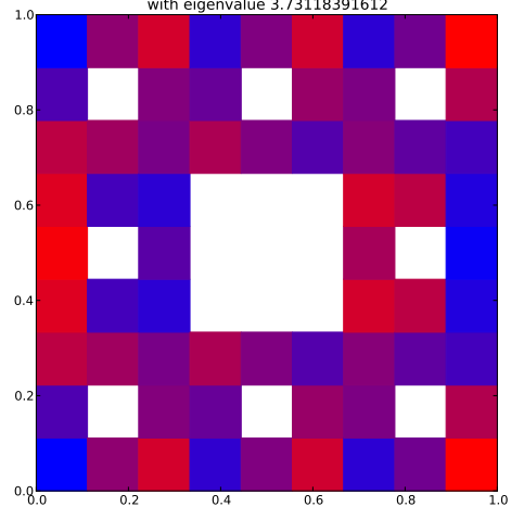
Klein Bottle Horizontal Glued Eigenfunction 29 with eigenvalue 3.73118391612
