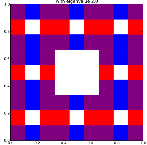
Klein Bottle Horizontal Glued Eigenfunction 13 with eigenvalue 2.0
