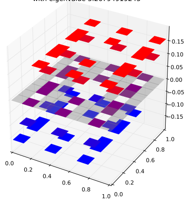
Klein Bottle Horizontal Glued Eigenfunction 24 with eigenvalue 3.26794919243
