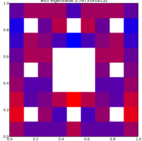
Klein Bottle Horizontal Glued Eigenfunction 30 with eigenvalue 3.76733918152
