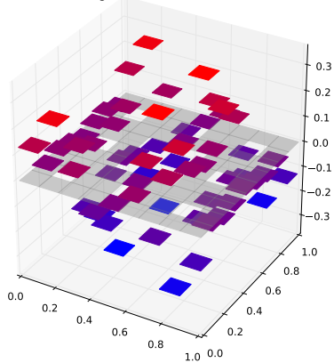
Klein Bottle Horizontal Glued Eigenfunction 11 with eigenvalue 1.88363690629
