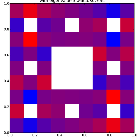
Klein Bottle Horizontal Glued Eigenfunction 21 with eigenvalue 3.06640307644
