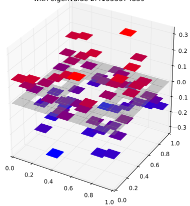
Klein Bottle Horizontal Glued Eigenfunction 16 with eigenvalue 2.41553374839
