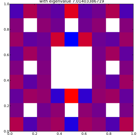
Klein Bottle Horizontal Glued Eigenfunction 57 with eigenvalue 7.01403386719
