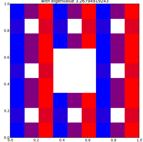
Klein Bottle Horizontal Glued Eigenfunction 24 with eigenvalue 3.26794919243
