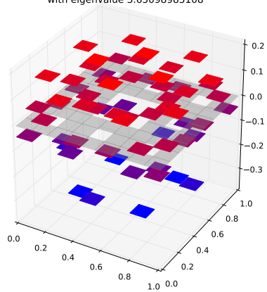
Klein Bottle Horizontal Glued Eigenfunction 28 with eigenvalue 3.65098985108
