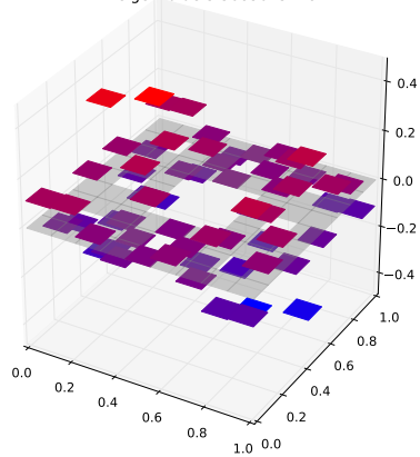
Klein Bottle Horizontal Glued Eigenfunction 26 with eigenvalue 3.3683025148
