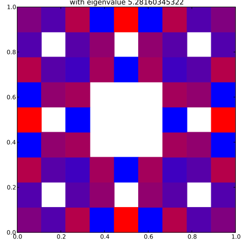
Klein Bottle Horizontal Glued Eigenfunction 45 with eigenvalue 5.28160345322
