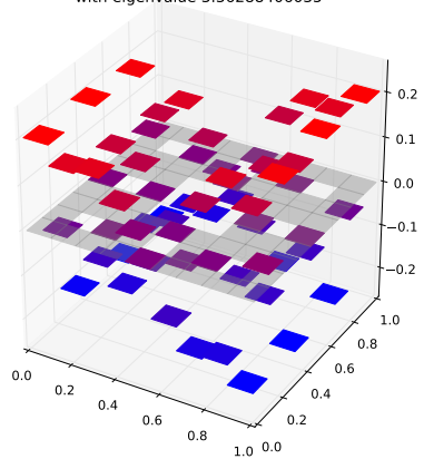
Klein Bottle Horizontal Glued Eigenfunction 25 with eigenvalue 3.36288406035
