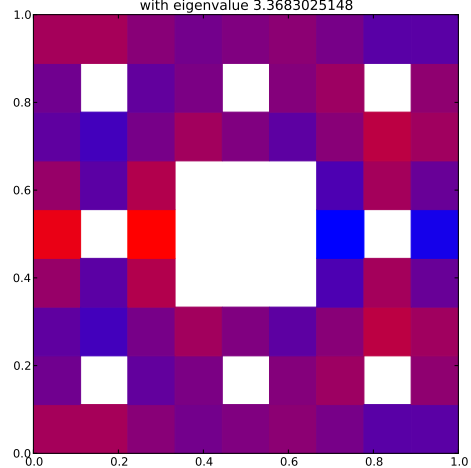
Klein Bottle Horizontal Glued Eigenfunction 26 with eigenvalue 3.3683025148
