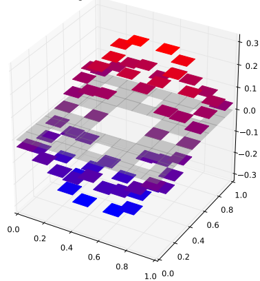
Klein Bottle Horizontal Glued Eigenfunction 5 with eigenvalue 1.12507512074
