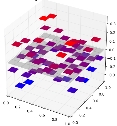
Klein Bottle Horizontal Glued Eigenfunction 21 with eigenvalue 3.06640307644
