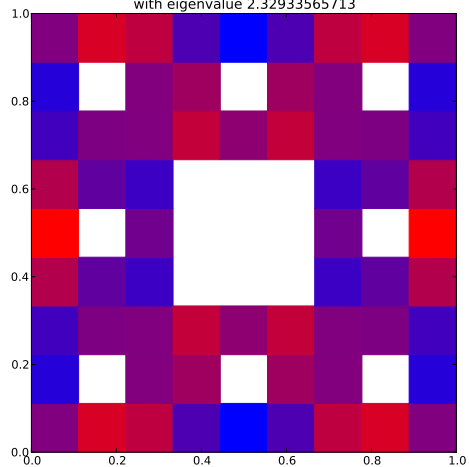
Klein Bottle Horizontal Glued Eigenfunction 15 with eigenvalue 2.32933565713
