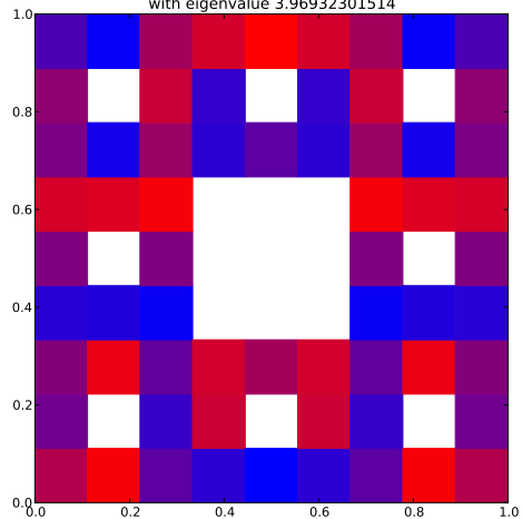
Klein Bottle Horizontal Glued Eigenfunction 32 with eigenvalue 3.96932301514
