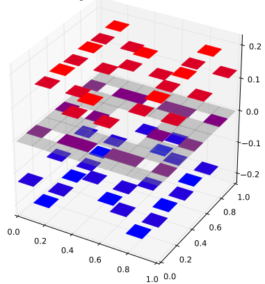
Klein Bottle Horizontal Glued Eigenfunction 37 with eigenvalue 4.58578643763
