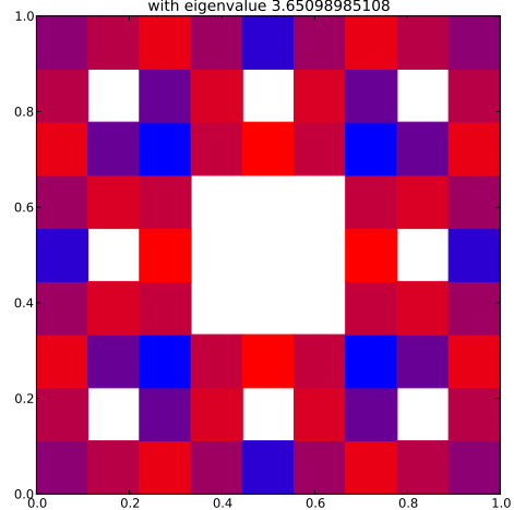
Klein Bottle Horizontal Glued Eigenfunction 28 with eigenvalue 3.65098985108
