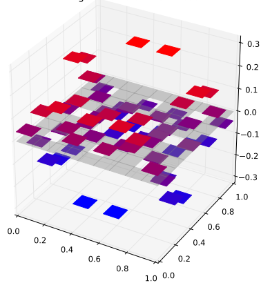
Klein Bottle Horizontal Glued Eigenfunction 27 with eigenvalue 3.51128162693
