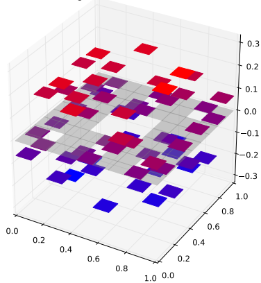
Klein Bottle Horizontal Glued Eigenfunction 31 with eigenvalue 3.84320023286
