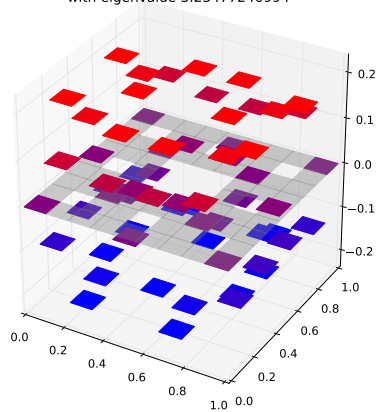
Klein Bottle Horizontal Glued Eigenfunction 23 with eigenvalue 3.23477240994
