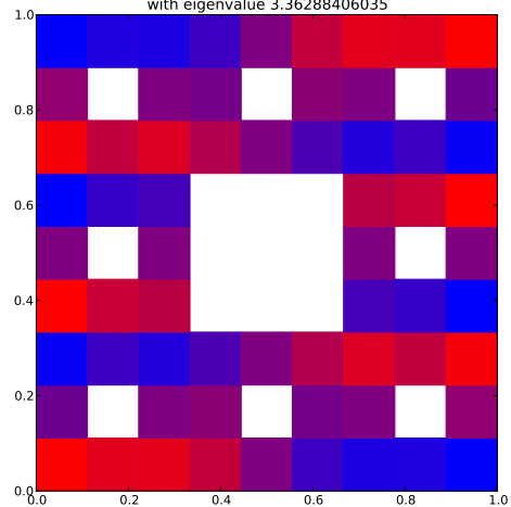
Klein Bottle Horizontal Glued Eigenfunction 25 with eigenvalue 3.36288406035
