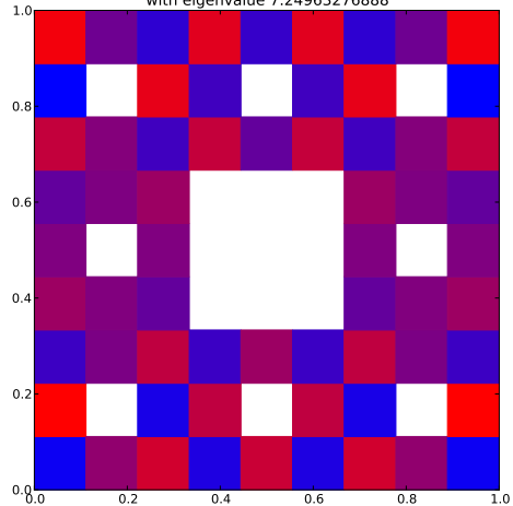
Klein Bottle Horizontal Glued Eigenfunction 59 with eigenvalue 7.24963276888
