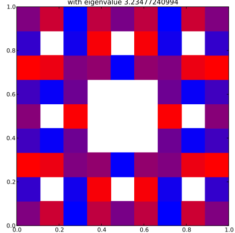
Klein Bottle Horizontal Glued Eigenfunction 23 with eigenvalue 3.23477240994
