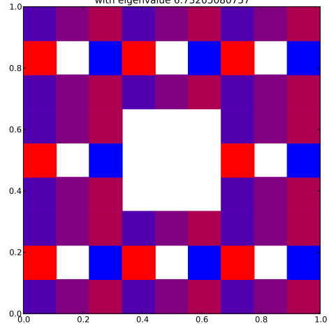
Klein Bottle Horizontal Glued Eigenfunction 55 with eigenvalue 6.73205080757
