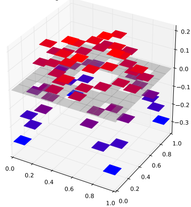
Klein Bottle Horizontal Glued Eigenfunction 4 with eigenvalue 0.758799842469
