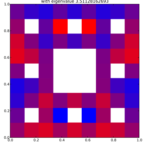
Klein Bottle Horizontal Glued Eigenfunction 27 with eigenvalue 3.51128162693
