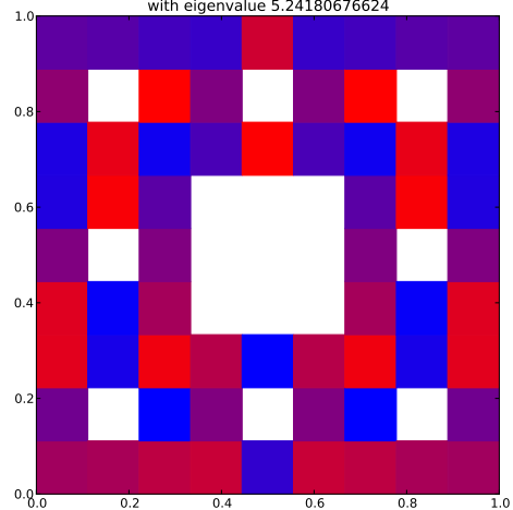
Klein Bottle Horizontal Glued Eigenfunction 44 with eigenvalue 5.24180676624
