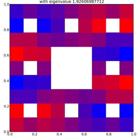
Klein Bottle Horizontal Glued Eigenfunction 12 with eigenvalue 1.92606987712
