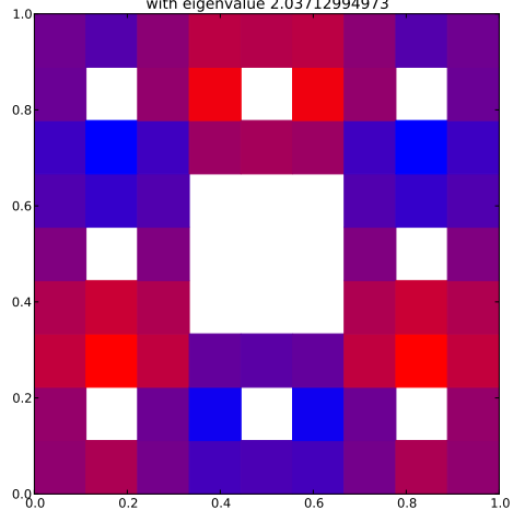
Klein Bottle Horizontal Glued Eigenfunction 14 with eigenvalue 2.03712994973
