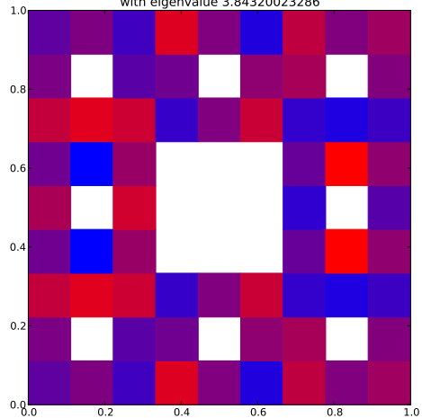
Klein Bottle Horizontal Glued Eigenfunction 31 with eigenvalue 3.84320023286
