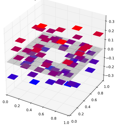
Klein Bottle Horizontal Glued Eigenfunction 42 with eigenvalue 4.91395612707
