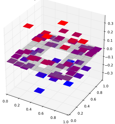
Klein Bottle Horizontal Glued Eigenfunction 43 with eigenvalue 5.02616265324
