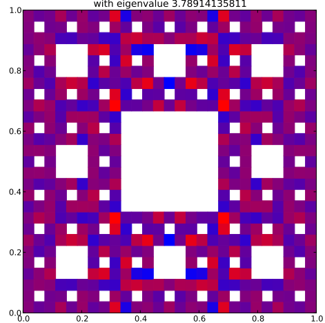
Klein Bottle Horizontal Glued Eigenfunction 250 with eigenvalue 3.78914135811
