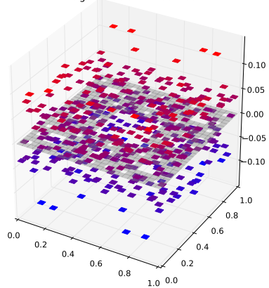
Klein Bottle Horizontal Glued Eigenfunction 363 with eigenvalue 5.21178882954
