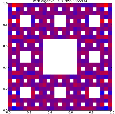
Klein Bottle Horizontal Glued Eigenfunction 251 with eigenvalue 3.78993365934
