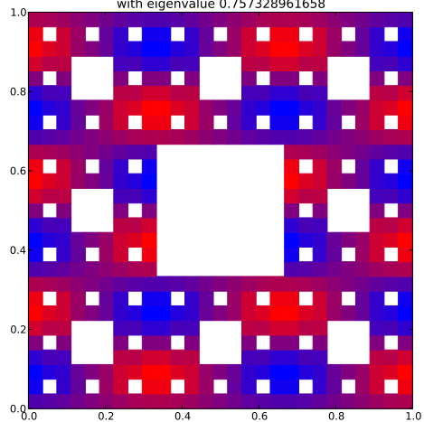
Klein Bottle Horizontal Glued Eigenfunction 29 with eigenvalue 0.757328961658
