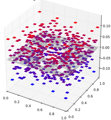
Klein Bottle Horizontal Glued Eigenfunction 205 with eigenvalue 3.34792599125
