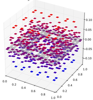
Klein Bottle Horizontal Glued Eigenfunction 469 with eigenvalue 7.13083618949
