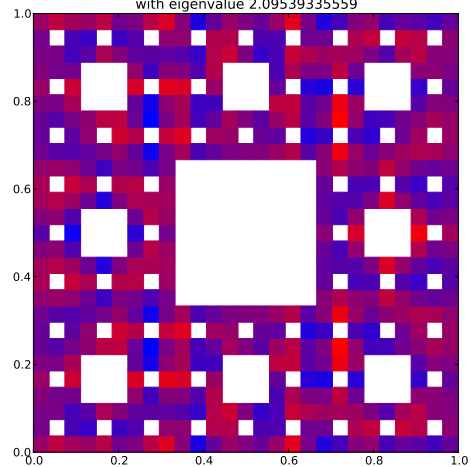
Klein Bottle Horizontal Glued Eigenfunction 109 with eigenvalue 2.09539335559
