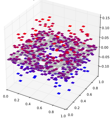
Klein Bottle Horizontal Glued Eigenfunction 447 with eigenvalue 6.74042214356
