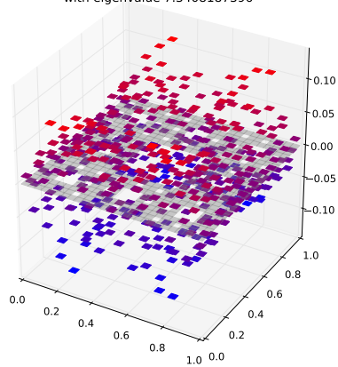
Klein Bottle Horizontal Glued Eigenfunction 504 with eigenvalue 7.3408187396
