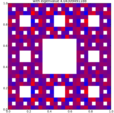
Klein Bottle Horizontal Glued Eigenfunction 265 with eigenvalue 4.04309491188
