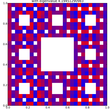
Klein Bottle Horizontal Glued Eigenfunction 271 with eigenvalue 4.19451290983
