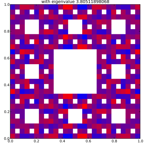
Klein Bottle Horizontal Glued Eigenfunction 252 with eigenvalue 3.80511898068
