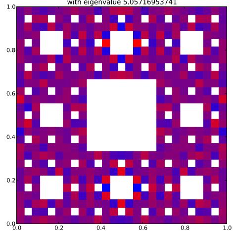
Klein Bottle Horizontal Glued Eigenfunction 349 with eigenvalue 5.05716953741
