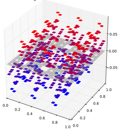
Klein Bottle Horizontal Glued Eigenfunction 25 with eigenvalue 0.690590970621
