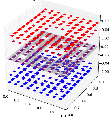
Klein Bottle Horizontal Glued Eigenfunction 193 with eigenvalue 3.26794919243
