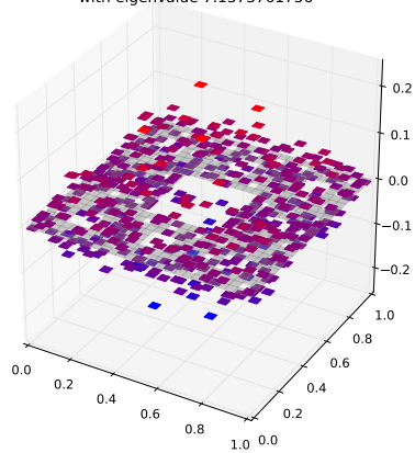
Klein Bottle Horizontal Glued Eigenfunction 470 with eigenvalue 7.1373761756
