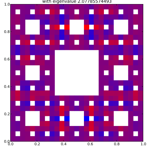
Klein Bottle Horizontal Glued Eigenfunction 107 with eigenvalue 2.07785574493
