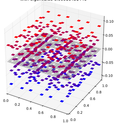
Klein Bottle Horizontal Glued Eigenfunction 409 with eigenvalue 6.00016431446
