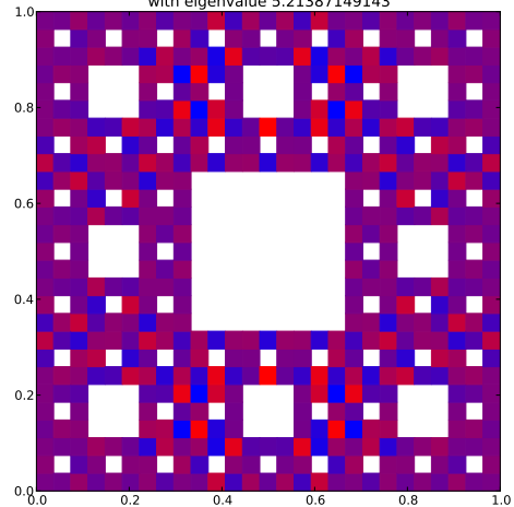
Klein Bottle Horizontal Glued Eigenfunction 364 with eigenvalue 5.21387149143
