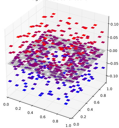
Klein Bottle Horizontal Glued Eigenfunction 386 with eigenvalue 5.55157856194
