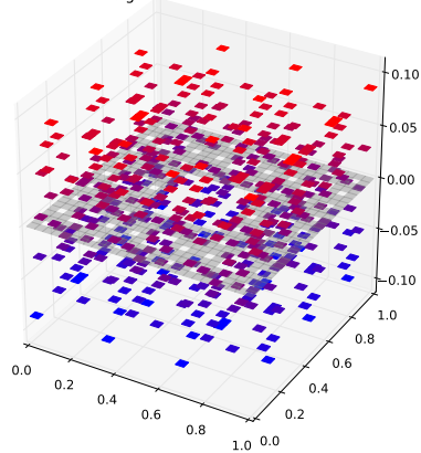
Klein Bottle Horizontal Glued Eigenfunction 245 with eigenvalue 3.73118391612
