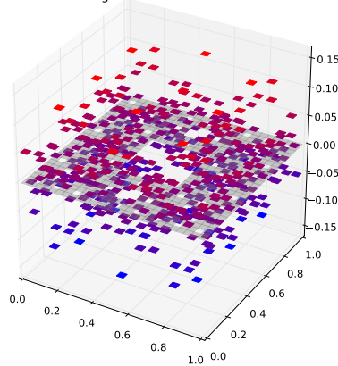
Klein Bottle Horizontal Glued Eigenfunction 457 with eigenvalue 7.01403386719
