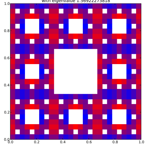
Klein Bottle Horizontal Glued Eigenfunction 67 with eigenvalue 1.56922273818
