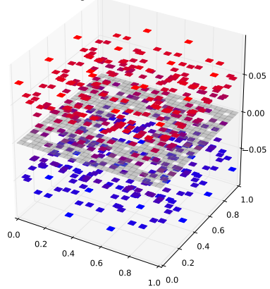
Klein Bottle Horizontal Glued Eigenfunction 491 with eigenvalue 7.25326741767
