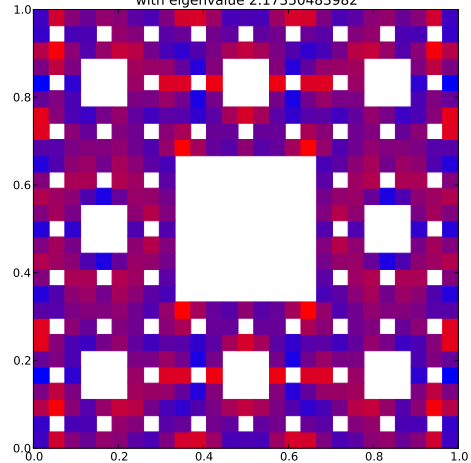
Klein Bottle Horizontal Glued Eigenfunction 117 with eigenvalue 2.17350483982
