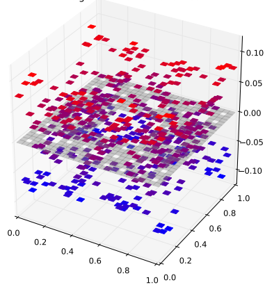
Klein Bottle Horizontal Glued Eigenfunction 399 with eigenvalue 5.76075182339
