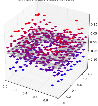
Klein Bottle Horizontal Glued Eigenfunction 448 with eigenvalue 6.83304643249
