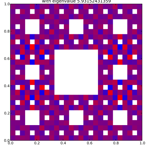
Klein Bottle Horizontal Glued Eigenfunction 404 with eigenvalue 5.93152431359
