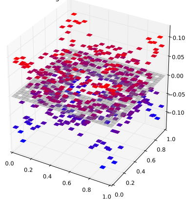
Klein Bottle Horizontal Glued Eigenfunction 273 with eigenvalue 4.21303549507
