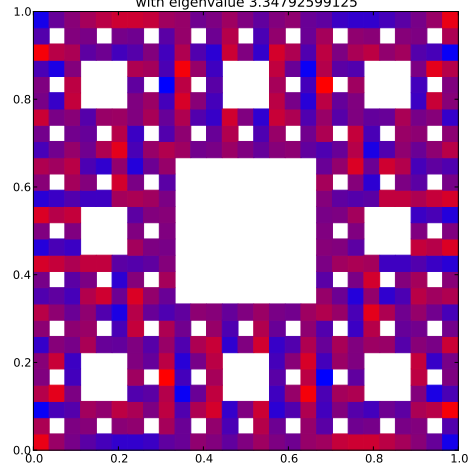
Klein Bottle Horizontal Glued Eigenfunction 205 with eigenvalue 3.34792599125
