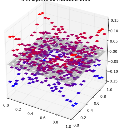
Klein Bottle Horizontal Glued Eigenfunction 508 with eigenvalue 7.35195175996
