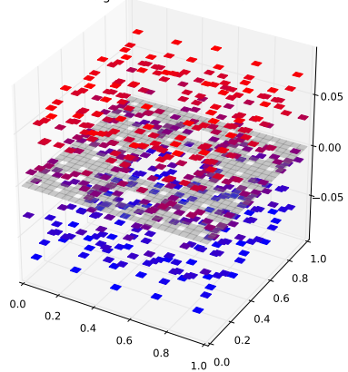
Klein Bottle Horizontal Glued Eigenfunction 261 with eigenvalue 3.96932301514
