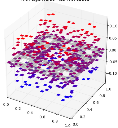
Klein Bottle Horizontal Glued Eigenfunction 478 with eigenvalue 7.19466783395
