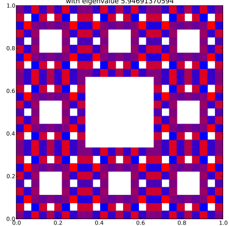
Klein Bottle Horizontal Glued Eigenfunction 407 with eigenvalue 5.94691370594
