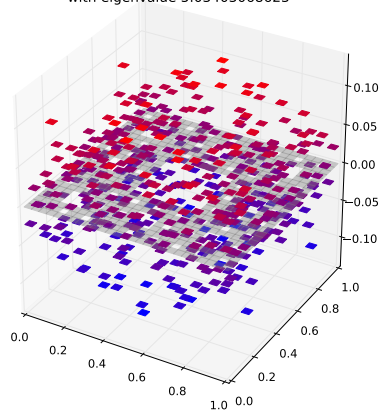
Klein Bottle Horizontal Glued Eigenfunction 347 with eigenvalue 5.03403068623
