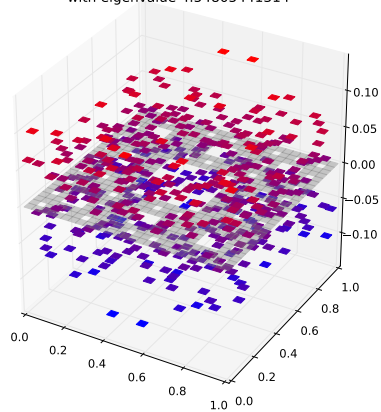
Klein Bottle Horizontal Glued Eigenfunction 301 with eigenvalue 4.54805441314
