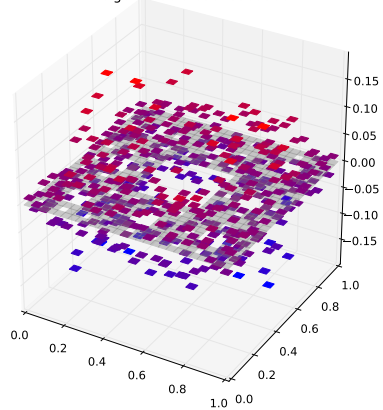
Klein Bottle Horizontal Glued Eigenfunction 351 with eigenvalue 5.09828369988
