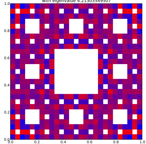
Klein Bottle Horizontal Glued Eigenfunction 273 with eigenvalue 4.21303549507
