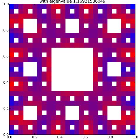
Klein Bottle Horizontal Glued Eigenfunction 45 with eigenvalue 1.16921586049
