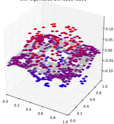
Klein Bottle Horizontal Glued Eigenfunction 41 with eigenvalue 1.04620341896
