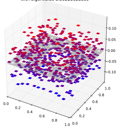
Klein Bottle Horizontal Glued Eigenfunction 198 with eigenvalue 3.30223628869
