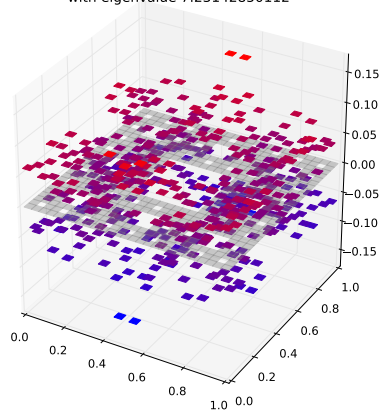
Klein Bottle Horizontal Glued Eigenfunction 485 with eigenvalue 7.23142850112
