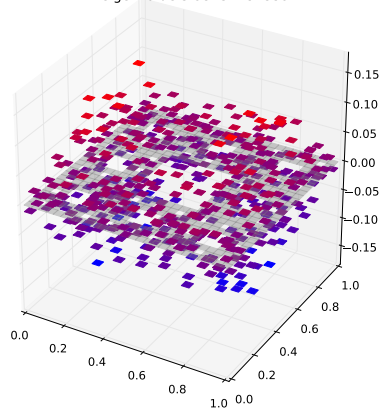
Klein Bottle Horizontal Glued Eigenfunction 404 with eigenvalue 5.93152431359
