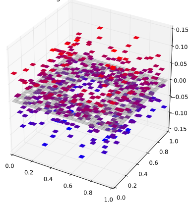
Klein Bottle Horizontal Glued Eigenfunction 389 with eigenvalue 5.62209746285
