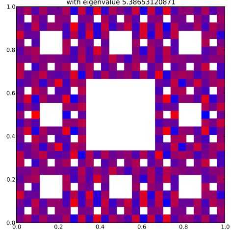
Klein Bottle Horizontal Glued Eigenfunction 379 with eigenvalue 5.38653120871
