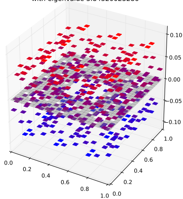
Klein Bottle Horizontal Glued Eigenfunction 255 with eigenvalue 3.84320023286
