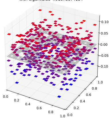
Klein Bottle Horizontal Glued Eigenfunction 331 with eigenvalue 4.91078674184
