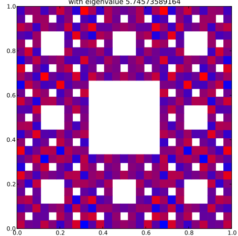
Klein Bottle Horizontal Glued Eigenfunction 398 with eigenvalue 5.74573589164
