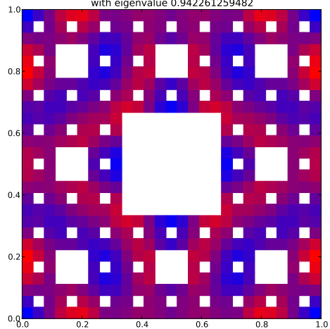
Klein Bottle Horizontal Glued Eigenfunction 35 with eigenvalue 0.942261259482
