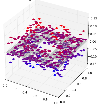
Klein Bottle Horizontal Glued Eigenfunction 480 with eigenvalue 7.20710721045
