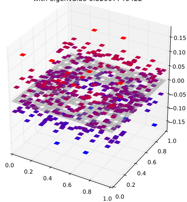
Klein Bottle Horizontal Glued Eigenfunction 429 with eigenvalue 6.32997746422
