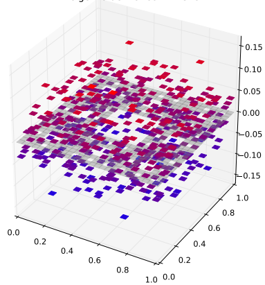
Klein Bottle Horizontal Glued Eigenfunction 334 with eigenvalue 4.91892742519
