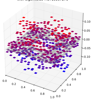
Klein Bottle Horizontal Glued Eigenfunction 510 with eigenvalue 7.3719507276
