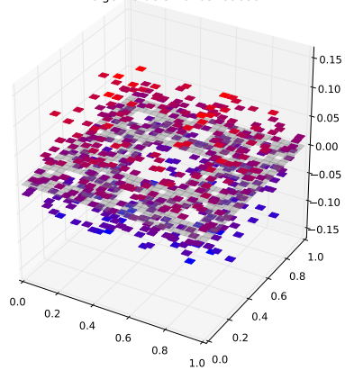
Klein Bottle Horizontal Glued Eigenfunction 240 with eigenvalue 3.70163789659
