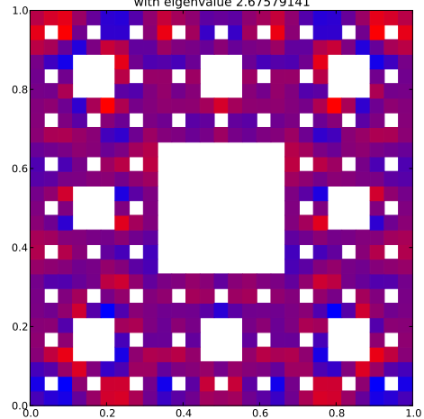
Klein Bottle Horizontal Glued Eigenfunction 139 with eigenvalue 2.67579141
