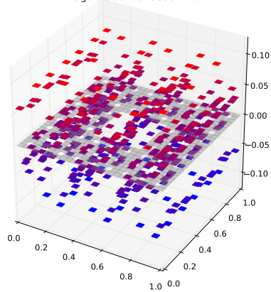
Klein Bottle Horizontal Glued Eigenfunction 332 with eigenvalue 4.91395612707
