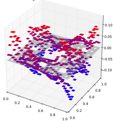
Klein Bottle Horizontal Glued Eigenfunction 13 with eigenvalue 0.356564951405
