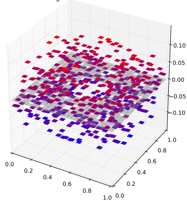
Klein Bottle Horizontal Glued Eigenfunction 327 with eigenvalue 4.85459398679
