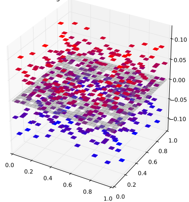
Klein Bottle Horizontal Glued Eigenfunction 257 with eigenvalue 3.91213676482
