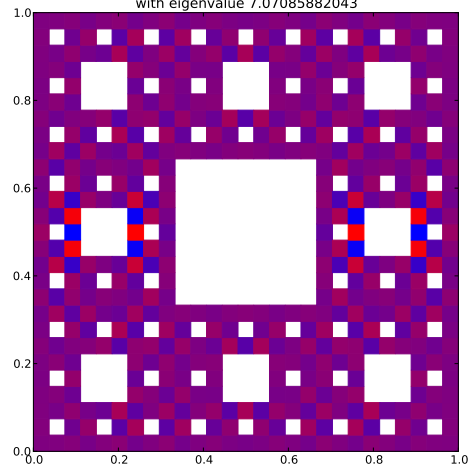
Klein Bottle Horizontal Glued Eigenfunction 462 with eigenvalue 7.07085882043
