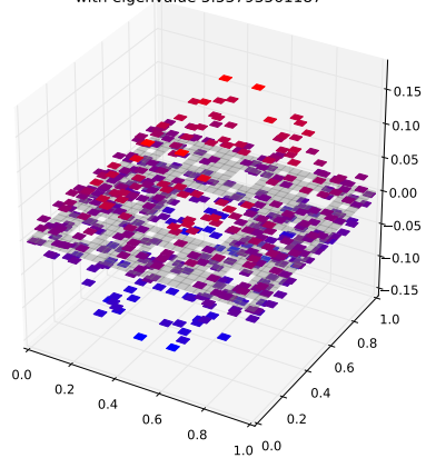
Klein Bottle Horizontal Glued Eigenfunction 385 with eigenvalue 5.53793561187
