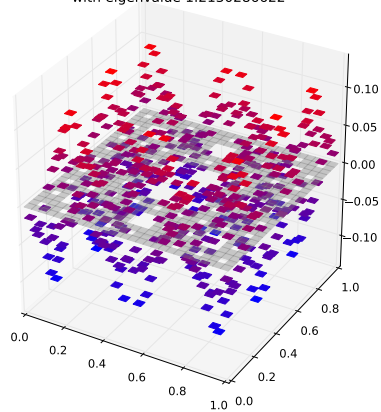
Klein Bottle Horizontal Glued Eigenfunction 49 with eigenvalue 1.2130286622
