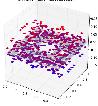
Klein Bottle Horizontal Glued Eigenfunction 275 with eigenvalue 4.21872101267
