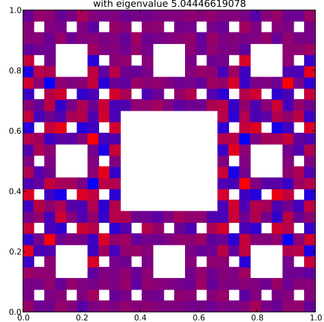
Klein Bottle Horizontal Glued Eigenfunction 348 with eigenvalue 5.04446619078
