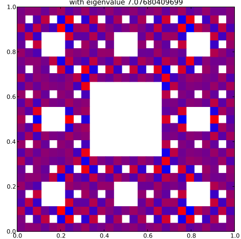
Klein Bottle Horizontal Glued Eigenfunction 463 with eigenvalue 7.07680409699
