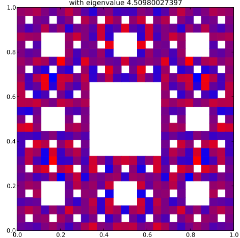
Klein Bottle Horizontal Glued Eigenfunction 298 with eigenvalue 4.50980027397
