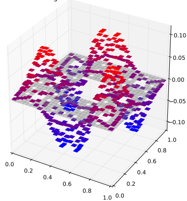
Klein Bottle Horizontal Glued Eigenfunction 11 with eigenvalue 0.342985495142
