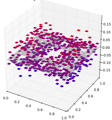
Klein Bottle Horizontal Glued Eigenfunction 421 with eigenvalue 6.2156890866
