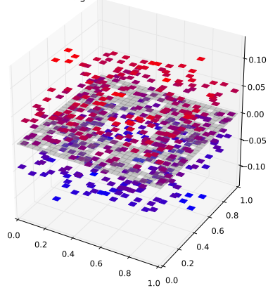
Klein Bottle Horizontal Glued Eigenfunction 333 with eigenvalue 4.91525014378
