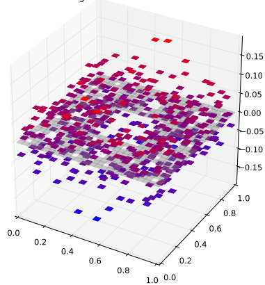
Klein Bottle Horizontal Glued Eigenfunction 367 with eigenvalue 5.24909229705
