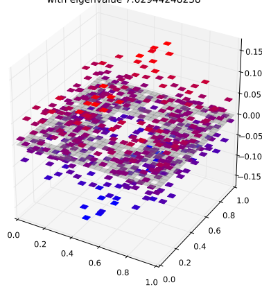
Klein Bottle Horizontal Glued Eigenfunction 459 with eigenvalue 7.02944248238
