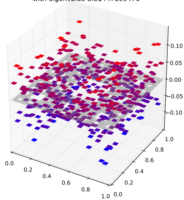
Klein Bottle Horizontal Glued Eigenfunction 200 with eigenvalue 3.31447899476
