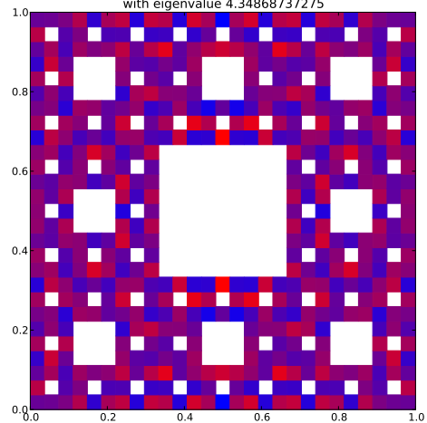
Klein Bottle Horizontal Glued Eigenfunction 283 with eigenvalue 4.34868737275
