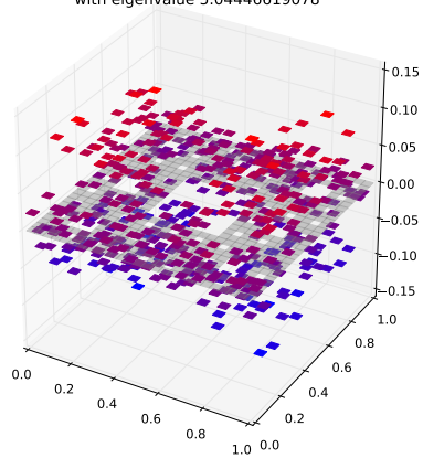
Klein Bottle Horizontal Glued Eigenfunction 348 with eigenvalue 5.04446619078
