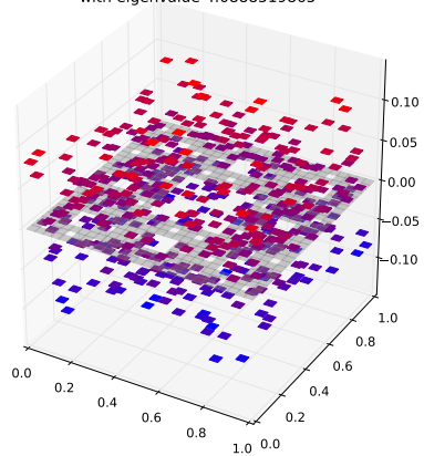
Klein Bottle Horizontal Glued Eigenfunction 267 with eigenvalue 4.0888519865
