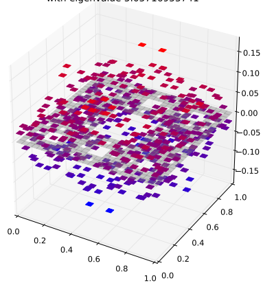
Klein Bottle Horizontal Glued Eigenfunction 349 with eigenvalue 5.05716953741
