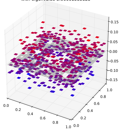
Klein Bottle Horizontal Glued Eigenfunction 173 with eigenvalue 3.06661385825
