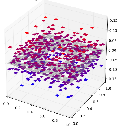
Klein Bottle Horizontal Glued Eigenfunction 441 with eigenvalue 6.60403777192
