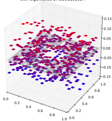
Klein Bottle Horizontal Glued Eigenfunction 219 with eigenvalue 3.48098166924
