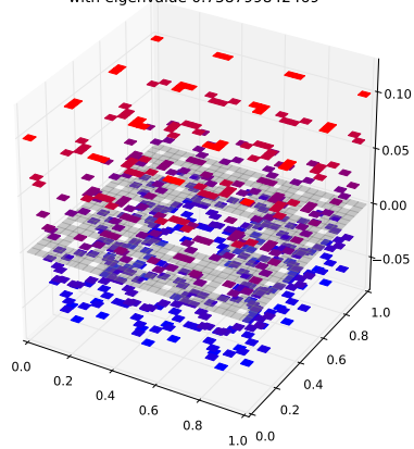
Klein Bottle Horizontal Glued Eigenfunction 30 with eigenvalue 0.758799842469
