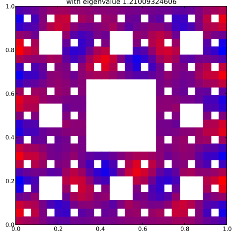
Klein Bottle Horizontal Glued Eigenfunction 48 with eigenvalue 1.21009324606
