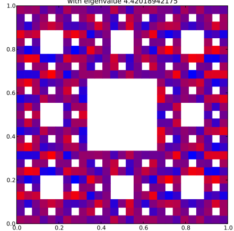
Klein Bottle Horizontal Glued Eigenfunction 289 with eigenvalue 4.42018942175
