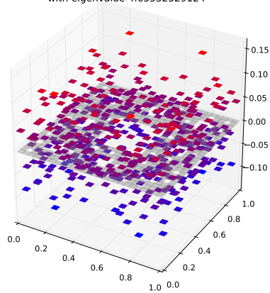
Klein Bottle Horizontal Glued Eigenfunction 310 with eigenvalue 4.65532329124
