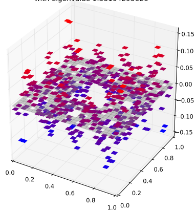
Klein Bottle Horizontal Glued Eigenfunction 65 with eigenvalue 1.53104293626
