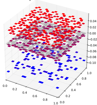
Klein Bottle Horizontal Glued Eigenfunction 83 with eigenvalue 1.87462446692
