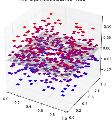
Klein Bottle Horizontal Glued Eigenfunction 202 with eigenvalue 3.32375344531
