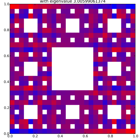
Klein Bottle Horizontal Glued Eigenfunction 165 with eigenvalue 3.00599061374
