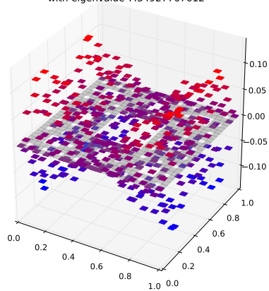
Klein Bottle Horizontal Glued Eigenfunction 507 with eigenvalue 7.34927767612
