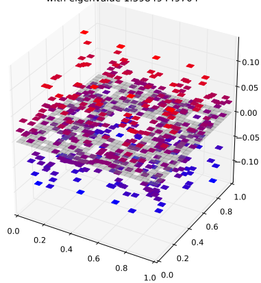
Klein Bottle Horizontal Glued Eigenfunction 68 with eigenvalue 1.59849449704
