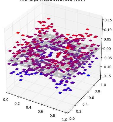
Klein Bottle Horizontal Glued Eigenfunction 346 with eigenvalue 5.02785546004
