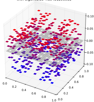
Klein Bottle Horizontal Glued Eigenfunction 271 with eigenvalue 4.19451290983
