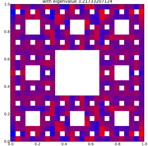
Klein Bottle Horizontal Glued Eigenfunction 187 with eigenvalue 3.21733207124
