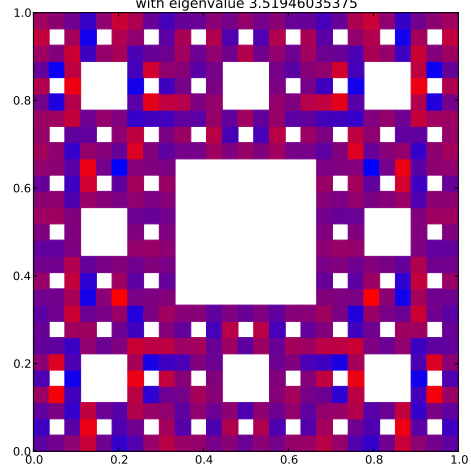
Klein Bottle Horizontal Glued Eigenfunction 224 with eigenvalue 3.51946035375
