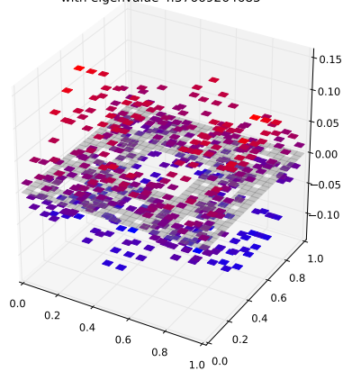
Klein Bottle Horizontal Glued Eigenfunction 285 with eigenvalue 4.37669264685
