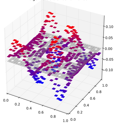
Klein Bottle Horizontal Glued Eigenfunction 12 with eigenvalue 0.346340470289
