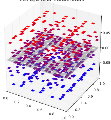
Klein Bottle Horizontal Glued Eigenfunction 311 with eigenvalue 4.65856481536
