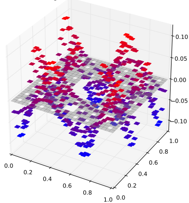
Klein Bottle Horizontal Glued Eigenfunction 17 with eigenvalue 0.502699310322
