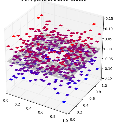
Klein Bottle Horizontal Glued Eigenfunction 384 with eigenvalue 5.53087032815
