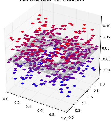
Klein Bottle Horizontal Glued Eigenfunction 330 with eigenvalue 4.87473314084
