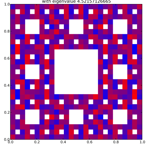
Klein Bottle Horizontal Glued Eigenfunction 299 with eigenvalue 4.52157126665
