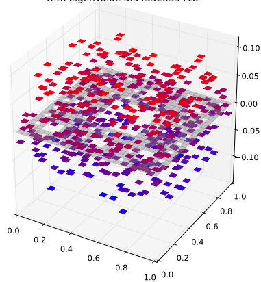
Klein Bottle Horizontal Glued Eigenfunction 203 with eigenvalue 3.34352539418
