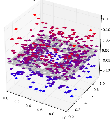
Klein Bottle Horizontal Glued Eigenfunction 209 with eigenvalue 3.37953552792
