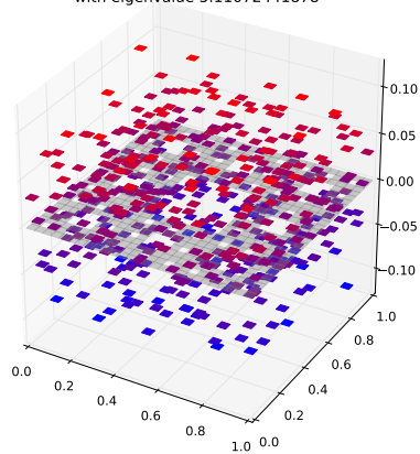
Klein Bottle Horizontal Glued Eigenfunction 353 with eigenvalue 5.11072441878
