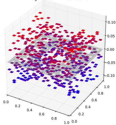
Klein Bottle Horizontal Glued Eigenfunction 272 with eigenvalue 4.21193453676
