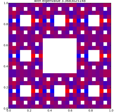
Klein Bottle Horizontal Glued Eigenfunction 208 with eigenvalue 3.3683025148
