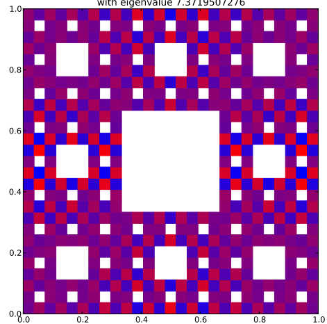
Klein Bottle Horizontal Glued Eigenfunction 510 with eigenvalue 7.3719507276
