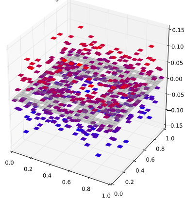
Klein Bottle Horizontal Glued Eigenfunction 373 with eigenvalue 5.30448162208
