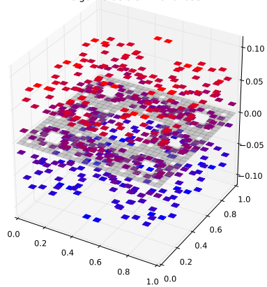
Klein Bottle Horizontal Glued Eigenfunction 222 with eigenvalue 3.51128162693
