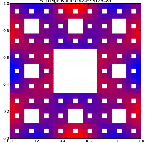
Klein Bottle Horizontal Glued Eigenfunction 15 with eigenvalue 0.424598126489
