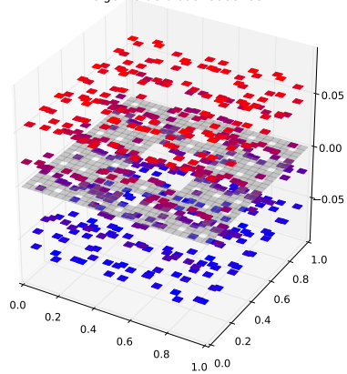
Klein Bottle Horizontal Glued Eigenfunction 416 with eigenvalue 6.0957393235
