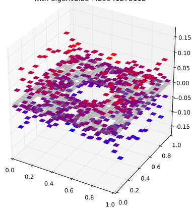
Klein Bottle Horizontal Glued Eigenfunction 499 with eigenvalue 7.29941275112
