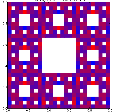
Klein Bottle Horizontal Glued Eigenfunction 249 with eigenvalue 3.76733918152
