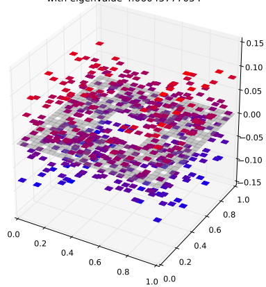
Klein Bottle Horizontal Glued Eigenfunction 266 with eigenvalue 4.06045777054
