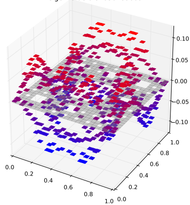
Klein Bottle Horizontal Glued Eigenfunction 32 with eigenvalue 0.810304896091
