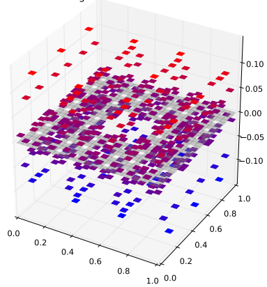
Klein Bottle Horizontal Glued Eigenfunction 497 with eigenvalue 7.27755947968
