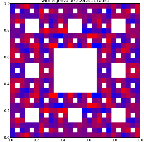
Klein Bottle Horizontal Glued Eigenfunction 149 with eigenvalue 2.84241170051
