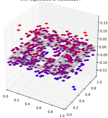
Klein Bottle Horizontal Glued Eigenfunction 60 with eigenvalue 1.4926015234
