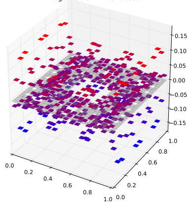
Klein Bottle Horizontal Glued Eigenfunction 488 with eigenvalue 7.2403480935
