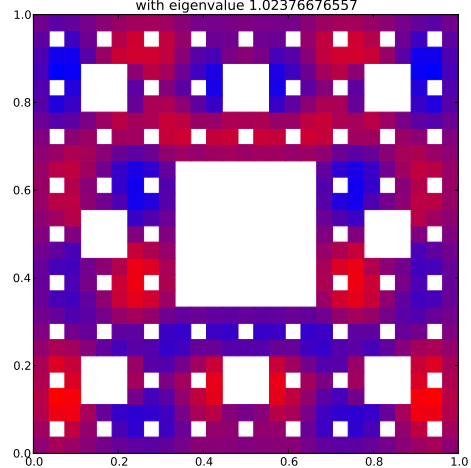
Klein Bottle Horizontal Glued Eigenfunction 40 with eigenvalue 1.02376676557
