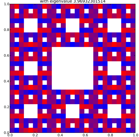
Klein Bottle Horizontal Glued Eigenfunction 261 with eigenvalue 3.96932301514
