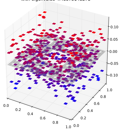
Klein Bottle Horizontal Glued Eigenfunction 297 with eigenvalue 4.48375148278
