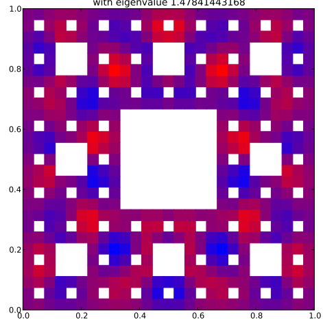
Klein Bottle Horizontal Glued Eigenfunction 58 with eigenvalue 1.47841443168
