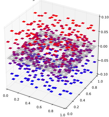
Klein Bottle Horizontal Glued Eigenfunction 395 with eigenvalue 5.73371692438
