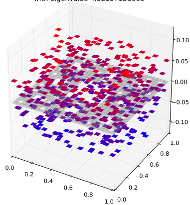
Klein Bottle Horizontal Glued Eigenfunction 299 with eigenvalue 4.52157126665
