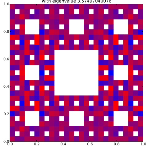
Klein Bottle Horizontal Glued Eigenfunction 228 with eigenvalue 3.57497040076
