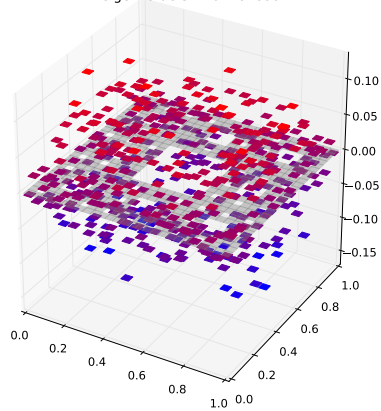
Klein Bottle Horizontal Glued Eigenfunction 366 with eigenvalue 5.24674818992
