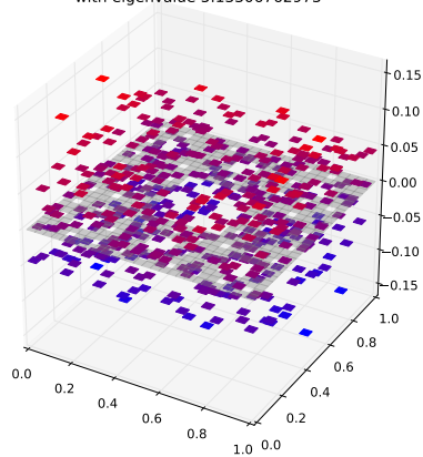
Klein Bottle Horizontal Glued Eigenfunction 355 with eigenvalue 5.13306762973
