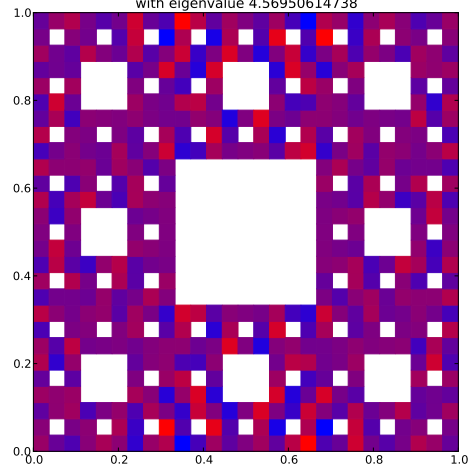
Klein Bottle Horizontal Glued Eigenfunction 304 with eigenvalue 4.56950614738
