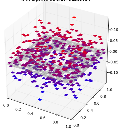
Klein Bottle Horizontal Glued Eigenfunction 184 with eigenvalue 3.19791269934
