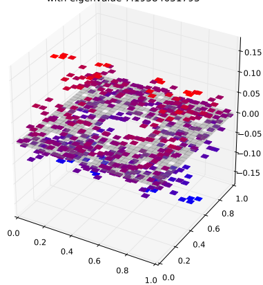
Klein Bottle Horizontal Glued Eigenfunction 477 with eigenvalue 7.19384631793
