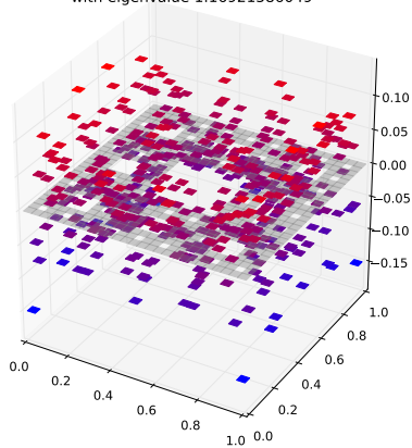
Klein Bottle Horizontal Glued Eigenfunction 45 with eigenvalue 1.16921586049
