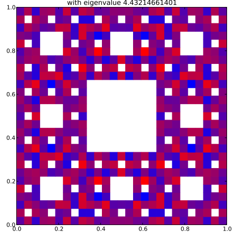
Klein Bottle Horizontal Glued Eigenfunction 290 with eigenvalue 4.43214661401
