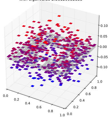
Klein Bottle Horizontal Glued Eigenfunction 151 with eigenvalue 2.86120932853
