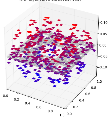
Klein Bottle Horizontal Glued Eigenfunction 53 with eigenvalue 1.31065578057
