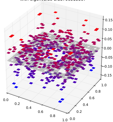
Klein Bottle Horizontal Glued Eigenfunction 47 with eigenvalue 1.18706513867
