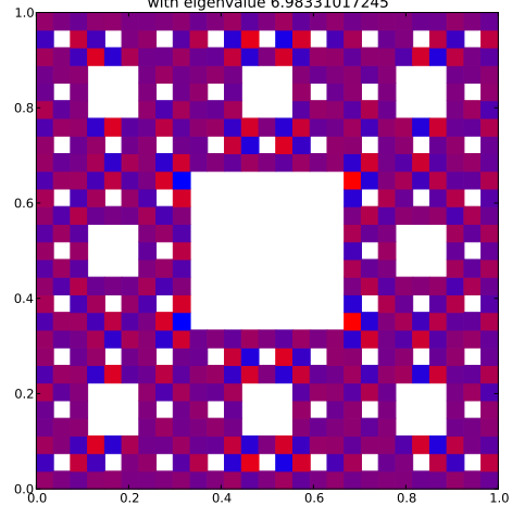
Klein Bottle Horizontal Glued Eigenfunction 455 with eigenvalue 6.98331017245
