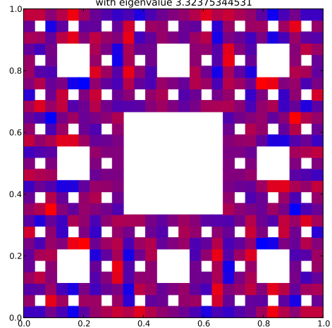
Klein Bottle Horizontal Glued Eigenfunction 202 with eigenvalue 3.32375344531
