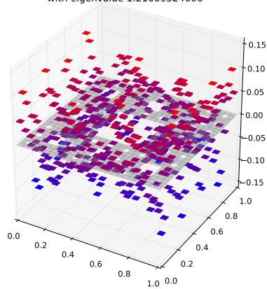
Klein Bottle Horizontal Glued Eigenfunction 48 with eigenvalue 1.21009324606
