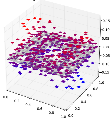
Klein Bottle Horizontal Glued Eigenfunction 362 with eigenvalue 5.19269487775
