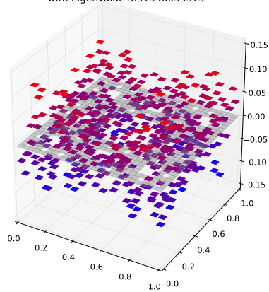
Klein Bottle Horizontal Glued Eigenfunction 224 with eigenvalue 3.51946035375
