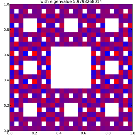
Klein Bottle Horizontal Glued Eigenfunction 408 with eigenvalue 5.9798268014
