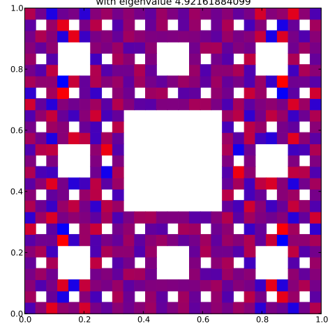
Klein Bottle Horizontal Glued Eigenfunction 335 with eigenvalue 4.92161884099
