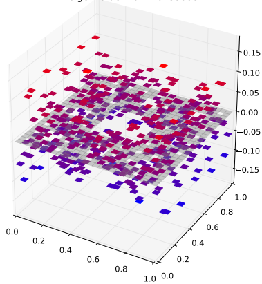
Klein Bottle Horizontal Glued Eigenfunction 72 with eigenvalue 1.67276435995
