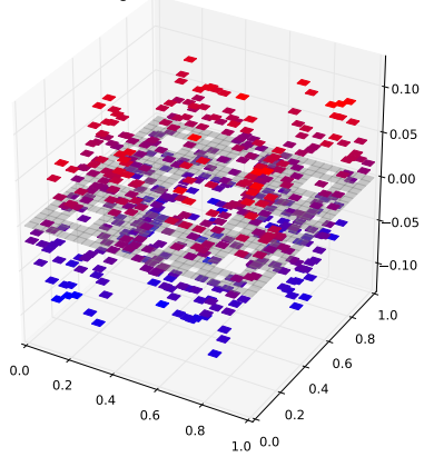
Klein Bottle Horizontal Glued Eigenfunction 38 with eigenvalue 0.977740186195
