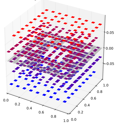
Klein Bottle Horizontal Glued Eigenfunction 446 with eigenvalue 6.73205080757
