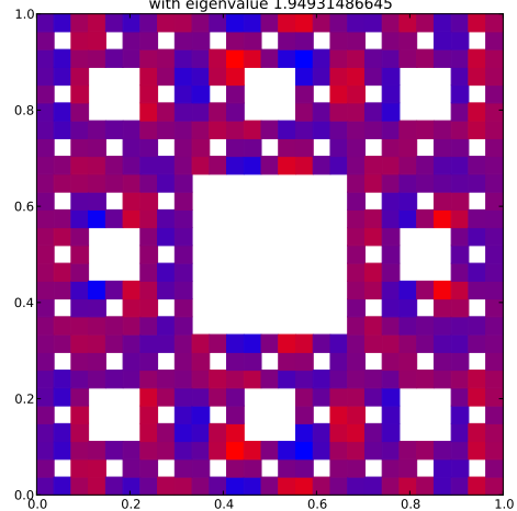
Klein Bottle Horizontal Glued Eigenfunction 90 with eigenvalue 1.94931486645
