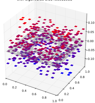
Klein Bottle Horizontal Glued Eigenfunction 206 with eigenvalue 3.35466988938
