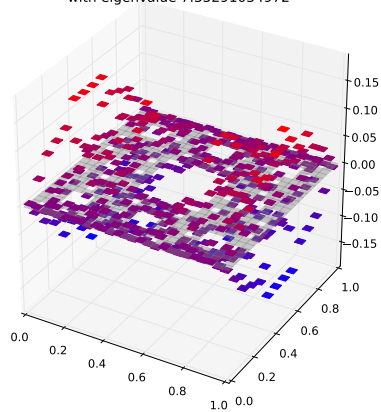
Klein Bottle Horizontal Glued Eigenfunction 509 with eigenvalue 7.35291034972
