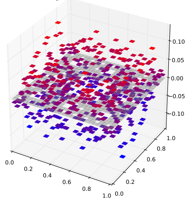
Klein Bottle Horizontal Glued Eigenfunction 191 with eigenvalue 3.23637917059
