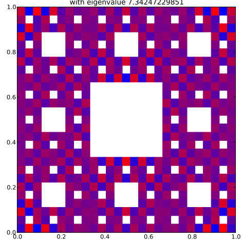
Klein Bottle Horizontal Glued Eigenfunction 505 with eigenvalue 7.34247229851
