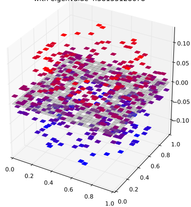
Klein Bottle Horizontal Glued Eigenfunction 287 with eigenvalue 4.38133128678
