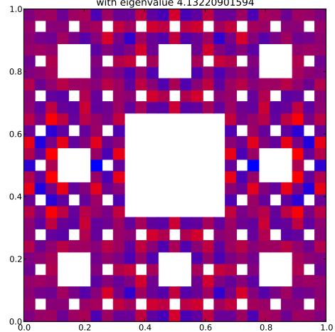
Klein Bottle Horizontal Glued Eigenfunction 270 with eigenvalue 4.13220901594
