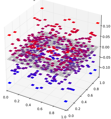
Klein Bottle Horizontal Glued Eigenfunction 501 with eigenvalue 7.31164817726
