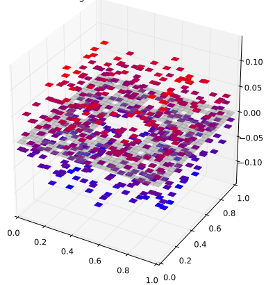
Klein Bottle Horizontal Glued Eigenfunction 241 with eigenvalue 3.70904651627
