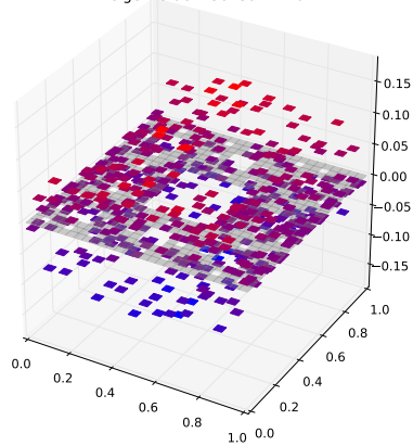
Klein Bottle Horizontal Glued Eigenfunction 500 with eigenvalue 7.30739274407
