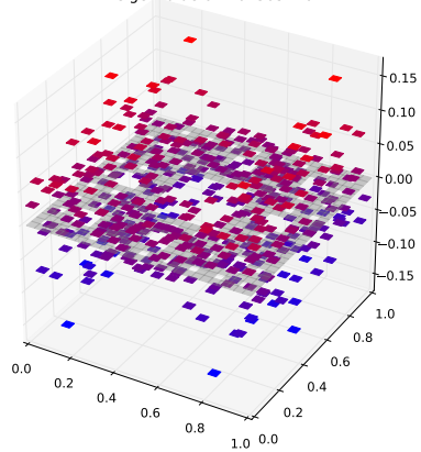
Klein Bottle Horizontal Glued Eigenfunction 420 with eigenvalue 6.2107305226
