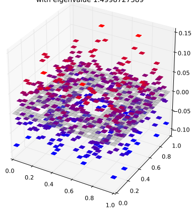
Klein Bottle Horizontal Glued Eigenfunction 62 with eigenvalue 1.4998727589
