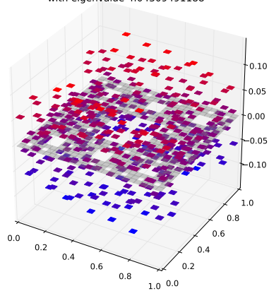
Klein Bottle Horizontal Glued Eigenfunction 265 with eigenvalue 4.04309491188
