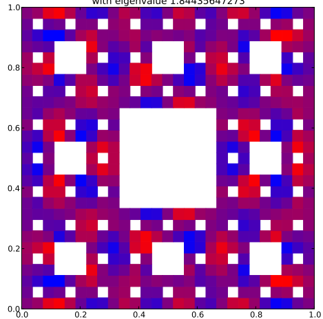
Klein Bottle Horizontal Glued Eigenfunction 80 with eigenvalue 1.84435647273
