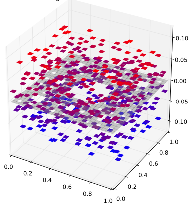
Klein Bottle Horizontal Glued Eigenfunction 289 with eigenvalue 4.42018942175
