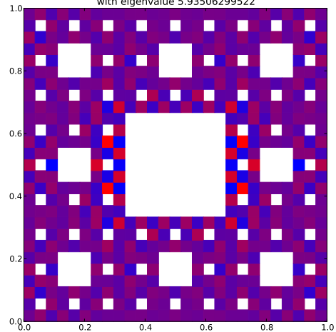
Klein Bottle Horizontal Glued Eigenfunction 405 with eigenvalue 5.93506299522
