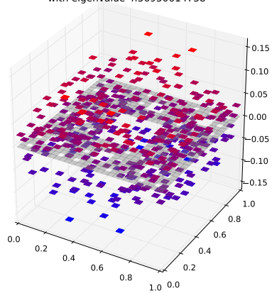
Klein Bottle Horizontal Glued Eigenfunction 304 with eigenvalue 4.56950614738
