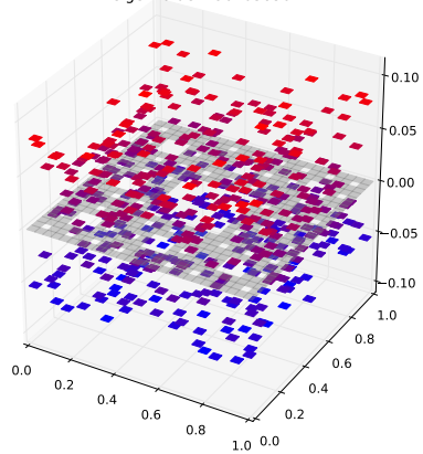
Klein Bottle Horizontal Glued Eigenfunction 336 with eigenvalue 4.96203836772
