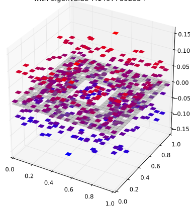
Klein Bottle Horizontal Glued Eigenfunction 471 with eigenvalue 7.14977602954
