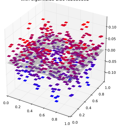
Klein Bottle Horizontal Glued Eigenfunction 52 with eigenvalue 1.30432639392
