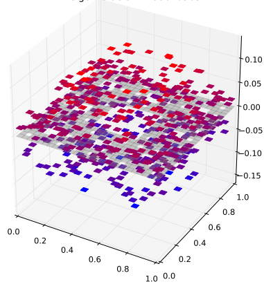
Klein Bottle Horizontal Glued Eigenfunction 214 with eigenvalue 3.42233676563
