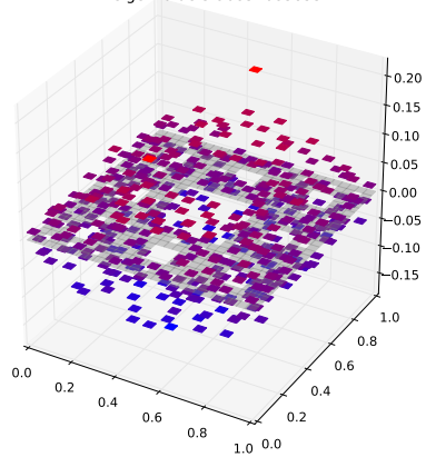
Klein Bottle Horizontal Glued Eigenfunction 260 with eigenvalue 3.96857683855
