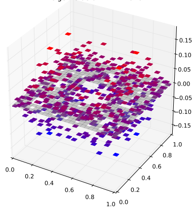
Klein Bottle Horizontal Glued Eigenfunction 422 with eigenvalue 6.22712429782
