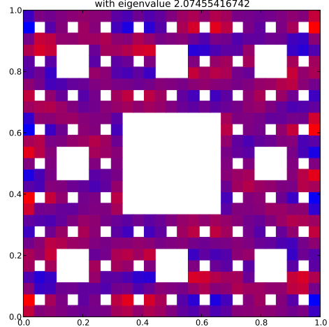
Klein Bottle Horizontal Glued Eigenfunction 106 with eigenvalue 2.07455416742
