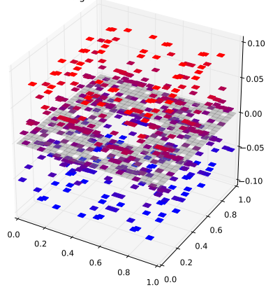
Klein Bottle Horizontal Glued Eigenfunction 277 with eigenvalue 4.23864505151
