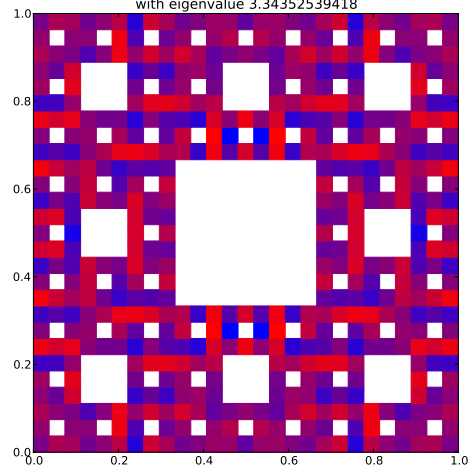
Klein Bottle Horizontal Glued Eigenfunction 203 with eigenvalue 3.34352539418
