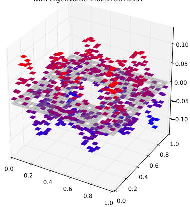
Klein Bottle Horizontal Glued Eigenfunction 40 with eigenvalue 1.02376676557
