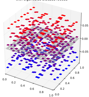
Klein Bottle Horizontal Glued Eigenfunction 207 with eigenvalue 3.36288406035
