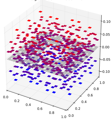
Klein Bottle Horizontal Glued Eigenfunction 320 with eigenvalue 4.7279682249
