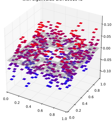
Klein Bottle Horizontal Glued Eigenfunction 42 with eigenvalue 1.071901948
