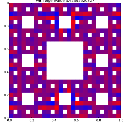
Klein Bottle Horizontal Glued Eigenfunction 215 with eigenvalue 3.42395520327
