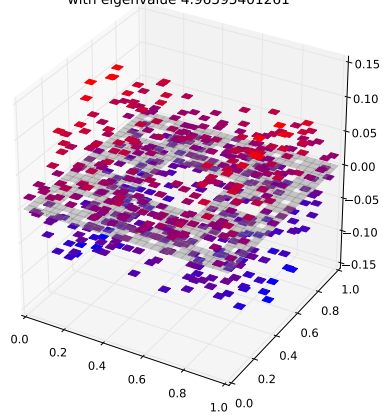
Klein Bottle Horizontal Glued Eigenfunction 338 with eigenvalue 4.96595401261
