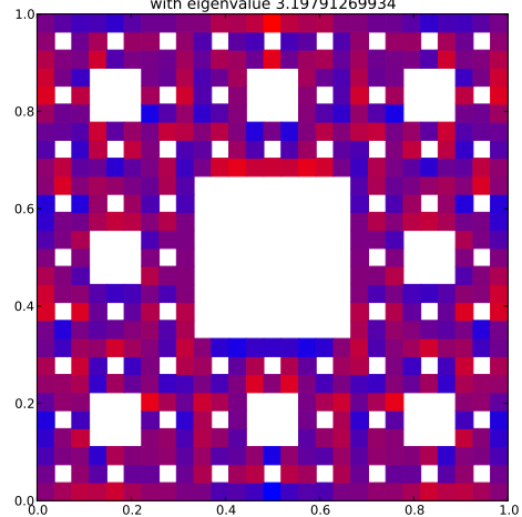
Klein Bottle Horizontal Glued Eigenfunction 184 with eigenvalue 3.19791269934
