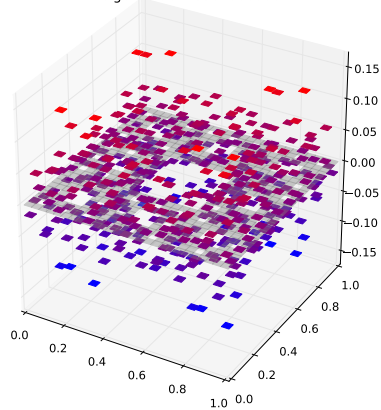
Klein Bottle Horizontal Glued Eigenfunction 461 with eigenvalue 7.05810689884
