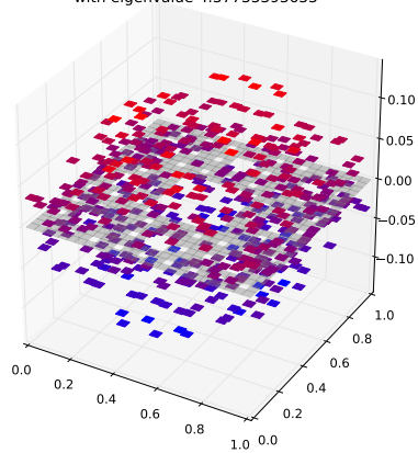
Klein Bottle Horizontal Glued Eigenfunction 286 with eigenvalue 4.37733393633
