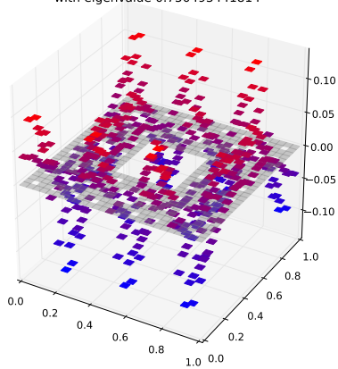
Klein Bottle Horizontal Glued Eigenfunction 28 with eigenvalue 0.750493441814
