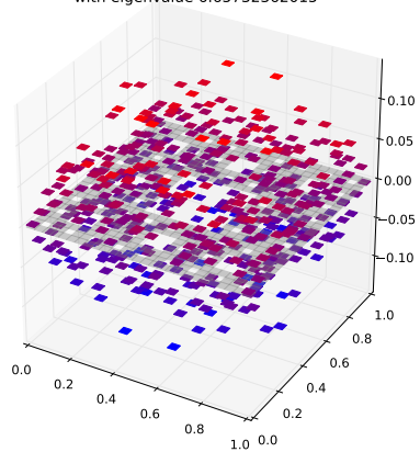
Klein Bottle Horizontal Glued Eigenfunction 443 with eigenvalue 6.65732362015
