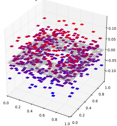
Klein Bottle Horizontal Glued Eigenfunction 217 with eigenvalue 3.43432819629
