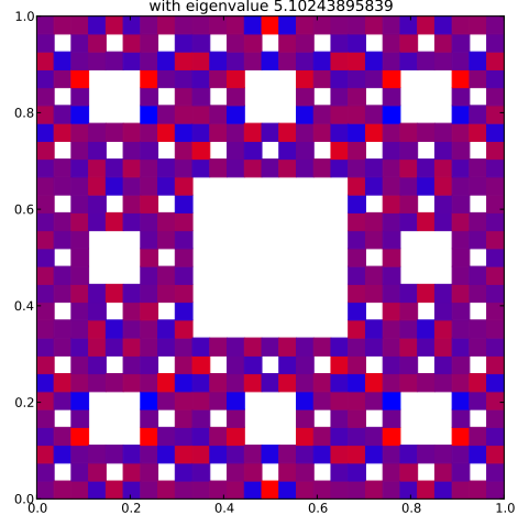
Klein Bottle Horizontal Glued Eigenfunction 352 with eigenvalue 5.10243895839
