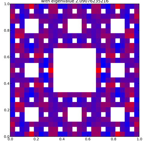
Klein Bottle Horizontal Glued Eigenfunction 108 with eigenvalue 2.09076235216
