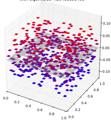
Klein Bottle Horizontal Glued Eigenfunction 279 with eigenvalue 4.29468898498
