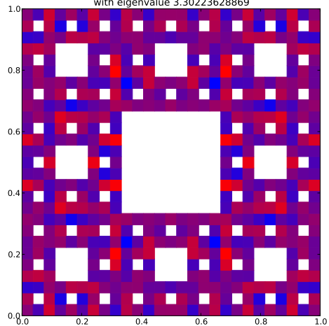
Klein Bottle Horizontal Glued Eigenfunction 198 with eigenvalue 3.30223628869
