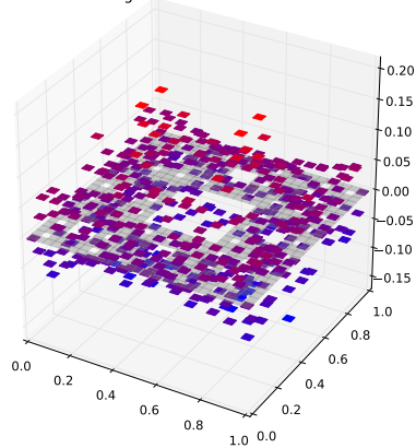
Klein Bottle Horizontal Glued Eigenfunction 405 with eigenvalue 5.93506299522
