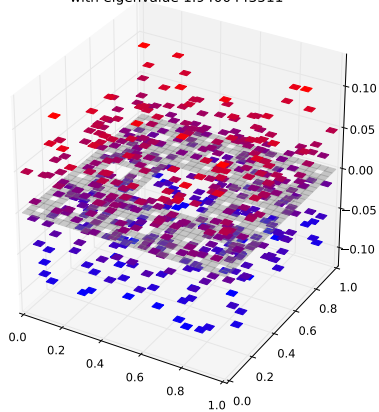
Klein Bottle Horizontal Glued Eigenfunction 89 with eigenvalue 1.9400443511
