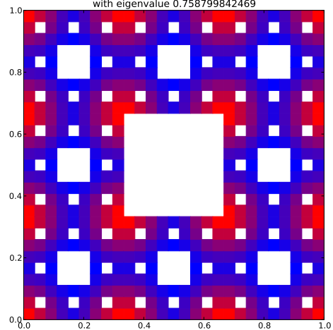
Klein Bottle Horizontal Glued Eigenfunction 30 with eigenvalue 0.758799842469
