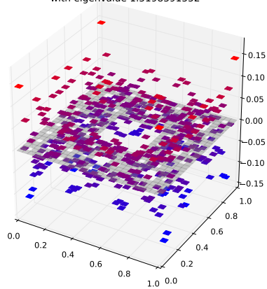
Klein Bottle Horizontal Glued Eigenfunction 64 with eigenvalue 1.5198391552
