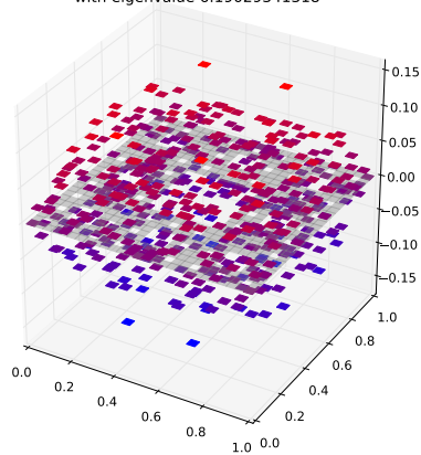
Klein Bottle Horizontal Glued Eigenfunction 419 with eigenvalue 6.19029341318
