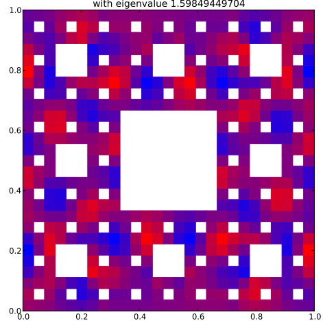
Klein Bottle Horizontal Glued Eigenfunction 68 with eigenvalue 1.59849449704
