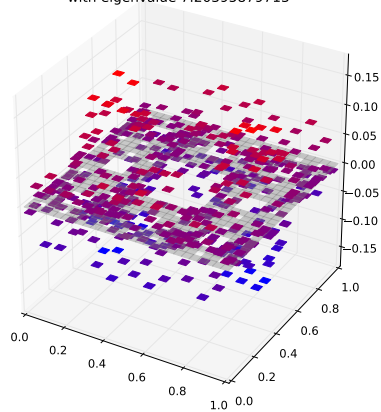
Klein Bottle Horizontal Glued Eigenfunction 479 with eigenvalue 7.20395879713
