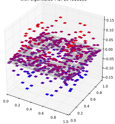
Klein Bottle Horizontal Glued Eigenfunction 496 with eigenvalue 7.2719461135
