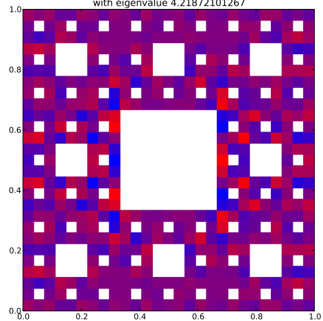
Klein Bottle Horizontal Glued Eigenfunction 275 with eigenvalue 4.21872101267
