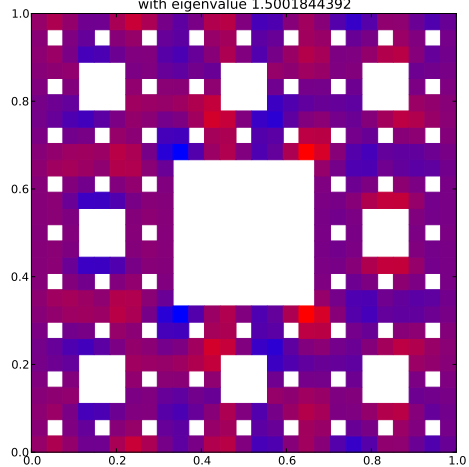
Klein Bottle Horizontal Glued Eigenfunction 63 with eigenvalue 1.5001844392
