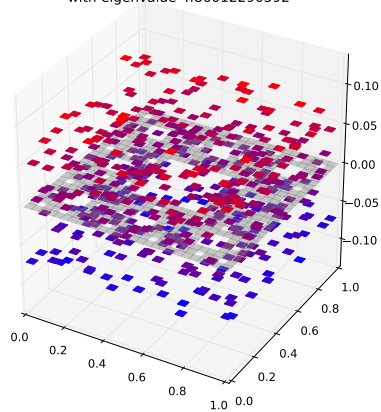
Klein Bottle Horizontal Glued Eigenfunction 329 with eigenvalue 4.86012290592
