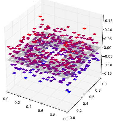
Klein Bottle Horizontal Glued Eigenfunction 321 with eigenvalue 4.72990654701
