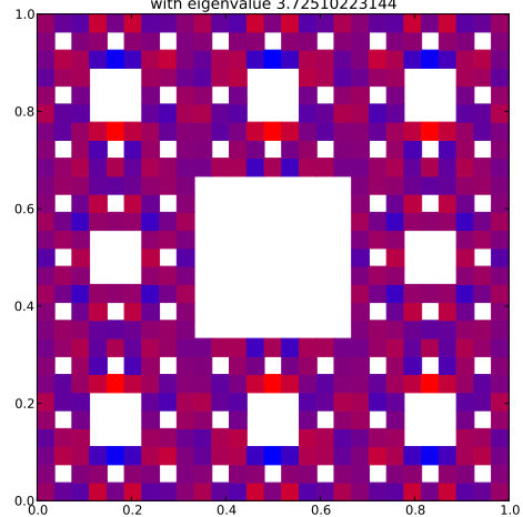
Klein Bottle Horizontal Glued Eigenfunction 244 with eigenvalue 3.72510223144
