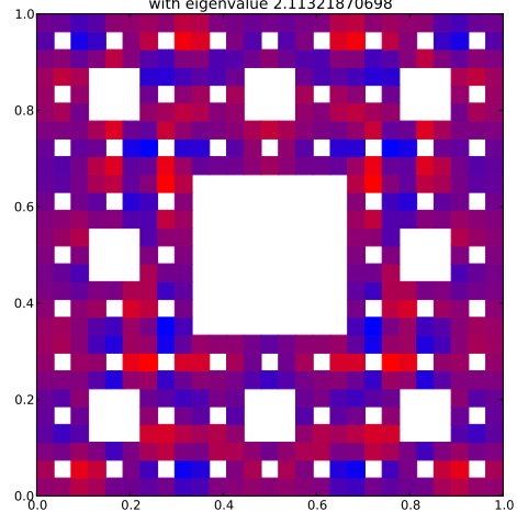
Klein Bottle Horizontal Glued Eigenfunction 110 with eigenvalue 2.11321870698
