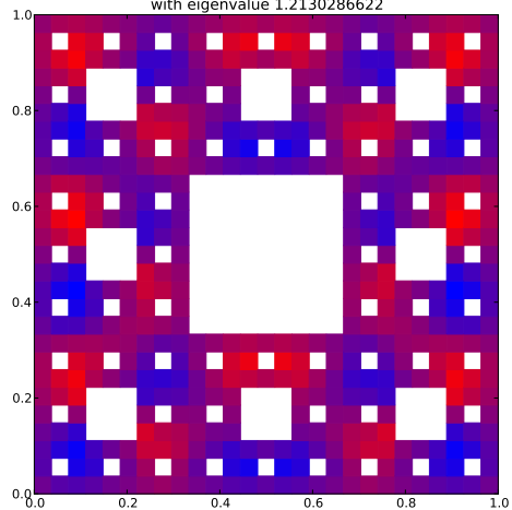
Klein Bottle Horizontal Glued Eigenfunction 49 with eigenvalue 1.2130286622
