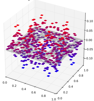
Klein Bottle Horizontal Glued Eigenfunction 51 with eigenvalue 1.29307032415
