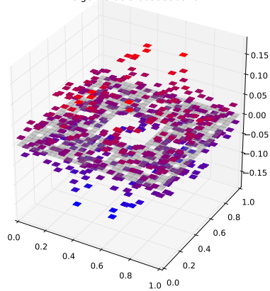
Klein Bottle Horizontal Glued Eigenfunction 402 with eigenvalue 5.88955963182
