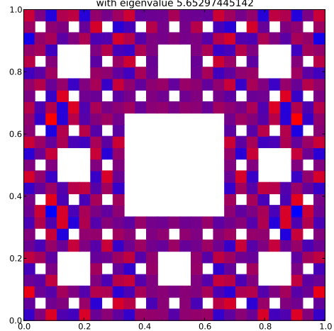
Klein Bottle Horizontal Glued Eigenfunction 391 with eigenvalue 5.65297445142
