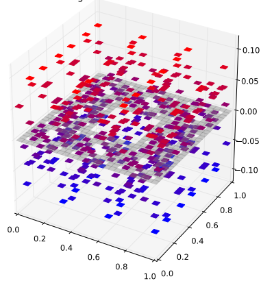
Klein Bottle Horizontal Glued Eigenfunction 387 with eigenvalue 5.57257068024
