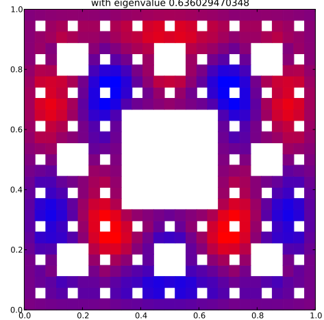
Klein Bottle Horizontal Glued Eigenfunction 21 with eigenvalue 0.636029470348
