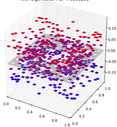
Klein Bottle Horizontal Glued Eigenfunction 475 with eigenvalue 7.17476050256
