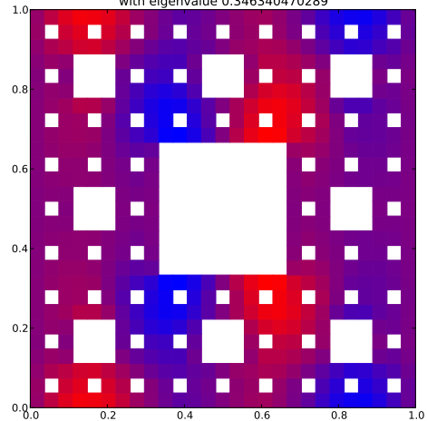
Klein Bottle Horizontal Glued Eigenfunction 12 with eigenvalue 0.346340470289
