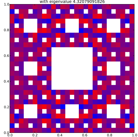
Klein Bottle Horizontal Glued Eigenfunction 282 with eigenvalue 4.32079091826
