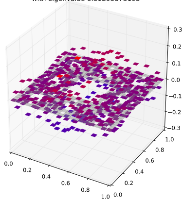
Klein Bottle Horizontal Glued Eigenfunction 427 with eigenvalue 6.31295873193
