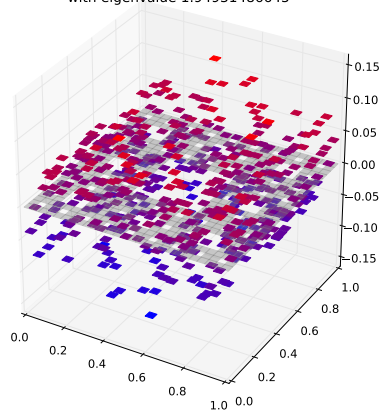
Klein Bottle Horizontal Glued Eigenfunction 90 with eigenvalue 1.94931486645
