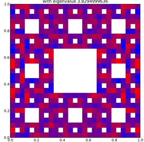
Klein Bottle Horizontal Glued Eigenfunction 253 with eigenvalue 3.8294999636
