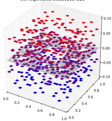
Klein Bottle Horizontal Glued Eigenfunction 374 with eigenvalue 5.31502684528
