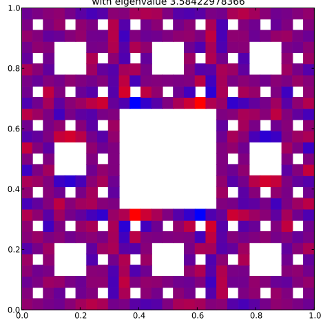
Klein Bottle Horizontal Glued Eigenfunction 229 with eigenvalue 3.58422978366
