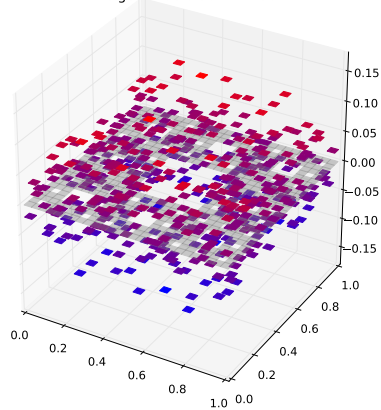
Klein Bottle Horizontal Glued Eigenfunction 435 with eigenvalue 6.5027171582
