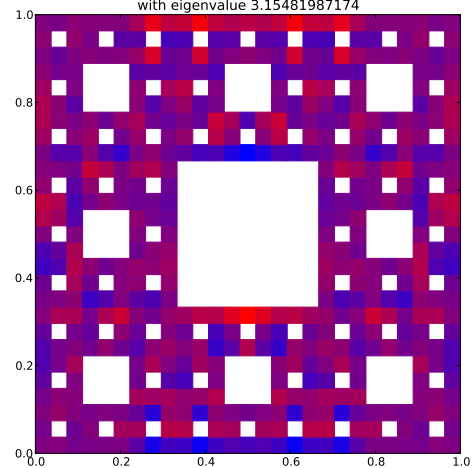
Klein Bottle Horizontal Glued Eigenfunction 180 with eigenvalue 3.15481987174
