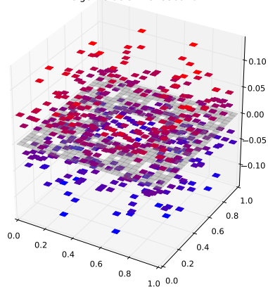
Klein Bottle Horizontal Glued Eigenfunction 398 with eigenvalue 5.74573589164
