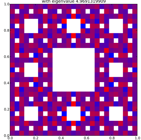
Klein Bottle Horizontal Glued Eigenfunction 339 with eigenvalue 4.9691319909
