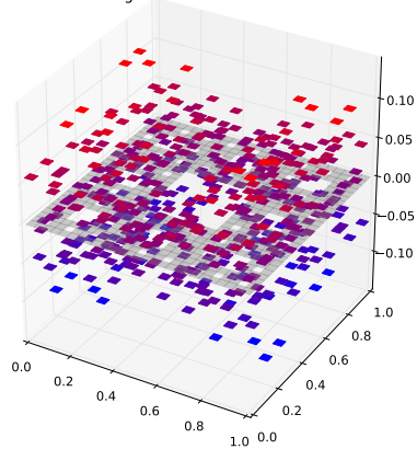
Klein Bottle Horizontal Glued Eigenfunction 451 with eigenvalue 6.91143080912
