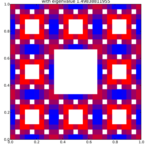
Klein Bottle Horizontal Glued Eigenfunction 61 with eigenvalue 1.49838811955
