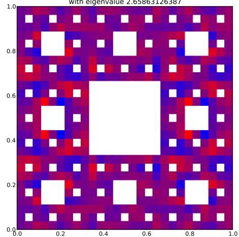
Klein Bottle Horizontal Glued Eigenfunction 138 with eigenvalue 2.65863126387
