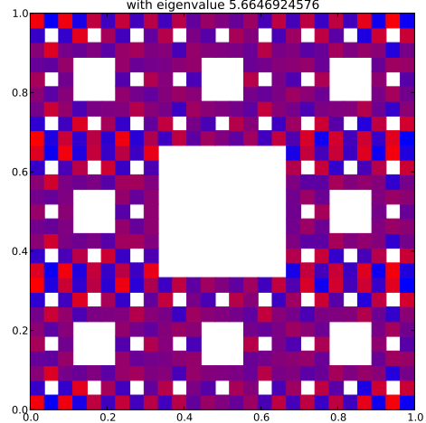
Klein Bottle Horizontal Glued Eigenfunction 392 with eigenvalue 5.6646924576
