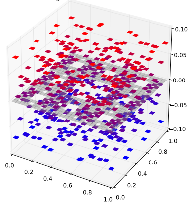
Klein Bottle Horizontal Glued Eigenfunction 490 with eigenvalue 7.24963276888
