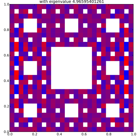
Klein Bottle Horizontal Glued Eigenfunction 338 with eigenvalue 4.96595401261
