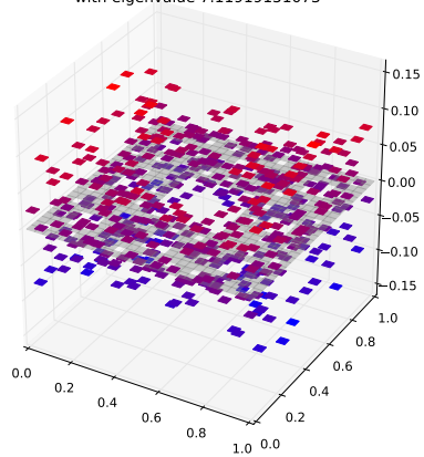
Klein Bottle Horizontal Glued Eigenfunction 468 with eigenvalue 7.11919151073
