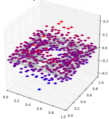
Klein Bottle Horizontal Glued Eigenfunction 440 with eigenvalue 6.59421013638
