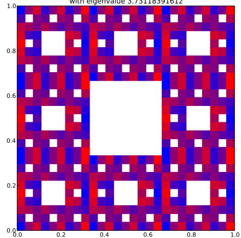
Klein Bottle Horizontal Glued Eigenfunction 245 with eigenvalue 3.73118391612
