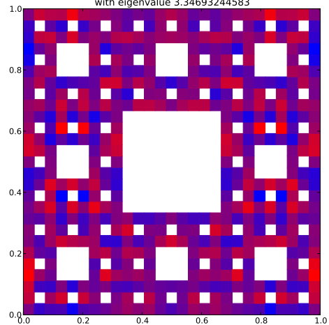
Klein Bottle Horizontal Glued Eigenfunction 204 with eigenvalue 3.34693244583
