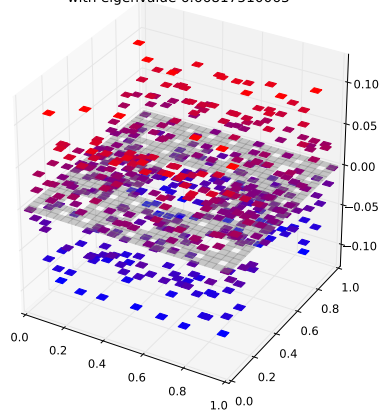
Klein Bottle Horizontal Glued Eigenfunction 444 with eigenvalue 6.66817510063
