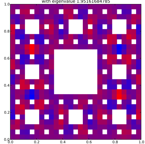
Klein Bottle Horizontal Glued Eigenfunction 91 with eigenvalue 1.95161684785
