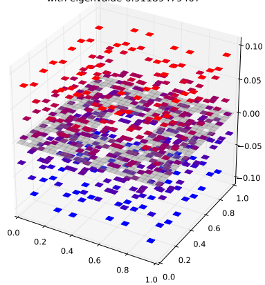
Klein Bottle Horizontal Glued Eigenfunction 452 with eigenvalue 6.91189479407
