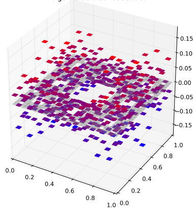
Klein Bottle Horizontal Glued Eigenfunction 450 with eigenvalue 6.89709536506
