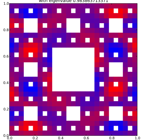
Klein Bottle Horizontal Glued Eigenfunction 39 with eigenvalue 0.983863713371
