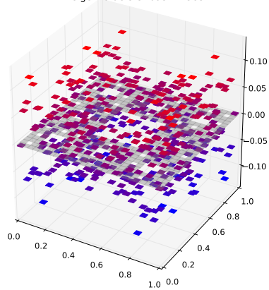
Klein Bottle Horizontal Glued Eigenfunction 204 with eigenvalue 3.34693244583
