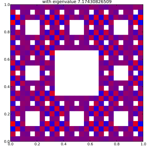
Klein Bottle Horizontal Glued Eigenfunction 474 with eigenvalue 7.17430826509
