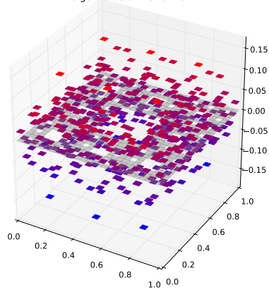
Klein Bottle Horizontal Glued Eigenfunction 244 with eigenvalue 3.72510223144
