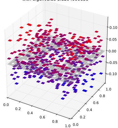
Klein Bottle Horizontal Glued Eigenfunction 253 with eigenvalue 3.8294999636
