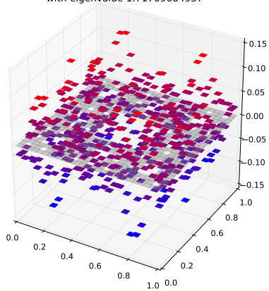
Klein Bottle Horizontal Glued Eigenfunction 74 with eigenvalue 1.71709684957
