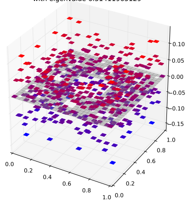
Klein Bottle Horizontal Glued Eigenfunction 428 with eigenvalue 6.31411965129
