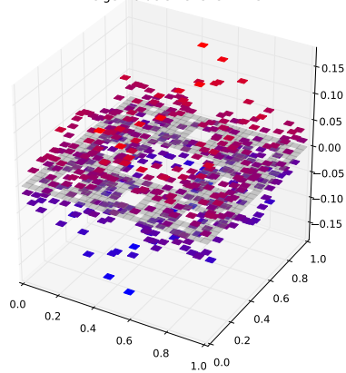
Klein Bottle Horizontal Glued Eigenfunction 216 with eigenvalue 3.43134324145
