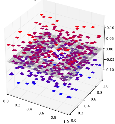
Klein Bottle Horizontal Glued Eigenfunction 382 with eigenvalue 5.51777818923
