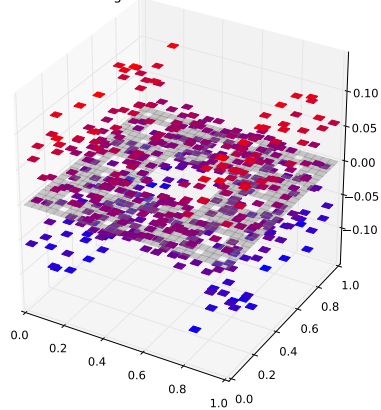
Klein Bottle Horizontal Glued Eigenfunction 361 with eigenvalue 5.17745867101
