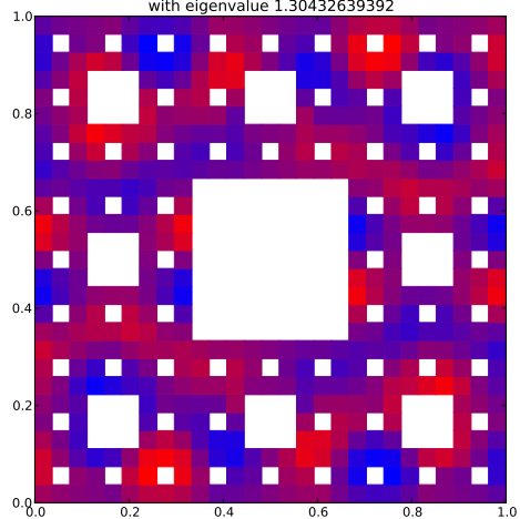
Klein Bottle Horizontal Glued Eigenfunction 52 with eigenvalue 1.30432639392
