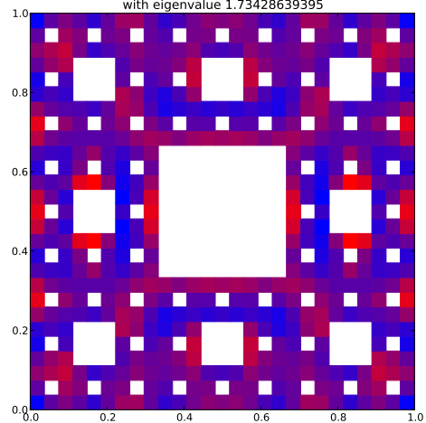
Klein Bottle Horizontal Glued Eigenfunction 76 with eigenvalue 1.73428639395
