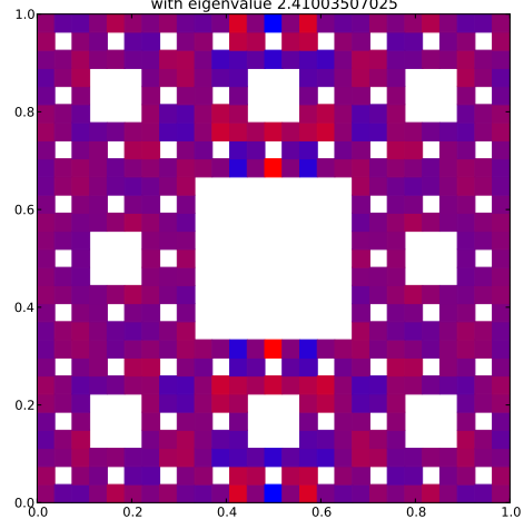
Klein Bottle Horizontal Glued Eigenfunction 128 with eigenvalue 2.41003507025
