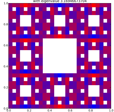
Klein Bottle Horizontal Glued Eigenfunction 181 with eigenvalue 3.16946673704
