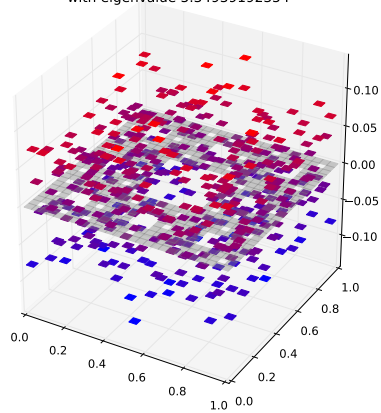
Klein Bottle Horizontal Glued Eigenfunction 376 with eigenvalue 5.34939192354
