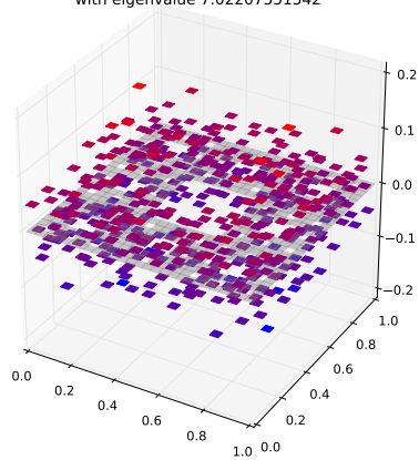
Klein Bottle Horizontal Glued Eigenfunction 458 with eigenvalue 7.02207551542
