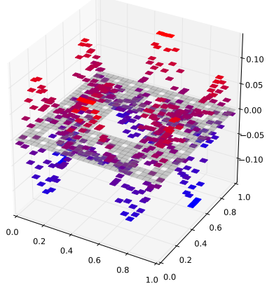
Klein Bottle Horizontal Glued Eigenfunction 15 with eigenvalue 0.424598126489
