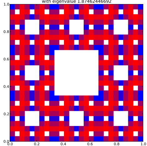
Klein Bottle Horizontal Glued Eigenfunction 83 with eigenvalue 1.87462446692
