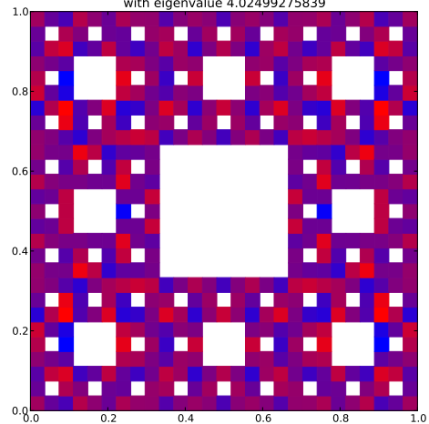
Klein Bottle Horizontal Glued Eigenfunction 264 with eigenvalue 4.02499275839
