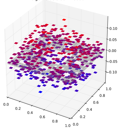
Klein Bottle Horizontal Glued Eigenfunction 210 with eigenvalue 3.38214395047
