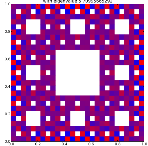
Klein Bottle Horizontal Glued Eigenfunction 394 with eigenvalue 5.70995665292
