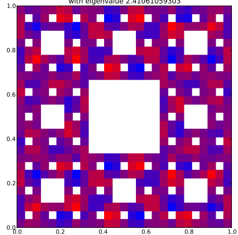
Klein Bottle Horizontal Glued Eigenfunction 129 with eigenvalue 2.41061059303
