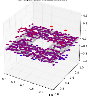
Klein Bottle Horizontal Glued Eigenfunction 426 with eigenvalue 6.31126311638
