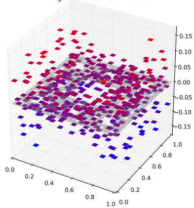
Klein Bottle Horizontal Glued Eigenfunction 256 with eigenvalue 3.84837272846
