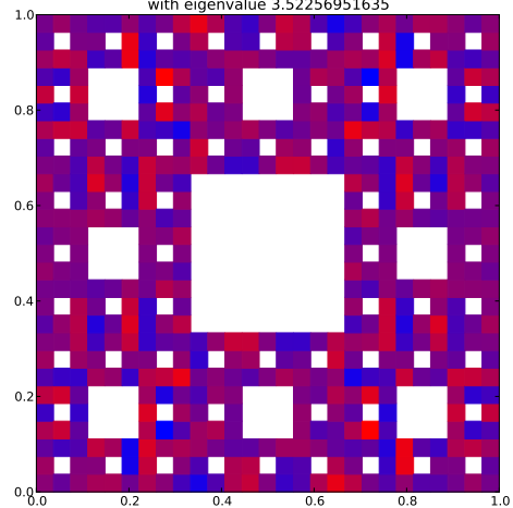
Klein Bottle Horizontal Glued Eigenfunction 225 with eigenvalue 3.52256951635
