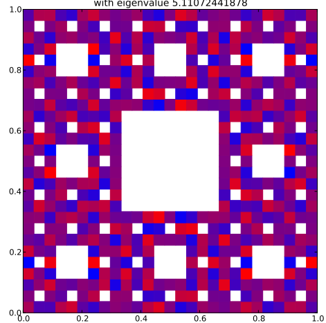
Klein Bottle Horizontal Glued Eigenfunction 353 with eigenvalue 5.11072441878
