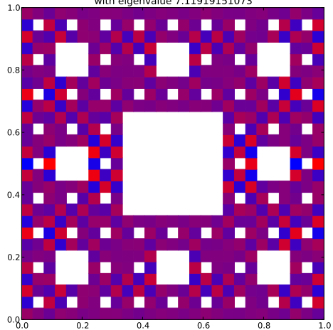
Klein Bottle Horizontal Glued Eigenfunction 468 with eigenvalue 7.11919151073
