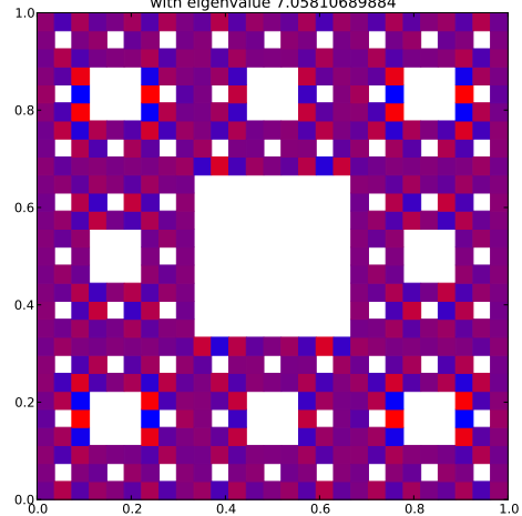
Klein Bottle Horizontal Glued Eigenfunction 461 with eigenvalue 7.05810689884
