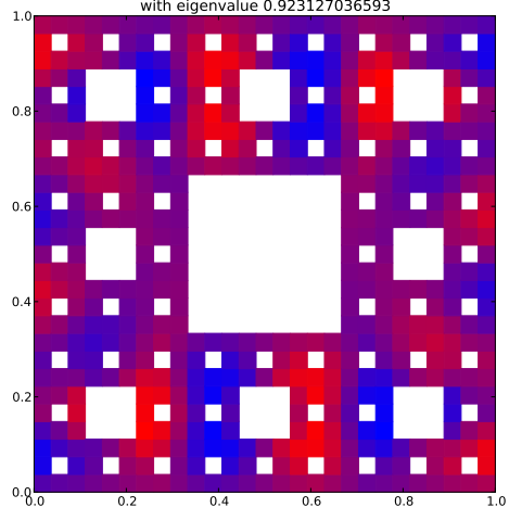
Klein Bottle Horizontal Glued Eigenfunction 34 with eigenvalue 0.923127036593
