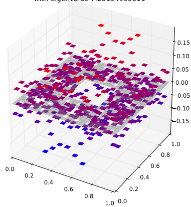
Klein Bottle Horizontal Glued Eigenfunction 498 with eigenvalue 7.28194995011
