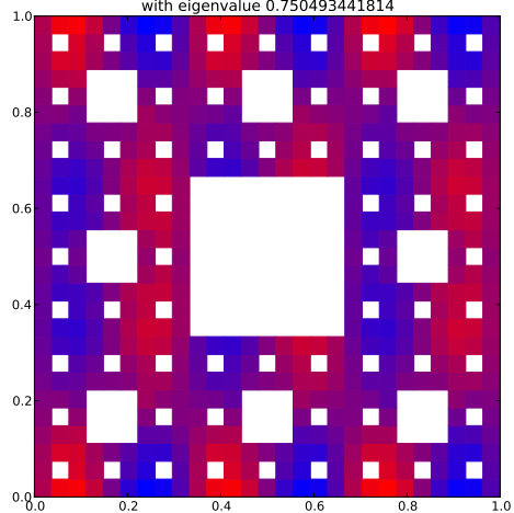
Klein Bottle Horizontal Glued Eigenfunction 28 with eigenvalue 0.750493441814
