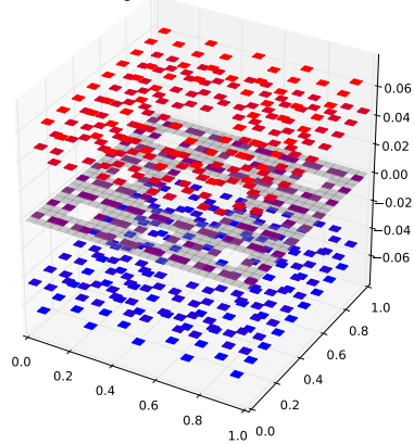
Klein Bottle Horizontal Glued Eigenfunction 306 with eigenvalue 4.58578643763
