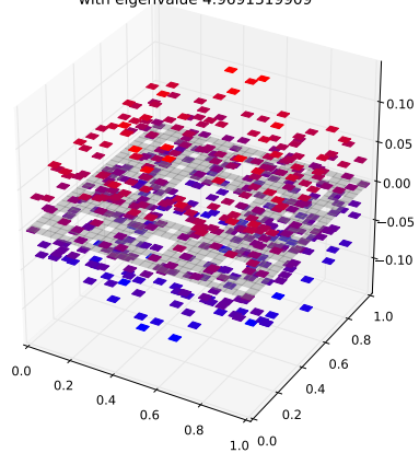
Klein Bottle Horizontal Glued Eigenfunction 339 with eigenvalue 4.9691319909
