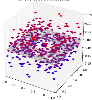
Klein Bottle Horizontal Glued Eigenfunction 71 with eigenvalue 1.64941553723
