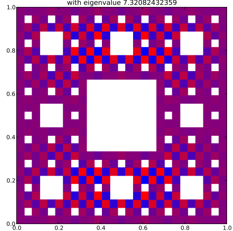
Klein Bottle Horizontal Glued Eigenfunction 502 with eigenvalue 7.32082432359
