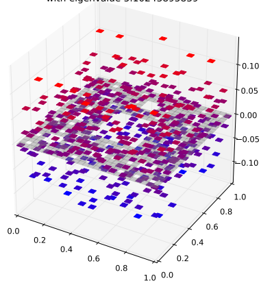
Klein Bottle Horizontal Glued Eigenfunction 352 with eigenvalue 5.10243895839
