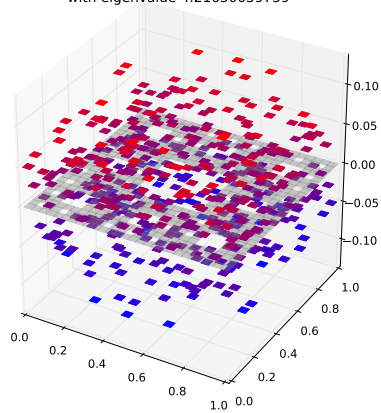
Klein Bottle Horizontal Glued Eigenfunction 274 with eigenvalue 4.21650059759
