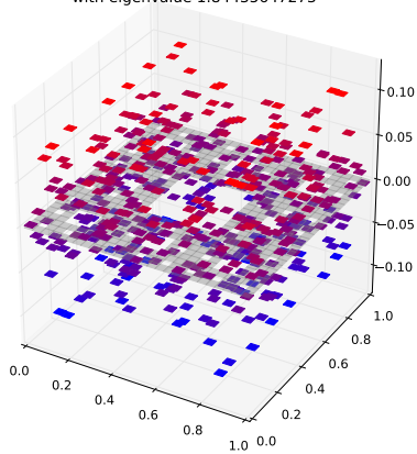
Klein Bottle Horizontal Glued Eigenfunction 80 with eigenvalue 1.84435647273
