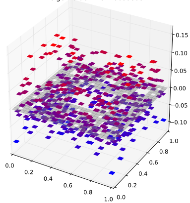
Klein Bottle Horizontal Glued Eigenfunction 76 with eigenvalue 1.73428639395
