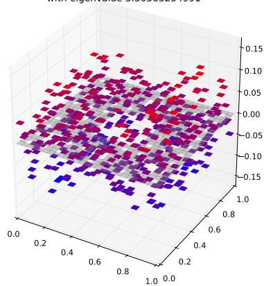
Klein Bottle Horizontal Glued Eigenfunction 199 with eigenvalue 3.30563254991
