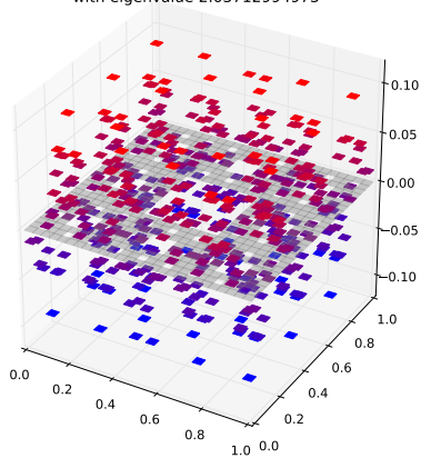
Klein Bottle Horizontal Glued Eigenfunction 99 with eigenvalue 2.03712994973
