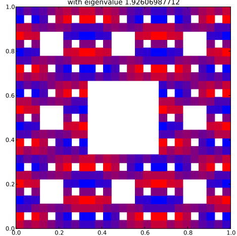
Klein Bottle Horizontal Glued Eigenfunction 87 with eigenvalue 1.92606987712
