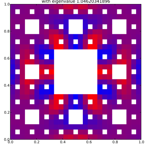
Klein Bottle Horizontal Glued Eigenfunction 41 with eigenvalue 1.04620341896
