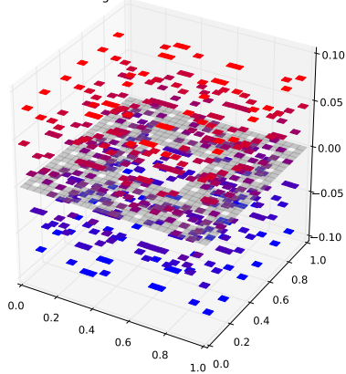
Klein Bottle Horizontal Glued Eigenfunction 87 with eigenvalue 1.92606987712
