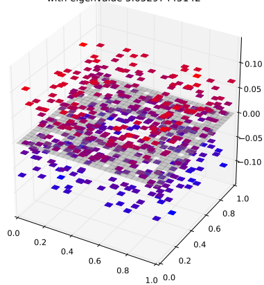
Klein Bottle Horizontal Glued Eigenfunction 391 with eigenvalue 5.65297445142
