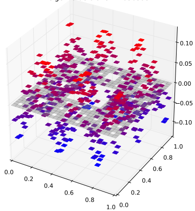
Klein Bottle Horizontal Glued Eigenfunction 34 with eigenvalue 0.923127036593
