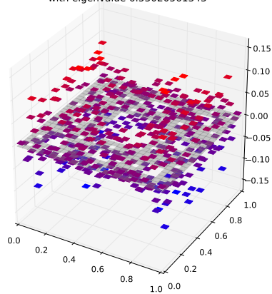
Klein Bottle Horizontal Glued Eigenfunction 437 with eigenvalue 6.53020561343
