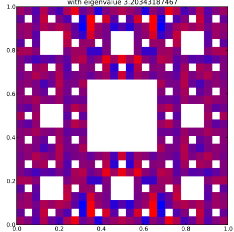
Klein Bottle Horizontal Glued Eigenfunction 185 with eigenvalue 3.20343187467
