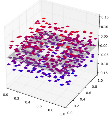
Klein Bottle Horizontal Glued Eigenfunction 371 with eigenvalue 5.28926706108
