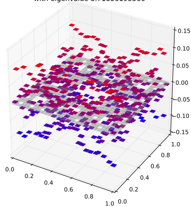
Klein Bottle Horizontal Glued Eigenfunction 243 with eigenvalue 3.71856193566
