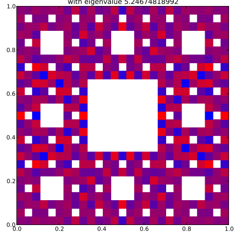
Klein Bottle Horizontal Glued Eigenfunction 366 with eigenvalue 5.24674818992
