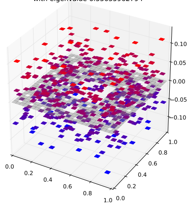
Klein Bottle Horizontal Glued Eigenfunction 430 with eigenvalue 6.33635962794
