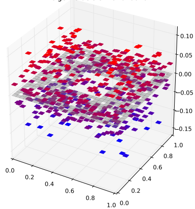
Klein Bottle Horizontal Glued Eigenfunction 228 with eigenvalue 3.57497040076
