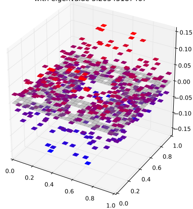
Klein Bottle Horizontal Glued Eigenfunction 185 with eigenvalue 3.20343187467
