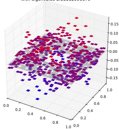
Klein Bottle Horizontal Glued Eigenfunction 153 with eigenvalue 2.88582990679
