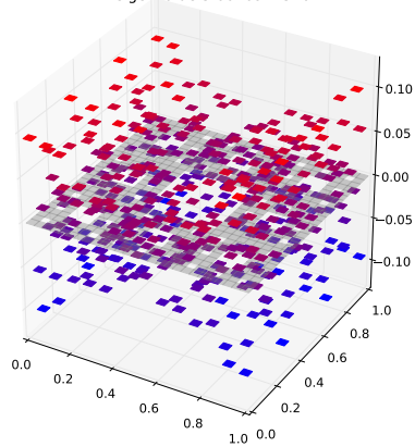
Klein Bottle Horizontal Glued Eigenfunction 392 with eigenvalue 5.6646924576
