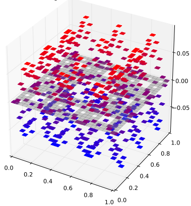
Klein Bottle Horizontal Glued Eigenfunction 16 with eigenvalue 0.441021780966
