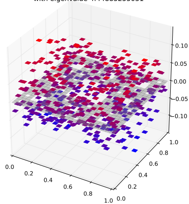
Klein Bottle Horizontal Glued Eigenfunction 291 with eigenvalue 4.44885255031
