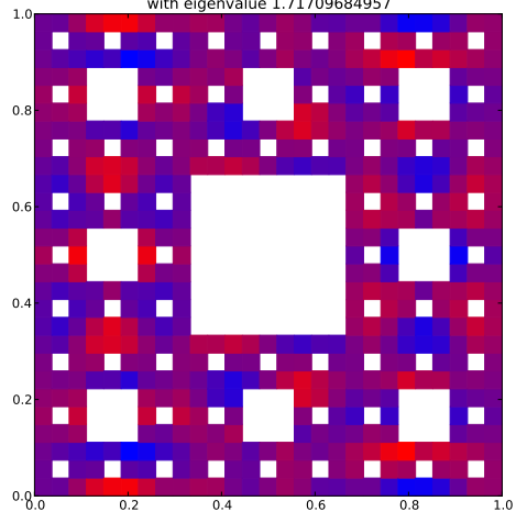
Klein Bottle Horizontal Glued Eigenfunction 74 with eigenvalue 1.71709684957
