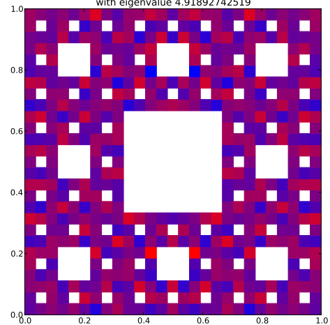
Klein Bottle Horizontal Glued Eigenfunction 334 with eigenvalue 4.91892742519
