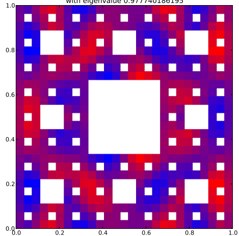
Klein Bottle Horizontal Glued Eigenfunction 38 with eigenvalue 0.977740186195
