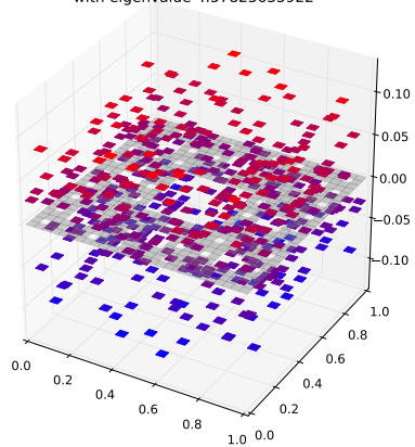
Klein Bottle Horizontal Glued Eigenfunction 305 with eigenvalue 4.57825635922
