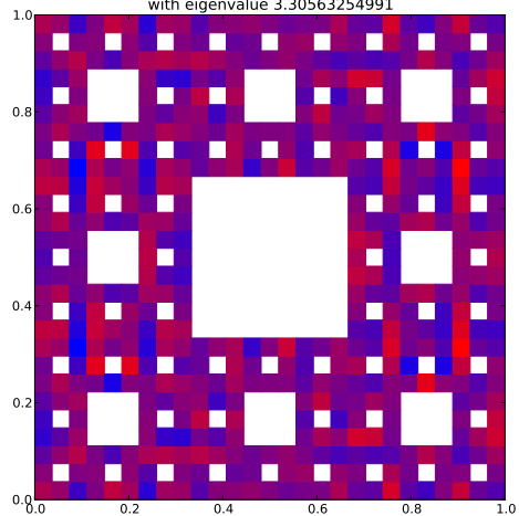
Klein Bottle Horizontal Glued Eigenfunction 199 with eigenvalue 3.30563254991
