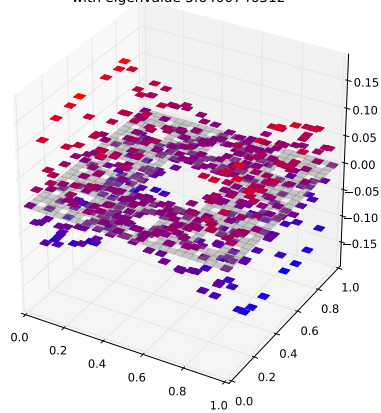
Klein Bottle Horizontal Glued Eigenfunction 390 with eigenvalue 5.6400746512
