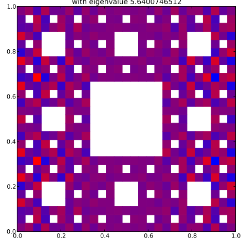
Klein Bottle Horizontal Glued Eigenfunction 390 with eigenvalue 5.6400746512
