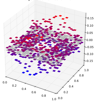
Klein Bottle Horizontal Glued Eigenfunction 340 with eigenvalue 4.97783494729
