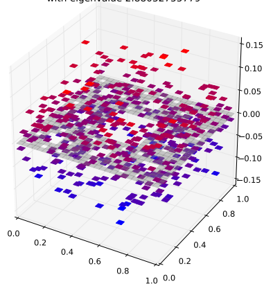
Klein Bottle Horizontal Glued Eigenfunction 152 with eigenvalue 2.88032755779
