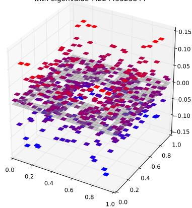
Klein Bottle Horizontal Glued Eigenfunction 484 with eigenvalue 7.22445523844
