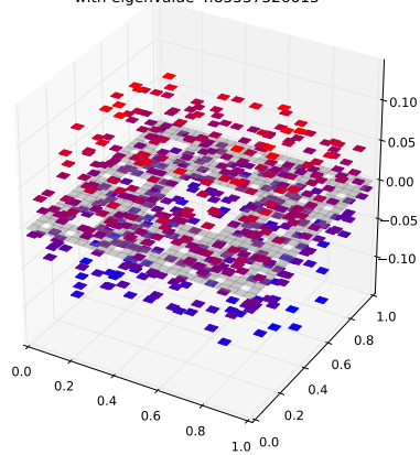
Klein Bottle Horizontal Glued Eigenfunction 328 with eigenvalue 4.85537326613
