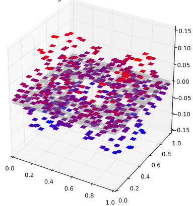
Klein Bottle Horizontal Glued Eigenfunction 77 with eigenvalue 1.74392114232
