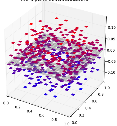
Klein Bottle Horizontal Glued Eigenfunction 379 with eigenvalue 5.38653120871
