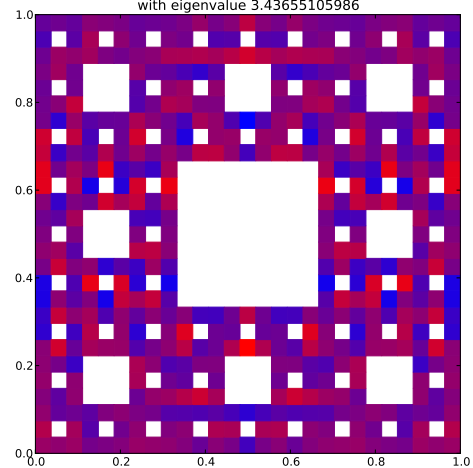
Klein Bottle Horizontal Glued Eigenfunction 218 with eigenvalue 3.43655105986
