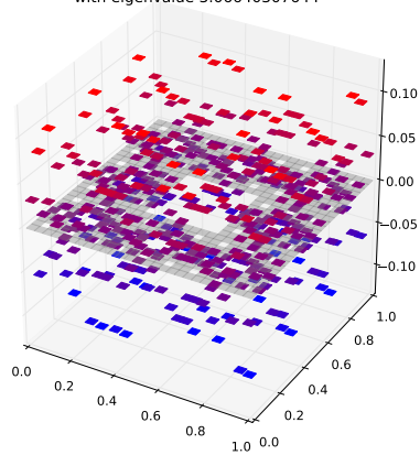
Klein Bottle Horizontal Glued Eigenfunction 172 with eigenvalue 3.06640307644
