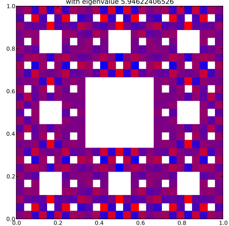
Klein Bottle Horizontal Glued Eigenfunction 406 with eigenvalue 5.94622406526
