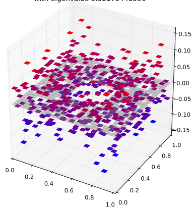
Klein Bottle Horizontal Glued Eigenfunction 201 with eigenvalue 3.32173448596
