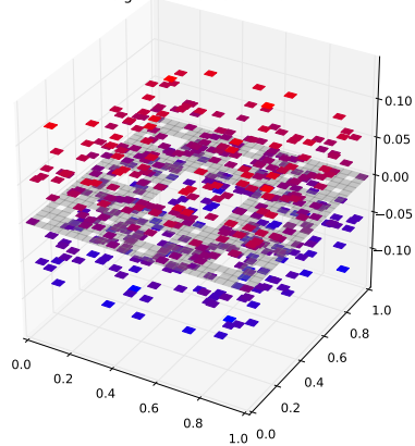
Klein Bottle Horizontal Glued Eigenfunction 211 with eigenvalue 3.38632743125
