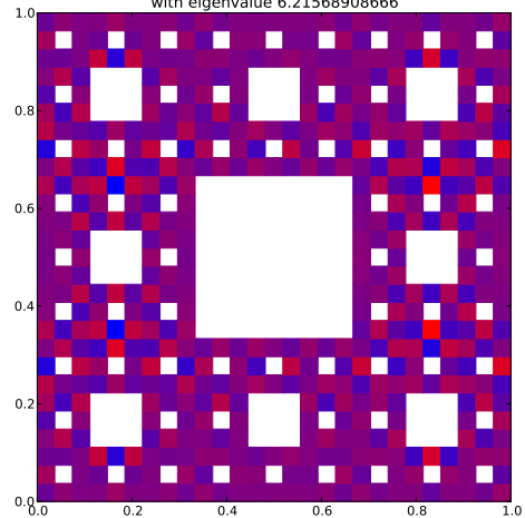
Klein Bottle Horizontal Glued Eigenfunction 421 with eigenvalue 6.2156890866
