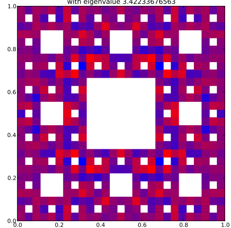
Klein Bottle Horizontal Glued Eigenfunction 214 with eigenvalue 3.42233676563
