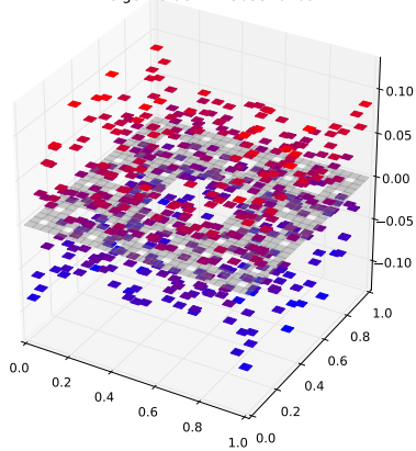
Klein Bottle Horizontal Glued Eigenfunction 288 with eigenvalue 4.41365370209
