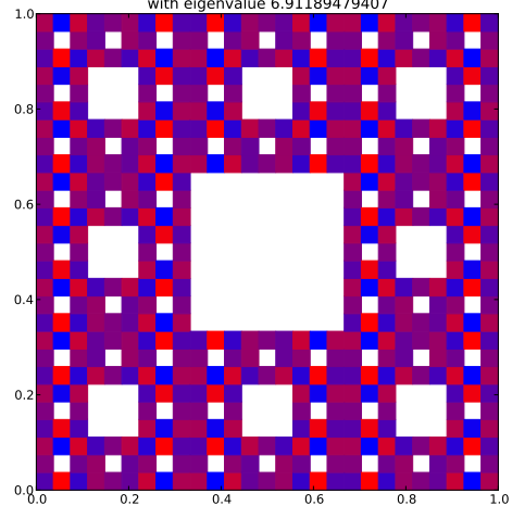
Klein Bottle Horizontal Glued Eigenfunction 452 with eigenvalue 6.91189479407
