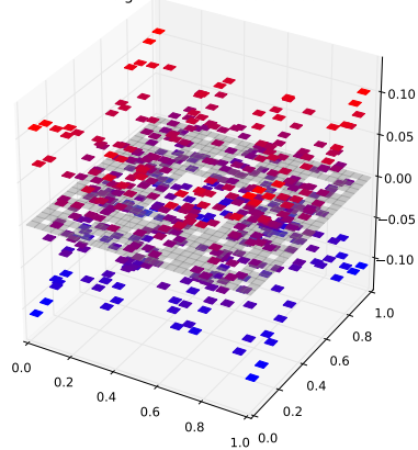
Klein Bottle Horizontal Glued Eigenfunction 393 with eigenvalue 5.67168457166
