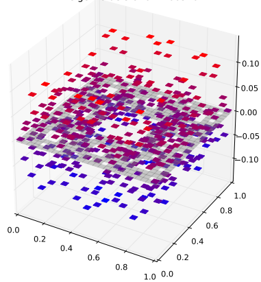
Klein Bottle Horizontal Glued Eigenfunction 406 with eigenvalue 5.94622406526
