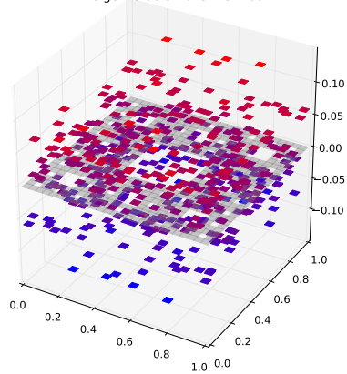
Klein Bottle Horizontal Glued Eigenfunction 380 with eigenvalue 5.46457752268
