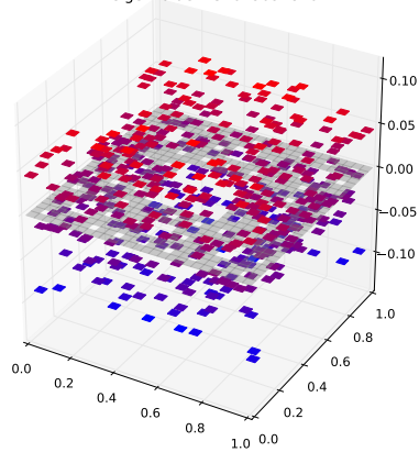
Klein Bottle Horizontal Glued Eigenfunction 282 with eigenvalue 4.32079091826
