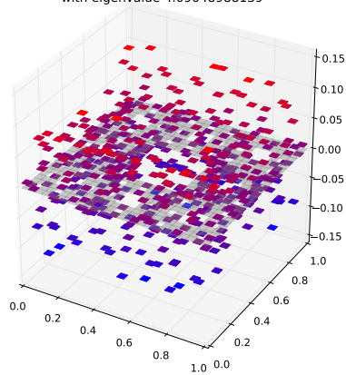
Klein Bottle Horizontal Glued Eigenfunction 268 with eigenvalue 4.09048988139
