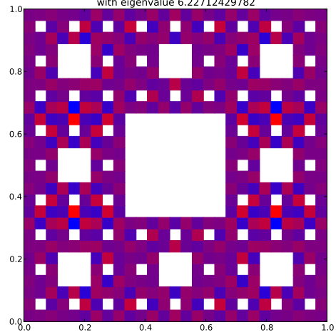
Klein Bottle Horizontal Glued Eigenfunction 422 with eigenvalue 6.22712429782
