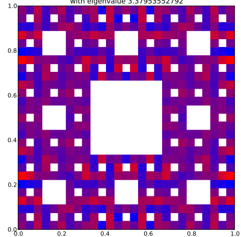
Klein Bottle Horizontal Glued Eigenfunction 209 with eigenvalue 3.37953552792
