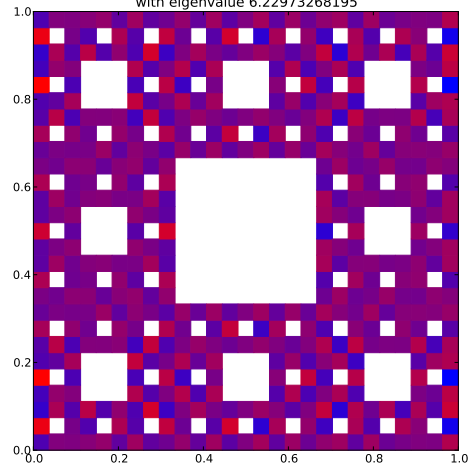
Klein Bottle Horizontal Glued Eigenfunction 423 with eigenvalue 6.22973268195
