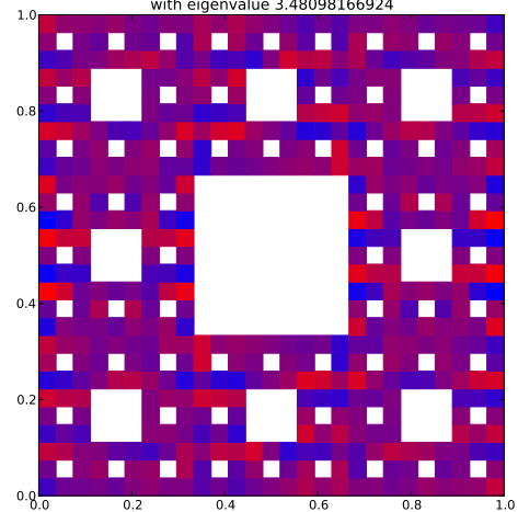
Klein Bottle Horizontal Glued Eigenfunction 219 with eigenvalue 3.48098166924
