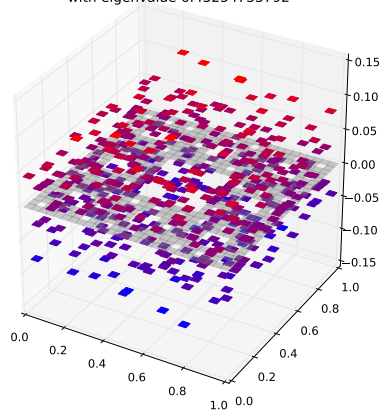
Klein Bottle Horizontal Glued Eigenfunction 431 with eigenvalue 6.43254733792
