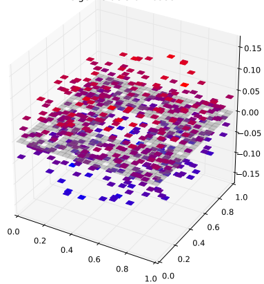
Klein Bottle Horizontal Glued Eigenfunction 350 with eigenvalue 5.0726994221
