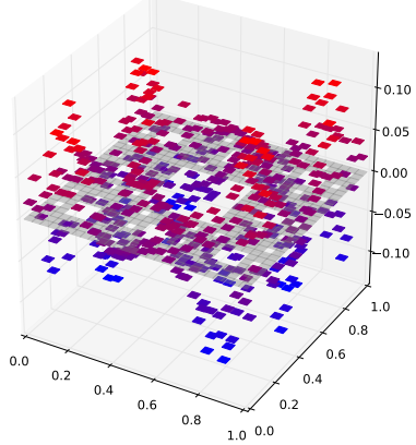
Klein Bottle Horizontal Glued Eigenfunction 39 with eigenvalue 0.983863713371
