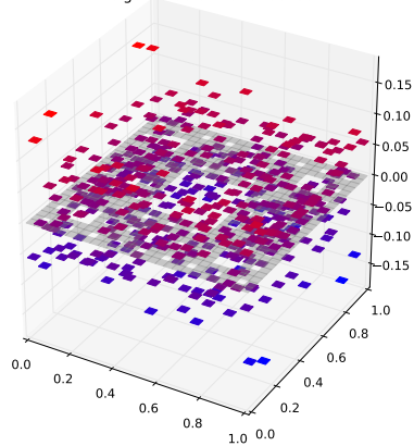
Klein Bottle Horizontal Glued Eigenfunction 423 with eigenvalue 6.22973268195
