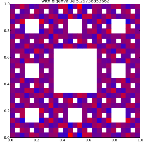
Klein Bottle Horizontal Glued Eigenfunction 372 with eigenvalue 5.29736853662
