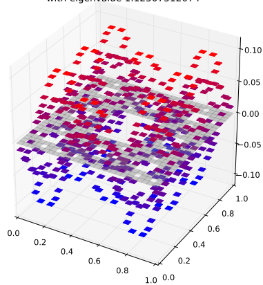
Klein Bottle Horizontal Glued Eigenfunction 43 with eigenvalue 1.12507512074
