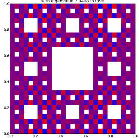
Klein Bottle Horizontal Glued Eigenfunction 504 with eigenvalue 7.3408187396
