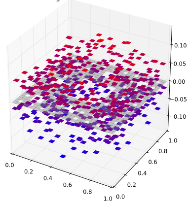
Klein Bottle Horizontal Glued Eigenfunction 283 with eigenvalue 4.34868737275
