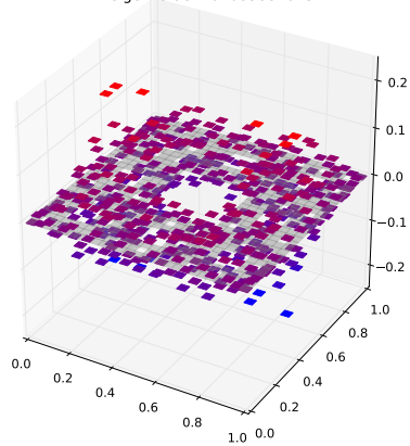
Klein Bottle Horizontal Glued Eigenfunction 462 with eigenvalue 7.07085882043
