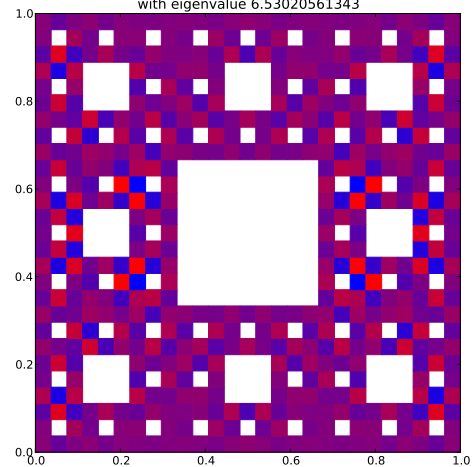
Klein Bottle Horizontal Glued Eigenfunction 437 with eigenvalue 6.53020561343
