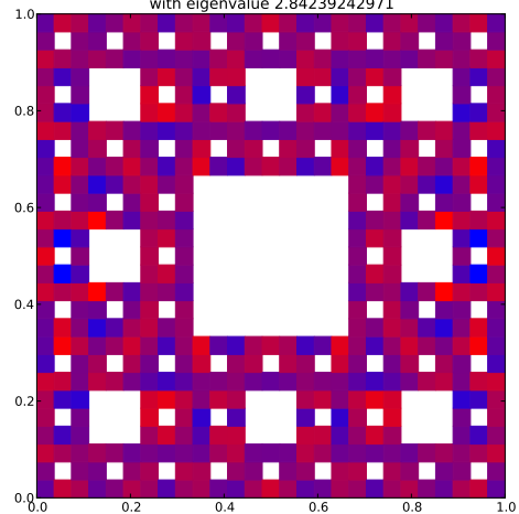
Klein Bottle Horizontal Glued Eigenfunction 148 with eigenvalue 2.84239242971
