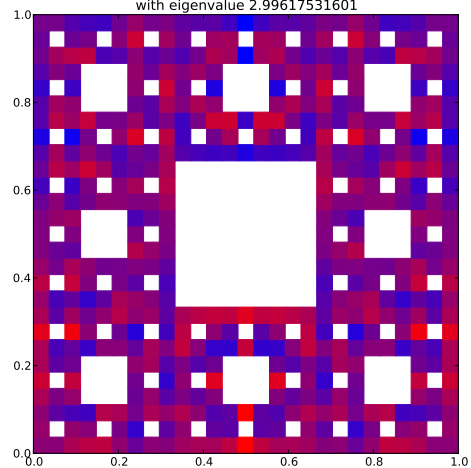
Klein Bottle Horizontal Glued Eigenfunction 164 with eigenvalue 2.99617531601
