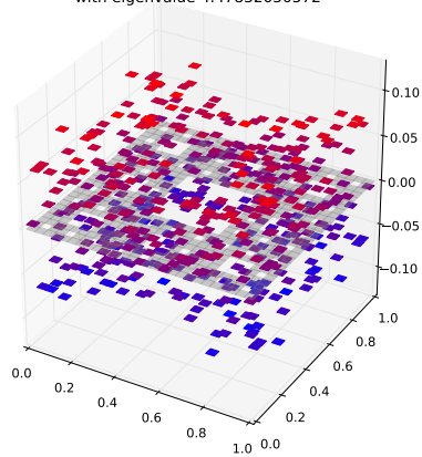
Klein Bottle Horizontal Glued Eigenfunction 296 with eigenvalue 4.47832050572
