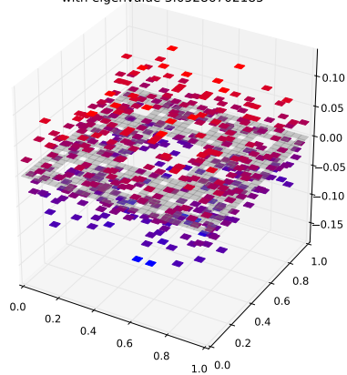
Klein Bottle Horizontal Glued Eigenfunction 171 with eigenvalue 3.05286702185
