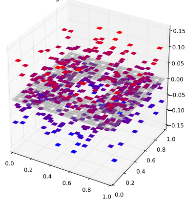
Klein Bottle Horizontal Glued Eigenfunction 215 with eigenvalue 3.42395520327
