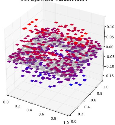
Klein Bottle Horizontal Glued Eigenfunction 270 with eigenvalue 4.13220901594
