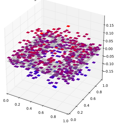
Klein Bottle Horizontal Glued Eigenfunction 229 with eigenvalue 3.58422978366
