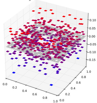
Klein Bottle Horizontal Glued Eigenfunction 223 with eigenvalue 3.51183477532
