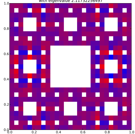
Klein Bottle Horizontal Glued Eigenfunction 111 with eigenvalue 2.11732256497
