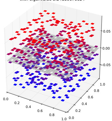
Klein Bottle Horizontal Glued Eigenfunction 365 with eigenvalue 5.24180676624
