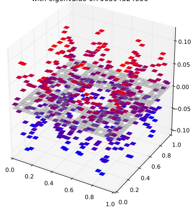
Klein Bottle Horizontal Glued Eigenfunction 26 with eigenvalue 0.706394324056
