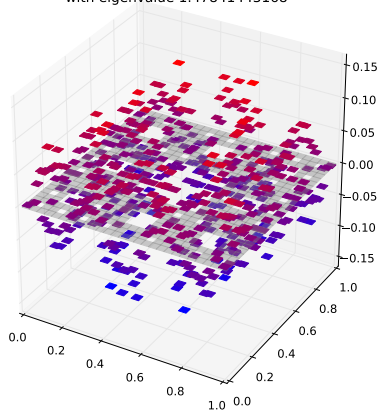
Klein Bottle Horizontal Glued Eigenfunction 58 with eigenvalue 1.47841443168
