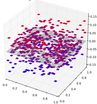
Klein Bottle Horizontal Glued Eigenfunction 187 with eigenvalue 3.21733207124
