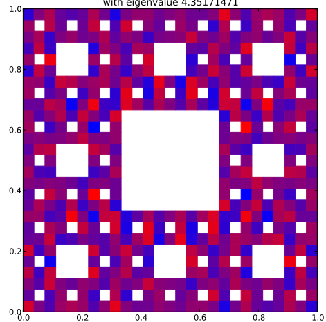
Klein Bottle Horizontal Glued Eigenfunction 284 with eigenvalue 4.35171471
