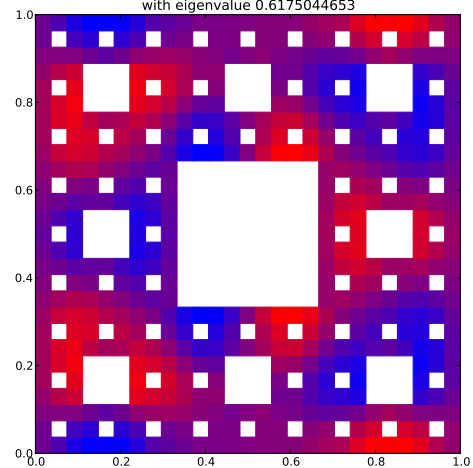
Klein Bottle Horizontal Glued Eigenfunction 20 with eigenvalue 0.6175044653
