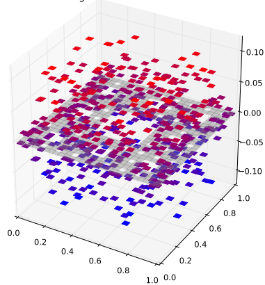
Klein Bottle Horizontal Glued Eigenfunction 383 with eigenvalue 5.52276335632
