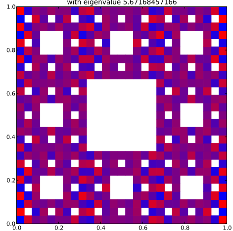
Klein Bottle Horizontal Glued Eigenfunction 393 with eigenvalue 5.67168457166
