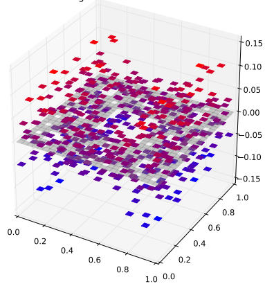
Klein Bottle Horizontal Glued Eigenfunction 335 with eigenvalue 4.92161884099
