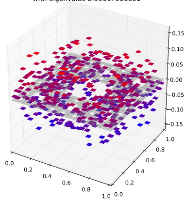
Klein Bottle Horizontal Glued Eigenfunction 164 with eigenvalue 2.99617531601
