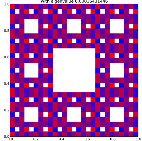
Klein Bottle Horizontal Glued Eigenfunction 409 with eigenvalue 6.00016431446
