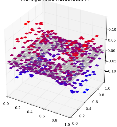
Klein Bottle Horizontal Glued Eigenfunction 476 with eigenvalue 7.19187555644
