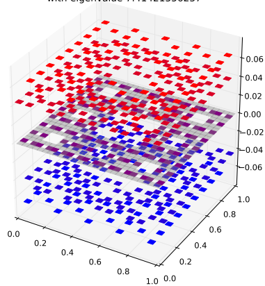
Klein Bottle Horizontal Glued Eigenfunction 511 with eigenvalue 7.41421356237
