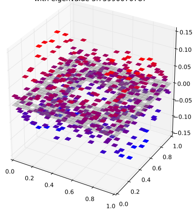
Klein Bottle Horizontal Glued Eigenfunction 248 with eigenvalue 3.75990070787
