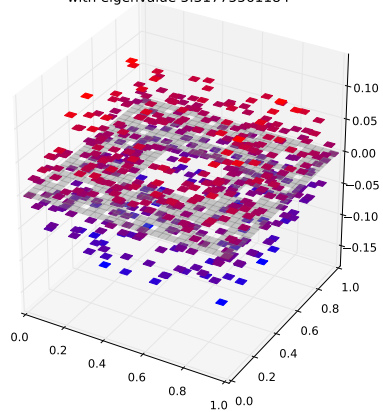
Klein Bottle Horizontal Glued Eigenfunction 375 with eigenvalue 5.31775561184
