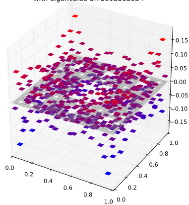
Klein Bottle Horizontal Glued Eigenfunction 251 with eigenvalue 3.78993365934
