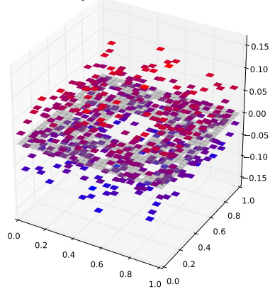
Klein Bottle Horizontal Glued Eigenfunction 455 with eigenvalue 6.98331017245
