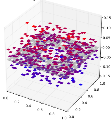
Klein Bottle Horizontal Glued Eigenfunction 337 with eigenvalue 4.96267288307
