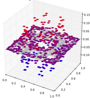
Klein Bottle Horizontal Glued Eigenfunction 493 with eigenvalue 7.269557156
