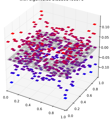
Klein Bottle Horizontal Glued Eigenfunction 377 with eigenvalue 5.35398400376
