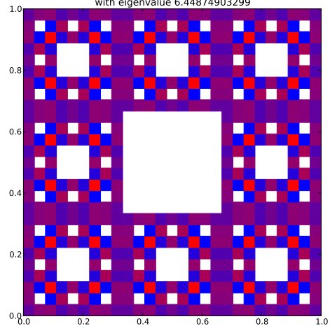
Klein Bottle Horizontal Glued Eigenfunction 432 with eigenvalue 6.44874903299
