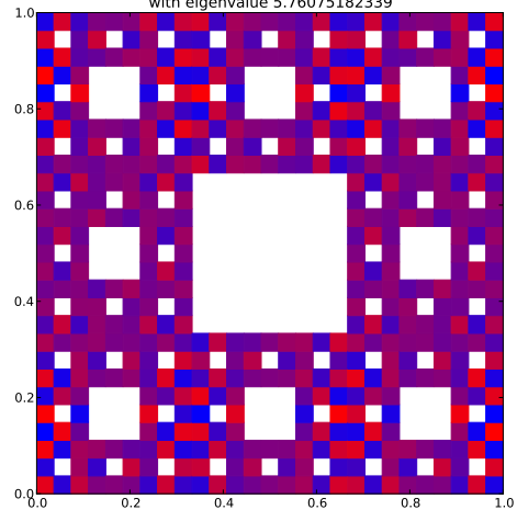
Klein Bottle Horizontal Glued Eigenfunction 399 with eigenvalue 5.76075182339
