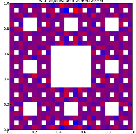
Klein Bottle Horizontal Glued Eigenfunction 367 with eigenvalue 5.24909229705
