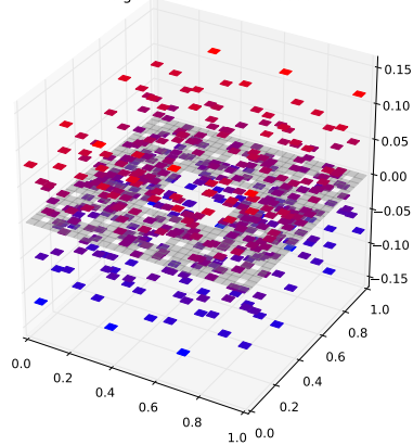
Klein Bottle Horizontal Glued Eigenfunction 417 with eigenvalue 6.11412133859
