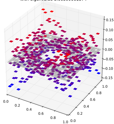
Klein Bottle Horizontal Glued Eigenfunction 165 with eigenvalue 3.00599061374
