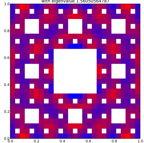
Klein Bottle Horizontal Glued Eigenfunction 66 with eigenvalue 1.56050564787
