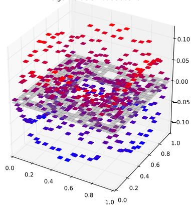
Klein Bottle Horizontal Glued Eigenfunction 394 with eigenvalue 5.70995665292
