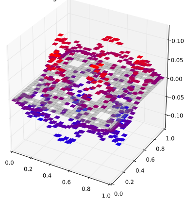
Klein Bottle Horizontal Glued Eigenfunction 21 with eigenvalue 0.636029470348
