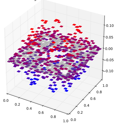
Klein Bottle Horizontal Glued Eigenfunction 481 with eigenvalue 7.21192826379
