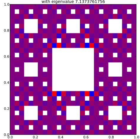
Klein Bottle Horizontal Glued Eigenfunction 470 with eigenvalue 7.1373761756
