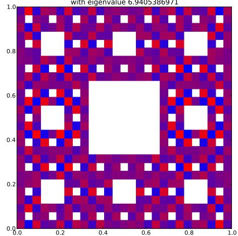
Klein Bottle Horizontal Glued Eigenfunction 453 with eigenvalue 6.9405386971
