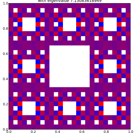
Klein Bottle Horizontal Glued Eigenfunction 469 with eigenvalue 7.13083618949
