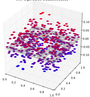
Klein Bottle Horizontal Glued Eigenfunction 225 with eigenvalue 3.52256951635
