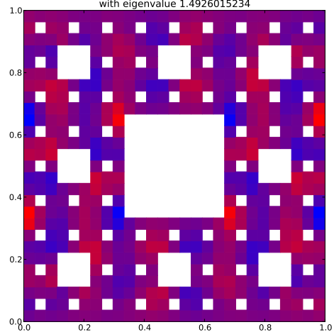
Klein Bottle Horizontal Glued Eigenfunction 60 with eigenvalue 1.4926015234
