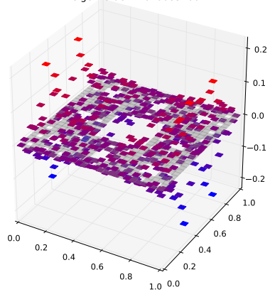
Klein Bottle Horizontal Glued Eigenfunction 492 with eigenvalue 7.26206831667
