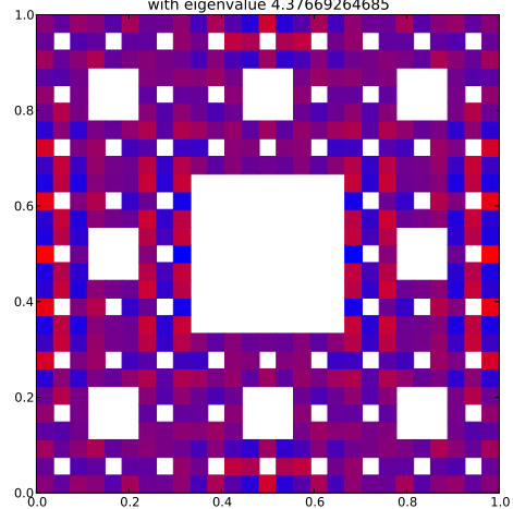
Klein Bottle Horizontal Glued Eigenfunction 285 with eigenvalue 4.37669264685
