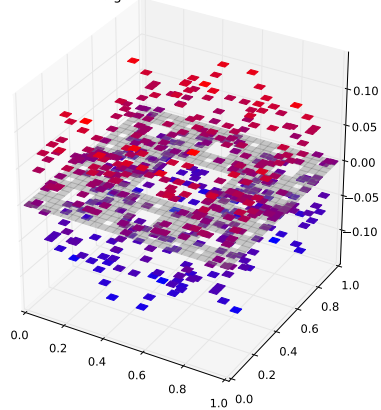
Klein Bottle Horizontal Glued Eigenfunction 197 with eigenvalue 3.29674107773
