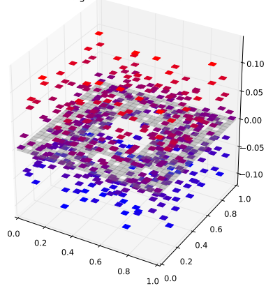
Klein Bottle Horizontal Glued Eigenfunction 403 with eigenvalue 5.92958265775
