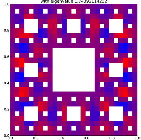
Klein Bottle Horizontal Glued Eigenfunction 77 with eigenvalue 1.74392114232
