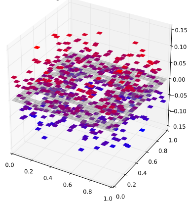
Klein Bottle Horizontal Glued Eigenfunction 307 with eigenvalue 4.59890480479
