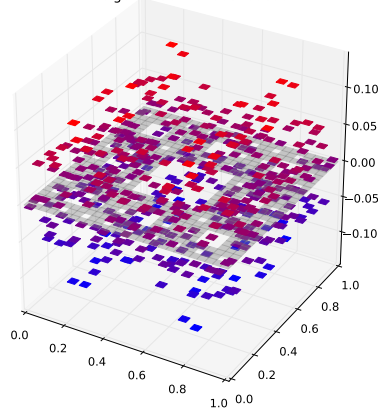
Klein Bottle Horizontal Glued Eigenfunction 463 with eigenvalue 7.07680409699
