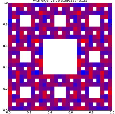
Klein Bottle Horizontal Glued Eigenfunction 211 with eigenvalue 3.38632743125
