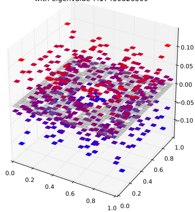
Klein Bottle Horizontal Glued Eigenfunction 474 with eigenvalue 7.17430826509
