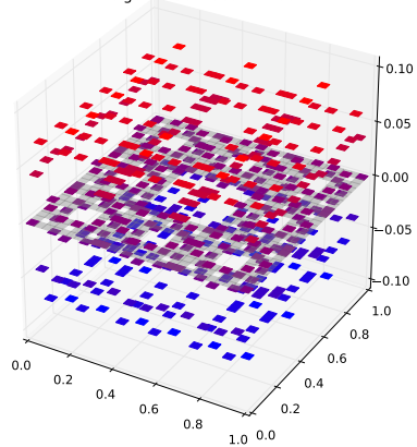
Klein Bottle Horizontal Glued Eigenfunction 67 with eigenvalue 1.56922273818
