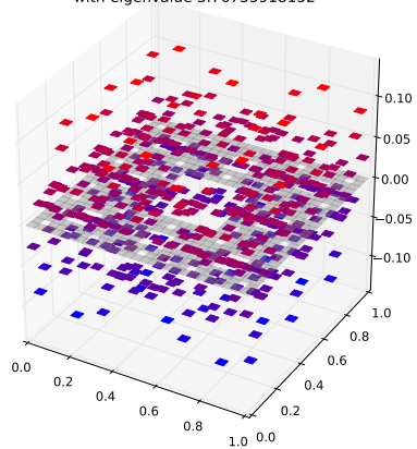
Klein Bottle Horizontal Glued Eigenfunction 249 with eigenvalue 3.76733918152
