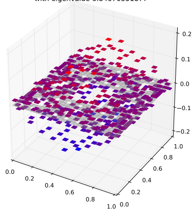
Klein Bottle Horizontal Glued Eigenfunction 449 with eigenvalue 6.84070551877
