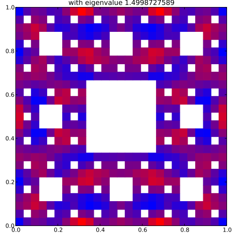
Klein Bottle Horizontal Glued Eigenfunction 62 with eigenvalue 1.4998727589
