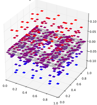
Klein Bottle Horizontal Glued Eigenfunction 345 with eigenvalue 5.02616265324
