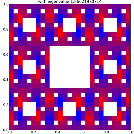
Klein Bottle Horizontal Glued Eigenfunction 82 with eigenvalue 1.86621970714
