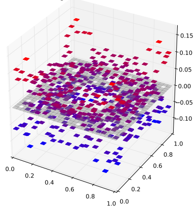
Klein Bottle Horizontal Glued Eigenfunction 343 with eigenvalue 4.9982907522
