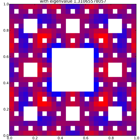
Klein Bottle Horizontal Glued Eigenfunction 53 with eigenvalue 1.31065578057
