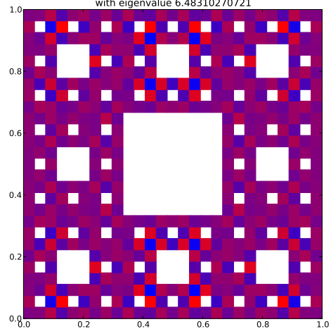
Klein Bottle Horizontal Glued Eigenfunction 433 with eigenvalue 6.48310270721
