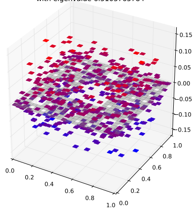
Klein Bottle Horizontal Glued Eigenfunction 436 with eigenvalue 6.5103765784
