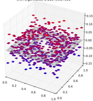
Klein Bottle Horizontal Glued Eigenfunction 354 with eigenvalue 5.11349017955
