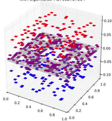
Klein Bottle Horizontal Glued Eigenfunction 495 with eigenvalue 7.27082737554
