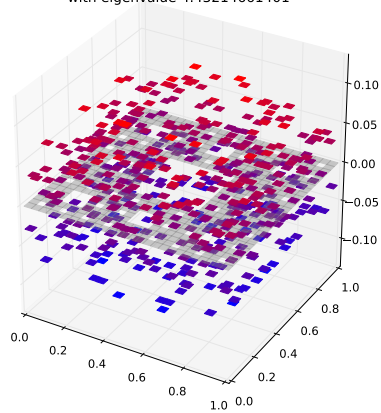
Klein Bottle Horizontal Glued Eigenfunction 290 with eigenvalue 4.43214661401
