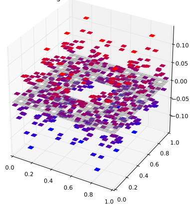
Klein Bottle Horizontal Glued Eigenfunction 181 with eigenvalue 3.16946673704
