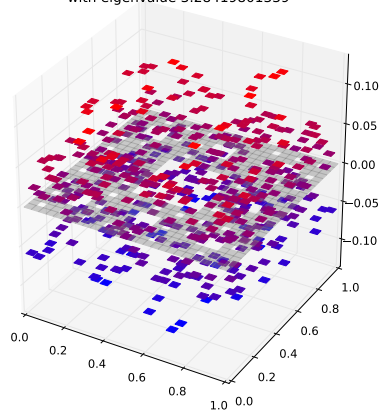
Klein Bottle Horizontal Glued Eigenfunction 196 with eigenvalue 3.28419801339
