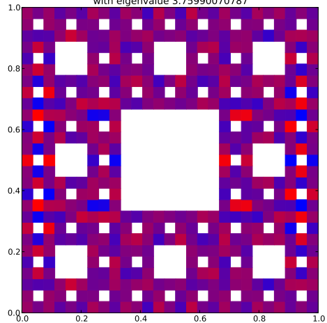
Klein Bottle Horizontal Glued Eigenfunction 248 with eigenvalue 3.75990070787
