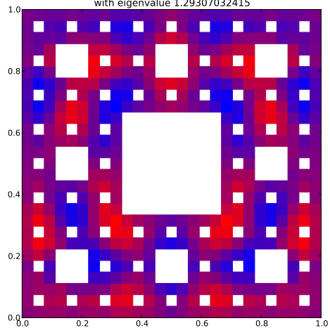
Klein Bottle Horizontal Glued Eigenfunction 51 with eigenvalue 1.29307032415
