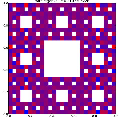
Klein Bottle Horizontal Glued Eigenfunction 420 with eigenvalue 6.2107305226
