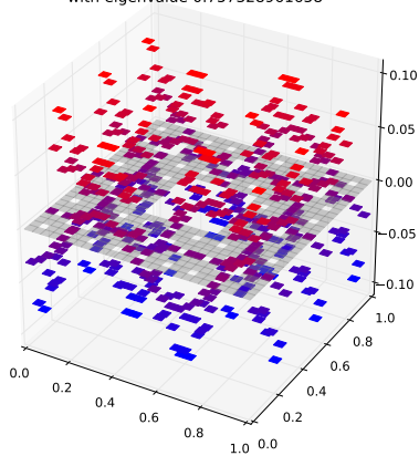
Klein Bottle Horizontal Glued Eigenfunction 29 with eigenvalue 0.757328961658
