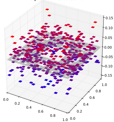
Klein Bottle Horizontal Glued Eigenfunction 66 with eigenvalue 1.56050564787
