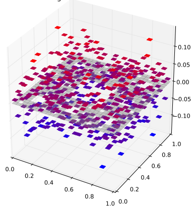
Klein Bottle Horizontal Glued Eigenfunction 317 with eigenvalue 4.71631227434
