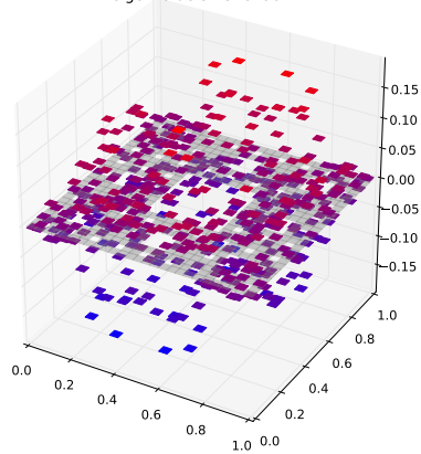
Klein Bottle Horizontal Glued Eigenfunction 180 with eigenvalue 3.15481987174
