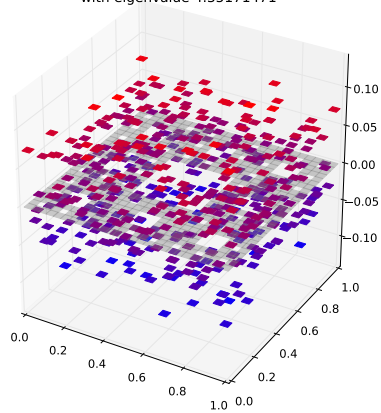
Klein Bottle Horizontal Glued Eigenfunction 284 with eigenvalue 4.35171471
