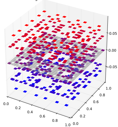
Klein Bottle Horizontal Glued Eigenfunction 407 with eigenvalue 5.94691370594
