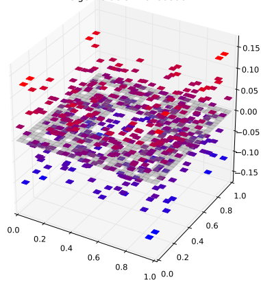
Klein Bottle Horizontal Glued Eigenfunction 186 with eigenvalue 3.21323959822
