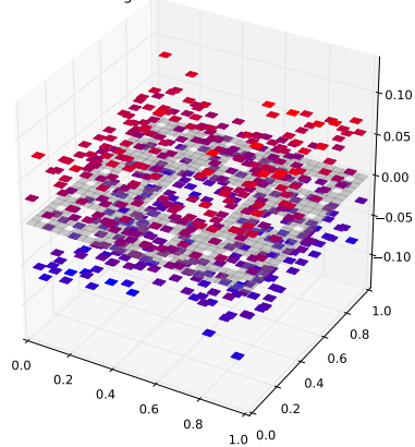
Klein Bottle Horizontal Glued Eigenfunction 183 with eigenvalue 3.19715619694
