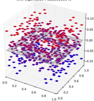
Klein Bottle Horizontal Glued Eigenfunction 503 with eigenvalue 7.32263103949
