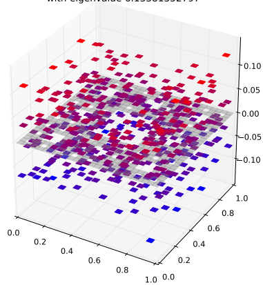
Klein Bottle Horizontal Glued Eigenfunction 418 with eigenvalue 6.13381352797
