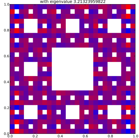
Klein Bottle Horizontal Glued Eigenfunction 186 with eigenvalue 3.21323959822
