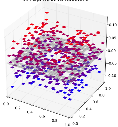
Klein Bottle Horizontal Glued Eigenfunction 453 with eigenvalue 6.9405386971
