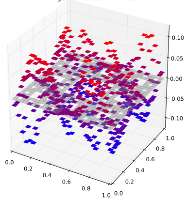
Klein Bottle Horizontal Glued Eigenfunction 20 with eigenvalue 0.6175044653
