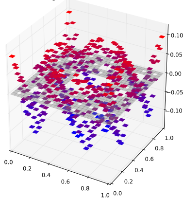
Klein Bottle Horizontal Glued Eigenfunction 18 with eigenvalue 0.542930732843
