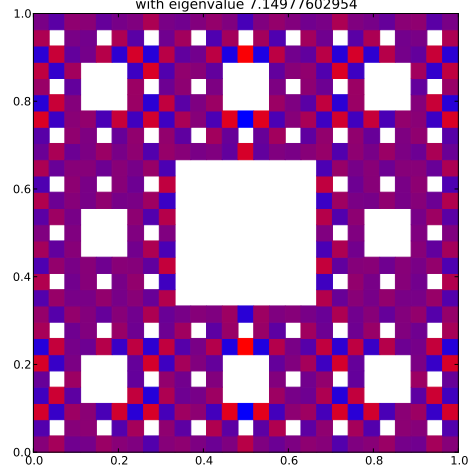
Klein Bottle Horizontal Glued Eigenfunction 471 with eigenvalue 7.14977602954
