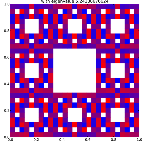
Klein Bottle Horizontal Glued Eigenfunction 365 with eigenvalue 5.24180676624
