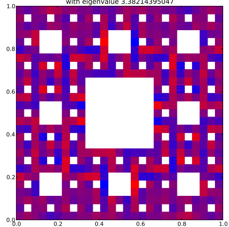
Klein Bottle Horizontal Glued Eigenfunction 210 with eigenvalue 3.38214395047
