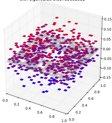
Klein Bottle Horizontal Glued Eigenfunction 254 with eigenvalue 3.83783602582
