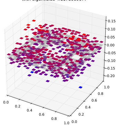
Klein Bottle Horizontal Glued Eigenfunction 269 with eigenvalue 4.1178069677
