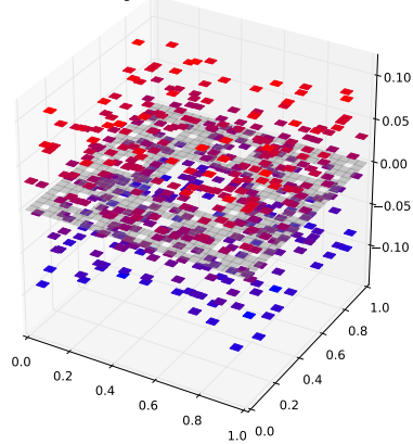
Klein Bottle Horizontal Glued Eigenfunction 342 with eigenvalue 4.98624177107
