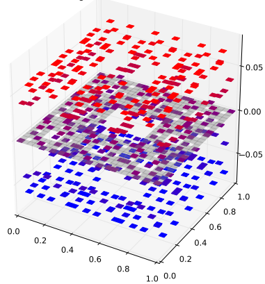
Klein Bottle Horizontal Glued Eigenfunction 190 with eigenvalue 3.23477240994
