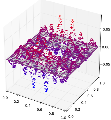
Eigenfunction with eigenvalue 0.433770296824
