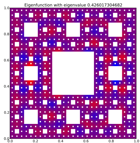
Eigenfunction 95 with eigenvalue 0.426017304682
