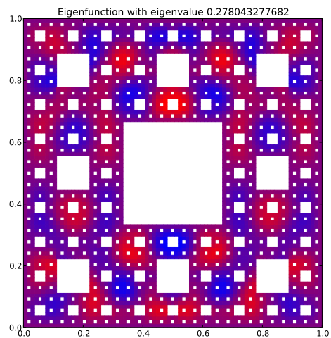
Eigenfunction 55 with eigenvalue 0.278043277682
