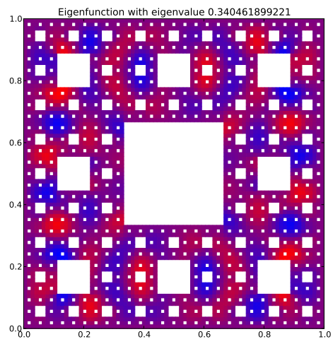
Eigenfunction 71 with eigenvalue 0.340461899221
