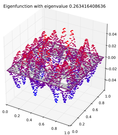
Eigenfunction 51 with eigenvalue 0.263416408636
