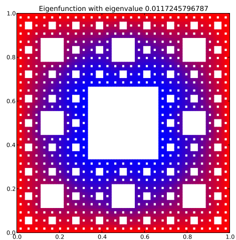
Eigenfunction 0 with eigenvalue 0.0117245796787
