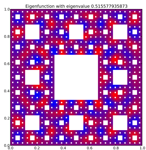
Eigenfunction 122 with eigenvalue 0.515577935873
