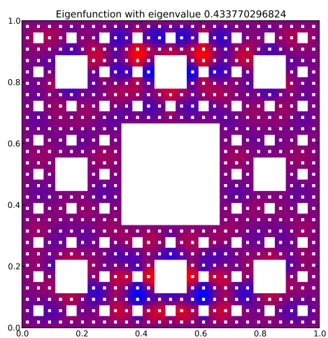
Eigenfunction 98 with eigenvalue 0.433770296824
