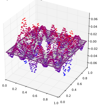
Eigenfunction with eigenvalue 0.385247579469
