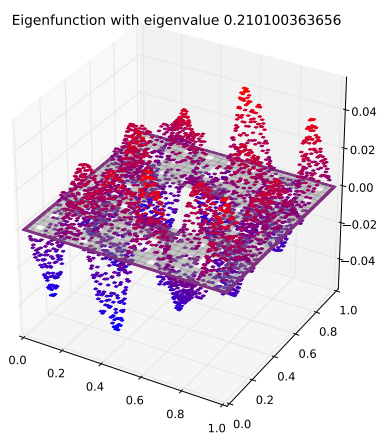
Eigenfunction 41 with eigenvalue 0.210100363656
