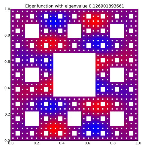
Eigenfunction 20 with eigenvalue 0.126901893661
