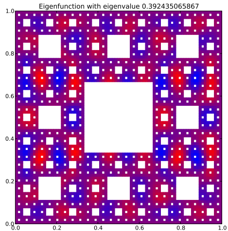
Eigenfunction with eigenvalue 0.392435065867
