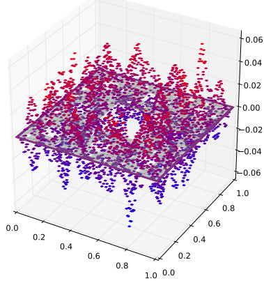
Eigenfunction with eigenvalue 0.545990782068
