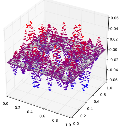
Eigenfunction with eigenvalue 0.43414160355
