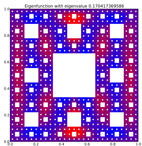
Eigenfunction 30 with eigenvalue 0.170417369586
