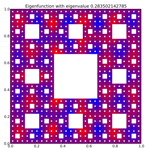
Eigenfunction 56 with eigenvalue 0.283502142785
