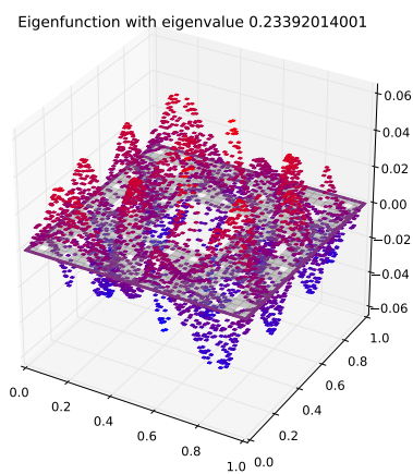
Eigenfunction 47 with eigenvalue 0.23392014001
