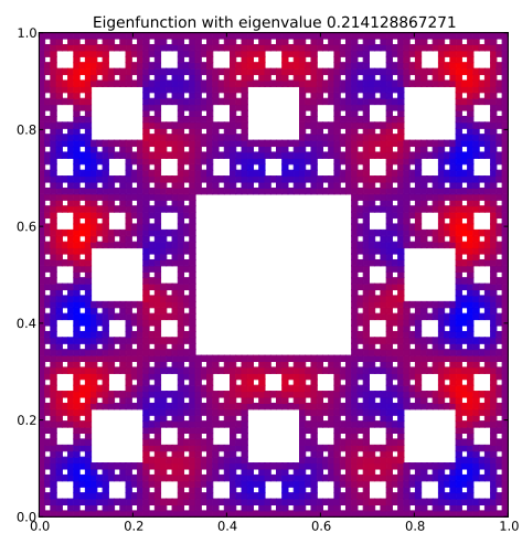
Eigenfunction 42 with eigenvalue 0.214128867271
