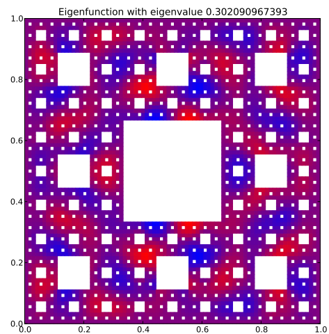
Eigenfunction 61 with eigenvalue 0.302090967393
