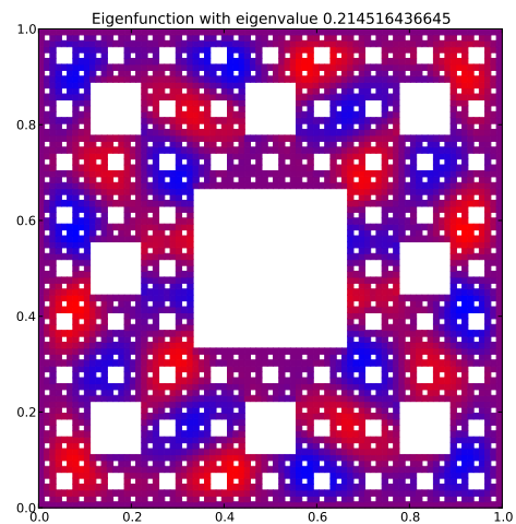
Eigenfunction 43 with eigenvalue 0.214516436645
