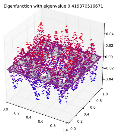
Eigenfunction 93 with eigenvalue 0.419370516671
