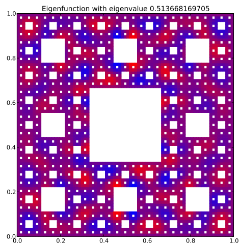
Eigenfunction 121 with eigenvalue 0.513668169705
