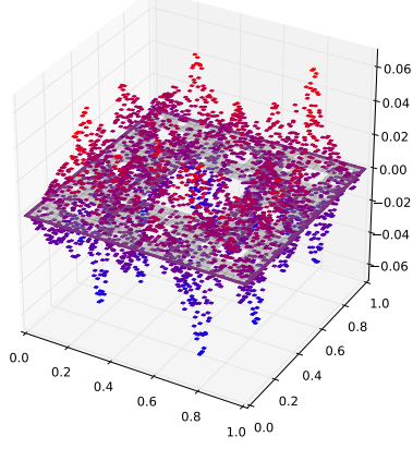
Eigenfunction with eigenvalue 0.440370526421
