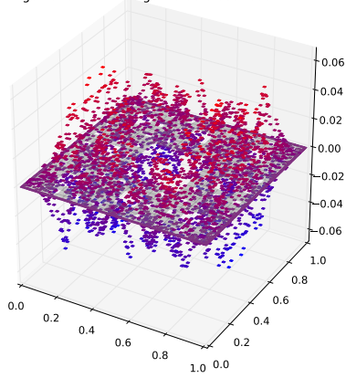
Eigenfunction with eigenvalue 0.609483014107
