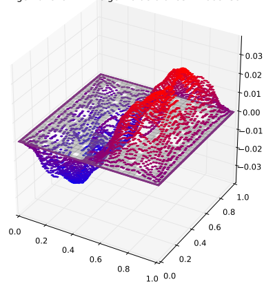
Eigenfunction with eigenvalue 0.0283122068459
