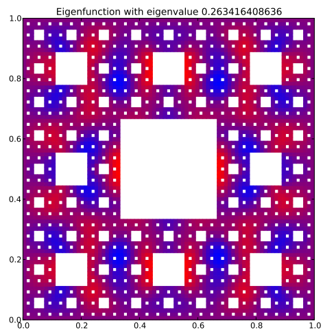
Eigenfunction 51 with eigenvalue 0.263416408636
