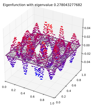
Eigenfunction 55 with eigenvalue 0.278043277682
