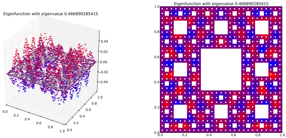
Eigenfunction 111 with eigenvalue 0.466890285415
