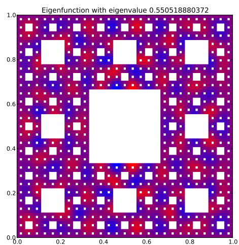
Eigenfunction 132 with eigenvalue 0.550518880372
