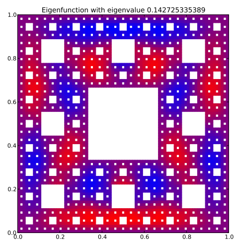
Eigenfunction 24 with eigenvalue 0.142725335389
