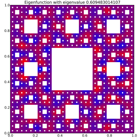
Eigenfunction with eigenvalue 0.609483014107
