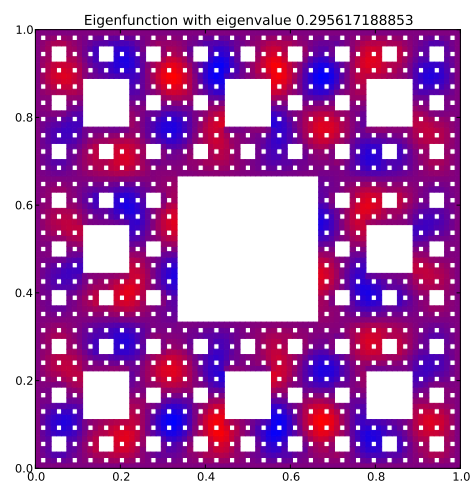
Eigenfunction 60 with eigenvalue 0.295617188853
