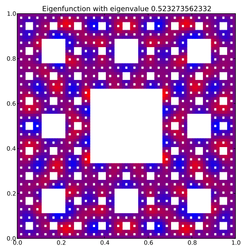
Eigenfunction 123 with eigenvalue 0.523273562332
