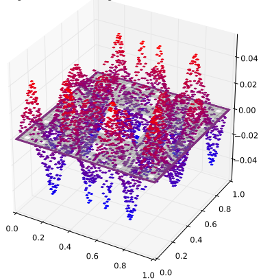
Eigenfunction with eigenvalue 0.253000733772
