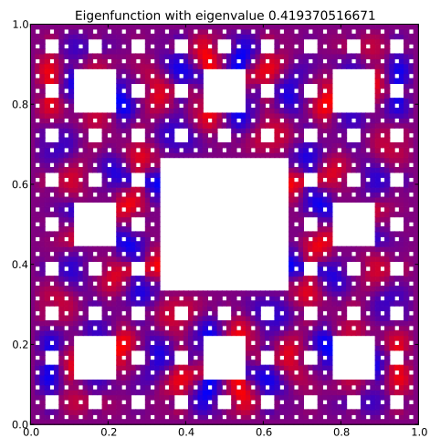
Eigenfunction 93 with eigenvalue 0.419370516671
