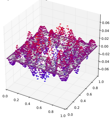
Eigenfunction with eigenvalue 0.428148986196
