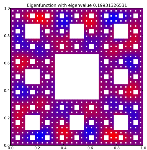
Eigenfunction 37 with eigenvalue 0.19931326531
