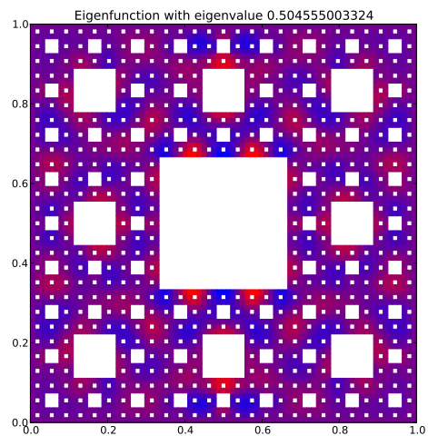
Eigenfunction 119 with eigenvalue 0.504555003324
