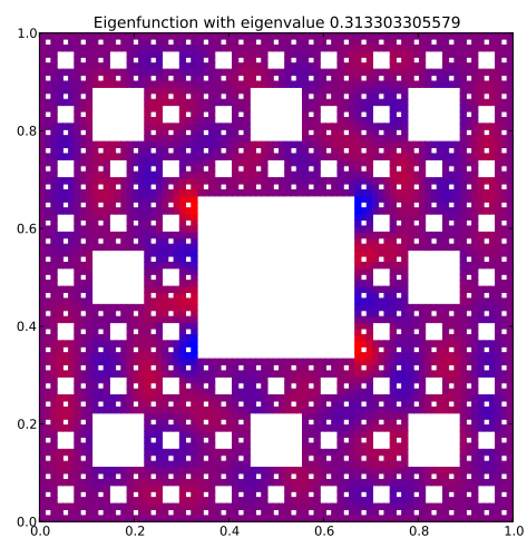
Eigenfunction 64 with eigenvalue 0.313303305579
