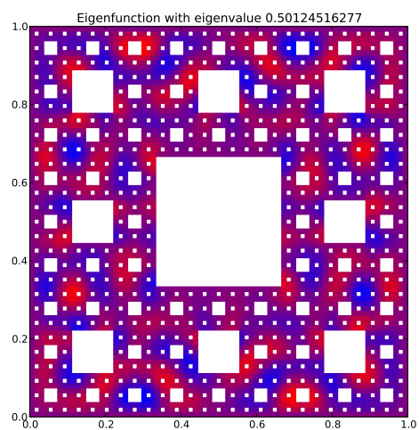
Eigenfunction 118 with eigenvalue 0.50124516277
