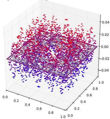
Eigenfunction with eigenvalue 0.585684424634
