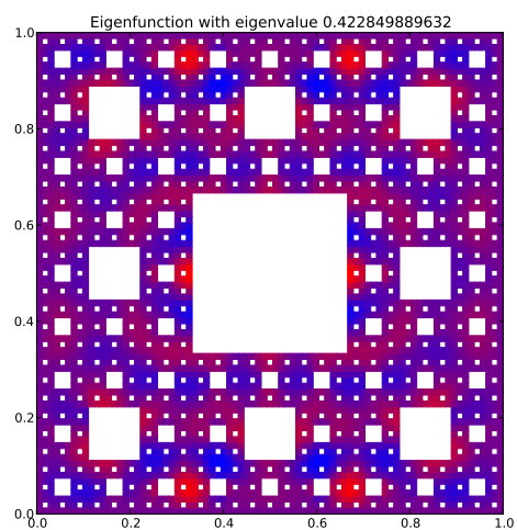
Eigenfunction 94 with eigenvalue 0.422849889632
