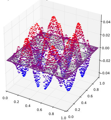
Eigenfunction with eigenvalue 0.140714665001
