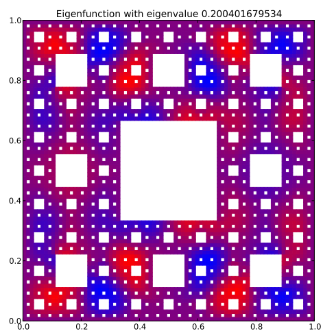
Eigenfunction 38 with eigenvalue 0.200401679534
