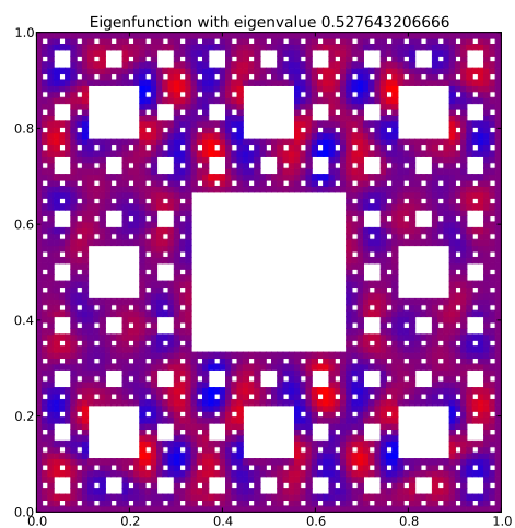
Eigenfunction 126 with eigenvalue 0.52764320666
