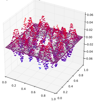
Eigenfunction with eigenvalue 0.405565252909
