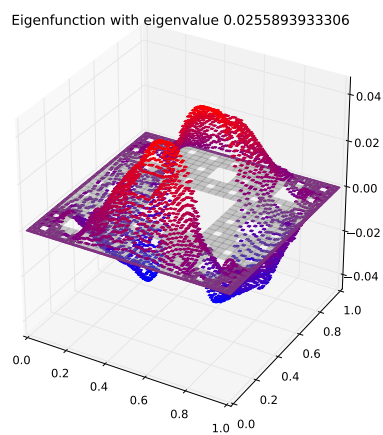
Eigenfunction 1 with eigenvalue 0.0255893933306
