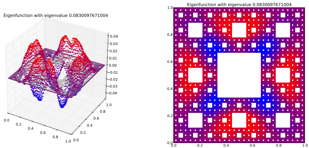
Eigenfunction 11 with eigenvalue 0.0830097671004
