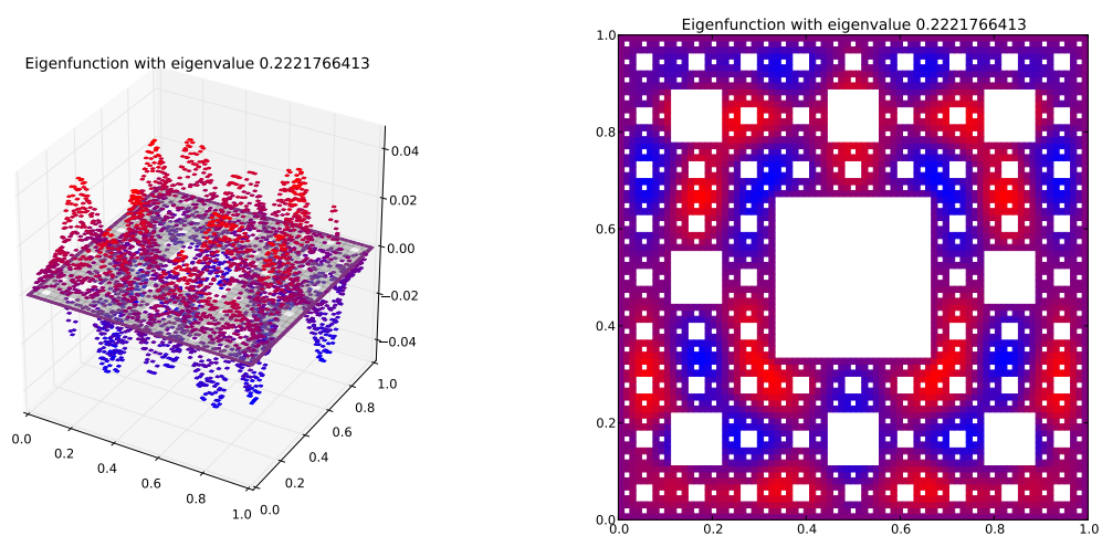
Eigenfunction 44 with eigenvalue 0.2221766413
