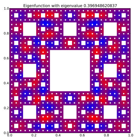
Eigenfunction 86 with eigenvalue 0.396948620837
