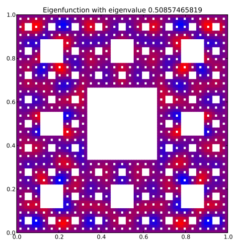
Eigenfunction 120 with eigenvalue 0.50857465819
