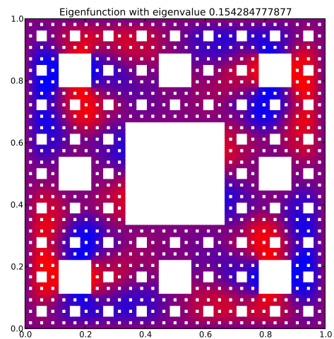
Eigenfunction 25 with eigenvalue 0.154284777877
