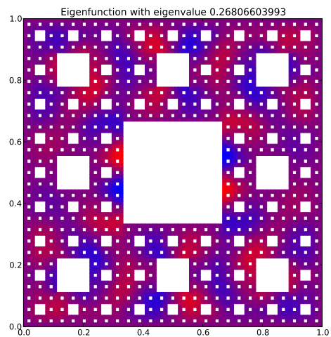
Eigenfunction 53 with eigenvalue 0.26806603993
