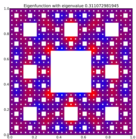
Eigenfunction 62 with eigenvalue 0.311072981945
