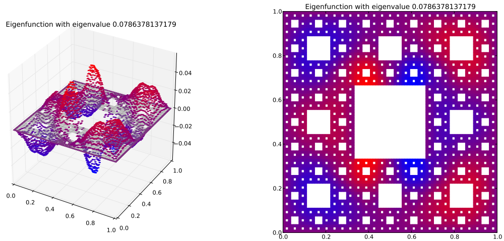
Eigenfunction 10 with eigenvalue 0.0786378137179
