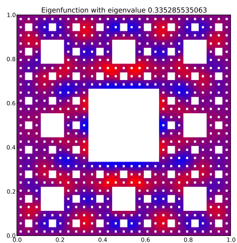
Eigenfunction 70 with eigenvalue 0.335285535063
