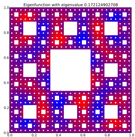
Eigenfunction 31 with eigenvalue 0.172124902708
