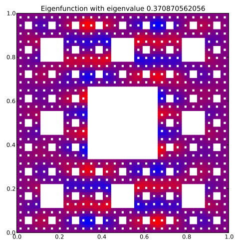
Eigenfunction 79 with eigenvalue 0.370870562056
