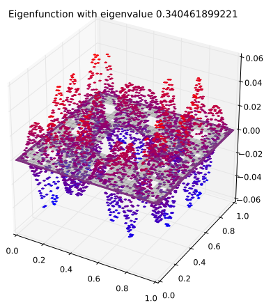
Eigenfunction 71 with eigenvalue 0.340461899221
