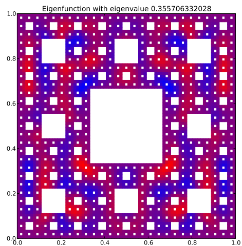
Eigenfunction 75 with eigenvalue 0.355706332028
