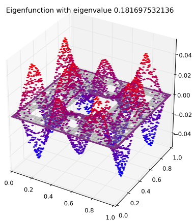
Eigenfunction 35 with eigenvalue 0.181697532136
