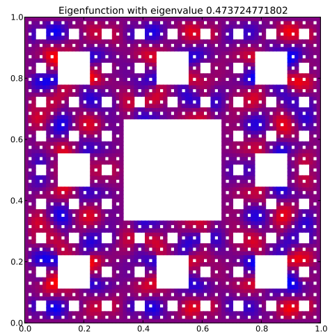
Eigenfunction 113 with eigenvalue 0.473724771802
