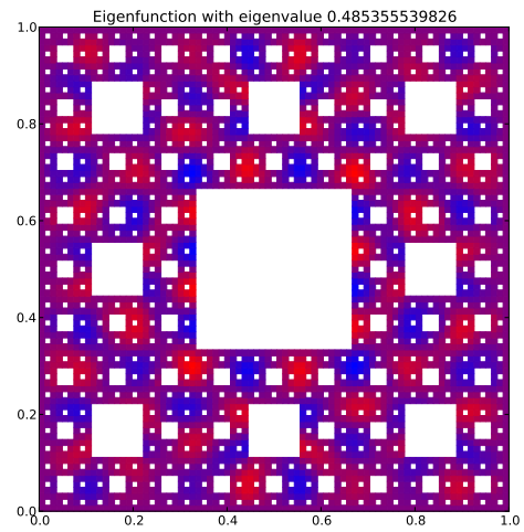
Eigenfunction 115 with eigenvalue 0.485355539826
