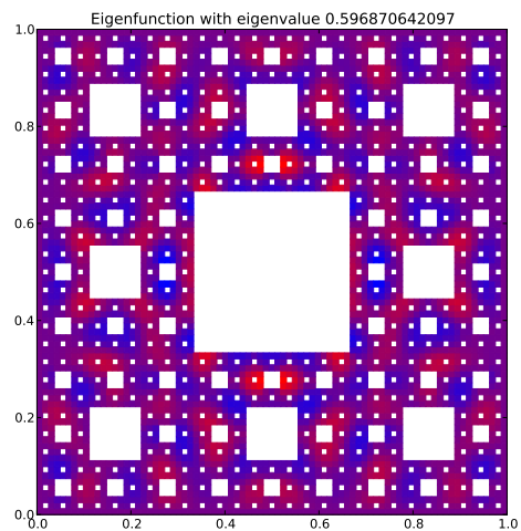
Eigenfunction 141 with eigenvalue 0.596870642097
