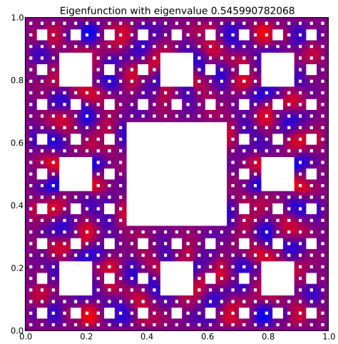
Eigenfunction 131 with eigenvalue 0.545990782068
