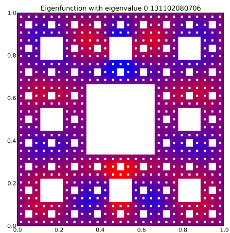
Eigenfunction 21 with eigenvalue 0.131102080706
