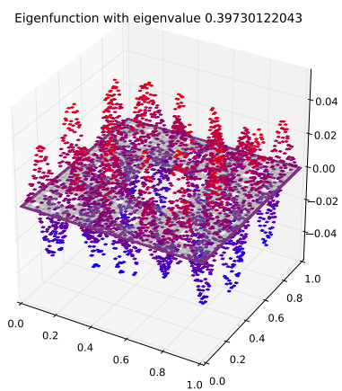
Eigenfunction 87 with eigenvalue 0.39730122043
