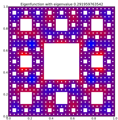
Eigenfunction 59 with eigenvalue 0.291959763542
