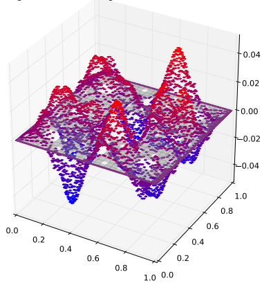
Eigenfunction with eigenvalue 0.099477354286
