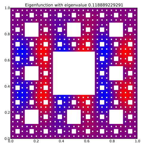
Eigenfunction 17 with eigenvalue 0.118889229291
