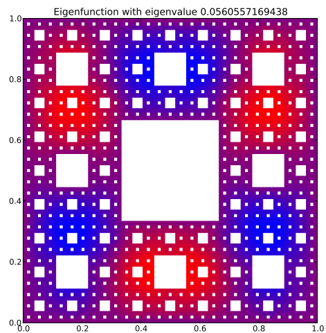
Eigenfunction 7 with eigenvalue 0.0560557169438
