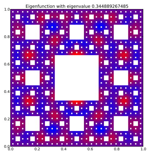
Eigenfunction 72 with eigenvalue 0.344889267485
