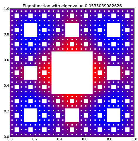
Eigenfunction 6 with eigenvalue 0.0535039982626
