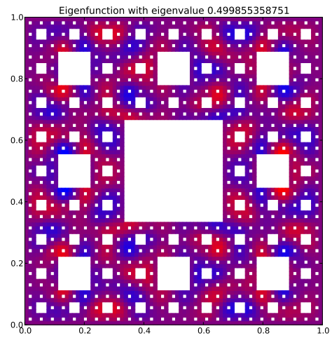
Eigenfunction 117 with eigenvalue 0.499855358751
