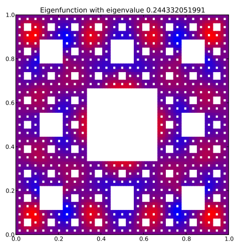
Eigenfunction 48 with eigenvalue 0.244332051991
