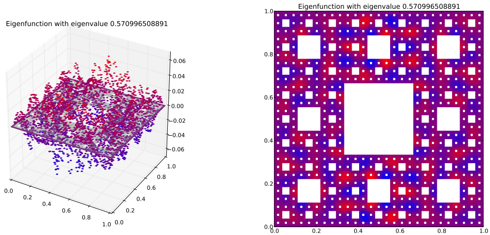
Eigenfunction 134 with eigenvalue 0.570996508891
