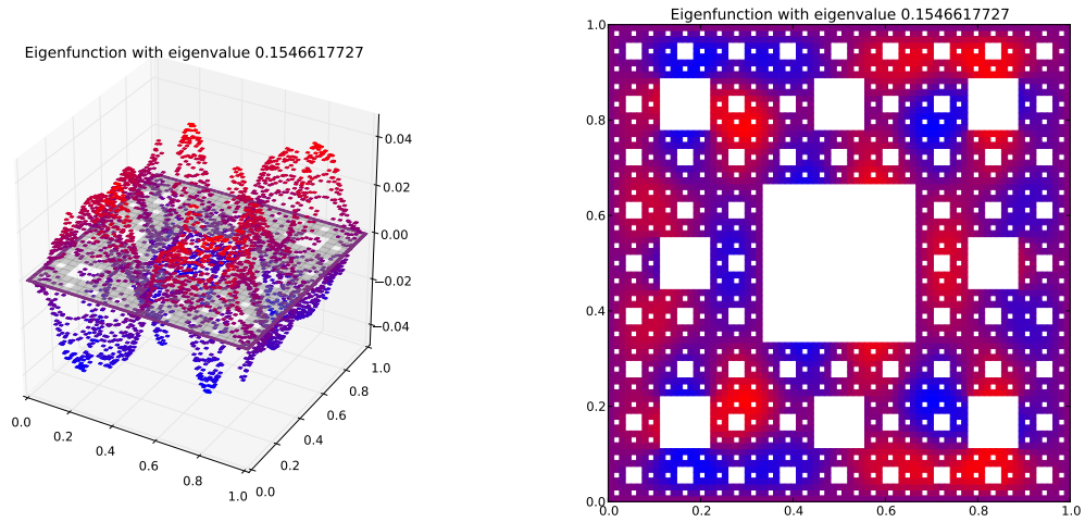
Eigenfunction 26 with eigenvalue 0.1546617727
