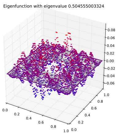
Eigenfunction 119 with eigenvalue 0.504555003324
