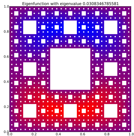
Eigenfunction with eigenvalue 0.0308346785581
