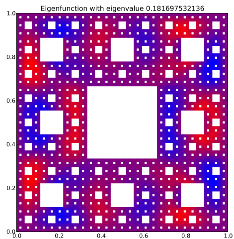
Eigenfunction 35 with eigenvalue 0.181697532136
