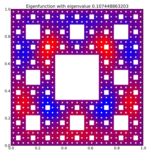
Eigenfunction 16 with eigenvalue 0.107448863203
