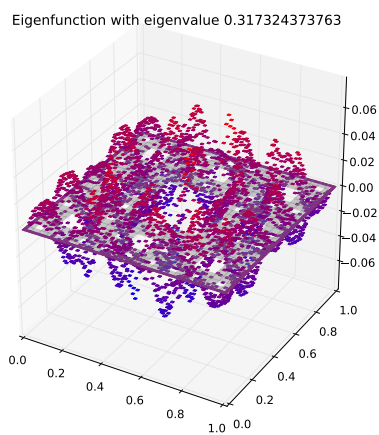
Eigenfunction 65 with eigenvalue 0.317324373763
