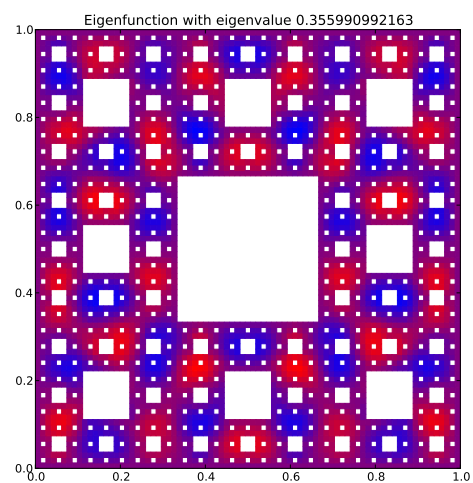
Eigenfunction 76 with eigenvalue 0.355990992163
