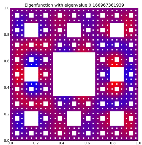
Eigenfunction 29 with eigenvalue 0.166967361939
