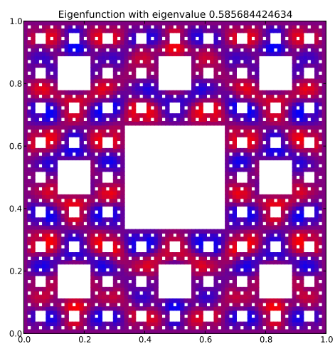
Eigenfunction 138 with eigenvalue 0.585684424634
