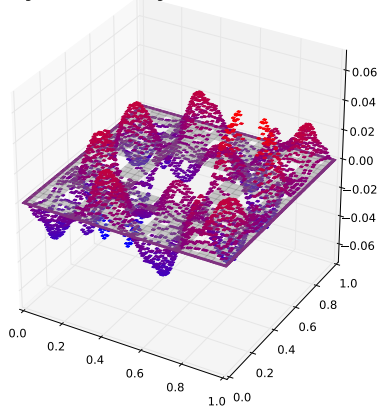
Eigenfunction with eigenvalue 0.132934238075
