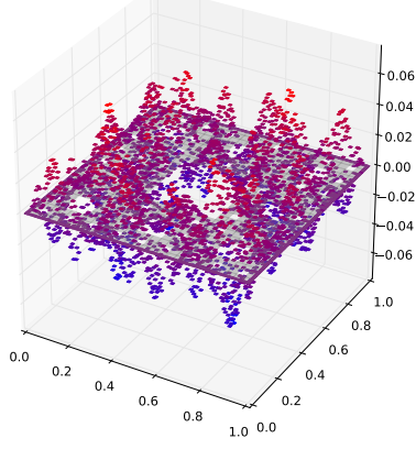
Eigenfunction with eigenvalue 0.445930165834
