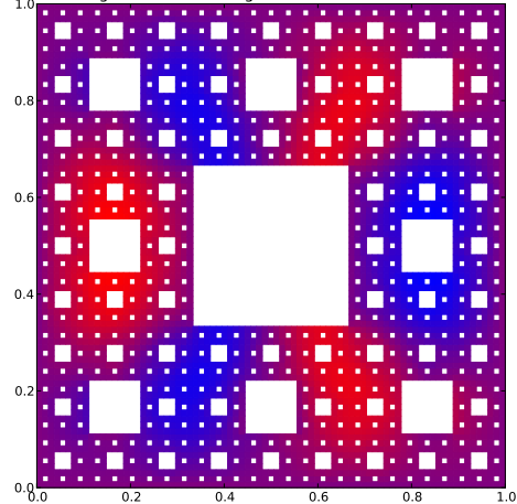
Eigenfunction with eigenvalue 0.0511512200244
