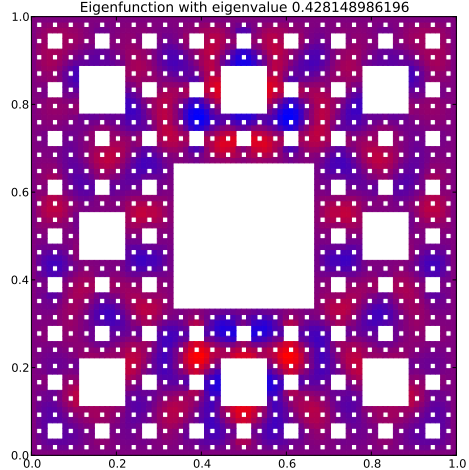
Eigenfunction with eigenvalue 0.428148986196
