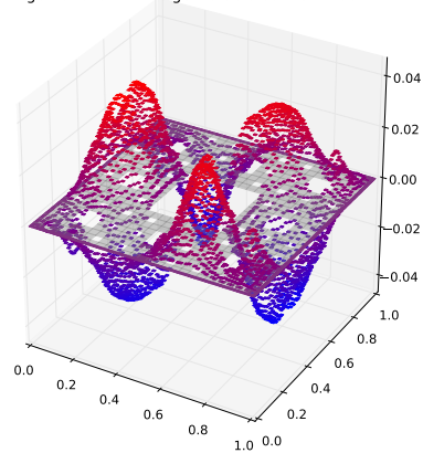
Eigenfunction with eigenvalue 0.0511512200244
