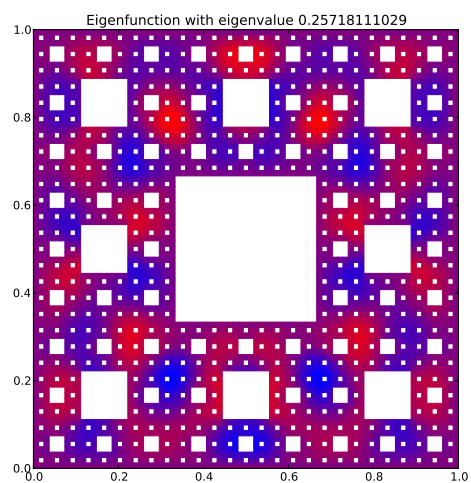
Eigenfunction 50 with eigenvalue 0.25718111029
