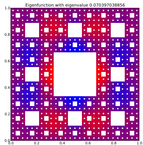
Eigenfunction 9 with eigenvalue 0.070397038856
