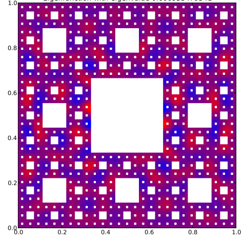
Eigenfunction with eigenvalue 0.606933479541
