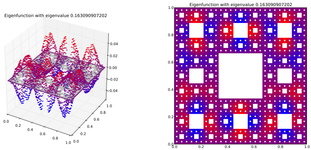
Eigenfunction 27 with eigenvalue 0.163090907202
