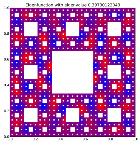
Eigenfunction 87 with eigenvalue 0.39730122043
