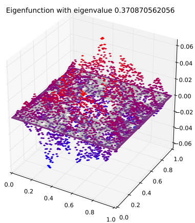
Eigenfunction 79 with eigenvalue 0.370870562056
