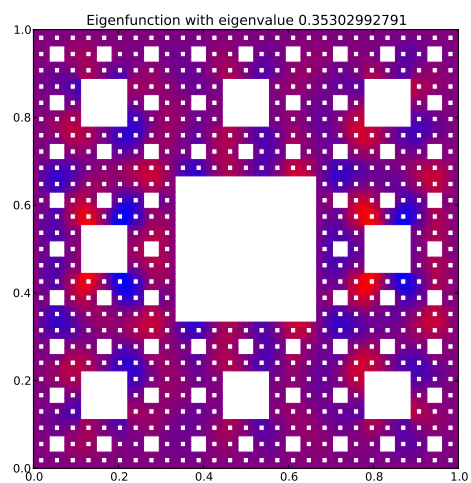
Eigenfunction 74 with eigenvalue 0.35302992791
