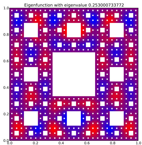
Eigenfunction 49 with eigenvalue 0.253000733772
