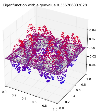
Eigenfunction 75 with eigenvalue 0.355706332028
