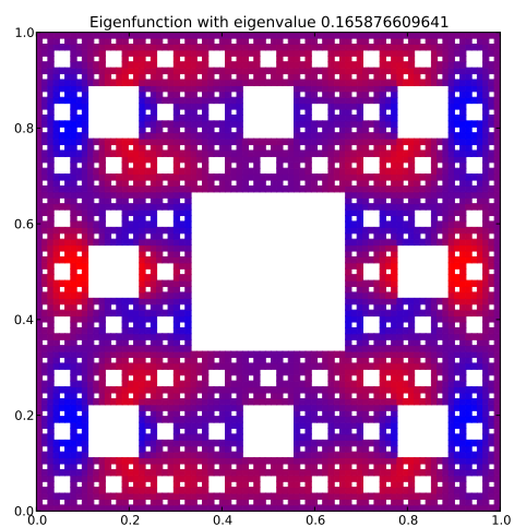
Eigenfunction 28 with eigenvalue 0.165876609641
