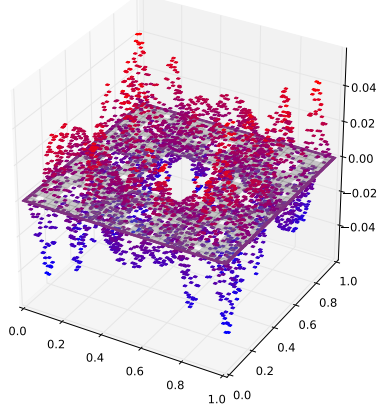
Eigenfunction with eigenvalue 0.440869249207
