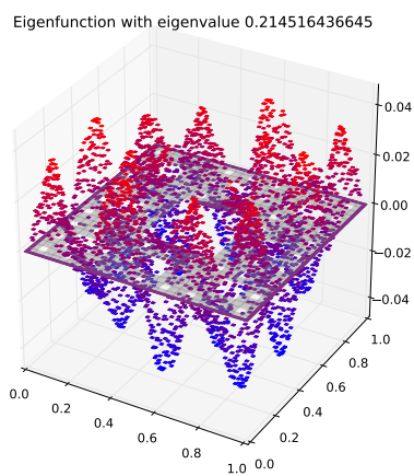
Eigenfunction 43 with eigenvalue 0.214516436645
