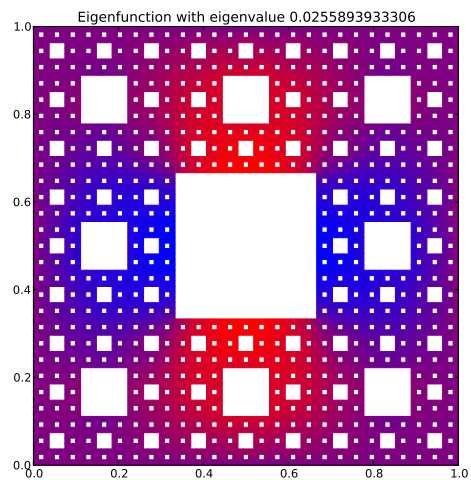
Eigenfunction 1 with eigenvalue 0.0255893933306
