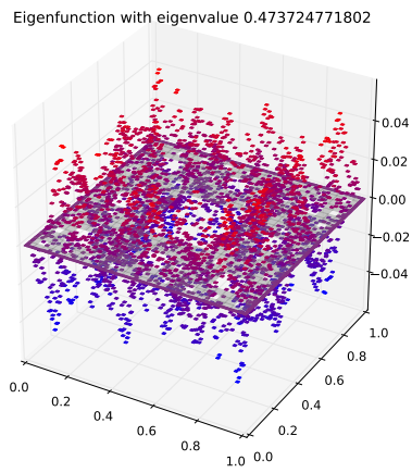
Eigenfunction 113 with eigenvalue 0.473724771802
