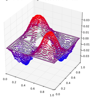
Eigenfunction with eigenvalue 0.0346262438971
