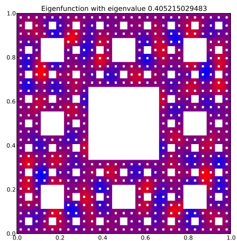
Eigenfunction 89 with eigenvalue 0.405215029483
