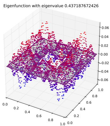
Eigenfunction 101 with eigenvalue 0.437187672426
