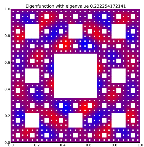
Eigenfunction 46 with eigenvalue 0.232254172141
