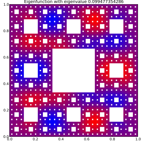
Eigenfunction with eigenvalue 0.099477354286
