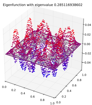
Eigenfunction 57 with eigenvalue 0.285116938602
