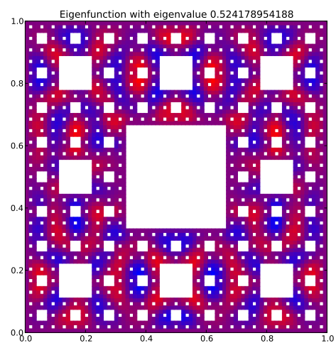
Eigenfunction 124 with eigenvalue 0.524178954188
