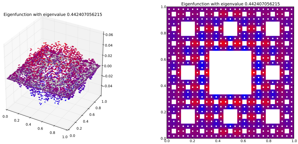
Eigenfunction 106 with eigenvalue 0.442407056215
