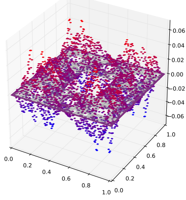
Eigenfunction with eigenvalue 0.439110760894
