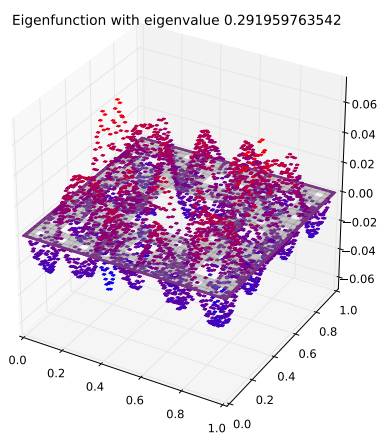
Eigenfunction 59 with eigenvalue 0.291959763542
