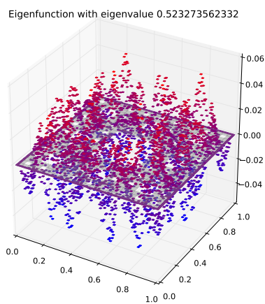
Eigenfunction 123 with eigenvalue 0.523273562332
