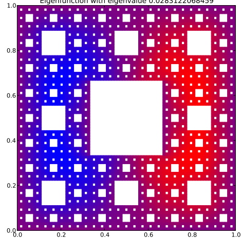
Eigenfunction with eigenvalue 0.0283122068459
