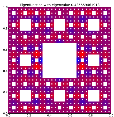
Eigenfunction 100 with eigenvalue 0.435559461913
