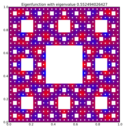
Eigenfunction 133 with eigenvalue 0.552494026427
