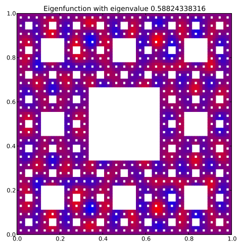
Eigenfunction 139 with eigenvalue 0.58824338316
