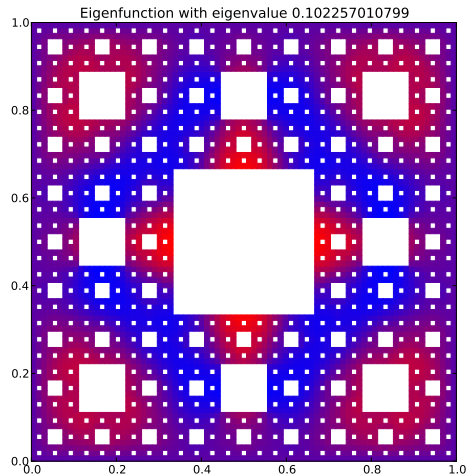
Eigenfunction with eigenvalue 0.102257010799
