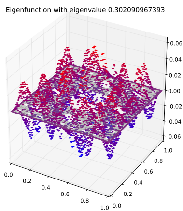
Eigenfunction 61 with eigenvalue 0.302090967393
