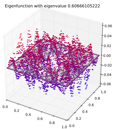
Eigenfunction 143 with eigenvalue 0.60666105222
