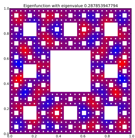
Eigenfunction 58 with eigenvalue 0.287853947794
