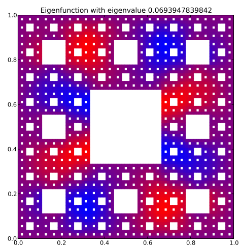
Eigenfunction 8 with eigenvalue 0.0693947839842
