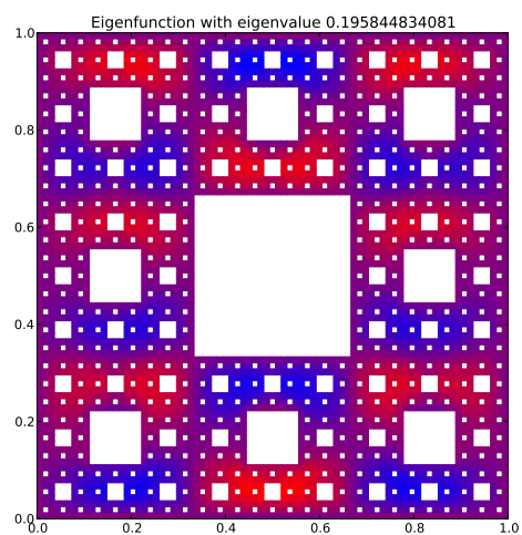
Eigenfunction 36 with eigenvalue 0.195844834081
