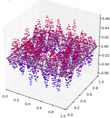
Eigenfunction with eigenvalue 0.58824338316
