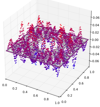
Eigenfunction with eigenvalue 0.541756709857
