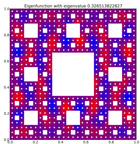
Eigenfunction 68 with eigenvalue 0.326513822827
