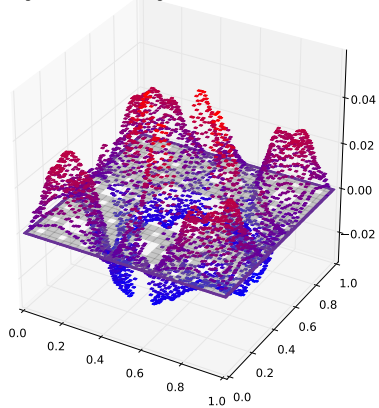
Eigenfunction with eigenvalue 0.102257010799
