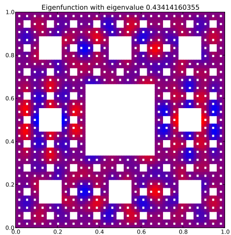
Eigenfunction 99 with eigenvalue 0.43414160355
