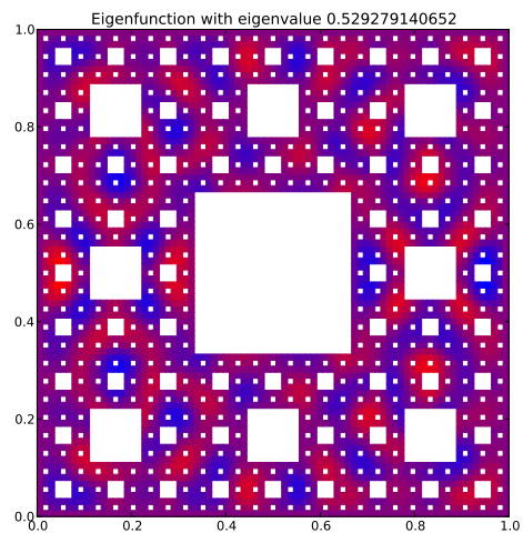
Eigenfunction 127 with eigenvalue 0.529279140652
