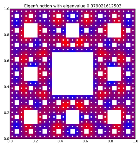
Eigenfunction 82 with eigenvalue 0.379021612503
