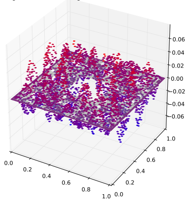
Eigenfunction with eigenvalue 0.606933479541
