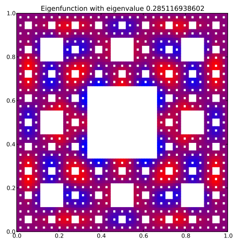
Eigenfunction 57 with eigenvalue 0.285116938602
