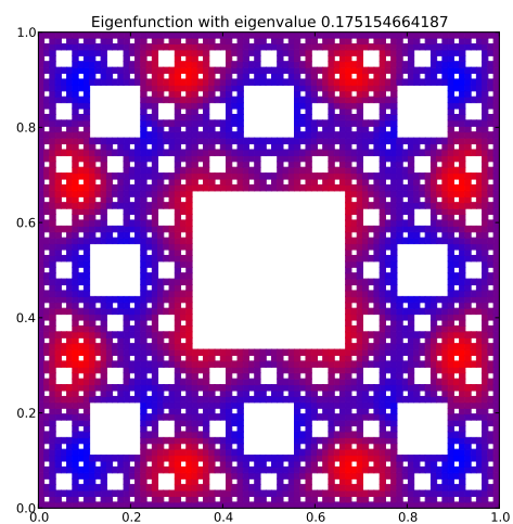
Eigenfunction 32 with eigenvalue 0.175154664187
