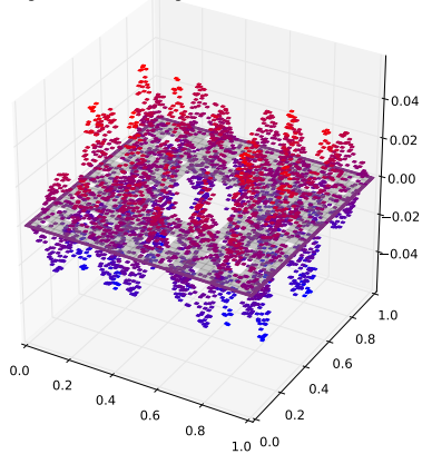
Eigenfunction with eigenvalue 0.392435065867
