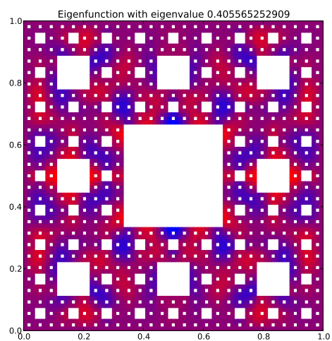
Eigenfunction 90 with eigenvalue 0.405565252909
