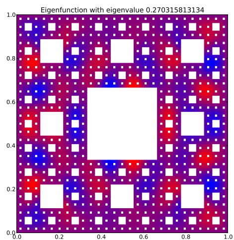
Eigenfunction 54 with eigenvalue 0.270315813134
