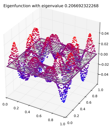
Eigenfunction 39 with eigenvalue 0.206692322268
