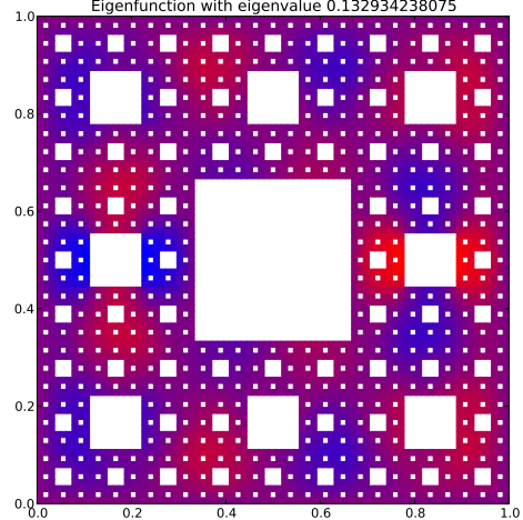
Eigenfunction with eigenvalue 0.132934238075
