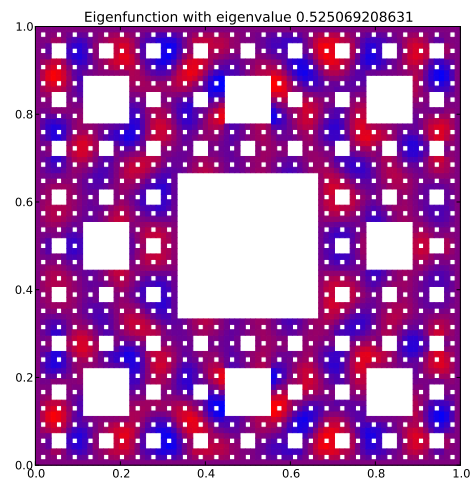
Eigenfunction 125 with eigenvalue 0.525069208631
