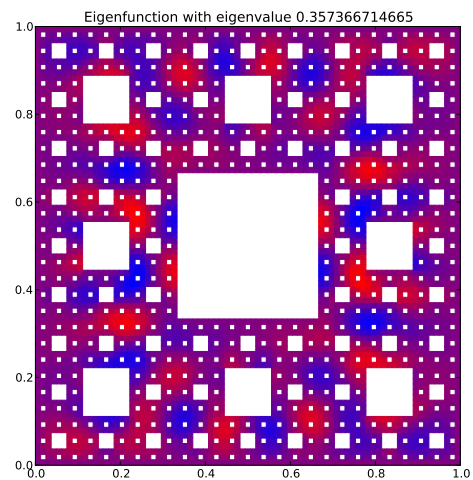
Eigenfunction 77 with eigenvalue 0.357366714665
