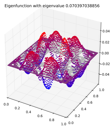
Eigenfunction 9 with eigenvalue 0.070397038856
