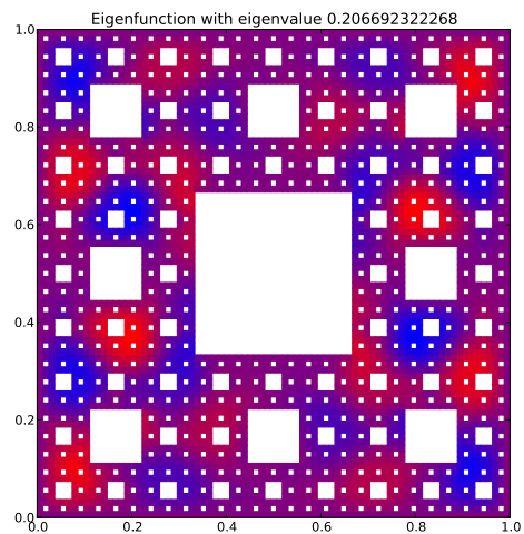
Eigenfunction 39 with eigenvalue 0.206692322268
