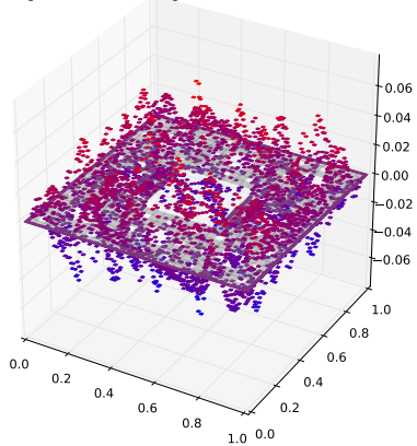
Eigenfunction with eigenvalue 0.406742914017
