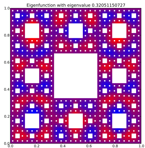
Eigenfunction 67 with eigenvalue 0.32051150727
