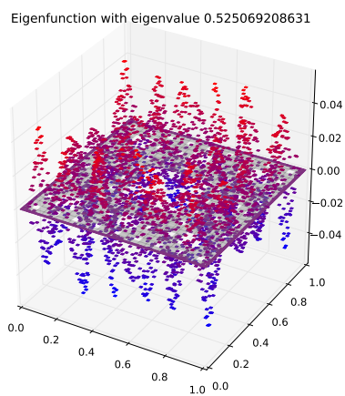
Eigenfunction 125 with eigenvalue 0.525069208631
