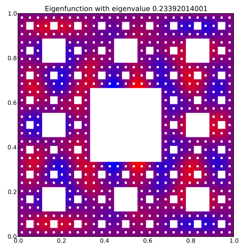
Eigenfunction 47 with eigenvalue 0.23392014001
