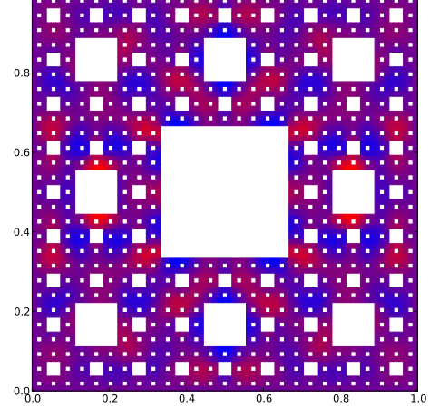
Eigenfunction with eigenvalue 0.43949500471
