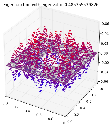
Eigenfunction 115 with eigenvalue 0.485355539826
