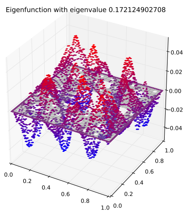
Eigenfunction 31 with eigenvalue 0.172124902708
