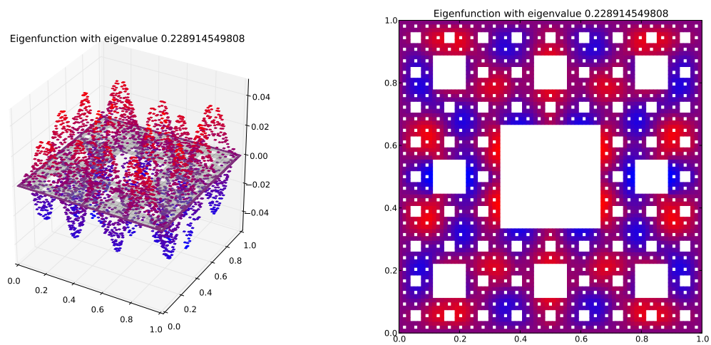
Eigenfunction 45 with eigenvalue 0.228914549808
