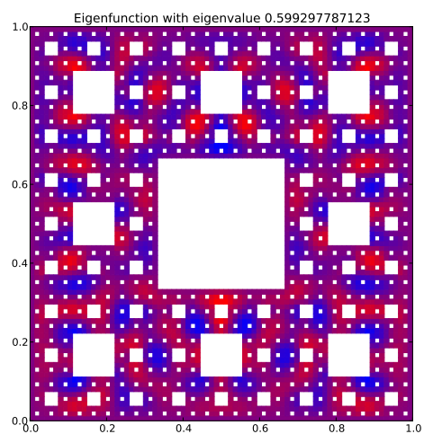
Eigenfunction 142 with eigenvalue 0.599297787123
