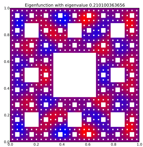
Eigenfunction 41 with eigenvalue 0.210100363656
