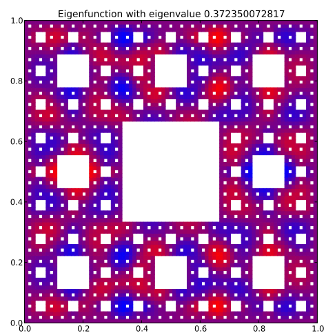
Eigenfunction 80 with eigenvalue 0.372350072817
