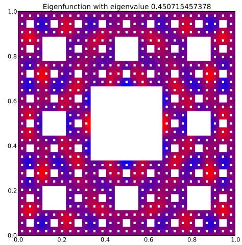
Eigenfunction 109 with eigenvalue 0.450715457378
