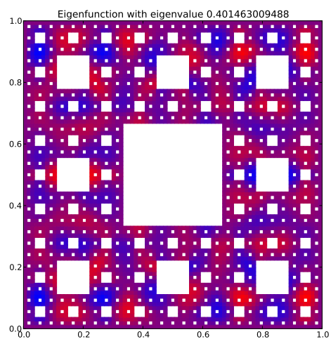
Eigenfunction 88 with eigenvalue 0.401463009488
