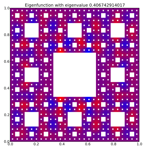
Eigenfunction 91 with eigenvalue 0.406742914017
