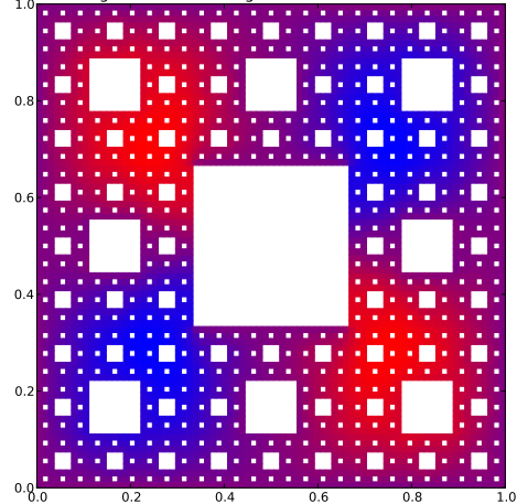
Eigenfunction with eigenvalue 0.0346262438971
