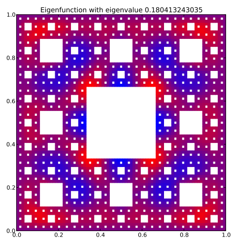
Eigenfunction 34 with eigenvalue 0.180413243035
