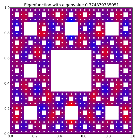
Eigenfunction 81 with eigenvalue 0.374879735051
