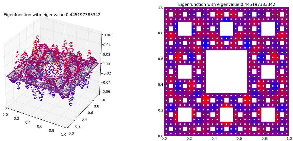
Eigenfunction 107 with eigenvalue 0.445197383342
