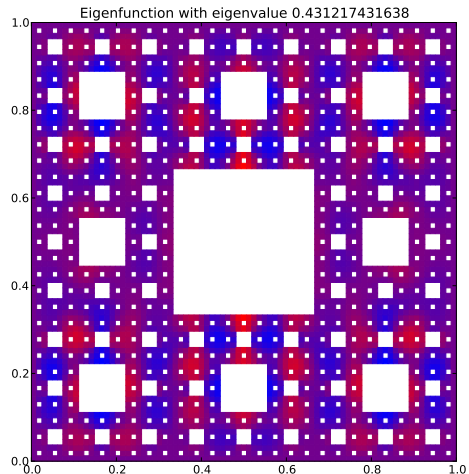
Eigenfunction with eigenvalue 0.431217431638
