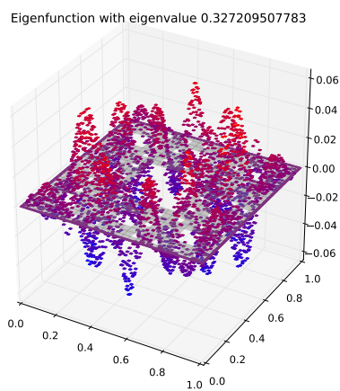
Eigenfunction 69 with eigenvalue 0.327209507783
