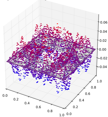
Eigenfunction with eigenvalue 0.431217431638
