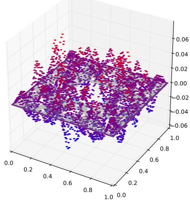
Eigenfunction with eigenvalue 0.43949500471
