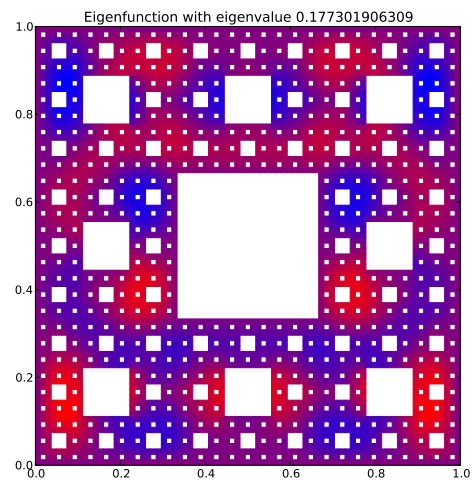
Eigenfunction 33 with eigenvalue 0.177301906309
