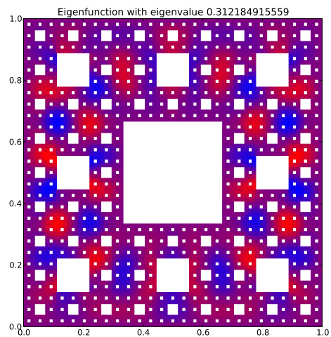
Eigenfunction 63 with eigenvalue 0.312184915559
