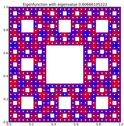
Eigenfunction 143 with eigenvalue 0.60666105222
