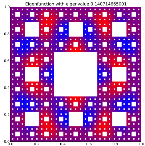
Eigenfunction with eigenvalue 0.140714665001
