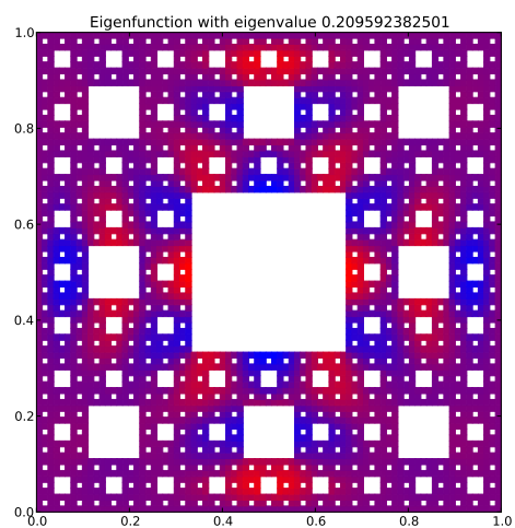
Eigenfunction 40 with eigenvalue 0.209592382501
