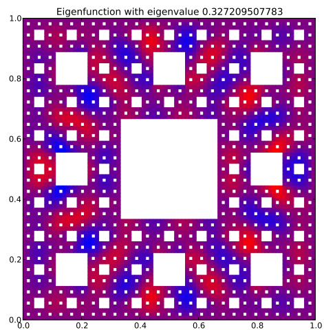
Eigenfunction 69 with eigenvalue 0.327209507783
