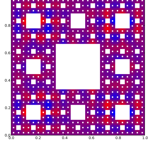
Eigenfunction with eigenvalue 0.439110760894
