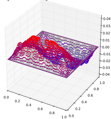
Eigenfunction with eigenvalue 0.0308346785581
