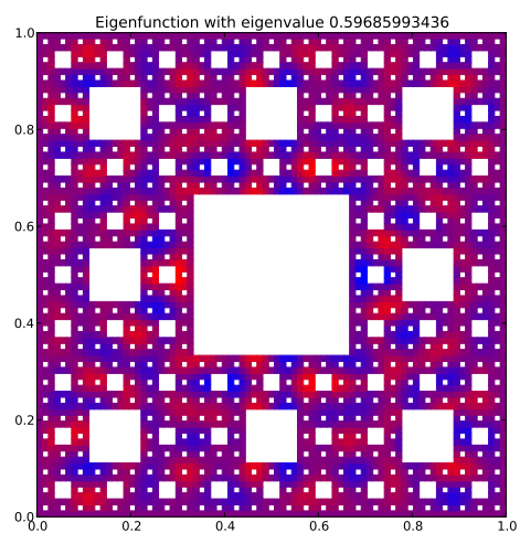
Eigenfunction 140 with eigenvalue 0.59685993436
