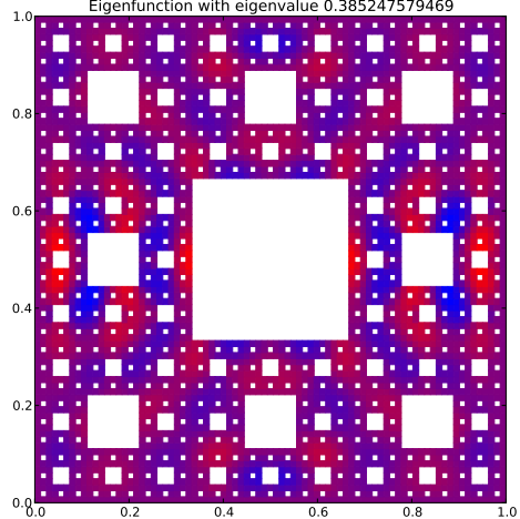
Eigenfunction with eigenvalue 0.385247579469
