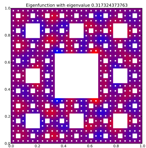
Eigenfunction 65 with eigenvalue 0.317324373763
