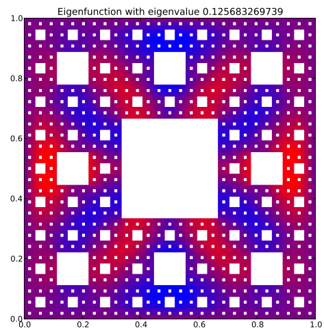
Eigenfunction 19 with eigenvalue 0.125683269739
