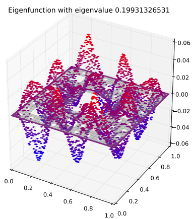
Eigenfunction 37 with eigenvalue 0.19931326531
