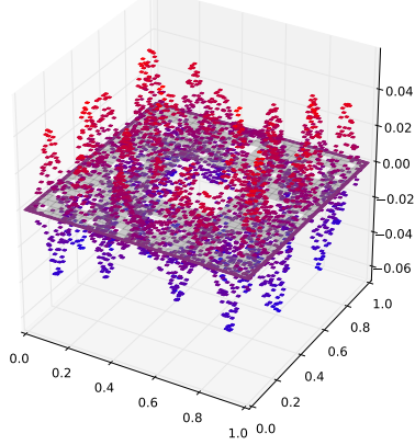
Eigenfunction with eigenvalue 0.450715457378
