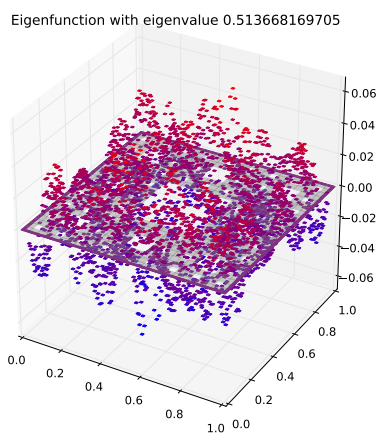
Eigenfunction 121 with eigenvalue 0.513668169705
