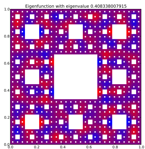
Eigenfunction 92 with eigenvalue 0.408338007915
