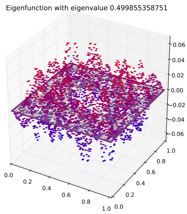
Eigenfunction 117 with eigenvalue 0.499855358751
