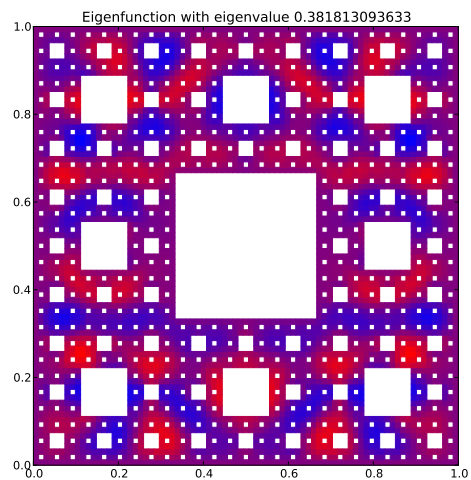
Eigenfunction 83 with eigenvalue 0.381813093633
