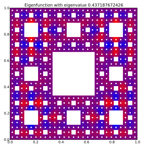
Eigenfunction 101 with eigenvalue 0.437187672426
