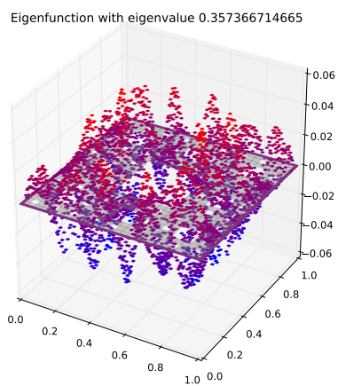
Eigenfunction 77 with eigenvalue 0.357366714665
