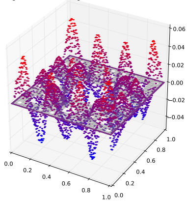
Eigenfunction with eigenvalue 0.244332051991
