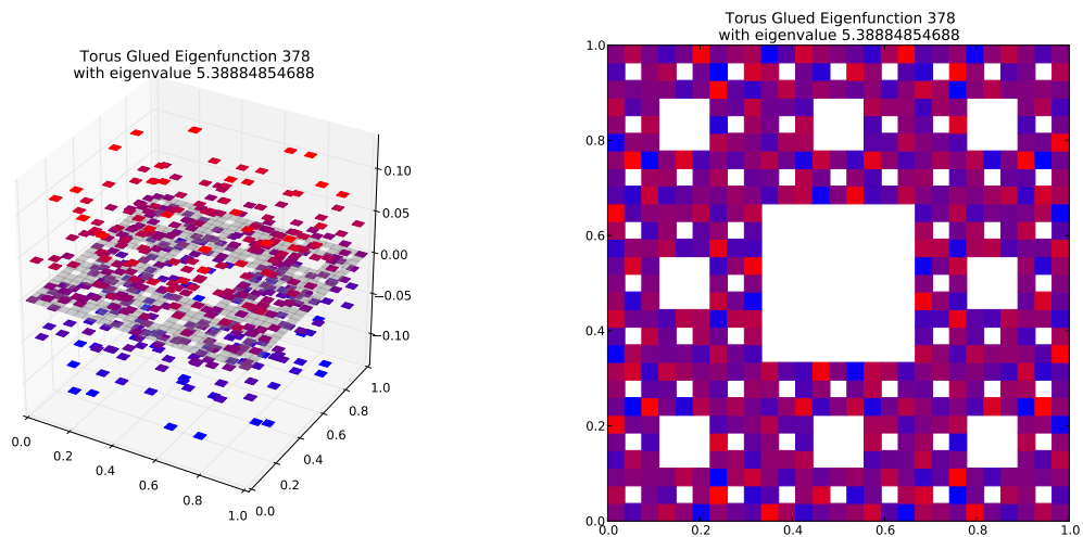
Eigenfunction 378 with eigenvalue 5.38884854688
