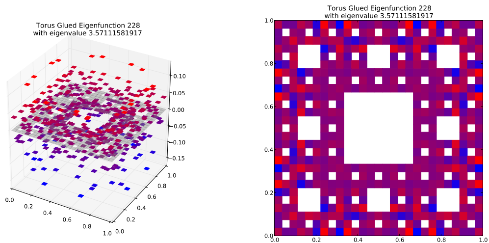
Eigenfunction 228 with eigenvalue 3.57111581917
