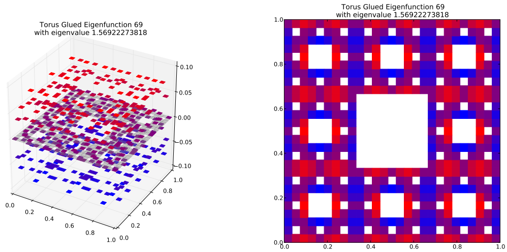
Eigenfunction 69 with eigenvalue 1.56922273818
