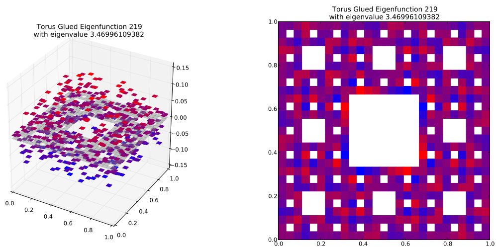
Eigenfunction 219 with eigenvalue 3.46996109382
