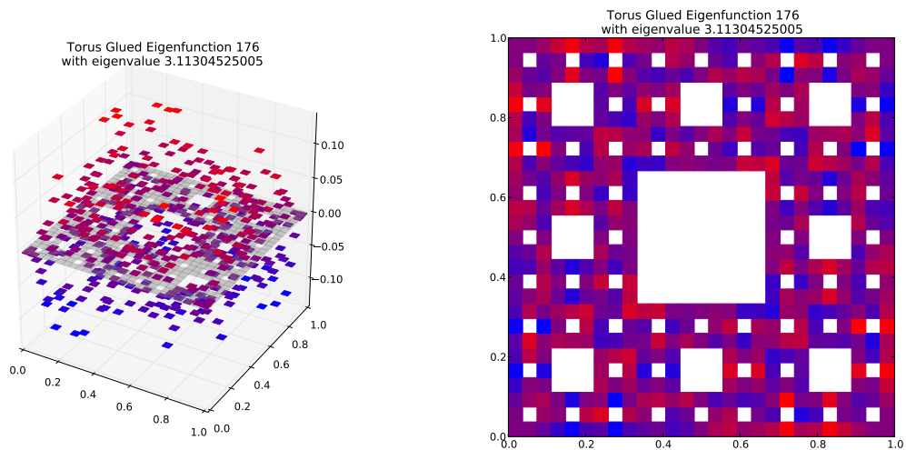
Eigenfunction 176 with eigenvalue 3.11304525005
