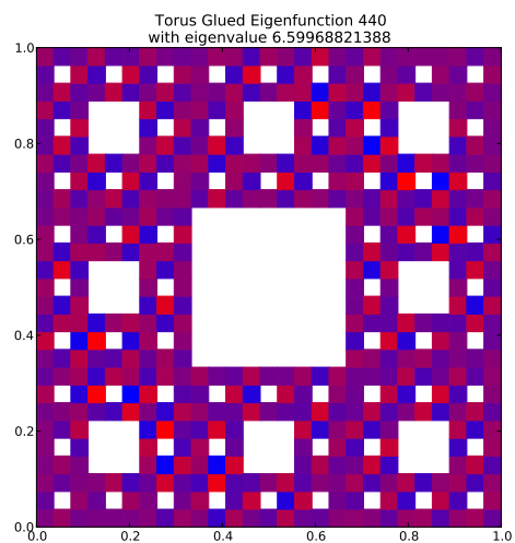
Eigenfunction 440 with eigenvalue 6.59968821388
