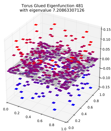
Eigenfunction 481 with eigenvalue 7.20863307126
