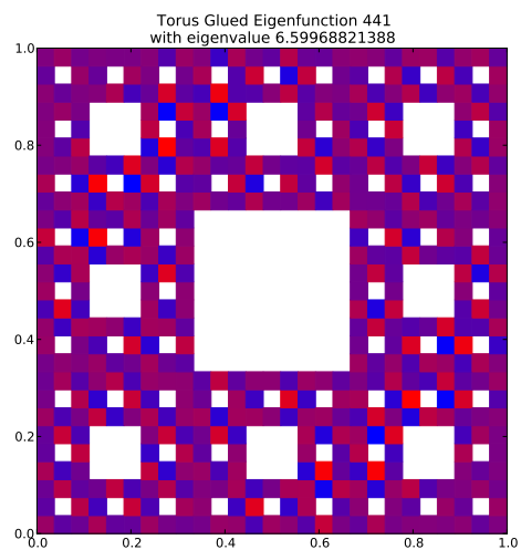
Eigenfunction 441 with eigenvalue 6.59968821388
