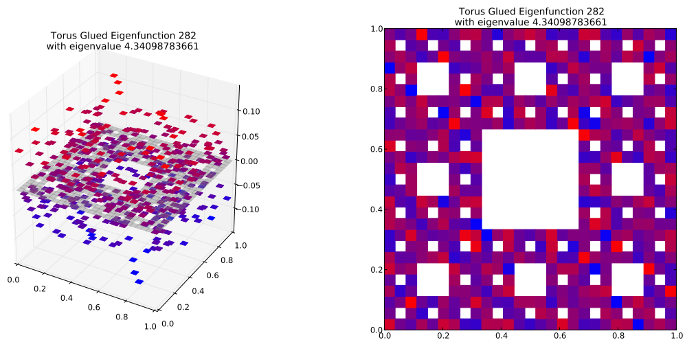
Eigenfunction 282 with eigenvalue 4.34098783661
