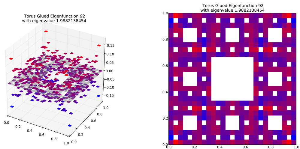
Eigenfunction 92 with eigenvalue 1.9882138454
