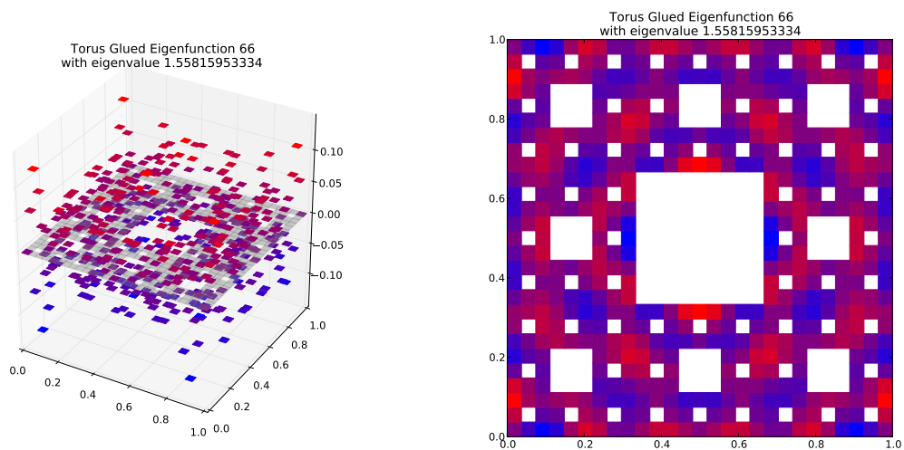
Eigenfunction 66 with eigenvalue 1.55815953334
