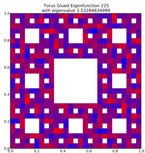
Eigenfunction 225 with eigenvalue 3.53284834999
