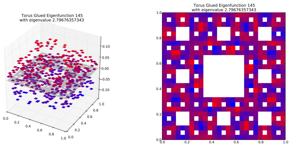
Eigenfunction 145 with eigenvalue 2.79676357343
