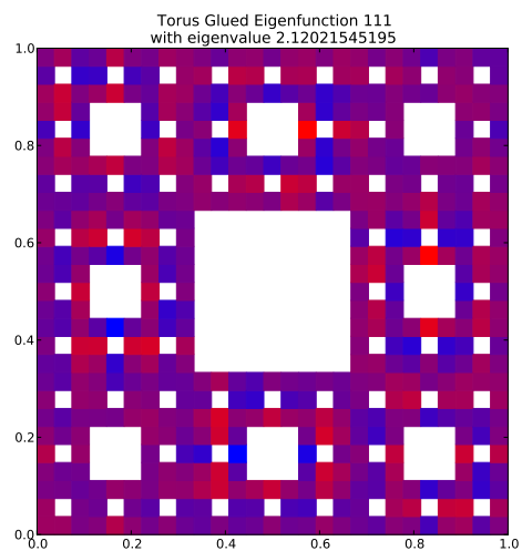
Eigenfunction 111 with eigenvalue 2.12021545195
