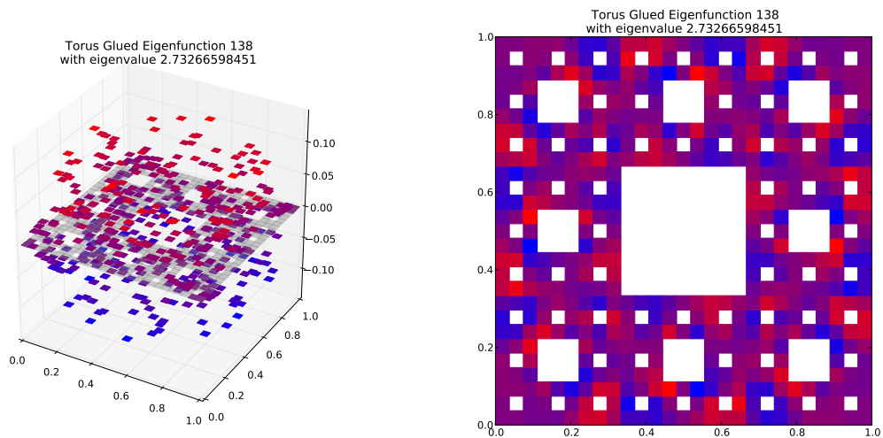
Eigenfunction 138 with eigenvalue 2.73266598451
