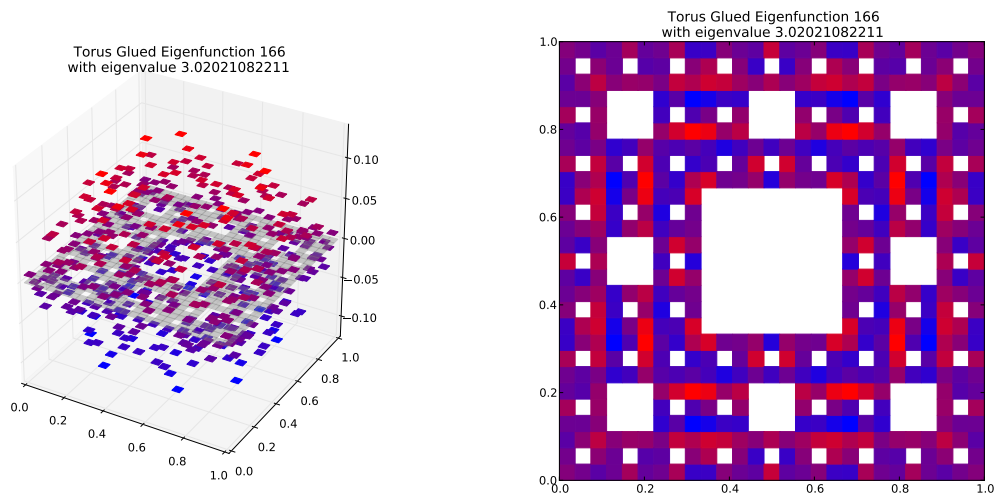
Eigenfunction 166 with eigenvalue 3.02021082211
