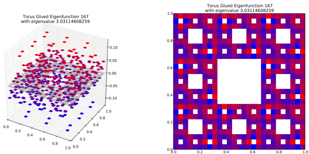
Eigenfunction 167 with eigenvalue 3.03114608259
