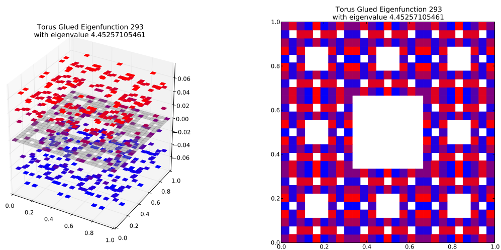
Eigenfunction 293 with eigenvalue 4.45257105461
