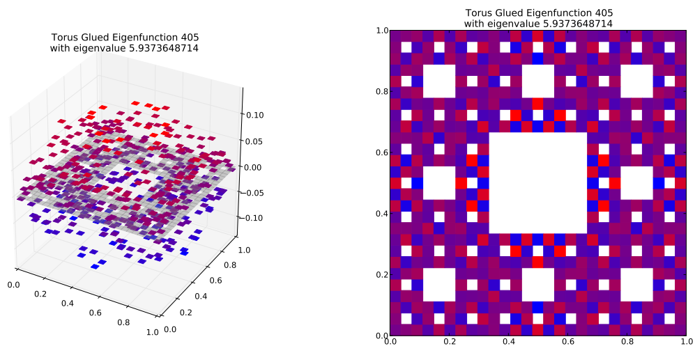
Eigenfunction 405 with eigenvalue 5.9373648714
