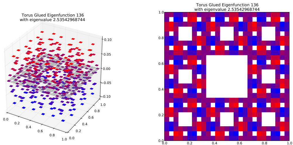
Eigenfunction 136 with eigenvalue 2.53542968744
