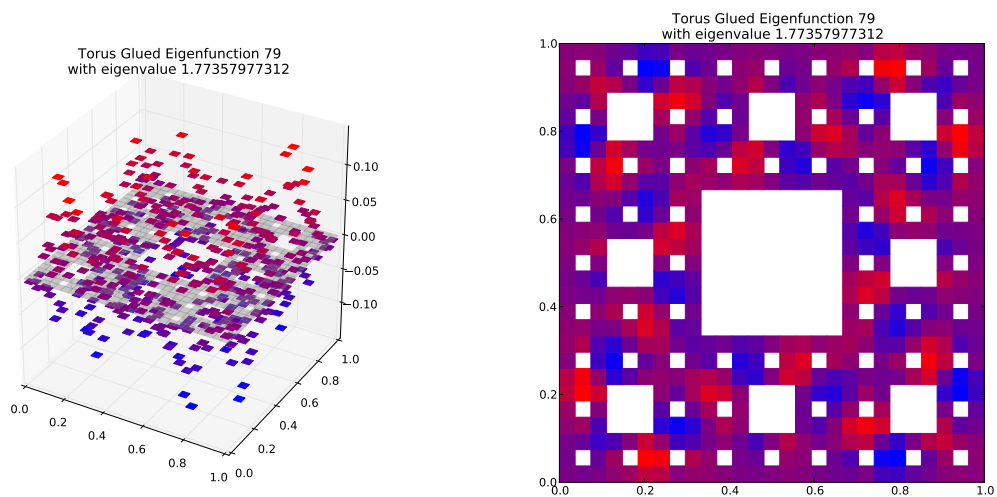
Eigenfunction 79 with eigenvalue 1.77357977312
