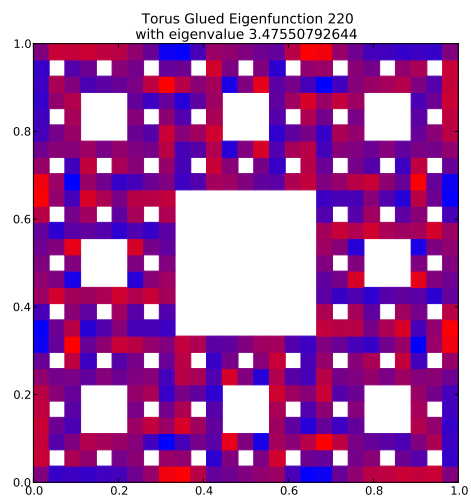
Eigenfunction 220 with eigenvalue 3.47550792644
