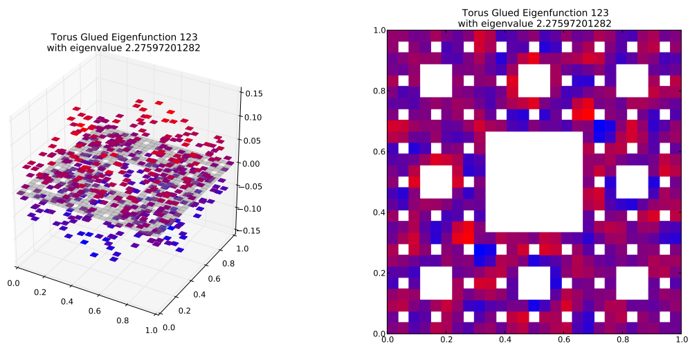
Eigenfunction 123 with eigenvalue 2.27597201282
