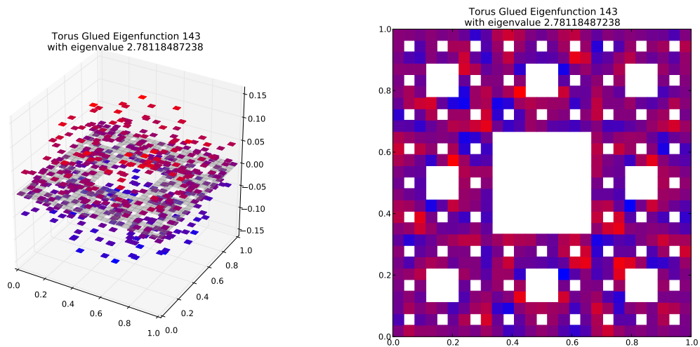
Eigenfunction 143 with eigenvalue 2.78118487238
