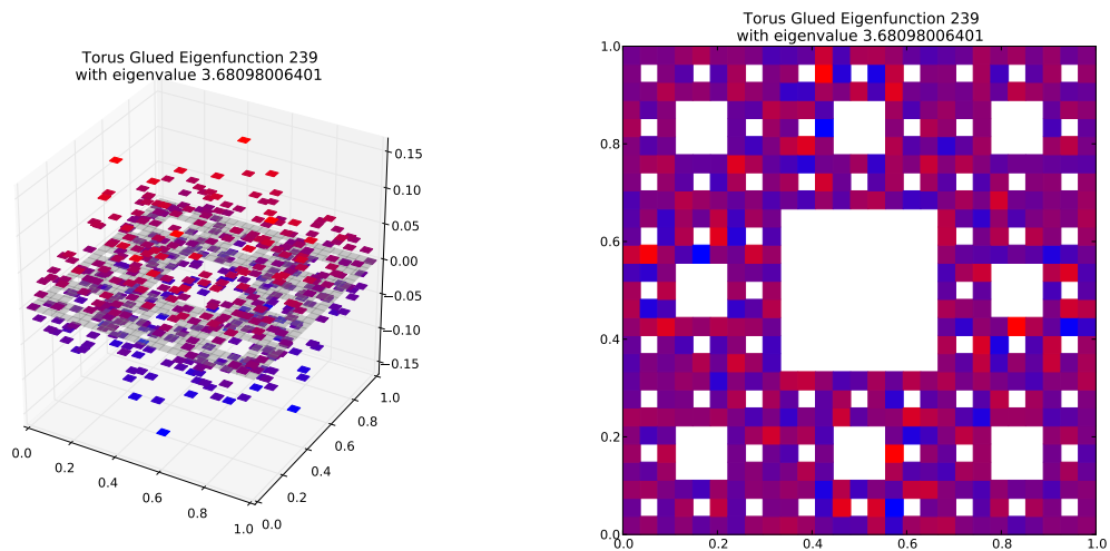
Eigenfunction 239 with eigenvalue 3.68098006401
