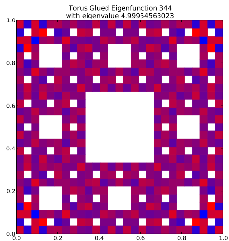
Eigenfunction 344 with eigenvalue 4.99954563023
