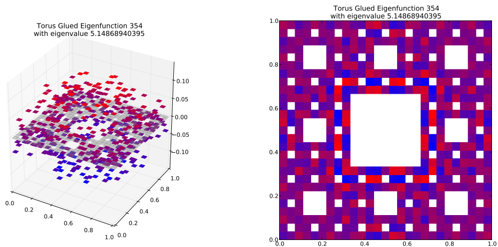
Eigenfunction 354 with eigenvalue 5.14868940395
