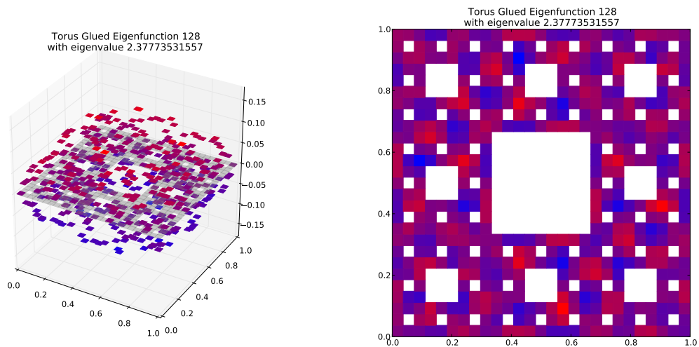
Eigenfunction 128 with eigenvalue 2.37773531557
