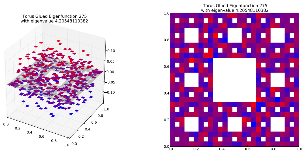
Eigenfunction 275 with eigenvalue 4.20548110382
