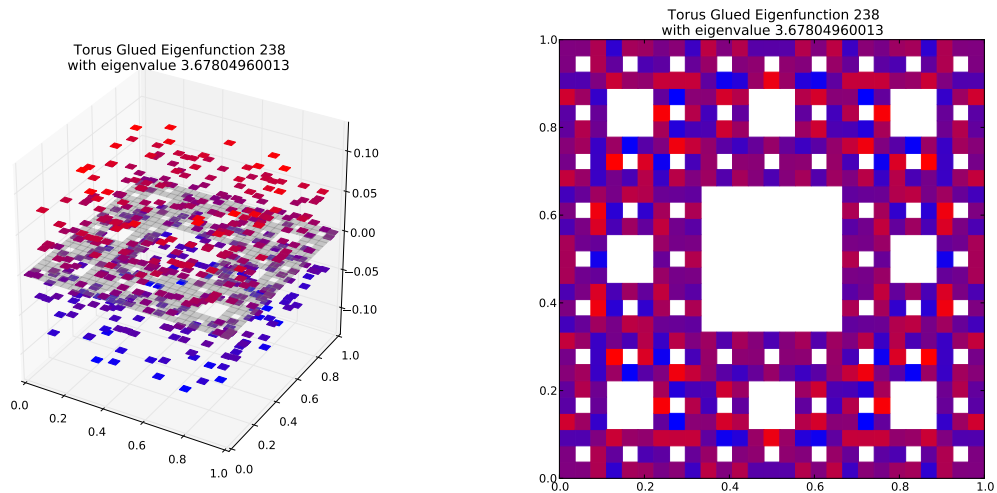
Eigenfunction 238 with eigenvalue 3.67804960013
