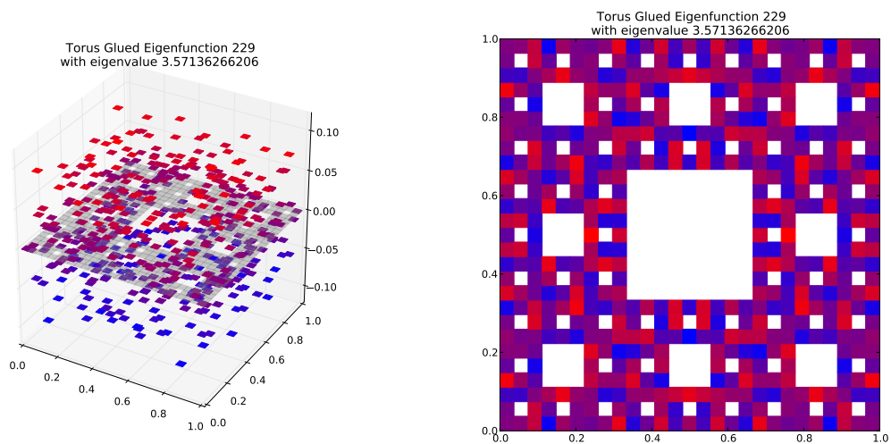
Eigenfunction 229 with eigenvalue 3.57136266206
