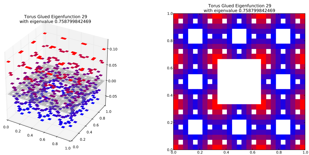
Eigenfunction 29 with eigenvalue 0.758799842469
