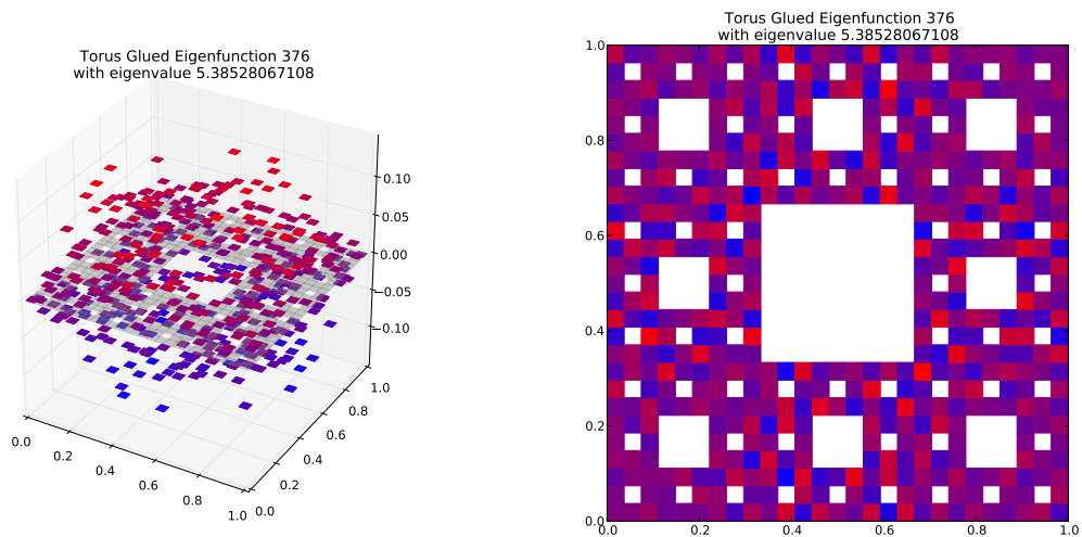
Eigenfunction 376 with eigenvalue 5.38528067108
