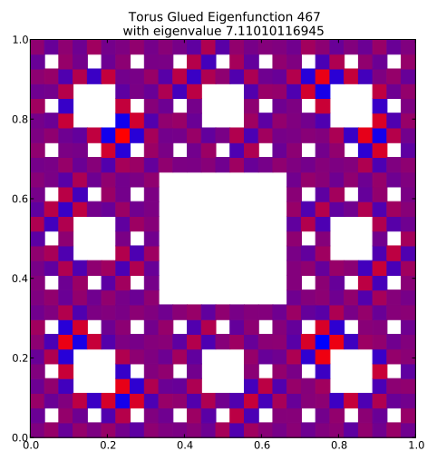
Eigenfunction 467 with eigenvalue 7.11010116945
