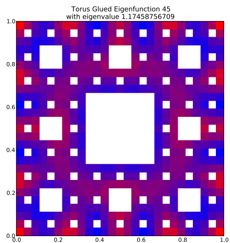
Eigenfunction 45 with eigenvalue 1.17458756709
