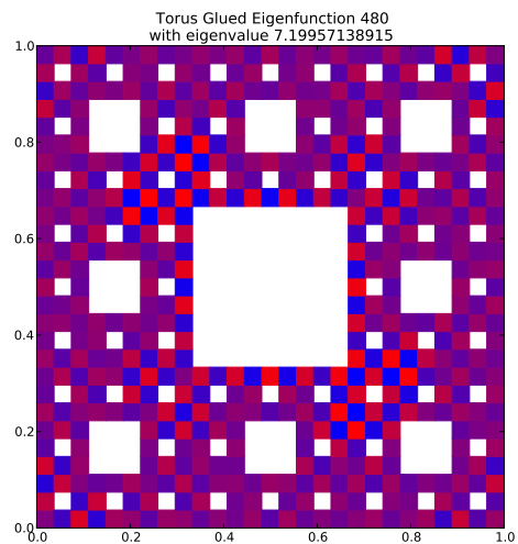
Eigenfunction 480 with eigenvalue 7.19957138915
