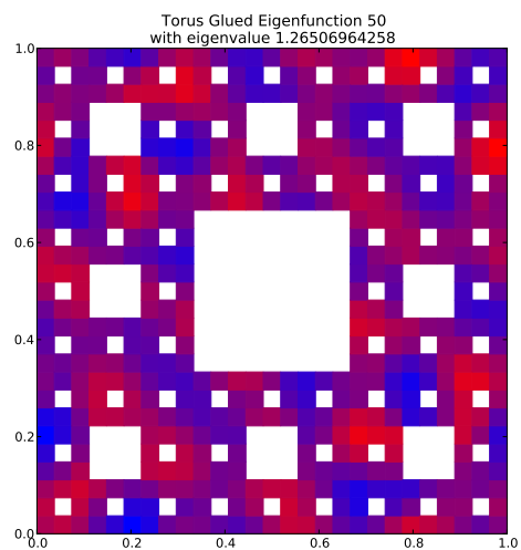
Eigenfunction 50 with eigenvalue 1.26506964258
