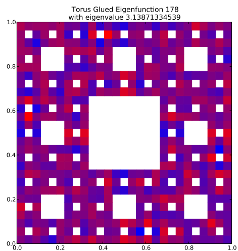
Eigenfunction 178 with eigenvalue 3.13871334539
