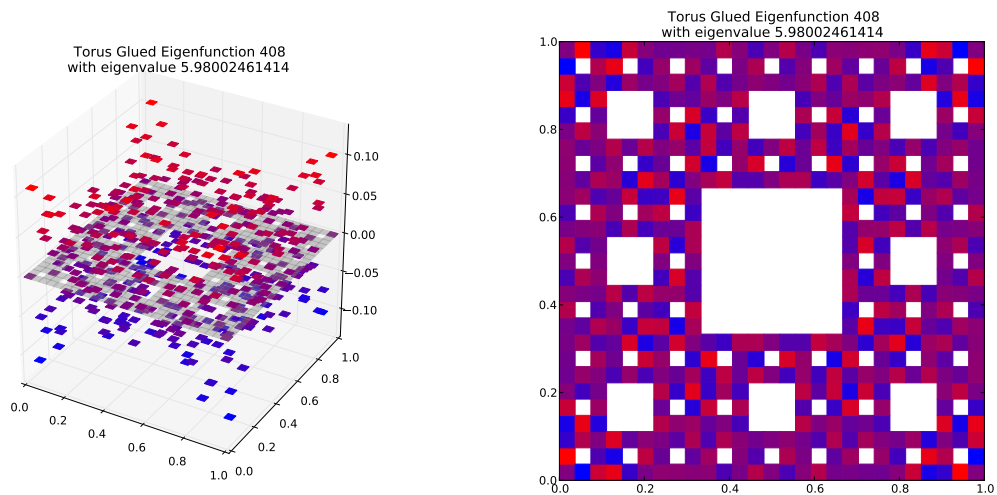
Eigenfunction 408 with eigenvalue 5.98002461414
