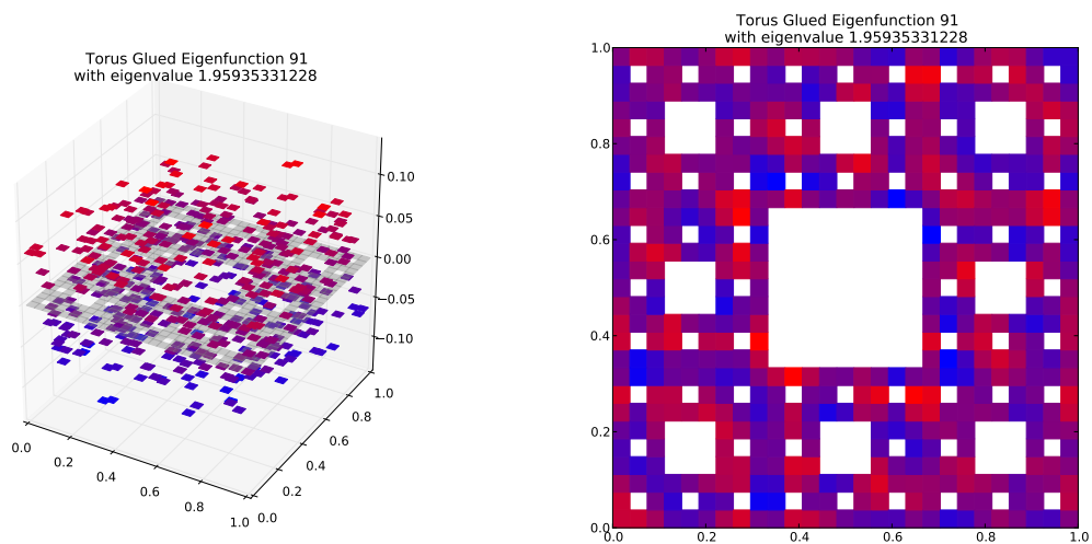
Eigenfunction 91 with eigenvalue 1.95935331228
