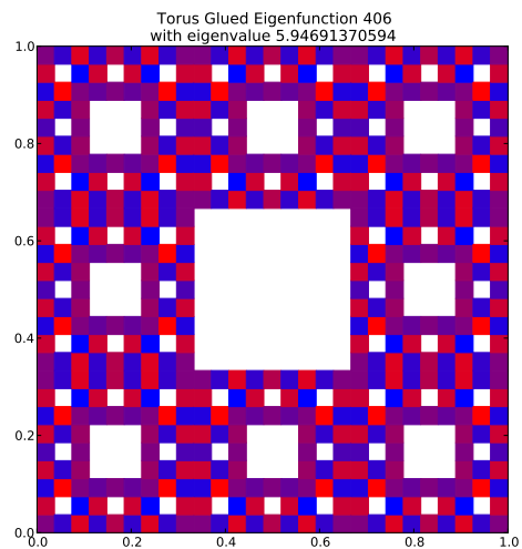
Eigenfunction 406 with eigenvalue 5.94691370594
