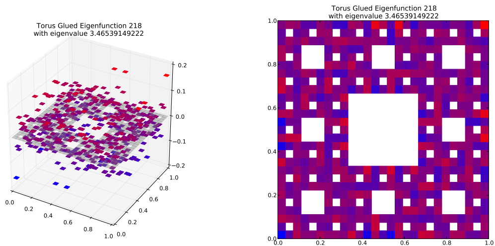
Eigenfunction 218 with eigenvalue 3.46539149222
