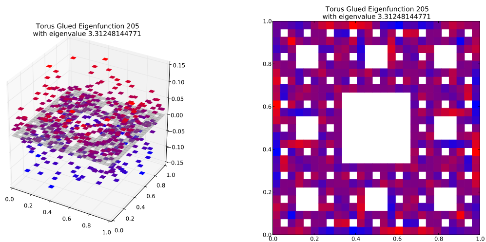
Eigenfunction 205 with eigenvalue 3.31248144771
