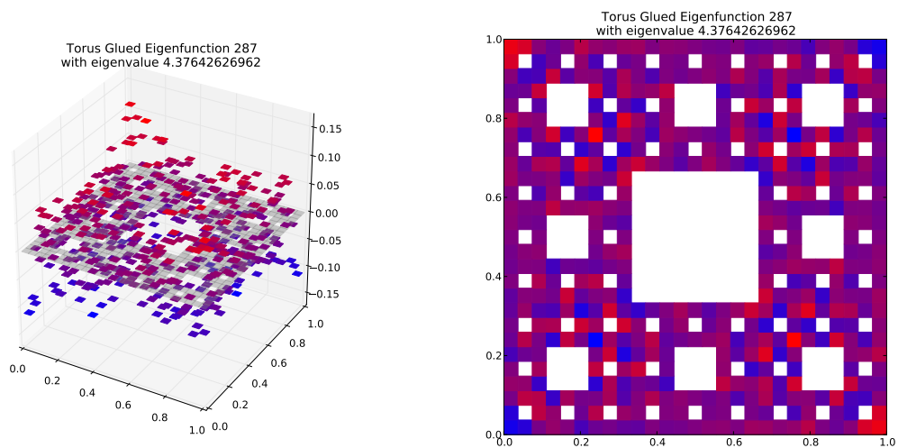
Eigenfunction 287 with eigenvalue 4.37642626962
