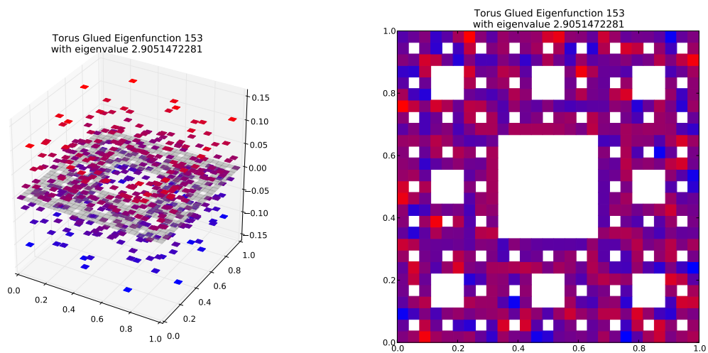
Eigenfunction 153 with eigenvalue 2.9051472281
