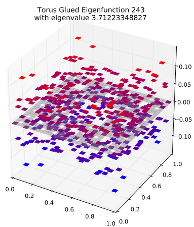
Eigenfunction 243 with eigenvalue 3.71223348827
