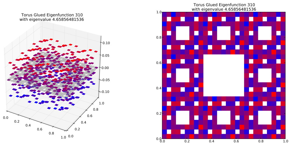
Eigenfunction 310 with eigenvalue 4.65856481536
