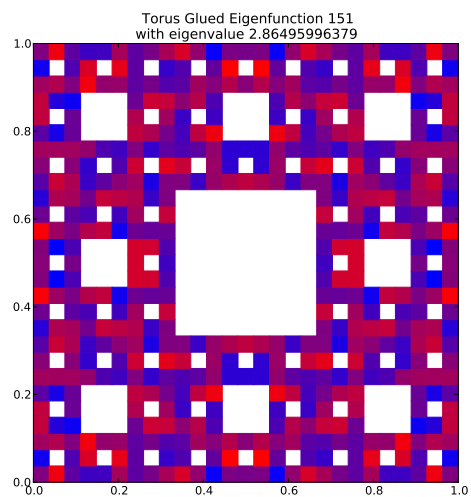
Eigenfunction 151 with eigenvalue 2.86495996379
