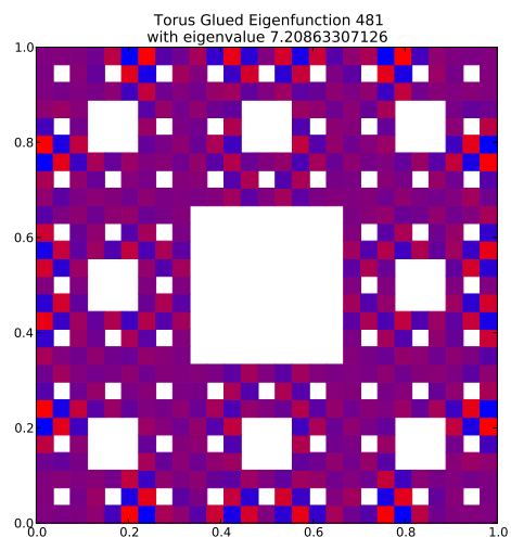
Eigenfunction 481 with eigenvalue 7.20863307126
