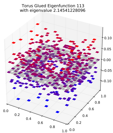
Eigenfunction 113 with eigenvalue 2.14541228096
