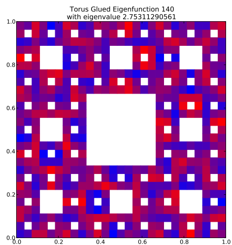
Eigenfunction 140 with eigenvalue 2.75311290561
