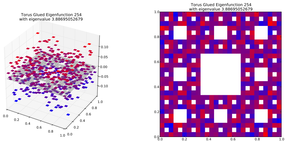
Eigenfunction 254 with eigenvalue 3.88695052679
