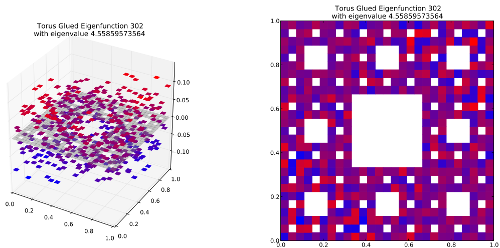
Eigenfunction 302 with eigenvalue 4.55859573564
