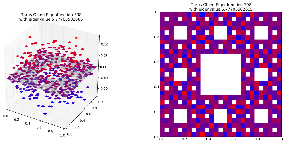
Eigenfunction 398 with eigenvalue 5.77705502665
