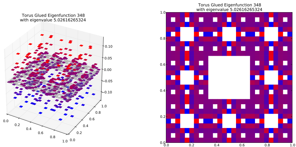
Eigenfunction 348 with eigenvalue 5.02616265324
