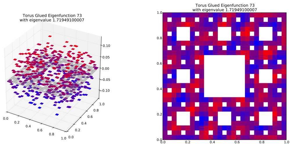
Eigenfunction 73 with eigenvalue 1.71949100007
