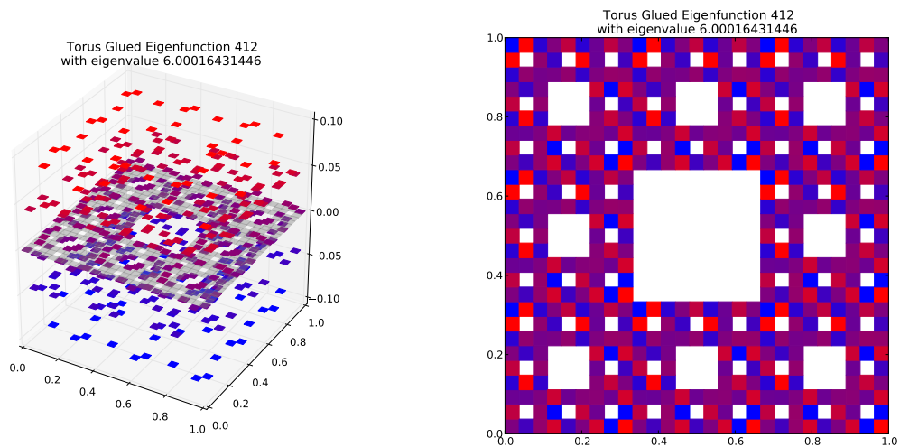
Eigenfunction 412 with eigenvalue 6.00016431446
