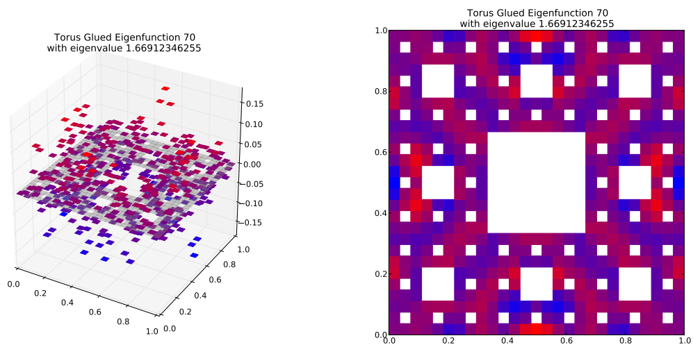
Eigenfunction 70 with eigenvalue 1.66912346255
