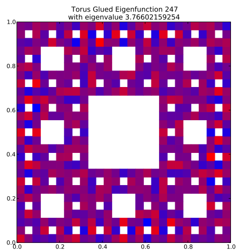
Eigenfunction 247 with eigenvalue 3.76602159254
