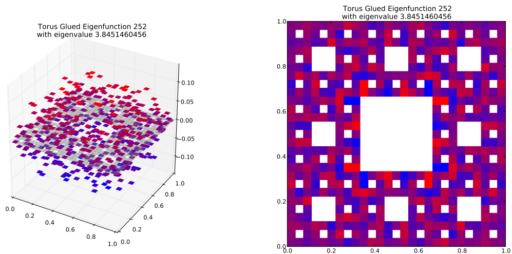
Eigenfunction 252 with eigenvalue 3.8451460456
