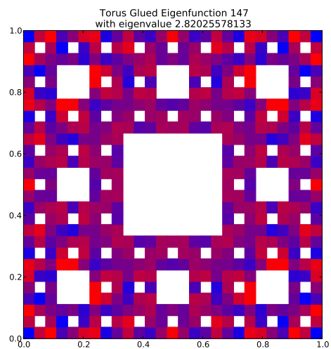
Eigenfunction 147 with eigenvalue 2.82025578133
