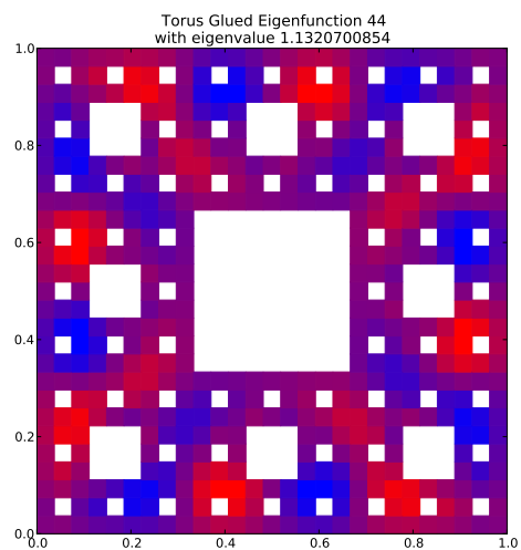
Eigenfunction 44 with eigenvalue 1.1320700854
