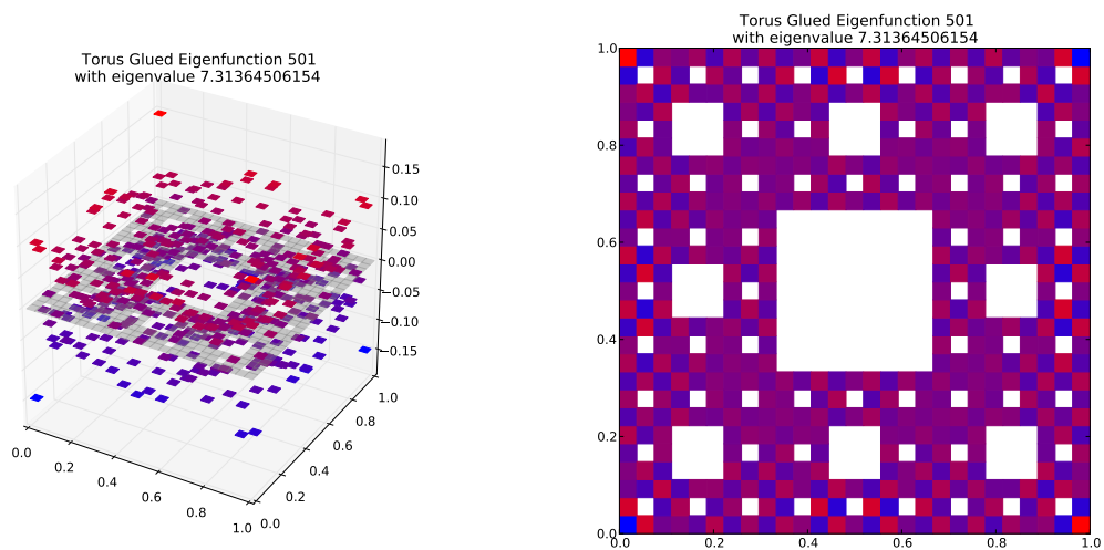
Eigenfunction 501 with eigenvalue 7.31364506154
