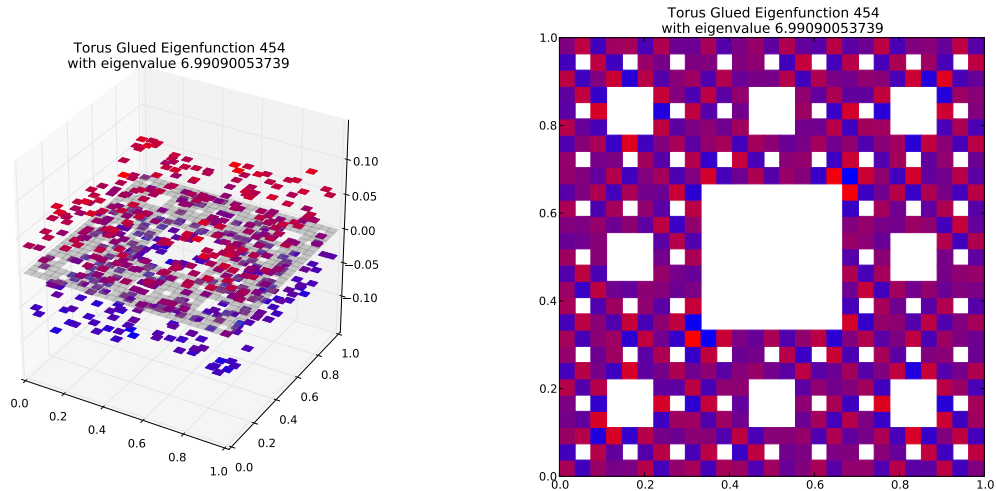
Eigenfunction 454 with eigenvalue 6.99090053739
