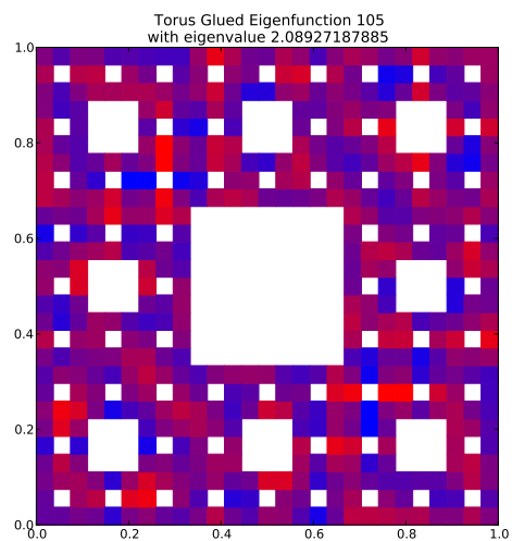
Eigenfunction 105 with eigenvalue 2.08927187885
