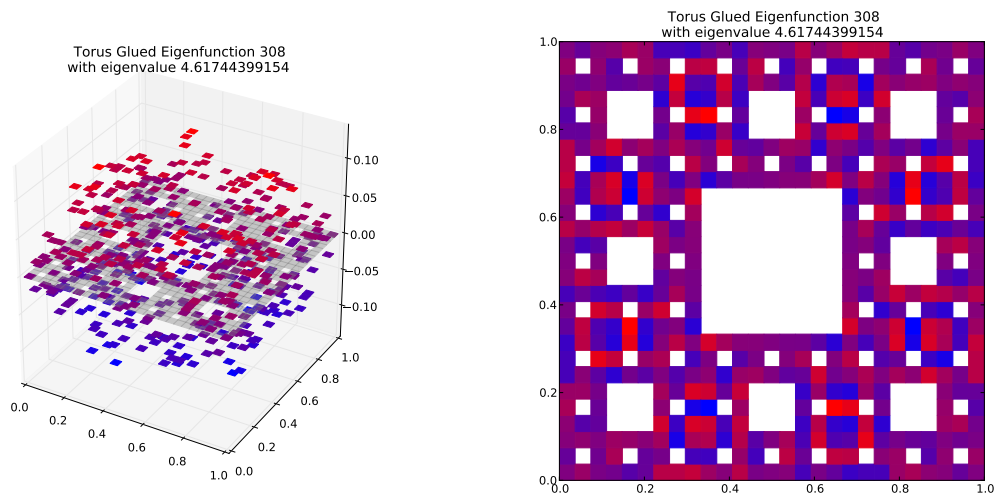
Eigenfunction 308 with eigenvalue 4.61744399154
