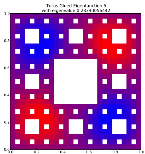
Eigenfunction 5 with eigenvalue 0.23340056442
