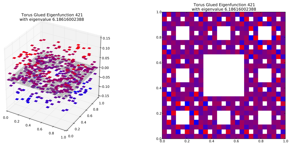
Eigenfunction 421 with eigenvalue 6.18616002388
