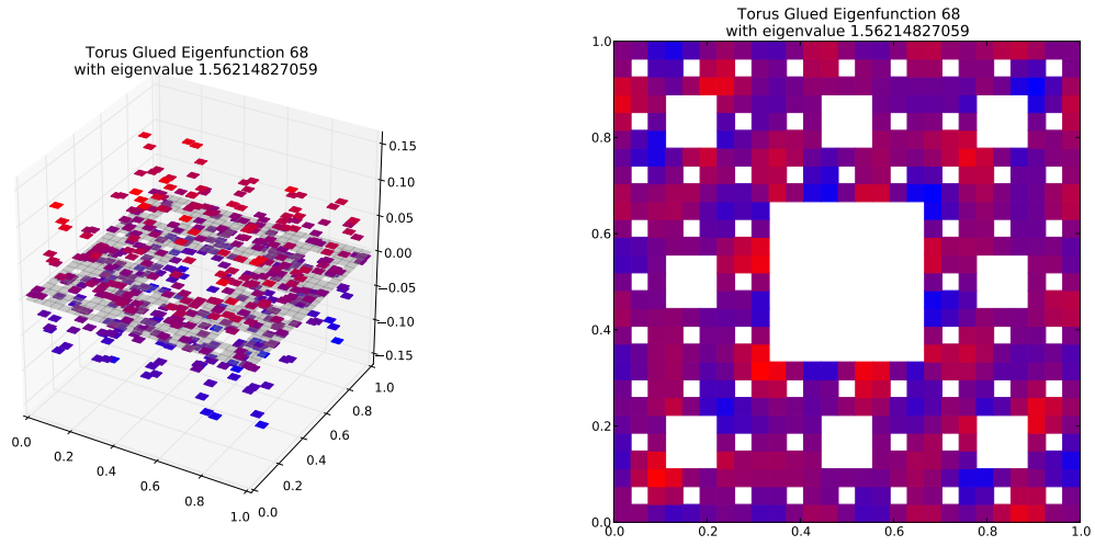
Eigenfunction 68 with eigenvalue 1.56214827059
