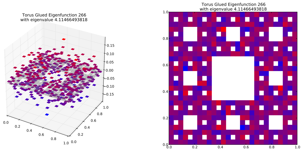
Eigenfunction 266 with eigenvalue 4.11466493818
