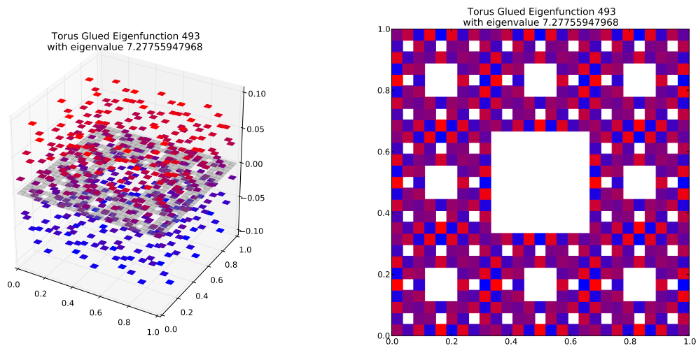
Eigenfunction 493 with eigenvalue 7.27755947968
