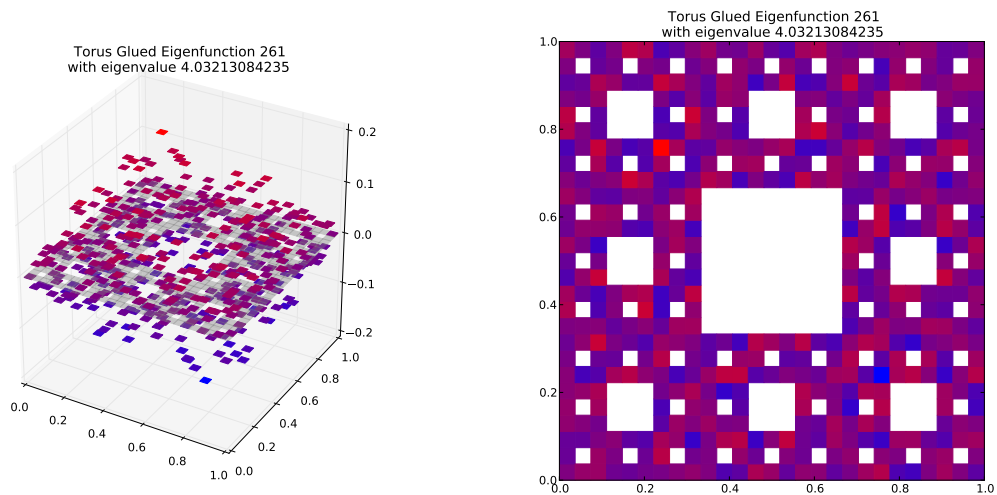
Eigenfunction 261 with eigenvalue 4.03213084235
