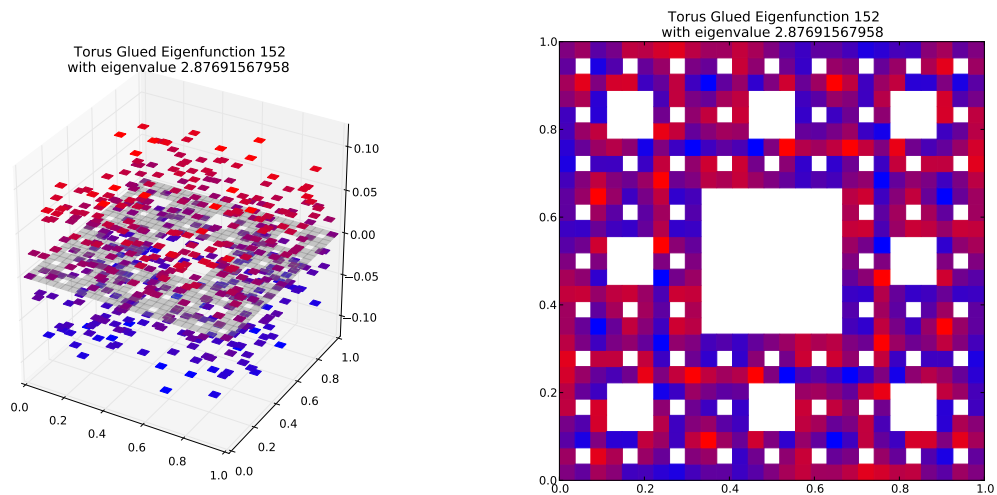
Eigenfunction 152 with eigenvalue 2.87691567958
