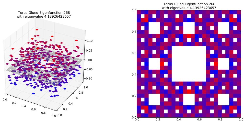
Eigenfunction 268 with eigenvalue 4.13926423657
