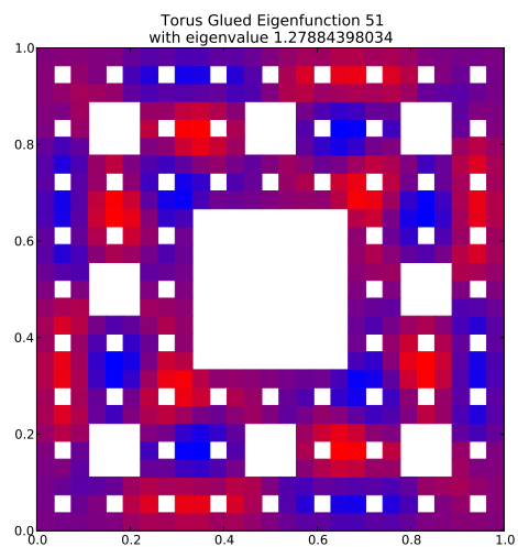
Eigenfunction 51 with eigenvalue 1.27884398034
