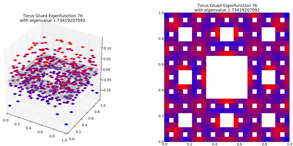
Eigenfunction 76 with eigenvalue 1.73419207092
