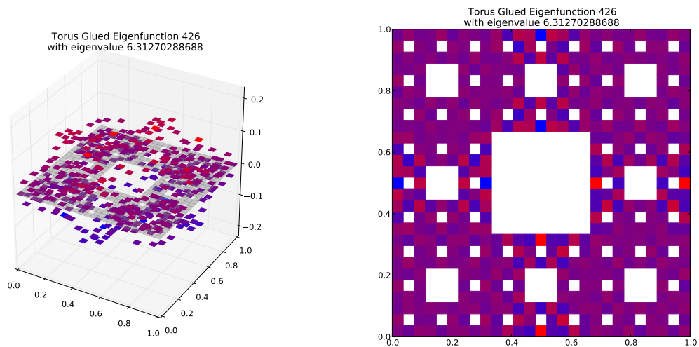
Eigenfunction 426 with eigenvalue 6.31270288688
