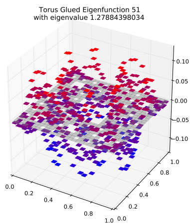
Eigenfunction 51 with eigenvalue 1.27884398034
