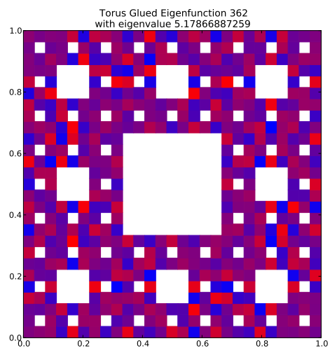
Eigenfunction 362 with eigenvalue 5.17866887259
