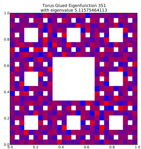
Eigenfunction 351 with eigenvalue 5.11575464113
