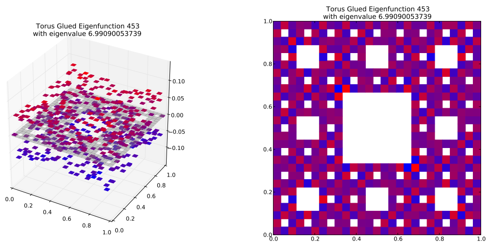
Eigenfunction 453 with eigenvalue 6.99090053739
