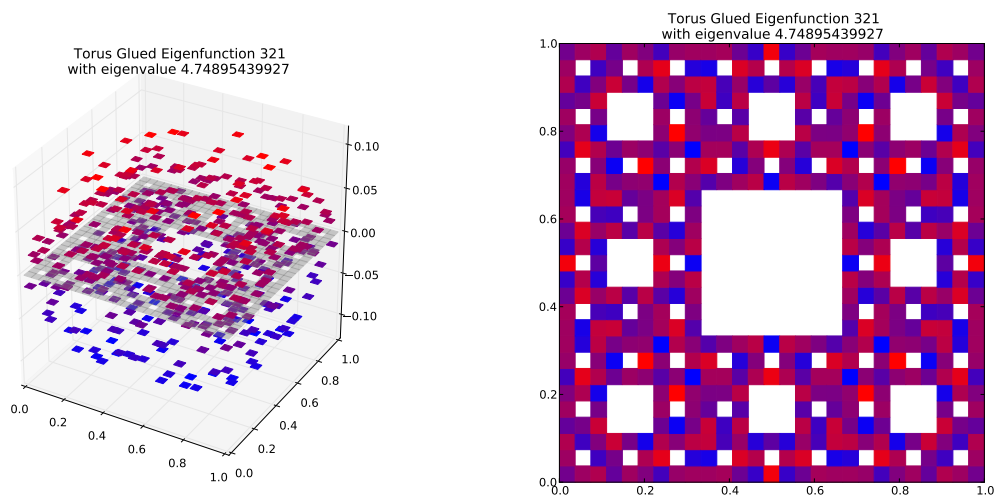
Eigenfunction 321 with eigenvalue 4.74895439927
