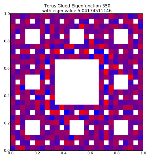
Eigenfunction 350 with eigenvalue 5.04174511146
