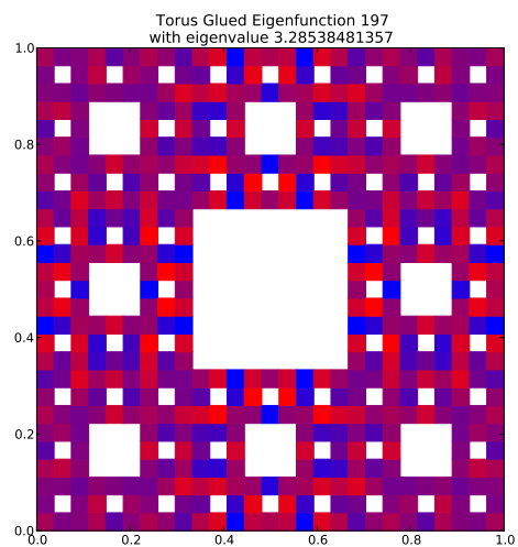
Eigenfunction 197 with eigenvalue 3.28538481357
