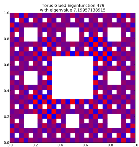
Eigenfunction 479 with eigenvalue 7.19957138915
