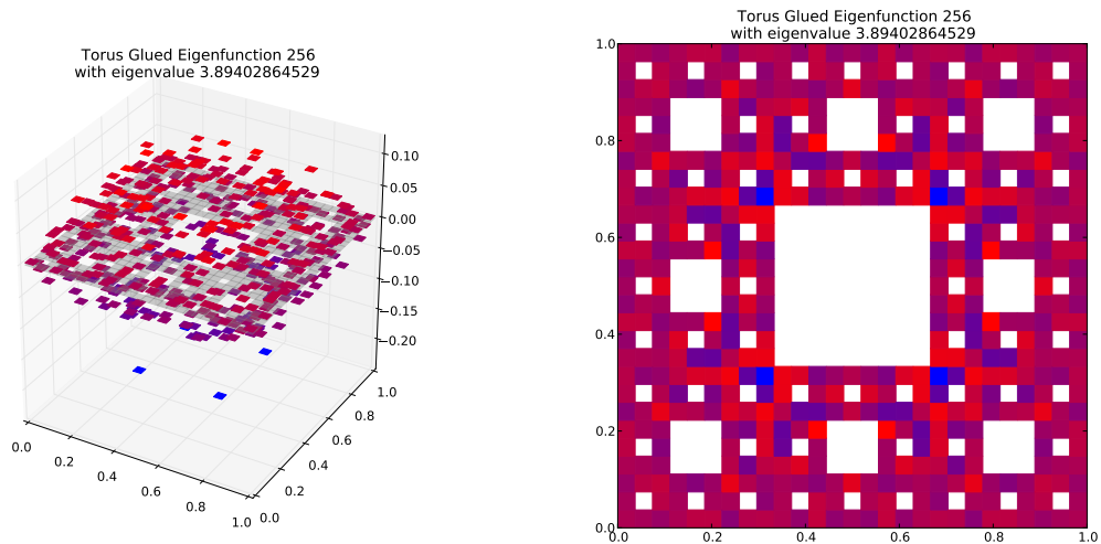
Eigenfunction 256 with eigenvalue 3.89402864529
