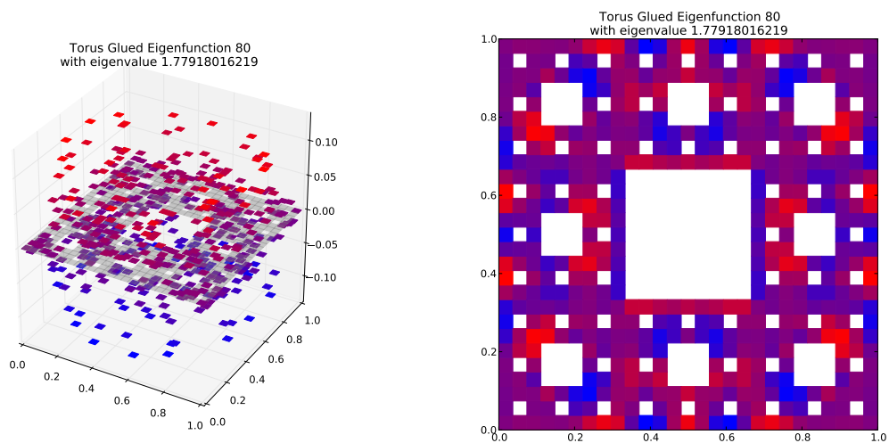
Eigenfunction 80 with eigenvalue 1.77918016219
