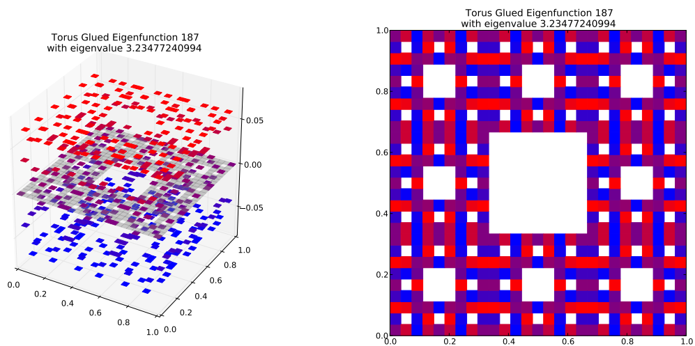
Eigenfunction 187 with eigenvalue 3.23477240994
