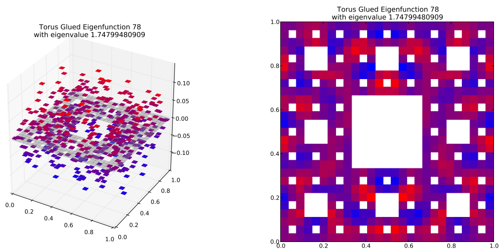
Eigenfunction 78 with eigenvalue 1.74799480909
