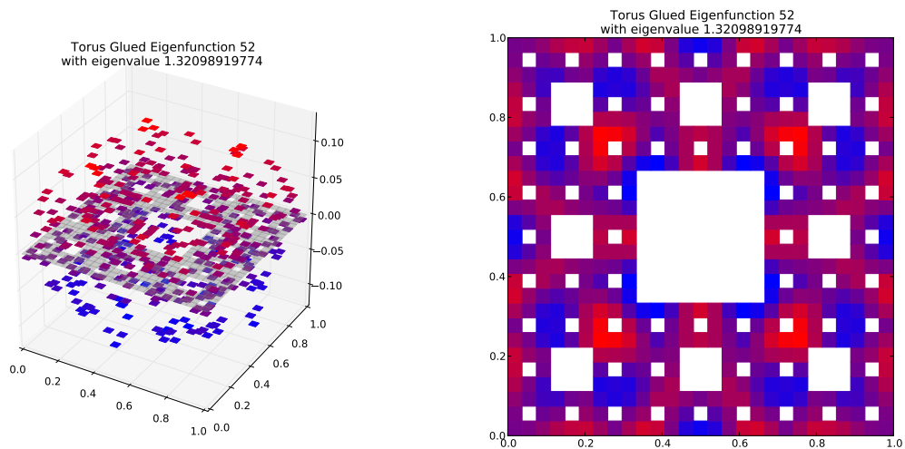
Eigenfunction 52 with eigenvalue 1.32098919774
