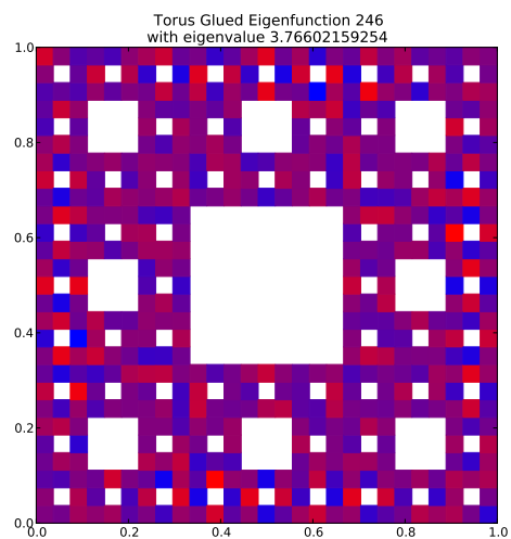
Eigenfunction 246 with eigenvalue 3.76602159254
