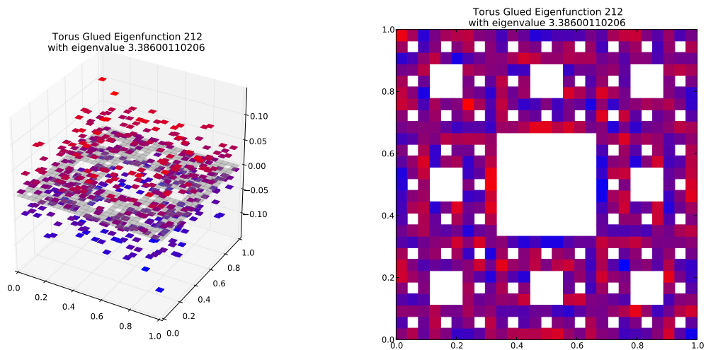
Eigenfunction 212 with eigenvalue 3.38600110206
