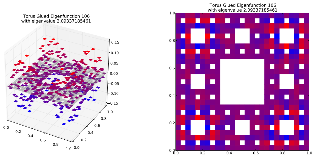
Eigenfunction 106 with eigenvalue 2.09337185461
