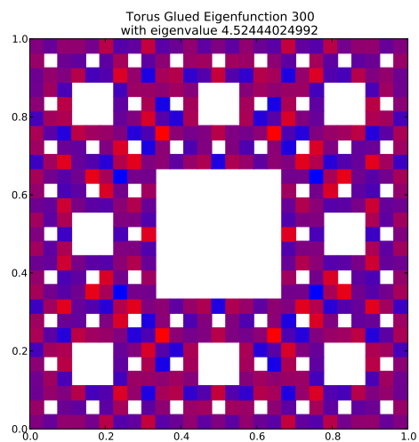
Eigenfunction 300 with eigenvalue 4.52444024992
