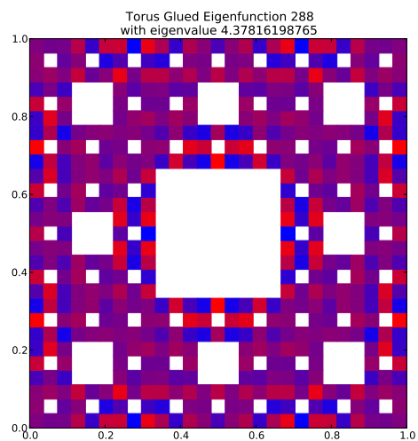
Eigenfunction 288 with eigenvalue 4.37816198765
