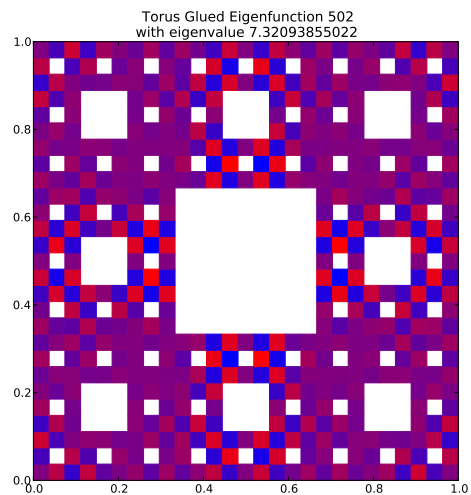
Eigenfunction 502 with eigenvalue 7.32093855022
