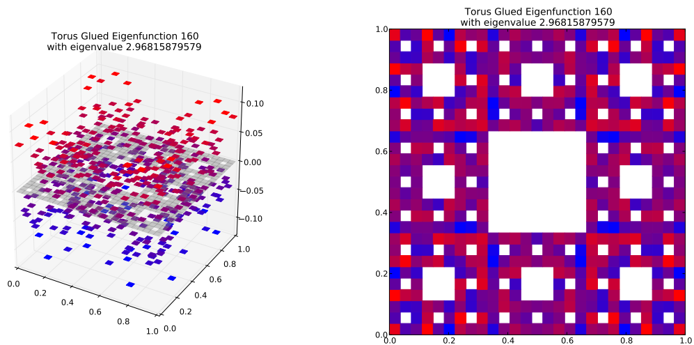
Eigenfunction 160 with eigenvalue 2.96815879579
