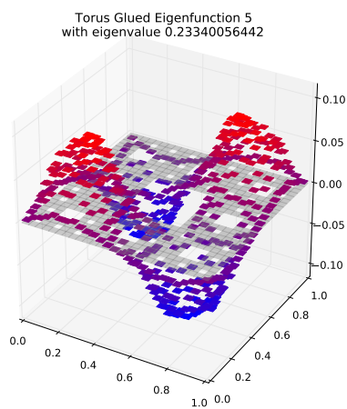
Eigenfunction 5 with eigenvalue 0.23340056442
