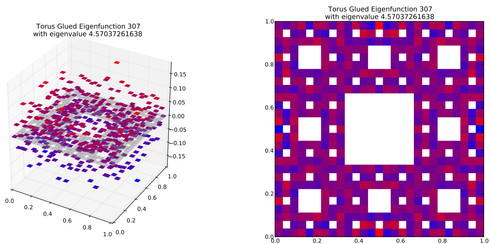
Eigenfunction 307 with eigenvalue 4.57037261638
