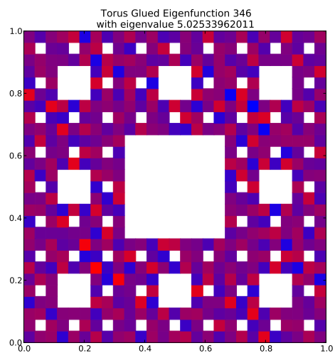
Eigenfunction 346 with eigenvalue 5.02533962011
