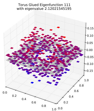
Eigenfunction 111 with eigenvalue 2.12021545195
