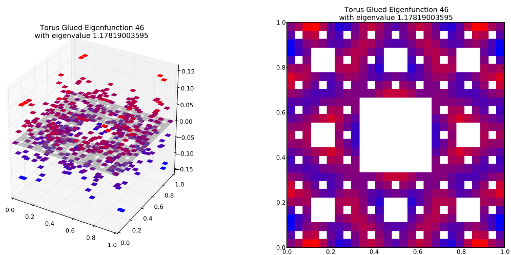
Eigenfunction 46 with eigenvalue 1.17819003595
