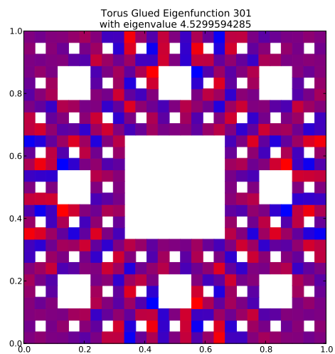
Eigenfunction 301 with eigenvalue 4.5299594285
