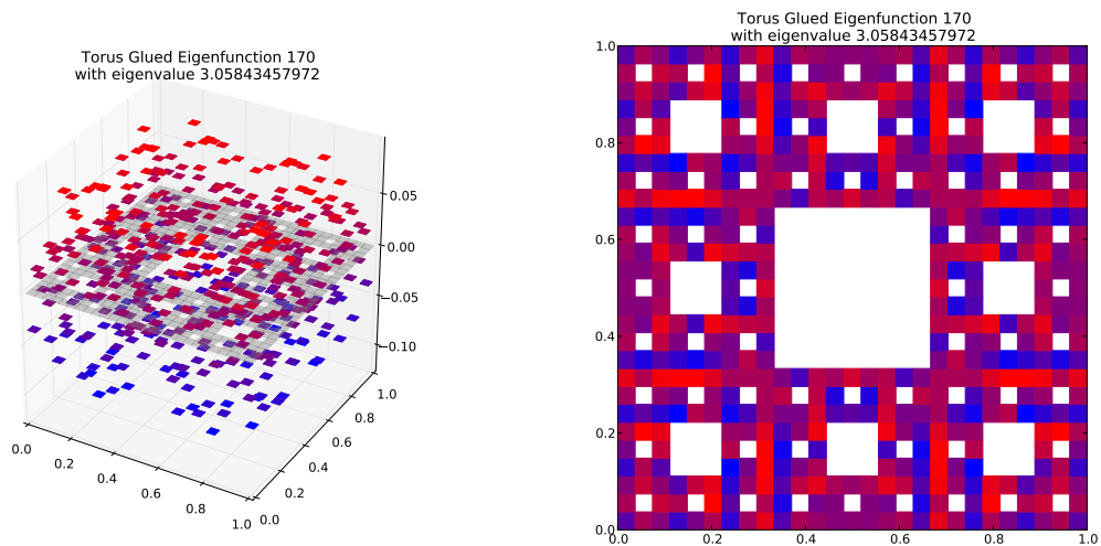
Eigenfunction 170 with eigenvalue 3.05843457972
