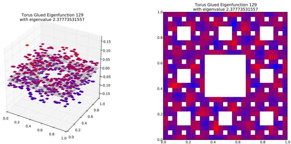
Eigenfunction 129 with eigenvalue 2.37773531557
