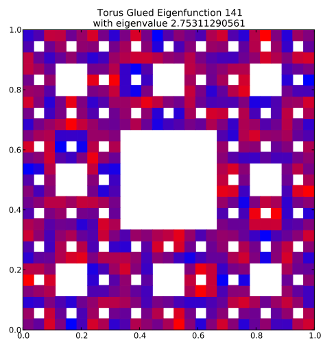
Eigenfunction 141 with eigenvalue 2.75311290561
