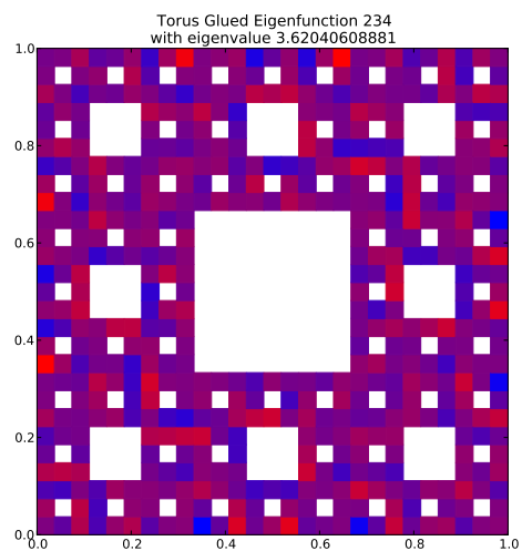
Eigenfunction 234 with eigenvalue 3.62040608881
