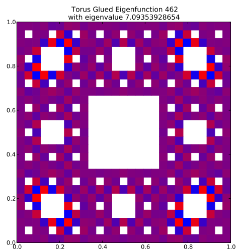
Eigenfunction 462 with eigenvalue 7.09353928654
