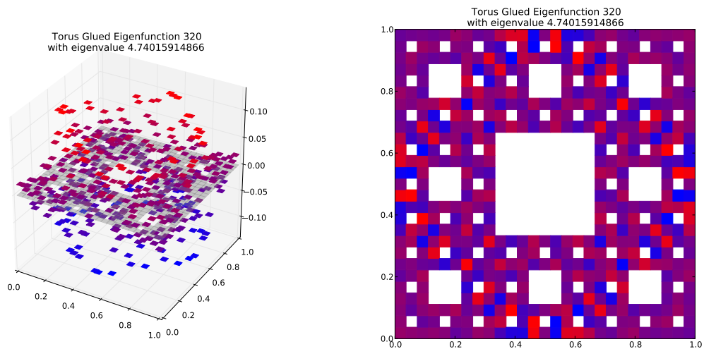
Eigenfunction 320 with eigenvalue 4.74015914866
