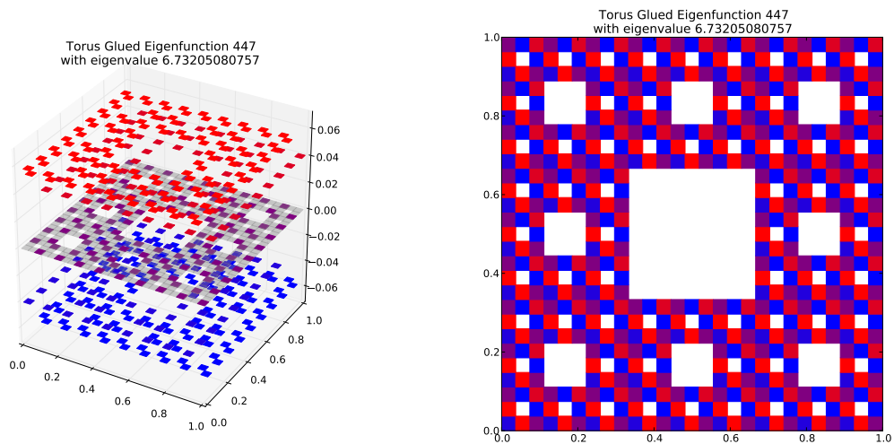
Eigenfunction 447 with eigenvalue 6.73205080757
