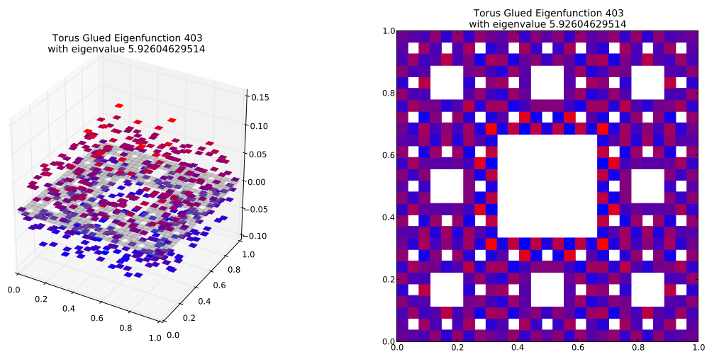
Eigenfunction 403 with eigenvalue 5.92604629514
