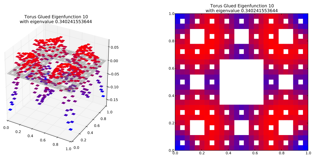
Eigenfunction 10 with eigenvalue 0.340241553644
