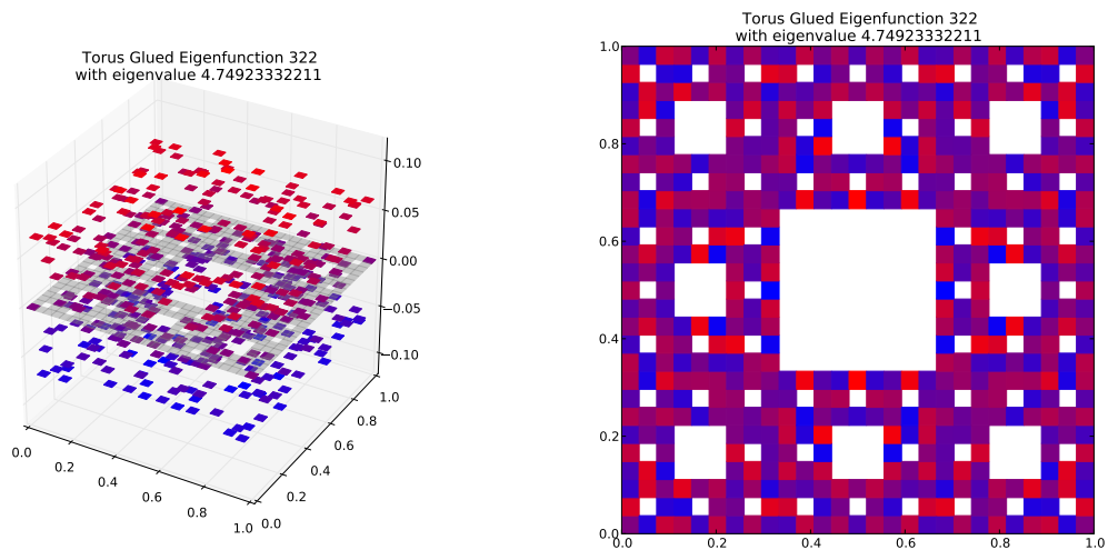
Eigenfunction 322 with eigenvalue 4.74923332211
