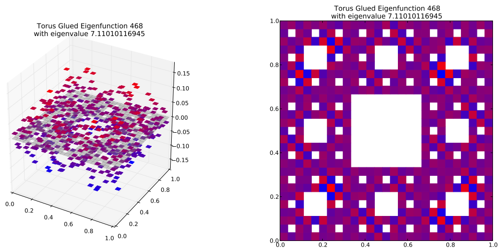
Eigenfunction 468 with eigenvalue 7.11010116945
