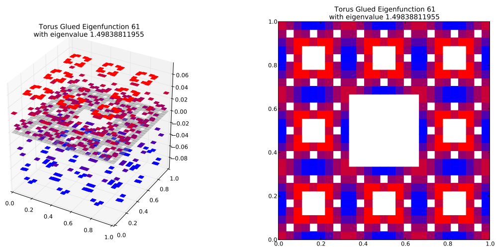
Eigenfunction 61 with eigenvalue 1.49838811955
