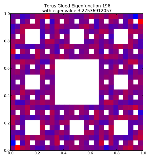
Eigenfunction 196 with eigenvalue 3.27536912057
