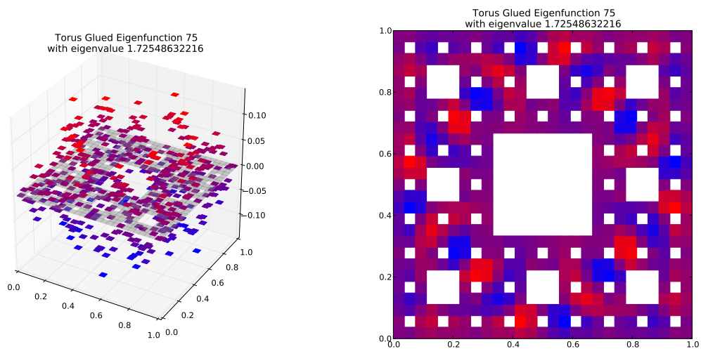
Eigenfunction 75 with eigenvalue 1.72548632216
