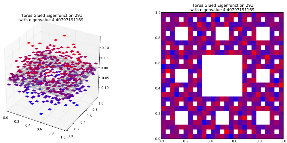
Eigenfunction 291 with eigenvalue 4.40797191169
