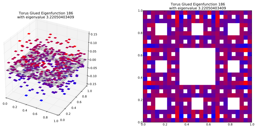
Eigenfunction 186 with eigenvalue 3.22050403409
