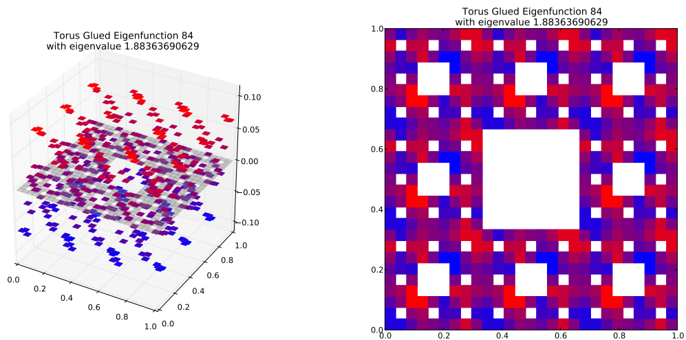
Eigenfunction 84 with eigenvalue 1.88363690629
