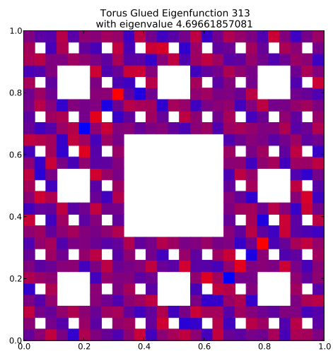
Eigenfunction 313 with eigenvalue 4.69661857081
