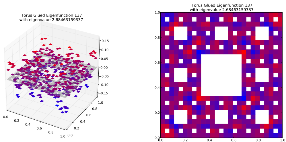
Eigenfunction 137 with eigenvalue 2.68463159337
