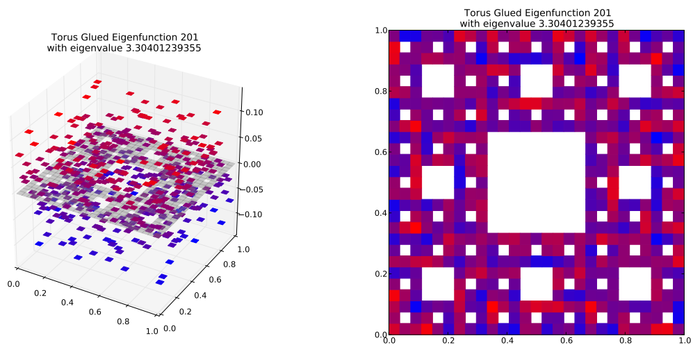
Eigenfunction 201 with eigenvalue 3.30401239355
