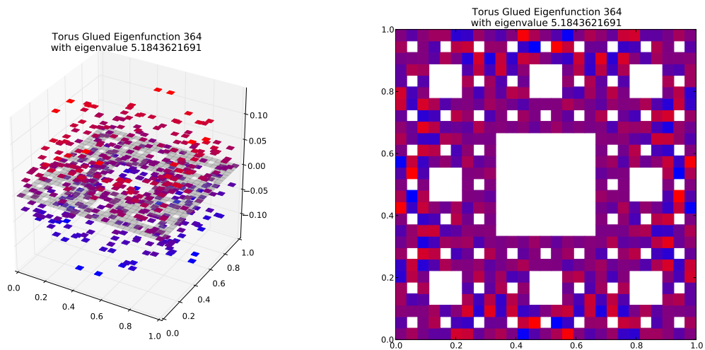
Eigenfunction 364 with eigenvalue 5.1843621691
