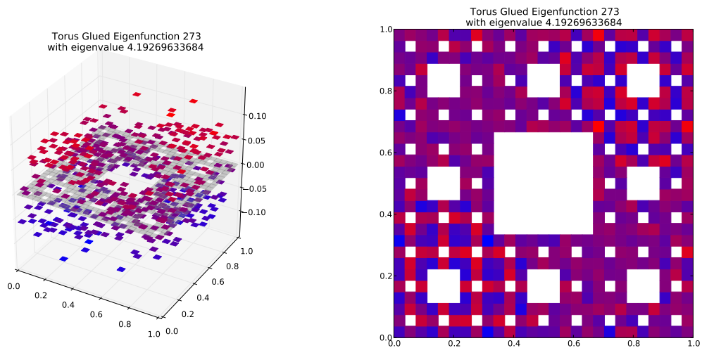
Eigenfunction 273 with eigenvalue 4.19269633684
