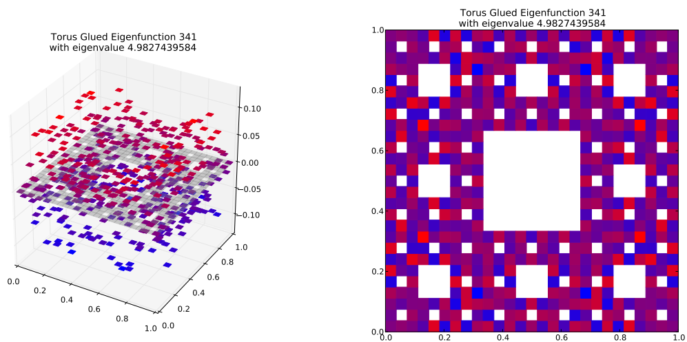
Eigenfunction 341 with eigenvalue 4.9827439584
