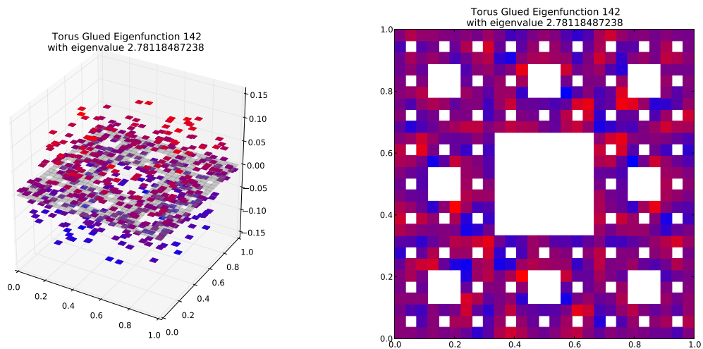
Eigenfunction 142 with eigenvalue 2.78118487238
