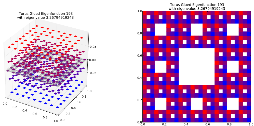
Eigenfunction 193 with eigenvalue 3.26794919243
