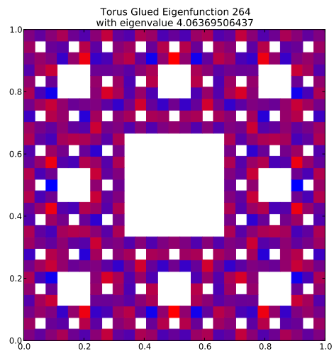
Eigenfunction 264 with eigenvalue 4.06369506437
