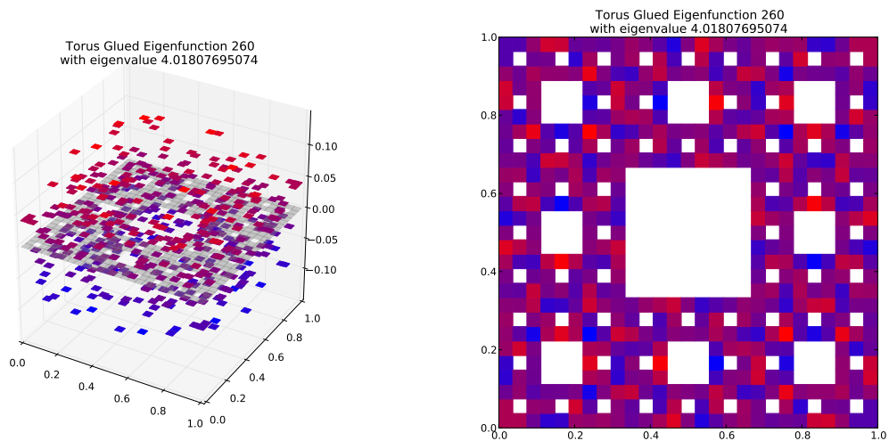
Eigenfunction 260 with eigenvalue 4.01807695074
