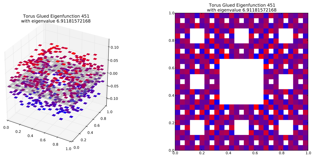
Eigenfunction 451 with eigenvalue 6.91181572168
