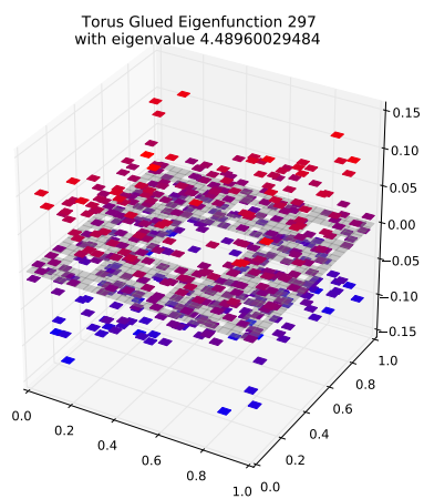
Eigenfunction 297 with eigenvalue 4.48960029484
