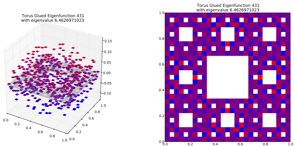
Eigenfunction 431 with eigenvalue 6.4626971023
