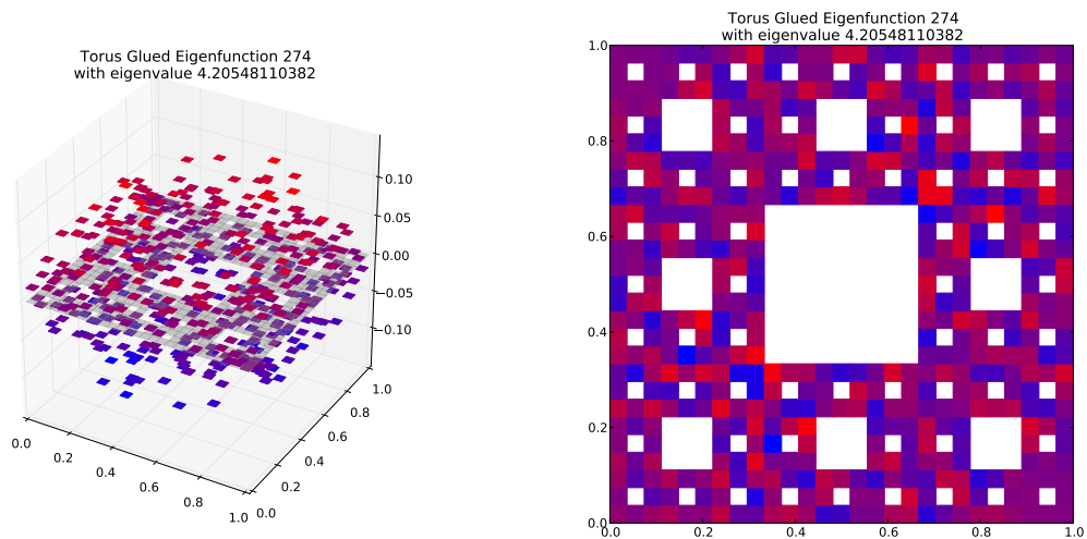
Eigenfunction 274 with eigenvalue 4.20548110382
