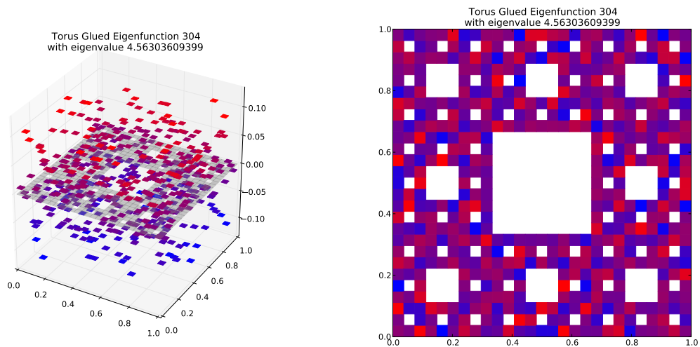
Eigenfunction 304 with eigenvalue 4.56303609399
