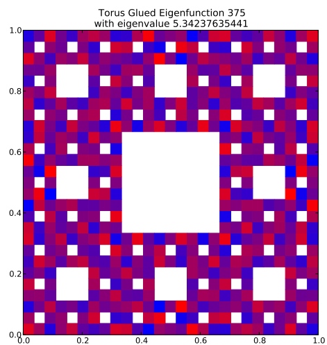
Eigenfunction 375 with eigenvalue 5.34237635441
