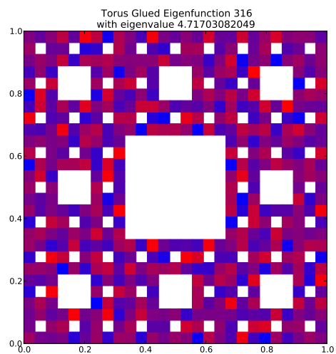
Eigenfunction 316 with eigenvalue 4.71703082049
