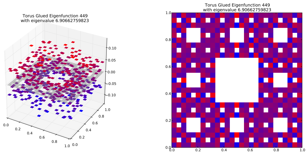
Eigenfunction 449 with eigenvalue 6.90662759823
