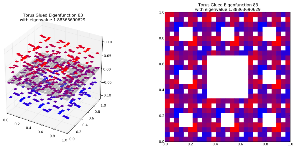
Eigenfunction 83 with eigenvalue 1.88363690629
