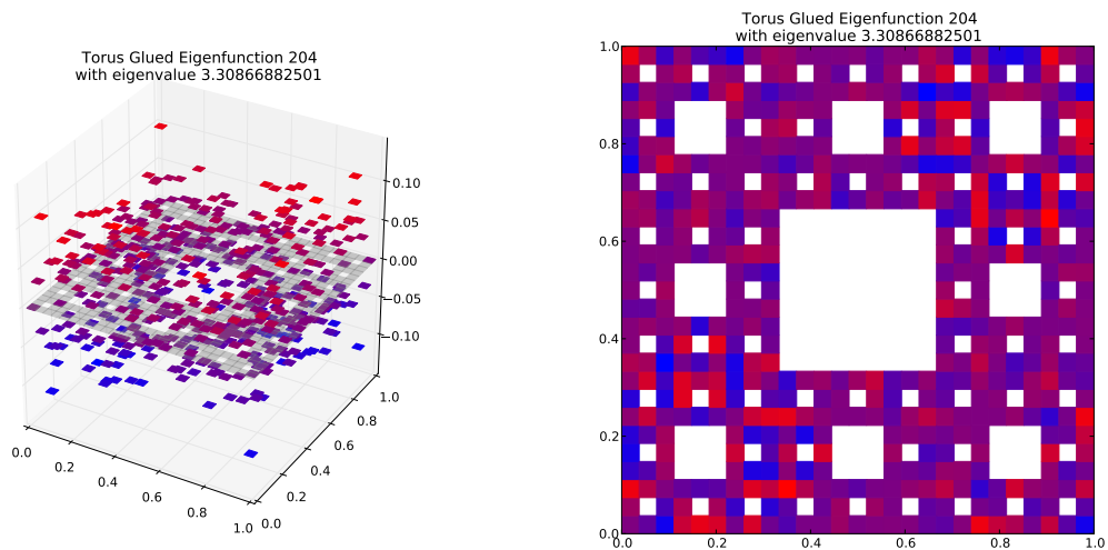
Eigenfunction 204 with eigenvalue 3.30866882501
