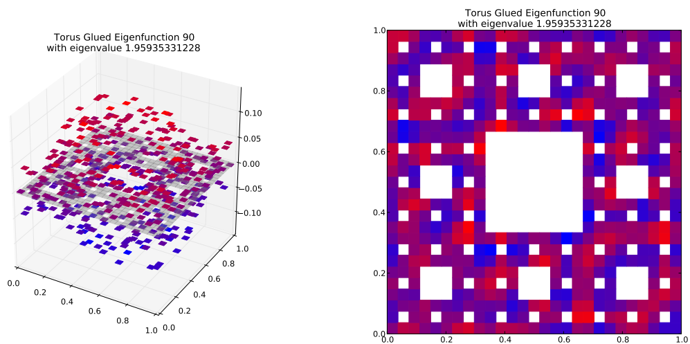
Eigenfunction 90 with eigenvalue 1.95935331228
