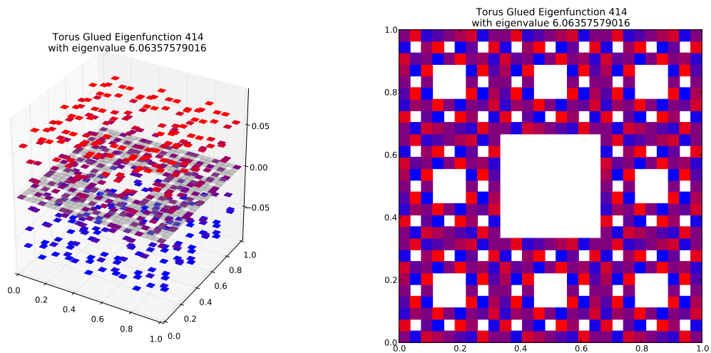
Eigenfunction 414 with eigenvalue 6.06357579016
