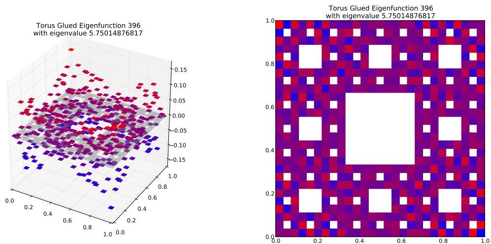
Eigenfunction 396 with eigenvalue 5.75014876817
