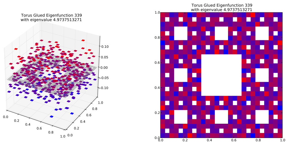
Eigenfunction 339 with eigenvalue 4.9737513271
