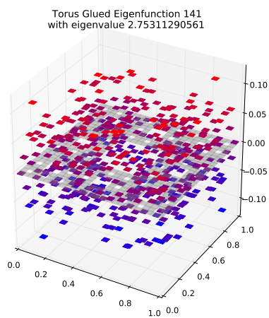
Eigenfunction 141 with eigenvalue 2.75311290561
