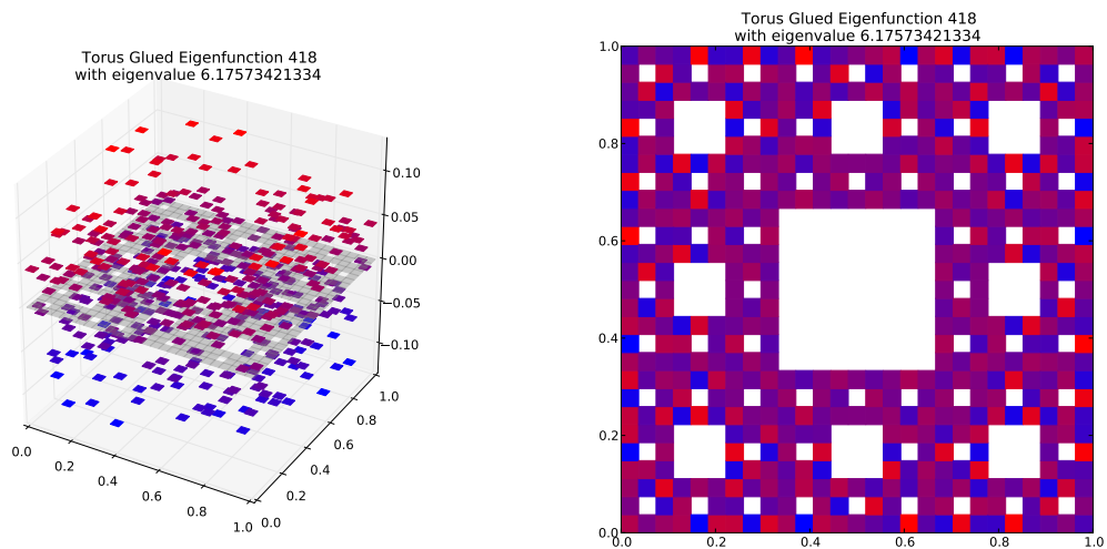
Eigenfunction 418 with eigenvalue 6.17573421334
