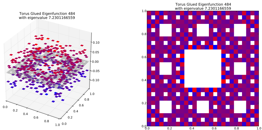
Eigenfunction 484 with eigenvalue 7.2301166559
