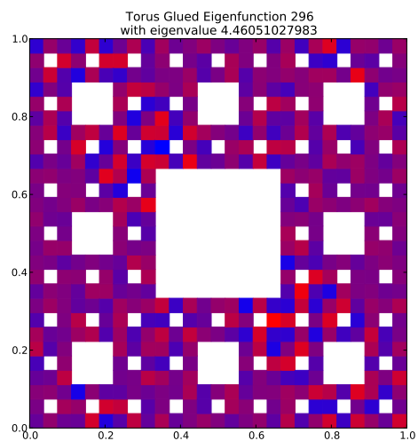
Eigenfunction 296 with eigenvalue 4.46051027983
