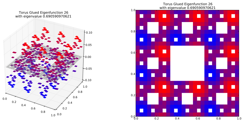
Eigenfunction 26 with eigenvalue 0.690590970621
