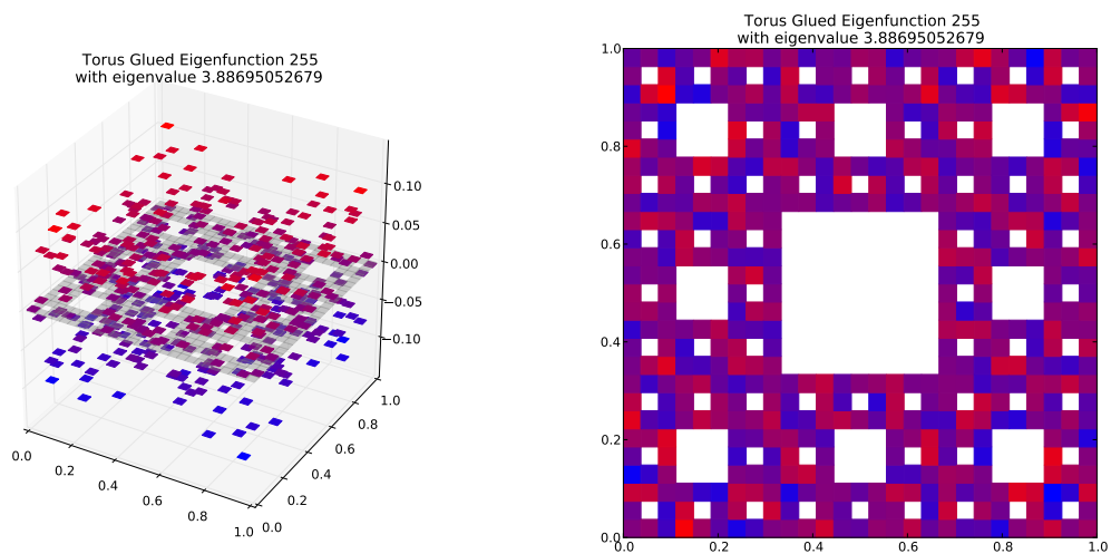
Eigenfunction 255 with eigenvalue 3.88695052679
