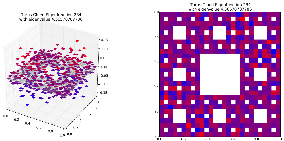
Eigenfunction 284 with eigenvalue 4.36578787786
