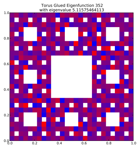
Eigenfunction 352 with eigenvalue 5.11575464113
