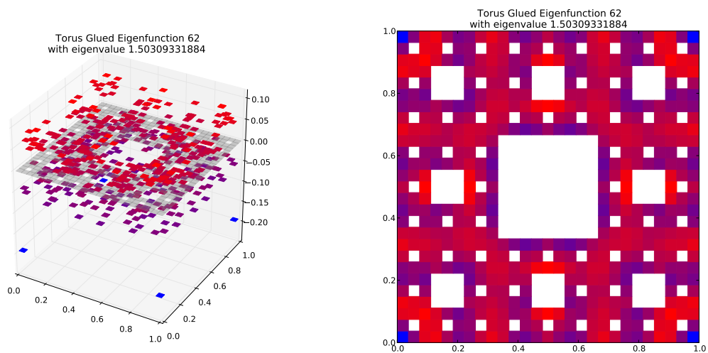
Eigenfunction 62 with eigenvalue 1.50309331884
