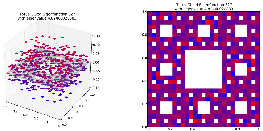
Eigenfunction 327 with eigenvalue 4.82460020883
