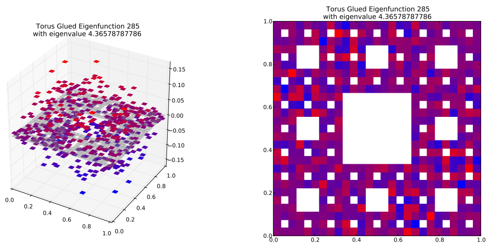
Eigenfunction 285 with eigenvalue 4.36578787786
