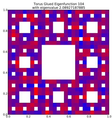
Eigenfunction 104 with eigenvalue 2.08927187885
