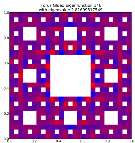
Eigenfunction 146 with eigenvalue 2.81699517549
