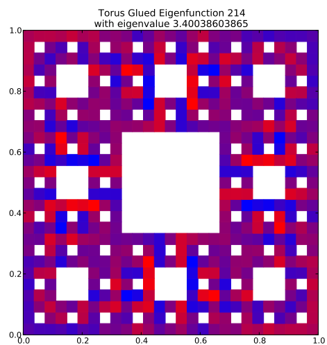
Eigenfunction 214 with eigenvalue 3.40038603865
