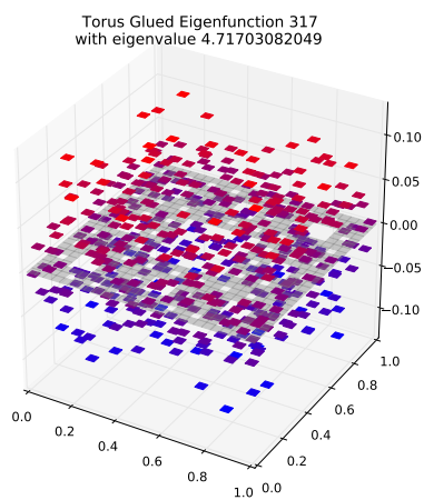
Eigenfunction 317 with eigenvalue 4.71703082049
