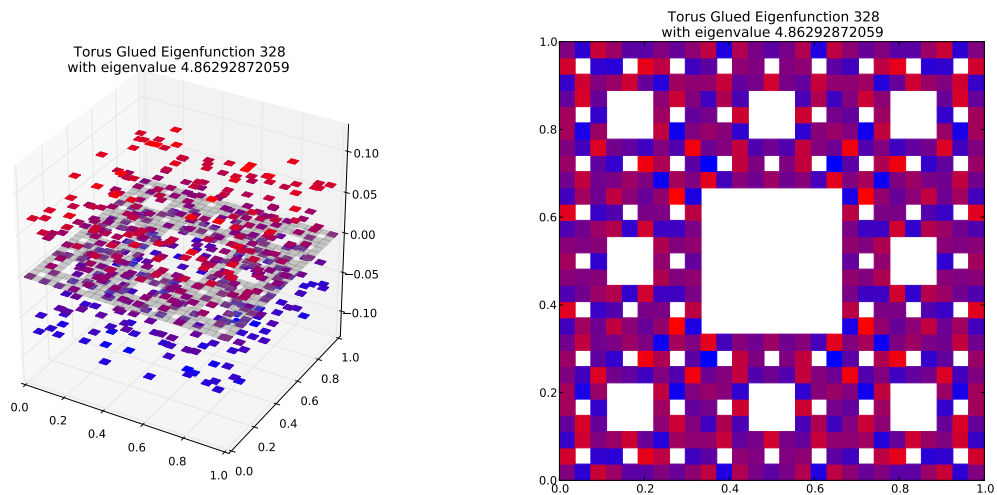
Eigenfunction 328 with eigenvalue 4.86292872059
