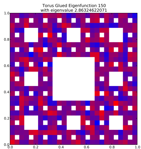
Eigenfunction 150 with eigenvalue 2.86324622071
