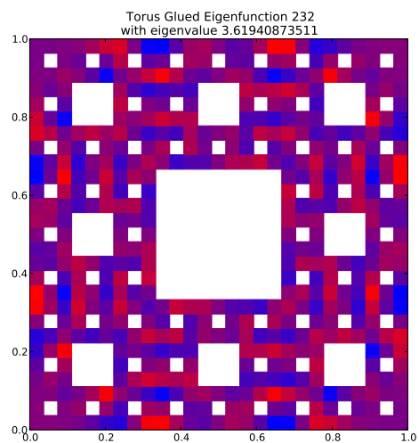
Eigenfunction 232 with eigenvalue 3.61940873511
