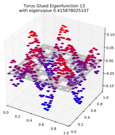
Eigenfunction 13 with eigenvalue 0.415878025107
