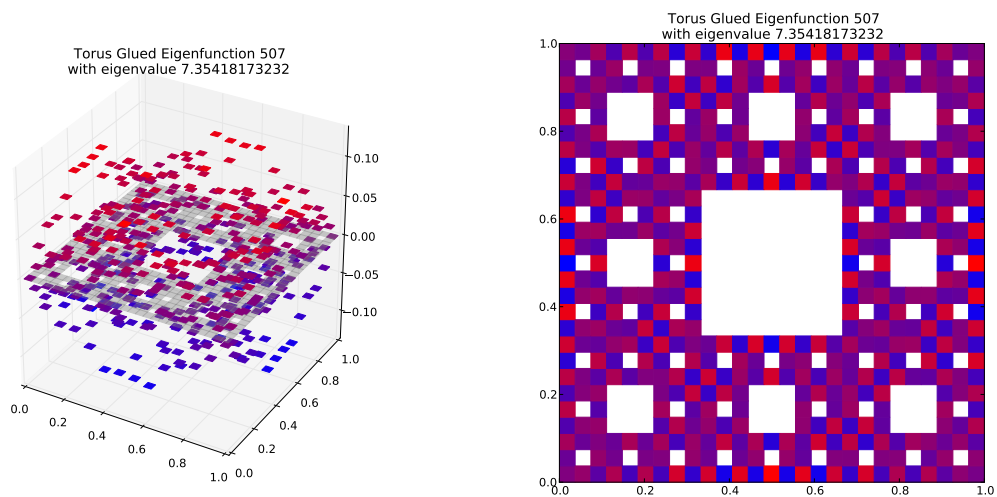
Eigenfunction 507 with eigenvalue 7.35418173232
