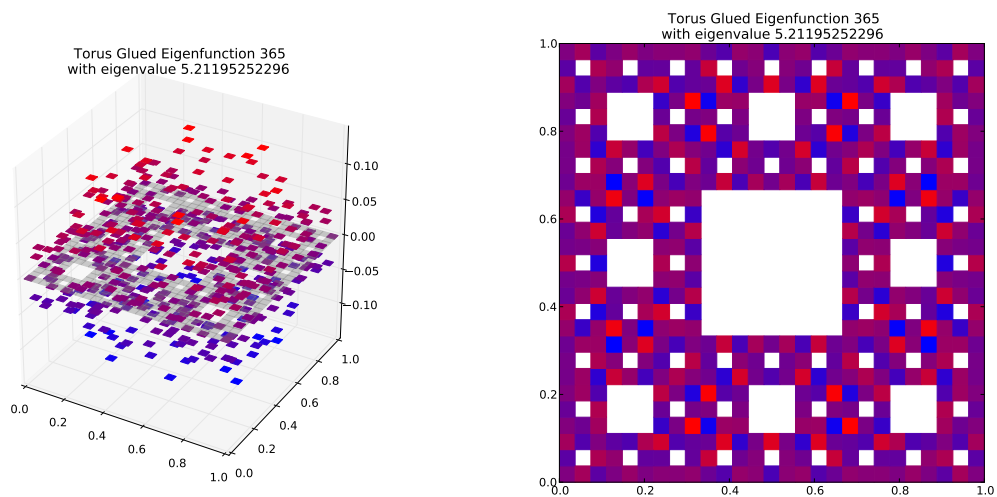
Eigenfunction 365 with eigenvalue 5.21195252296
