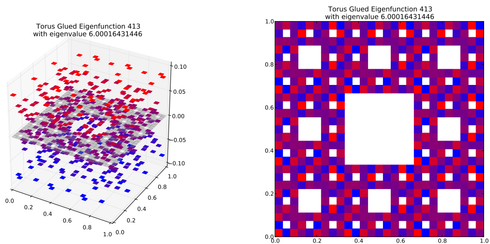
Eigenfunction 413 with eigenvalue 6.00016431446
