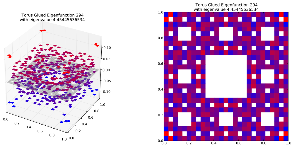
Eigenfunction 294 with eigenvalue 4.45445636534
