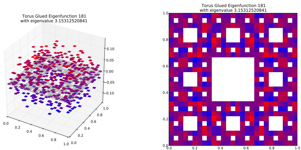
Eigenfunction 181 with eigenvalue 3.15312520841
