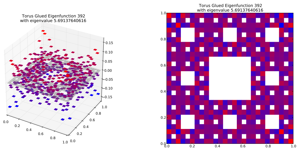
Eigenfunction 392 with eigenvalue 5.69137640616
