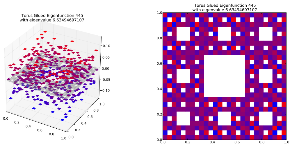
Eigenfunction 445 with eigenvalue 6.63494697107
