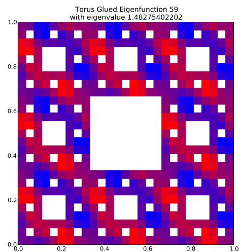
Eigenfunction 59 with eigenvalue 1.48275402202
