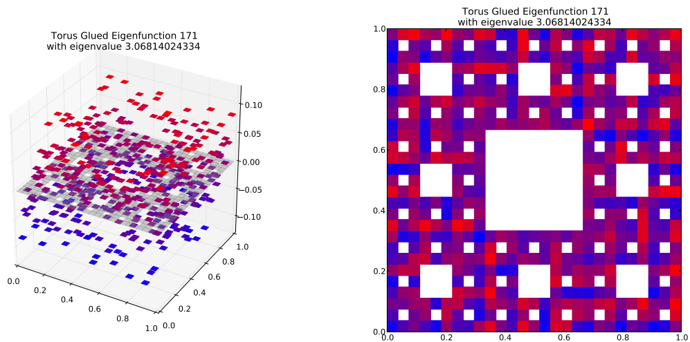
Eigenfunction 171 with eigenvalue 3.06814024334
