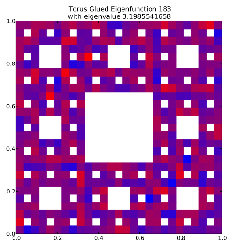
Eigenfunction 183 with eigenvalue 3.1985541658
