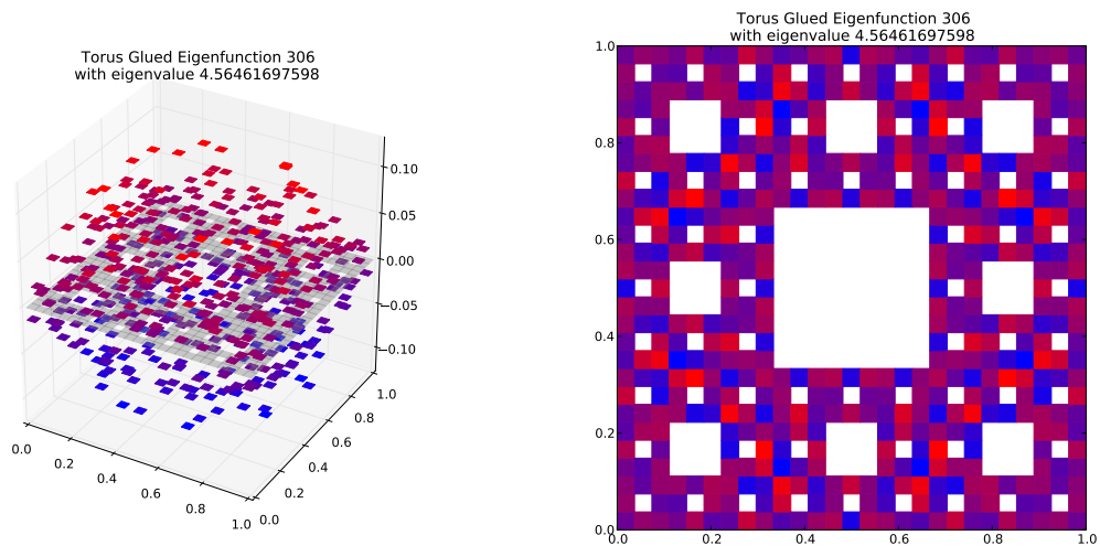
Eigenfunction 306 with eigenvalue 4.56461697598
