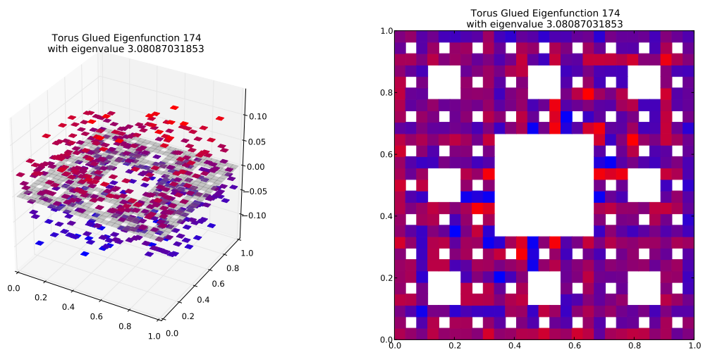
Eigenfunction 174 with eigenvalue 3.08087031853
