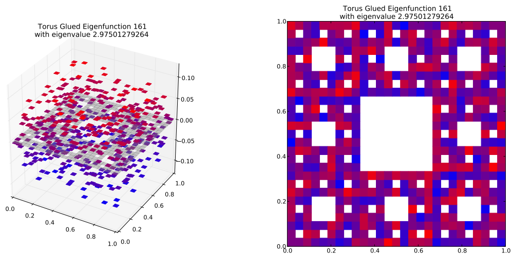
Eigenfunction 161 with eigenvalue 2.97501279264
