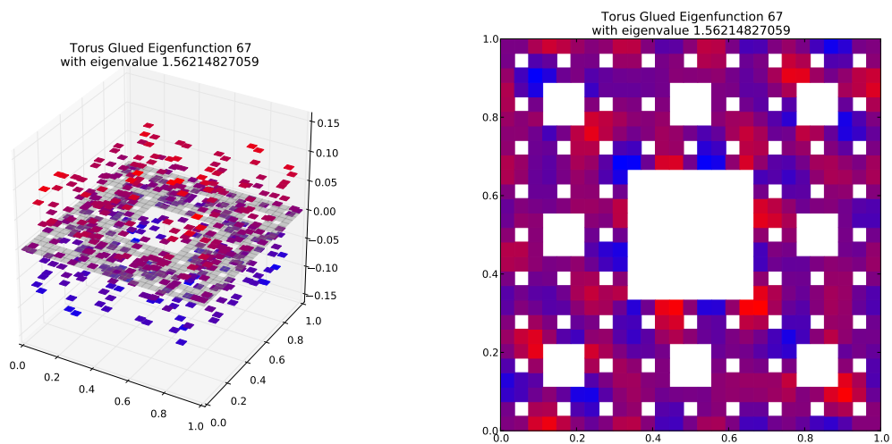
Eigenfunction 67 with eigenvalue 1.56214827059
