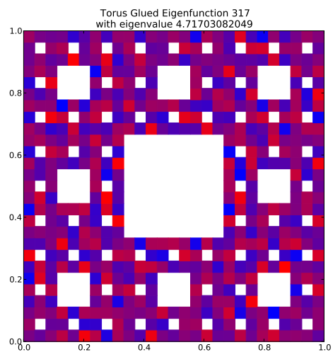
Eigenfunction 317 with eigenvalue 4.71703082049
