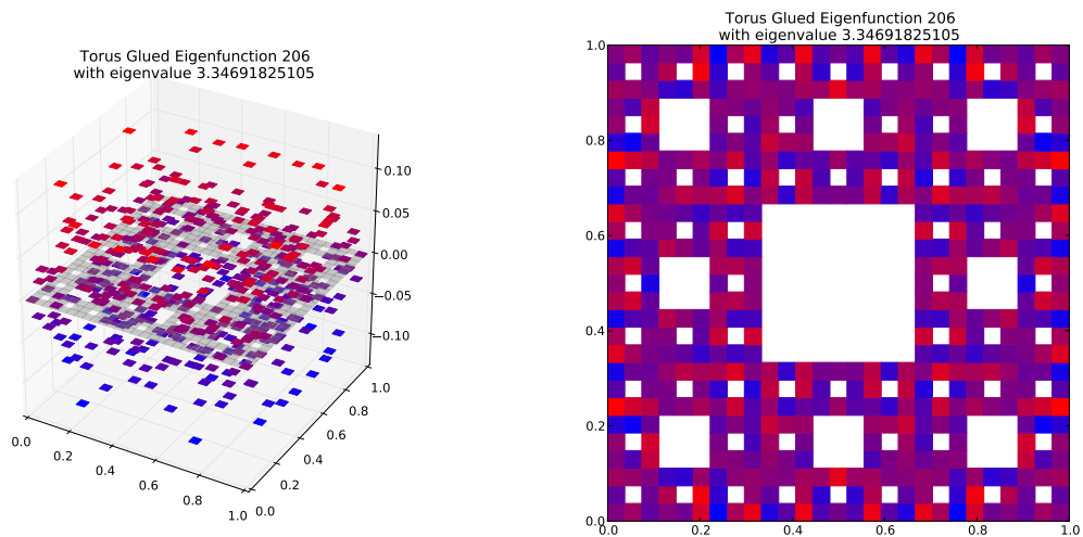
Eigenfunction 206 with eigenvalue 3.34691825105
