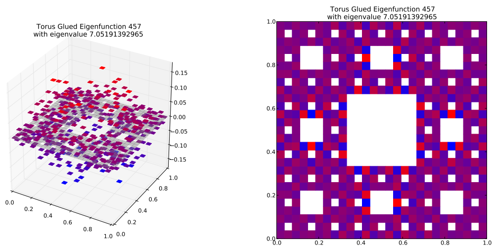
Eigenfunction 457 with eigenvalue 7.05191392965
