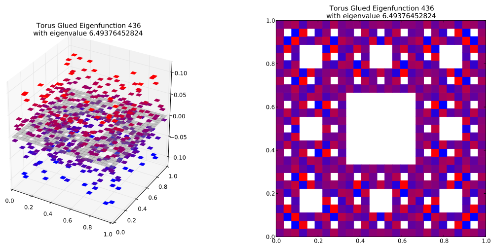
Eigenfunction 436 with eigenvalue 6.49376452824
