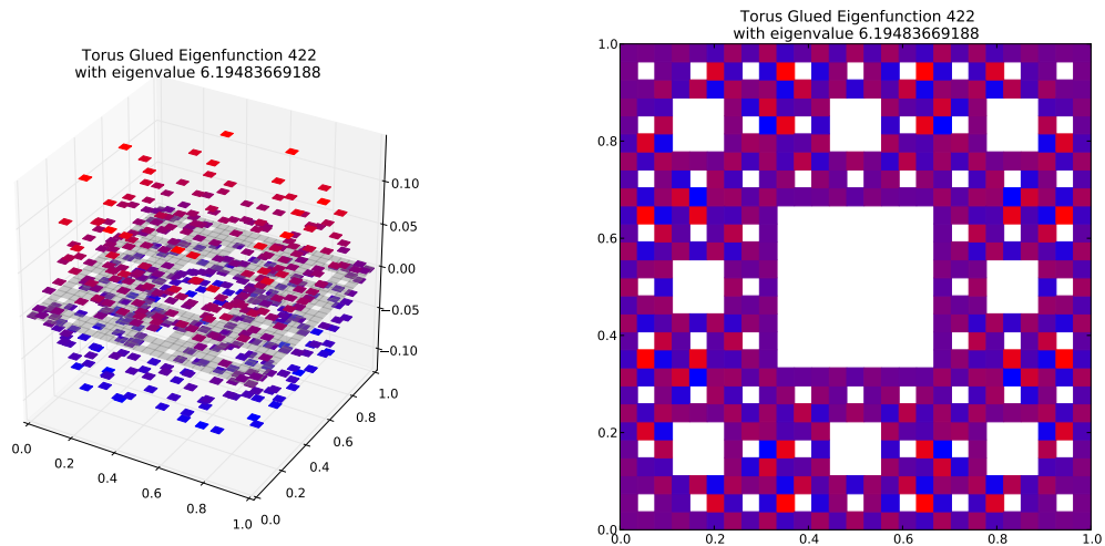
Eigenfunction 422 with eigenvalue 6.19483669188
