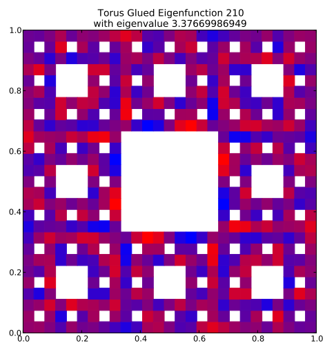
Eigenfunction 210 with eigenvalue 3.37669986949
