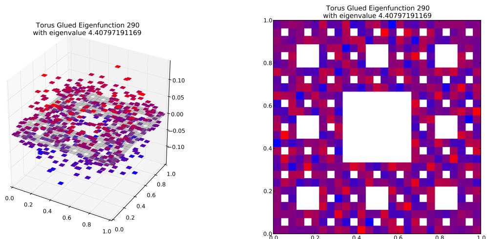
Eigenfunction 290 with eigenvalue 4.40797191169
