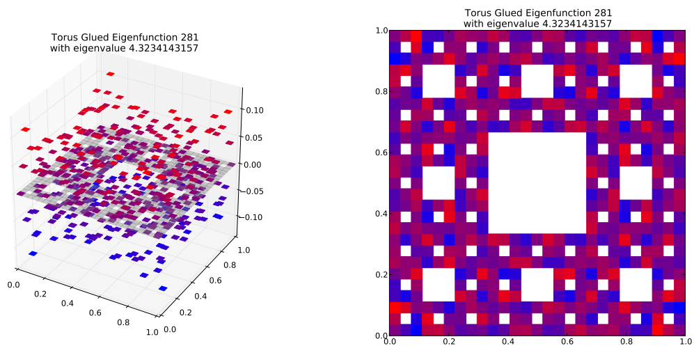
Eigenfunction 281 with eigenvalue 4.3234143157
