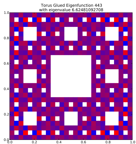
Eigenfunction 443 with eigenvalue 6.62481092708
