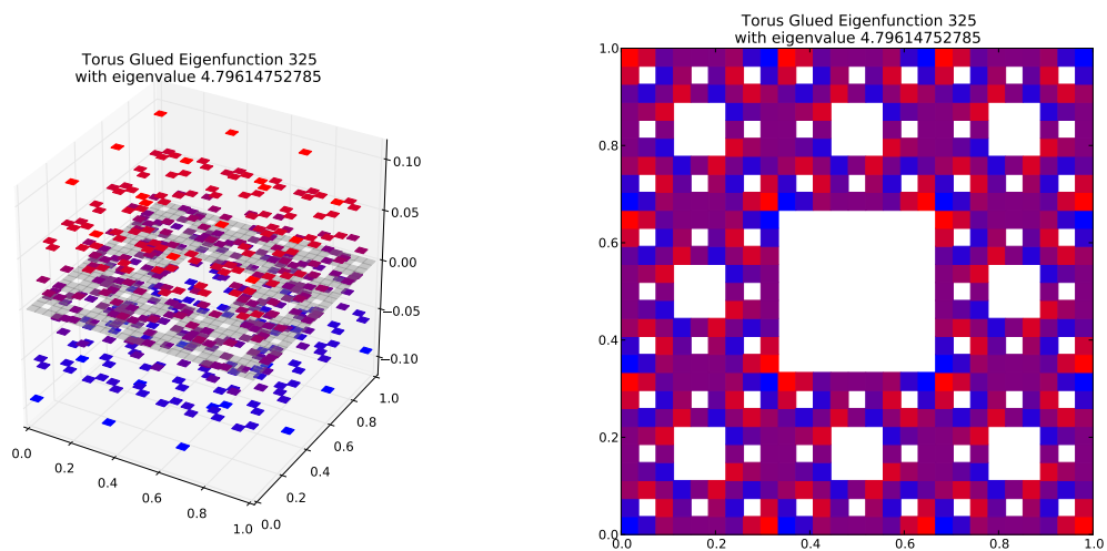
Eigenfunction 325 with eigenvalue 4.79614752785
