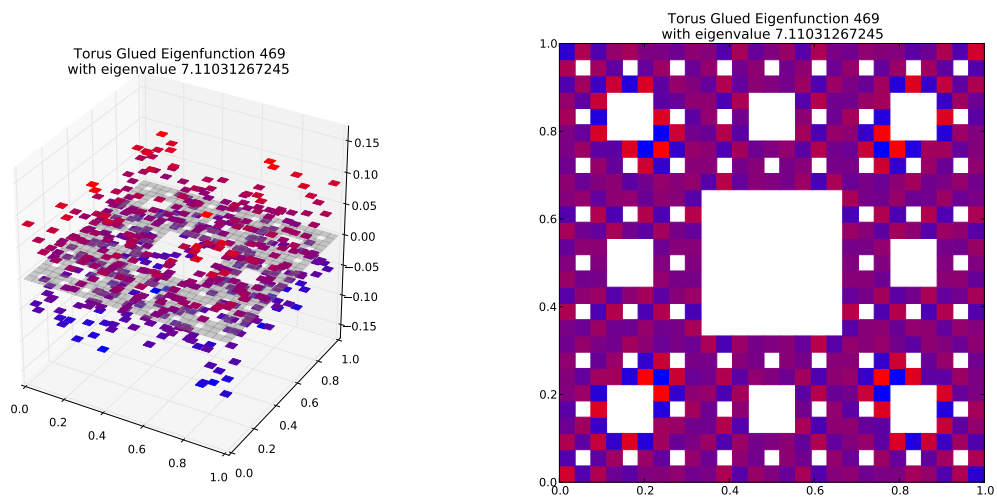
Eigenfunction 469 with eigenvalue 7.11031267245
