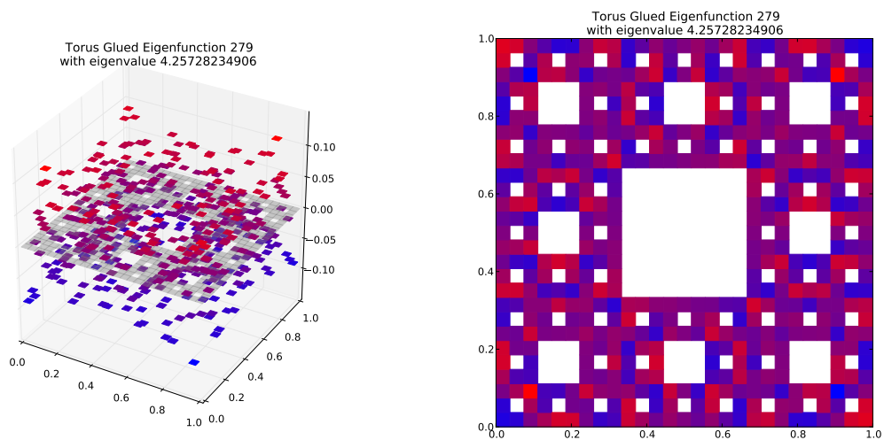
Eigenfunction 279 with eigenvalue 4.25728234906
