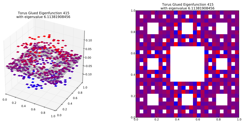
Eigenfunction 415 with eigenvalue 6.11381908456
