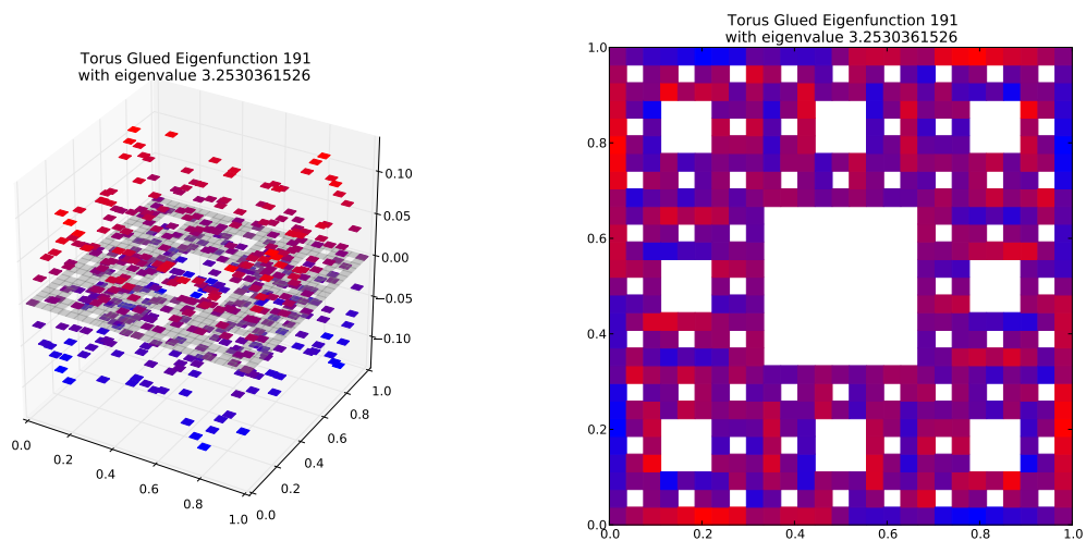
Eigenfunction 191 with eigenvalue 3.2530361526
