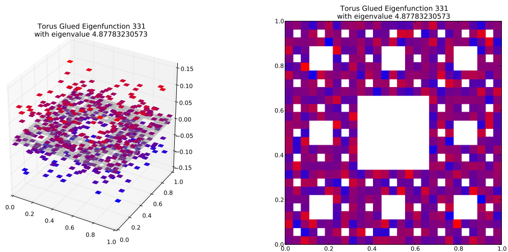
Eigenfunction 331 with eigenvalue 4.87783230573
