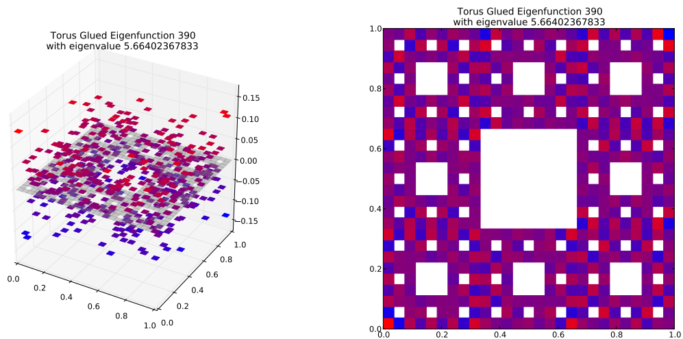
Eigenfunction 390 with eigenvalue 5.66402367833
