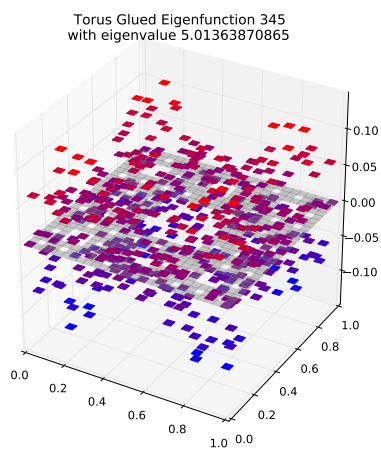
Eigenfunction 345 with eigenvalue 5.01363870865
