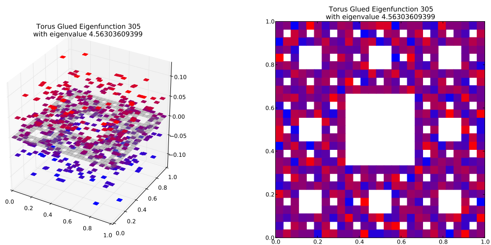
Eigenfunction 305 with eigenvalue 4.56303609399
