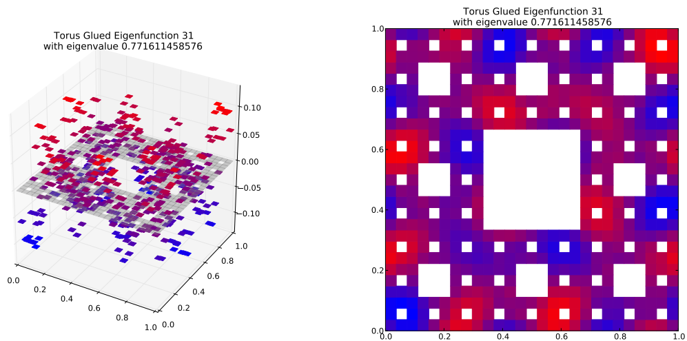
Eigenfunction 31 with eigenvalue 0.771611458576
