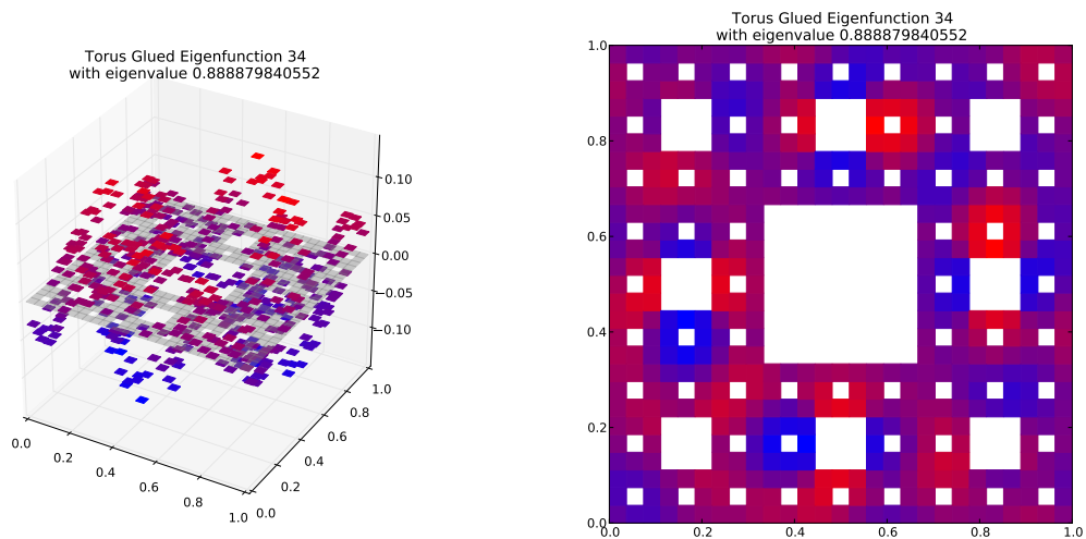
Eigenfunction 34 with eigenvalue 0.888879840552
