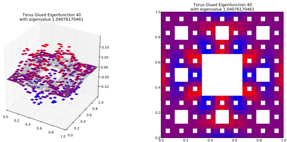
Eigenfunction 40 with eigenvalue 1.04076170461
