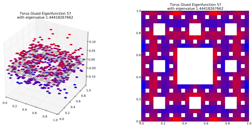
Eigenfunction 57 with eigenvalue 1.44418267662
