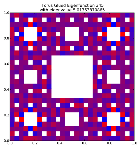
Eigenfunction 345 with eigenvalue 5.01363870865
