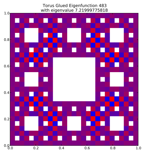
Eigenfunction 483 with eigenvalue 7.21999775818
