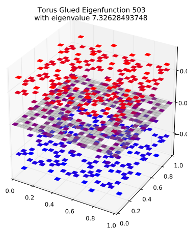
Eigenfunction 503 with eigenvalue 7.32628493748
