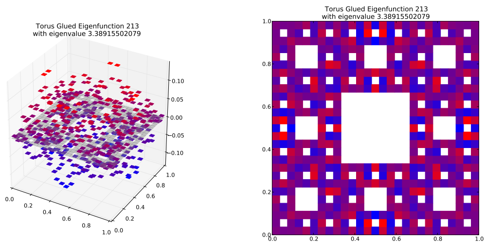
Eigenfunction 213 with eigenvalue 3.38915502079
