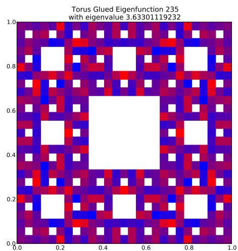
Eigenfunction 235 with eigenvalue 3.63301119232
