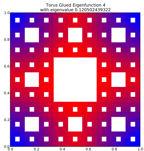
Eigenfunction 4 with eigenvalue 0.120502439322
