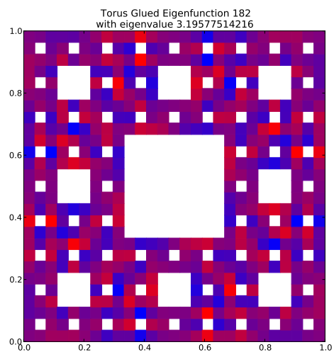
Eigenfunction 182 with eigenvalue 3.19577514216
