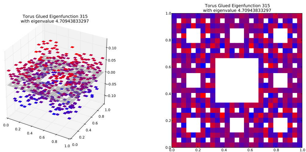
Eigenfunction 315 with eigenvalue 4.70943833297
