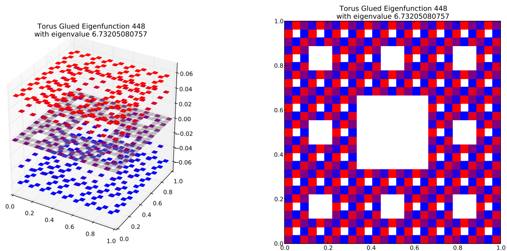
Eigenfunction 448 with eigenvalue 6.73205080757
