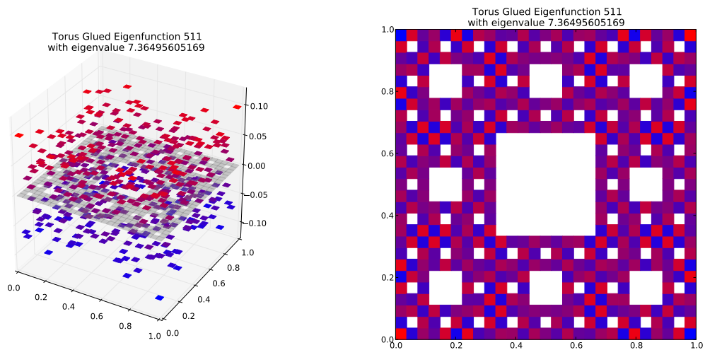
Eigenfunction 511 with eigenvalue 7.36495605169
