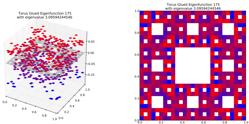
Eigenfunction 175 with eigenvalue 3.09594244546
