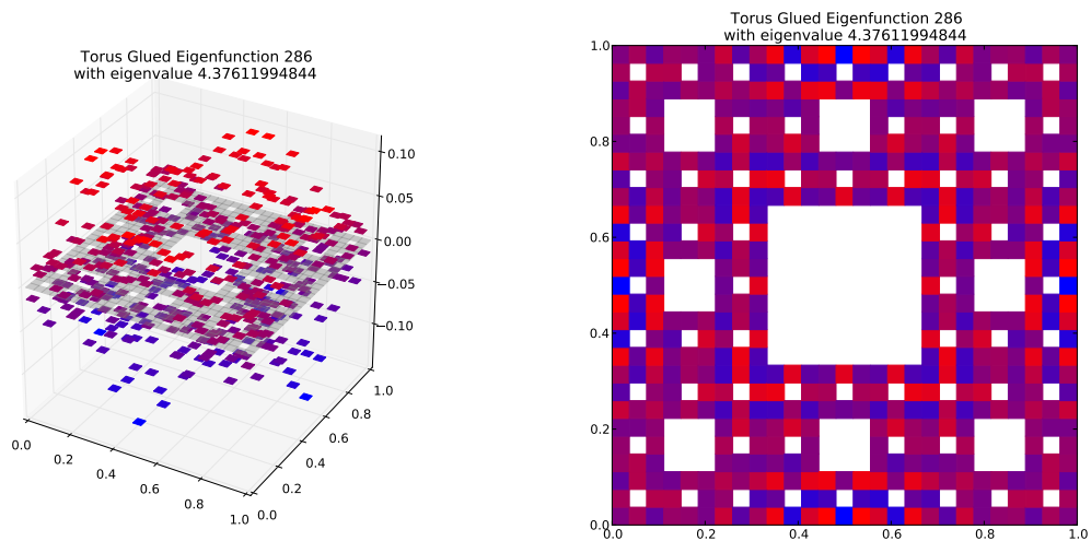
Eigenfunction 286 with eigenvalue 4.37611994844
