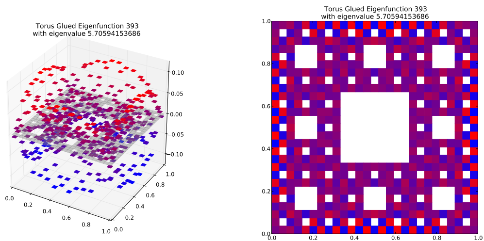
Eigenfunction 393 with eigenvalue 5.70594153686
