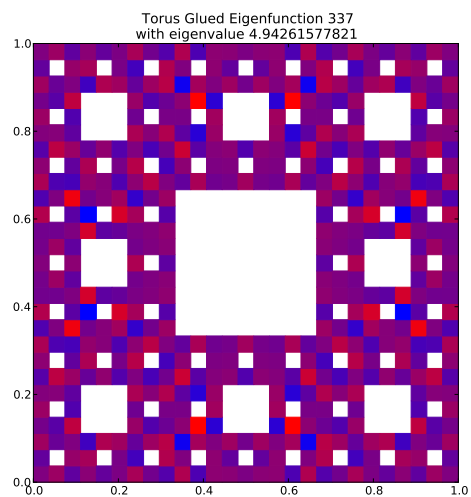
Eigenfunction 337 with eigenvalue 4.94261577821
