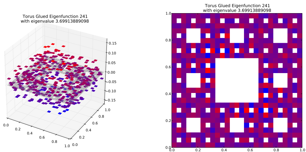
Eigenfunction 241 with eigenvalue 3.69913889098
