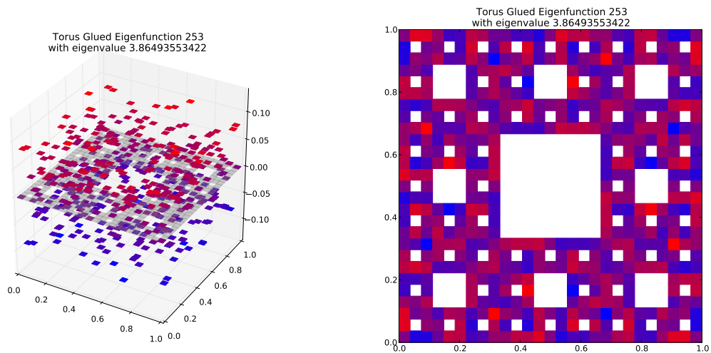
Eigenfunction 253 with eigenvalue 3.86493553422
