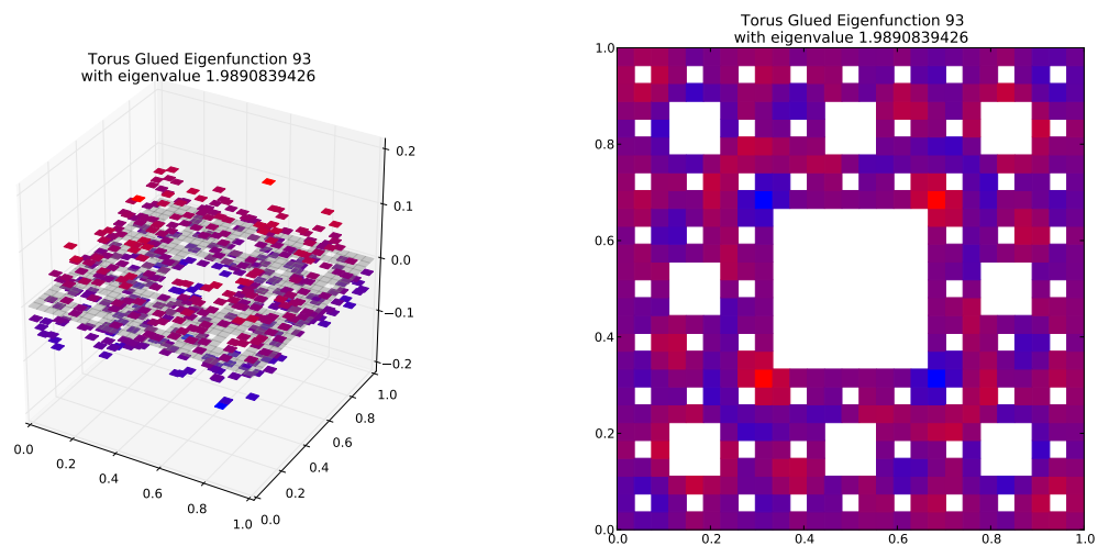
Eigenfunction 93 with eigenvalue 1.9890839426
