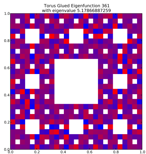
Eigenfunction 361 with eigenvalue 5.17866887259
