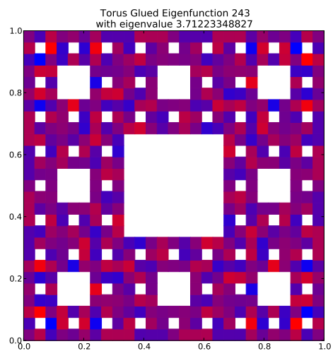
Eigenfunction 243 with eigenvalue 3.71223348827
