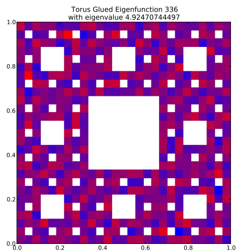
Eigenfunction 336 with eigenvalue 4.92470744497
