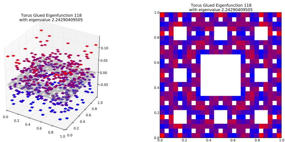
Eigenfunction 118 with eigenvalue 2.24290409505
