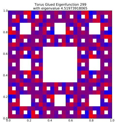
Eigenfunction 299 with eigenvalue 4.51973918065
