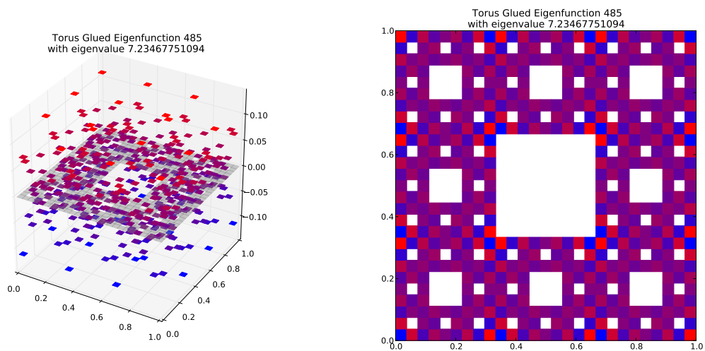
Eigenfunction 485 with eigenvalue 7.23467751094
