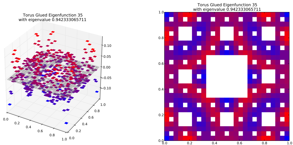
Eigenfunction 35 with eigenvalue 0.942333065711
