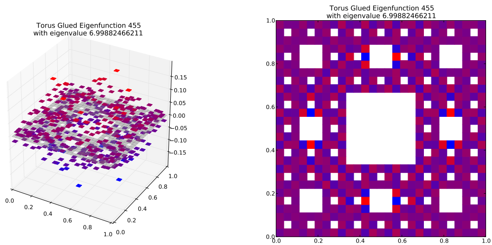
Eigenfunction 455 with eigenvalue 6.99882466211
