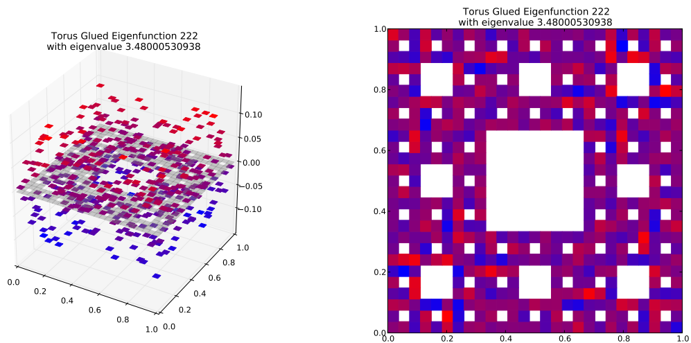
Eigenfunction 222 with eigenvalue 3.48000530938
