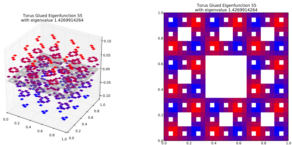
Eigenfunction 55 with eigenvalue 1.4269914264
