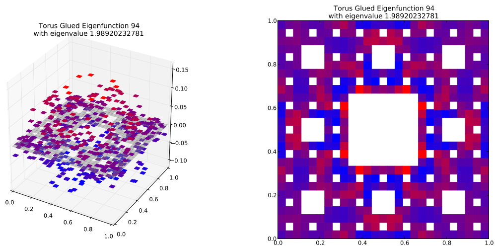
Eigenfunction 94 with eigenvalue 1.98920232781
