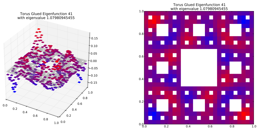
Eigenfunction 41 with eigenvalue 1.07980945455
