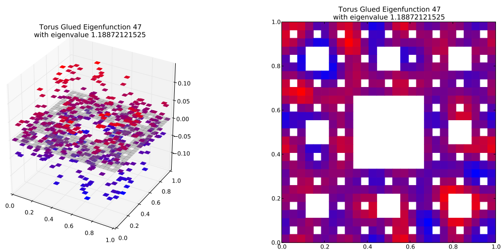
Eigenfunction 47 with eigenvalue 1.18872121525
