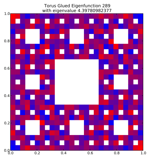
Eigenfunction 289 with eigenvalue 4.39780982377
