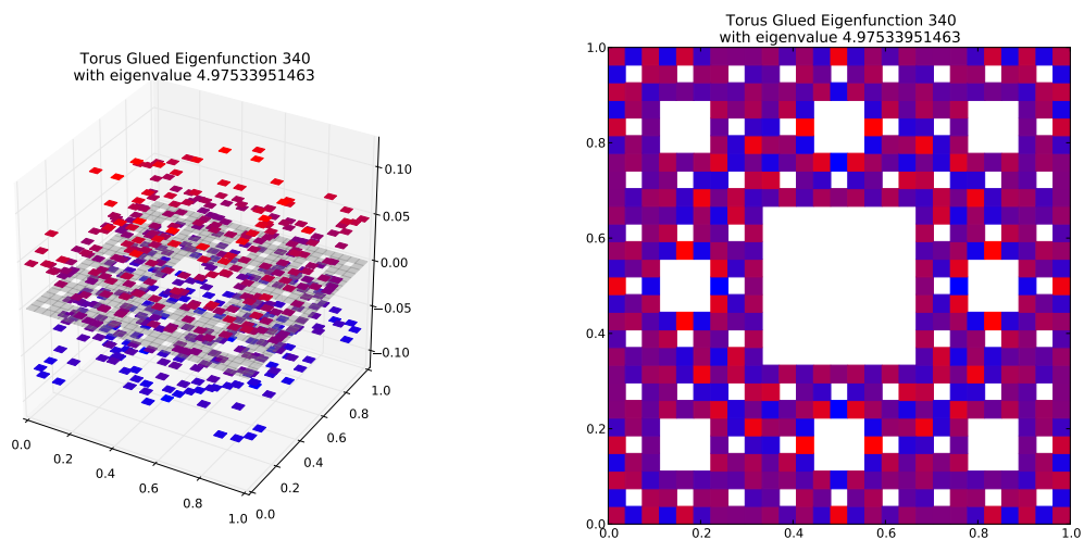
Eigenfunction 340 with eigenvalue 4.97533951463
