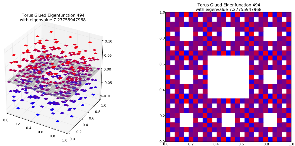
Eigenfunction 494 with eigenvalue 7.27755947968
