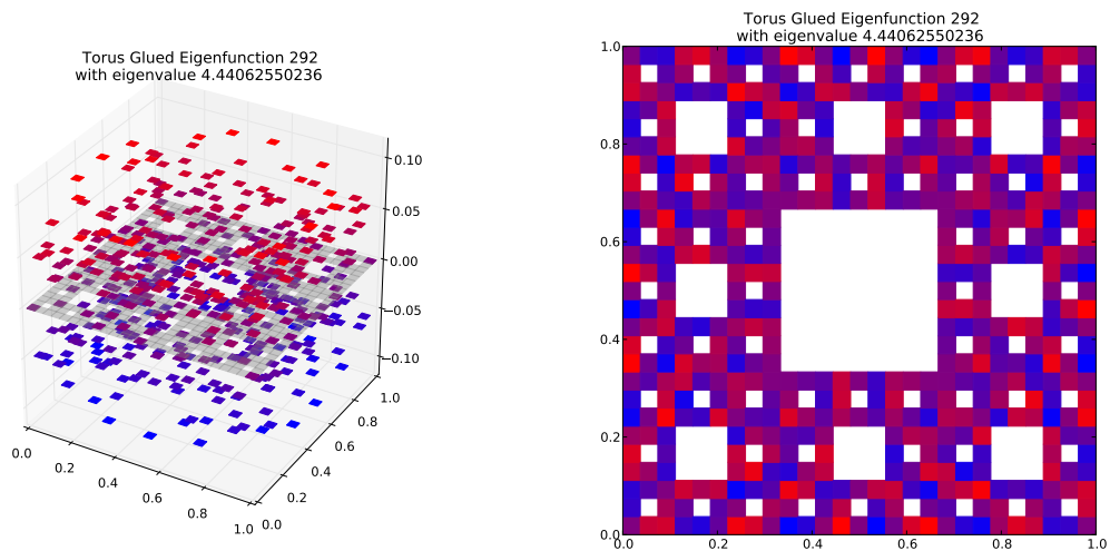
Eigenfunction 292 with eigenvalue 4.44062550236
