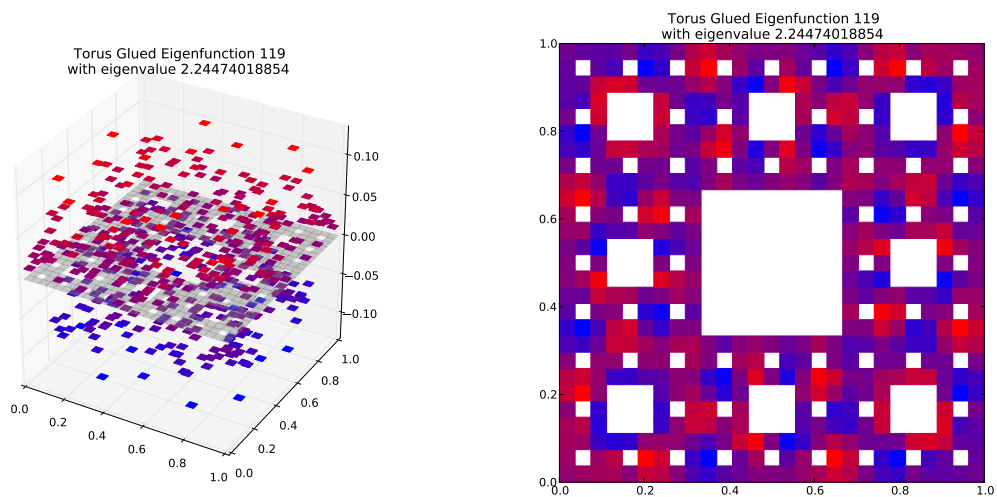
Eigenfunction 119 with eigenvalue 2.24474018854
