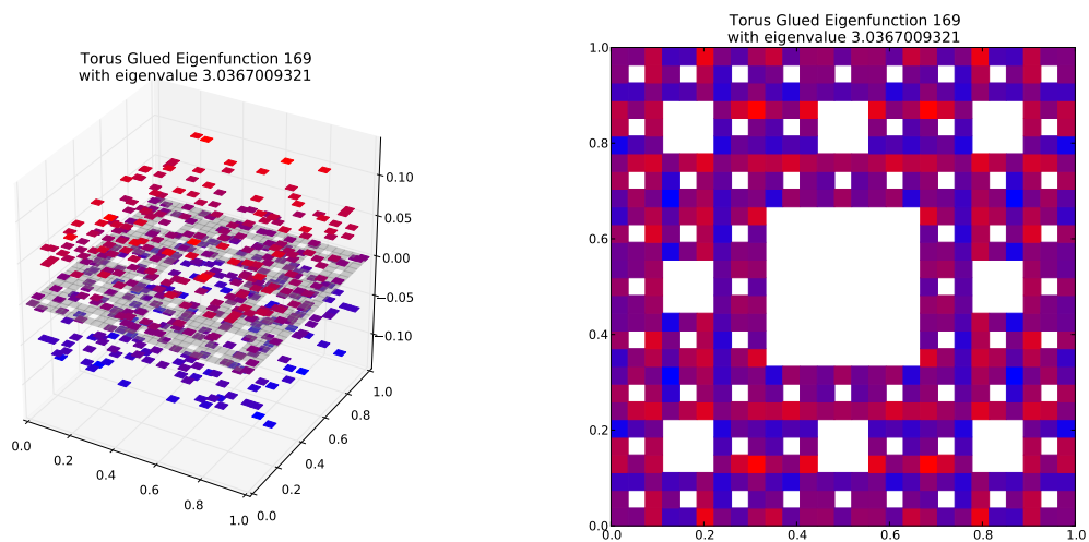
Eigenfunction 169 with eigenvalue 3.0367009321
