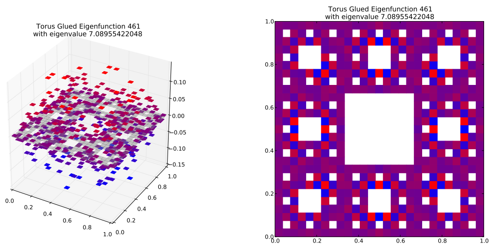
Eigenfunction 461 with eigenvalue 7.08955422048
