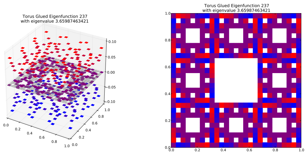
Eigenfunction 237 with eigenvalue 3.65987463421
