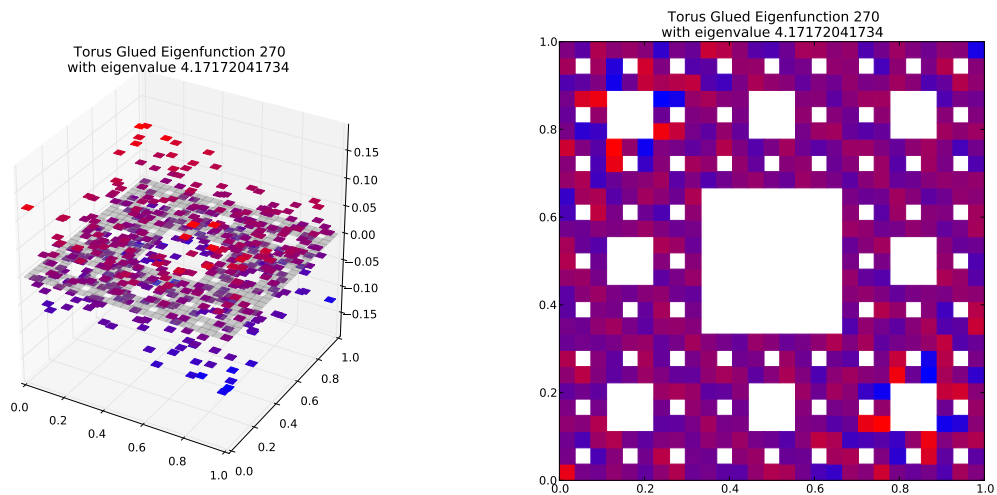
Eigenfunction 270 with eigenvalue 4.17172041734
