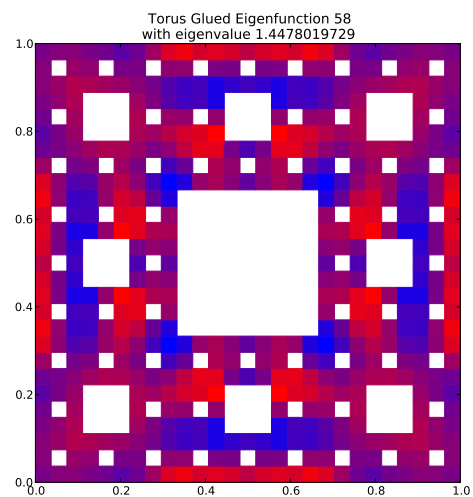
Eigenfunction 58 with eigenvalue 1.4478019729
