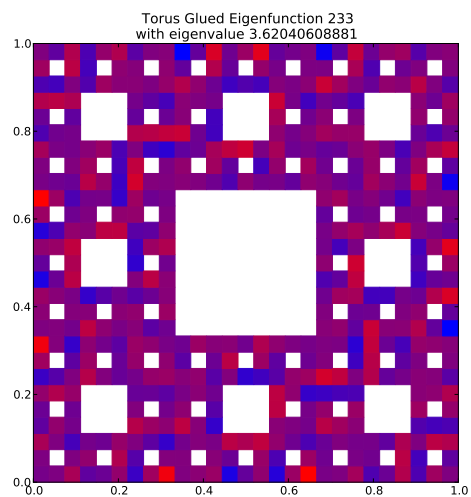
Eigenfunction 233 with eigenvalue 3.62040608881
