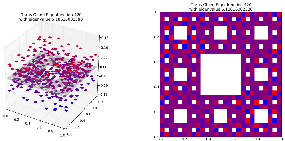
Eigenfunction 420 with eigenvalue 6.18616002388
