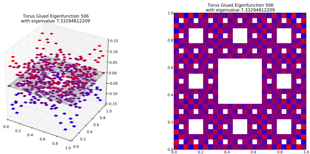
Eigenfunction 506 with eigenvalue 7.33294812209
