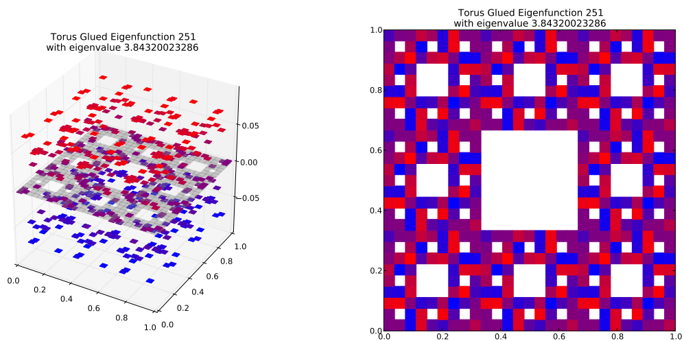
Eigenfunction 251 with eigenvalue 3.84320023286
