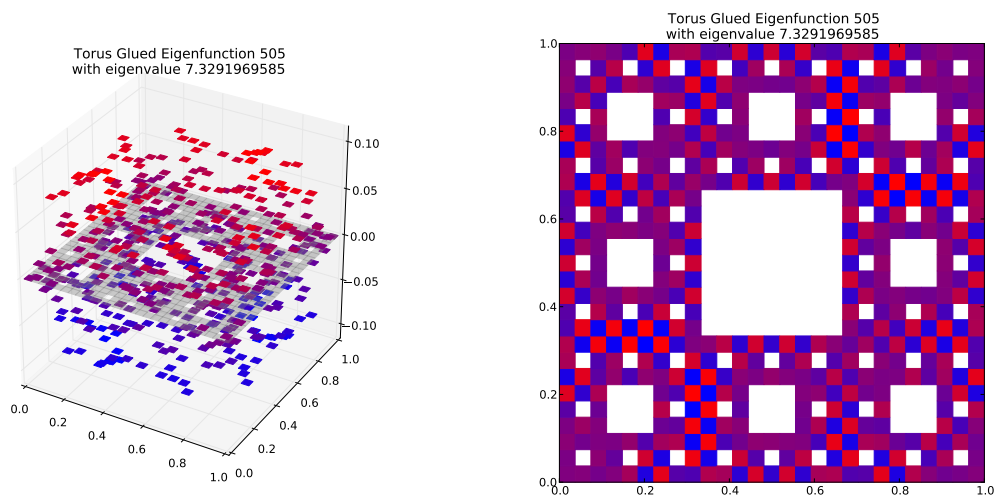
Eigenfunction 505 with eigenvalue 7.3291969585
