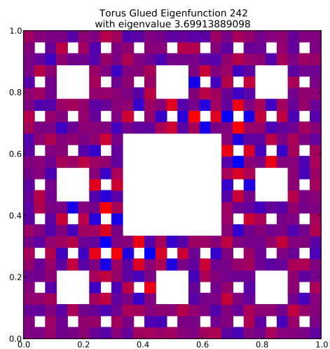
Eigenfunction 242 with eigenvalue 3.69913889098
