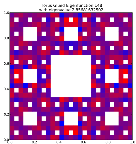
Eigenfunction 148 with eigenvalue 2.85681632502
