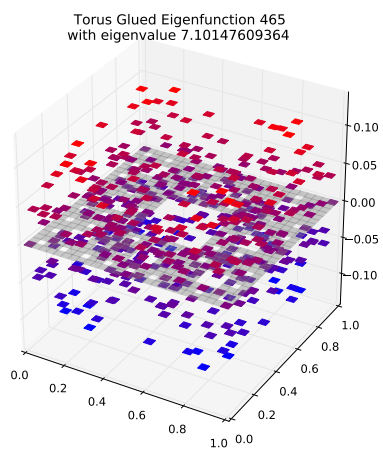
Eigenfunction 465 with eigenvalue 7.10147609364
