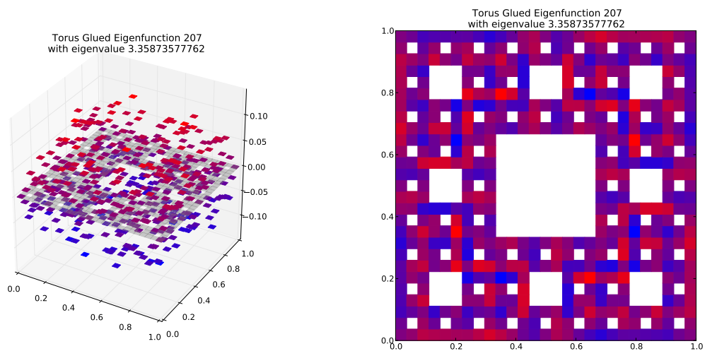
Eigenfunction 207 with eigenvalue 3.35873577762
