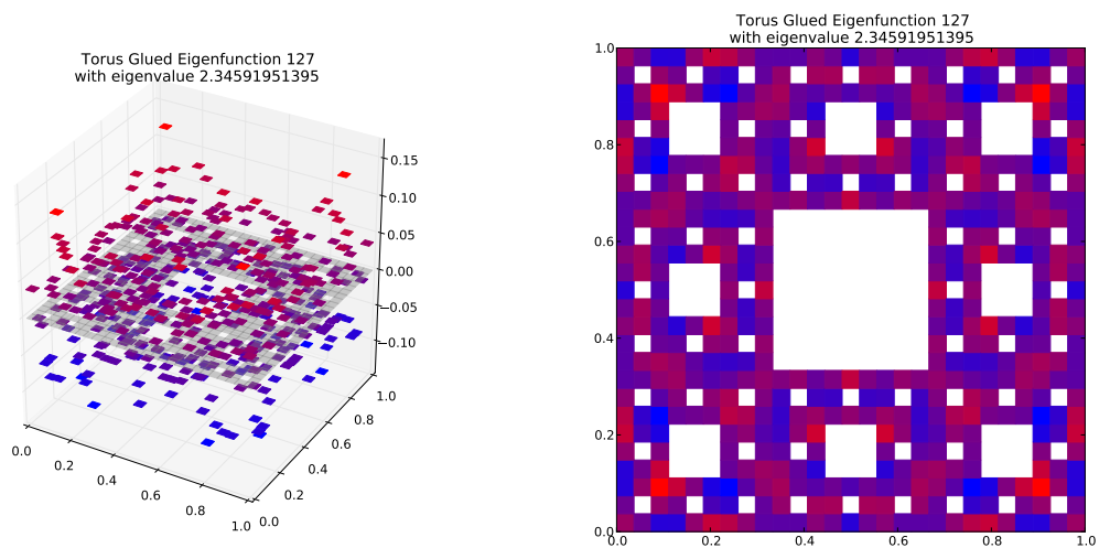
Eigenfunction 127 with eigenvalue 2.34591951395
