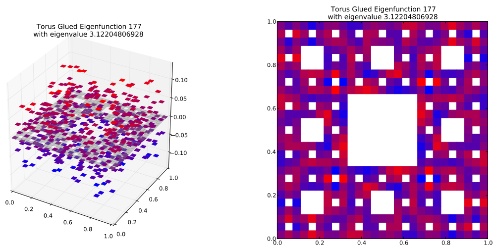
Eigenfunction 177 with eigenvalue 3.12204806928
