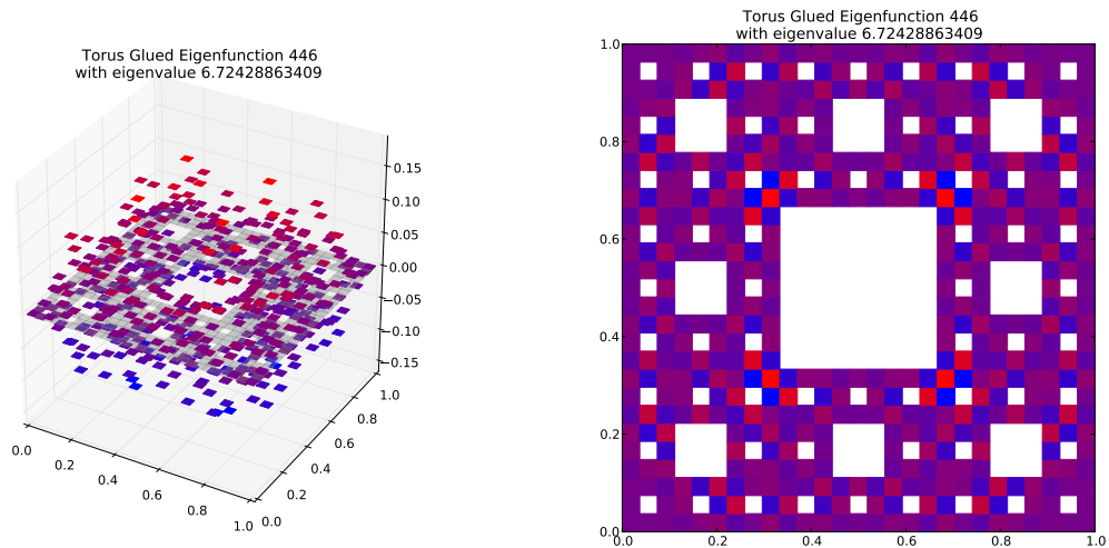
Eigenfunction 446 with eigenvalue 6.72428863409
