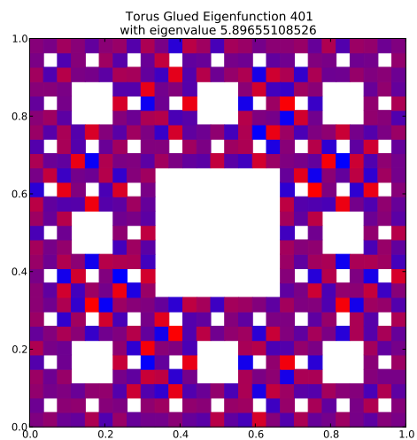
Eigenfunction 401 with eigenvalue 5.89655108526
