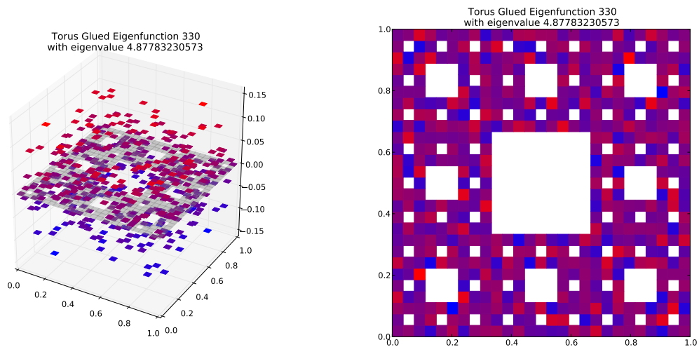
Eigenfunction 330 with eigenvalue 4.87783230573
