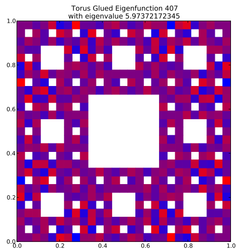
Eigenfunction 407 with eigenvalue 5.97372172345
