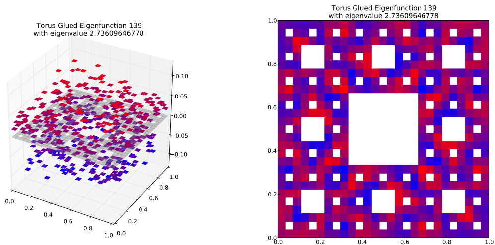
Eigenfunction 139 with eigenvalue 2.73609646778
