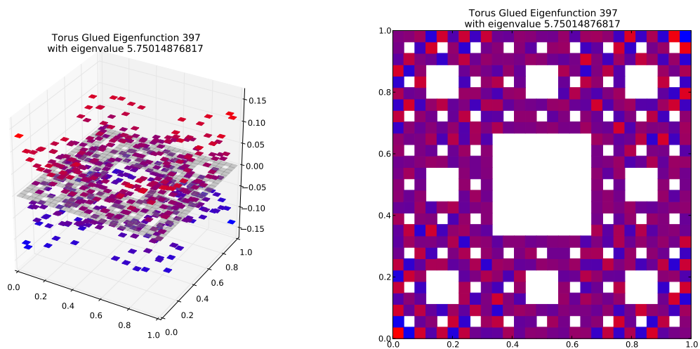
Eigenfunction 397 with eigenvalue 5.75014876817
