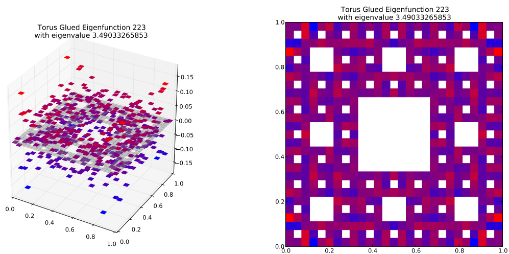
Eigenfunction 223 with eigenvalue 3.49033265853
