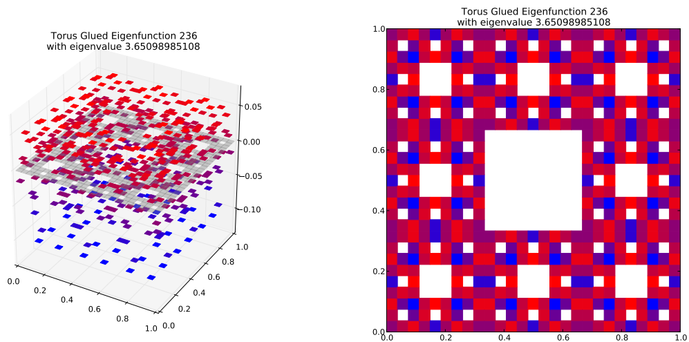
Eigenfunction 236 with eigenvalue 3.65098985108
