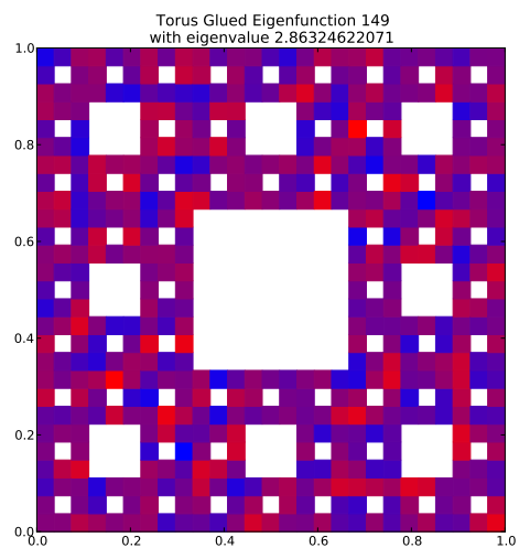
Eigenfunction 149 with eigenvalue 2.86324622071
