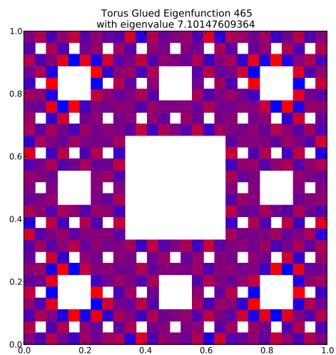
Eigenfunction 465 with eigenvalue 7.10147609364
