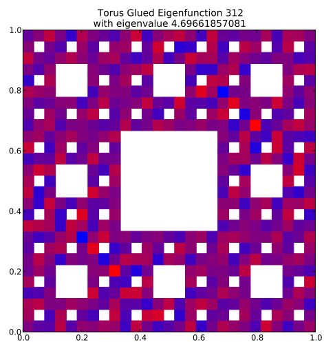
Eigenfunction 312 with eigenvalue 4.69661857081
