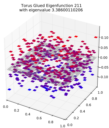
Eigenfunction 211 with eigenvalue 3.38600110206
