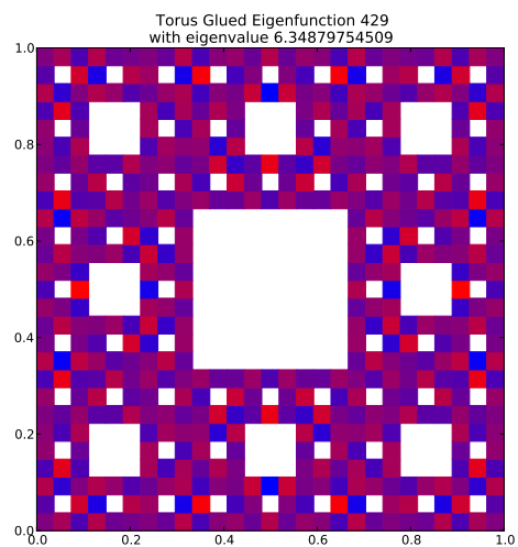
Eigenfunction 429 with eigenvalue 6.34879754509
