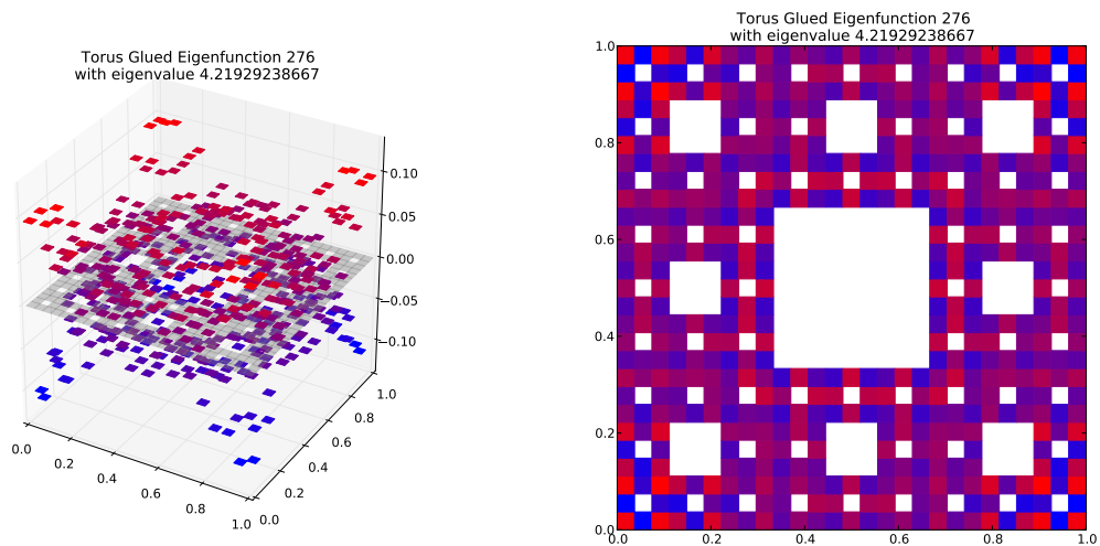
Eigenfunction 276 with eigenvalue 4.21929238667
