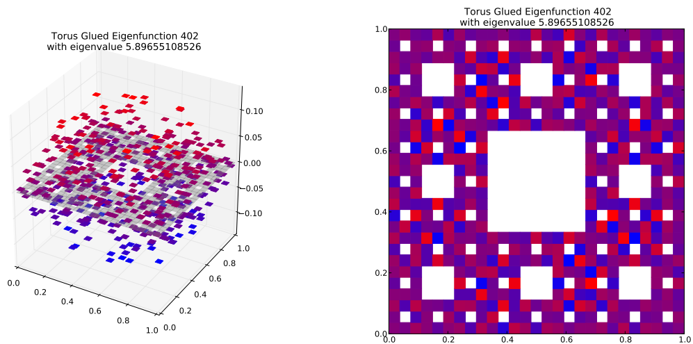
Eigenfunction 402 with eigenvalue 5.89655108526
