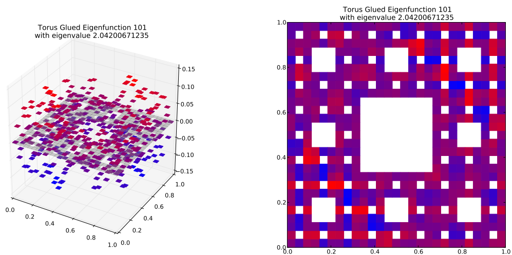
Eigenfunction 101 with eigenvalue 2.04200671235
