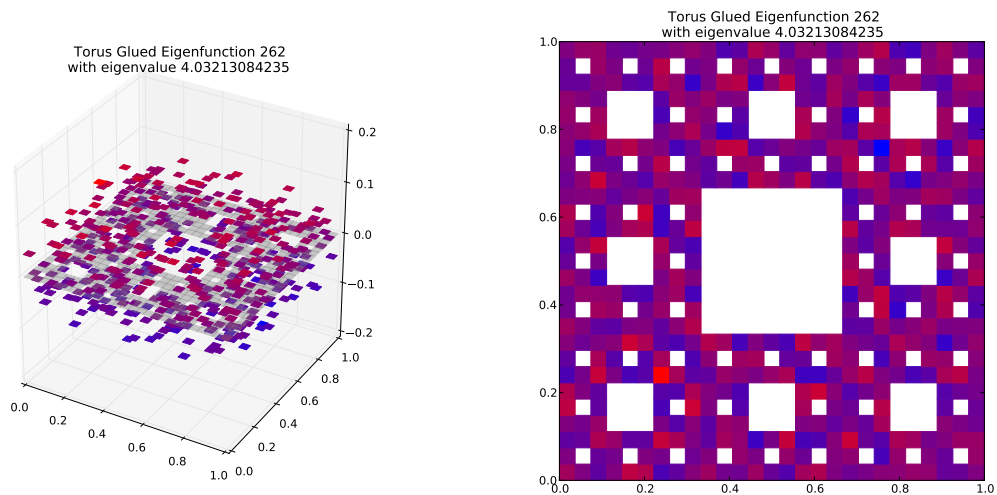
Eigenfunction 262 with eigenvalue 4.03213084235
