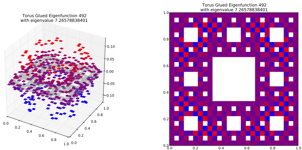
Eigenfunction 492 with eigenvalue 7.26578838401
