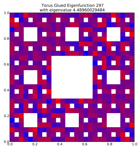
Eigenfunction 297 with eigenvalue 4.48960029484
