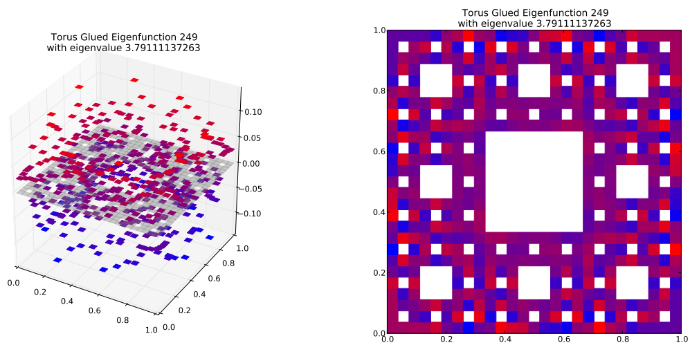
Eigenfunction 249 with eigenvalue 3.79111137263
