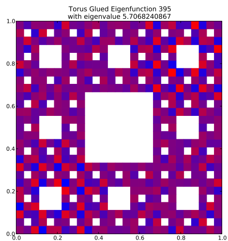
Eigenfunction 395 with eigenvalue 5.7068240867
