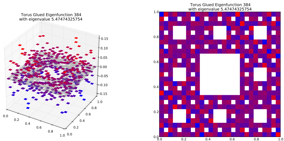
Eigenfunction 384 with eigenvalue 5.47474325754
