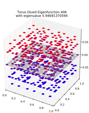
Eigenfunction 406 with eigenvalue 5.94691370594
