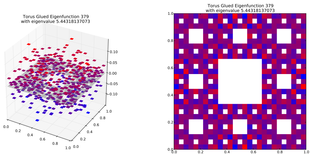
Eigenfunction 379 with eigenvalue 5.44318137073
