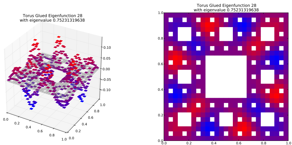
Eigenfunction 28 with eigenvalue 0.75231319638
