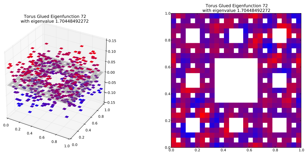
Eigenfunction 72 with eigenvalue 1.70448492272
