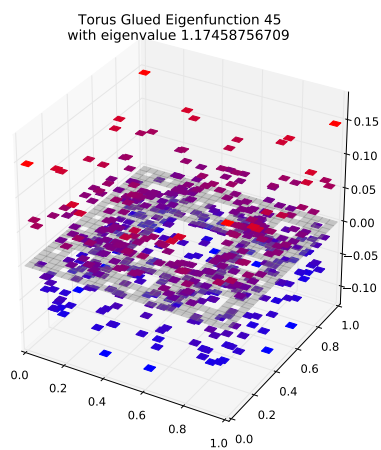
Eigenfunction 45 with eigenvalue 1.17458756709
