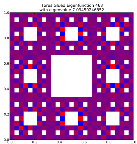
Eigenfunction 463 with eigenvalue 7.09450246852
