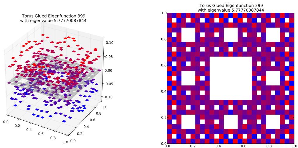
Eigenfunction 399 with eigenvalue 5.77770087844
