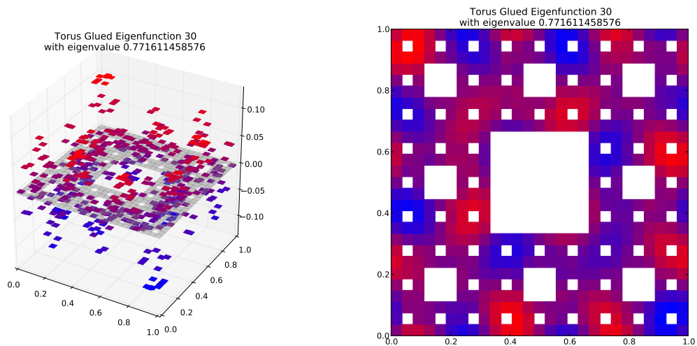
Eigenfunction 30 with eigenvalue 0.771611458576
