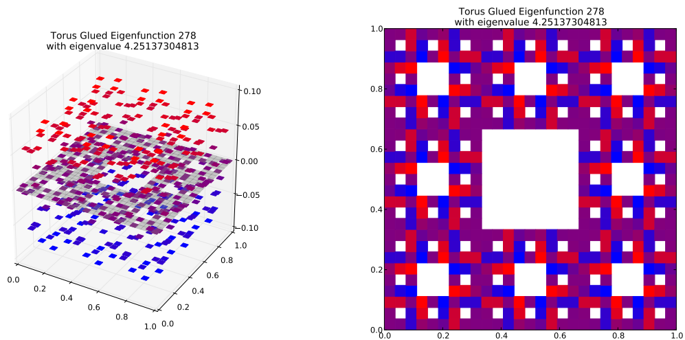
Eigenfunction 278 with eigenvalue 4.25137304813
