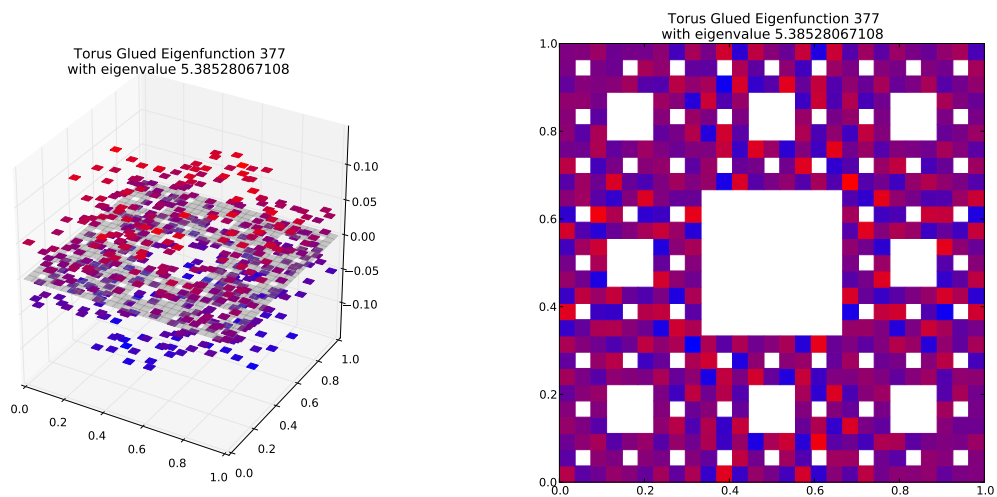
Eigenfunction 377 with eigenvalue 5.38528067108
