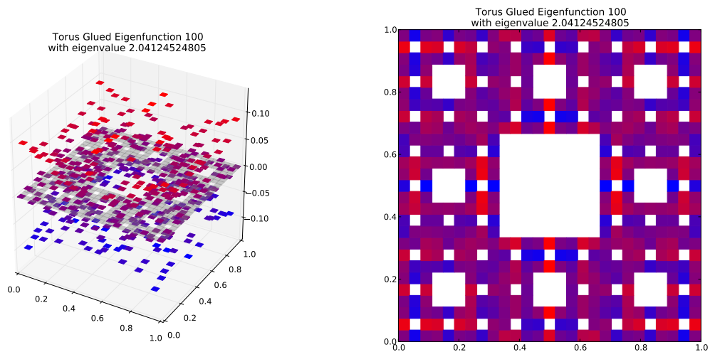
Eigenfunction 100 with eigenvalue 2.04124524805
