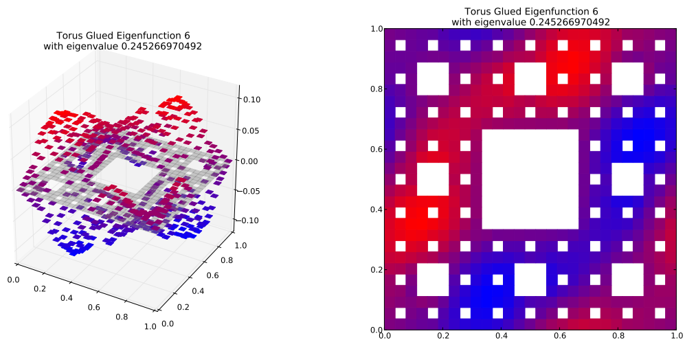
Eigenfunction 6 with eigenvalue 0.245266970492
