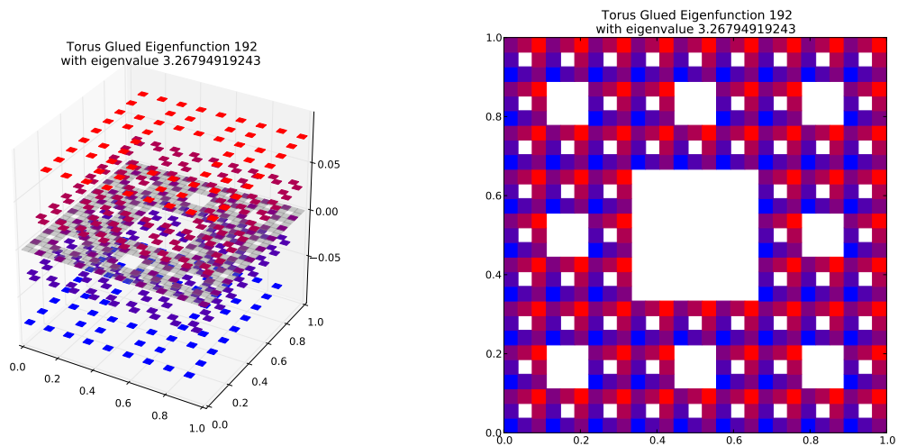
Eigenfunction 192 with eigenvalue 3.26794919243
