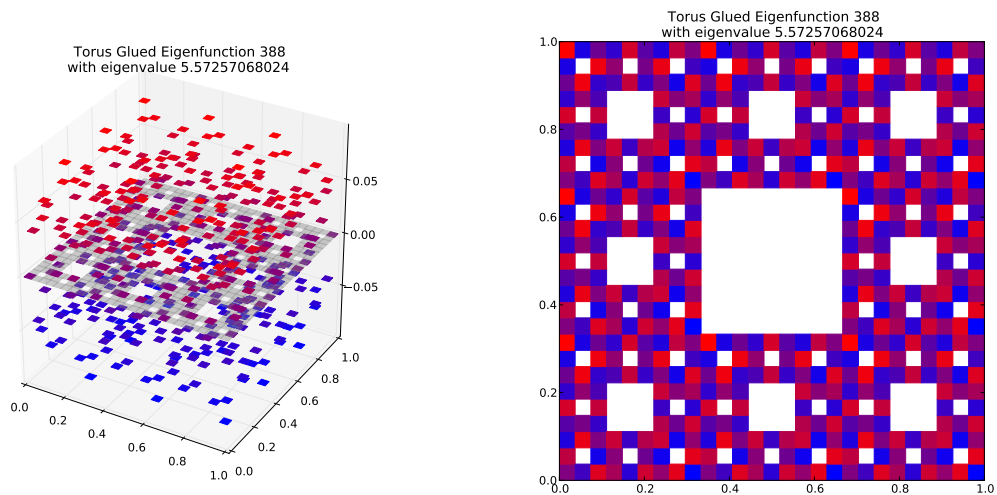
Eigenfunction 388 with eigenvalue 5.57257068024
