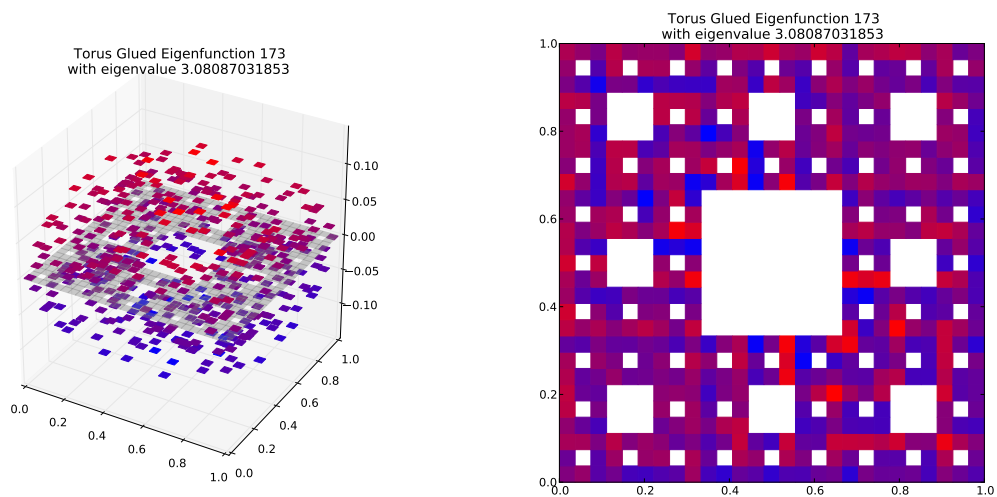
Eigenfunction 173 with eigenvalue 3.08087031853
