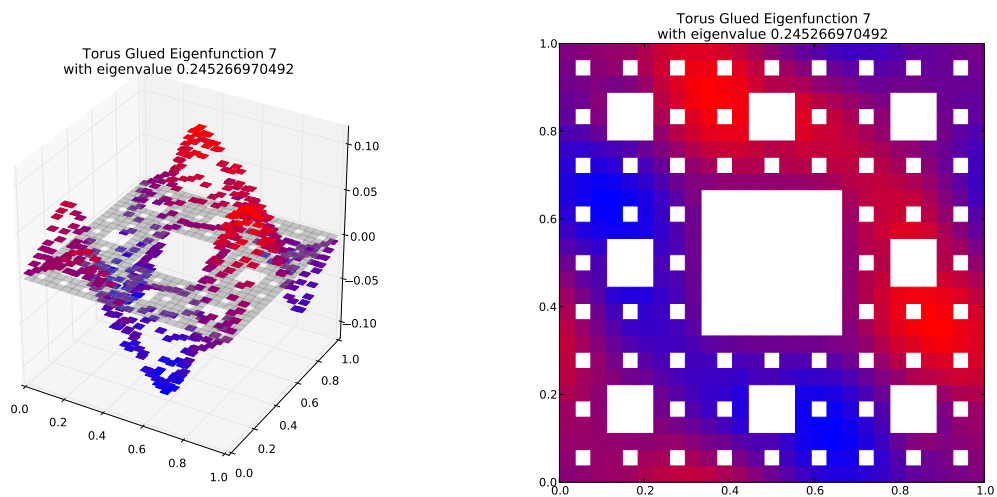
Eigenfunction 7 with eigenvalue 0.245266970492
