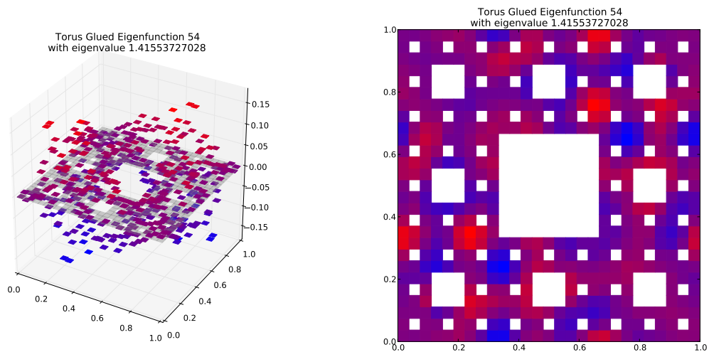
Eigenfunction 54 with eigenvalue 1.41553727028
