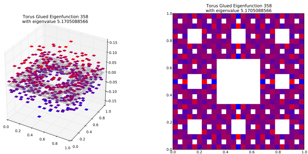
Eigenfunction 358 with eigenvalue 5.1705088566
