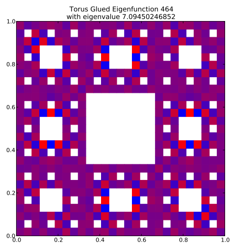
Eigenfunction 464 with eigenvalue 7.09450246852
