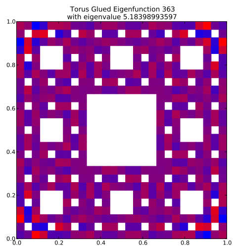
Eigenfunction 363 with eigenvalue 5.18398993597
