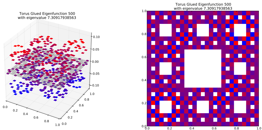
Eigenfunction 500 with eigenvalue 7.30917938563
