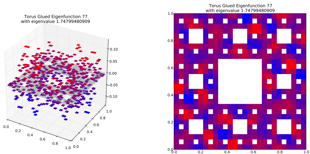
Eigenfunction 77 with eigenvalue 1.74799480909
