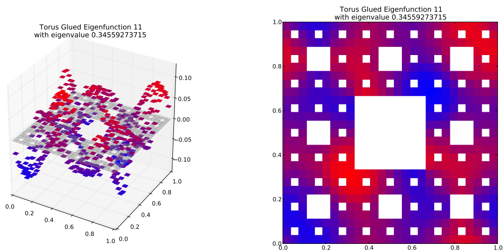
Eigenfunction 11 with eigenvalue 0.34559273715
