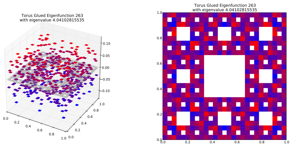
Eigenfunction 263 with eigenvalue 4.04102815535
