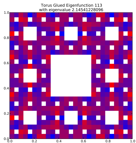
Eigenfunction 113 with eigenvalue 2.14541228096
