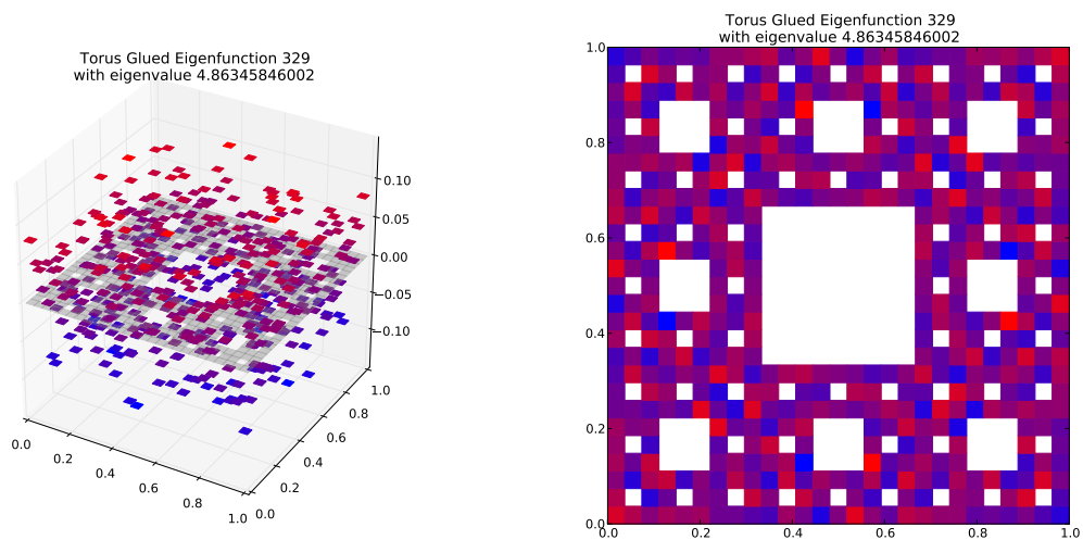
Eigenfunction 329 with eigenvalue 4.86345846002
