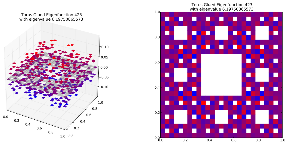
Eigenfunction 423 with eigenvalue 6.19750865573
