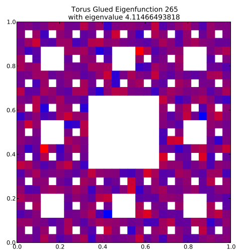
Eigenfunction 265 with eigenvalue 4.11466493818
