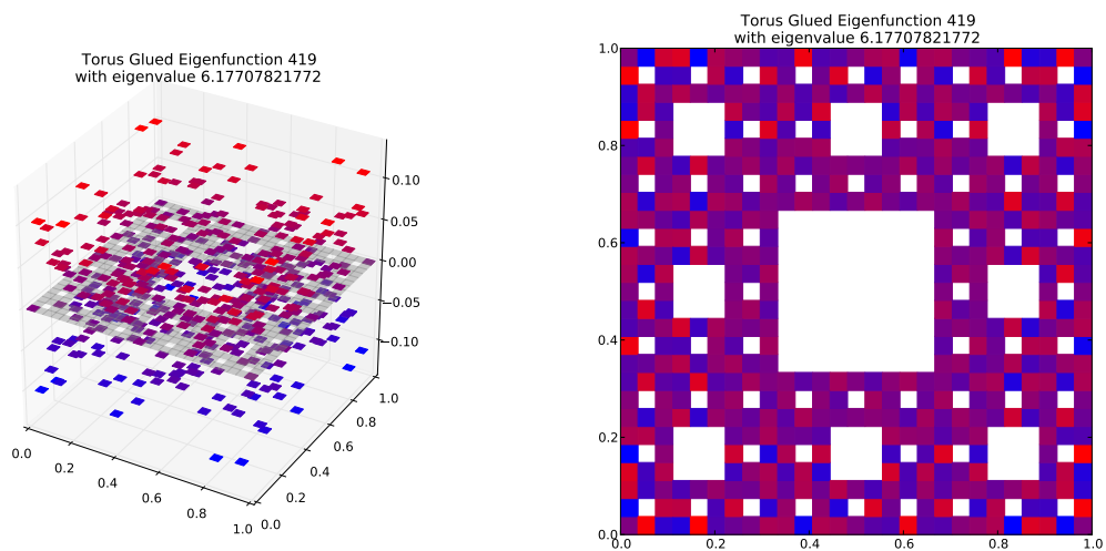
Eigenfunction 419 with eigenvalue 6.17707821772
