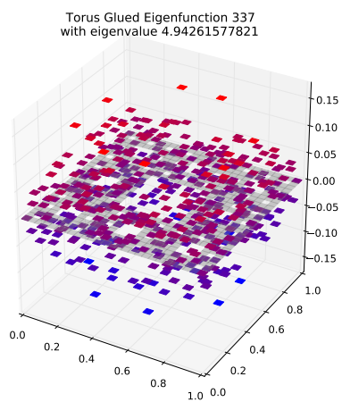
Eigenfunction 337 with eigenvalue 4.94261577821
