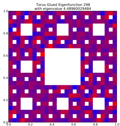
Eigenfunction 298 with eigenvalue 4.48960029484
