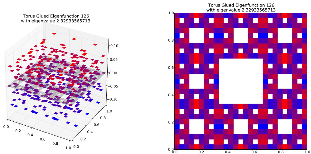
Eigenfunction 126 with eigenvalue 2.32933565713
