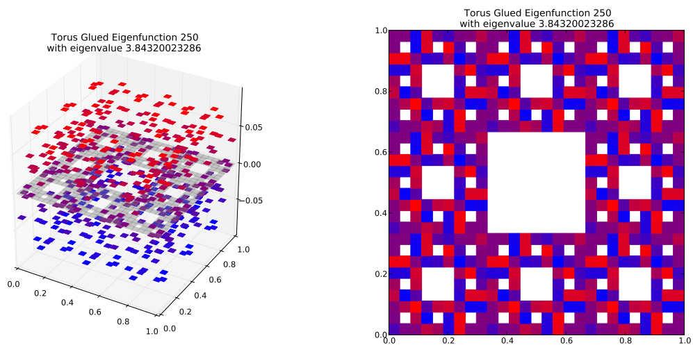
Eigenfunction 250 with eigenvalue 3.84320023286
