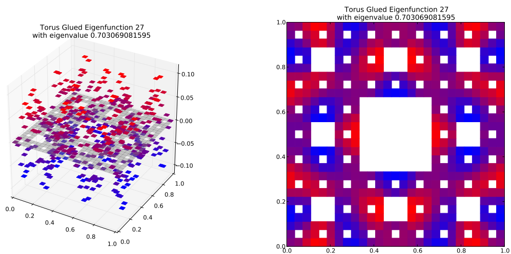
Eigenfunction 27 with eigenvalue 0.703069081595
