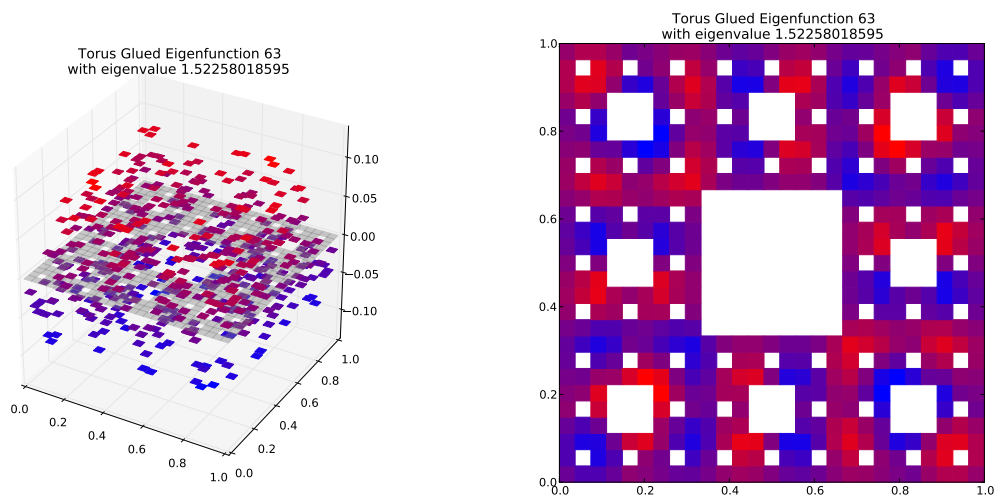
Eigenfunction 63 with eigenvalue 1.52258018595
