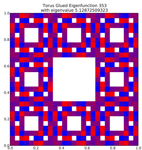
Eigenfunction 353 with eigenvalue 5.12872509323
