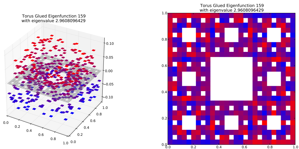
Eigenfunction 159 with eigenvalue 2.9608096429
