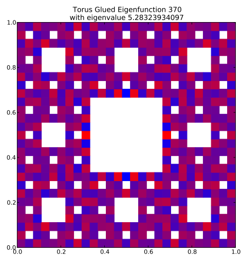
Eigenfunction 370 with eigenvalue 5.28323934097
