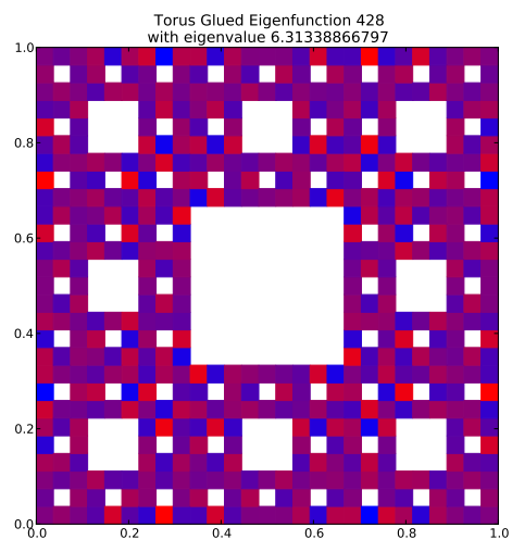
Eigenfunction 428 with eigenvalue 6.31338866797
