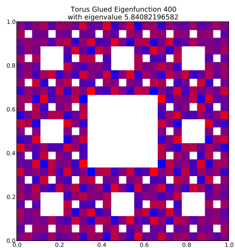
Eigenfunction 400 with eigenvalue 5.84082196582
