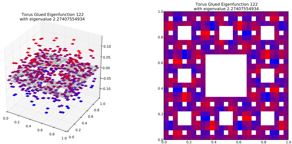
Eigenfunction 122 with eigenvalue 2.27407554934
