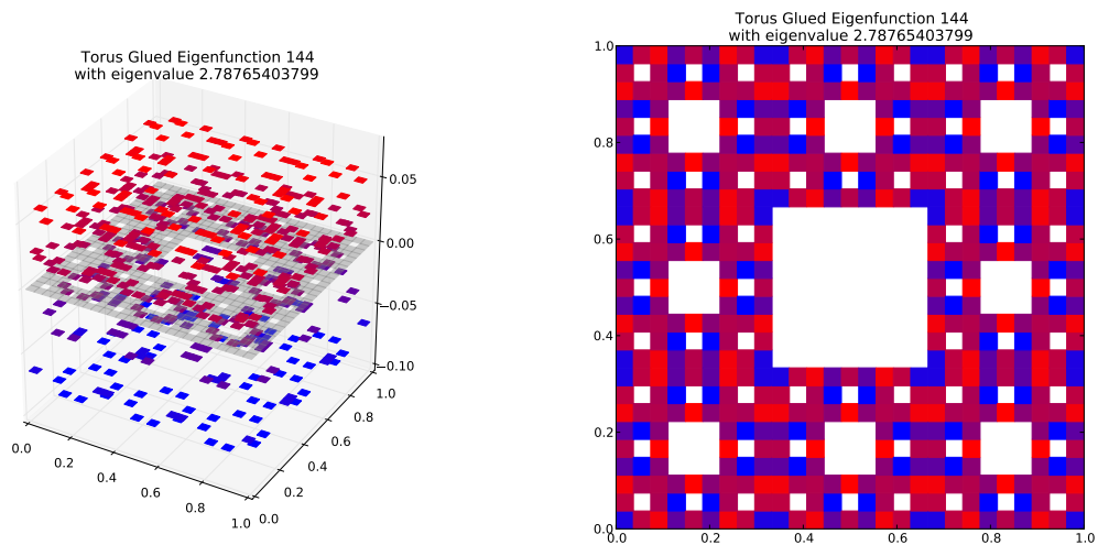
Eigenfunction 144 with eigenvalue 2.78765403799
