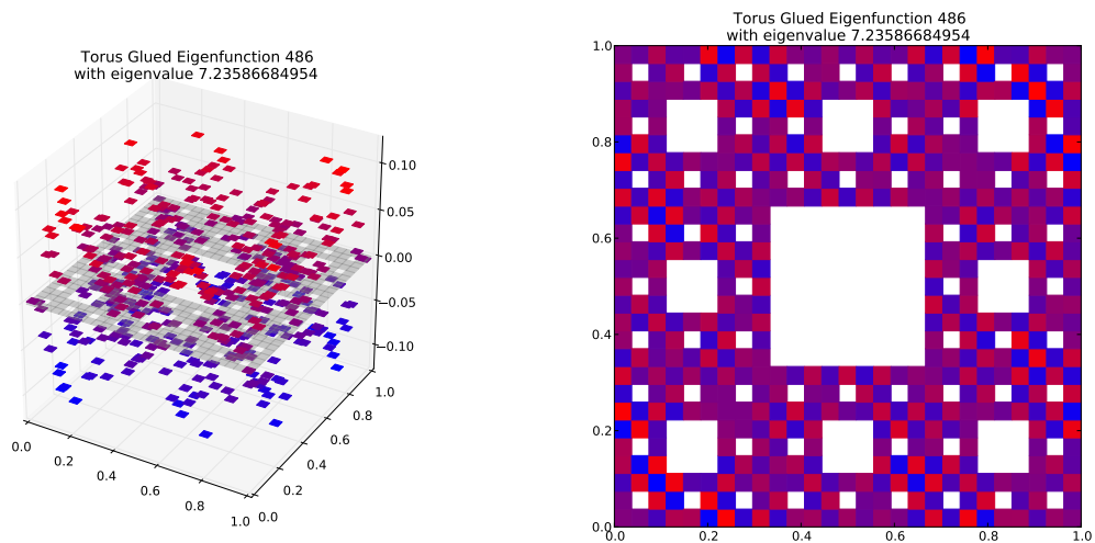
Eigenfunction 486 with eigenvalue 7.23586684954
