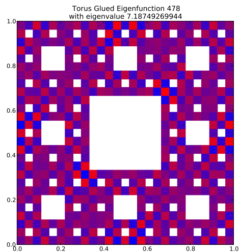
Eigenfunction 478 with eigenvalue 7.18749269944
