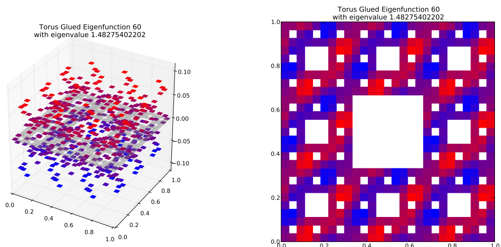
Eigenfunction 60 with eigenvalue 1.48275402202
