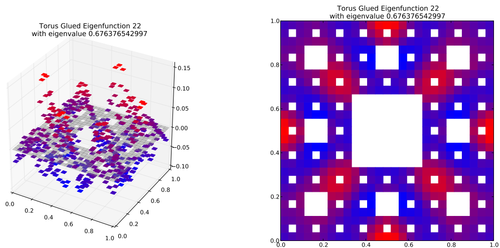
Eigenfunction 22 with eigenvalue 0.676376542997
