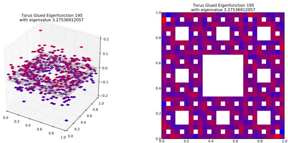
Eigenfunction 195 with eigenvalue 3.27536912057
