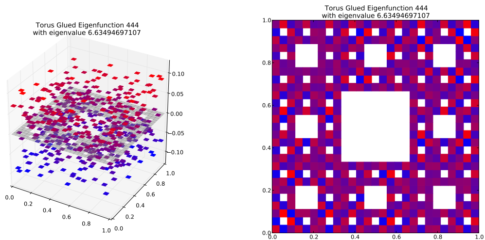
Eigenfunction 444 with eigenvalue 6.63494697107
