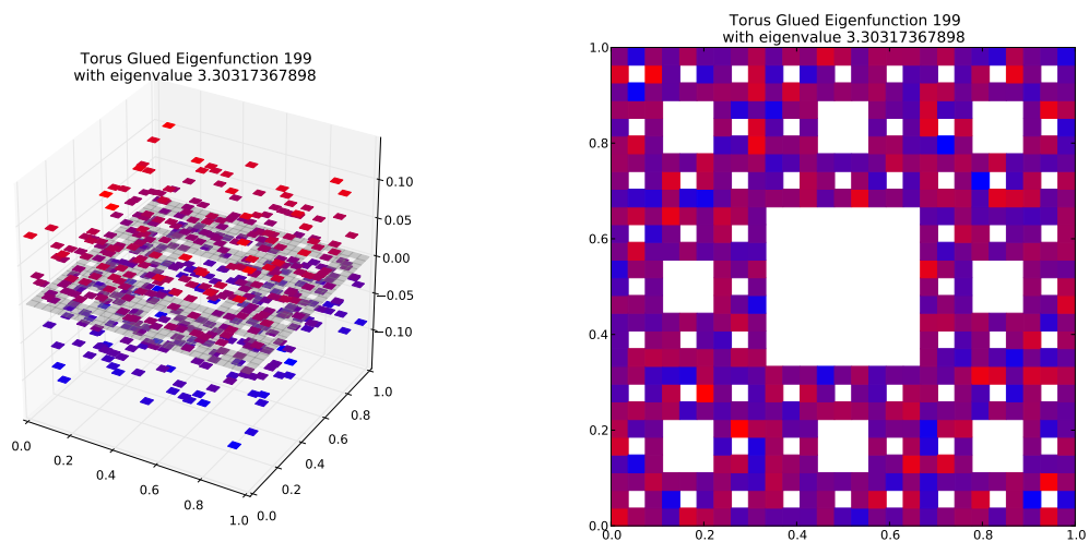
Eigenfunction 199 with eigenvalue 3.30317367898
