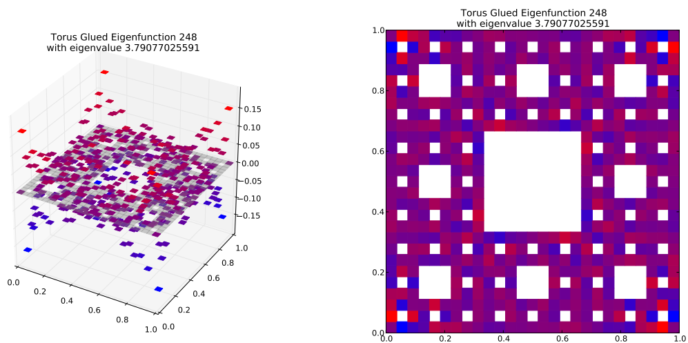
Eigenfunction 248 with eigenvalue 3.79077025591
