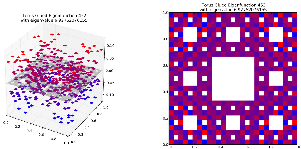
Eigenfunction 452 with eigenvalue 6.92752076155
