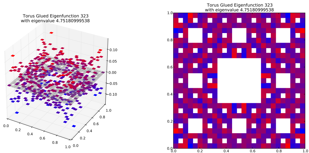
Eigenfunction 323 with eigenvalue 4.75180999538
