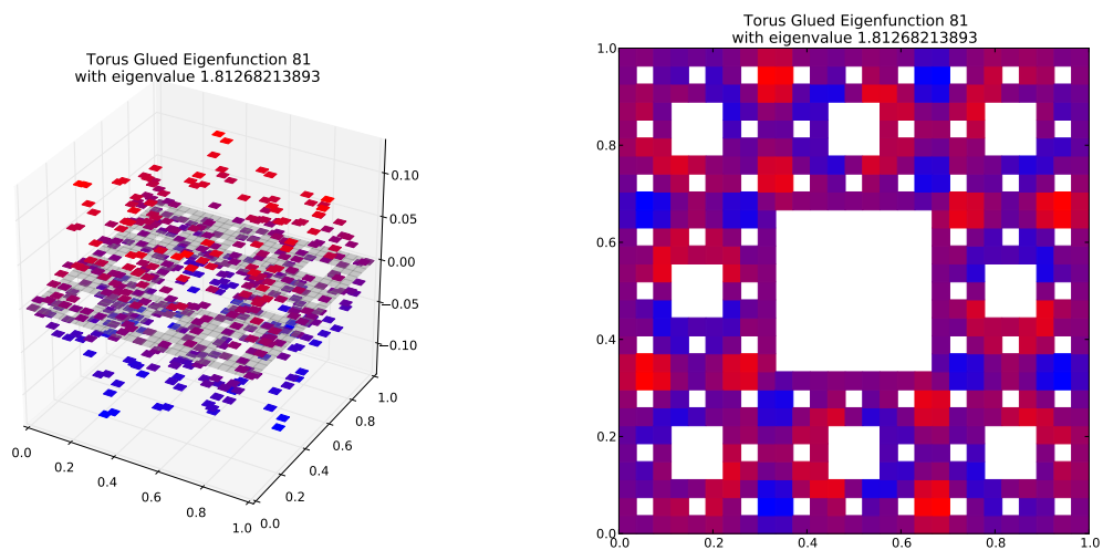
Eigenfunction 81 with eigenvalue 1.81268213893
