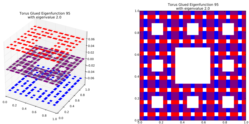
Eigenfunction 95 with eigenvalue 2.0
