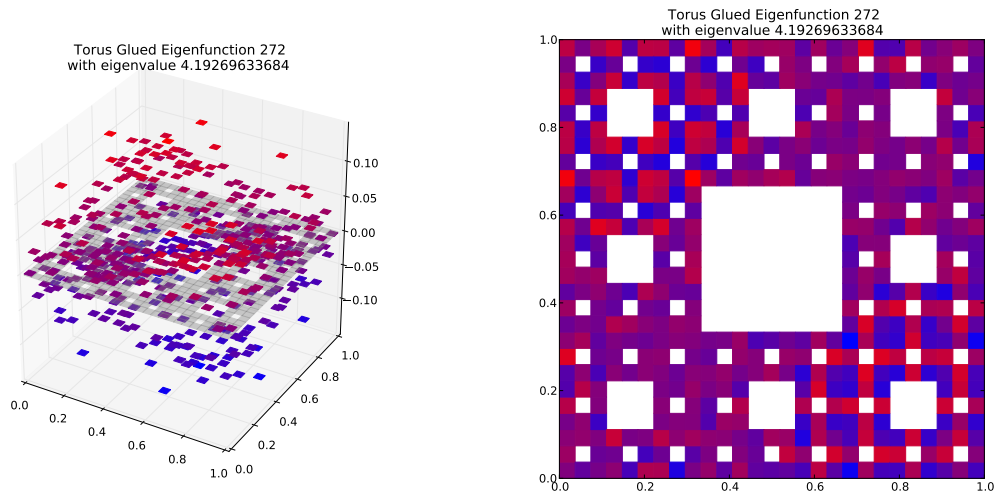
Eigenfunction 272 with eigenvalue 4.19269633684
