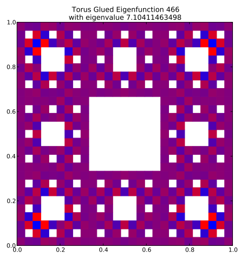
Eigenfunction 466 with eigenvalue 7.10411463498
