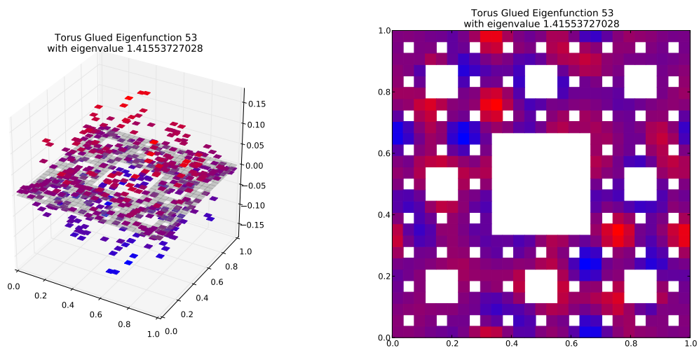
Eigenfunction 53 with eigenvalue 1.41553727028
