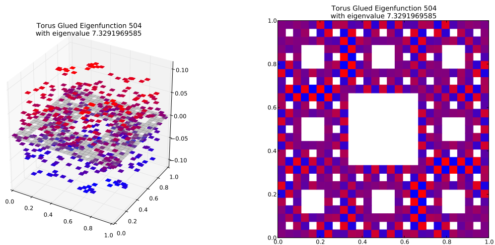
Eigenfunction 504 with eigenvalue 7.3291969585
