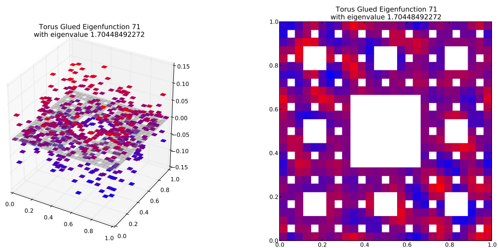
Eigenfunction 71 with eigenvalue 1.70448492272
