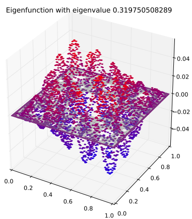
Eigenfunction 67 with eigenvalue 0.319750508289
