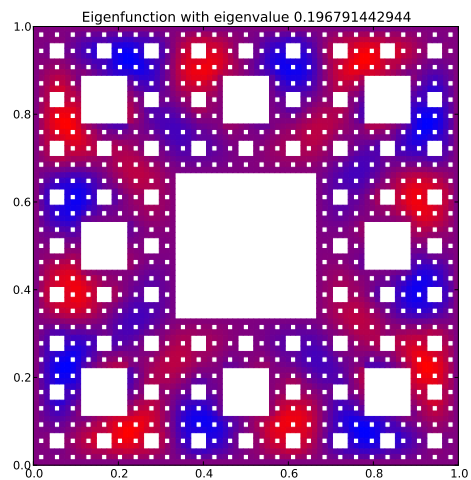
Eigenfunction 37 with eigenvalue 0.196791442944
