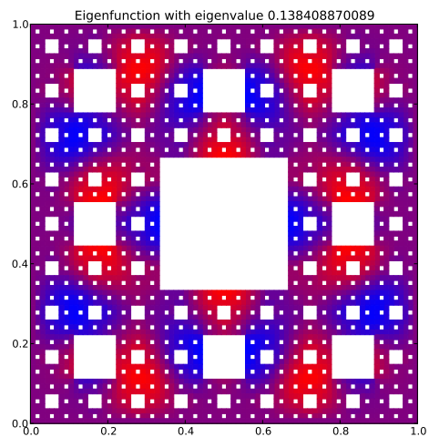
Eigenfunction 23 with eigenvalue 0.138408870089
