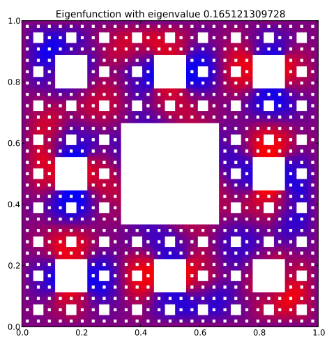
Eigenfunction 30 with eigenvalue 0.165121309728
