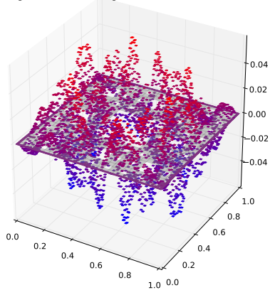
Eigenfunction with eigenvalue 0.399901205527
