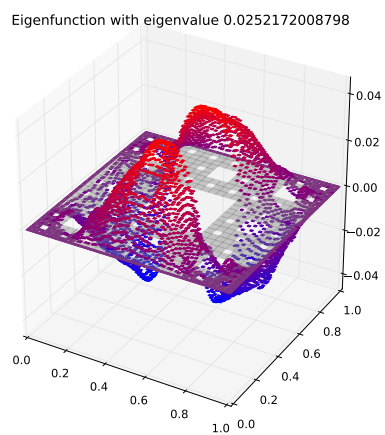
Eigenfunction 1 with eigenvalue 0.0252172008798
