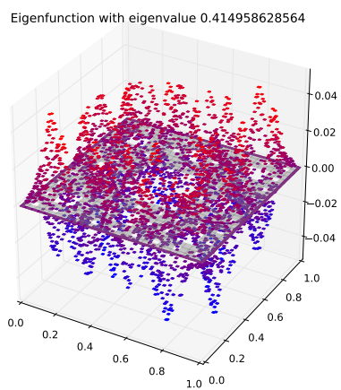
Eigenfunction 95 with eigenvalue 0.414958628564
