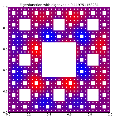
Eigenfunction 18 with eigenvalue 0.119751158231
