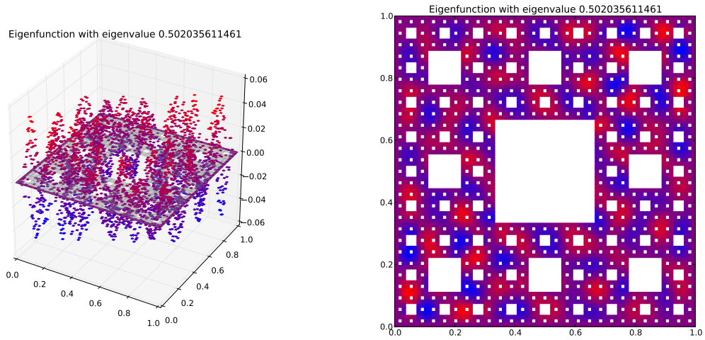
Eigenfunction 117 with eigenvalue 0.502035611461
