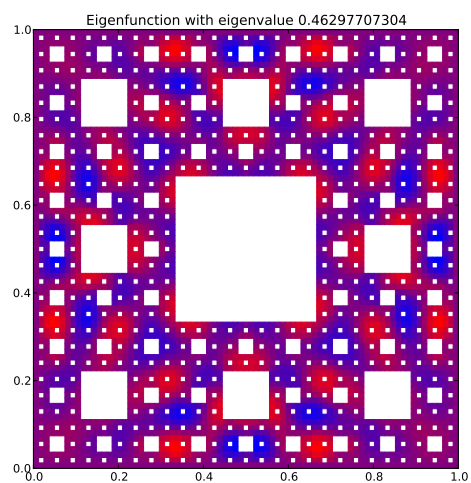
Eigenfunction 112 with eigenvalue 0.46297707304
