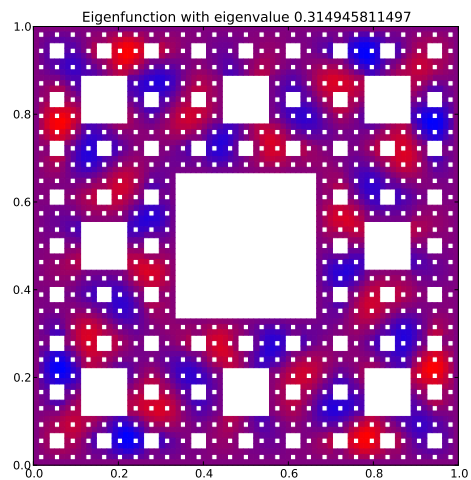
Eigenfunction 65 with eigenvalue 0.314945811497
