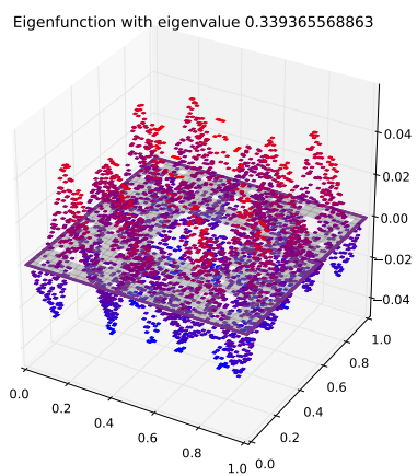
Eigenfunction 71 with eigenvalue 0.339365568863
