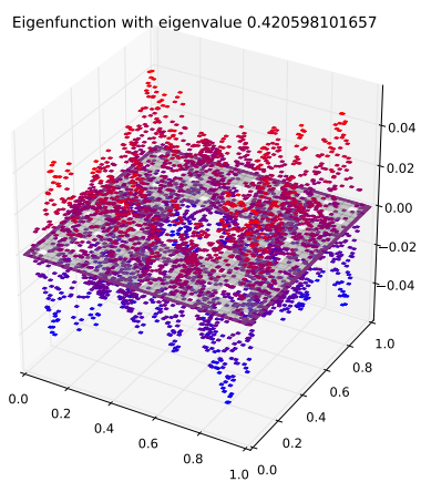
Eigenfunction 97 with eigenvalue 0.420598101657
