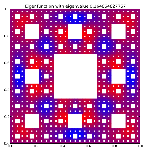
Eigenfunction 28 with eigenvalue 0.164864827757
