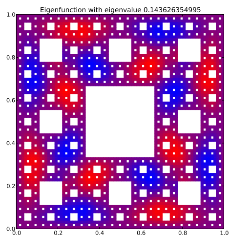
Eigenfunction 24 with eigenvalue 0.143626354995
