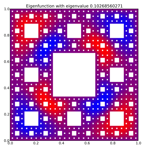
Eigenfunction 16 with eigenvalue 0.10268560271
