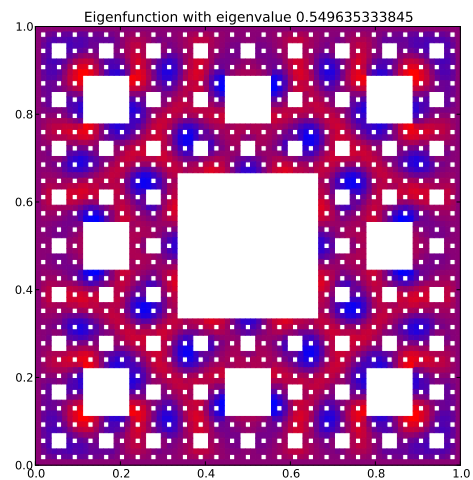
Eigenfunction 129 with eigenvalue 0.549635333845
