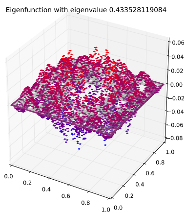
Eigenfunction 101 with eigenvalue 0.433528119084
