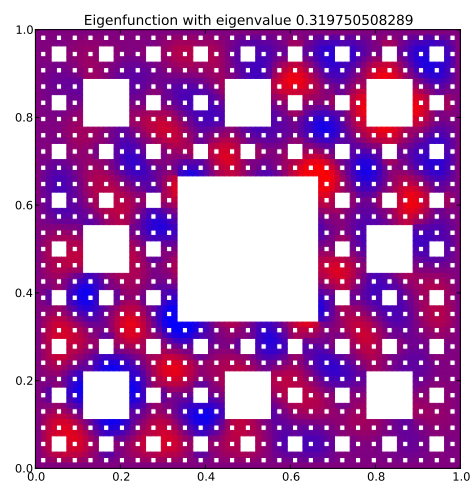
Eigenfunction 66 with eigenvalue 0.319750508289
