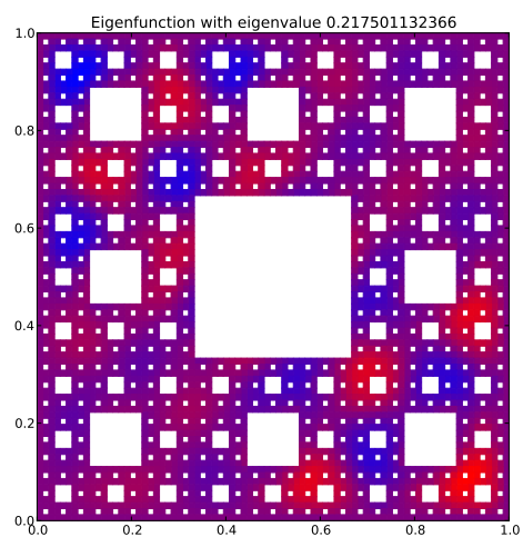
Eigenfunction 42 with eigenvalue 0.217501132366
