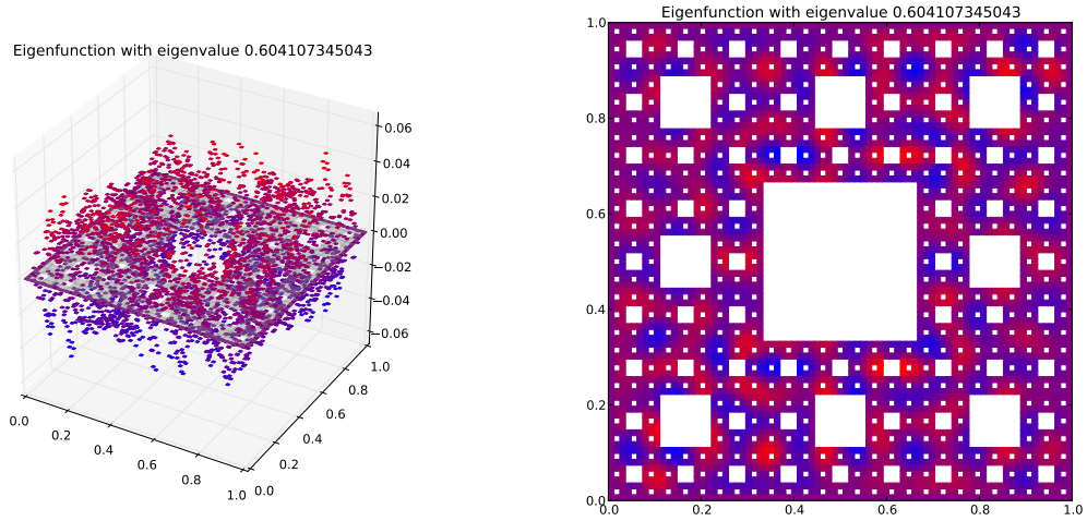
Eigenfunction 146 with eigenvalue 0.604107345043
