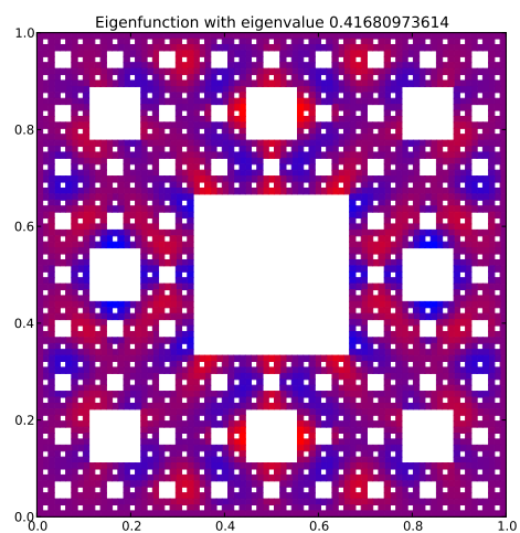
Eigenfunction 96 with eigenvalue 0.41680973614
