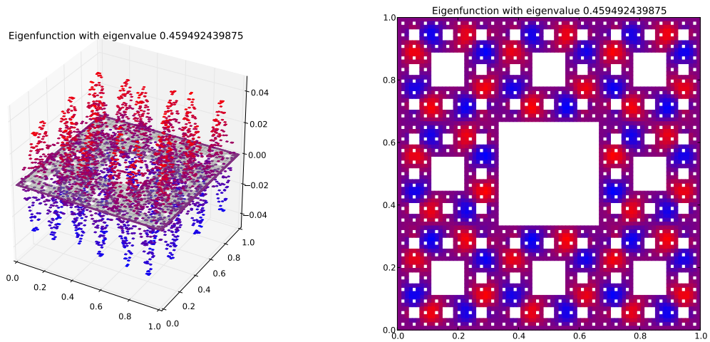
Eigenfunction 111 with eigenvalue 0.459492439875
