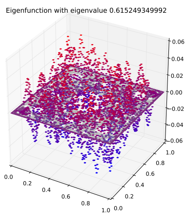
Eigenfunction 149 with eigenvalue 0.615249349992
