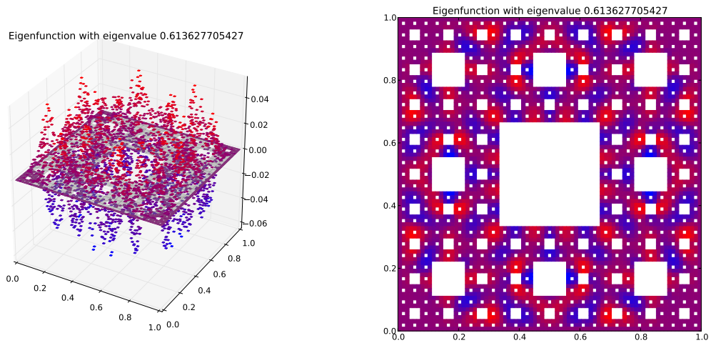
Eigenfunction 147 with eigenvalue 0.613627705427
