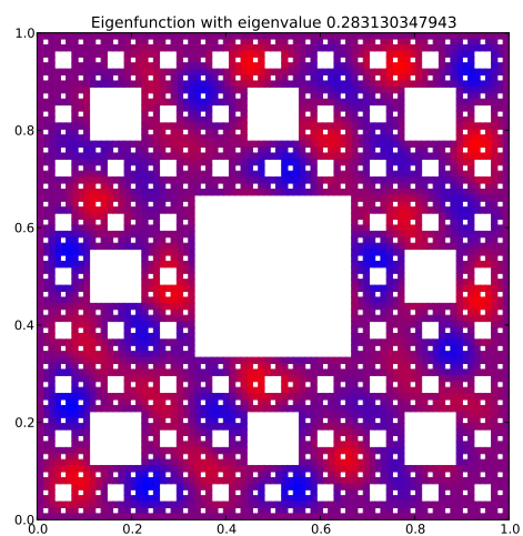
Eigenfunction 58 with eigenvalue 0.283130347943
