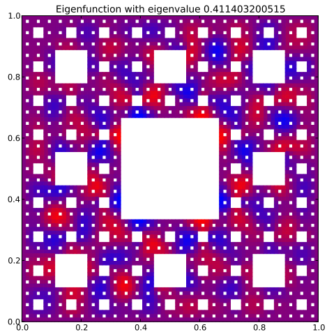
Eigenfunction with eigenvalue 0.411403200515
