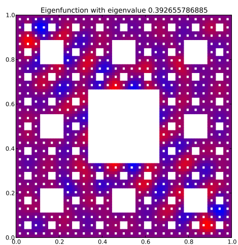
Eigenfunction 86 with eigenvalue 0.392655786885
