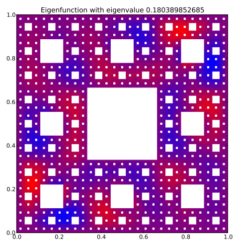
Eigenfunction 34 with eigenvalue 0.180389852685
