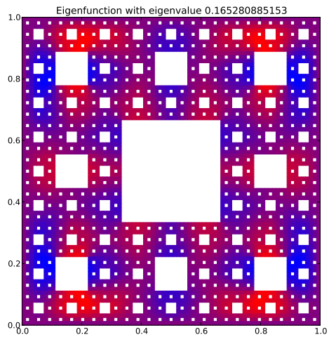
Eigenfunction 31 with eigenvalue 0.165280885153
