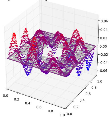
Eigenfunction with eigenvalue 0.217501132366
