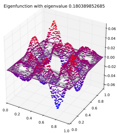
Eigenfunction 35 with eigenvalue 0.180389852685
