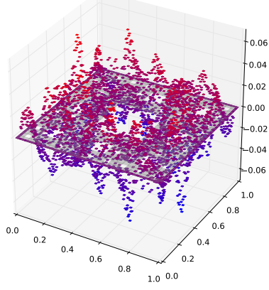
Eigenfunction with eigenvalue 0.564997851529
