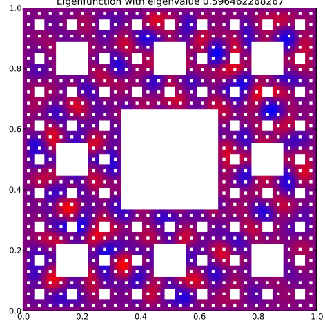
Eigenfunction with eigenvalue 0.596462268267
