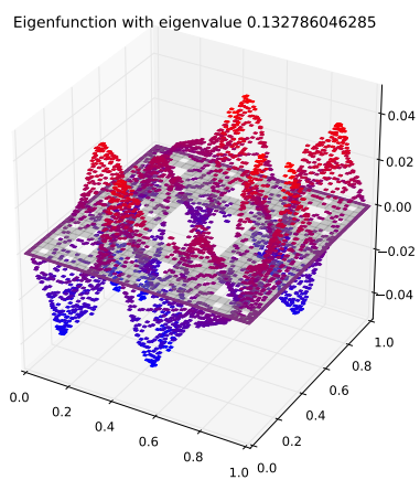
Eigenfunction 21 with eigenvalue 0.132786046285
