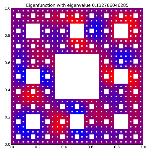
Eigenfunction 21 with eigenvalue 0.132786046285
