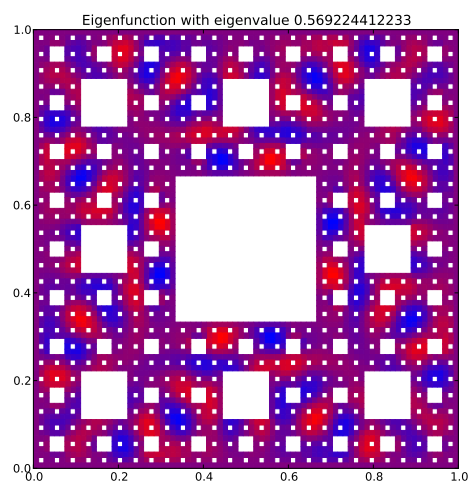
Eigenfunction 134 with eigenvalue 0.569224412233
