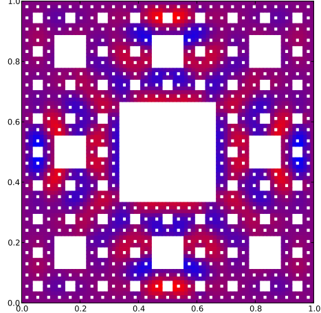
Eigenfunction with eigenvalue 0.379167854833
