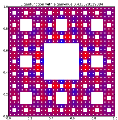
Eigenfunction 101 with eigenvalue 0.433528119084
