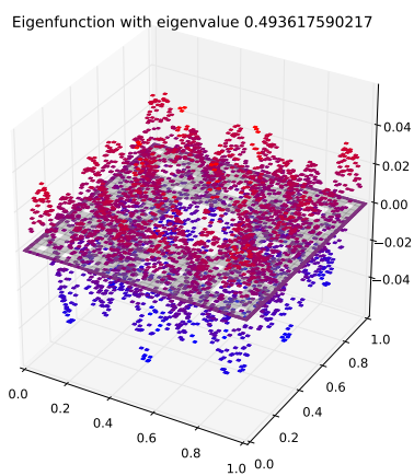
Eigenfunction 113 with eigenvalue 0.493617590217
