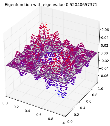
Eigenfunction 121 with eigenvalue 0.52040657371
