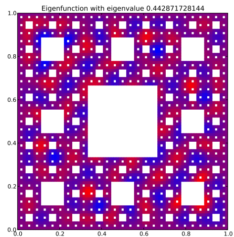
Eigenfunction 105 with eigenvalue 0.442871728144
