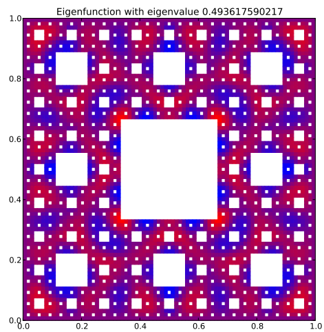
Eigenfunction 113 with eigenvalue 0.493617590217
