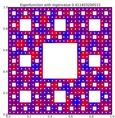
Eigenfunction 94 with eigenvalue 0.411403200515
