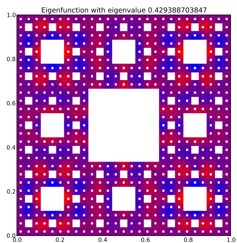
Eigenfunction 100 with eigenvalue 0.429388703847
