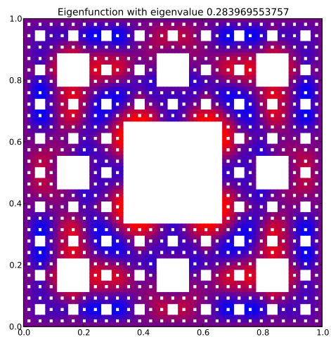
Eigenfunction 59 with eigenvalue 0.283969553757
