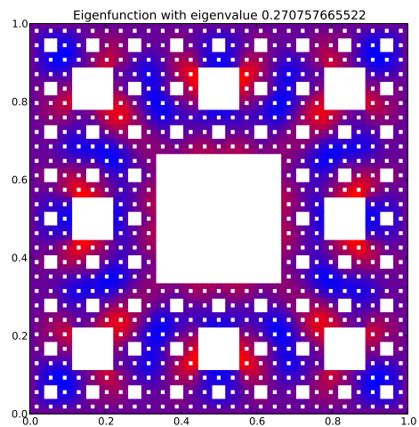
Eigenfunction 53 with eigenvalue 0.270757665522
