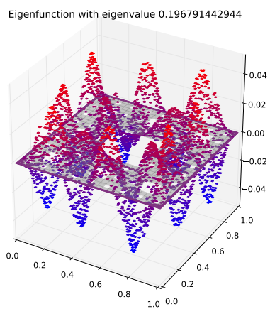
Eigenfunction 37 with eigenvalue 0.196791442944
