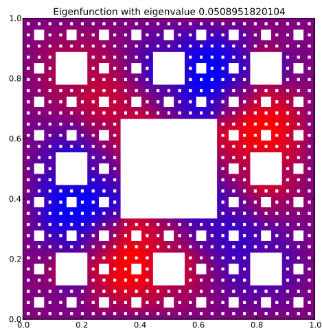
Eigenfunction with eigenvalue 0.0508951820104
