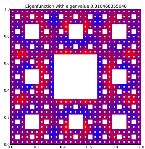
Eigenfunction 64 with eigenvalue 0.310468355648
