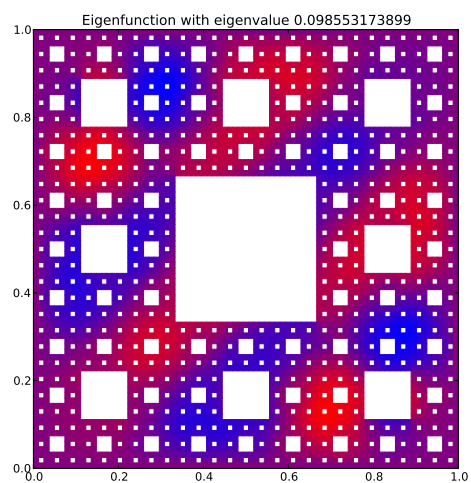
Eigenfunction 14 with eigenvalue 0.098553173899
