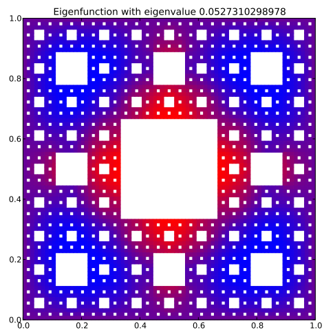
Eigenfunction 7 with eigenvalue 0.0527310298978
