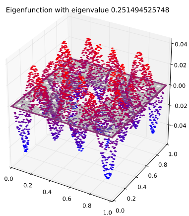
Eigenfunction 49 with eigenvalue 0.251494525748
