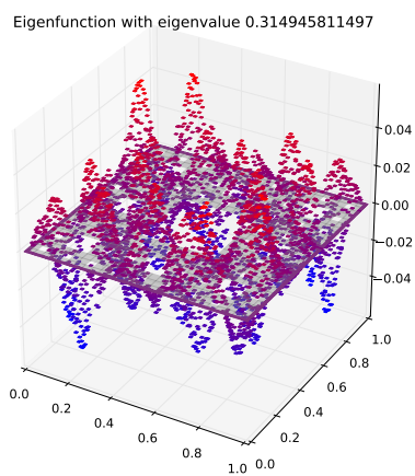
Eigenfunction 65 with eigenvalue 0.314945811497
