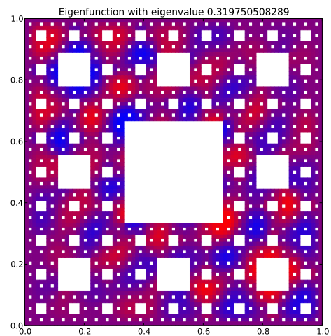
Eigenfunction 67 with eigenvalue 0.319750508289
