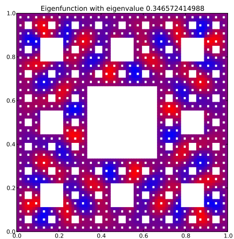
Eigenfunction 73 with eigenvalue 0.346572414988
