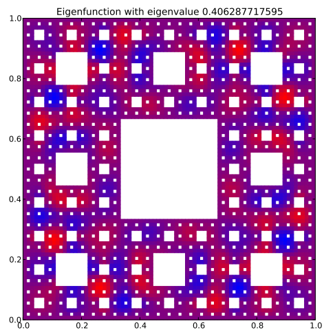
Eigenfunction 91 with eigenvalue 0.406287717595
