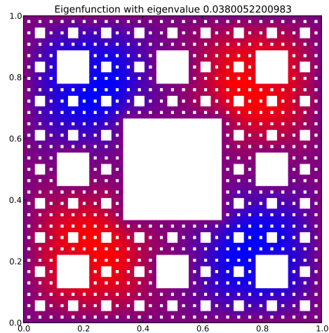
Eigenfunction with eigenvalue 0.0380052200983
