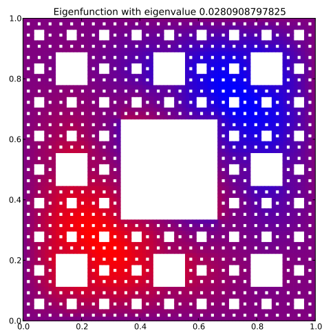
Eigenfunction 3 with eigenvalue 0.0280908797825
