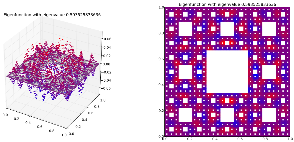
Eigenfunction 141 with eigenvalue 0.593525833636
