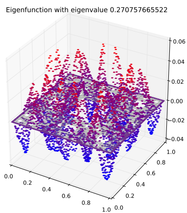
Eigenfunction 53 with eigenvalue 0.270757665522
