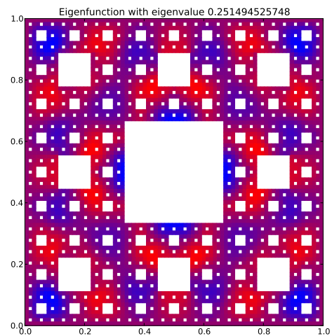
Eigenfunction 49 with eigenvalue 0.251494525748
