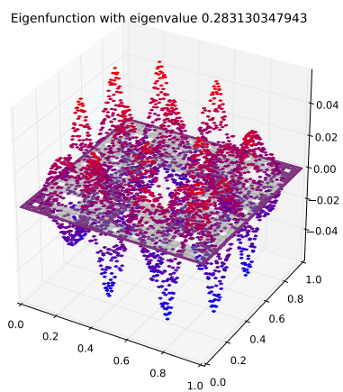
Eigenfunction 57 with eigenvalue 0.283130347943
