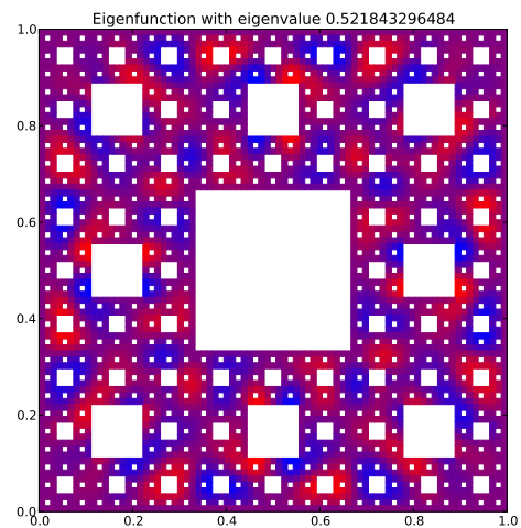
Eigenfunction 123 with eigenvalue 0.521843296484
