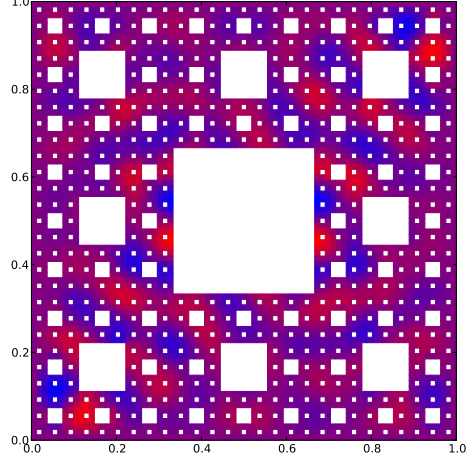
Eigenfunction with eigenvalue 0.392655786885
