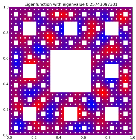
Eigenfunction 51 with eigenvalue 0.25743097301
