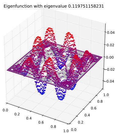
Eigenfunction 17 with eigenvalue 0.119751158231
