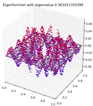
Eigenfunction 77 with eigenvalue 0.363551703399
