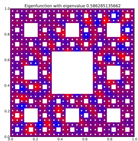
Eigenfunction 138 with eigenvalue 0.586285135662
