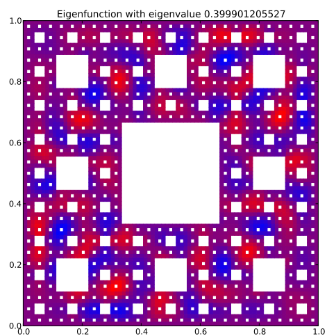
Eigenfunction 88 with eigenvalue 0.399901205527
