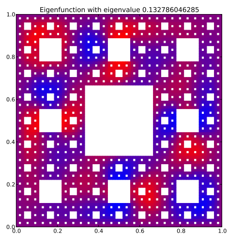
Eigenfunction 22 with eigenvalue 0.132786046285
