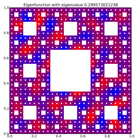
Eigenfunction 61 with eigenvalue 0.299573021238
