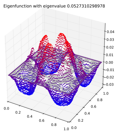
Eigenfunction 7 with eigenvalue 0.0527310298978
