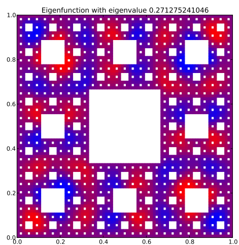
Eigenfunction 54 with eigenvalue 0.271275241046
