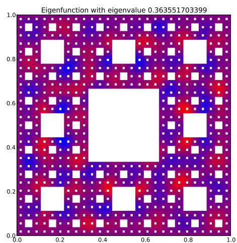
Eigenfunction 78 with eigenvalue 0.363551703399
