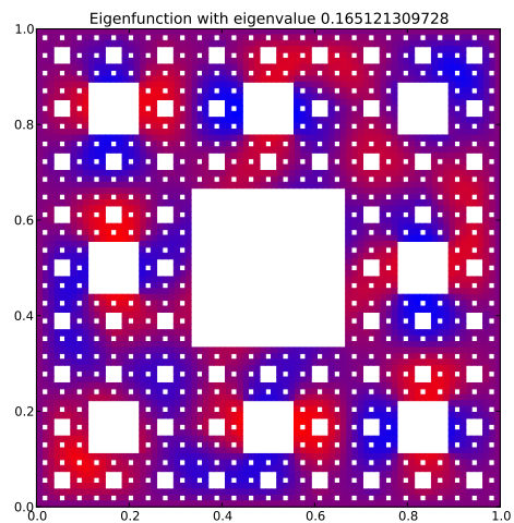
Eigenfunction 29 with eigenvalue 0.165121309728
