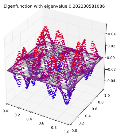
Eigenfunction 39 with eigenvalue 0.202230581086
