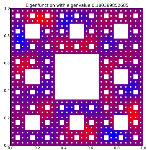
Eigenfunction 35 with eigenvalue 0.180389852685
