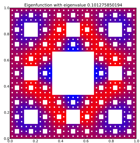
Eigenfunction 15 with eigenvalue 0.101275850194
