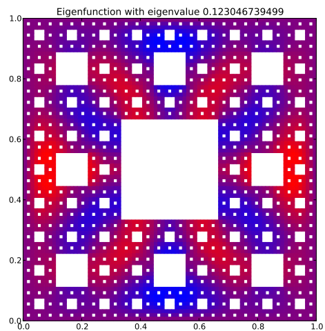
Eigenfunction 19 with eigenvalue 0.123046739499
