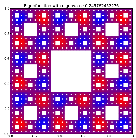
Eigenfunction 48 with eigenvalue 0.245762452276
