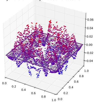
Eigenfunction with eigenvalue 0.407668364622
