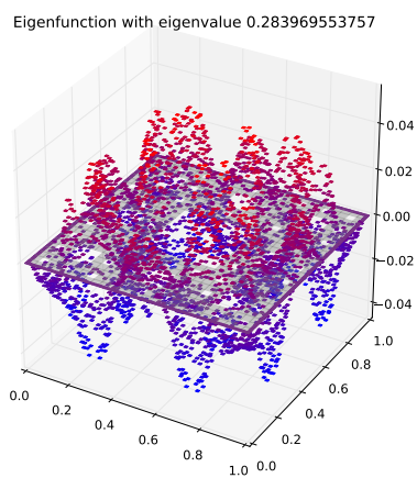
Eigenfunction 59 with eigenvalue 0.283969553757
