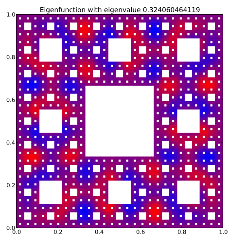
Eigenfunction 68 with eigenvalue 0.324060464119
