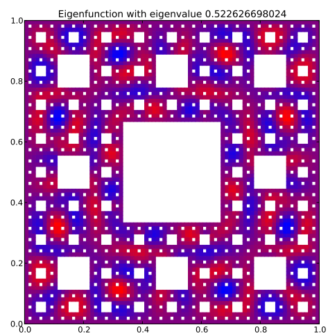
Eigenfunction 124 with eigenvalue 0.522626698024
