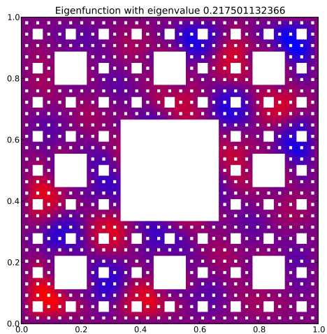
Eigenfunction with eigenvalue 0.217501132366
