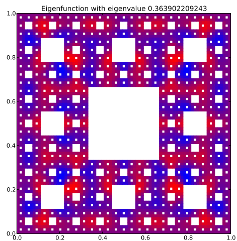
Eigenfunction 79 with eigenvalue 0.363902209243
