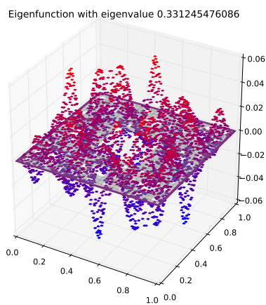
Eigenfunction 69 with eigenvalue 0.331245476086
