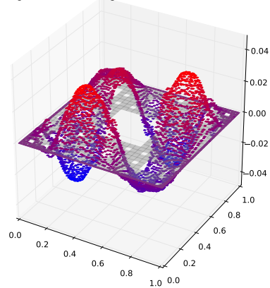
Eigenfunction with eigenvalue 0.0508951820104
