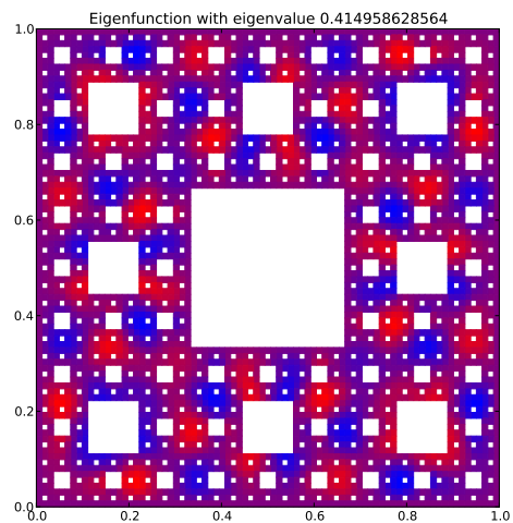
Eigenfunction 95 with eigenvalue 0.414958628564
