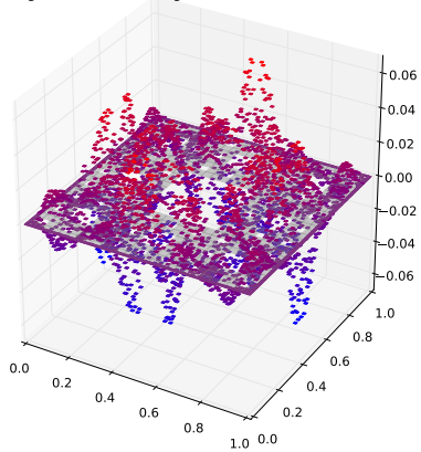
Eigenfunction with eigenvalue 0.379167854833
