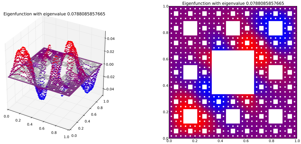
Eigenfunction 10 with eigenvalue 0.0788085857665
