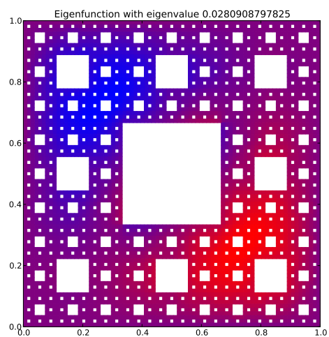
Eigenfunction 2 with eigenvalue 0.0280908797825
