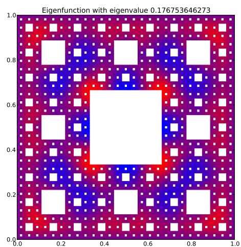
Eigenfunction 32 with eigenvalue 0.176753646273
