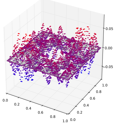
Eigenfunction with eigenvalue 0.436817242062
