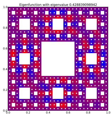
Eigenfunction 98 with eigenvalue 0.428839098942
