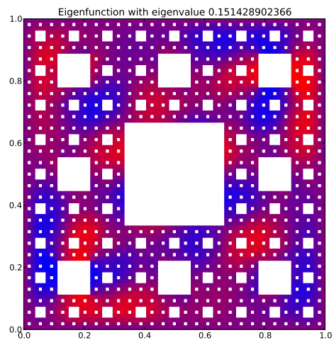
Eigenfunction 25 with eigenvalue 0.151428902366
