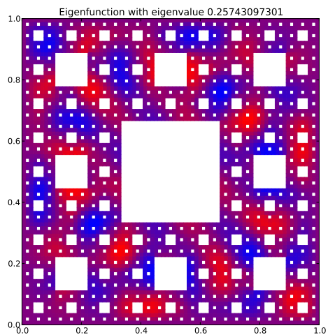
Eigenfunction 50 with eigenvalue 0.25743097301
