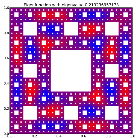
Eigenfunction 43 with eigenvalue 0.219236957173
