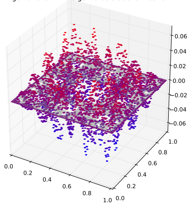
Eigenfunction with eigenvalue 0.596462268267
