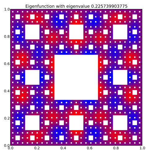
Eigenfunction 44 with eigenvalue 0.225739903775
