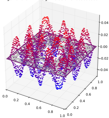
Eigenfunction with eigenvalue 0.232663696599
