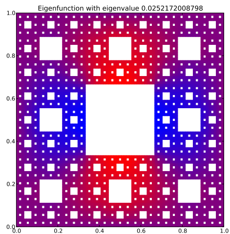
Eigenfunction 1 with eigenvalue 0.0252172008798
