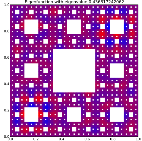
Eigenfunction with eigenvalue 0.436817242062
