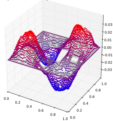
Eigenfunction with eigenvalue 0.0380052200983
