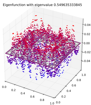
Eigenfunction 129 with eigenvalue 0.549635333845
