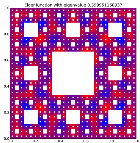
Eigenfunction 89 with eigenvalue 0.399951168937
