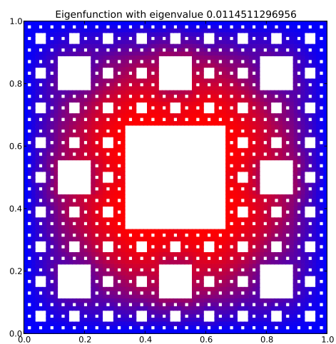
Eigenfunction 0 with eigenvalue 0.0114511296956
