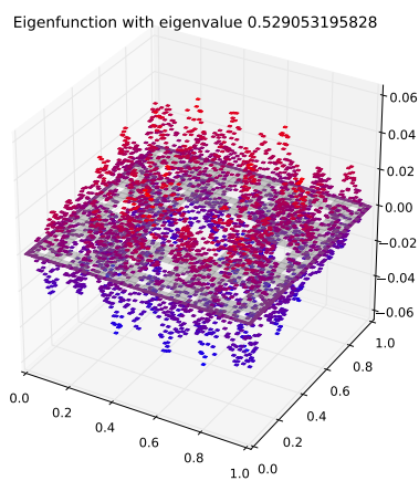
Eigenfunction 125 with eigenvalue 0.529053195828
