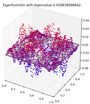
Eigenfunction 99 with eigenvalue 0.428839098942
