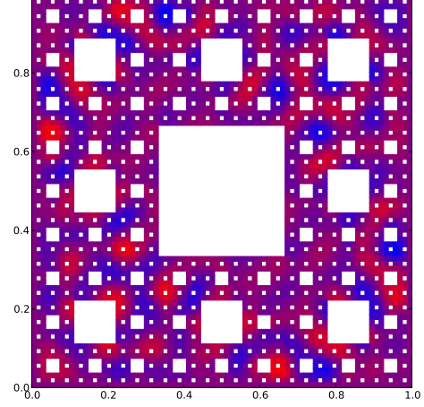
Eigenfunction with eigenvalue 0.564997851529
