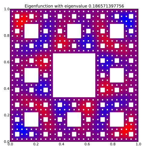
Eigenfunction 36 with eigenvalue 0.186571397756
