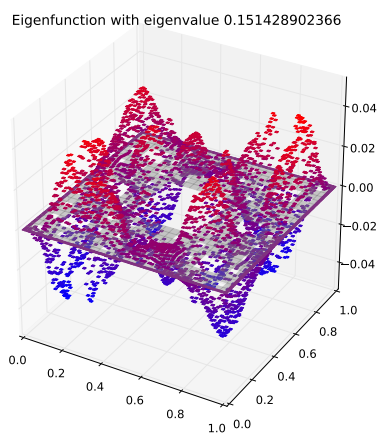
Eigenfunction 25 with eigenvalue 0.151428902366
