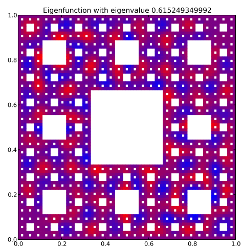
Eigenfunction 148 with eigenvalue 0.615249349992
