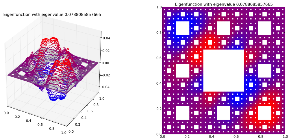
Eigenfunction 11 with eigenvalue 0.0788085857665
