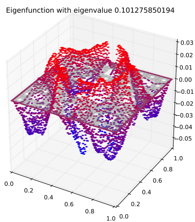
Eigenfunction 15 with eigenvalue 0.101275850194
