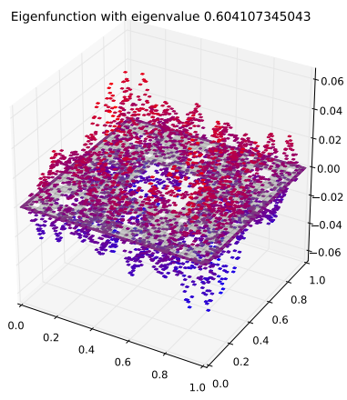
Eigenfunction 145 with eigenvalue 0.604107345043
