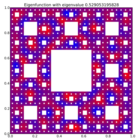
Eigenfunction 125 with eigenvalue 0.529053195828
