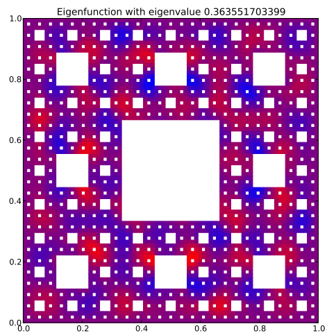
Eigenfunction 77 with eigenvalue 0.363551703399
