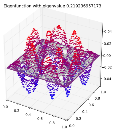
Eigenfunction 43 with eigenvalue 0.219236957173
