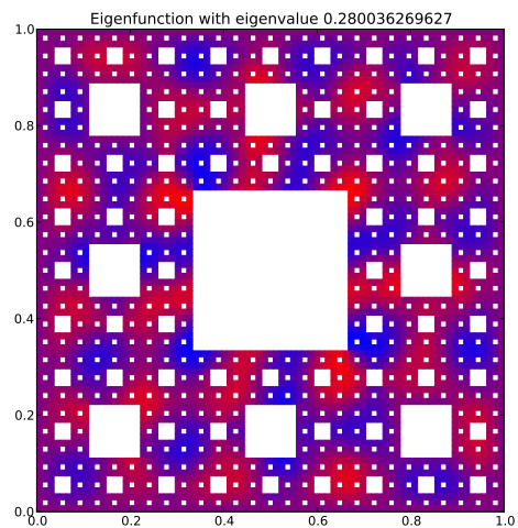
Eigenfunction 55 with eigenvalue 0.280036269627
