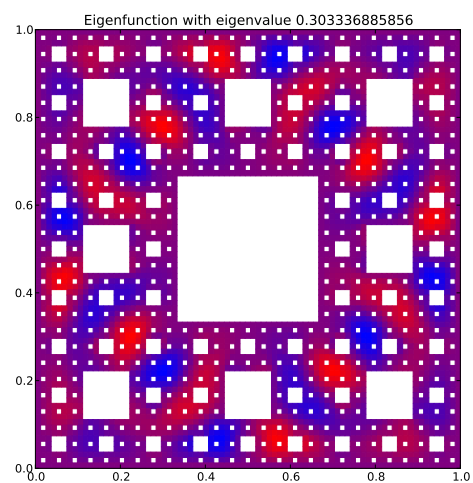
Eigenfunction 62 with eigenvalue 0.303336885856
