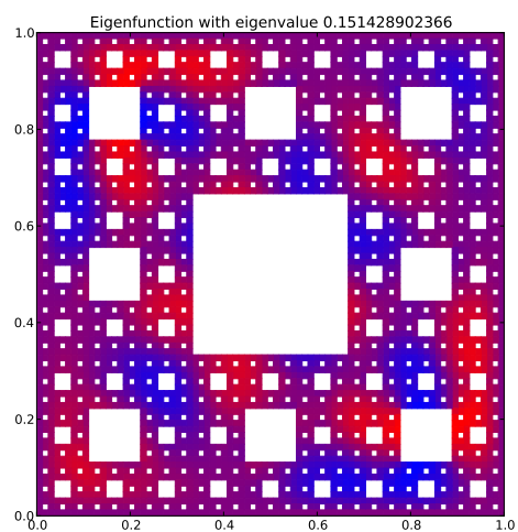
Eigenfunction 26 with eigenvalue 0.151428902366
