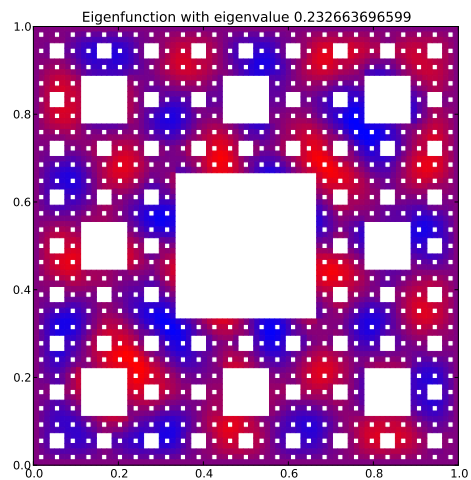
Eigenfunction 45 with eigenvalue 0.232663696599
