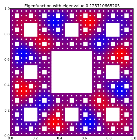
Eigenfunction 20 with eigenvalue 0.125710668205
