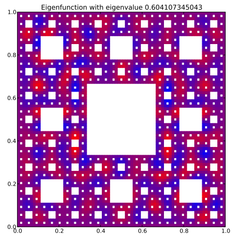
Eigenfunction 145 with eigenvalue 0.604107345043
