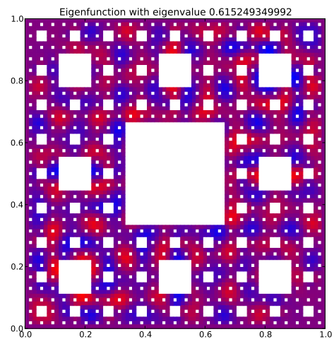
Eigenfunction 149 with eigenvalue 0.615249349992
