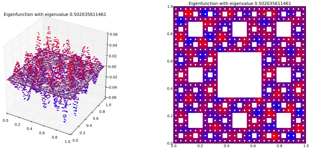
Eigenfunction 116 with eigenvalue 0.502035611461
