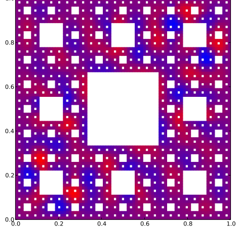
Eigenfunction with eigenvalue 0.360678510889
