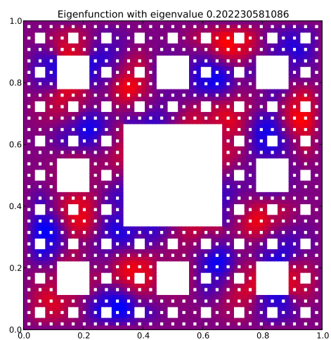
Eigenfunction 38 with eigenvalue 0.202230581086
