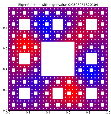
Eigenfunction 6 with eigenvalue 0.0508951820104
