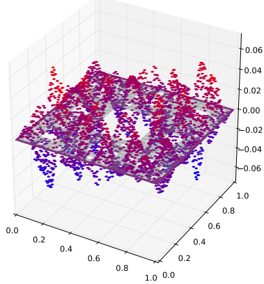
Eigenfunction with eigenvalue 0.360678510889
