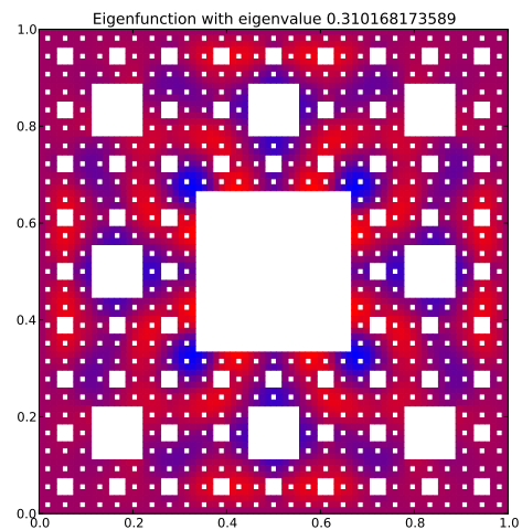
Eigenfunction 63 with eigenvalue 0.310168173589
