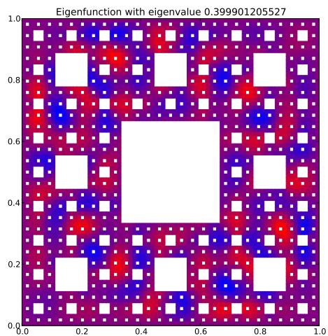
Eigenfunction 87 with eigenvalue 0.399901205527
