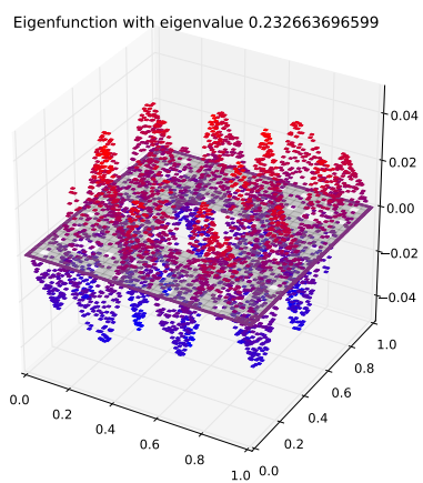
Eigenfunction 45 with eigenvalue 0.232663696599
