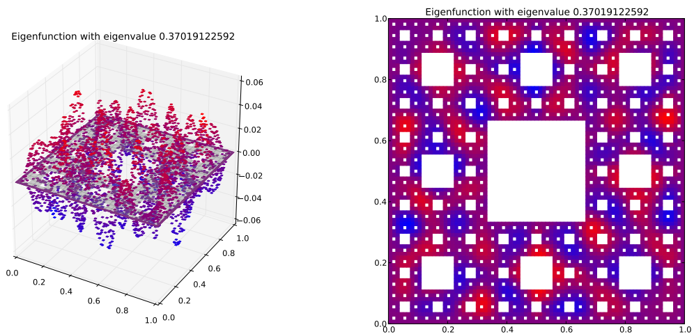
Eigenfunction 82 with eigenvalue 0.37019122592
