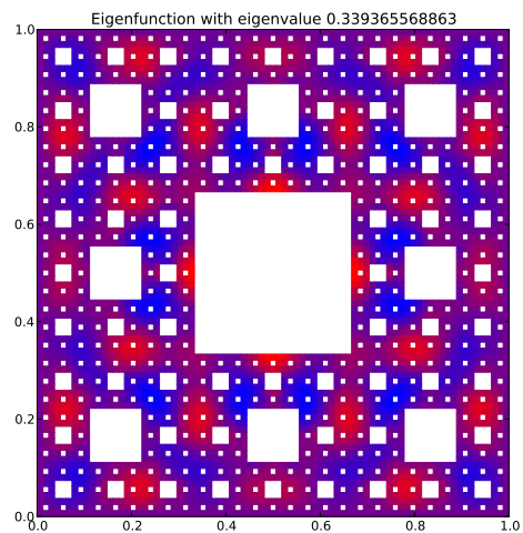
Eigenfunction 71 with eigenvalue 0.339365568863
