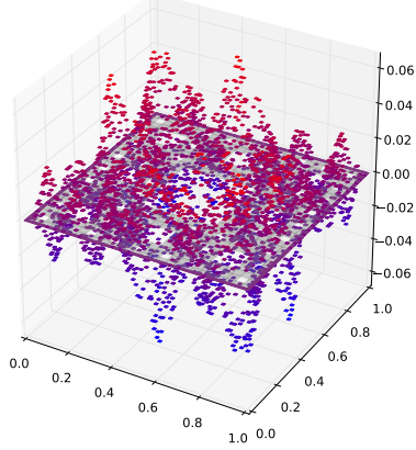
Eigenfunction with eigenvalue 0.577741707105
