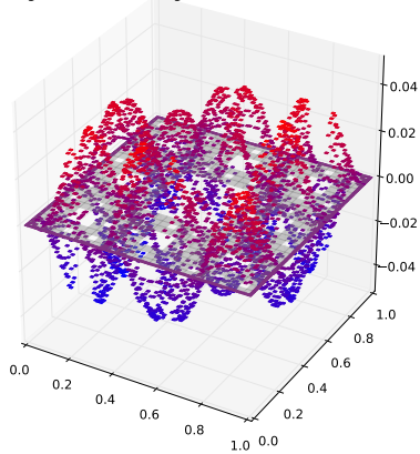
Eigenfunction with eigenvalue 0.165121309728
