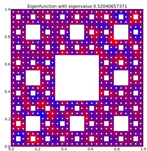
Eigenfunction 122 with eigenvalue 0.52040657371
