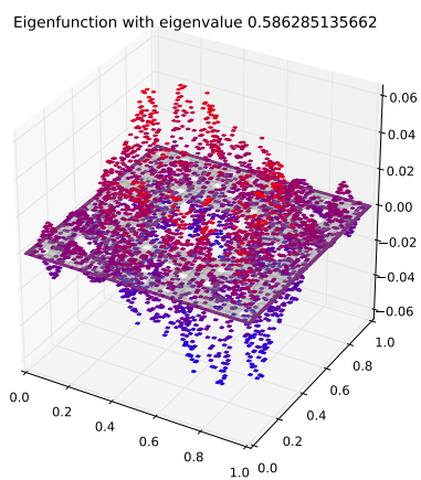
Eigenfunction 139 with eigenvalue 0.586285135662
