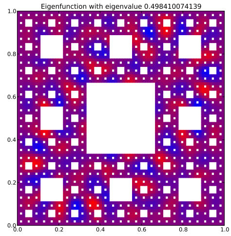
Eigenfunction 115 with eigenvalue 0.498410074139
