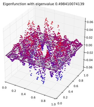
Eigenfunction 115 with eigenvalue 0.498410074139
