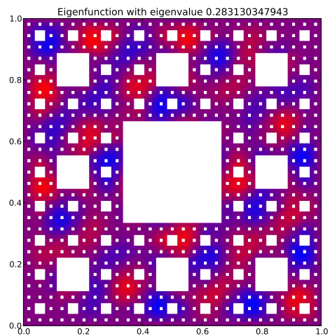
Eigenfunction 57 with eigenvalue 0.283130347943
