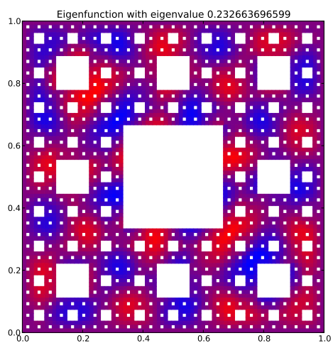
Eigenfunction 46 with eigenvalue 0.232663696599
