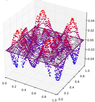
Eigenfunction with eigenvalue 0.165280885153
