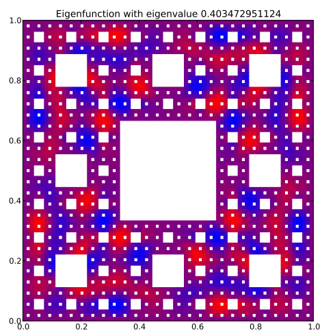
Eigenfunction 90 with eigenvalue 0.403472951124
