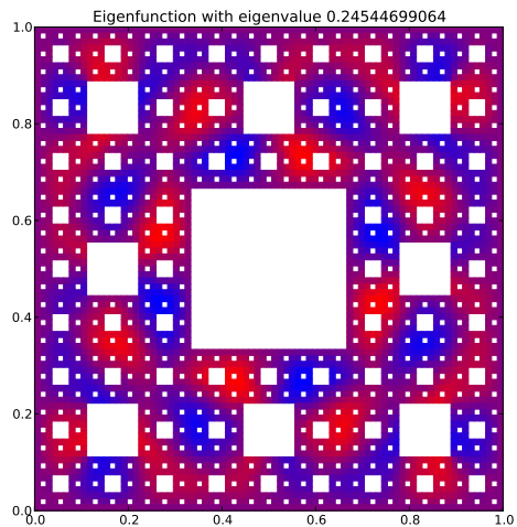
Eigenfunction 47 with eigenvalue 0.24544699064
