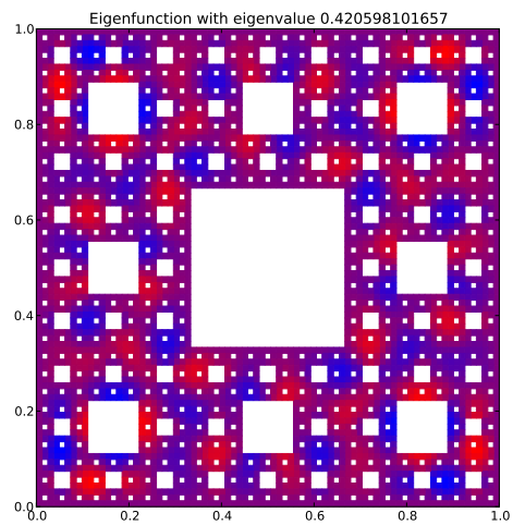
Eigenfunction 97 with eigenvalue 0.420598101657
