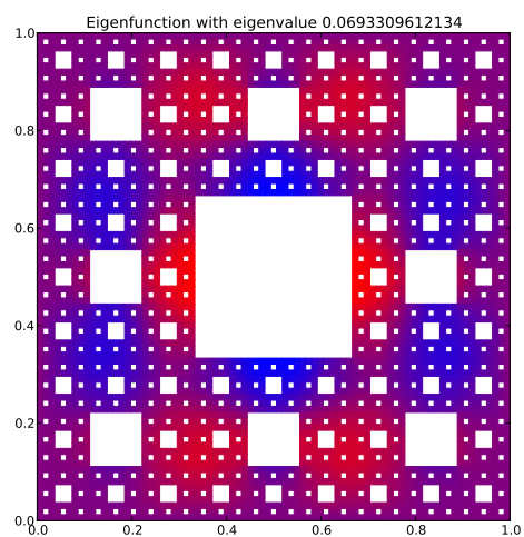
Eigenfunction 8 with eigenvalue 0.0693309612134
