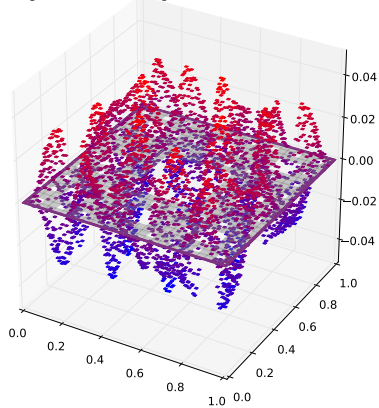
Eigenfunction with eigenvalue 0.24544699064
