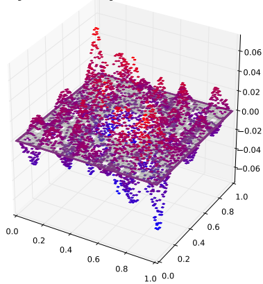
Eigenfunction with eigenvalue 0.392655786885
