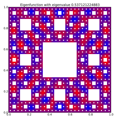
Eigenfunction 128 with eigenvalue 0.537121224883
