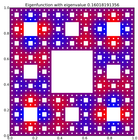
Eigenfunction 27 with eigenvalue 0.16018191356
