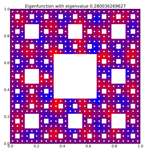
Eigenfunction 56 with eigenvalue 0.280036269627
