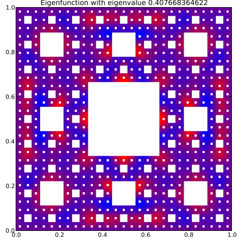
Eigenfunction with eigenvalue 0.407668364622
