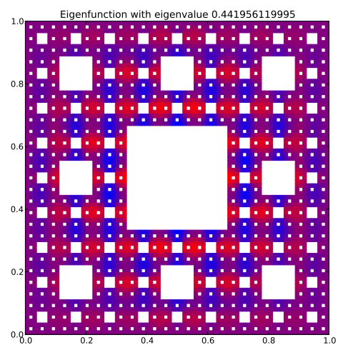
Eigenfunction 104 with eigenvalue 0.441956119995
