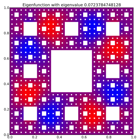
Eigenfunction 9 with eigenvalue 0.0723784748128
