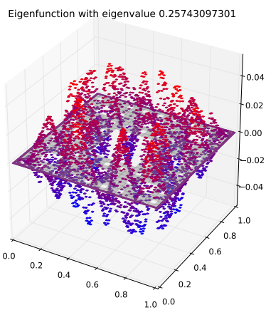
Eigenfunction 51 with eigenvalue 0.25743097301
