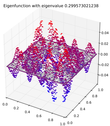
Eigenfunction 61 with eigenvalue 0.299573021238
