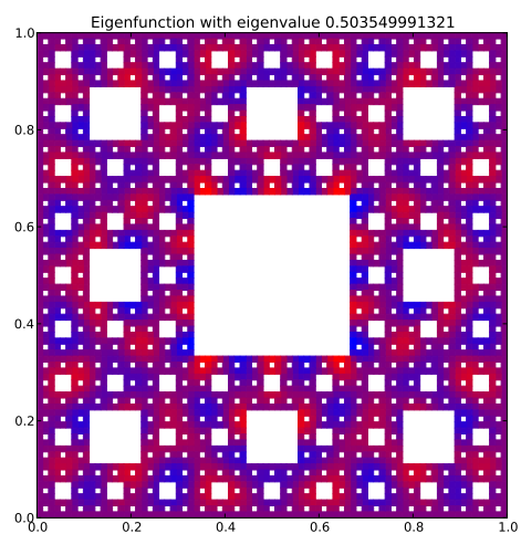
Eigenfunction 118 with eigenvalue 0.503549991321
