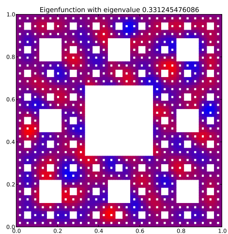
Eigenfunction 70 with eigenvalue 0.331245476086
