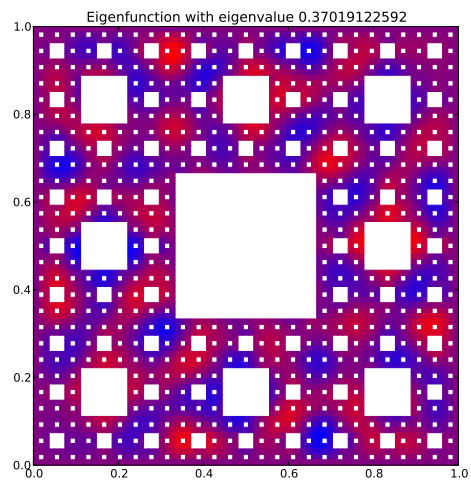
Eigenfunction 81 with eigenvalue 0.37019122592
