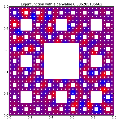
Eigenfunction 139 with eigenvalue 0.586285135662
