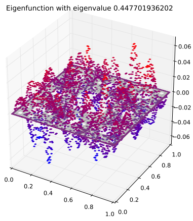
Eigenfunction 109 with eigenvalue 0.447701936202
