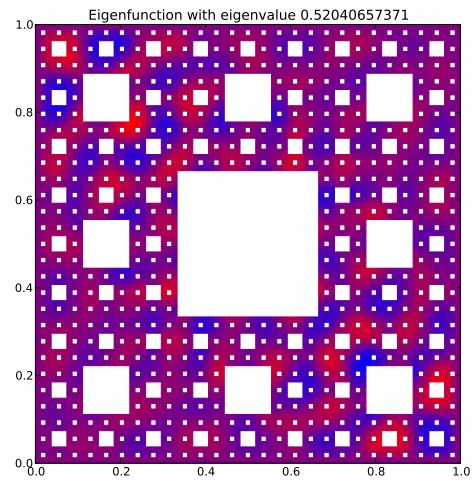
Eigenfunction 121 with eigenvalue 0.52040657371
