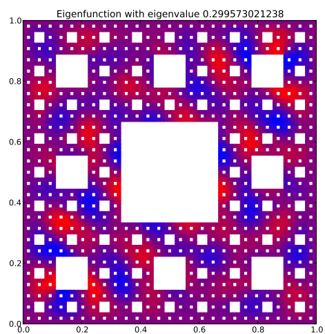
Eigenfunction 60 with eigenvalue 0.299573021238
