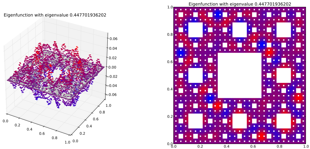
Eigenfunction 110 with eigenvalue 0.447701936202
