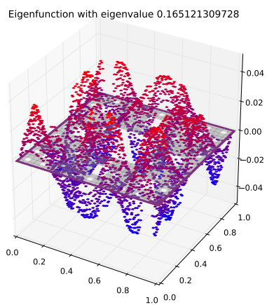
Eigenfunction 29 with eigenvalue 0.165121309728
