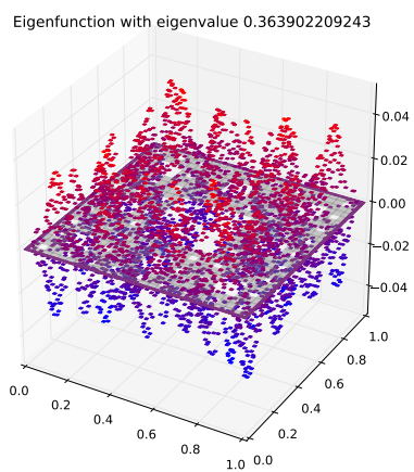
Eigenfunction 79 with eigenvalue 0.363902209243
