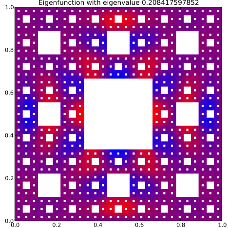
Eigenfunction with eigenvalue 0.208417597852
