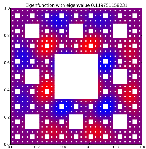
Eigenfunction 17 with eigenvalue 0.119751158231
