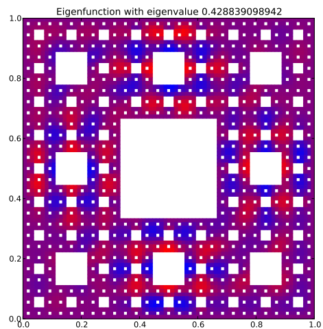
Eigenfunction 99 with eigenvalue 0.428839098942
