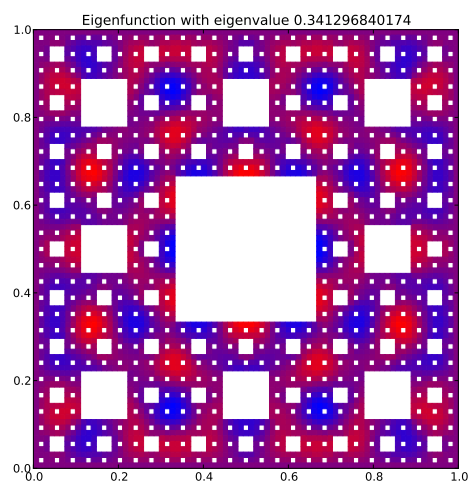
Eigenfunction 72 with eigenvalue 0.341296840174
