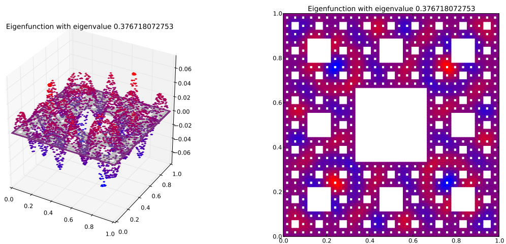
Eigenfunction 83 with eigenvalue 0.376718072753
