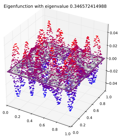
Eigenfunction 73 with eigenvalue 0.346572414988
