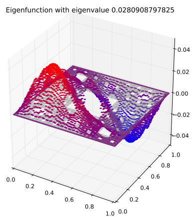
Eigenfunction 3 with eigenvalue 0.0280908797825
