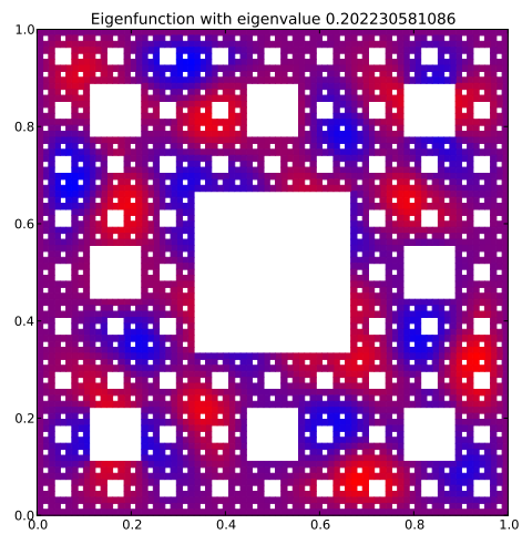
Eigenfunction 39 with eigenvalue 0.202230581086
