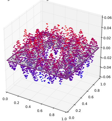
Eigenfunction with eigenvalue 0.411403200515
