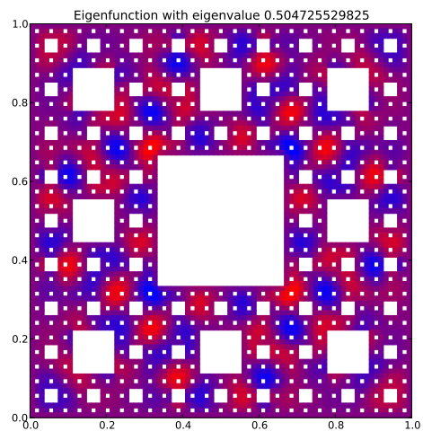
Eigenfunction 119 with eigenvalue 0.504725529825
