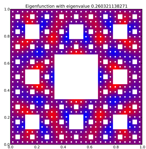
Eigenfunction 52 with eigenvalue 0.260321138271
