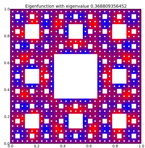
Eigenfunction 80 with eigenvalue 0.368809356452
