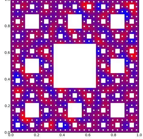
Eigenfunction with eigenvalue 0.577741707105
