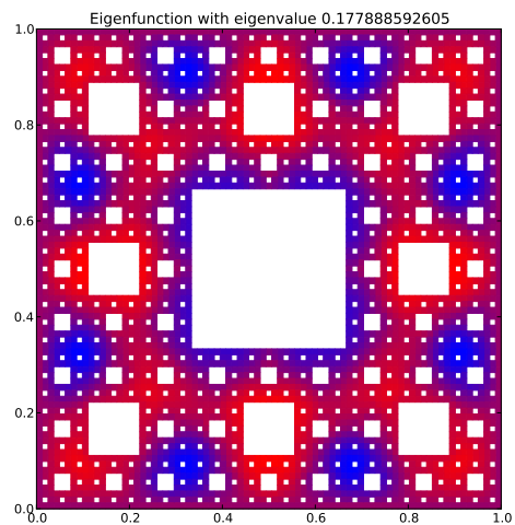
Eigenfunction 33 with eigenvalue 0.177888592605
