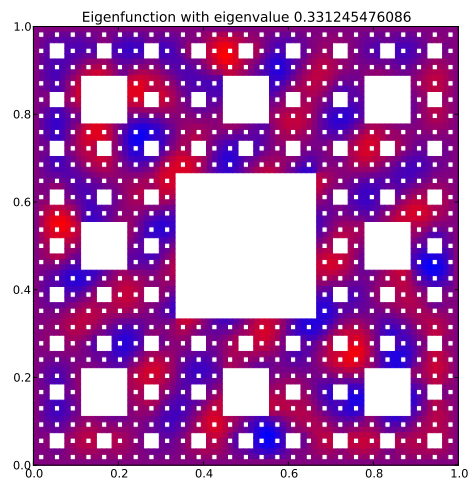
Eigenfunction 69 with eigenvalue 0.331245476086
