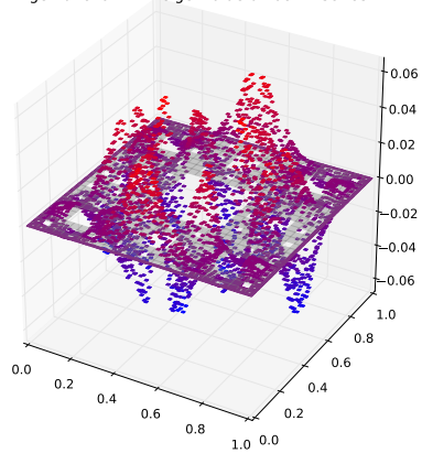
Eigenfunction with eigenvalue 0.208417597852
