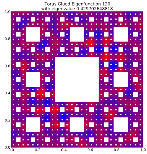
Eigenfunction 120 with eigenvalue 0.429702648818
