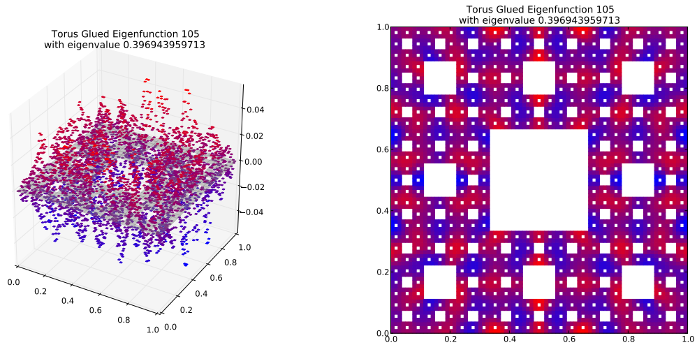
Eigenfunction 105 with eigenvalue 0.396943959713
