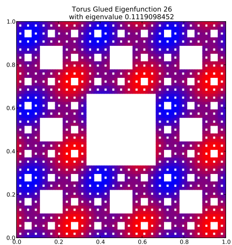
Eigenfunction 26 with eigenvalue 0.1119098452
