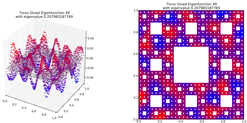
Eigenfunction 49 with eigenvalue 0.207983187769
