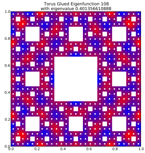
Eigenfunction 108 with eigenvalue 0.401356610888
