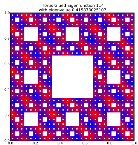
Eigenfunction 114 with eigenvalue 0.415878025107
