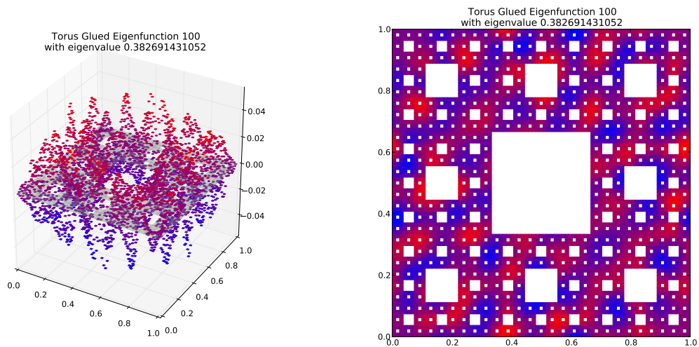
Eigenfunction 100 with eigenvalue 0.382691431052
