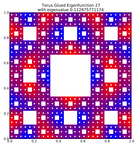
Eigenfunction 27 with eigenvalue 0.112975771174
