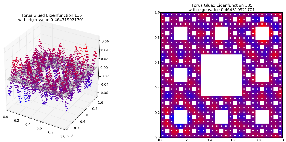
Eigenfunction 135 with eigenvalue 0.464319921701
