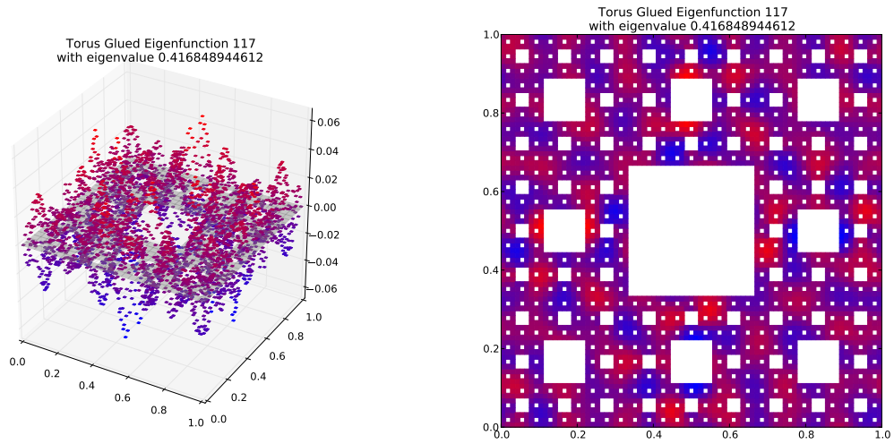
Eigenfunction 117 with eigenvalue 0.416848944612
