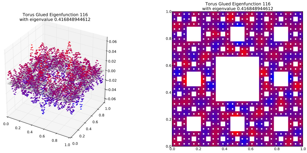
Eigenfunction 116 with eigenvalue 0.416848944612
