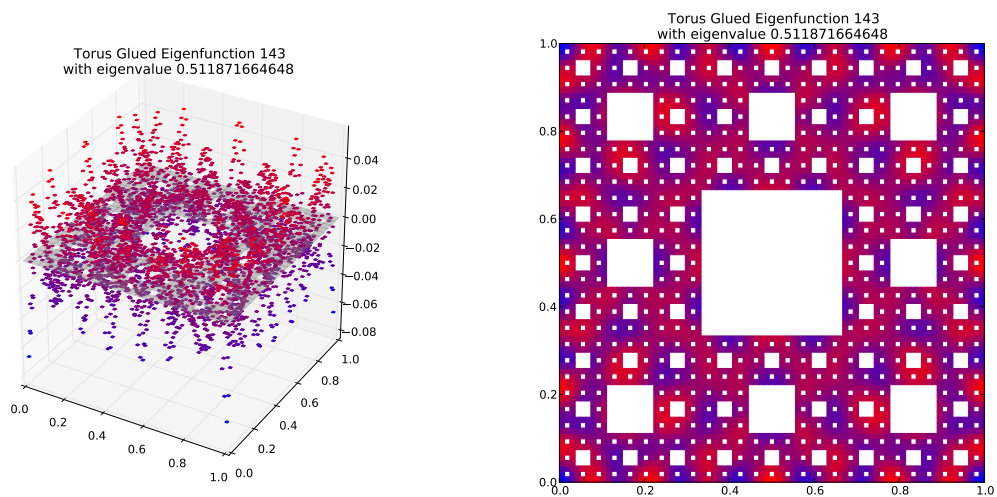
Eigenfunction 143 with eigenvalue 0.511871664648
