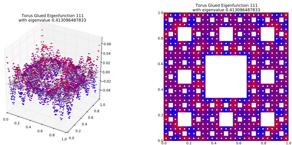
Eigenfunction 111 with eigenvalue 0.413096487833
