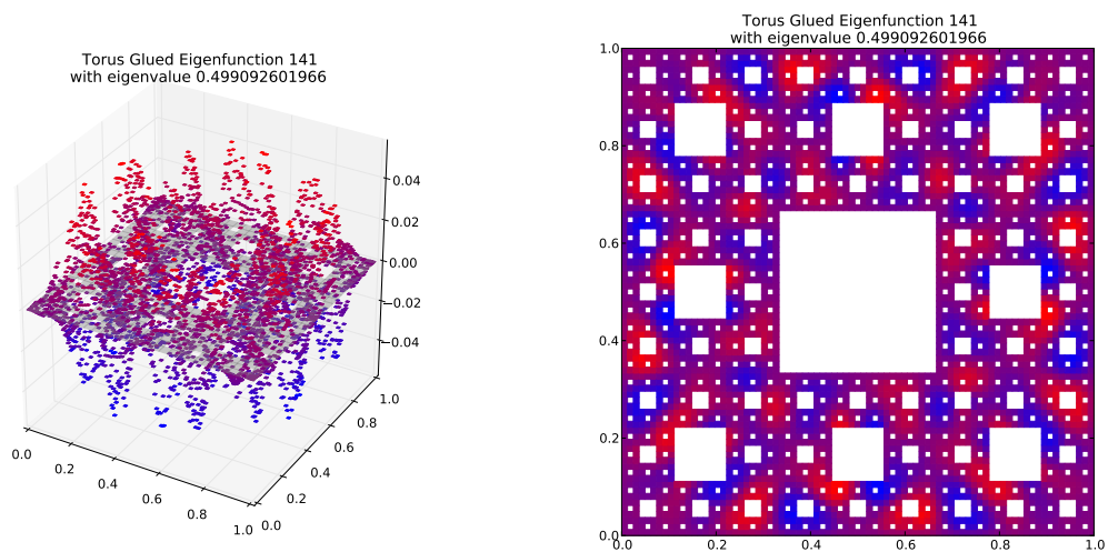
Eigenfunction 141 with eigenvalue 0.499092601966
