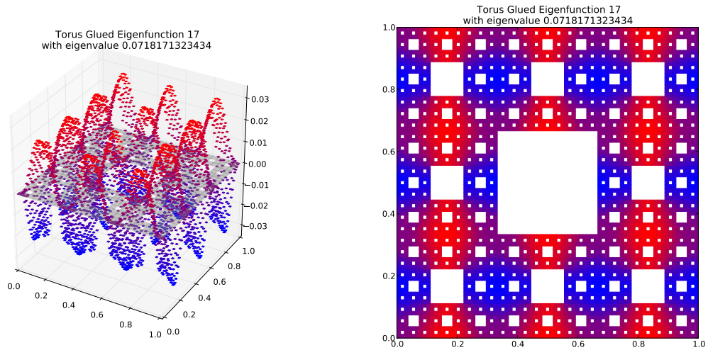
Eigenfunction 17 with eigenvalue 0.0718171323434
