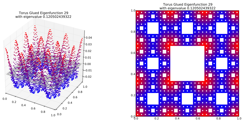
Eigenfunction 29 with eigenvalue 0.120502439322
