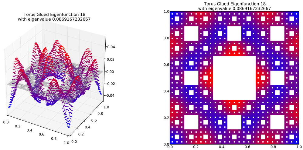
Eigenfunction 18 with eigenvalue 0.0869167232667
