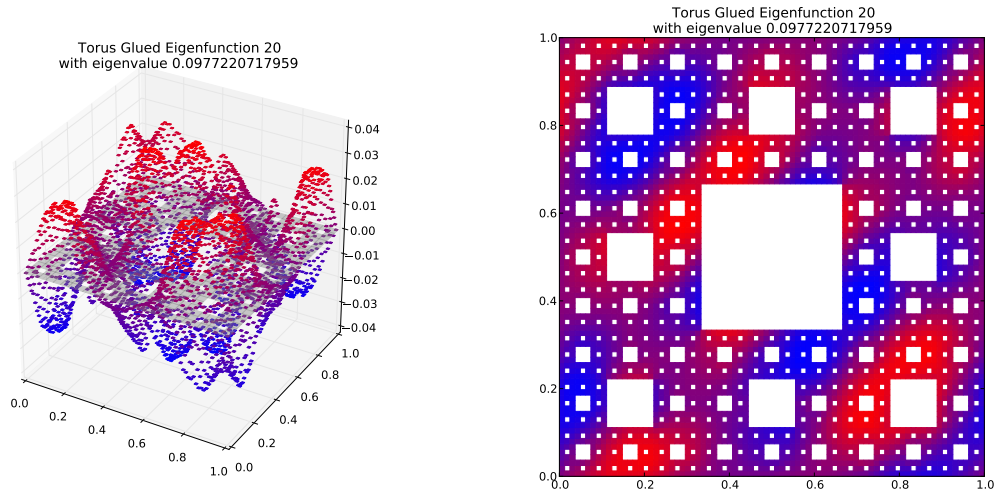
Eigenfunction 20 with eigenvalue 0.0977220717959
