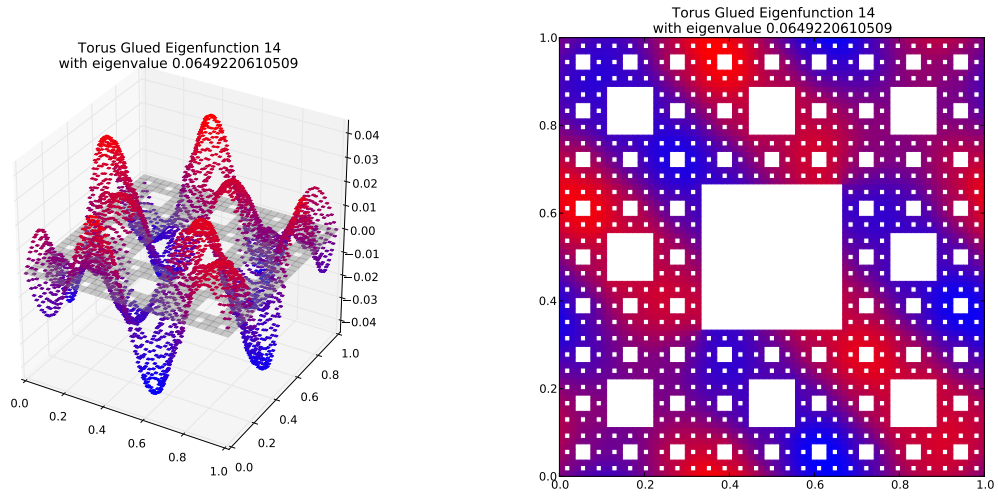
Eigenfunction 14 with eigenvalue 0.0649220610509
