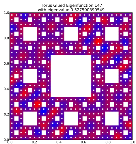
Eigenfunction 147 with eigenvalue 0.527590390549
