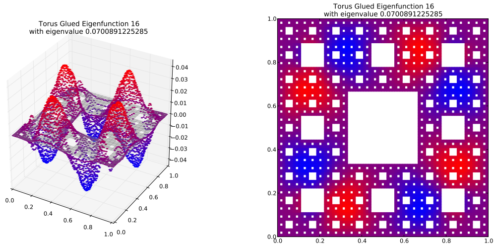
Eigenfunction 16 with eigenvalue 0.0700891225285
