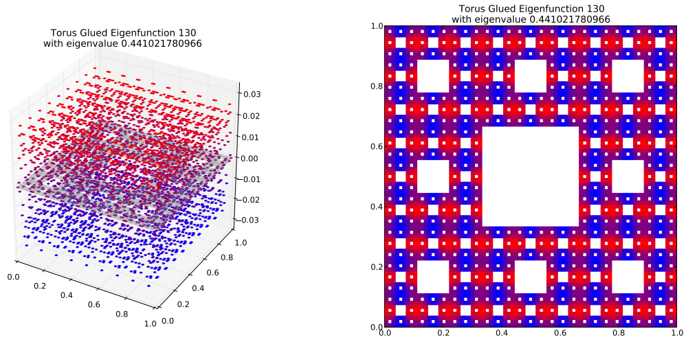
Eigenfunction 130 with eigenvalue 0.441021780966
