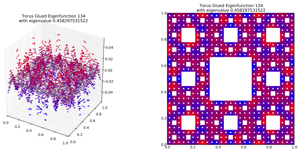
Eigenfunction 134 with eigenvalue 0.458297531522
