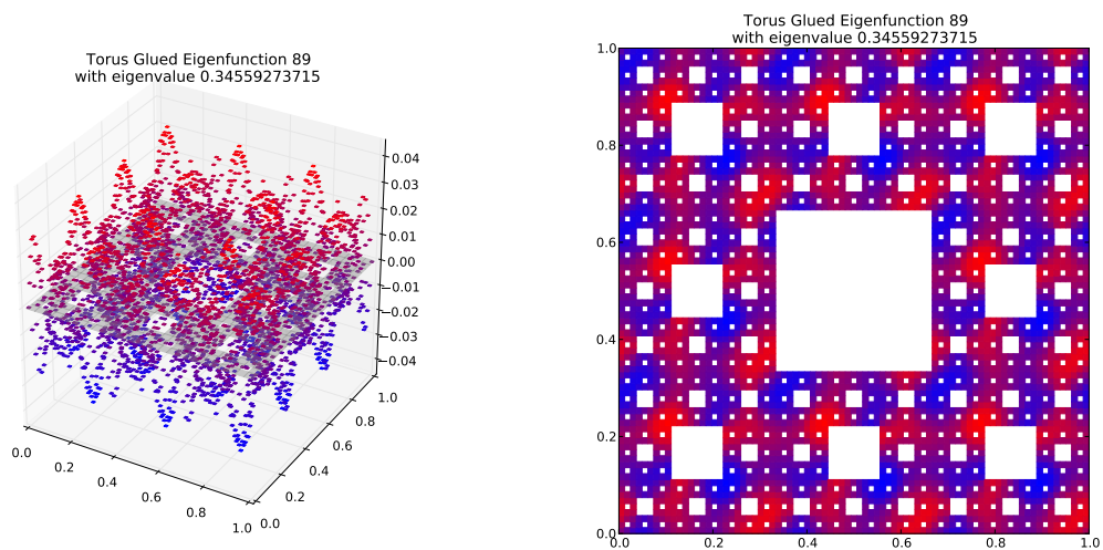
Eigenfunction 89 with eigenvalue 0.34559273715
