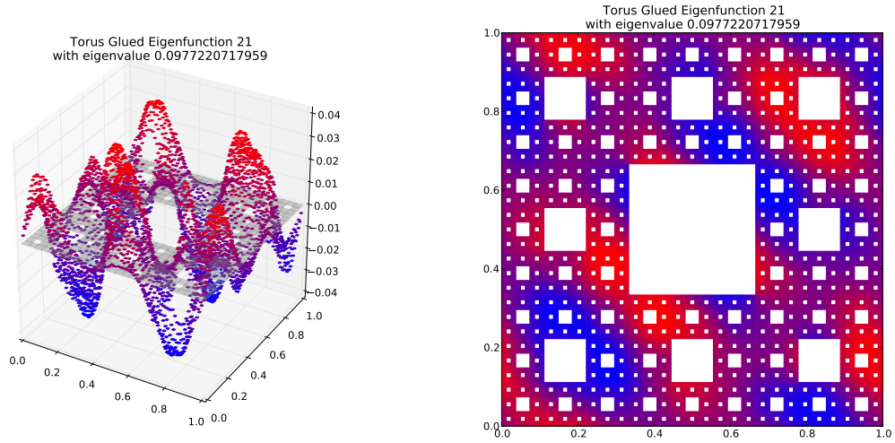
Eigenfunction 21 with eigenvalue 0.0977220717959
