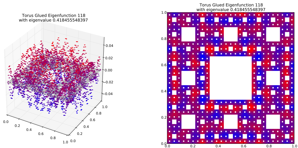
Eigenfunction 118 with eigenvalue 0.418455548397
