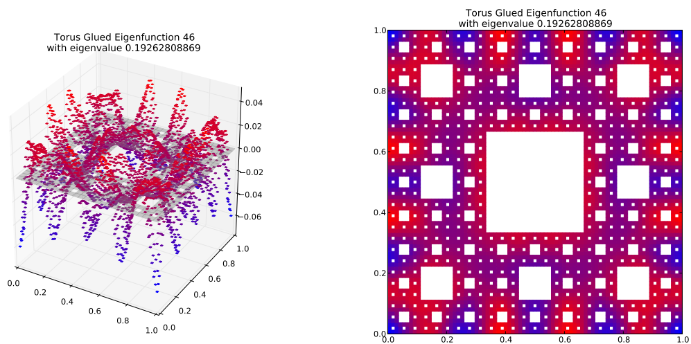
Eigenfunction 46 with eigenvalue 0.19262808869
