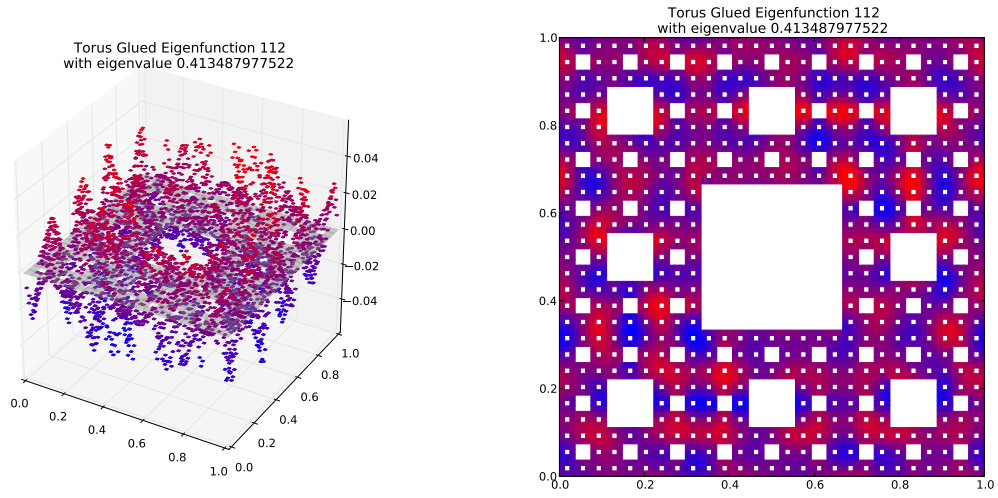
Eigenfunction 112 with eigenvalue 0.413487977522
