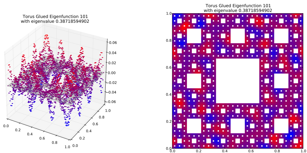
Eigenfunction 101 with eigenvalue 0.38718594902
