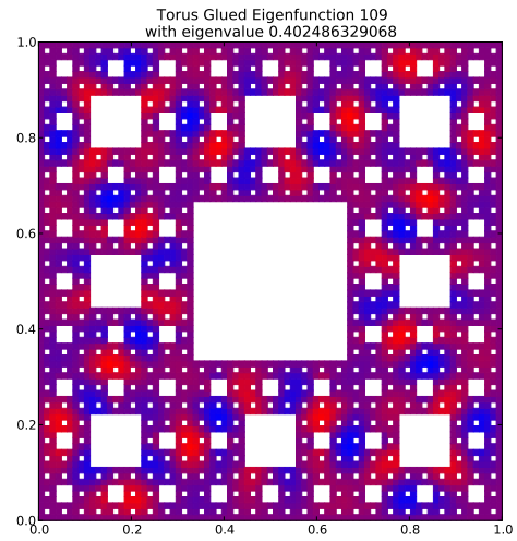
Eigenfunction 109 with eigenvalue 0.402486329068
