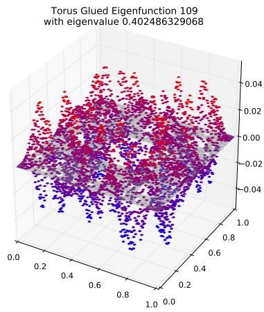
Eigenfunction 109 with eigenvalue 0.402486329068
