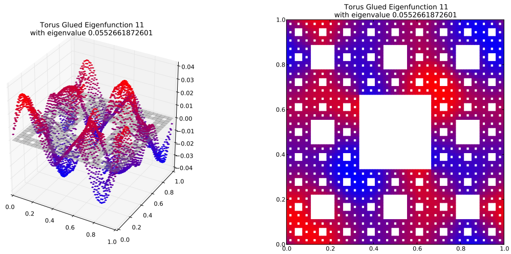
Eigenfunction 11 with eigenvalue 0.0552661872601
