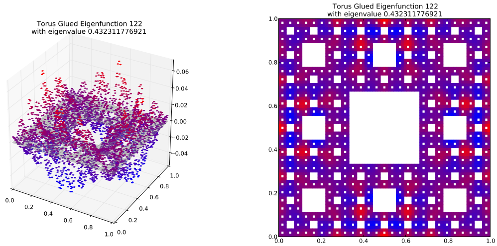
Eigenfunction 122 with eigenvalue 0.432311776921
