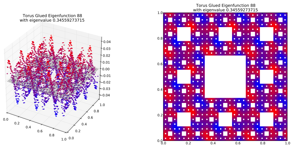
Eigenfunction 88 with eigenvalue 0.34559273715
