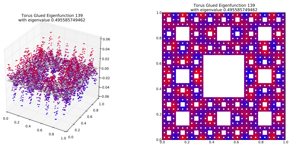
Eigenfunction 139 with eigenvalue 0.495585749462
