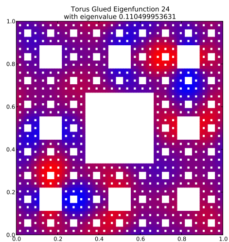
Eigenfunction 24 with eigenvalue 0.110499953631
