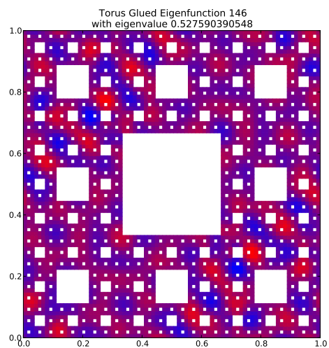
Eigenfunction 146 with eigenvalue 0.527590390548
