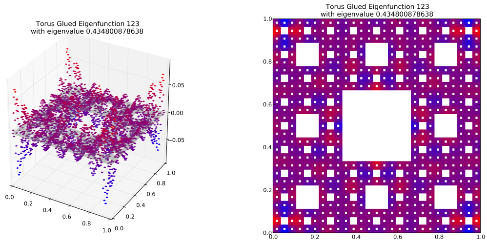
Eigenfunction 123 with eigenvalue 0.434800878638
