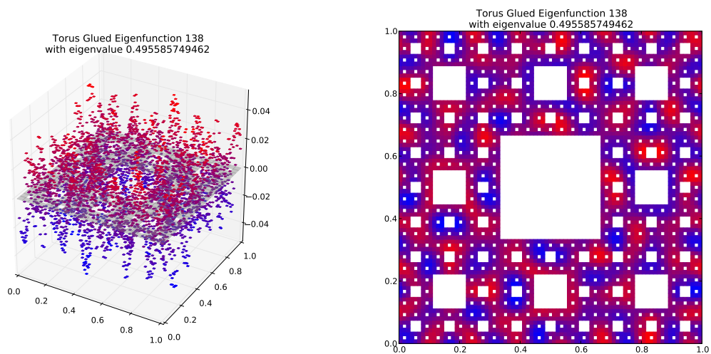
Eigenfunction 138 with eigenvalue 0.495585749462
