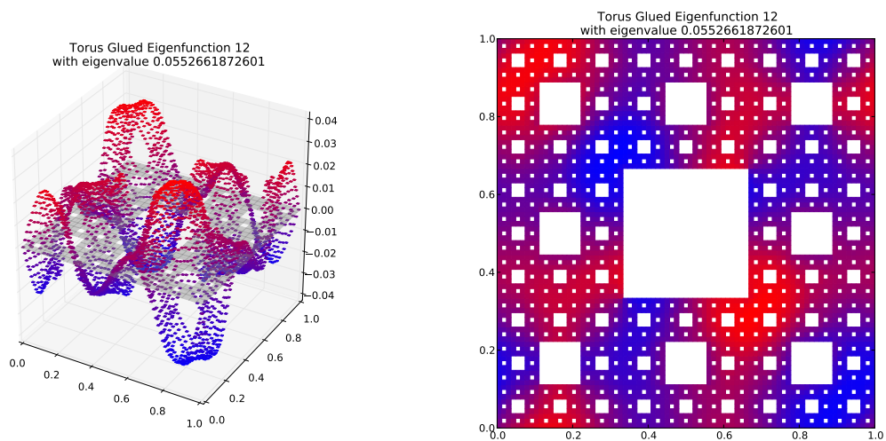
Eigenfunction 12 with eigenvalue 0.0552661872601
