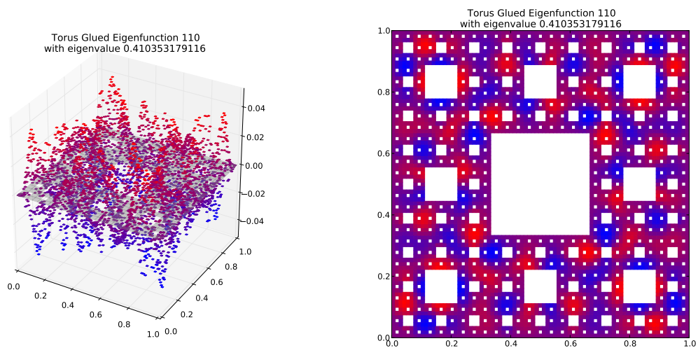
Eigenfunction 110 with eigenvalue 0.410353179116
