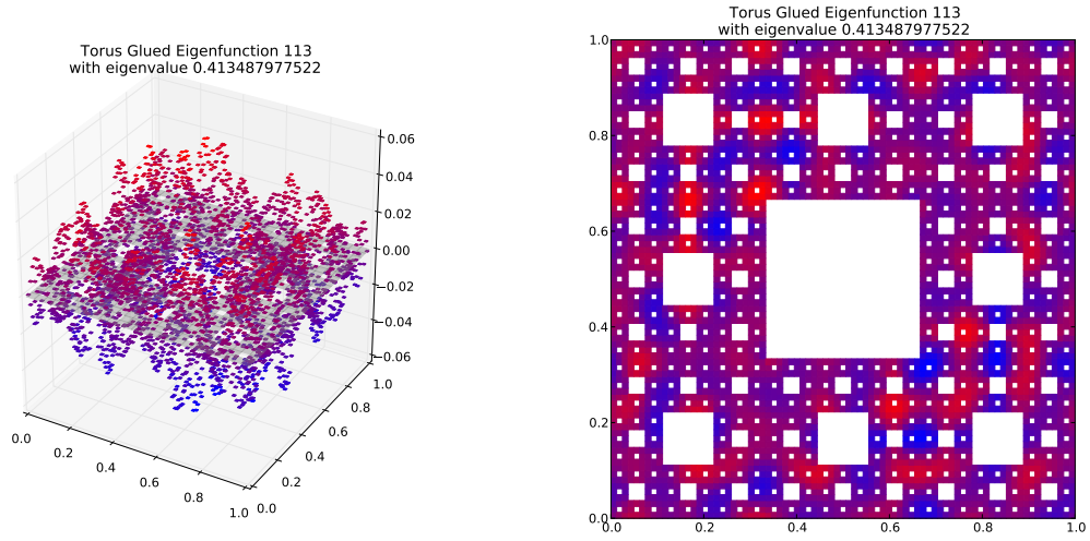
Eigenfunction 113 with eigenvalue 0.413487977522
