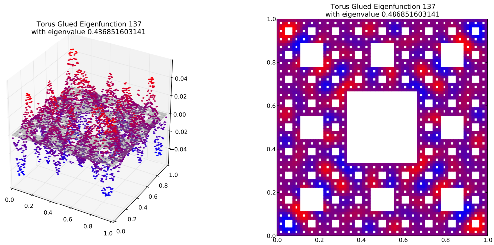
Eigenfunction 137 with eigenvalue 0.486851603141
