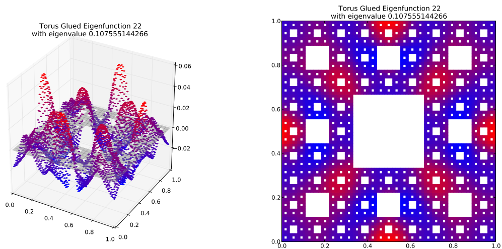
Eigenfunction 22 with eigenvalue 0.107555144266
