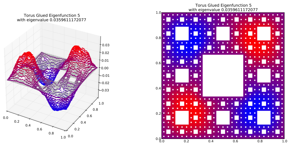
Eigenfunction 5 with eigenvalue 0.0359611172077
