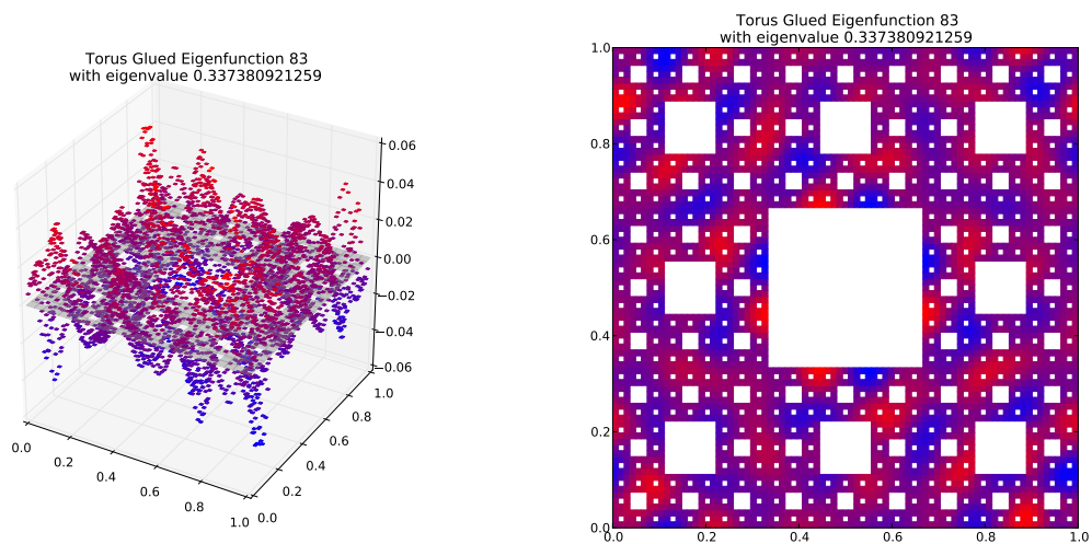
Eigenfunction 83 with eigenvalue 0.337380921259
