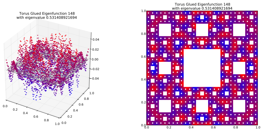
Eigenfunction 148 with eigenvalue 0.531408921694
