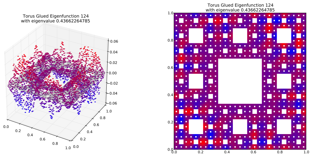
Eigenfunction 124 with eigenvalue 0.43662264785
