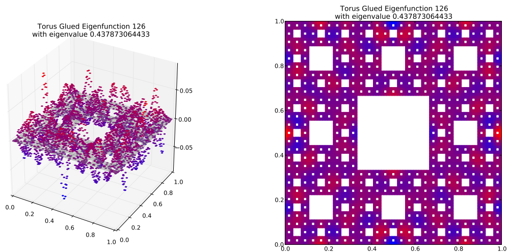
Eigenfunction 126 with eigenvalue 0.437873064433
