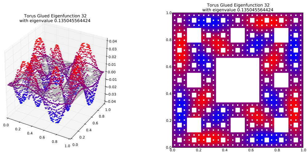
Eigenfunction 32 with eigenvalue 0.135045564424
