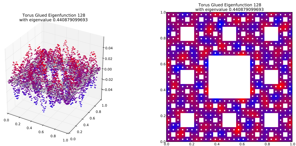
Eigenfunction 128 with eigenvalue 0.440879099693
