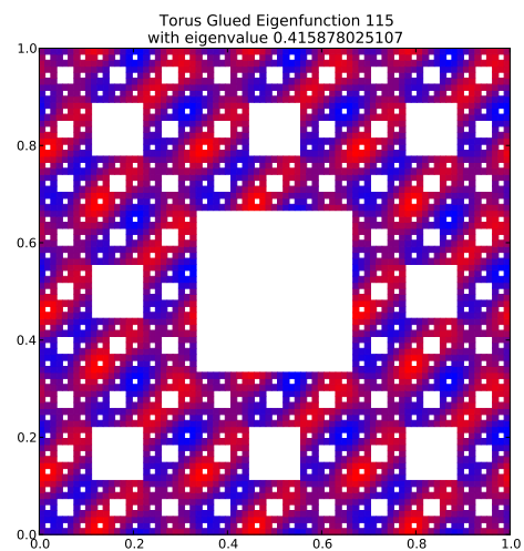
Eigenfunction 115 with eigenvalue 0.415878025107
