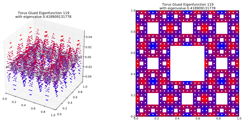
Eigenfunction 119 with eigenvalue 0.418909131778
