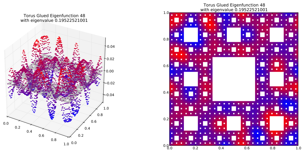
Eigenfunction 48 with eigenvalue 0.19522521001
