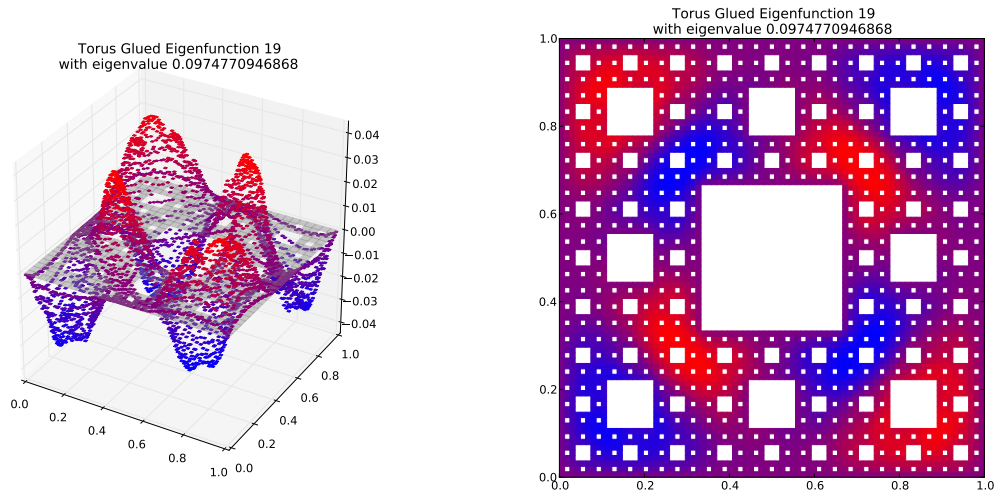
Eigenfunction 19 with eigenvalue 0.0974770946868
