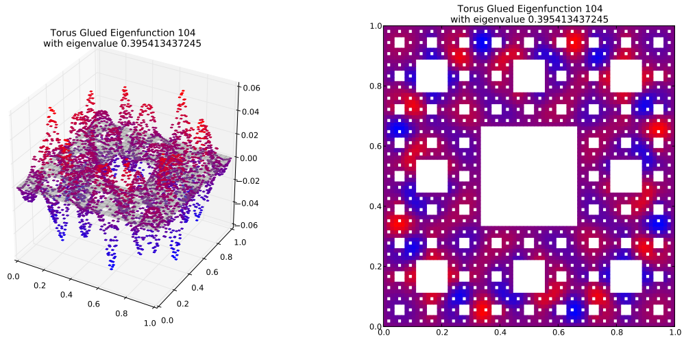
Eigenfunction 104 with eigenvalue 0.395413437245
