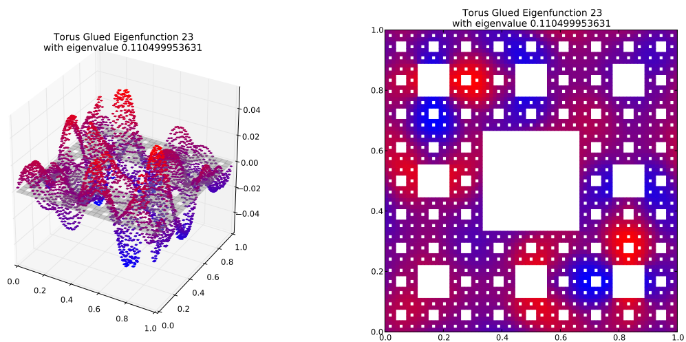
Eigenfunction 23 with eigenvalue 0.110499953631
