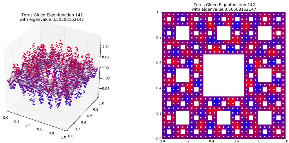
Eigenfunction 142 with eigenvalue 0.50508162147
