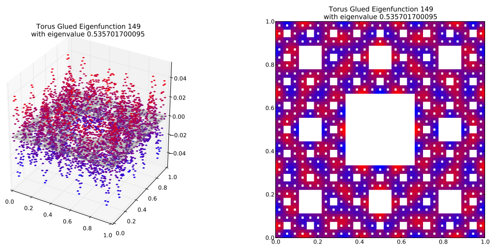
Eigenfunction 149 with eigenvalue 0.535701700095
