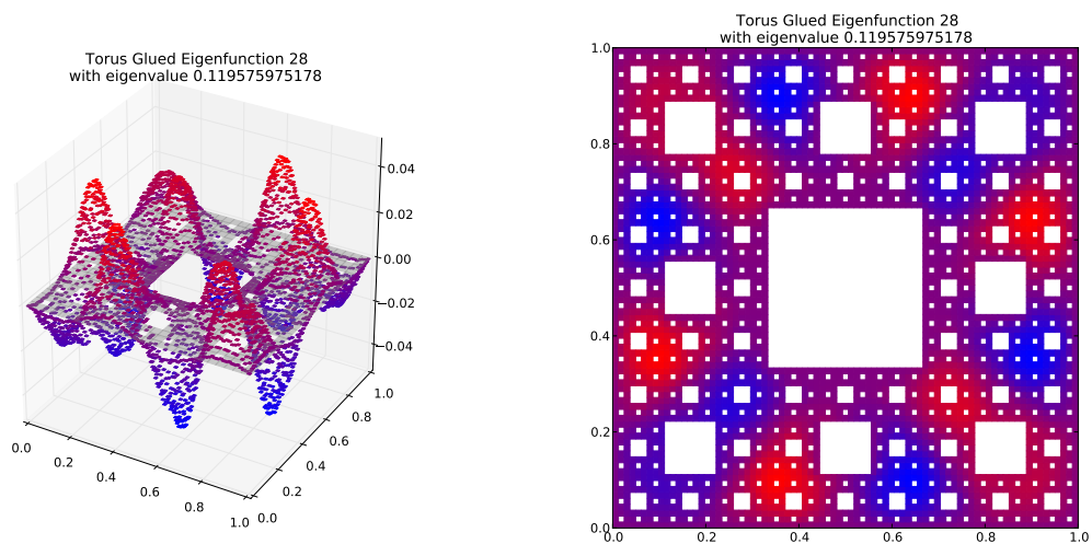
Eigenfunction 28 with eigenvalue 0.119575975178
