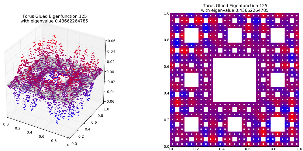
Eigenfunction 125 with eigenvalue 0.43662264785
