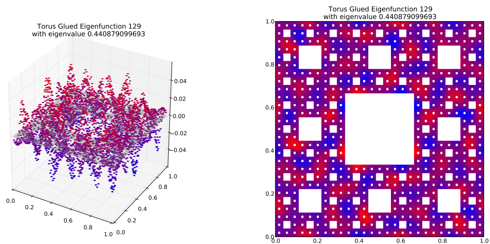
Eigenfunction 129 with eigenvalue 0.440879099693
