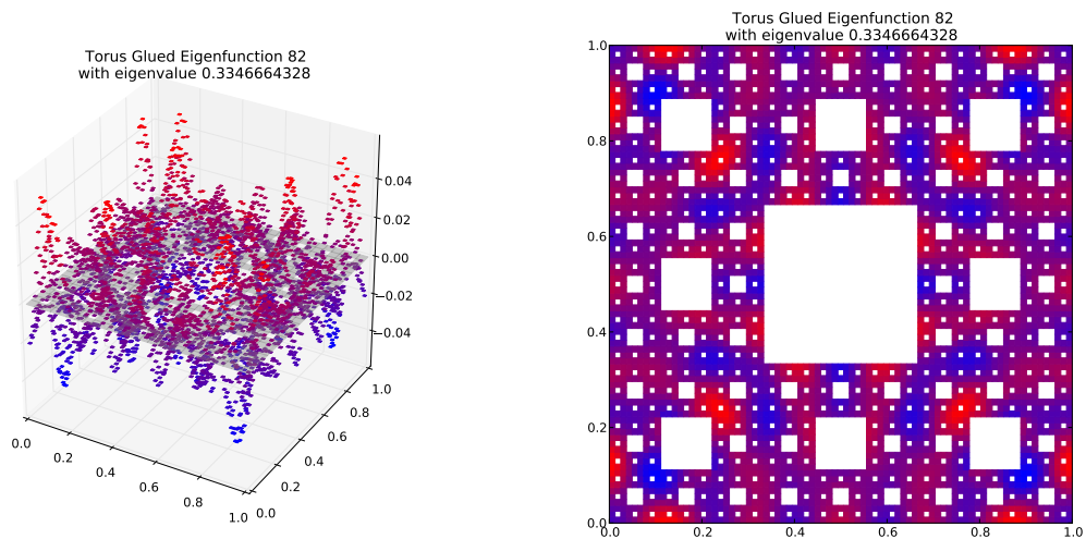
Eigenfunction 82 with eigenvalue 0.3346664328
