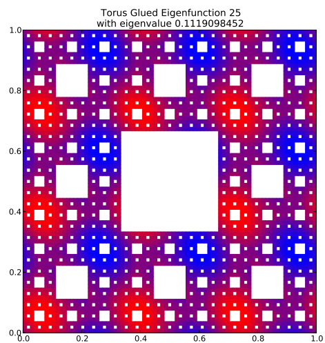
Eigenfunction 25 with eigenvalue 0.1119098452
