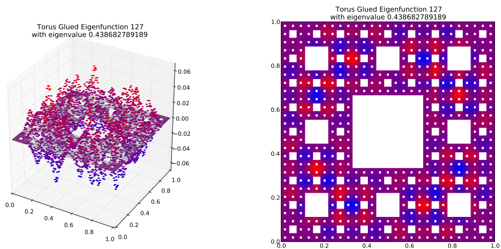
Eigenfunction 127 with eigenvalue 0.438682789189
