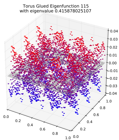
Eigenfunction 115 with eigenvalue 0.415878025107
