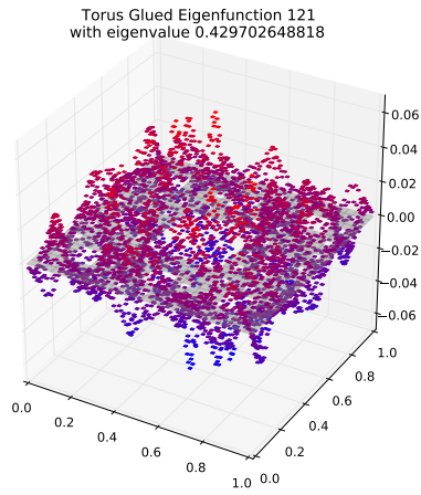
Eigenfunction 121 with eigenvalue 0.429702648818
