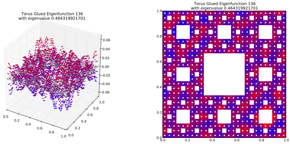
Eigenfunction 136 with eigenvalue 0.464319921701
