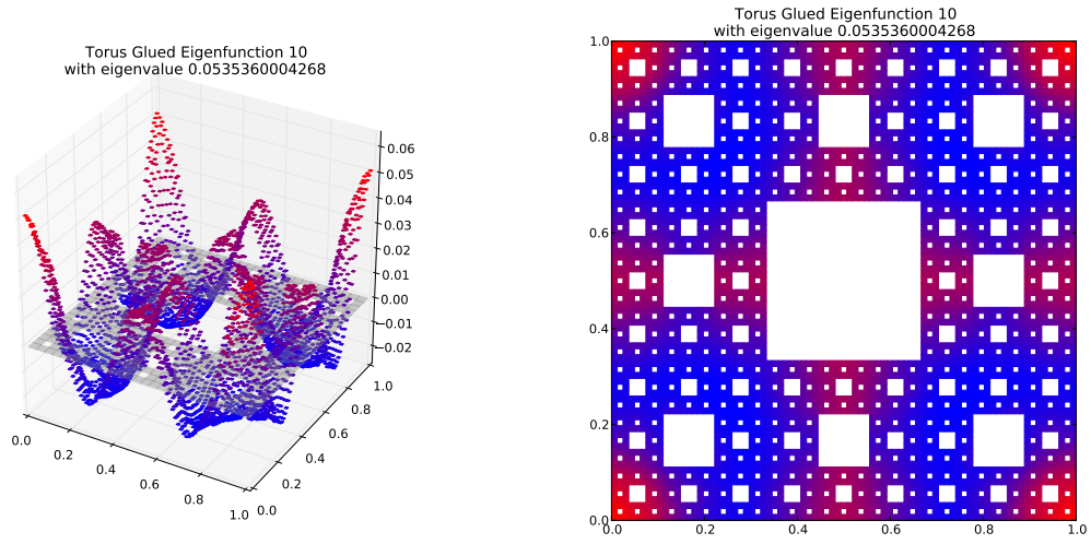
Eigenfunction 10 with eigenvalue 0.0535360004268
