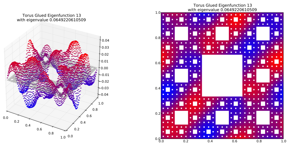
Eigenfunction 13 with eigenvalue 0.0649220610509
