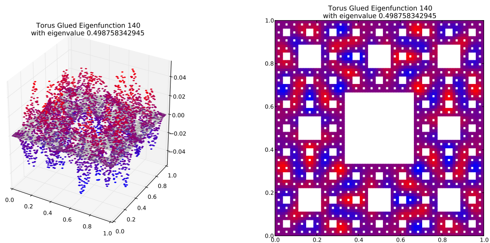
Eigenfunction 140 with eigenvalue 0.498758342945
