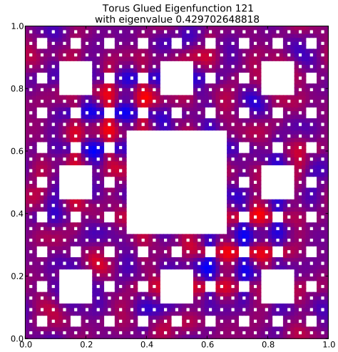
Eigenfunction 121 with eigenvalue 0.429702648818
