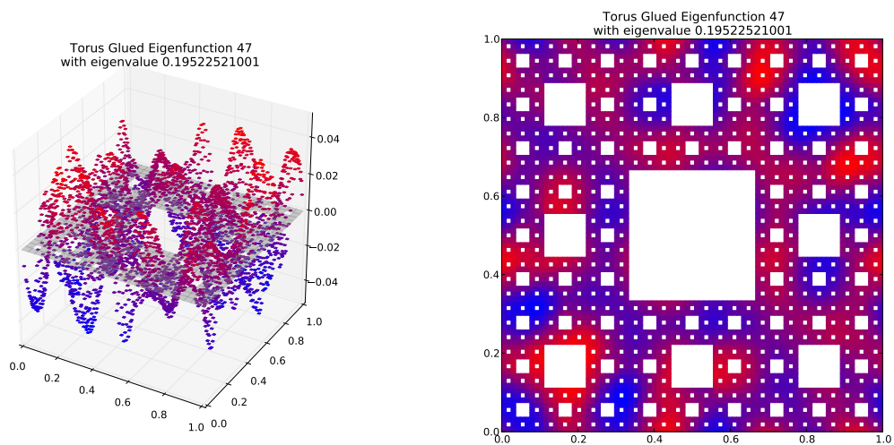
Eigenfunction 47 with eigenvalue 0.19522521001
