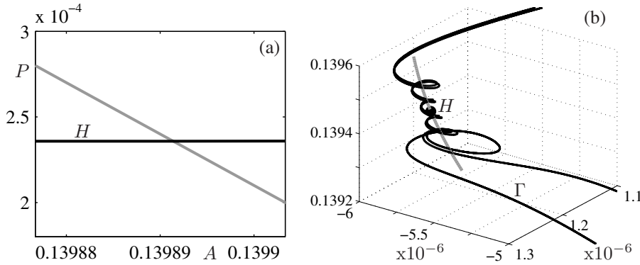
Fig. 32 Panel (a) shows the curve of Hopf bifurcations (black line) and the line defined by 2A + P = 2A_0 (gray) in the (A, P) -plane. Panel (b) shows the SAOs projected onto the three-dimensional space spanned by the center manifold of the Hopf bifurcation and the direction of the line \{2A + P = 2A_0\} in the (A, P) -plane. The MMO periodic orbit \Gamma visits this region twice and each time spirals around the center manifold of the Hopf bifurcation (gray); the Hopf bifurcation point of the layer system itself is the black dot.
