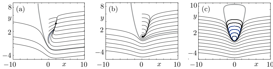
Fig. 12 Phase portraits of system (3.9) for three different values of z . Shown are several trajectories (black) and one trajectory (gray) that approximates a separatrix. For each z , there is a single equilibrium point p at (x, y) = (z, z^2) . Panels (a)–(c) are for z = 2 , z = 0.25 , and z = 0 , for which p is a stable node, a stable focus, and a center surrounded by a continuous family of periodic orbits, respectively. The boundary of this family is the maximal canard.
