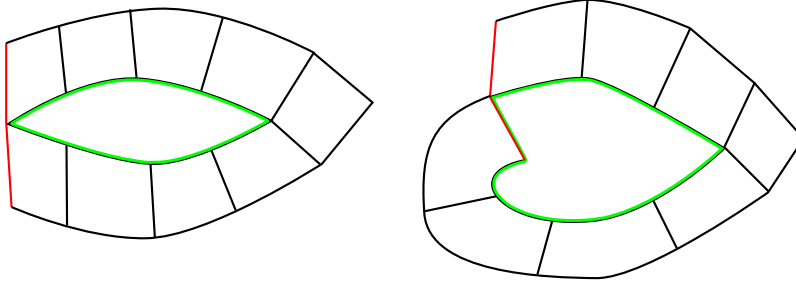
FIGURE 17. Possible interosculations. The red edges represent an osculation. Fill the green loop with a least area filling.
