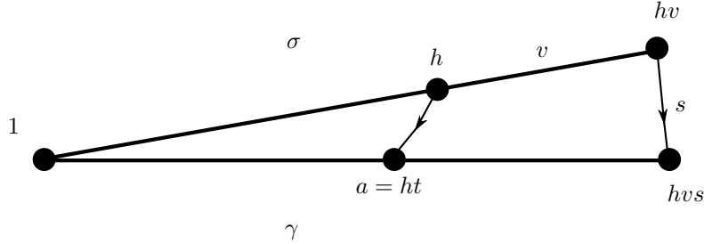
FIGURE 1. The difference between h and a lies in the tail of h .
