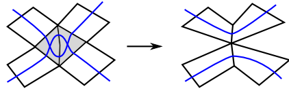
FIGURE 9. Removing a minimal bigon.
