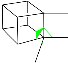
FIGURE 1. Picture of the link of a vertex in a simple cube complex
