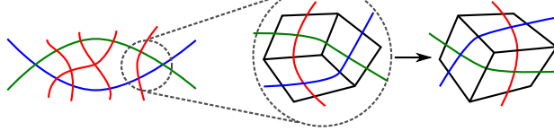
FIGURE 12. On the left, a bigon is formed by a blue and green dual curve. Red dual curves cross the bigon. If there is a red curve which forms an empty 3-gon with the dual curves, then we can do a hexagon move to decrease the area of the bigon.
