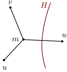
FIGURE 3. If H doesn't separate v from Q , it must come close to w \in Q realizing d(w, Q) .
