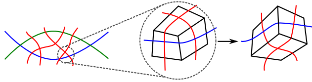
FIGURE 13. A hexagon move coming from an empty 3-gon using \sigma_1 but not \sigma_2 .
