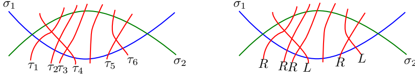
FIGURE 14. Finding an empty 3-gon.
