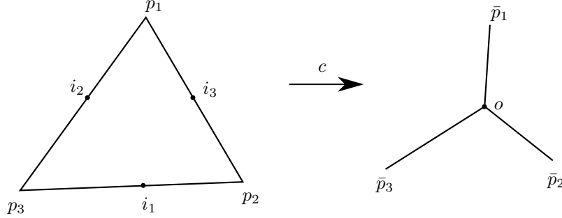
FIGURE 3. Comparison tripod and comparison map.
