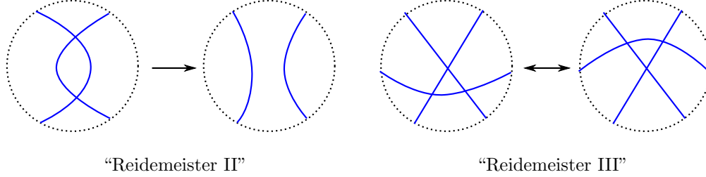
FIGURE 8. Lemmas 7.8 and 7.9 say that we can make local changes to a disk diagram which induce the pictured changes on dual curve diagrams.
