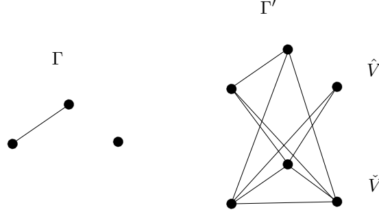
FIGURE 2. Davis-Januszkiewicz' construction.
