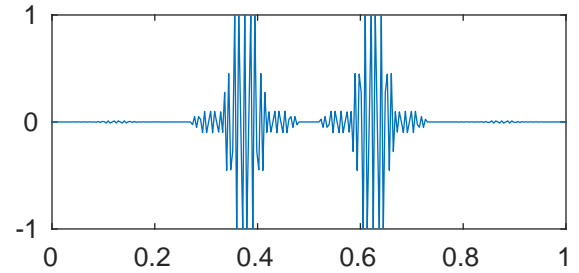
m=4 p=0.99 \lambda_{204} = 106333684458.0787
