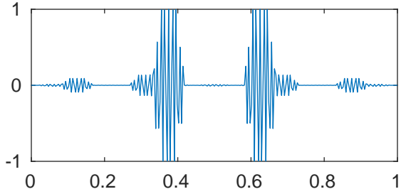
m=4 p=0.99 \lambda_{199} = 106333627862.4043
