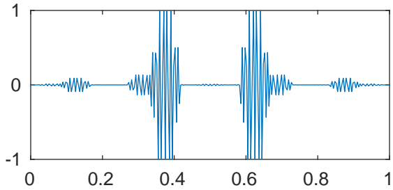
m=4 p=0.99 \lambda_{201} = 106333673222.6645
