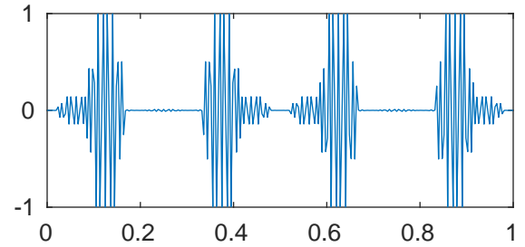
m=4 p=0.99 \lambda_{202} = 106333674456.5582
