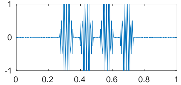
m=4 p=0.99 \lambda_{200} = 106333650532.9904
