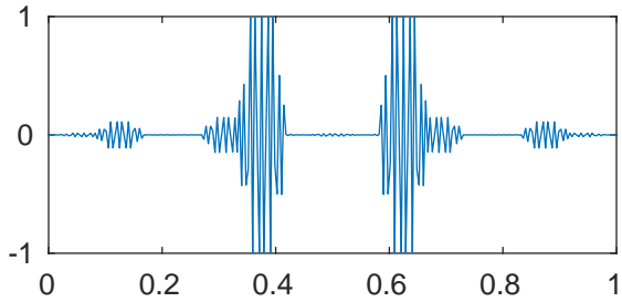
m=4 p=0.99 \lambda_{203} = 106333675631.0976
