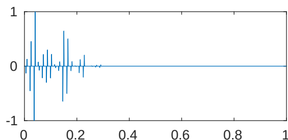
m=5 p=1 \lambda_{264}=2.047353394600163\text{e}+38
