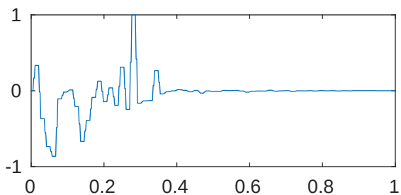
m=5 p=1 \lambda_{17} = 3.478052946974551e+22
