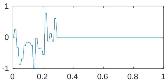
m=5 p=1 \lambda_{15} = 8.936302913733543e+21
