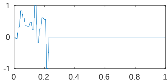
m=5 p=1 \lambda_{14} = -1.413444358354109e+21
