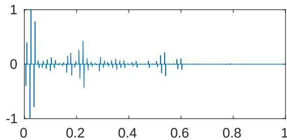
m=5 p=1 \lambda_{260}=2.047353394599646\text{e}+38
