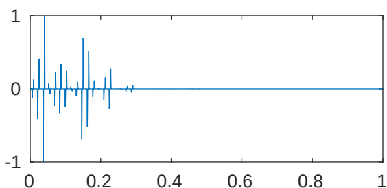
m=5 p=1 \lambda_{263}=2.047353394600118\text{e}+38
