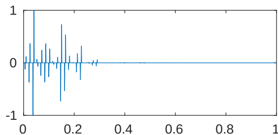
m=5 p=1 \lambda_{262}=2.047353394600095\text{e}+38
