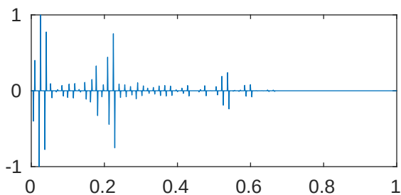
m=5 p=1 \lambda_{261}=2.04735339459989\text{e}+38
