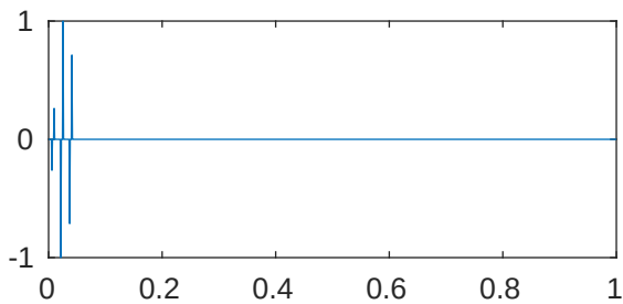
m=5 p=1 \lambda_{259}=2.047353394599538\text{e}+38
