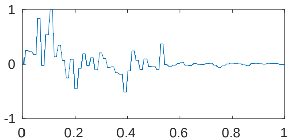
m=5 p=1 \lambda_{13} = -2.214068547647834e+21
