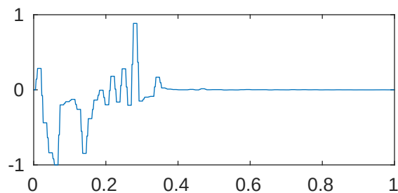
m=5 p=1 \lambda_{18} = 3.748446601110554e+22
