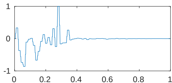
m=5 p=1 \lambda_{16} = 3.478052946974551e+22
