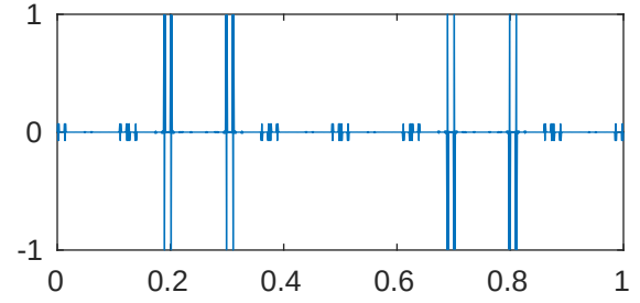
m=5 p=0.01 \lambda_{822}=42963228610094.19
