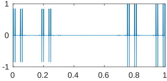
m=5 p=0.01 \lambda_{819}=42963228286501.09
