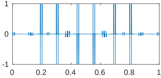
m=5 p=0.01 \lambda_{821}=42963228599881.86
