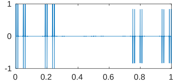
m=5 p=0.01 \lambda_{820}=42963228286505.66
