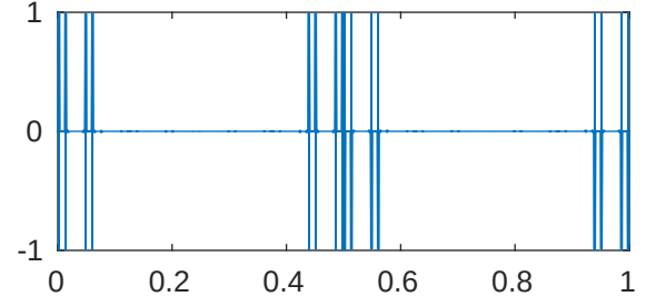
m=5 p=0.01 \lambda_{818}=42963228285616.8
