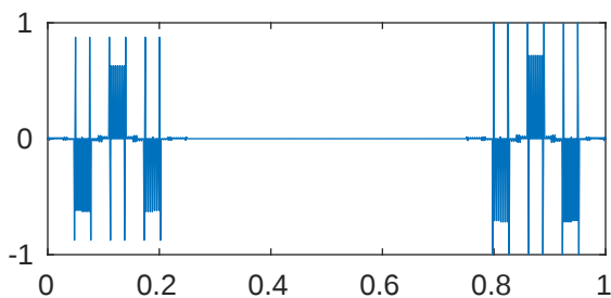
m=5 p=0.001 \lambda_{531}=2.05898640378432\text{e}+18
