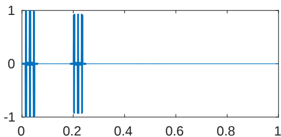
m=5 p=0.001 \lambda_{945}=4.116043482977629\text{e+18}
