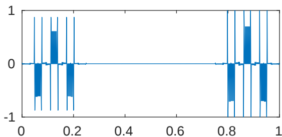
m=5 p=0.001 \lambda_{467}=2.05753216914744e+18
