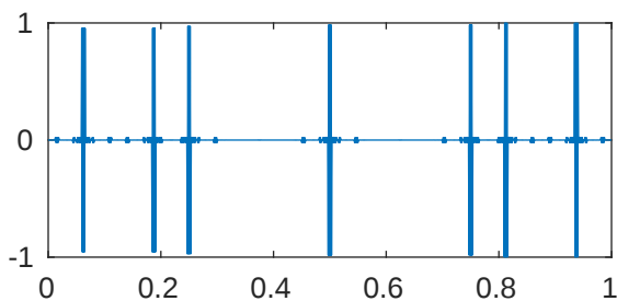
m=5 p=0.001 \lambda_{857}=4.116015575047466\text{e}+18
