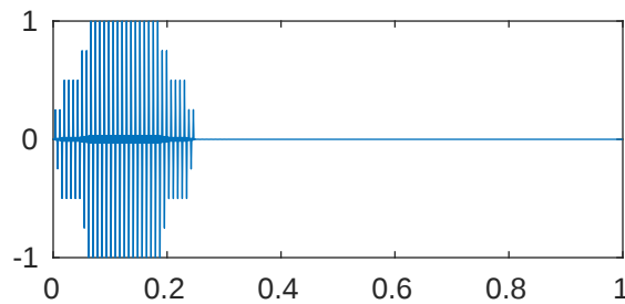
m=5 p=0.001 \lambda_{764}=2.123359029258725\text{e+18}
