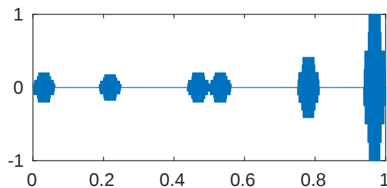
m=5 p=0.001 \lambda_{1012}=4.116541583583052\text{e}+18
