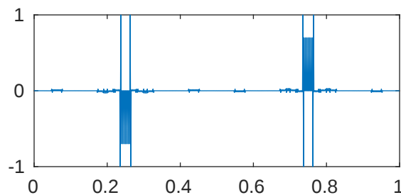
m=5 p=0.001 \lambda_{550}=2.059005998073684\text{e}+18
