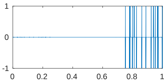
m=5 p=0.001 \lambda_{803}=4.115512319690011\text{e+18}
