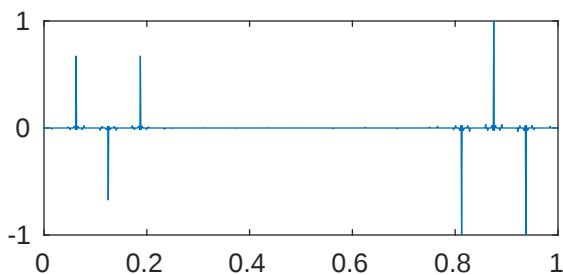
m=5 p=0.001 \lambda_{621}=2.103774432095472\text{e}+18
