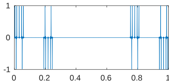
m=5 p=0.001 \lambda_{656}=2.104295110057375\text{e}+18
