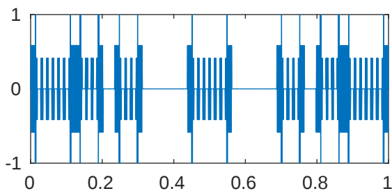
m=5 p=0.001 \lambda_{905}=4.116027391110769e+18
