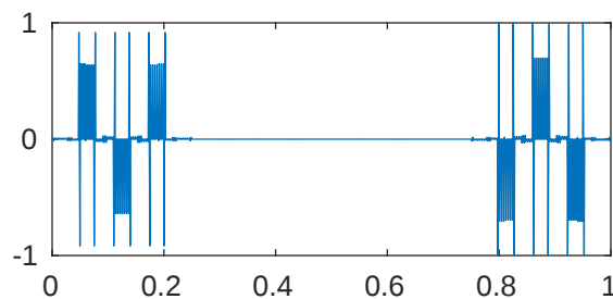
m=5 p=0.001 \lambda_{556}=2.059009414499452\text{e}+18
