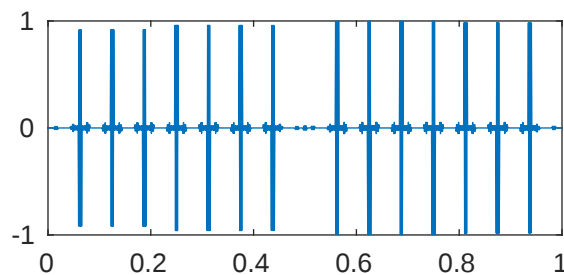
m=5 p=0.001 \lambda_{942}=4.116038895717679\text{e+18}
