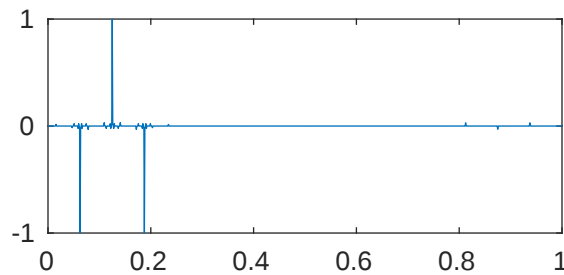
m=5 p=0.001 \lambda_{404}=2.012767151555812\text{e+18}
