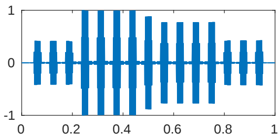
m=5 p=0.001 \lambda_{977}=4.116541451117218\text{e}+18
