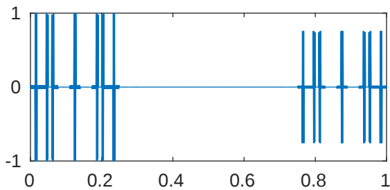
m=5 p=0.001 \lambda_{925}=4.116038712253697\text{e}+18
