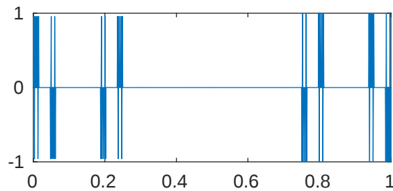
m=5 p=0.001 \lambda_{572}=2.059299541253337e+18
