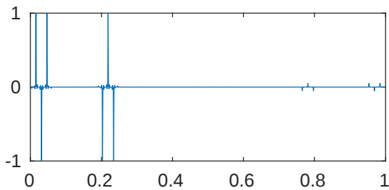
m=5 p=0.001 \lambda_{433}=2.012991613218305e+18
