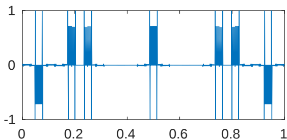
m=5 p=0.001 \lambda_{537}=2.058989822623627\text{e}+18
