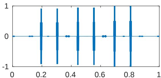
m=5 p=0.001 \lambda_{971}=4.116541326589439\text{e}+18
