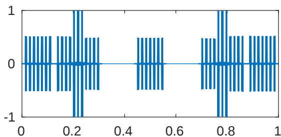
m=5 p=0.001 \lambda_{839}=4.116010933794714\text{e}+18
