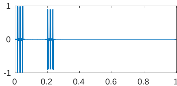
m=5 p=0.001 \lambda_{848}=4.116010934814601\text{e}+18
