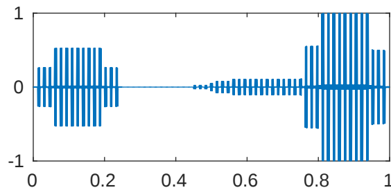
m=5 p=0.001 \lambda_{956}=4.116043485014213\text{e}+18
