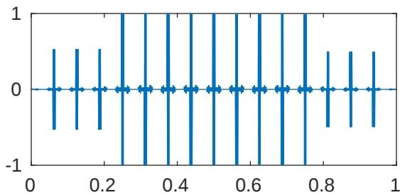
m=5 p=0.001 \lambda_{943}=4.116038895728745\text{e+18}
