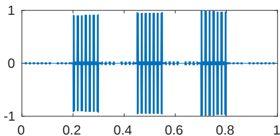
m=5 p=0.001 \lambda_{837}=4.116010933763133\text{e}+18
