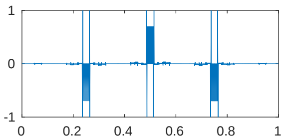
m=5 p=0.001 \lambda_{549}=2.059005960276378\text{e}+18
