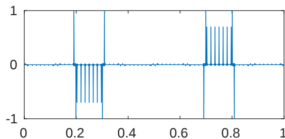
m=5 p=0.001 \lambda_{630}=2.104275383195394\text{e}+18
