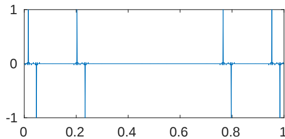
m=5 p=0.001 \lambda_{416}=2.01277544828625\text{e}+18
