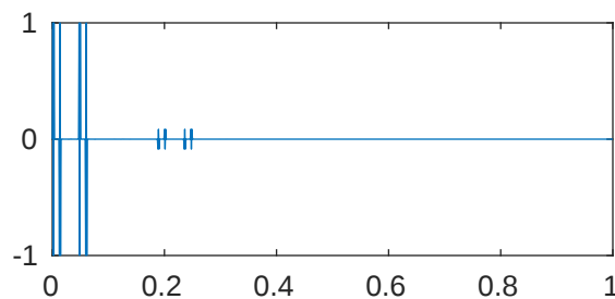
m=5 p=0.001 \lambda_{772}=4.115512190838994\text{e}+18
