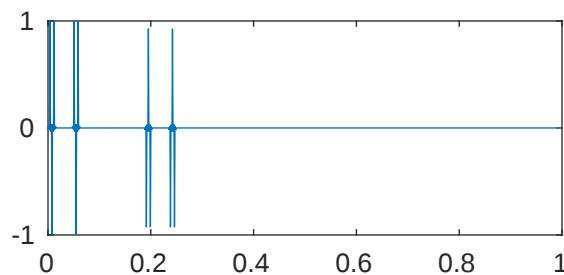
m=5 p=0.001 \lambda_{720}=2.123350884572232\text{e+18}
