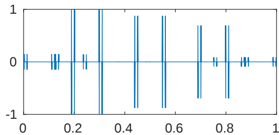
m=5 p=0.001 \lambda_{776}=4.115512190870963\text{e}+18
