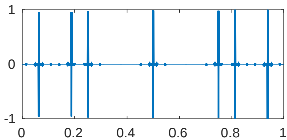
m=5 p=0.001 \lambda_{871}=4.11601583235544\text{e+18}
