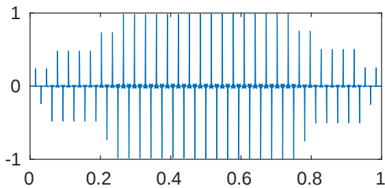
m=5 p=0.001 \lambda_{703}=2.105005840580276\text{e+18}
