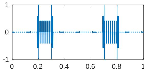
m=5 p=0.001 \lambda_{902}=4.116027389019973e+18
