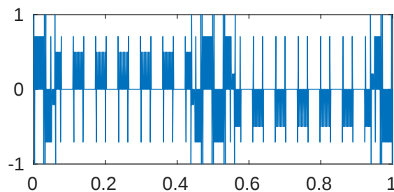
m=5 p=0.001 \lambda_{546}=2.058998128468856\text{e+18}
