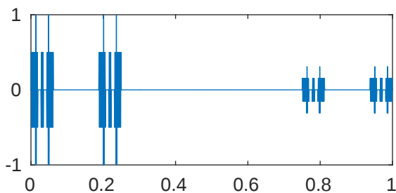
m=5 p=0.001 \lambda_{909}=4.116027466437214\text{e}+18
