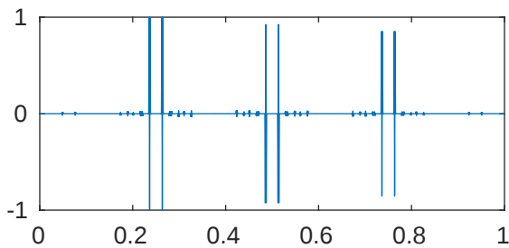
m=5 p=0.001 \lambda_{811}=4.115512322552226\text{e+18}
