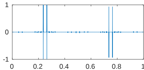
m=5 p=0.001 \lambda_{794}=4.115512316775946\text{e+18}
