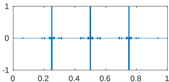
m=5 p=0.001 \lambda_{939}=4.116038845088077\text{e+18}
