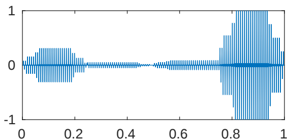
m=5 p=0.001 \lambda_{765}=2.123359029258758\text{e+18}
