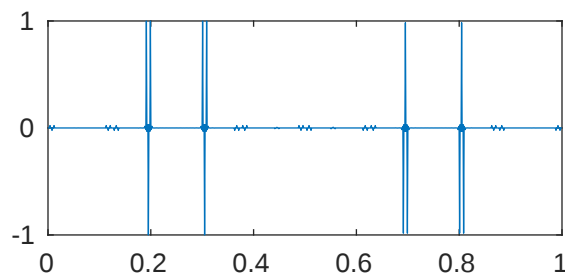
m=5 p=0.001 \lambda_{714}=2.123350883574589\text{e}+18
