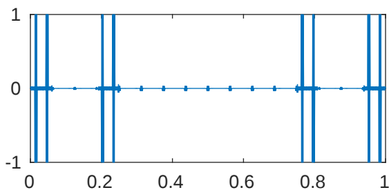
m=5 p=0.001 \lambda_{929}=4.116038715175628\text{e}+18
