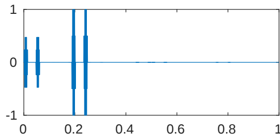
m=5 p=0.001 \lambda_{962}=4.116541326556308\text{e}+18
