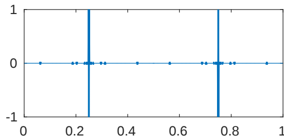
m=5 p=0.001 \lambda_{854}=4.116015573598966\text{e}+18
