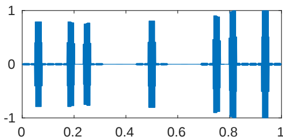
m=5 p=0.001 \lambda_{999}=4.116541458055067\text{e}+18
