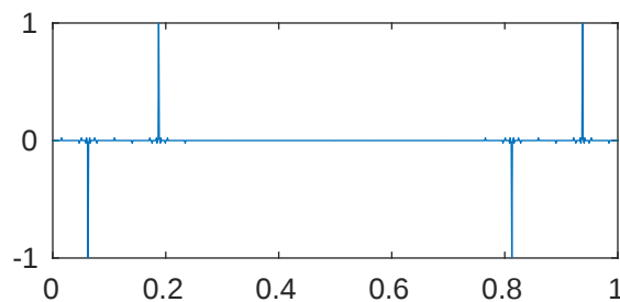
m=5 p=0.001 \lambda_{408}=2.012769596019414\text{e+18}
