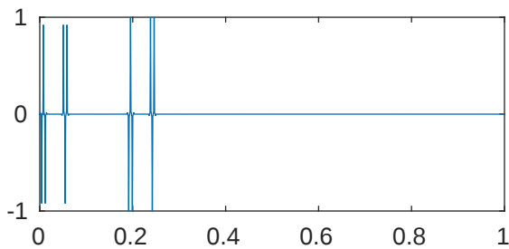
m=5 p=0.001 \lambda_{319}=1.99319070111487\text{e}+18
