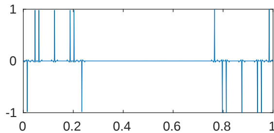
m=5 p=0.001 \lambda_{356}=2.011746376429026\text{e}+18
