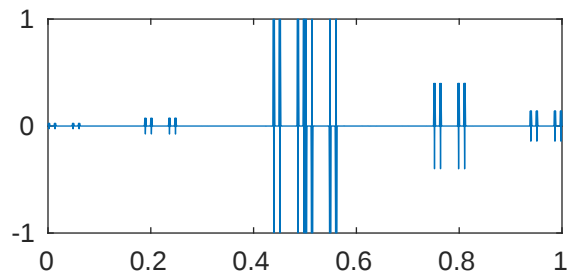
m=5 p=0.001 \lambda_{818}=4.115512448509153\text{e+18}
