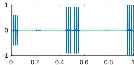
m=5 p=0.001 \lambda_{946}=4.116043482977851\text{e+18}
