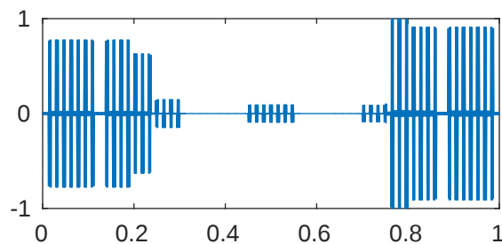
m=5 p=0.001 \lambda_{952}=4.116043483996786\text{e}+18
