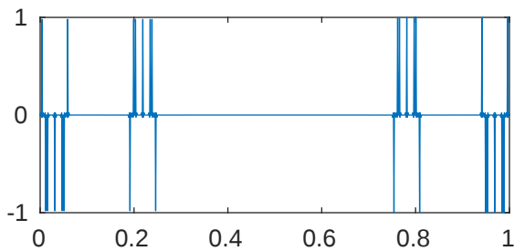
m=5 p=0.001 \lambda_{625}=2.104272100772421\text{e}+18
