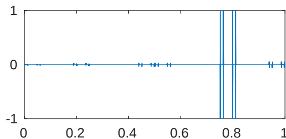
m=5 p=0.001 \lambda_{768}=4.115512190838761\text{e+18}
