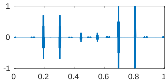
m=5 p=0.001 \lambda_{966}=4.116541326587786\text{e}+18
