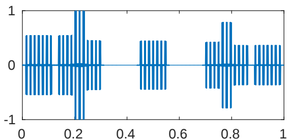
m=5 p=0.001 \lambda_{953}=4.116043483997329\text{e}+18
