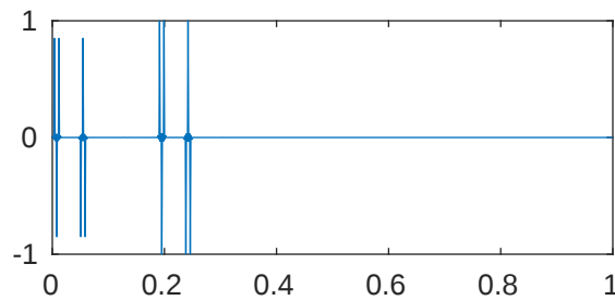
m=5 p=0.001 \lambda_{704}=2.123350882532373\text{e+18}
