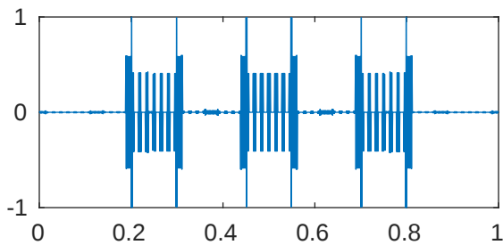
m=5 p=0.001 \lambda_{907}=4.116027393919636\text{e}+18
