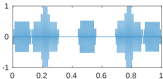
m=5 p=0.001 \lambda_{263}=1.993182555404139\text{e}+18
