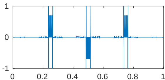
m=5 p=0.001 \lambda_{555}=2.059006214786689\text{e}+18
