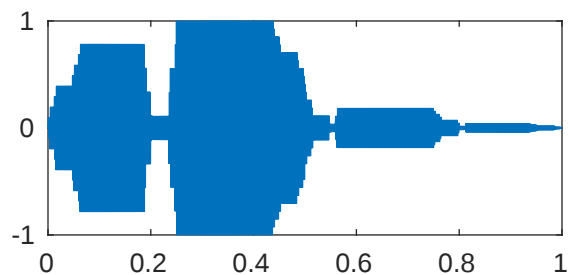
m=5 p=0.001 \lambda_{1020}=4.116541583647214\text{e}+18
