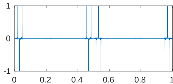
m=5 p=0.001 \lambda_{434}=2.012991613229657e+18
