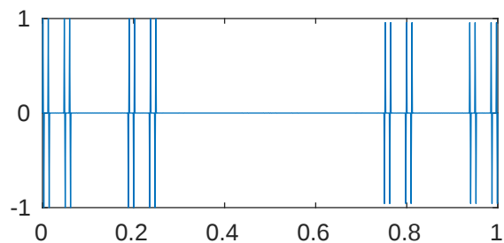
m=5 p=0.001 \lambda_{516}=2.058271048753122\text{e}+18
