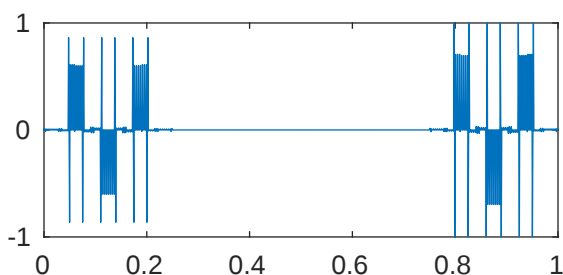
m=5 p=0.001 \lambda_{557}=2.059009414499768\text{e}+18
