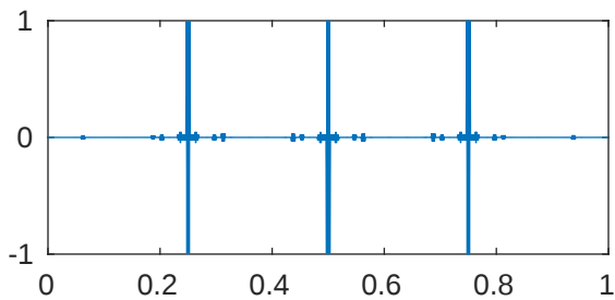
m=5 p=0.001 \lambda_{869}=4.116015830312087\text{e}+18
