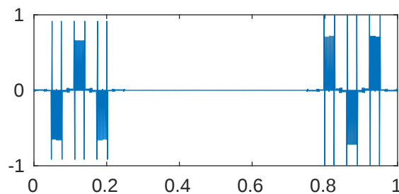
m=5 p=0.001 \lambda_{532}=2.058986403784647\text{e}+18
