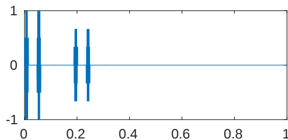
m=5 p=0.001 \lambda_{960}=4.116541326556288\text{e}+18
