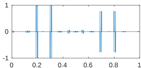
m=5 p=0.001 \lambda_{778}=4.115512190871783\text{e}+18
