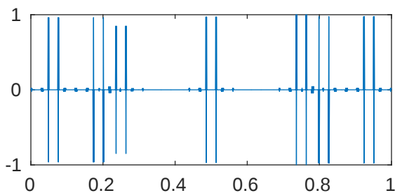
m=5 p=0.001 \lambda_{809}=4.115512322507233\text{e}+18
