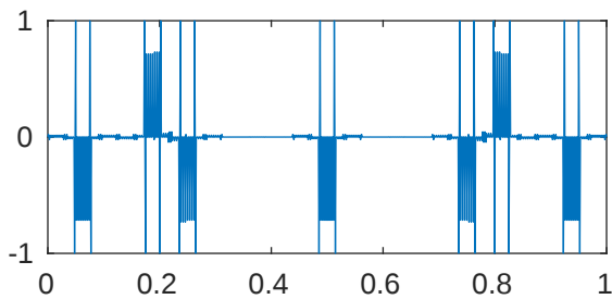
m=5 p=0.001 \lambda_{535}=2.058989818510255\text{e}+18
