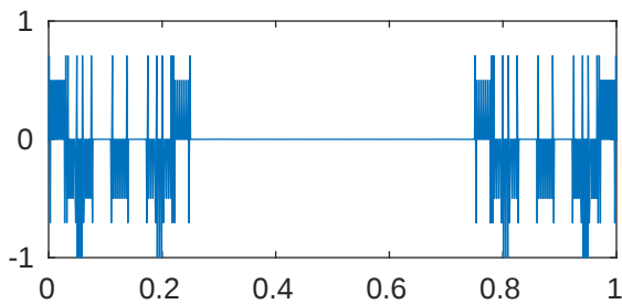
m=5 p=0.001 \lambda_{541}=2.058997818087406\text{e+18}
