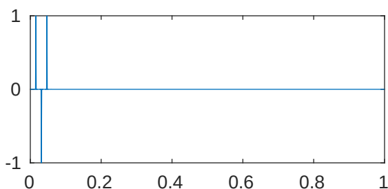
m=5 p=1e-05 \lambda_{689}=2.052689323268772\text{e}+28
