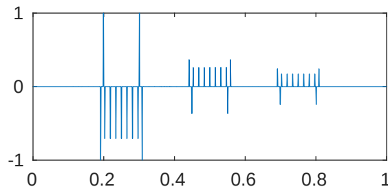
m=5 p=1e-05 \lambda_{374}=2.043522710237051\text{e}+28
