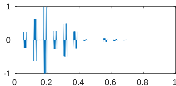
m=5 p=1e-05 \lambda_{748}=2.05457906754544\text{e}+28
