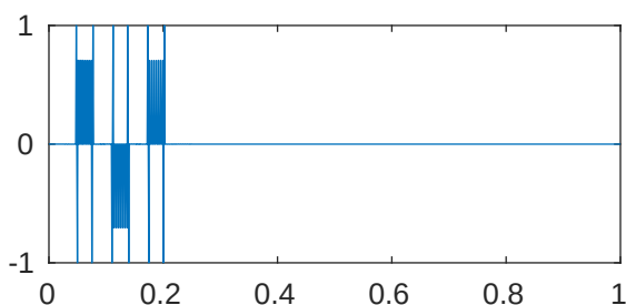
m=5 p=1e-05 \lambda_{557}=2.048109655622863\text{e}+28
