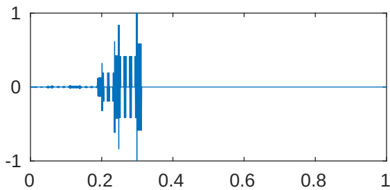
m=5 p=1e-05 \lambda_{905}=4.096199685981414\text{e}+28
