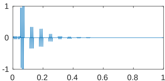
m=5 p=1e-05 \lambda_{735}=2.054579067526171\text{e}+28
