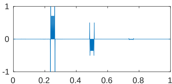
m=5 p=1e-05 \lambda_{489}=2.048095170114929\text{e}+28
