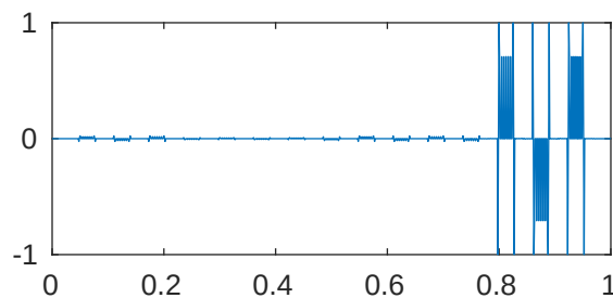
m=5 p=1e-05 \lambda_{492}=2.048095173468188\text{e}+28
