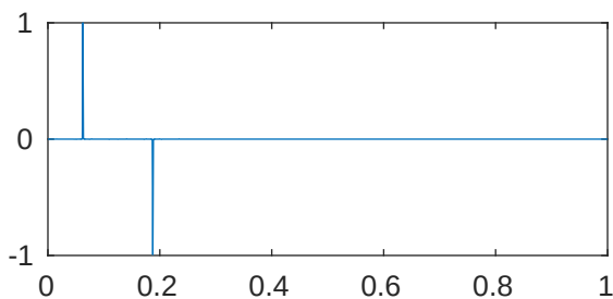
m=5 p=1e-05 \lambda_{407}=2.043527835349527\text{e}+28
