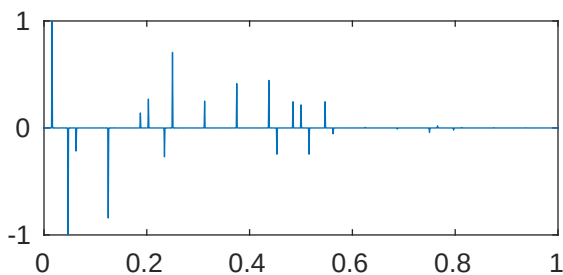
m=5 p=1e-05 \lambda_{419}=2.043527841486727\text{e}+28
