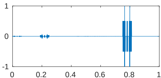
m=5 p=1e-05 \lambda_{899}=4.096199685970264\text{e}+28
