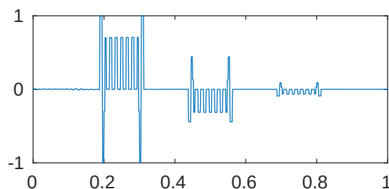
m=5 p=1e-05 \lambda_{138}=5.120254923506986\text{e}+22
