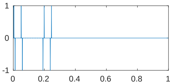
m=5 p=1e-05 \lambda_{637}=2.052682087809822\text{e}+28
