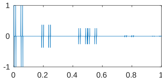
m=5 p=1e-05 \lambda_{510}=2.048102403034179\text{e}+28
