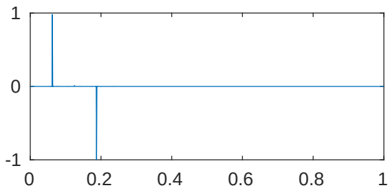
m=5 p=1e-05 \lambda_{663}=2.052687199127481\text{e}+28
