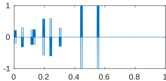
m=5 p=1e-05 \lambda_{572}=2.048112643557949\text{e}+28
