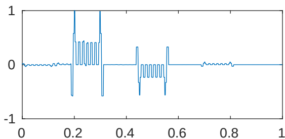
m=5 p=1e-05 \lambda_{123}=5.120218729790028\text{e}+22
