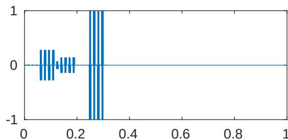
m=5 p=1e-05 \lambda_{838}=4.096199669780441\text{e}+28
