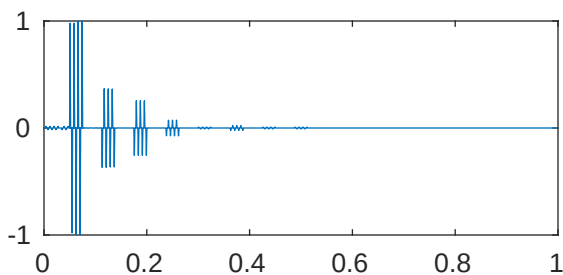
m=5 p=1e-05 \lambda_{741}=2.05457906753221\text{e}+28
