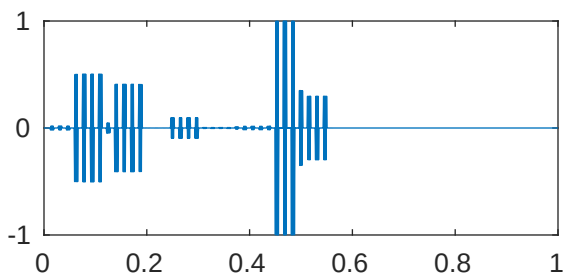
m=5 p=1e-05 \lambda_{951}=4.096199702164239\text{e}+28
