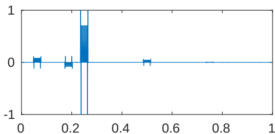
m=5 p=1e-05 \lambda_{551}=2.048109652272381\text{e}+28
