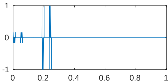
m=5 p=1e-05 \lambda_{451}=2.048092162607828e+28
