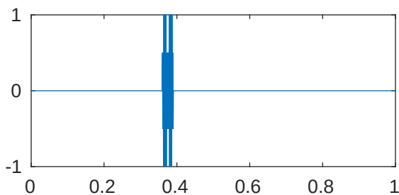
m=5 p=1e-05 \lambda_{989}=4.096204806193157\text{e}+28
