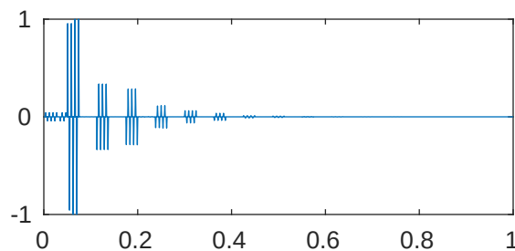
m=5 p=1e-05 \lambda_{736}=2.0545790675264\text{e}+28
