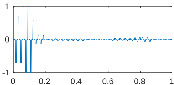
m=5 p=1e-05 \lambda_{71}=5.104045069160051\text{e}+22
