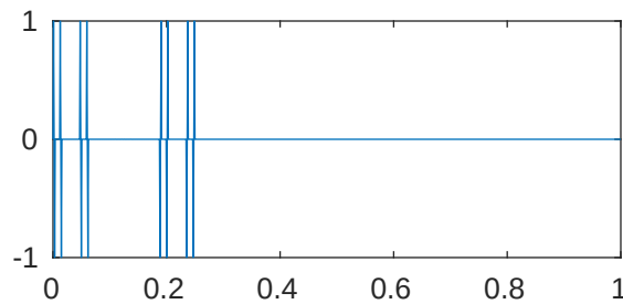
m=5 p=1e-05 \lambda_{508}=2.048102402988958\text{e}+28
