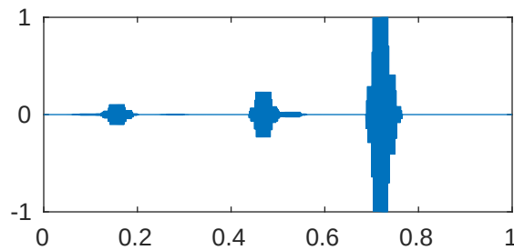
m=5 p=1e-05 \lambda_{1010}=4.096204806218721\text{e}+28
