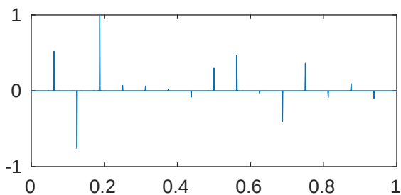
m=5 p=1e-05 \lambda_{623}=2.052676973022115\text{e}+28
