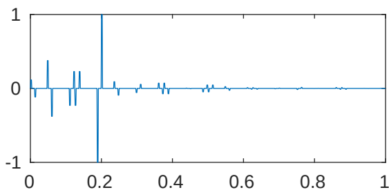
m=5 p=1e-05 \lambda_{249}=1.024053761713184\text{e}+23
