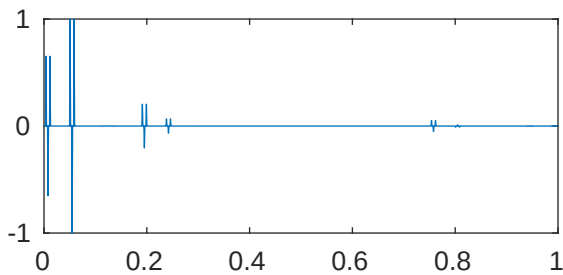
m=5 p=1e-05 \lambda_{709}=2.054579063465284\text{e}+28
