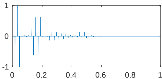
m=5 p=1e-05 \lambda_{589}=2.052674840972626\text{e}+28
