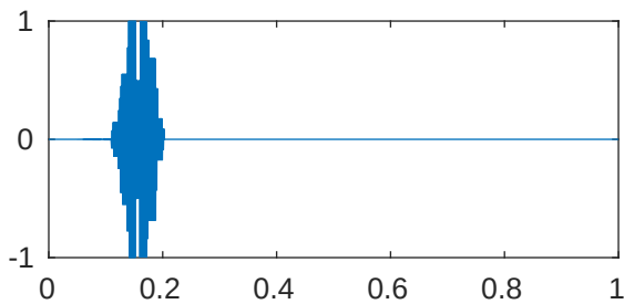
m=5 p=1e-05 \lambda_{997}=4.09620480620591e+28
