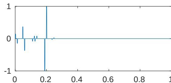
m=5 p=1e-05 \lambda_{250}=1.024053761733927\text{e}+23
