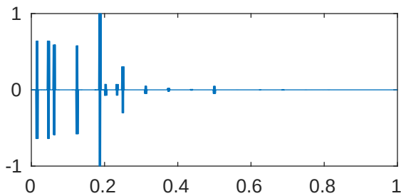
m=5 p=1e-05 \lambda_{919}=4.096199697402688\text{e}+28
