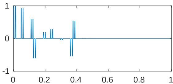
m=5 p=1e-05 \lambda_{199}=1.024051201529642\text{e}+23
