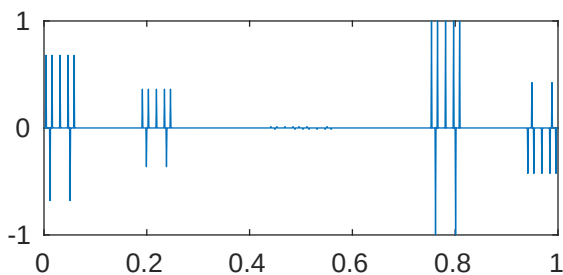
m=5 p=1e-05 \lambda_{653}=2.05268209928408\text{e}+28
