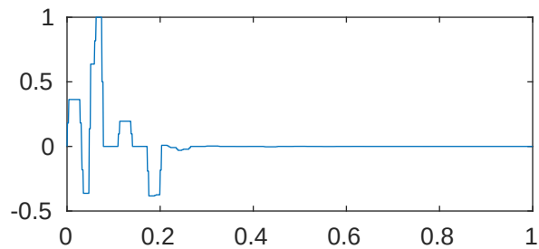
m=5 p=1e-05 \lambda_{38}=1.280285595733988\text{e}+17
