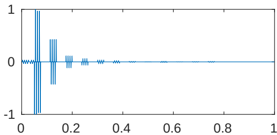
m=5 p=1e-05 \lambda_{727}=2.054579067518614\text{e}+28
