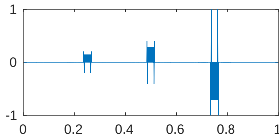
m=5 p=1e-05 \lambda_{554}=2.048109652277054\text{e}+28
