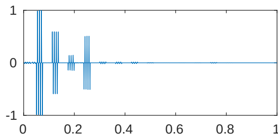
m=5 p=1e-05 \lambda_{276}=2.041625738662419\text{e}+28
