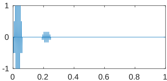
m=5 p=1e-05 \lambda_{259}=2.041625734620359\text{e}+28
