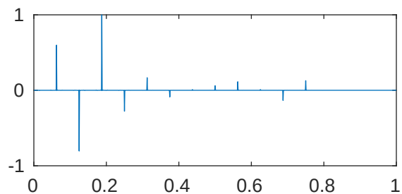
m=5 p=1e-05 \lambda_{622}=2.052676972894784\text{e}+28
