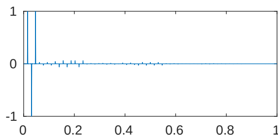
m=5 p=1e-05 \lambda_{690}=2.052689323272231\text{e}+28
