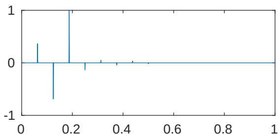
m=5 p=1e-05 \lambda_{621}=2.052676972479943\text{e}+28
