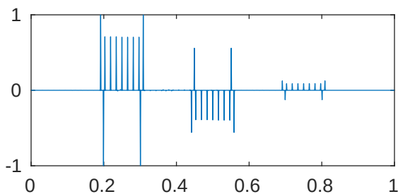
m=5 p=1e-05 \lambda_{651}=2.052682095973357\text{e}+28
