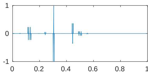
m=5 p=1e-05 \lambda_{718}=2.054579063474601\text{e}+28
