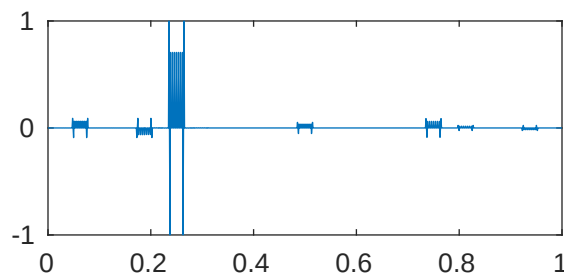
m=5 p=1e-05 \lambda_{552}=2.048109652272413\text{e}+28
