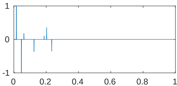
m=5 p=1e-05 \lambda_{673}=2.052687205236064\text{e}+28
