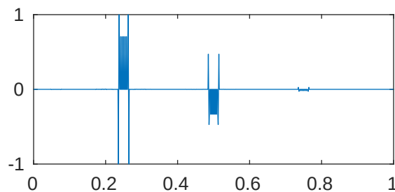
m=5 p=1e-05 \lambda_{474}=2.048095153922764\text{e}+28
