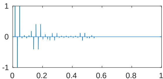
m=5 p=1e-05 \lambda_{435}=2.043529965227391\text{e}+28
