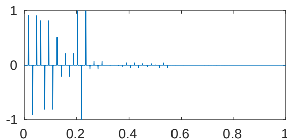
m=5 p=1e-05 \lambda_{436}=2.043529965230511\text{e}+28
