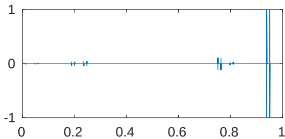
m=5 p=1e-05 \lambda_{775}=4.096194565625171\text{e}+28
