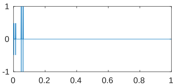
m=5 p=1e-05 \lambda_{783}=4.0961945656507e+28
