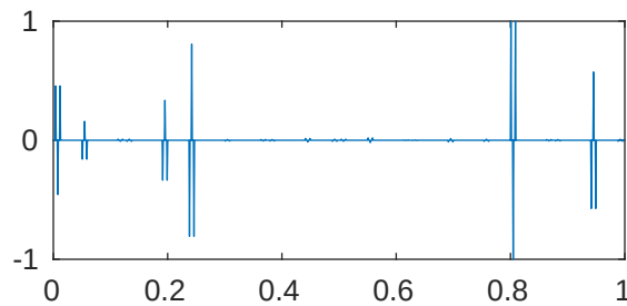
m=5 p=1e-05 \lambda_{704}=2.054579063464988\text{e}+28
