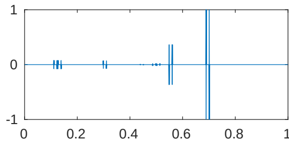
m=5 p=1e-05 \lambda_{776}=4.096194565643791\text{e}+28
