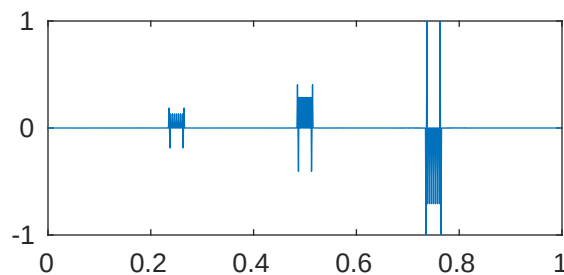
m=5 p=1e-05 \lambda_{538}=2.048109636085394\text{e}+28
