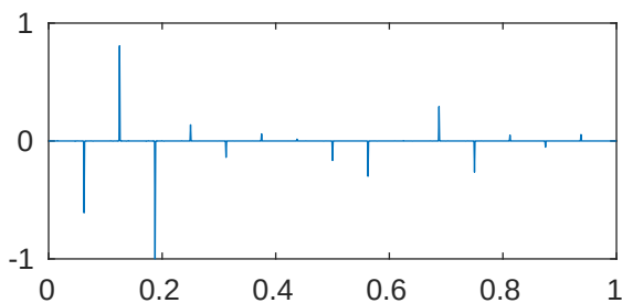
m=5 p=1e-05 \lambda_{401}=2.043527833136656\text{e}+28
