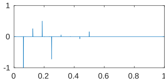
m=5 p=1e-05 \lambda_{602}=2.052676959769259\text{e}+28
