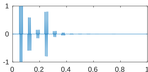
m=5 p=1e-05 \lambda_{744}=2.054579067538262\text{e}+28
