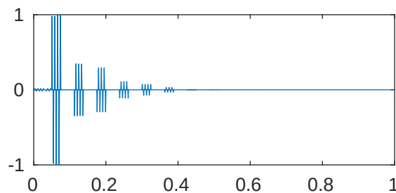
m=5 p=1e-05 \lambda_{738}=2.054579067531049\text{e}+28
