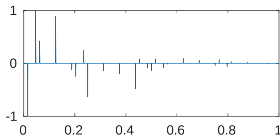
m=5 p=1e-05 \lambda_{348}=2.043517600923978\text{e}+28
