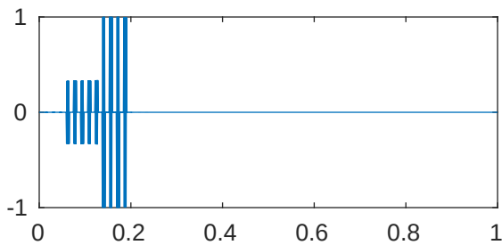
m=5 p=1e-05 \lambda_{949}=4.096199702164029\text{e}+28
