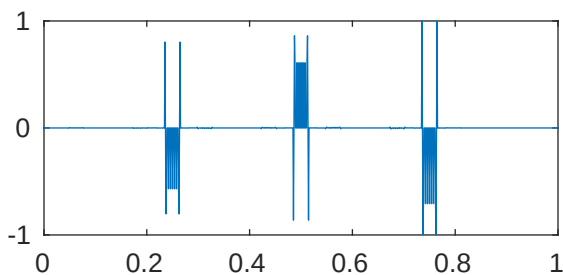
m=5 p=1e-05 \lambda_{485}=2.048095170074555e+28
