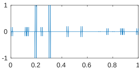
m=5 p=1e-05 \lambda_{503}=2.048102391646637\text{e}+28
