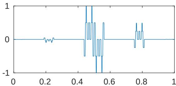
m=5 p=1e-05 \lambda_{115}=5.120211205763889\text{e}+22
