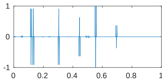
m=5 p=1e-05 \lambda_{712}=2.054579063474485\text{e}+28
