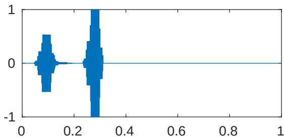
m=5 p=1e-05 \lambda_{1015}=4.096204806218786\text{e}+28
