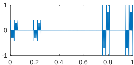
m=5 p=1e-05 \lambda_{479}=2.048095162004999\text{e}+28
