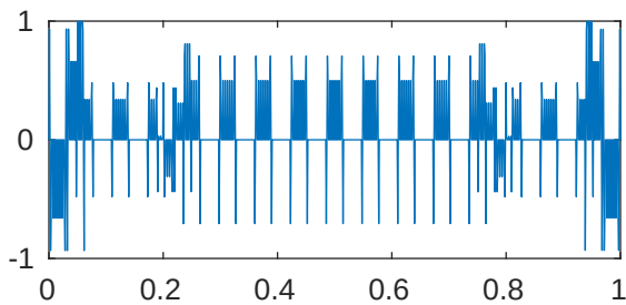
m=5 p=1e-05 \lambda_{481}=2.048095162014346e+28
