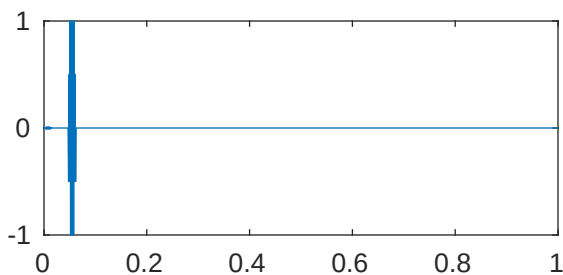
m=5 p=1e-05 \lambda_{963}=4.096204806155877\text{e}+28
