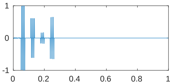
m=5 p=1e-05 \lambda_{277}=2.041625738662551\text{e}+28
