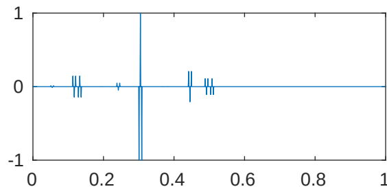
m=5 p=1e-05 \lambda_{716}=2.054579063474589\text{e}+28
