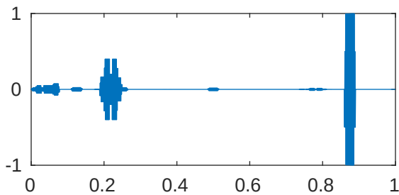
m=5 p=1e-05 \lambda_{985}=4.096204806187327\text{e}+28
