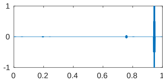
m=5 p=1e-05 \lambda_{960}=4.096204806155778\text{e}+28
