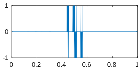
m=5 p=1e-05 \lambda_{564}=2.048112643551536\text{e}+28
