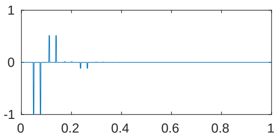
m=5 p=1e-05 \lambda_{213}=1.024052478211951\text{e}+23
