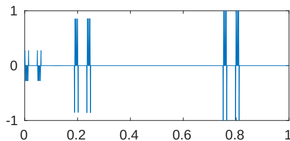
m=5 p=1e-05 \lambda_{454}=2.048092162620592e+28
