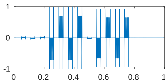
m=5 p=1e-05 \lambda_{558}=2.048109655630395\text{e}+28
