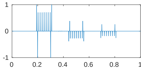
m=5 p=1e-05 \lambda_{378}=2.043522710273829\text{e}+28
