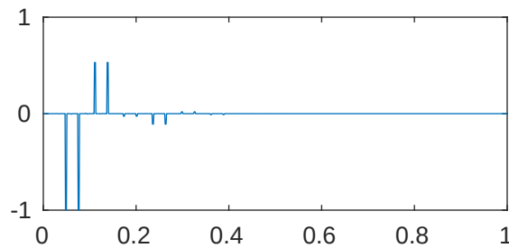
m=5 p=1e-05 \lambda_{212}=1.024052477435912\text{e}+23
