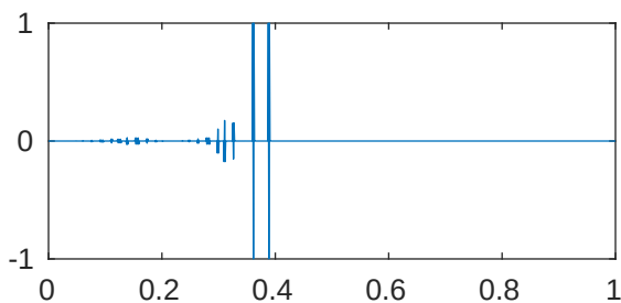
m=5 p=1e-05 \lambda_{819}=4.096194565675264\text{e}+28
