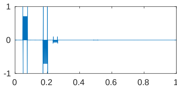
m=5 p=1e-05 \lambda_{550}=2.048109652271892\text{e}+28
