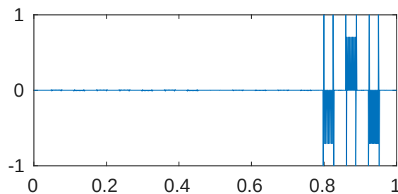
m=5 p=1e-05 \lambda_{556}=2.048109655621051\text{e}+28
