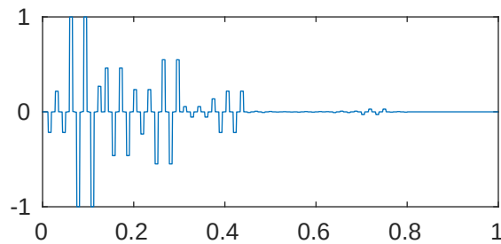
m=5 p=1e-05 \lambda_{68}=5.104045044234509\text{e}+22
