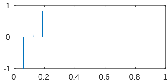
m=5 p=1e-05 \lambda_{680}=2.052687210958666e+28
