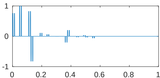
m=5 p=1e-05 \lambda_{203}=1.024051201539789\text{e}+23
