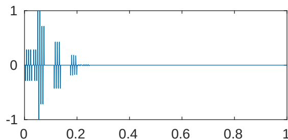
m=5 p=1e-05 \lambda_{286}=2.041625738668748\text{e}+28
