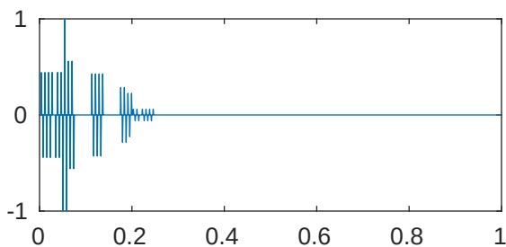
m=5 p=1e-05 \lambda_{729}=2.054579067522235\text{e}+28
