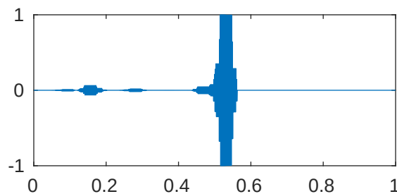
m=5 p=1e-05 \lambda_{1008}=4.096204806218696\text{e}+28
