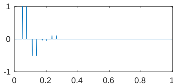
m=5 p=1e-05 \lambda_{214}=1.024052478751498\text{e}+23
