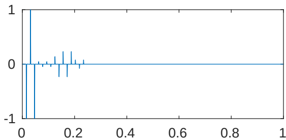
m=5 p=1e-05 \lambda_{331}=2.043515482915931\text{e}+28
