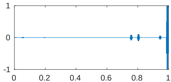
m=5 p=1e-05 \lambda_{962}=4.096204806155836\text{e}+28
