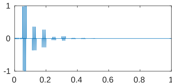
m=5 p=1e-05 \lambda_{740}=2.054579067531856\text{e}+28
