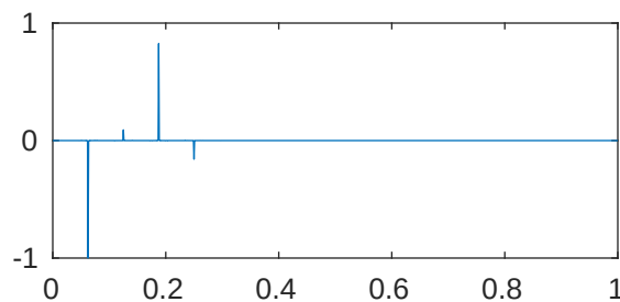
m=5 p=1e-05 \lambda_{424}=2.043527847198822\text{e}+28
