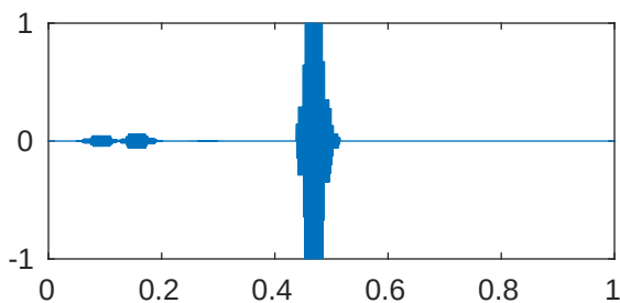
m=5 p=1e-05 \lambda_{1011}=4.096204806218725\text{e}+28
