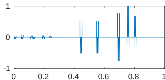
m=5 p=1e-05 \lambda_{460}=2.048092162623502\text{e}+28
