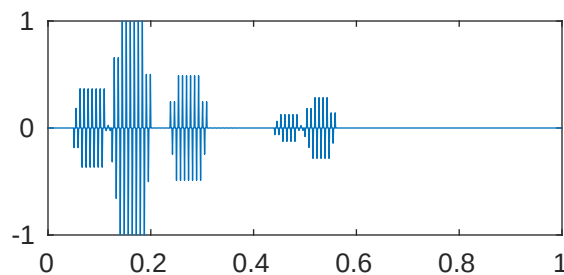
m=5 p=1e-05 \lambda_{268}=2.041625734629775\text{e}+28
