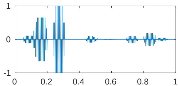
m=5 p=1e-05 \lambda_{262}=2.041625734629572\text{e}+28
