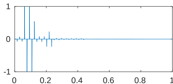
m=5 p=1e-05 \lambda_{322}=2.043515482902527\text{e}+28
