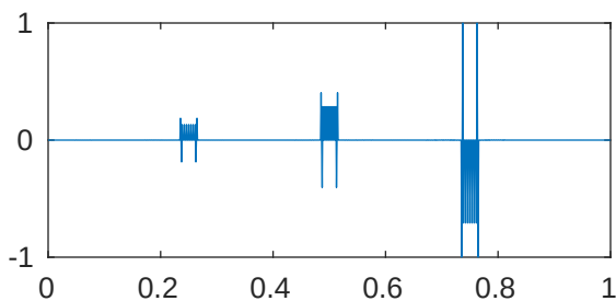
m=5 p=1e-05 \lambda_{537}=2.048109636085394\text{e}+28
