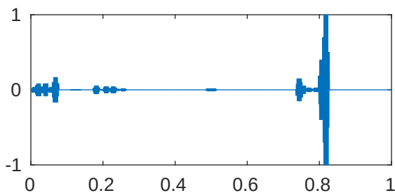
m=5 p=1e-05 \lambda_{981}=4.0962048061873\text{e}+28
