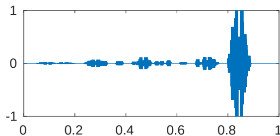
m=5 p=1e-05 \lambda_{1002}=4.096204806205943e+28
