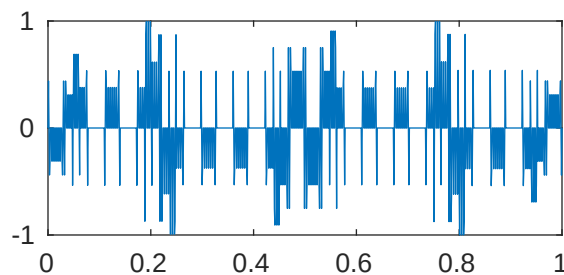
m=5 p=1e-05 \lambda_{484}=2.048095162027138e+28
