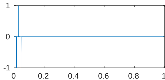
m=5 p=1e-05 \lambda_{584}=2.052674840961259\text{e}+28
