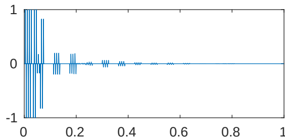
m=5 p=1e-05 \lambda_{734}=2.054579067522626\text{e}+28
