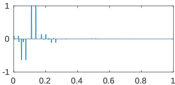
m=5 p=1e-05 \lambda_{217}=1.02405248143381\text{e}+23
