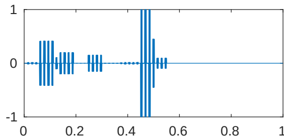
m=5 p=1e-05 \lambda_{950}=4.096199702164202\text{e}+28
