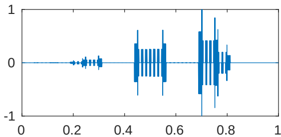
m=5 p=1e-05 \lambda_{903}=4.096199685981296\text{e}+28
