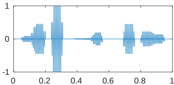
m=5 p=1e-05 \lambda_{261}=2.04162573462954\text{e}+28
