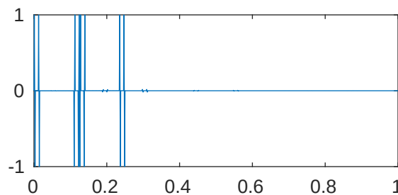
m=5 p=1e-05 \lambda_{504}=2.048102391648664\text{e}+28
