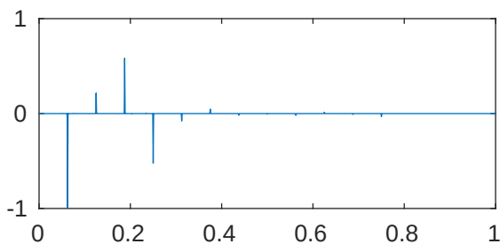
m=5 p=1e-05 \lambda_{603}=2.052676959973443\text{e}+28
