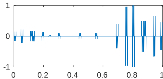
m=5 p=1e-05 \lambda_{458}=2.048092162623497\text{e}+28
