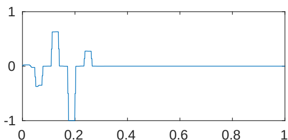
m=5 p=1e-05 \lambda_{23}=1.277400255814515\text{e}+17
