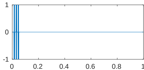
m=5 p=1e-05 \lambda_{944}=4.096199702145382\text{e}+28
