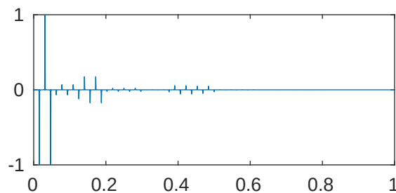
m=5 p=1e-05 \lambda_{588}=2.052674840968141\text{e}+28
