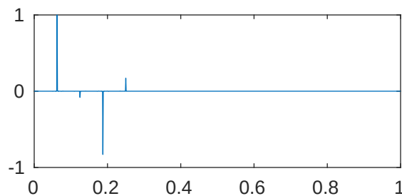
m=5 p=1e-05 \lambda_{408}=2.04352783573668\text{e}+28
