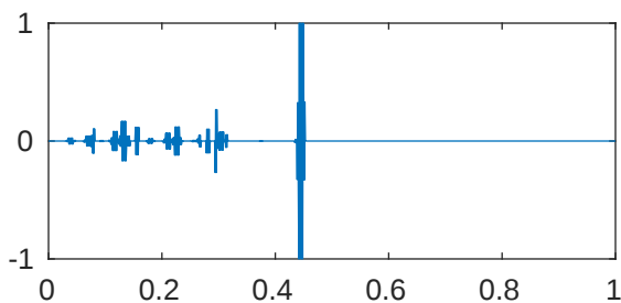
m=5 p=1e-08 \lambda_{879}=4.096000137935762\text{e}+43
