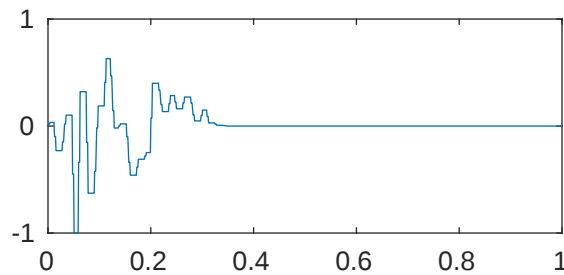
m=5 p=1e-08 \lambda_{56}=9.349045711709273\text{e}+27
