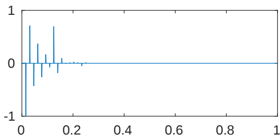
m=5 p=1e-08 \lambda_{425}=2.047855271103078\text{e}+43
