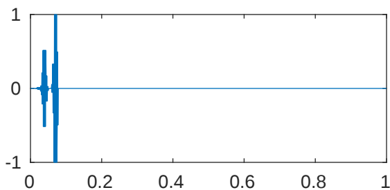
m=5 p=1e-08 \lambda_{921}=4.09600014305576e+43
