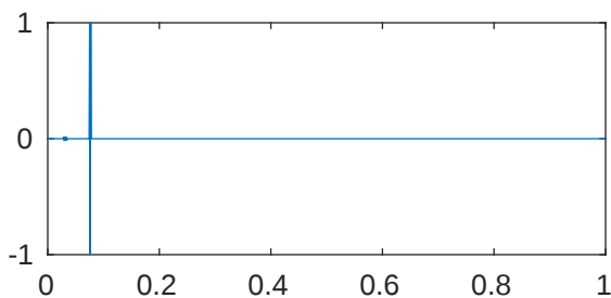
m=5 p=1e-08 \lambda_{945}=4.096000153397167\text{e}+43
