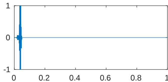
m=5 p=1e-08 \lambda_{920}=4.096000143055757e+43
