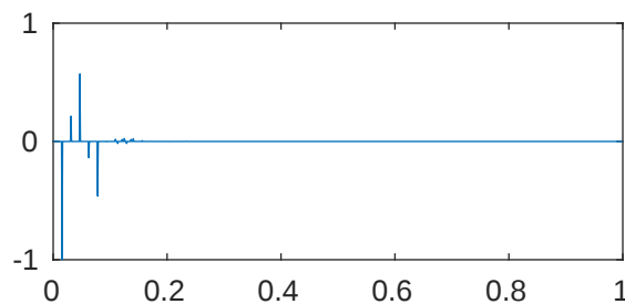
m=5 p=1e-08 \lambda_{390}=2.04785526119803e+43
