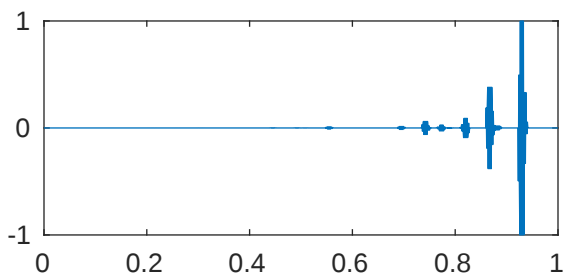
m=5 p=1e-08 \lambda_{941}=4.096000143055771\text{e}+43
