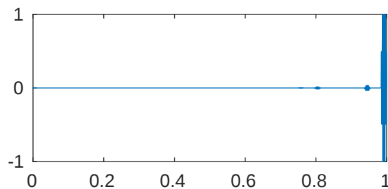
m=5 p=1e-08 \lambda_{1000}=4.096000163637174e+43
