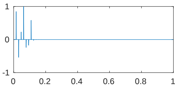
m=5 p=1e-08 \lambda_{599}=2.048144877625668e+43
