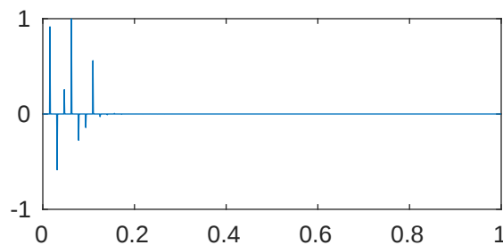
m=5 p=1e-08 \lambda_{600}=2.048144878058874e+43
