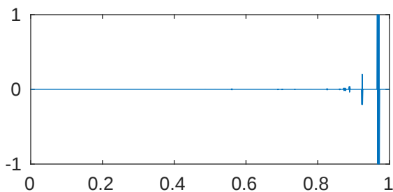
m=5 p=1e-08 \lambda_{951}=4.096000153397178\text{e}+43
