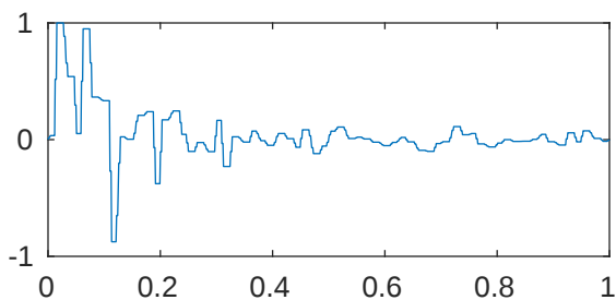
m=5 p=1e-08 \lambda_{45}=4.643153870700035e+27
