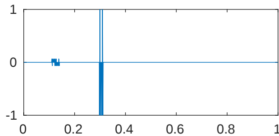
m=5 p=1e-08 \lambda_{560}=2.048000092058605e+43
