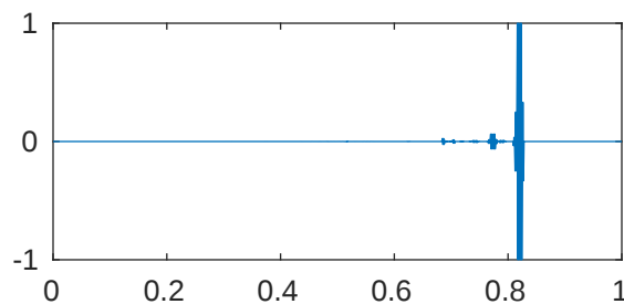
m=5 p=1e-08 \lambda_{916}=4.096000137935779\text{e}+43
