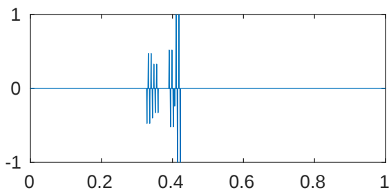
m=5 p=1e-08 \lambda_{711}=2.048204856103266\text{e}+43
