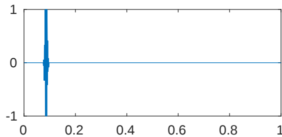
m=5 p=1e-08 \lambda_{846}=4.096000122474366\text{e}+43
