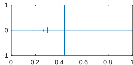
m=5 p=1e-08 \lambda_{970}=4.096000153397203\text{e}+43
