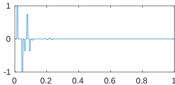
m=5 p=1e-08 \lambda_{74}=5.119024506734204\text{e}+34
