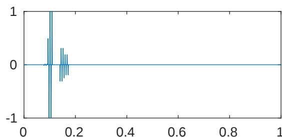
m=5 p=1e-08 \lambda_{270}=2.047795266374673\text{e}+43
