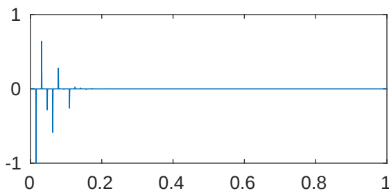
m=5 p=1e-08 \lambda_{605}=2.048144880563073\text{e}+43
