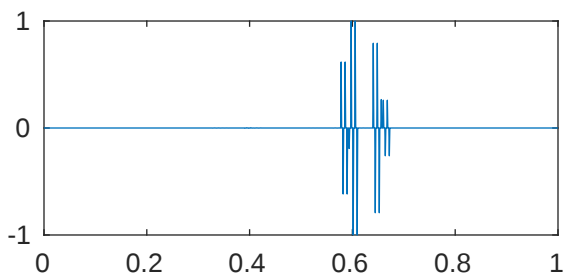
m=5 p=1e-08 \lambda_{705}=2.048204856093352\text{e}+43
