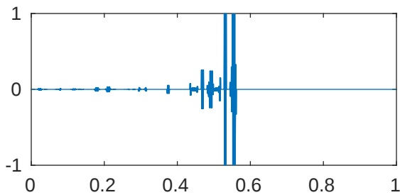
m=5 p=1e-08 \lambda_{895}=4.096000137935767\text{e}+43
