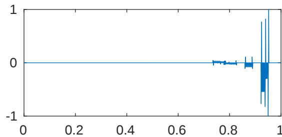
m=5 p=1e-08 \lambda_{542}=2.048000089059358e+43
