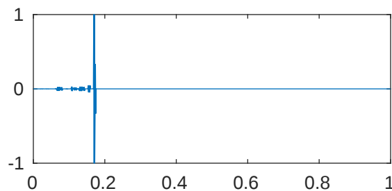
m=5 p=1e-08 \lambda_{918}=4.096000137935782\text{e}+43
