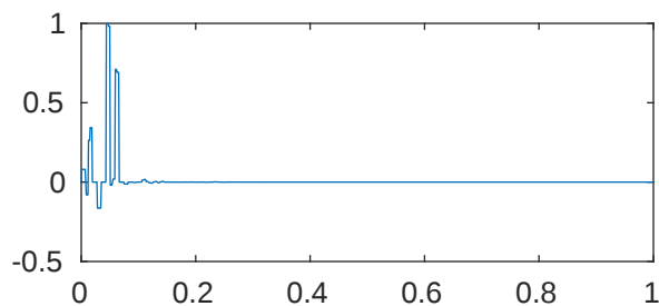
m=5 p=1e-08 \lambda_{147}=5.120000655105479\text{e}+34
