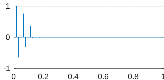
m=5 p=1e-08 \lambda_{346}=2.047855248748771\text{e}+43
