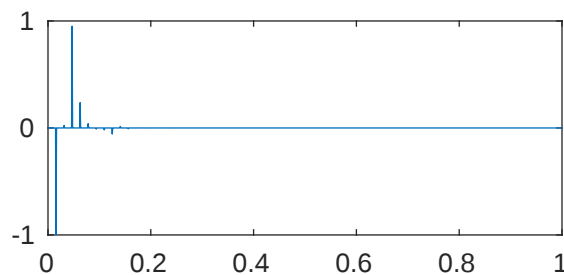
m=5 p=1e-08 \lambda_{672}=2.048144897787514\text{e}+43
