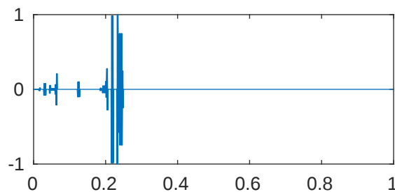
m=5 p=1e-08 \lambda_{972}=4.096000158517174\text{e}+43
