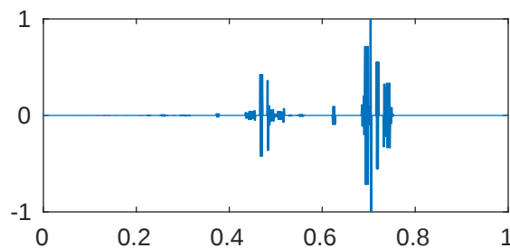
m=5 p=1e-08 \lambda_{904}=4.09600013793577\text{e}+43
