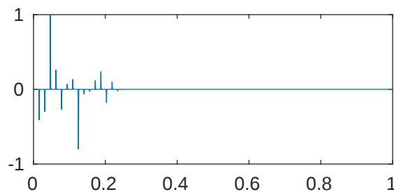
m=5 p=1e-08 \lambda_{444}=2.047855275506311\text{e}+43
