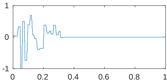
m=5 p=1e-08 \lambda_{55}=8.152853050964059\text{e}+27
