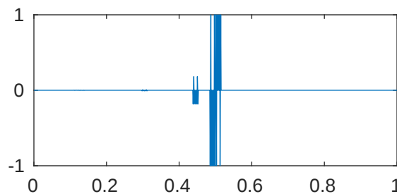
m=5 p=1e-08 \lambda_{558}=2.0480000920586\text{e}+43
