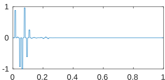
m=5 p=1e-08 \lambda_{71}=5.118813132521073\text{e}+34
