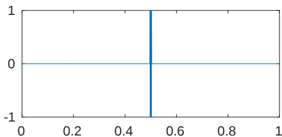
m=5 p=1e-08 \lambda_{993}=4.096000158517188\text{e}+43
