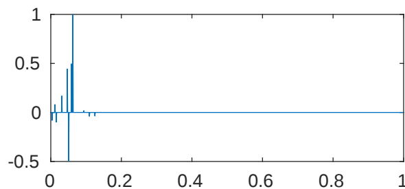
m=5 p=1e-08 \lambda_{426}=2.047855271483257\text{e}+43
