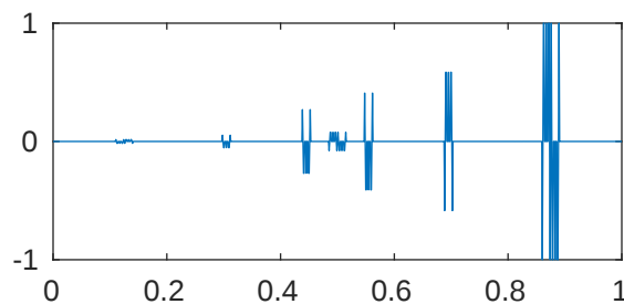
m=5 p=1e-08 \lambda_{492}=2.048000071578692\text{e}+43
