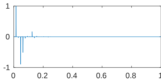
m=5 p=1e-08 \lambda_{682}=2.048144902284601\text{e}+43
