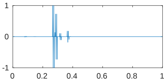
m=5 p=1e-08 \lambda_{721}=2.048204866386436\text{e}+43
