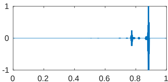
m=5 p=1e-08 \lambda_{923}=4.096000143055762e+43
