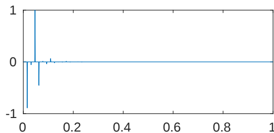
m=5 p=1e-08 \lambda_{666}=2.04814489729863e+43
