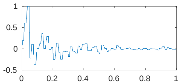
m=5 p=1e-08 \lambda_{17}=-4.831337695382168\text{e}+27
