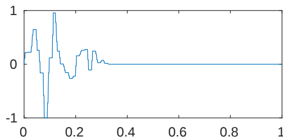
m=5 p=1e-08 \lambda_{34} = -5.898884854259076e+26
