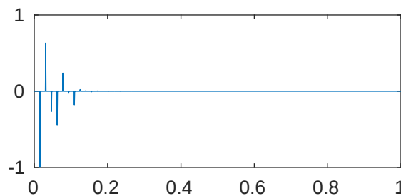
m=5 p=1e-08 \lambda_{606}=2.048144881300311\text{e}+43
