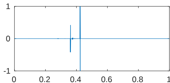
m=5 p=1e-08 \lambda_{858}=4.096000132815768\text{e}+43
