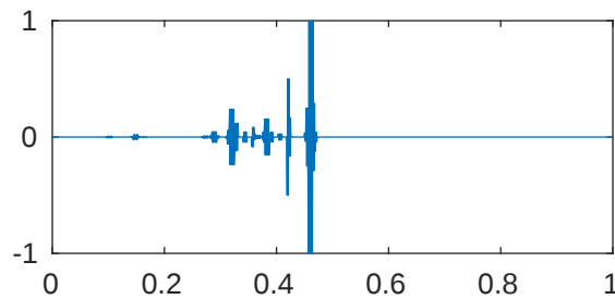
m=5 p=1e-08 \lambda_{794}=4.096000117354348\text{e}+43
