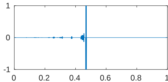
m=5 p=1e-08 \lambda_{902}=4.09600013793577\text{e}+43
