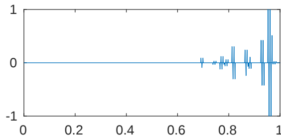
m=5 p=1e-08 \lambda_{308}=2.047795276670713\text{e}+43
