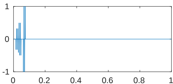
m=5 p=1e-08 \lambda_{309}=2.047795276670846\text{e}+43
