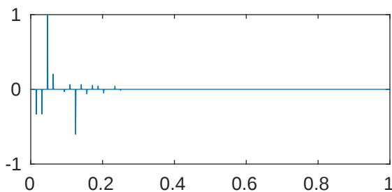
m=5 p=1e-08 \lambda_{695}=2.048144903785699\text{e}+43
