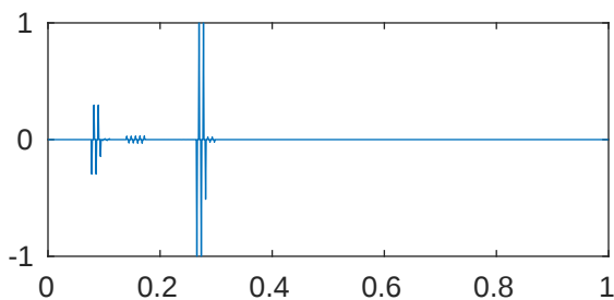
m=5 p=1e-08 \lambda_{725}=2.048204866388016\text{e}+43
