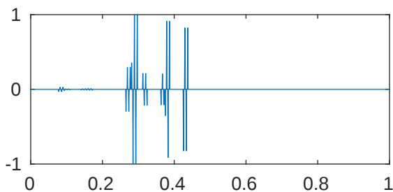
m=5 p=1e-08 \lambda_{713}=2.048204866382567\text{e}+43
