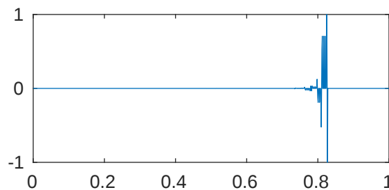
m=5 p=1e-08 \lambda_{504}=2.048000074577829\text{e}+43
