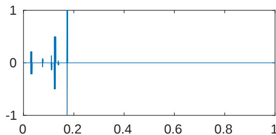
m=5 p=1e-08 \lambda_{952}=4.096000153397179\text{e}+43
