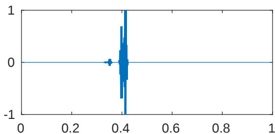
m=5 p=1e-08 \lambda_{783}=4.096000101892954\text{e}+43
