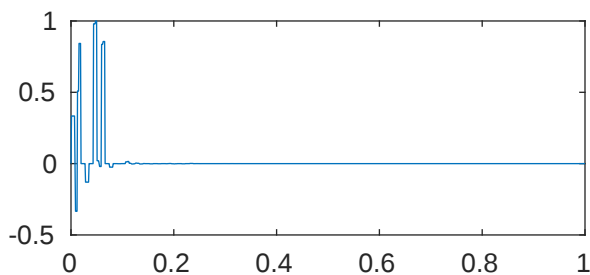
m=5 p=1e-08 \lambda_{119}=5.119999757772043\text{e}+34
