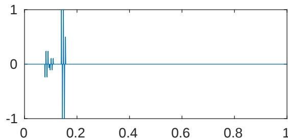
m=5 p=1e-08 \lambda_{266}=2.047795266371095\text{e}+43
