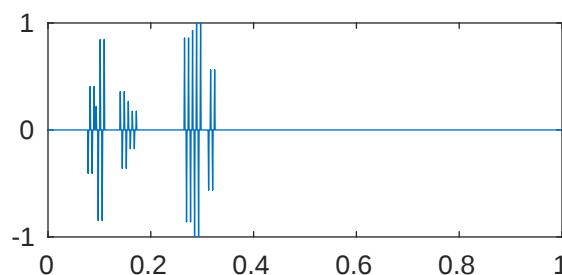
m=5 p=1e-08 \lambda_{732}=2.048204866391199\text{e}+43
