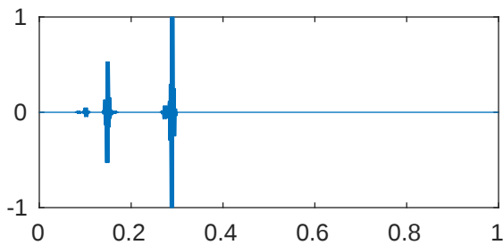
m=5 p=1e-08 \lambda_{793}=4.096000117354346\text{e}+43
