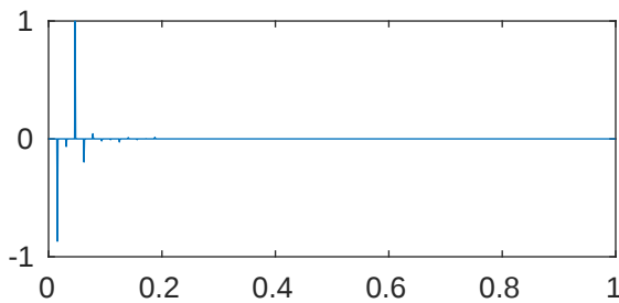
m=5 p=1e-08 \lambda_{679}=2.048144900168365\text{e}+43
