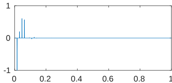
m=5 p=1e-08 \lambda_{380}=2.047855261102432\text{e}+43
