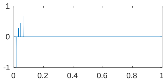
m=5 p=1e-08 \lambda_{630}=2.048144890037022e+43
