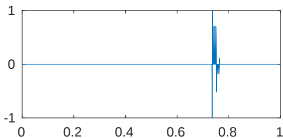
m=5 p=1e-08 \lambda_{497}=2.048000074577817\text{e}+43
