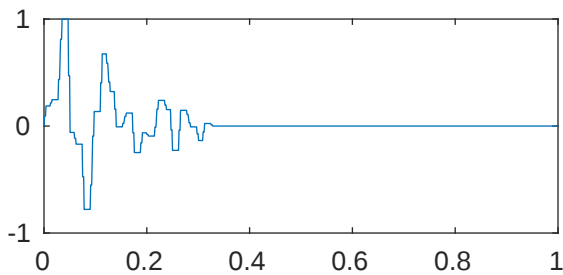
m=5 p=1e-08 \lambda_{19} = -4.292242720501172e+27
