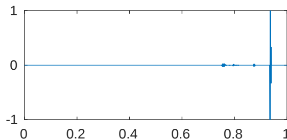
m=5 p=1e-08 \lambda_{982}=4.096000158517179\text{e}+43
