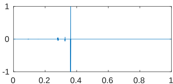
m=5 p=1e-08 \lambda_{855}=4.096000132815766\text{e}+43
