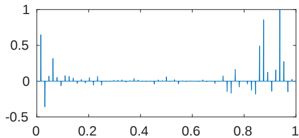
m=5 p=1e-08 \lambda_{703}=2.048144912448002\text{e}+43
