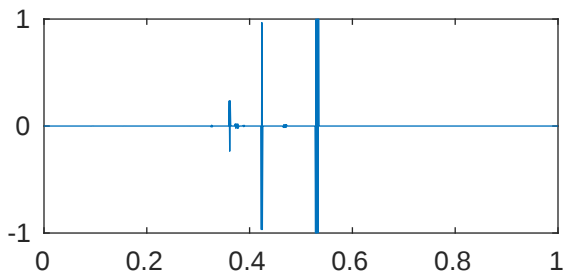
m=5 p=1e-08 \lambda_{859}=4.096000132815768\text{e}+43
