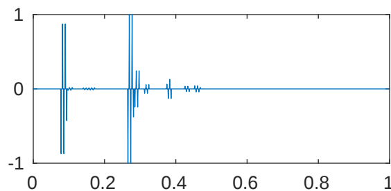
m=5 p=1e-08 \lambda_{724}=2.048204866387429\text{e}+43
