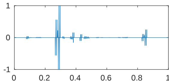
m=5 p=1e-08 \lambda_{716}=2.048204866384661\text{e}+43
