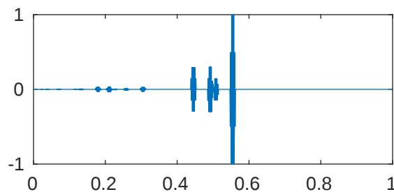
m=5 p=1e-08 \lambda_{934}=4.096000143055768e+43
