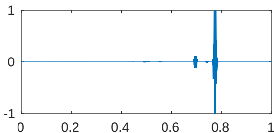
m=5 p=1e-08 \lambda_{927}=4.096000143055763\text{e}+43
