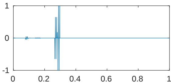
m=5 p=1e-08 \lambda_{283}=2.047795266380009\text{e}+43
