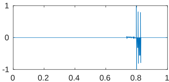
m=5 p=1e-08 \lambda_{547}=2.048000089059366\text{e}+43
