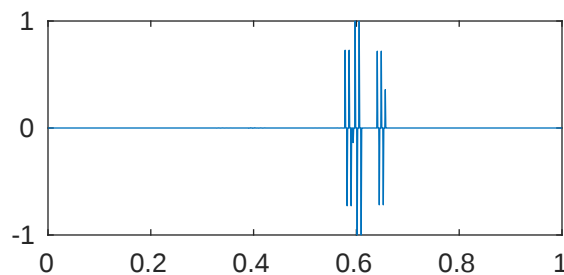
m=5 p=1e-08 \lambda_{262}=2.047795256089569\text{e}+43
