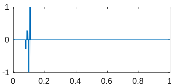
m=5 p=1e-08 \lambda_{731}=2.04820486639072\text{e}+43
