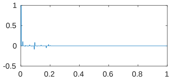
m=5 p=1e-08 \lambda_{217}=1.024000012822001\text{e}+35
