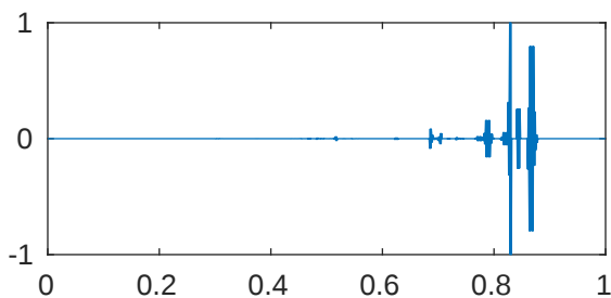
m=5 p=1e-08 \lambda_{911}=4.096000137935774\text{e}+43
