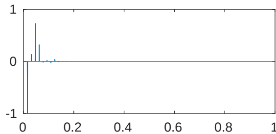
m=5 p=1e-08 \lambda_{656}=2.04814489462182\text{e}+43
