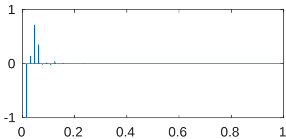
m=5 p=1e-08 \lambda_{655}=2.048144894261398\text{e}+43
