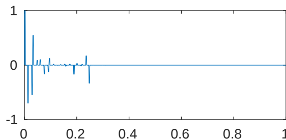
m=5 p=1e-08 \lambda_{192}=1.023999907626259\text{e}+35
