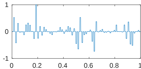
m=5 p=1e-08 \lambda_{140}=5.120000471514208\text{e}+34
