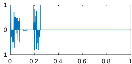
m=5 p=1e-08 \lambda_{545}=2.048000089059365e+43
