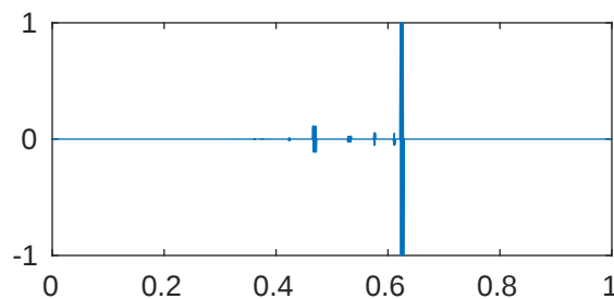
m=5 p=1e-08 \lambda_{864}=4.096000132815774\text{e}+43
