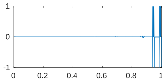
m=5 p=1e-08 \lambda_{522}=2.048000081818504\text{e}+43
