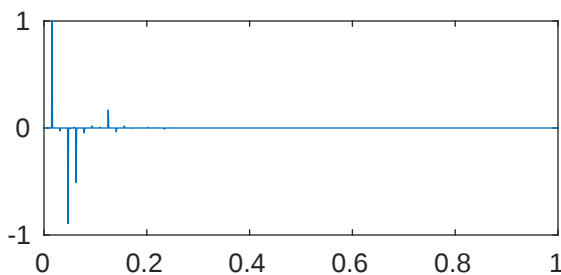
m=5 p=1e-08 \lambda_{681}=2.048144902284601\text{e}+43
