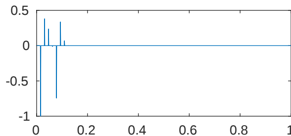
m=5 p=1e-08 \lambda_{618}=2.048144887103798\text{e}+43
