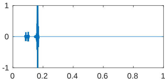
m=5 p=1e-08 \lambda_{843}=4.096000122474362\text{e}+43
