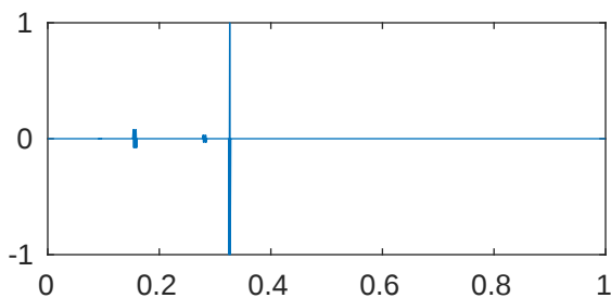
m=5 p=1e-08 \lambda_{849}=4.096000132815756\text{e}+43
