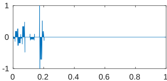
m=5 p=1e-08 \lambda_{499}=2.048000074577821\text{e}+43
