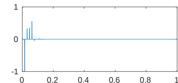
m=5 p=1e-08 \lambda_{624}=2.048144888946509\text{e}+43
