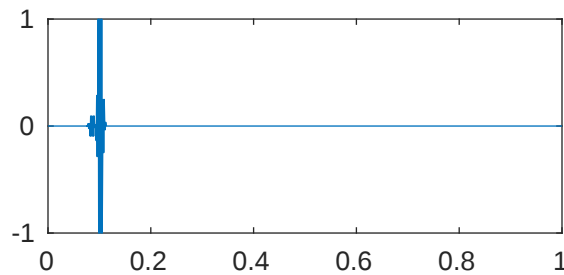
m=5 p=1e-08 \lambda_{806}=4.096000117354354\text{e}+43
