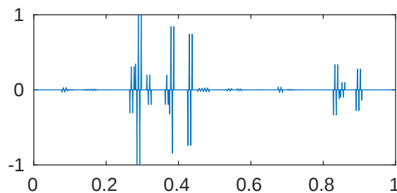
m=5 p=1e-08 \lambda_{286}=2.047795266382311\text{e}+43
