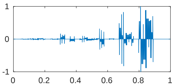
m=5 p=1e-08 \lambda_{519}=2.048000078768668\text{e}+43
