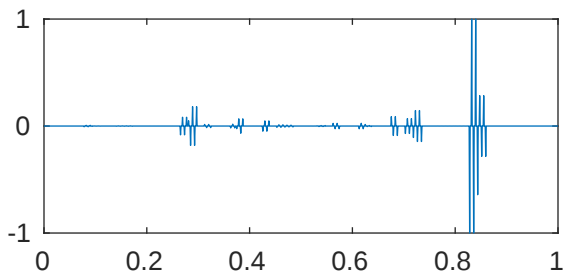
m=5 p=1e-08 \lambda_{715}=2.048204866384068\text{e}+43
