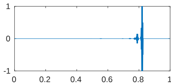
m=5 p=1e-08 \lambda_{942}=4.096000143055774\text{e}+43
