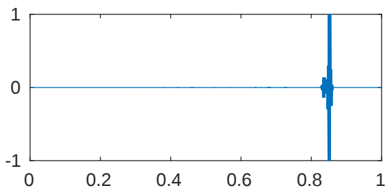
m=5 p=1e-08 \lambda_{797}=4.096000117354349\text{e}+43
