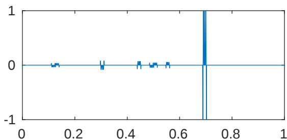
m=5 p=1e-08 \lambda_{489}=2.048000071578607\text{e}+43
