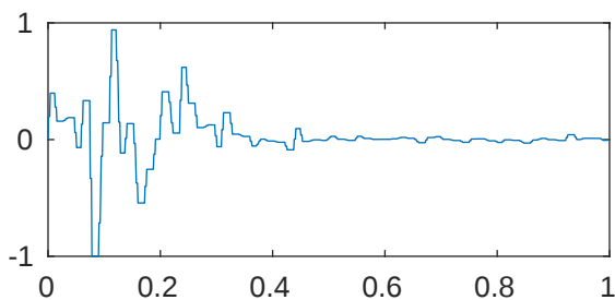
m=5 p=1e-08 \lambda_{53}=8.00514464729231e+27
