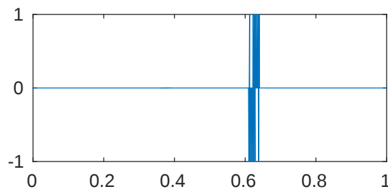
m=5 p=1e-08 \lambda_{520}=2.048000081767893\text{e}+43
