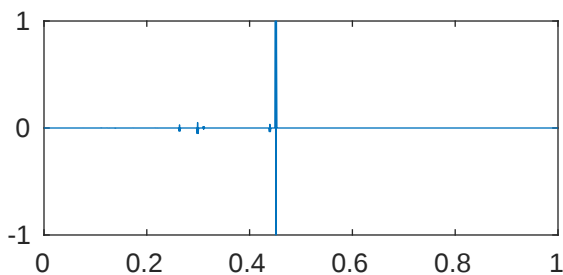
m=5 p=1e-08 \lambda_{969}=4.096000153397198\text{e}+43
