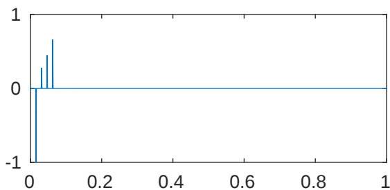
m=5 p=1e-08 \lambda_{627}=2.048144890010321e+43
