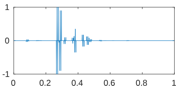
m=5 p=1e-08 \lambda_{281}=2.0477952663789\text{e}+43
