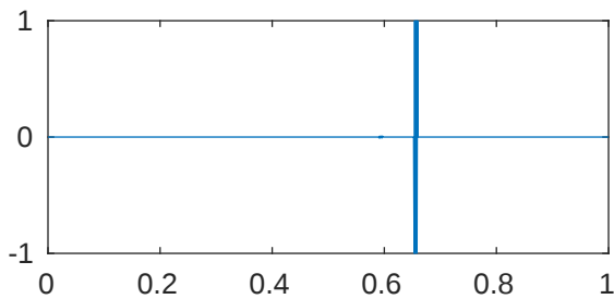
m=5 p=1e-08 \lambda_{787}=4.096000112234359\text{e}+43
