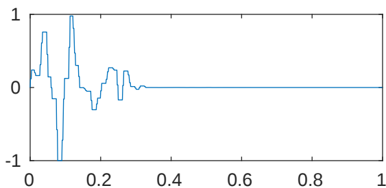
m=5 p=1e-08 \lambda_{27} = -1.611067487870294e+27
