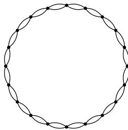
FIG. 2: The bracelet graph B_{20} .
