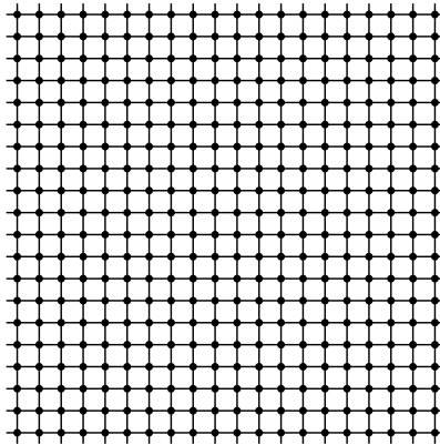
FIG. 1: The square grid \mathbb{Z}^2 .
