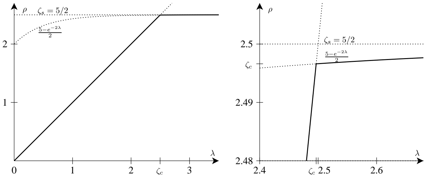
FIG. 3: Density \rho(\lambda) of the final stable configuration as a function of initial density \lambda , for the driven sandpile on the bracelet graph \hat{B}_n as n \rightarrow \infty . A second-order phase transition occurs at \lambda = \zeta_c . Beyond this transition, the density of the driven sandpile continues to increase, approaching the stationary density \zeta_s from below.
