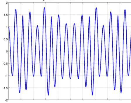
eigenvalue: 6132.7161, series: 0, word: 93111
