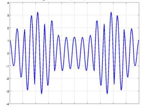
eigenvalue: 6452.9806, series: 0, word: 11-3-1-1-1
