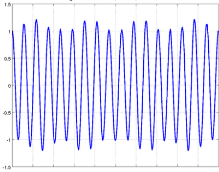
eigenvalue: 6835.5227, series: 0, word: 53111
