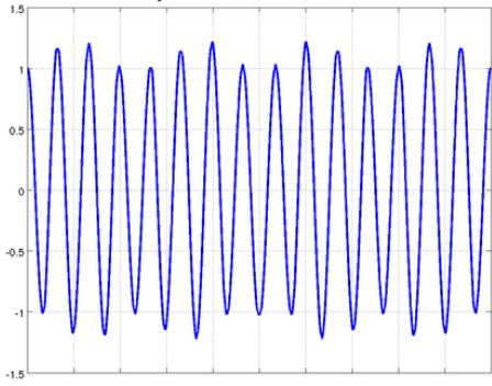
eigenvalue: 5230.4232, series: 0, word: 53111
