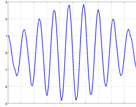
eigenvalue: 1789.6075, series: 1.33, word: 1211
