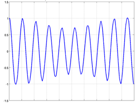
eigenvalue: 2167.811, series: 1.33, word: 1311
