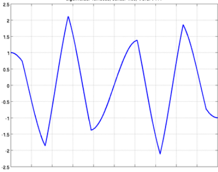
eigenvalue: 107.5659, series: 1.33, word: 7111
