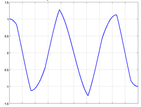
eigenvalue: 66.7754, series: 1.33, word: 5111
