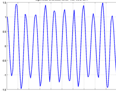
eigenvalue: 2799.6003, series: 1.33, word: 5311
