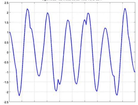
eigenvalue: 1324.7505, series: 1.33, word: 5211
