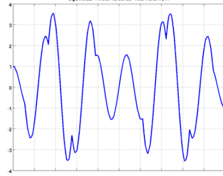
eigenvalue: 1173.9716, series: 1.33, word: 7211
