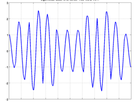
eigenvalue: 2958.1319, series: 1.33, word: 7311
