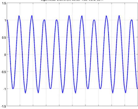
eigenvalue: 2454.6194, series: 1.33, word: 3311
