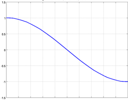
eigenvalue: 3.0911, series: 1.33, word: 1111
