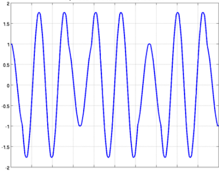
eigenvalue: 1542.5779, series: 1.33, word: 3211
