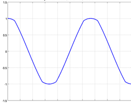
eigenvalue: 26.6267, series: 1.33, word: 3111
