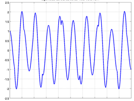
eigenvalue: 2870.2735, series: 1.33, word: 7211
