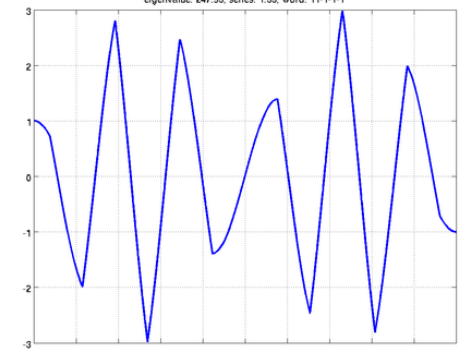
eigenvalue: 247.93, series: 1.33, word: 11-1-1-1
