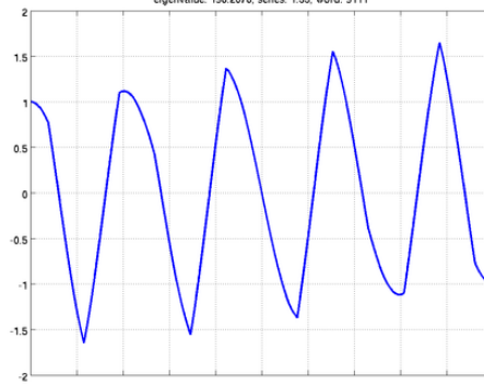
eigenvalue: 198.2078, series: 1.33, word: 9111
