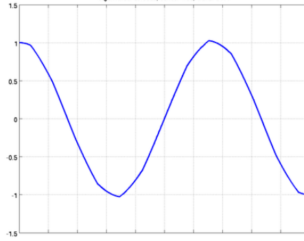
eigenvalue: 27.6329, series: 1.33, word: 3111
