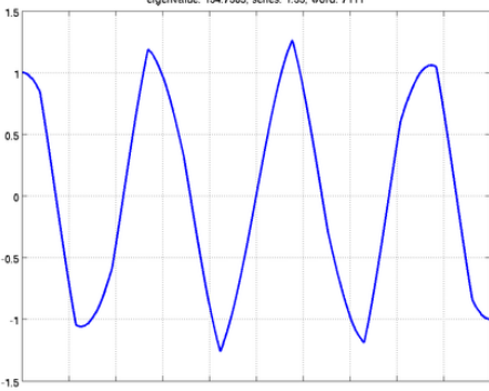
eigenvalue: 134.7385, series: 1.33, word: 7111
