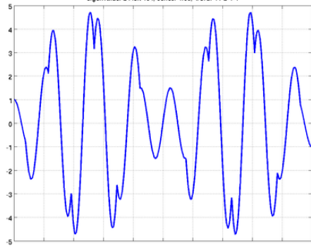
eigenvalue: 2449.7184, series: 1.33, word: 11-2-1-1
