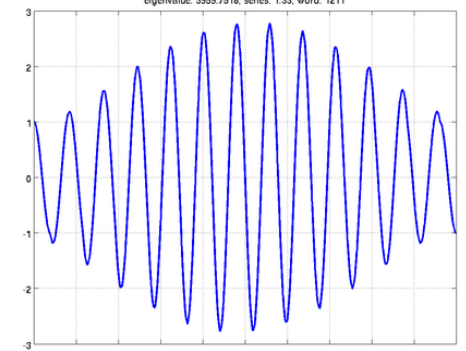
eigenvalue: 3959.7518, series: 1.33, word: 1211
