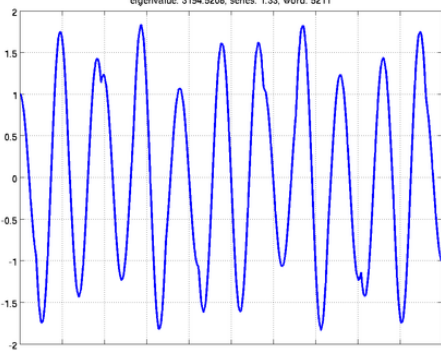
eigenvalue: 3194.5208, series: 1.33, word: 5211
