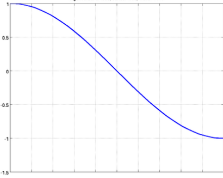
eigenvalue: 3.1556, series: 1.33, word: 1111
