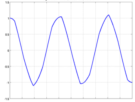
eigenvalue: 74.0207, series: 1.33, word: 5111
