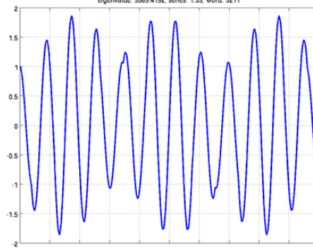
eigenvalue: 3569.4192, series: 1.33, word: 3211
