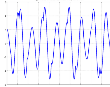
eigenvalue: 2615.9959, series: 1.33, word: 9211
