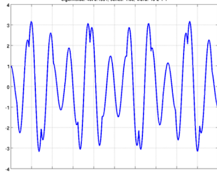
eigenvalue: 4370.1991, series: 1.33, word: 19-2-1-1
