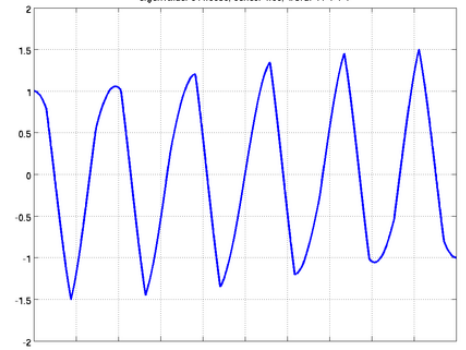
eigenvalue: 311.0653, series: 1.33, word: 11-1-1-1
