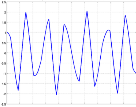
eigenvalue: 387.5424, series: 1.33, word: 13-1-1-1
