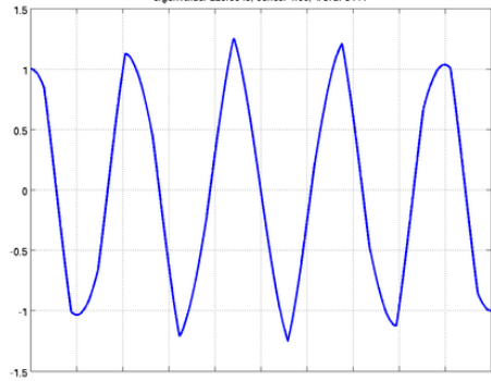
eigenvalue: 226.0845, series: 1.33, word: 9111
