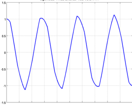
eigenvalue: 144.8245, series: 1.33, word: 7111
