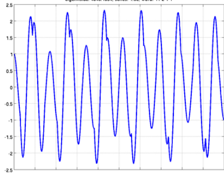
eigenvalue: 4643.1594, series: 1.33, word: 11-2-1-1
