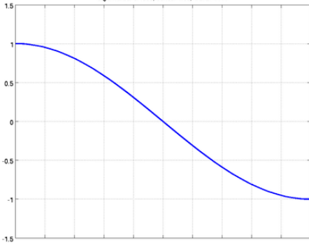
eigenvalue: 3.1685, series: 1.33, word: 1111
