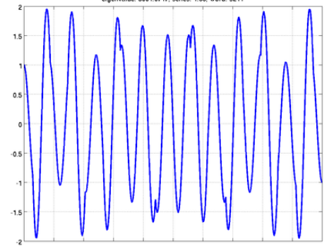
eigenvalue: 5001.0717, series: 1.33, word: 8211
