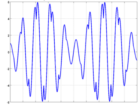
eigenvalue: 4197.7384, series: 1.33, word: 15-2-1-1
