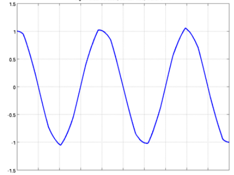
eigenvalue: 76.9003, series: 1.33, word: 5111
