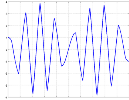
eigenvalue: 441.5383, series: 1.33, word: 15-1-1-1
