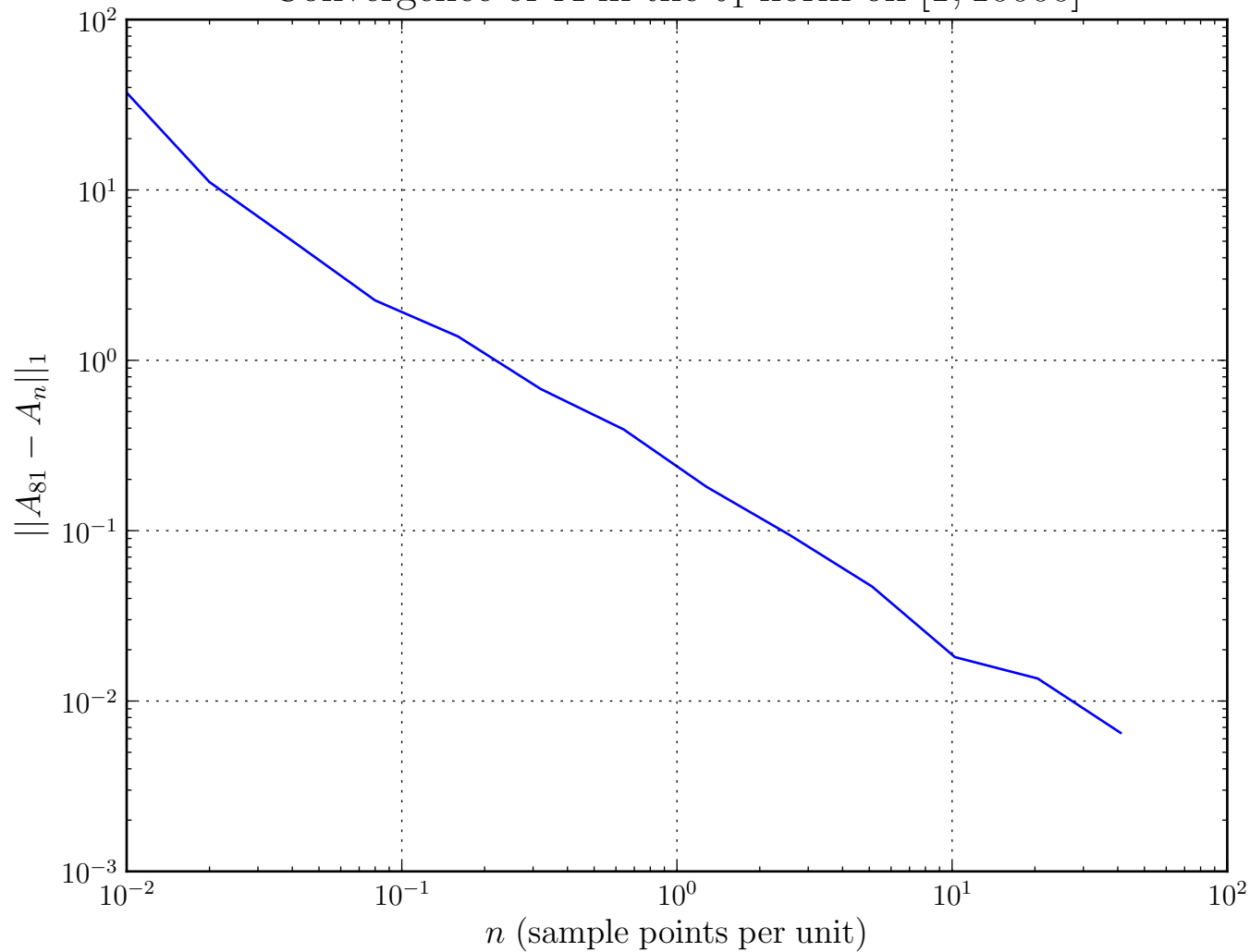
Convergence of A in the \ell_1 norm on [1, 10000]
