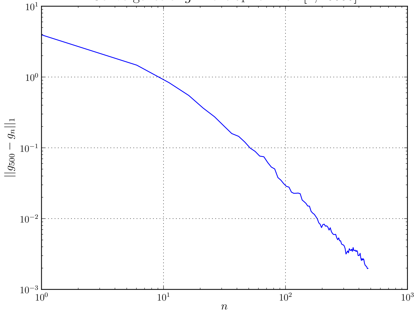
Convergence of g in the \ell_1 norm on [1, 10000]
