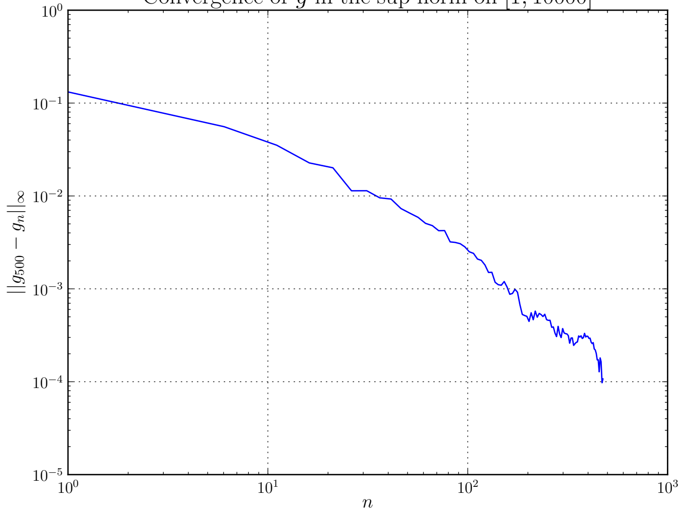
Convergence of g in the sup norm on [1, 10000]
