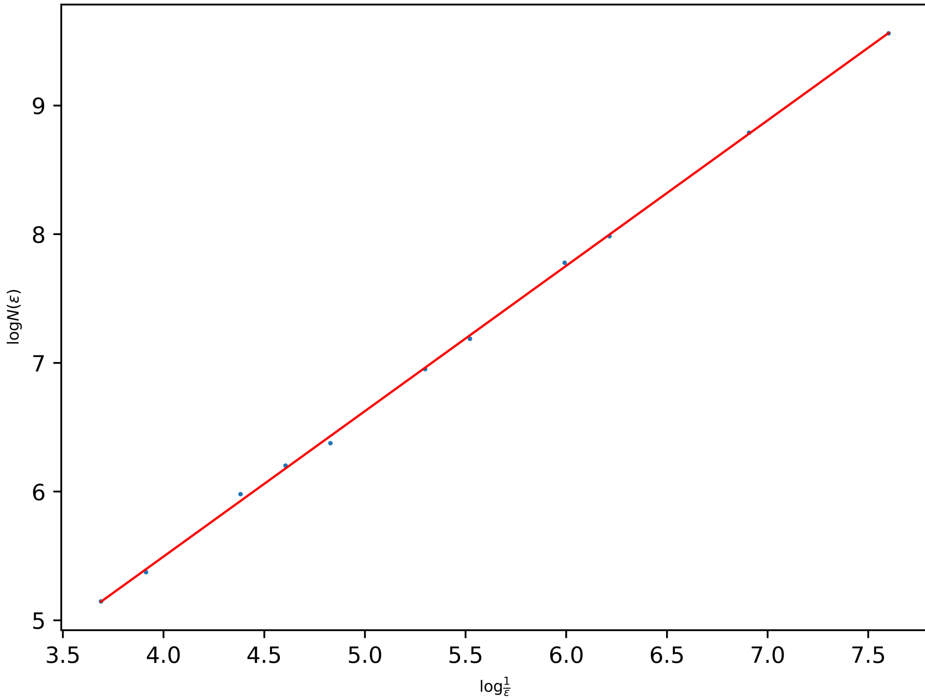
Power-Law of the BC-Dimension of the Quadratic Snowflake ( a = 0.1 , Level 8): 1.1296073169272889
