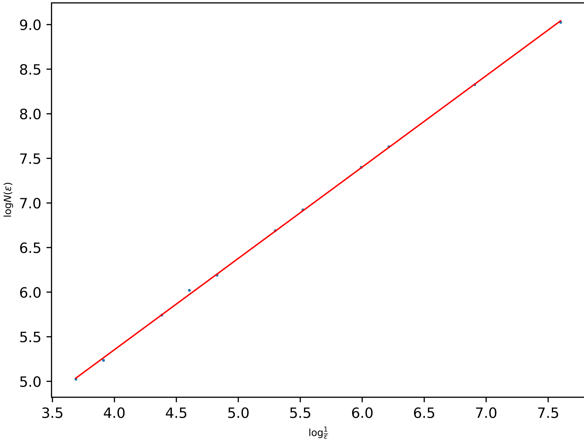
Power-Law of the BC-Dimension of the Quadratic Snowflake (a = 0.1, Level 4): 1.0241787993683944
