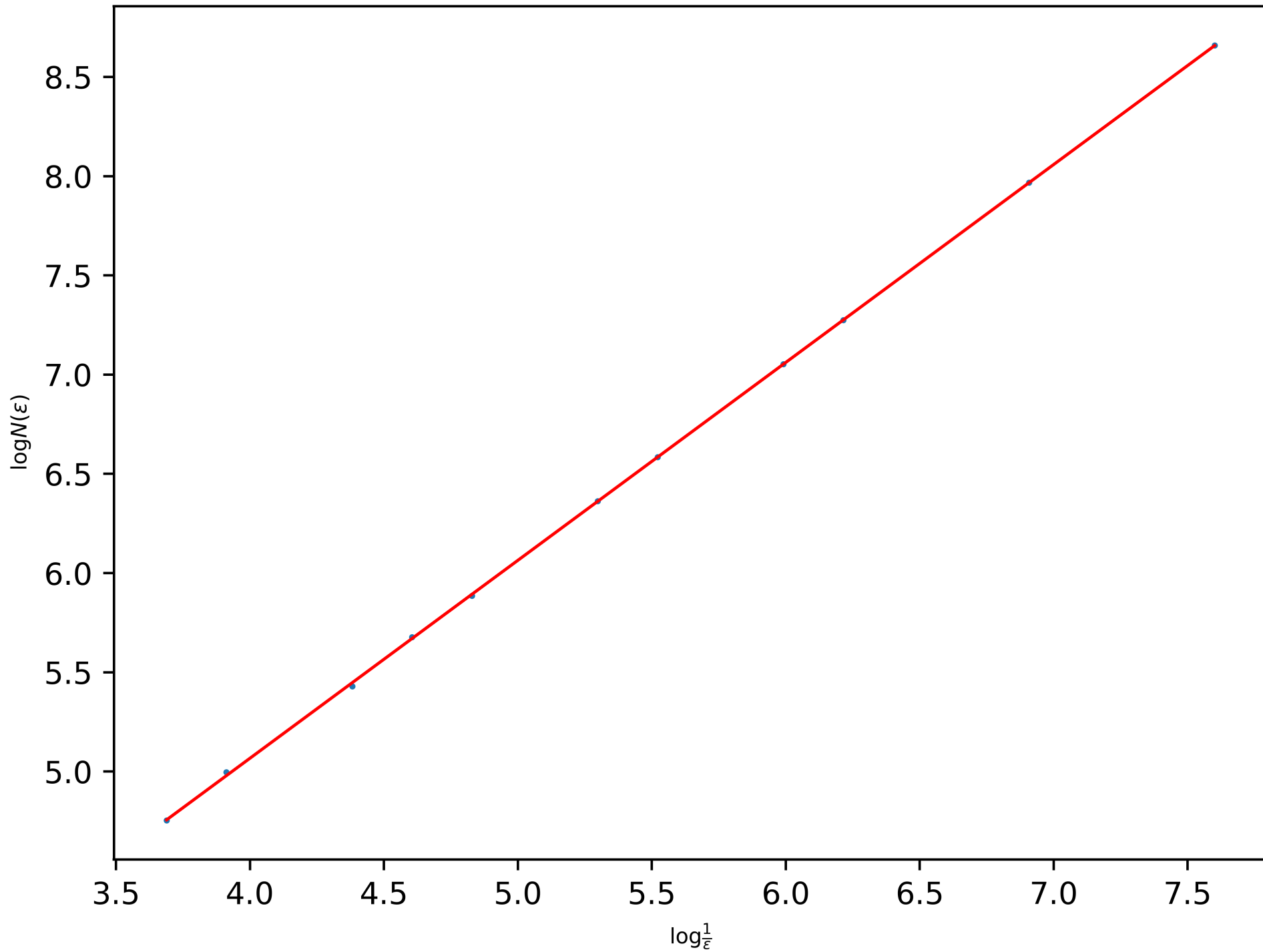
Power-Law of the BC-Dimension of the Quadratic Snowflake (a = 0.1, Level 2): 0.9972090529605772
