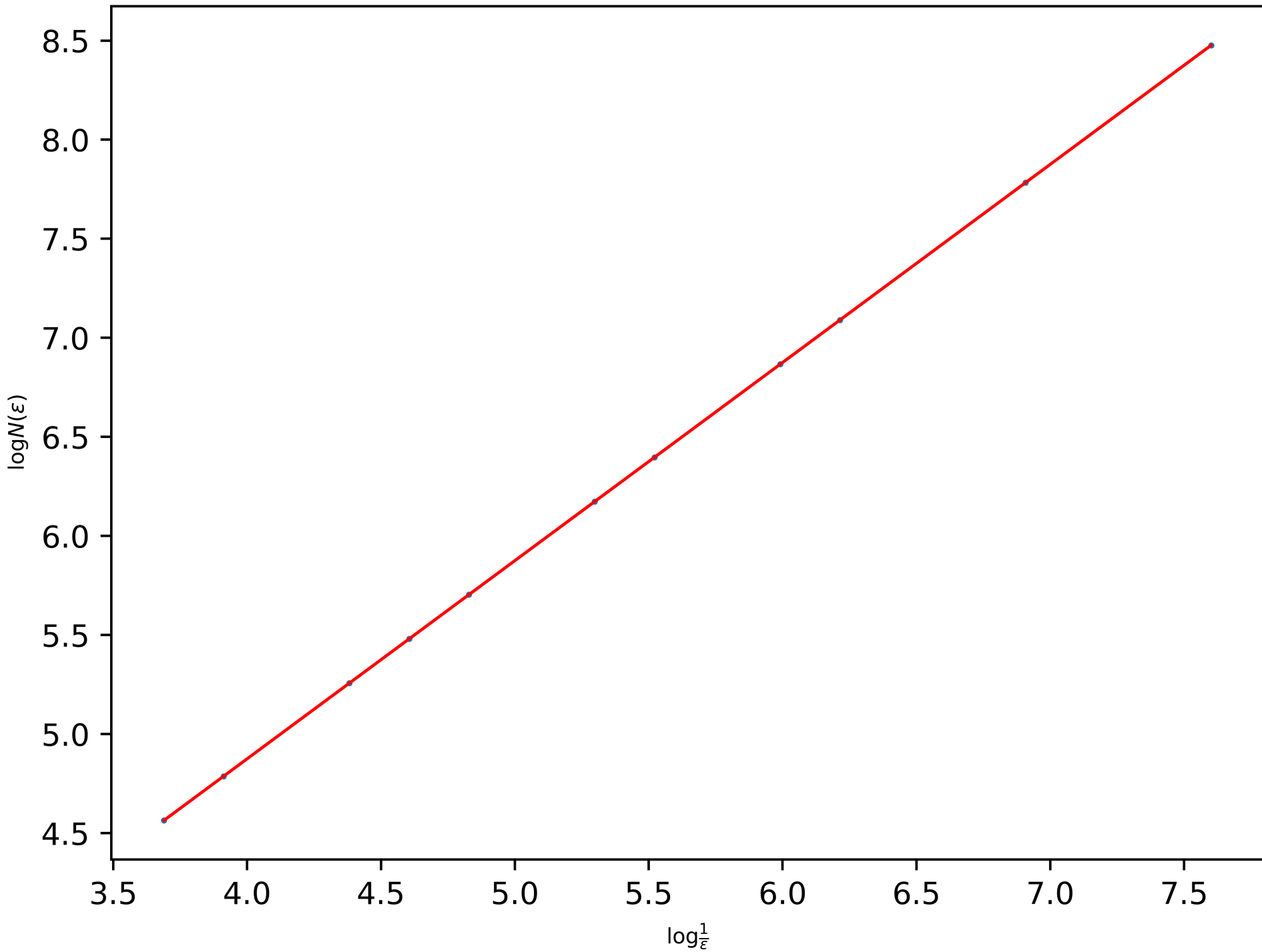
Power-Law of the BC-Dimension of the Quadratic Snowflake (a = 0.1, Level 1): 0.99999999999999996
