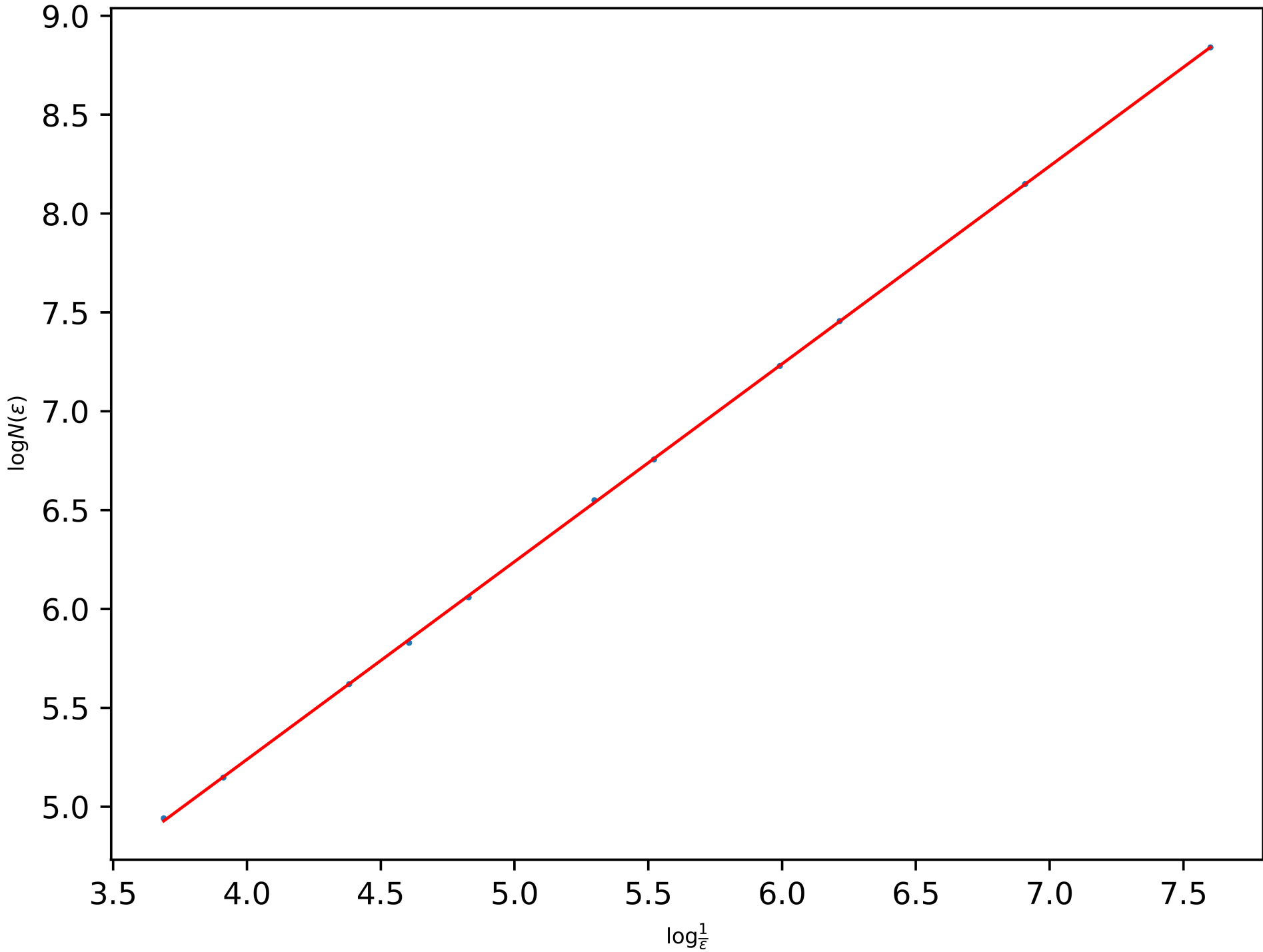
Power-Law of the BC-Dimension of the Quadratic Snowflake (a = 0.1, Level 3): 1.0004571458409588
