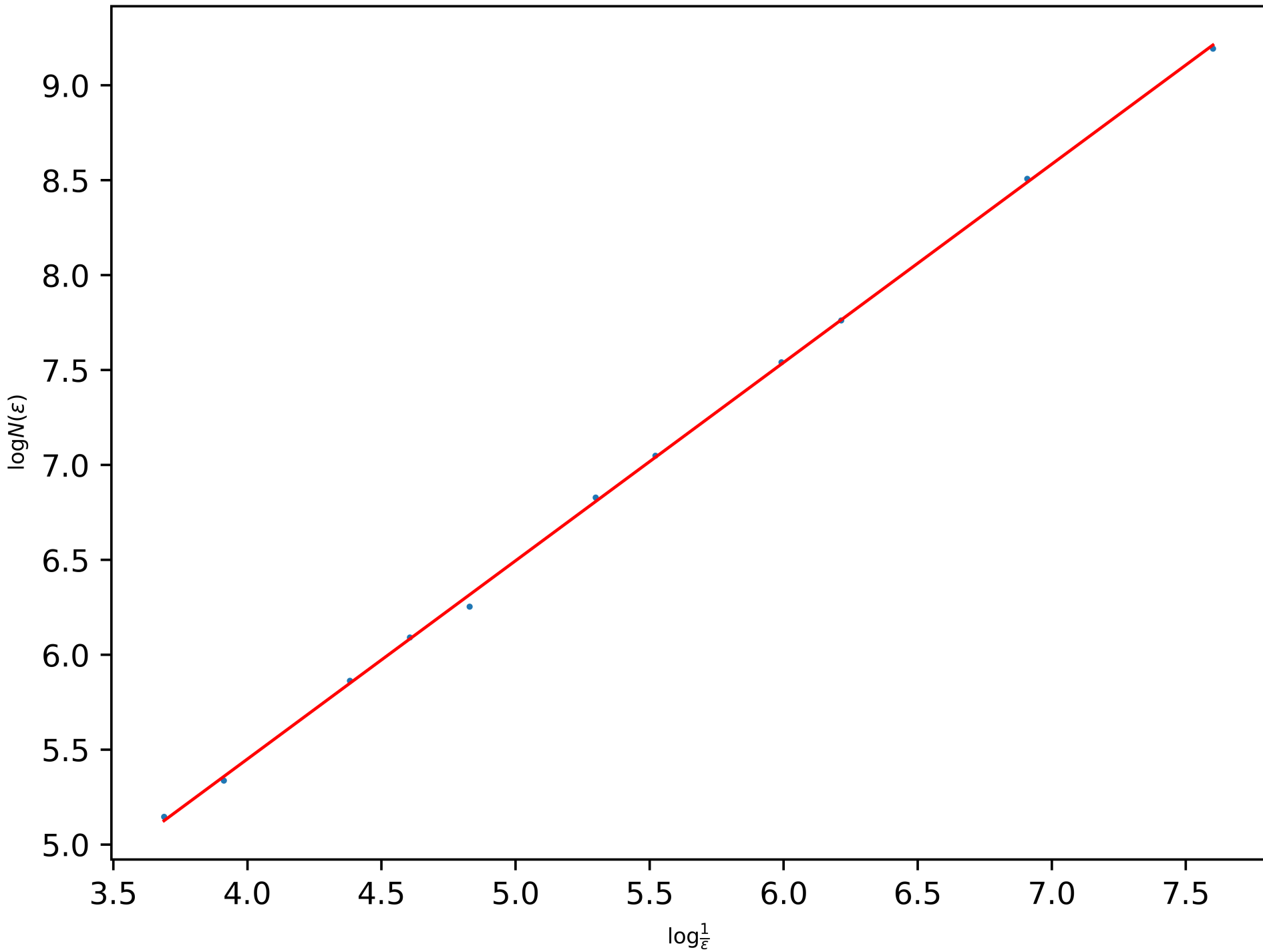
Power-Law of the BC-Dimension of the Quadratic Snowflake (a = 0.1, Level 5): 1.0445938826261858
