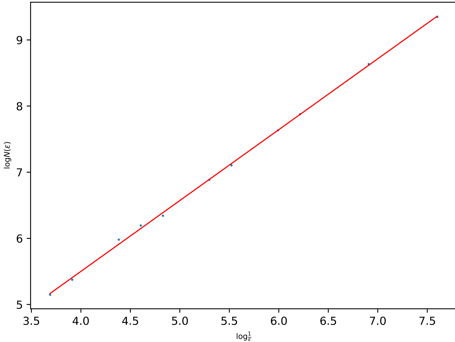
Power-Law of the BC-Dimension of the Quadratic Snowflake ( a = 0.1 , Level 6): 1.0715476279335996
