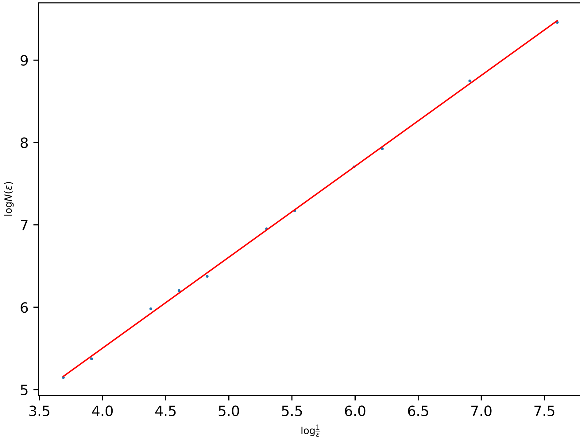
Power-Law of the BC-Dimension of the Quadratic Snowflake ( a = 0.1 , Level 7): 1.1036912889742125
