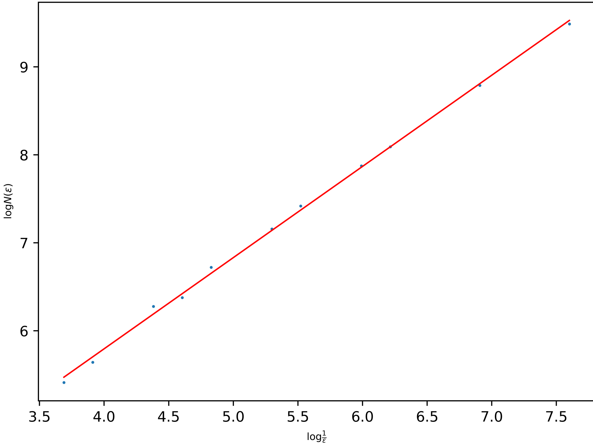
Power-Law of the BC-Dimension of the Quadratic Snowflake ( a = 0.2 , Level 4): 1.036760951205291
