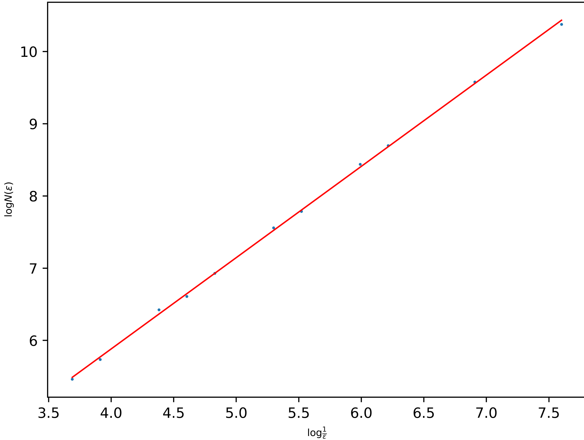
Power-Law of the BC-Dimension of the Quadratic Snowflake ( a = 0.2 , Level 7): 1.2638179241131393
