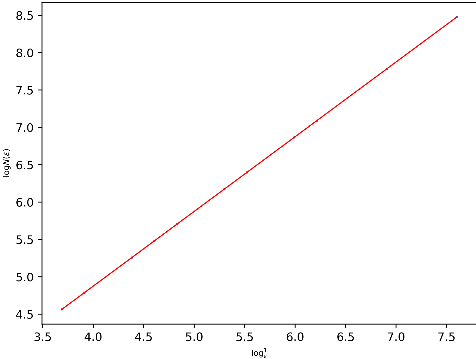
Power-Law of the BC-Dimension of the Quadratic Snowflake (a = 0.2, Level 1): 0.99999999999999996
