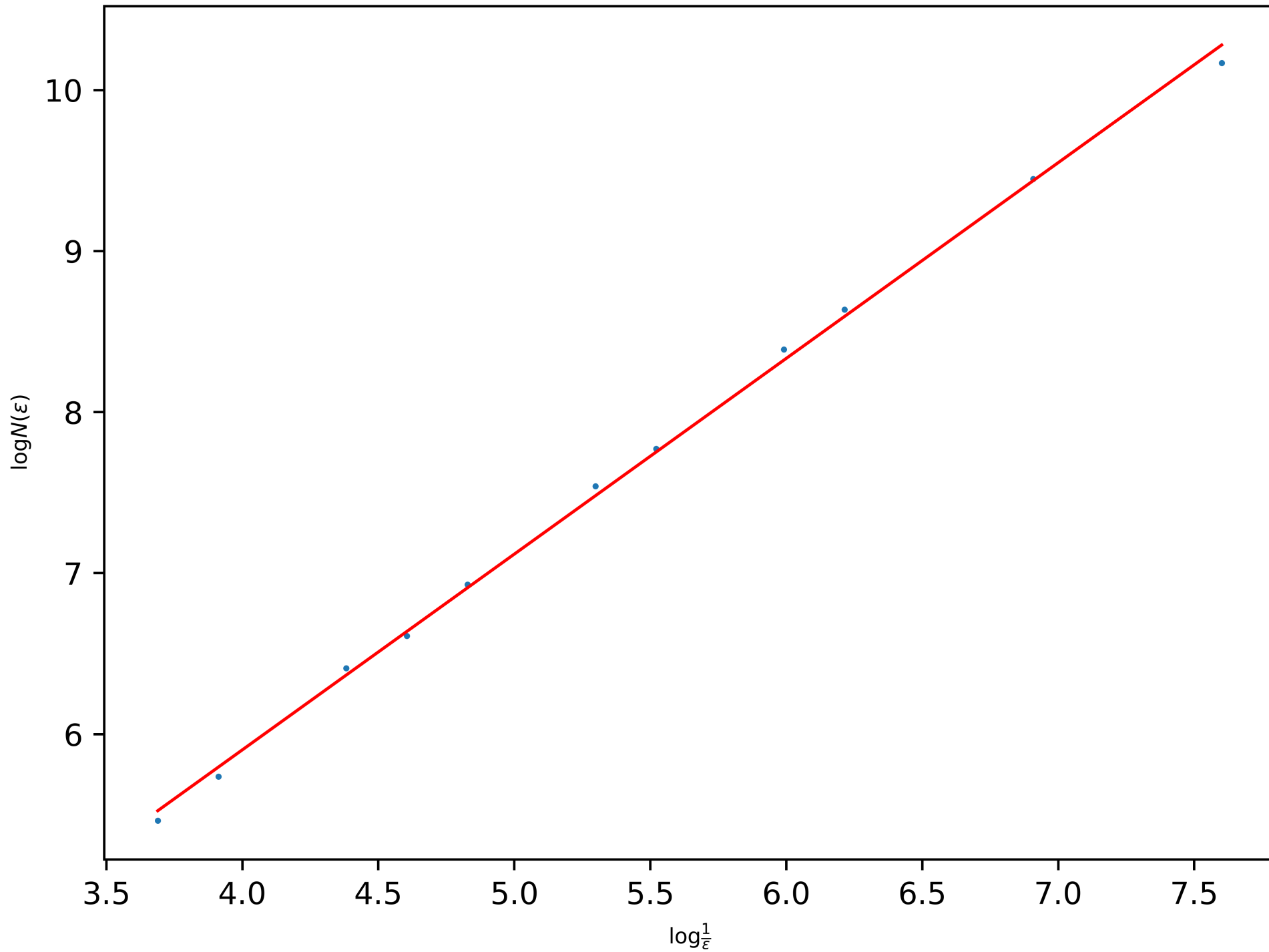
Power-Law of the BC-Dimension of the Quadratic Snowflake ( a = 0.2 , Level 6): 1.215490780771384
