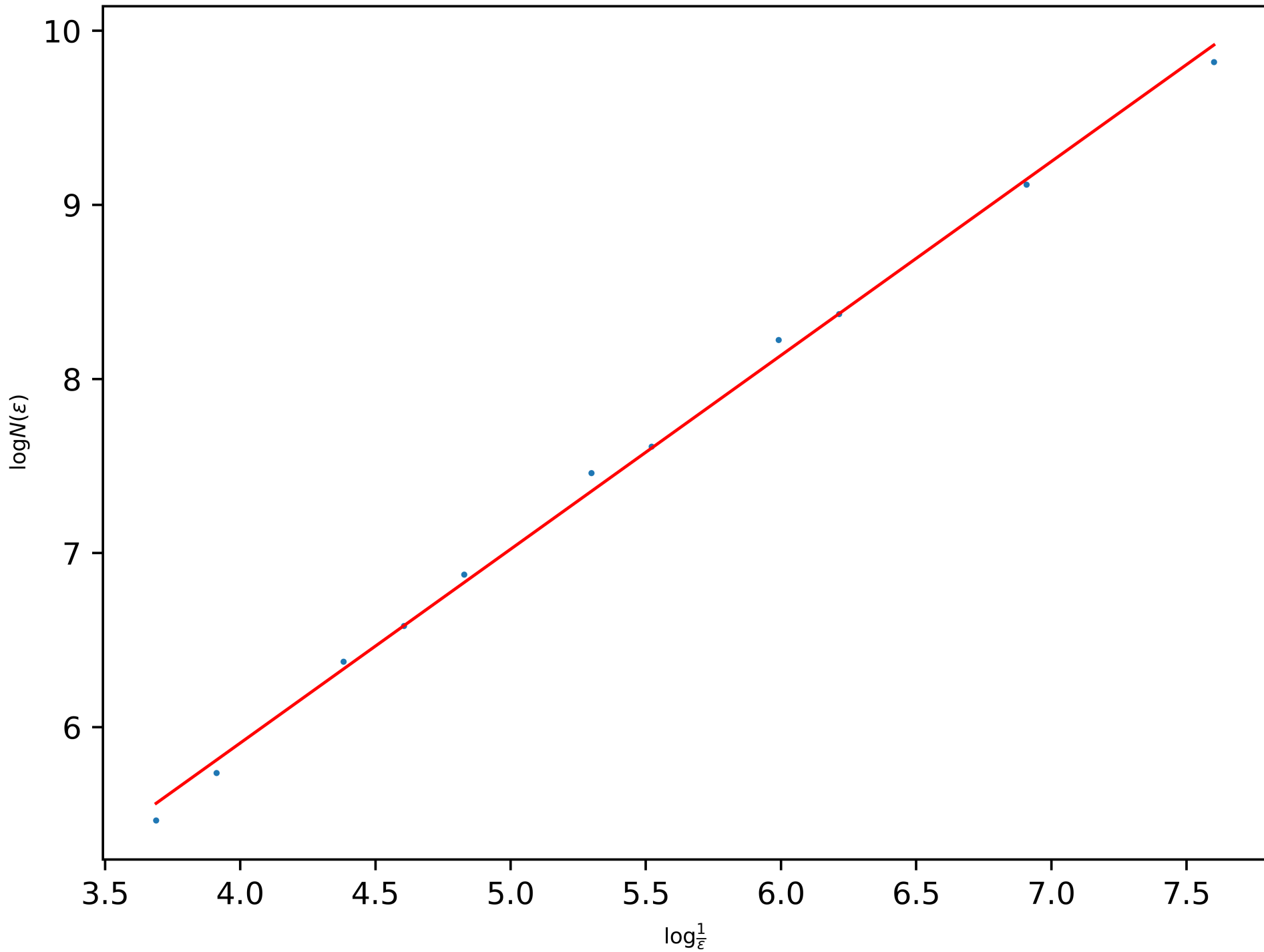
Power-Law of the BC-Dimension of the Quadratic Snowflake ( a = 0.2 , Level 5): 1.1134355918336423
