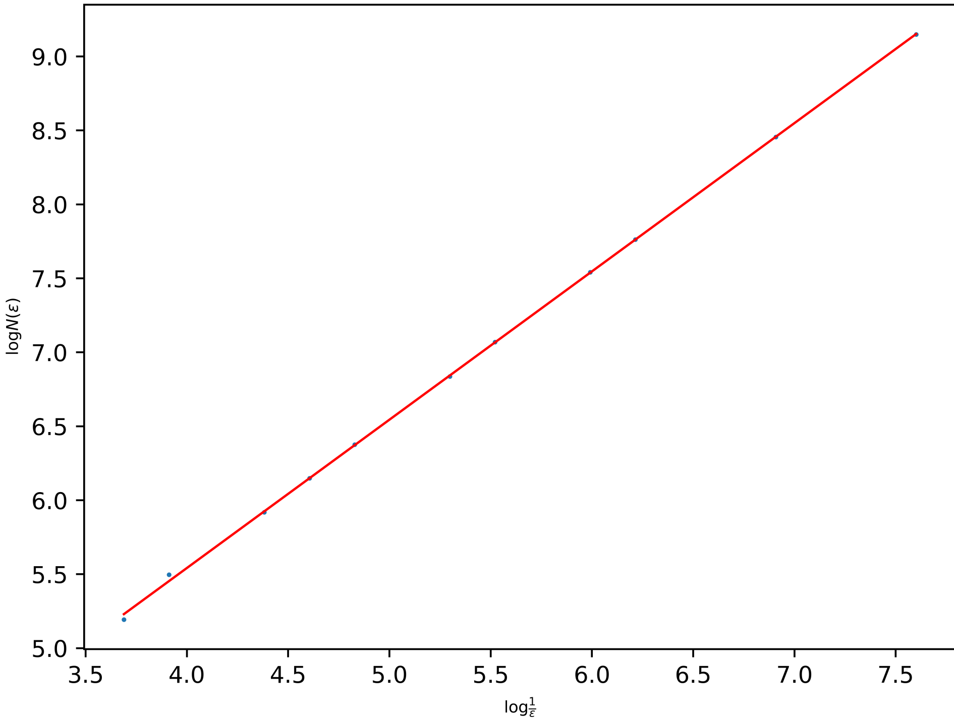
Power-Law of the BC-Dimension of the Quadratic Snowflake (a = 0.2, Level 3): 1.0024494665006298
