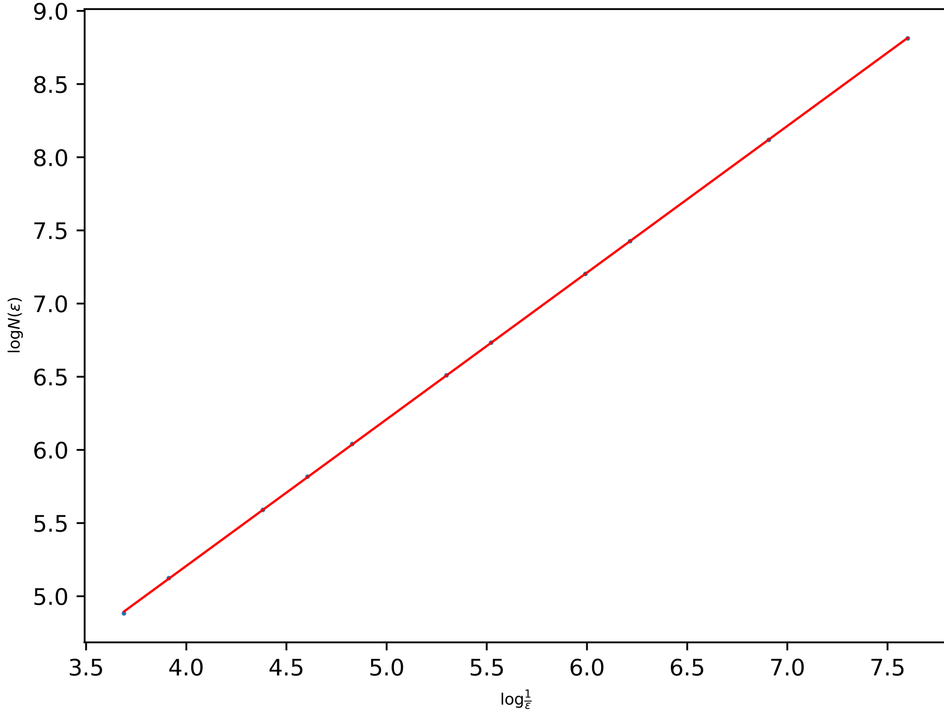
Power-Law of the BC-Dimension of the Quadratic Snowflake ( a = 0.2 , Level 2): 1.002161059550657
