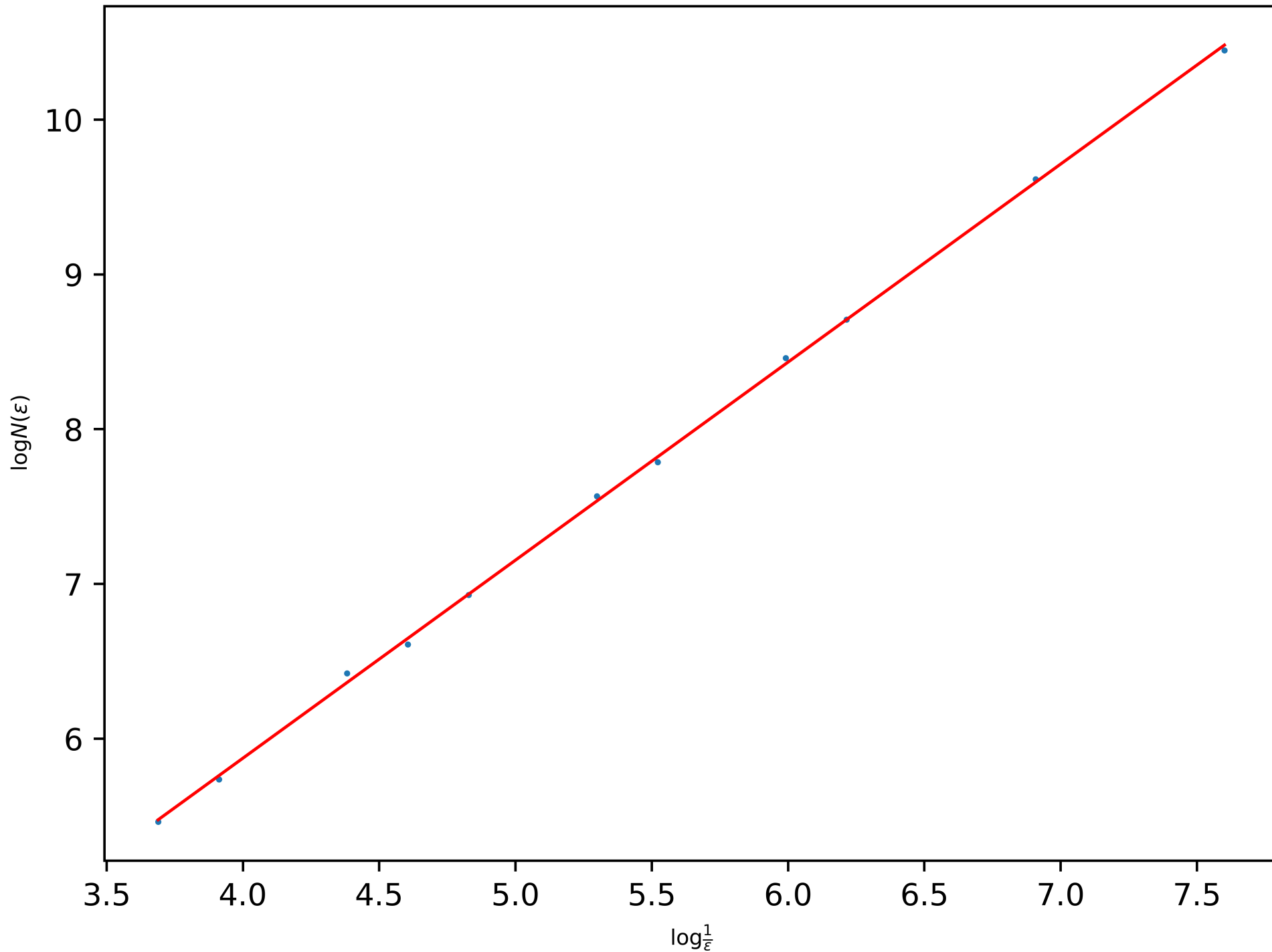
Power-Law of the BC-Dimension of the Quadratic Snowflake ( a = 0.2 , Level 8): 1.279675273855426
