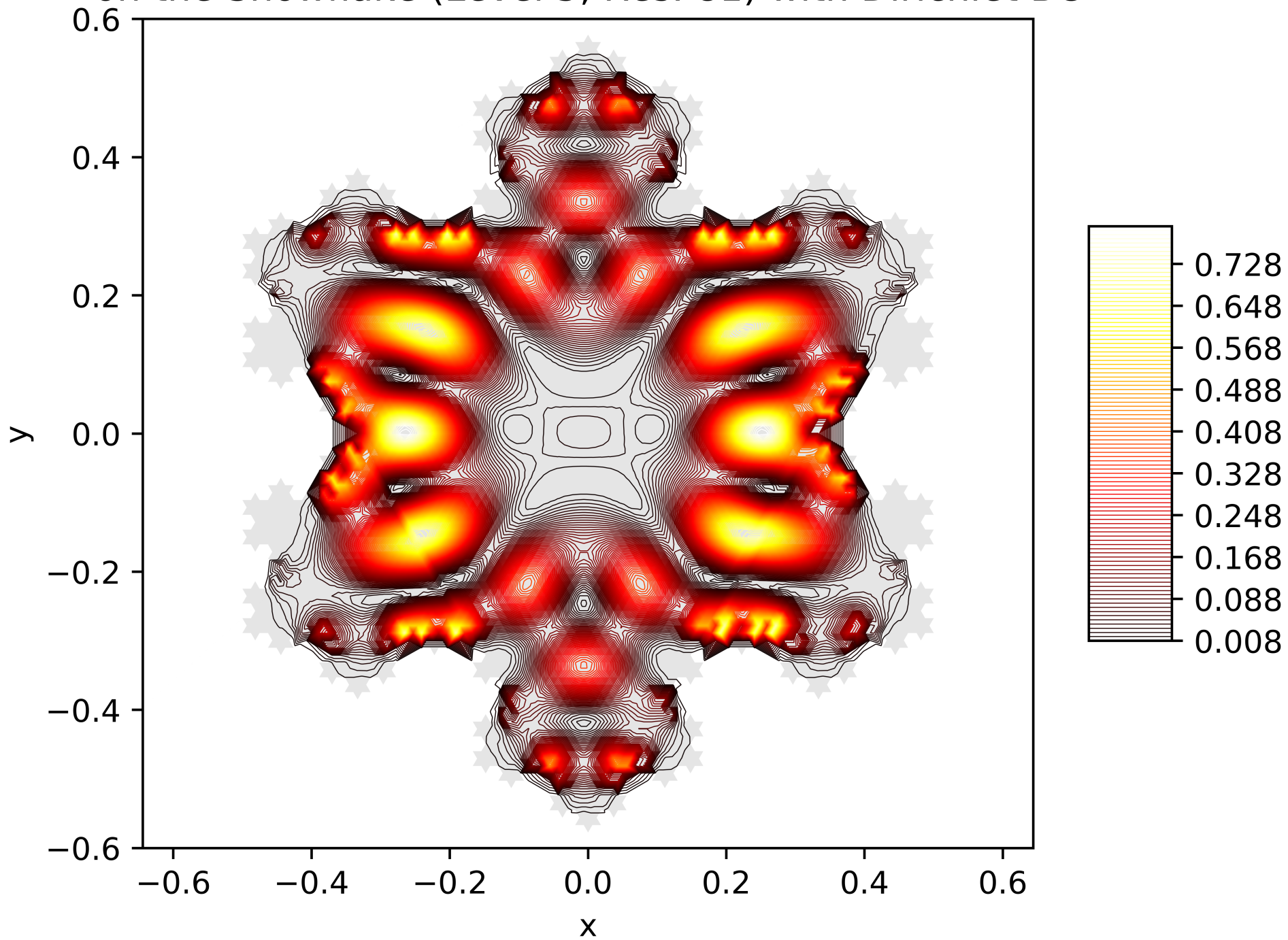
Contour Lines of the Energy Function of the 20. Eigenfunction on the Snowflake (Level 5, Res. 81) with Dirichlet BC
