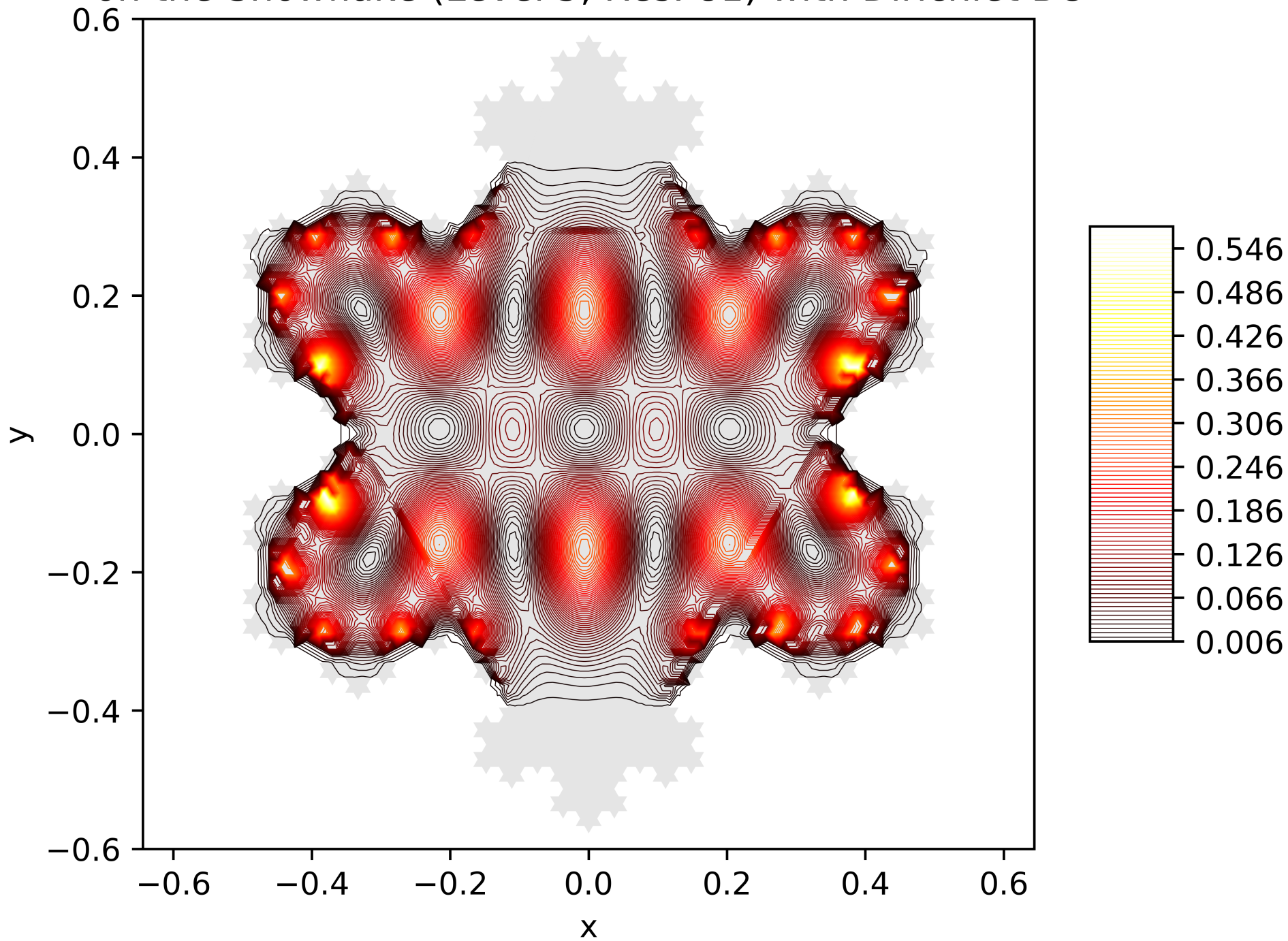
Contour Lines of the Energy Function of the 12. Eigenfunction on the Snowflake (Level 5, Res. 81) with Dirichlet BC
