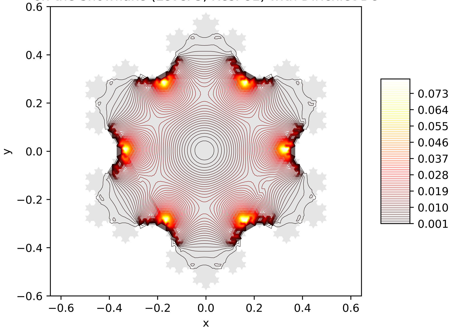
Contour Lines of the Energy Function of the 1. Eigenfunction on the Snowflake (Level 5, Res. 81) with Dirichlet BC
