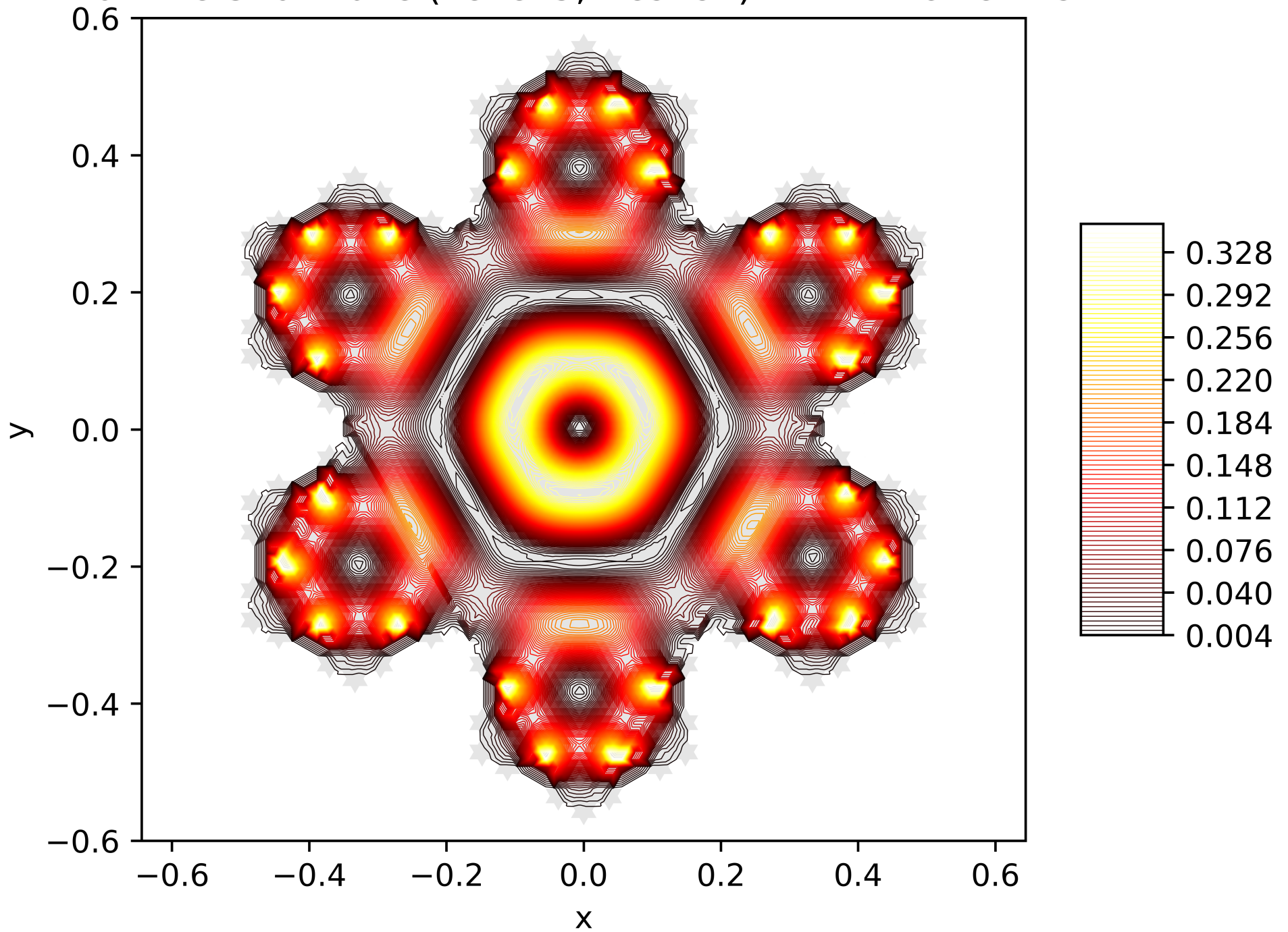
Contour Lines of the Energy Function of the 13. Eigenfunction on the Snowflake (Level 5, Res. 81) with Dirichlet BC
