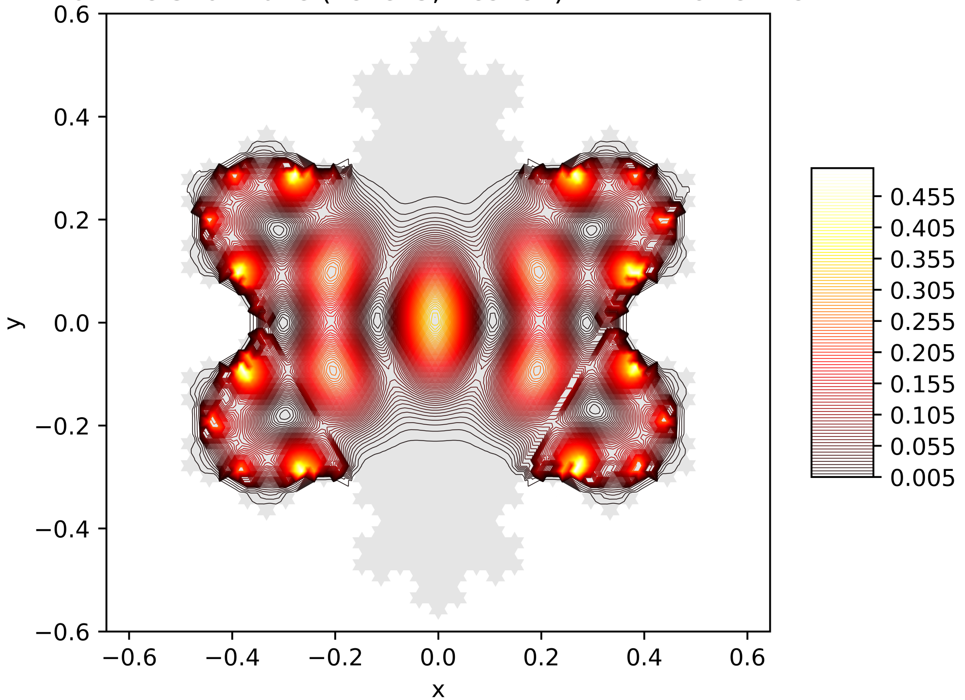
Contour Lines of the Energy Function of the 9. Eigenfunction on the Snowflake (Level 5, Res. 81) with Dirichlet BC
