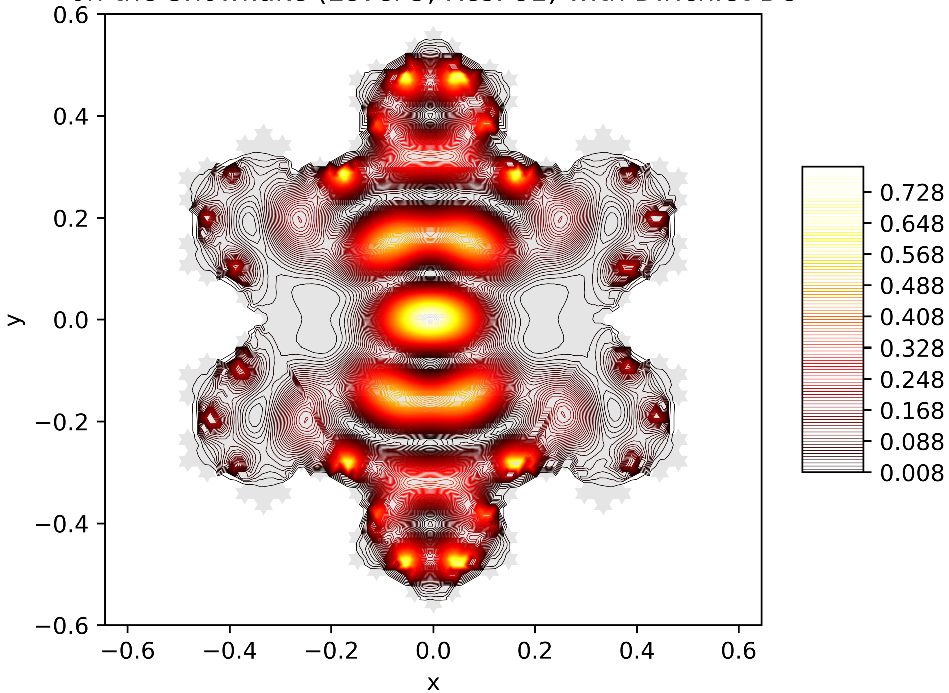
Contour Lines of the Energy Function of the 15. Eigenfunction on the Snowflake (Level 5, Res. 81) with Dirichlet BC
