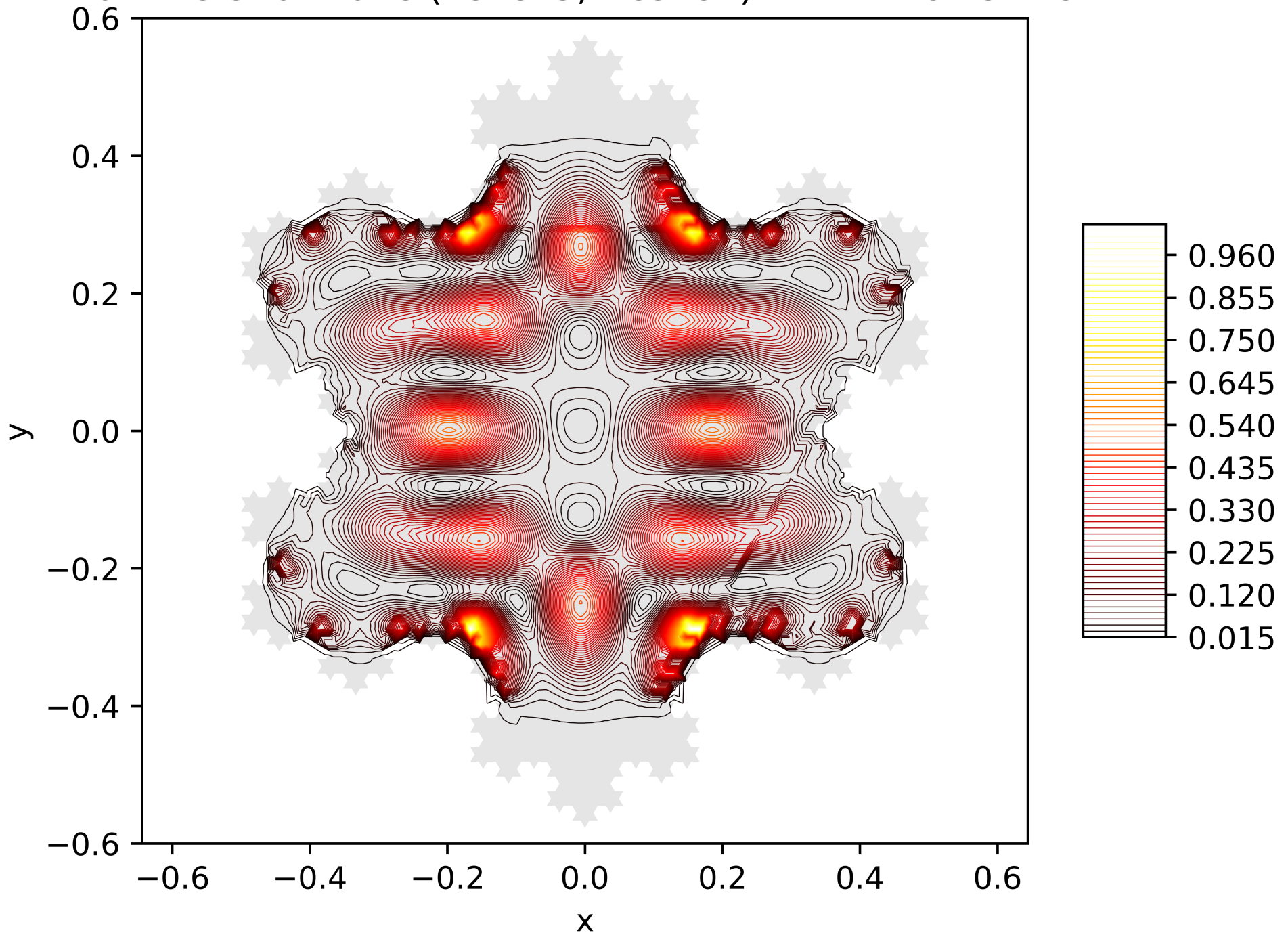
Contour Lines of the Energy Function of the 17. Eigenfunction on the Snowflake (Level 5, Res. 81) with Dirichlet BC
