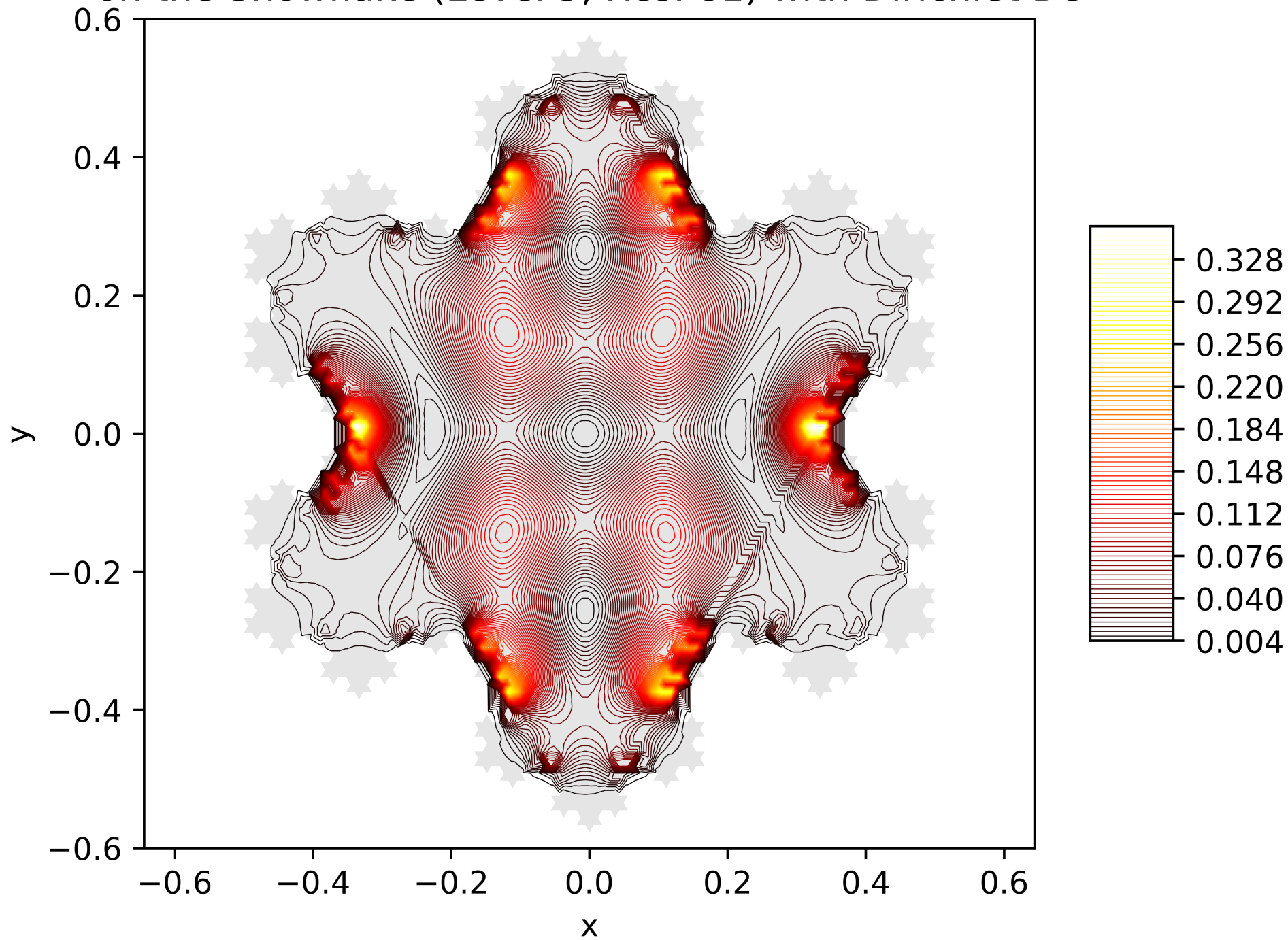
Contour Lines of the Energy Function of the 4. Eigenfunction on the Snowflake (Level 5, Res. 81) with Dirichlet BC
