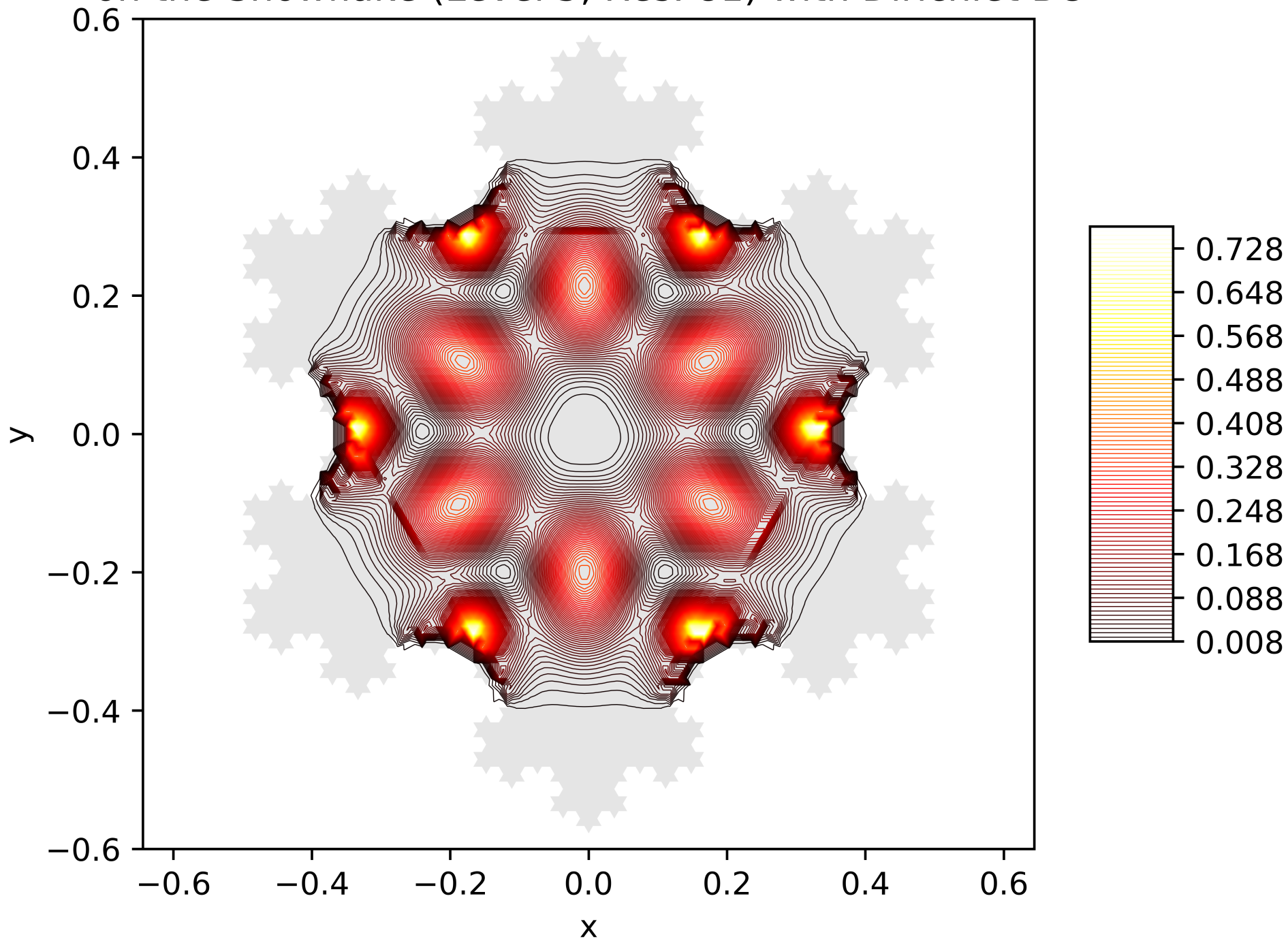
Contour Lines of the Energy Function of the 10. Eigenfunction on the Snowflake (Level 5, Res. 81) with Dirichlet BC
