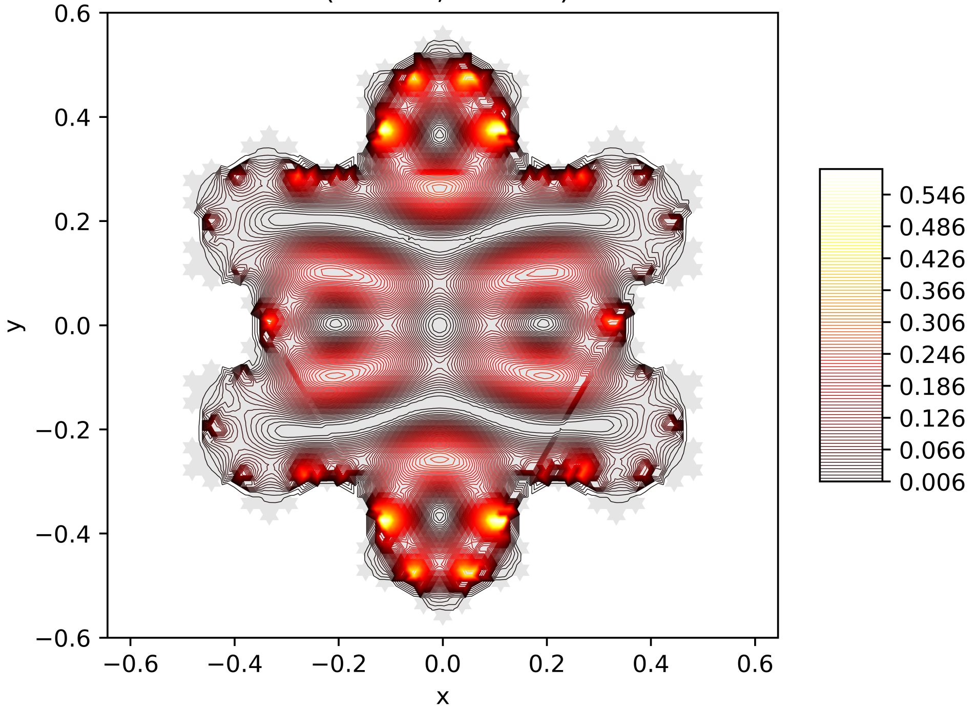
Contour Lines of the Energy Function of the 11. Eigenfunction on the Snowflake (Level 5, Res. 81) with Dirichlet BC
