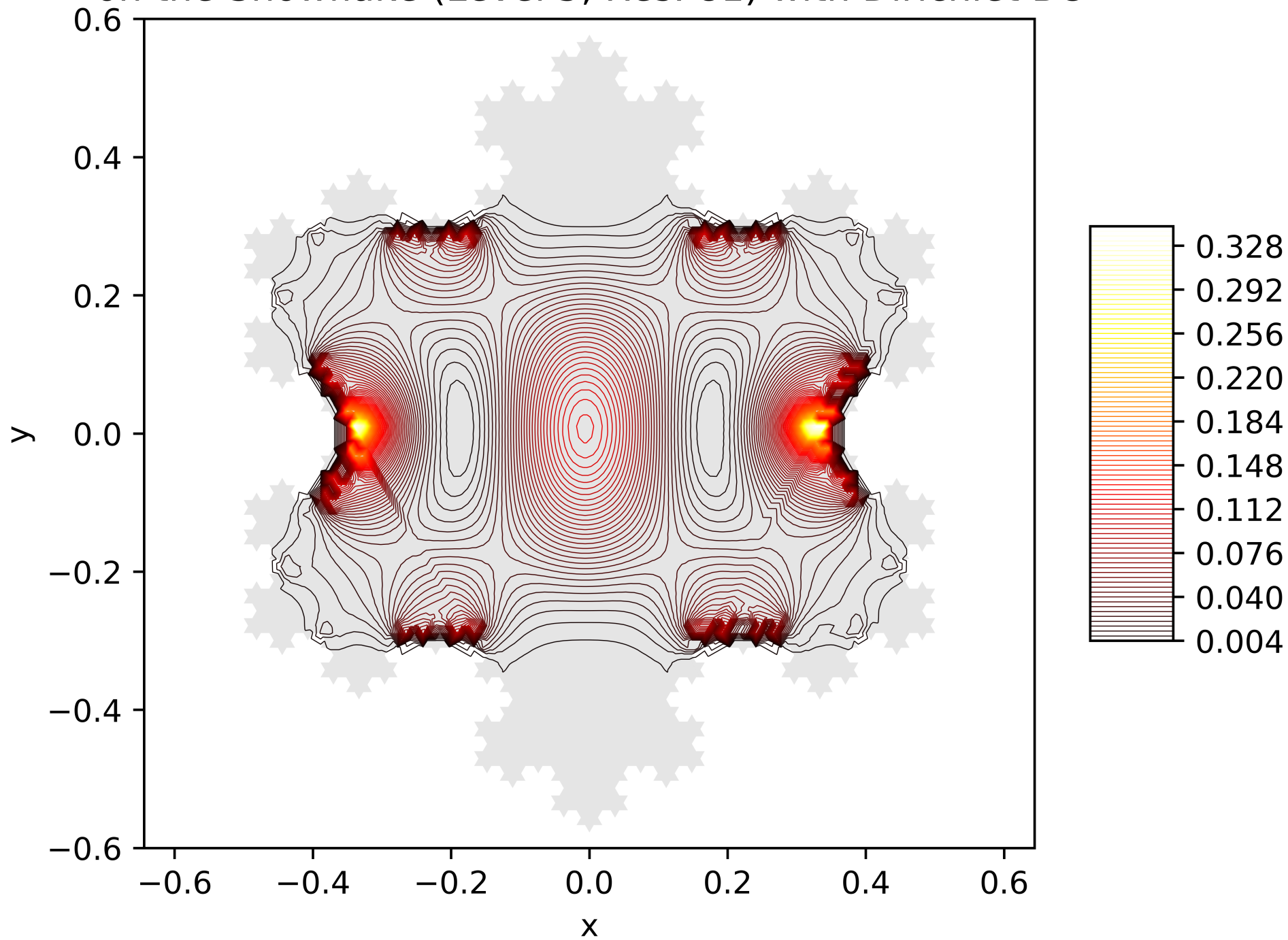
Contour Lines of the Energy Function of the 3. Eigenfunction on the Snowflake (Level 5, Res. 81) with Dirichlet BC
