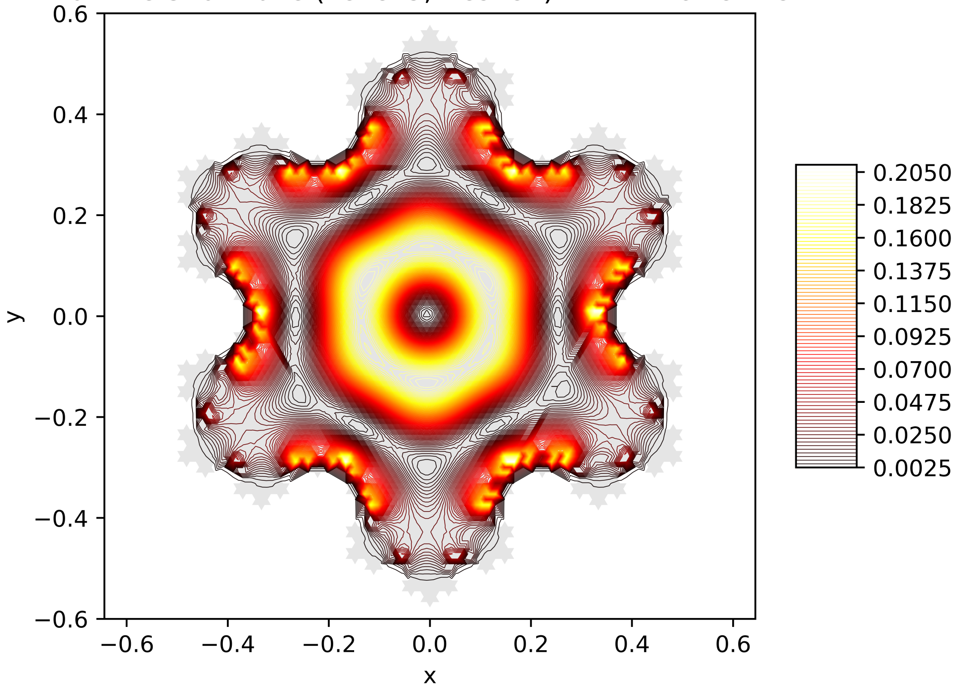
Contour Lines of the Energy Function of the 6. Eigenfunction on the Snowflake (Level 5, Res. 81) with Dirichlet BC
