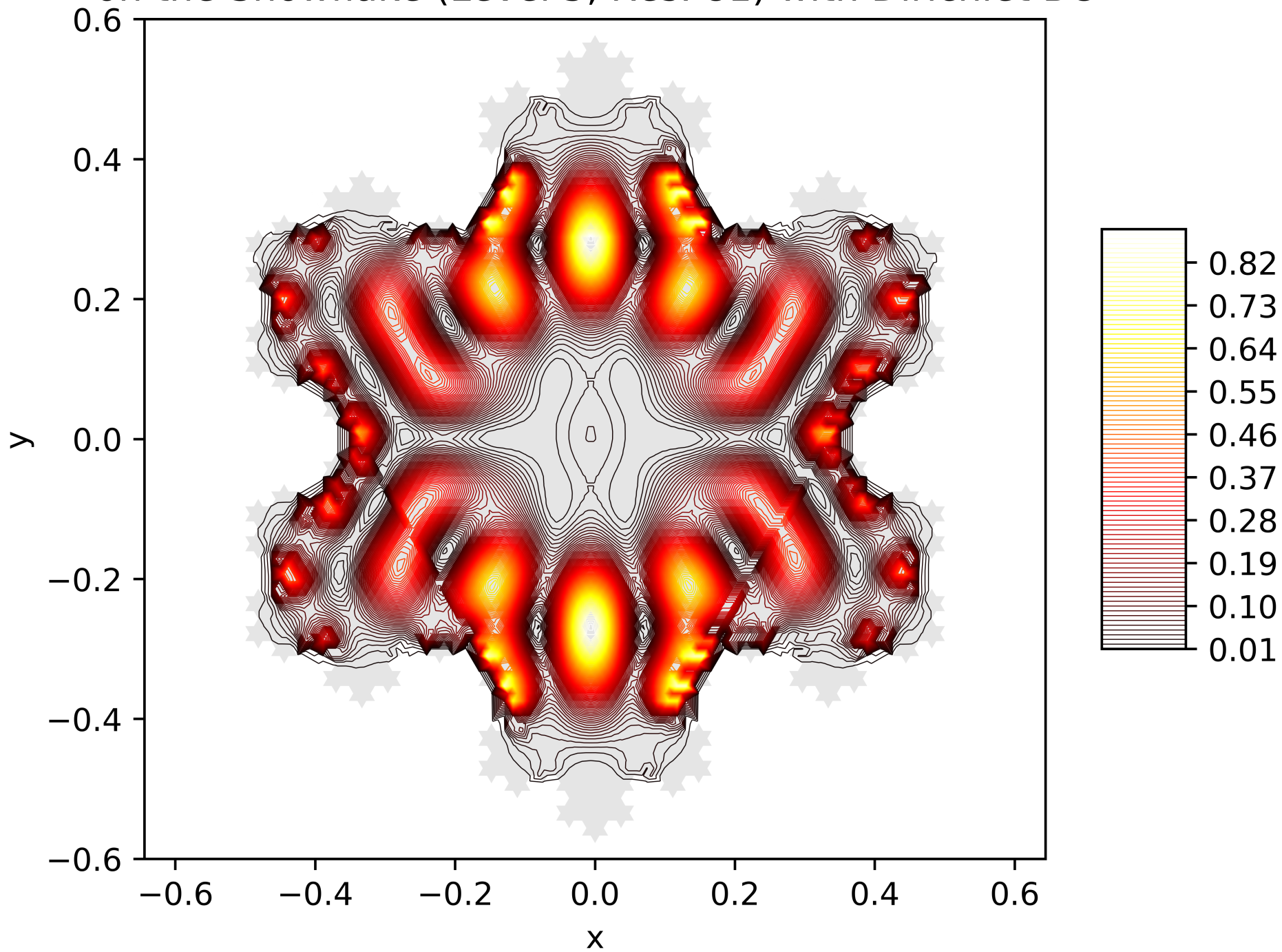
Contour Lines of the Energy Function of the 19. Eigenfunction on the Snowflake (Level 5, Res. 81) with Dirichlet BC
