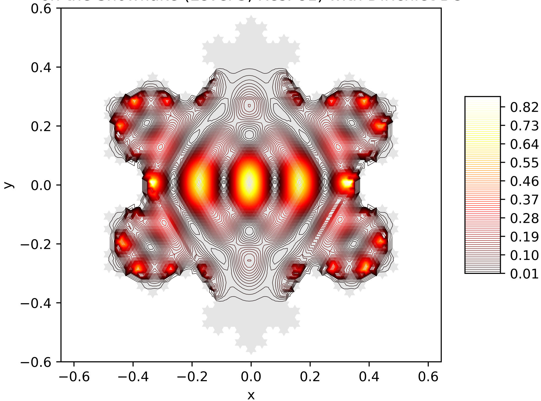
Contour Lines of the Energy Function of the 16. Eigenfunction on the Snowflake (Level 5, Res. 81) with Dirichlet BC
