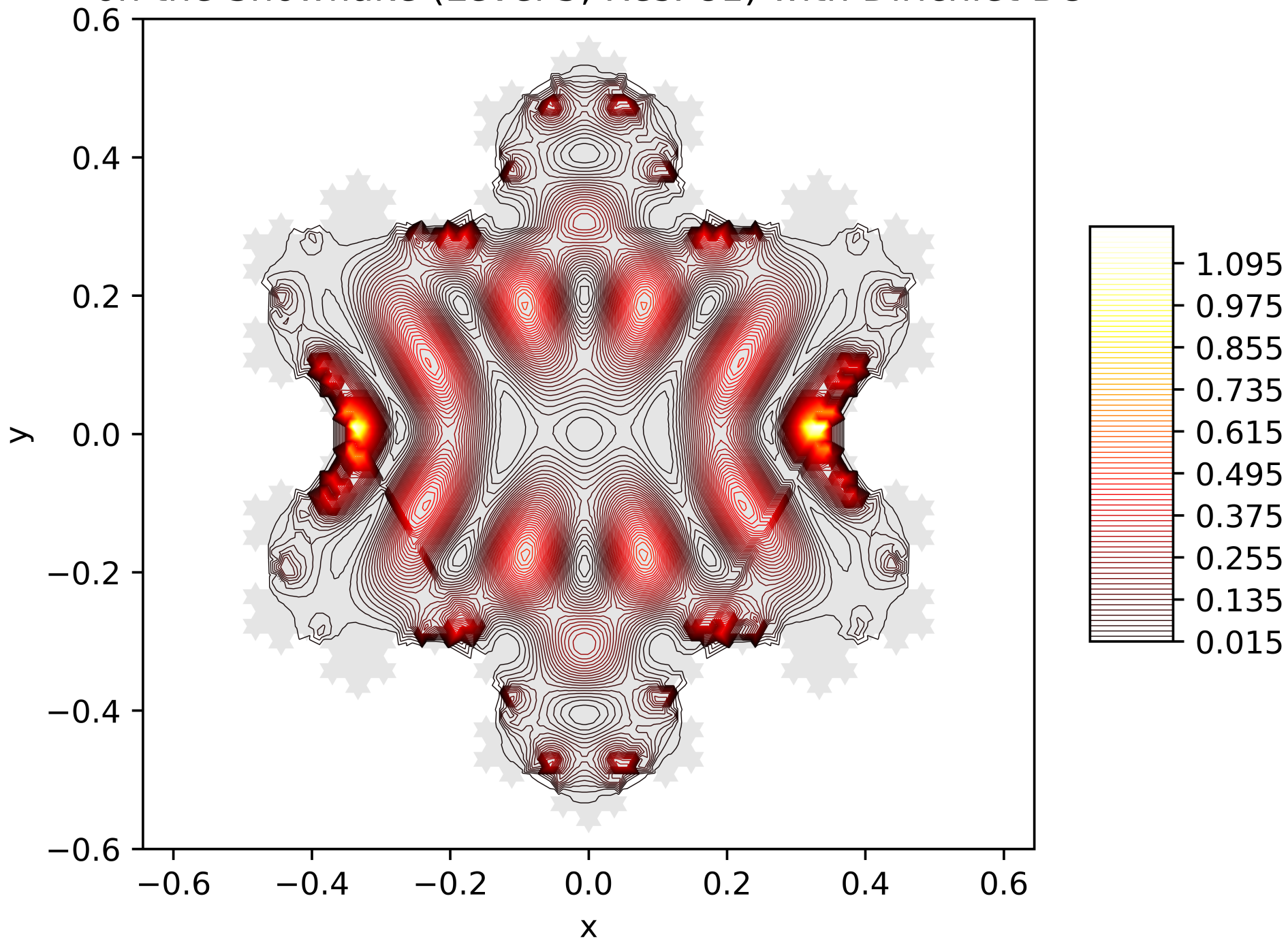
Contour Lines of the Energy Function of the 18. Eigenfunction on the Snowflake (Level 5, Res. 81) with Dirichlet BC
