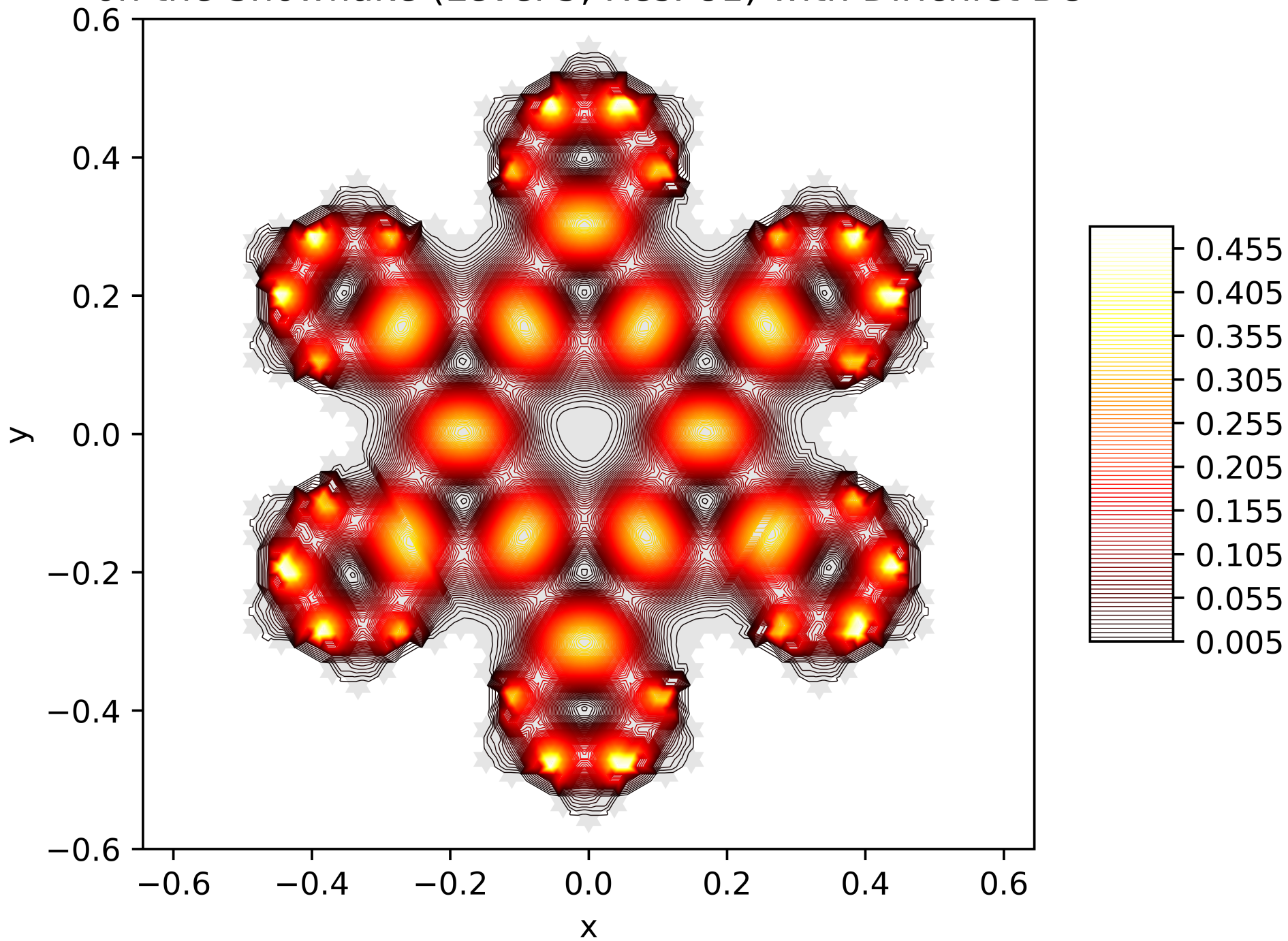
Contour Lines of the Energy Function of the 14. Eigenfunction on the Snowflake (Level 5, Res. 81) with Dirichlet BC
