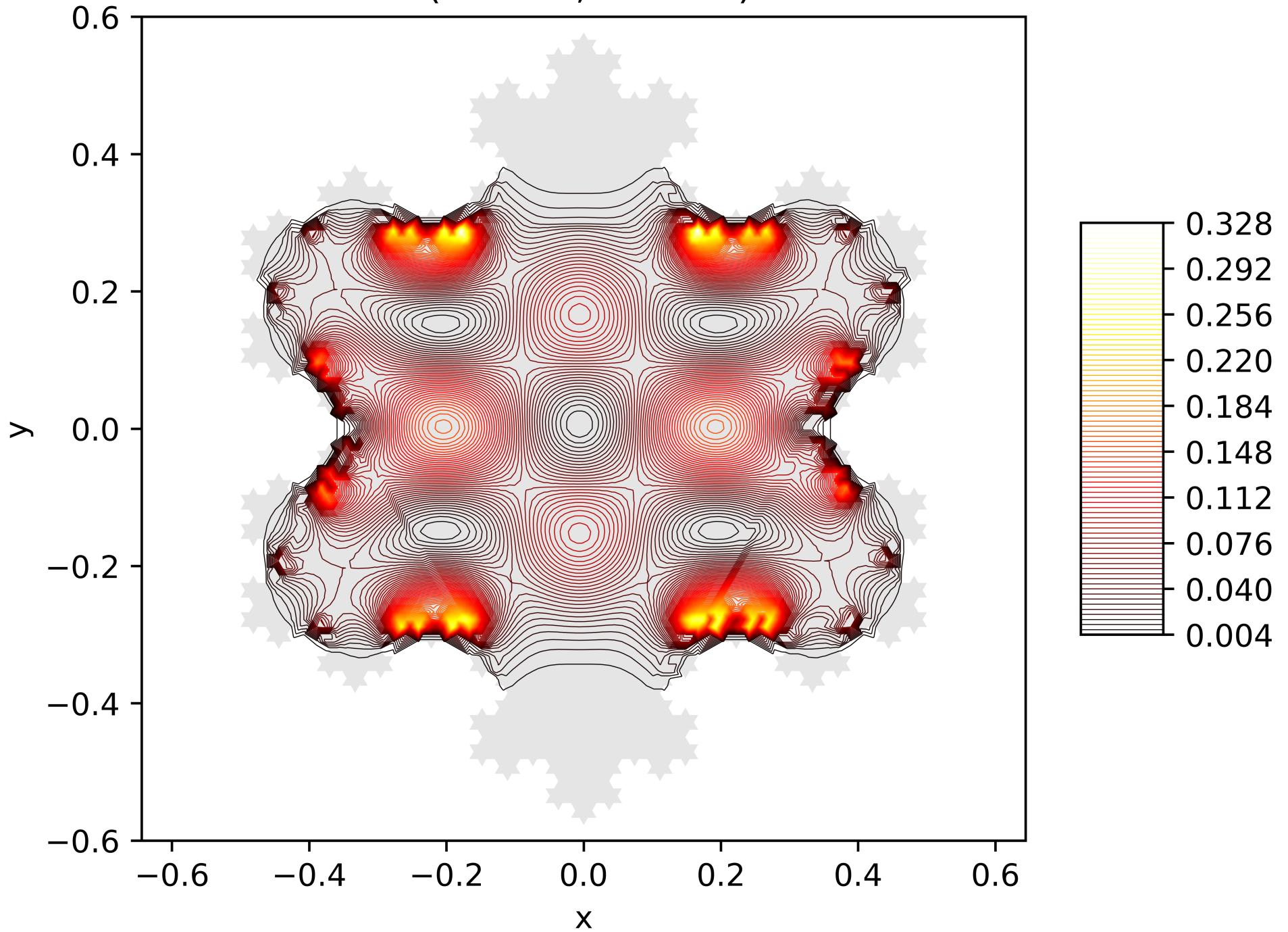
Contour Lines of the Energy Function of the 5. Eigenfunction on the Snowflake (Level 5, Res. 81) with Dirichlet BC
