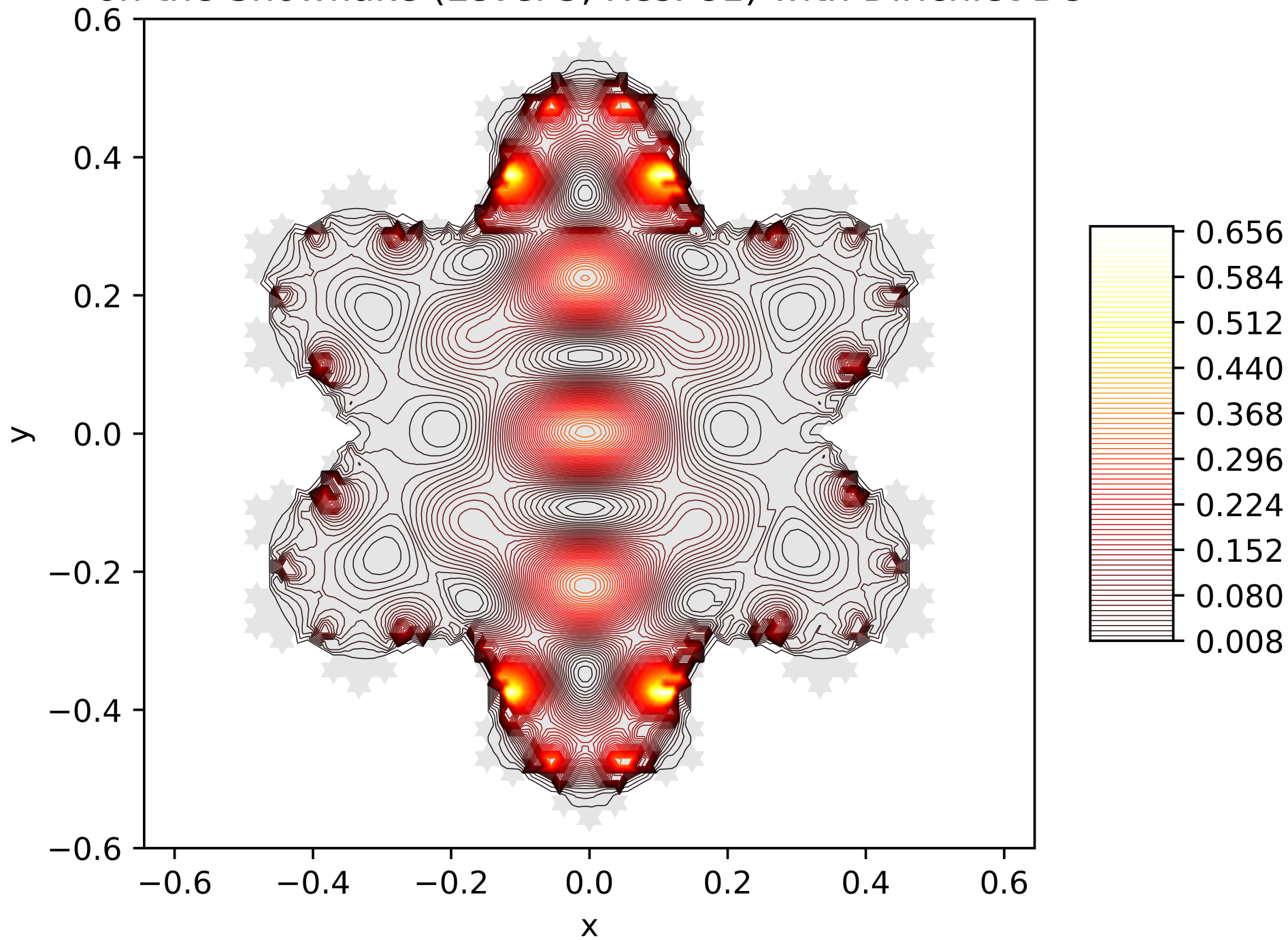
Contour Lines of the Energy Function of the 8. Eigenfunction on the Snowflake (Level 5, Res. 81) with Dirichlet BC
