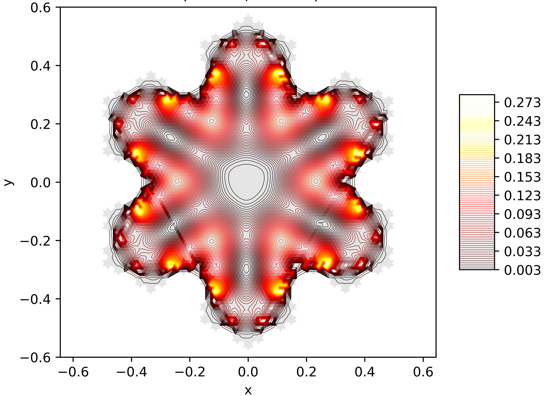
Contour Lines of the Energy Function of the 7. Eigenfunction on the Snowflake (Level 5, Res. 81) with Dirichlet BC
