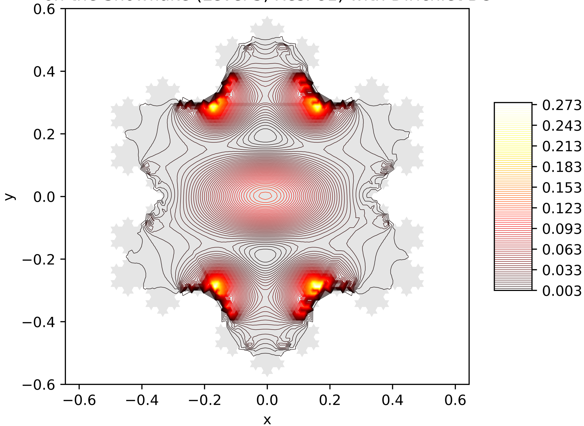
Contour Lines of the Energy Function of the 2. Eigenfunction on the Snowflake (Level 5, Res. 81) with Dirichlet BC
