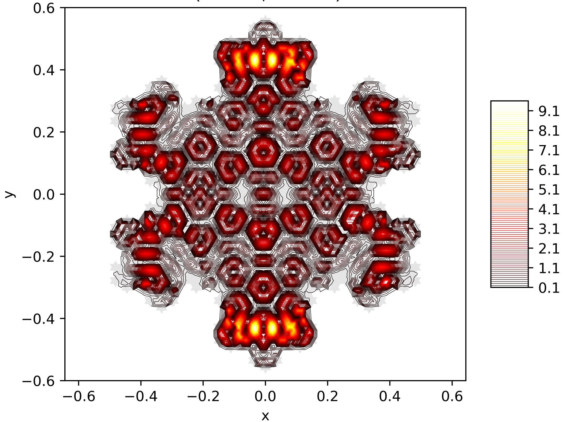
Contour Lines of the Energy Function of the 185. Eigenfunction on the Snowflake (Level 5, Res. 81) with Dirichlet BC
