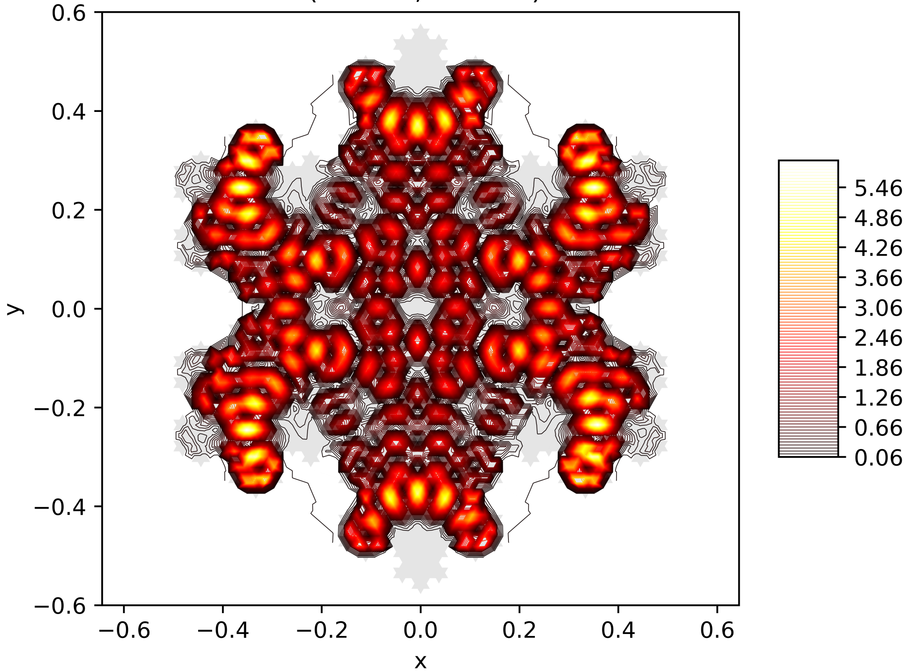
Contour Lines of the Energy Function of the 183. Eigenfunction on the Snowflake (Level 5, Res. 81) with Dirichlet BC
