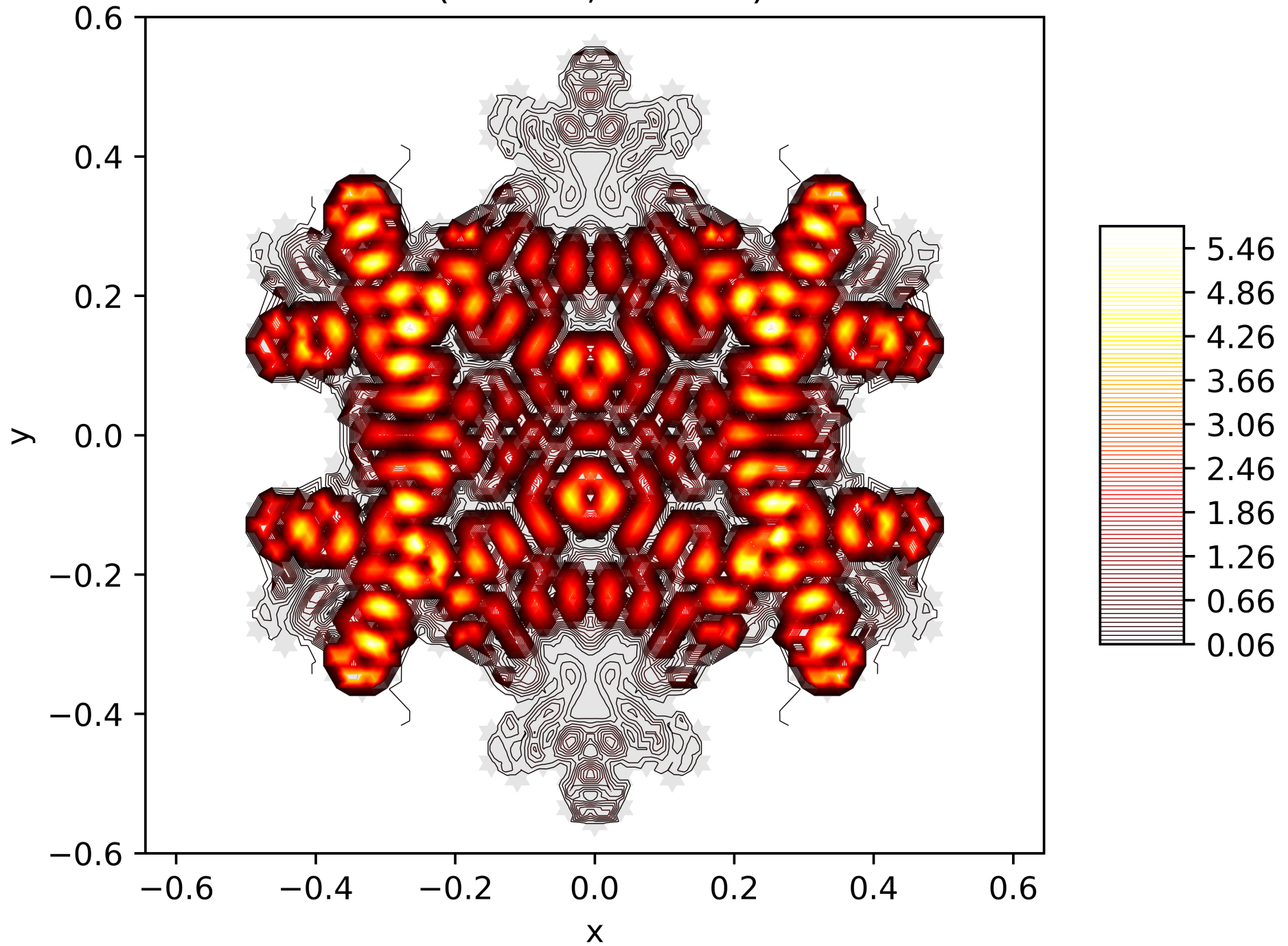
Contour Lines of the Energy Function of the 194. Eigenfunction on the Snowflake (Level 5, Res. 81) with Dirichlet BC
