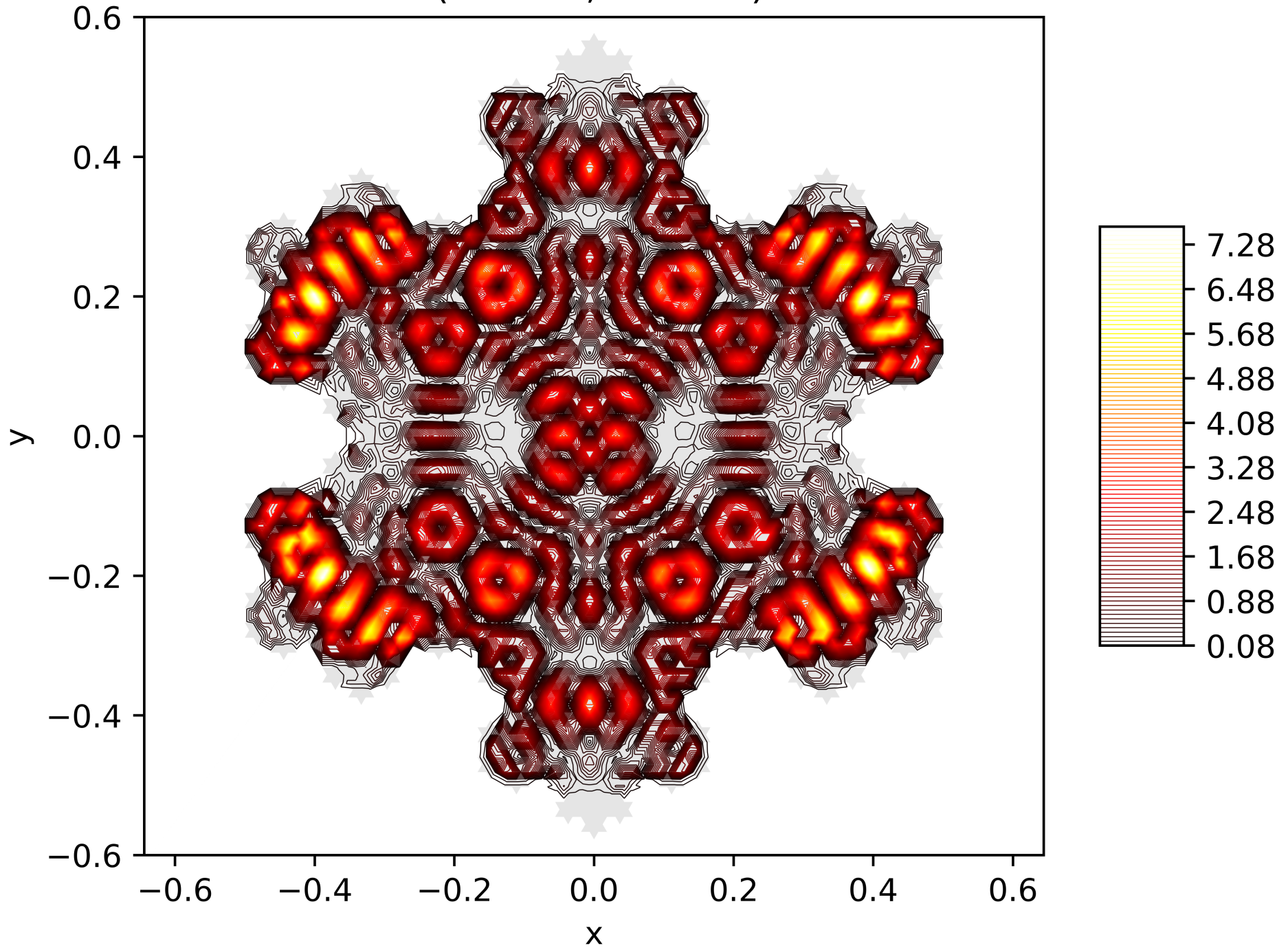
Contour Lines of the Energy Function of the 192. Eigenfunction on the Snowflake (Level 5, Res. 81) with Dirichlet BC
