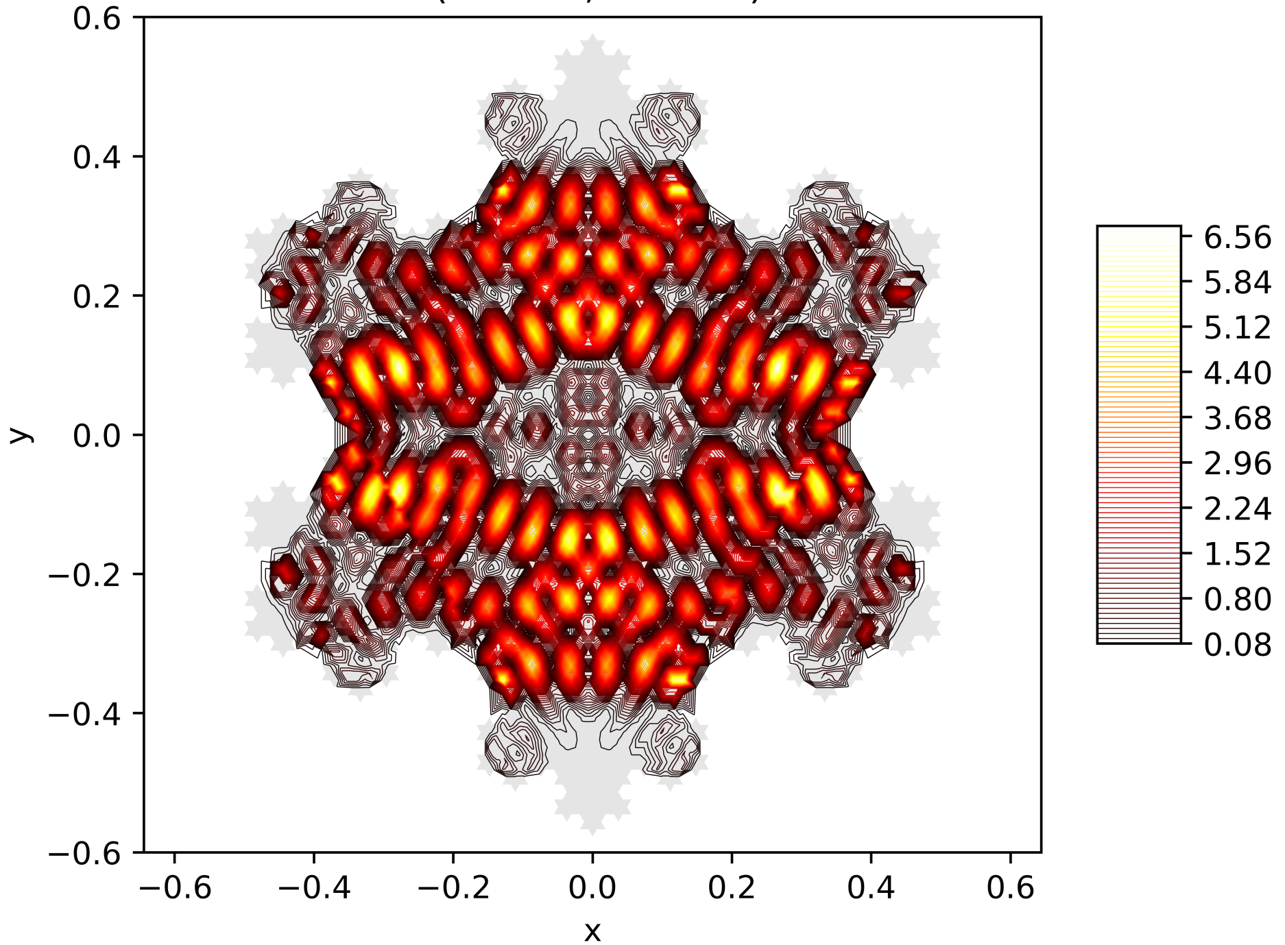
Contour Lines of the Energy Function of the 196. Eigenfunction on the Snowflake (Level 5, Res. 81) with Dirichlet BC
