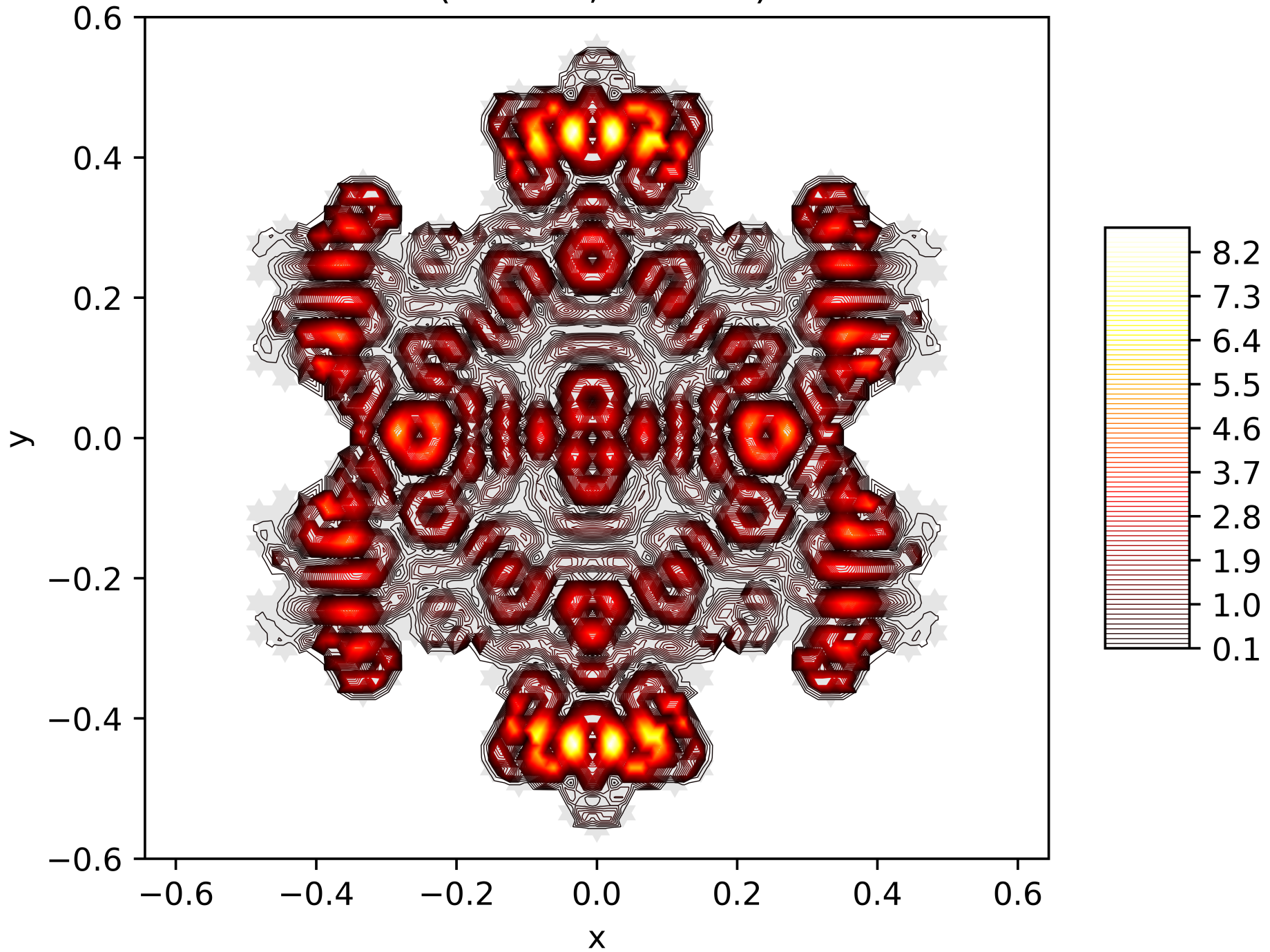
Contour Lines of the Energy Function of the 191. Eigenfunction on the Snowflake (Level 5, Res. 81) with Dirichlet BC
