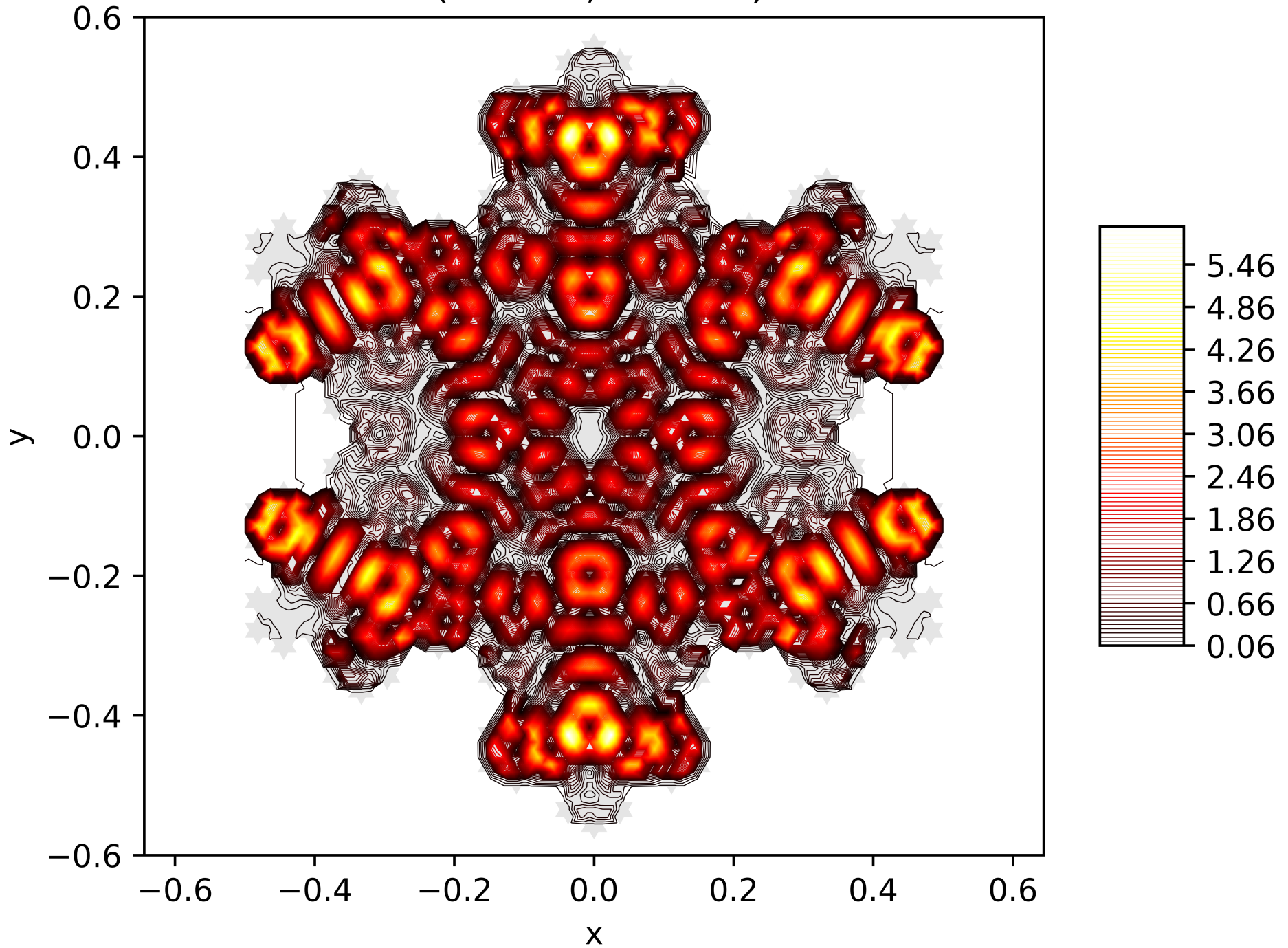
Contour Lines of the Energy Function of the 184. Eigenfunction on the Snowflake (Level 5, Res. 81) with Dirichlet BC
