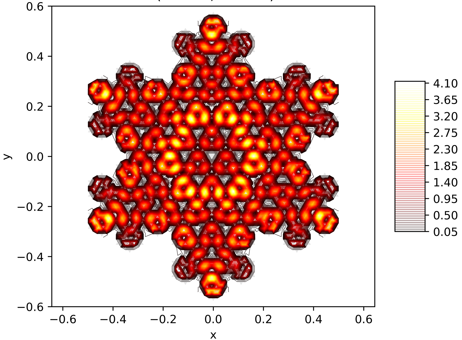
Contour Lines of the Energy Function of the 188. Eigenfunction on the Snowflake (Level 5, Res. 81) with Dirichlet BC
