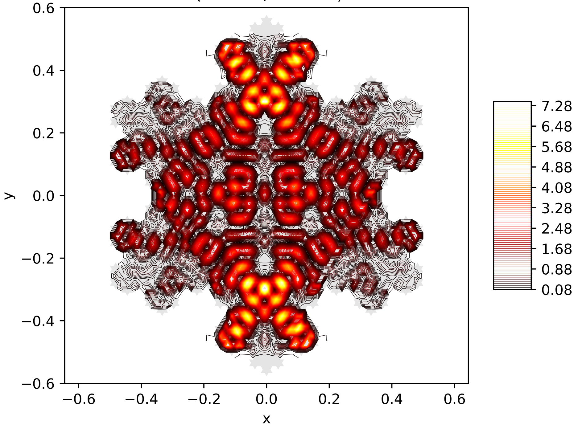
Contour Lines of the Energy Function of the 193. Eigenfunction on the Snowflake (Level 5, Res. 81) with Dirichlet BC
