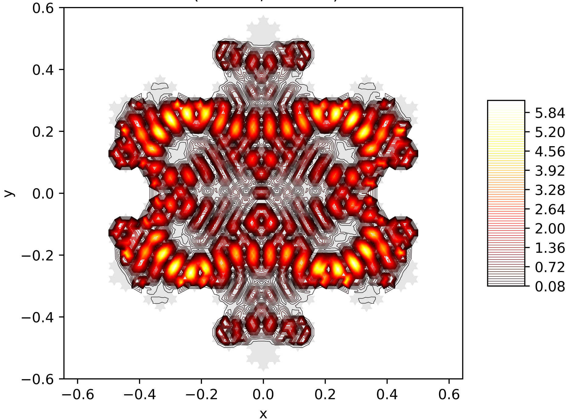
Contour Lines of the Energy Function of the 181. Eigenfunction on the Snowflake (Level 5, Res. 81) with Dirichlet BC
