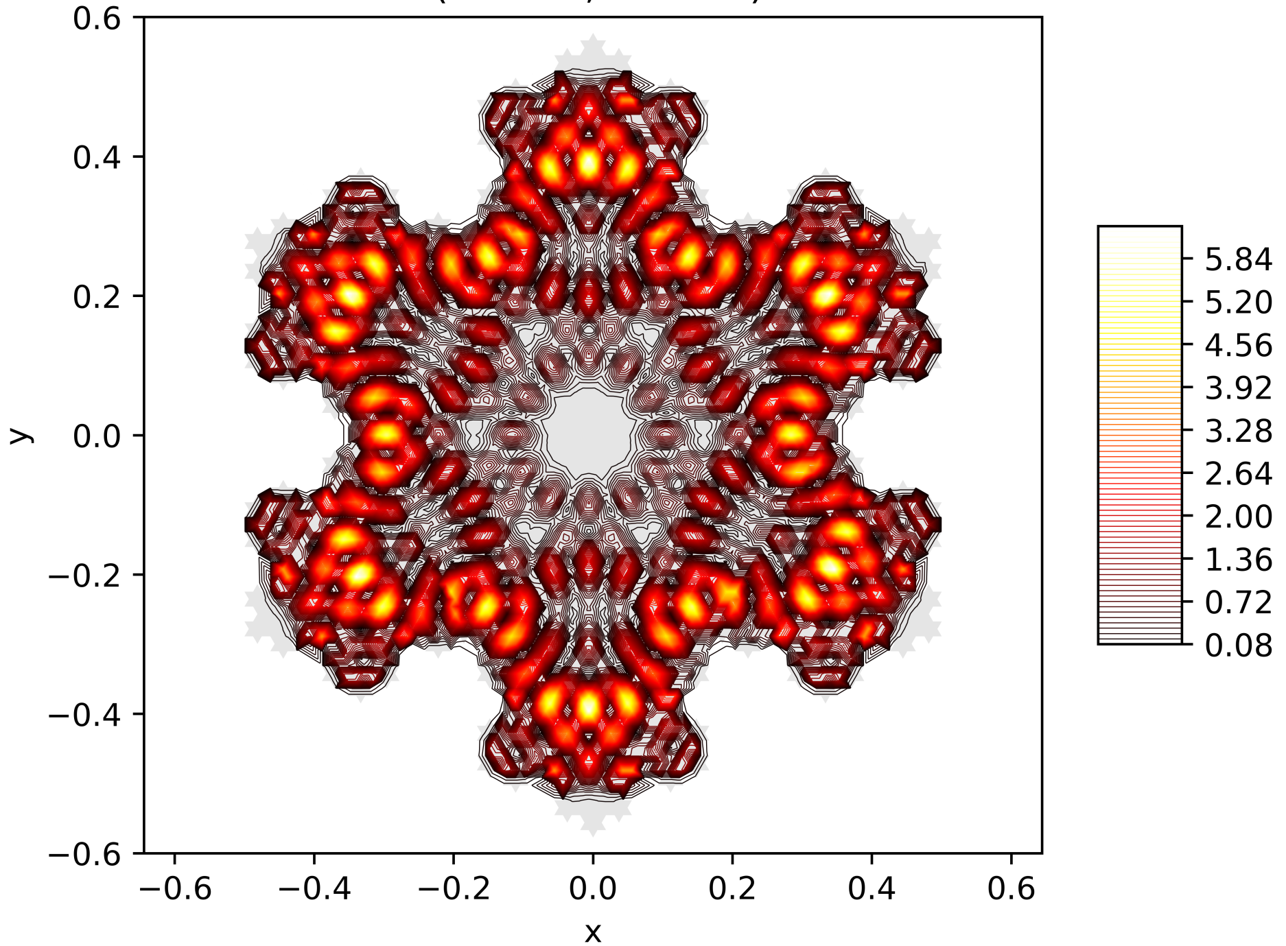
Contour Lines of the Energy Function of the 197. Eigenfunction on the Snowflake (Level 5, Res. 81) with Dirichlet BC
