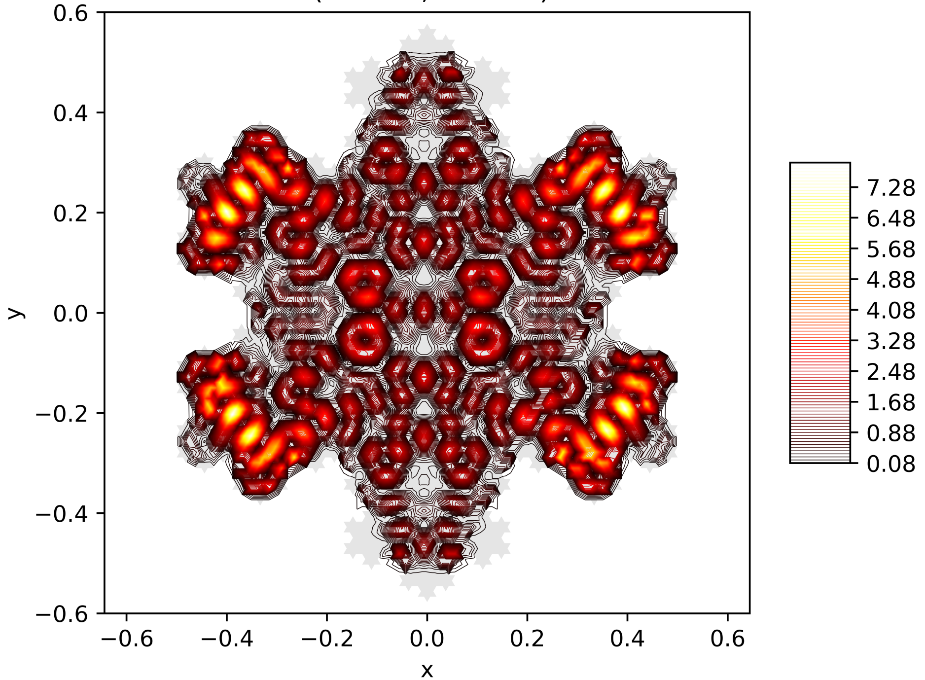
Contour Lines of the Energy Function of the 186. Eigenfunction on the Snowflake (Level 5, Res. 81) with Dirichlet BC
