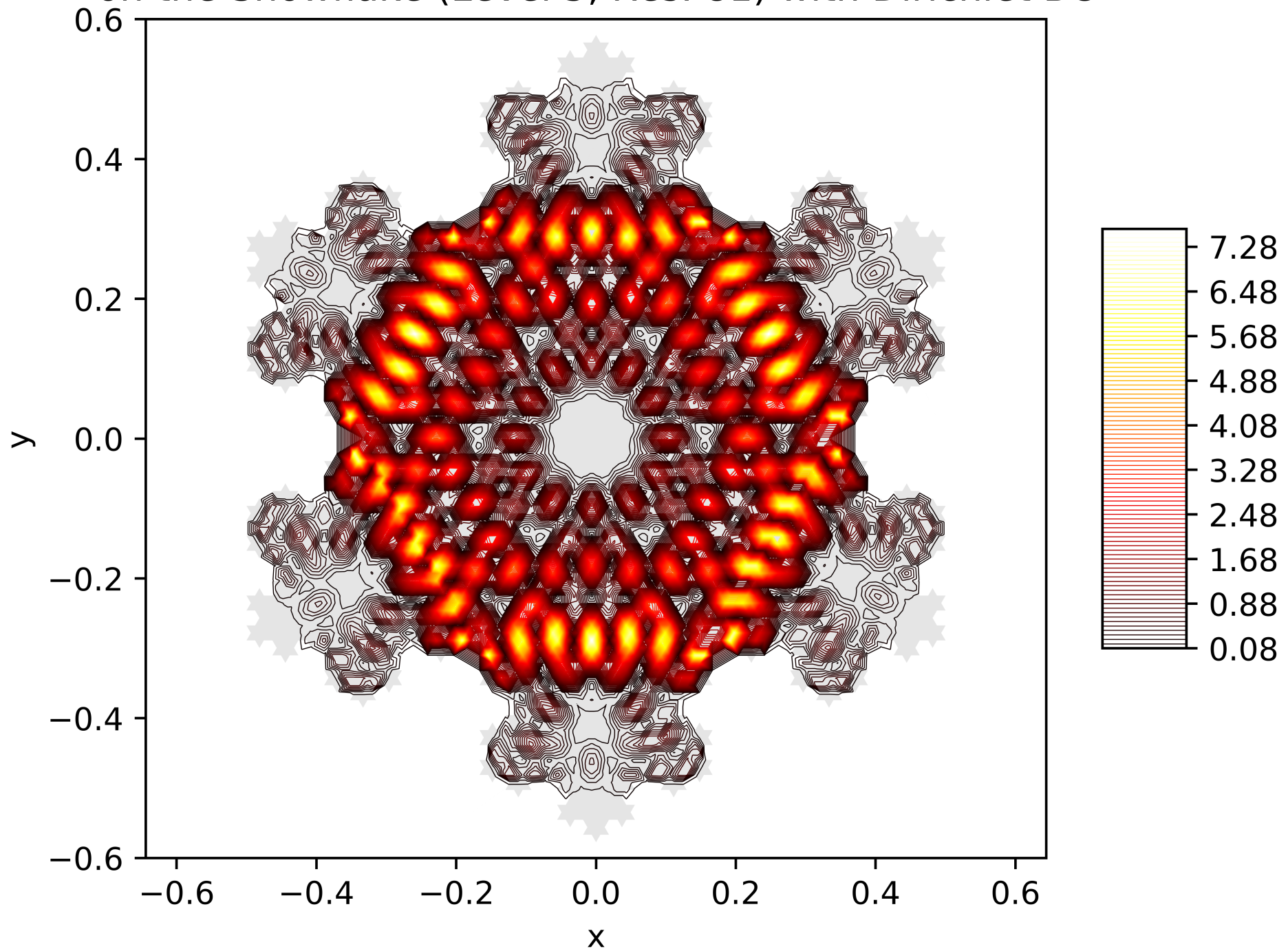
Contour Lines of the Energy Function of the 200. Eigenfunction on the Snowflake (Level 5, Res. 81) with Dirichlet BC
