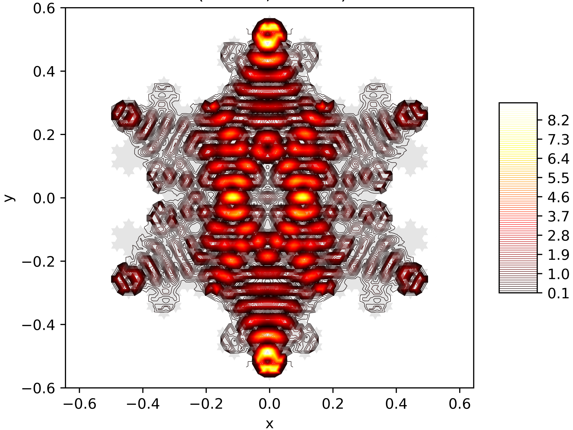
Contour Lines of the Energy Function of the 189. Eigenfunction on the Snowflake (Level 5, Res. 81) with Dirichlet BC
