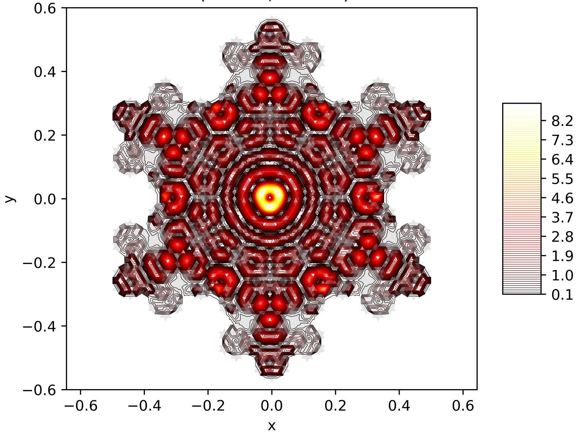
Contour Lines of the Energy Function of the 182. Eigenfunction on the Snowflake (Level 5, Res. 81) with Dirichlet BC
