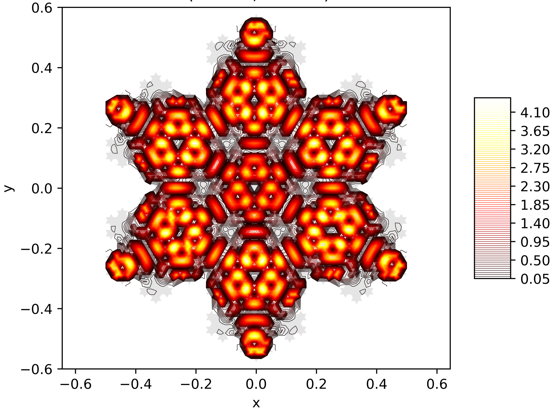
Contour Lines of the Energy Function of the 198. Eigenfunction on the Snowflake (Level 5, Res. 81) with Dirichlet BC
