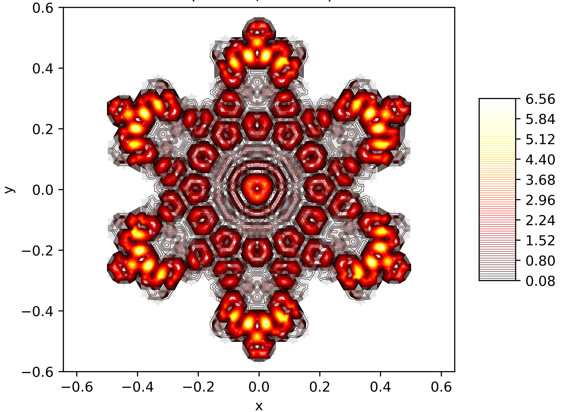
Contour Lines of the Energy Function of the 199. Eigenfunction on the Snowflake (Level 5, Res. 81) with Dirichlet BC
