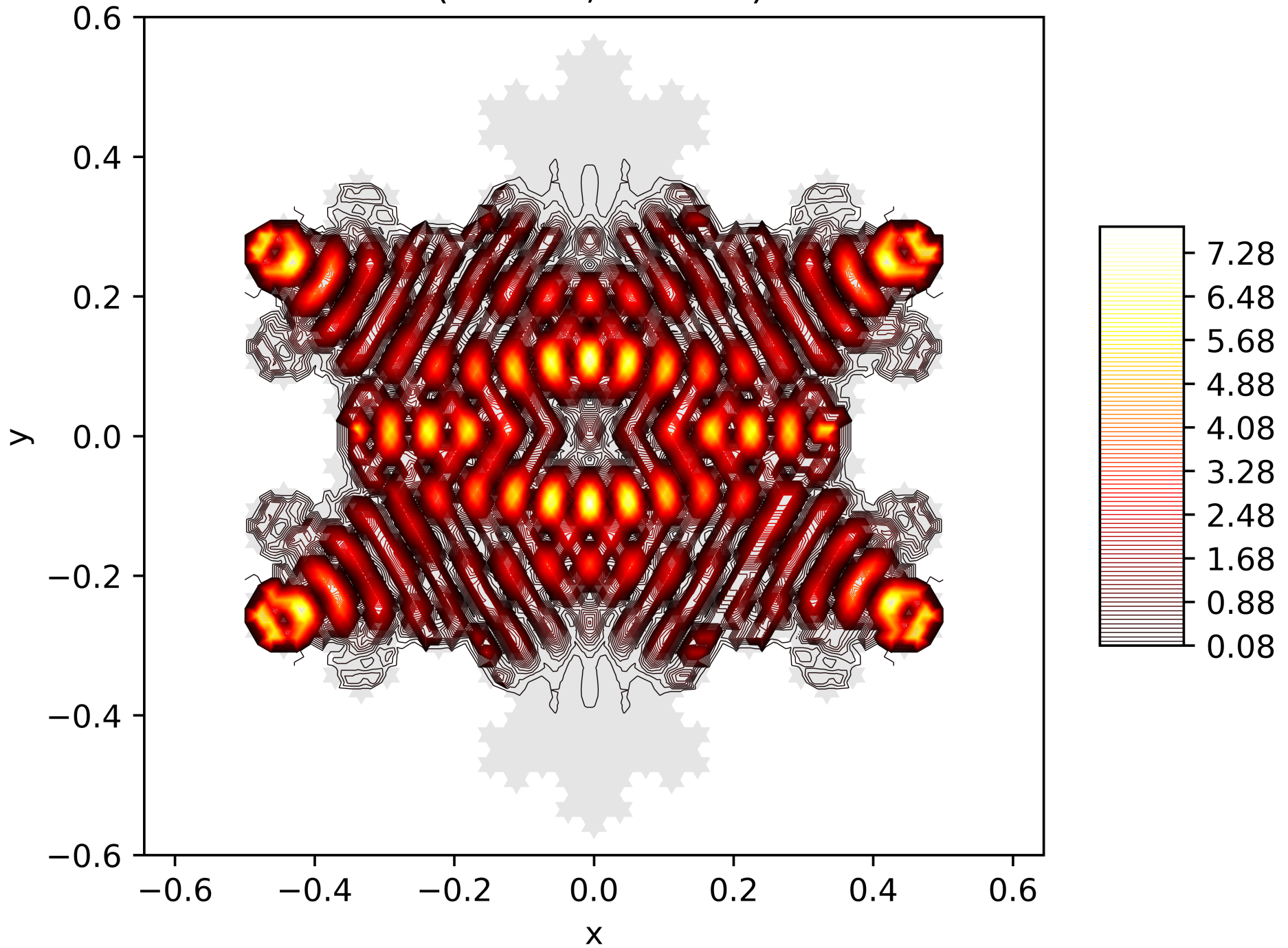
Contour Lines of the Energy Function of the 190. Eigenfunction on the Snowflake (Level 5, Res. 81) with Dirichlet BC
