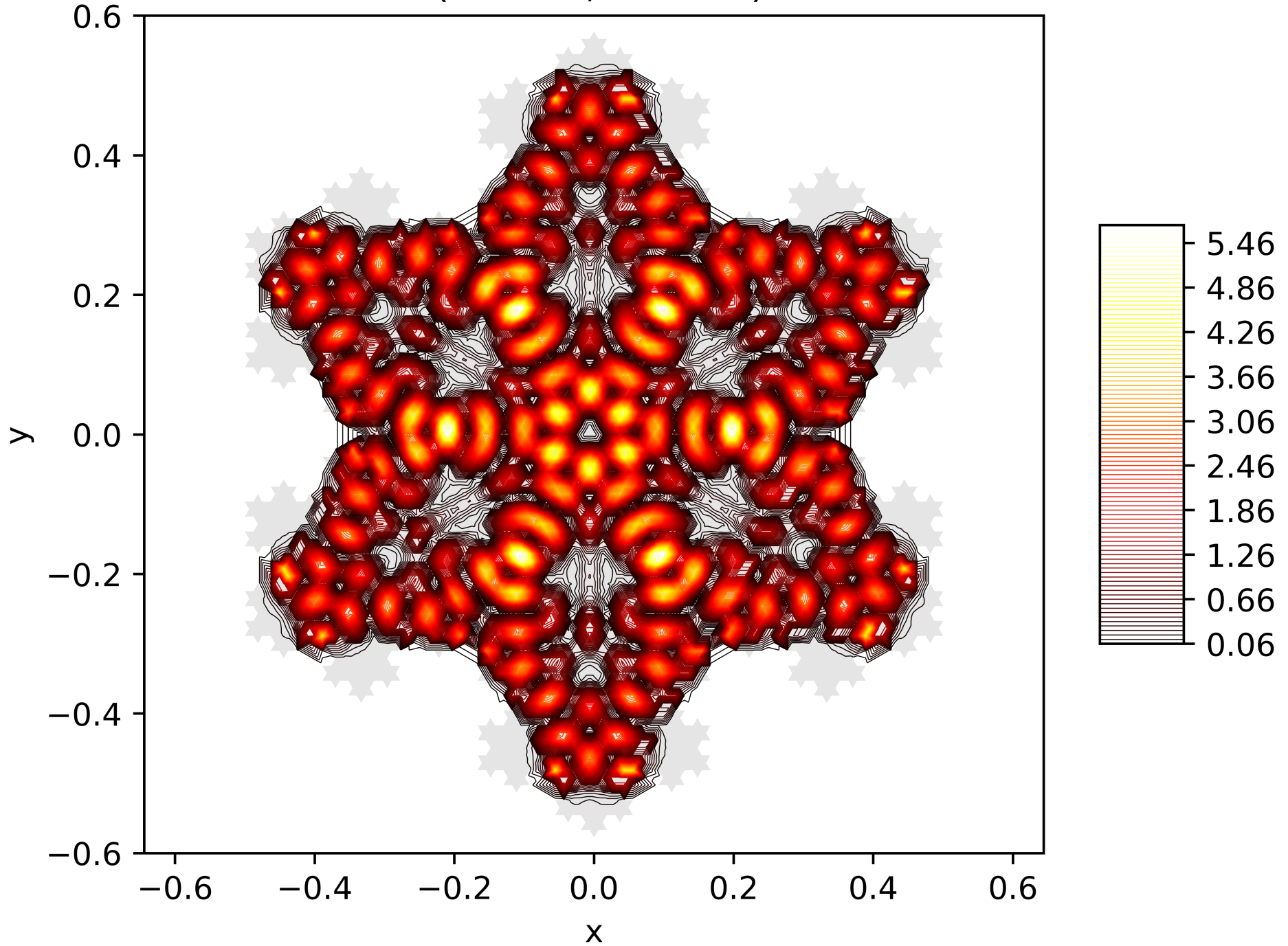
Contour Lines of the Energy Function of the 187. Eigenfunction on the Snowflake (Level 5, Res. 81) with Dirichlet BC
