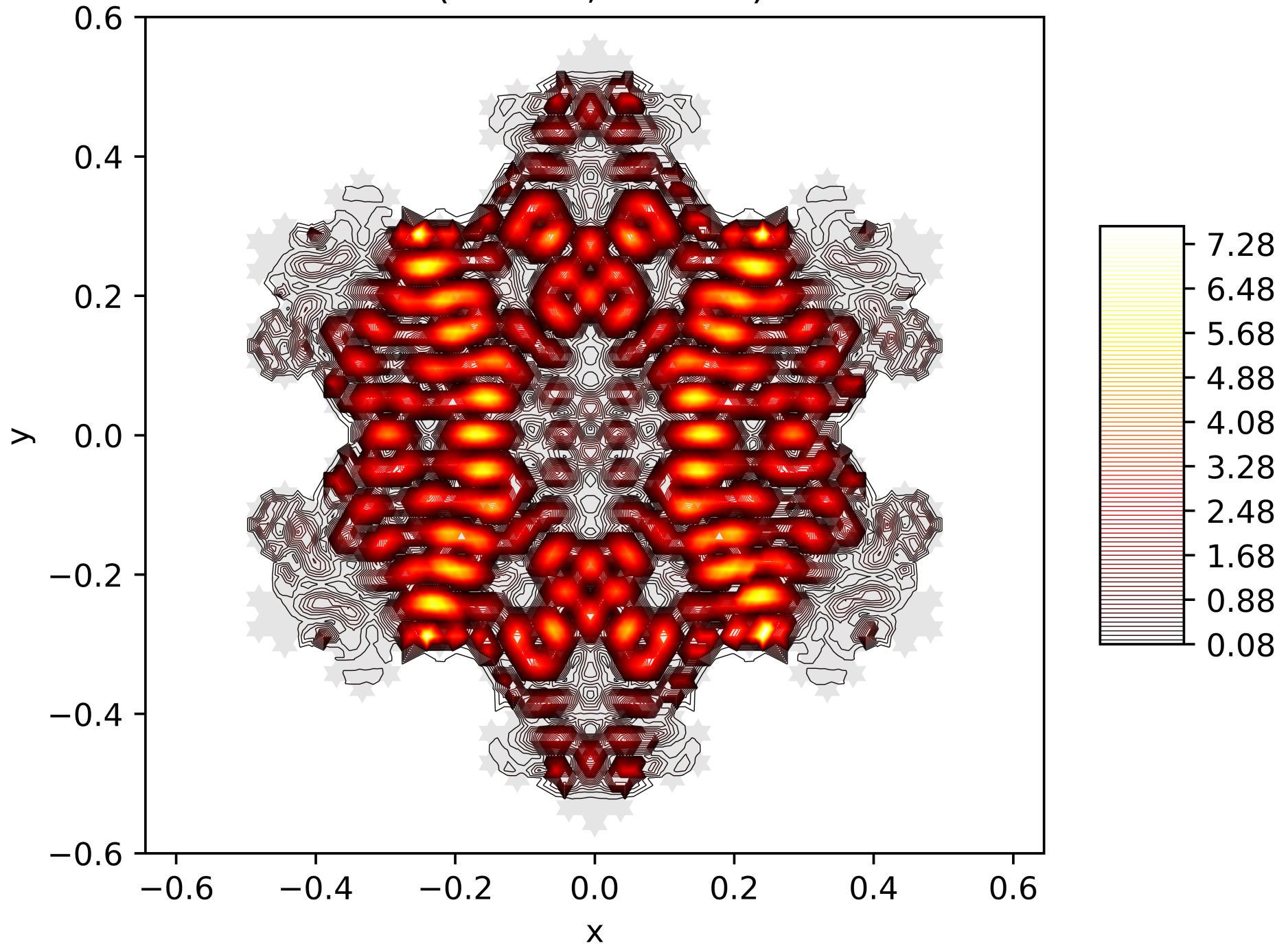
Contour Lines of the Energy Function of the 195. Eigenfunction on the Snowflake (Level 5, Res. 81) with Dirichlet BC
