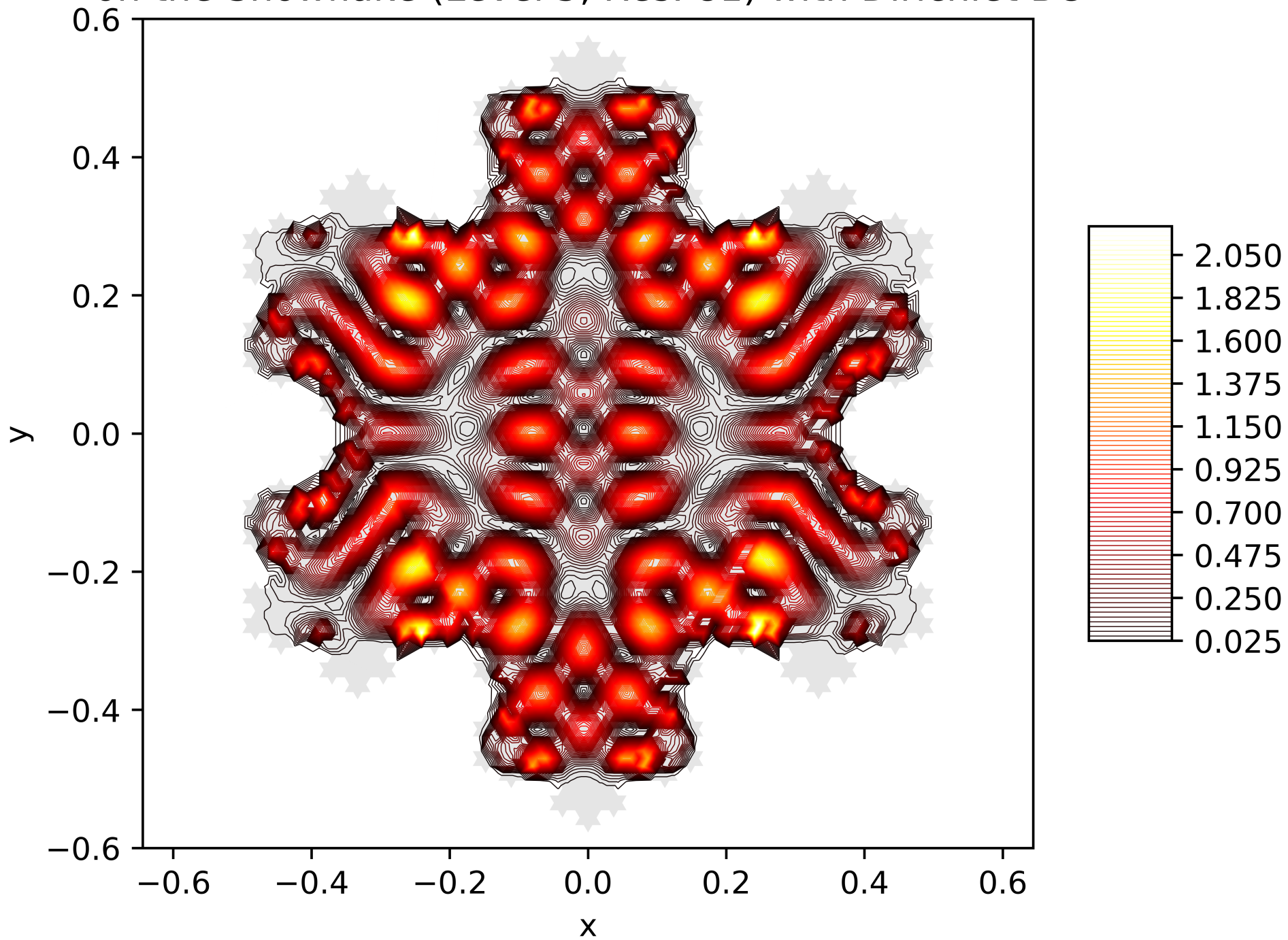
Contour Lines of the Energy Function of the 56. Eigenfunction on the Snowflake (Level 5, Res. 81) with Dirichlet BC
