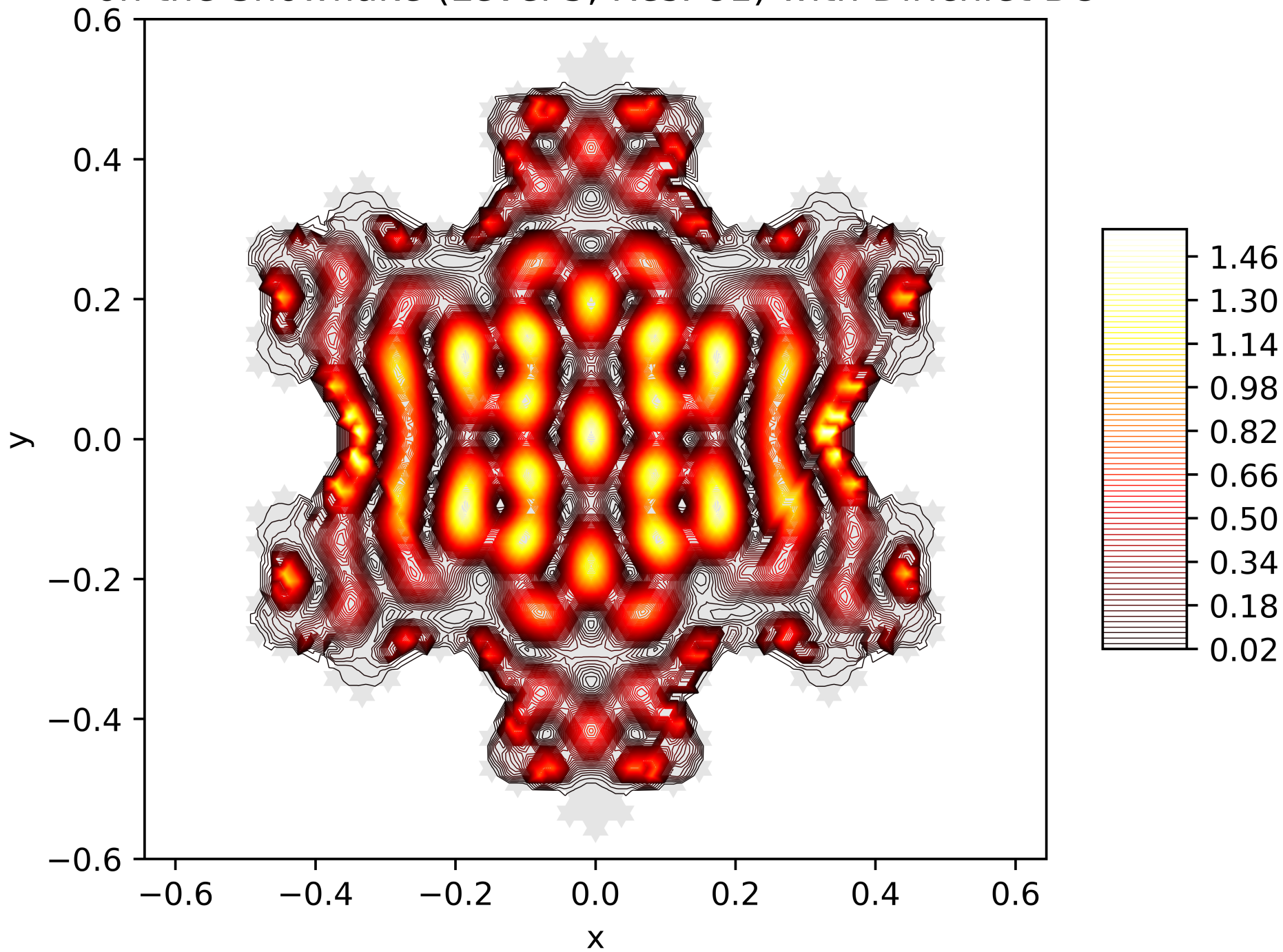
Contour Lines of the Energy Function of the 50. Eigenfunction on the Snowflake (Level 5, Res. 81) with Dirichlet BC
