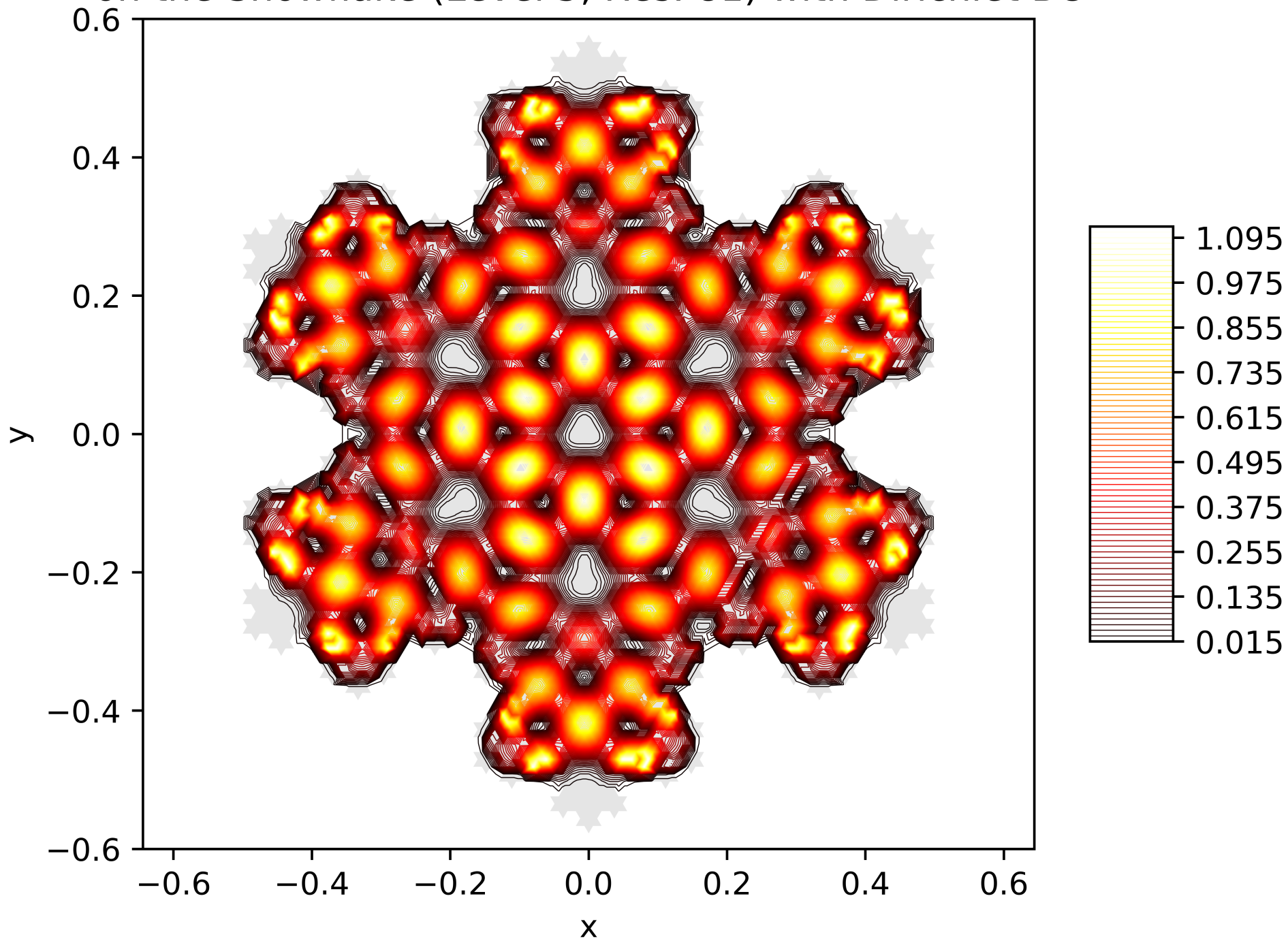
Contour Lines of the Energy Function of the 52. Eigenfunction on the Snowflake (Level 5, Res. 81) with Dirichlet BC
