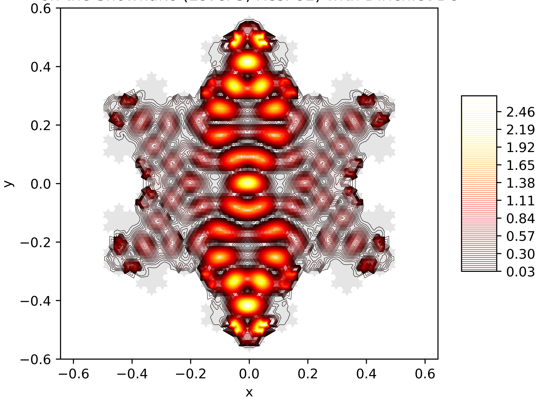
Contour Lines of the Energy Function of the 59. Eigenfunction on the Snowflake (Level 5, Res. 81) with Dirichlet BC
