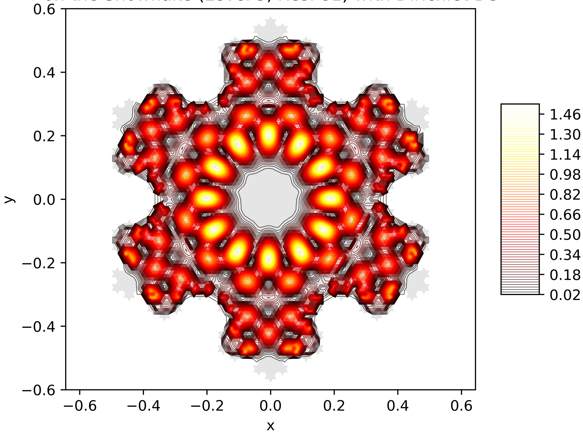
Contour Lines of the Energy Function of the 55. Eigenfunction on the Snowflake (Level 5, Res. 81) with Dirichlet BC
