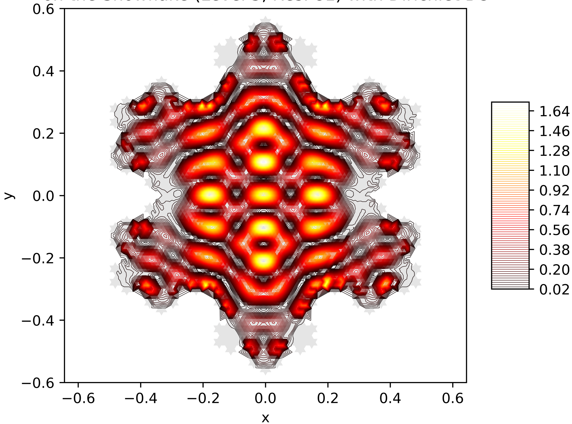
Contour Lines of the Energy Function of the 49. Eigenfunction on the Snowflake (Level 5, Res. 81) with Dirichlet BC
