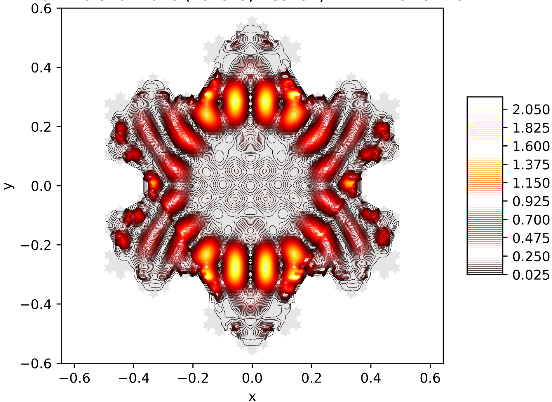
Contour Lines of the Energy Function of the 46. Eigenfunction on the Snowflake (Level 5, Res. 81) with Dirichlet BC
