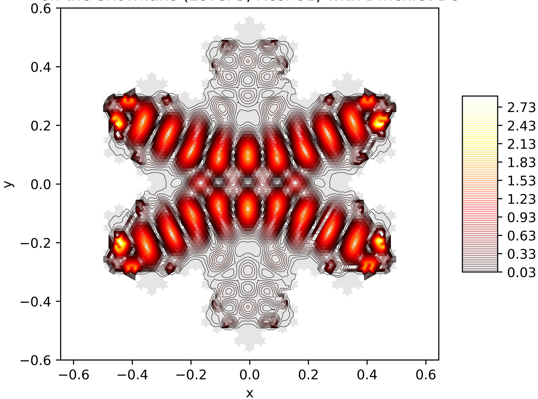
Contour Lines of the Energy Function of the 54. Eigenfunction on the Snowflake (Level 5, Res. 81) with Dirichlet BC
