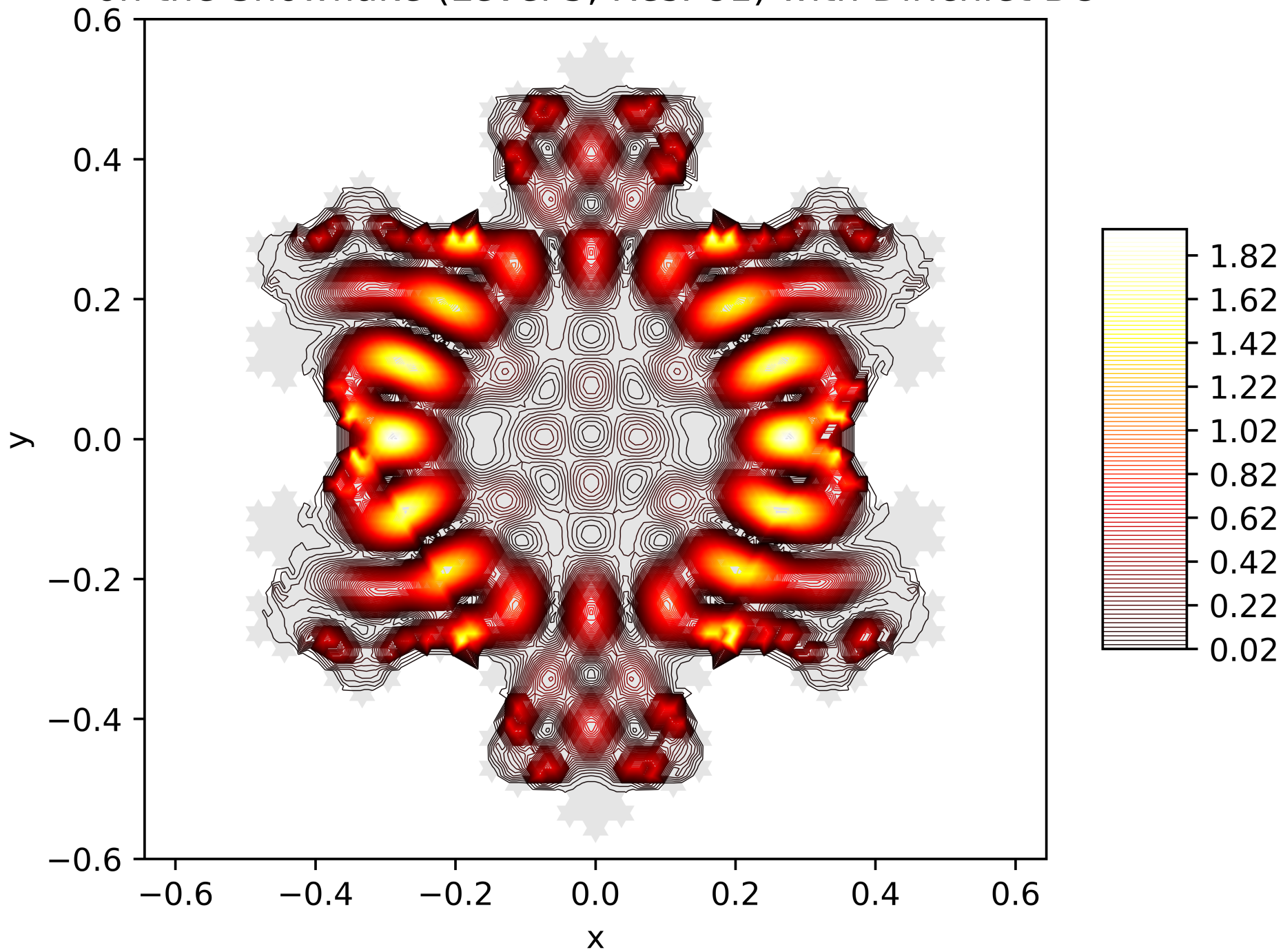
Contour Lines of the Energy Function of the 47. Eigenfunction on the Snowflake (Level 5, Res. 81) with Dirichlet BC
