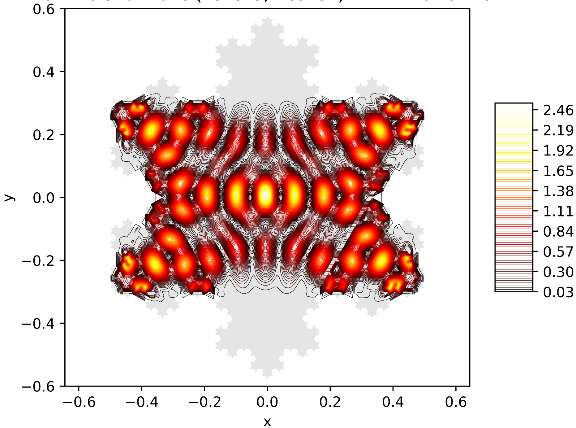
Contour Lines of the Energy Function of the 60. Eigenfunction on the Snowflake (Level 5, Res. 81) with Dirichlet BC
