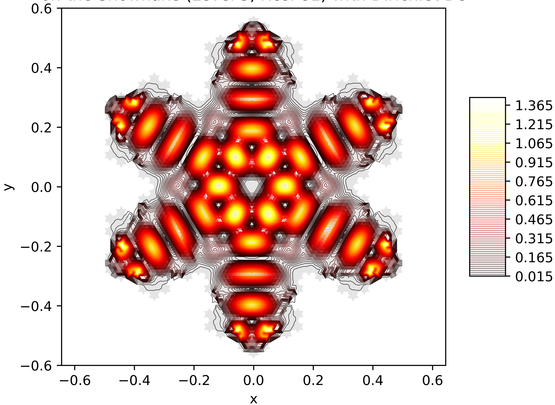
Contour Lines of the Energy Function of the 43. Eigenfunction on the Snowflake (Level 5, Res. 81) with Dirichlet BC
