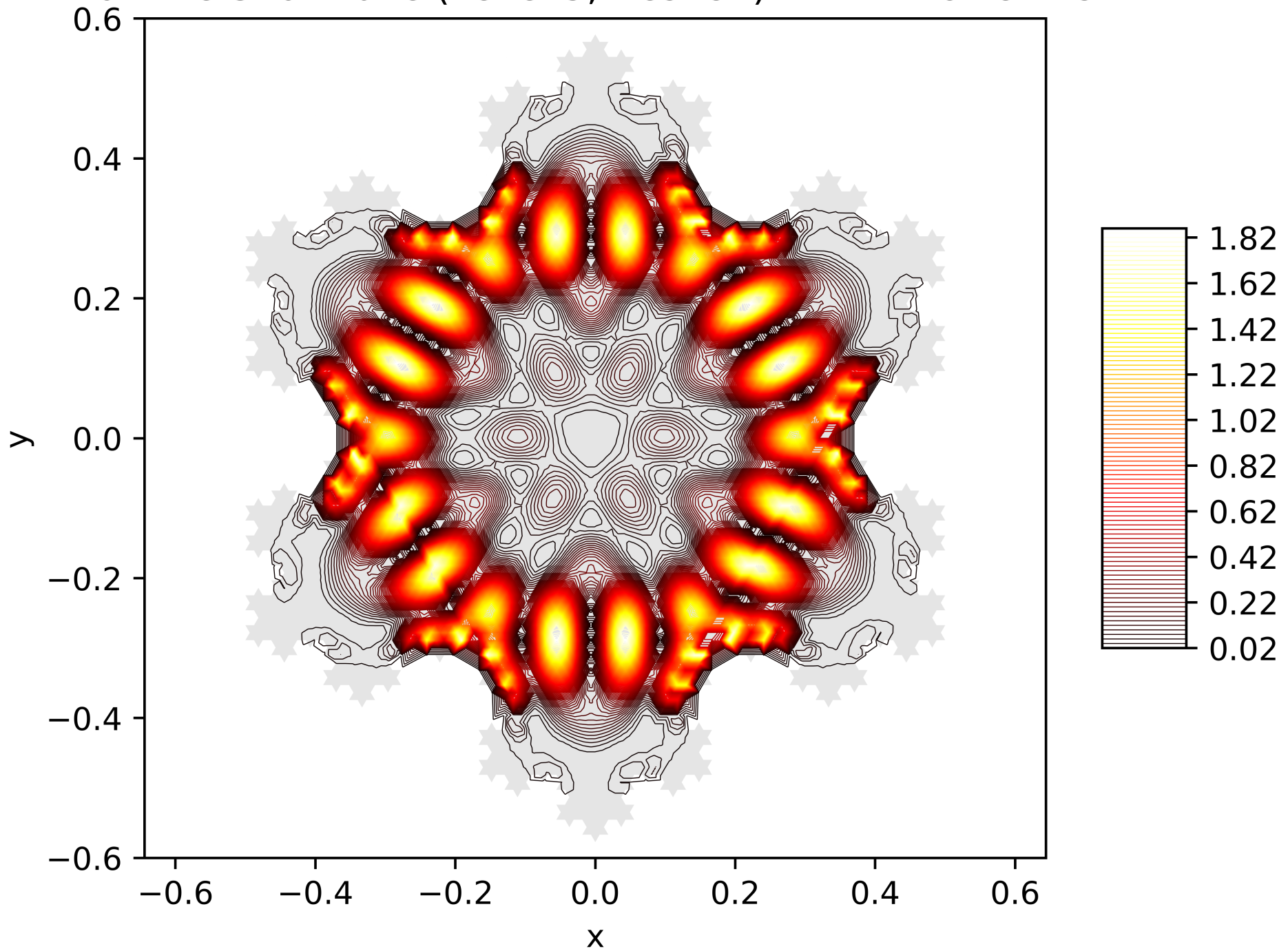
Contour Lines of the Energy Function of the 48. Eigenfunction on the Snowflake (Level 5, Res. 81) with Dirichlet BC
