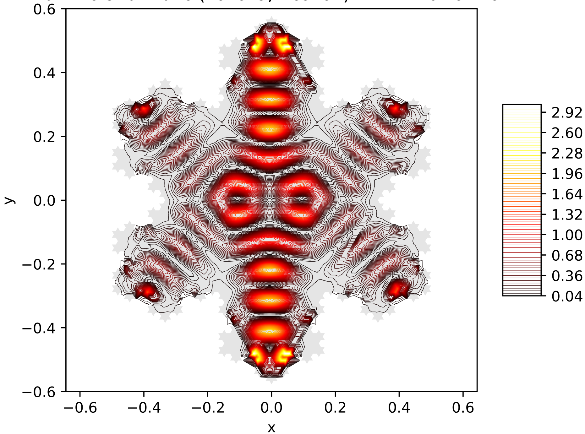
Contour Lines of the Energy Function of the 53. Eigenfunction on the Snowflake (Level 5, Res. 81) with Dirichlet BC
