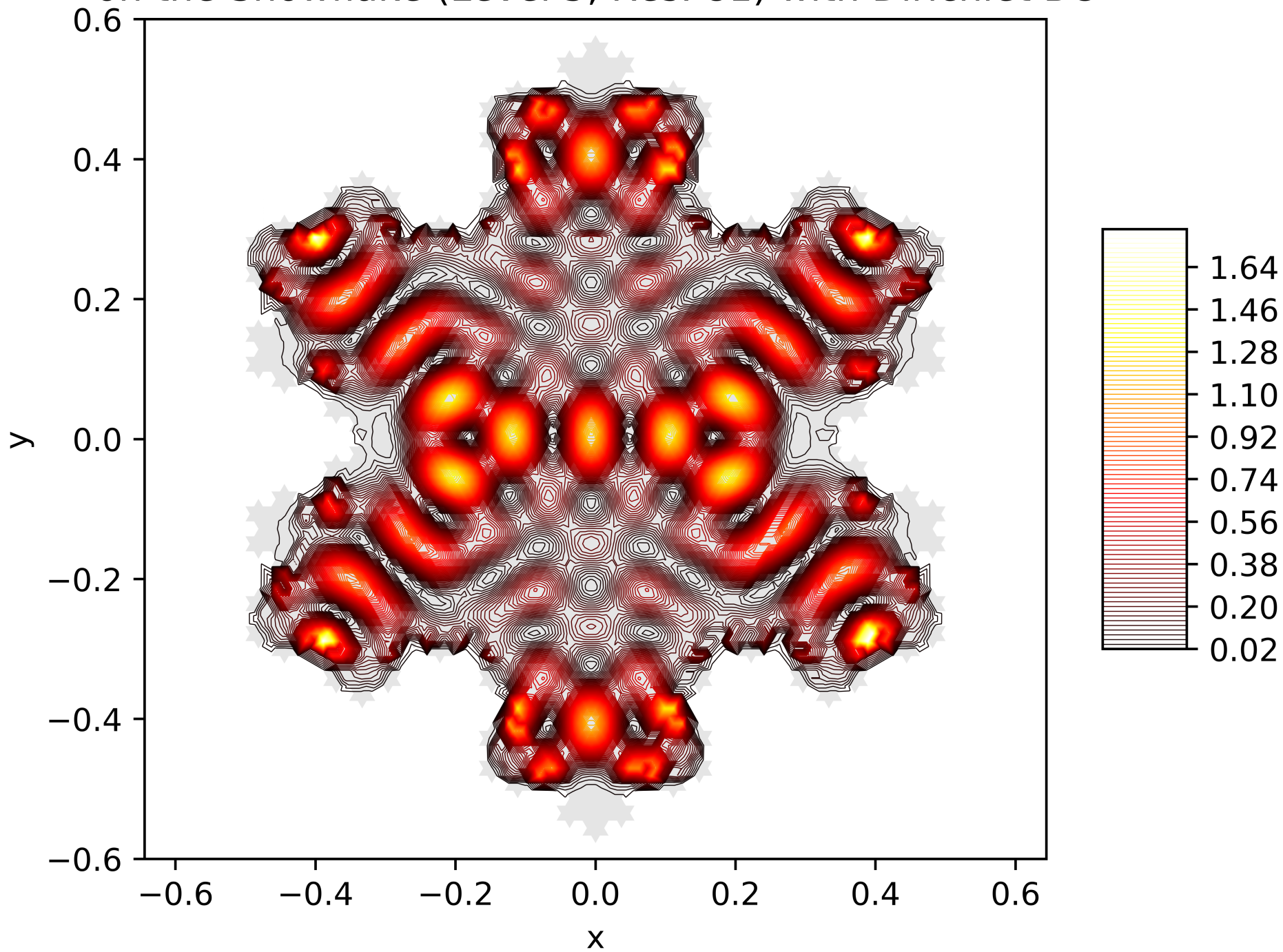
Contour Lines of the Energy Function of the 44. Eigenfunction on the Snowflake (Level 5, Res. 81) with Dirichlet BC
