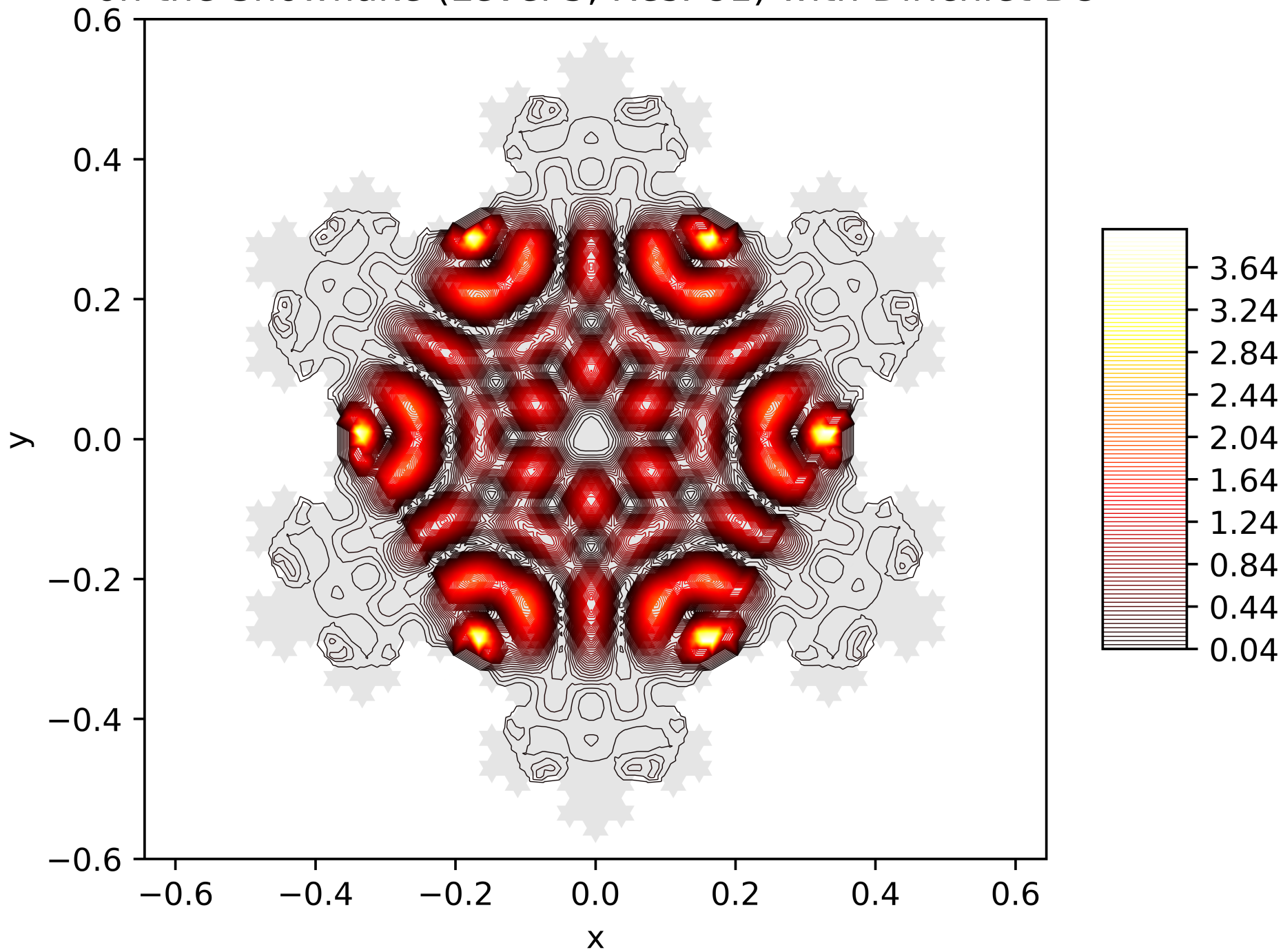
Contour Lines of the Energy Function of the 58. Eigenfunction on the Snowflake (Level 5, Res. 81) with Dirichlet BC
