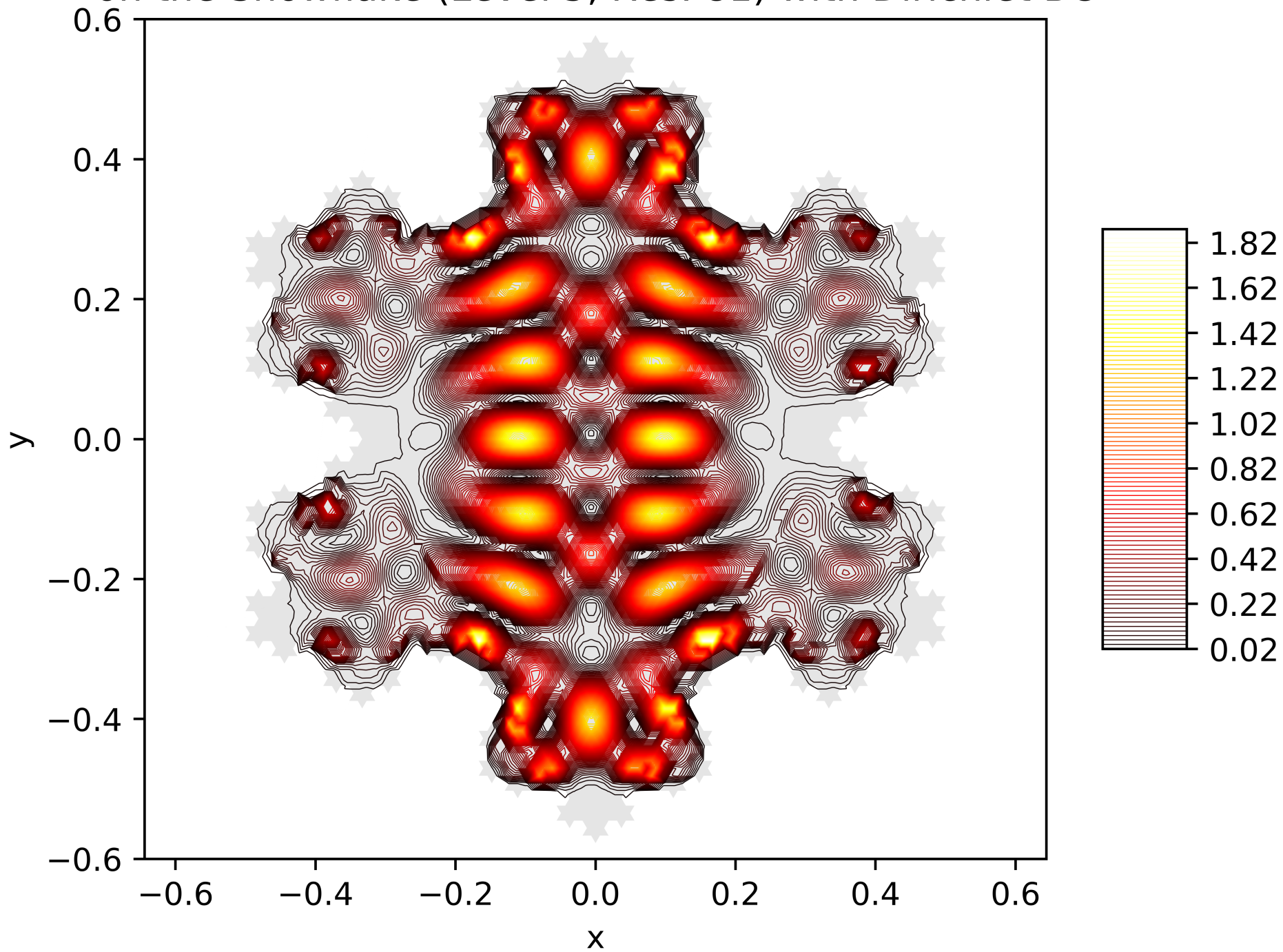
Contour Lines of the Energy Function of the 41. Eigenfunction on the Snowflake (Level 5, Res. 81) with Dirichlet BC
