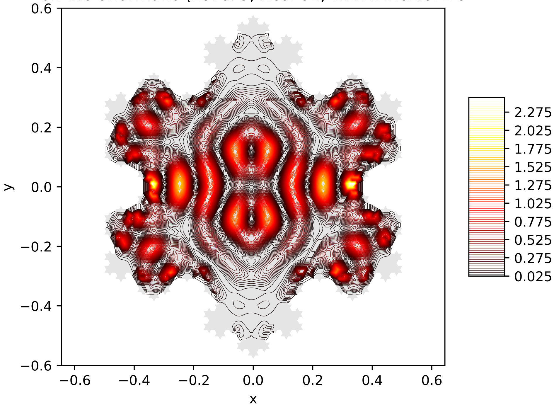
Contour Lines of the Energy Function of the 42. Eigenfunction on the Snowflake (Level 5, Res. 81) with Dirichlet BC
