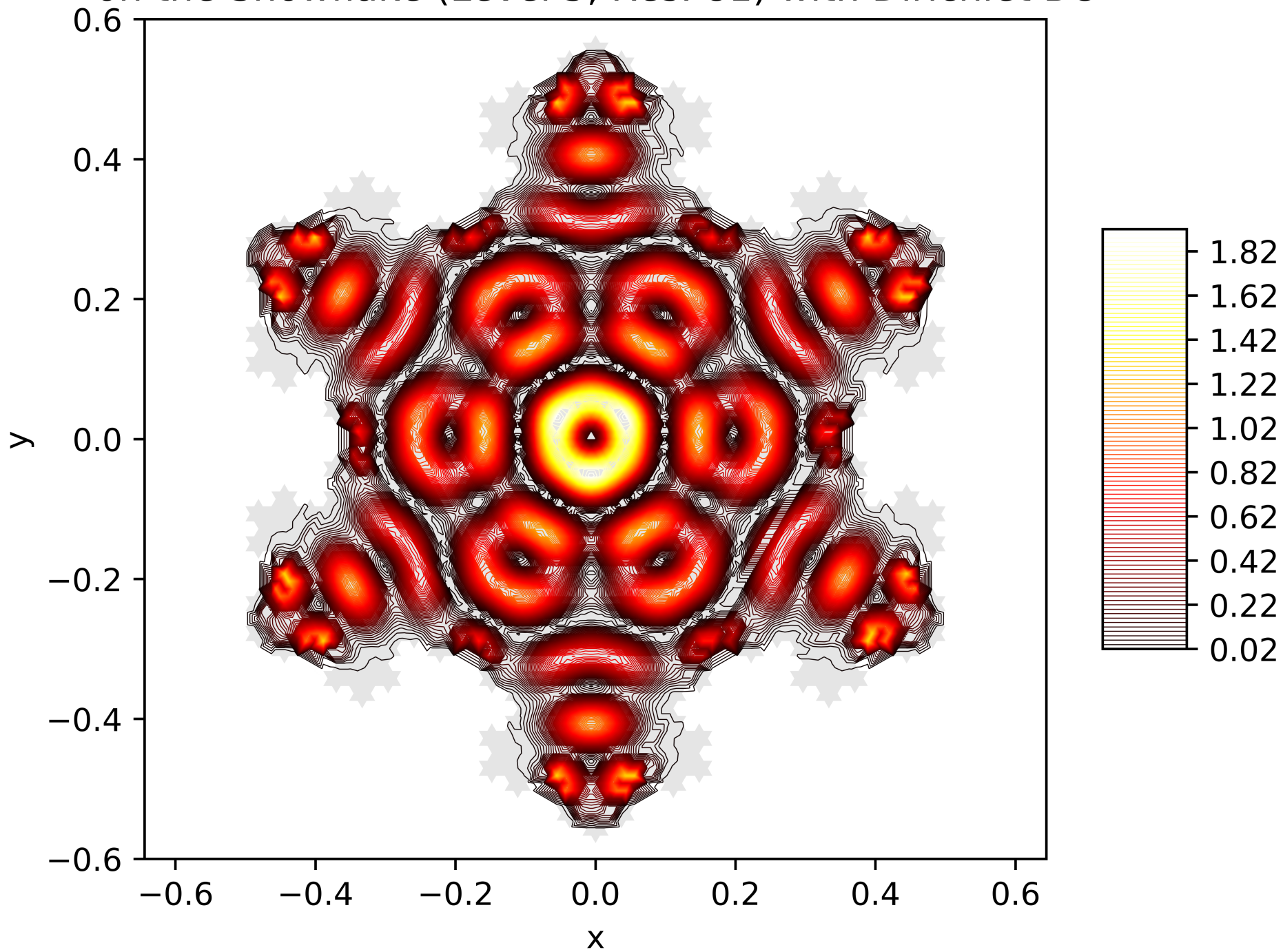
Contour Lines of the Energy Function of the 51. Eigenfunction on the Snowflake (Level 5, Res. 81) with Dirichlet BC
