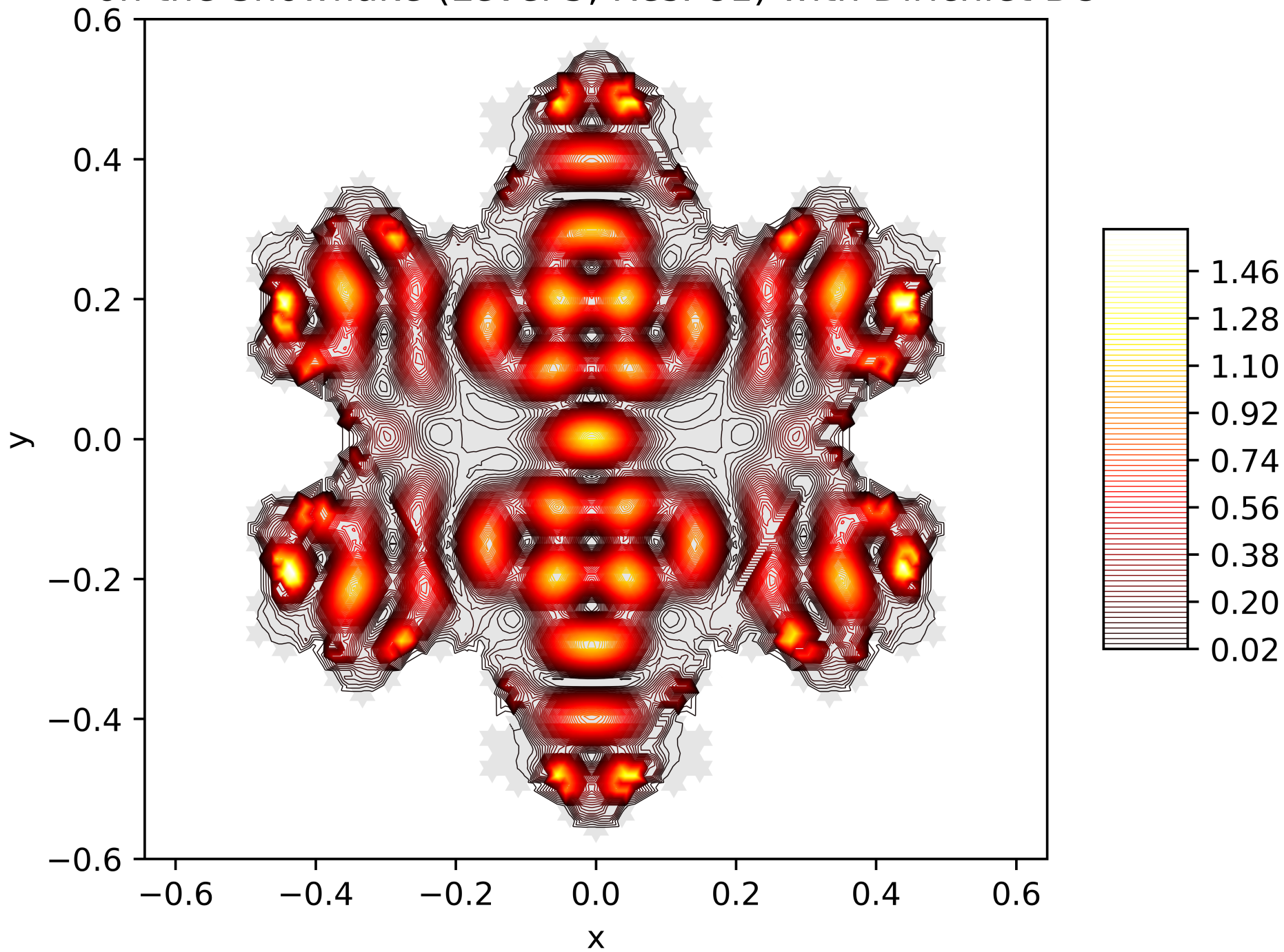
Contour Lines of the Energy Function of the 45. Eigenfunction on the Snowflake (Level 5, Res. 81) with Dirichlet BC
