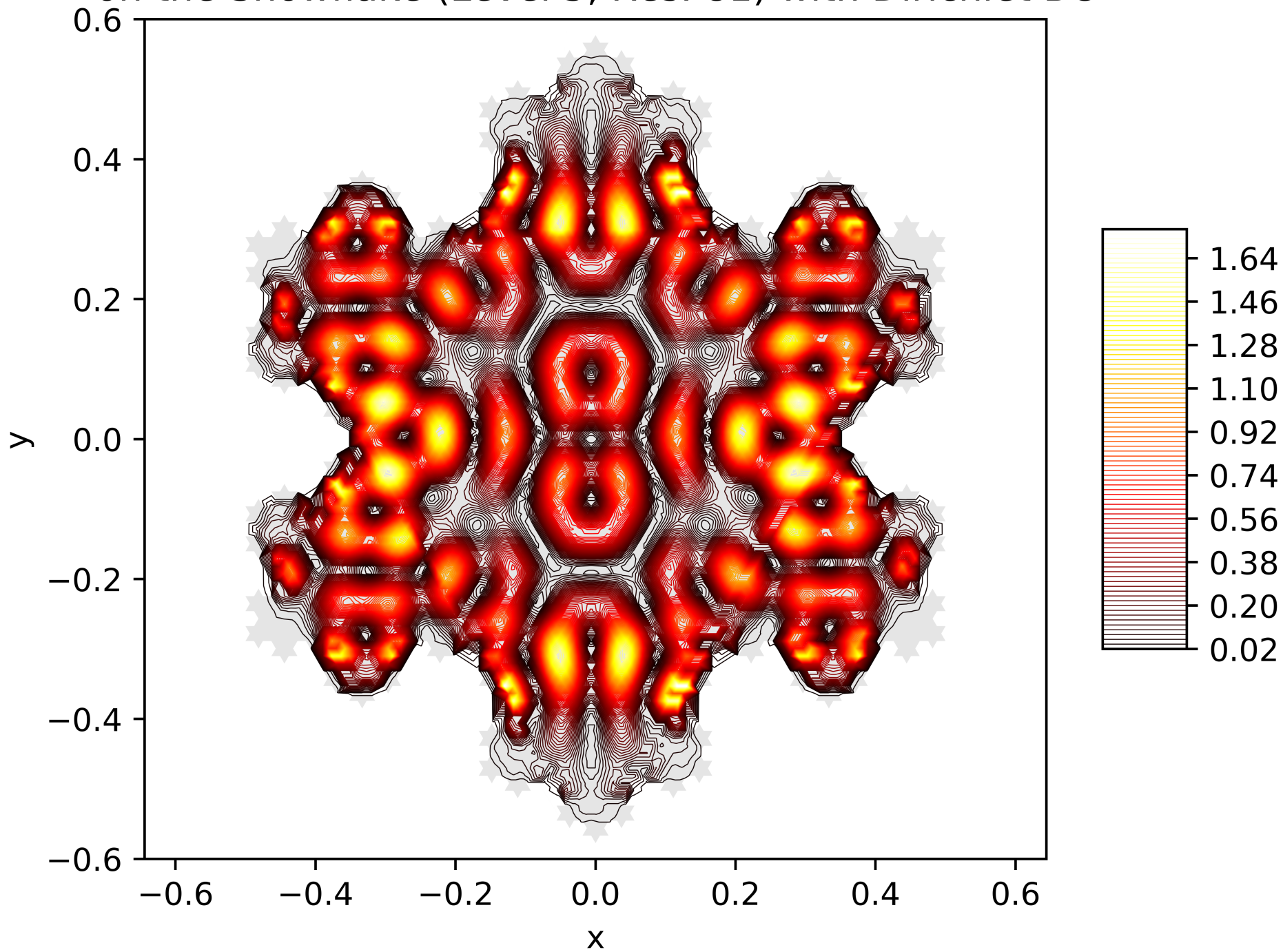
Contour Lines of the Energy Function of the 57. Eigenfunction on the Snowflake (Level 5, Res. 81) with Dirichlet BC
