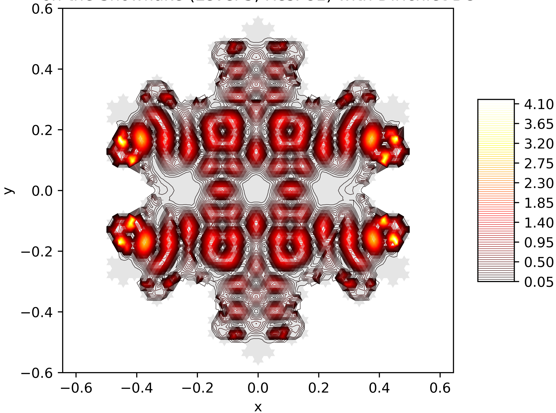
Contour Lines of the Energy Function of the 81. Eigenfunction on the Snowflake (Level 5, Res. 81) with Dirichlet BC
