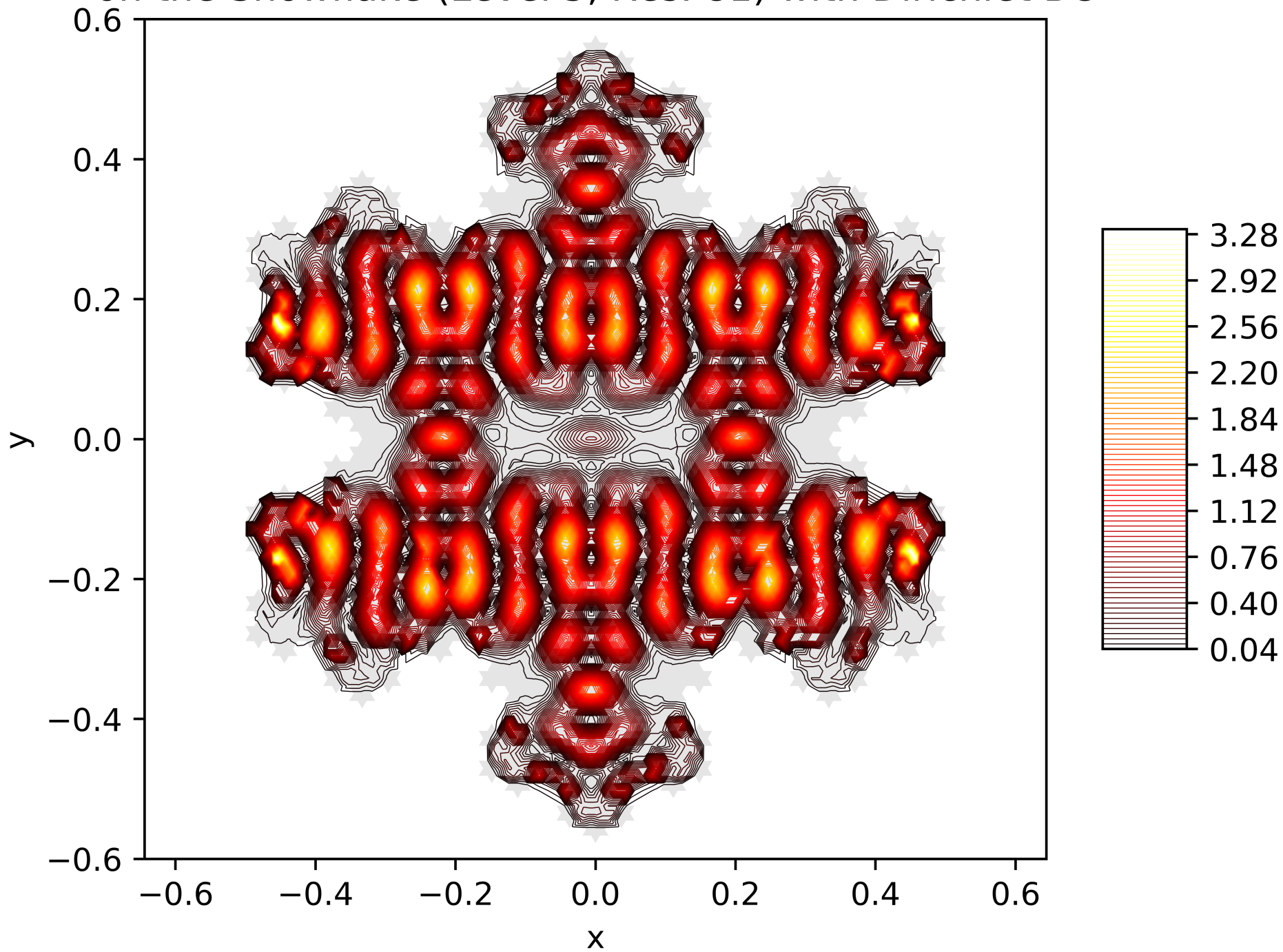
Contour Lines of the Energy Function of the 90. Eigenfunction on the Snowflake (Level 5, Res. 81) with Dirichlet BC
