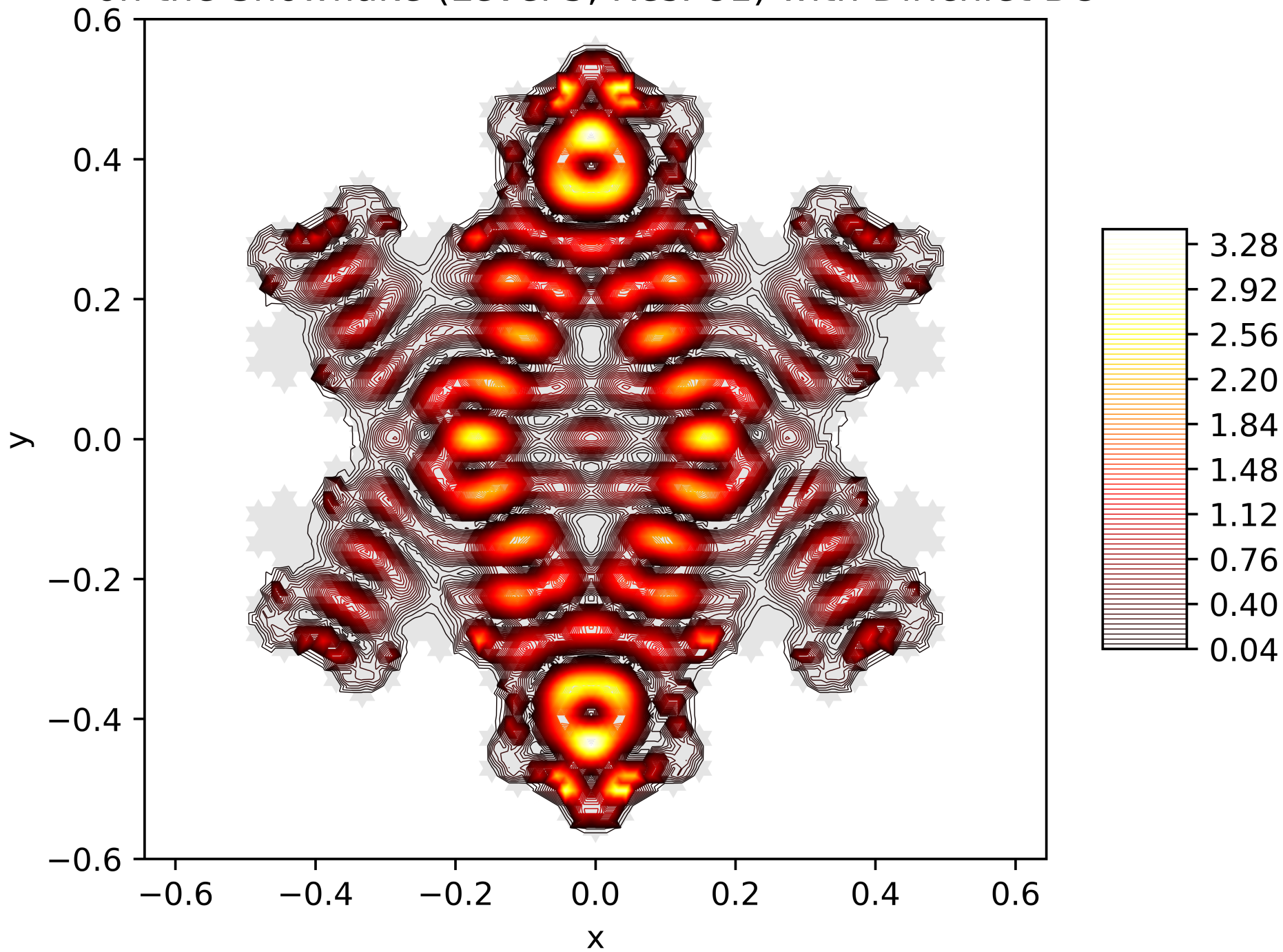
Contour Lines of the Energy Function of the 83. Eigenfunction on the Snowflake (Level 5, Res. 81) with Dirichlet BC
