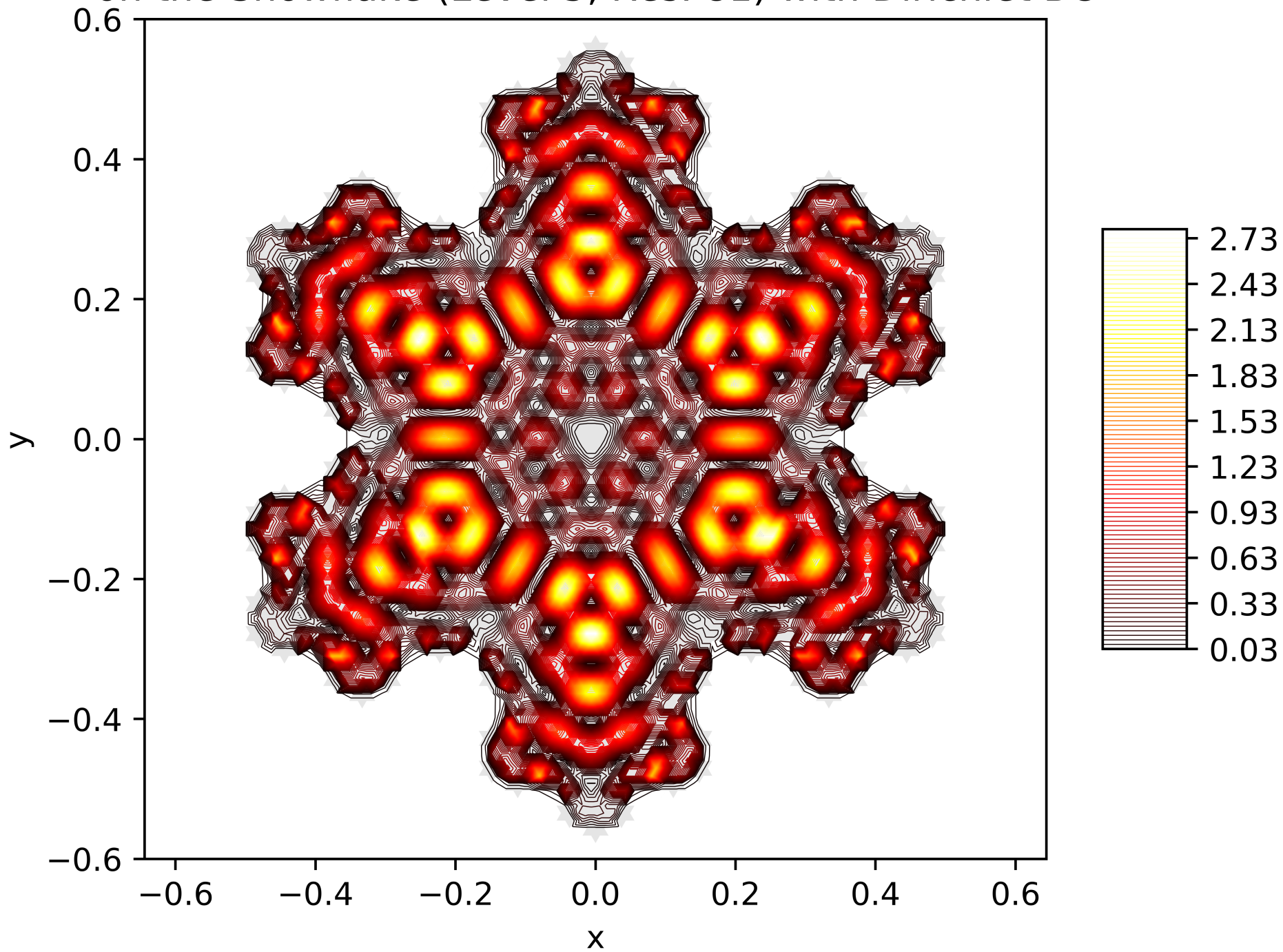
Contour Lines of the Energy Function of the 96. Eigenfunction on the Snowflake (Level 5, Res. 81) with Dirichlet BC
