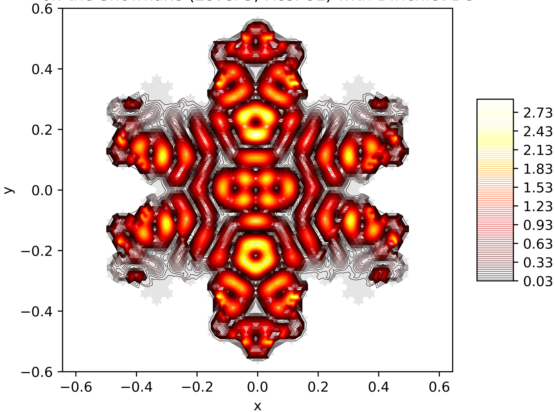
Contour Lines of the Energy Function of the 91. Eigenfunction on the Snowflake (Level 5, Res. 81) with Dirichlet BC
