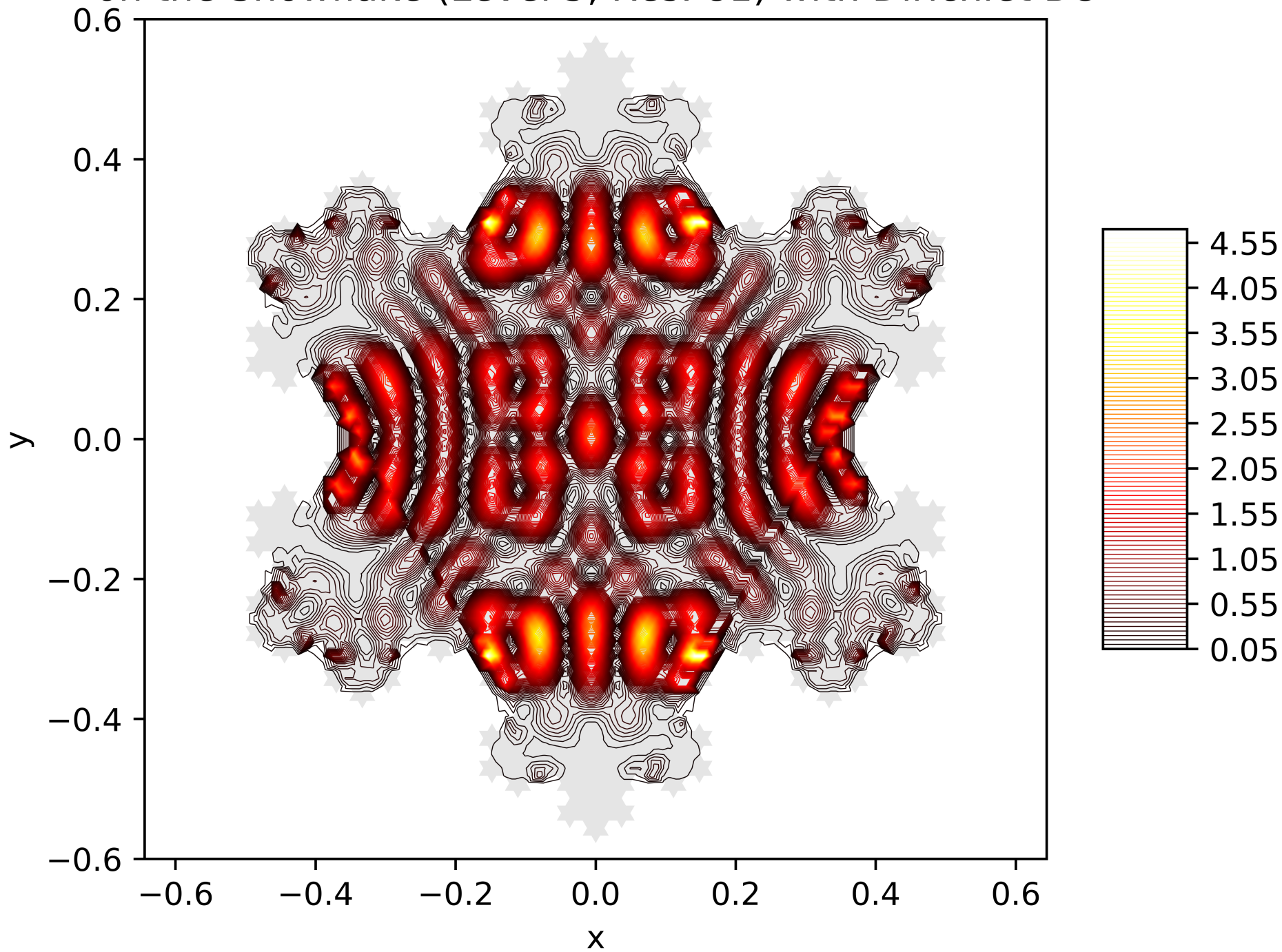
Contour Lines of the Energy Function of the 86. Eigenfunction on the Snowflake (Level 5, Res. 81) with Dirichlet BC
