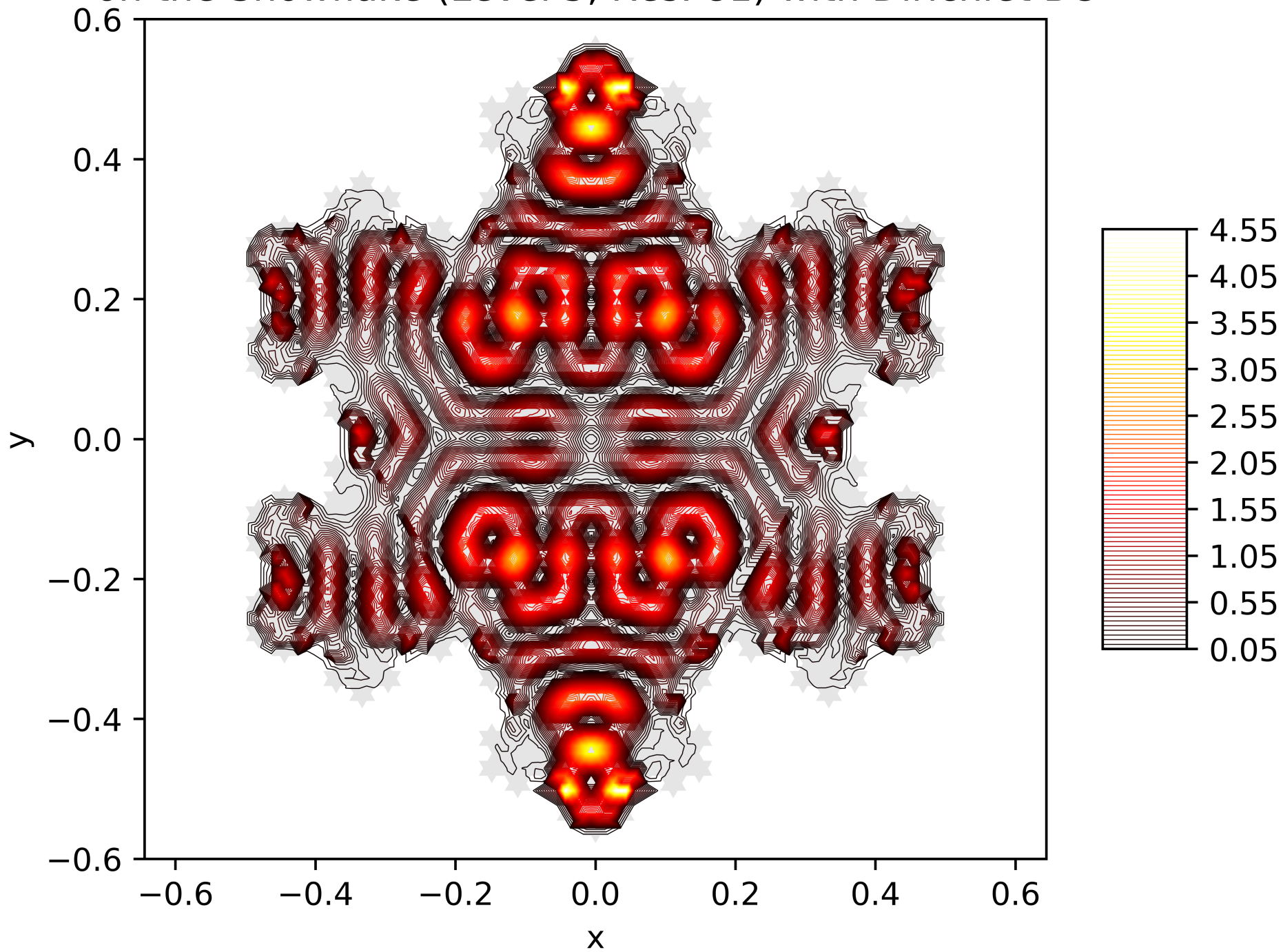
Contour Lines of the Energy Function of the 94. Eigenfunction on the Snowflake (Level 5, Res. 81) with Dirichlet BC
