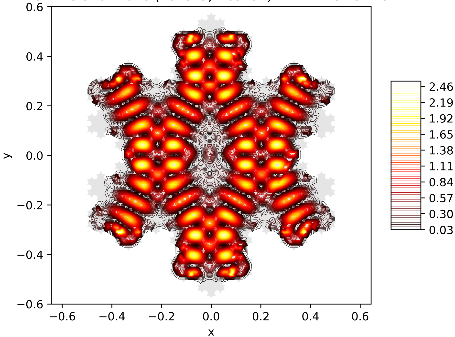
Contour Lines of the Energy Function of the 89. Eigenfunction on the Snowflake (Level 5, Res. 81) with Dirichlet BC
