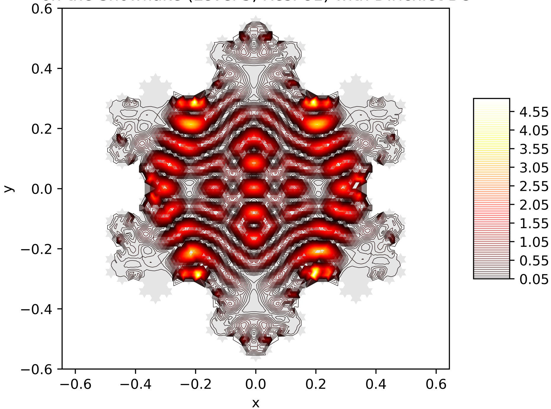
Contour Lines of the Energy Function of the 85. Eigenfunction on the Snowflake (Level 5, Res. 81) with Dirichlet BC
