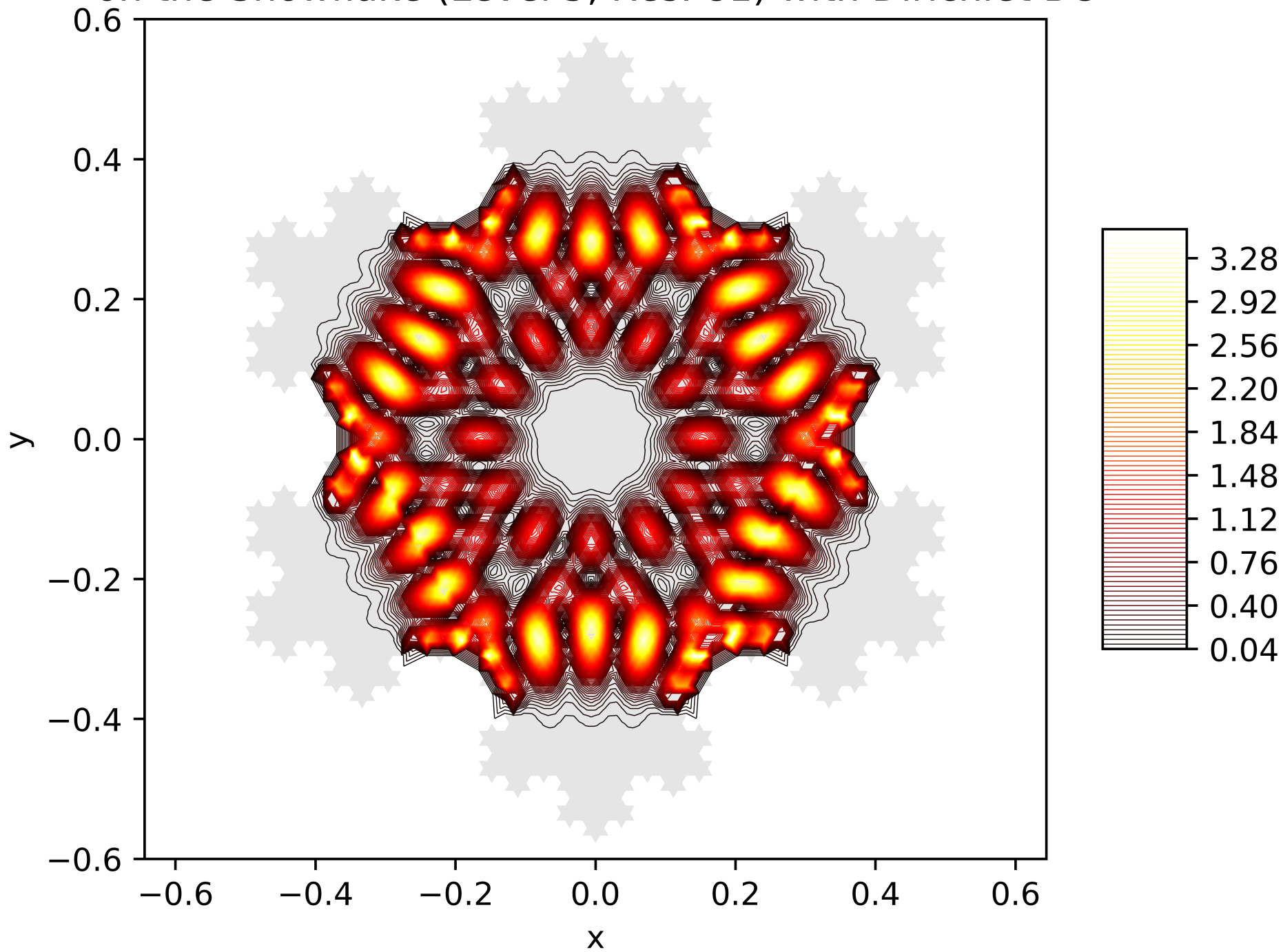
Contour Lines of the Energy Function of the 88. Eigenfunction on the Snowflake (Level 5, Res. 81) with Dirichlet BC
