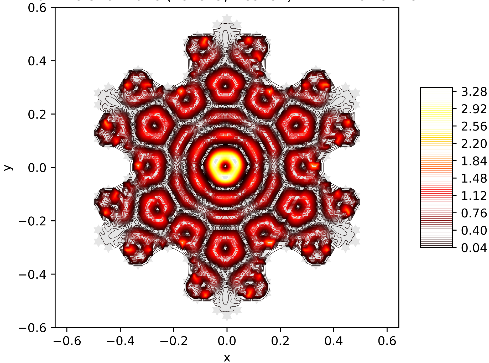
Contour Lines of the Energy Function of the 87. Eigenfunction on the Snowflake (Level 5, Res. 81) with Dirichlet BC
