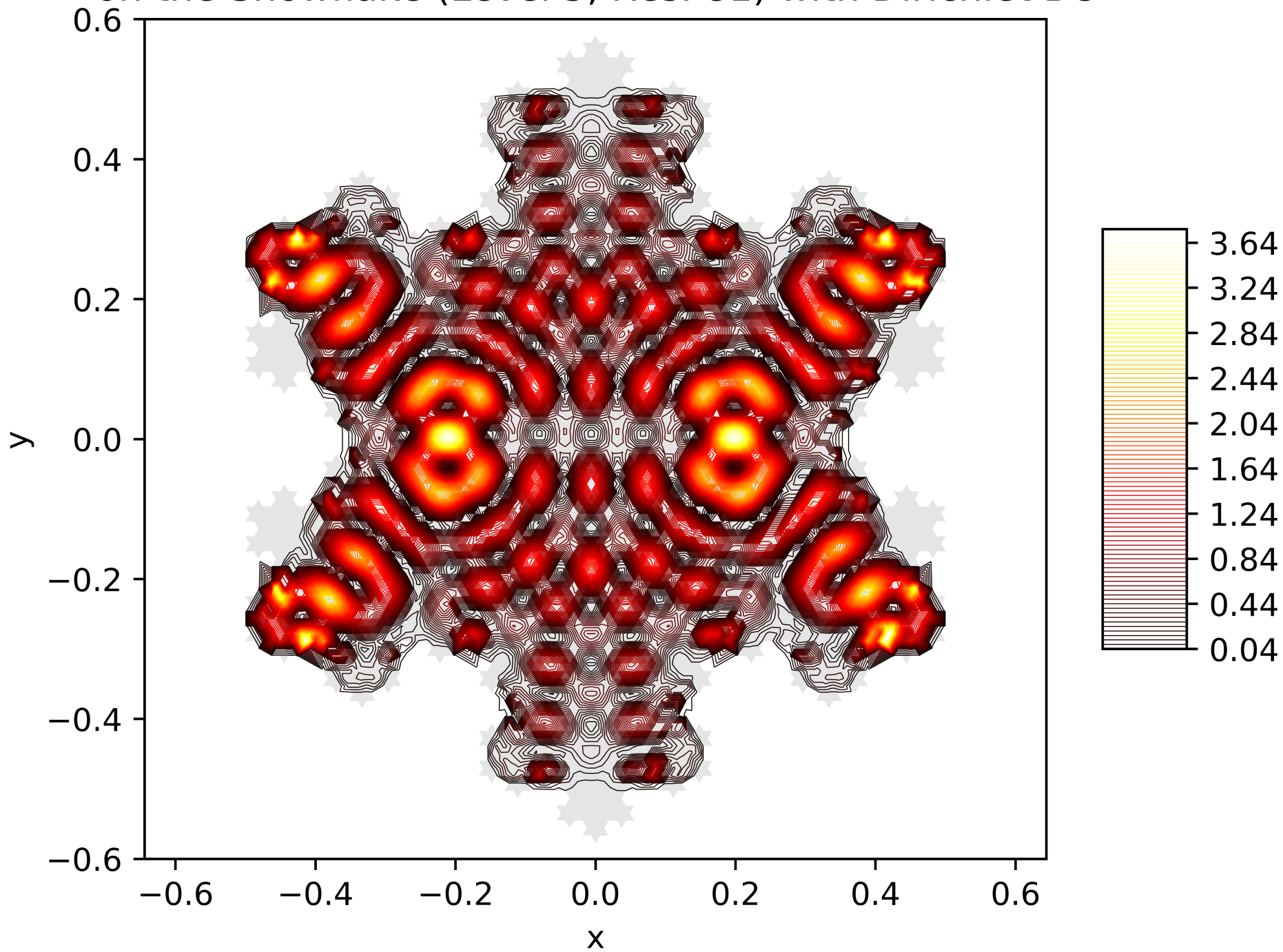
Contour Lines of the Energy Function of the 95. Eigenfunction on the Snowflake (Level 5, Res. 81) with Dirichlet BC
