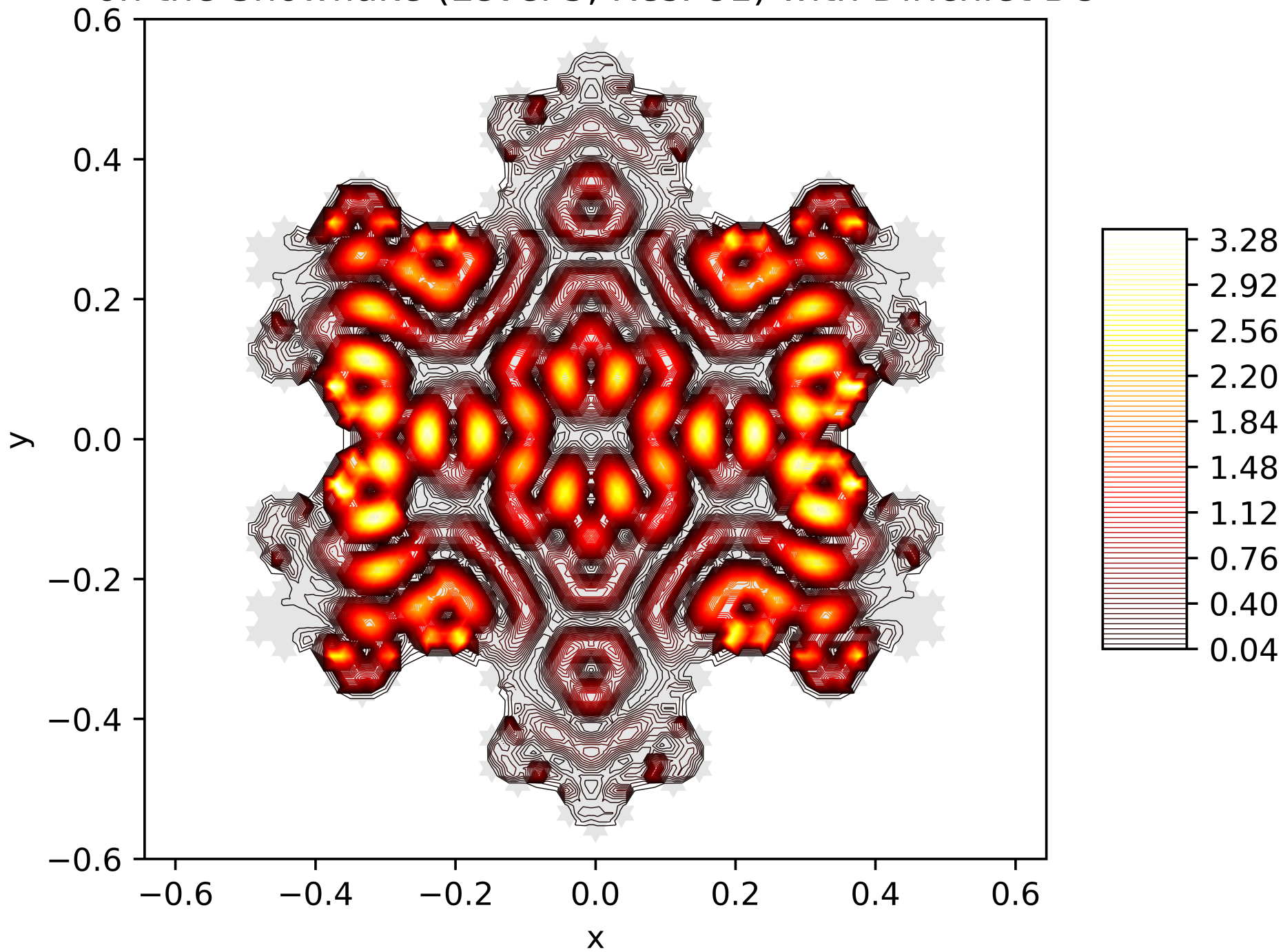
Contour Lines of the Energy Function of the 99. Eigenfunction on the Snowflake (Level 5, Res. 81) with Dirichlet BC
