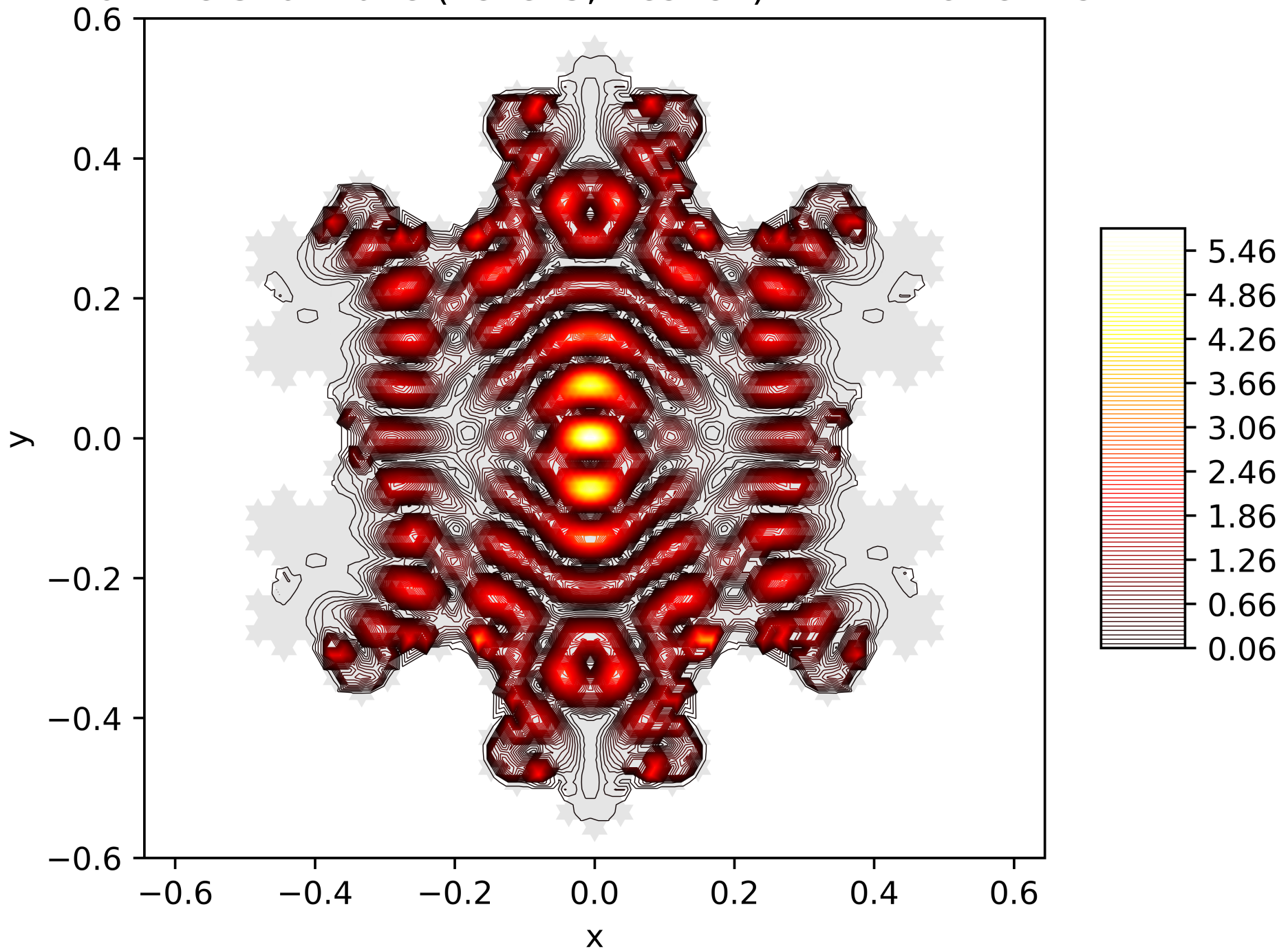
Contour Lines of the Energy Function of the 100. Eigenfunction on the Snowflake (Level 5, Res. 81) with Dirichlet BC
