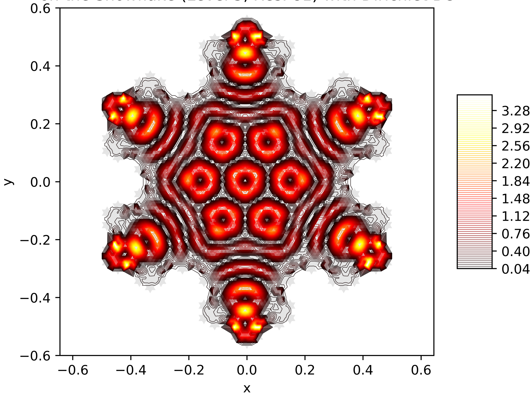
Contour Lines of the Energy Function of the 97. Eigenfunction on the Snowflake (Level 5, Res. 81) with Dirichlet BC
