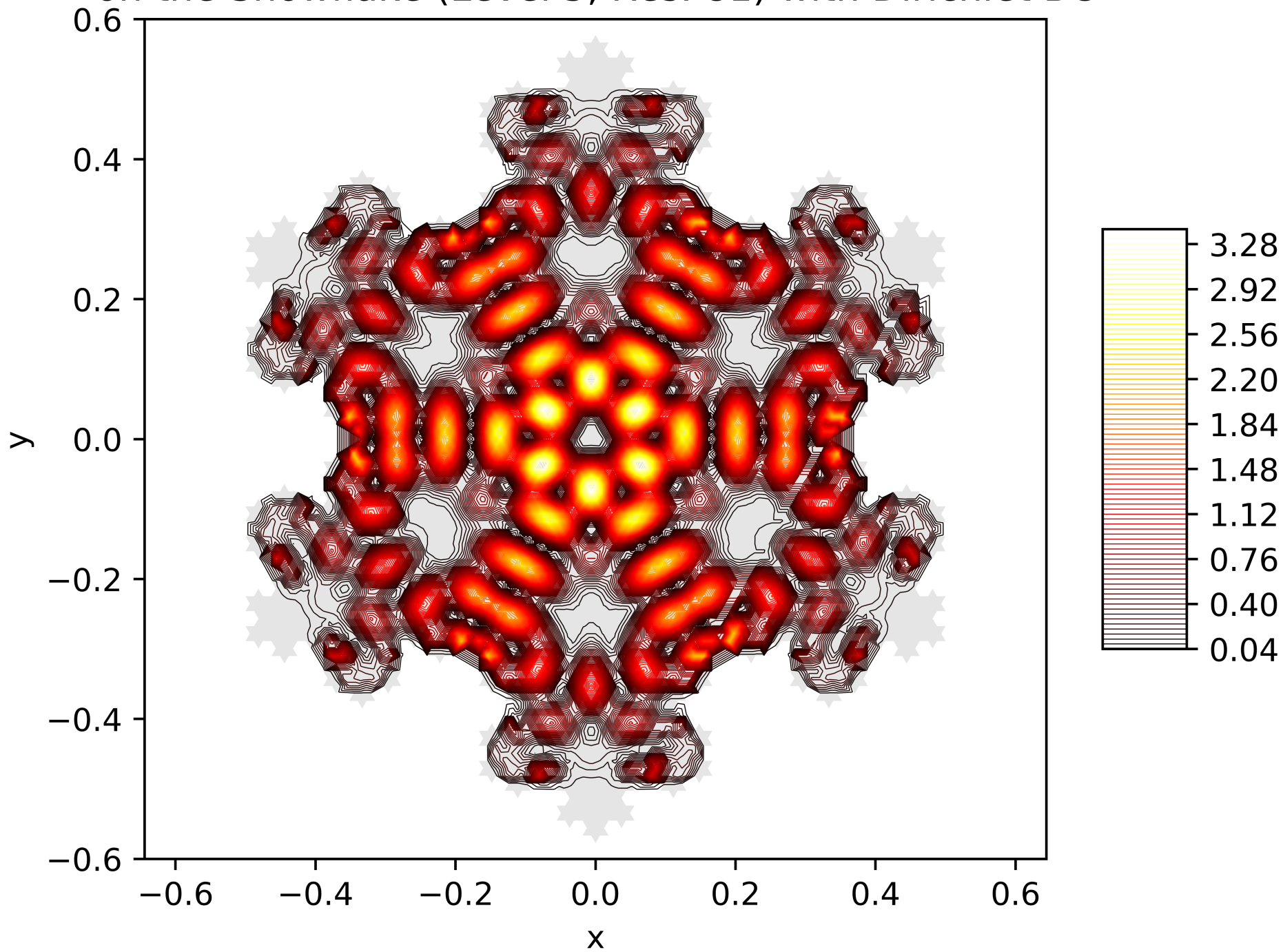
Contour Lines of the Energy Function of the 93. Eigenfunction on the Snowflake (Level 5, Res. 81) with Dirichlet BC
