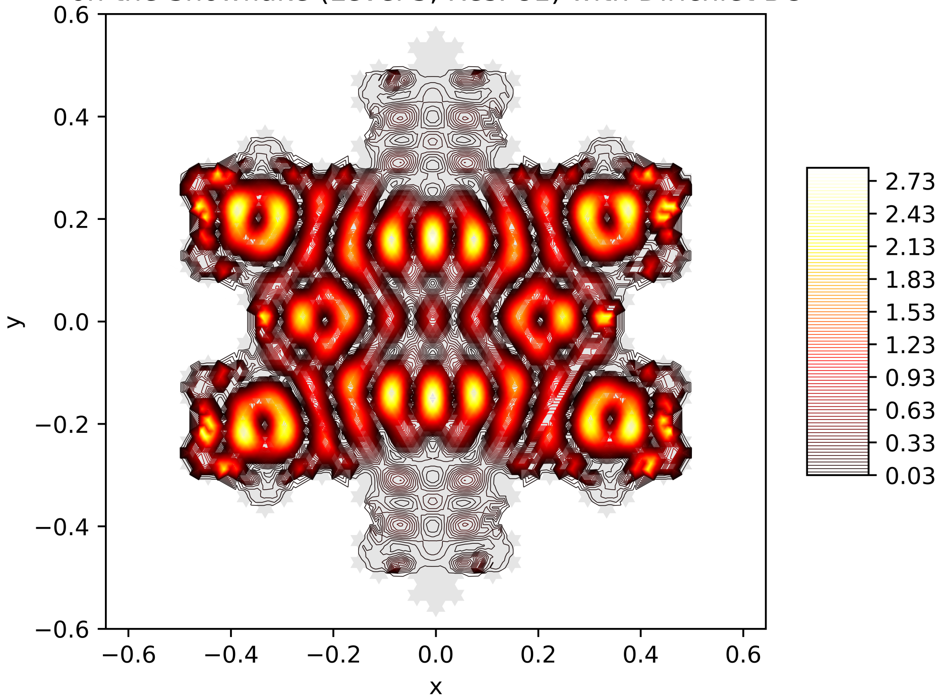
Contour Lines of the Energy Function of the 84. Eigenfunction on the Snowflake (Level 5, Res. 81) with Dirichlet BC
