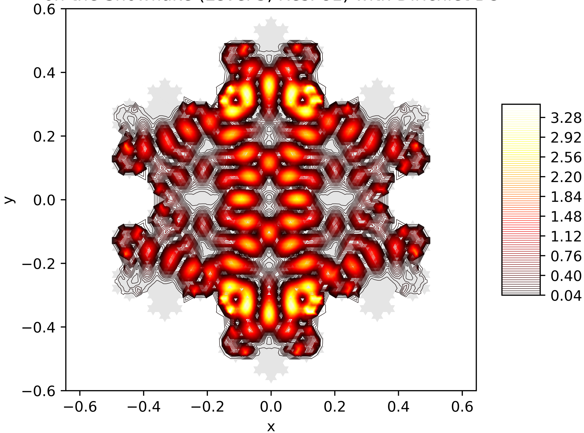
Contour Lines of the Energy Function of the 98. Eigenfunction on the Snowflake (Level 5, Res. 81) with Dirichlet BC
