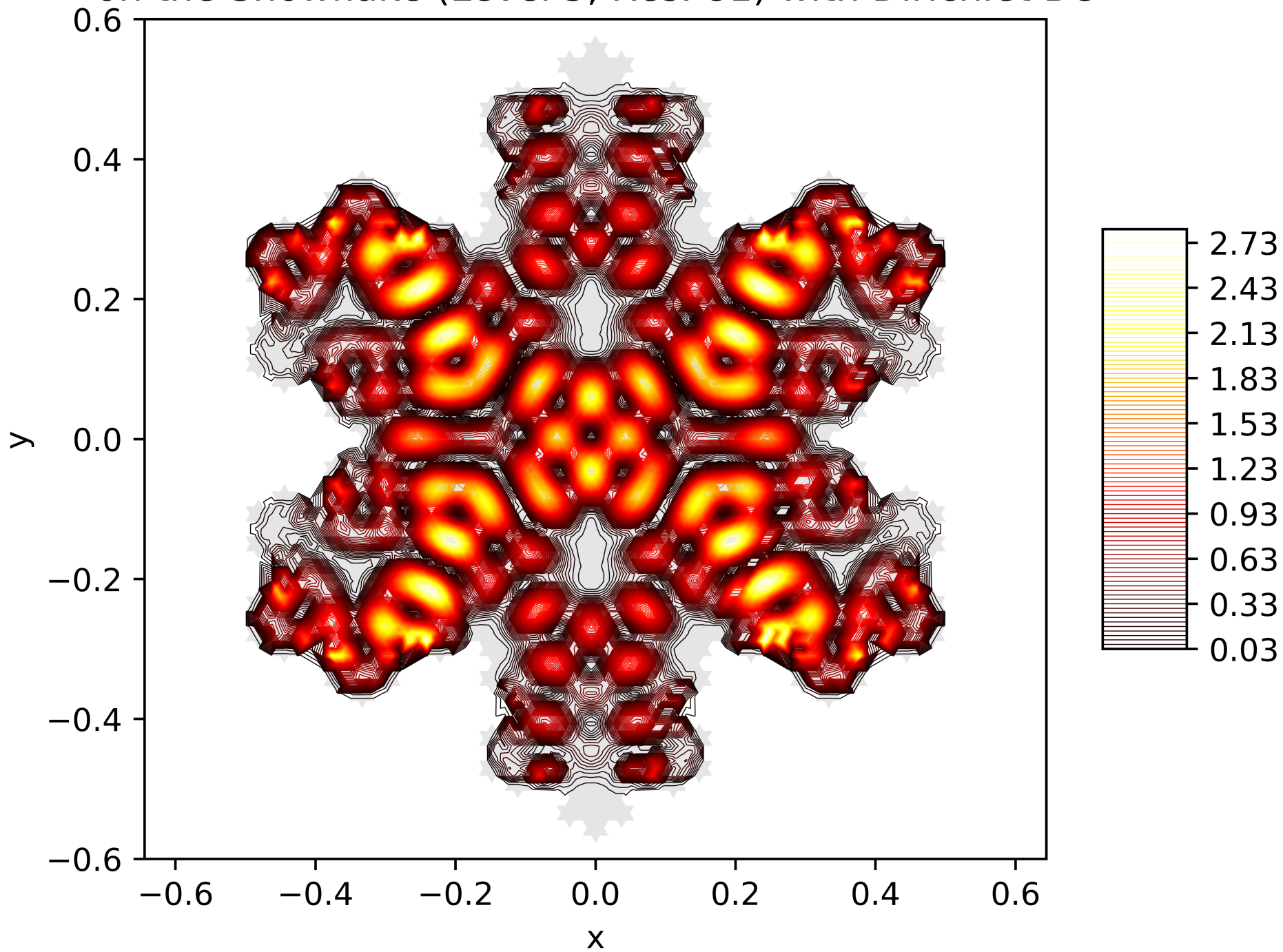
Contour Lines of the Energy Function of the 92. Eigenfunction on the Snowflake (Level 5, Res. 81) with Dirichlet BC
