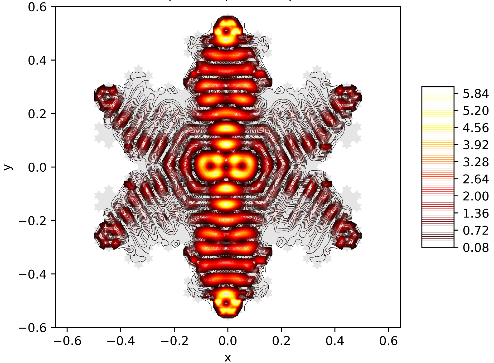
Contour Lines of the Energy Function of the 146. Eigenfunction on the Snowflake (Level 5, Res. 81) with Dirichlet BC
