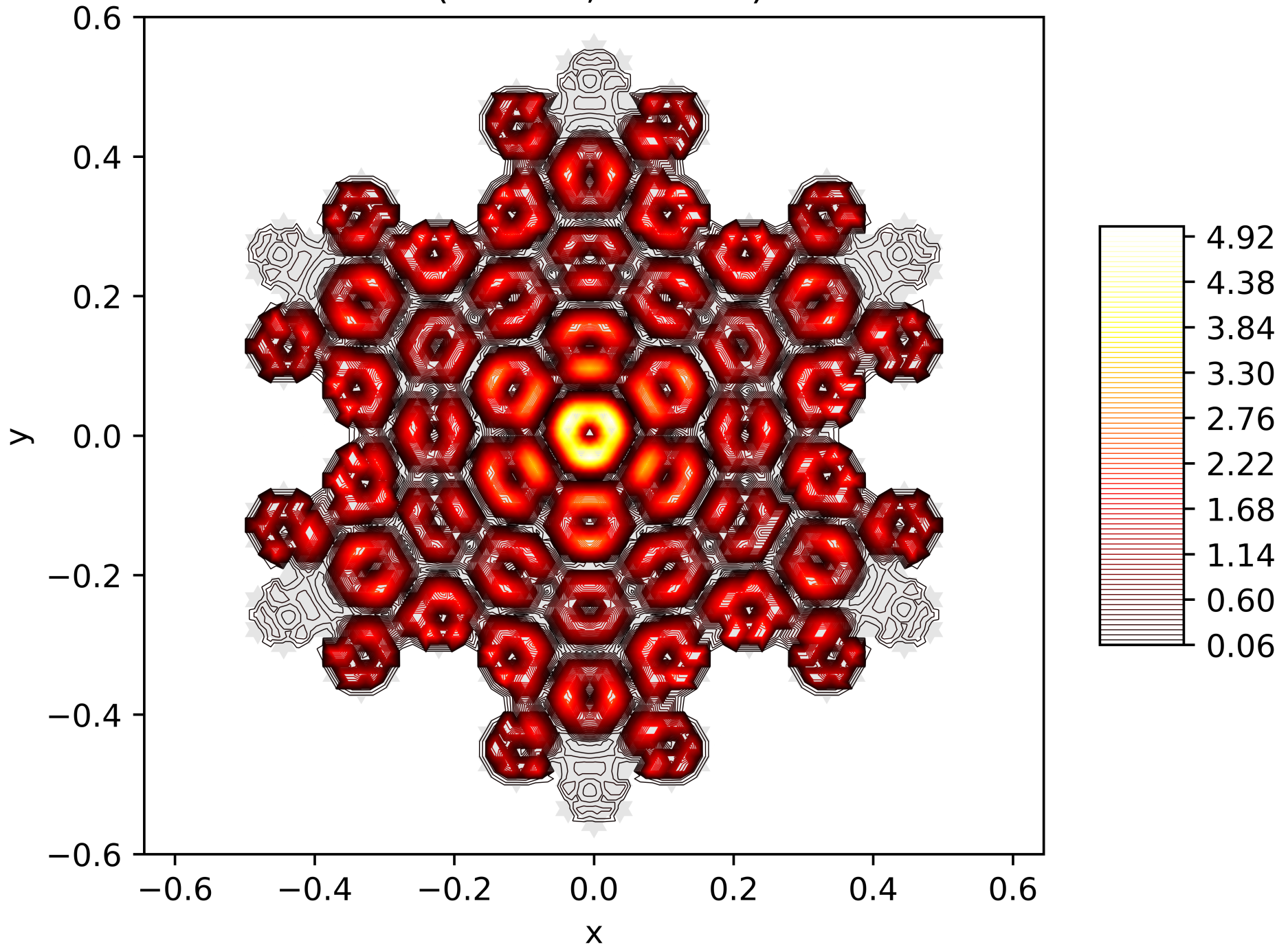
Contour Lines of the Energy Function of the 148. Eigenfunction on the Snowflake (Level 5, Res. 81) with Dirichlet BC
