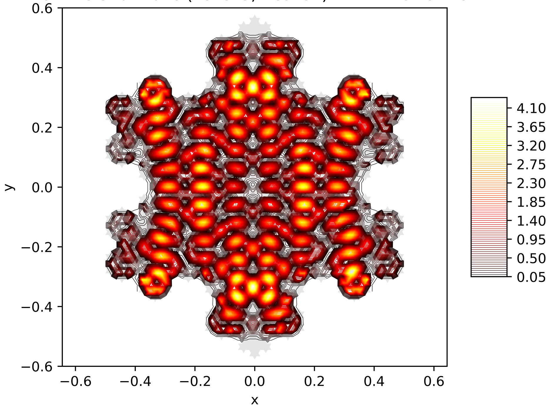
Contour Lines of the Energy Function of the 156. Eigenfunction on the Snowflake (Level 5, Res. 81) with Dirichlet BC
