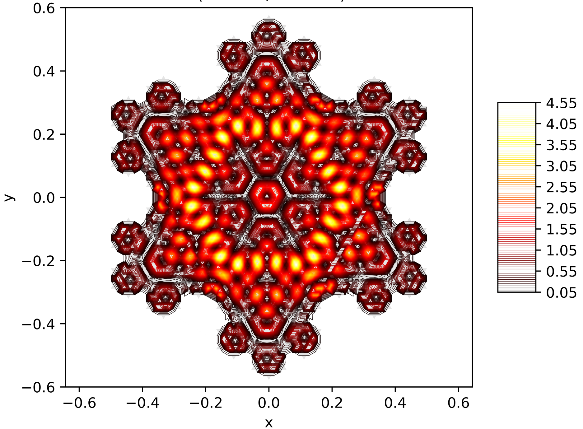
Contour Lines of the Energy Function of the 160. Eigenfunction on the Snowflake (Level 5, Res. 81) with Dirichlet BC
