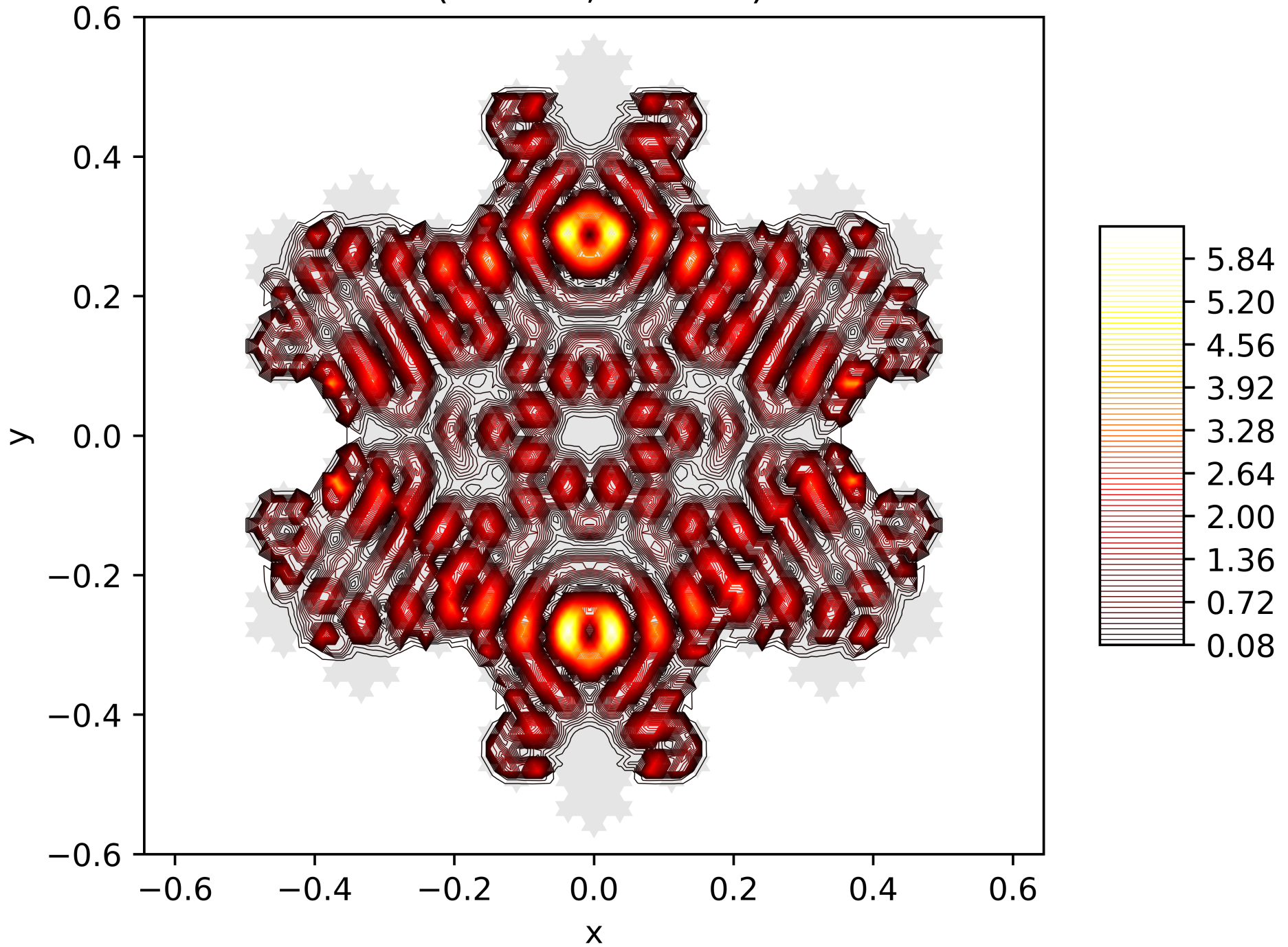
Contour Lines of the Energy Function of the 143. Eigenfunction on the Snowflake (Level 5, Res. 81) with Dirichlet BC
