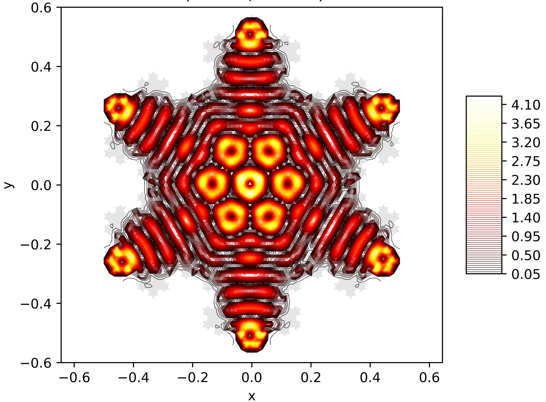
Contour Lines of the Energy Function of the 145. Eigenfunction on the Snowflake (Level 5, Res. 81) with Dirichlet BC
