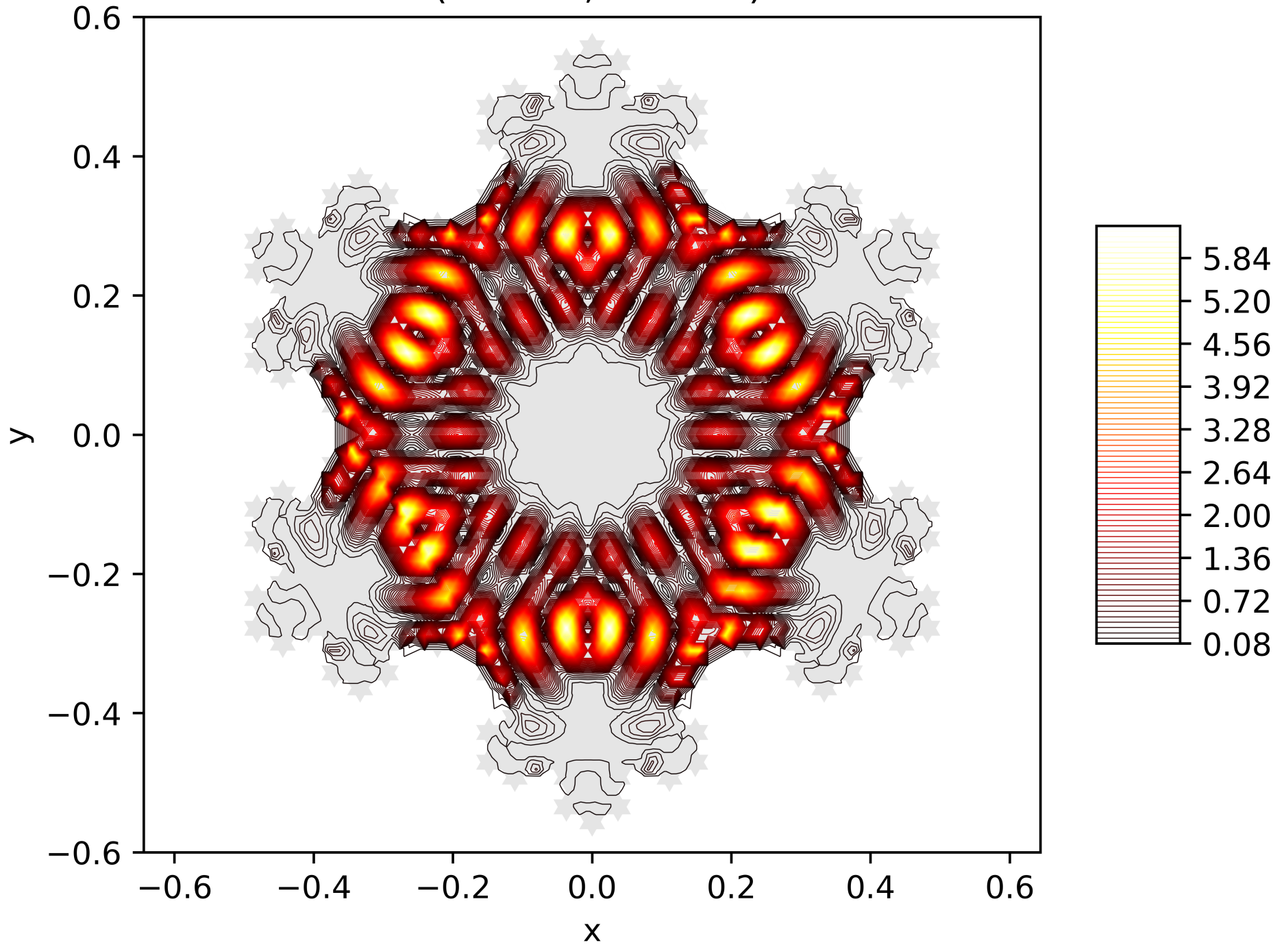
Contour Lines of the Energy Function of the 141. Eigenfunction on the Snowflake (Level 5, Res. 81) with Dirichlet BC
