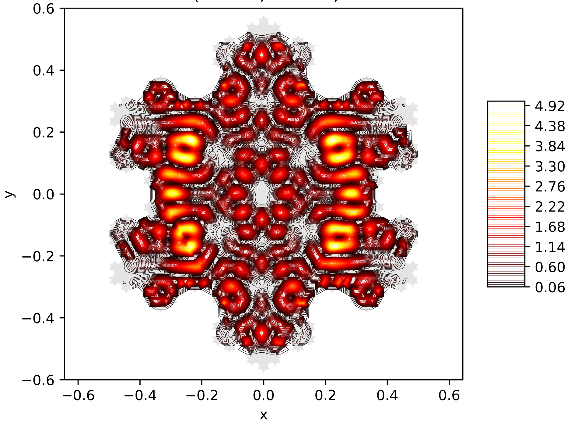
Contour Lines of the Energy Function of the 142. Eigenfunction on the Snowflake (Level 5, Res. 81) with Dirichlet BC
