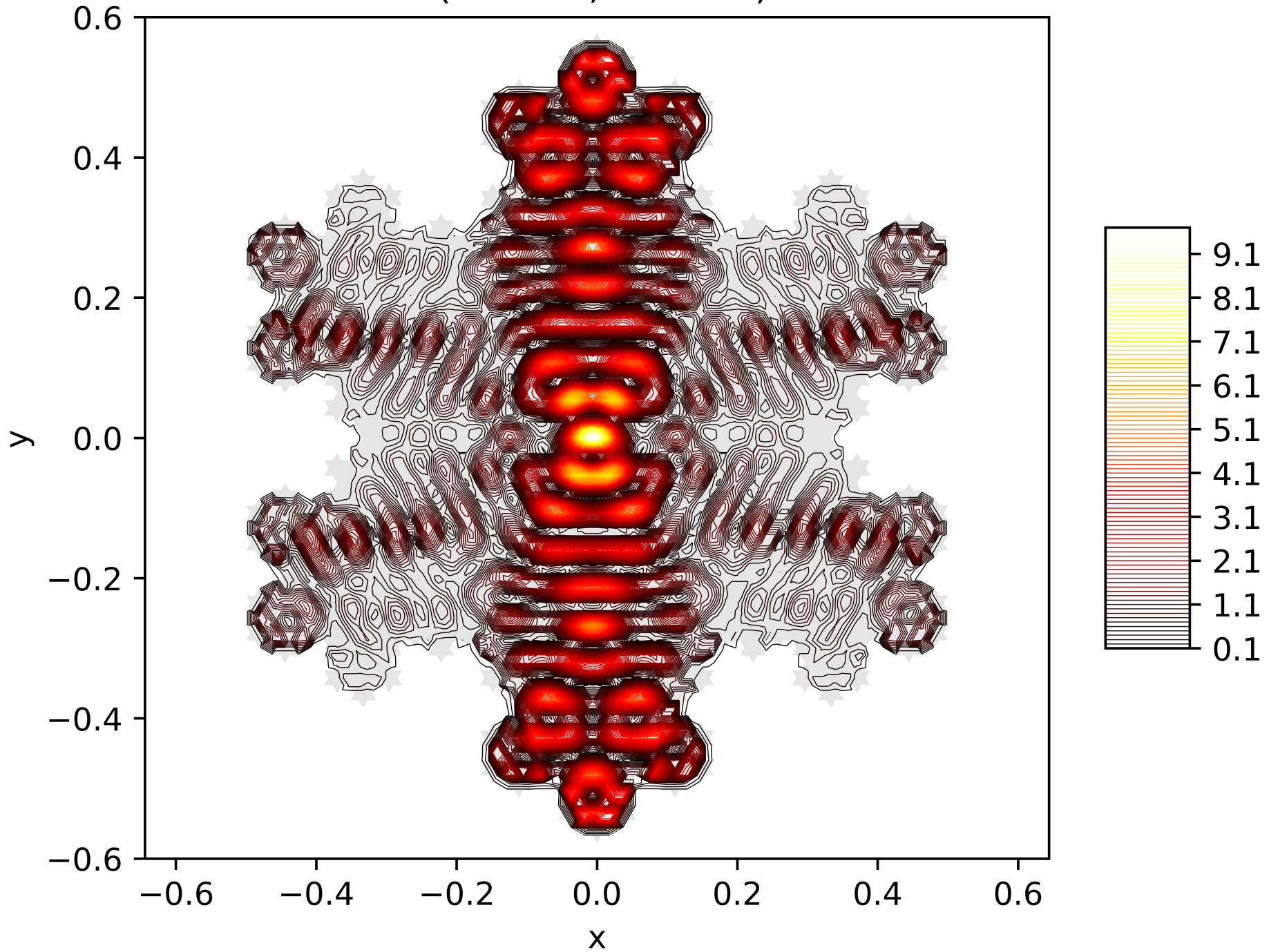
Contour Lines of the Energy Function of the 157. Eigenfunction on the Snowflake (Level 5, Res. 81) with Dirichlet BC
