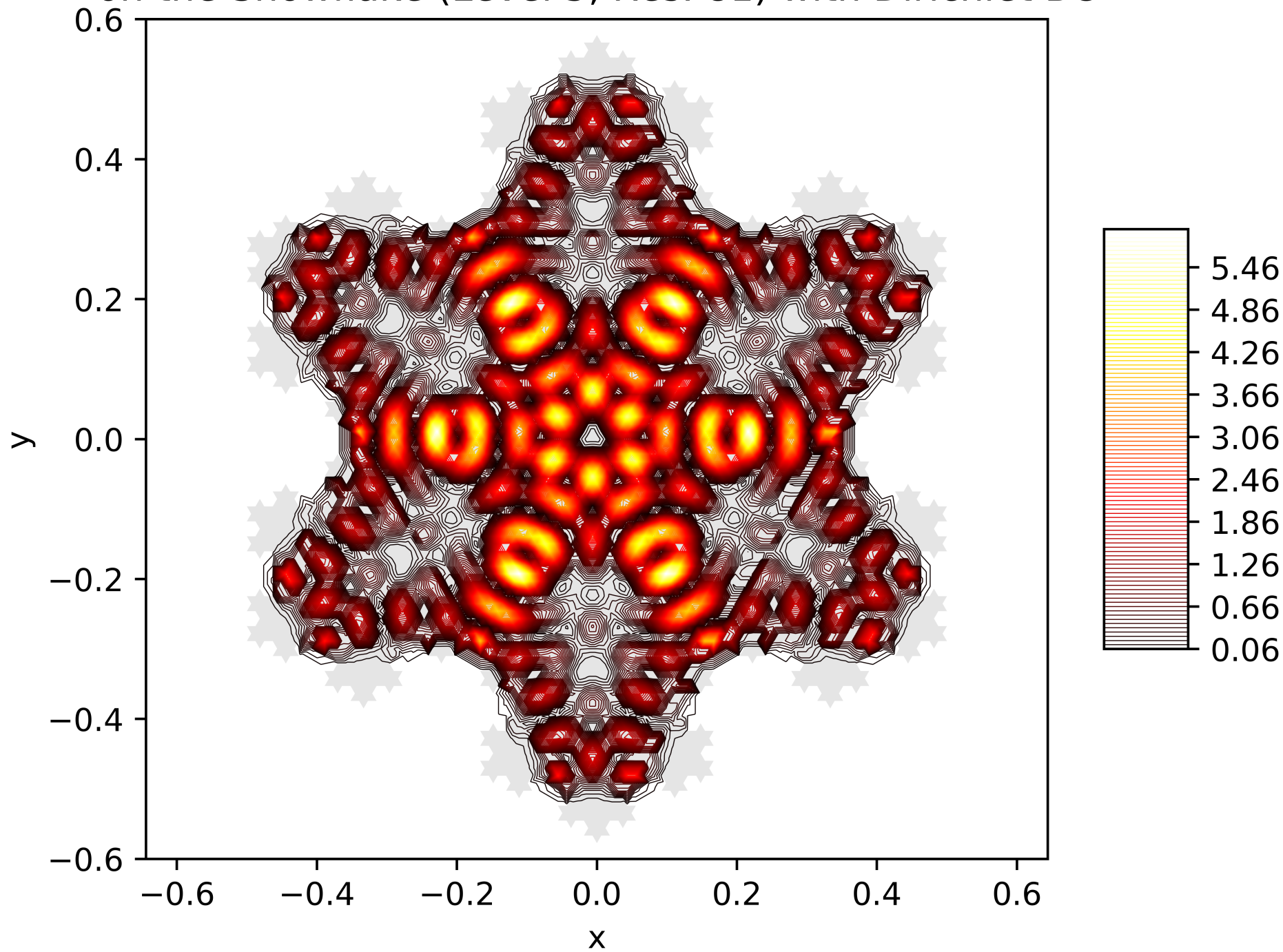
Contour Lines of the Energy Function of the 152. Eigenfunction on the Snowflake (Level 5, Res. 81) with Dirichlet BC
