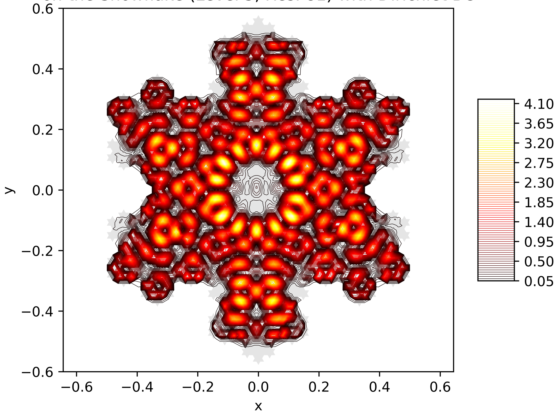
Contour Lines of the Energy Function of the 154. Eigenfunction on the Snowflake (Level 5, Res. 81) with Dirichlet BC
