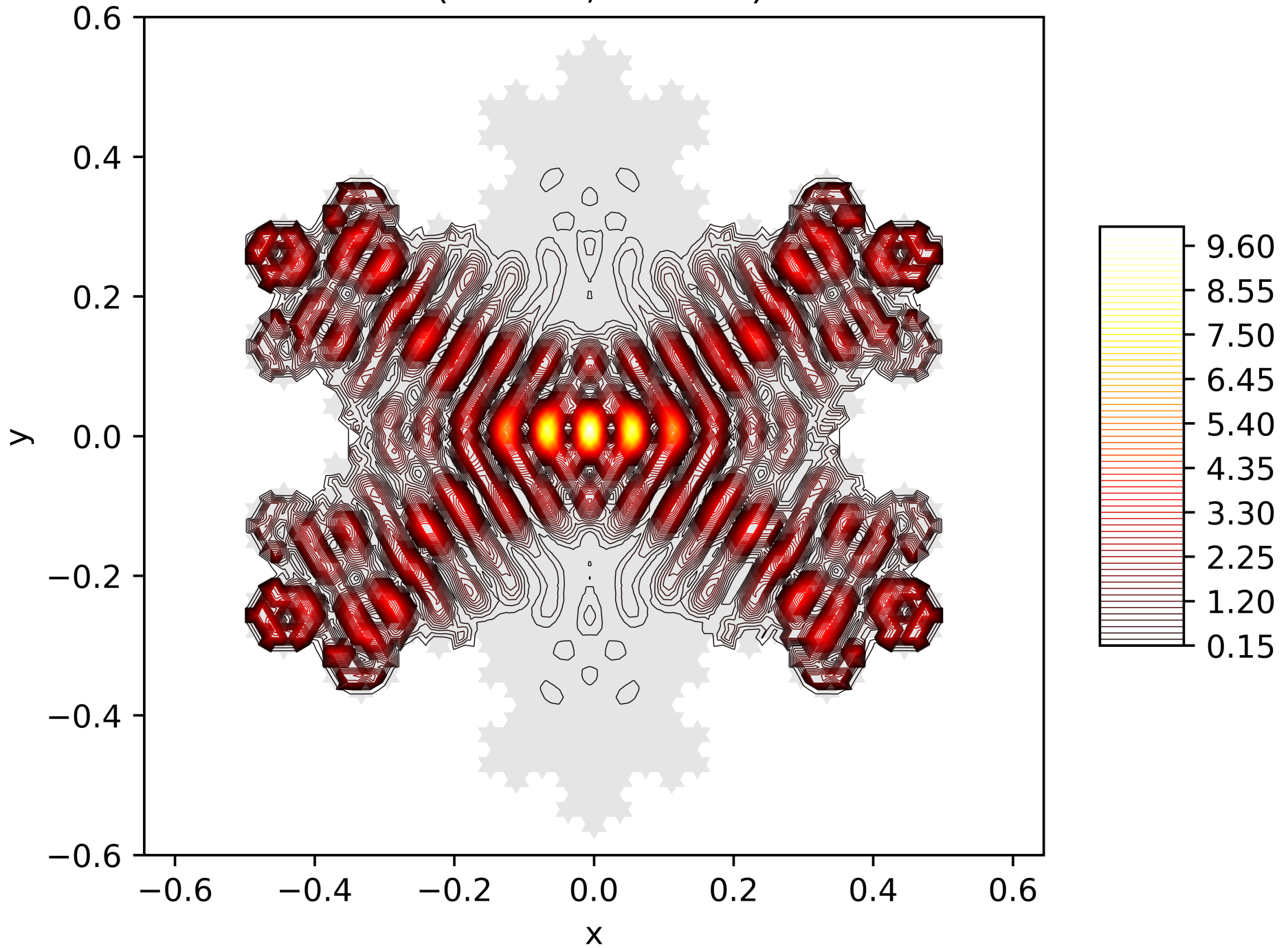
Contour Lines of the Energy Function of the 158. Eigenfunction on the Snowflake (Level 5, Res. 81) with Dirichlet BC
