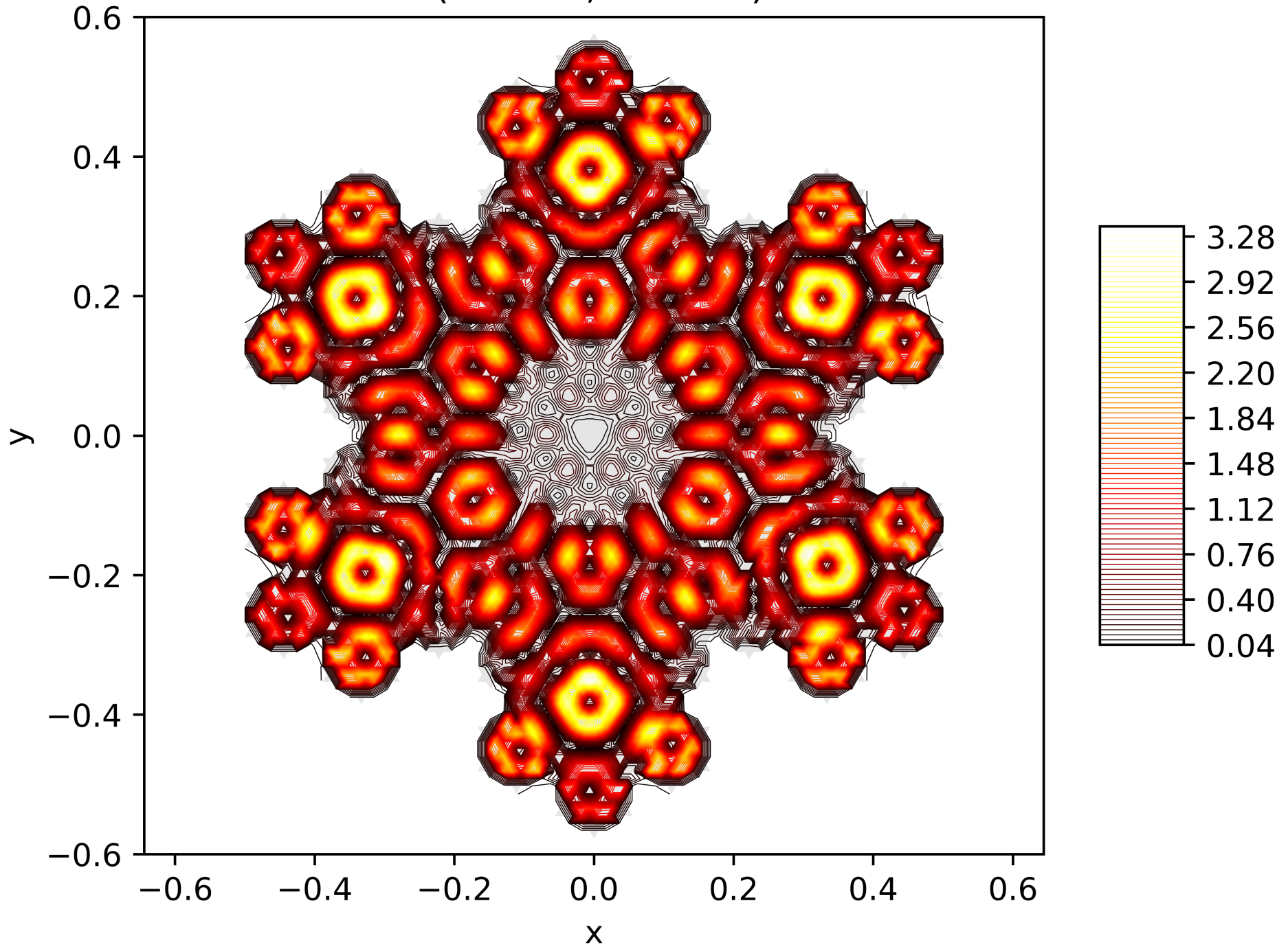
Contour Lines of the Energy Function of the 151. Eigenfunction on the Snowflake (Level 5, Res. 81) with Dirichlet BC
