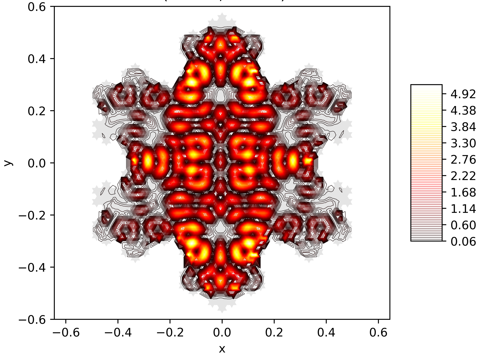
Contour Lines of the Energy Function of the 149. Eigenfunction on the Snowflake (Level 5, Res. 81) with Dirichlet BC
