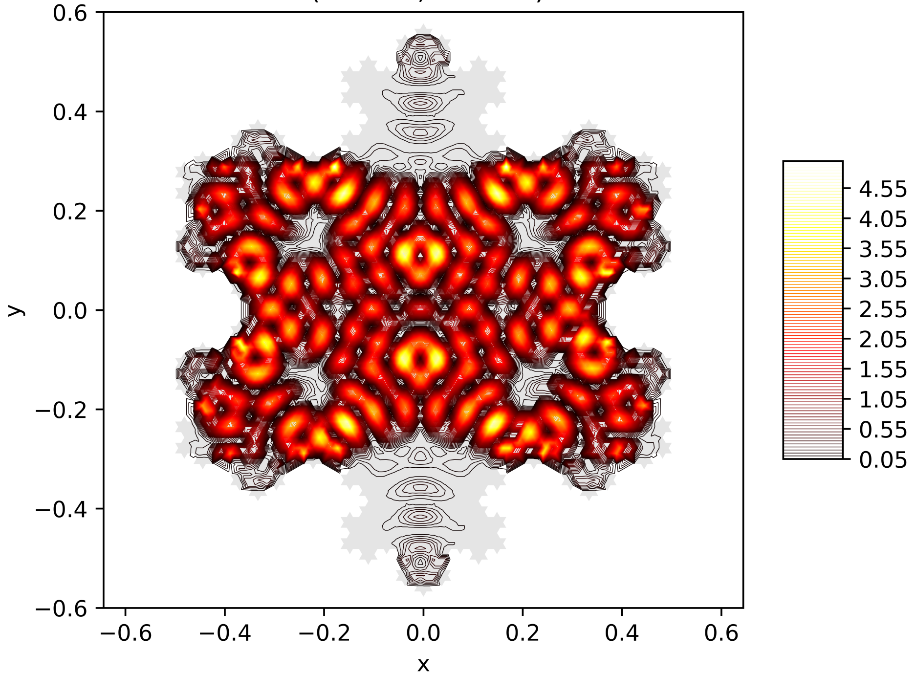
Contour Lines of the Energy Function of the 150. Eigenfunction on the Snowflake (Level 5, Res. 81) with Dirichlet BC
