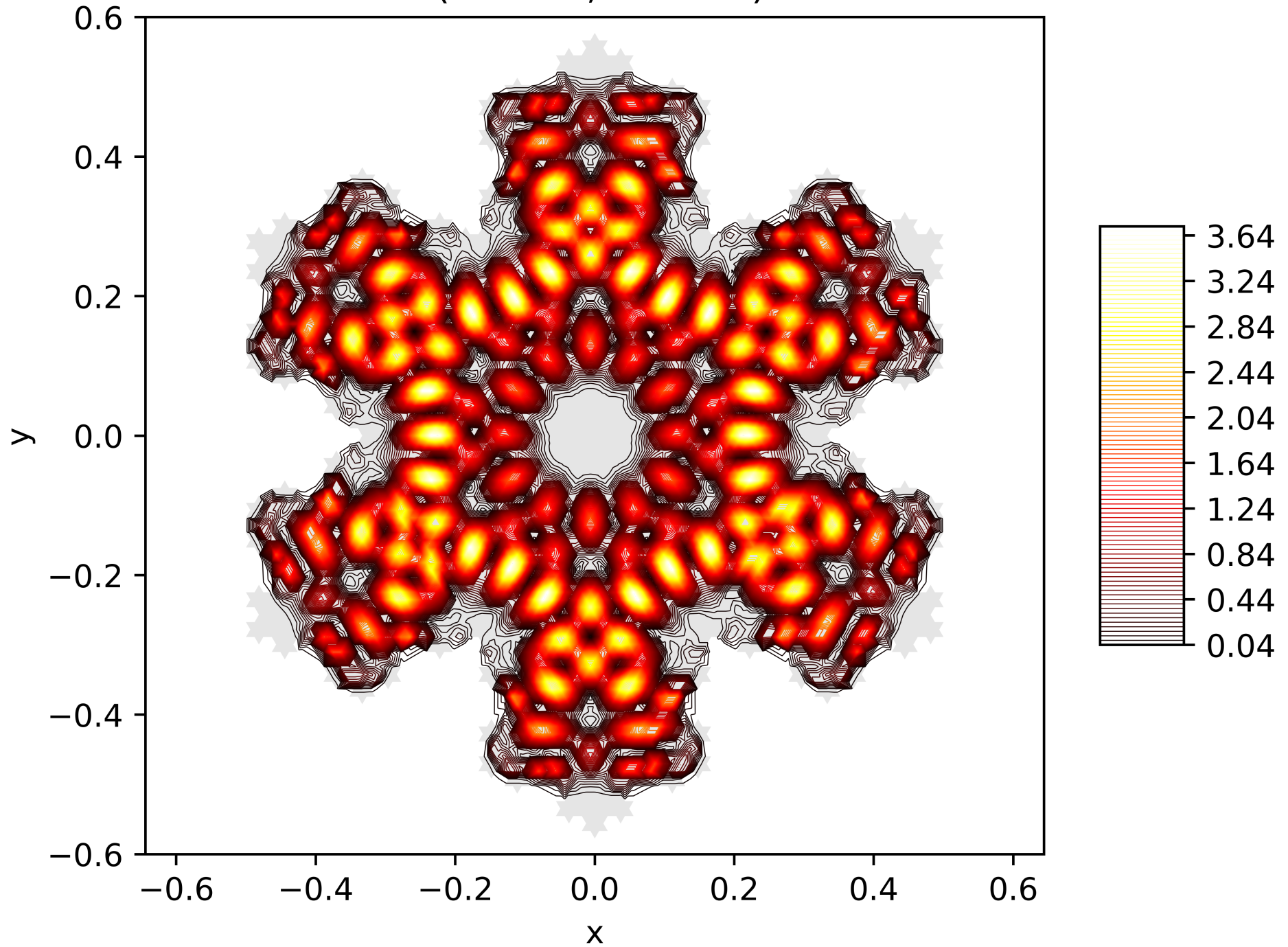
Contour Lines of the Energy Function of the 144. Eigenfunction on the Snowflake (Level 5, Res. 81) with Dirichlet BC
