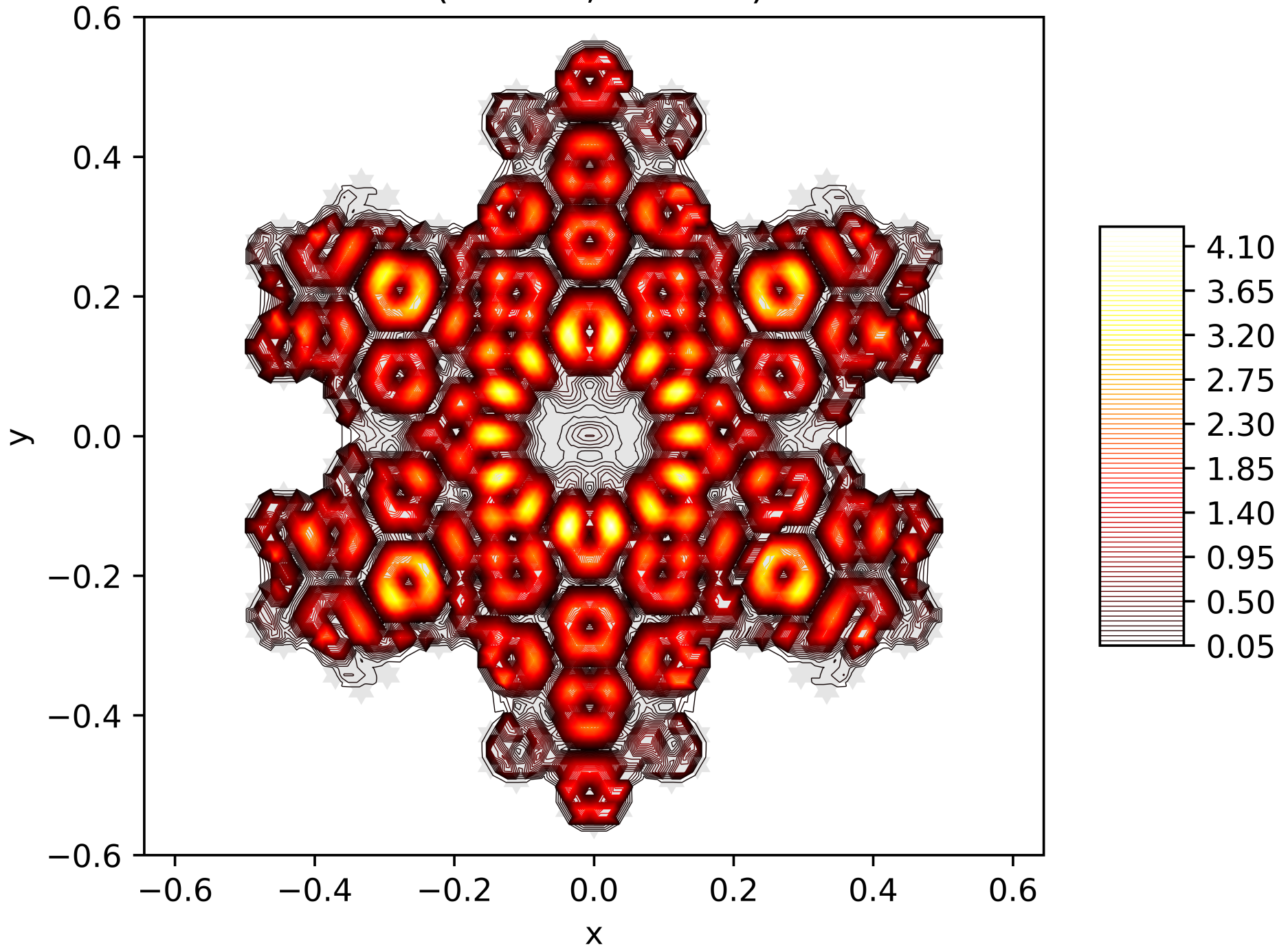
Contour Lines of the Energy Function of the 153. Eigenfunction on the Snowflake (Level 5, Res. 81) with Dirichlet BC
