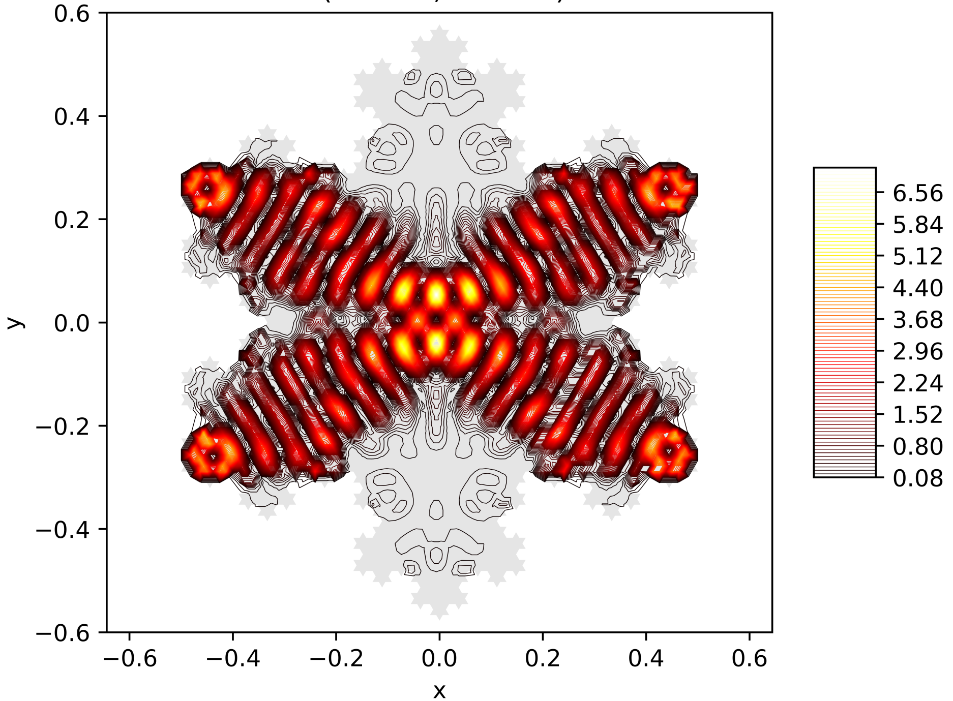
Contour Lines of the Energy Function of the 147. Eigenfunction on the Snowflake (Level 5, Res. 81) with Dirichlet BC
