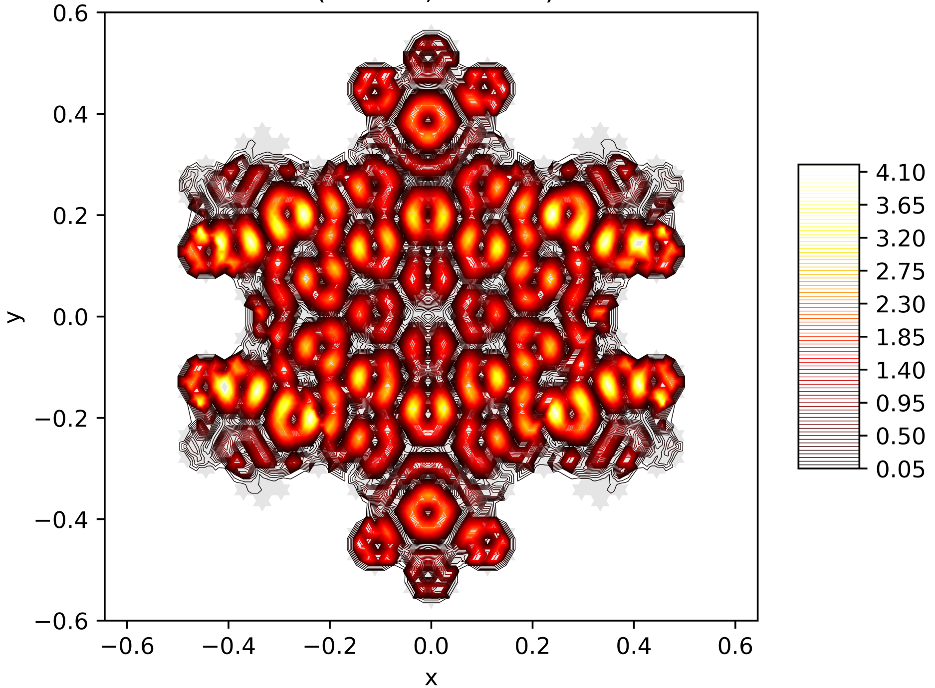
Contour Lines of the Energy Function of the 155. Eigenfunction on the Snowflake (Level 5, Res. 81) with Dirichlet BC
