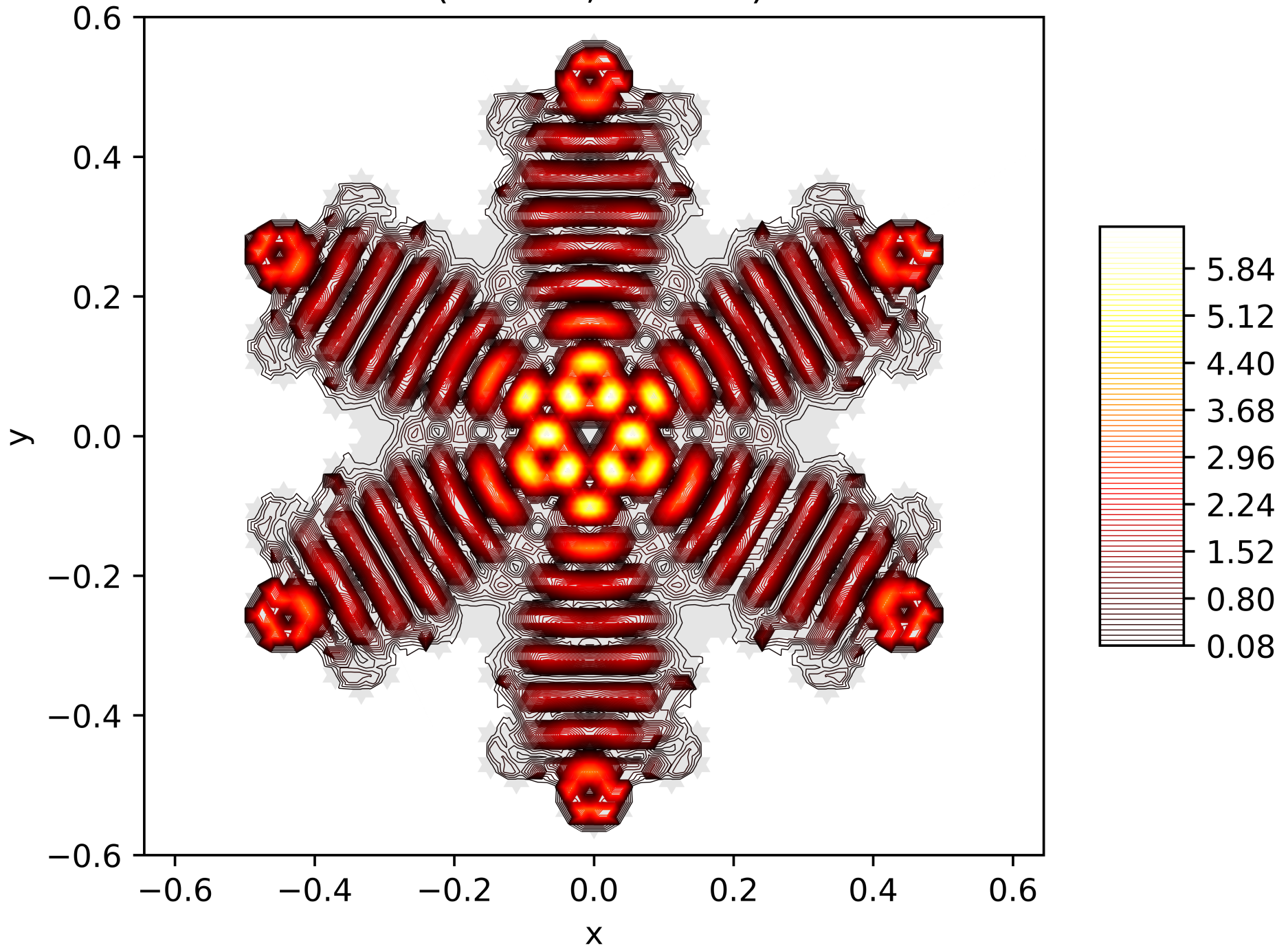
Contour Lines of the Energy Function of the 159. Eigenfunction on the Snowflake (Level 5, Res. 81) with Dirichlet BC
