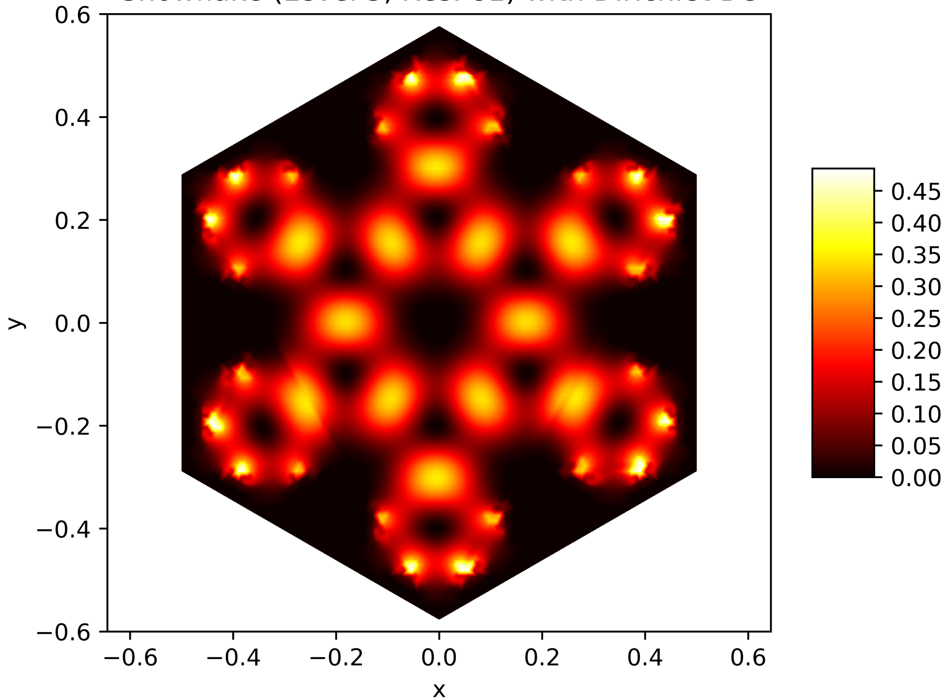
Energy Function of the 14. Eigenfunction on the Snowflake (Level 5, Res. 81) with Dirichlet BC
