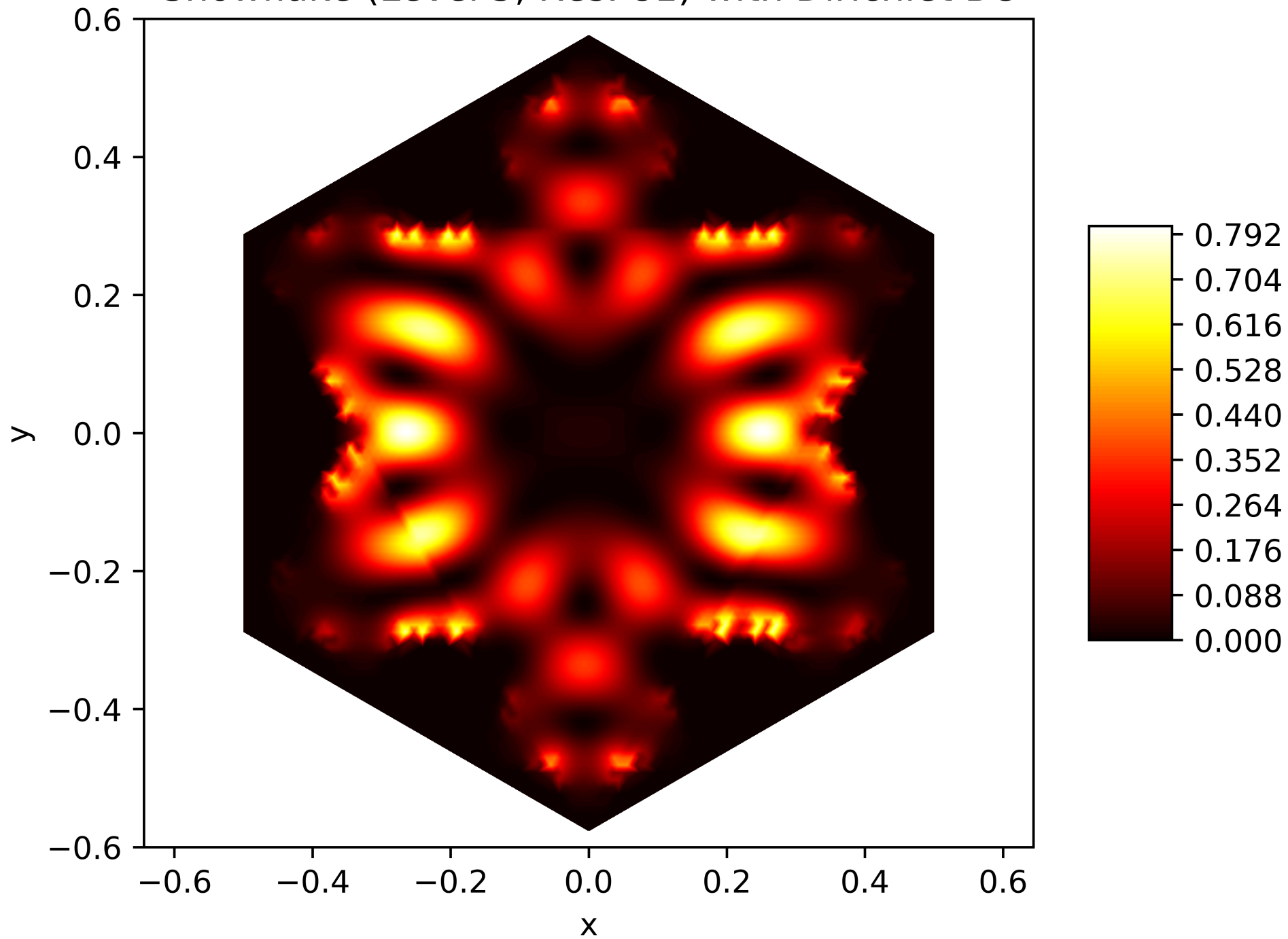
Energy Function of the 20. Eigenfunction on the Snowflake (Level 5, Res. 81) with Dirichlet BC
