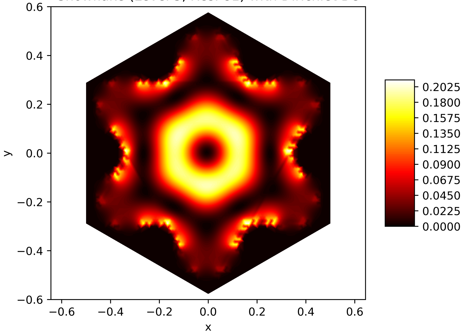
Energy Function of the 6. Eigenfunction on the Snowflake (Level 5, Res. 81) with Dirichlet BC
