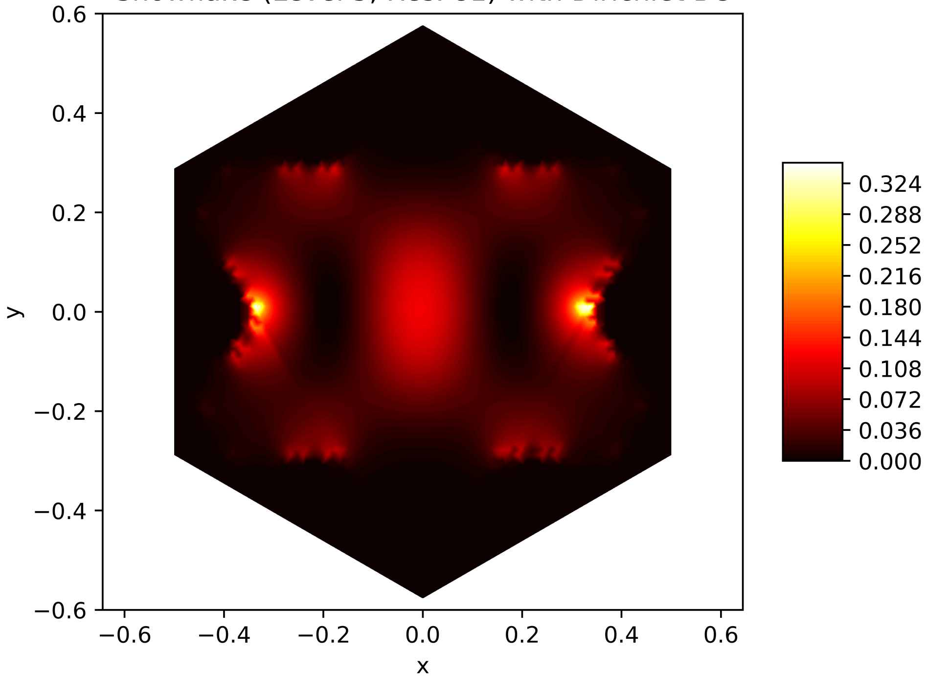
Energy Function of the 3. Eigenfunction on the Snowflake (Level 5, Res. 81) with Dirichlet BC
