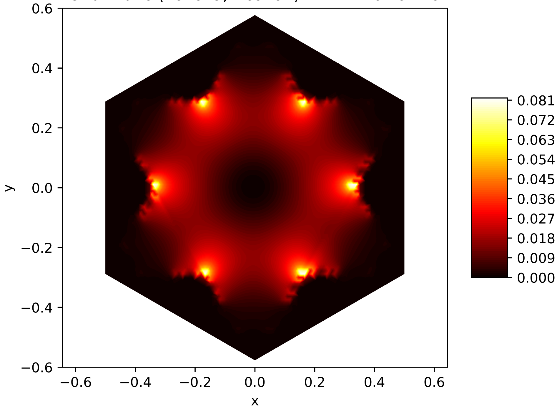
Energy Function of the 1. Eigenfunction on the Snowflake (Level 5, Res. 81) with Dirichlet BC
