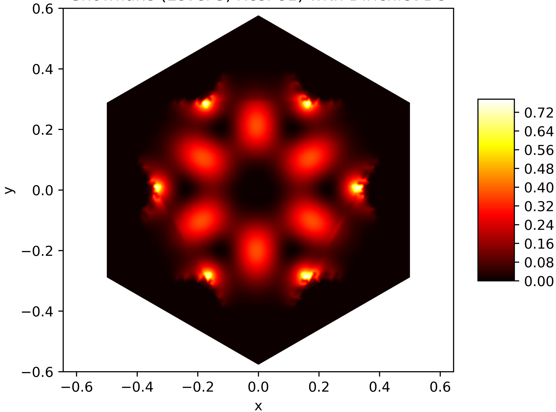
Energy Function of the 10. Eigenfunction on the Snowflake (Level 5, Res. 81) with Dirichlet BC
