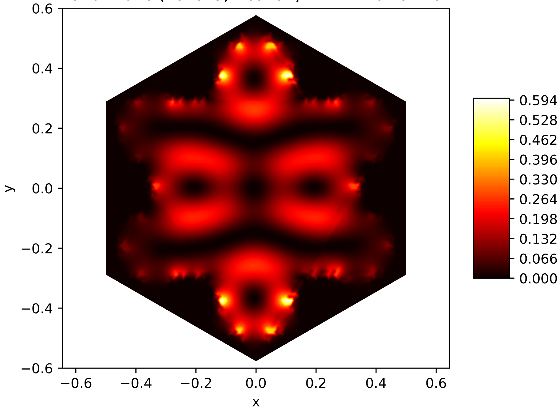
Energy Function of the 11. Eigenfunction on the Snowflake (Level 5, Res. 81) with Dirichlet BC
