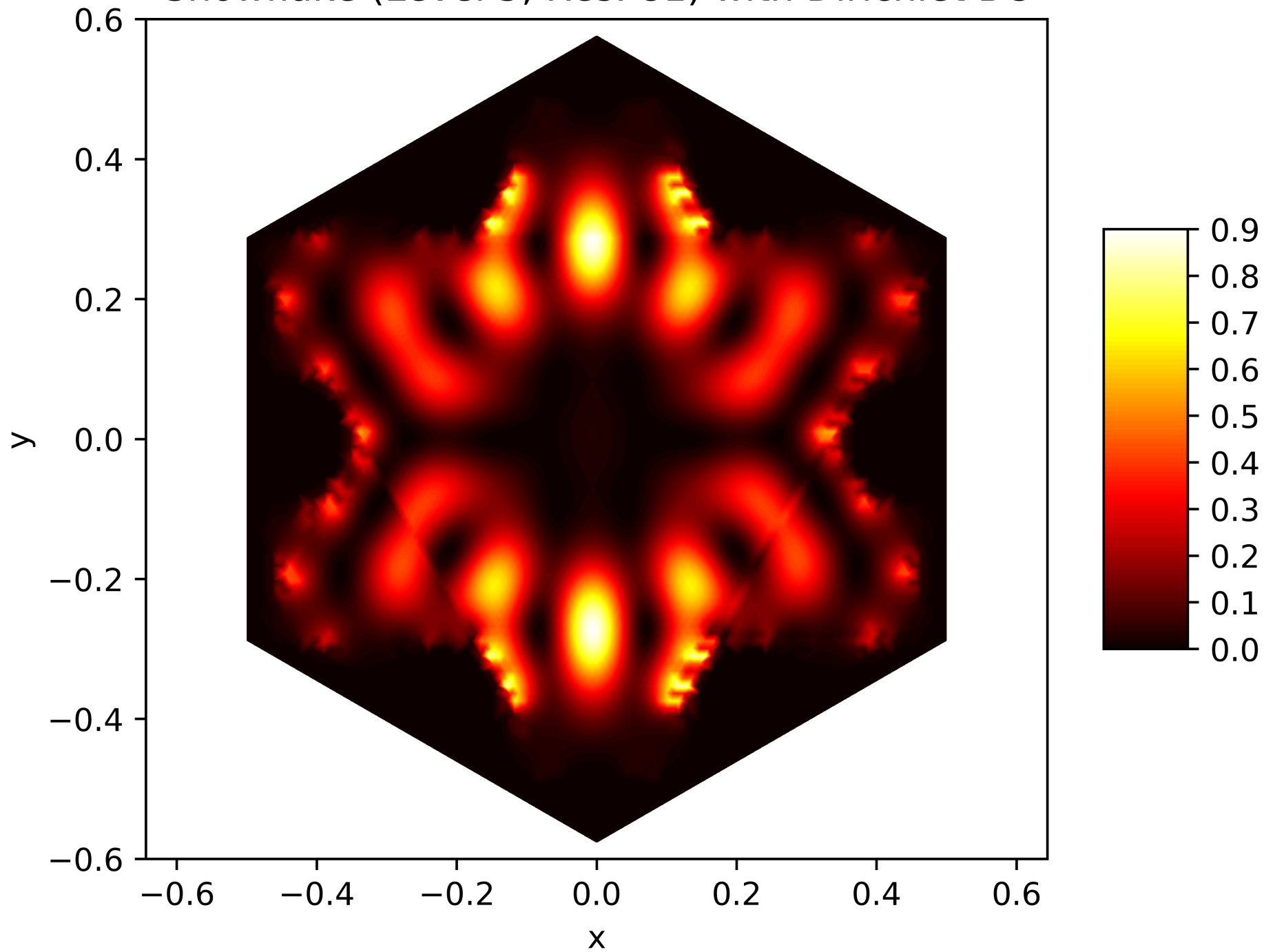
Energy Function of the 19. Eigenfunction on the Snowflake (Level 5, Res. 81) with Dirichlet BC
