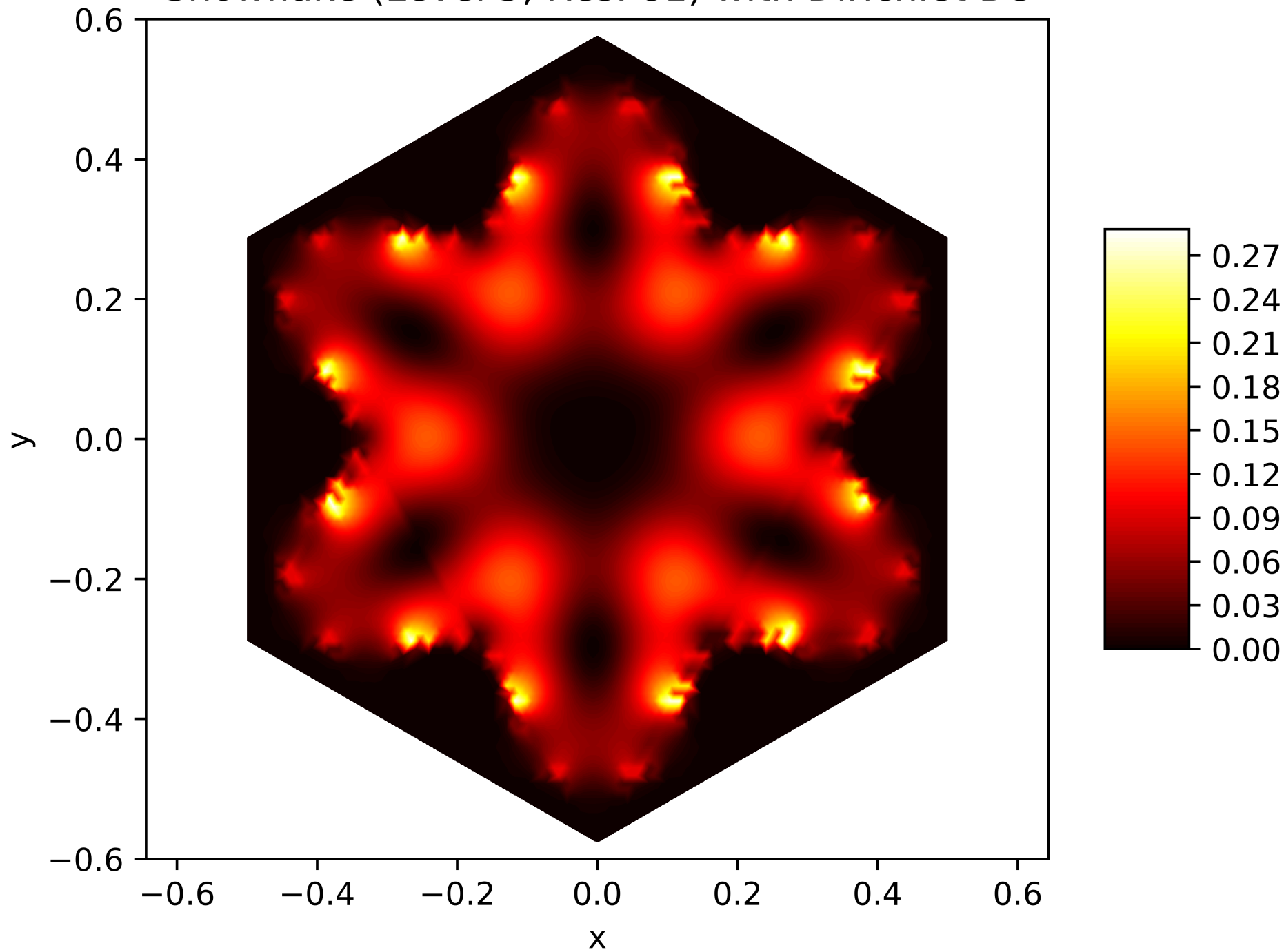
Energy Function of the 7. Eigenfunction on the Snowflake (Level 5, Res. 81) with Dirichlet BC
