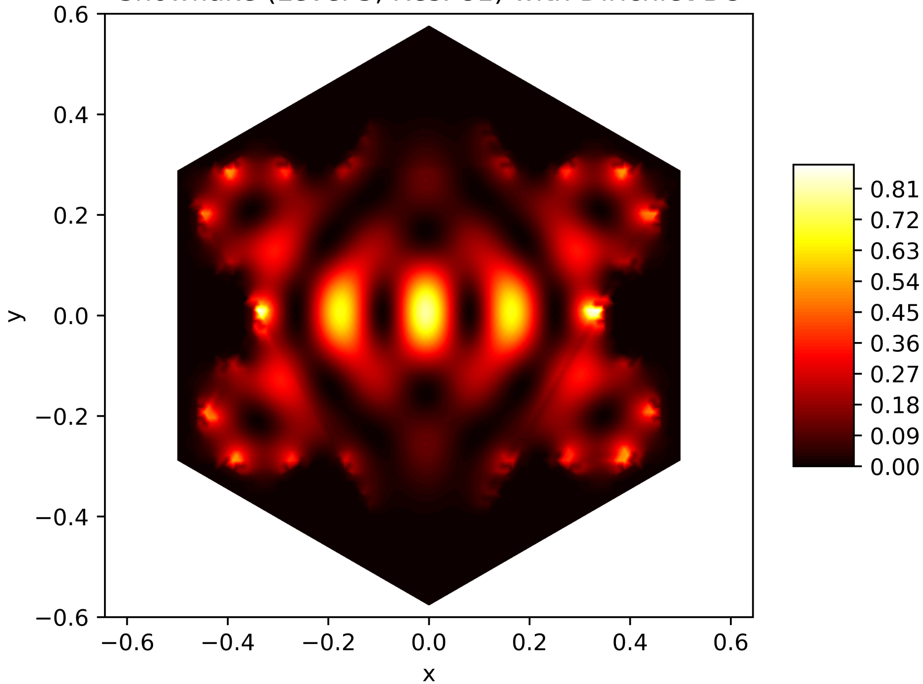
Energy Function of the 16. Eigenfunction on the Snowflake (Level 5, Res. 81) with Dirichlet BC
