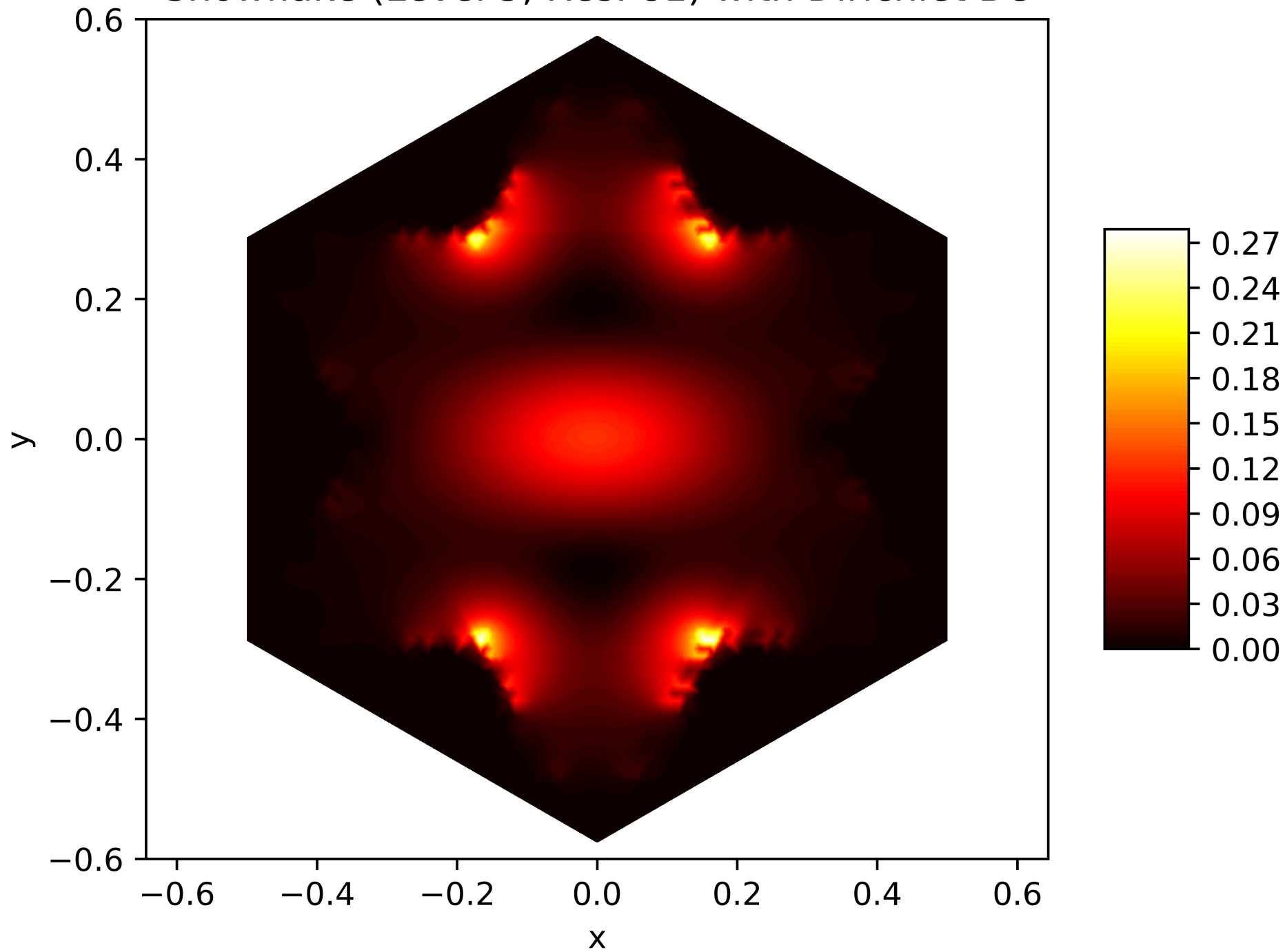
Energy Function of the 2. Eigenfunction on the Snowflake (Level 5, Res. 81) with Dirichlet BC
