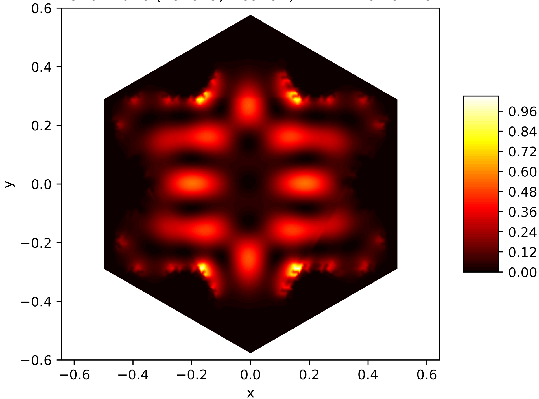
Energy Function of the 17. Eigenfunction on the Snowflake (Level 5, Res. 81) with Dirichlet BC
