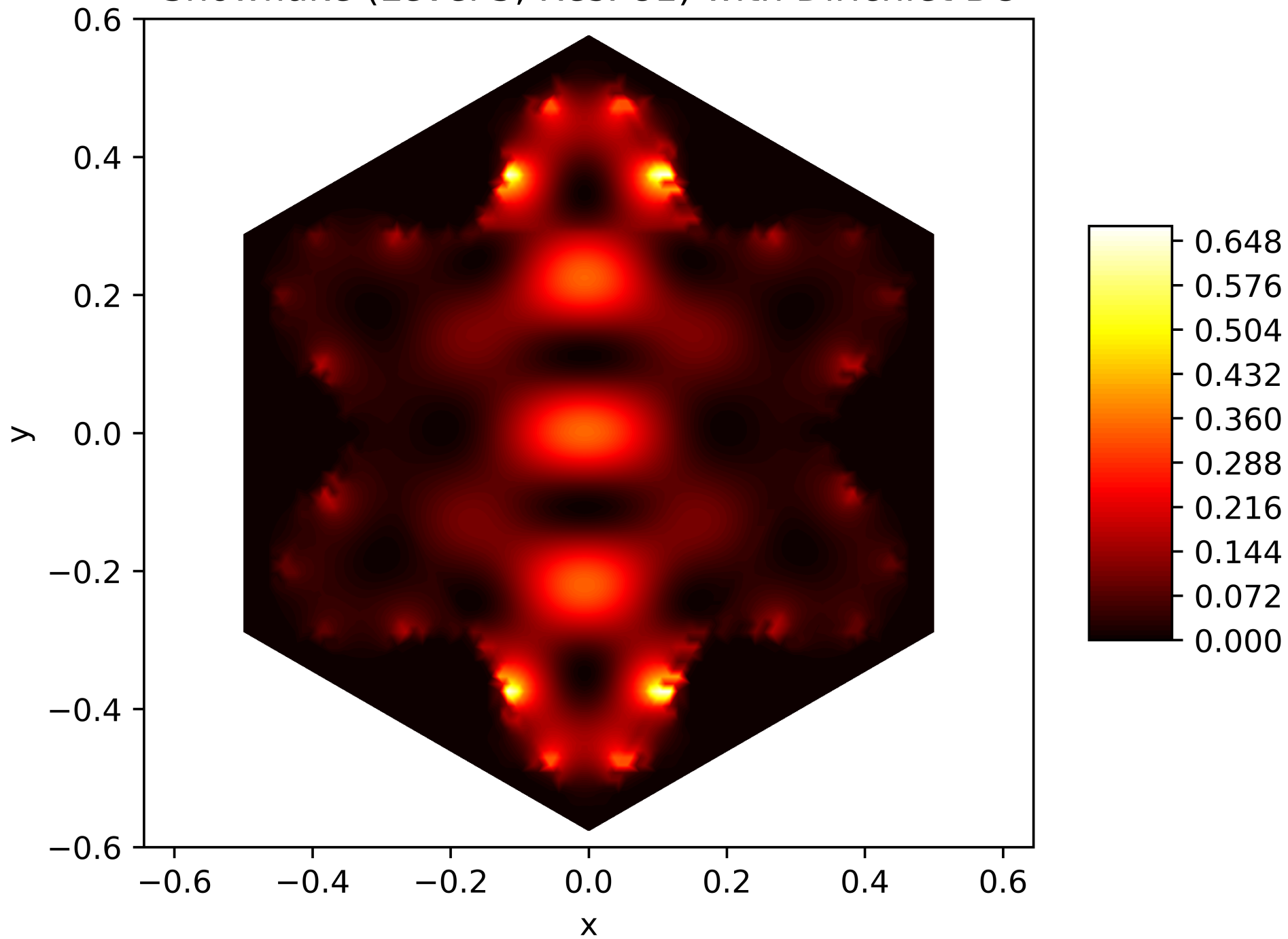
Energy Function of the 8. Eigenfunction on the Snowflake (Level 5, Res. 81) with Dirichlet BC
