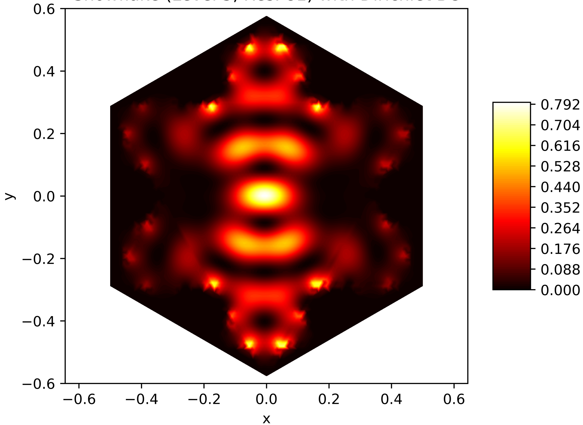
Energy Function of the 15. Eigenfunction on the Snowflake (Level 5, Res. 81) with Dirichlet BC
