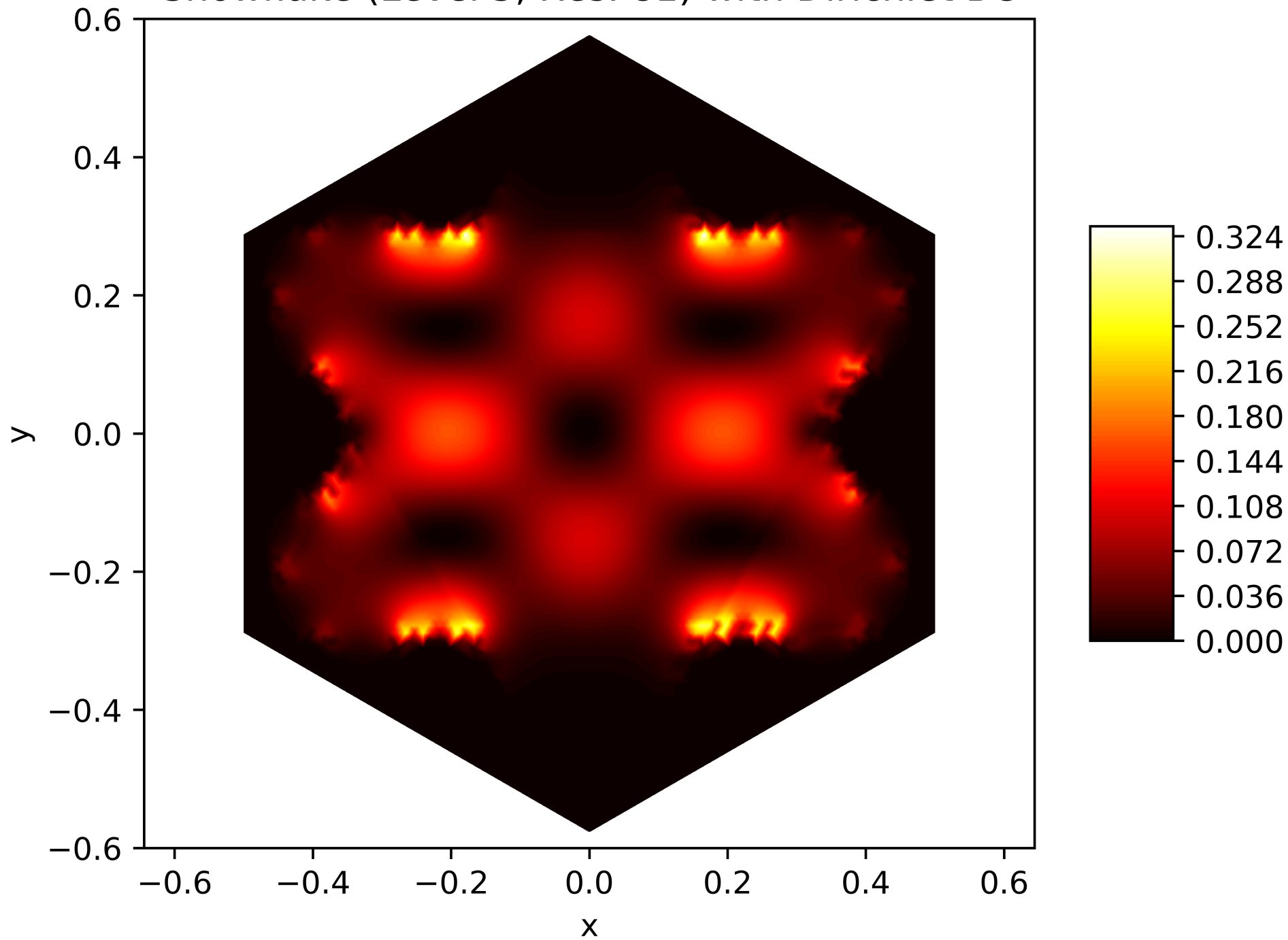
Energy Function of the 5. Eigenfunction on the Snowflake (Level 5, Res. 81) with Dirichlet BC
