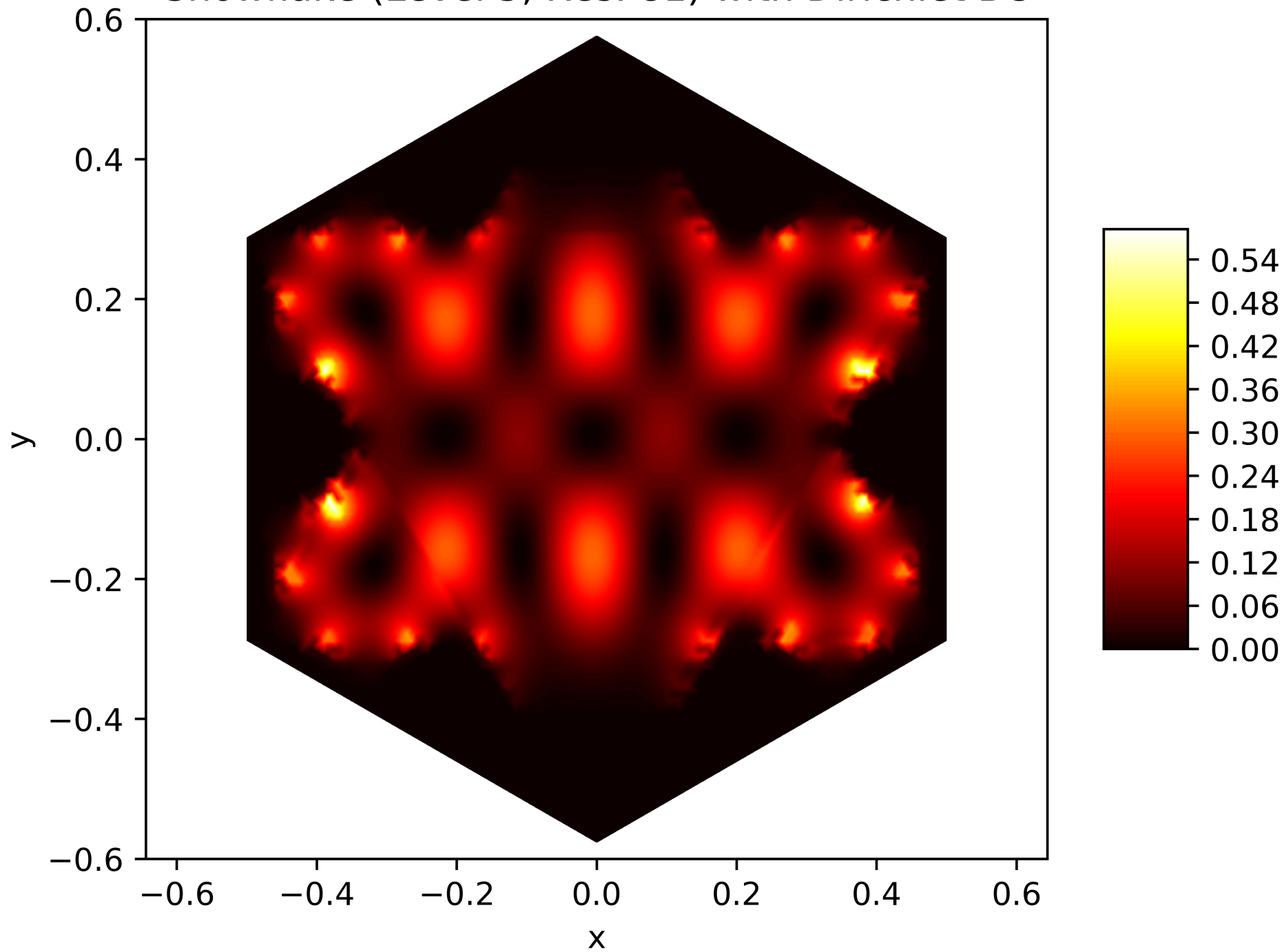
Energy Function of the 12. Eigenfunction on the Snowflake (Level 5, Res. 81) with Dirichlet BC
