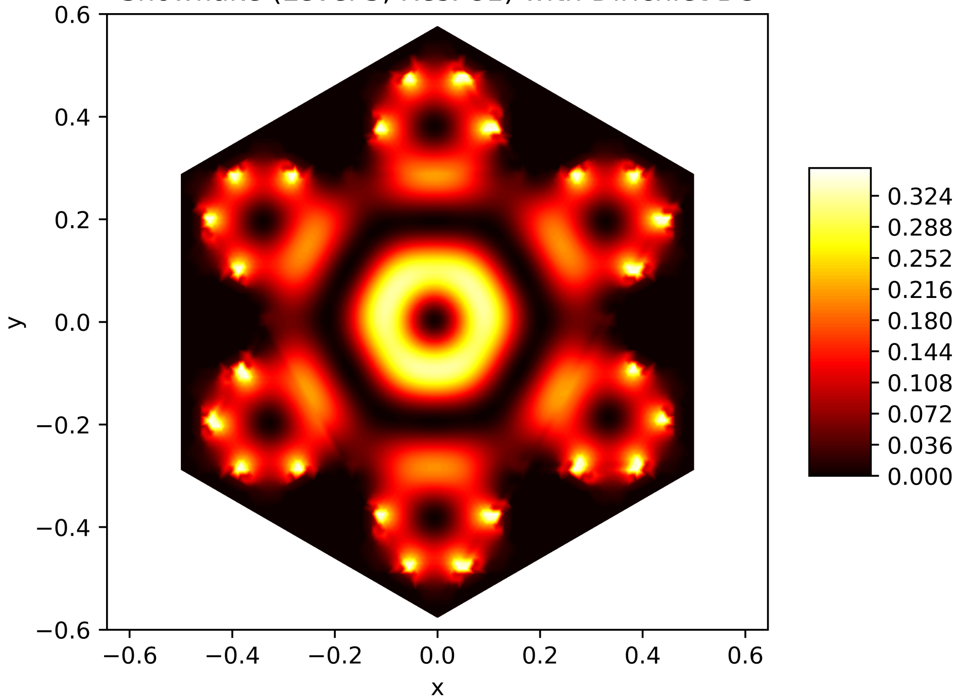
Energy Function of the 13. Eigenfunction on the Snowflake (Level 5, Res. 81) with Dirichlet BC
