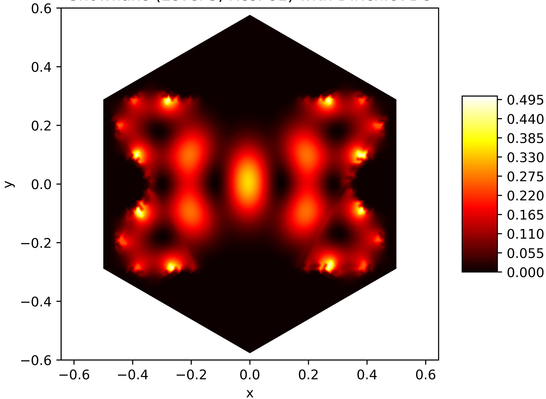
Energy Function of the 9. Eigenfunction on the Snowflake (Level 5, Res. 81) with Dirichlet BC
