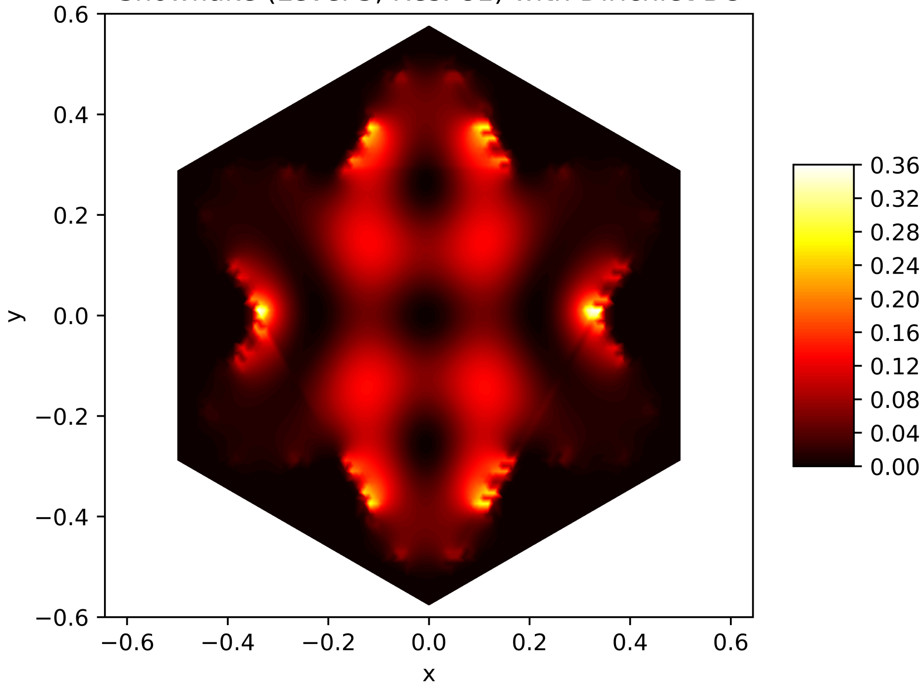
Energy Function of the 4. Eigenfunction on the Snowflake (Level 5, Res. 81) with Dirichlet BC
