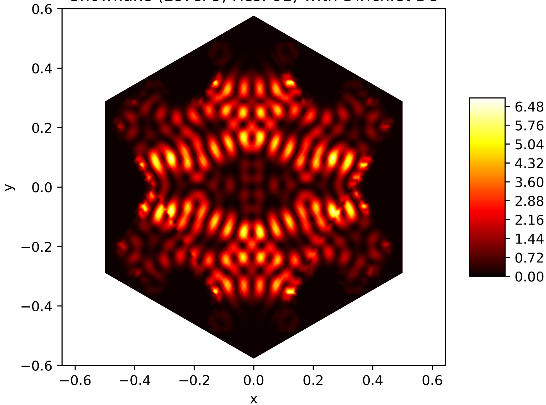
Energy Function of the 196. Eigenfunction on the Snowflake (Level 5, Res. 81) with Dirichlet BC
