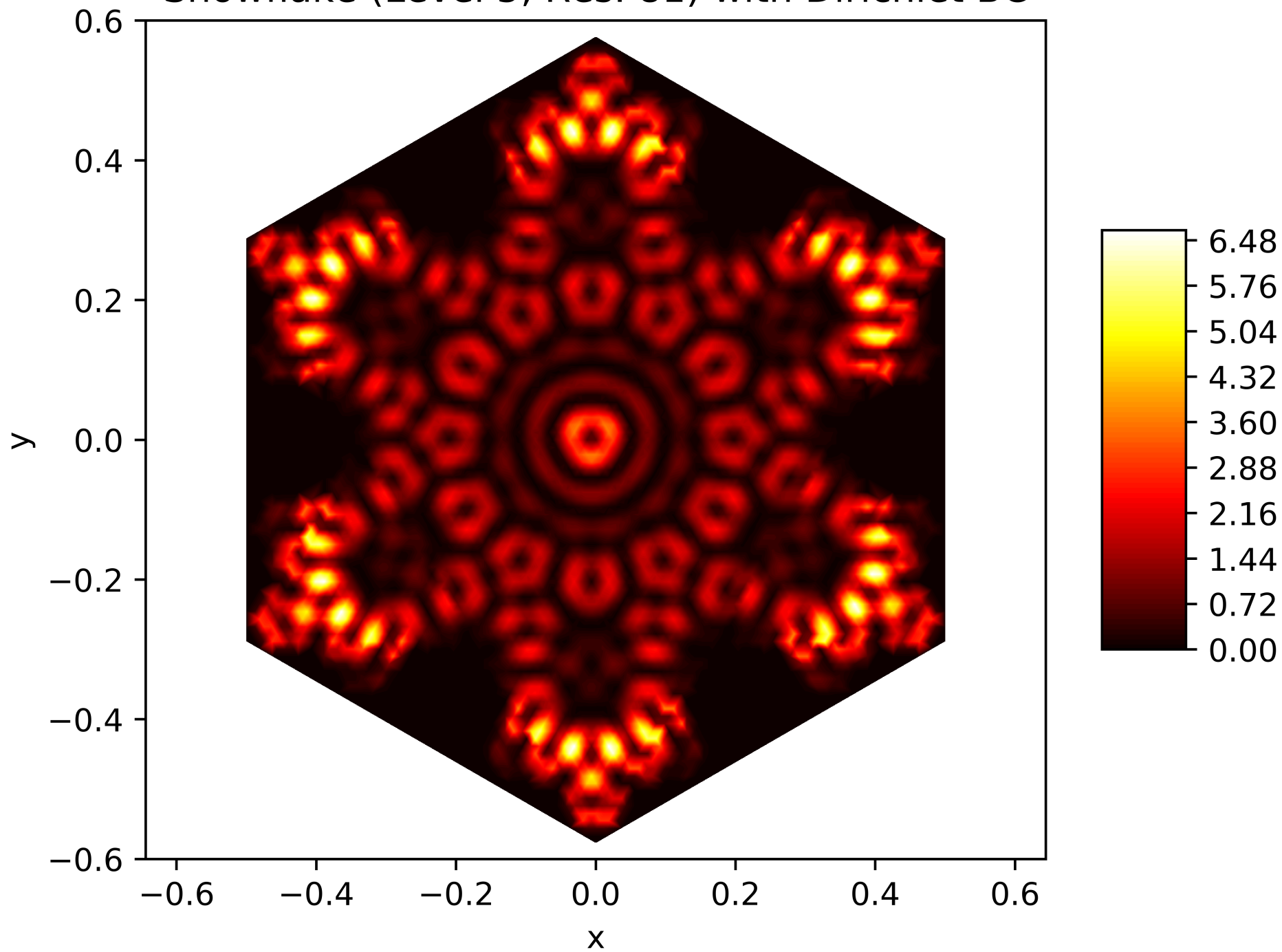
Energy Function of the 199. Eigenfunction on the Snowflake (Level 5, Res. 81) with Dirichlet BC
