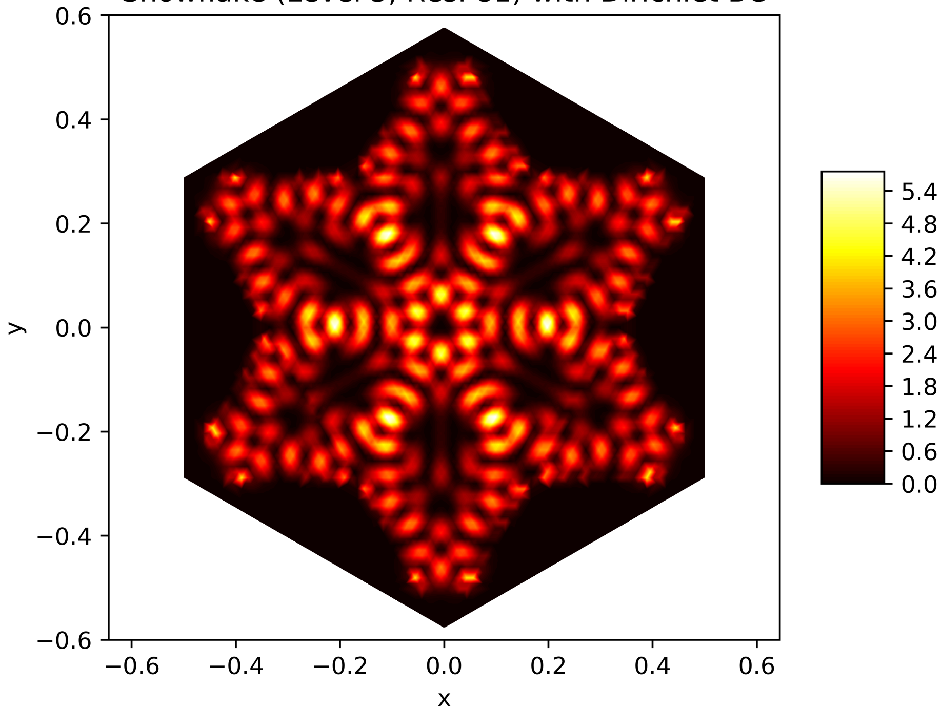
Energy Function of the 187. Eigenfunction on the Snowflake (Level 5, Res. 81) with Dirichlet BC
