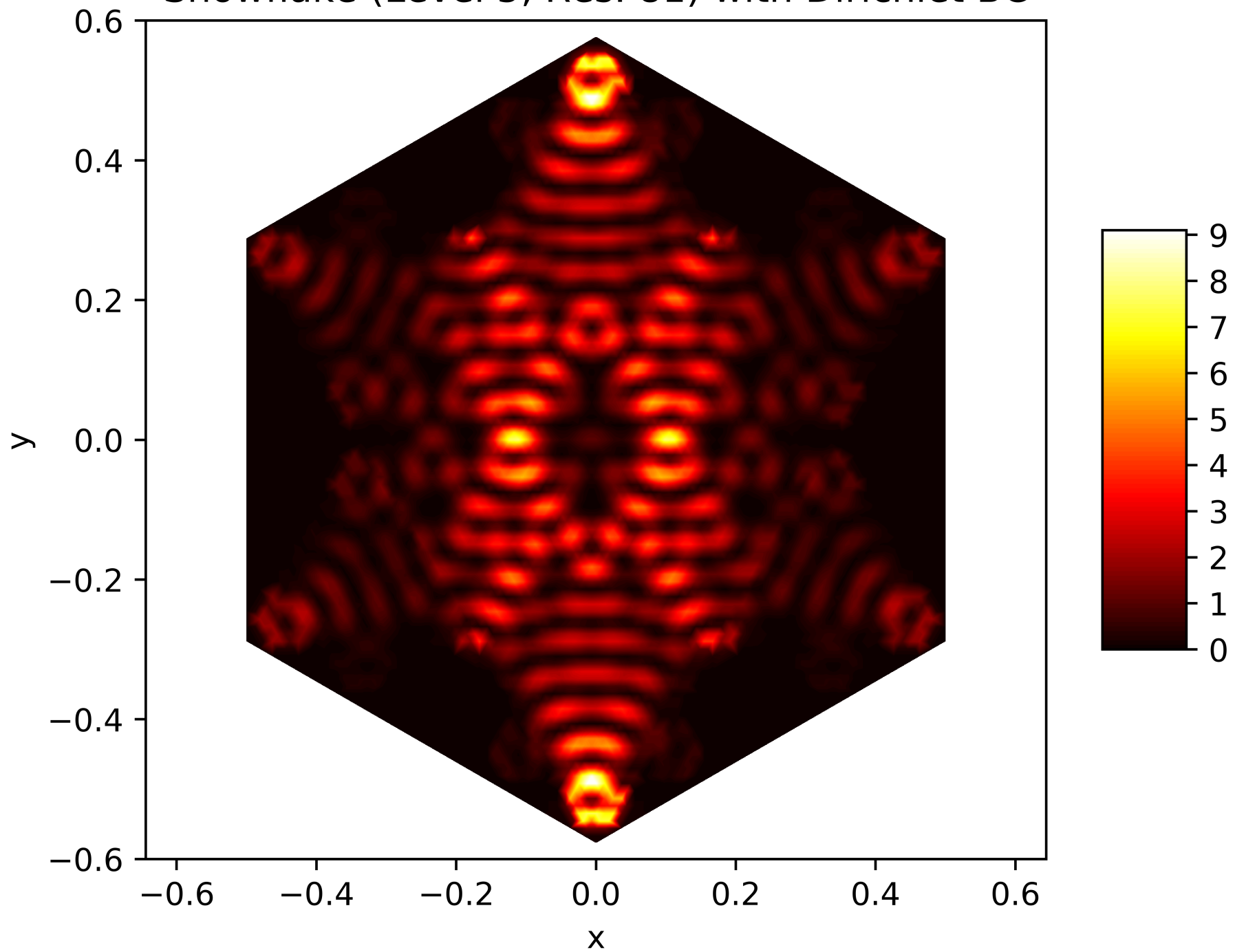
Energy Function of the 189. Eigenfunction on the Snowflake (Level 5, Res. 81) with Dirichlet BC
