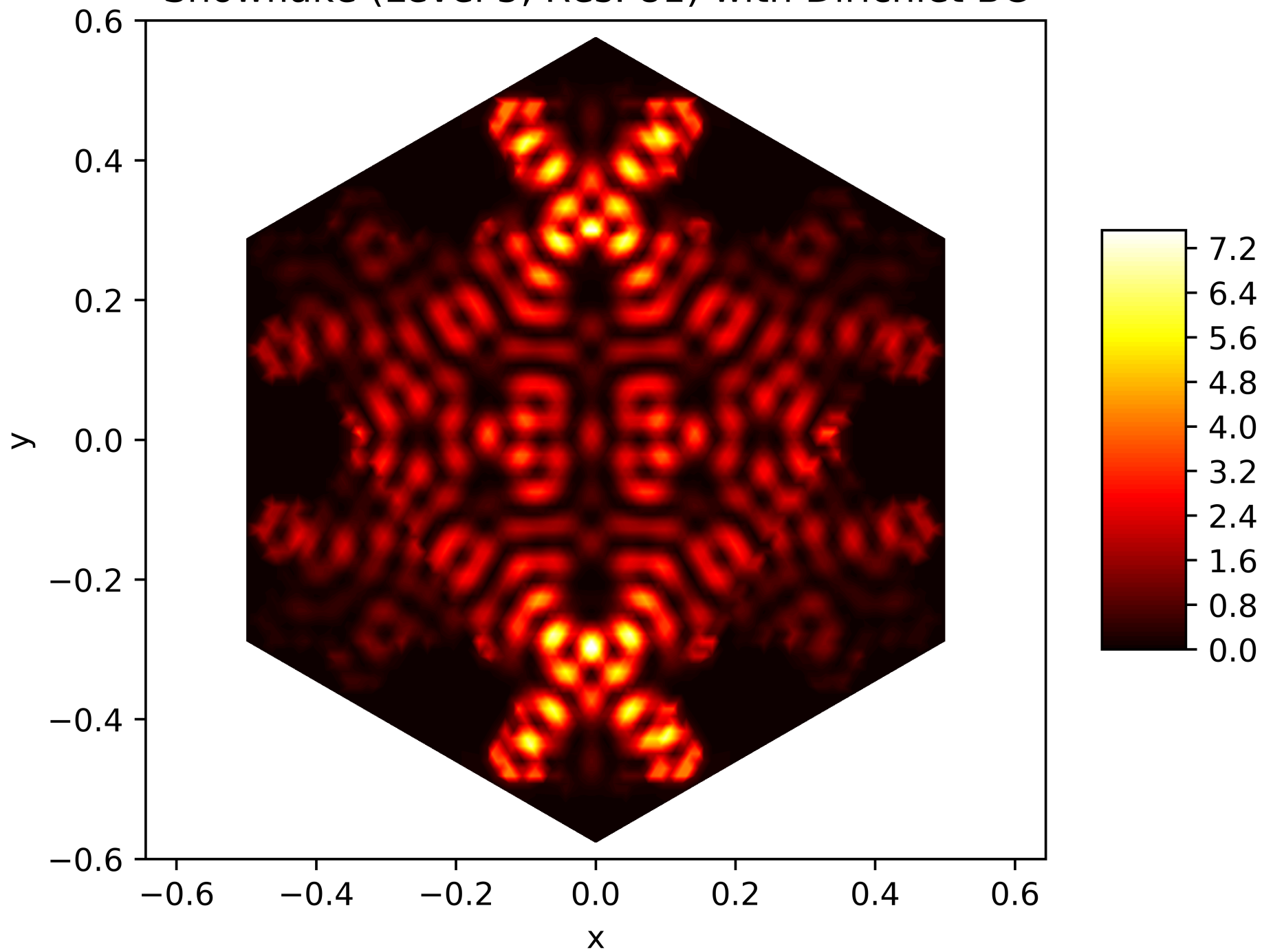
Energy Function of the 193. Eigenfunction on the Snowflake (Level 5, Res. 81) with Dirichlet BC
