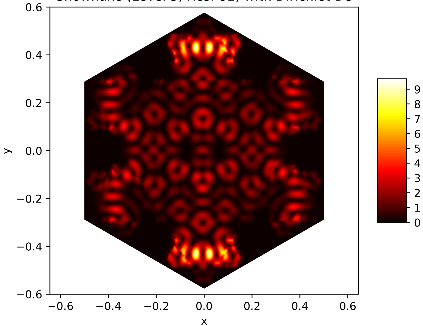
Energy Function of the 185. Eigenfunction on the Snowflake (Level 5, Res. 81) with Dirichlet BC
