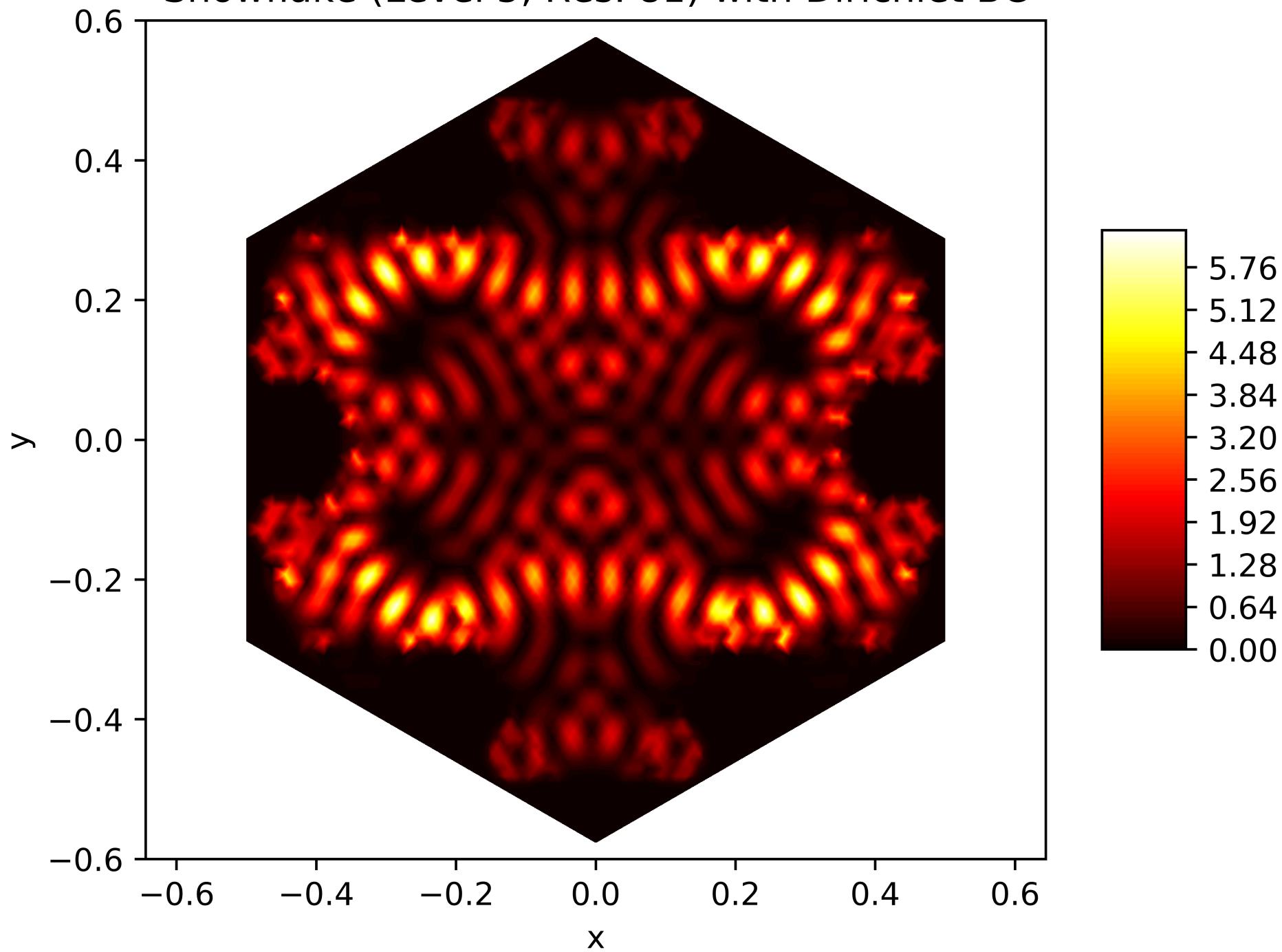
Energy Function of the 181. Eigenfunction on the Snowflake (Level 5, Res. 81) with Dirichlet BC
