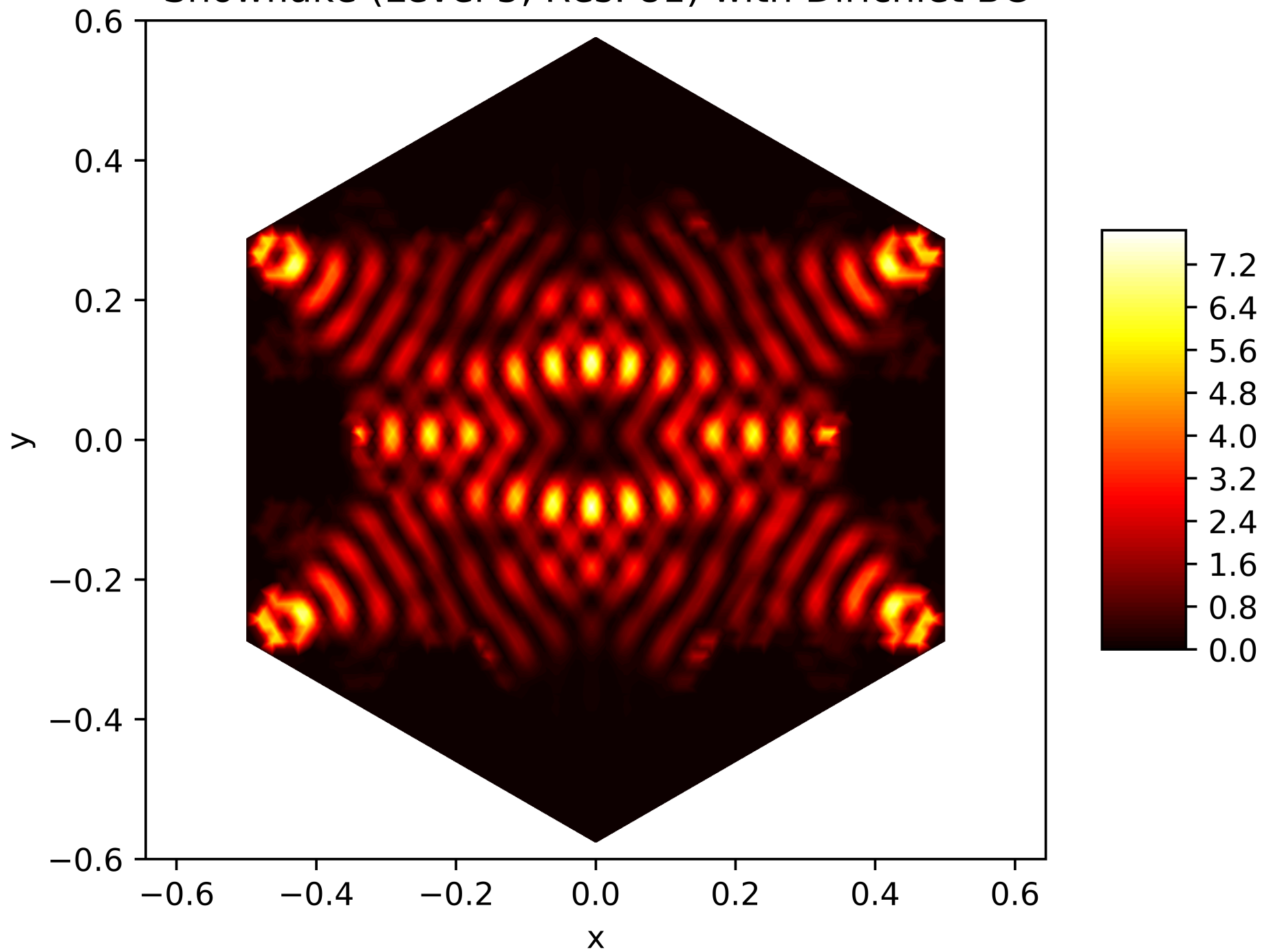
Energy Function of the 190. Eigenfunction on the Snowflake (Level 5, Res. 81) with Dirichlet BC
