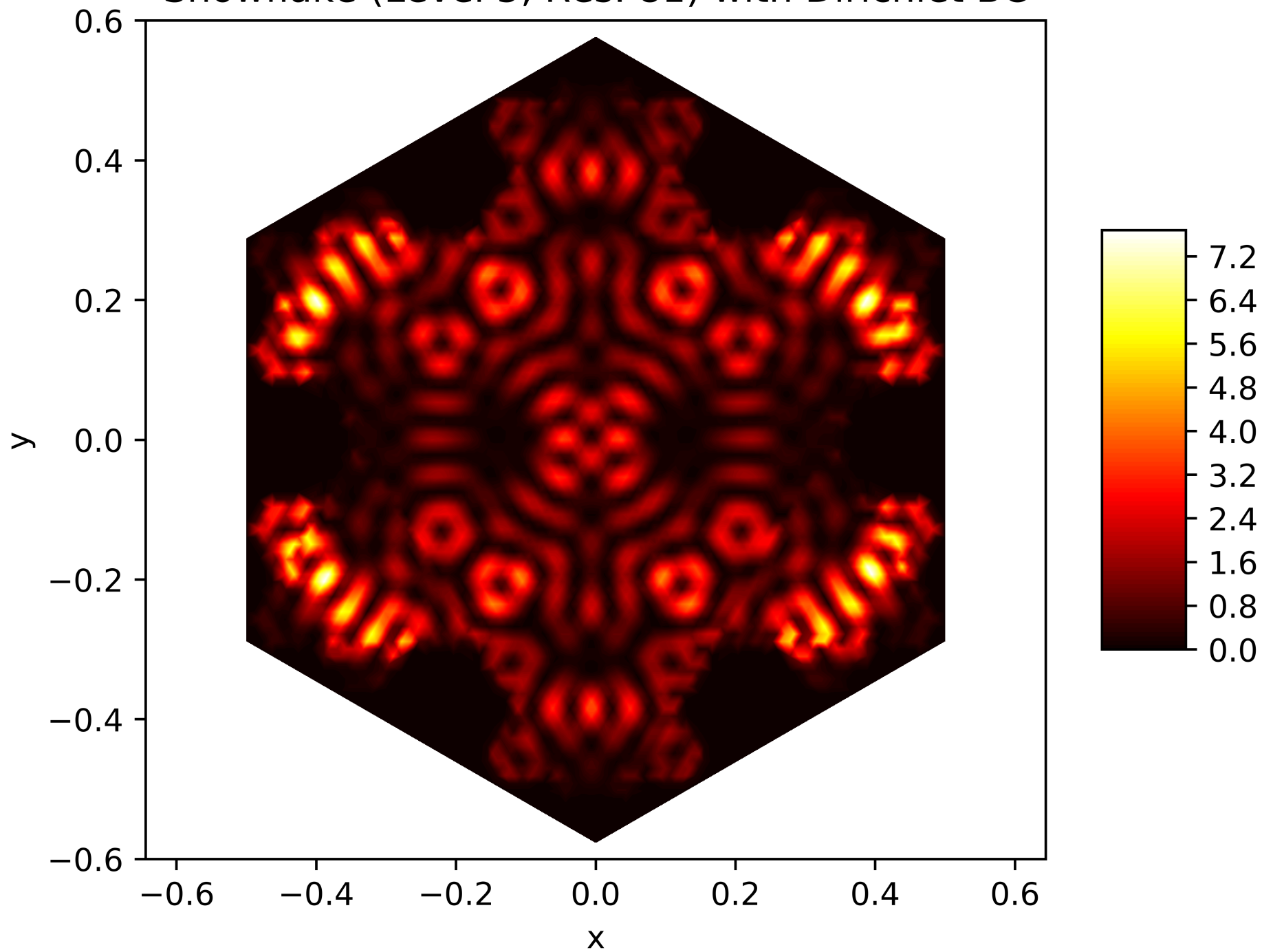
Energy Function of the 192. Eigenfunction on the Snowflake (Level 5, Res. 81) with Dirichlet BC
