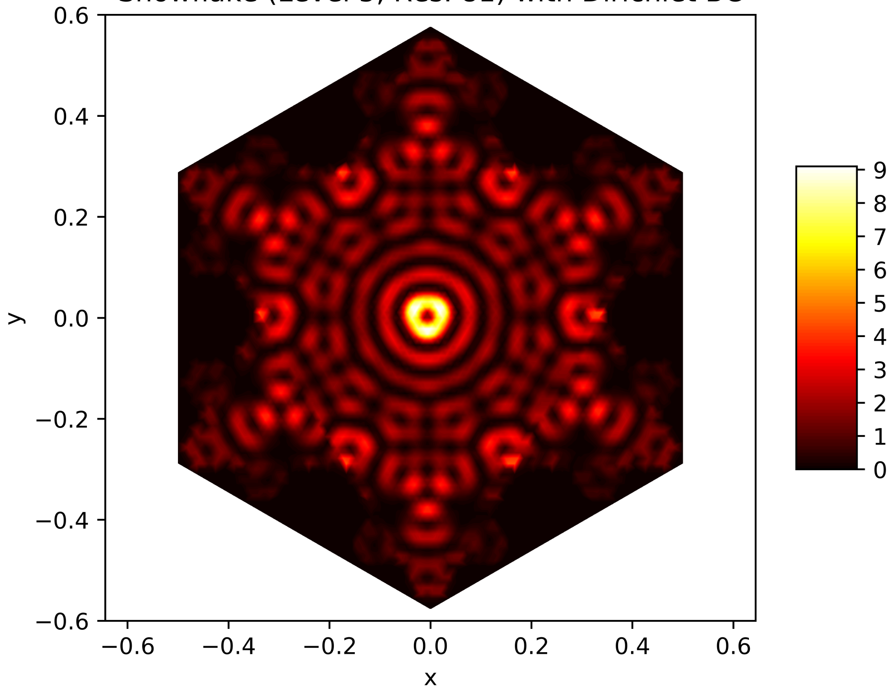
Energy Function of the 182. Eigenfunction on the Snowflake (Level 5, Res. 81) with Dirichlet BC
