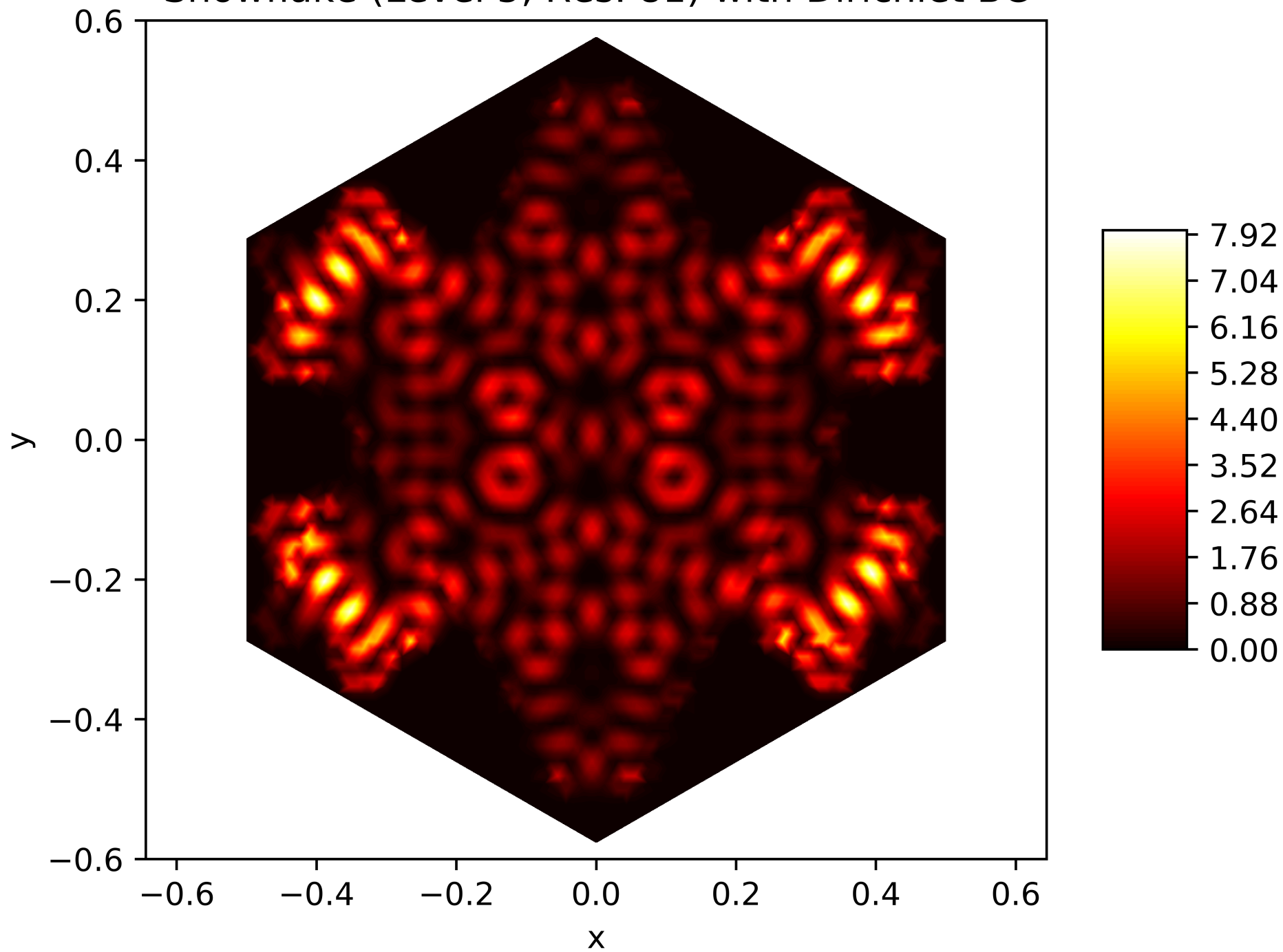
Energy Function of the 186. Eigenfunction on the Snowflake (Level 5, Res. 81) with Dirichlet BC
