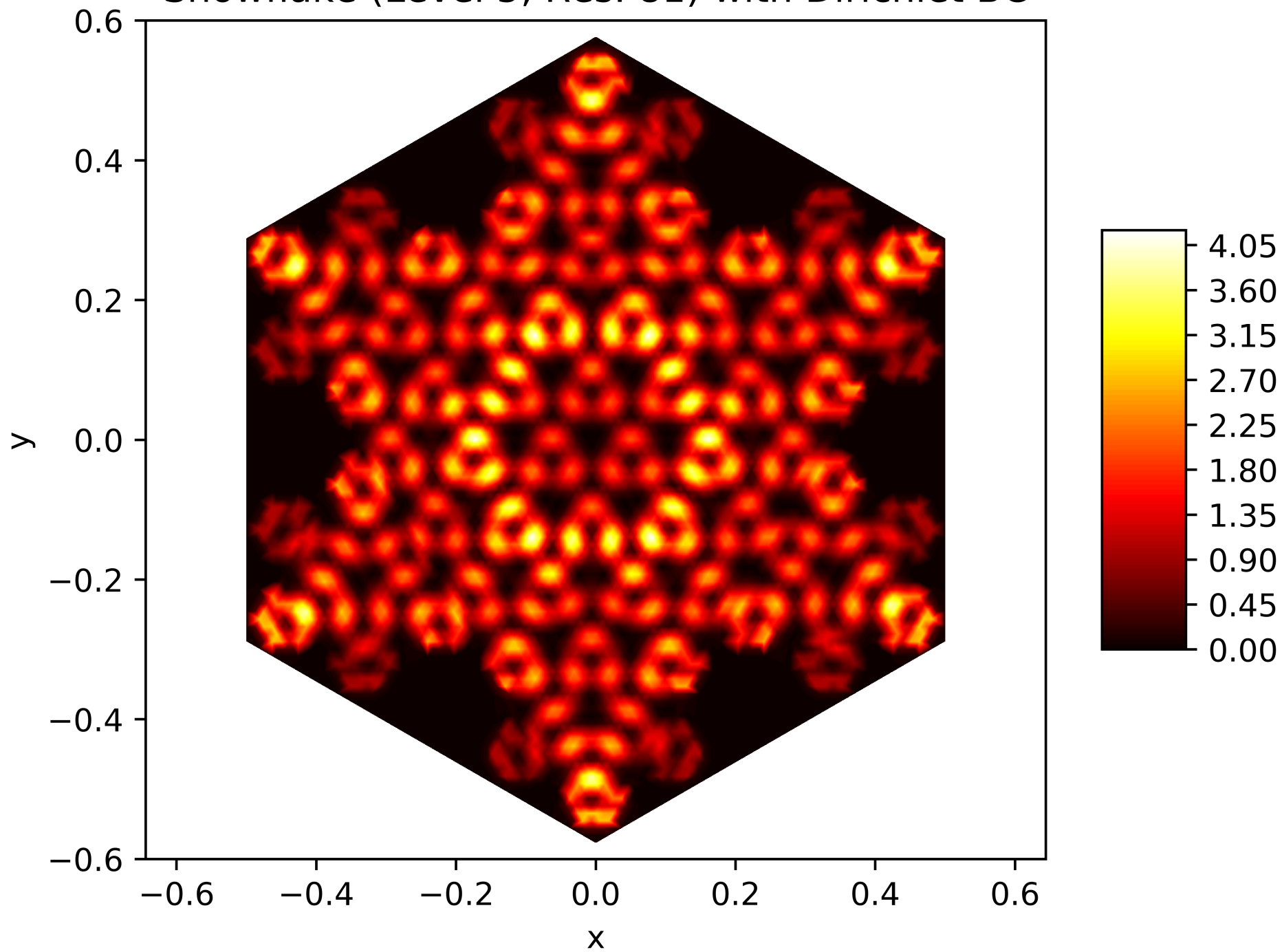
Energy Function of the 188. Eigenfunction on the Snowflake (Level 5, Res. 81) with Dirichlet BC
