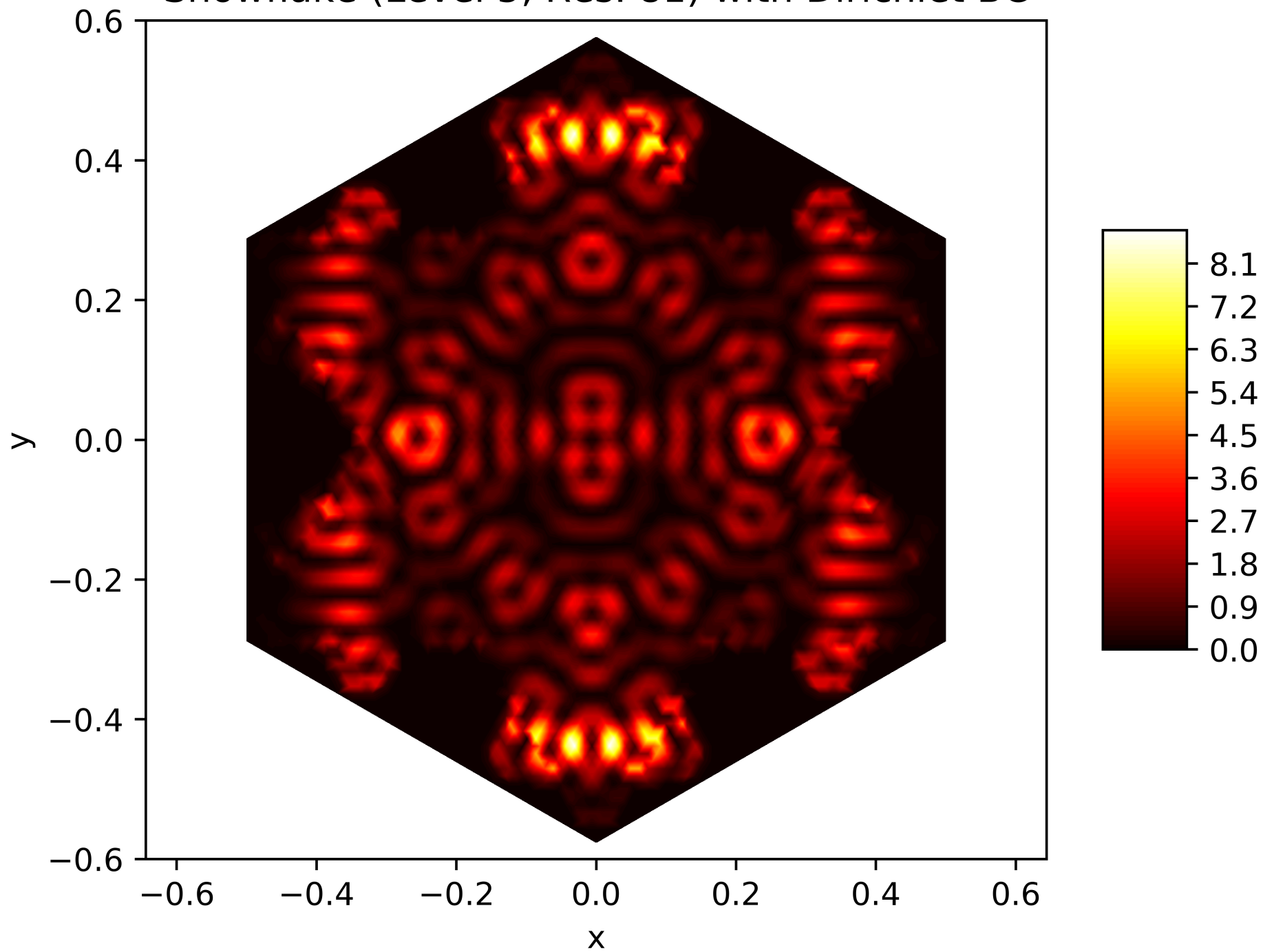
Energy Function of the 191. Eigenfunction on the Snowflake (Level 5, Res. 81) with Dirichlet BC
