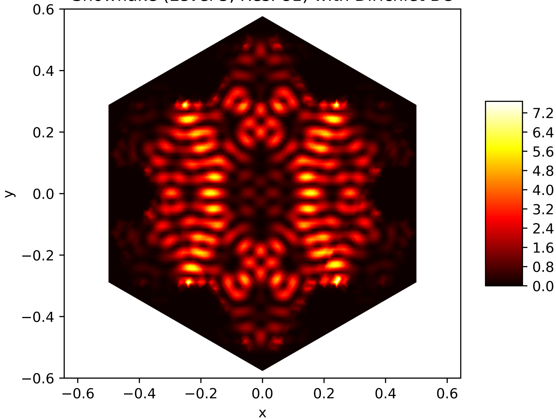
Energy Function of the 195. Eigenfunction on the Snowflake (Level 5, Res. 81) with Dirichlet BC
