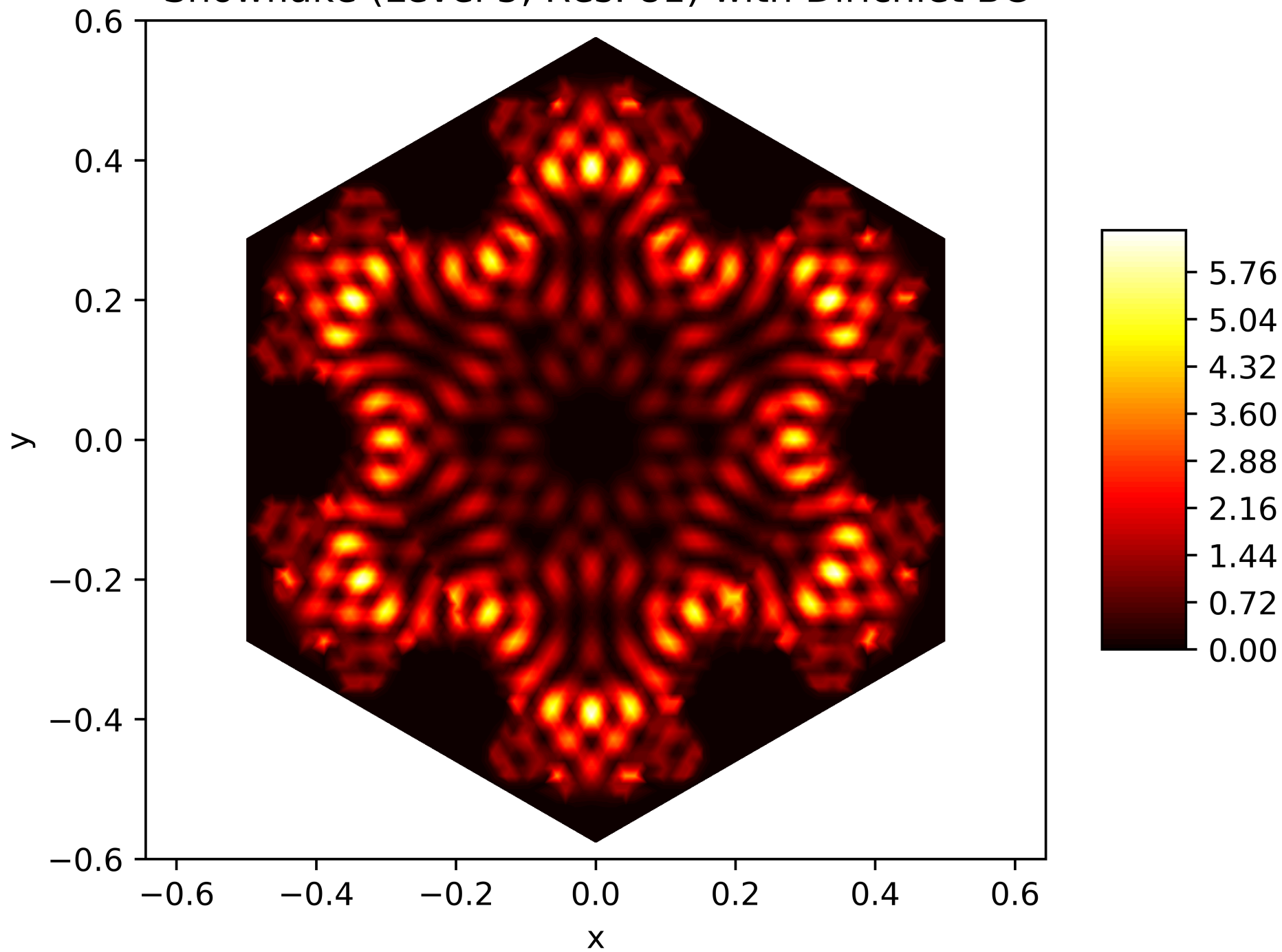
Energy Function of the 197. Eigenfunction on the Snowflake (Level 5, Res. 81) with Dirichlet BC
