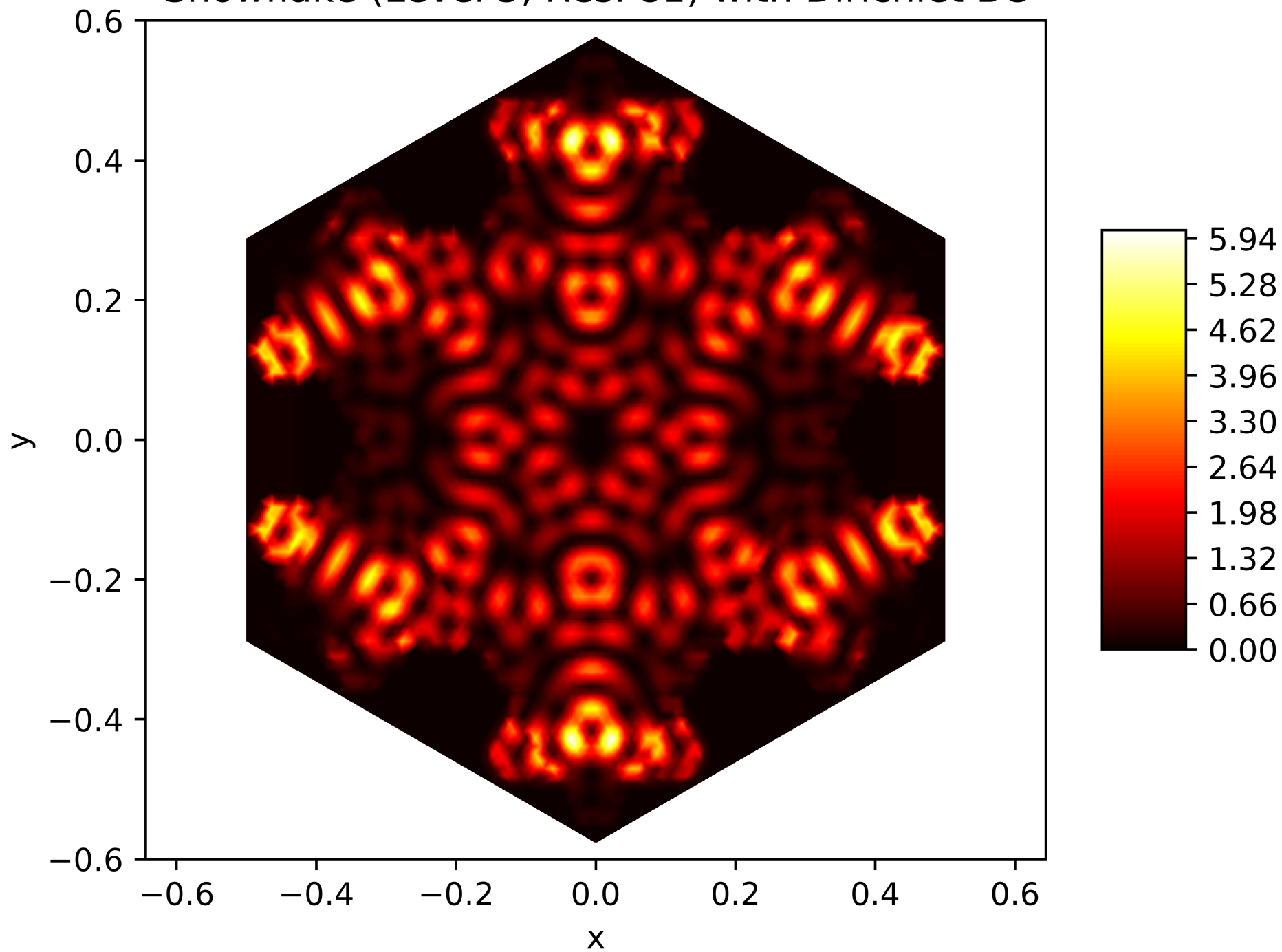
Energy Function of the 184. Eigenfunction on the Snowflake (Level 5, Res. 81) with Dirichlet BC
