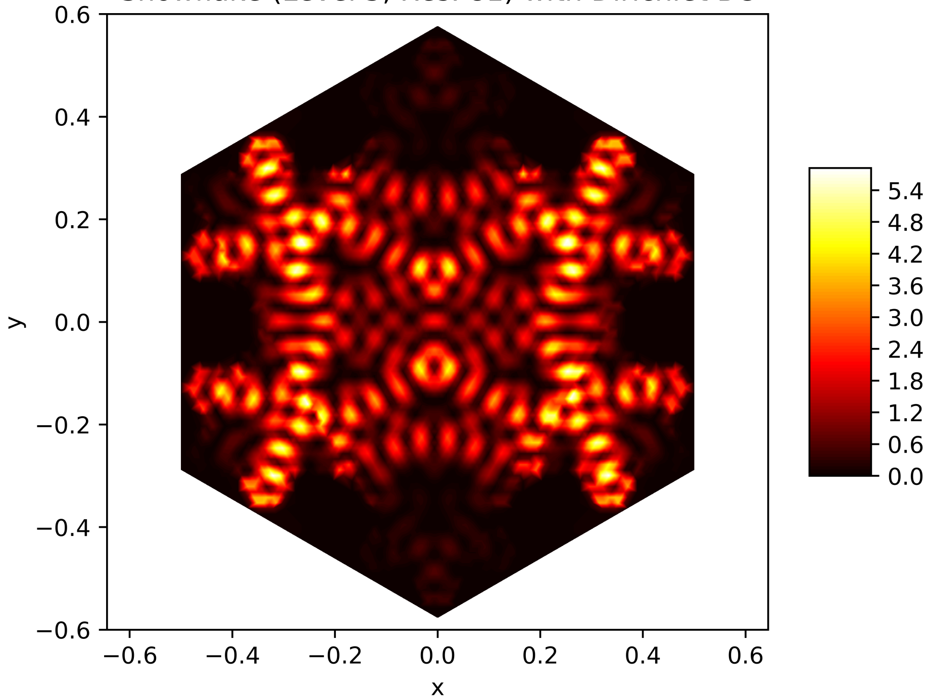
Energy Function of the 194. Eigenfunction on the Snowflake (Level 5, Res. 81) with Dirichlet BC
