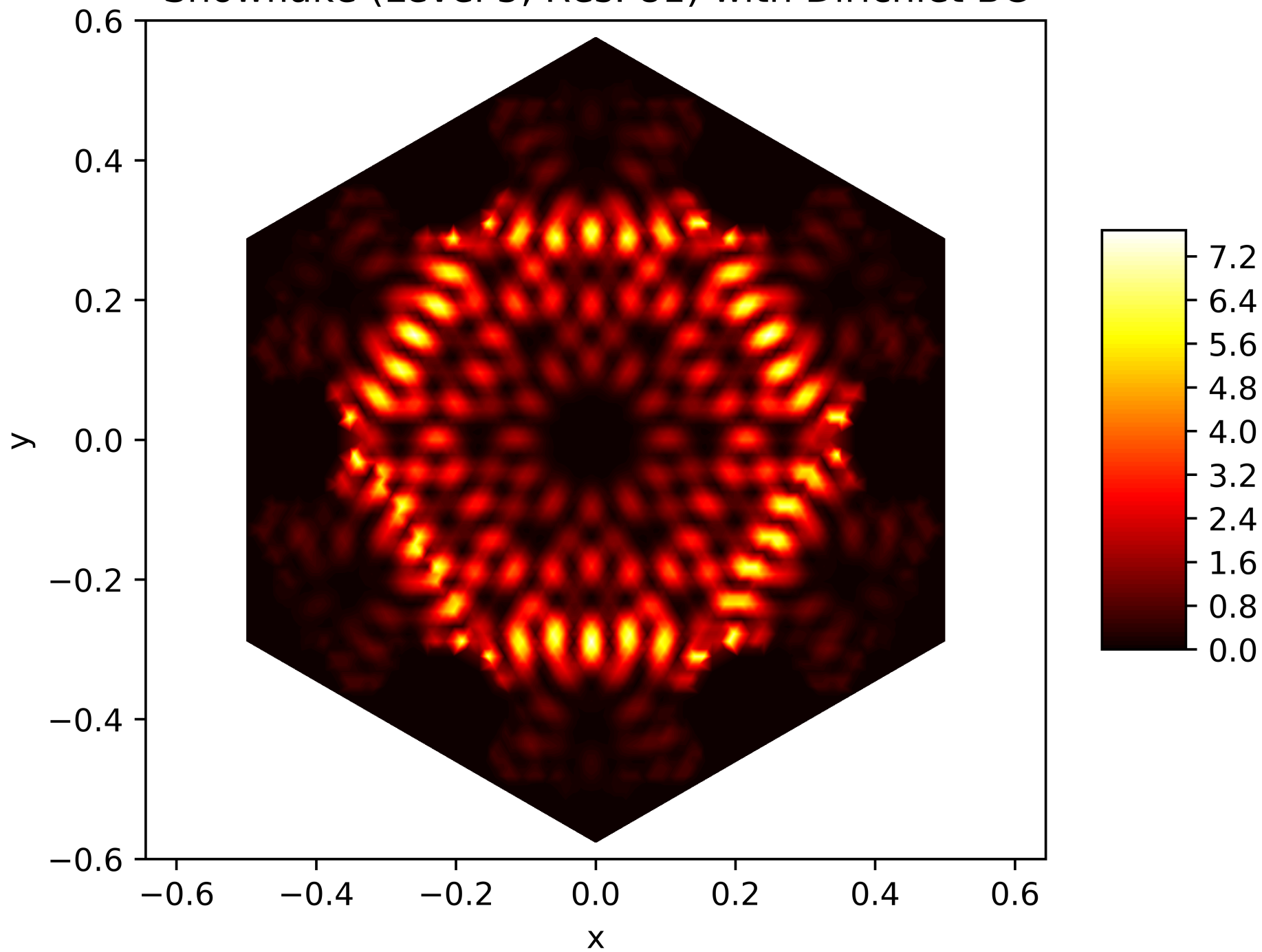
Energy Function of the 200. Eigenfunction on the Snowflake (Level 5, Res. 81) with Dirichlet BC
