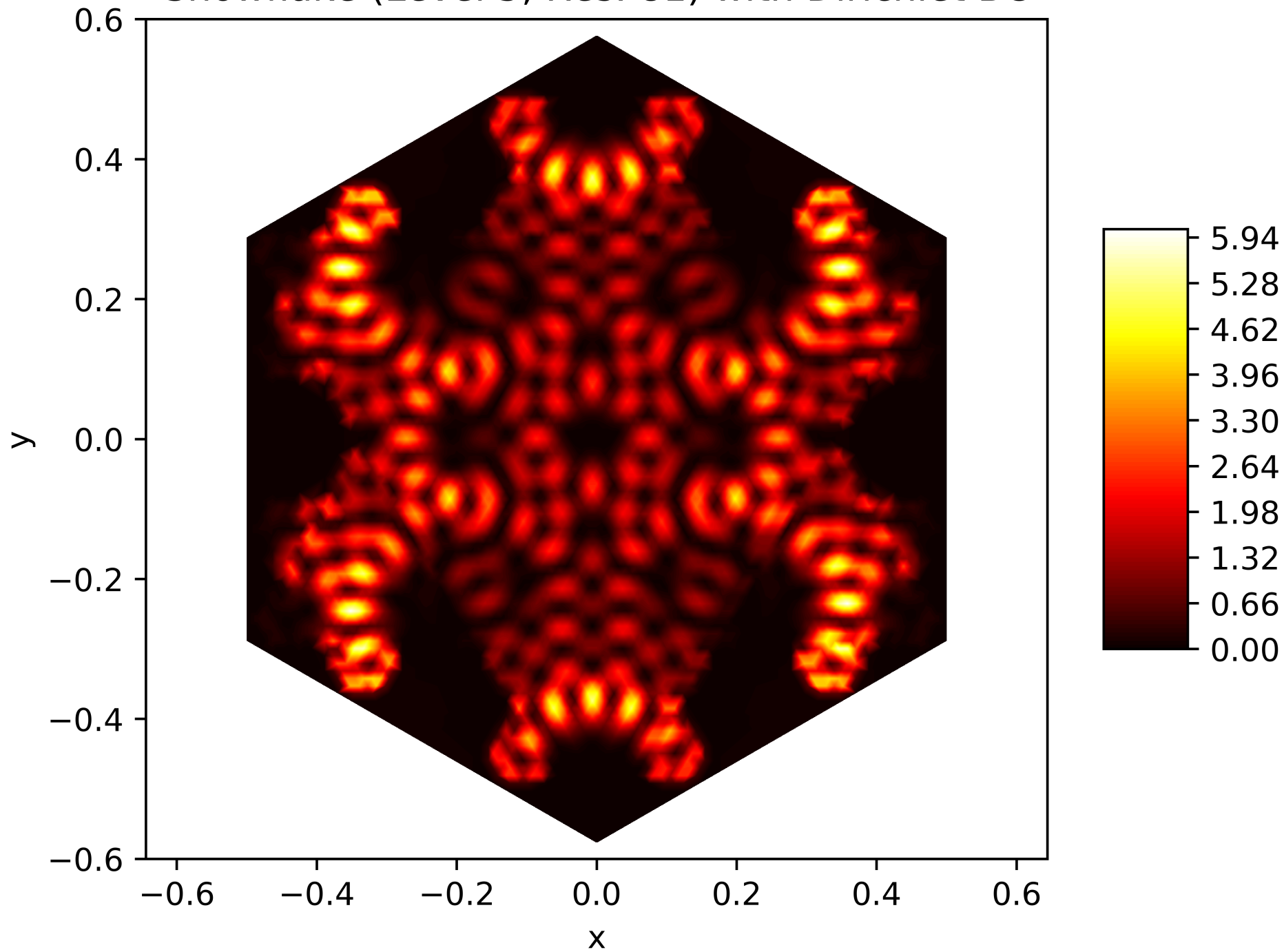
Energy Function of the 183. Eigenfunction on the Snowflake (Level 5, Res. 81) with Dirichlet BC
