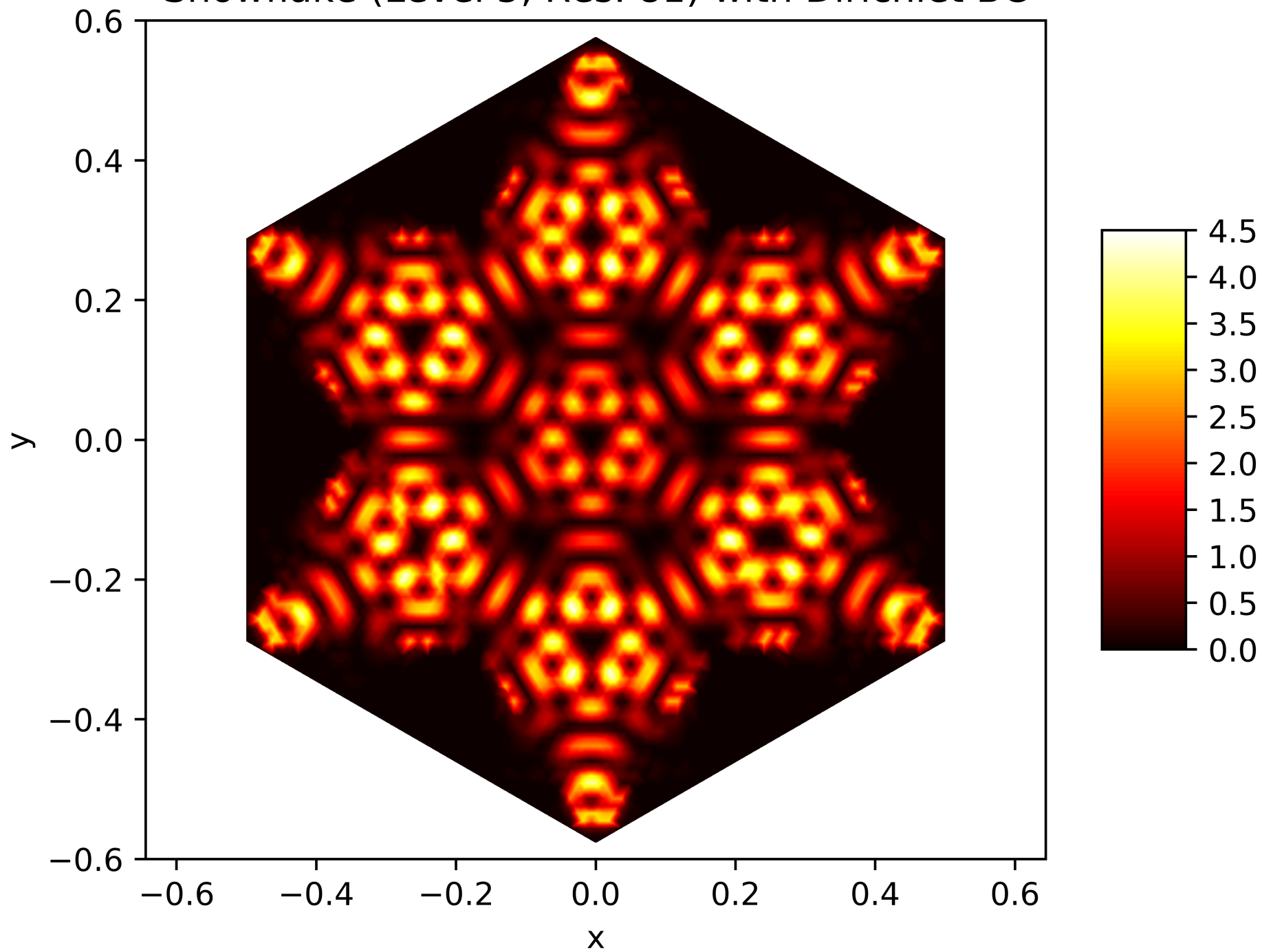
Energy Function of the 198. Eigenfunction on the Snowflake (Level 5, Res. 81) with Dirichlet BC
