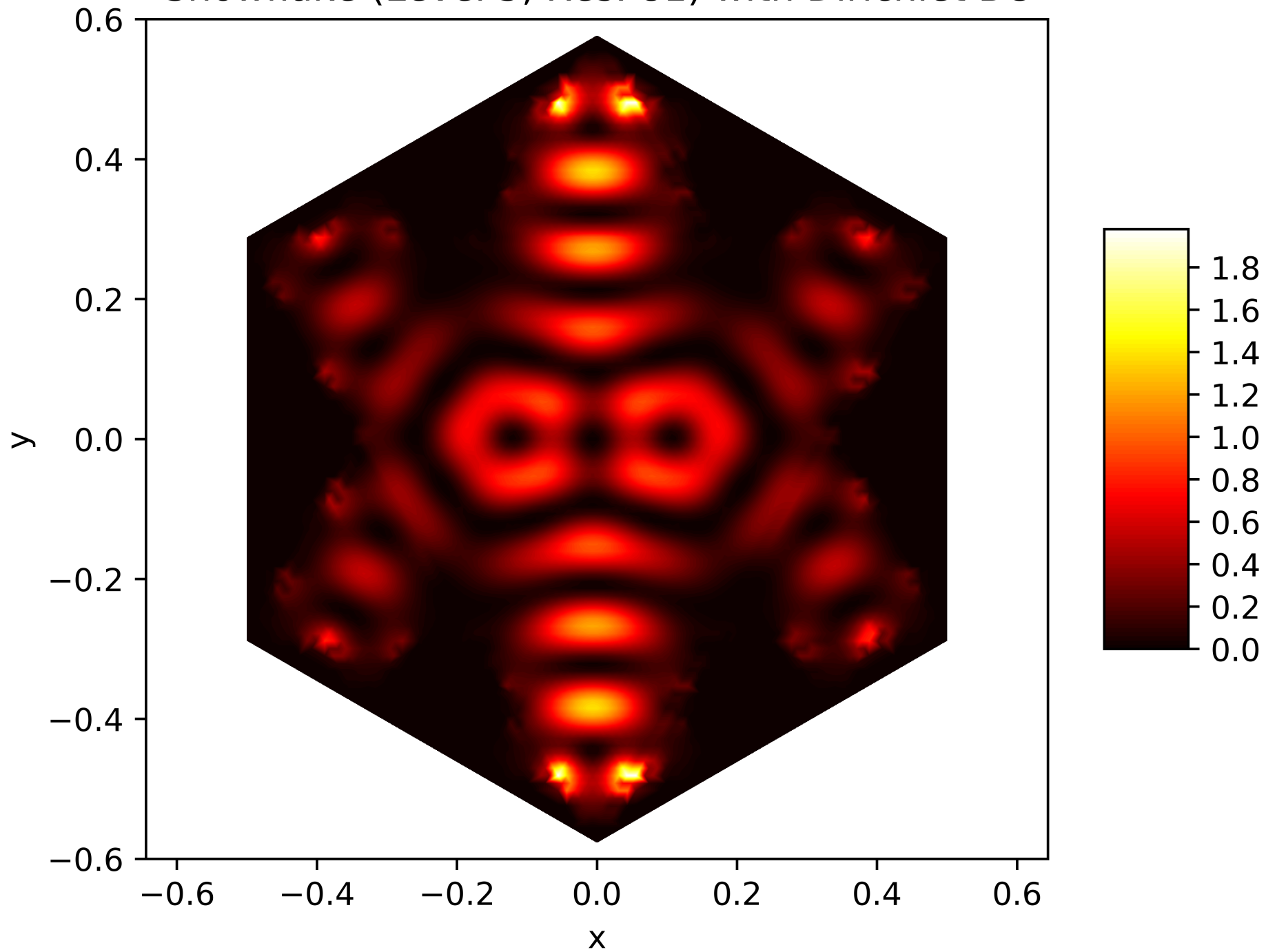
Energy Function of the 34. Eigenfunction on the Snowflake (Level 5, Res. 81) with Dirichlet BC
