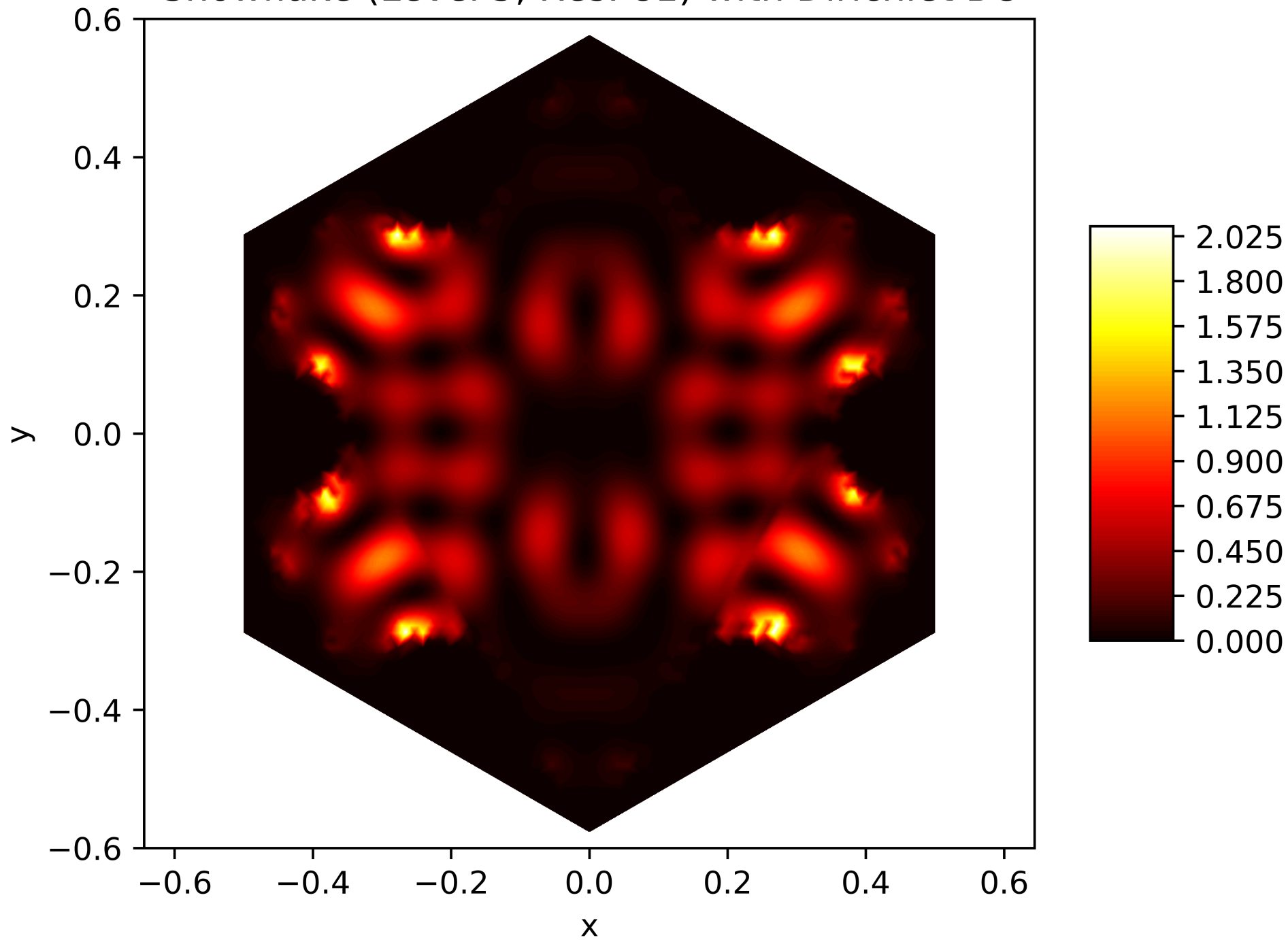
Energy Function of the 31. Eigenfunction on the Snowflake (Level 5, Res. 81) with Dirichlet BC
