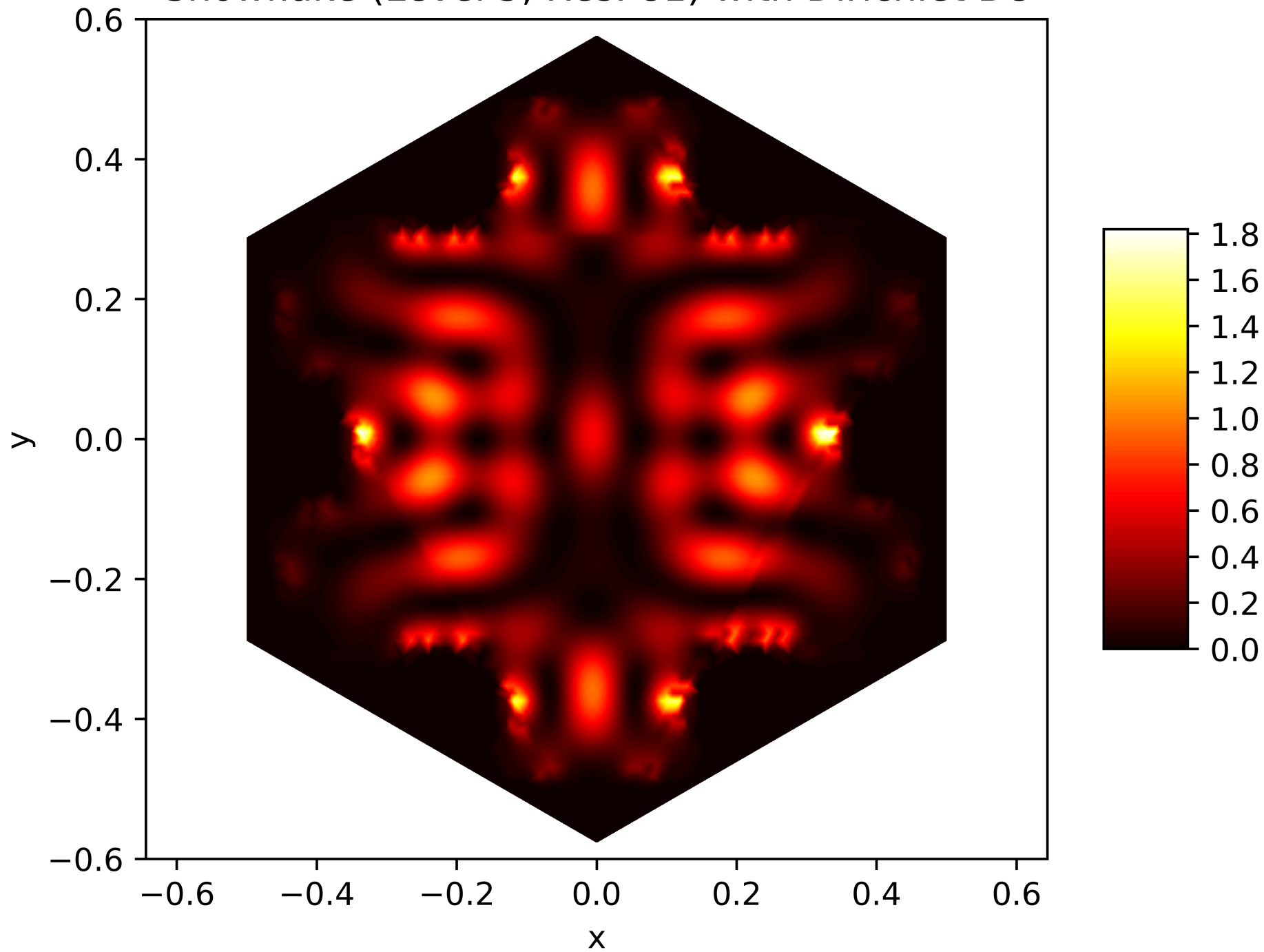
Energy Function of the 33. Eigenfunction on the Snowflake (Level 5, Res. 81) with Dirichlet BC
