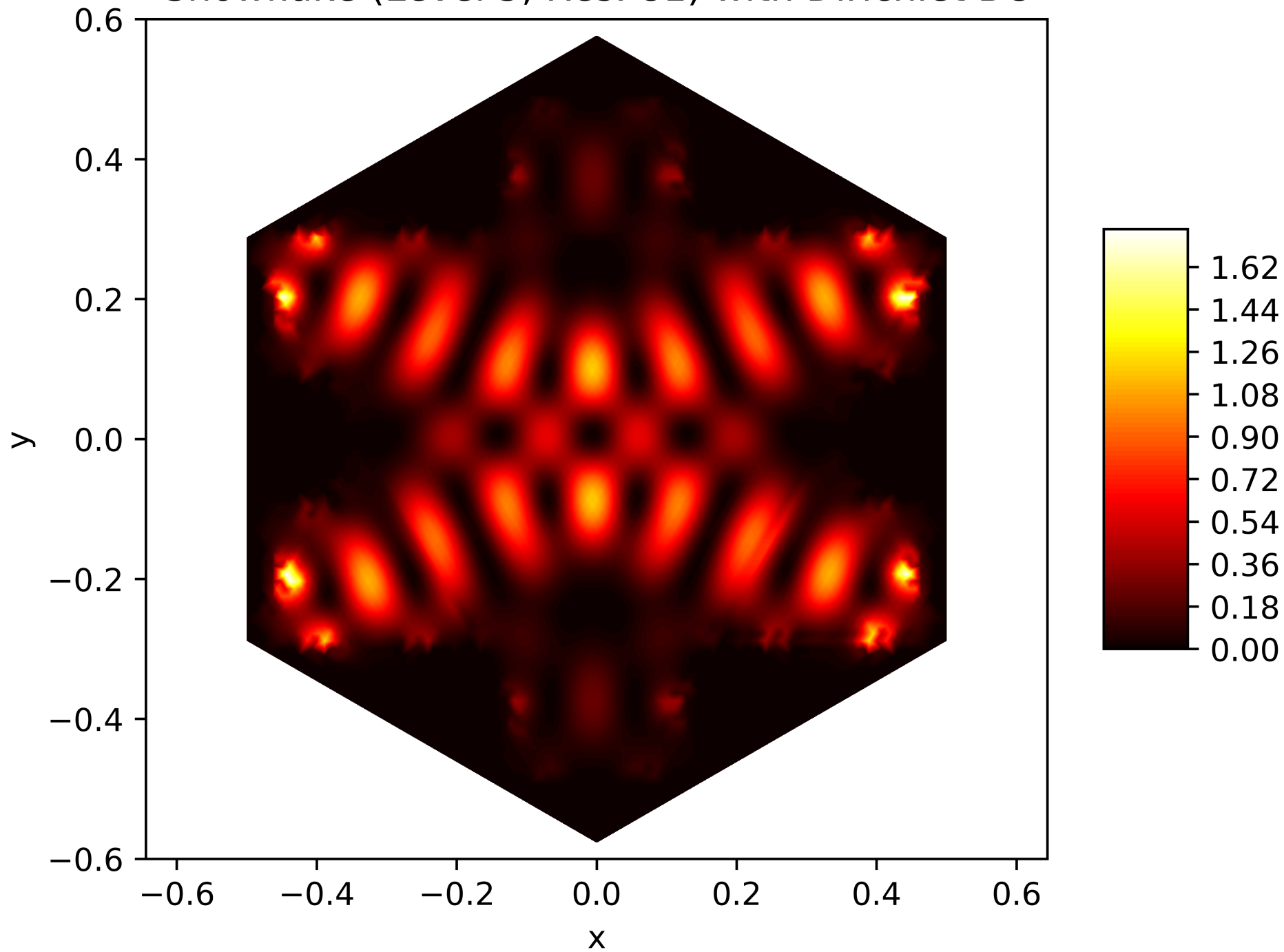
Energy Function of the 35. Eigenfunction on the Snowflake (Level 5, Res. 81) with Dirichlet BC
