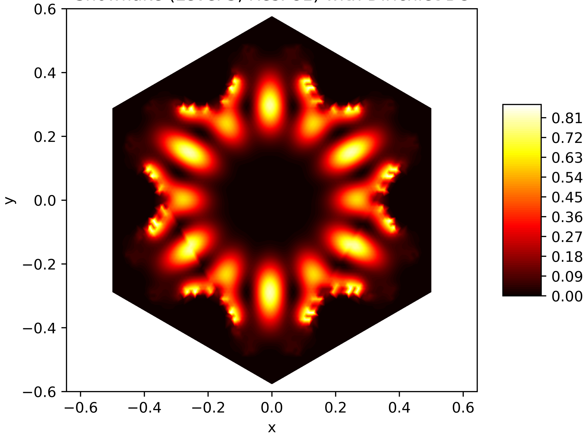
Energy Function of the 24. Eigenfunction on the Snowflake (Level 5, Res. 81) with Dirichlet BC
