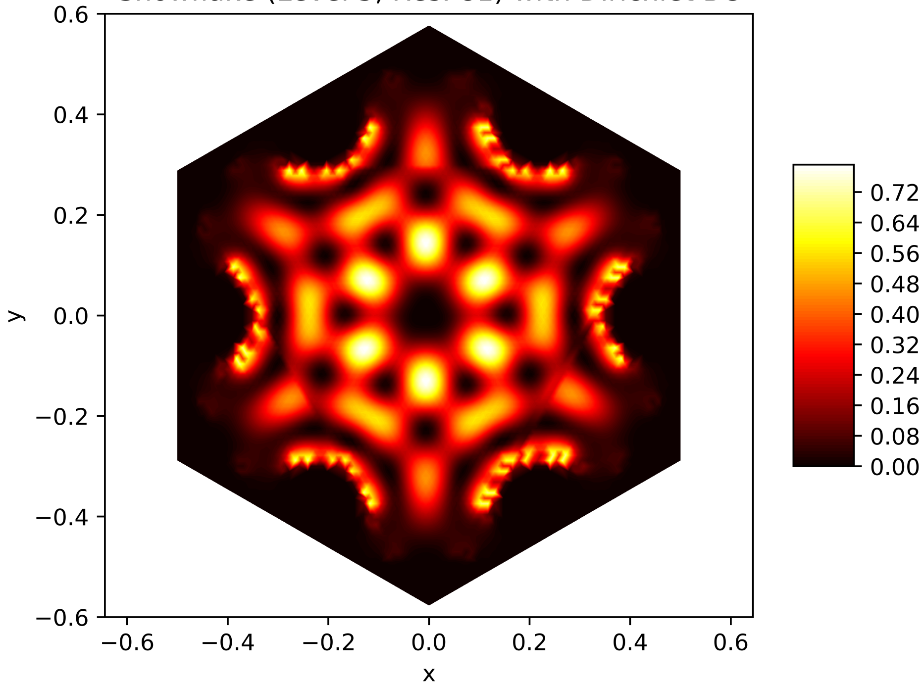
Energy Function of the 25. Eigenfunction on the Snowflake (Level 5, Res. 81) with Dirichlet BC
