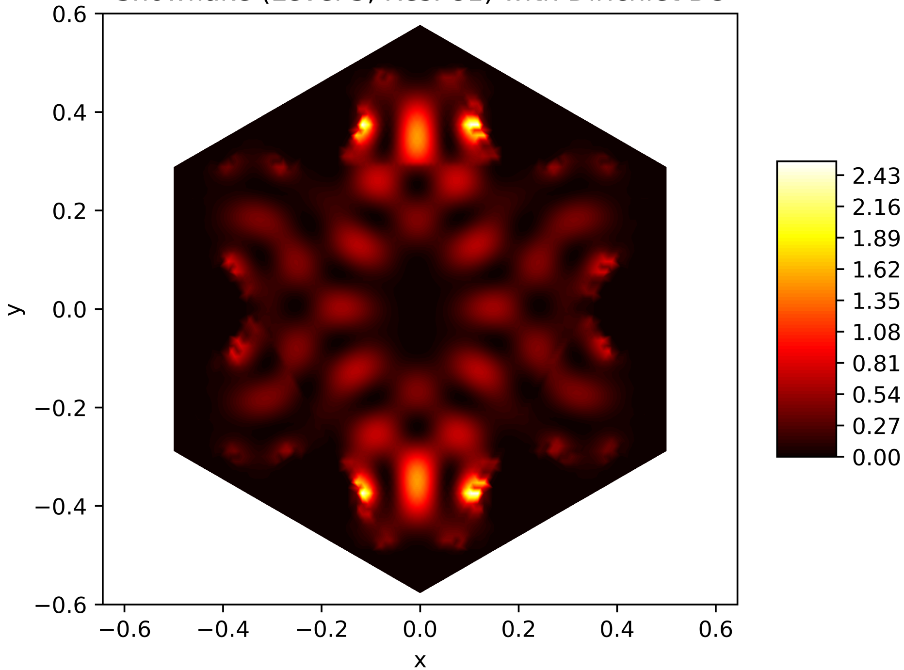
Energy Function of the 30. Eigenfunction on the Snowflake (Level 5, Res. 81) with Dirichlet BC
