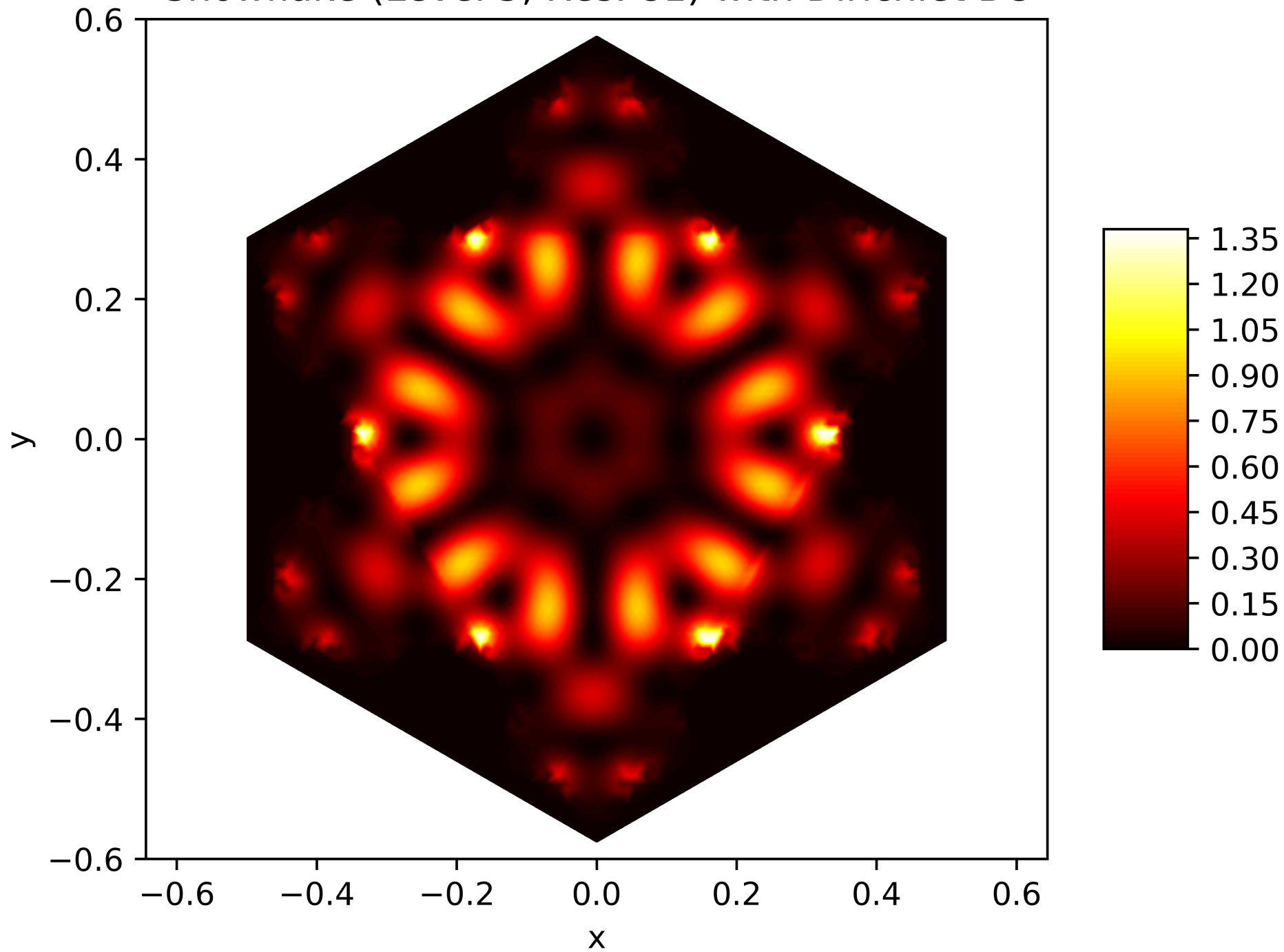
Energy Function of the 29. Eigenfunction on the Snowflake (Level 5, Res. 81) with Dirichlet BC
