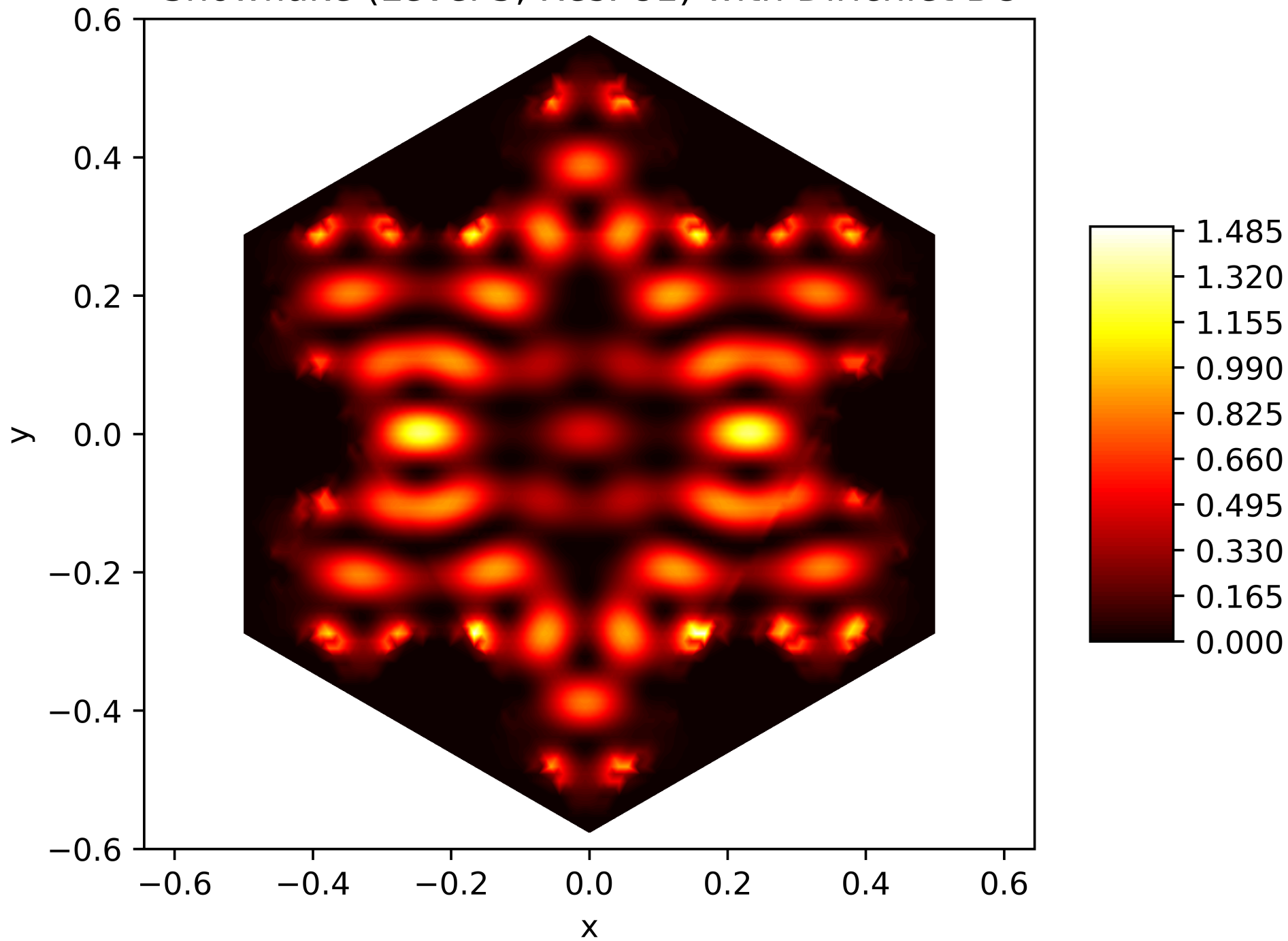
Energy Function of the 39. Eigenfunction on the Snowflake (Level 5, Res. 81) with Dirichlet BC
