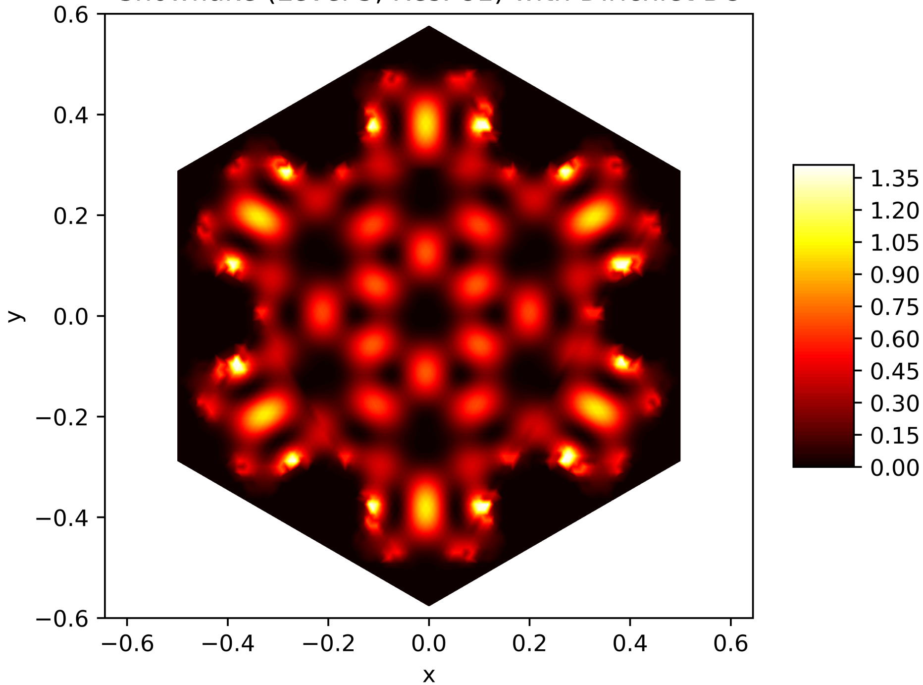
Energy Function of the 36. Eigenfunction on the Snowflake (Level 5, Res. 81) with Dirichlet BC
