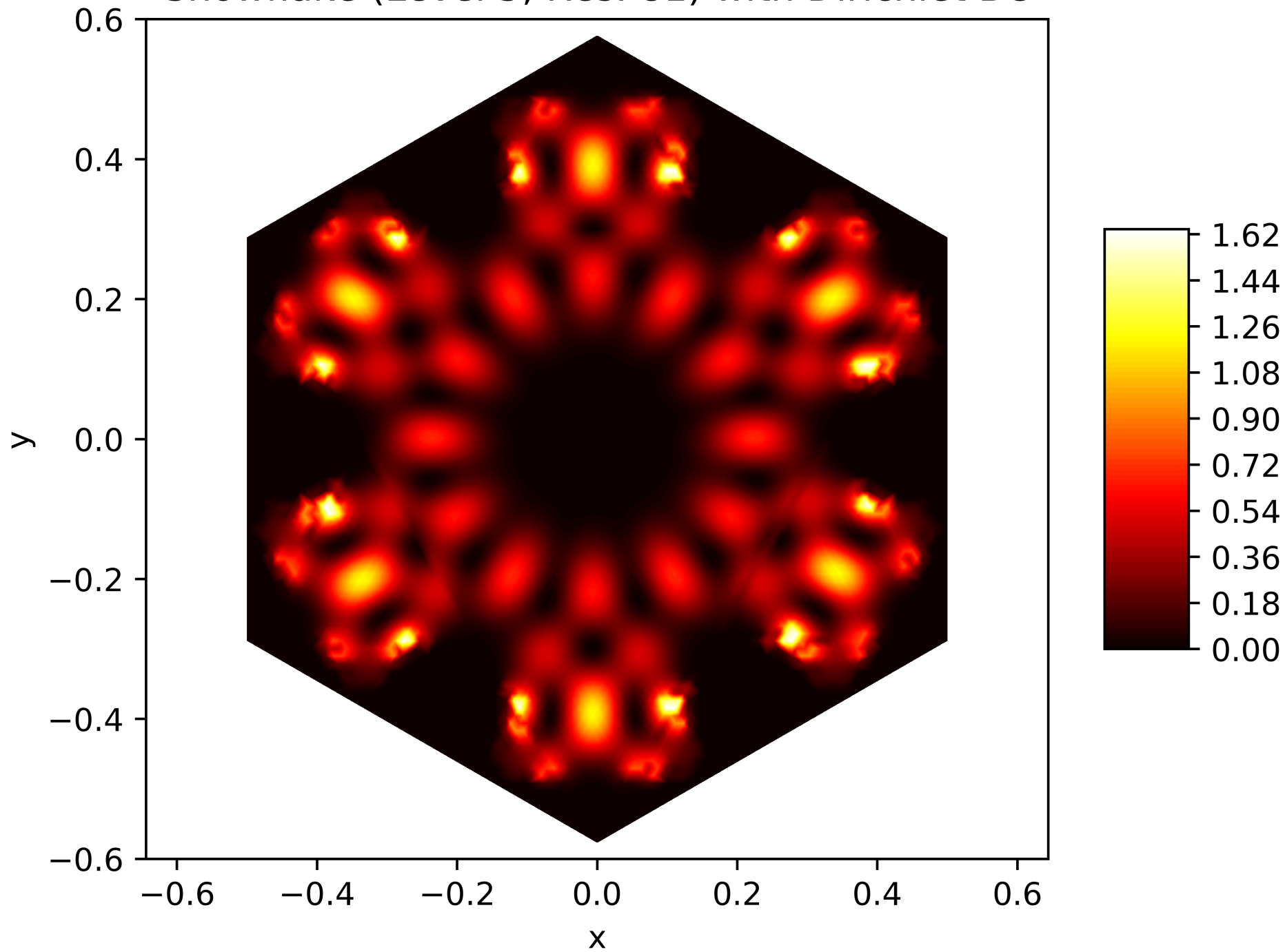
Energy Function of the 38. Eigenfunction on the Snowflake (Level 5, Res. 81) with Dirichlet BC
