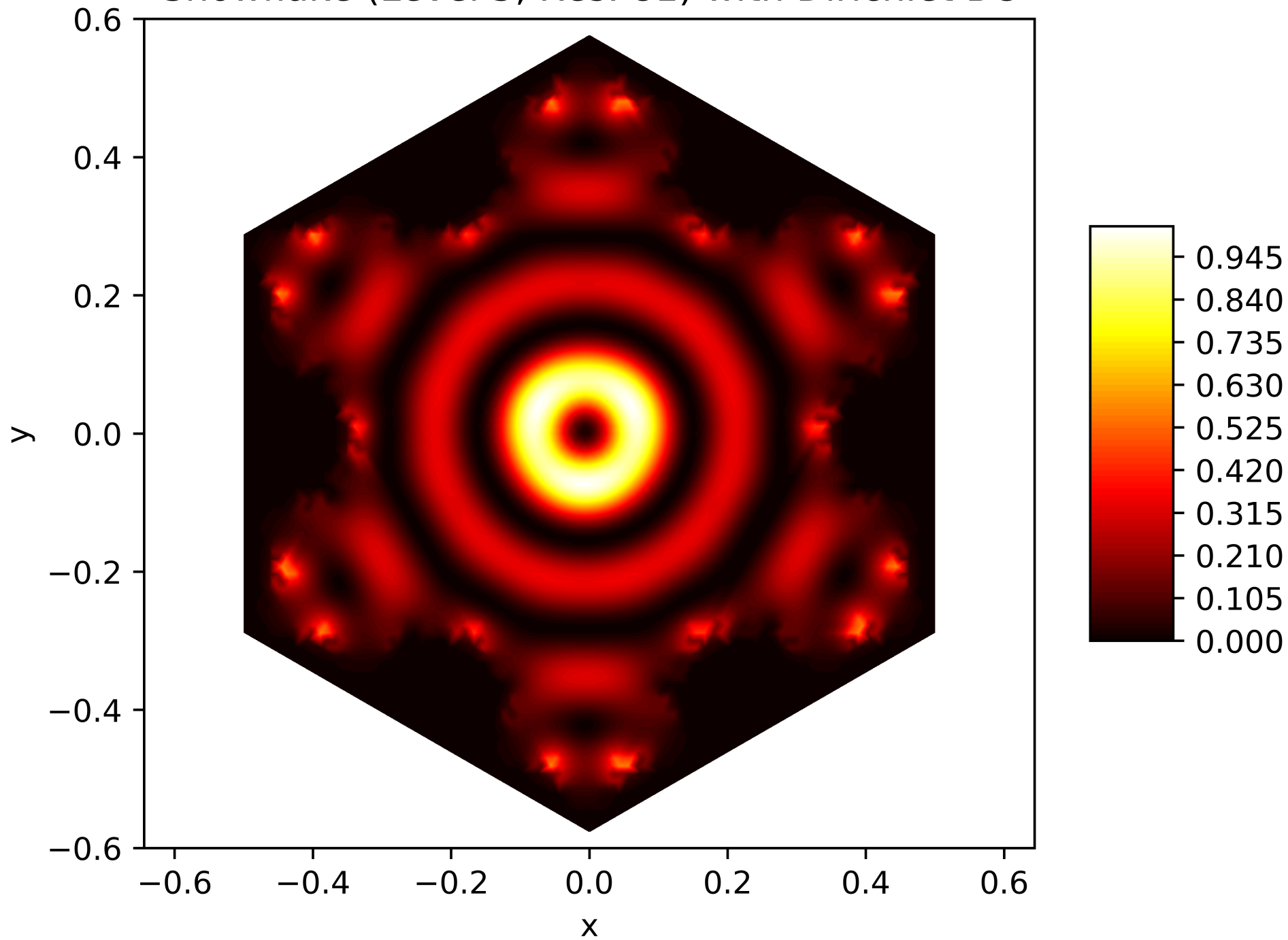
Energy Function of the 23. Eigenfunction on the Snowflake (Level 5, Res. 81) with Dirichlet BC
