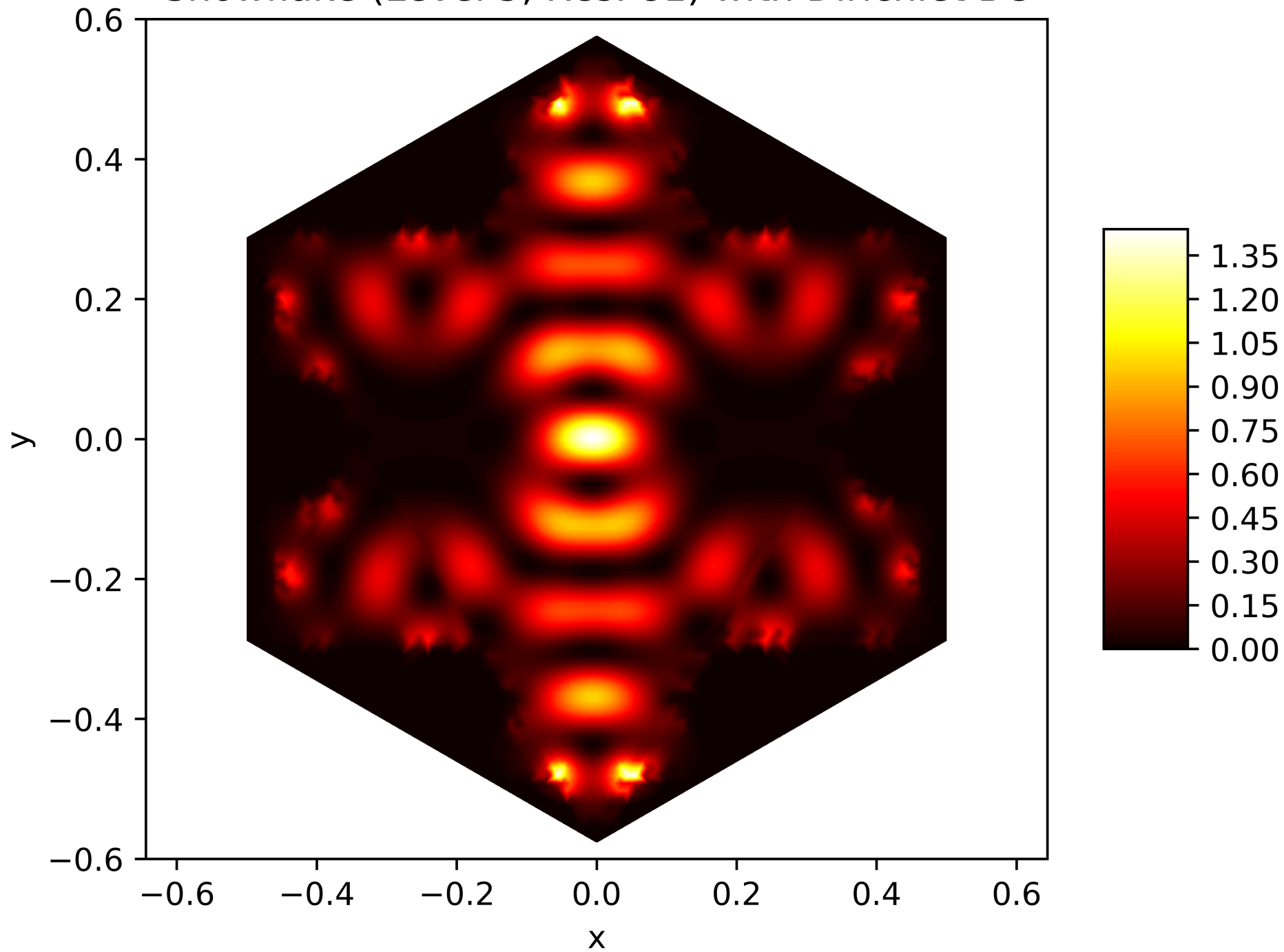
Energy Function of the 27. Eigenfunction on the Snowflake (Level 5, Res. 81) with Dirichlet BC
