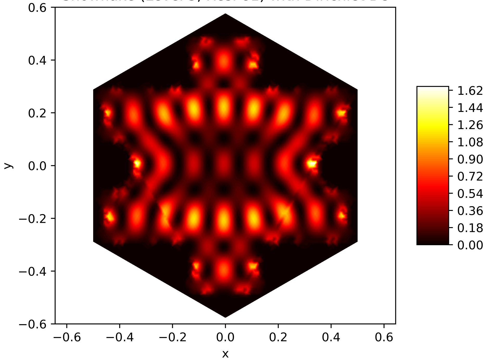
Energy Function of the 40. Eigenfunction on the Snowflake (Level 5, Res. 81) with Dirichlet BC
