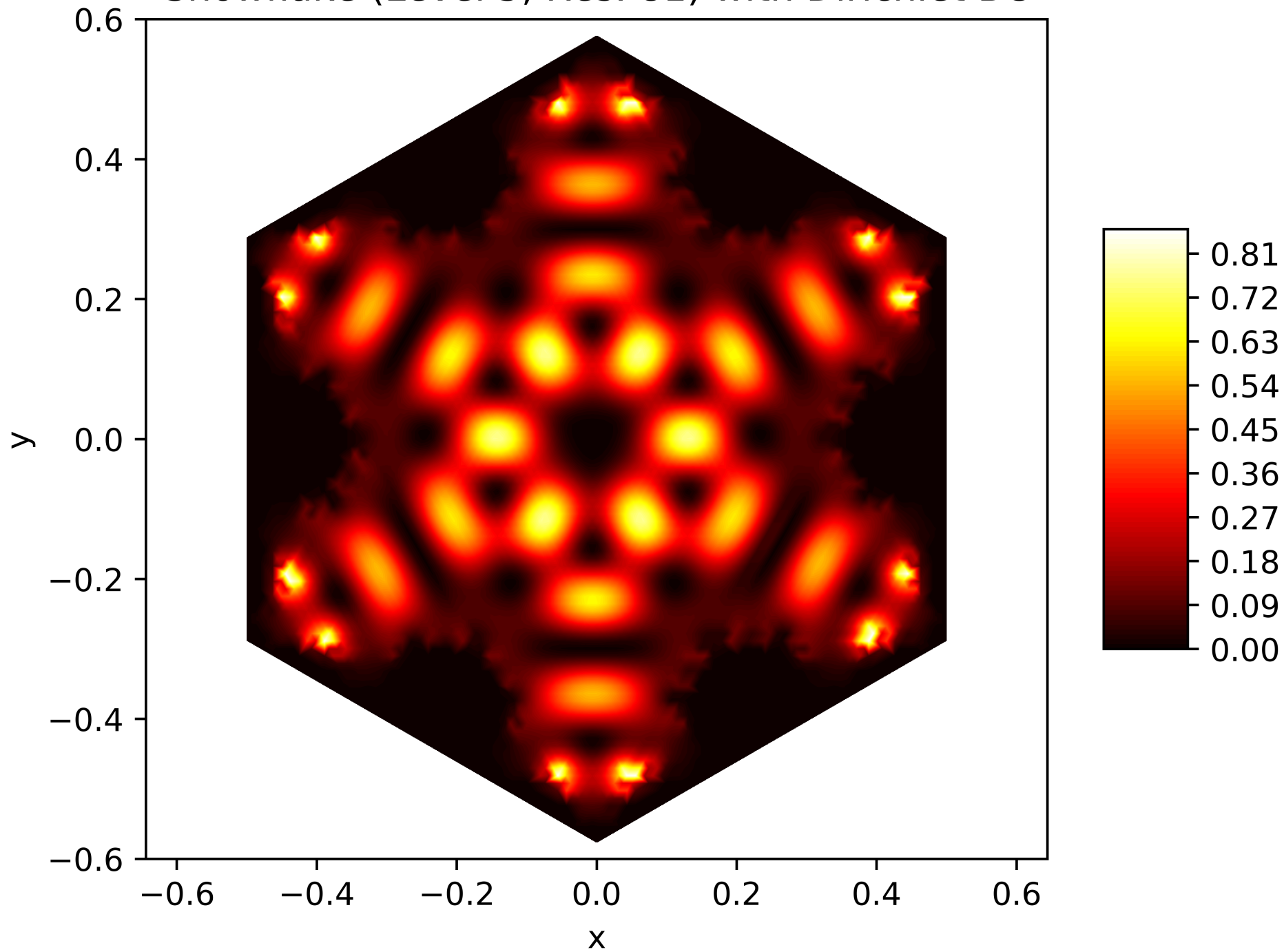
Energy Function of the 26. Eigenfunction on the Snowflake (Level 5, Res. 81) with Dirichlet BC
