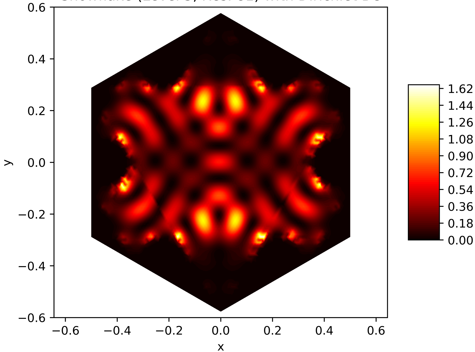
Energy Function of the 32. Eigenfunction on the Snowflake (Level 5, Res. 81) with Dirichlet BC
