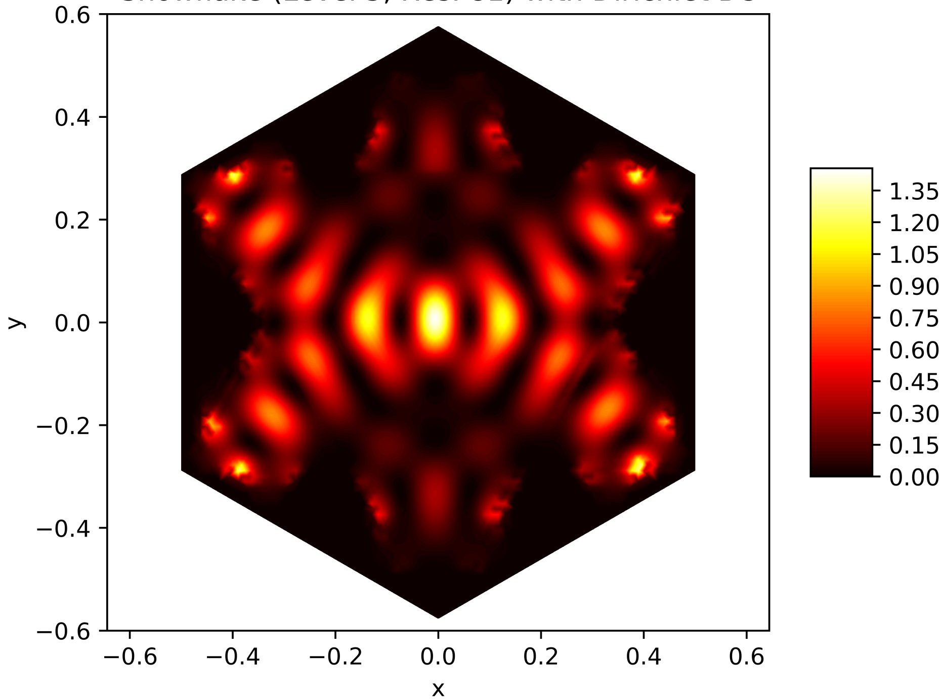
Energy Function of the 28. Eigenfunction on the Snowflake (Level 5, Res. 81) with Dirichlet BC
