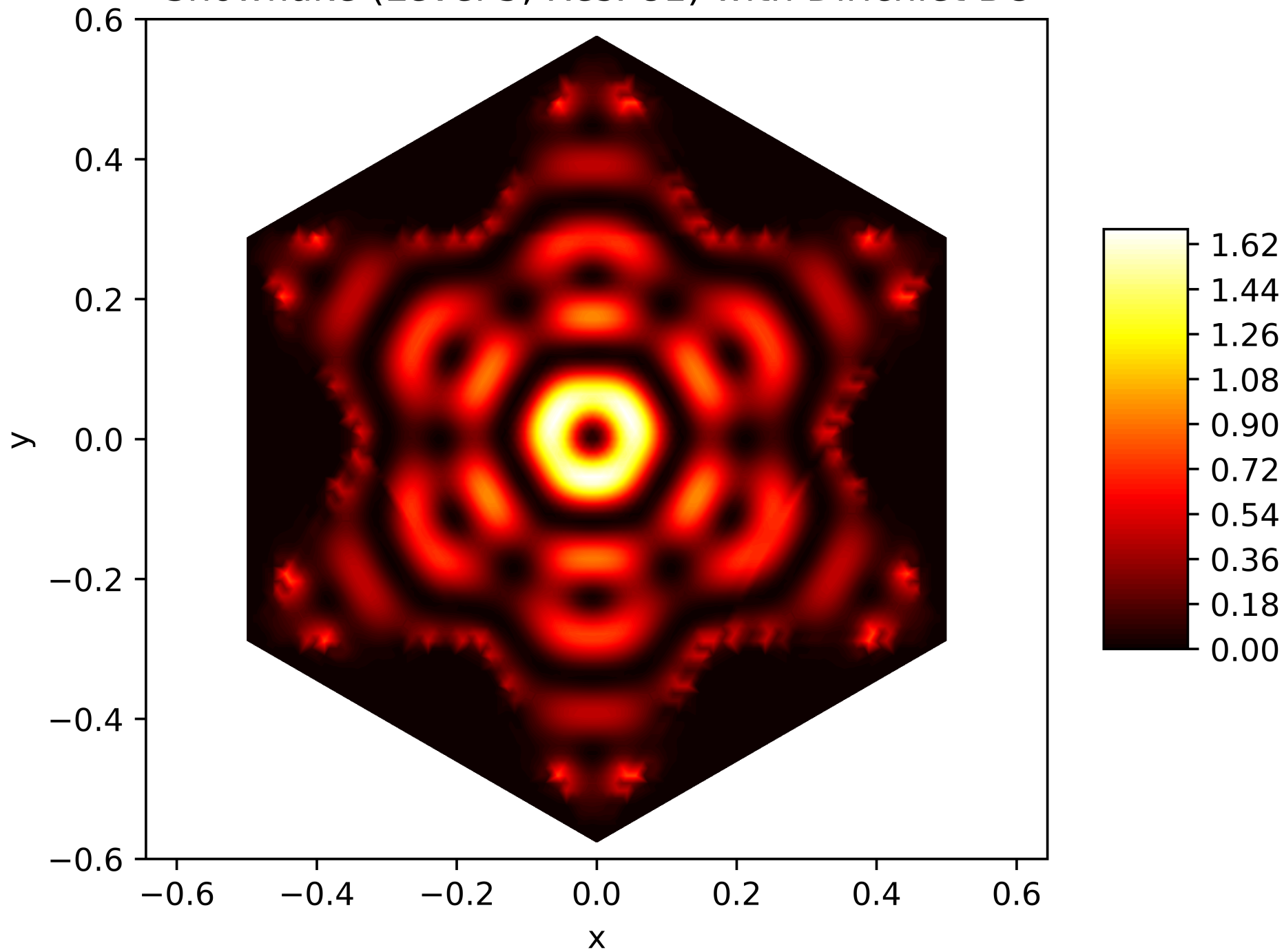
Energy Function of the 37. Eigenfunction on the Snowflake (Level 5, Res. 81) with Dirichlet BC
