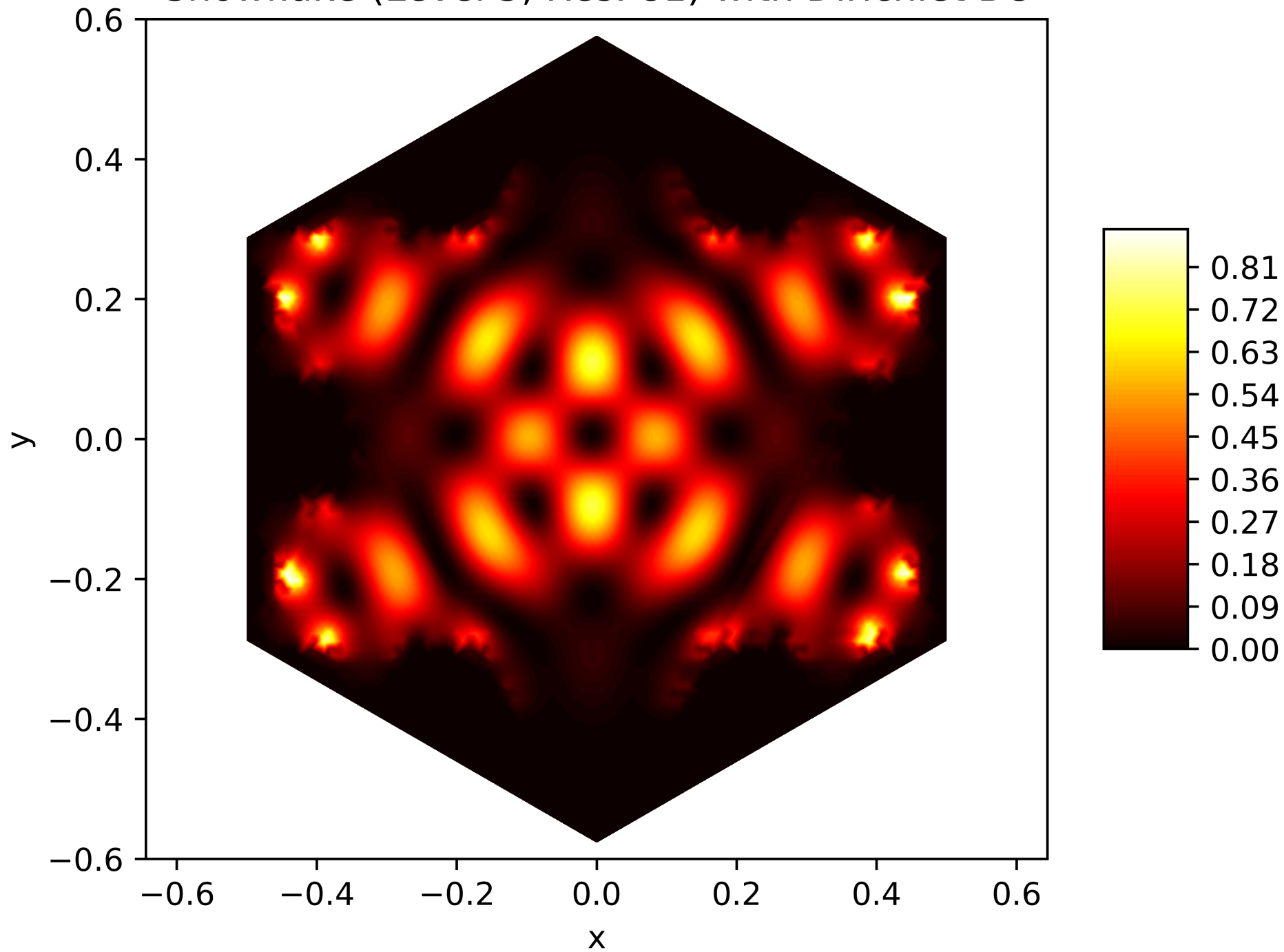
Energy Function of the 22. Eigenfunction on the Snowflake (Level 5, Res. 81) with Dirichlet BC
