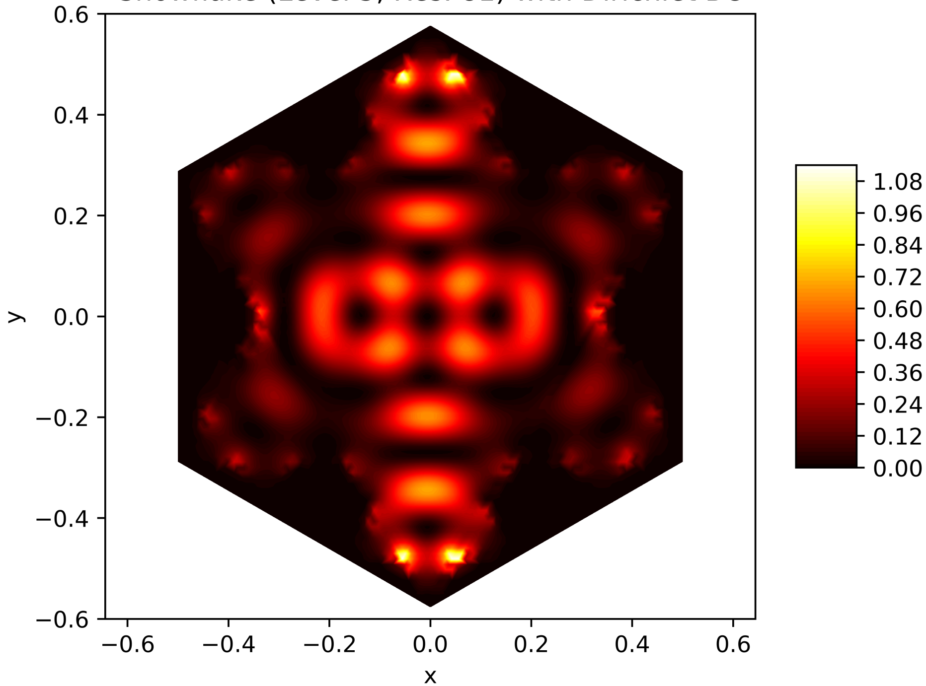
Energy Function of the 21. Eigenfunction on the Snowflake (Level 5, Res. 81) with Dirichlet BC
