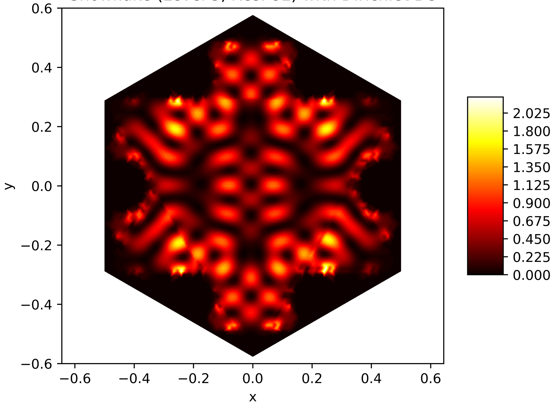
Energy Function of the 56. Eigenfunction on the Snowflake (Level 5, Res. 81) with Dirichlet BC
