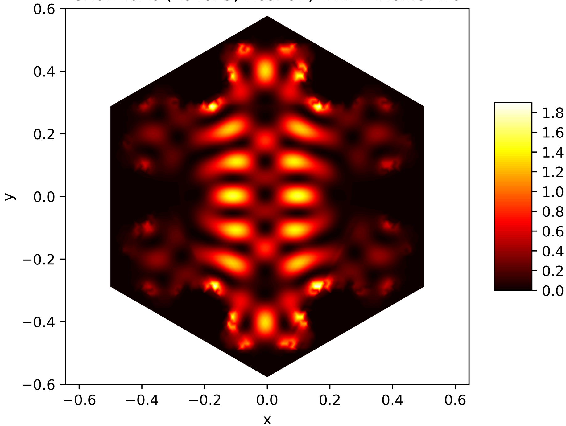
Energy Function of the 41. Eigenfunction on the Snowflake (Level 5, Res. 81) with Dirichlet BC
