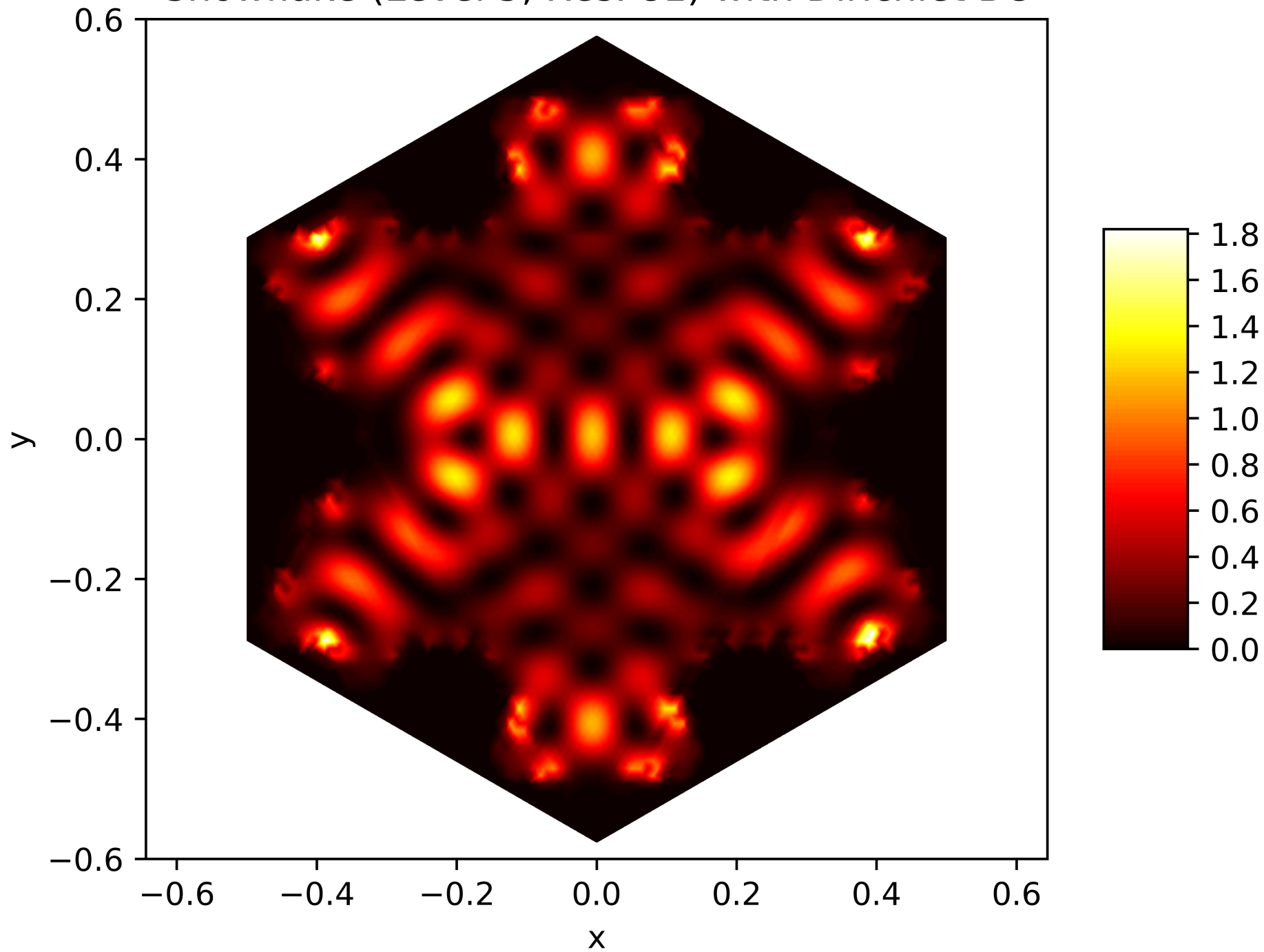
Energy Function of the 44. Eigenfunction on the Snowflake (Level 5, Res. 81) with Dirichlet BC
