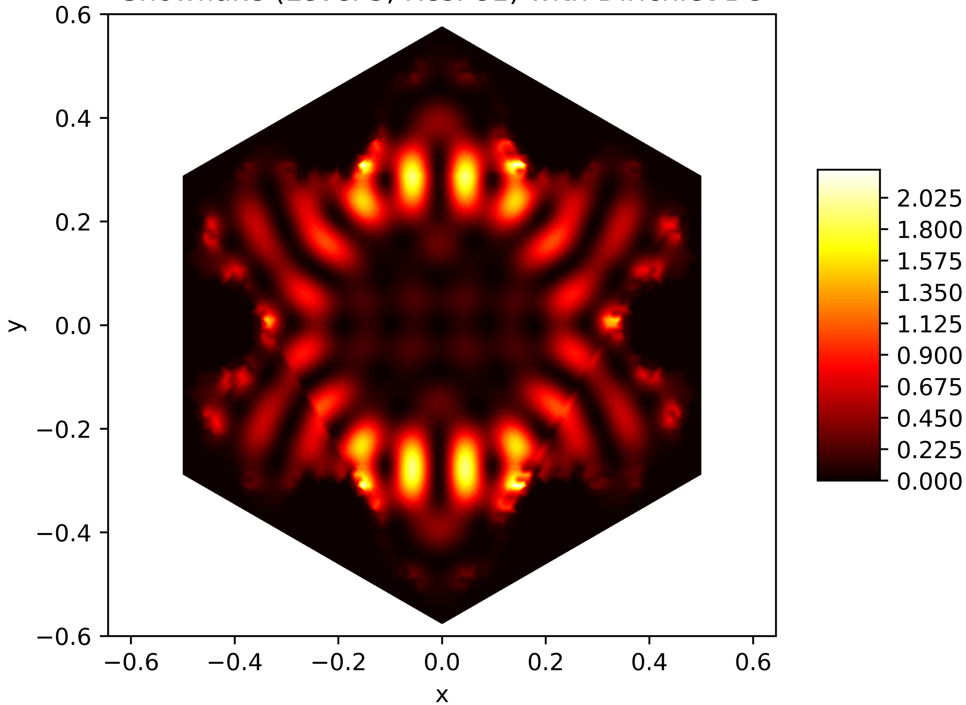
Energy Function of the 46. Eigenfunction on the Snowflake (Level 5, Res. 81) with Dirichlet BC
