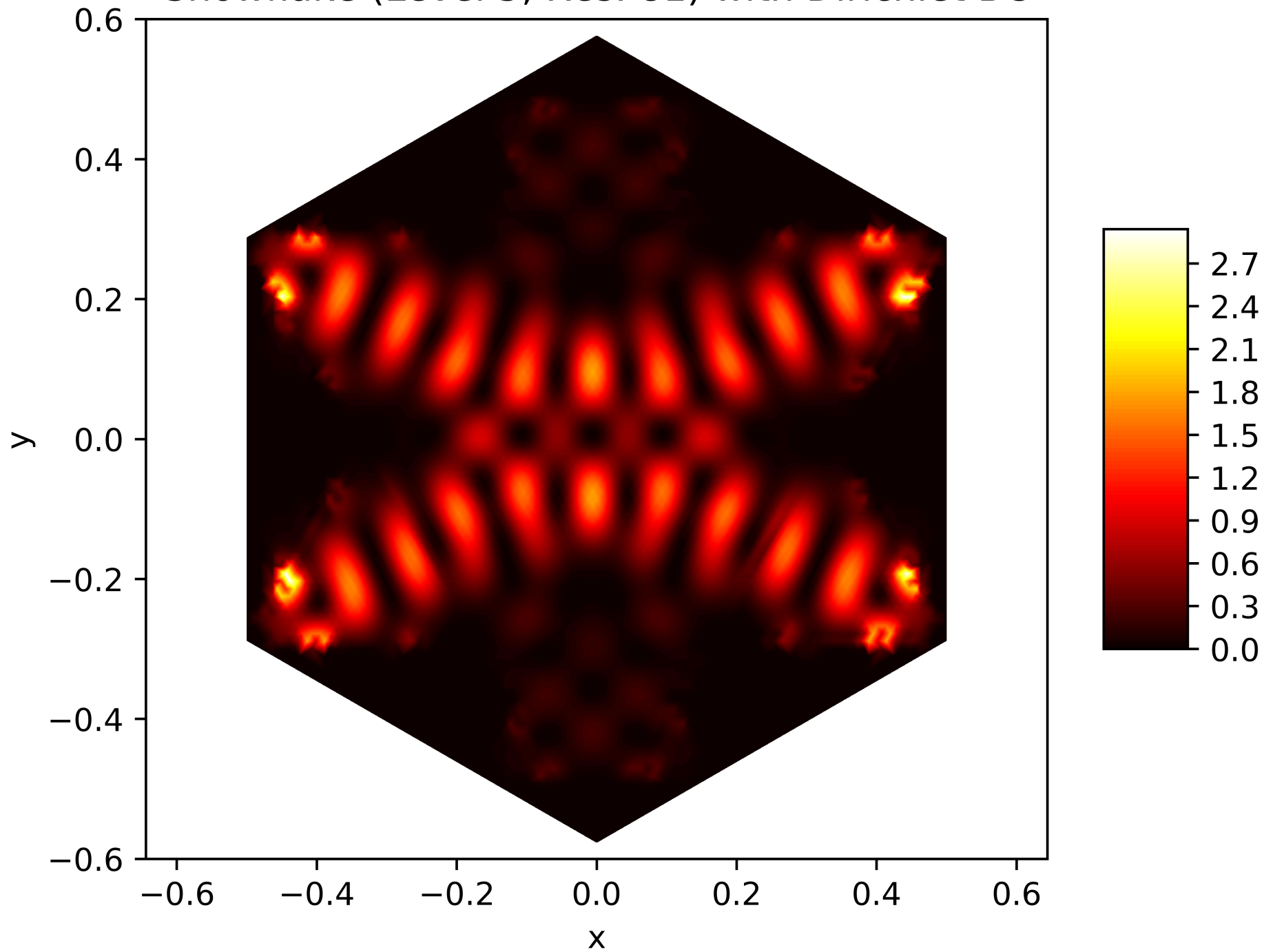
Energy Function of the 54. Eigenfunction on the Snowflake (Level 5, Res. 81) with Dirichlet BC
