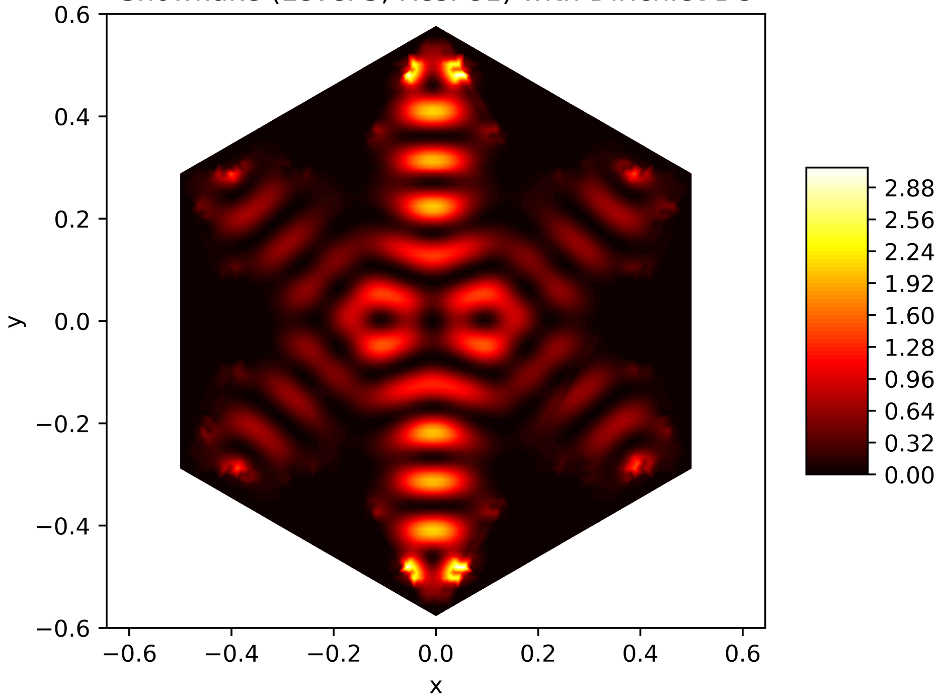
Energy Function of the 53. Eigenfunction on the Snowflake (Level 5, Res. 81) with Dirichlet BC
