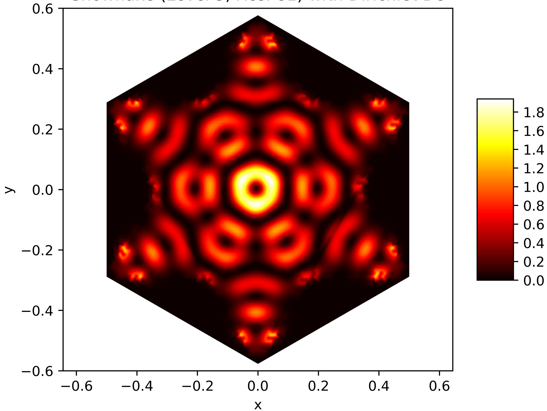
Energy Function of the 51. Eigenfunction on the Snowflake (Level 5, Res. 81) with Dirichlet BC
