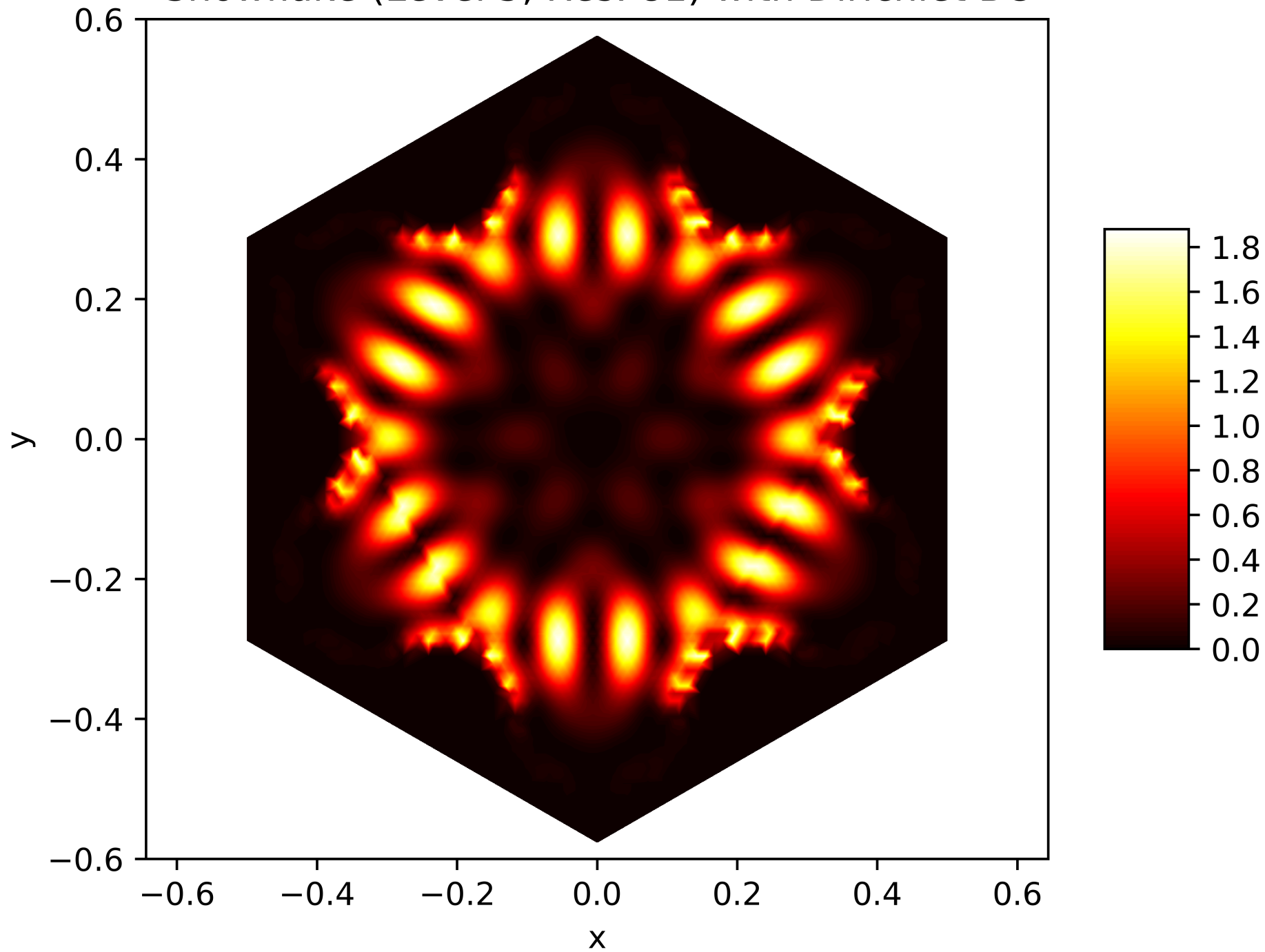
Energy Function of the 48. Eigenfunction on the Snowflake (Level 5, Res. 81) with Dirichlet BC
