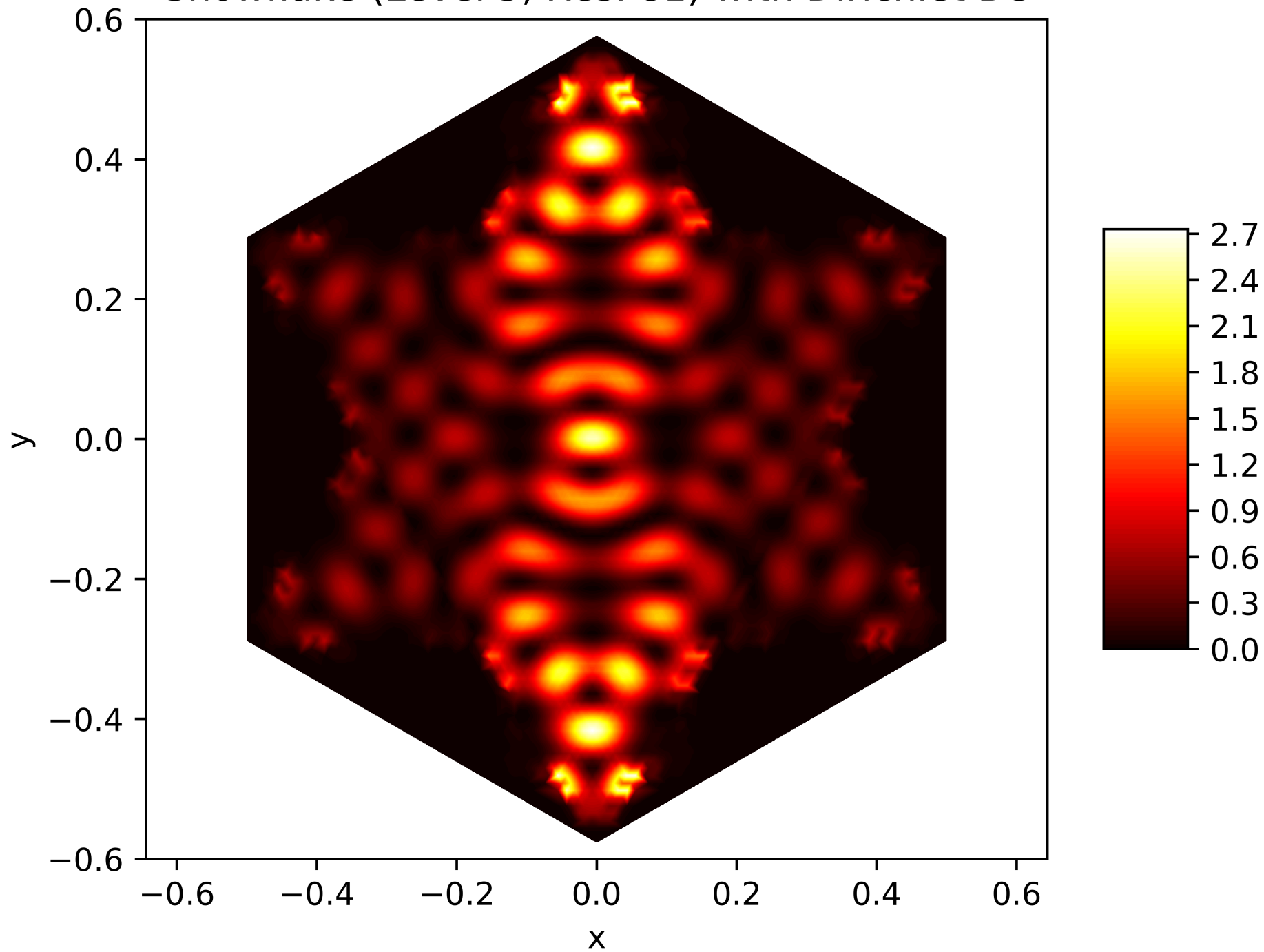
Energy Function of the 59. Eigenfunction on the Snowflake (Level 5, Res. 81) with Dirichlet BC
