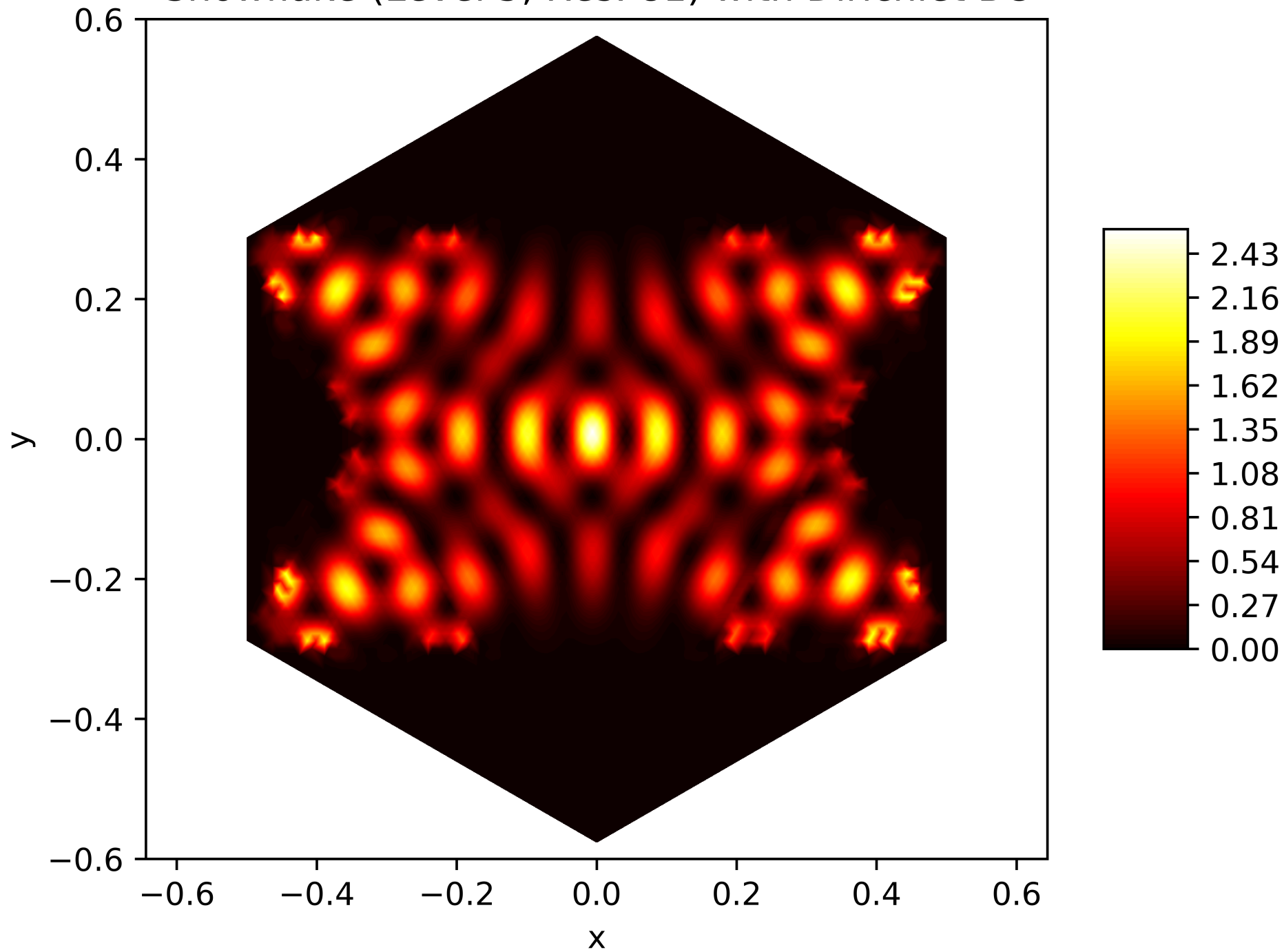
Energy Function of the 60. Eigenfunction on the Snowflake (Level 5, Res. 81) with Dirichlet BC
