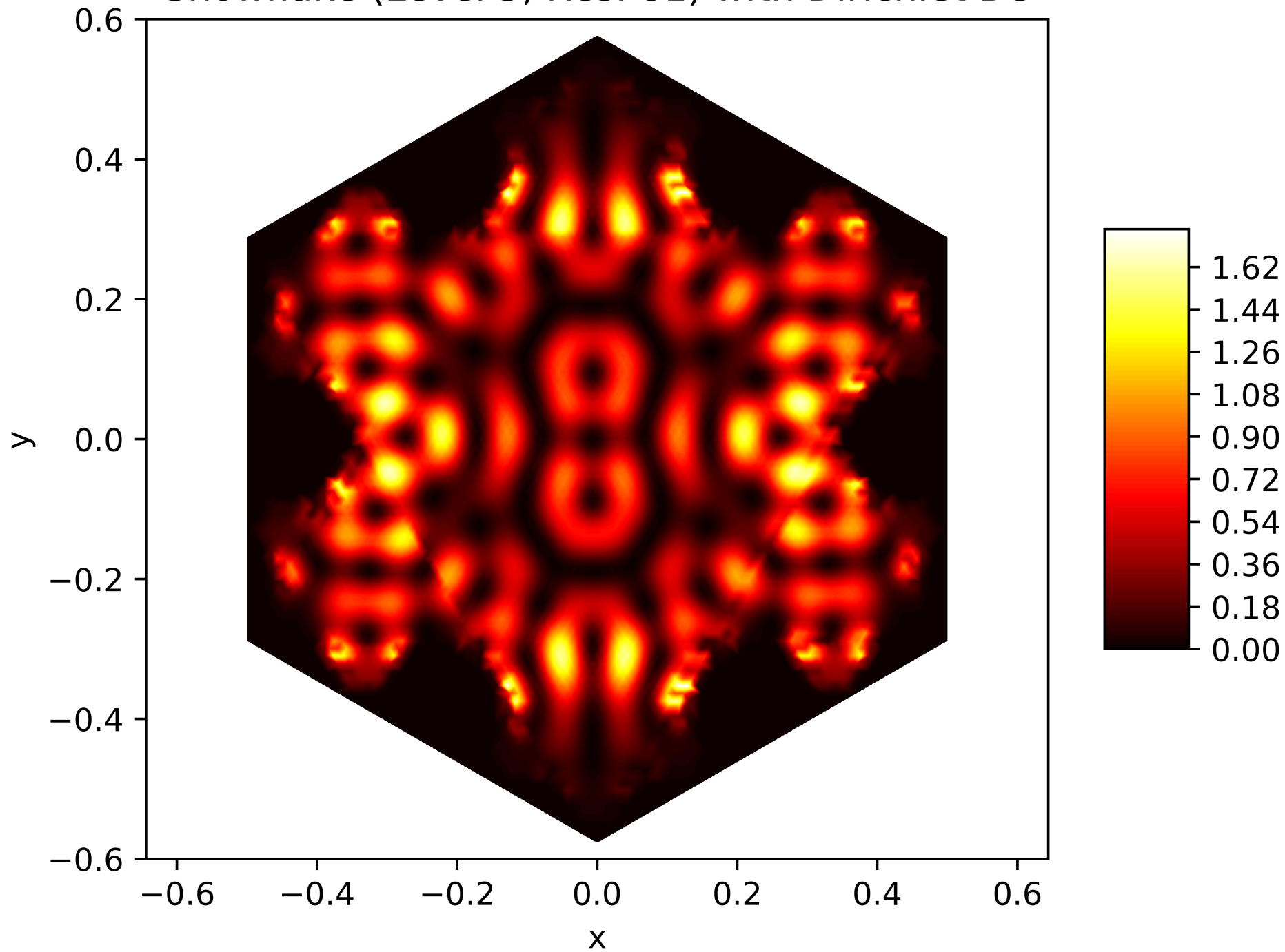
Energy Function of the 57. Eigenfunction on the Snowflake (Level 5, Res. 81) with Dirichlet BC
