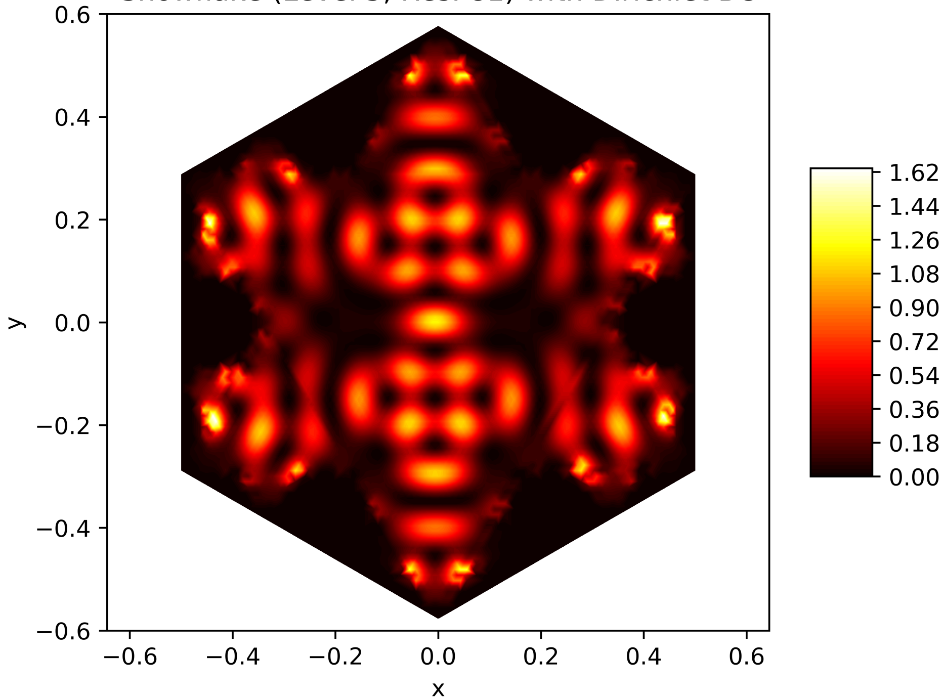
Energy Function of the 45. Eigenfunction on the Snowflake (Level 5, Res. 81) with Dirichlet BC
