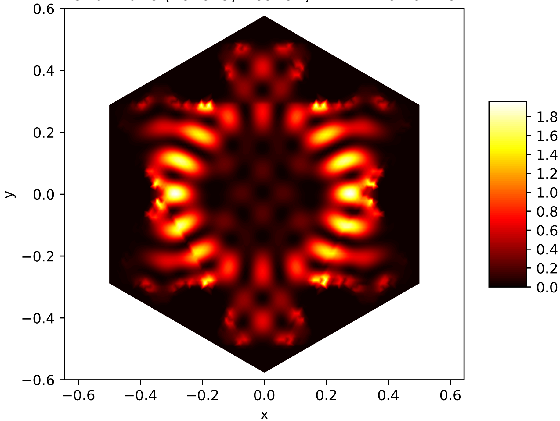
Energy Function of the 47. Eigenfunction on the Snowflake (Level 5, Res. 81) with Dirichlet BC
