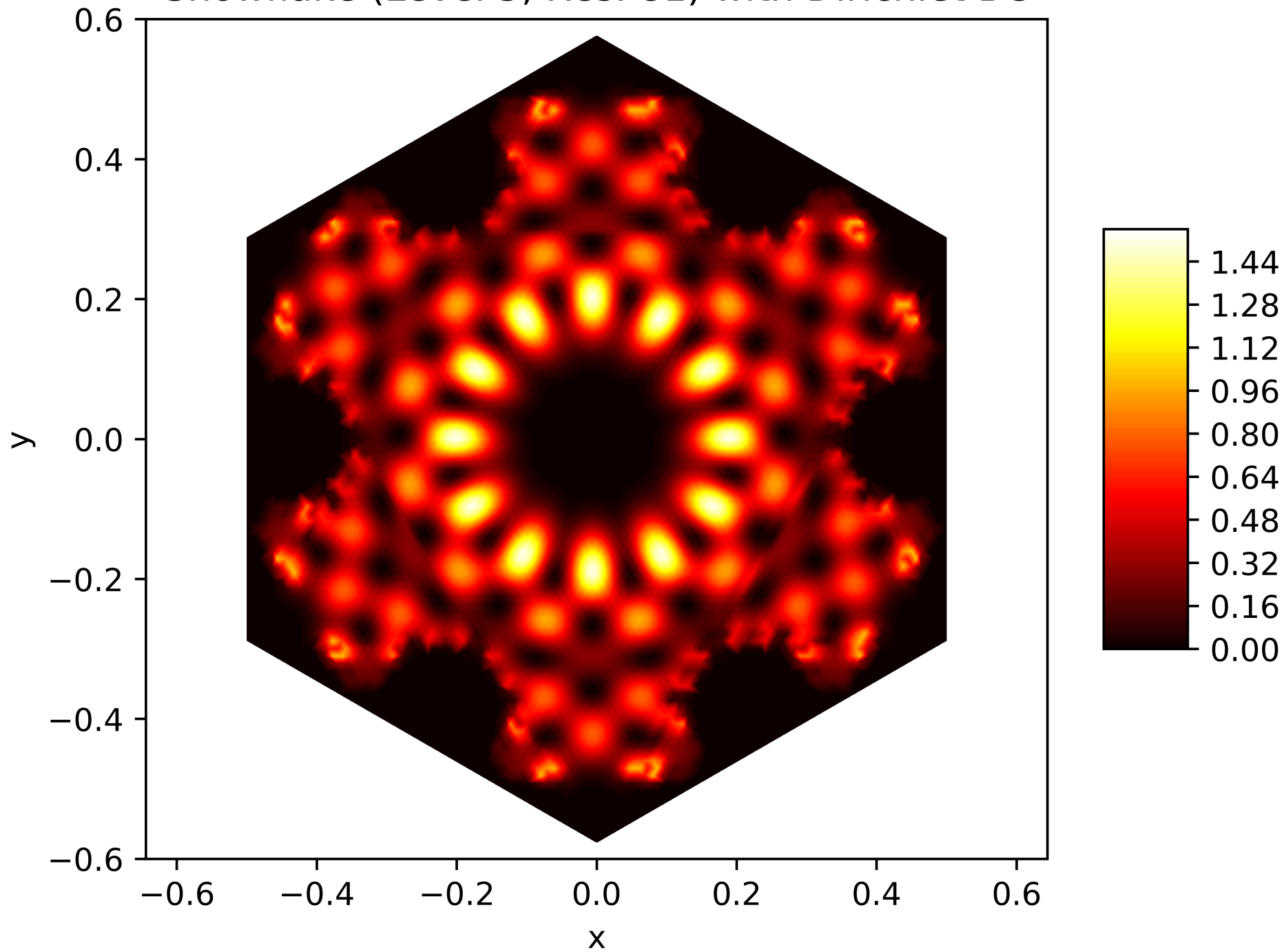
Energy Function of the 55. Eigenfunction on the Snowflake (Level 5, Res. 81) with Dirichlet BC
