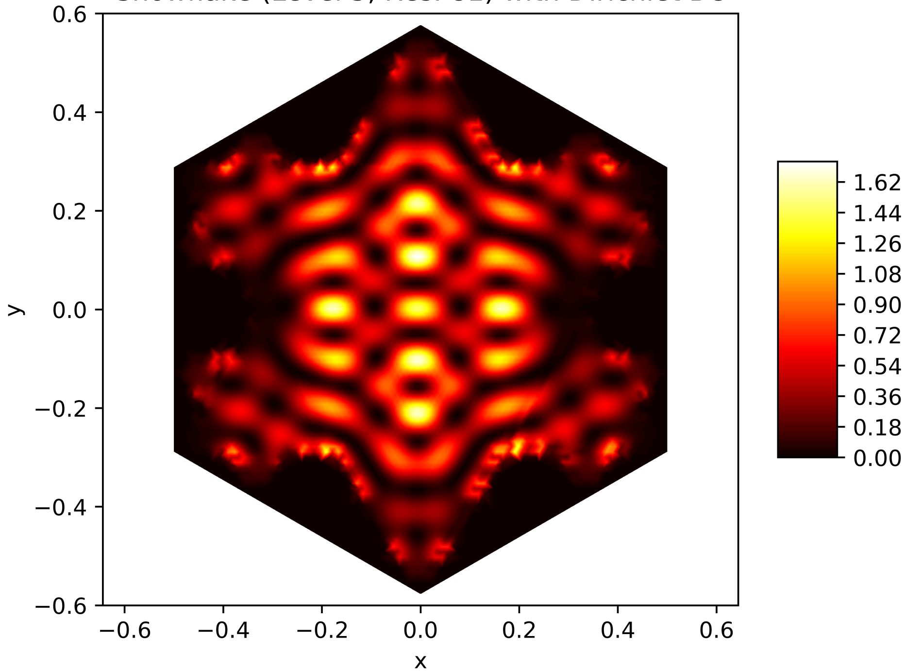
Energy Function of the 49. Eigenfunction on the Snowflake (Level 5, Res. 81) with Dirichlet BC
