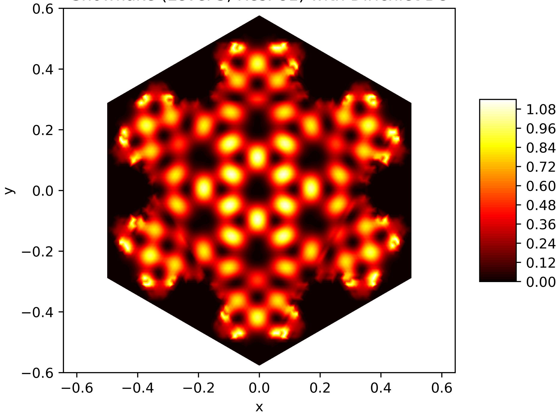
Energy Function of the 52. Eigenfunction on the Snowflake (Level 5, Res. 81) with Dirichlet BC
