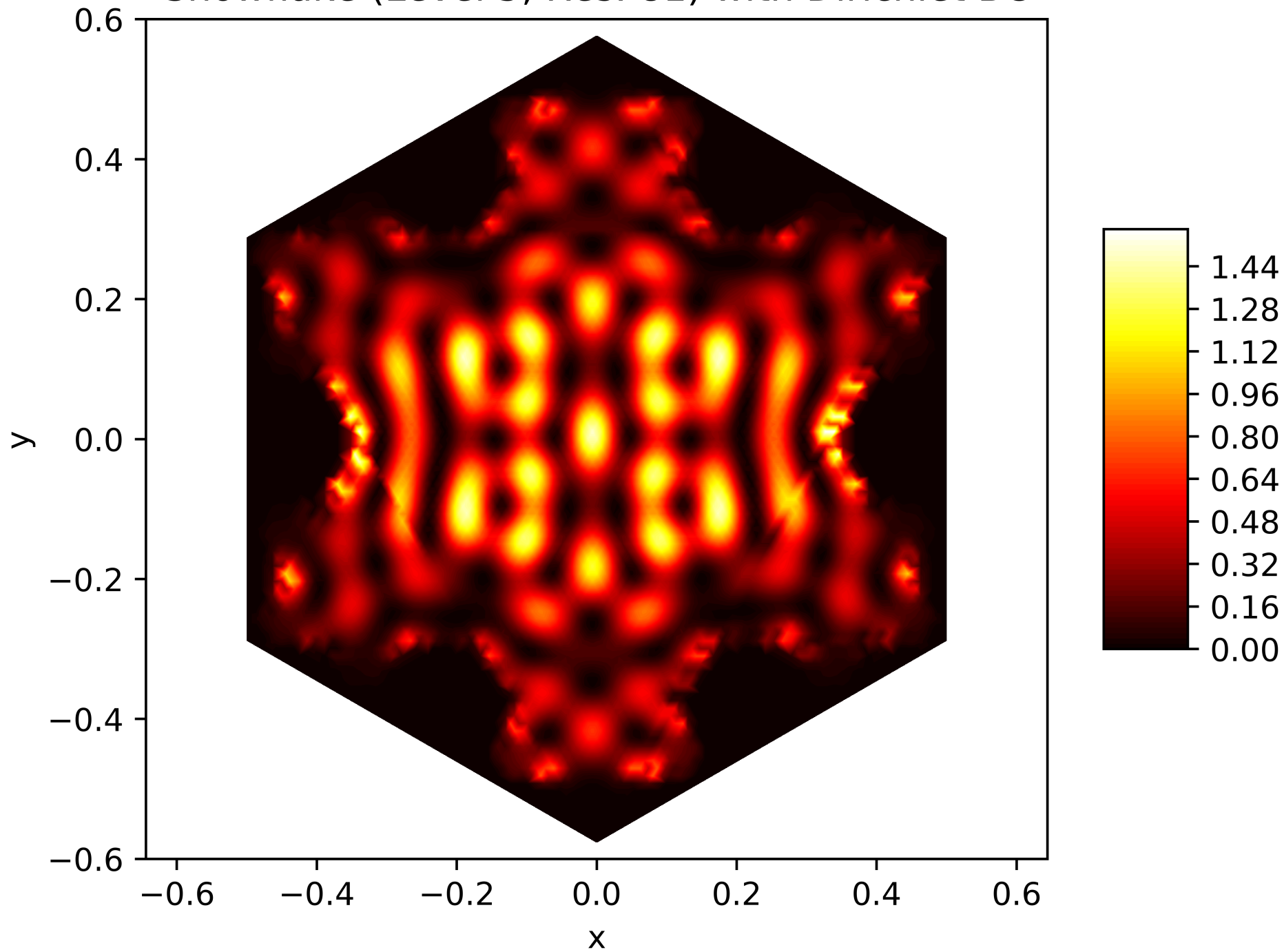
Energy Function of the 50. Eigenfunction on the Snowflake (Level 5, Res. 81) with Dirichlet BC
