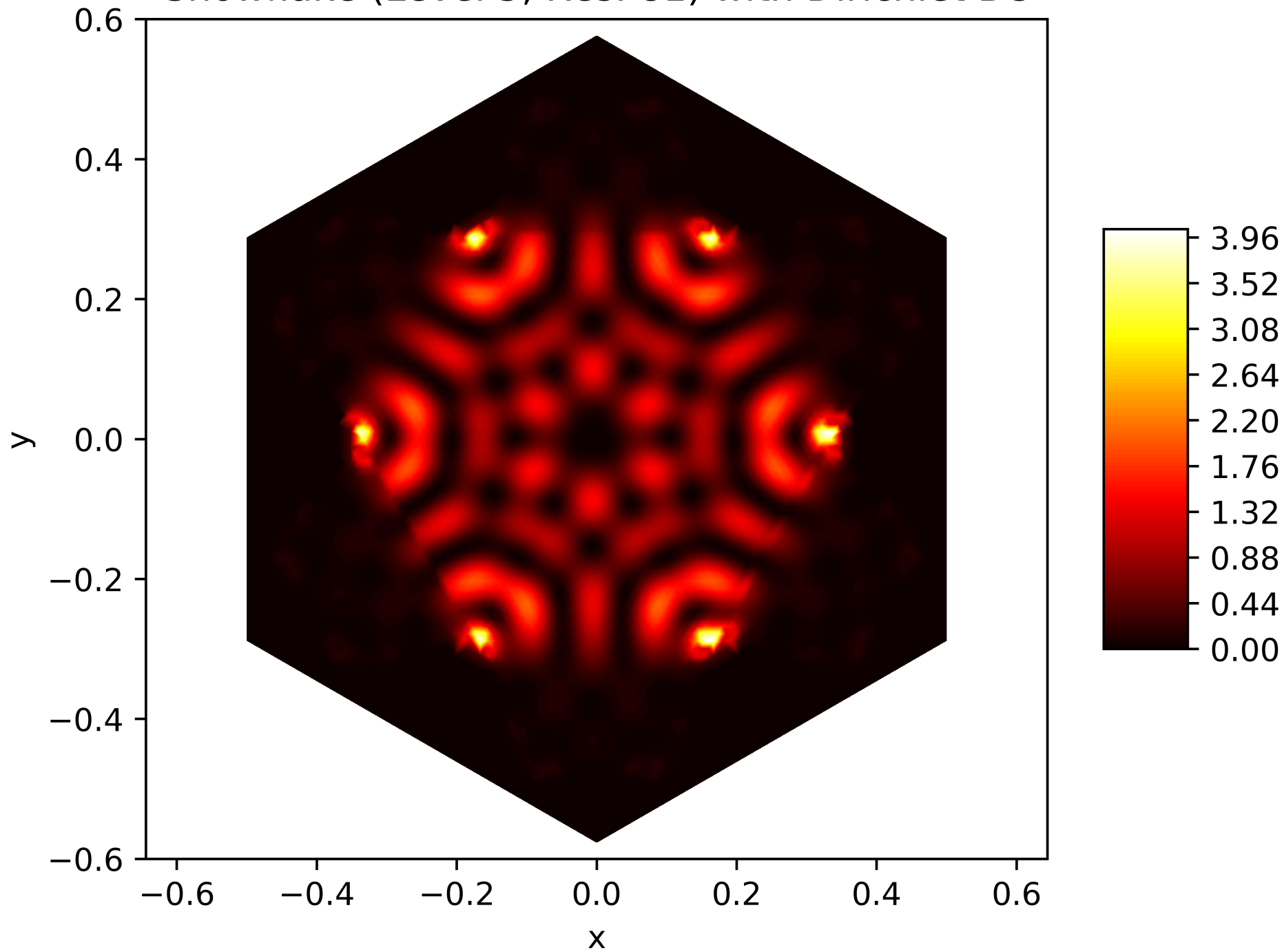
Energy Function of the 58. Eigenfunction on the Snowflake (Level 5, Res. 81) with Dirichlet BC
