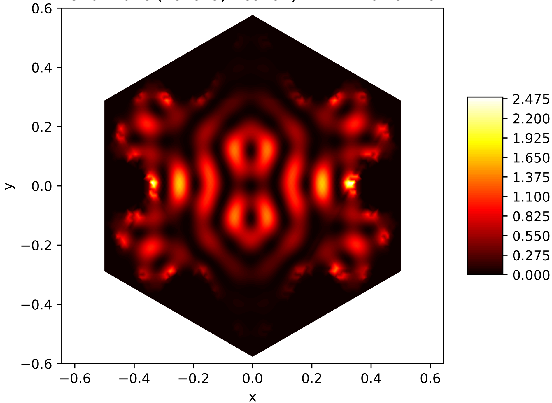
Energy Function of the 42. Eigenfunction on the Snowflake (Level 5, Res. 81) with Dirichlet BC
