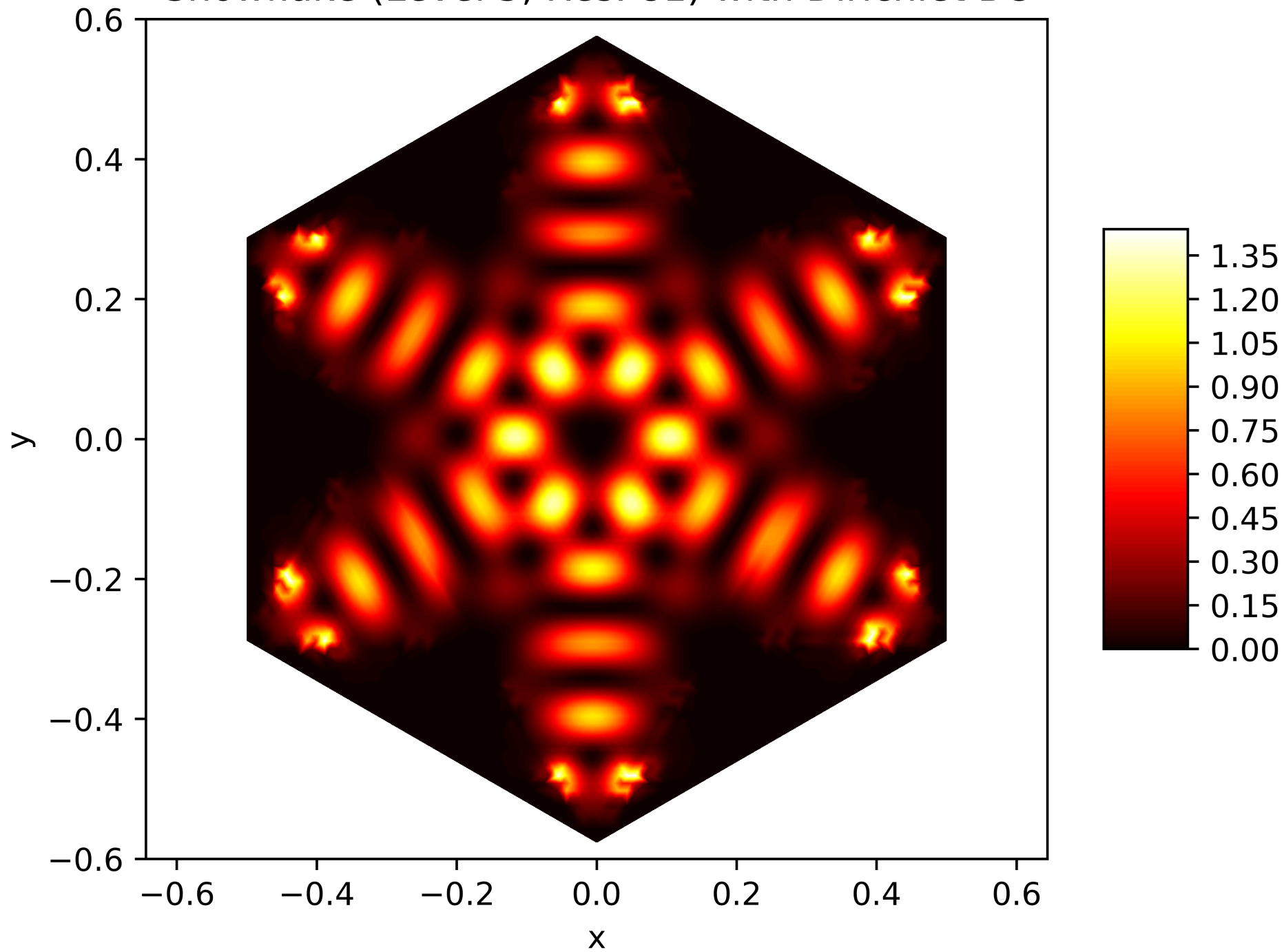
Energy Function of the 43. Eigenfunction on the Snowflake (Level 5, Res. 81) with Dirichlet BC
