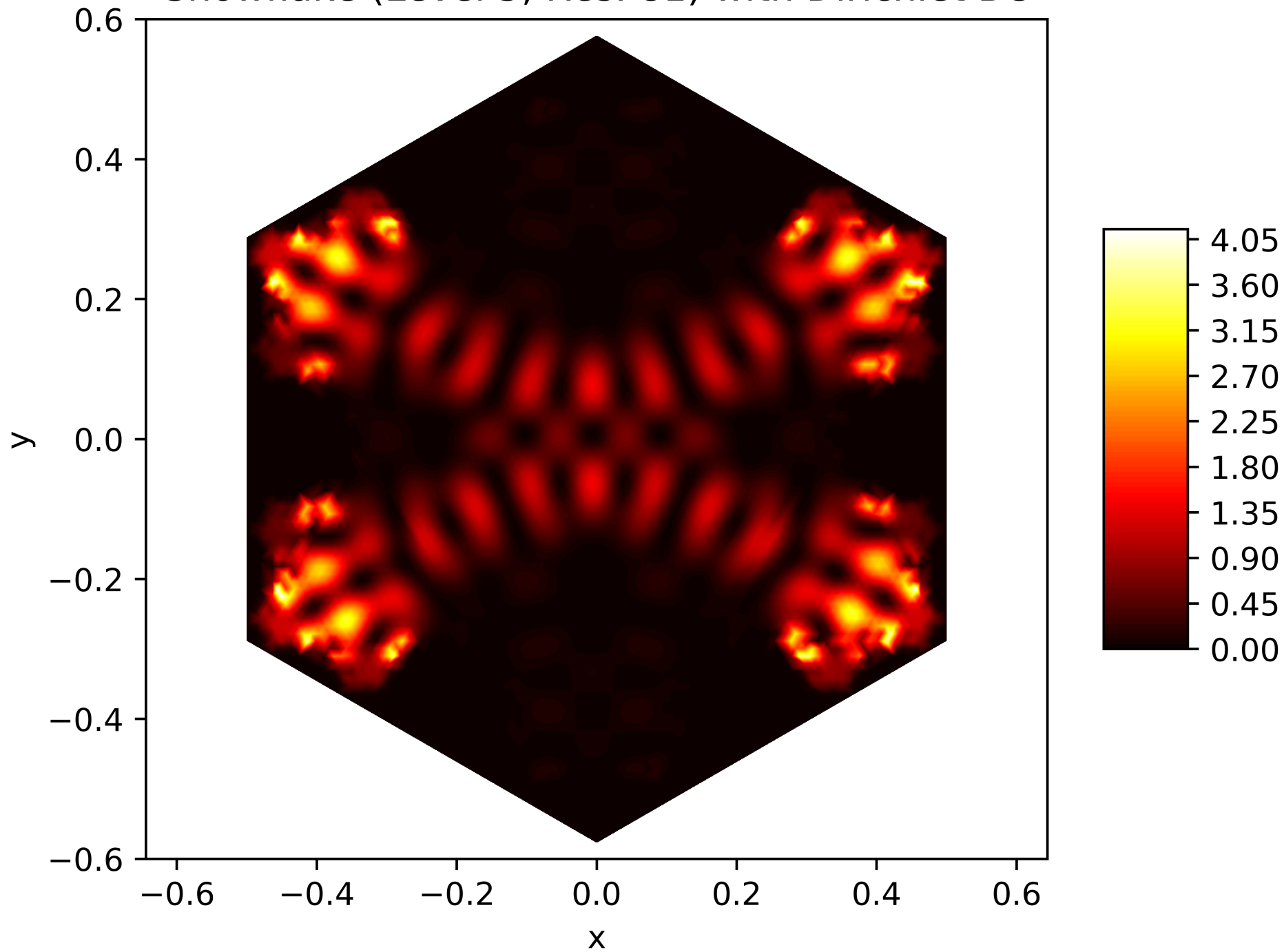
Energy Function of the 70. Eigenfunction on the Snowflake (Level 5, Res. 81) with Dirichlet BC
