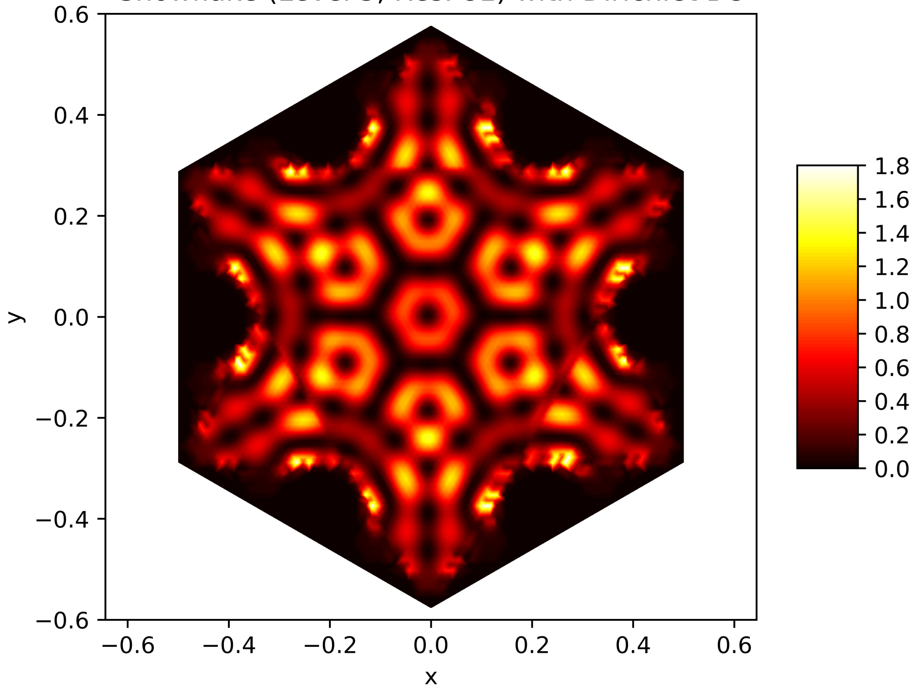
Energy Function of the 61. Eigenfunction on the Snowflake (Level 5, Res. 81) with Dirichlet BC
