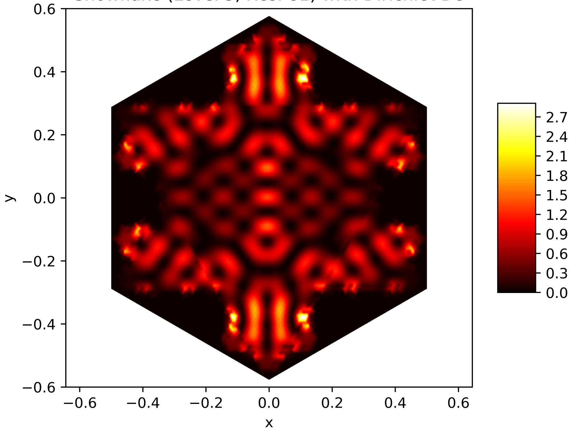
Energy Function of the 67. Eigenfunction on the Snowflake (Level 5, Res. 81) with Dirichlet BC
