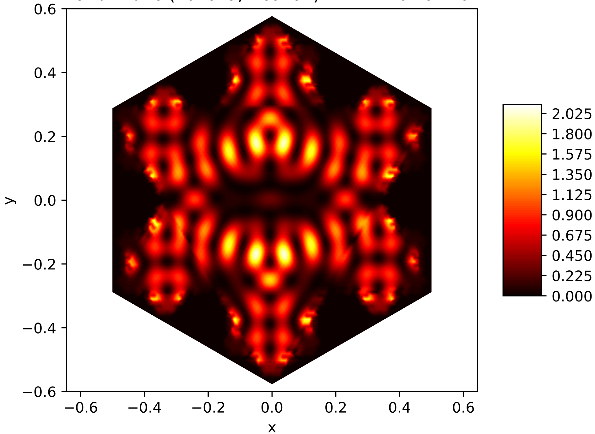
Energy Function of the 64. Eigenfunction on the Snowflake (Level 5, Res. 81) with Dirichlet BC
