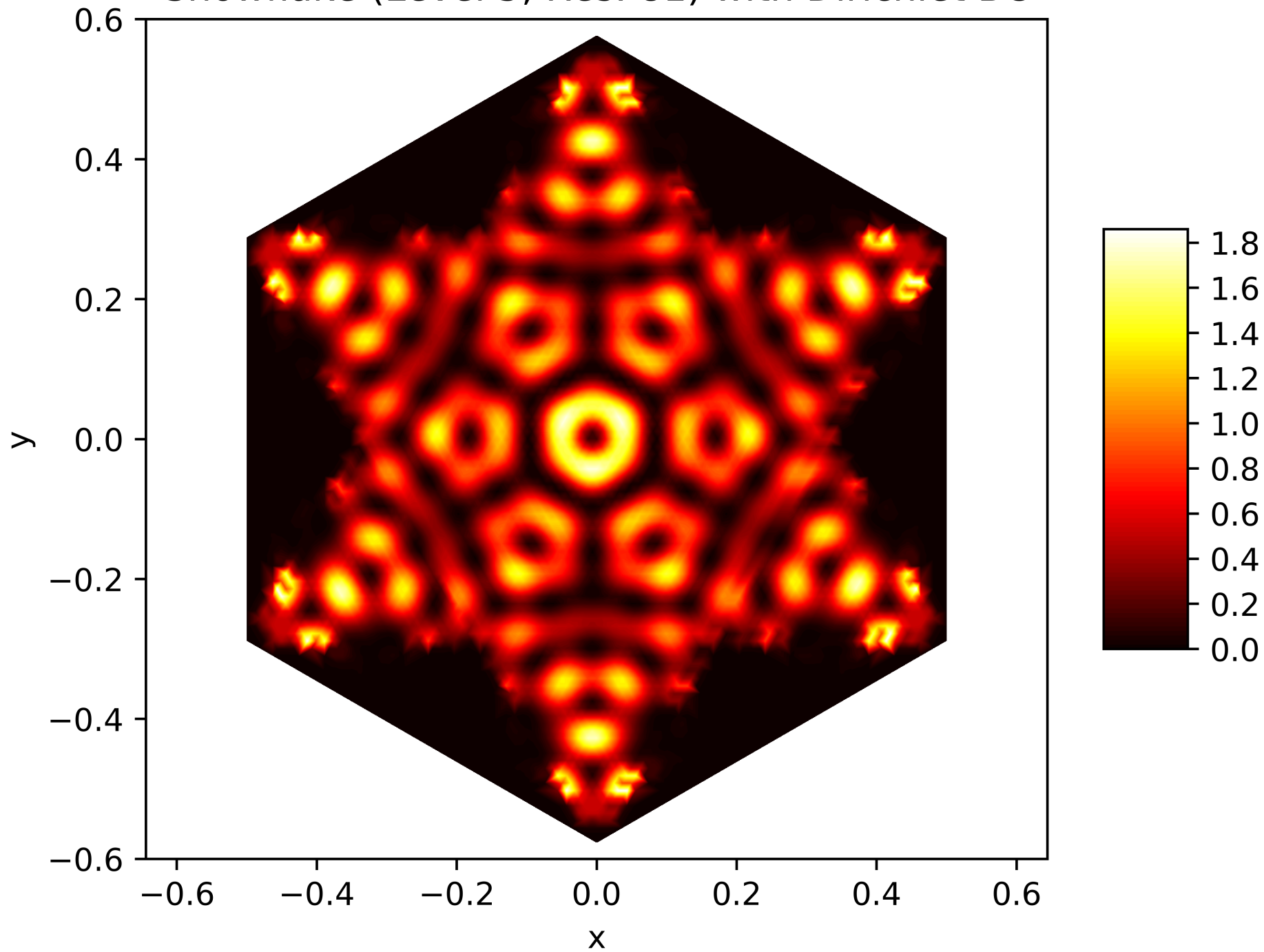
Energy Function of the 71. Eigenfunction on the Snowflake (Level 5, Res. 81) with Dirichlet BC
