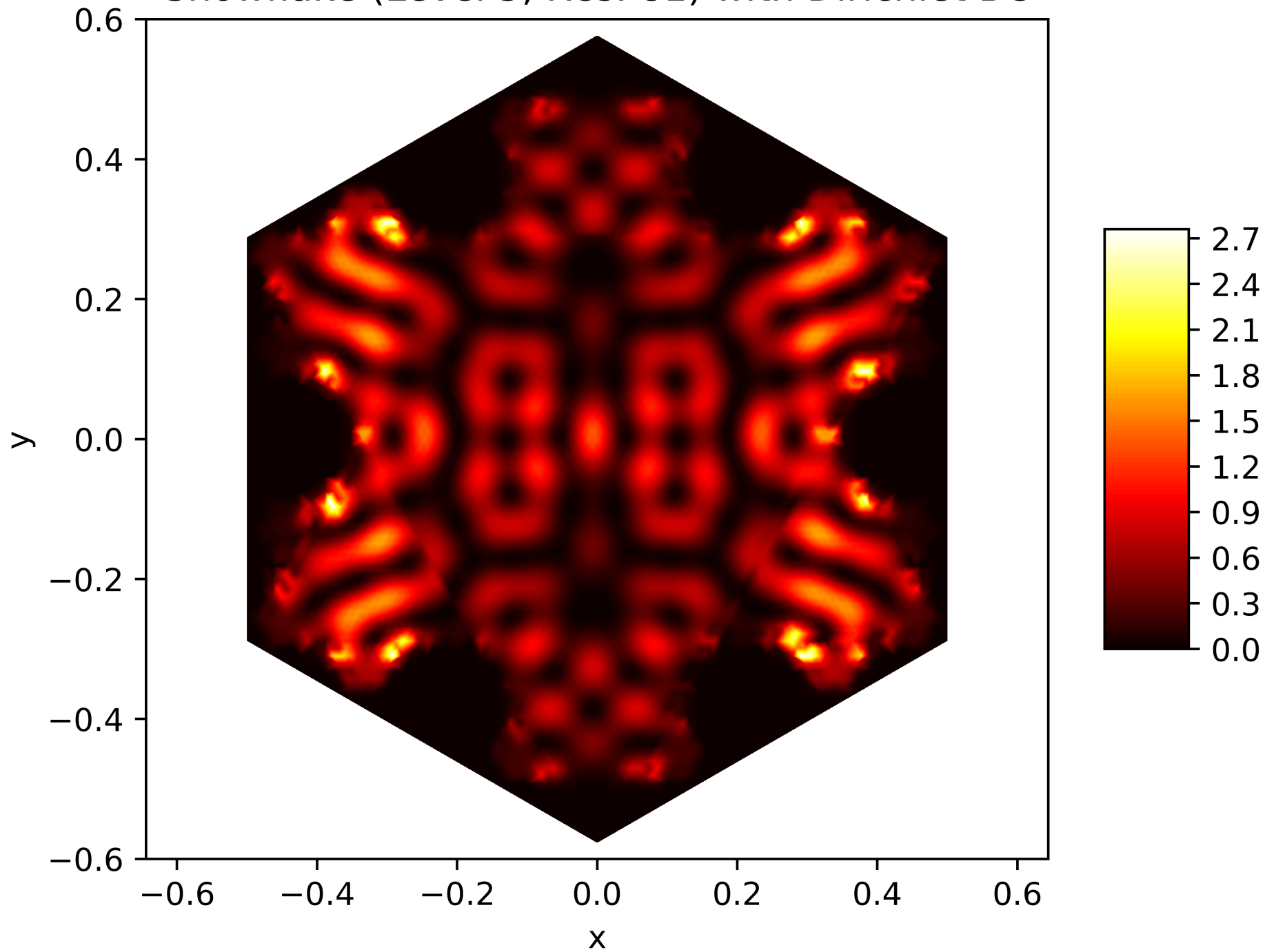
Energy Function of the 68. Eigenfunction on the Snowflake (Level 5, Res. 81) with Dirichlet BC
