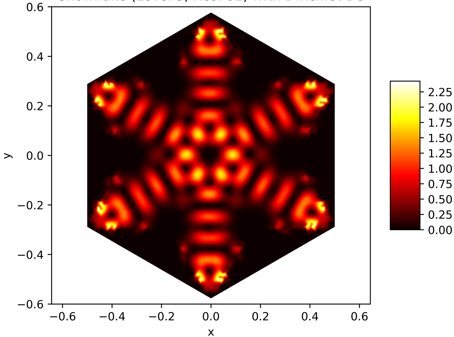
Energy Function of the 62. Eigenfunction on the Snowflake (Level 5, Res. 81) with Dirichlet BC
