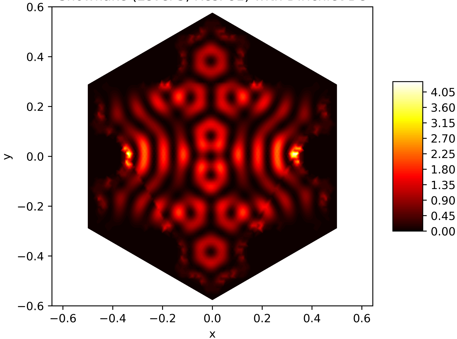
Energy Function of the 75. Eigenfunction on the Snowflake (Level 5, Res. 81) with Dirichlet BC
