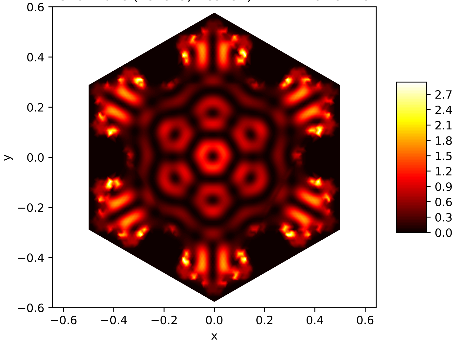
Energy Function of the 72. Eigenfunction on the Snowflake (Level 5, Res. 81) with Dirichlet BC
