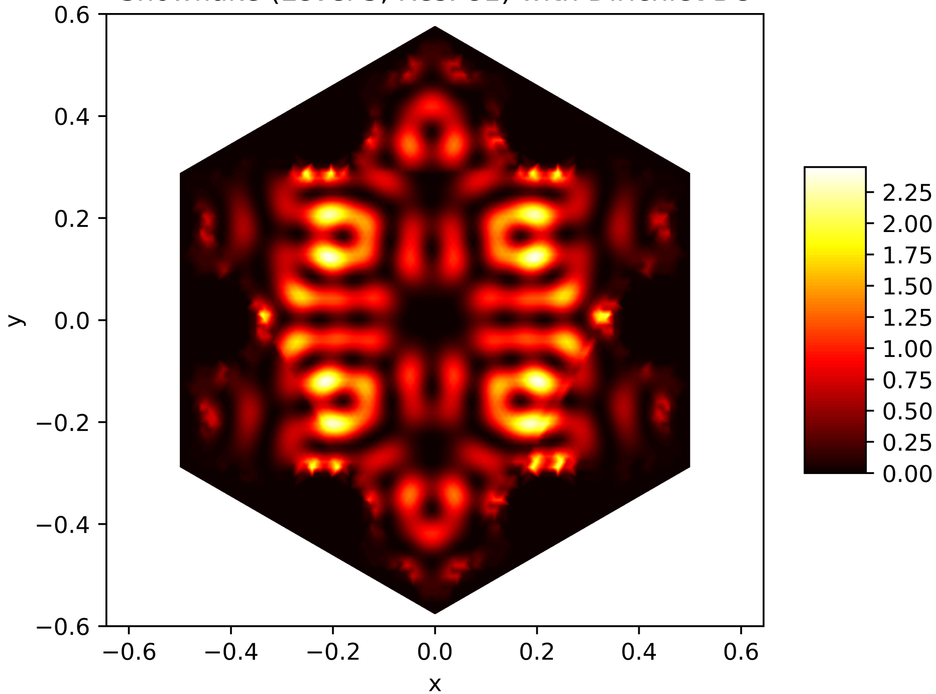
Energy Function of the 66. Eigenfunction on the Snowflake (Level 5, Res. 81) with Dirichlet BC
