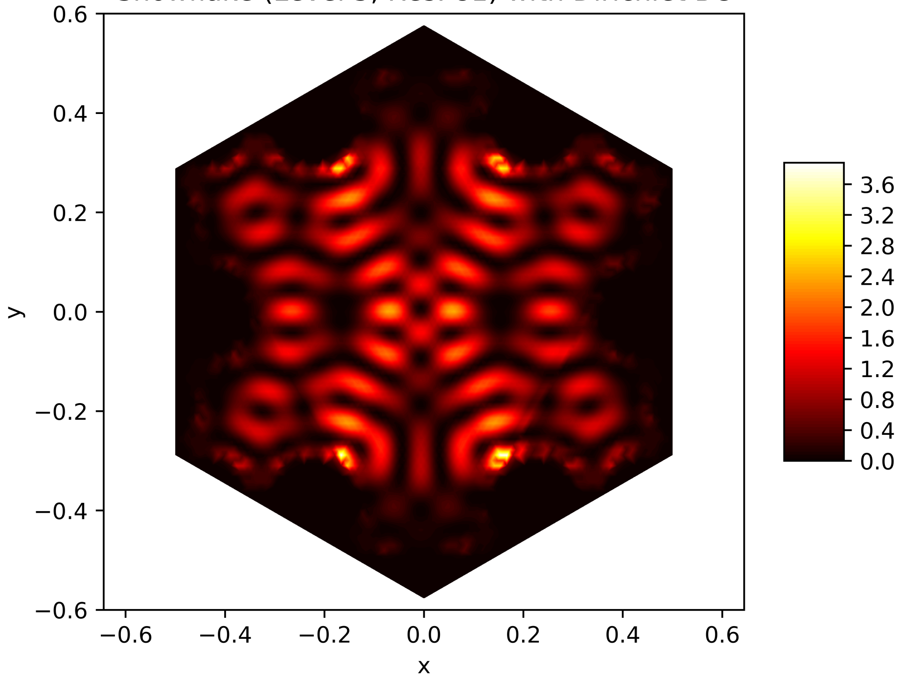
Energy Function of the 74. Eigenfunction on the Snowflake (Level 5, Res. 81) with Dirichlet BC
