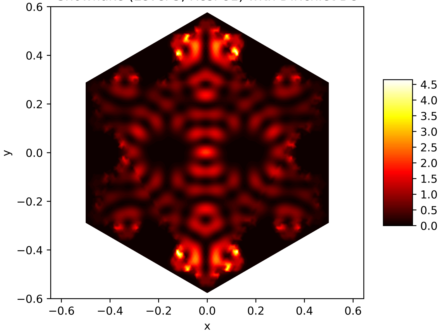
Energy Function of the 78. Eigenfunction on the Snowflake (Level 5, Res. 81) with Dirichlet BC
