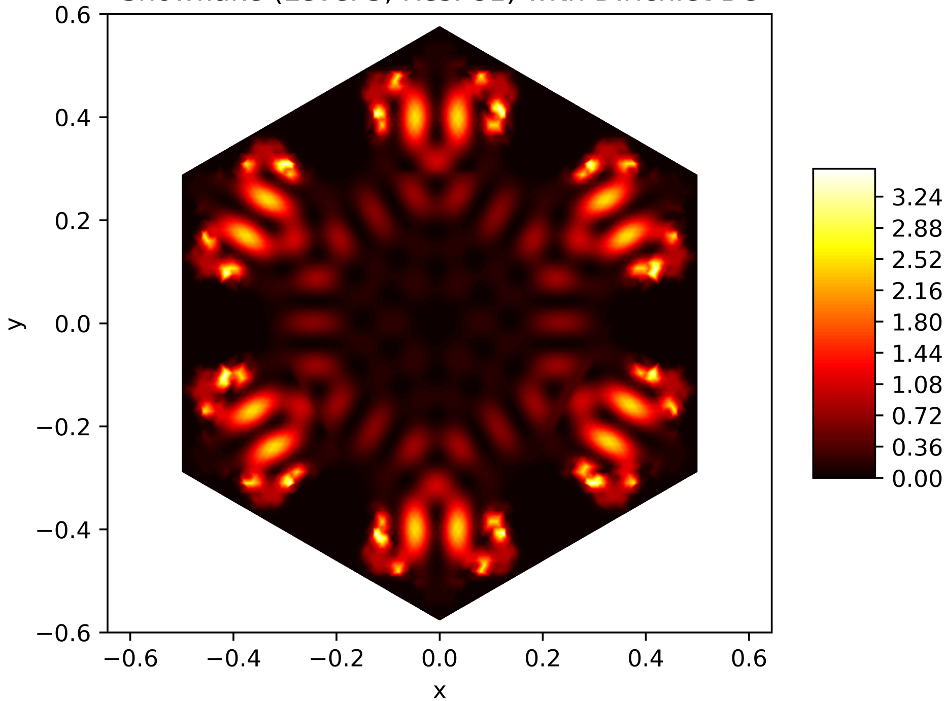
Energy Function of the 73. Eigenfunction on the Snowflake (Level 5, Res. 81) with Dirichlet BC
