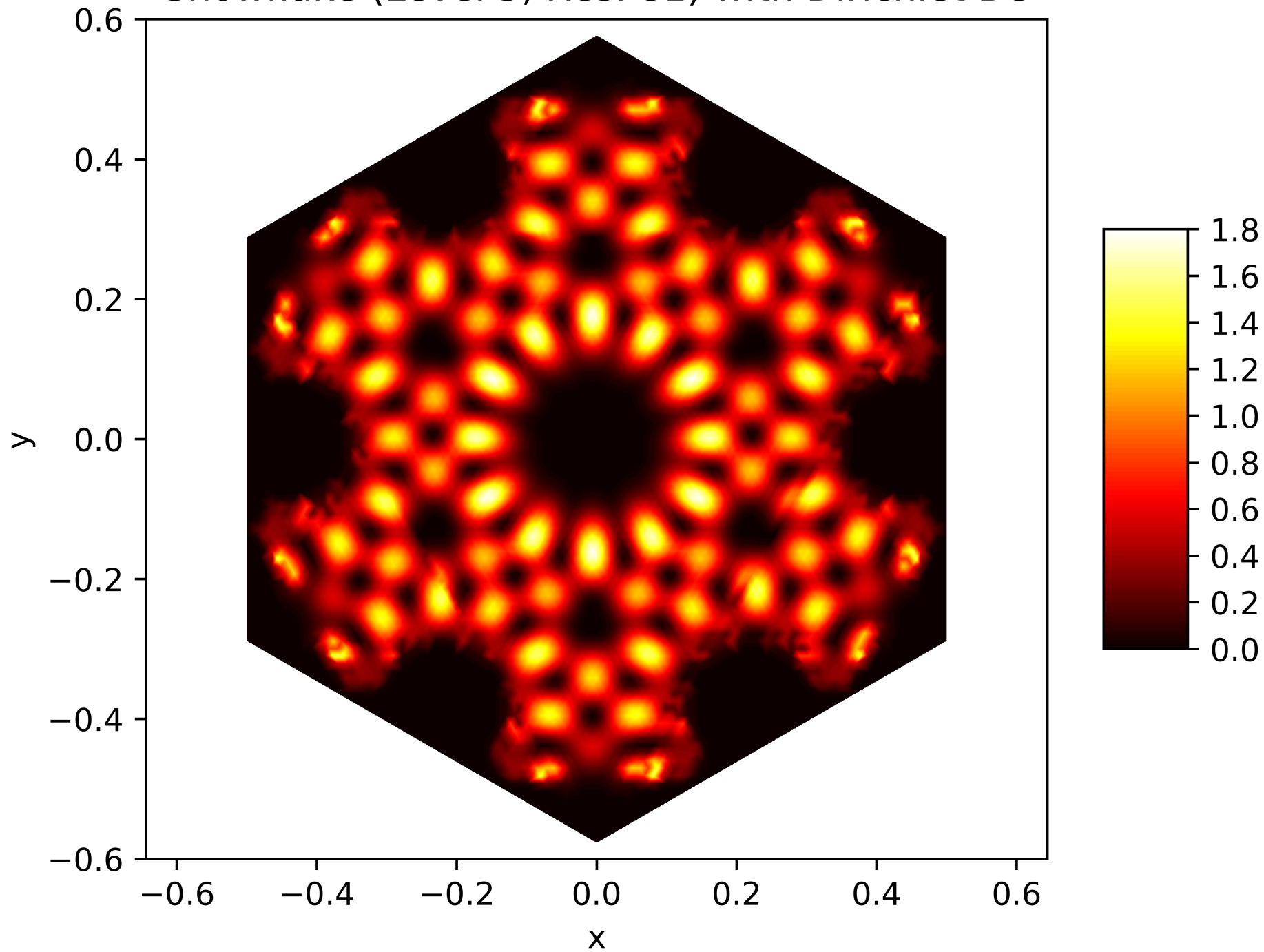
Energy Function of the 77. Eigenfunction on the Snowflake (Level 5, Res. 81) with Dirichlet BC
