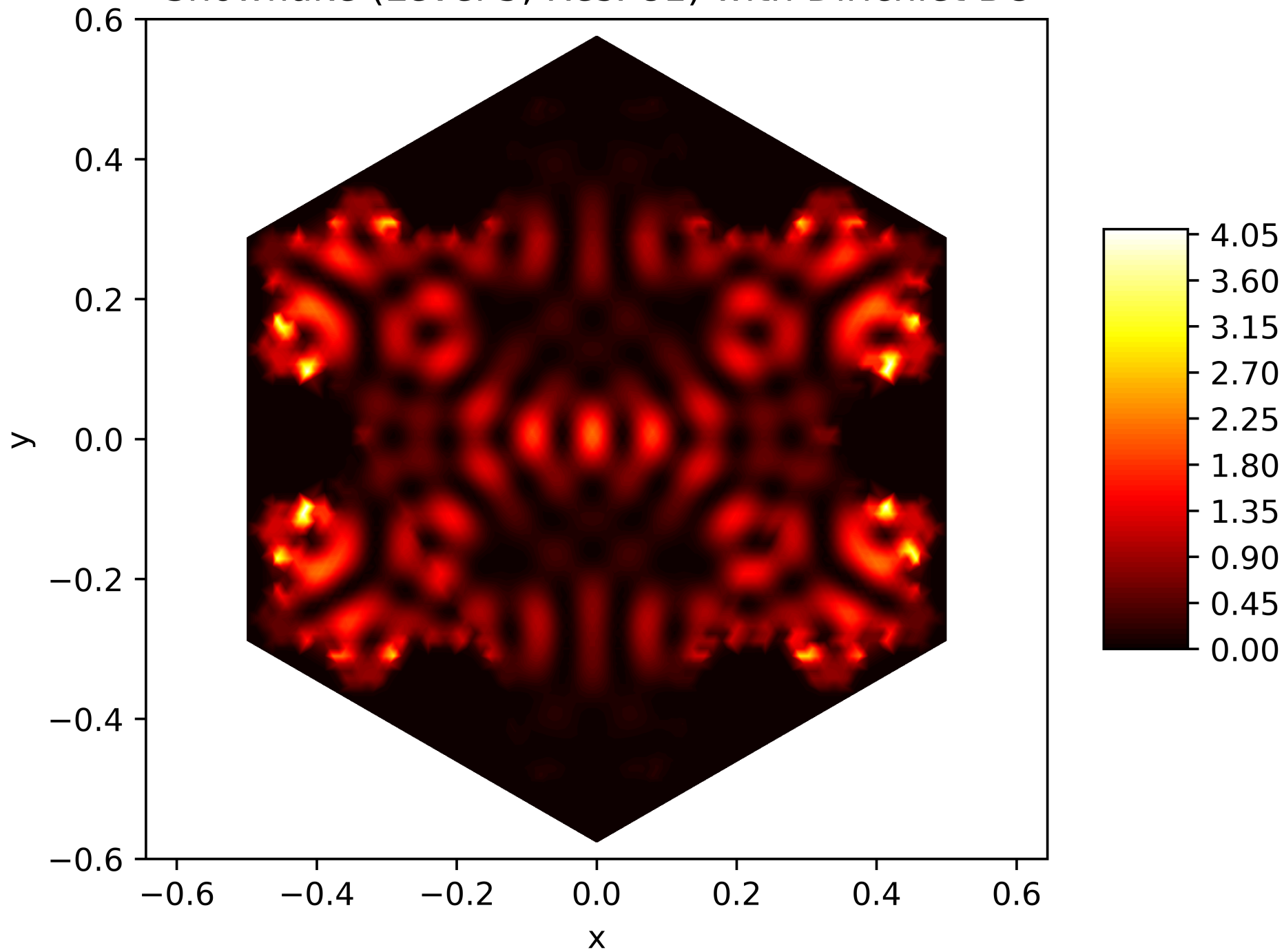
Energy Function of the 79. Eigenfunction on the Snowflake (Level 5, Res. 81) with Dirichlet BC
