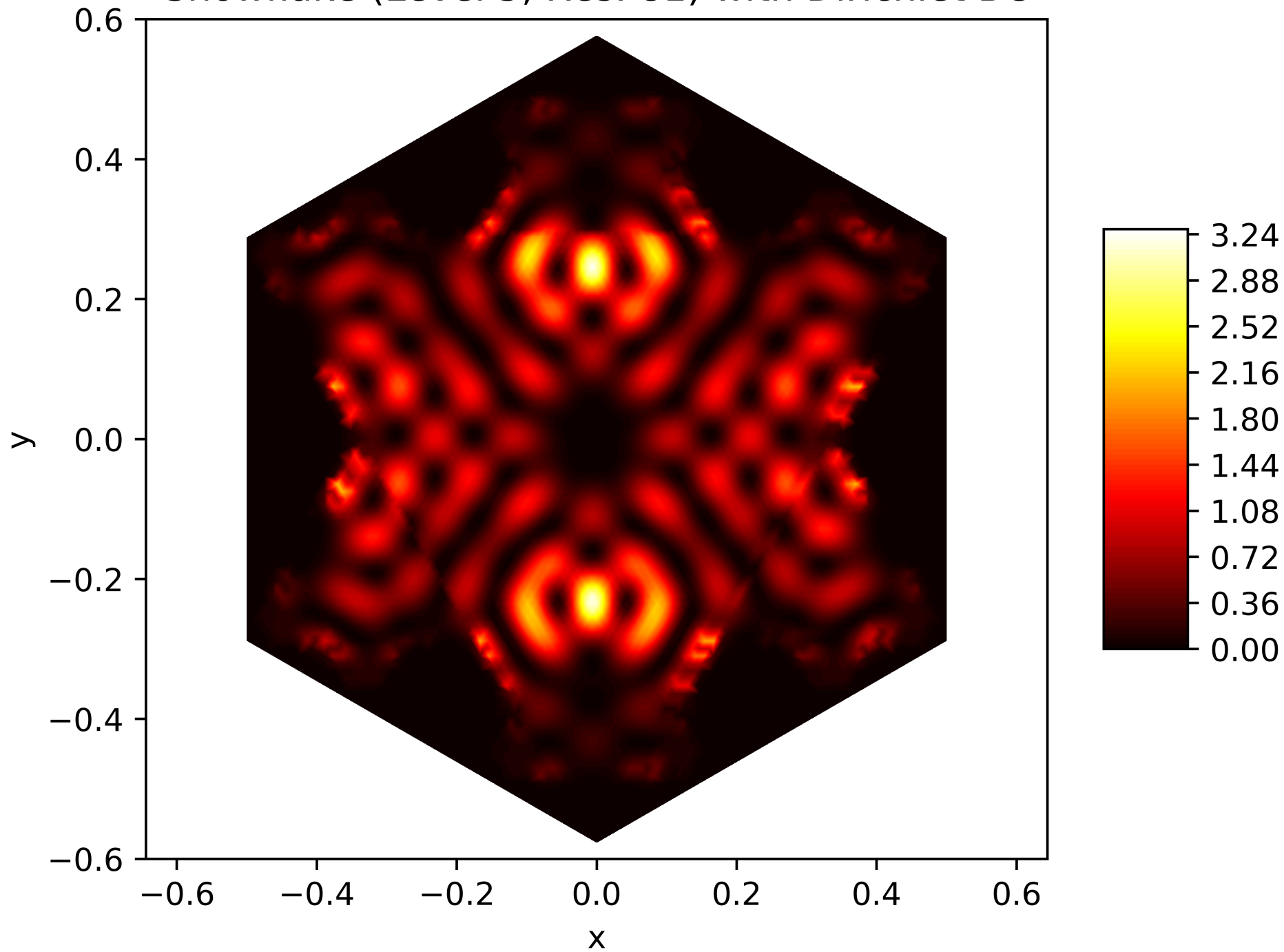
Energy Function of the 65. Eigenfunction on the Snowflake (Level 5, Res. 81) with Dirichlet BC
