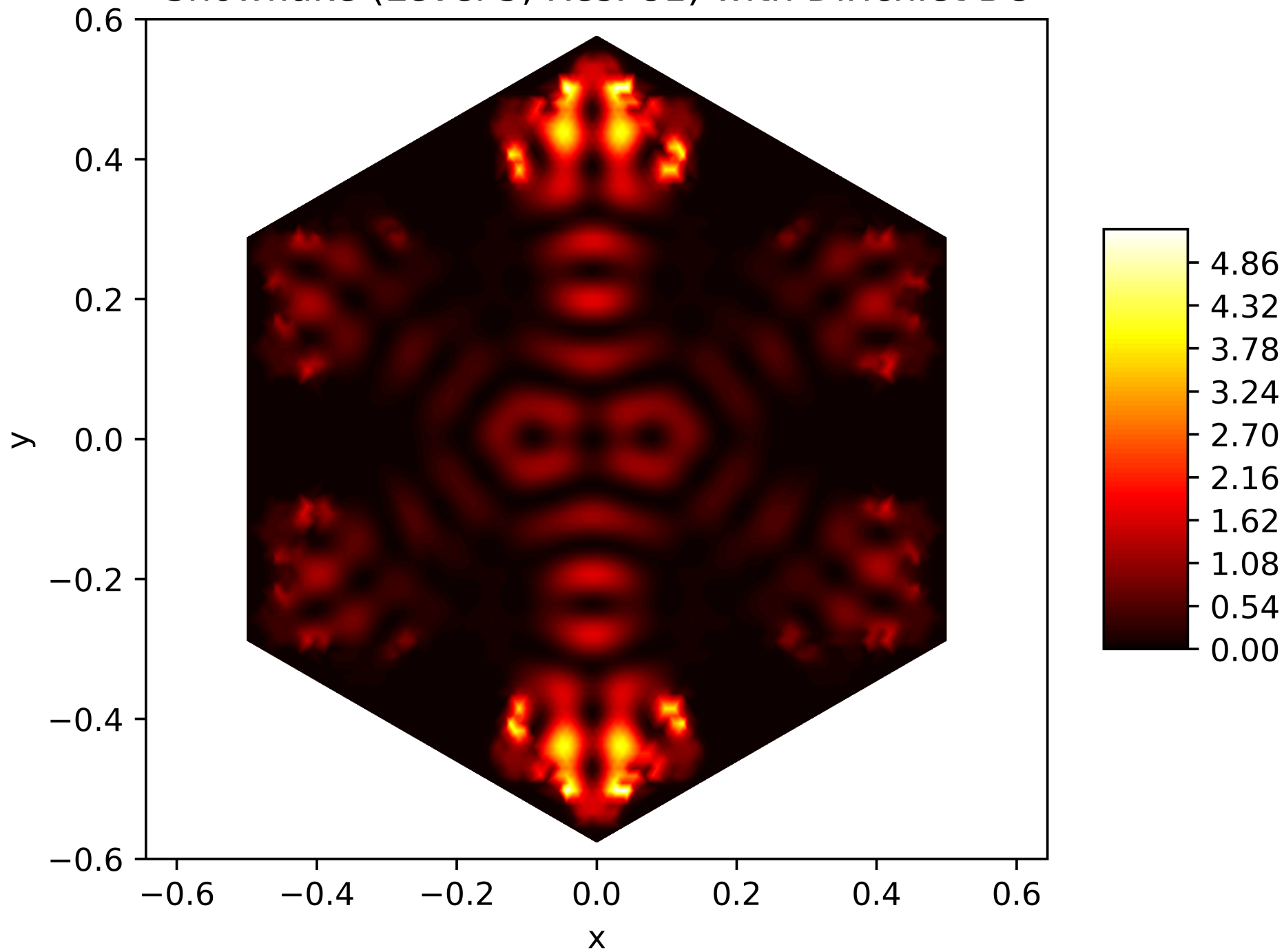
Energy Function of the 69. Eigenfunction on the Snowflake (Level 5, Res. 81) with Dirichlet BC
