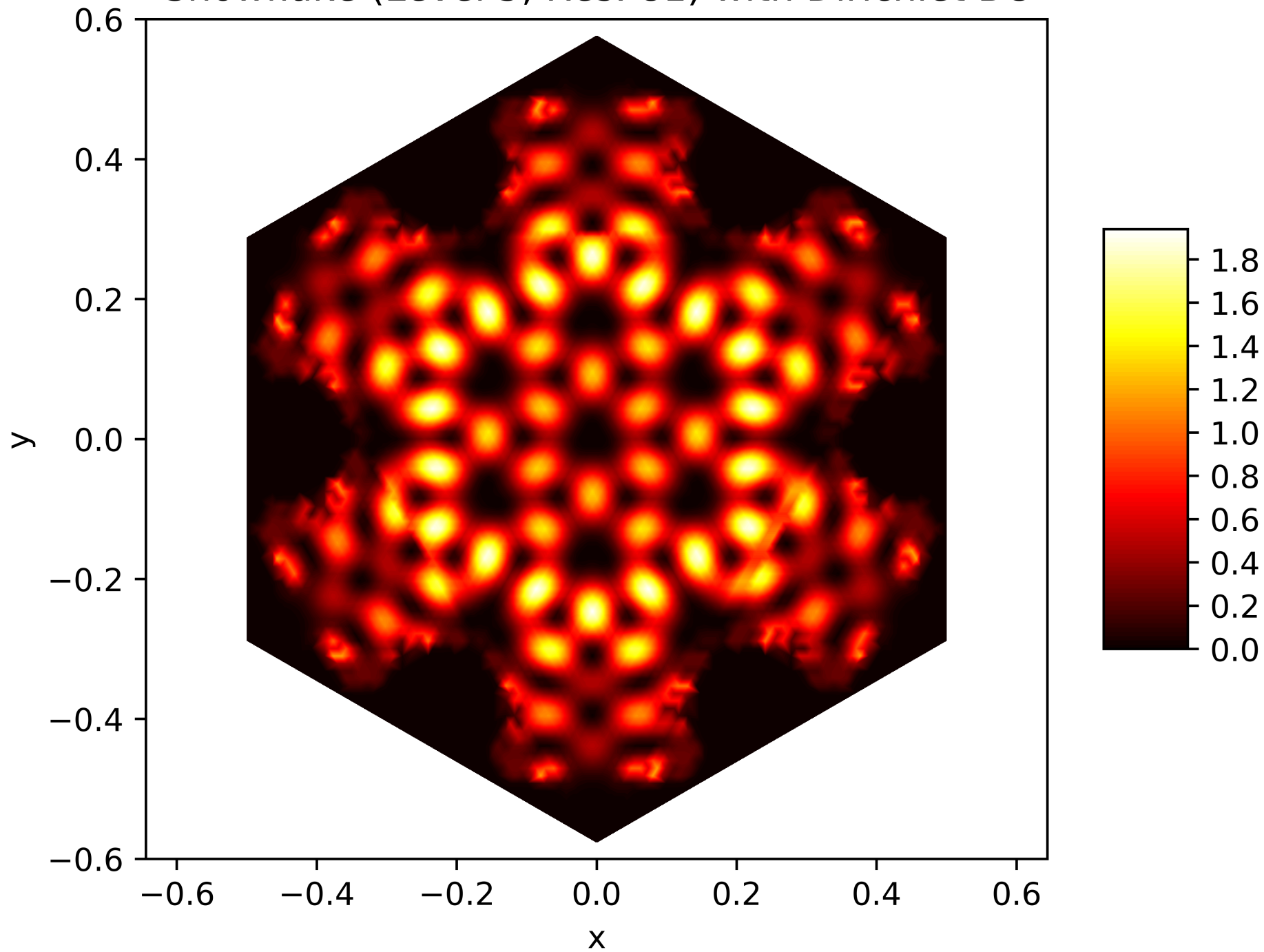
Energy Function of the 76. Eigenfunction on the Snowflake (Level 5, Res. 81) with Dirichlet BC
