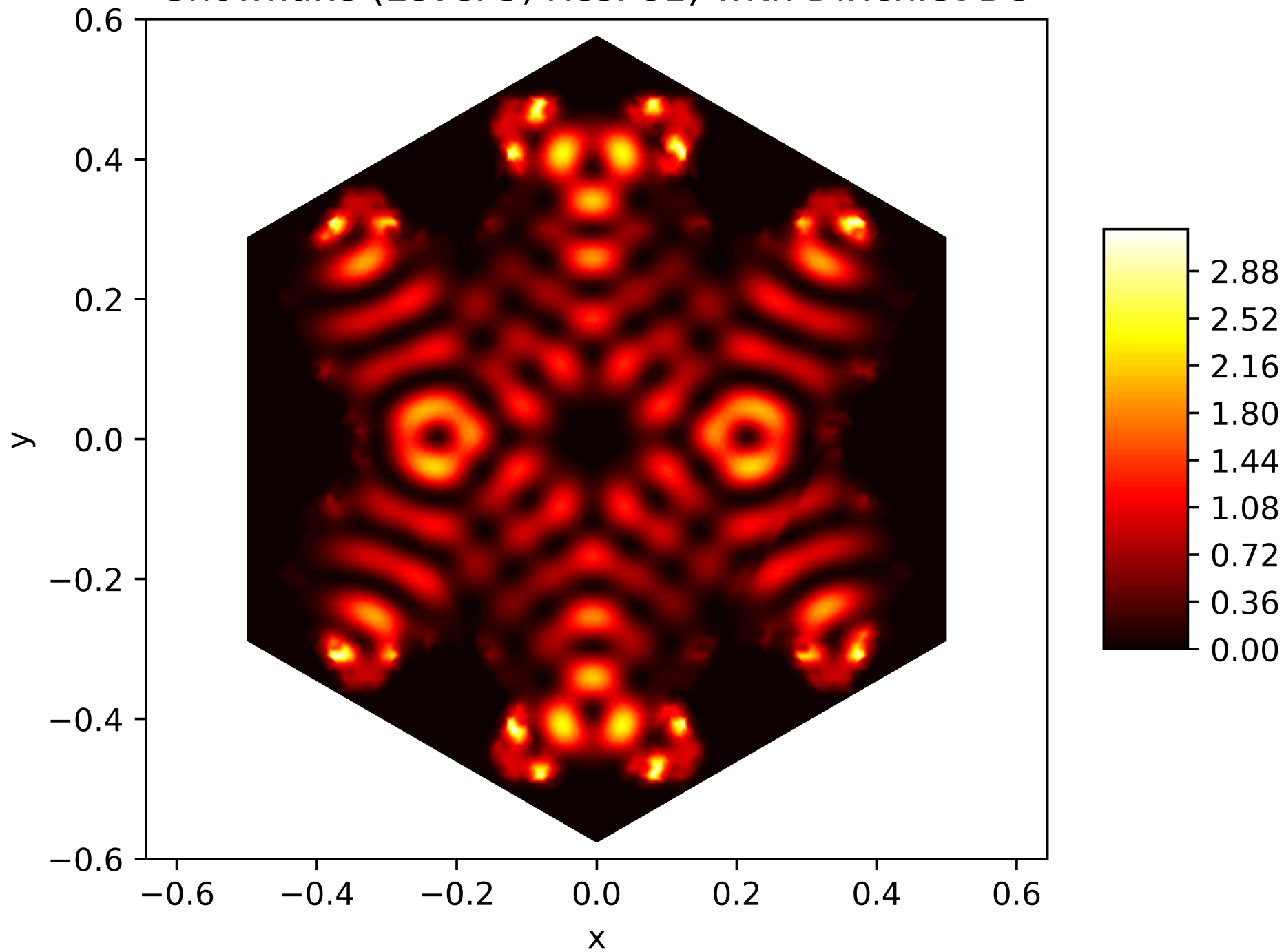
Energy Function of the 80. Eigenfunction on the Snowflake (Level 5, Res. 81) with Dirichlet BC
