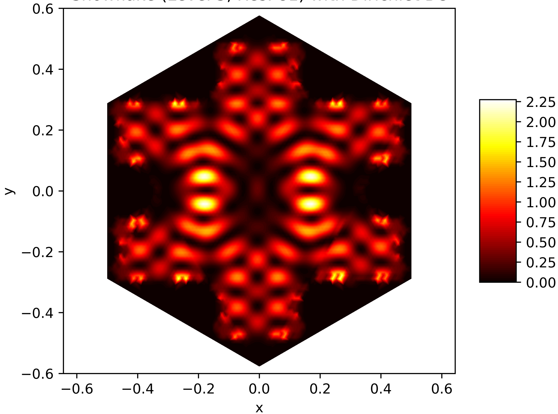
Energy Function of the 63. Eigenfunction on the Snowflake (Level 5, Res. 81) with Dirichlet BC
