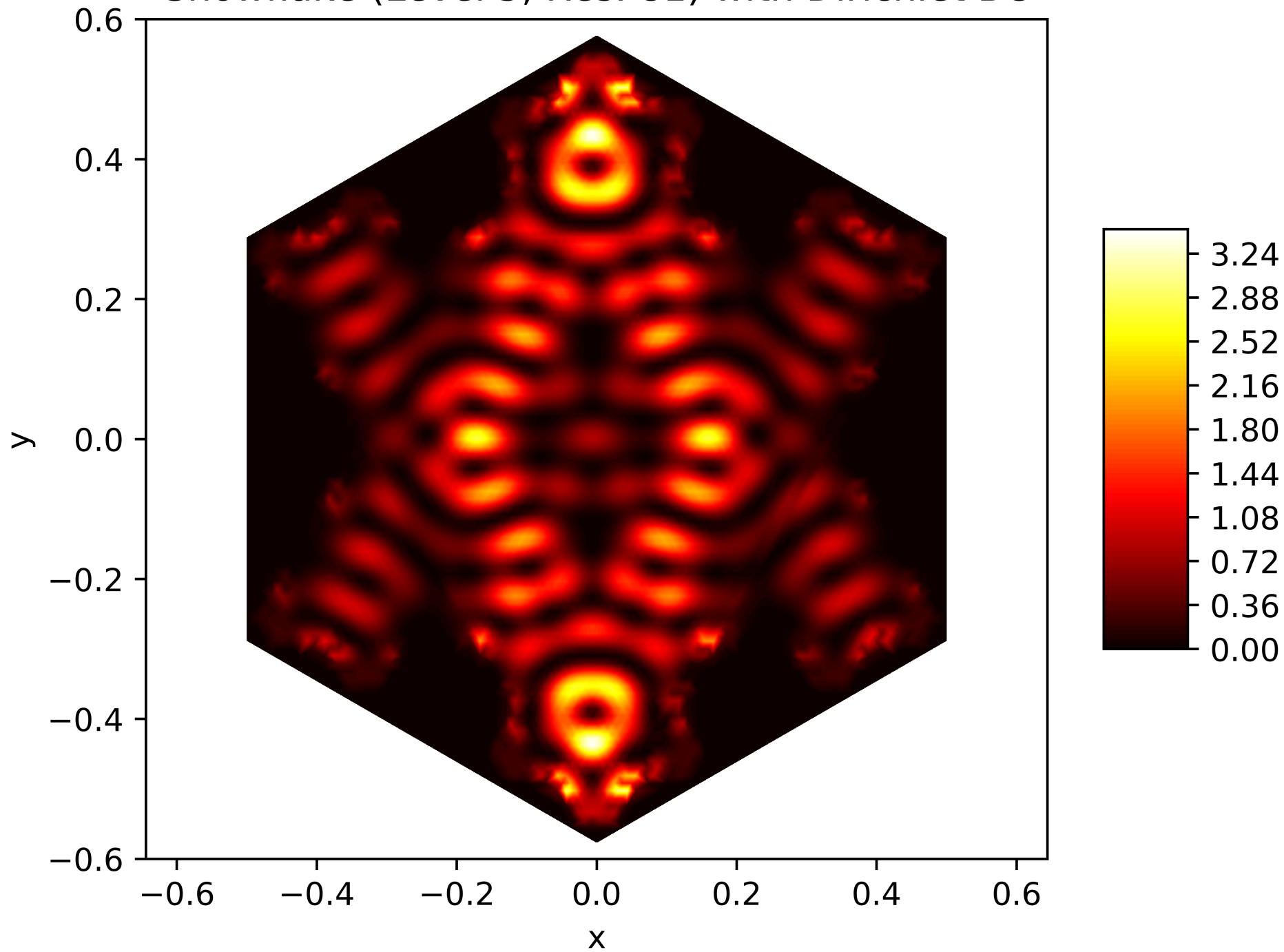
Energy Function of the 83. Eigenfunction on the Snowflake (Level 5, Res. 81) with Dirichlet BC
