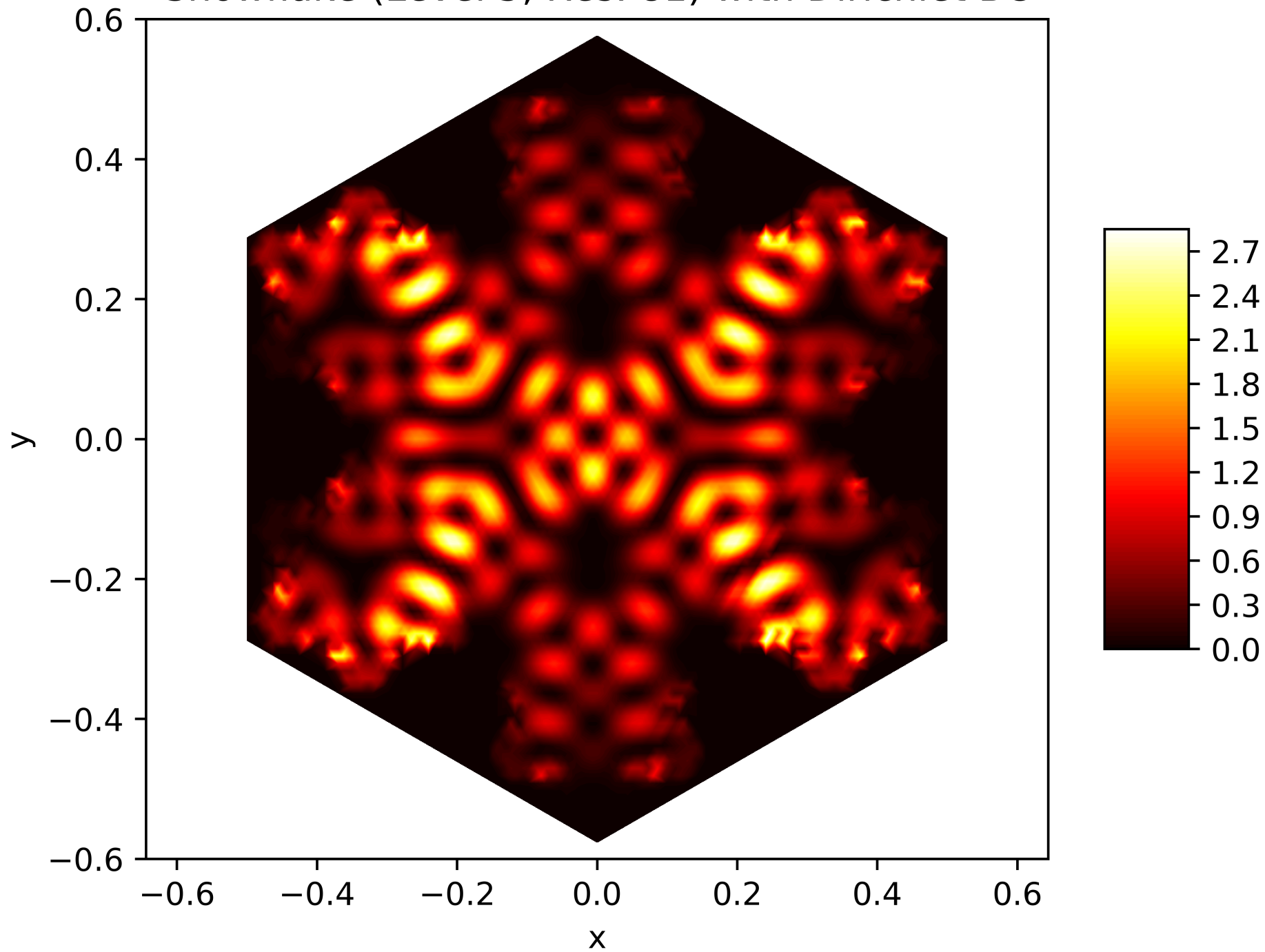
Energy Function of the 92. Eigenfunction on the Snowflake (Level 5, Res. 81) with Dirichlet BC
