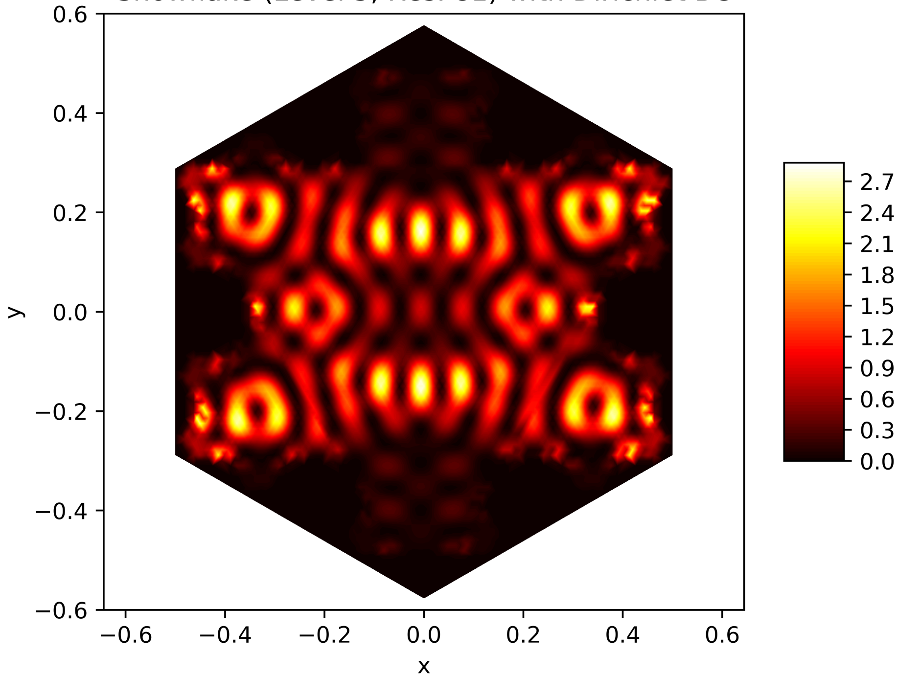
Energy Function of the 84. Eigenfunction on the Snowflake (Level 5, Res. 81) with Dirichlet BC
