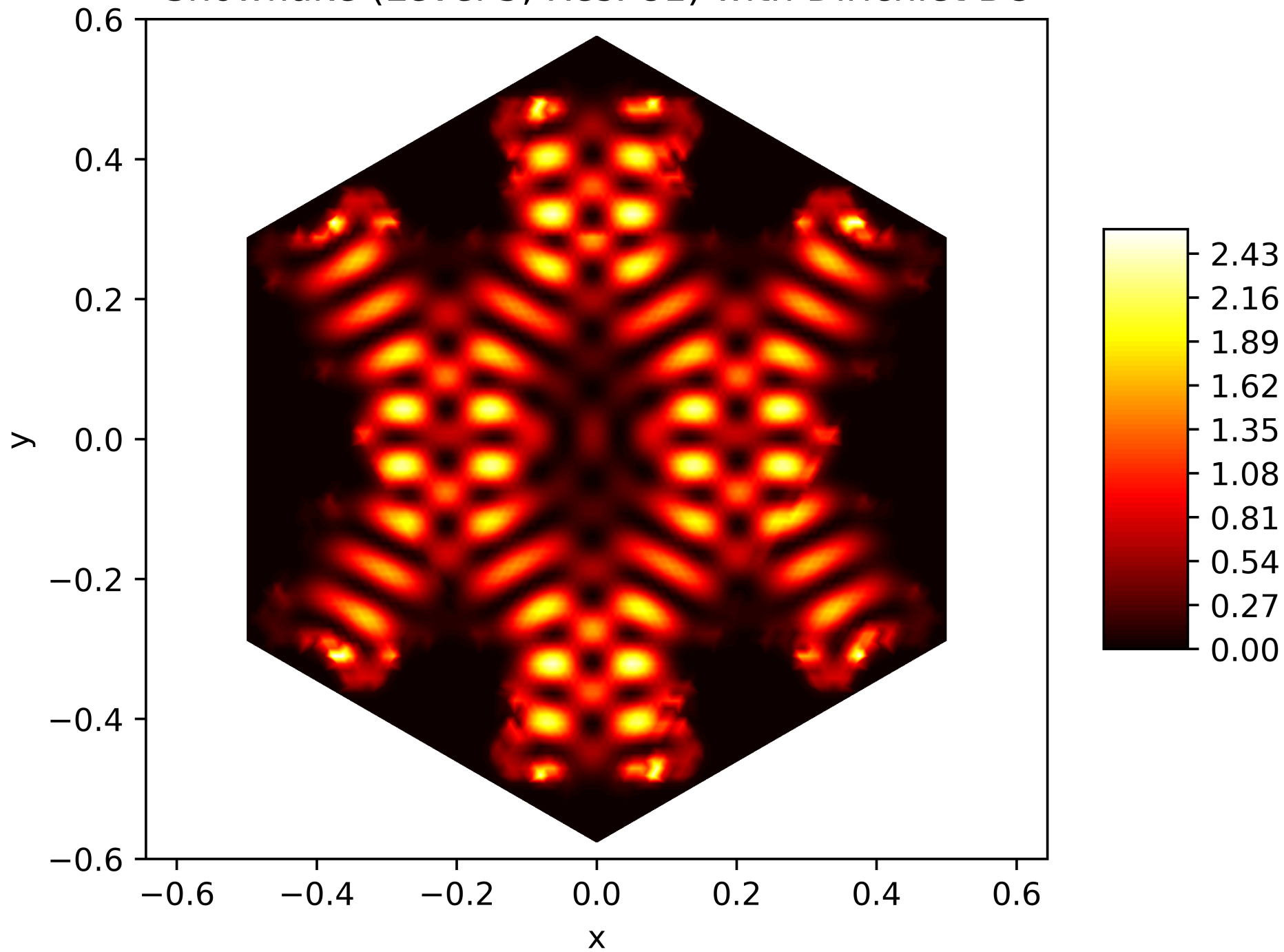
Energy Function of the 89. Eigenfunction on the Snowflake (Level 5, Res. 81) with Dirichlet BC
