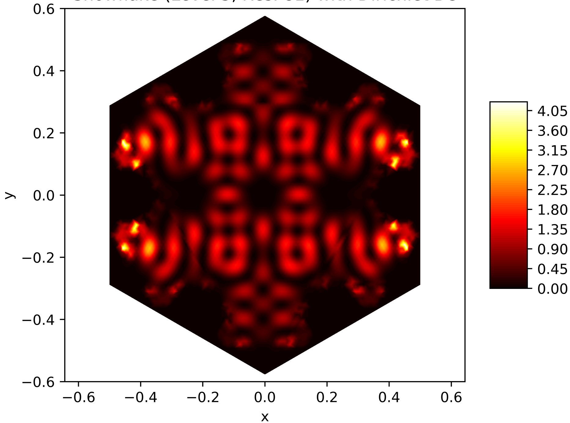
Energy Function of the 81. Eigenfunction on the Snowflake (Level 5, Res. 81) with Dirichlet BC
