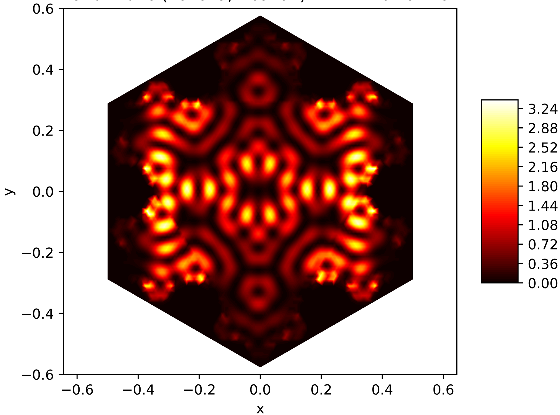
Energy Function of the 99. Eigenfunction on the Snowflake (Level 5, Res. 81) with Dirichlet BC
