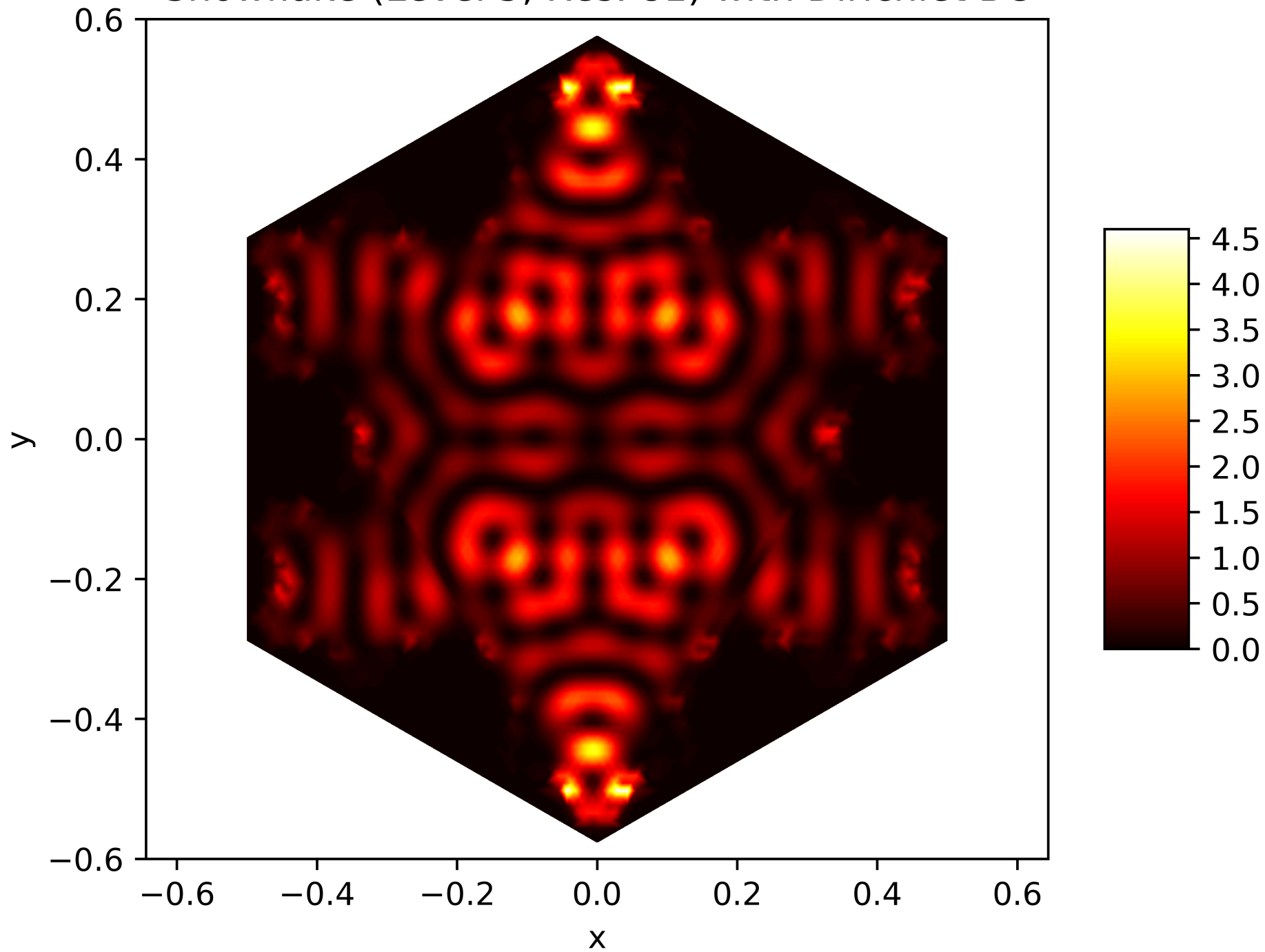
Energy Function of the 94. Eigenfunction on the Snowflake (Level 5, Res. 81) with Dirichlet BC
