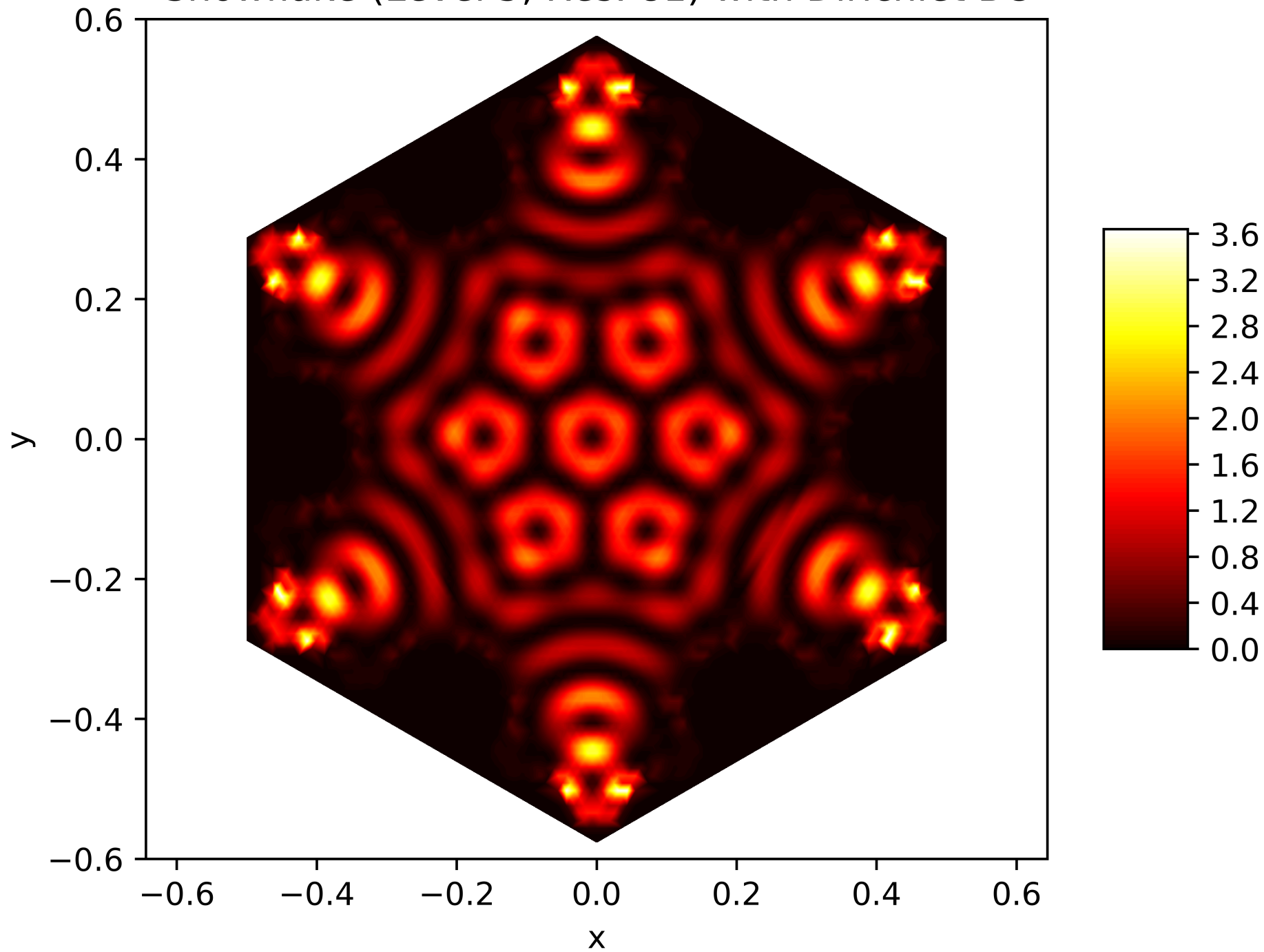
Energy Function of the 97. Eigenfunction on the Snowflake (Level 5, Res. 81) with Dirichlet BC
