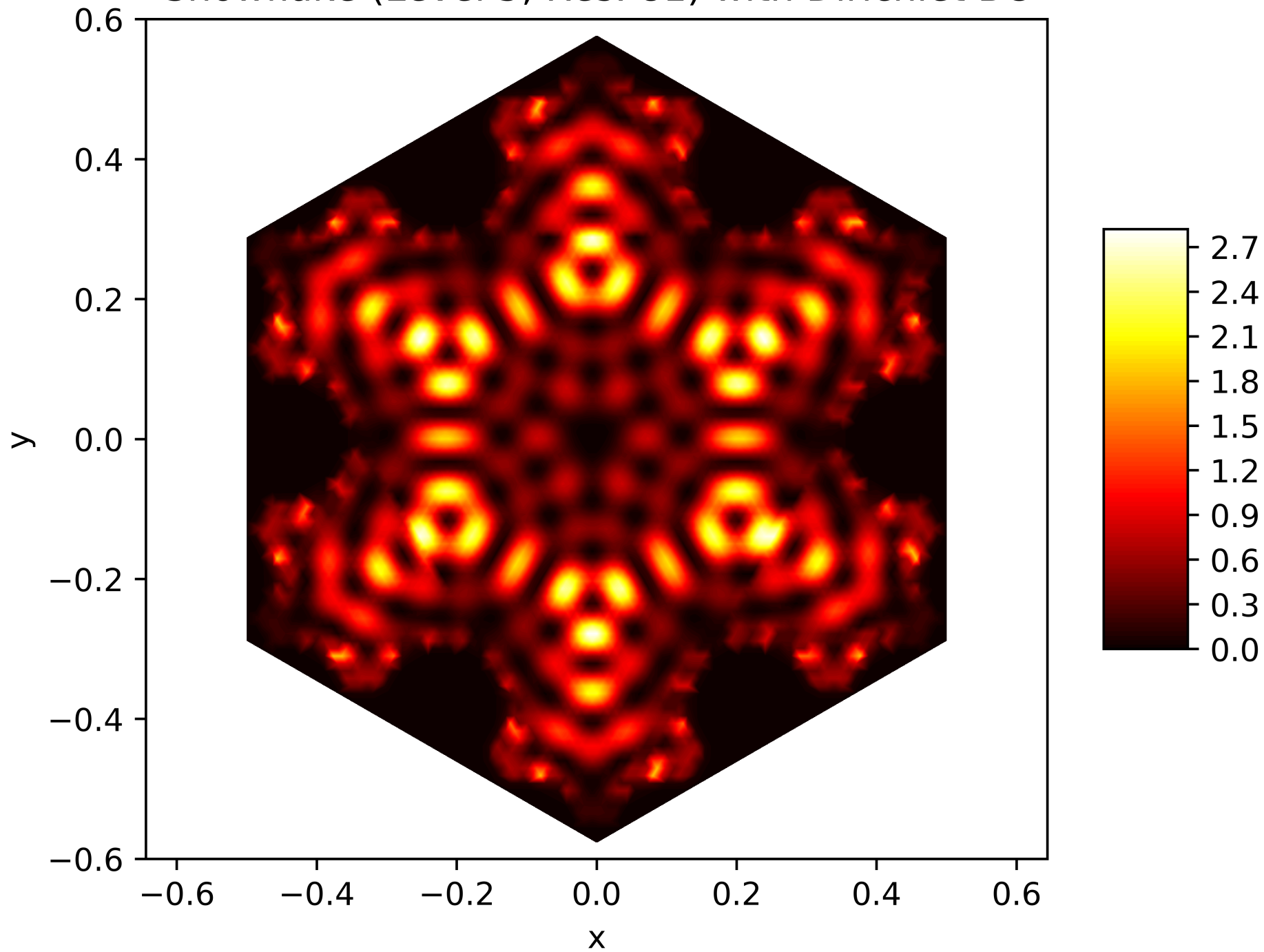
Energy Function of the 96. Eigenfunction on the Snowflake (Level 5, Res. 81) with Dirichlet BC
