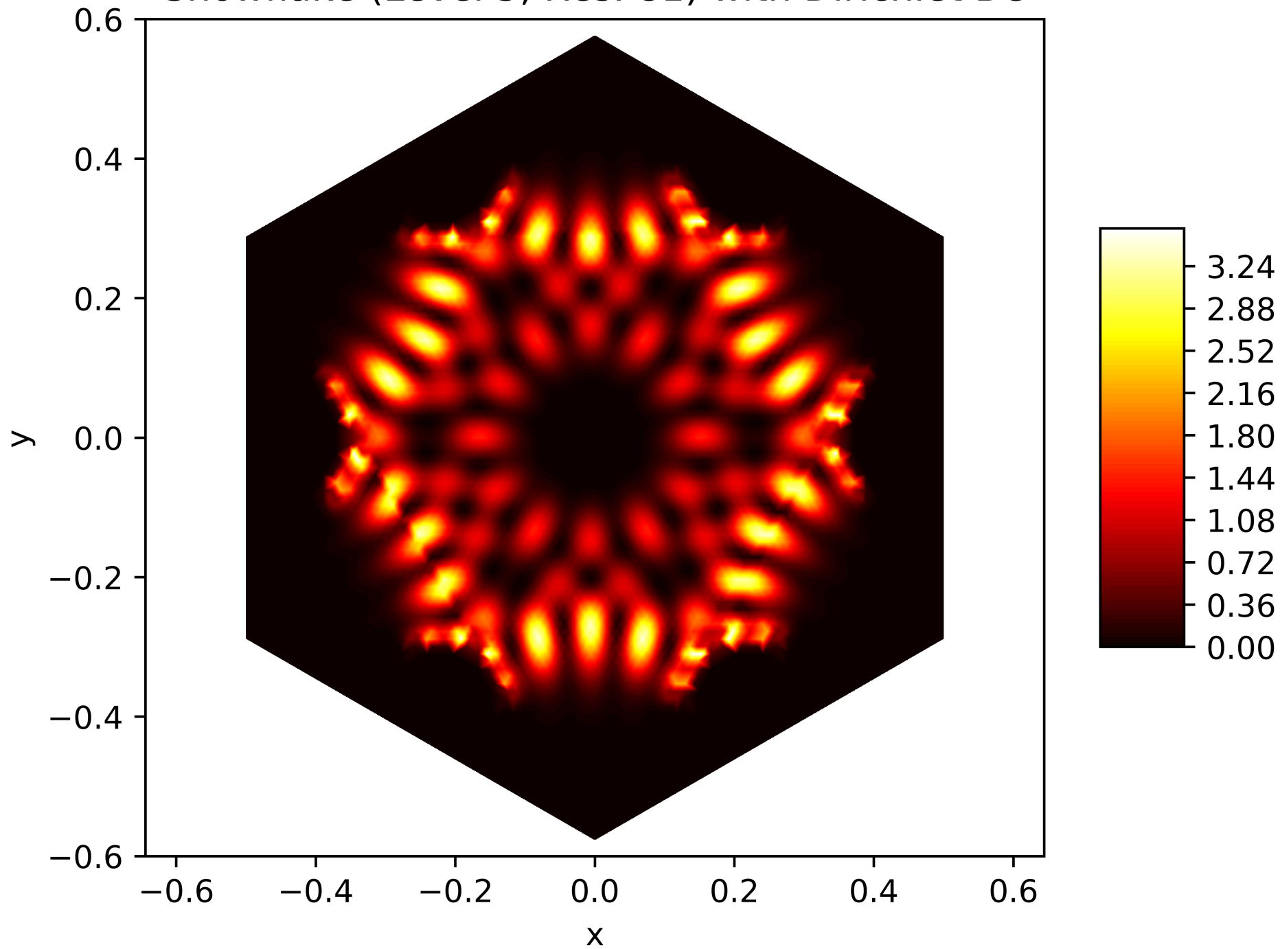
Energy Function of the 88. Eigenfunction on the Snowflake (Level 5, Res. 81) with Dirichlet BC
