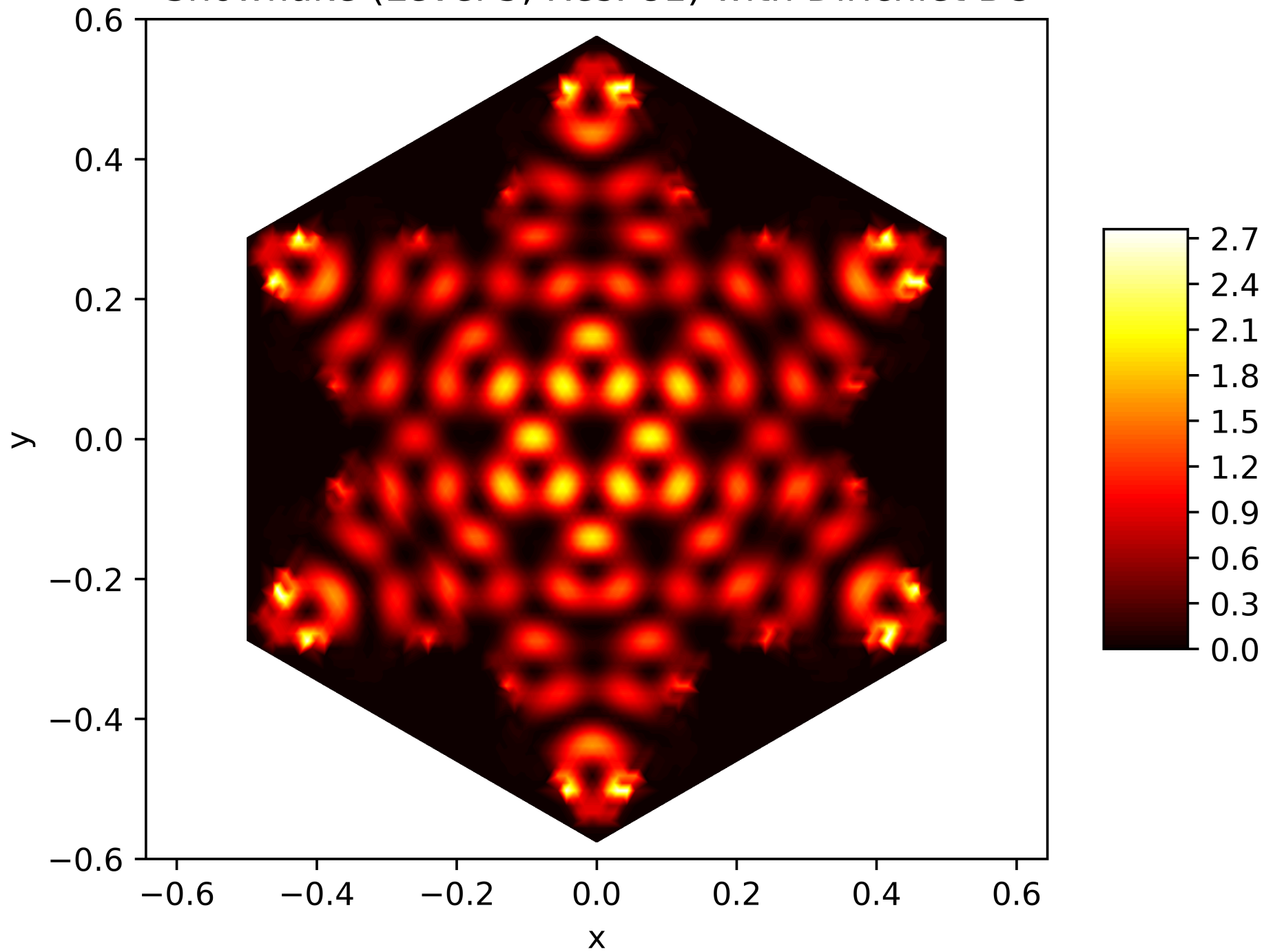
Energy Function of the 82. Eigenfunction on the Snowflake (Level 5, Res. 81) with Dirichlet BC
