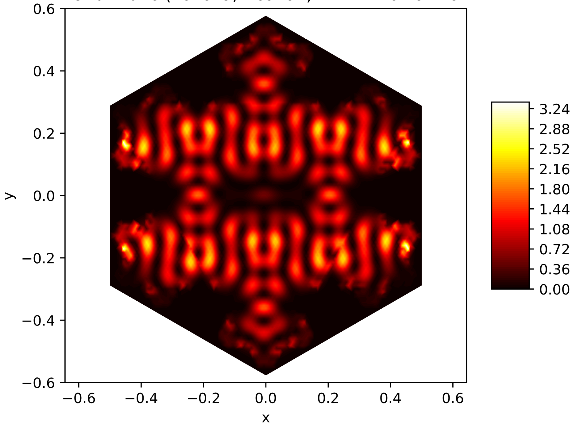
Energy Function of the 90. Eigenfunction on the Snowflake (Level 5, Res. 81) with Dirichlet BC
