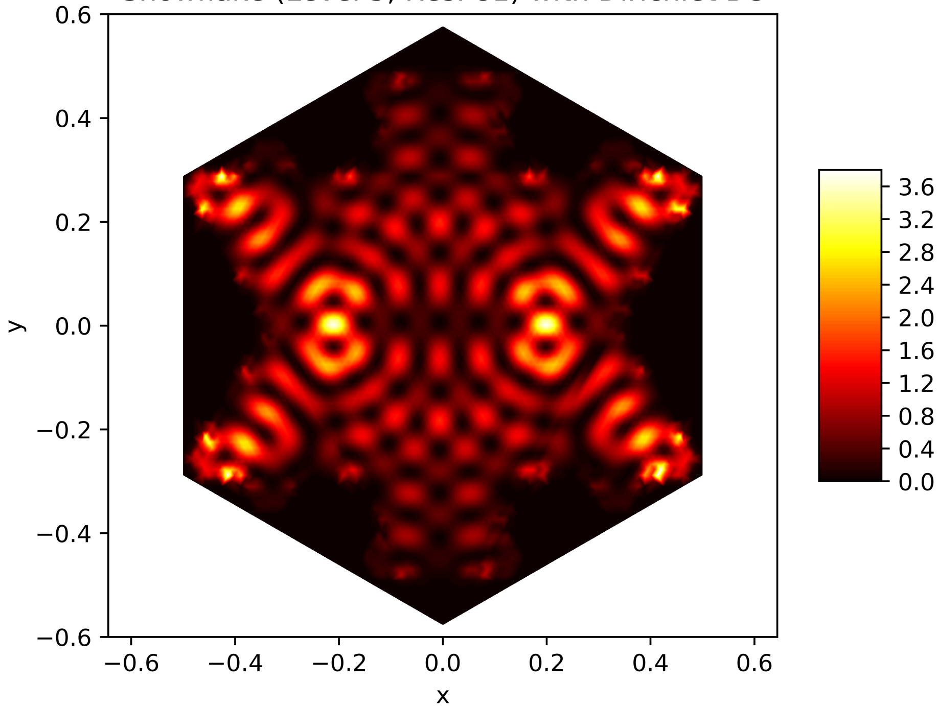
Energy Function of the 95. Eigenfunction on the Snowflake (Level 5, Res. 81) with Dirichlet BC
