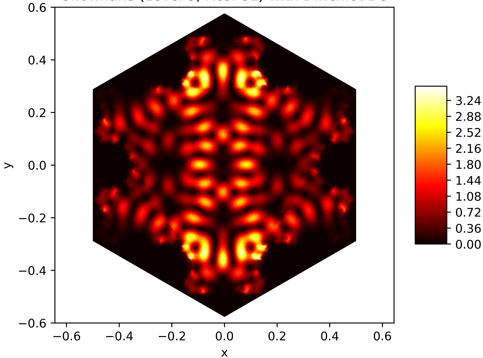
Energy Function of the 98. Eigenfunction on the Snowflake (Level 5, Res. 81) with Dirichlet BC
