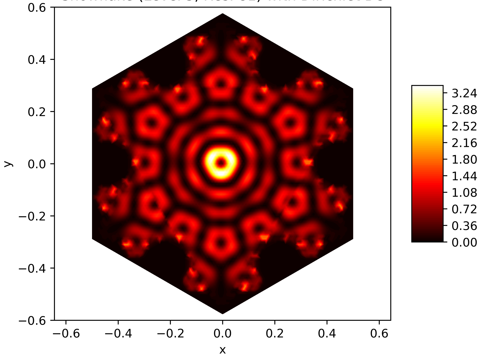
Energy Function of the 87. Eigenfunction on the Snowflake (Level 5, Res. 81) with Dirichlet BC
