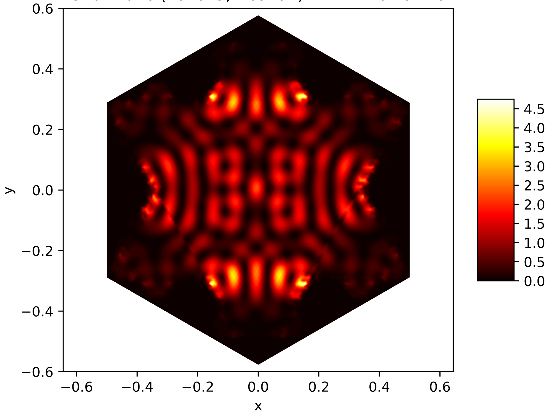
Energy Function of the 86. Eigenfunction on the Snowflake (Level 5, Res. 81) with Dirichlet BC
