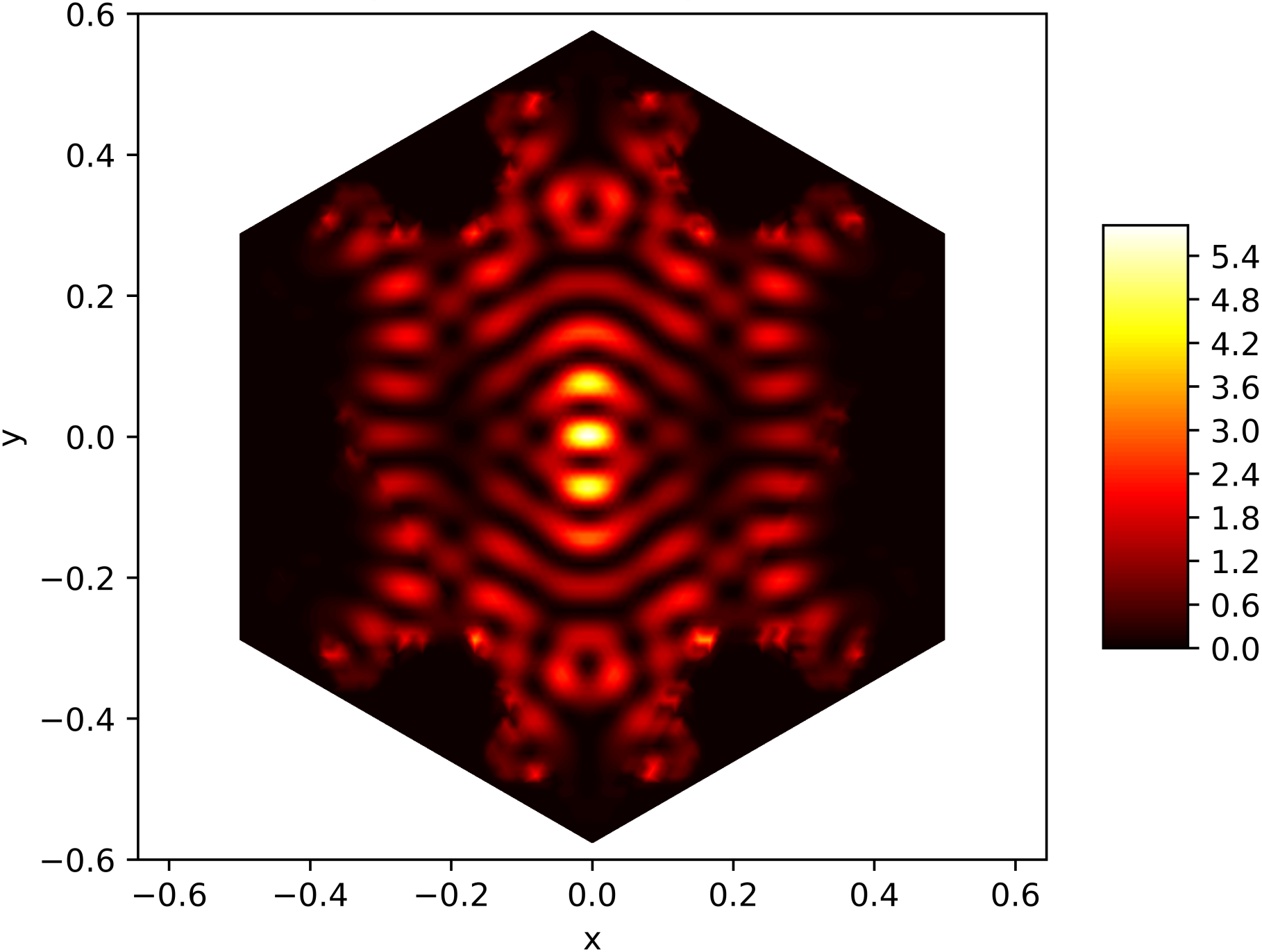
Energy Function of the 100. Eigenfunction on the Snowflake (Level 5, Res. 81) with Dirichlet BC
