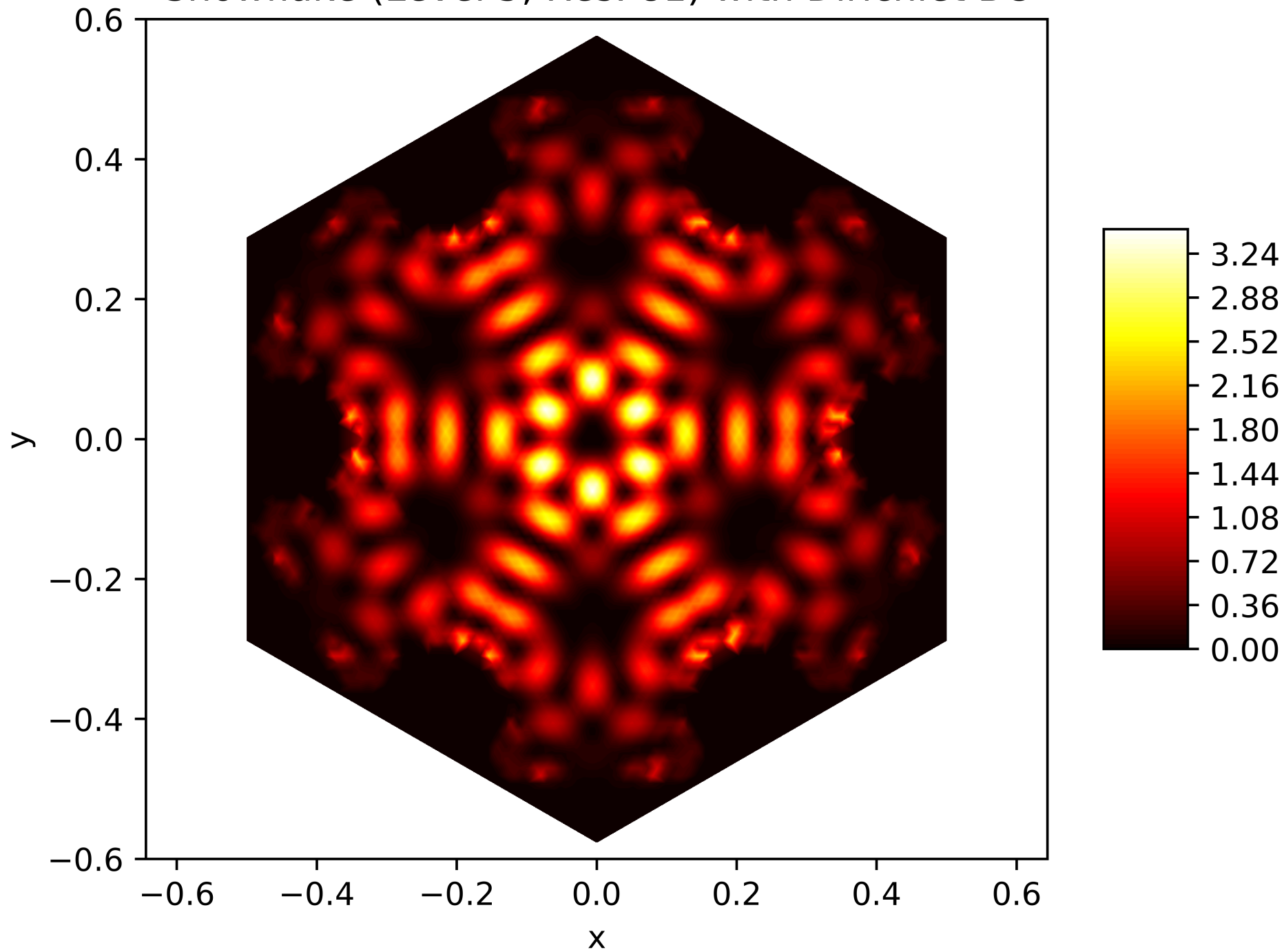
Energy Function of the 93. Eigenfunction on the Snowflake (Level 5, Res. 81) with Dirichlet BC
