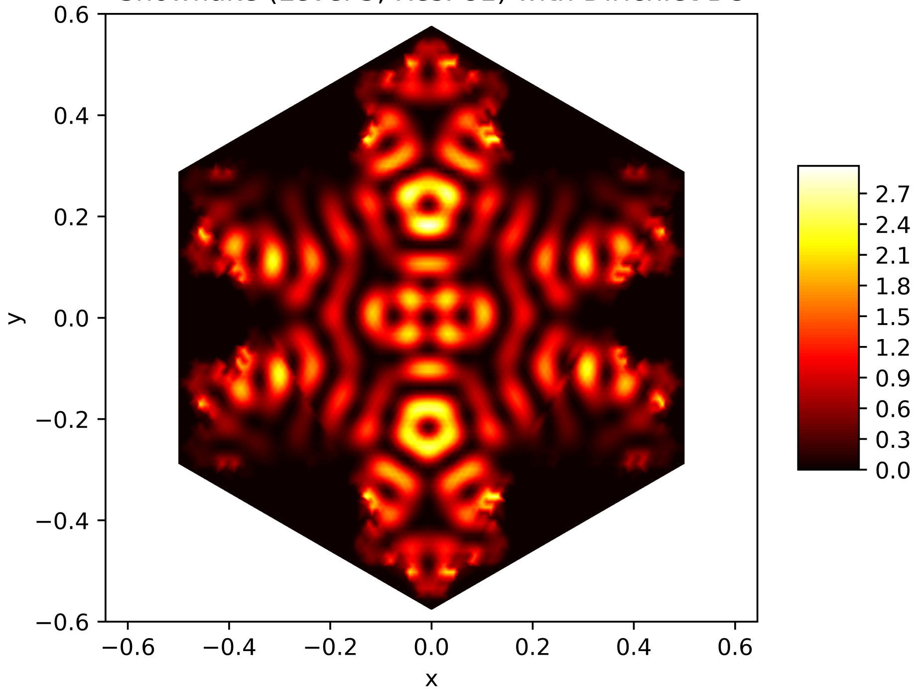
Energy Function of the 91. Eigenfunction on the Snowflake (Level 5, Res. 81) with Dirichlet BC
