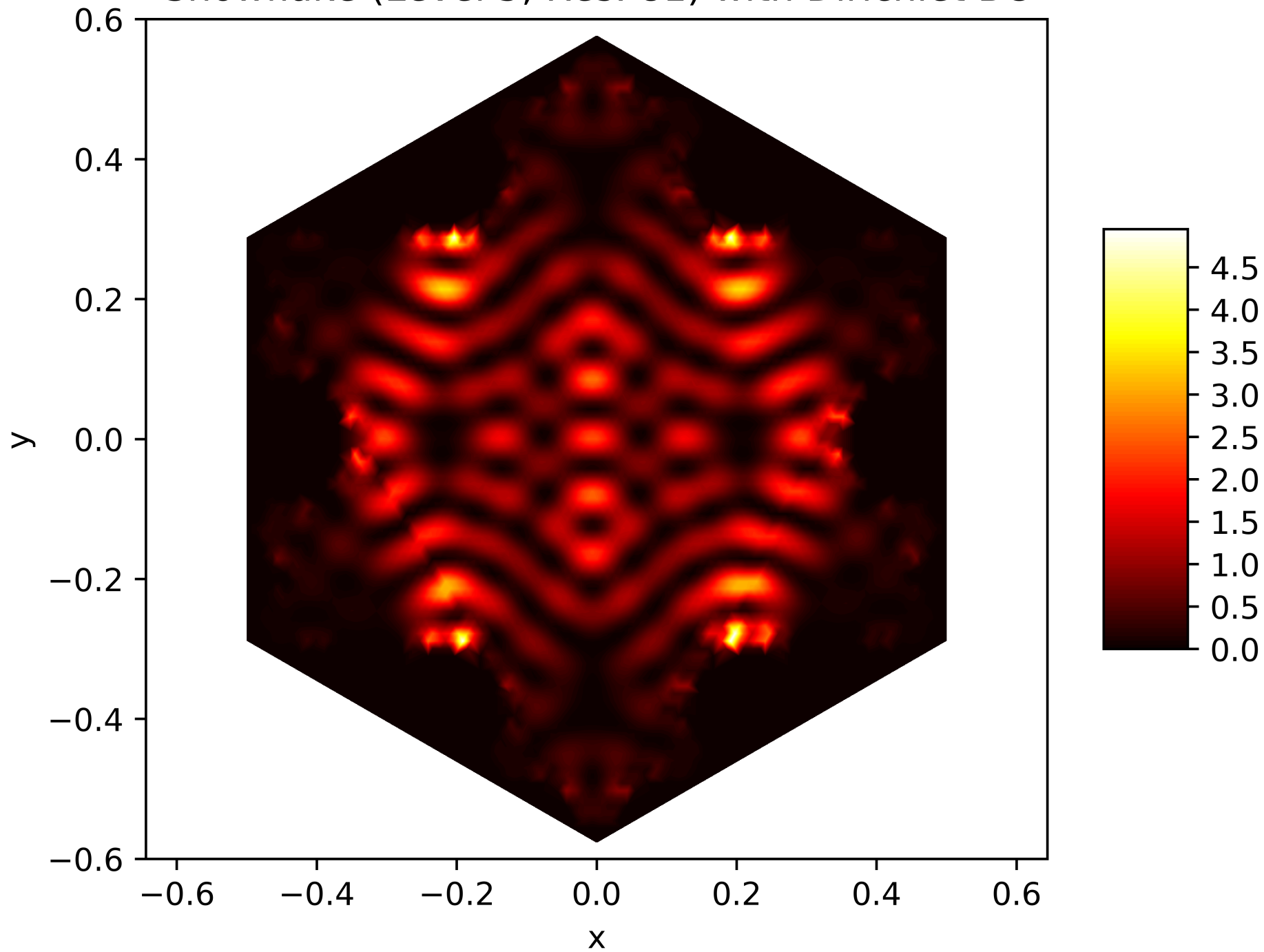
Energy Function of the 85. Eigenfunction on the Snowflake (Level 5, Res. 81) with Dirichlet BC
