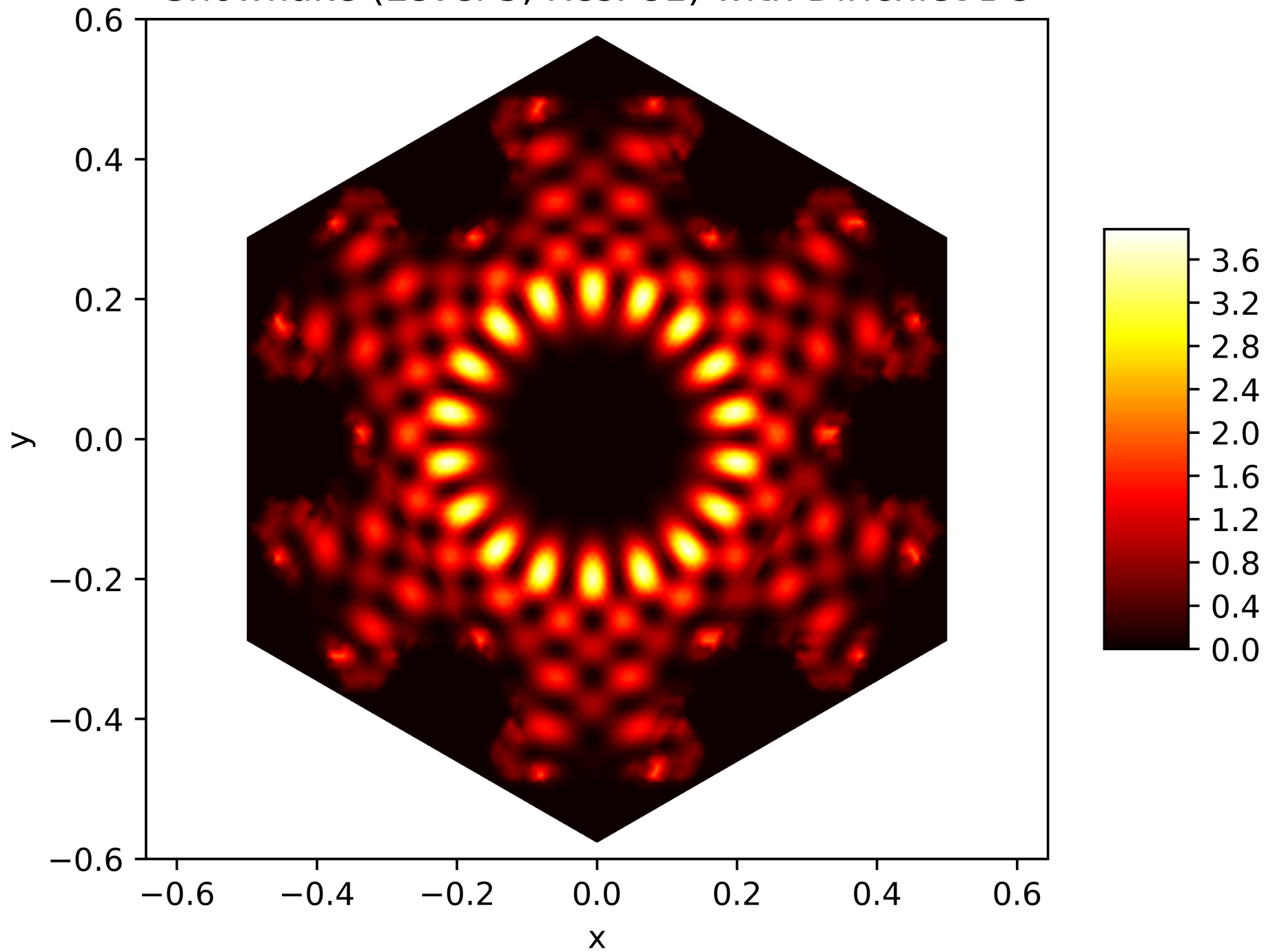
Energy Function of the 111. Eigenfunction on the Snowflake (Level 5, Res. 81) with Dirichlet BC
