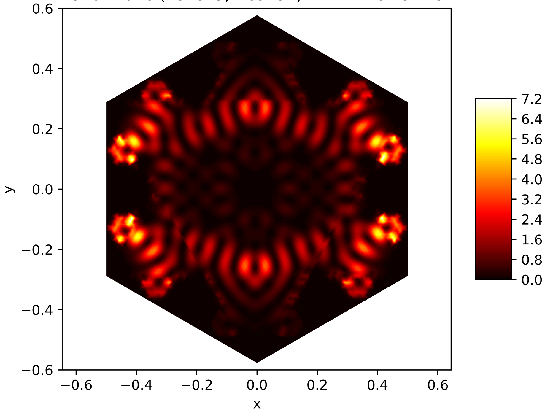
Energy Function of the 117. Eigenfunction on the Snowflake (Level 5, Res. 81) with Dirichlet BC
