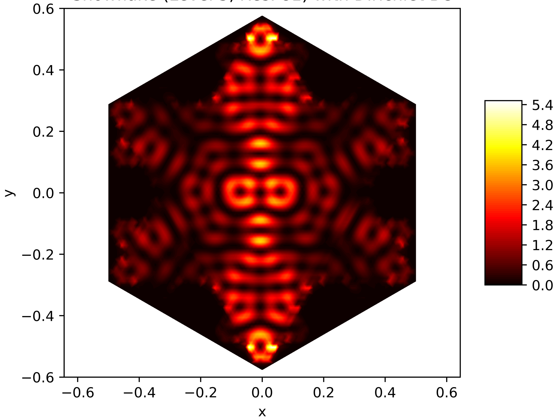
Energy Function of the 113. Eigenfunction on the Snowflake (Level 5, Res. 81) with Dirichlet BC
