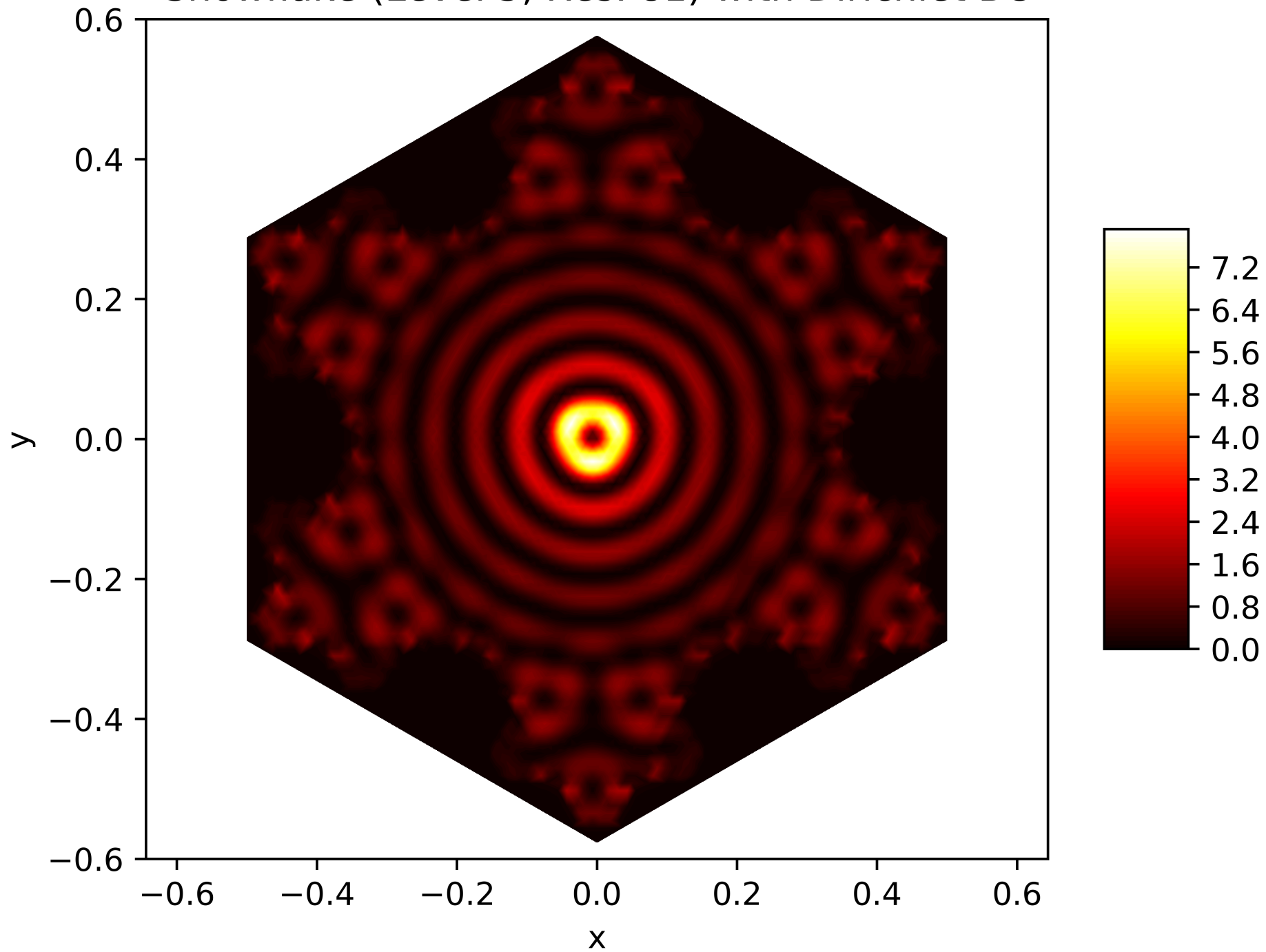
Energy Function of the 115. Eigenfunction on the Snowflake (Level 5, Res. 81) with Dirichlet BC
