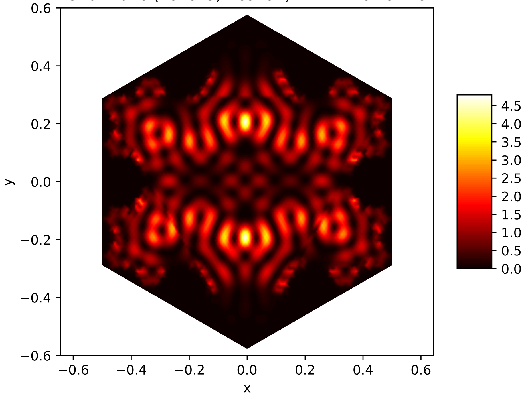
Energy Function of the 108. Eigenfunction on the Snowflake (Level 5, Res. 81) with Dirichlet BC
