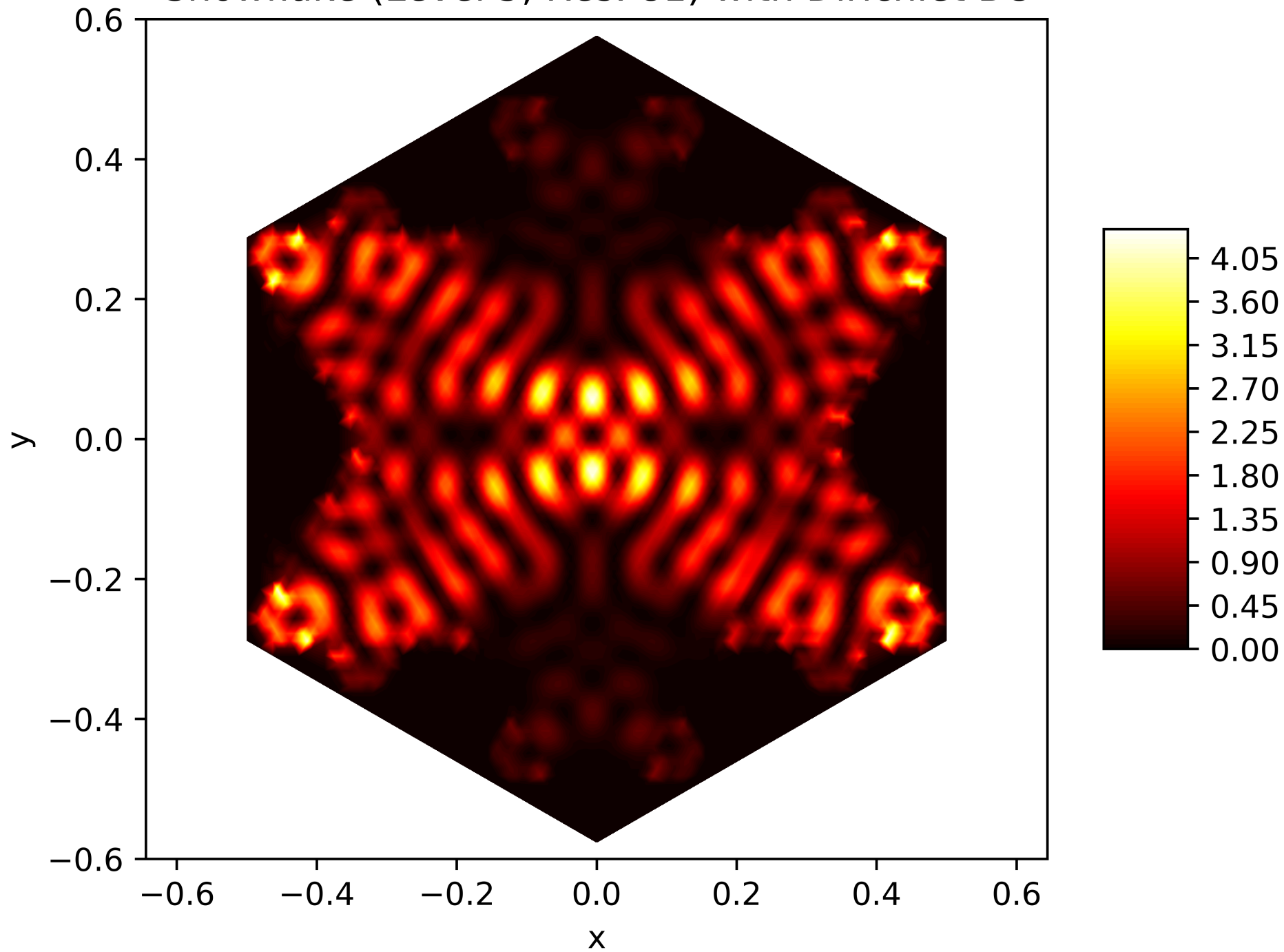
Energy Function of the 114. Eigenfunction on the Snowflake (Level 5, Res. 81) with Dirichlet BC
