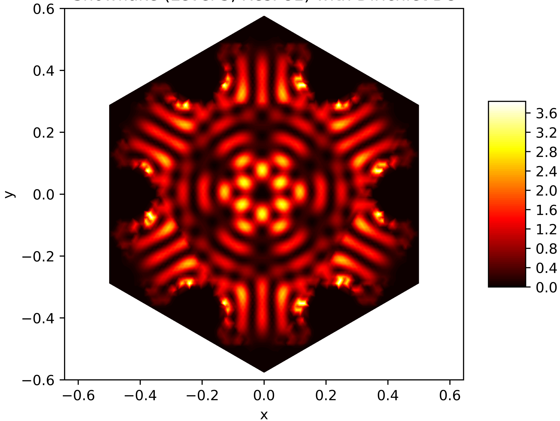
Energy Function of the 112. Eigenfunction on the Snowflake (Level 5, Res. 81) with Dirichlet BC
