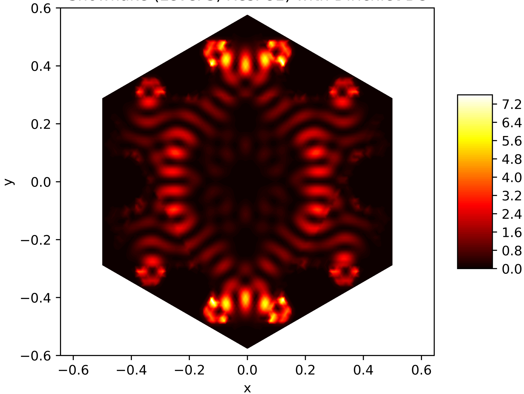
Energy Function of the 116. Eigenfunction on the Snowflake (Level 5, Res. 81) with Dirichlet BC
