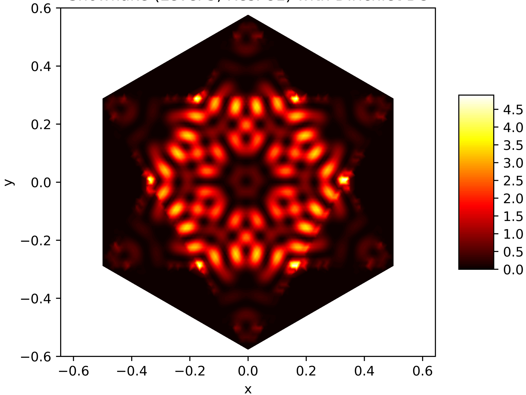
Energy Function of the 106. Eigenfunction on the Snowflake (Level 5, Res. 81) with Dirichlet BC
