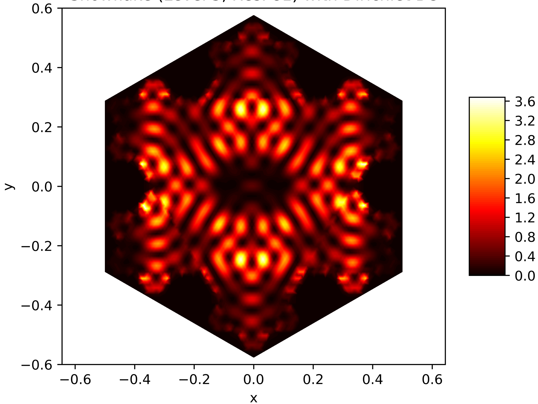
Energy Function of the 109. Eigenfunction on the Snowflake (Level 5, Res. 81) with Dirichlet BC
