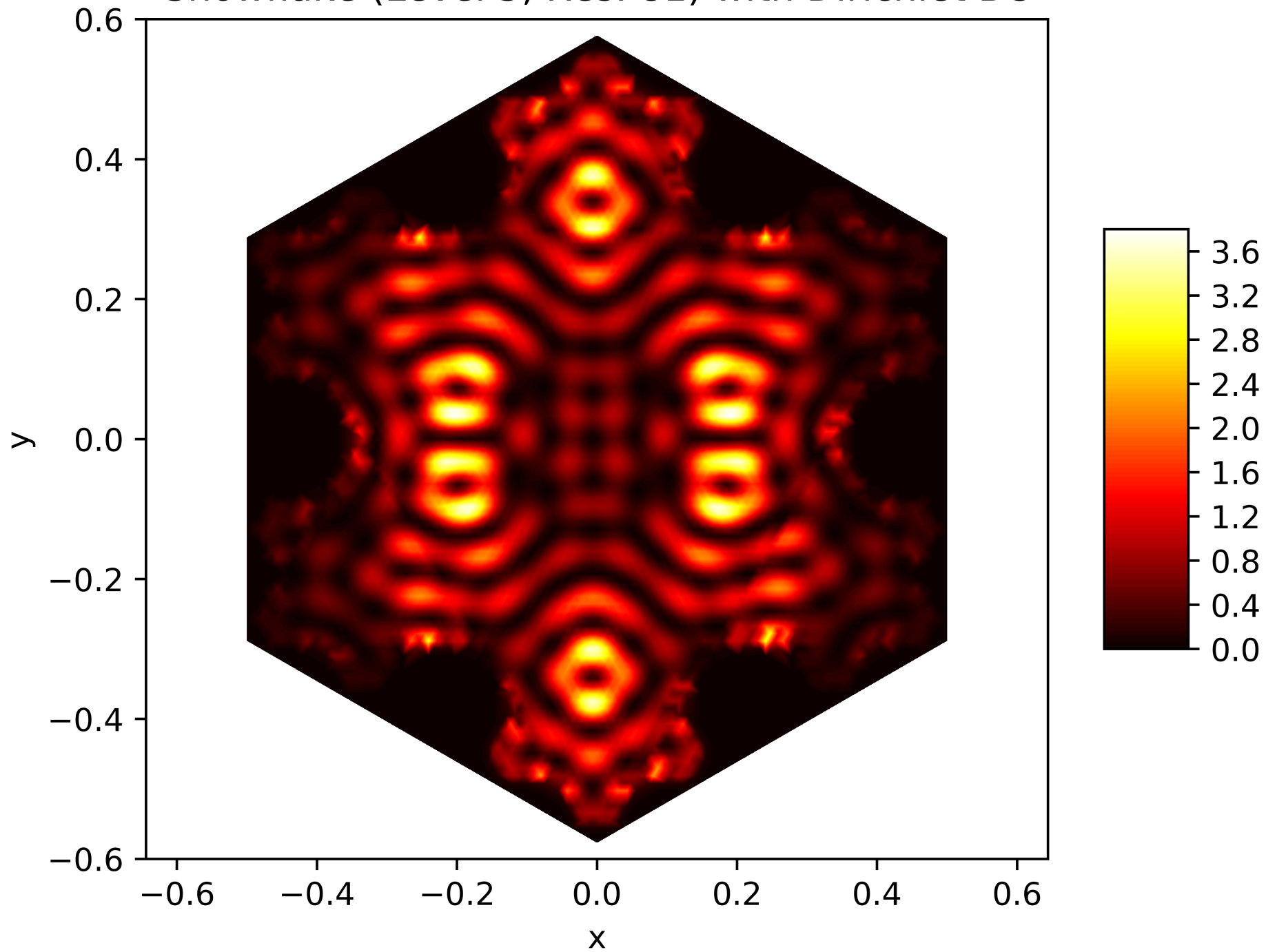
Energy Function of the 107. Eigenfunction on the Snowflake (Level 5, Res. 81) with Dirichlet BC
