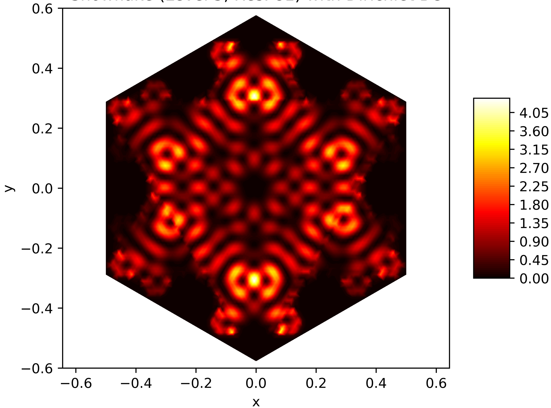
Energy Function of the 119. Eigenfunction on the Snowflake (Level 5, Res. 81) with Dirichlet BC
