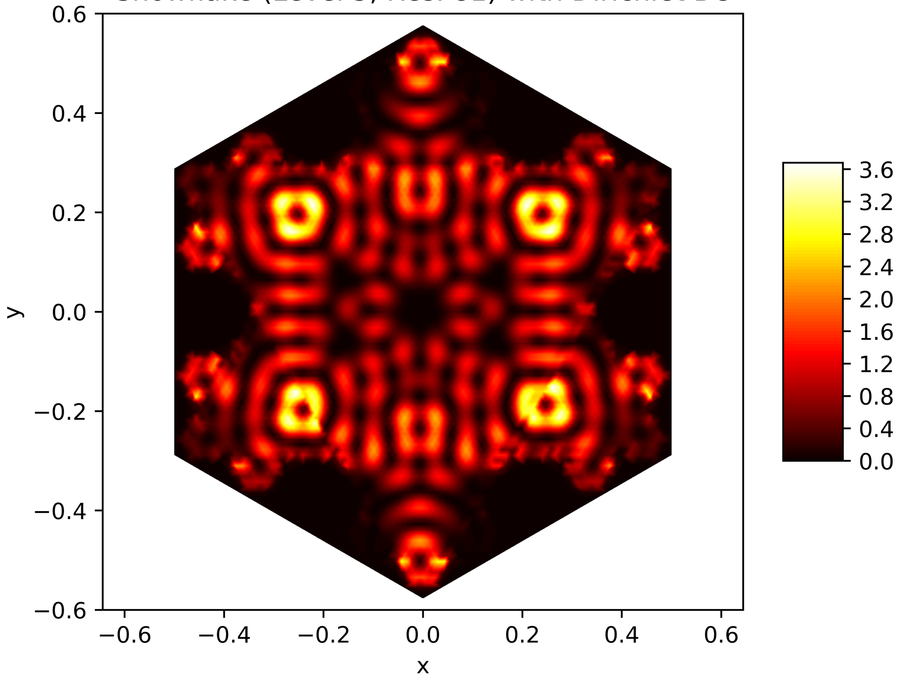
Energy Function of the 120. Eigenfunction on the Snowflake (Level 5, Res. 81) with Dirichlet BC
