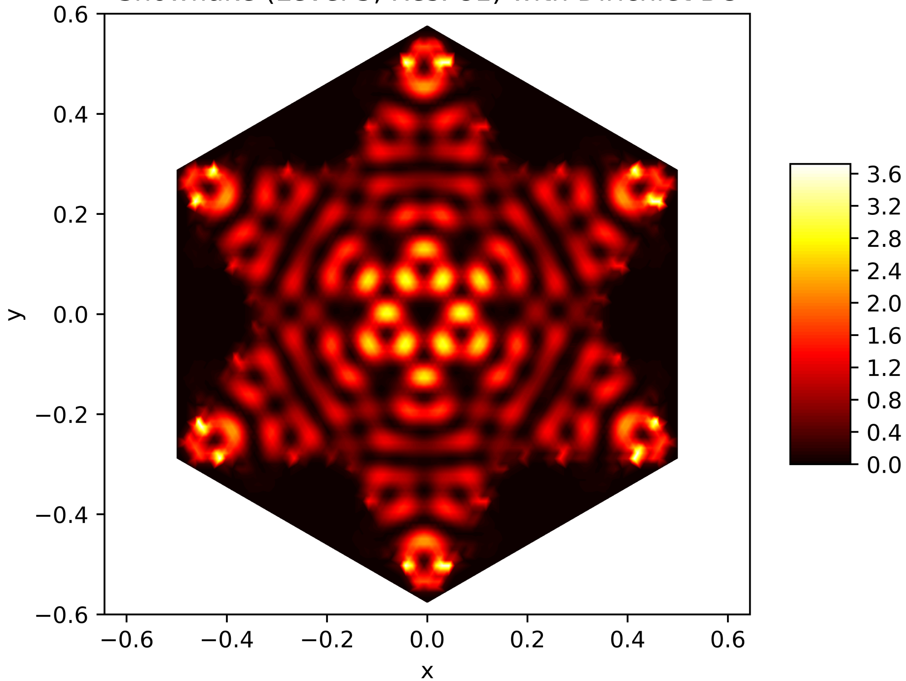
Energy Function of the 102. Eigenfunction on the Snowflake (Level 5, Res. 81) with Dirichlet BC
