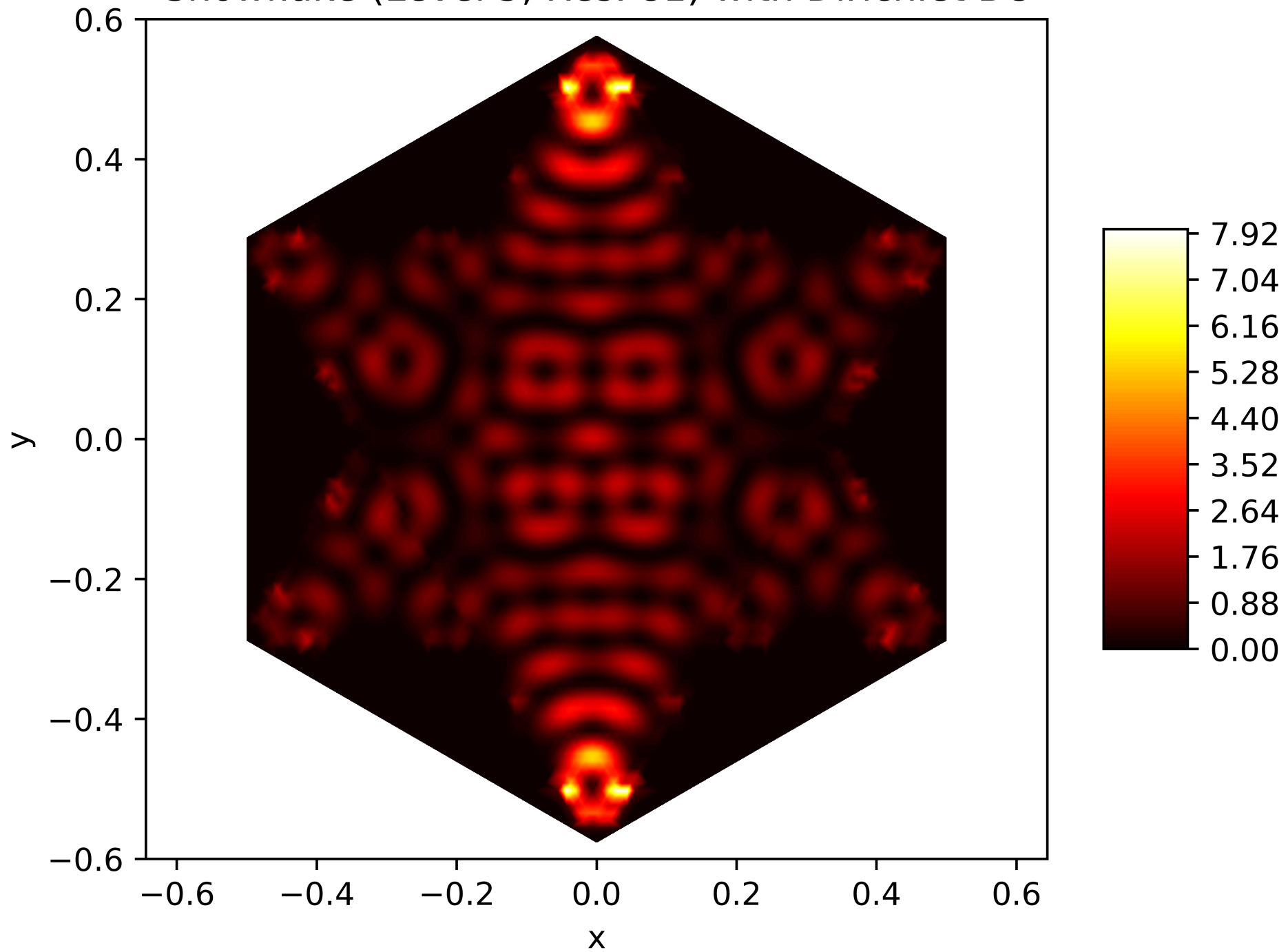
Energy Function of the 104. Eigenfunction on the Snowflake (Level 5, Res. 81) with Dirichlet BC
