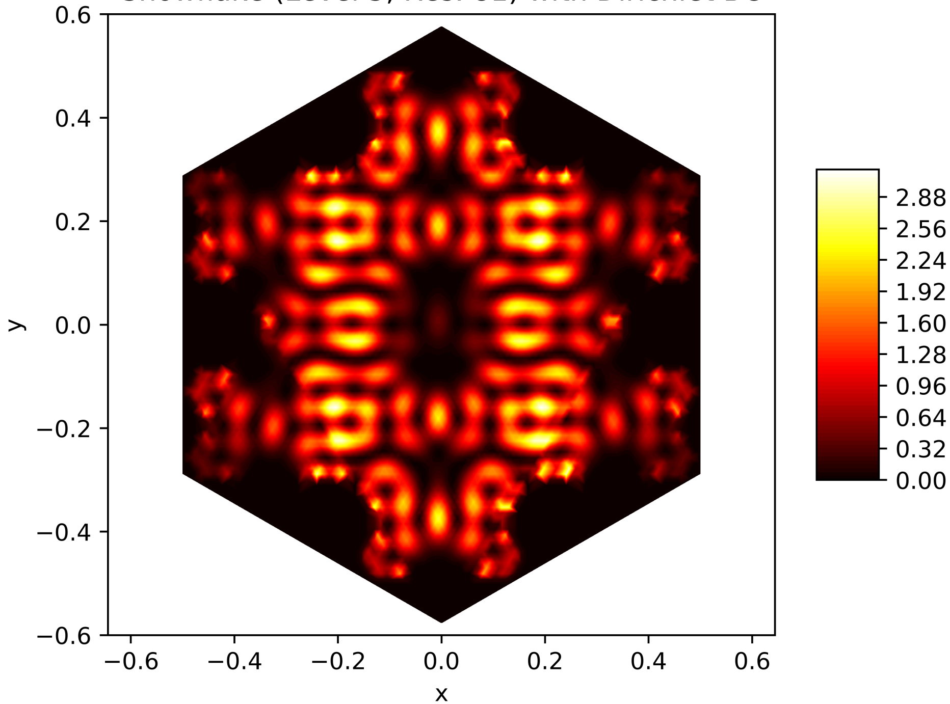
Energy Function of the 110. Eigenfunction on the Snowflake (Level 5, Res. 81) with Dirichlet BC
