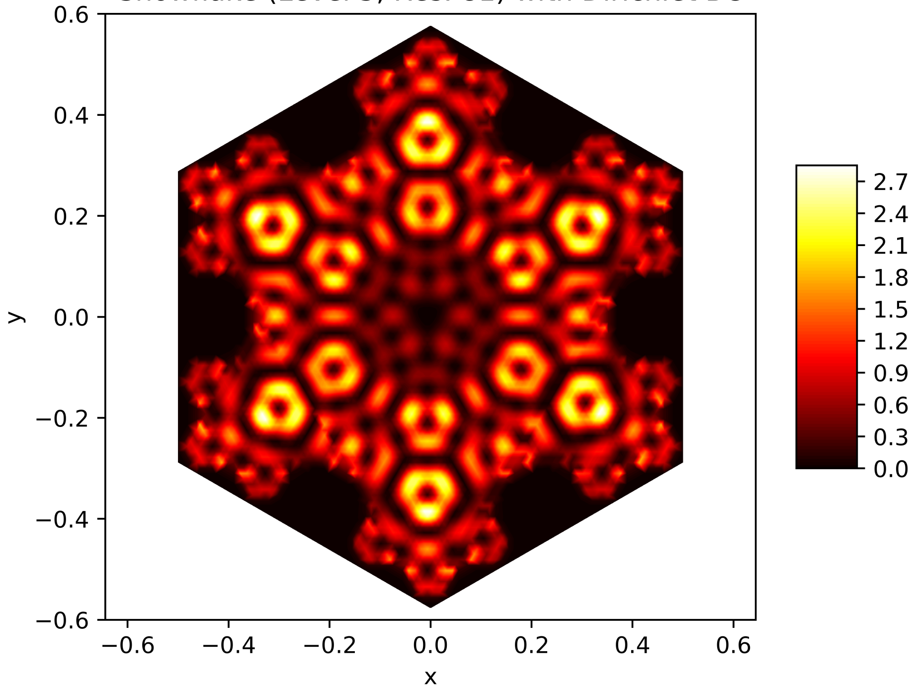
Energy Function of the 118. Eigenfunction on the Snowflake (Level 5, Res. 81) with Dirichlet BC
