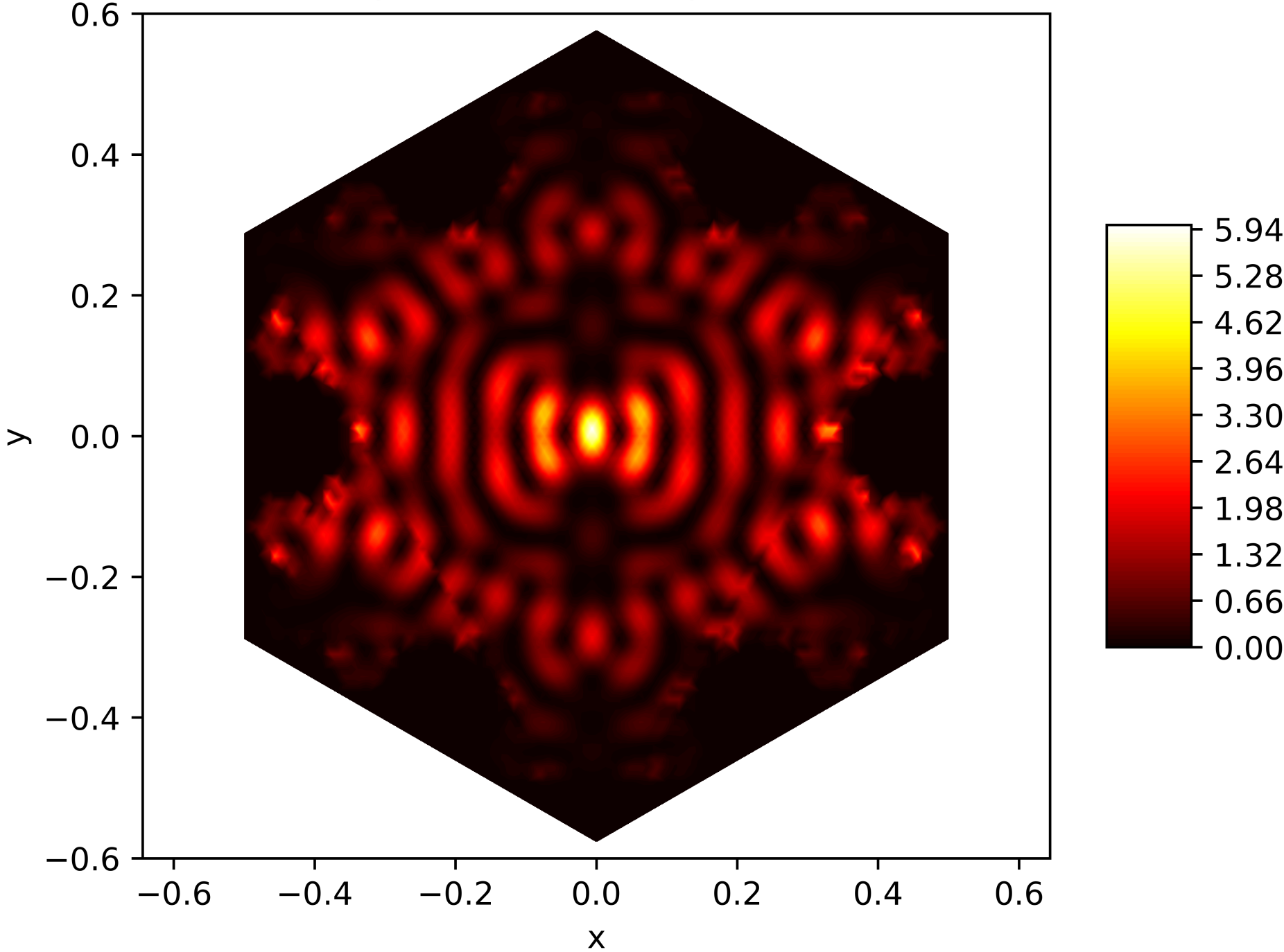
Energy Function of the 101. Eigenfunction on the Snowflake (Level 5, Res. 81) with Dirichlet BC
