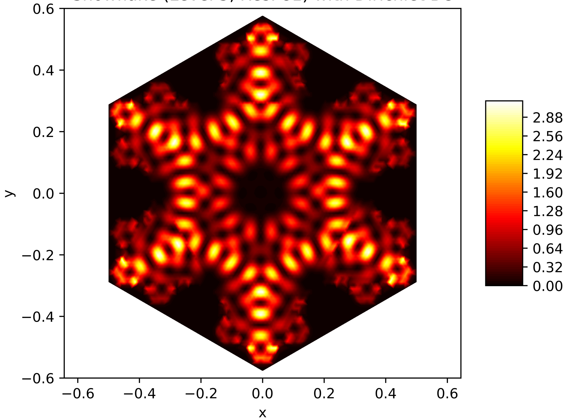
Energy Function of the 124. Eigenfunction on the Snowflake (Level 5, Res. 81) with Dirichlet BC
