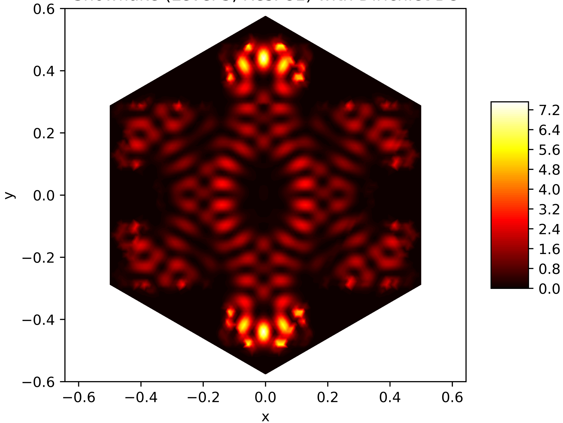
Energy Function of the 125. Eigenfunction on the Snowflake (Level 5, Res. 81) with Dirichlet BC
