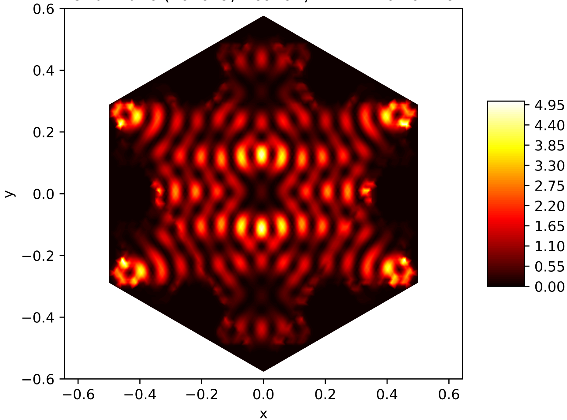
Energy Function of the 129. Eigenfunction on the Snowflake (Level 5, Res. 81) with Dirichlet BC
