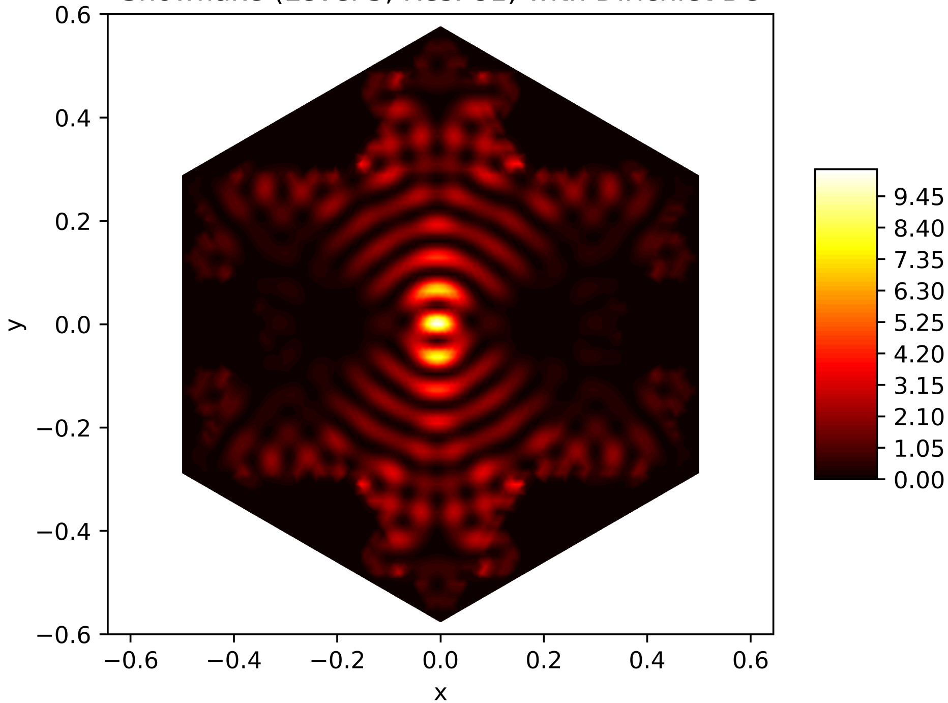
Energy Function of the 132. Eigenfunction on the Snowflake (Level 5, Res. 81) with Dirichlet BC
