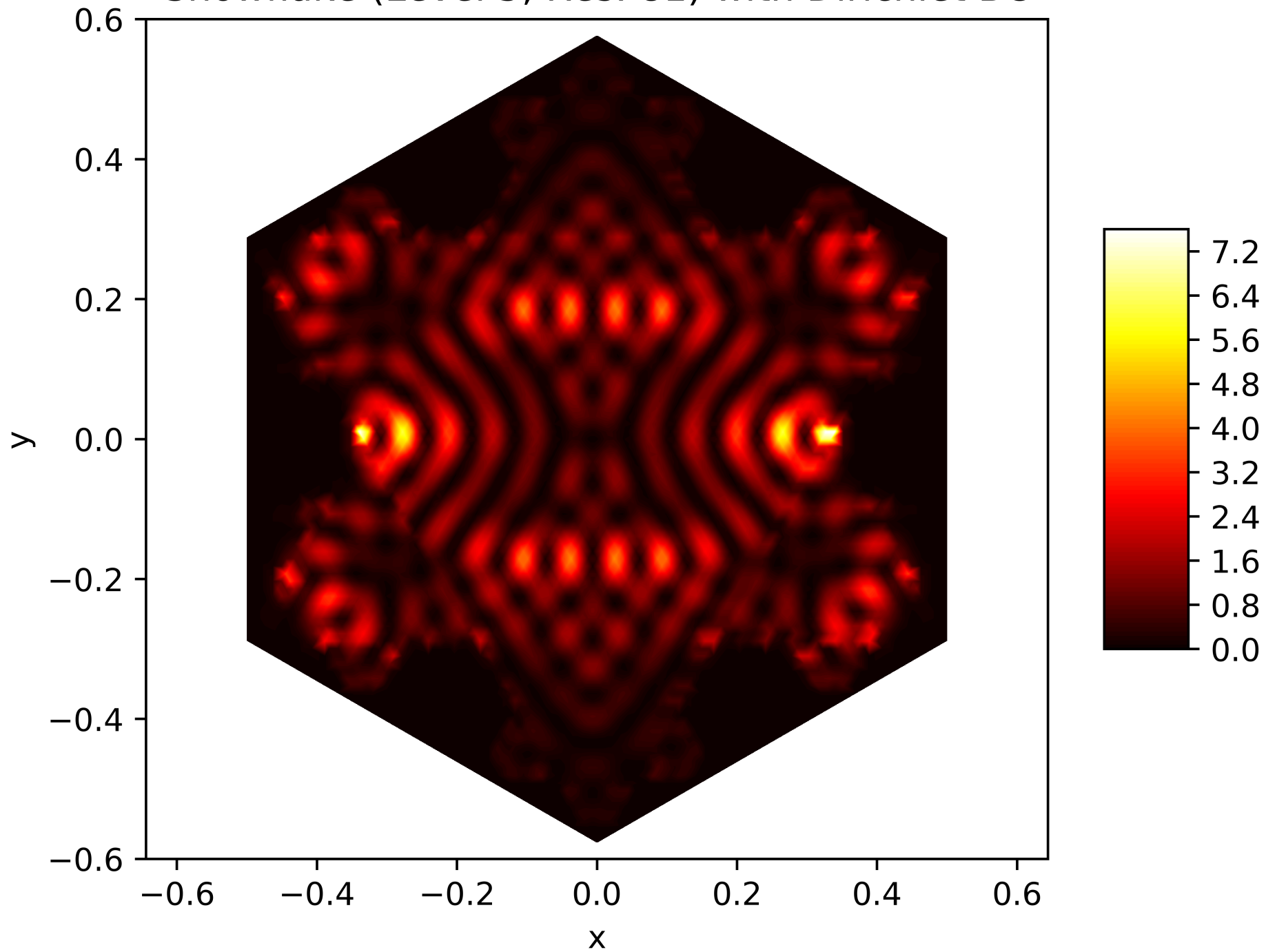
Energy Function of the 134. Eigenfunction on the Snowflake (Level 5, Res. 81) with Dirichlet BC
