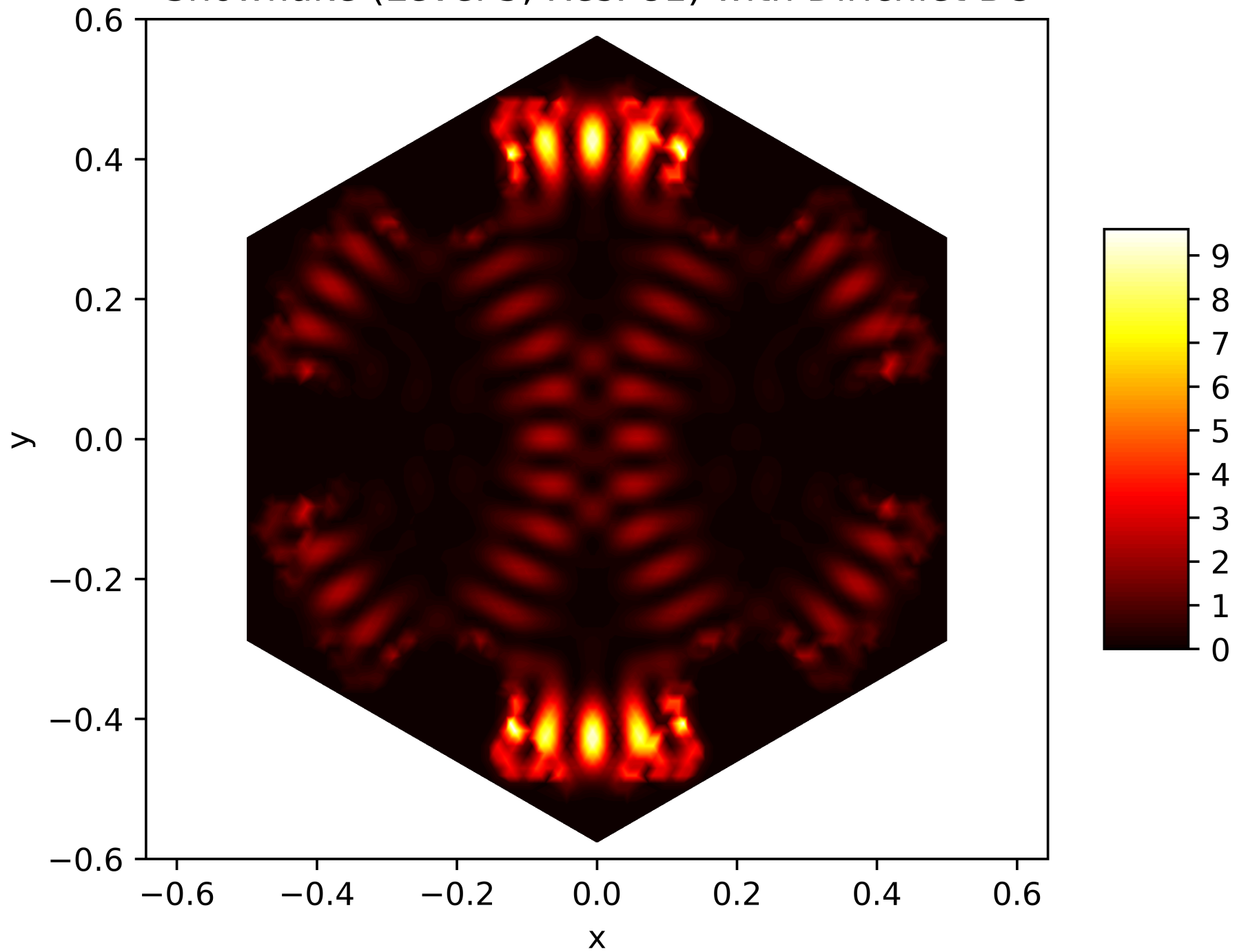
Energy Function of the 122. Eigenfunction on the Snowflake (Level 5, Res. 81) with Dirichlet BC
