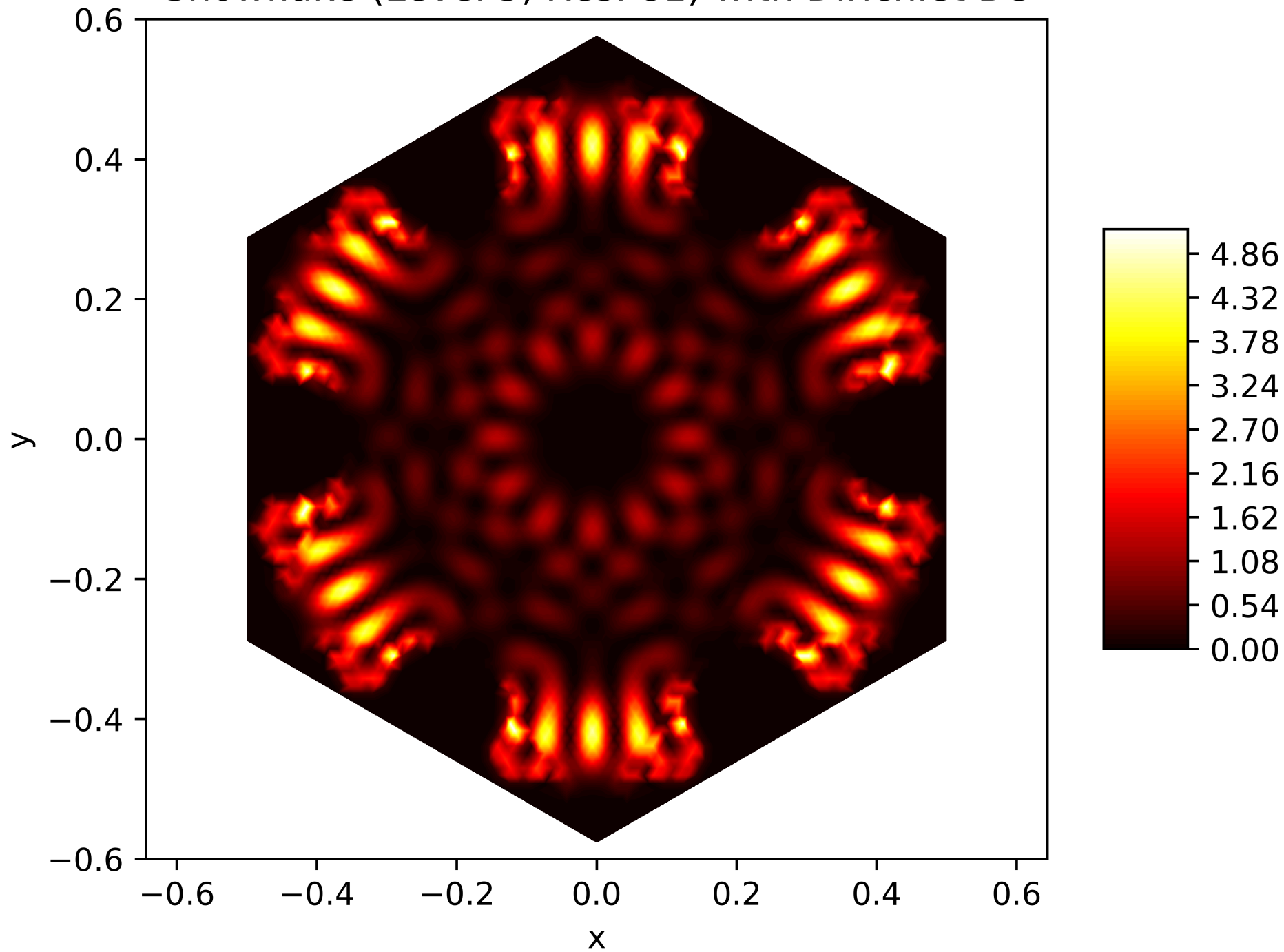
Energy Function of the 121. Eigenfunction on the Snowflake (Level 5, Res. 81) with Dirichlet BC
