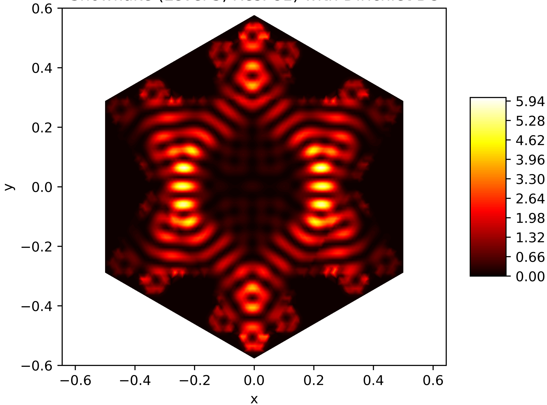
Energy Function of the 139. Eigenfunction on the Snowflake (Level 5, Res. 81) with Dirichlet BC
