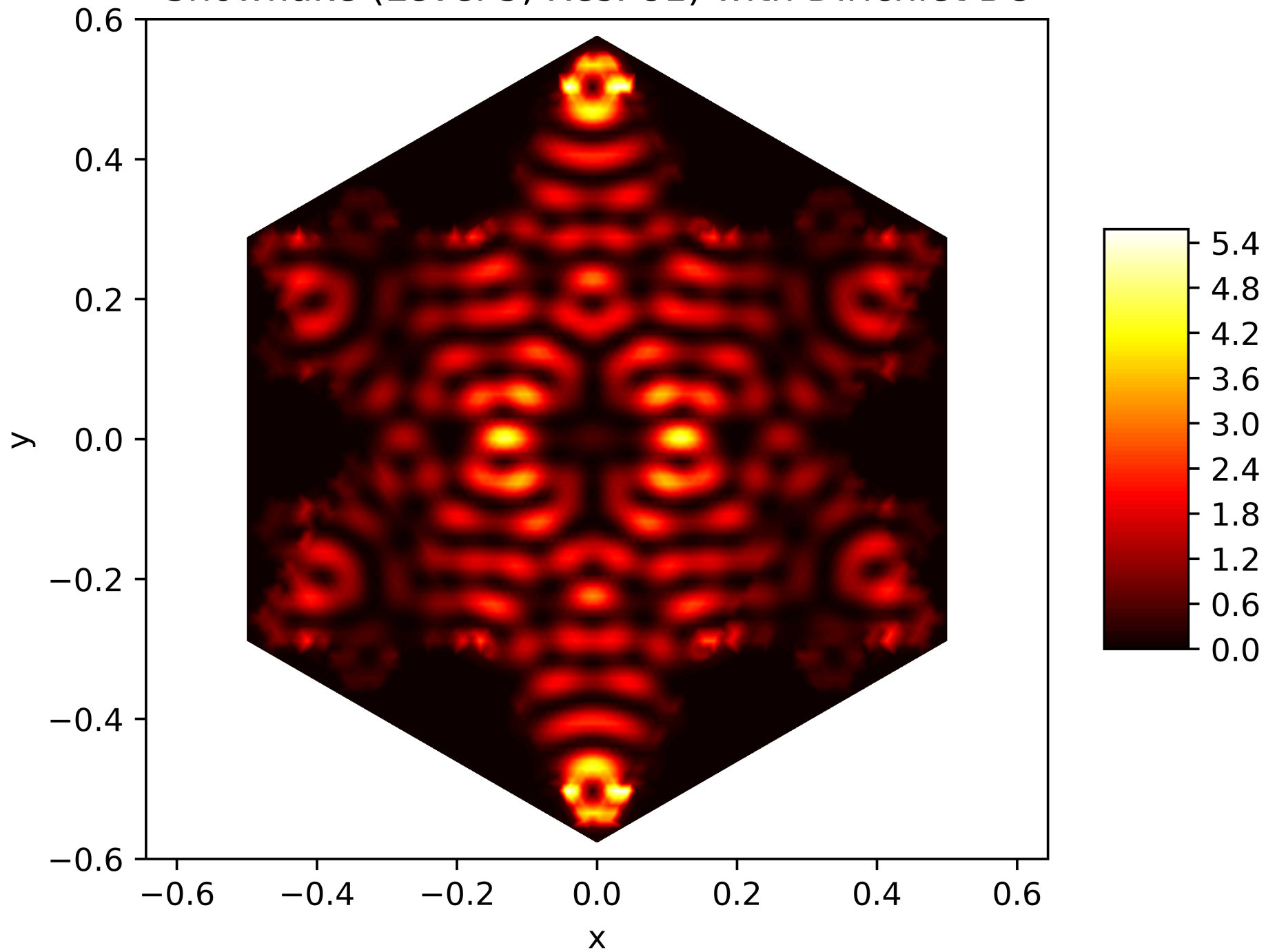
Energy Function of the 128. Eigenfunction on the Snowflake (Level 5, Res. 81) with Dirichlet BC
