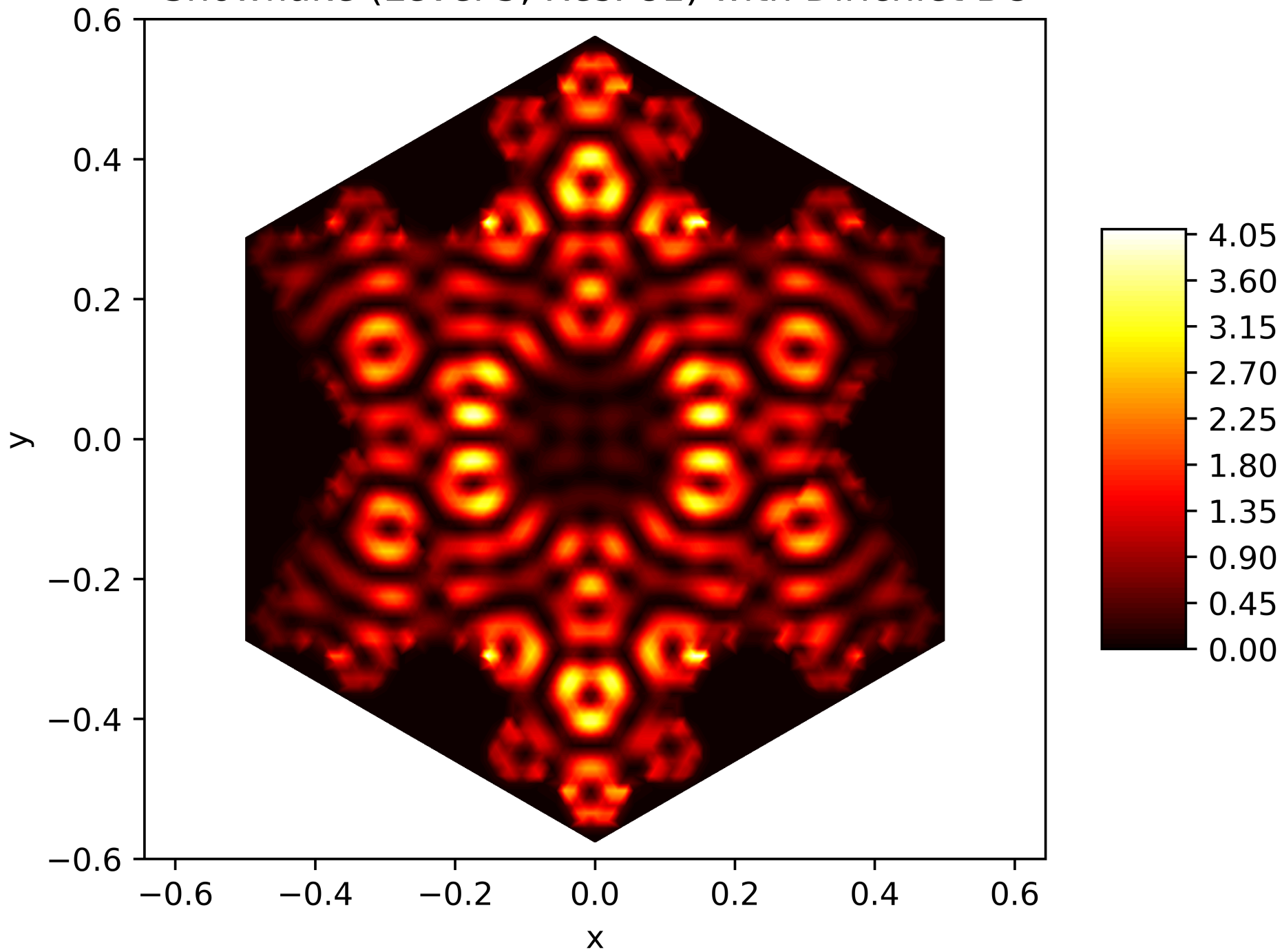
Energy Function of the 137. Eigenfunction on the Snowflake (Level 5, Res. 81) with Dirichlet BC
