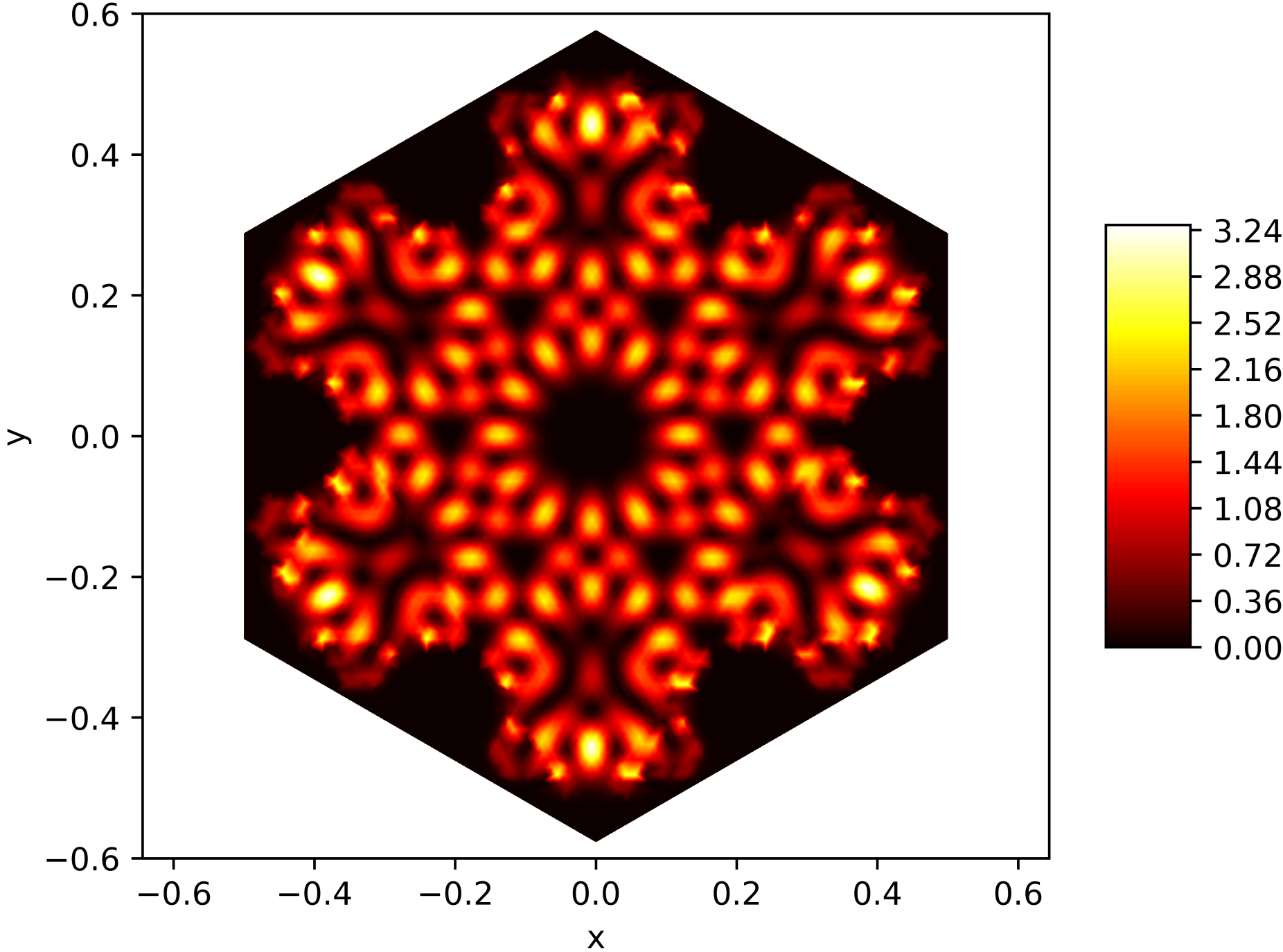
Energy Function of the 135. Eigenfunction on the Snowflake (Level 5, Res. 81) with Dirichlet BC
