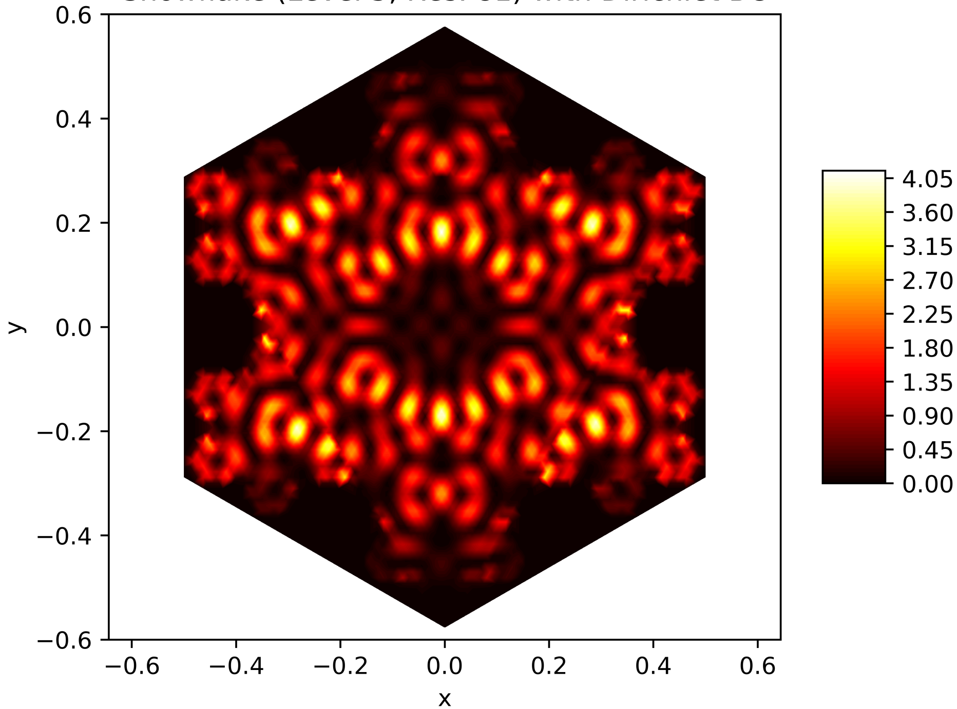
Energy Function of the 136. Eigenfunction on the Snowflake (Level 5, Res. 81) with Dirichlet BC
