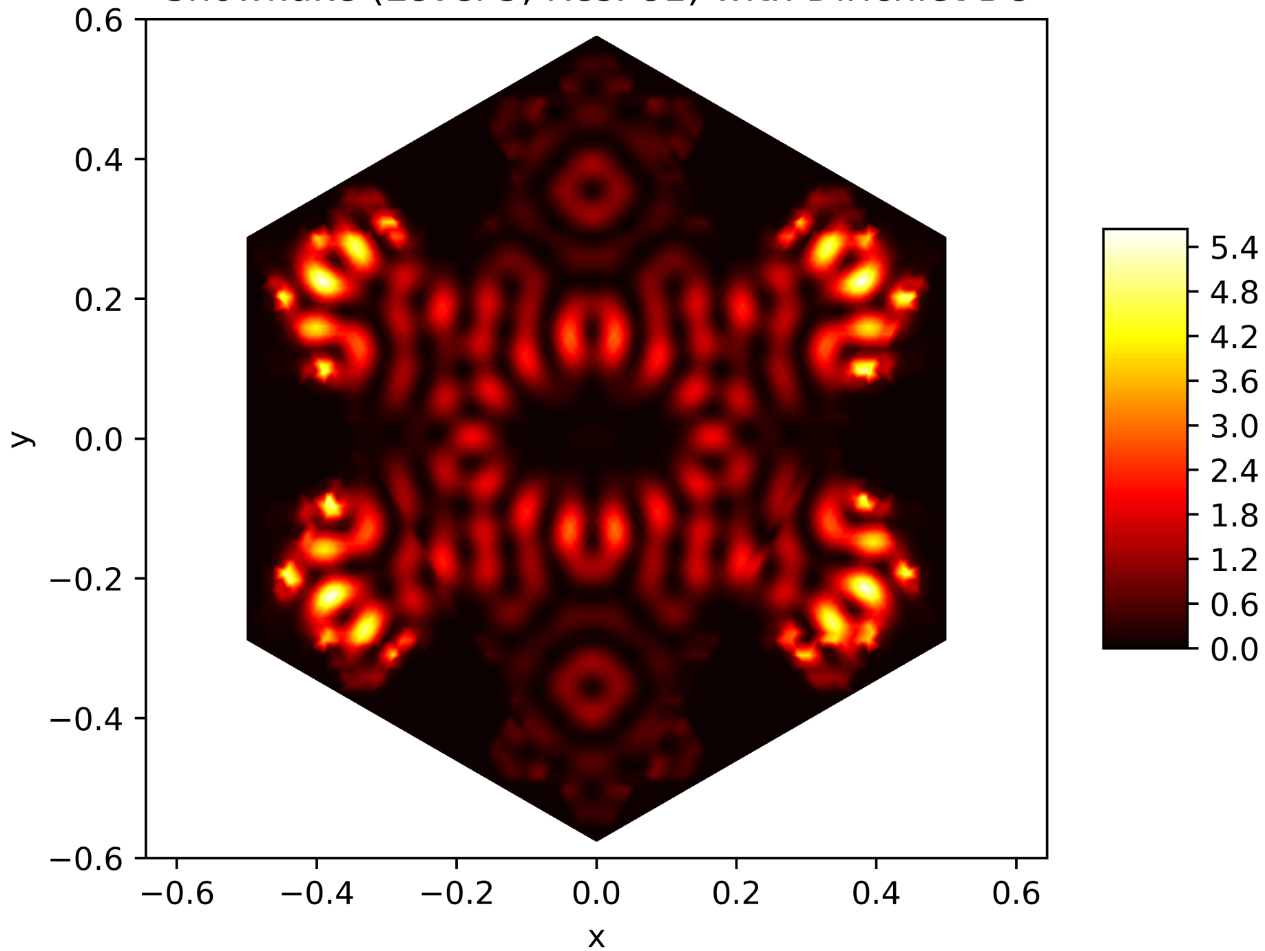
Energy Function of the 126. Eigenfunction on the Snowflake (Level 5, Res. 81) with Dirichlet BC
