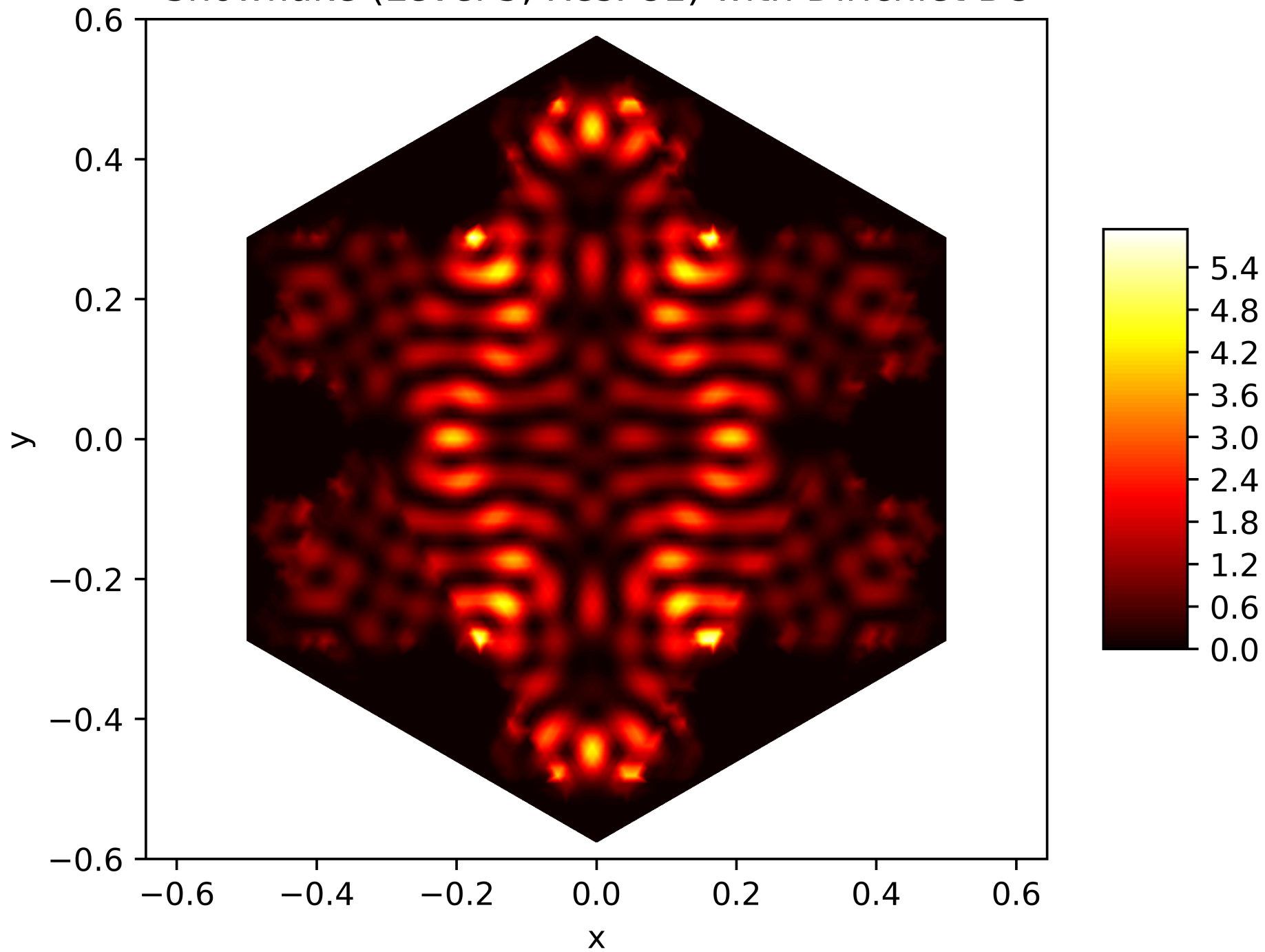
Energy Function of the 133. Eigenfunction on the Snowflake (Level 5, Res. 81) with Dirichlet BC
