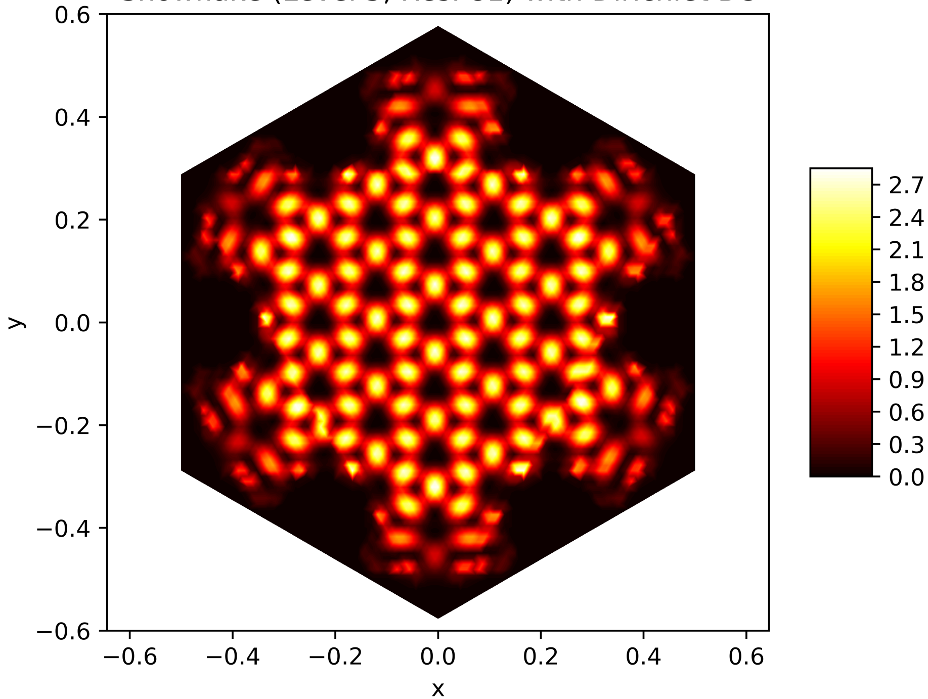
Energy Function of the 138. Eigenfunction on the Snowflake (Level 5, Res. 81) with Dirichlet BC
