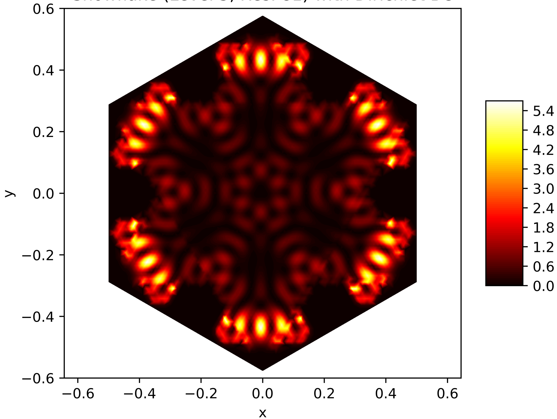
Energy Function of the 127. Eigenfunction on the Snowflake (Level 5, Res. 81) with Dirichlet BC
