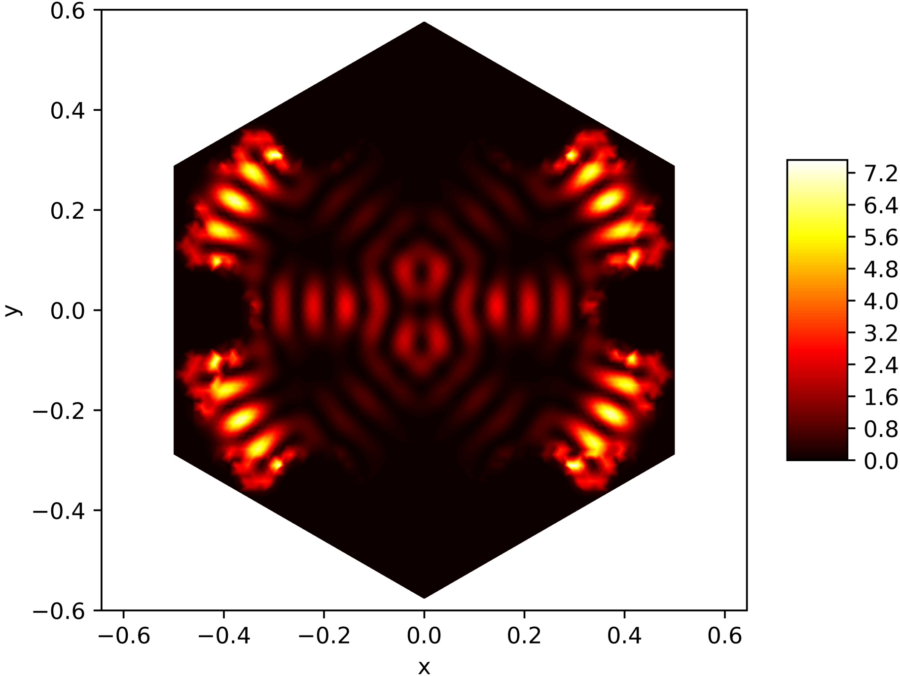
Energy Function of the 123. Eigenfunction on the Snowflake (Level 5, Res. 81) with Dirichlet BC
