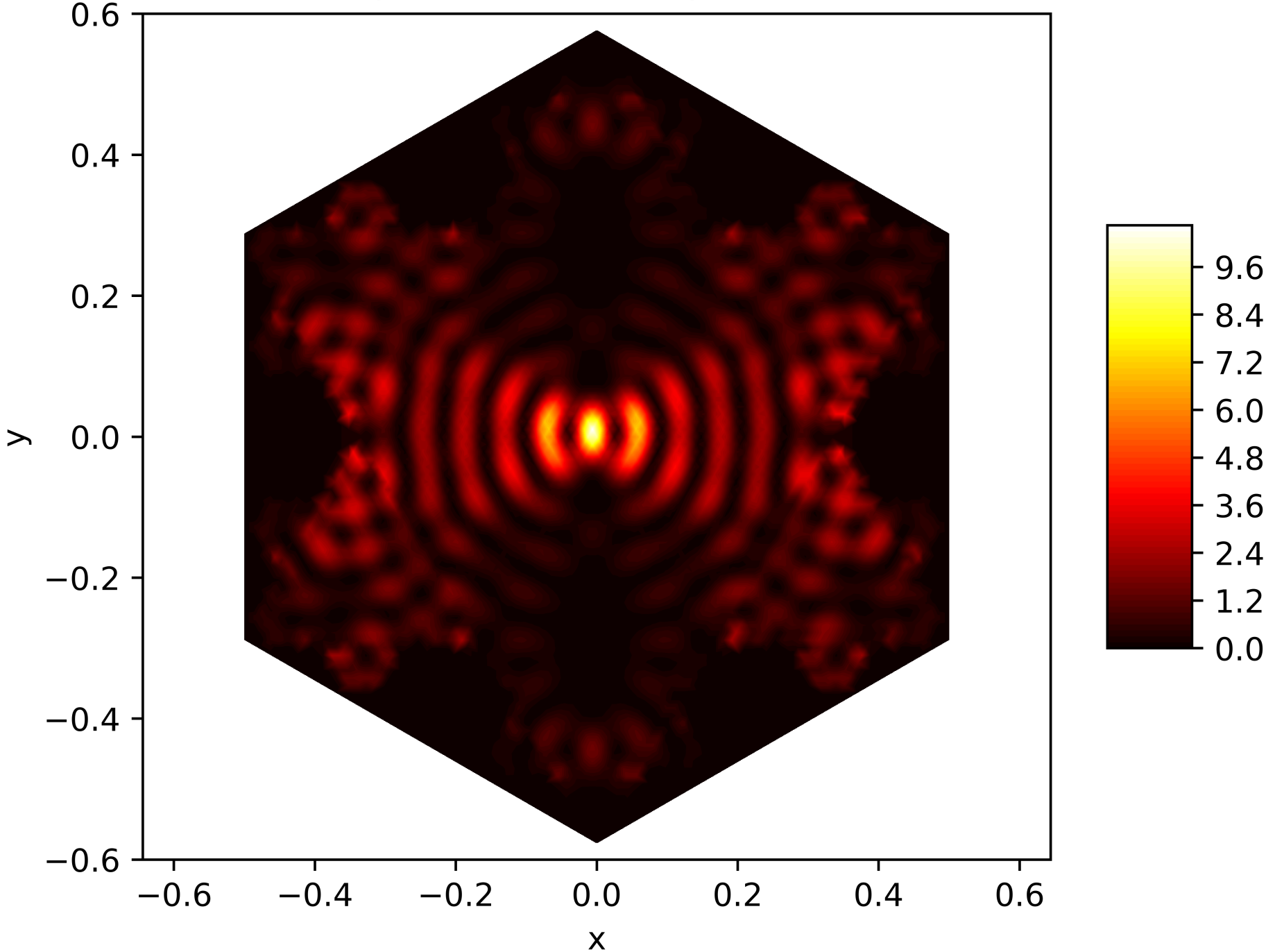
Energy Function of the 131. Eigenfunction on the Snowflake (Level 5, Res. 81) with Dirichlet BC
