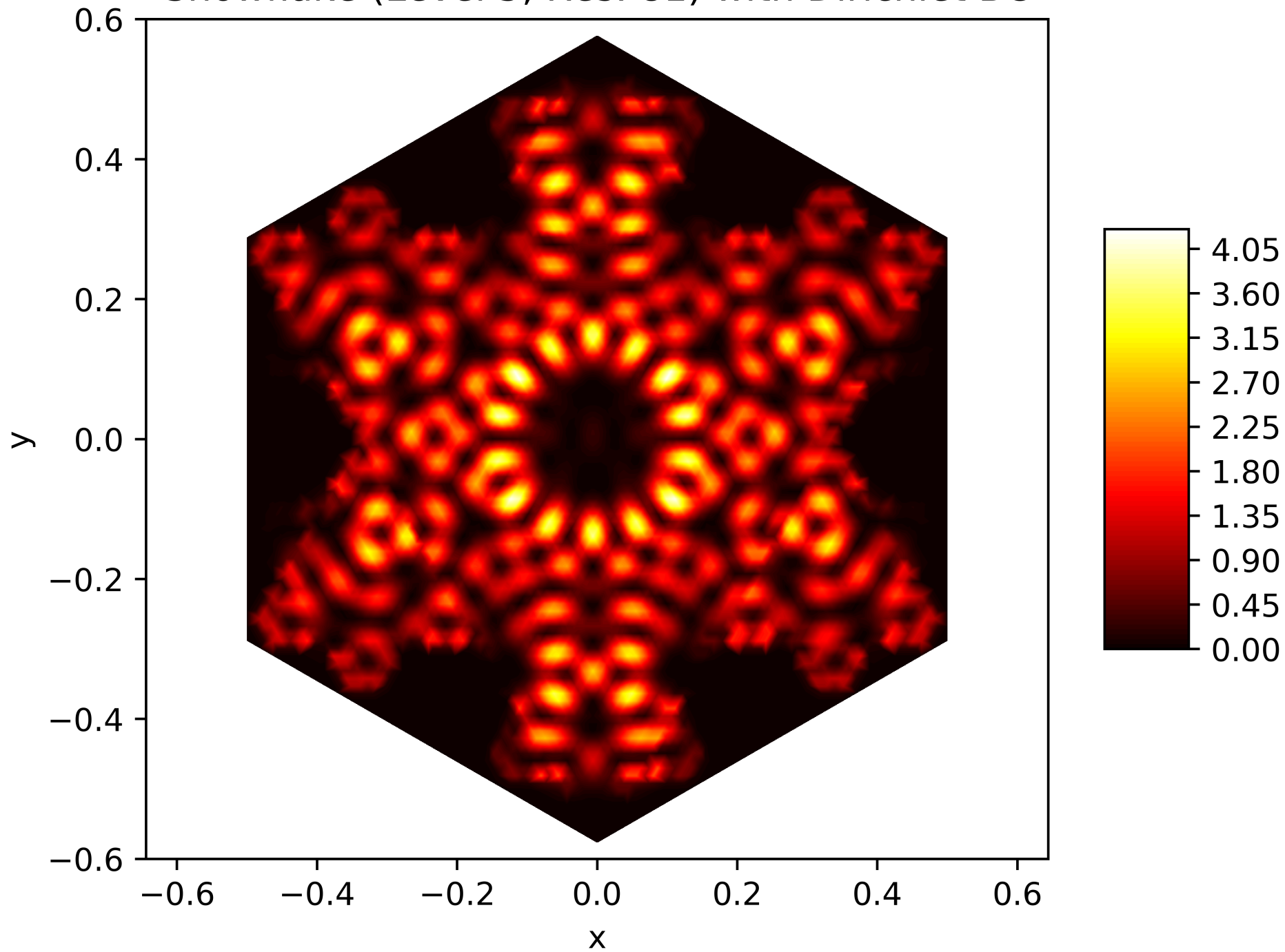
Energy Function of the 154. Eigenfunction on the Snowflake (Level 5, Res. 81) with Dirichlet BC
