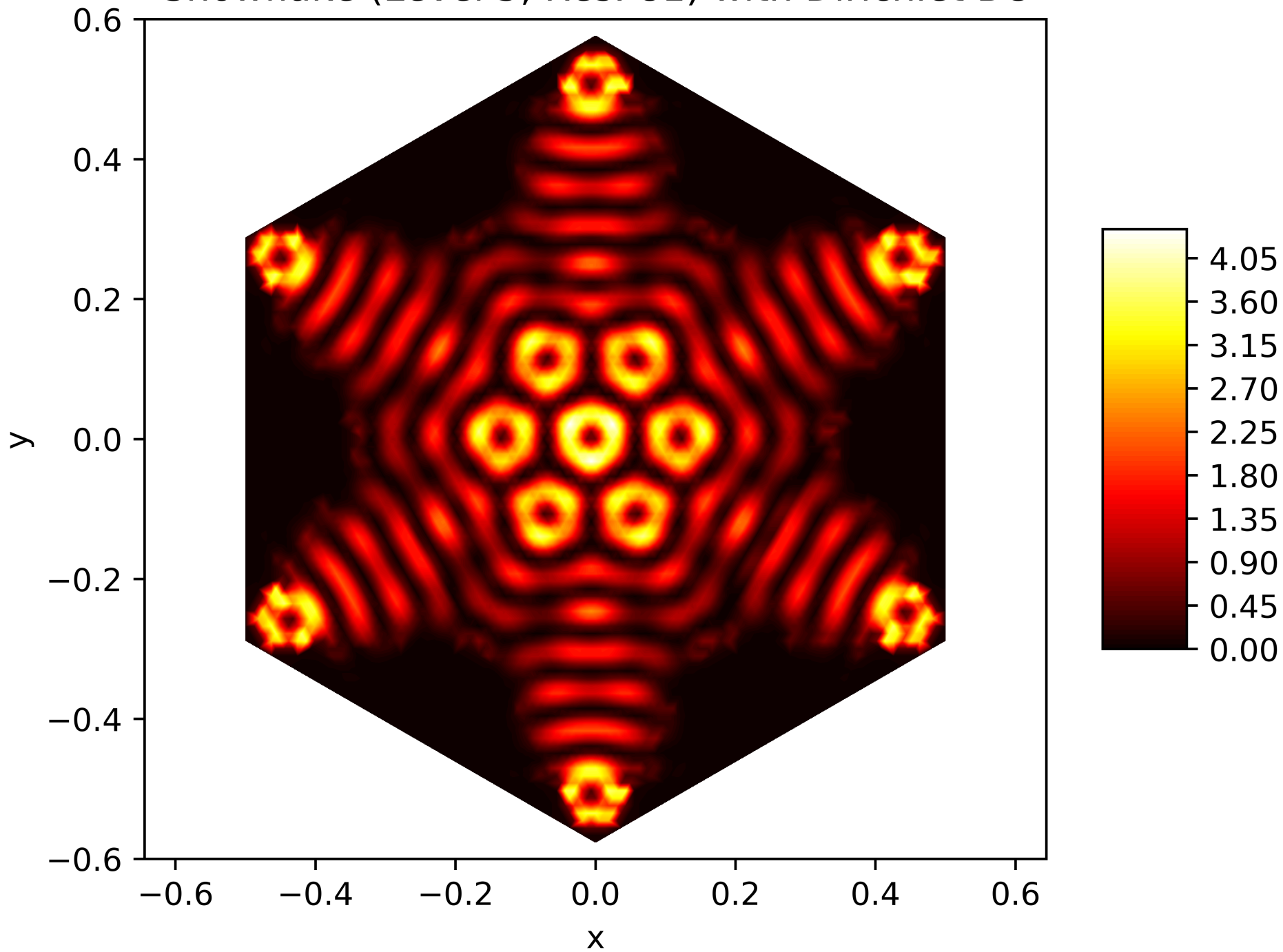
Energy Function of the 145. Eigenfunction on the Snowflake (Level 5, Res. 81) with Dirichlet BC
