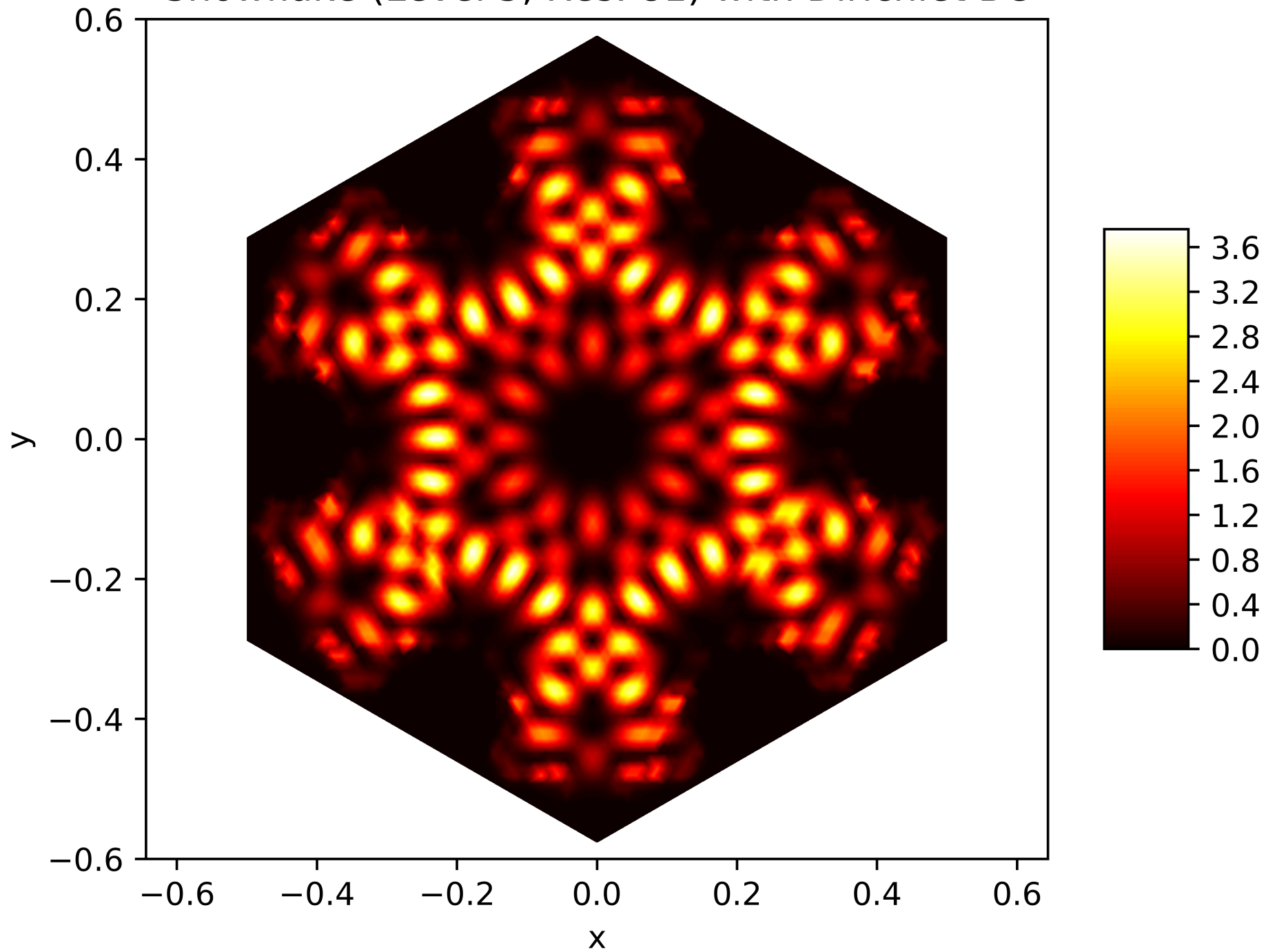
Energy Function of the 144. Eigenfunction on the Snowflake (Level 5, Res. 81) with Dirichlet BC
