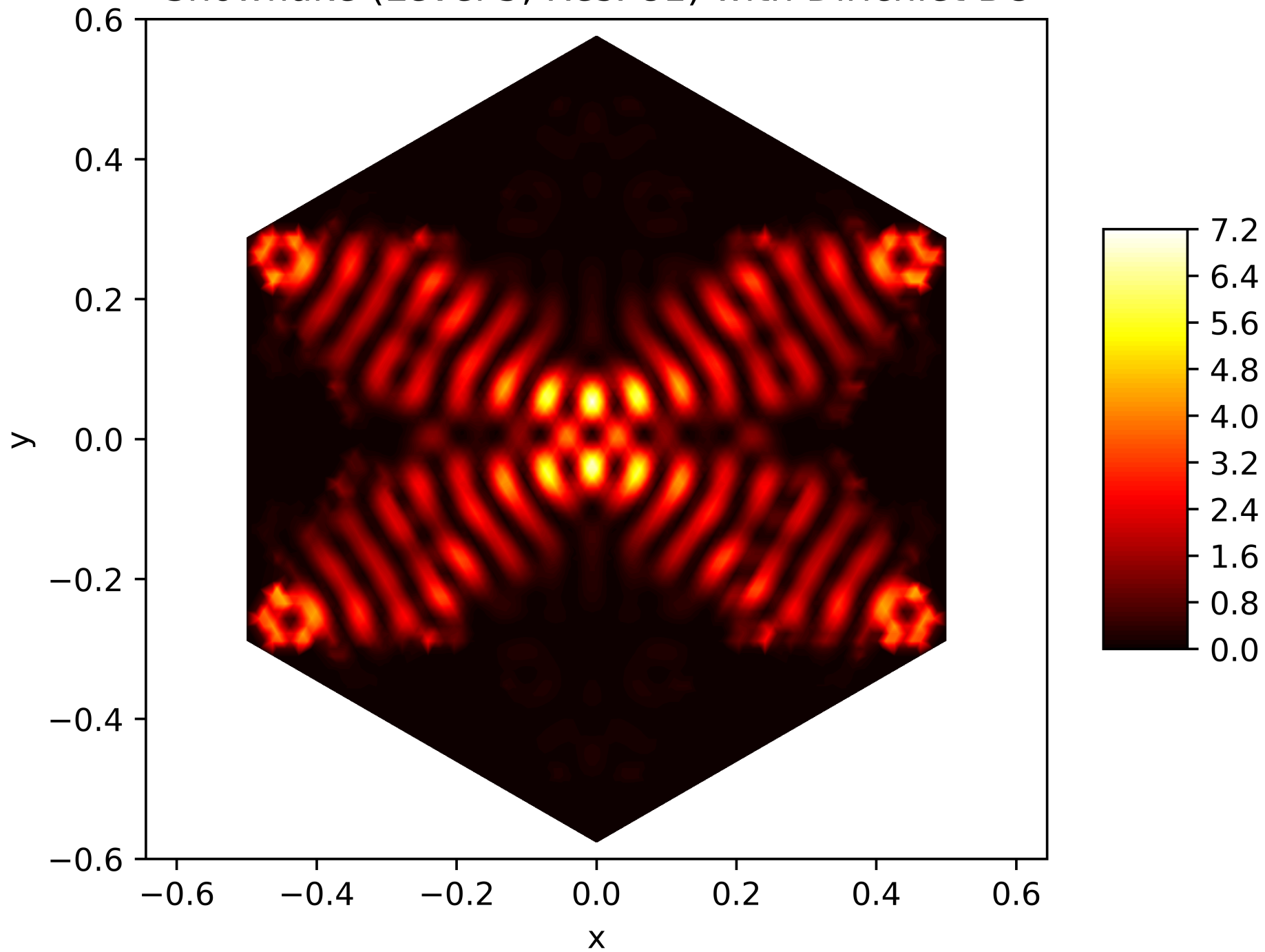
Energy Function of the 147. Eigenfunction on the Snowflake (Level 5, Res. 81) with Dirichlet BC
