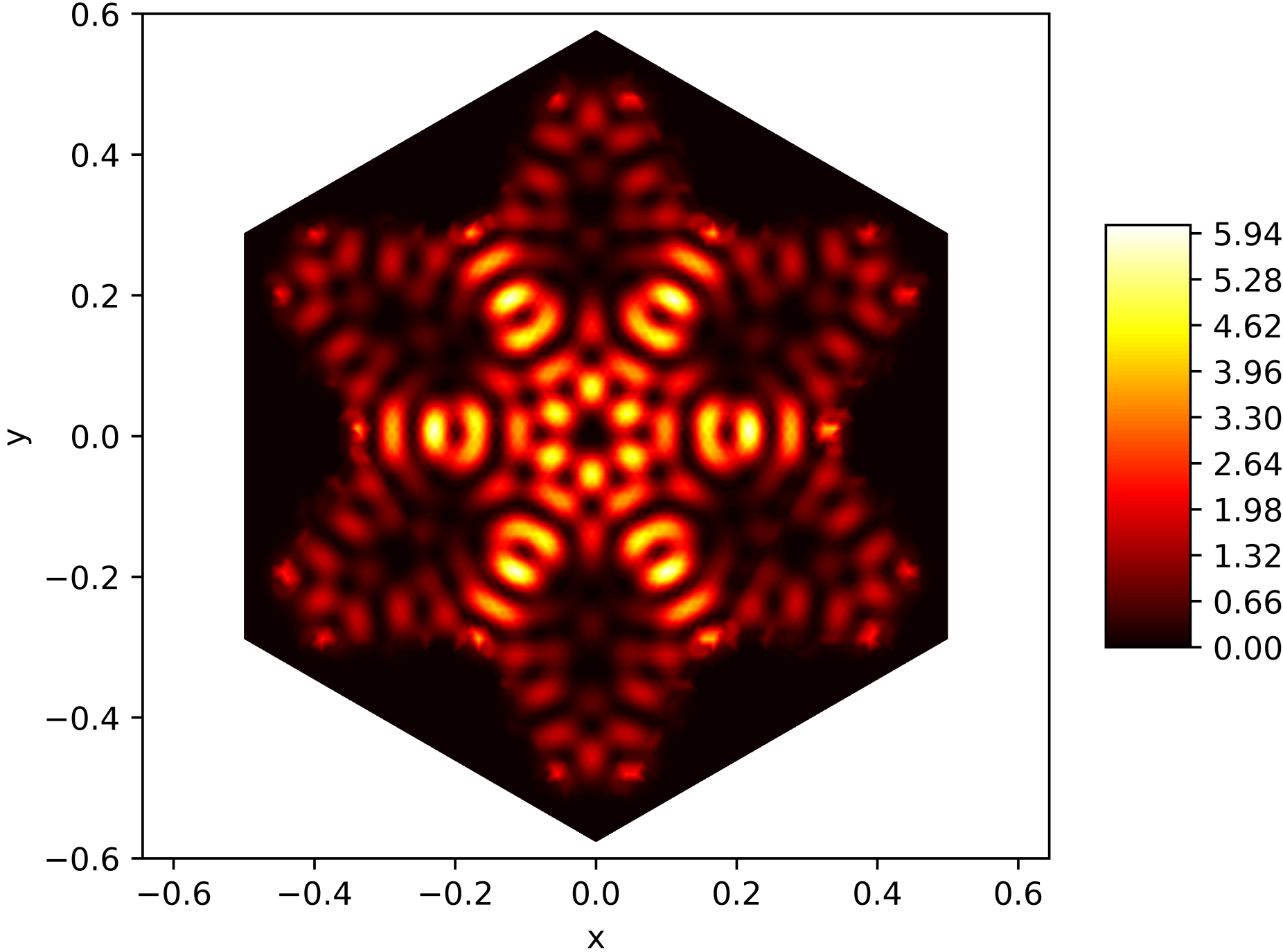
Energy Function of the 152. Eigenfunction on the Snowflake (Level 5, Res. 81) with Dirichlet BC
