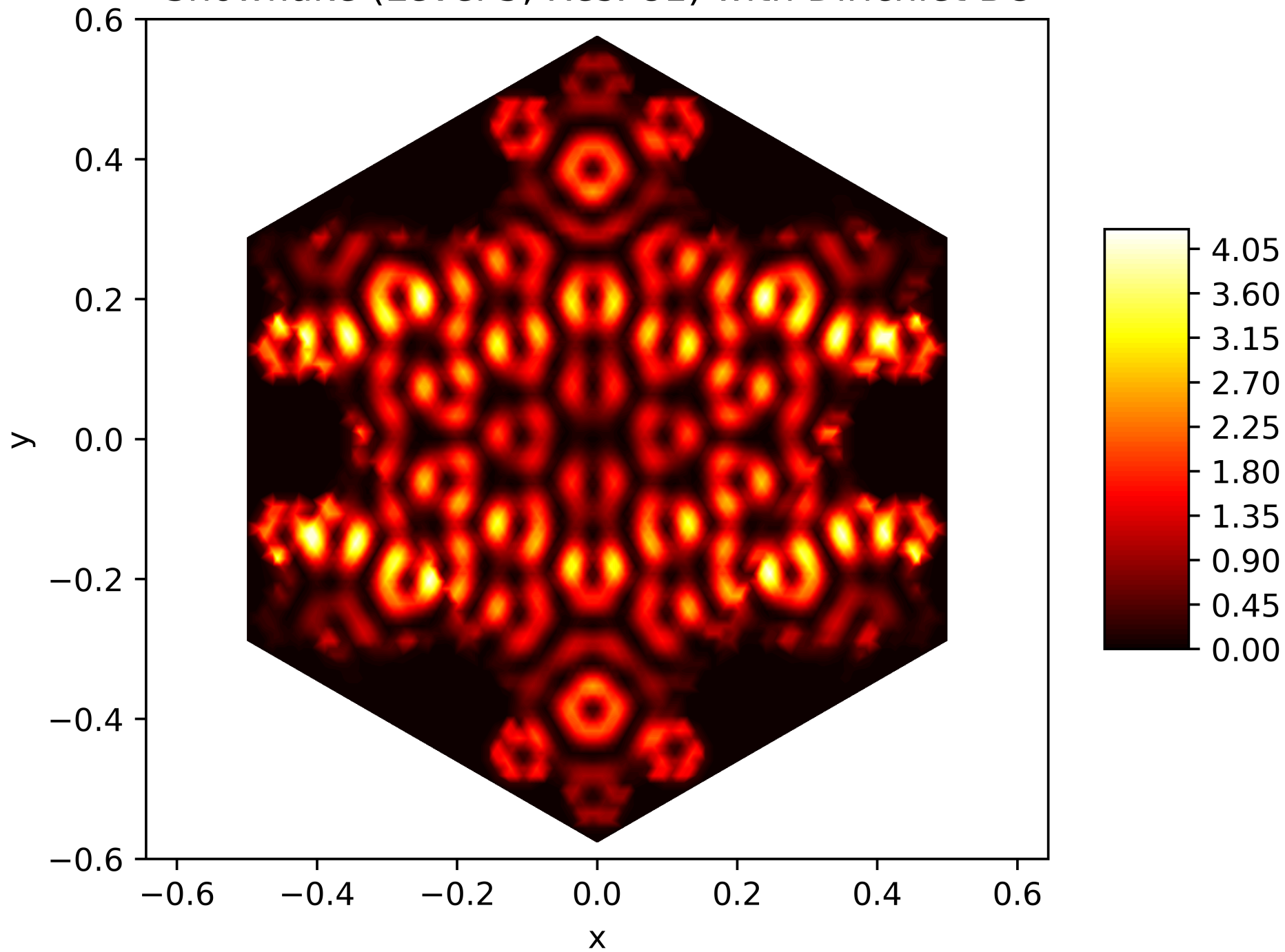
Energy Function of the 155. Eigenfunction on the Snowflake (Level 5, Res. 81) with Dirichlet BC
