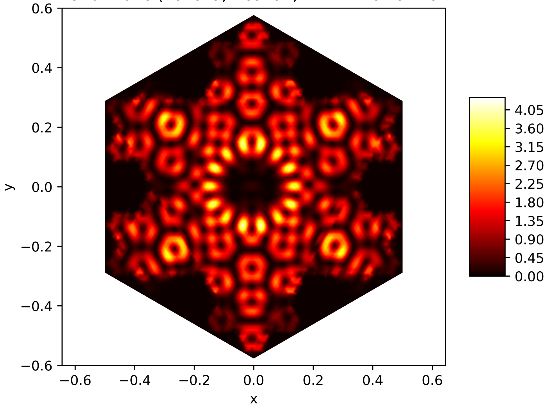
Energy Function of the 153. Eigenfunction on the Snowflake (Level 5, Res. 81) with Dirichlet BC
