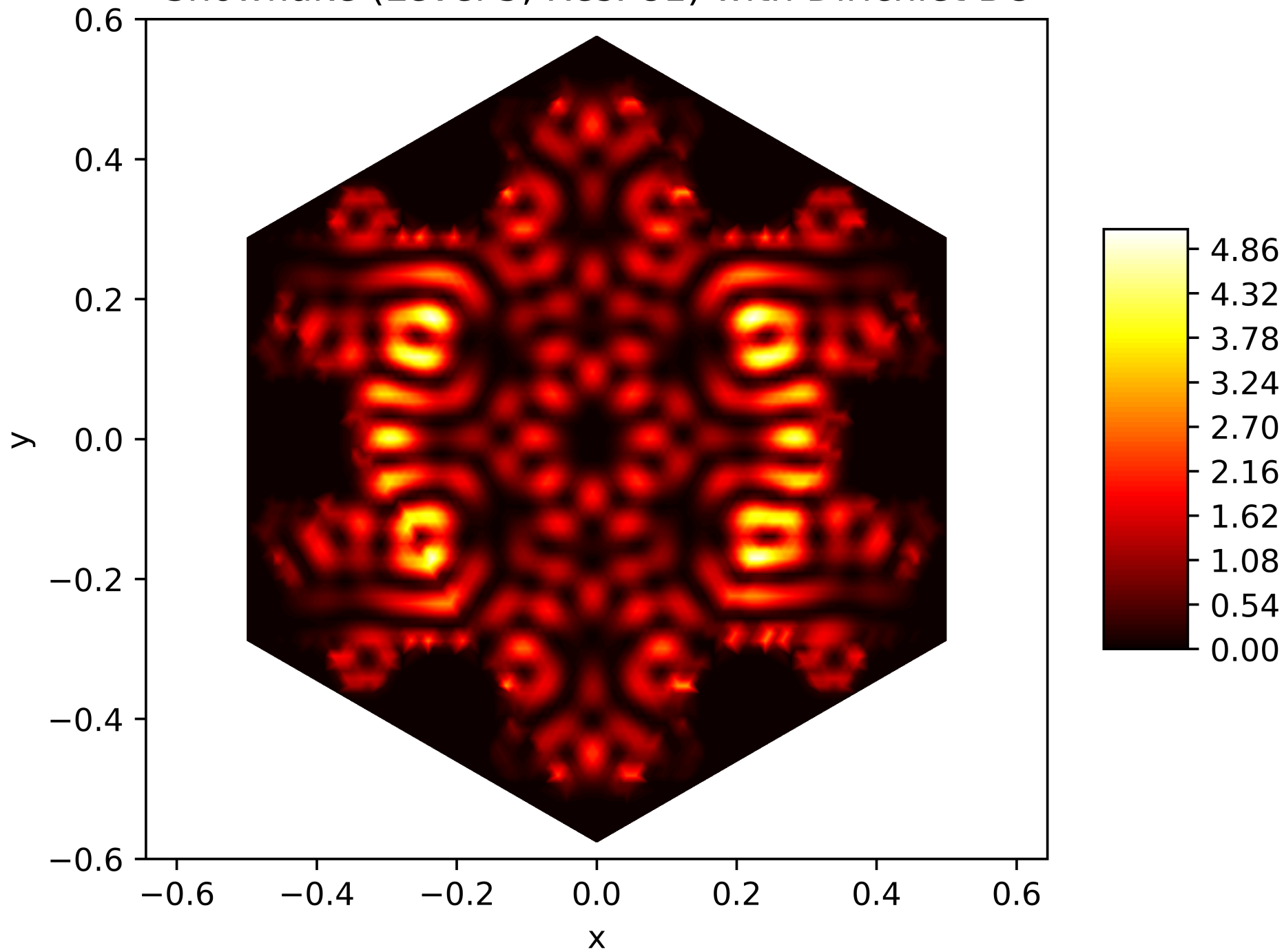
Energy Function of the 142. Eigenfunction on the Snowflake (Level 5, Res. 81) with Dirichlet BC
