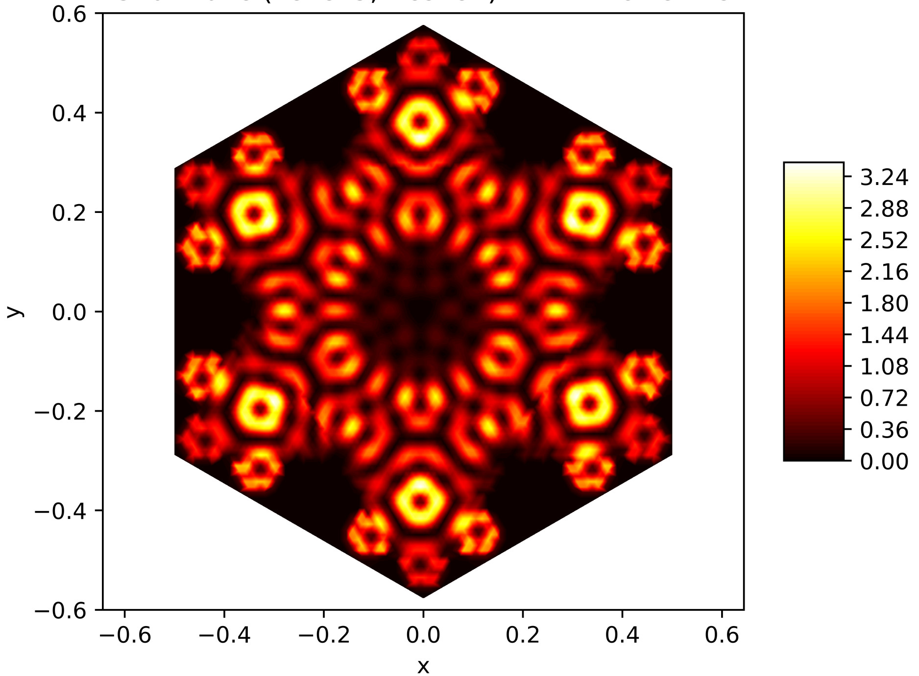
Energy Function of the 151. Eigenfunction on the Snowflake (Level 5, Res. 81) with Dirichlet BC
