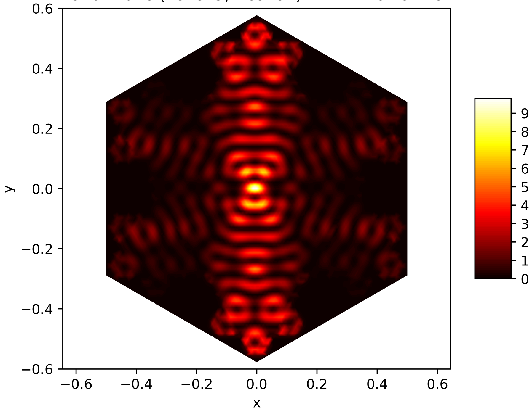
Energy Function of the 157. Eigenfunction on the Snowflake (Level 5, Res. 81) with Dirichlet BC
