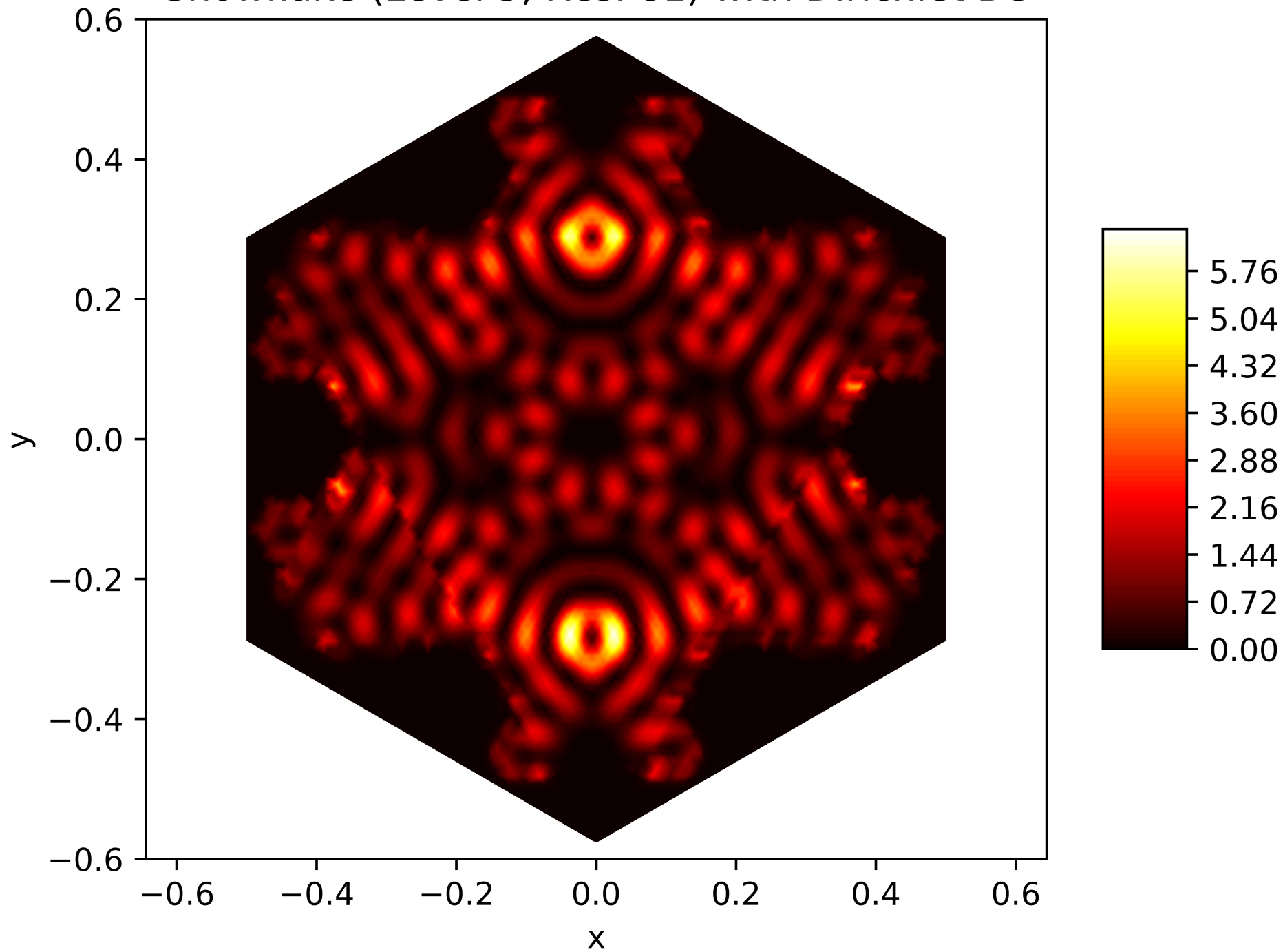
Energy Function of the 143. Eigenfunction on the Snowflake (Level 5, Res. 81) with Dirichlet BC
