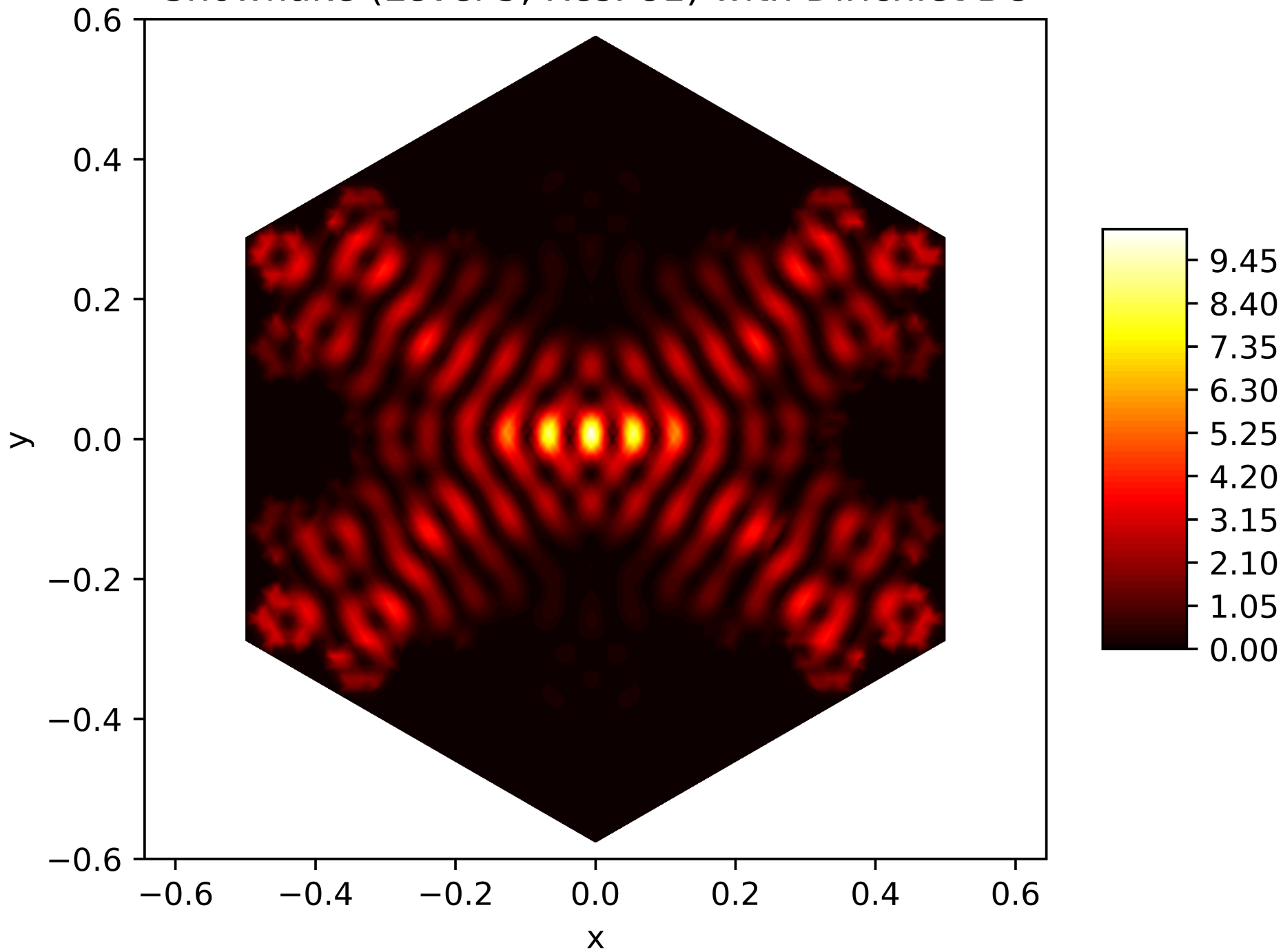
Energy Function of the 158. Eigenfunction on the Snowflake (Level 5, Res. 81) with Dirichlet BC
