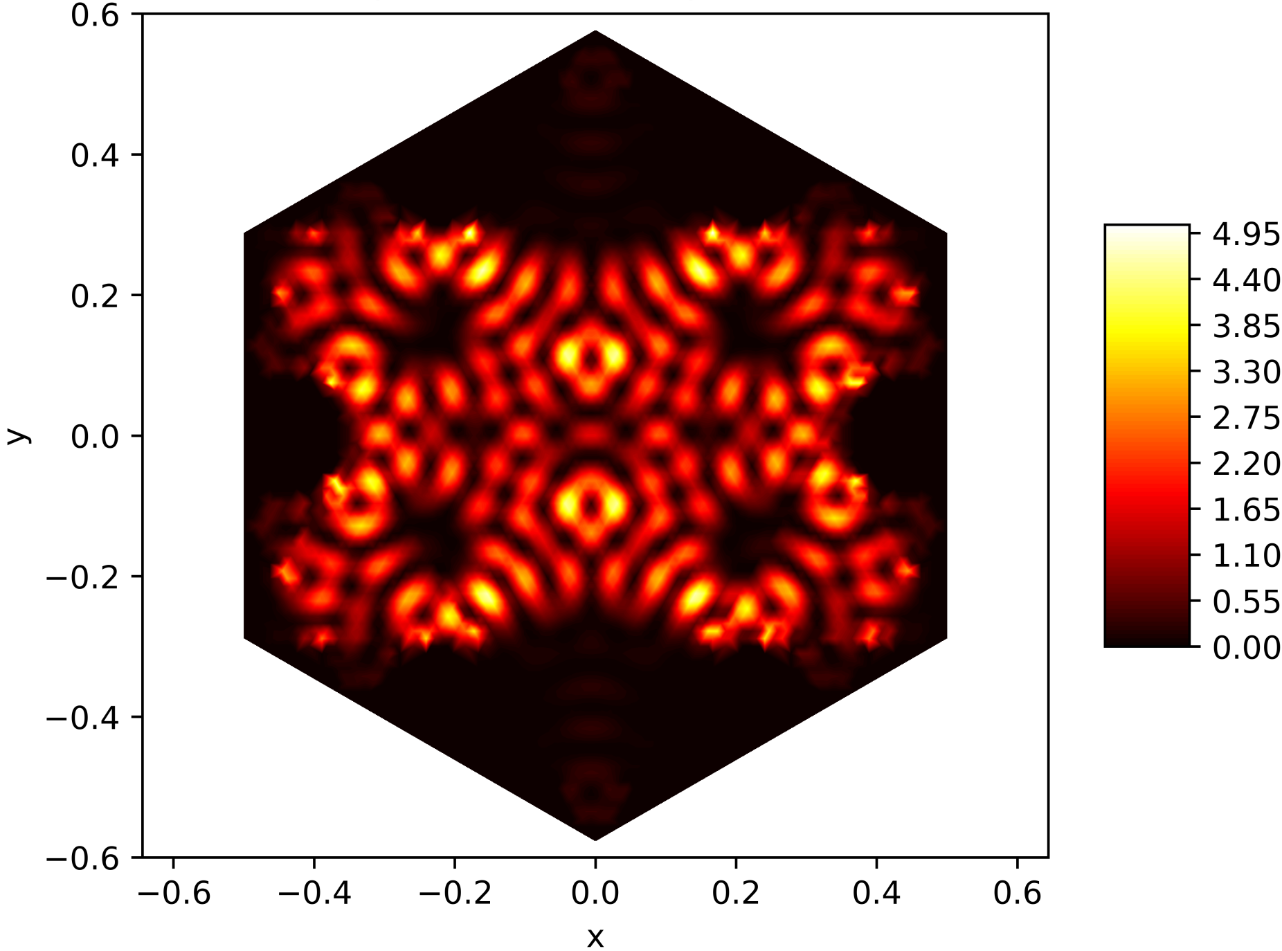
Energy Function of the 150. Eigenfunction on the Snowflake (Level 5, Res. 81) with Dirichlet BC
