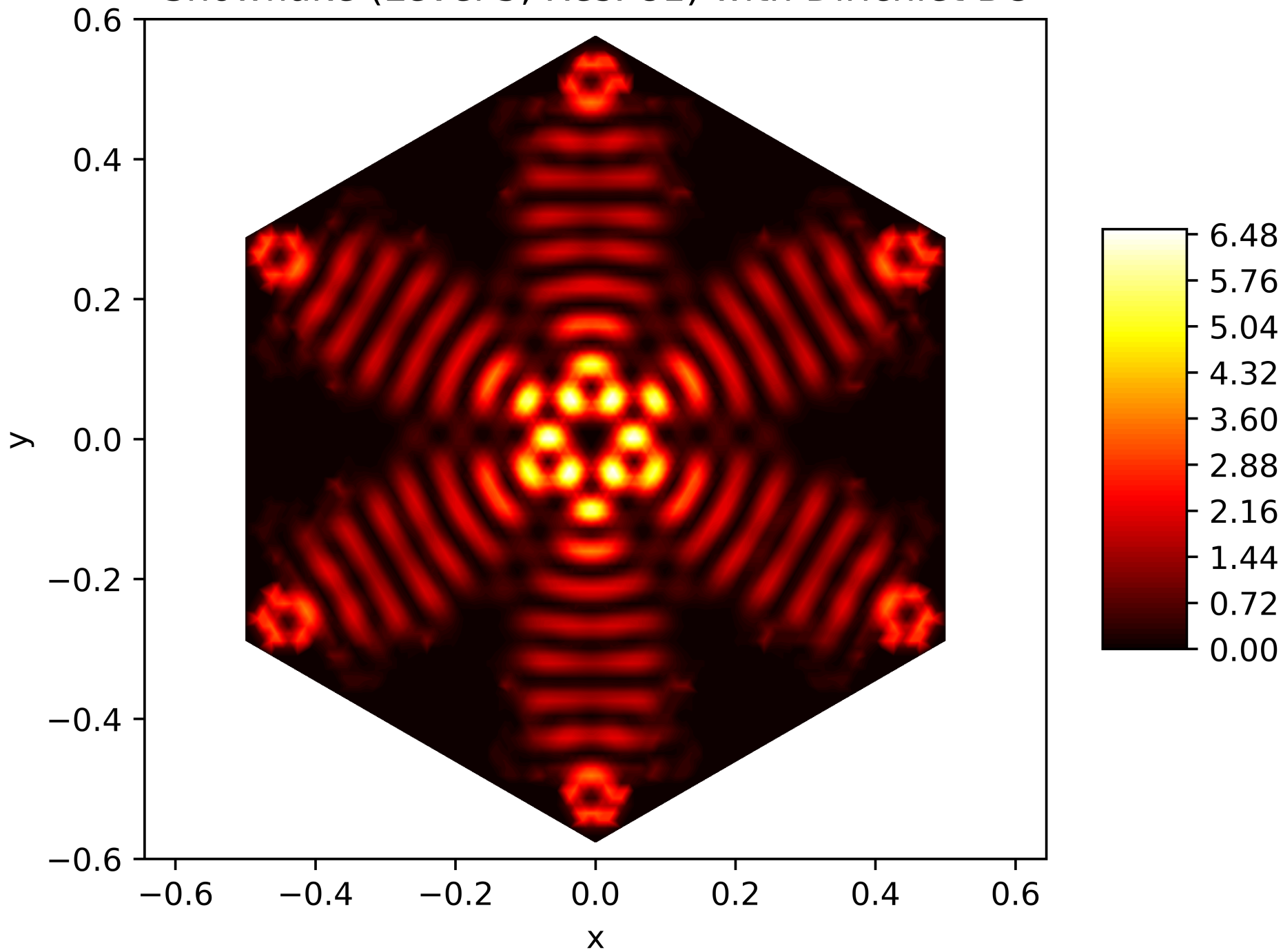
Energy Function of the 159. Eigenfunction on the Snowflake (Level 5, Res. 81) with Dirichlet BC
