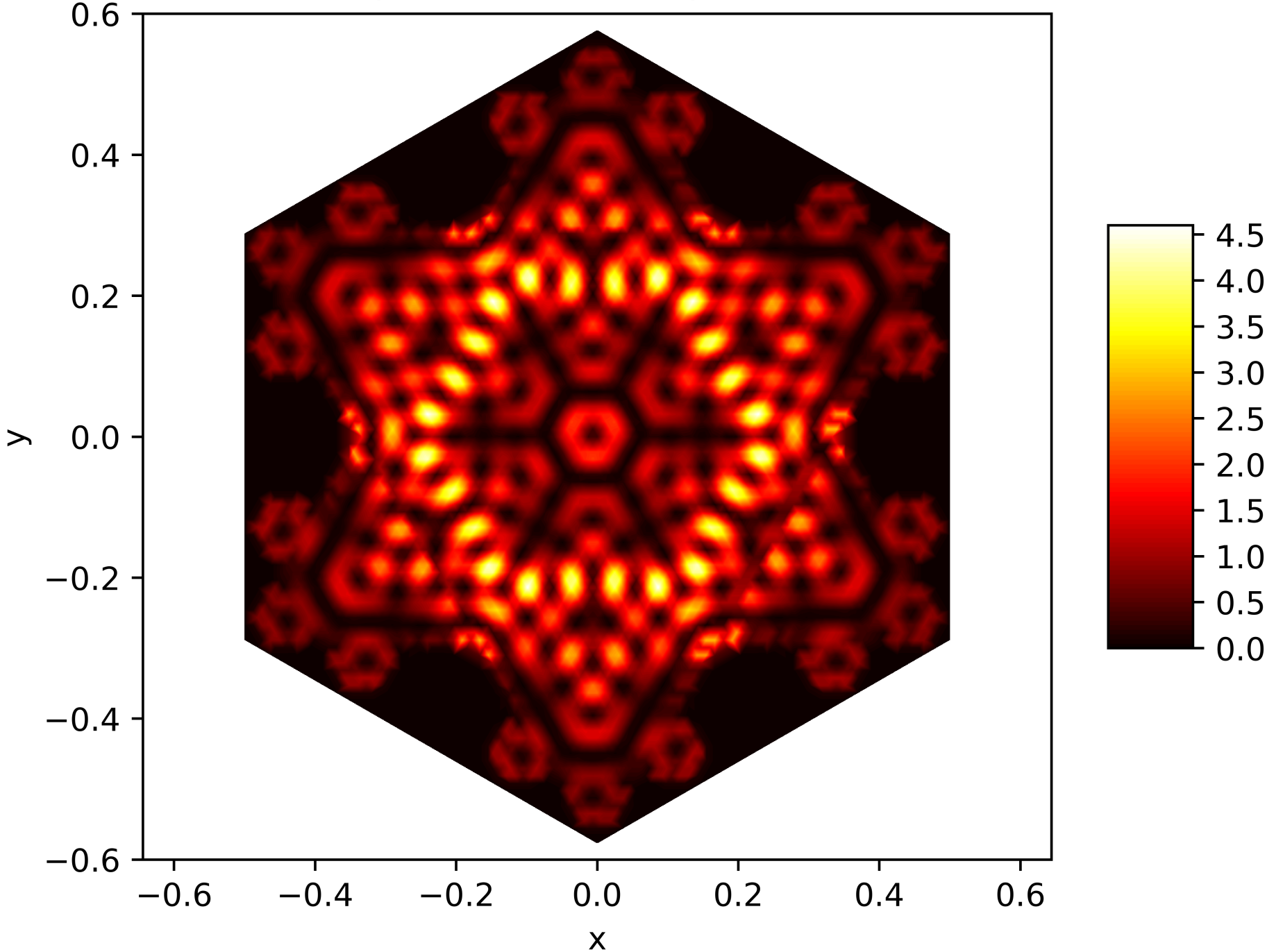
Energy Function of the 160. Eigenfunction on the Snowflake (Level 5, Res. 81) with Dirichlet BC
