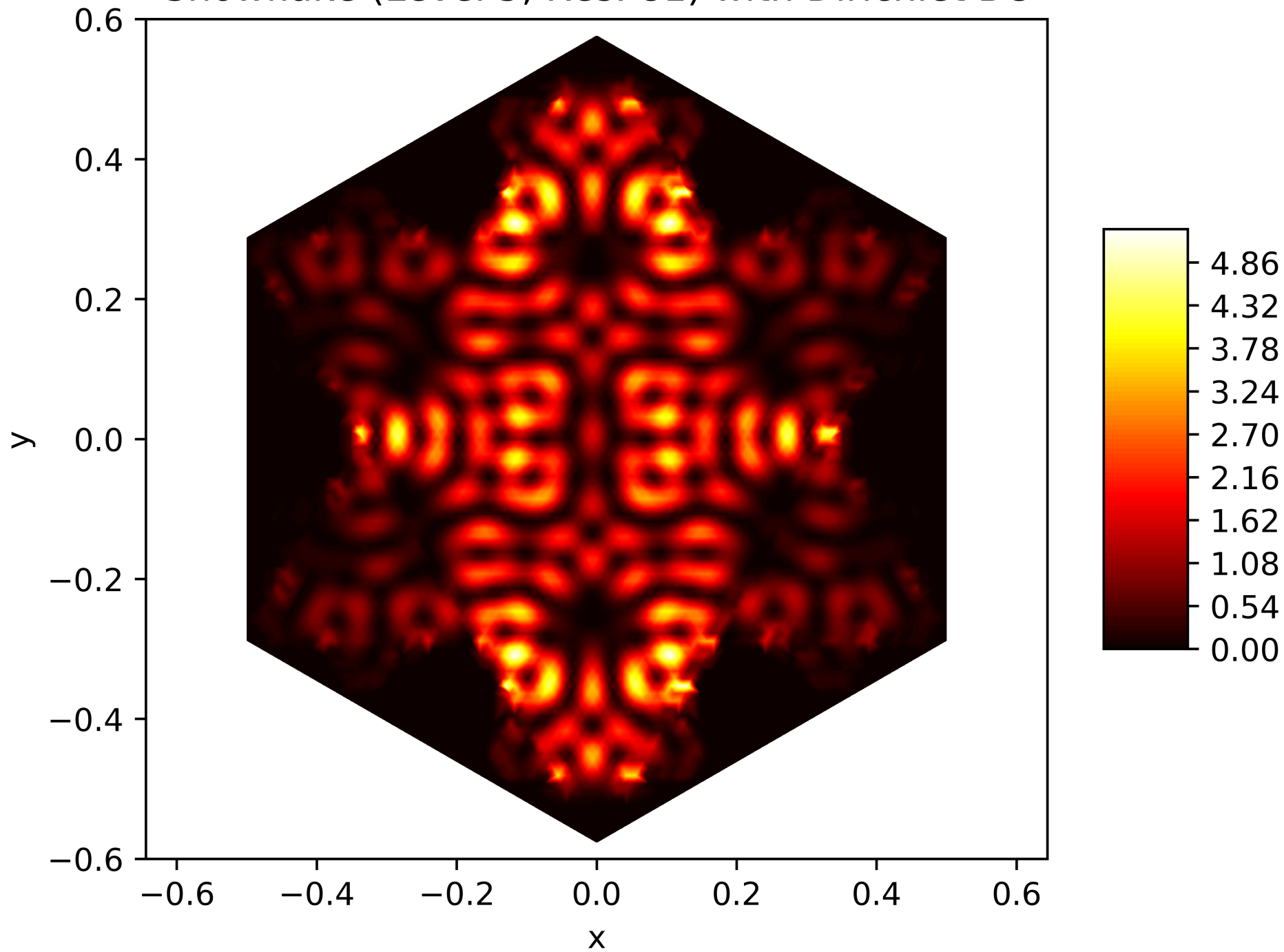
Energy Function of the 149. Eigenfunction on the Snowflake (Level 5, Res. 81) with Dirichlet BC
