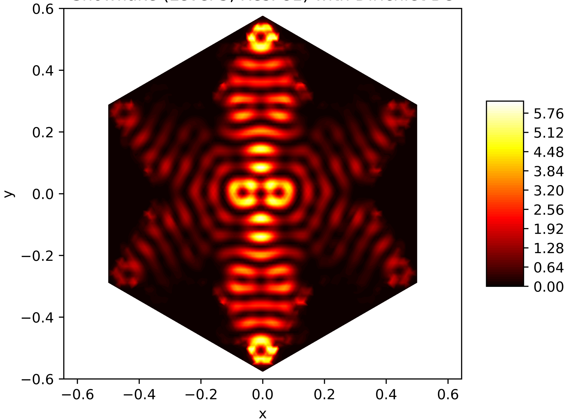
Energy Function of the 146. Eigenfunction on the Snowflake (Level 5, Res. 81) with Dirichlet BC
