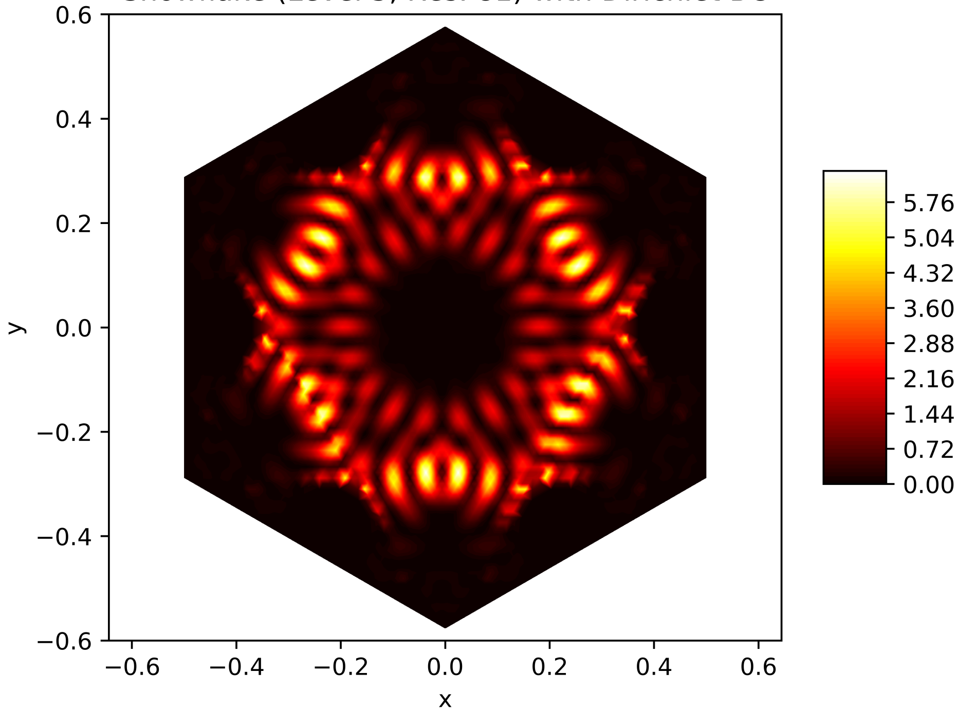
Energy Function of the 141. Eigenfunction on the Snowflake (Level 5, Res. 81) with Dirichlet BC
