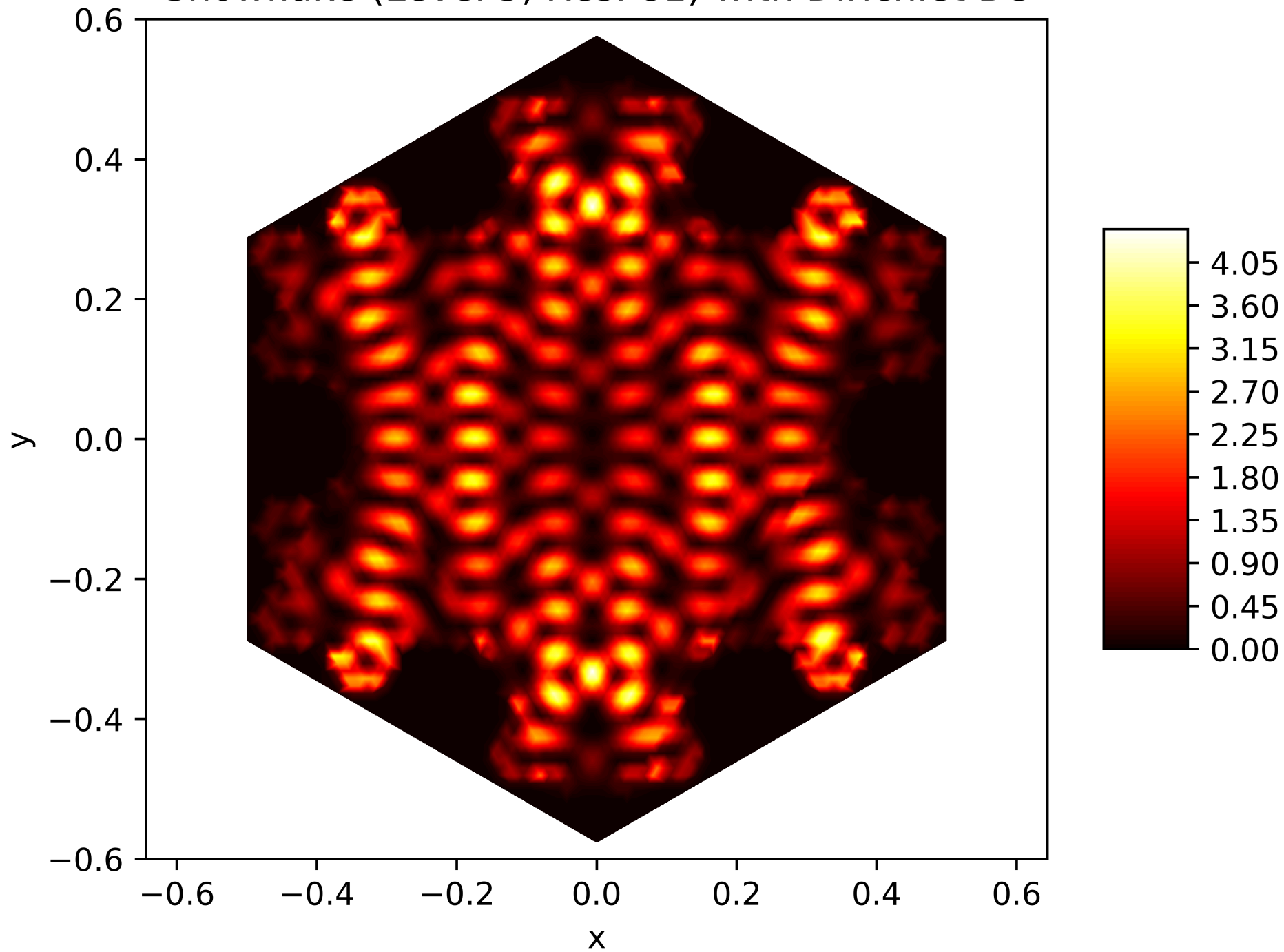
Energy Function of the 156. Eigenfunction on the Snowflake (Level 5, Res. 81) with Dirichlet BC
