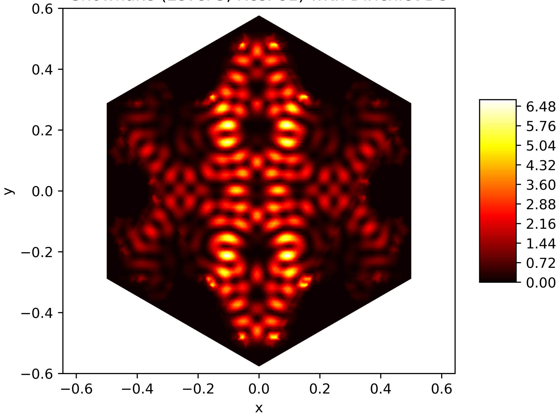
Energy Function of the 171. Eigenfunction on the Snowflake (Level 5, Res. 81) with Dirichlet BC
