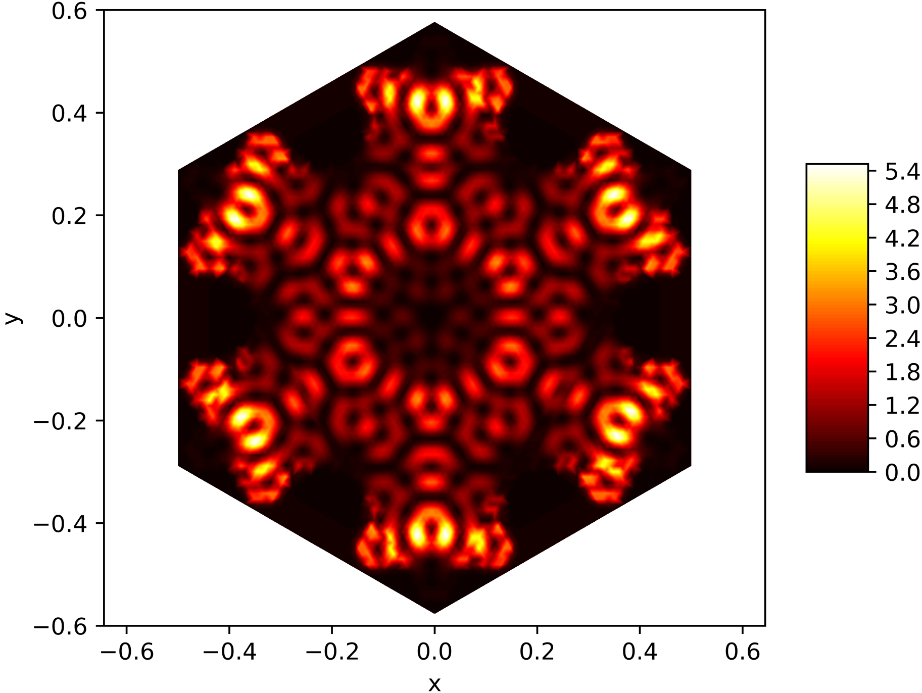
Energy Function of the 179. Eigenfunction on the Snowflake (Level 5, Res. 81) with Dirichlet BC
