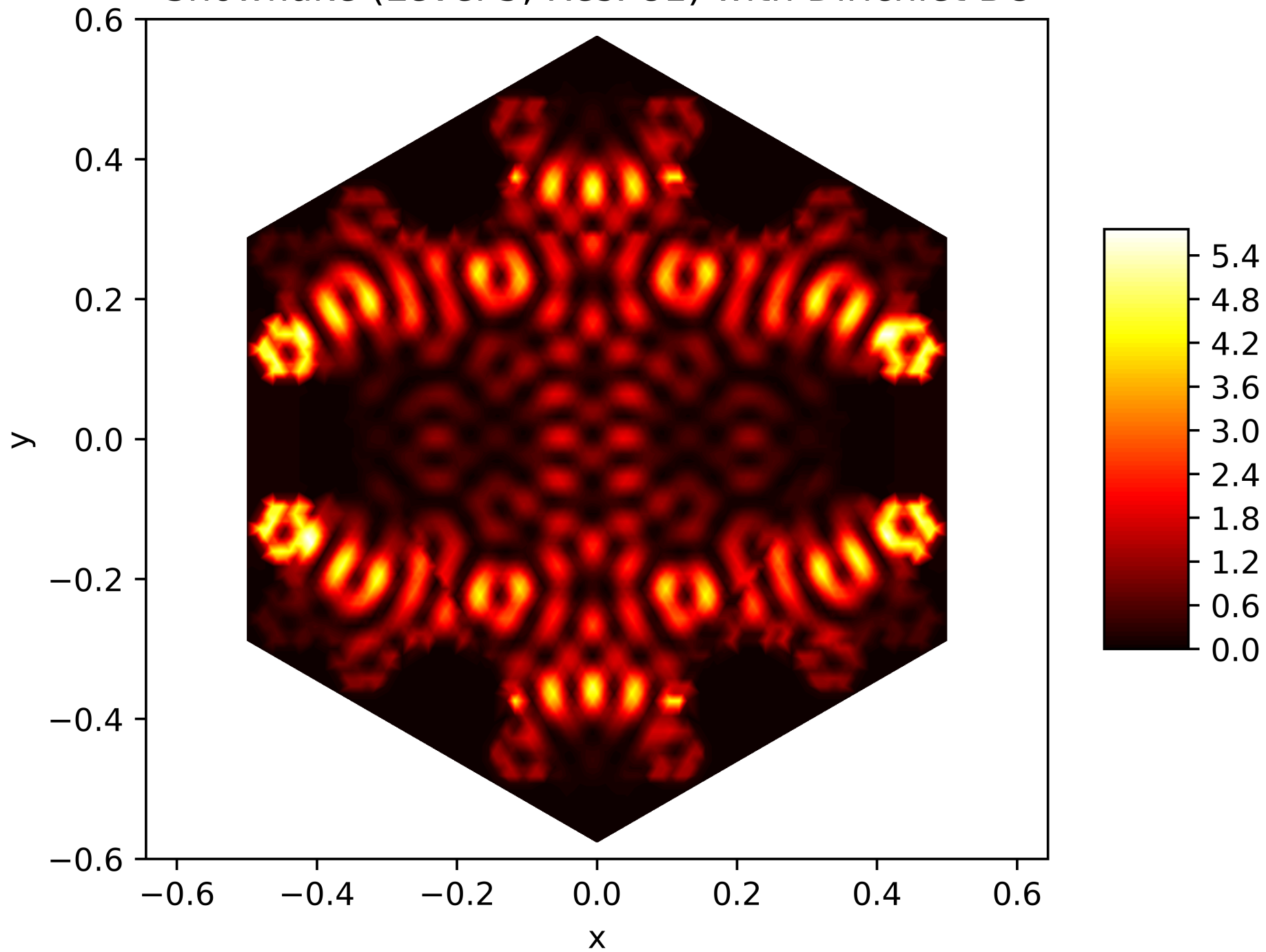
Energy Function of the 170. Eigenfunction on the Snowflake (Level 5, Res. 81) with Dirichlet BC
