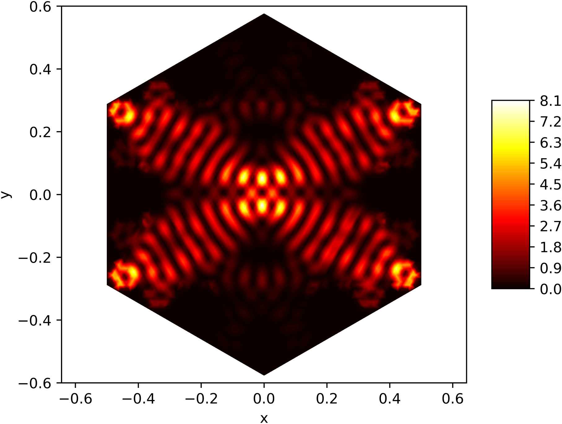
Energy Function of the 177. Eigenfunction on the Snowflake (Level 5, Res. 81) with Dirichlet BC
