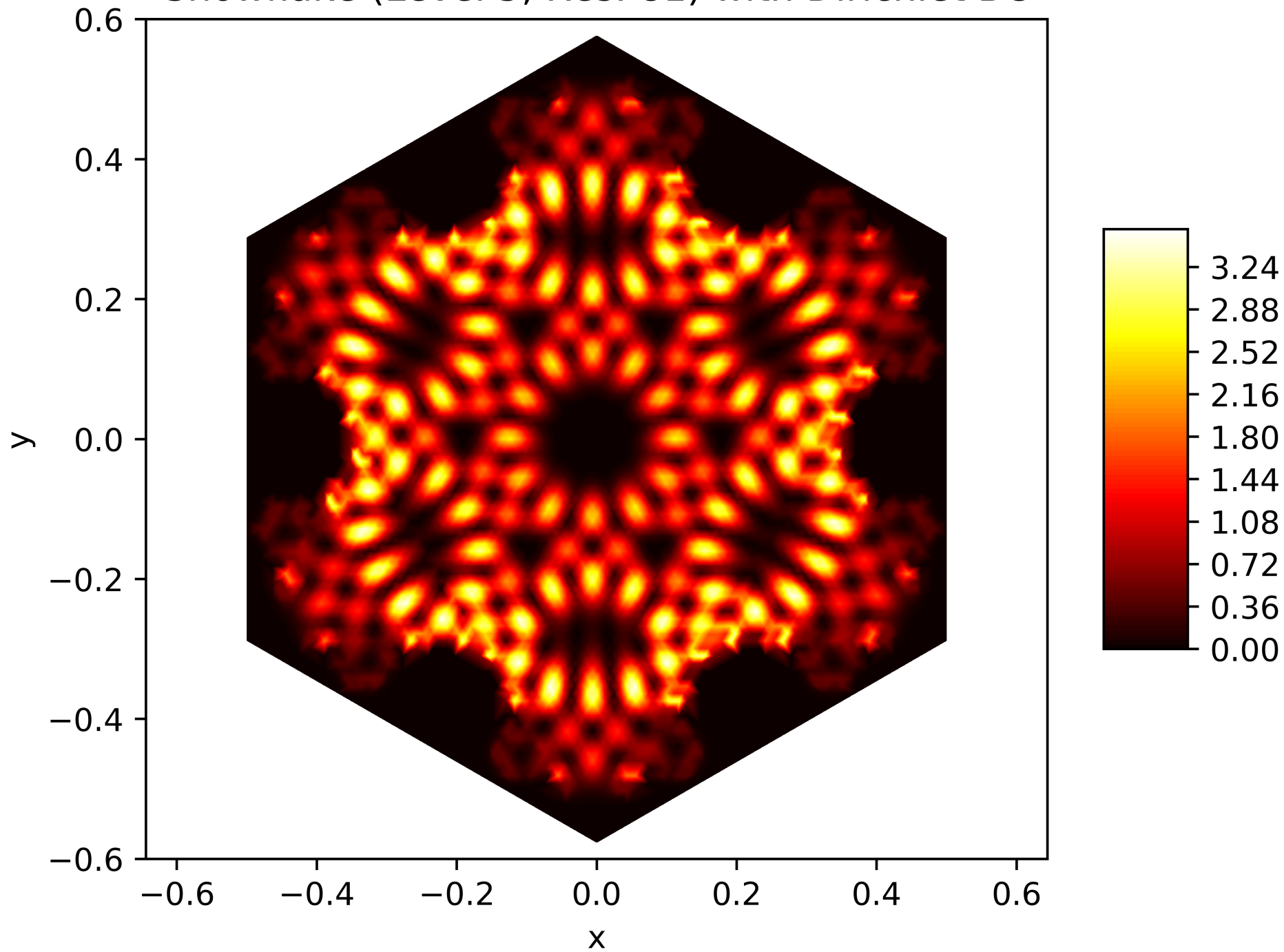
Energy Function of the 161. Eigenfunction on the Snowflake (Level 5, Res. 81) with Dirichlet BC
