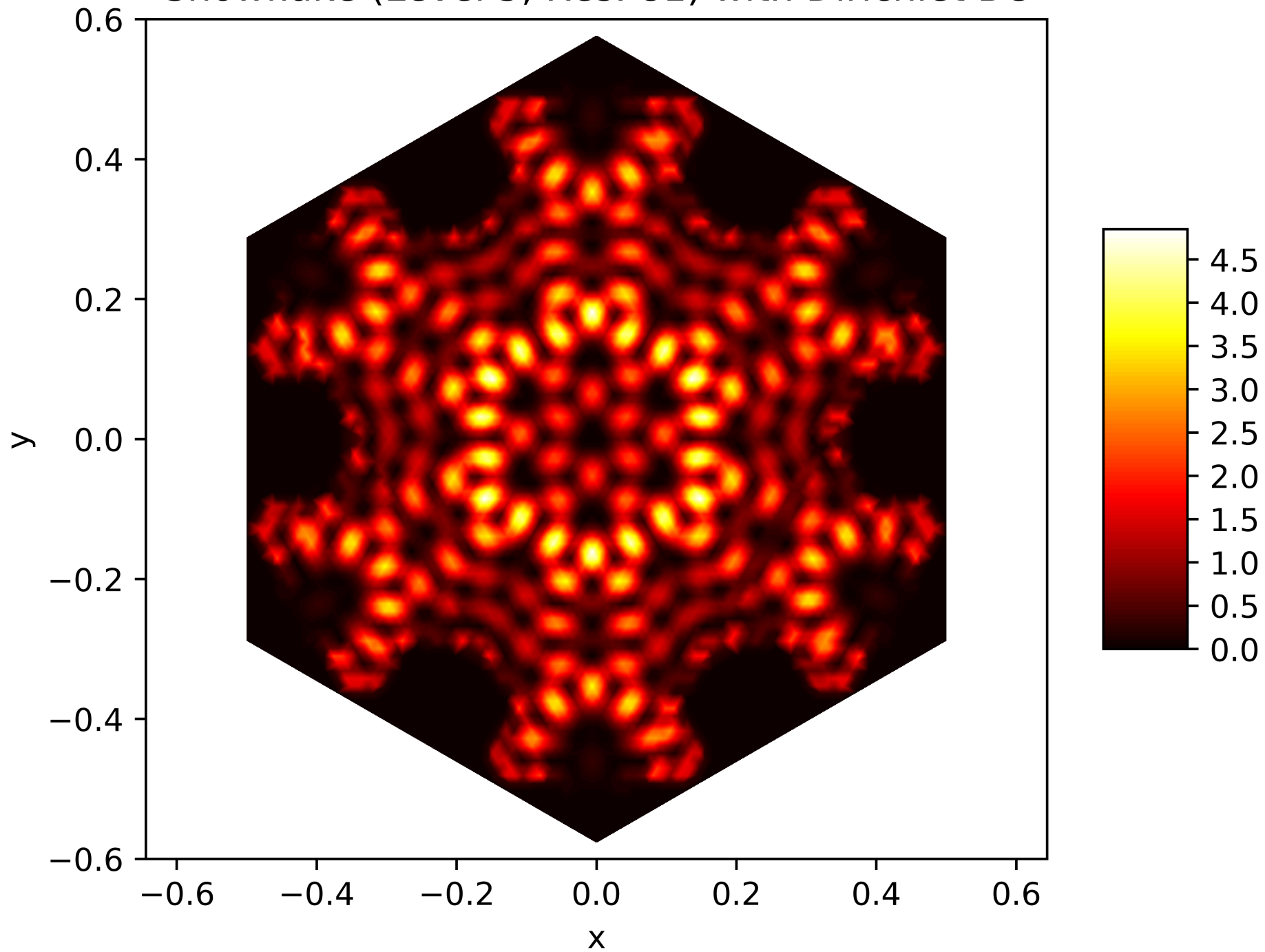
Energy Function of the 175. Eigenfunction on the Snowflake (Level 5, Res. 81) with Dirichlet BC
