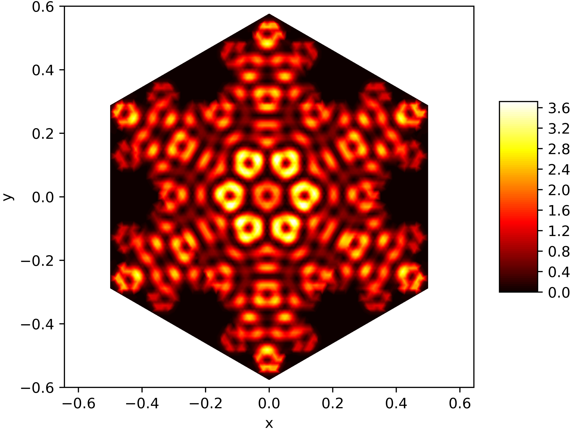
Energy Function of the 173. Eigenfunction on the Snowflake (Level 5, Res. 81) with Dirichlet BC
