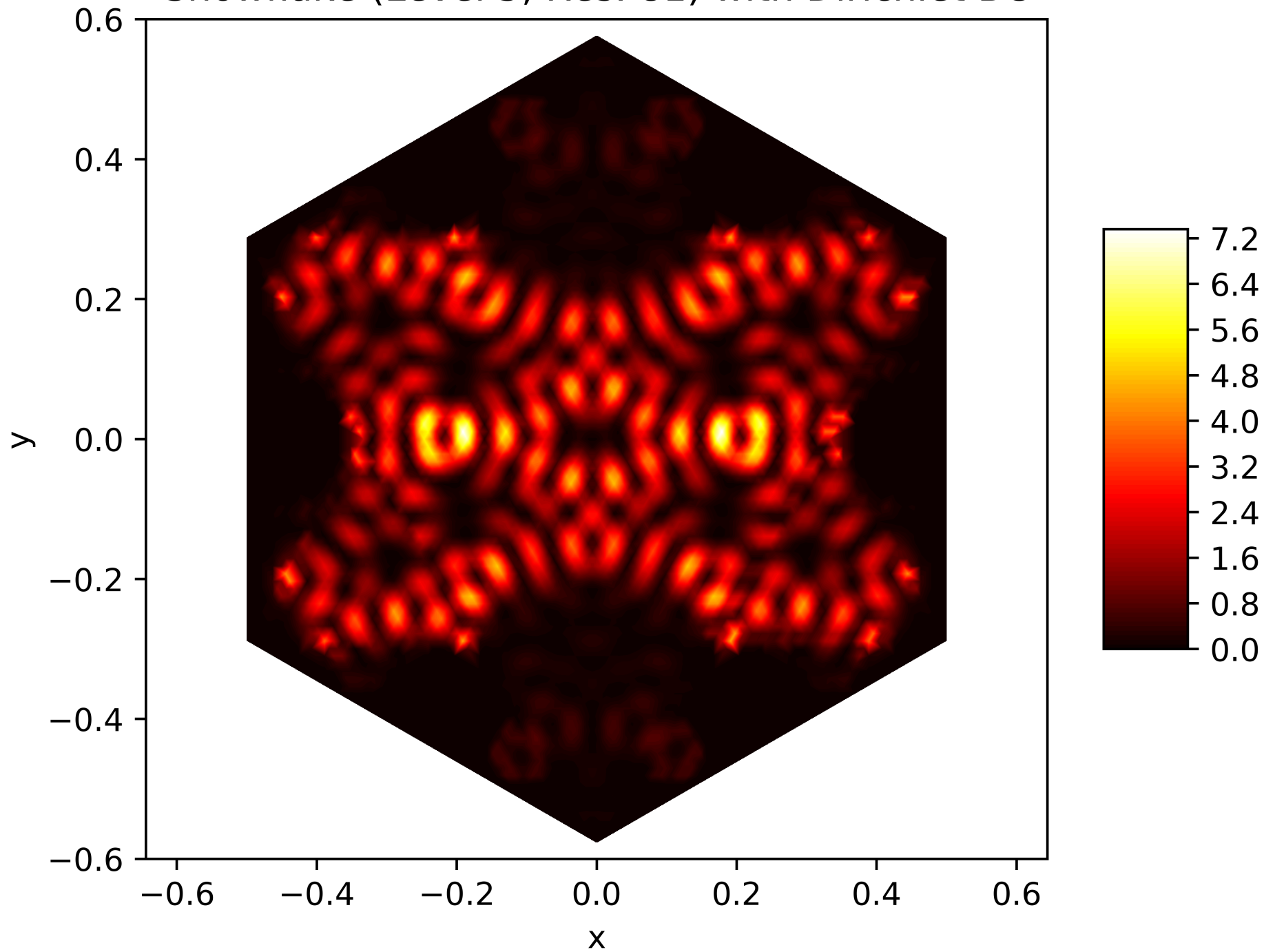
Energy Function of the 172. Eigenfunction on the Snowflake (Level 5, Res. 81) with Dirichlet BC
