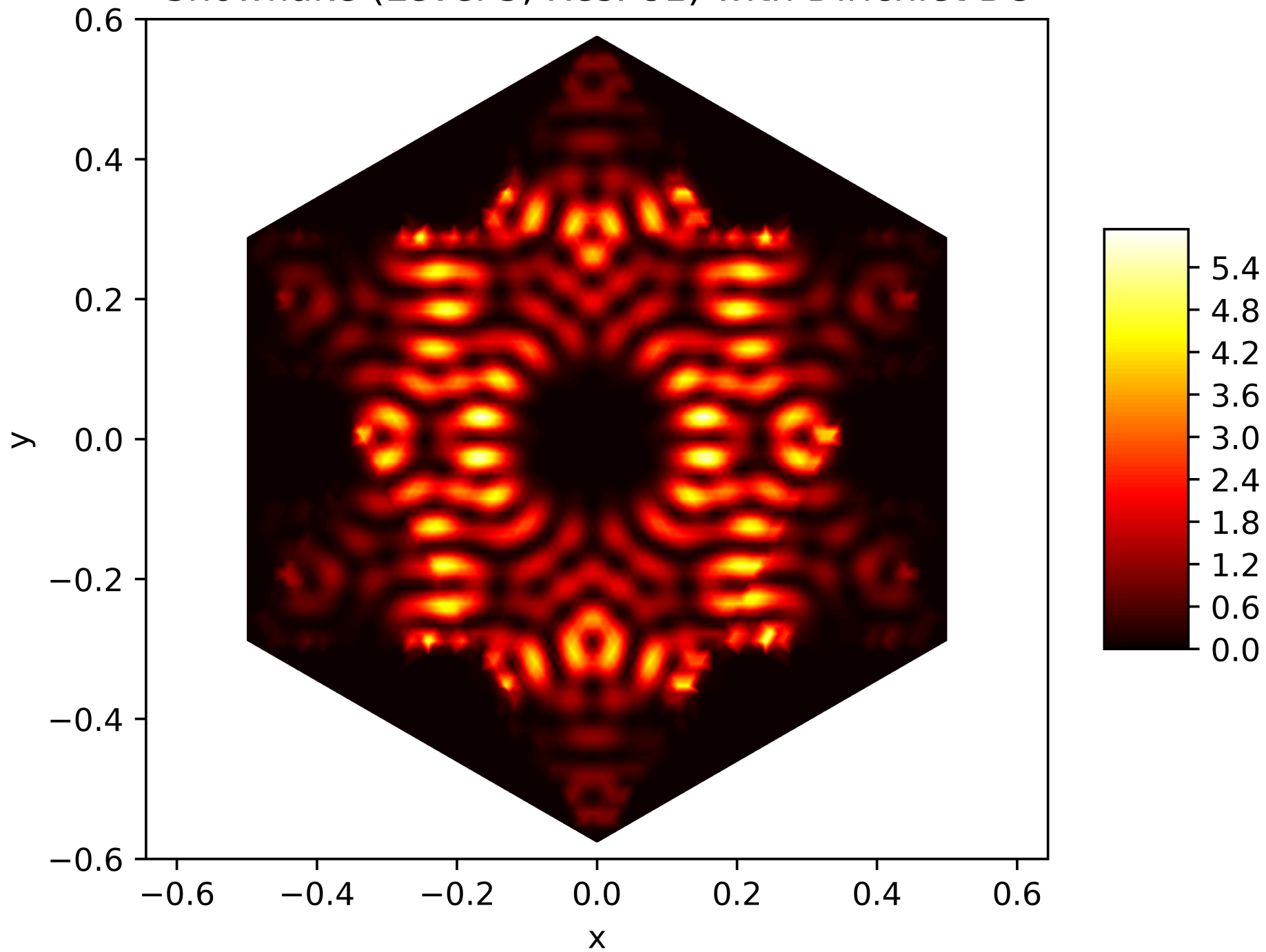
Energy Function of the 163. Eigenfunction on the Snowflake (Level 5, Res. 81) with Dirichlet BC
