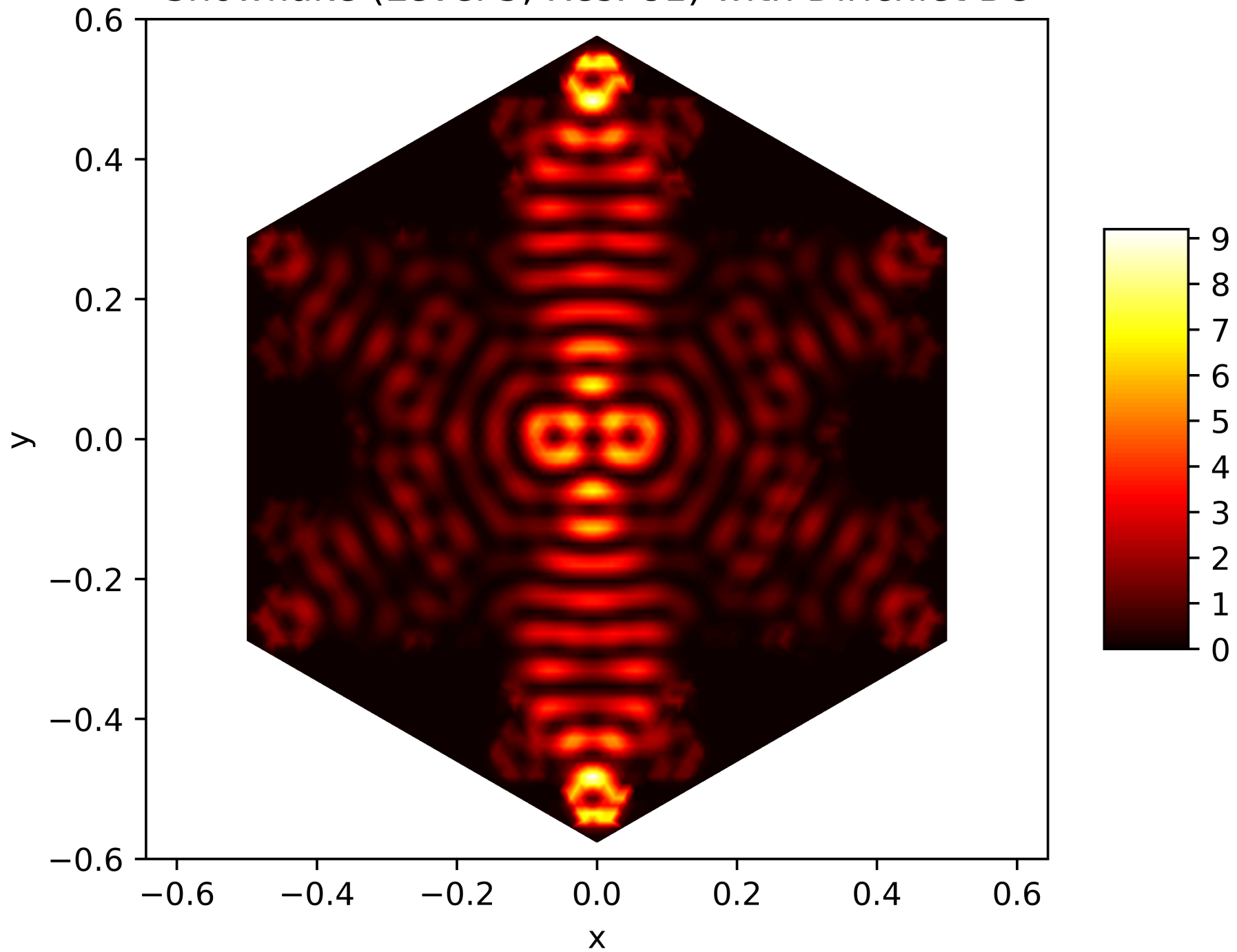
Energy Function of the 176. Eigenfunction on the Snowflake (Level 5, Res. 81) with Dirichlet BC
