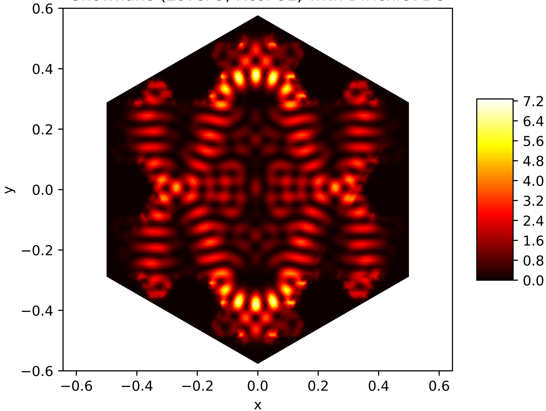
Energy Function of the 180. Eigenfunction on the Snowflake (Level 5, Res. 81) with Dirichlet BC
