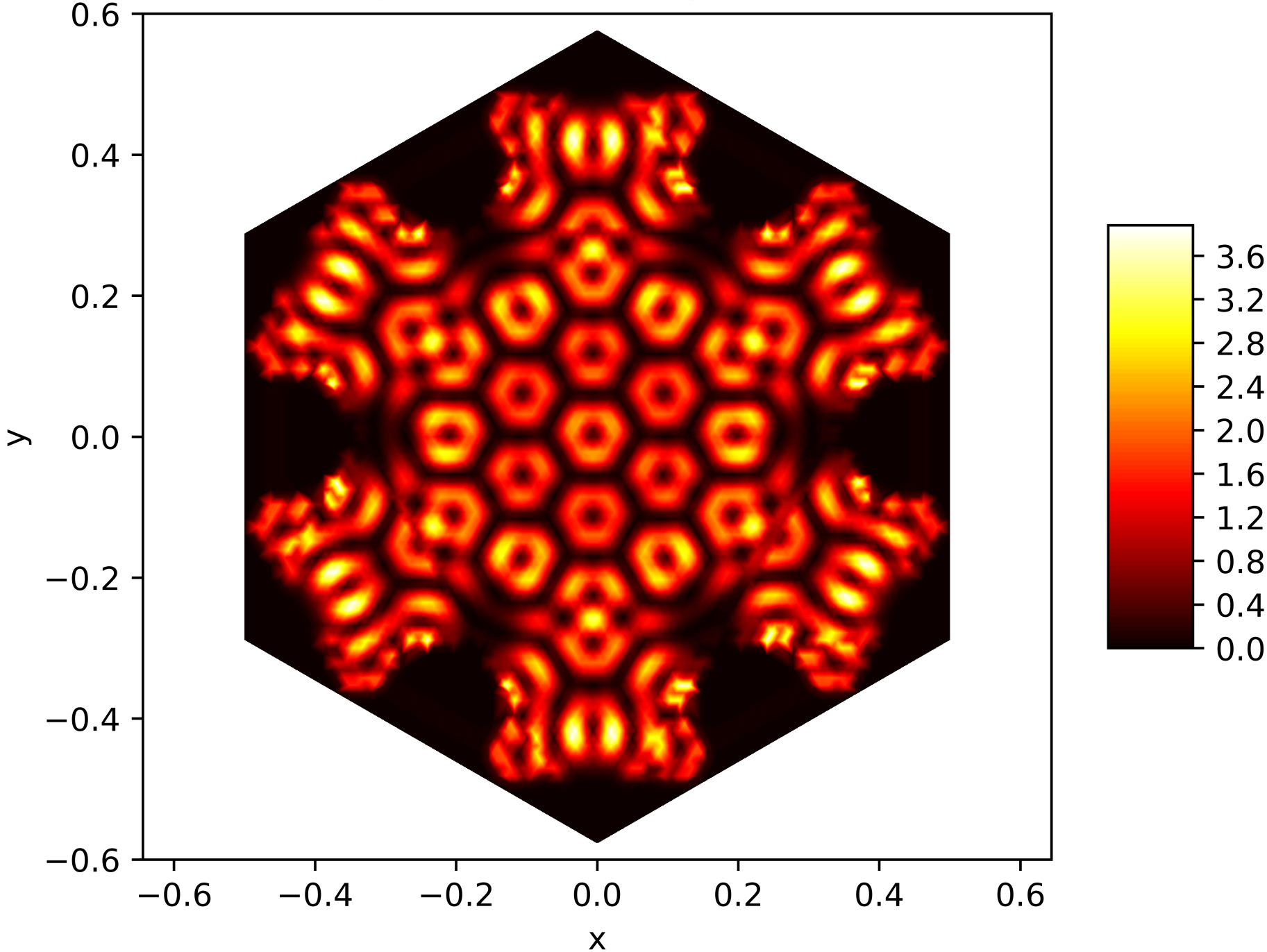
Energy Function of the 178. Eigenfunction on the Snowflake (Level 5, Res. 81) with Dirichlet BC
