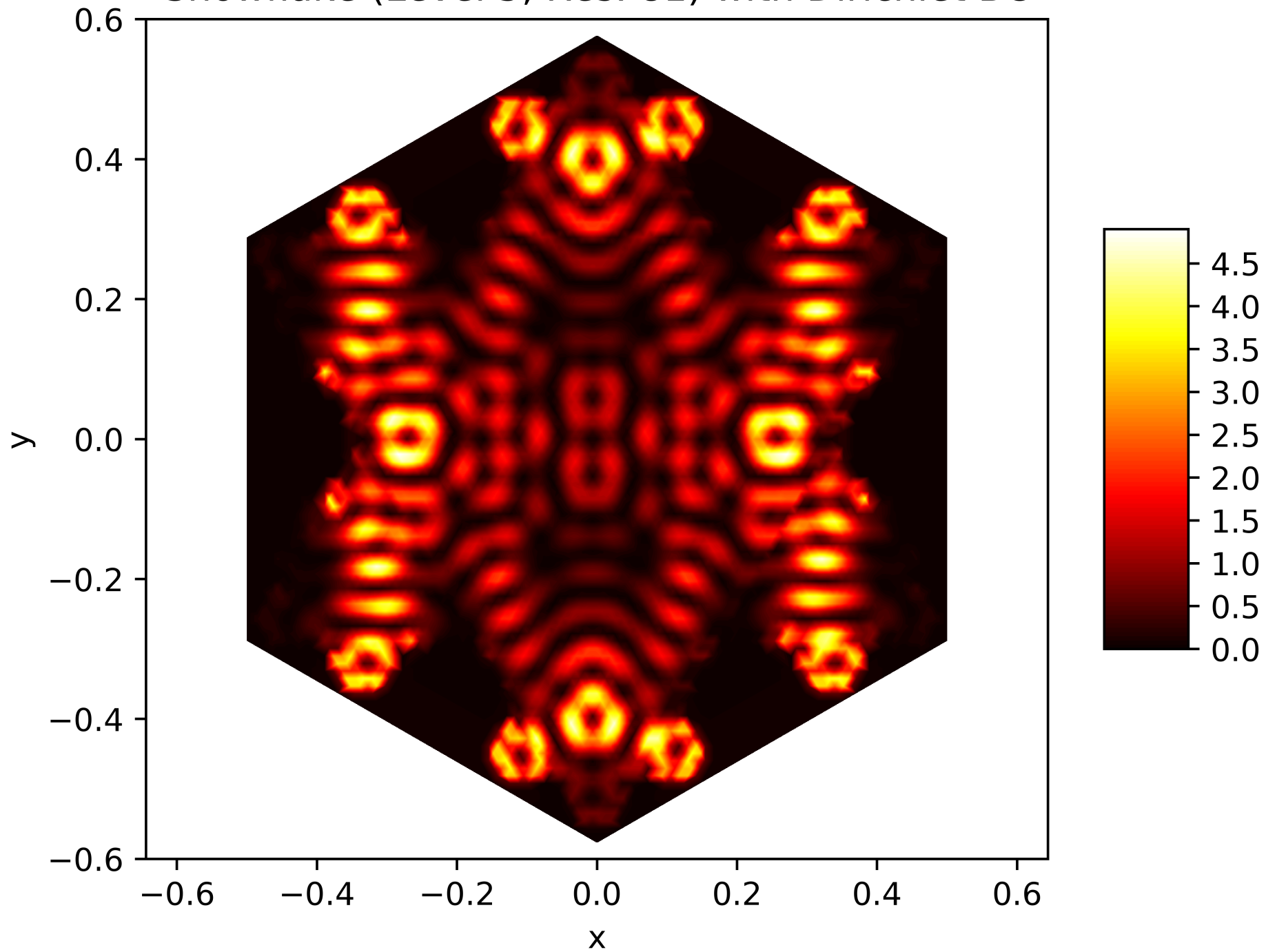
Energy Function of the 169. Eigenfunction on the Snowflake (Level 5, Res. 81) with Dirichlet BC
