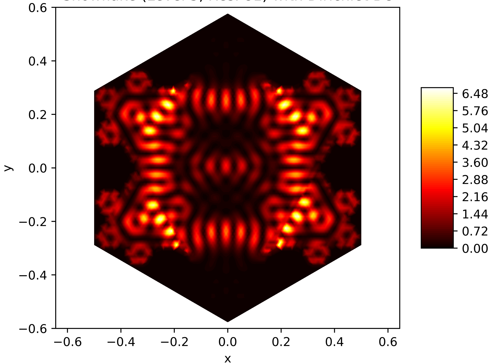
Energy Function of the 168. Eigenfunction on the Snowflake (Level 5, Res. 81) with Dirichlet BC
