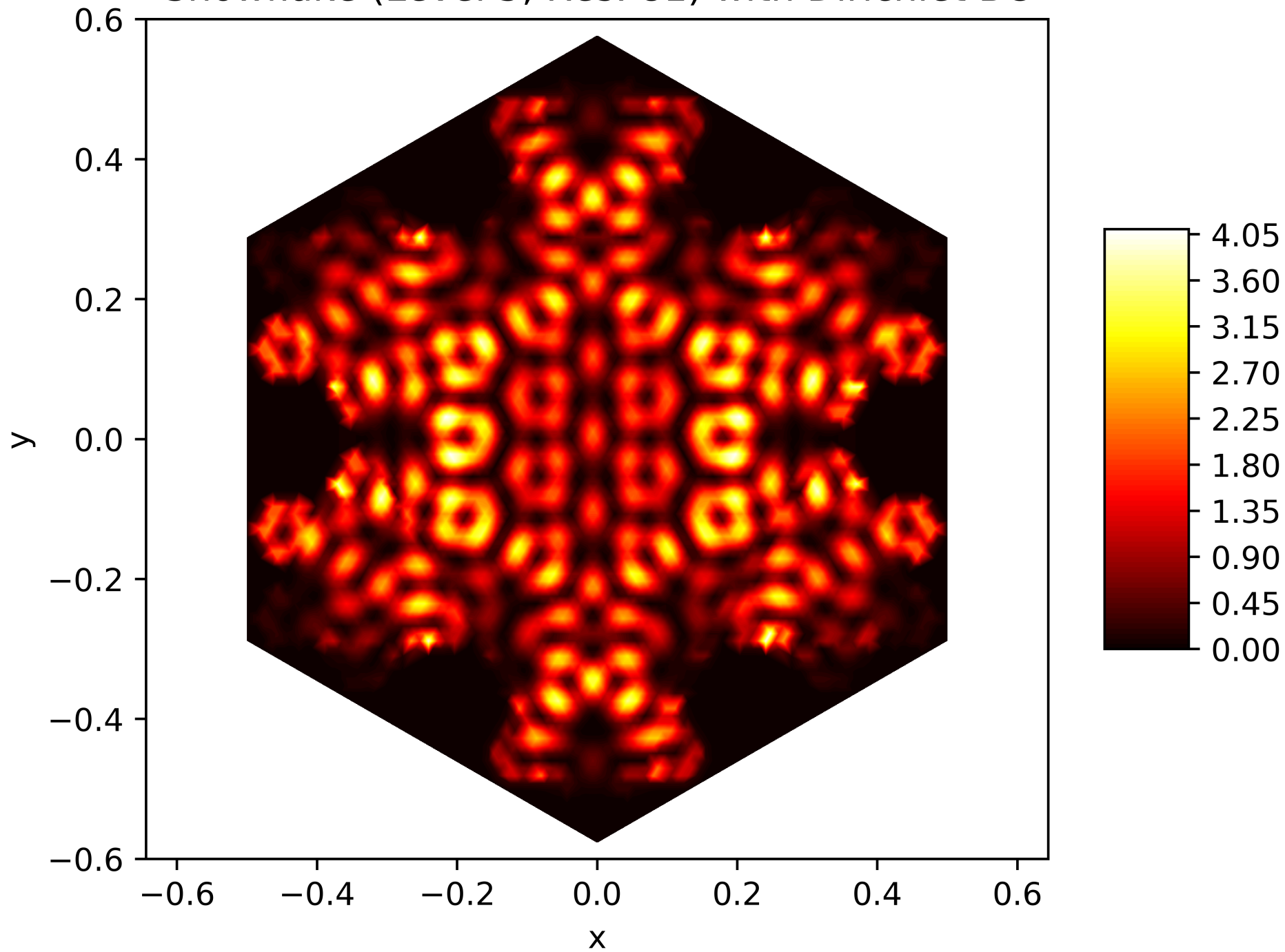
Energy Function of the 166. Eigenfunction on the Snowflake (Level 5, Res. 81) with Dirichlet BC
