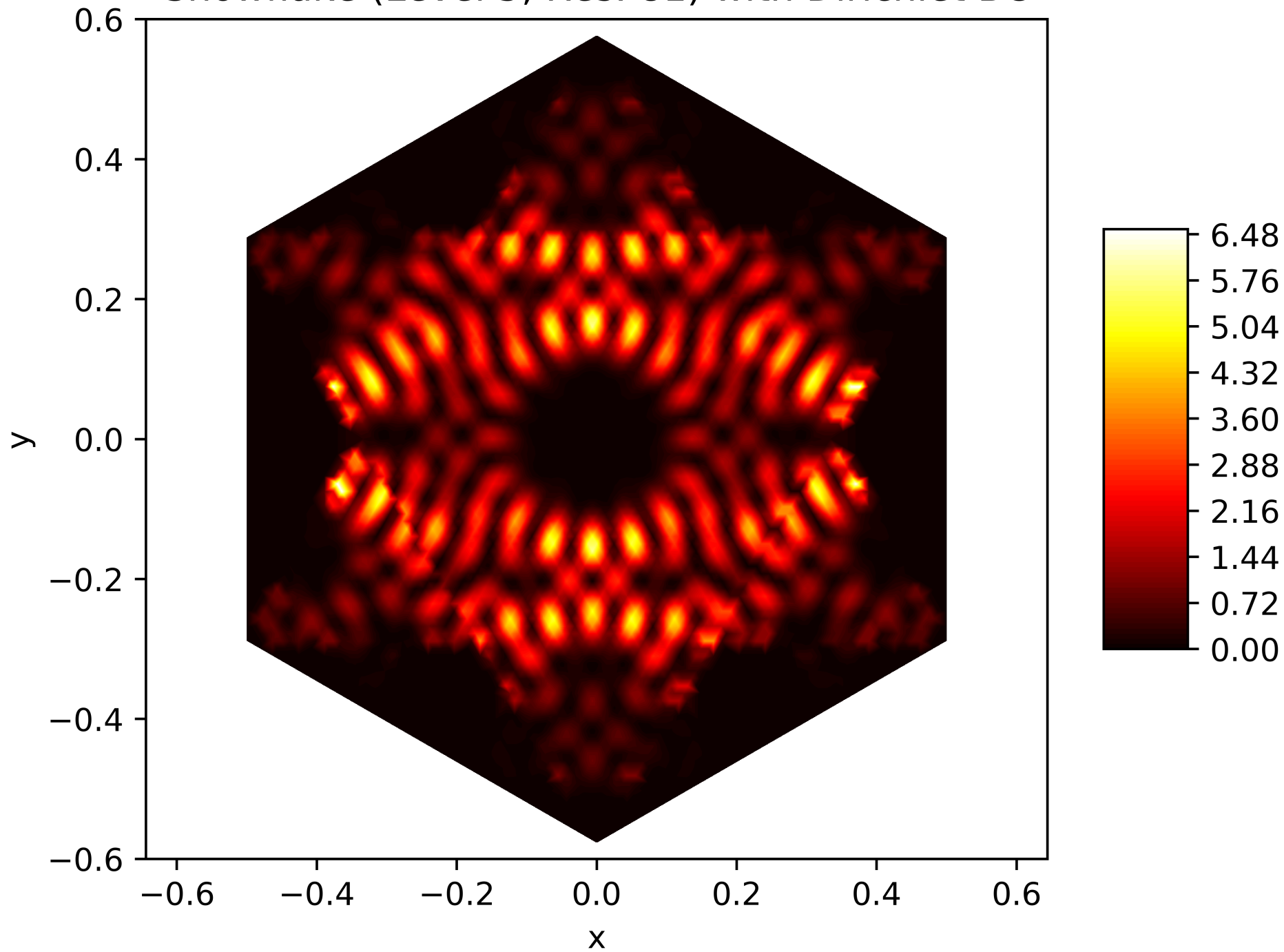
Energy Function of the 162. Eigenfunction on the Snowflake (Level 5, Res. 81) with Dirichlet BC
