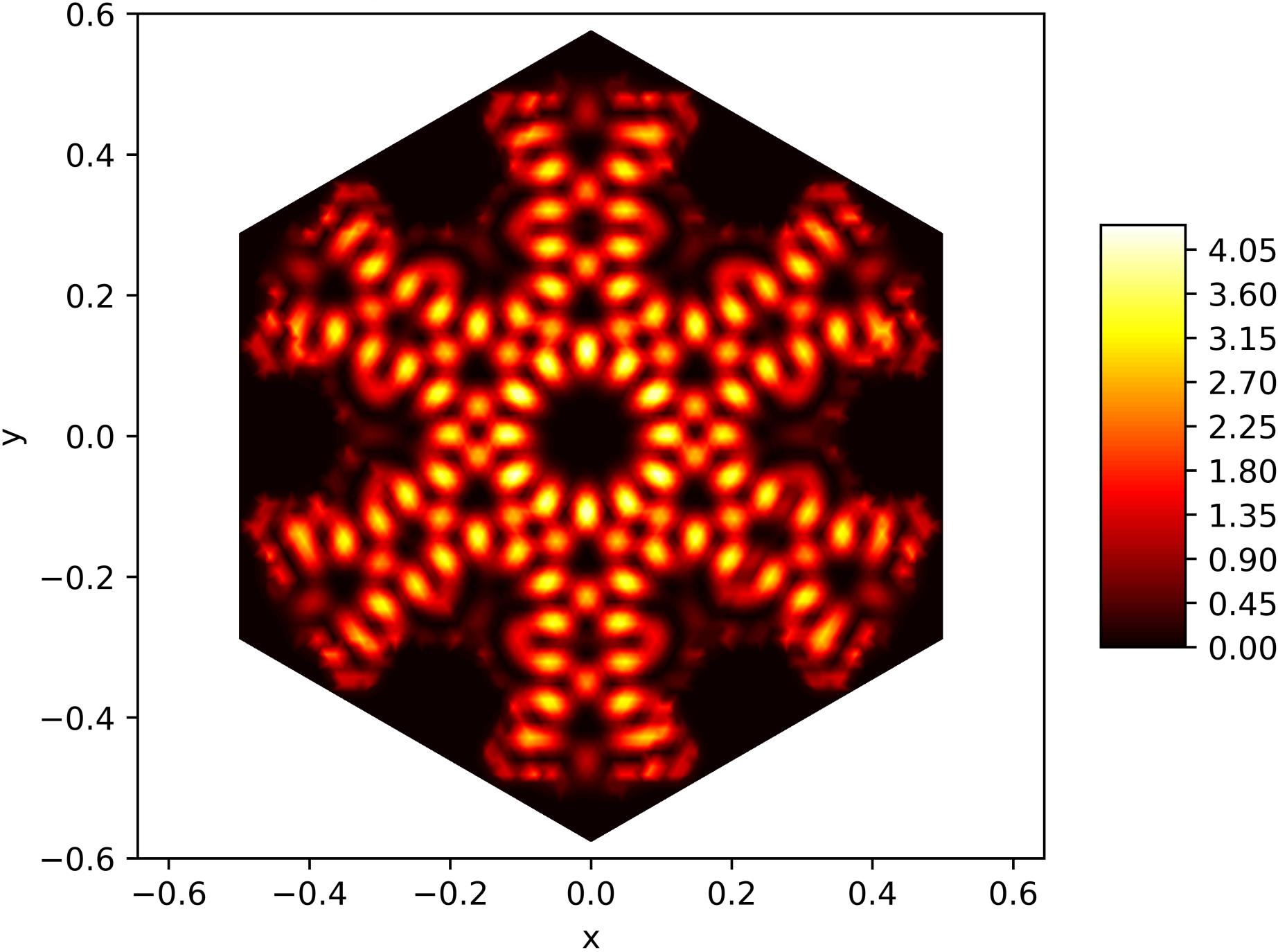
Energy Function of the 174. Eigenfunction on the Snowflake (Level 5, Res. 81) with Dirichlet BC
