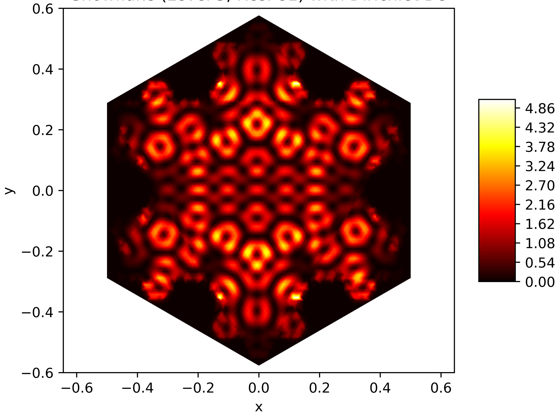
Energy Function of the 165. Eigenfunction on the Snowflake (Level 5, Res. 81) with Dirichlet BC
