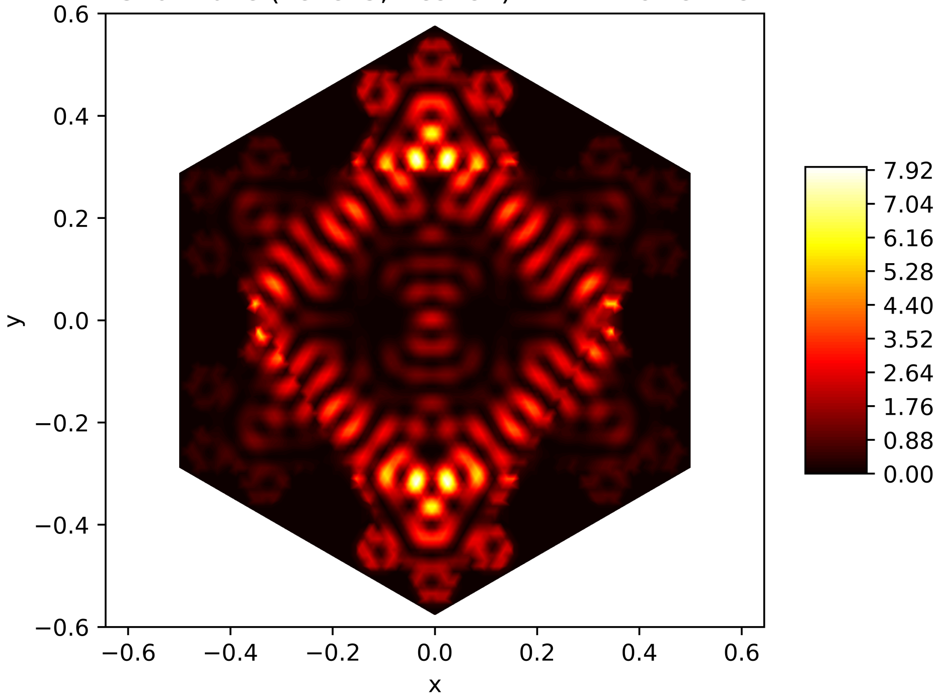
Energy Function of the 167. Eigenfunction on the Snowflake (Level 5, Res. 81) with Dirichlet BC
