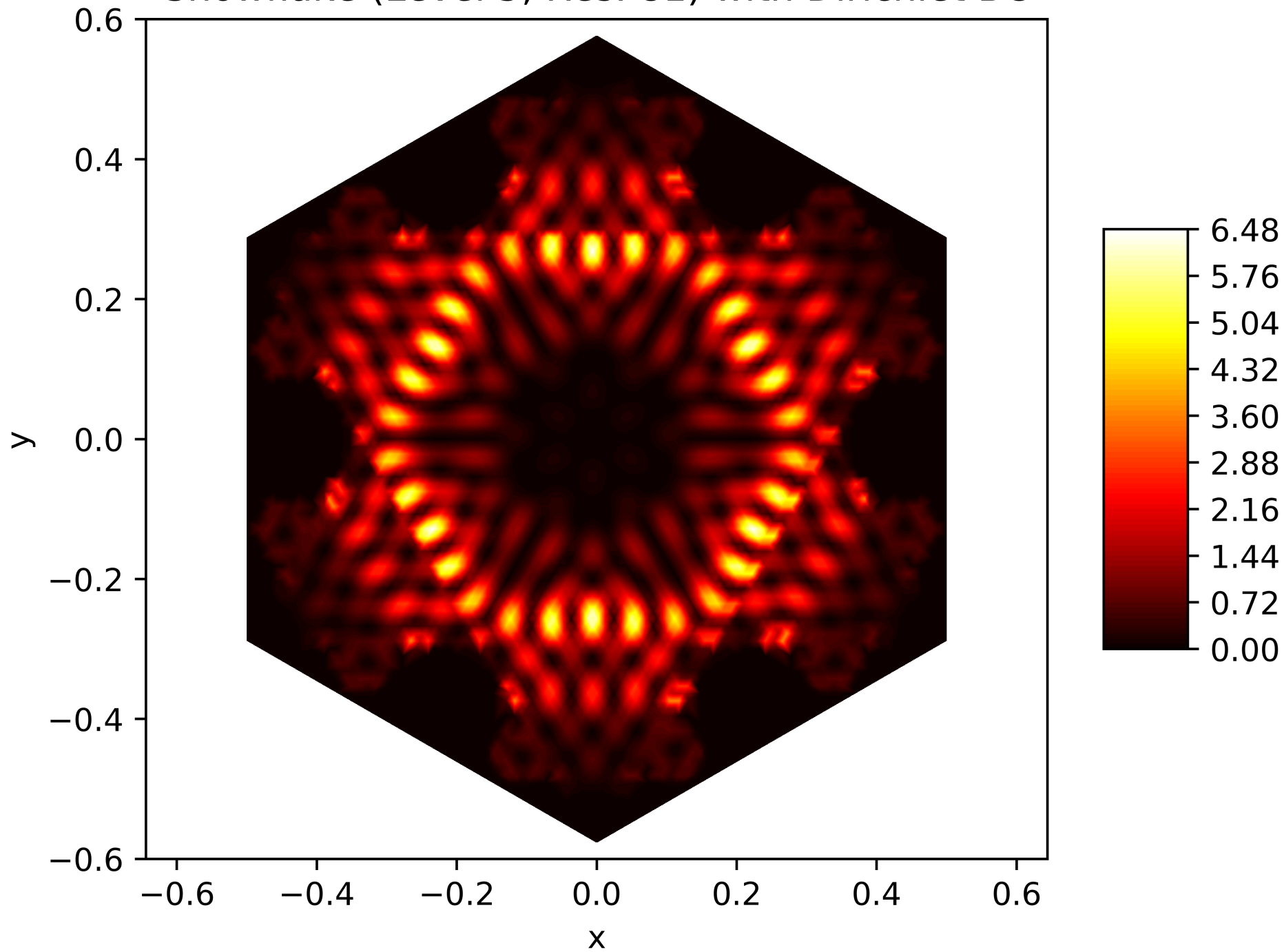
Energy Function of the 164. Eigenfunction on the Snowflake (Level 5, Res. 81) with Dirichlet BC
