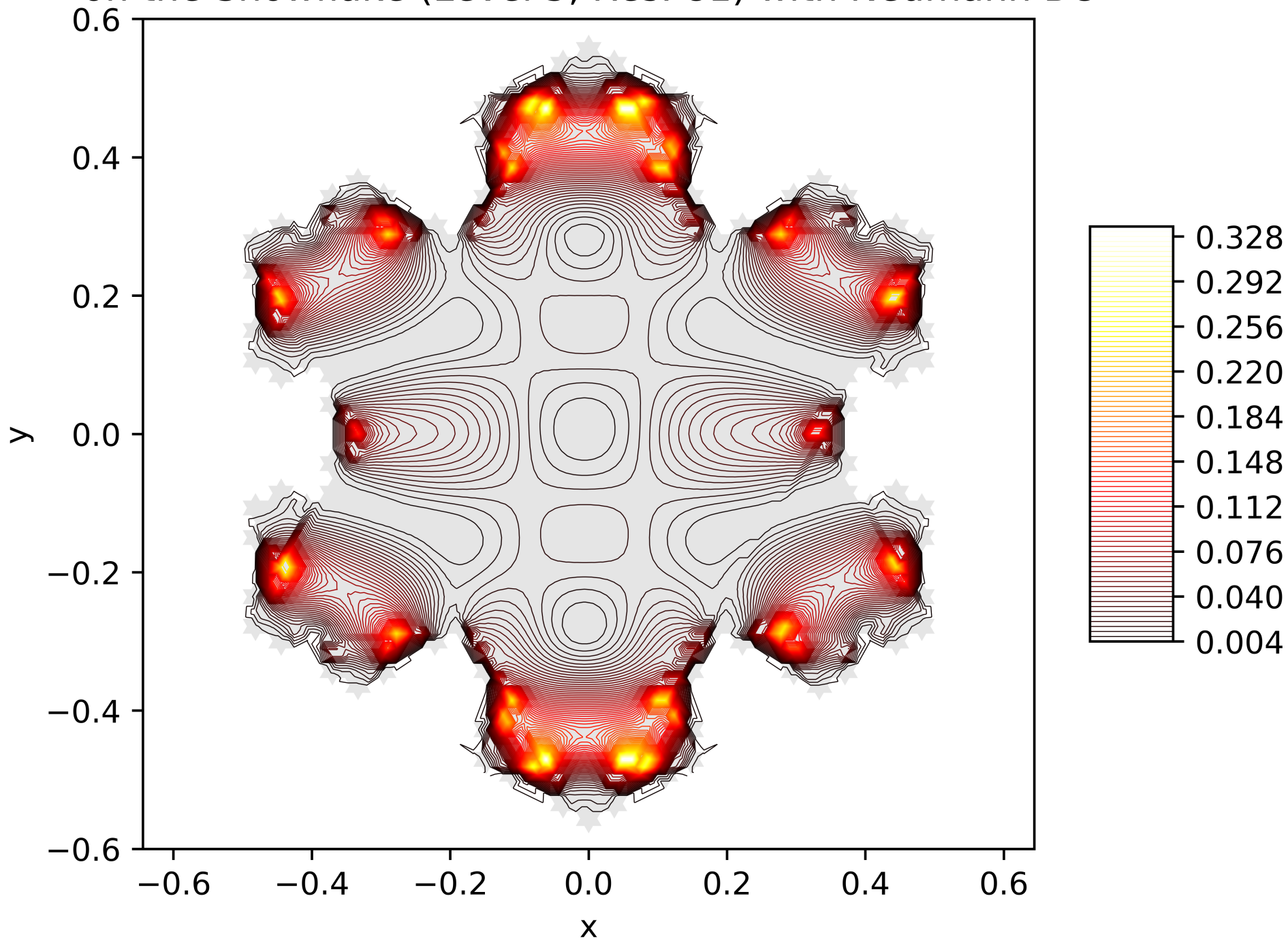
Contour Lines of the Energy Function of the 17. Eigenfunction on the Snowflake (Level 5, Res. 81) with Neumann BC
