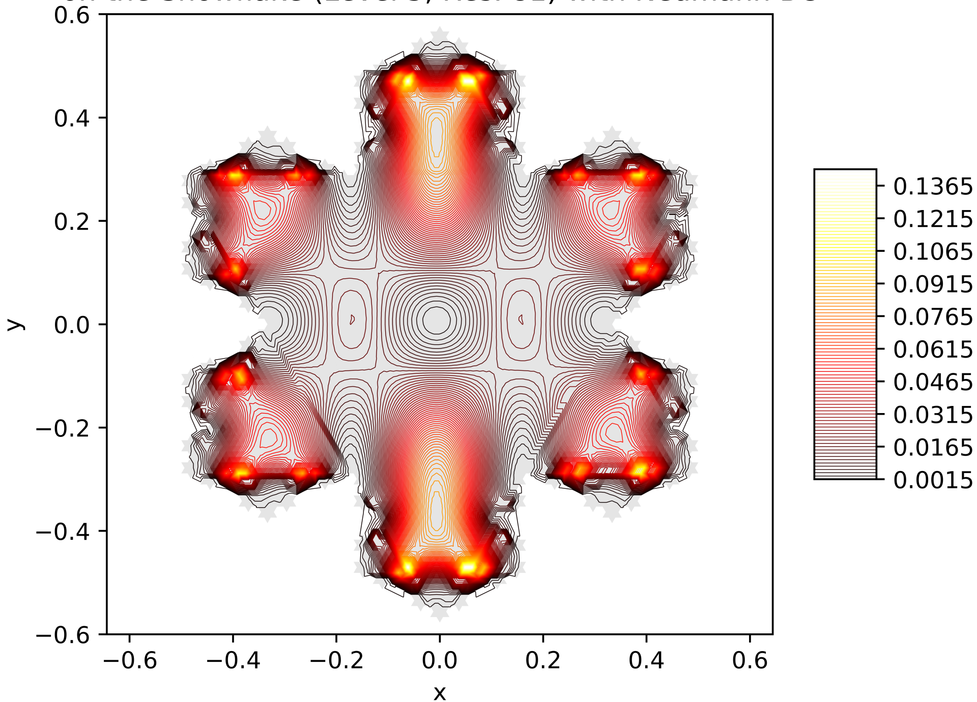
Contour Lines of the Energy Function of the 11. Eigenfunction on the Snowflake (Level 5, Res. 81) with Neumann BC
