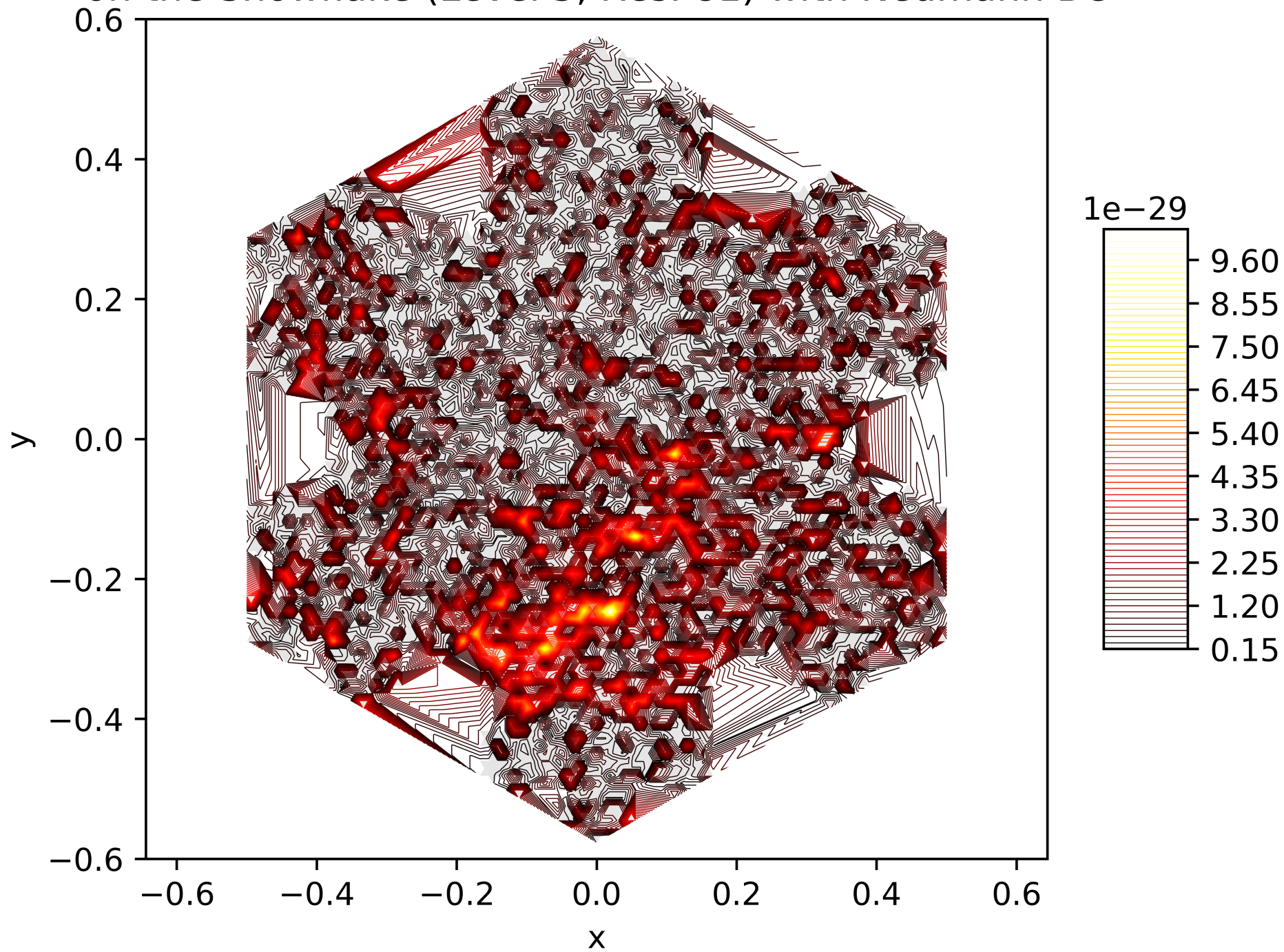
Contour Lines of the Energy Function of the 1. Eigenfunction on the Snowflake (Level 5, Res. 81) with Neumann BC
