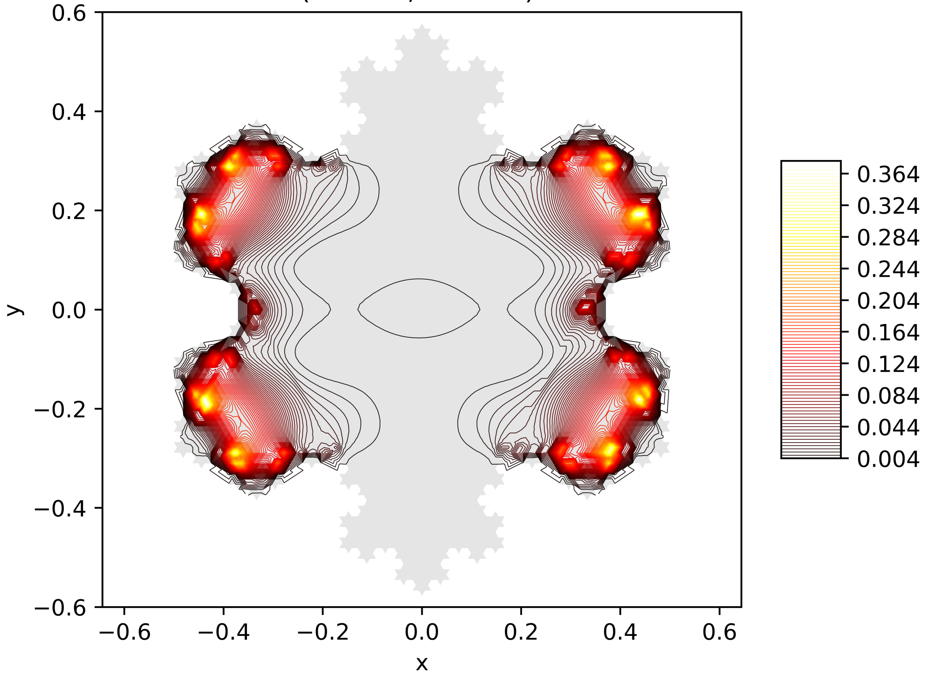
Contour Lines of the Energy Function of the 14. Eigenfunction on the Snowflake (Level 5, Res. 81) with Neumann BC
