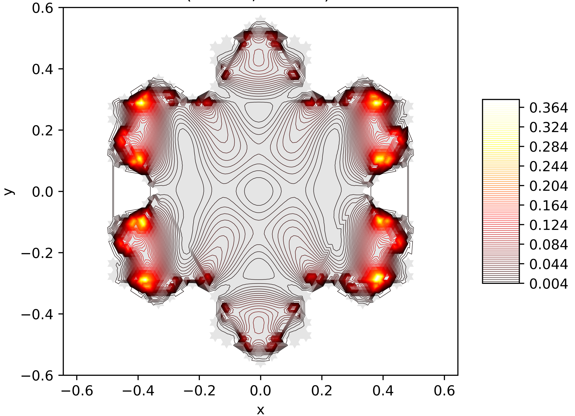
Contour Lines of the Energy Function of the 18. Eigenfunction on the Snowflake (Level 5, Res. 81) with Neumann BC
