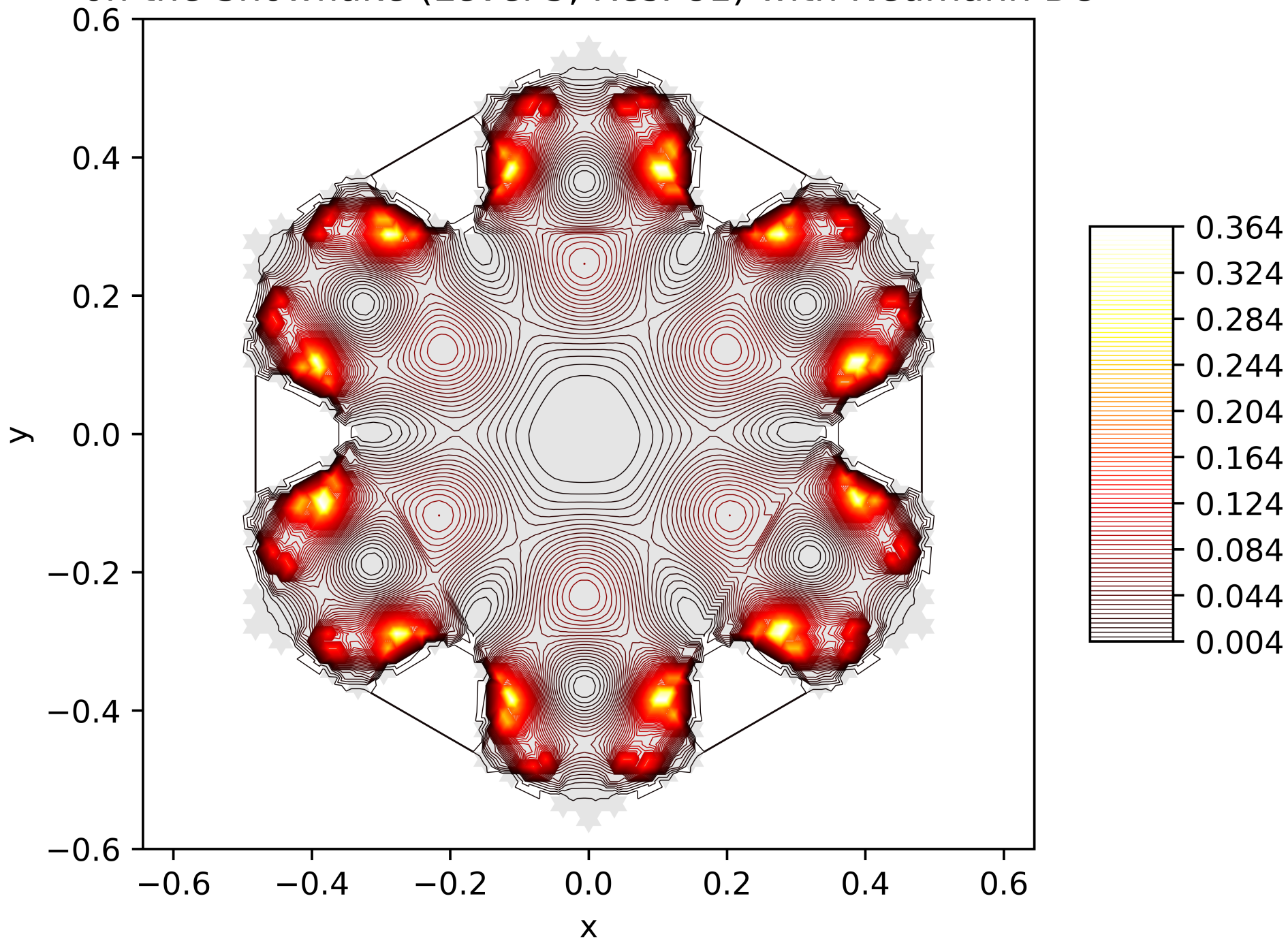
Contour Lines of the Energy Function of the 20. Eigenfunction on the Snowflake (Level 5, Res. 81) with Neumann BC
