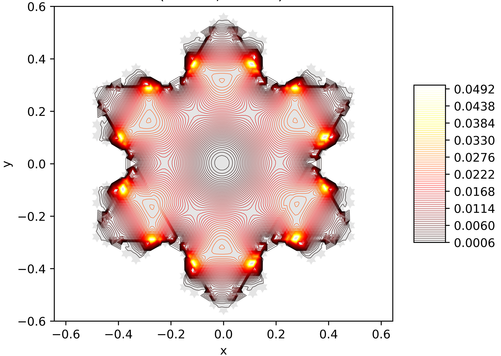
Contour Lines of the Energy Function of the 7. Eigenfunction on the Snowflake (Level 5, Res. 81) with Neumann BC
