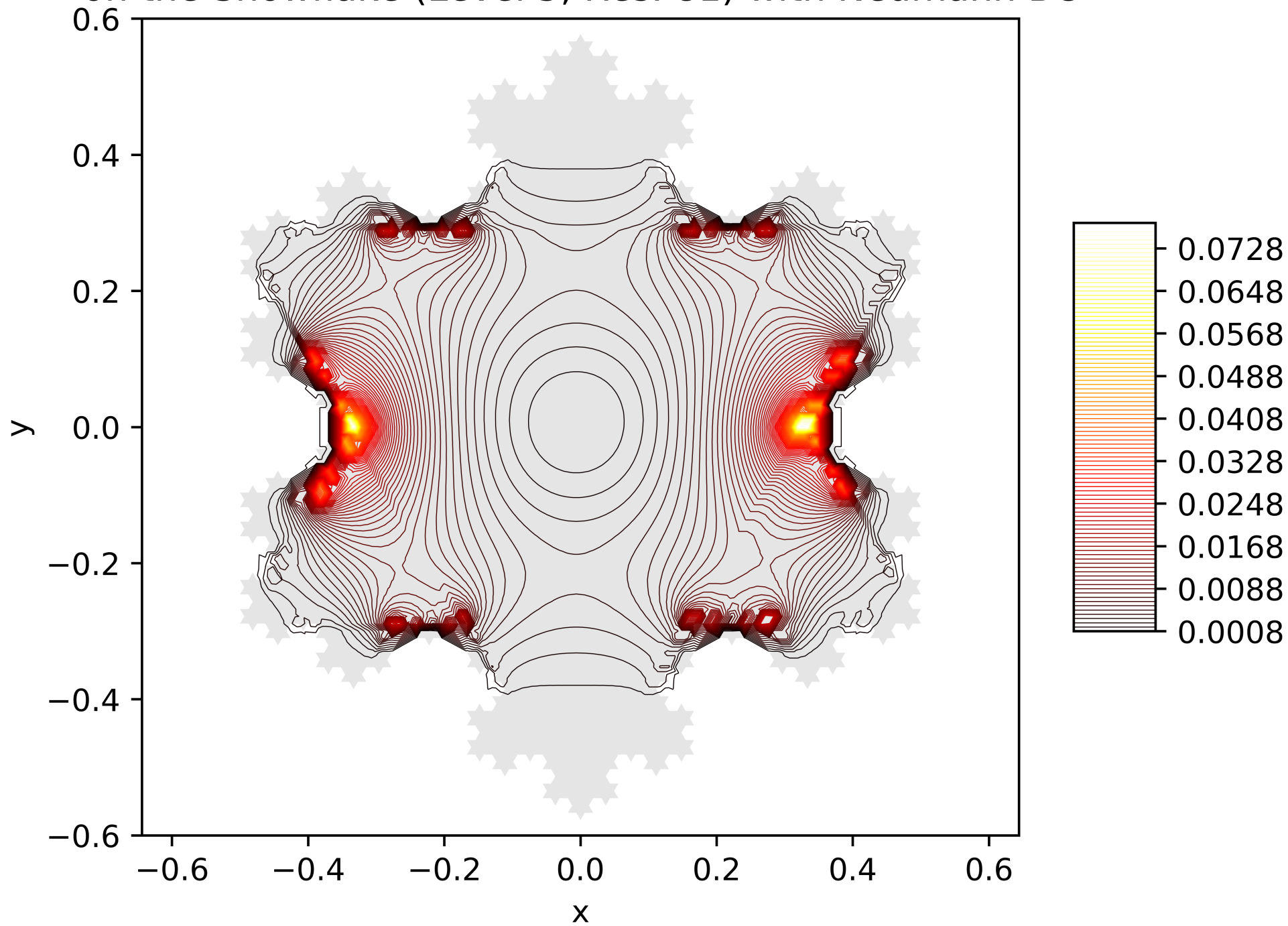
Contour Lines of the Energy Function of the 5. Eigenfunction on the Snowflake (Level 5, Res. 81) with Neumann BC
