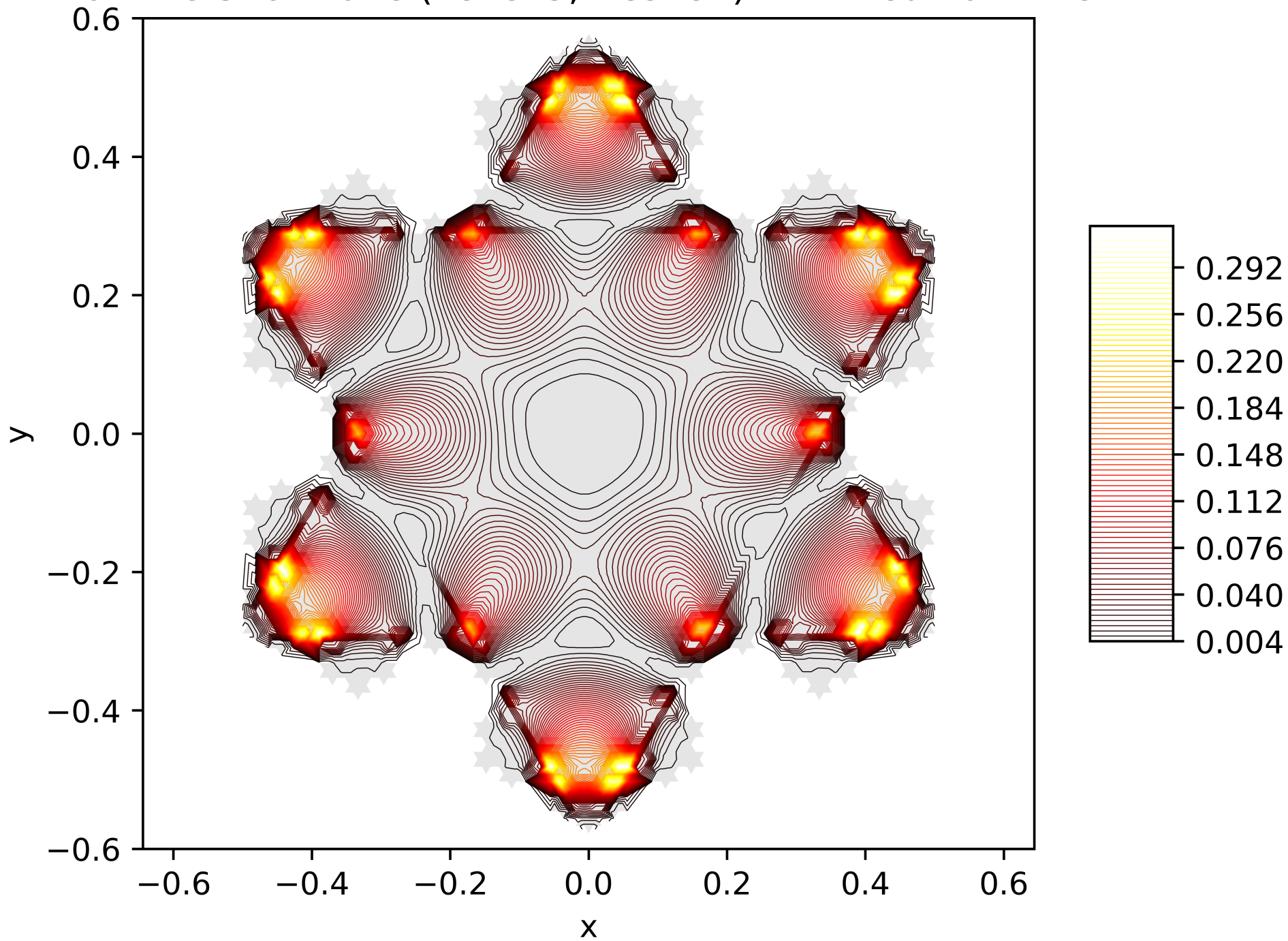
Contour Lines of the Energy Function of the 19. Eigenfunction on the Snowflake (Level 5, Res. 81) with Neumann BC
