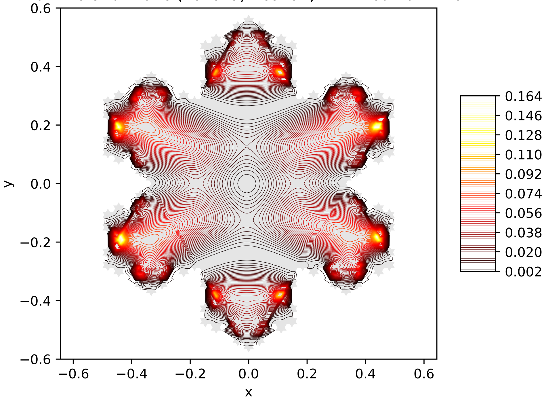
Contour Lines of the Energy Function of the 10. Eigenfunction on the Snowflake (Level 5, Res. 81) with Neumann BC
