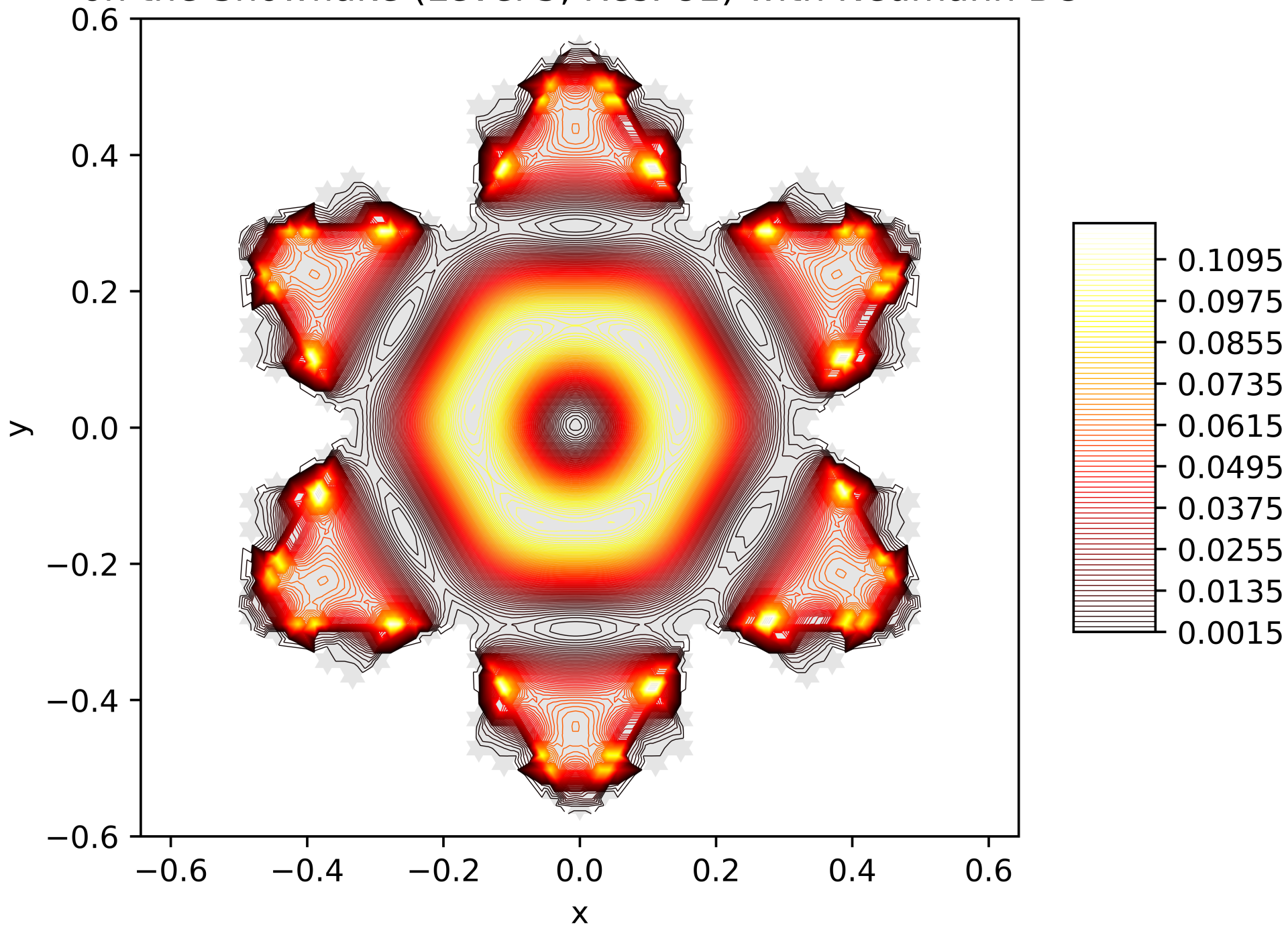
Contour Lines of the Energy Function of the 16. Eigenfunction on the Snowflake (Level 5, Res. 81) with Neumann BC
