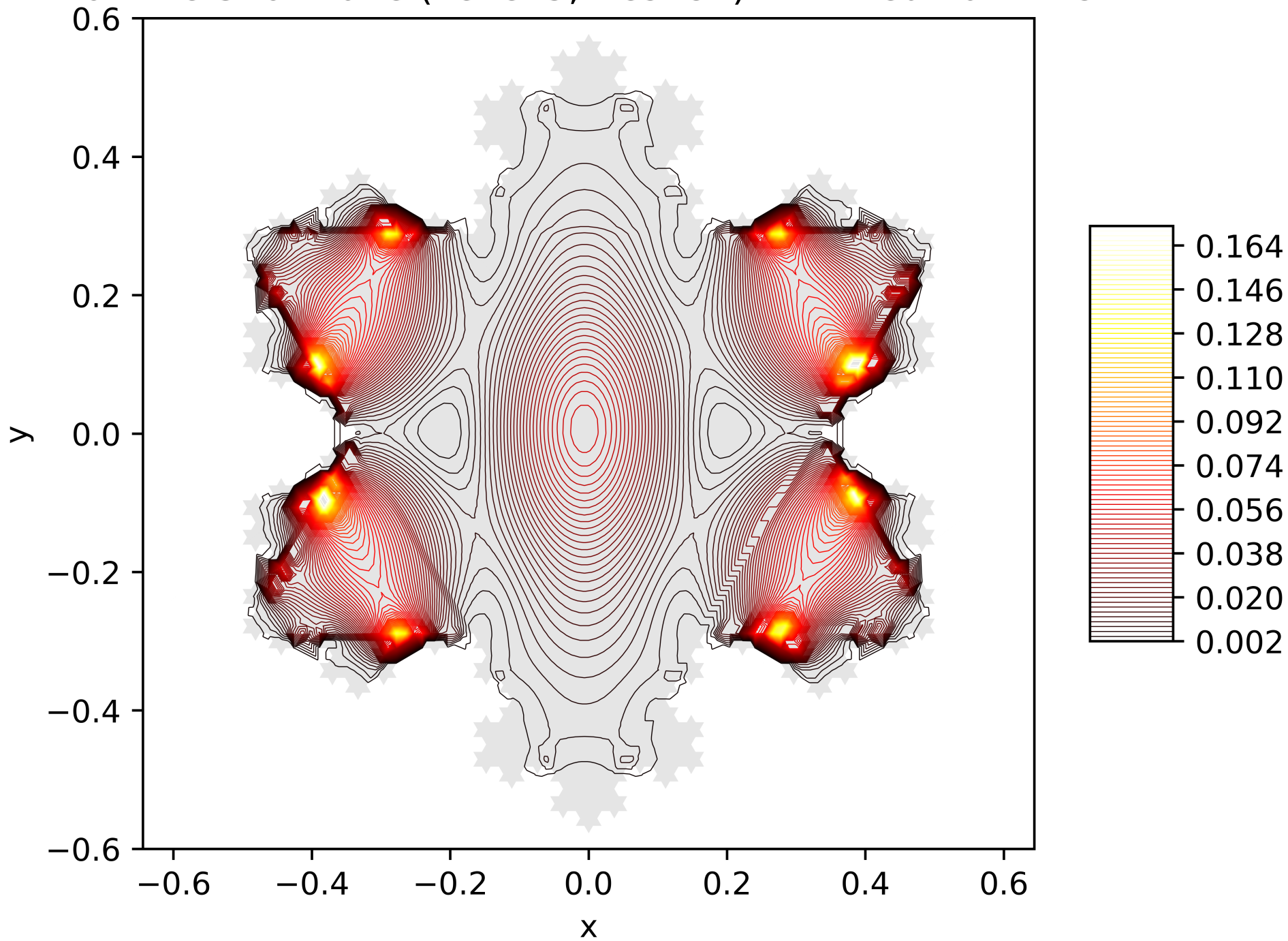
Contour Lines of the Energy Function of the 9. Eigenfunction on the Snowflake (Level 5, Res. 81) with Neumann BC
