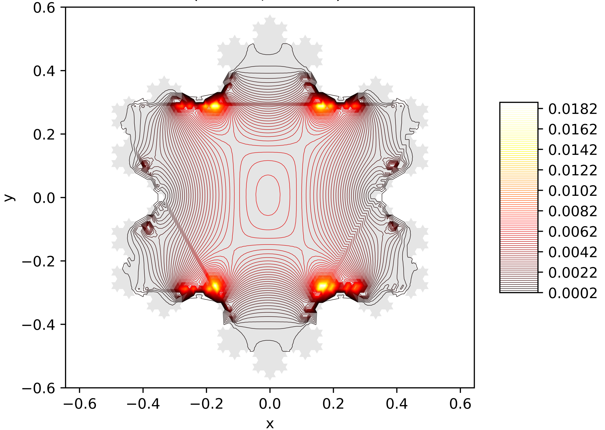
Contour Lines of the Energy Function of the 3. Eigenfunction on the Snowflake (Level 5, Res. 81) with Neumann BC
