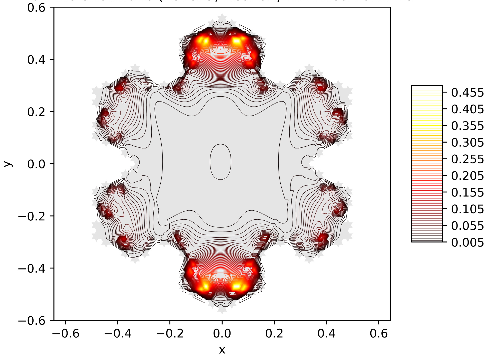
Contour Lines of the Energy Function of the 13. Eigenfunction on the Snowflake (Level 5, Res. 81) with Neumann BC
