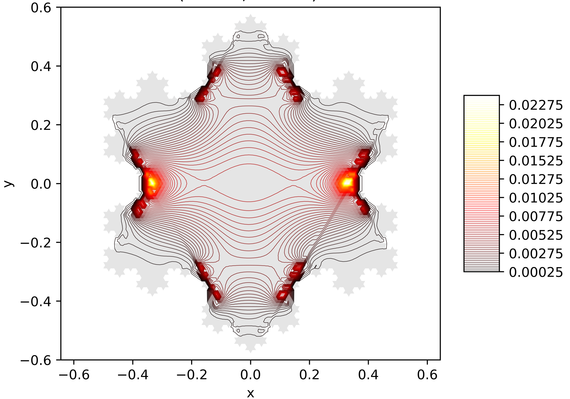
Contour Lines of the Energy Function of the 2. Eigenfunction on the Snowflake (Level 5, Res. 81) with Neumann BC
