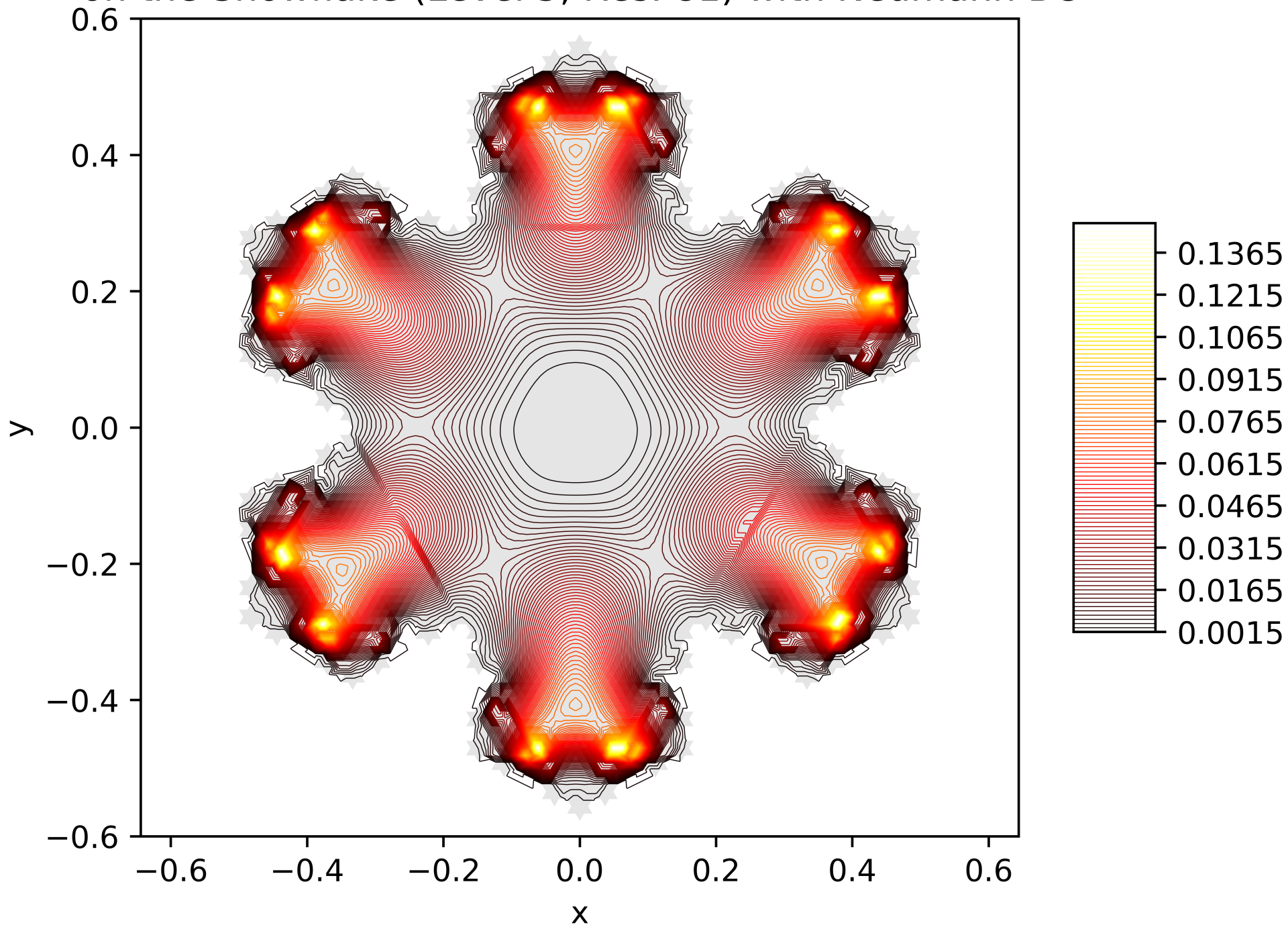
Contour Lines of the Energy Function of the 12. Eigenfunction on the Snowflake (Level 5, Res. 81) with Neumann BC
