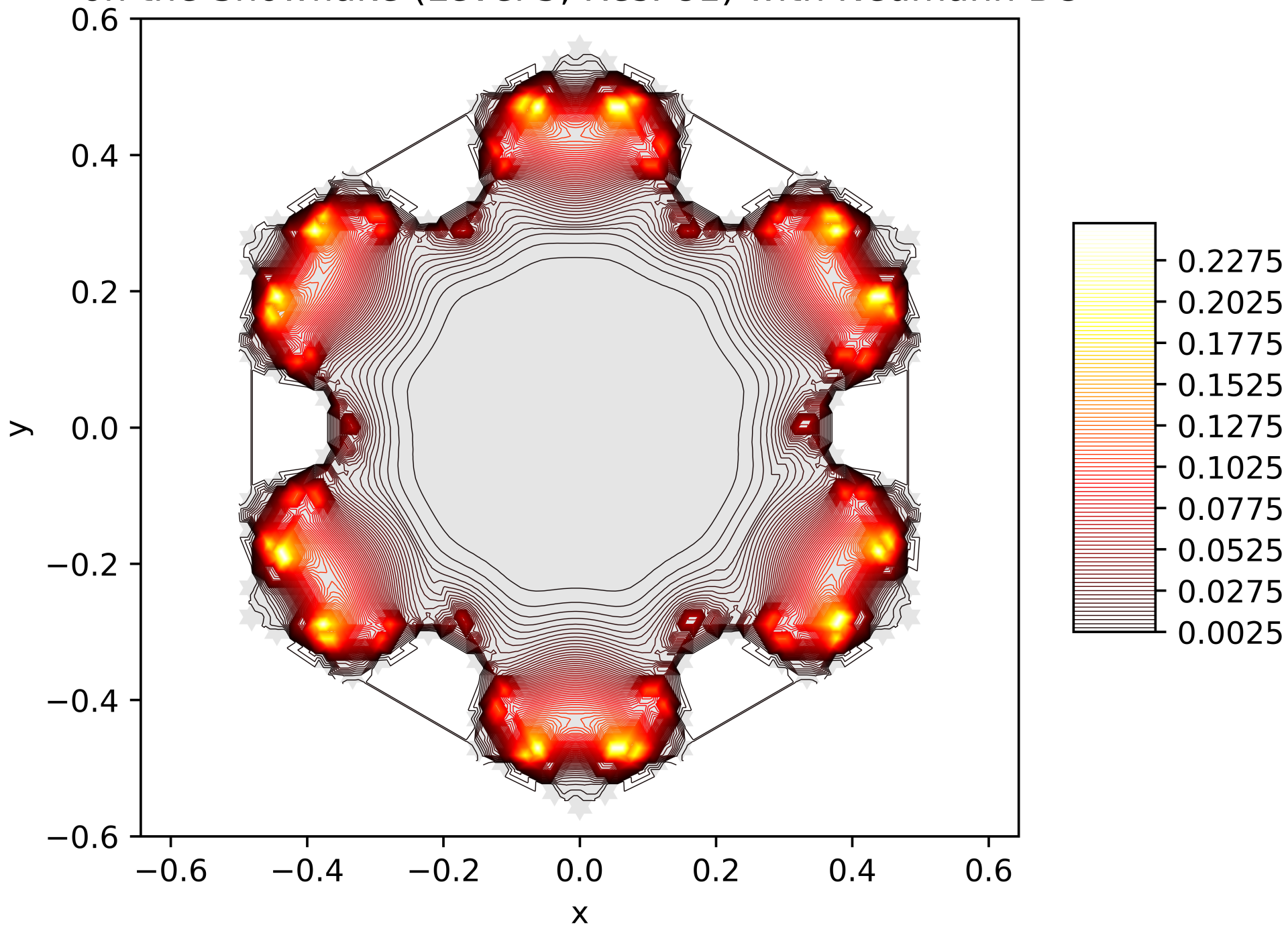
Contour Lines of the Energy Function of the 15. Eigenfunction on the Snowflake (Level 5, Res. 81) with Neumann BC
