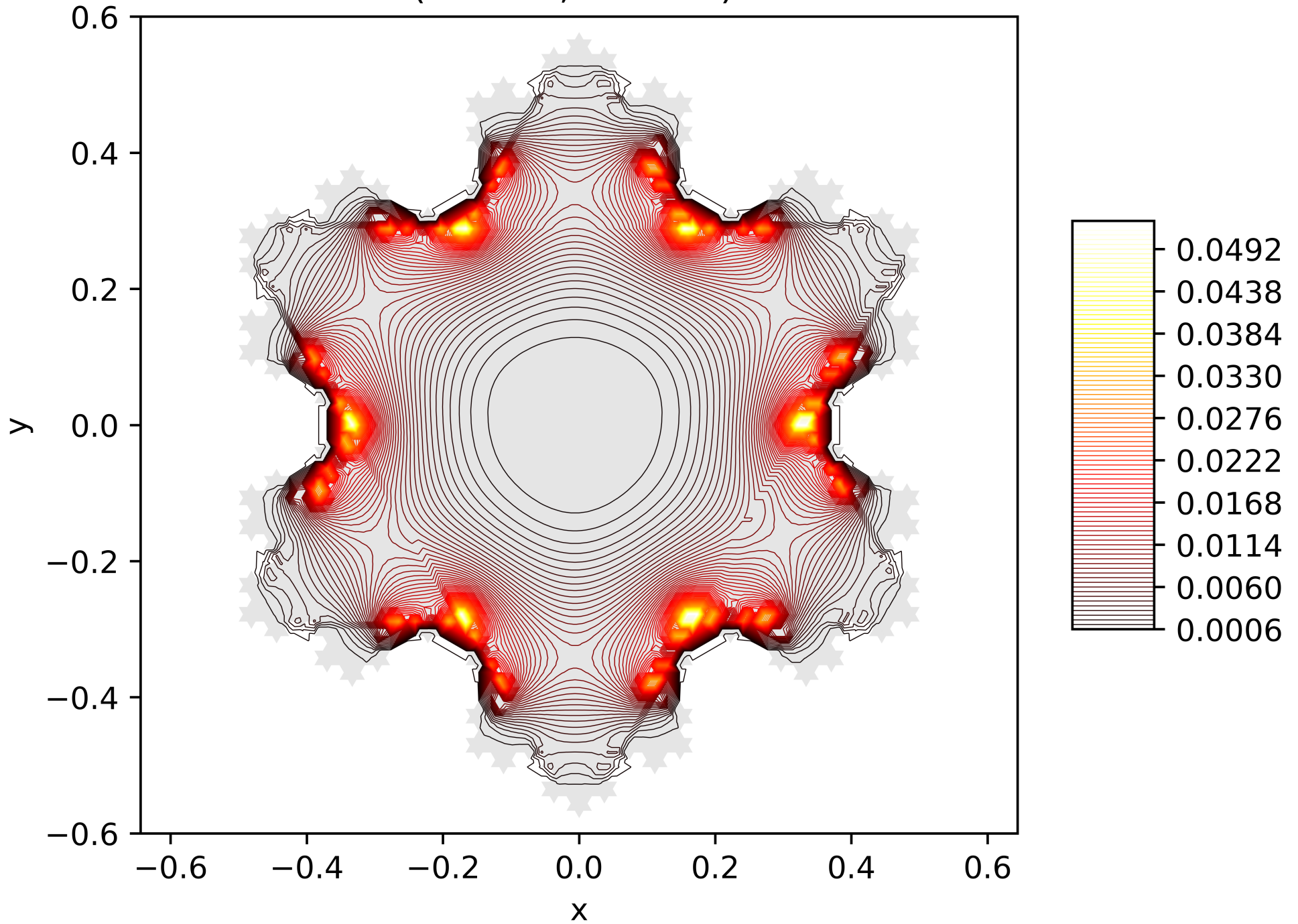
Contour Lines of the Energy Function of the 6. Eigenfunction on the Snowflake (Level 5, Res. 81) with Neumann BC
