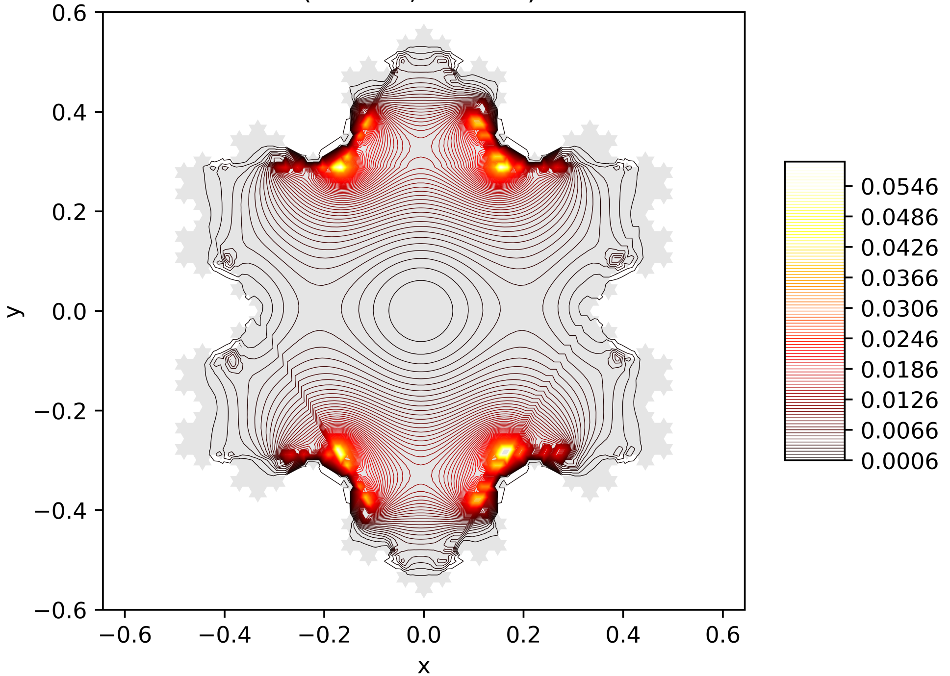
Contour Lines of the Energy Function of the 4. Eigenfunction on the Snowflake (Level 5, Res. 81) with Neumann BC
