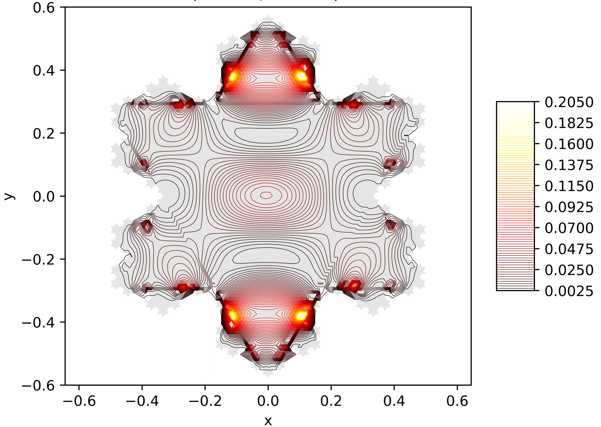
Contour Lines of the Energy Function of the 8. Eigenfunction on the Snowflake (Level 5, Res. 81) with Neumann BC
