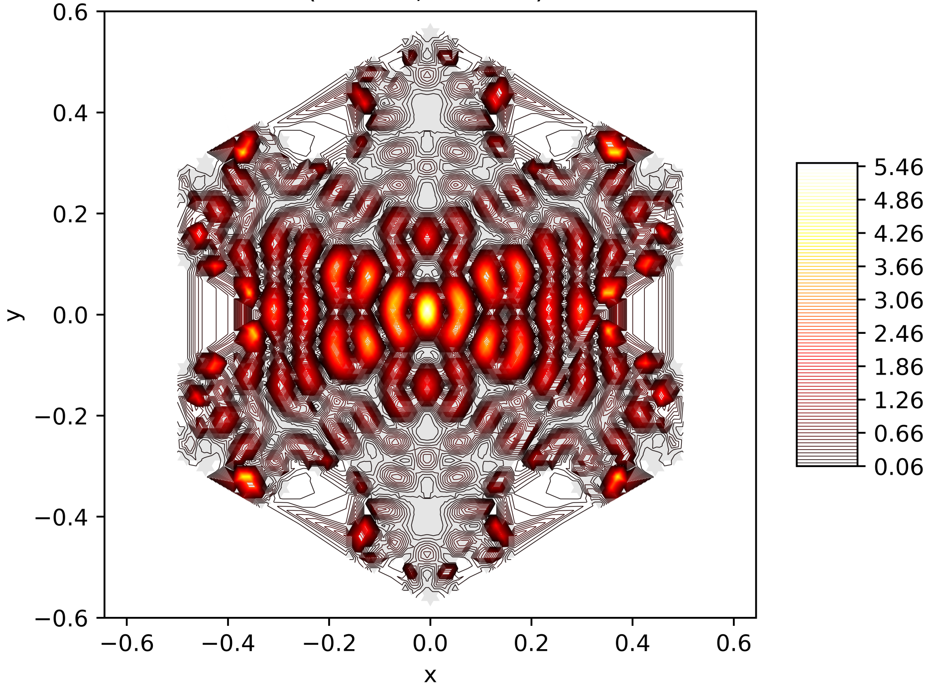
Contour Lines of the Energy Function of the 197. Eigenfunction on the Snowflake (Level 5, Res. 81) with Neumann BC
