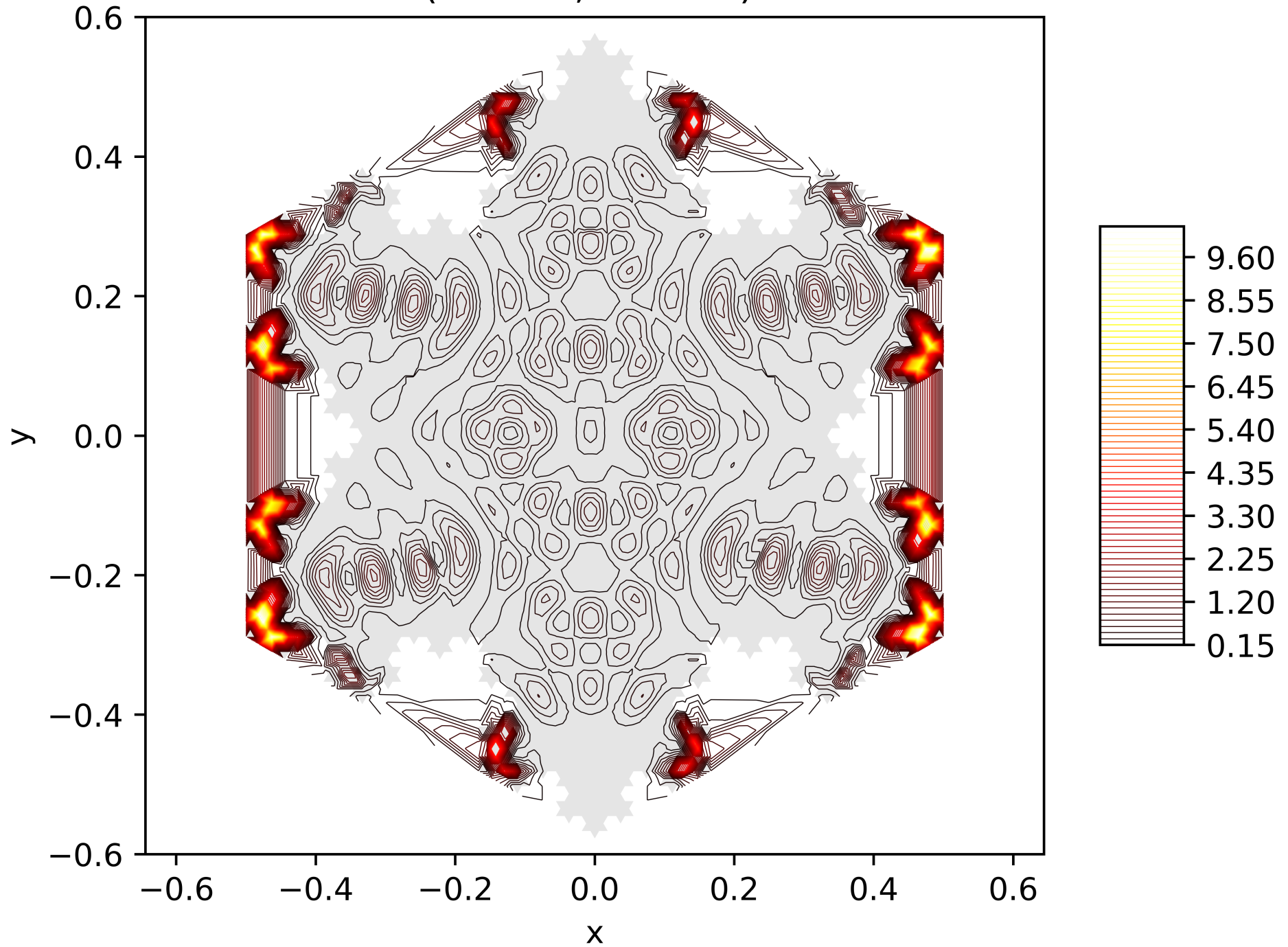
Contour Lines of the Energy Function of the 185. Eigenfunction on the Snowflake (Level 5, Res. 81) with Neumann BC
