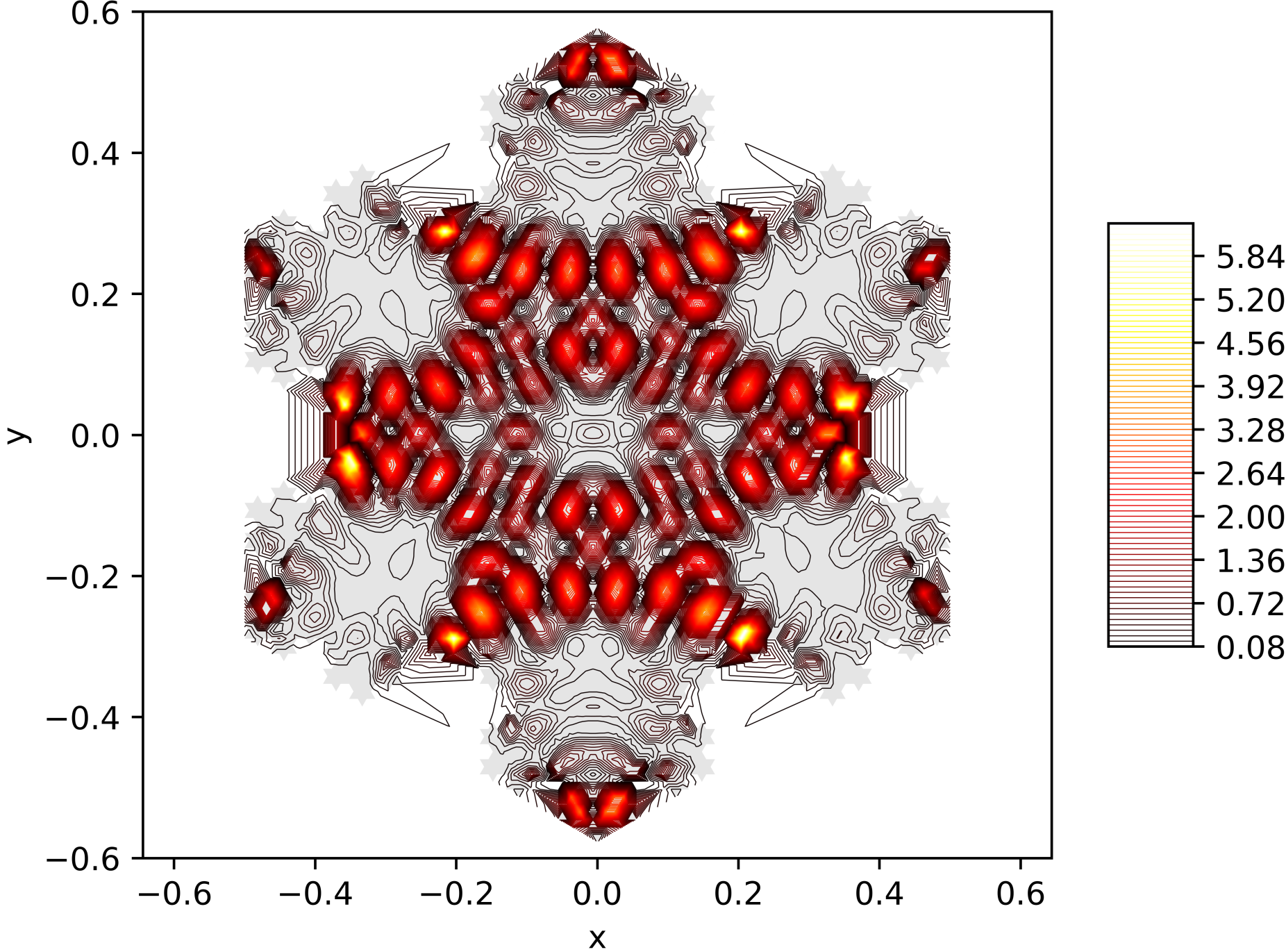
Contour Lines of the Energy Function of the 199. Eigenfunction on the Snowflake (Level 5, Res. 81) with Neumann BC
