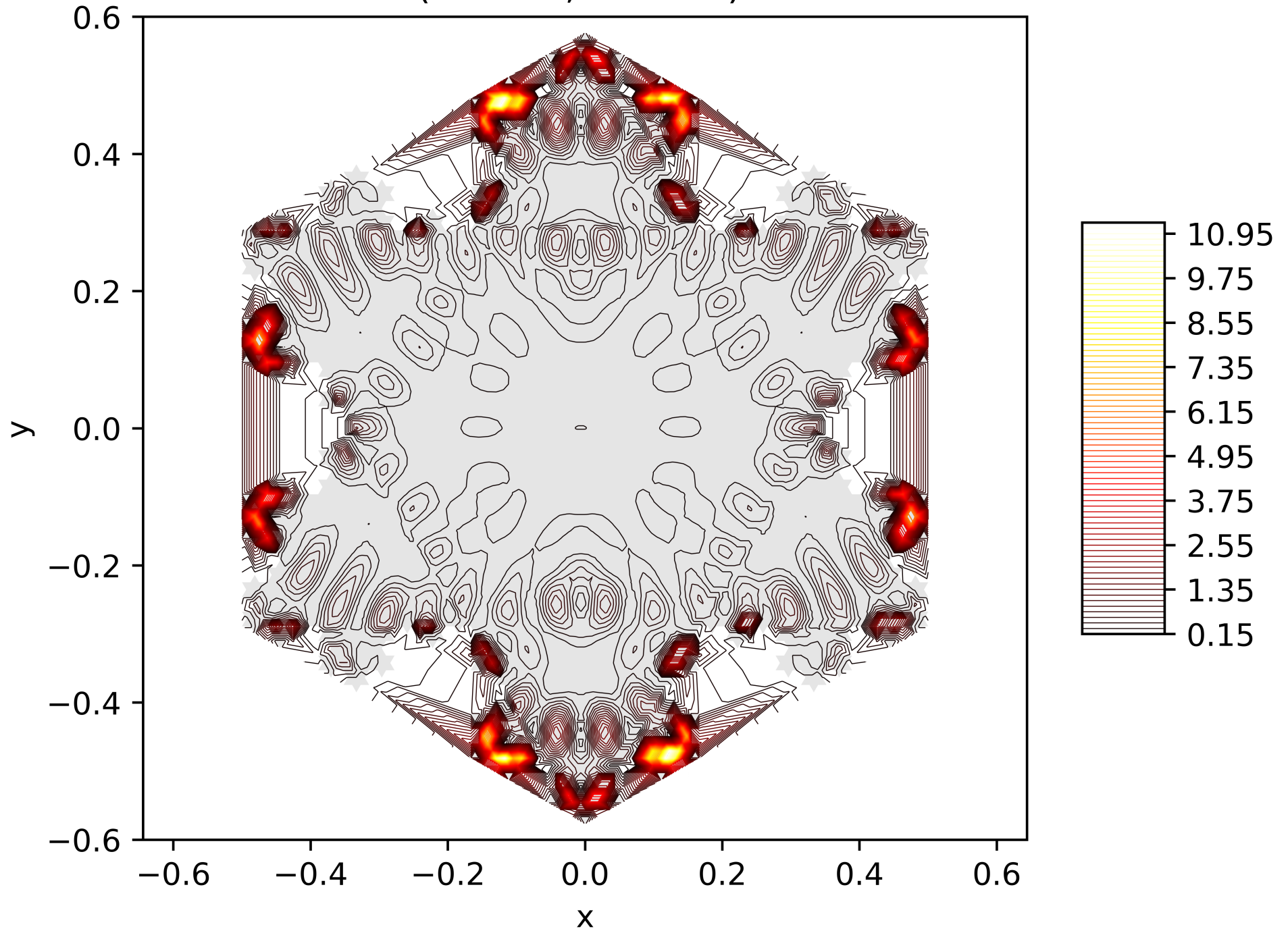
Contour Lines of the Energy Function of the 187. Eigenfunction on the Snowflake (Level 5, Res. 81) with Neumann BC
