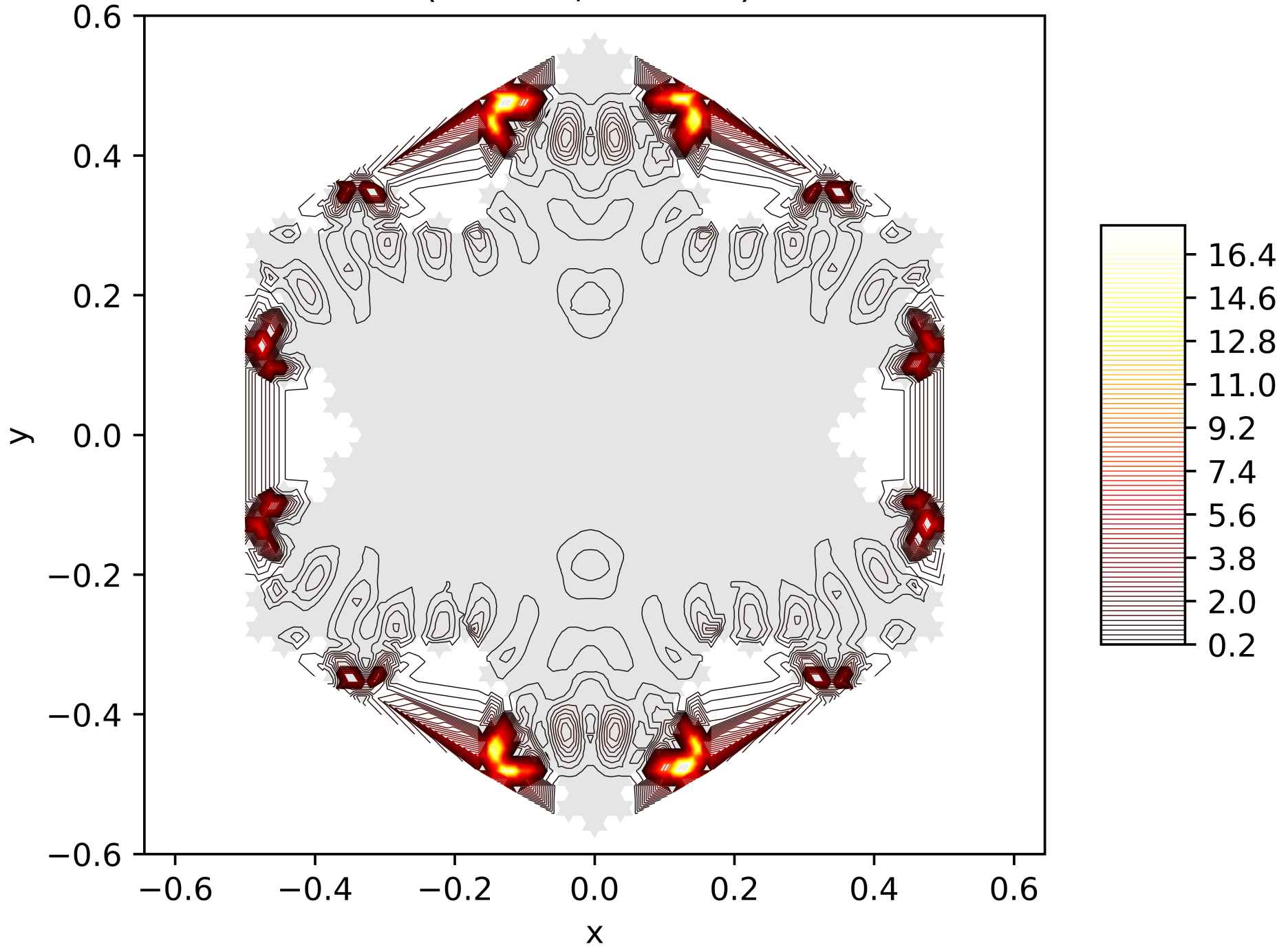
Contour Lines of the Energy Function of the 182. Eigenfunction on the Snowflake (Level 5, Res. 81) with Neumann BC
