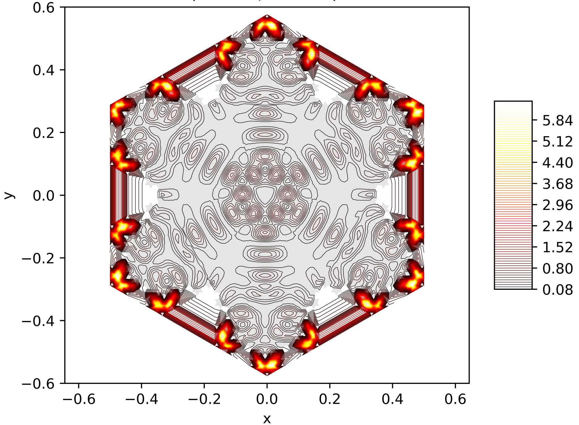
Contour Lines of the Energy Function of the 181. Eigenfunction on the Snowflake (Level 5, Res. 81) with Neumann BC
