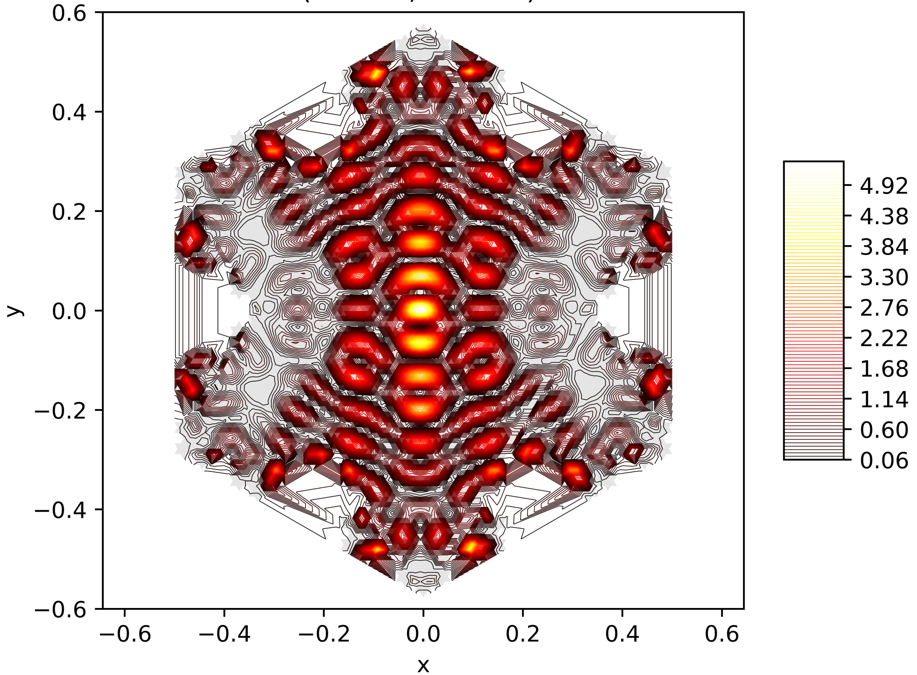
Contour Lines of the Energy Function of the 196. Eigenfunction on the Snowflake (Level 5, Res. 81) with Neumann BC
