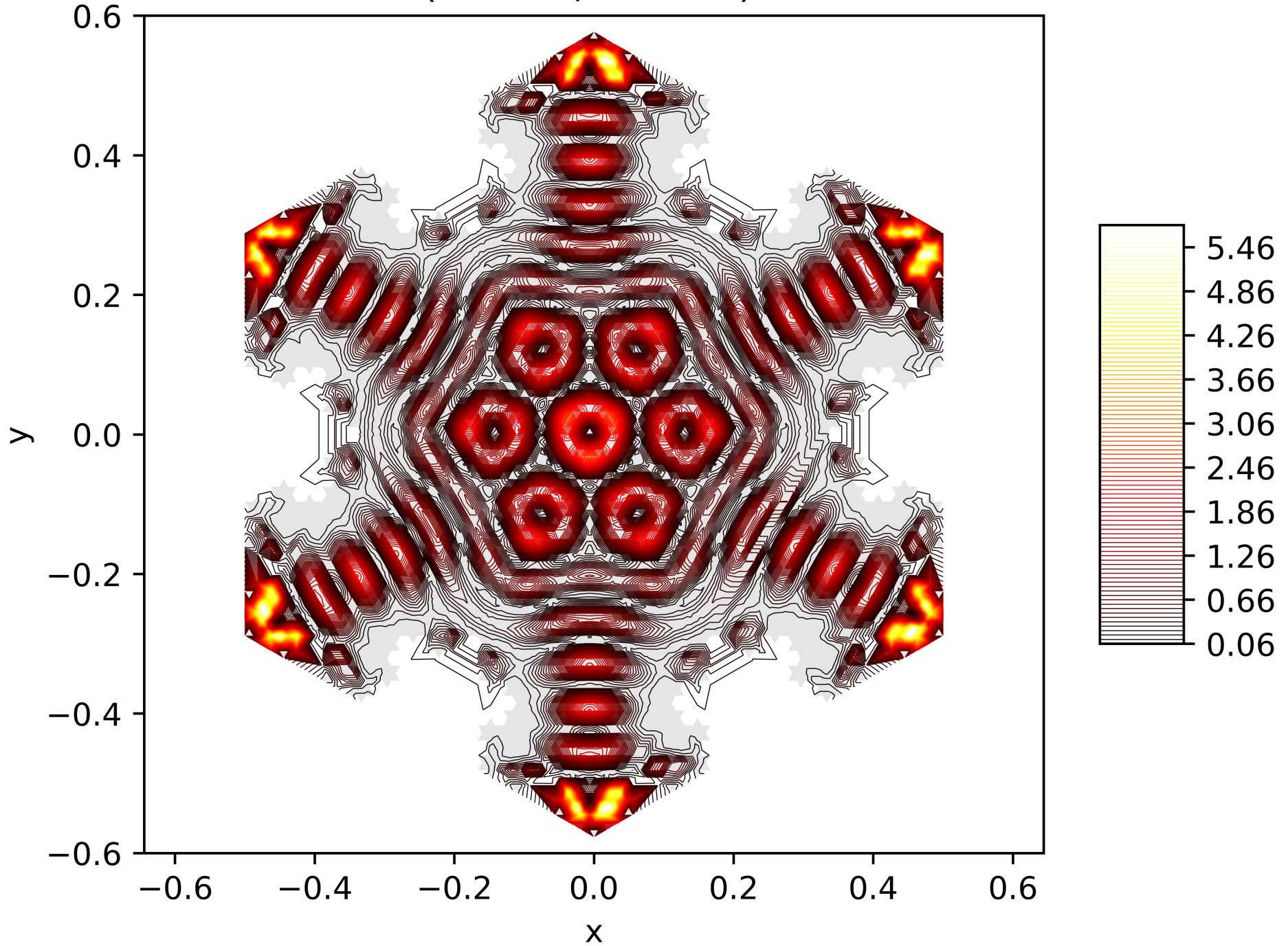
Contour Lines of the Energy Function of the 198. Eigenfunction on the Snowflake (Level 5, Res. 81) with Neumann BC
