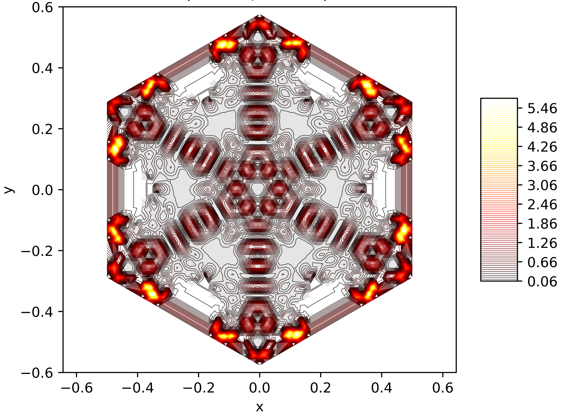
Contour Lines of the Energy Function of the 189. Eigenfunction on the Snowflake (Level 5, Res. 81) with Neumann BC
