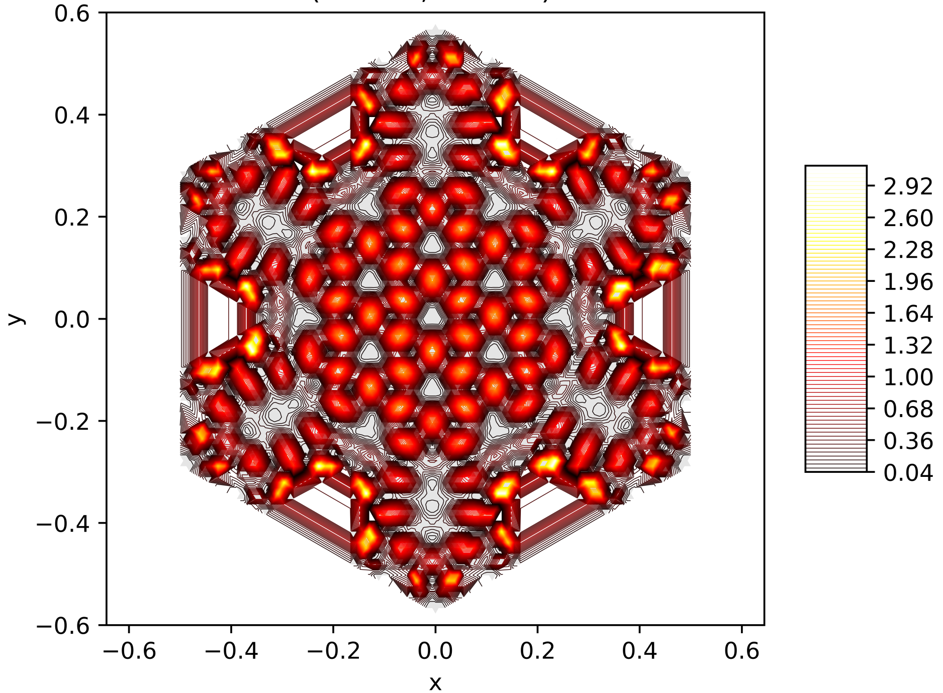
Contour Lines of the Energy Function of the 192. Eigenfunction on the Snowflake (Level 5, Res. 81) with Neumann BC
