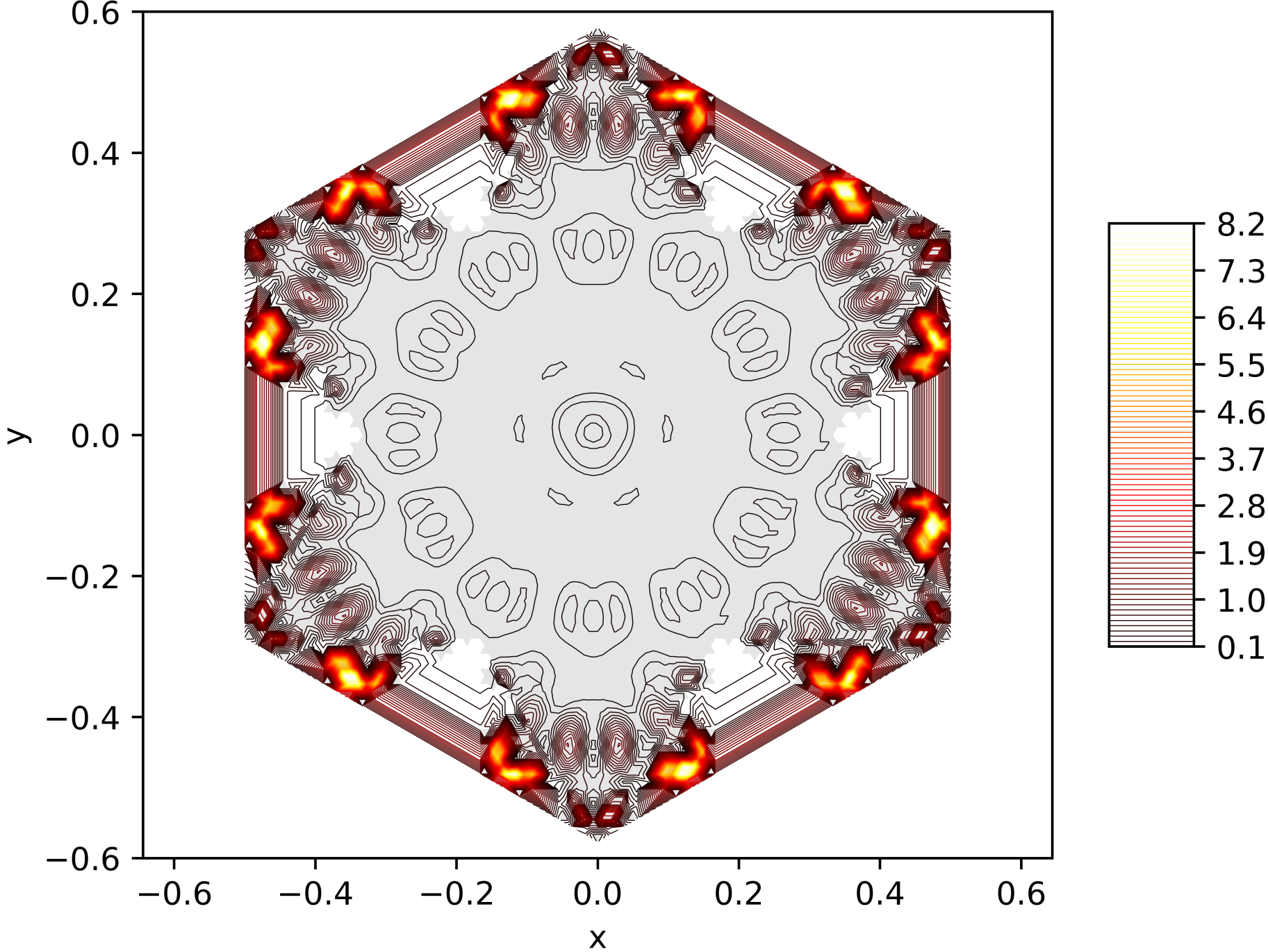
Contour Lines of the Energy Function of the 186. Eigenfunction on the Snowflake (Level 5, Res. 81) with Neumann BC
