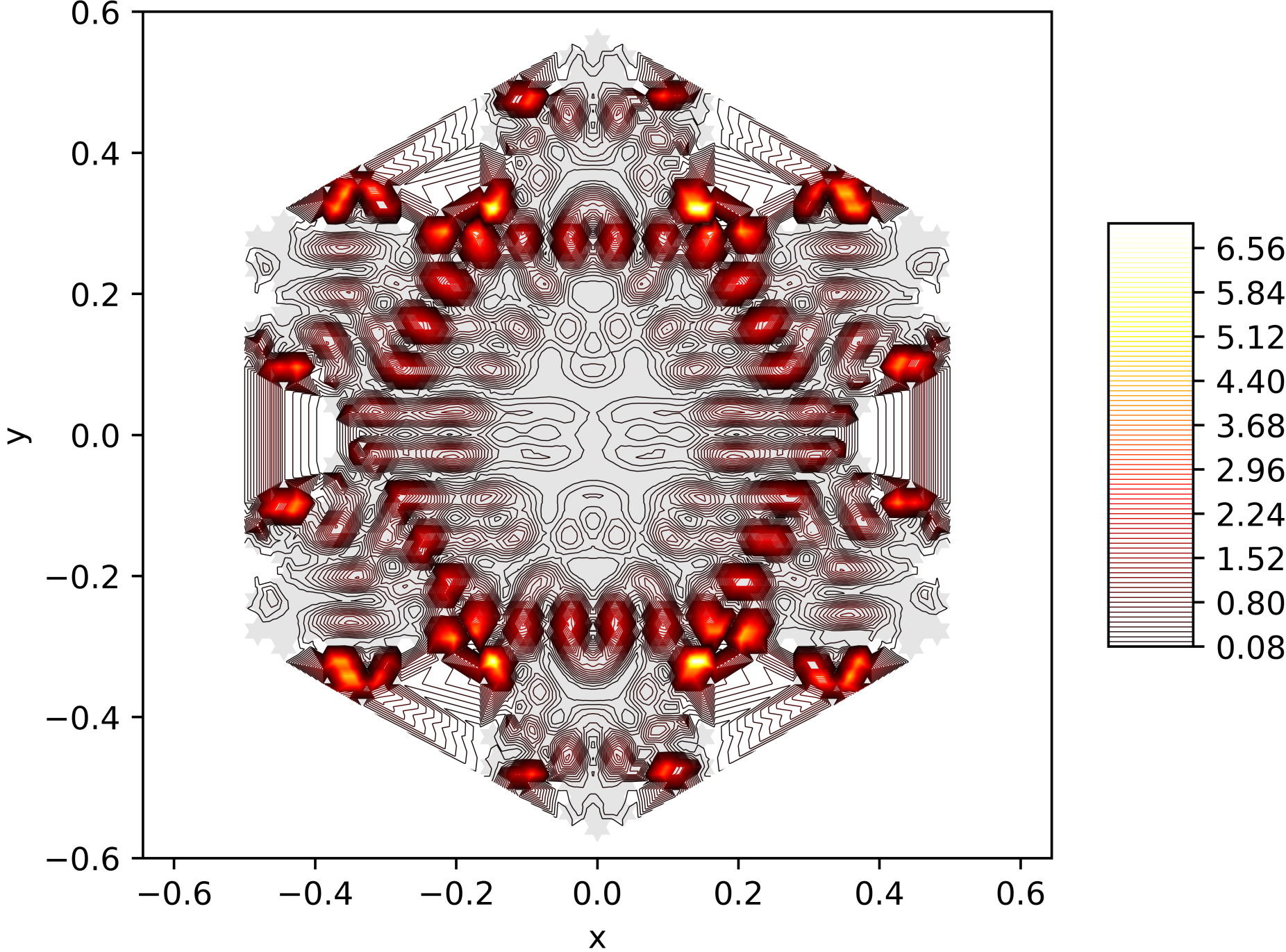
Contour Lines of the Energy Function of the 194. Eigenfunction on the Snowflake (Level 5, Res. 81) with Neumann BC
