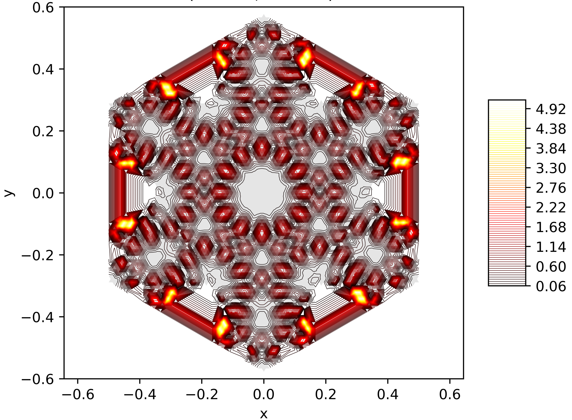
Contour Lines of the Energy Function of the 193. Eigenfunction on the Snowflake (Level 5, Res. 81) with Neumann BC
