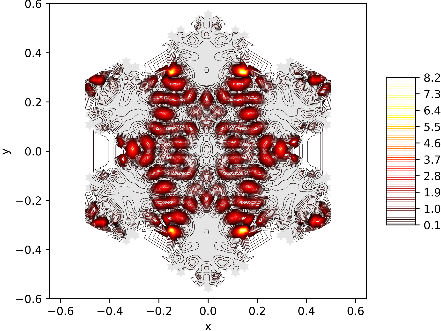
Contour Lines of the Energy Function of the 200. Eigenfunction on the Snowflake (Level 5, Res. 81) with Neumann BC
