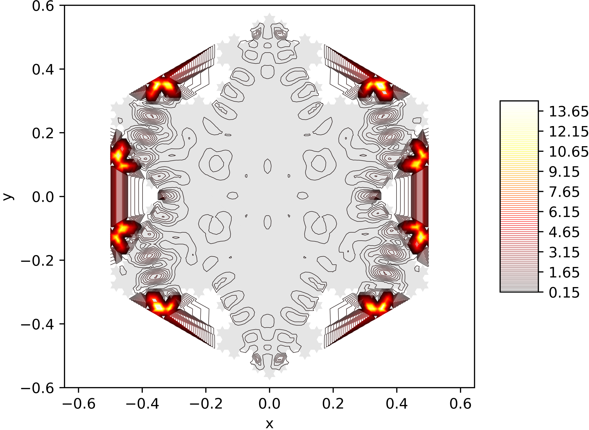
Contour Lines of the Energy Function of the 183. Eigenfunction on the Snowflake (Level 5, Res. 81) with Neumann BC
