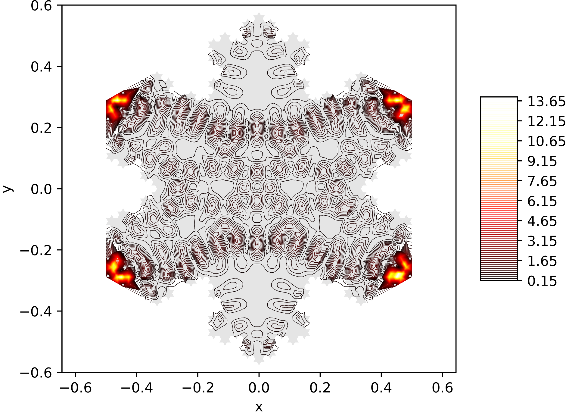
Contour Lines of the Energy Function of the 191. Eigenfunction on the Snowflake (Level 5, Res. 81) with Neumann BC
