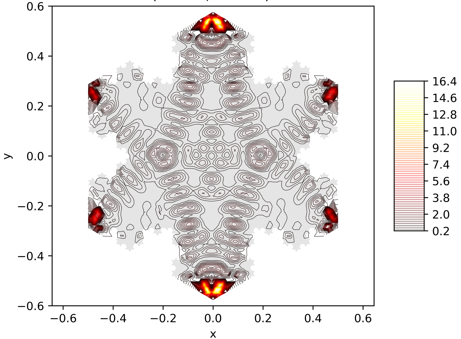
Contour Lines of the Energy Function of the 190. Eigenfunction on the Snowflake (Level 5, Res. 81) with Neumann BC
