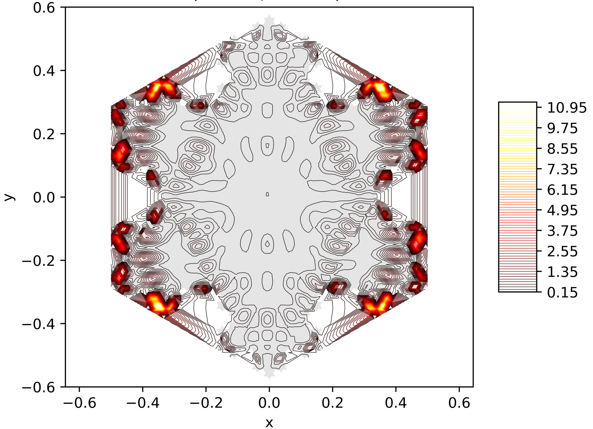
Contour Lines of the Energy Function of the 188. Eigenfunction on the Snowflake (Level 5, Res. 81) with Neumann BC
