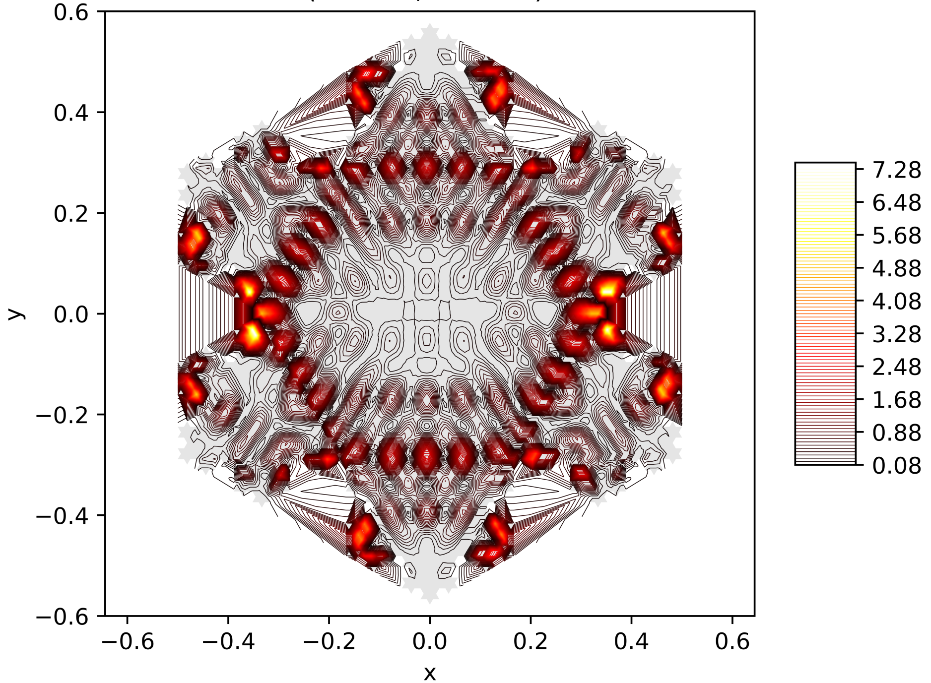
Contour Lines of the Energy Function of the 195. Eigenfunction on the Snowflake (Level 5, Res. 81) with Neumann BC
