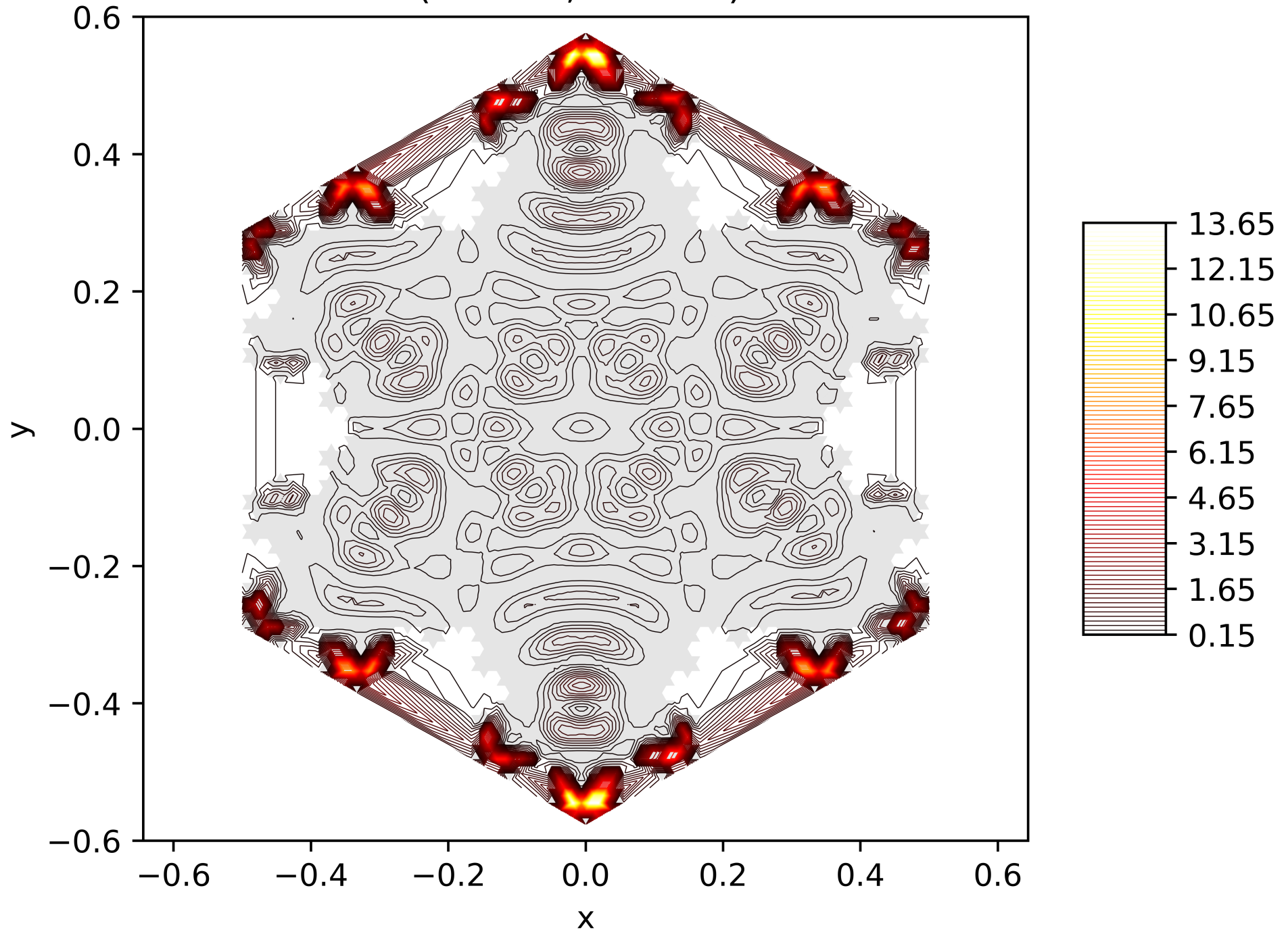
Contour Lines of the Energy Function of the 184. Eigenfunction on the Snowflake (Level 5, Res. 81) with Neumann BC
