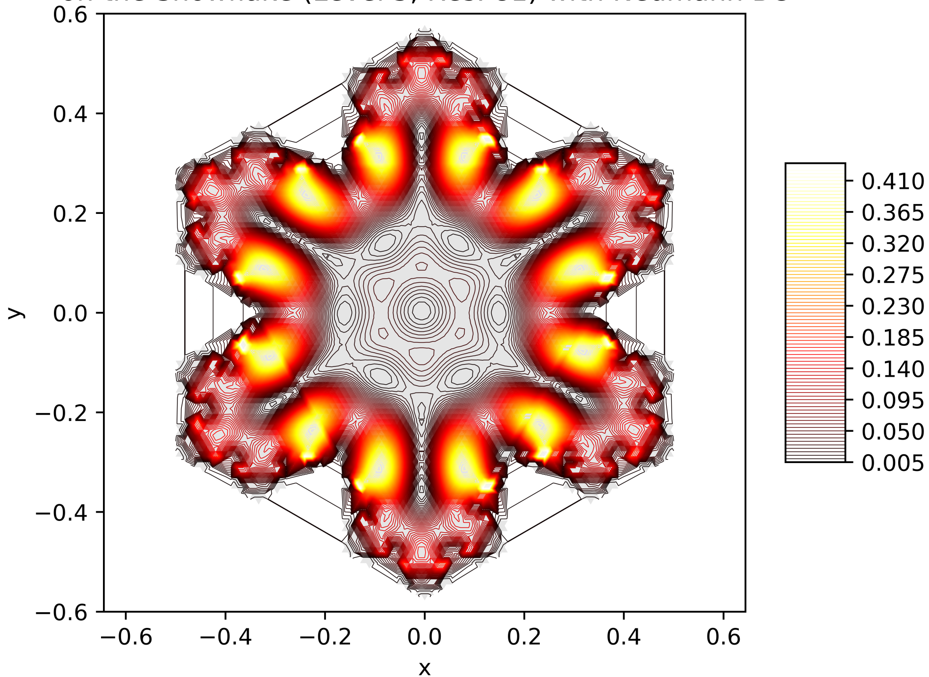
Contour Lines of the Energy Function of the 38. Eigenfunction on the Snowflake (Level 5, Res. 81) with Neumann BC
