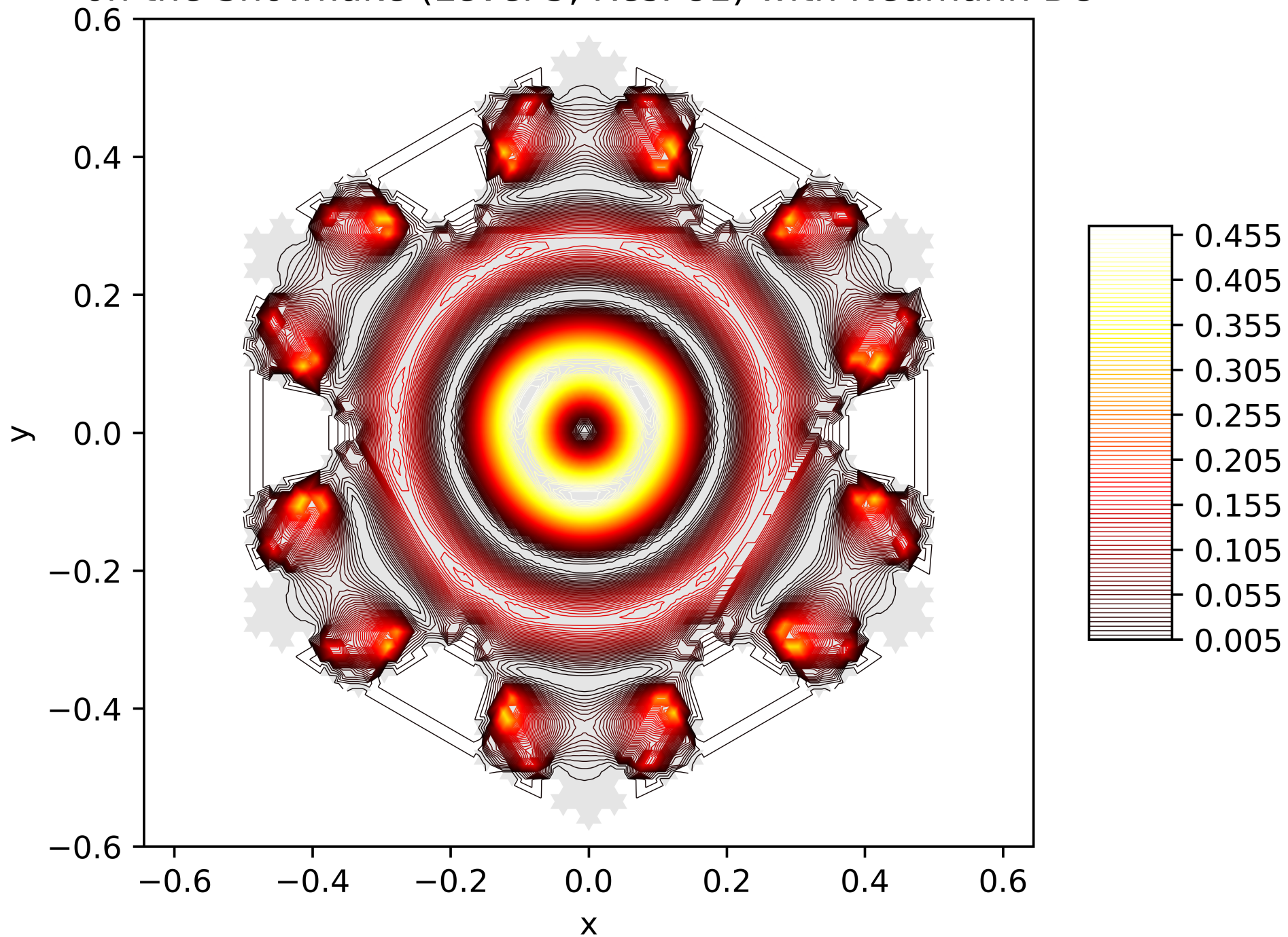
Contour Lines of the Energy Function of the 35. Eigenfunction on the Snowflake (Level 5, Res. 81) with Neumann BC
