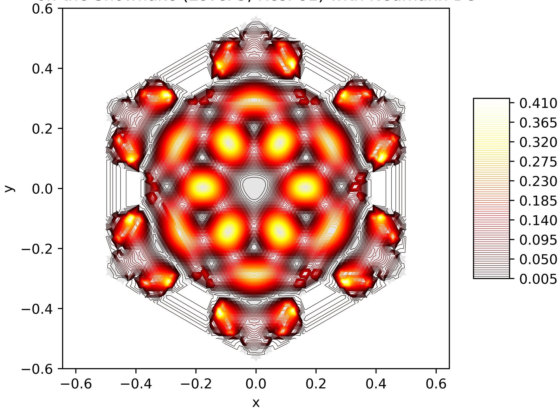
Contour Lines of the Energy Function of the 37. Eigenfunction on the Snowflake (Level 5, Res. 81) with Neumann BC
