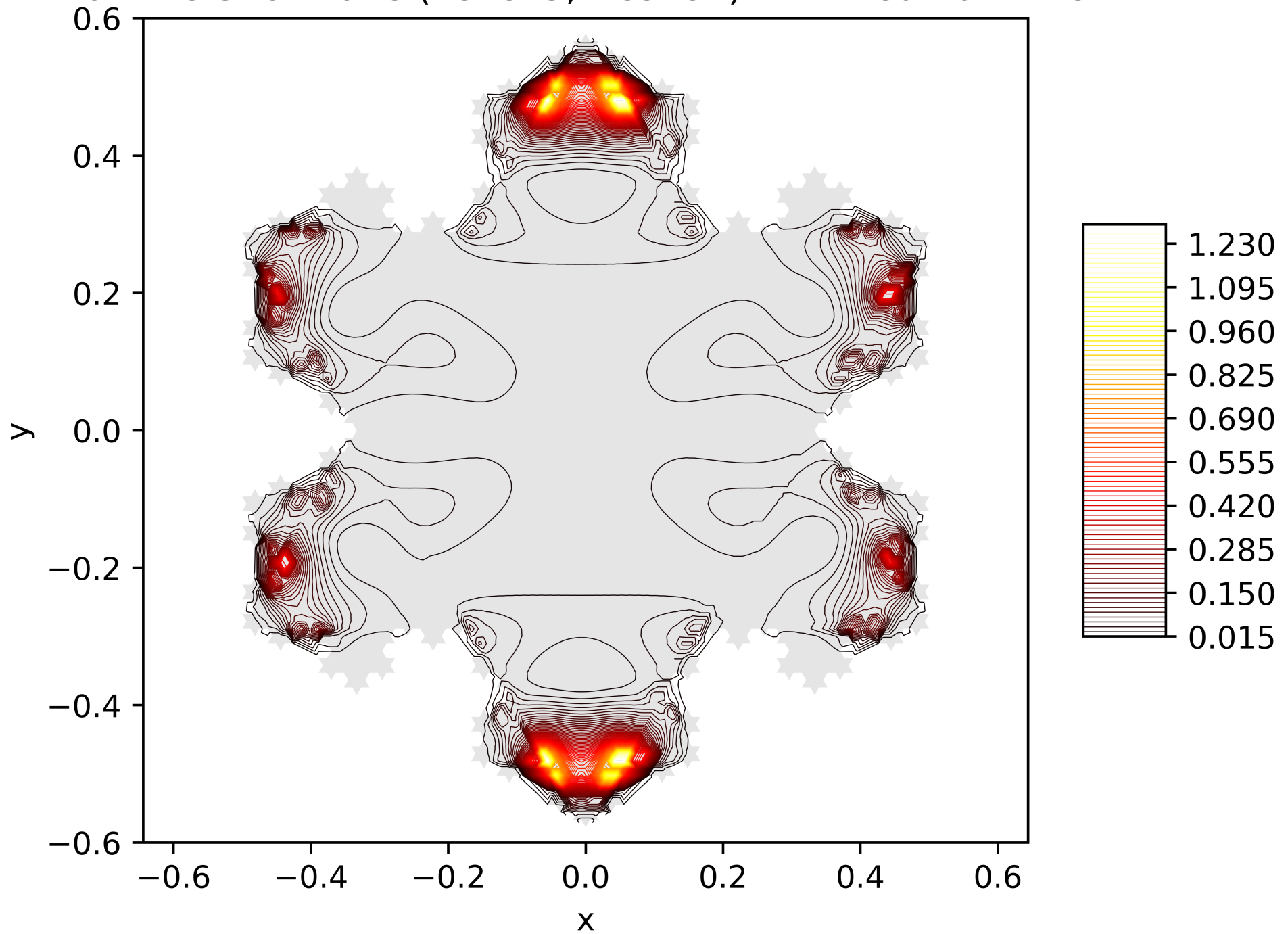
Contour Lines of the Energy Function of the 23. Eigenfunction on the Snowflake (Level 5, Res. 81) with Neumann BC
