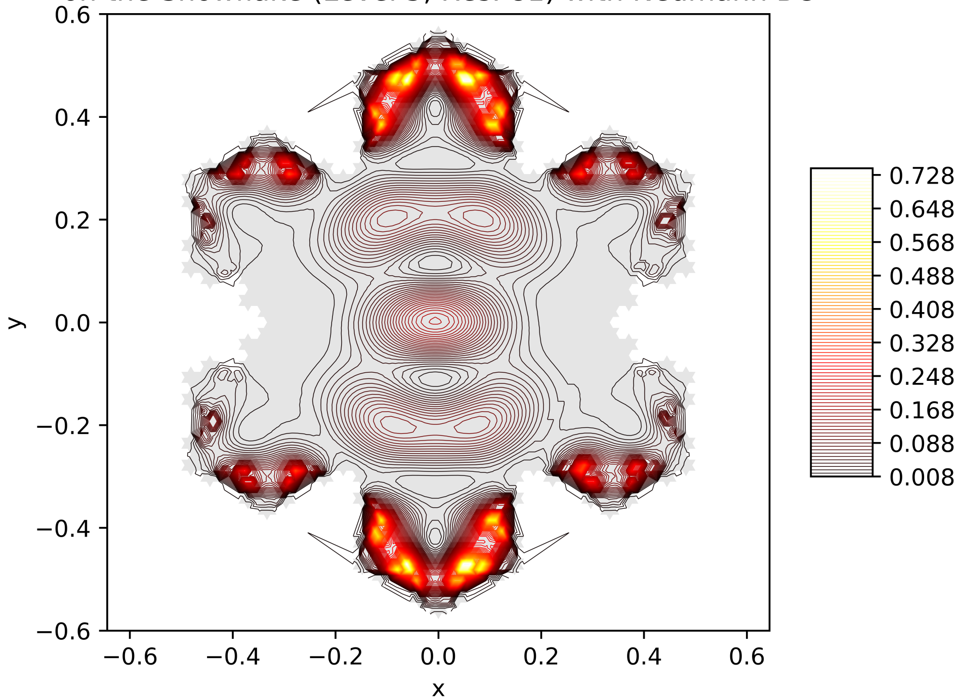
Contour Lines of the Energy Function of the 27. Eigenfunction on the Snowflake (Level 5, Res. 81) with Neumann BC
