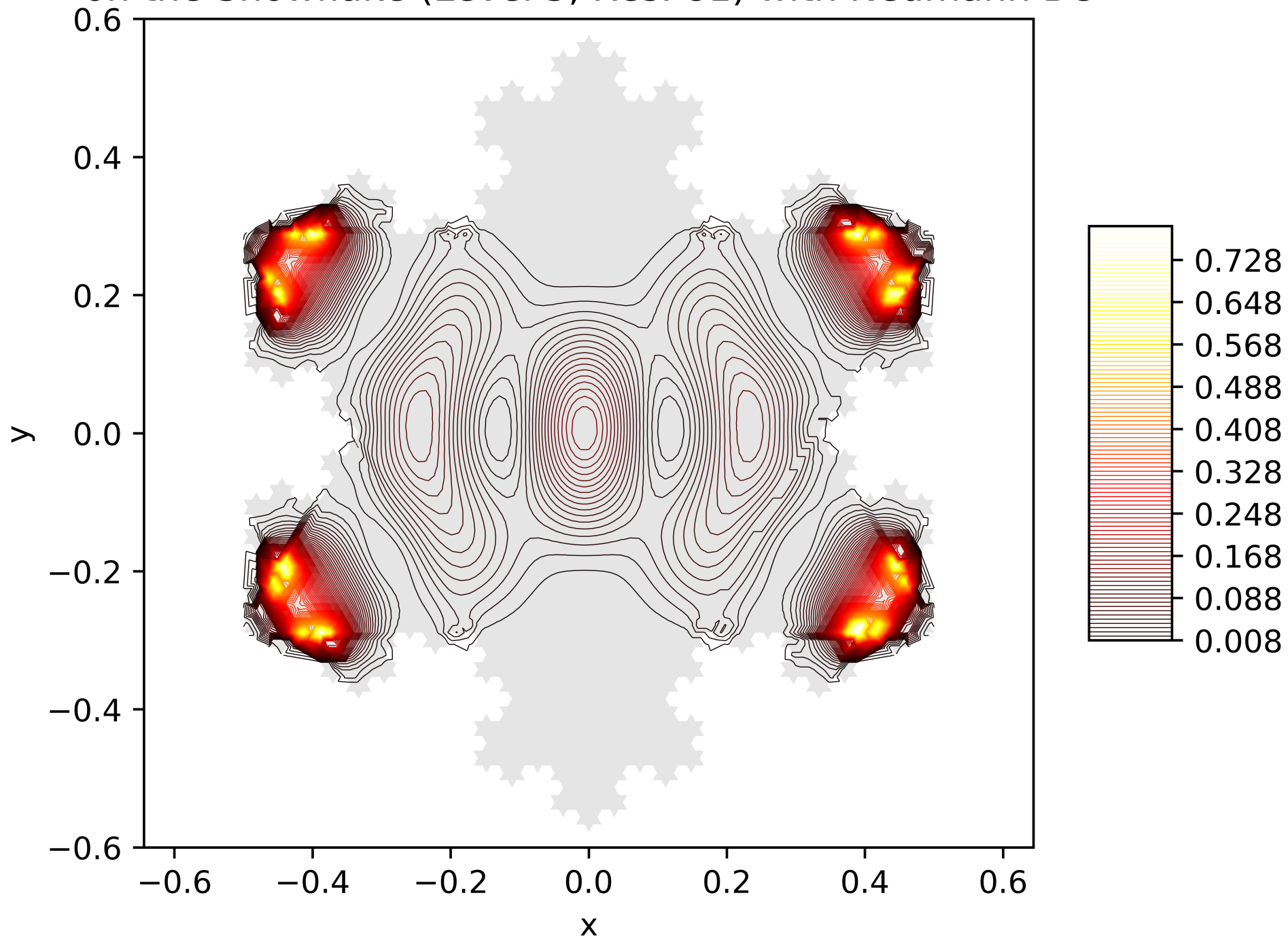
Contour Lines of the Energy Function of the 22. Eigenfunction on the Snowflake (Level 5, Res. 81) with Neumann BC
