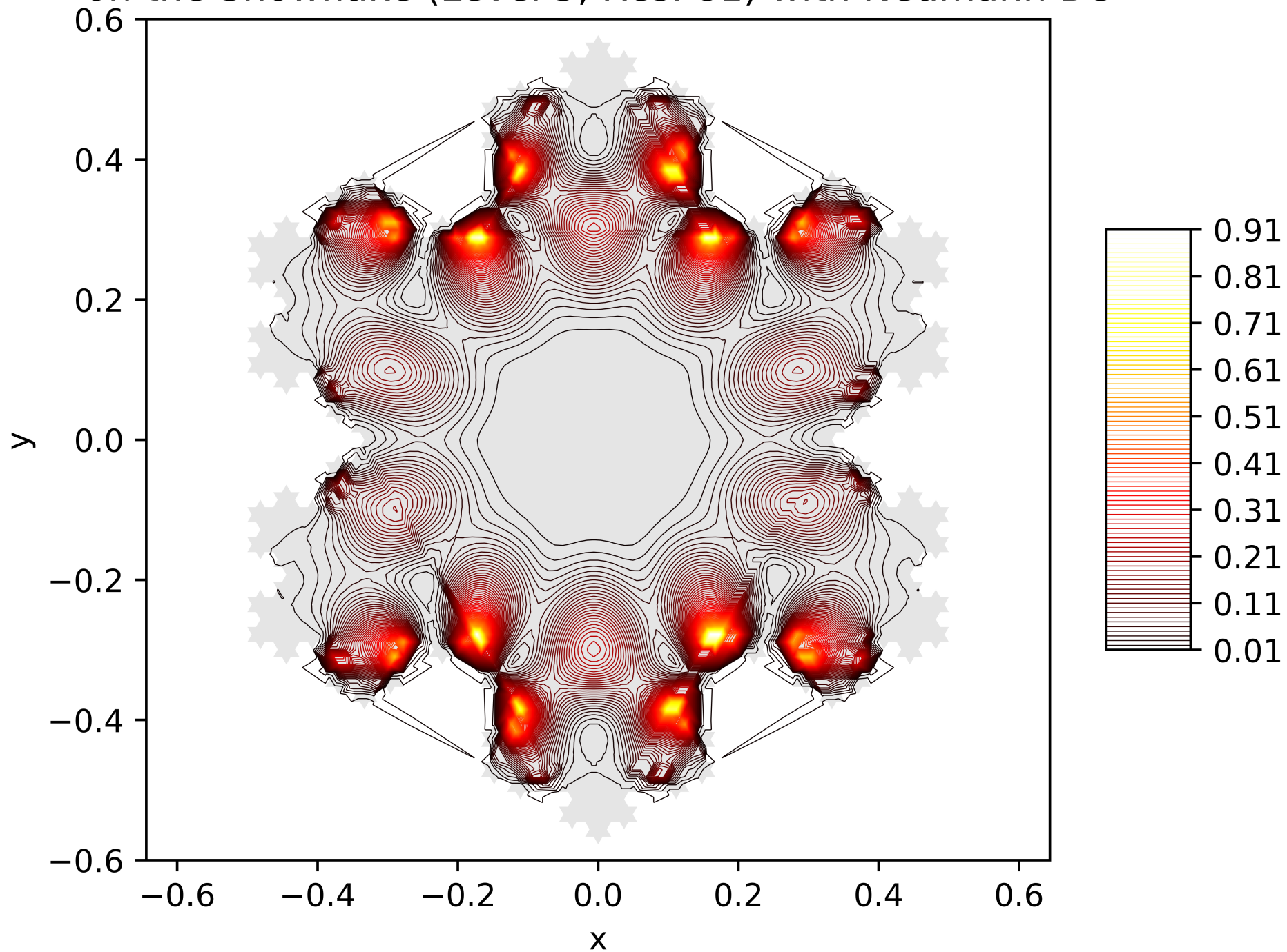
Contour Lines of the Energy Function of the 31. Eigenfunction on the Snowflake (Level 5, Res. 81) with Neumann BC
