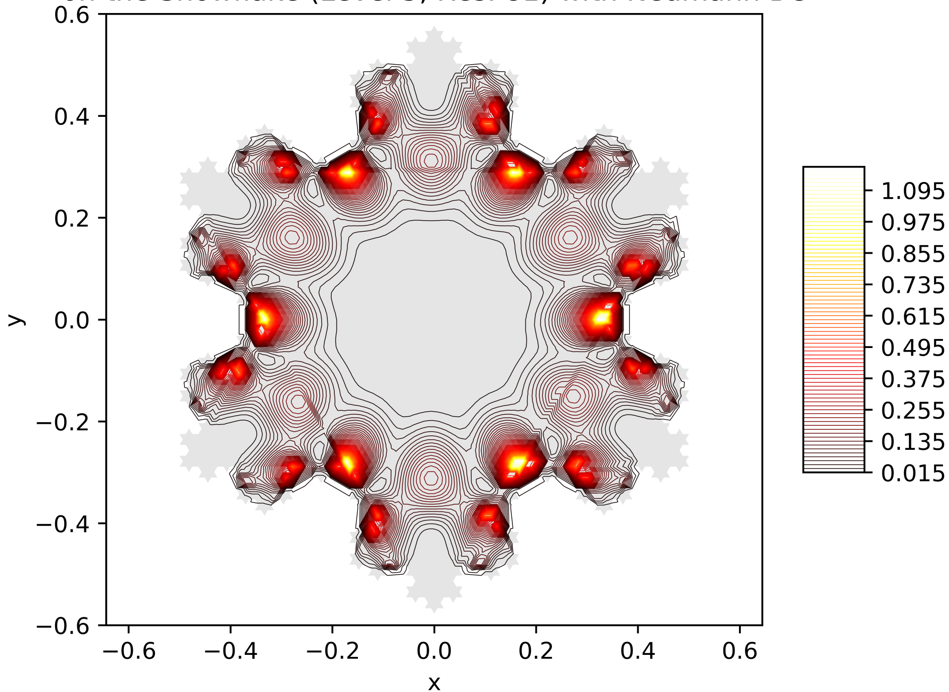
Contour Lines of the Energy Function of the 36. Eigenfunction on the Snowflake (Level 5, Res. 81) with Neumann BC
