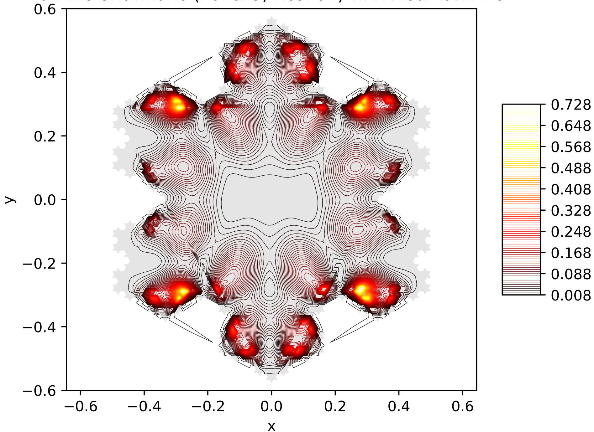
Contour Lines of the Energy Function of the 29. Eigenfunction on the Snowflake (Level 5, Res. 81) with Neumann BC
