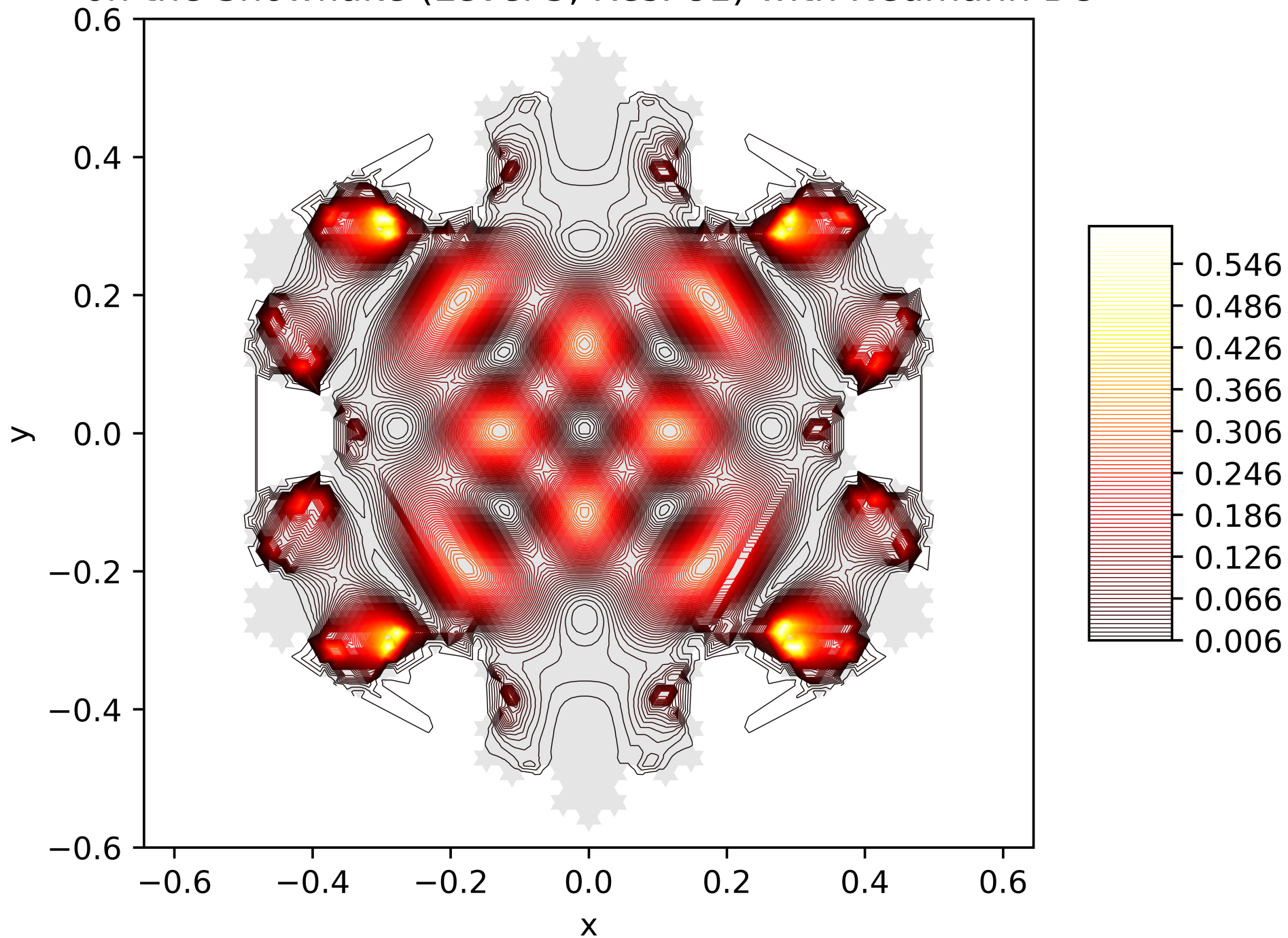
Contour Lines of the Energy Function of the 34. Eigenfunction on the Snowflake (Level 5, Res. 81) with Neumann BC
