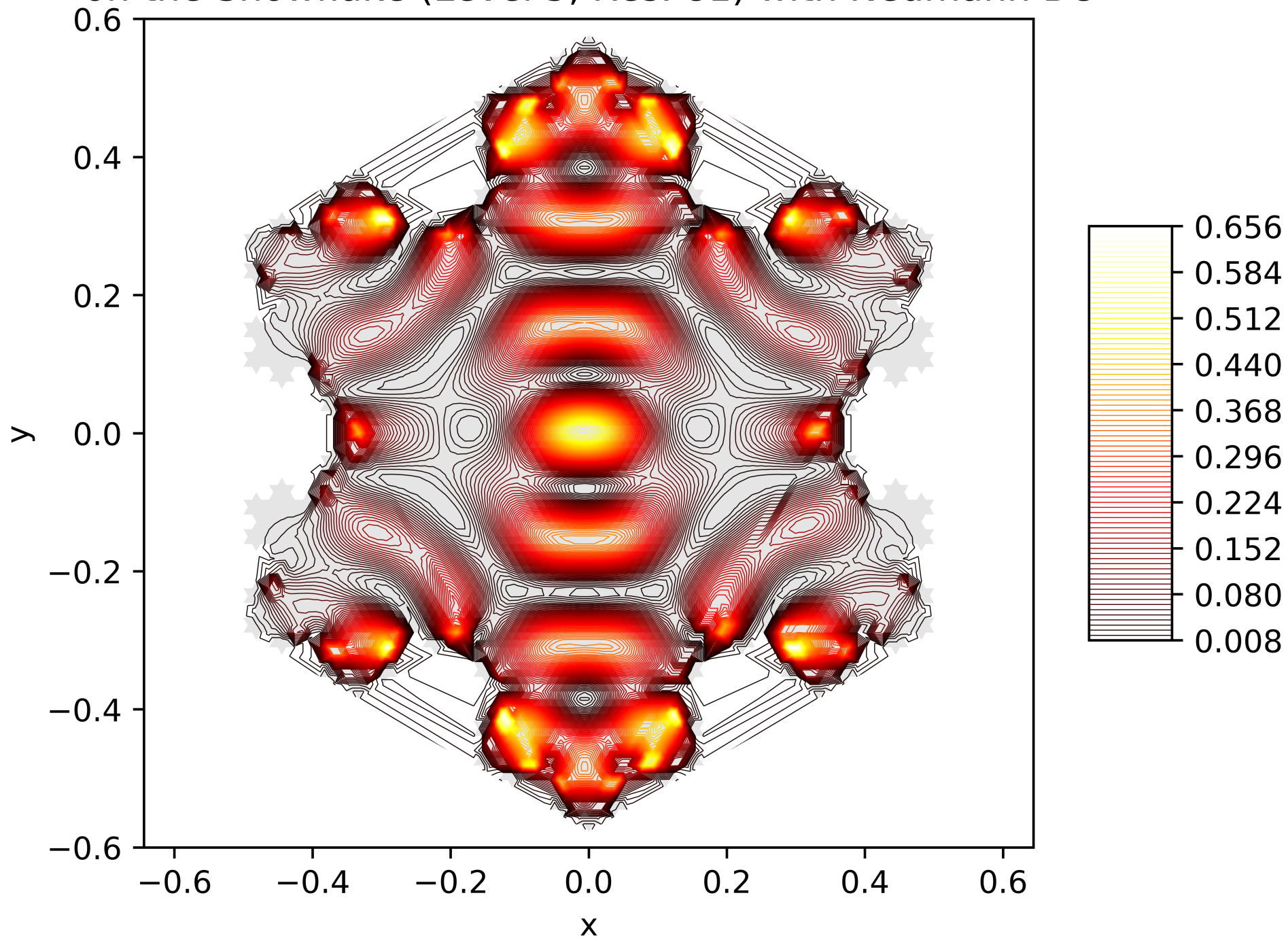
Contour Lines of the Energy Function of the 40. Eigenfunction on the Snowflake (Level 5, Res. 81) with Neumann BC
