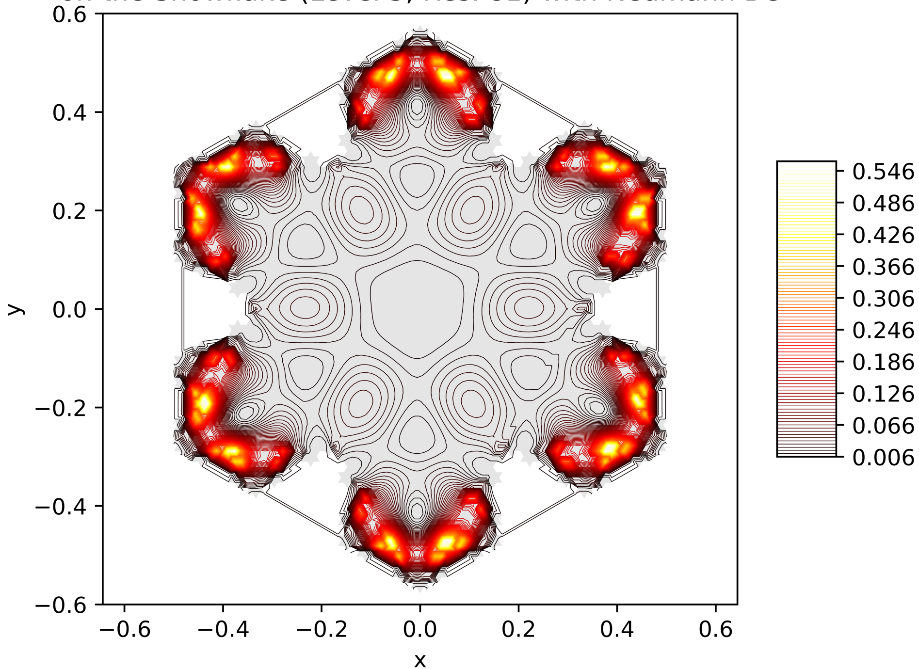
Contour Lines of the Energy Function of the 26. Eigenfunction on the Snowflake (Level 5, Res. 81) with Neumann BC
