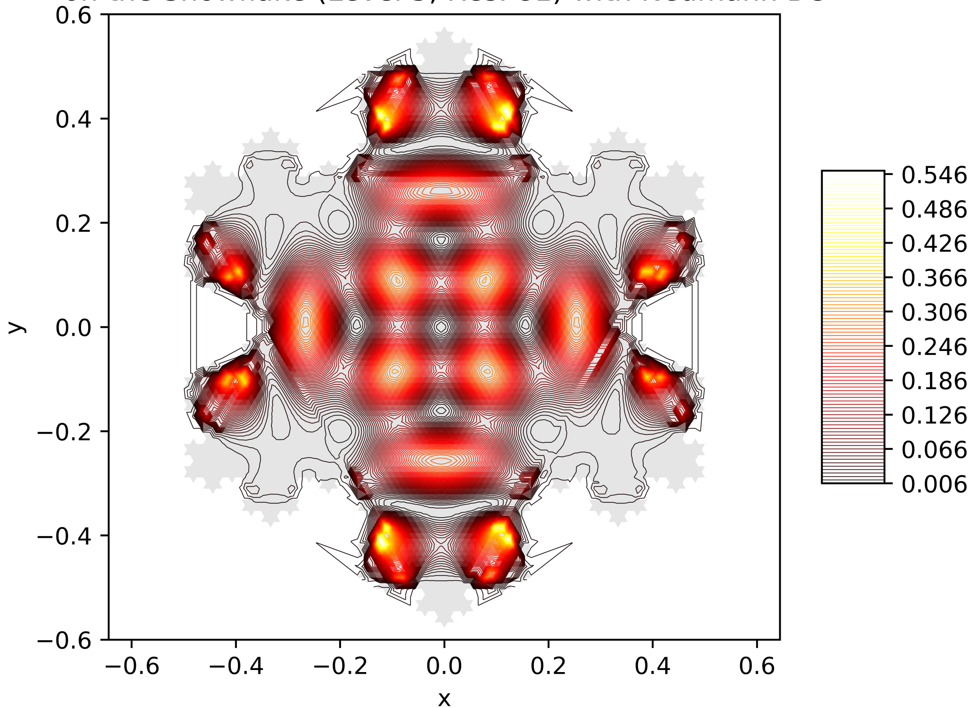
Contour Lines of the Energy Function of the 33. Eigenfunction on the Snowflake (Level 5, Res. 81) with Neumann BC
