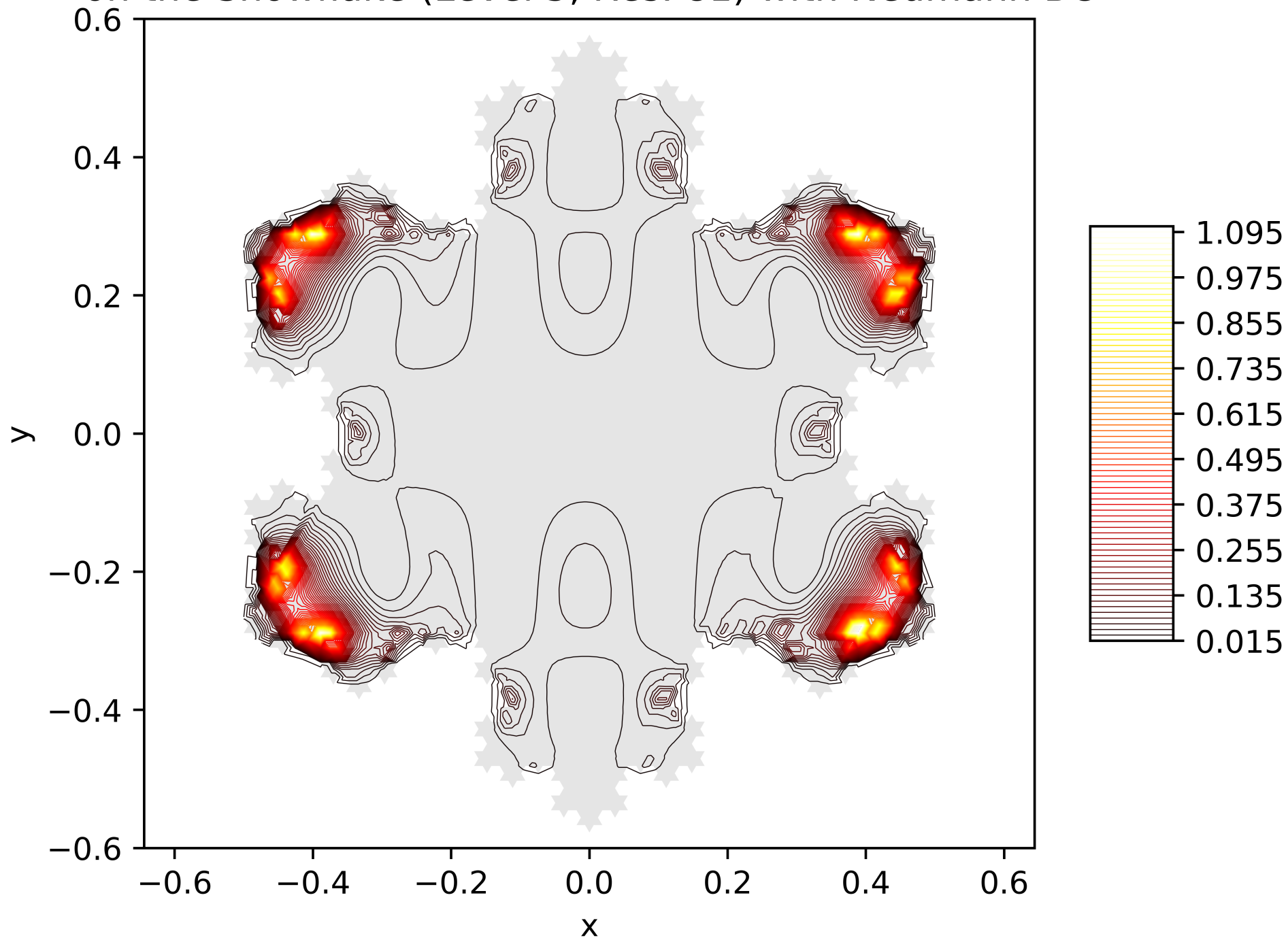
Contour Lines of the Energy Function of the 24. Eigenfunction on the Snowflake (Level 5, Res. 81) with Neumann BC
