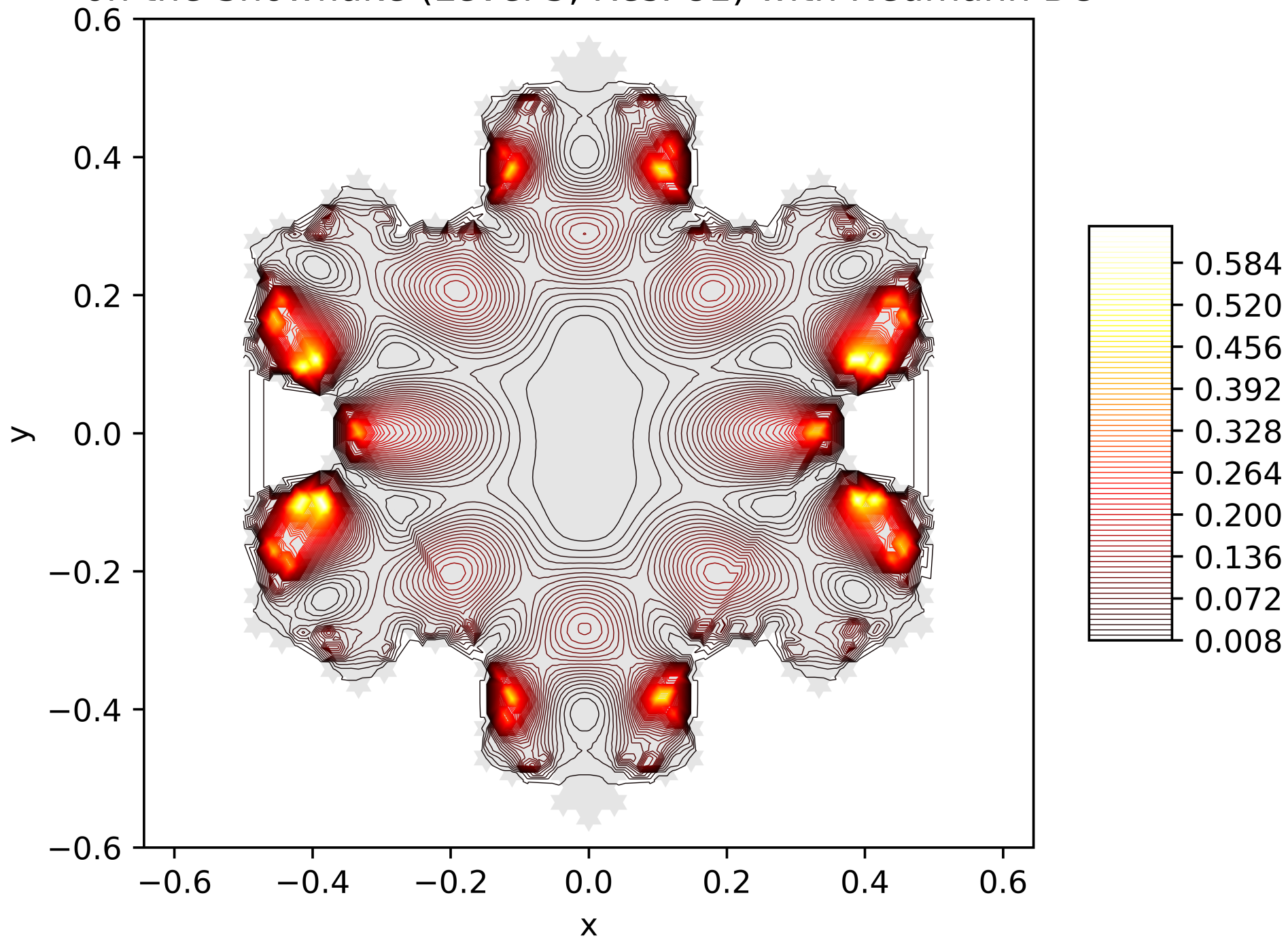
Contour Lines of the Energy Function of the 30. Eigenfunction on the Snowflake (Level 5, Res. 81) with Neumann BC
