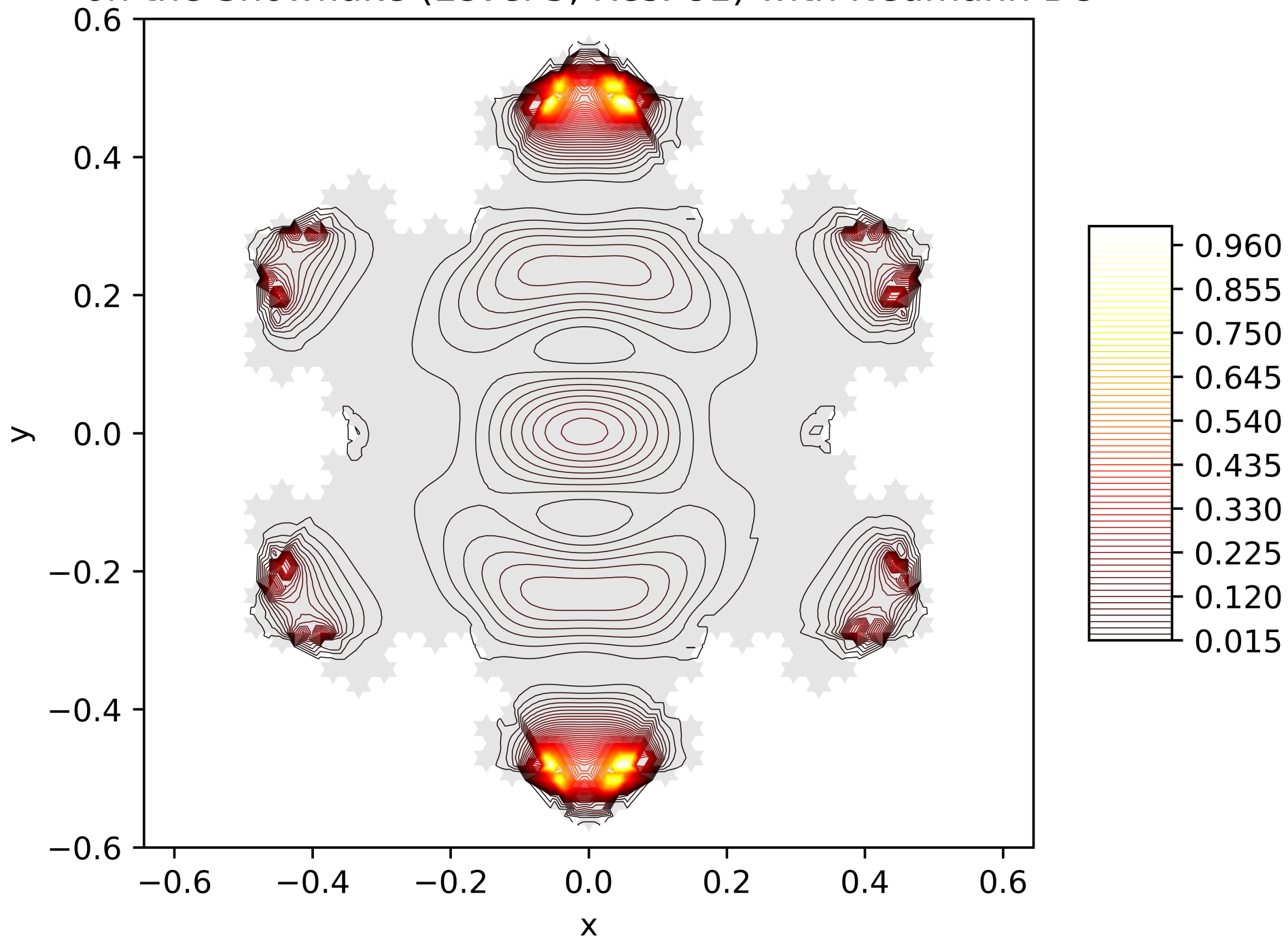
Contour Lines of the Energy Function of the 21. Eigenfunction on the Snowflake (Level 5, Res. 81) with Neumann BC
