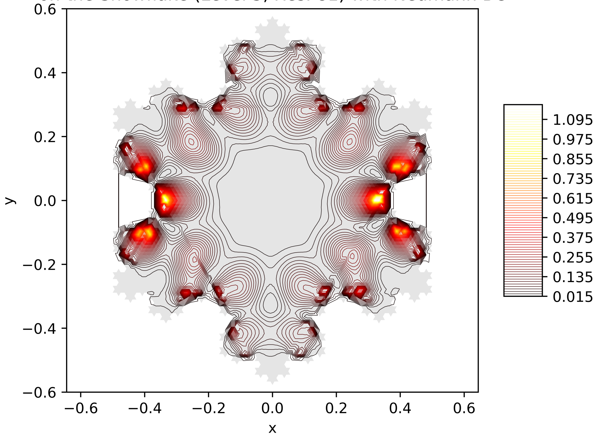
Contour Lines of the Energy Function of the 32. Eigenfunction on the Snowflake (Level 5, Res. 81) with Neumann BC
