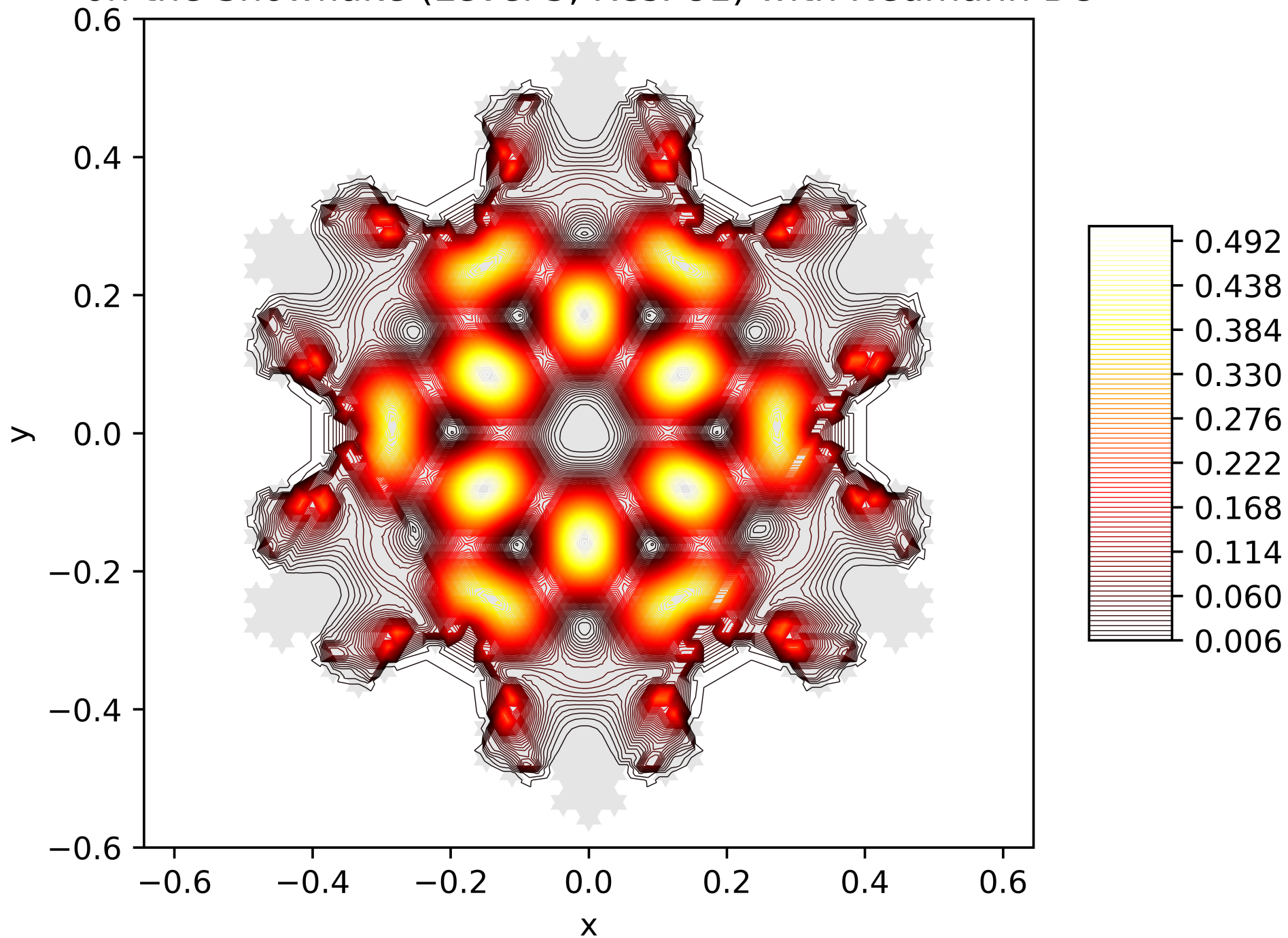
Contour Lines of the Energy Function of the 39. Eigenfunction on the Snowflake (Level 5, Res. 81) with Neumann BC
