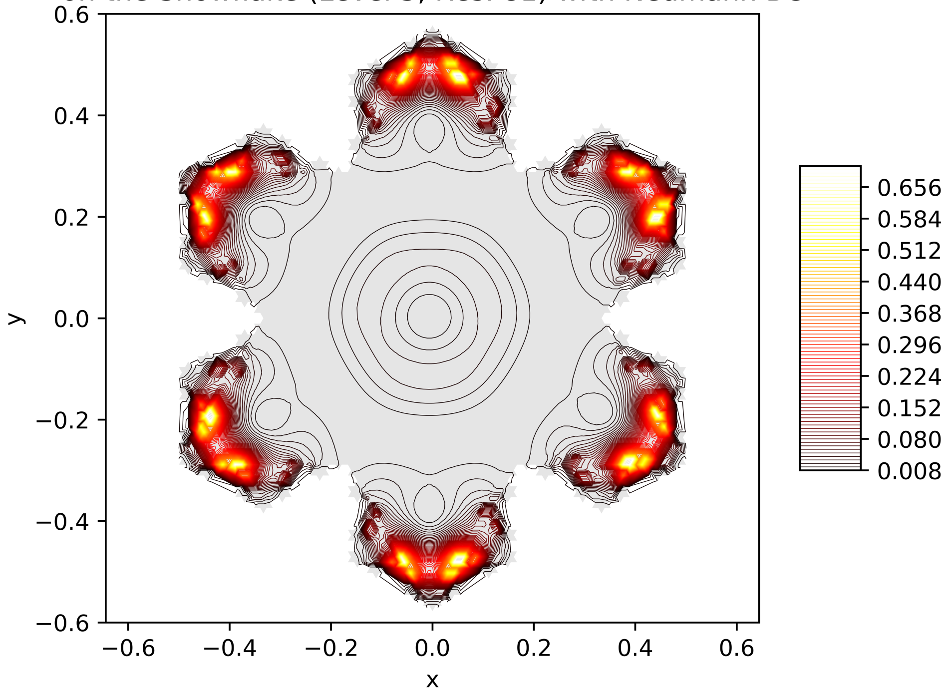
Contour Lines of the Energy Function of the 25. Eigenfunction on the Snowflake (Level 5, Res. 81) with Neumann BC
