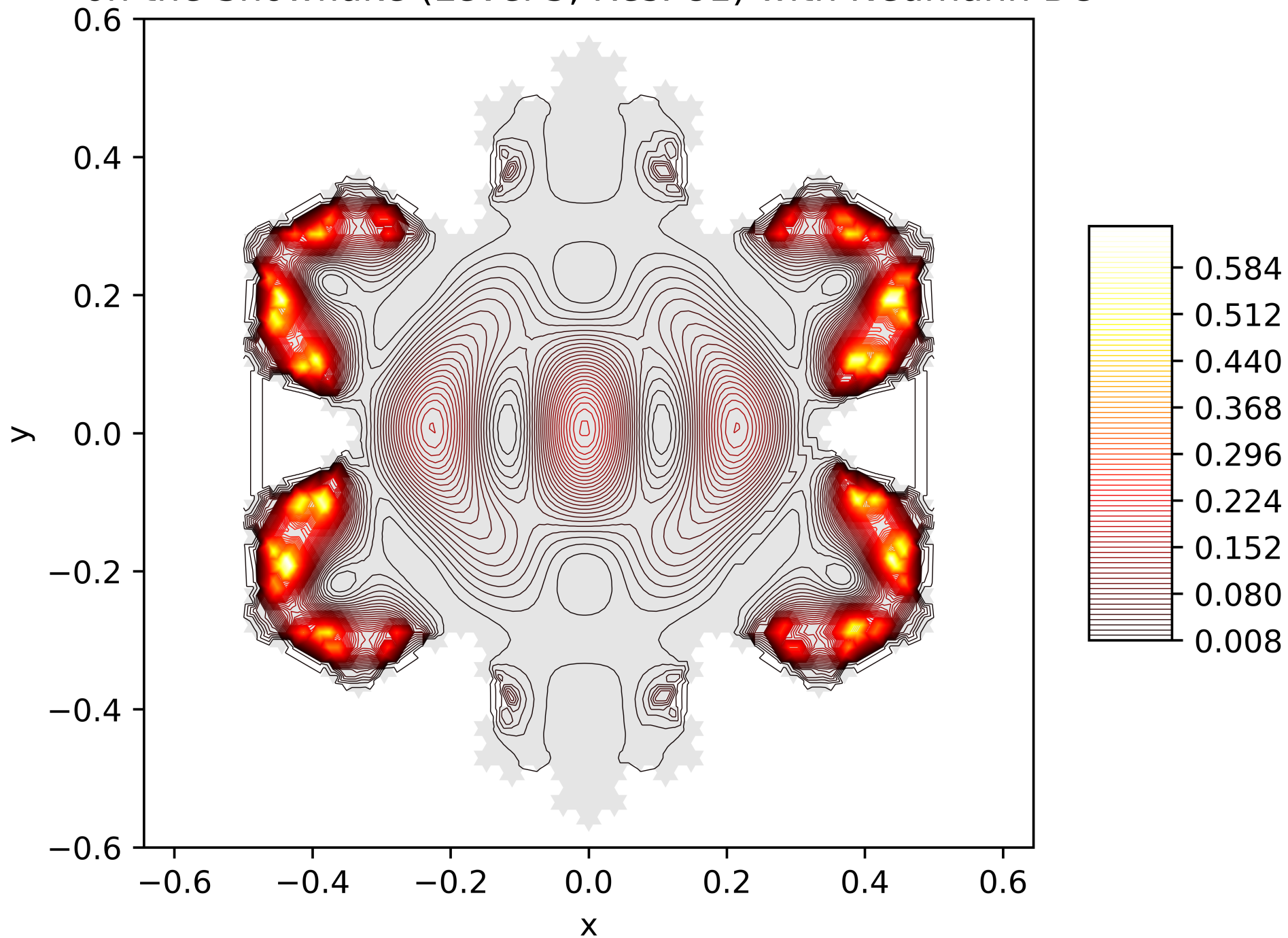
Contour Lines of the Energy Function of the 28. Eigenfunction on the Snowflake (Level 5, Res. 81) with Neumann BC
