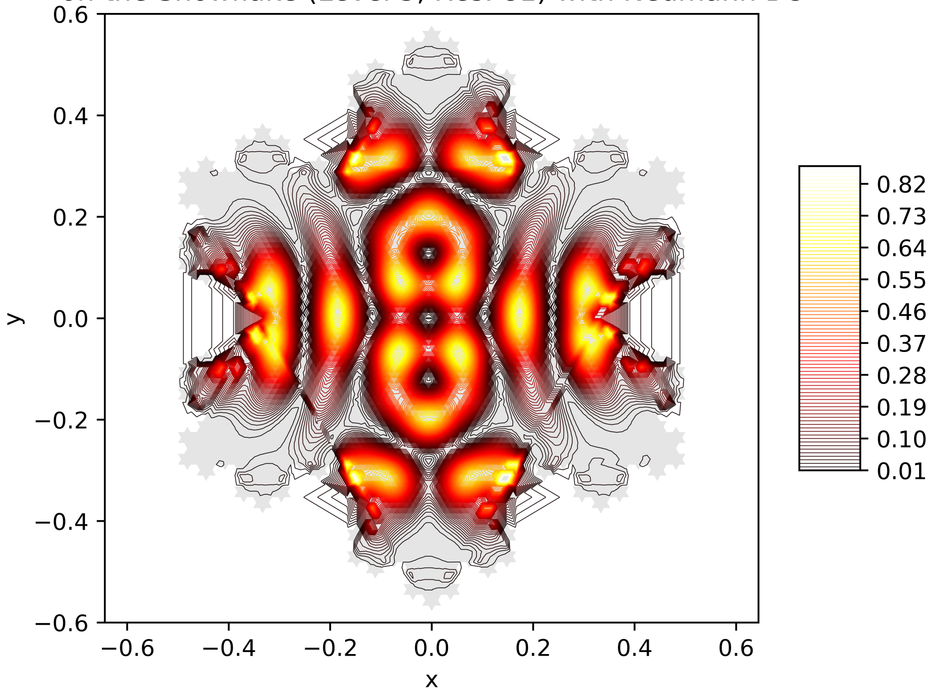
Contour Lines of the Energy Function of the 50. Eigenfunction on the Snowflake (Level 5, Res. 81) with Neumann BC
