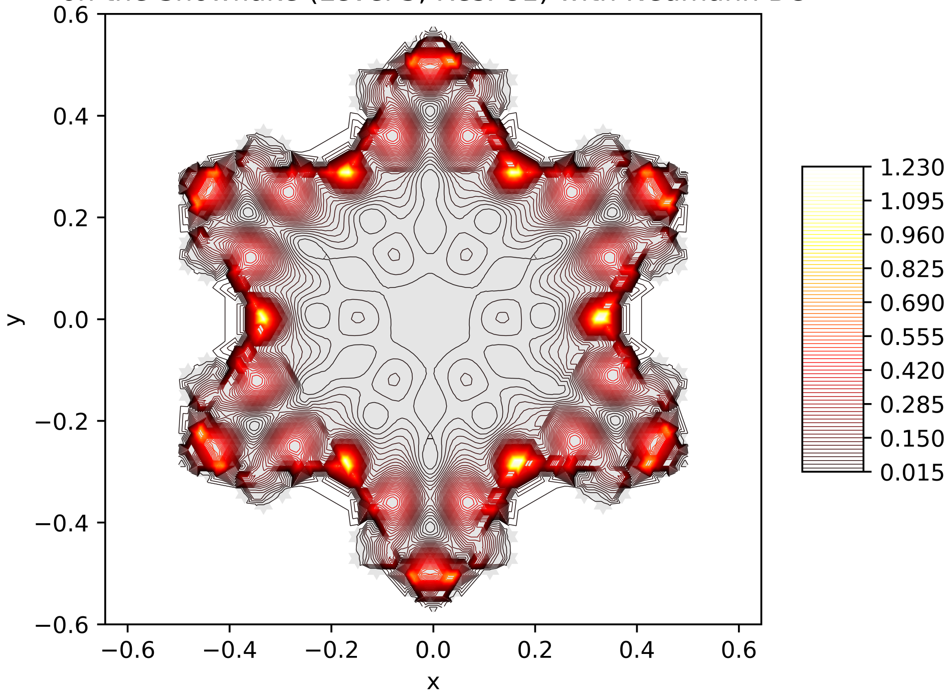
Contour Lines of the Energy Function of the 48. Eigenfunction on the Snowflake (Level 5, Res. 81) with Neumann BC
