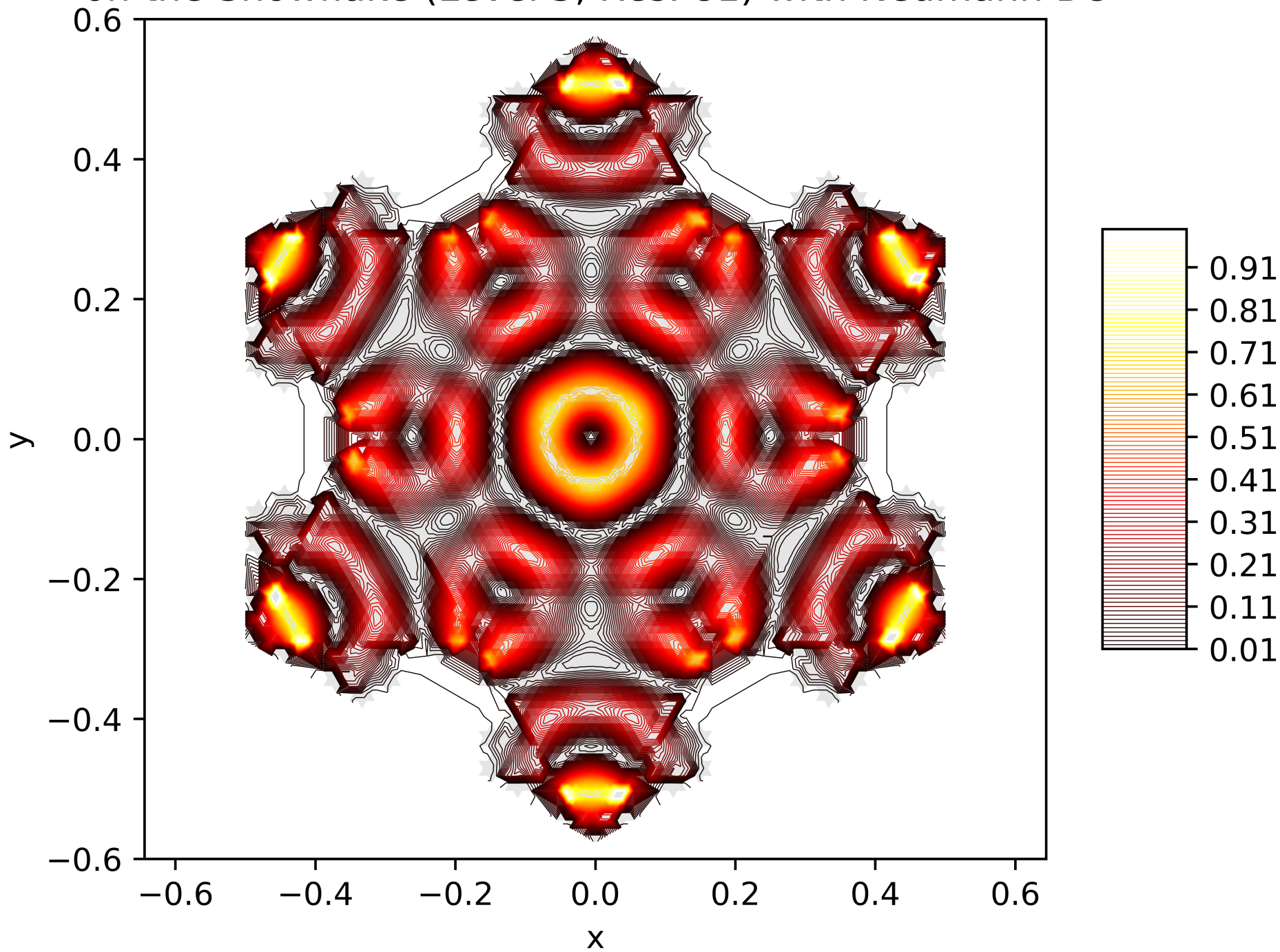
Contour Lines of the Energy Function of the 56. Eigenfunction on the Snowflake (Level 5, Res. 81) with Neumann BC
