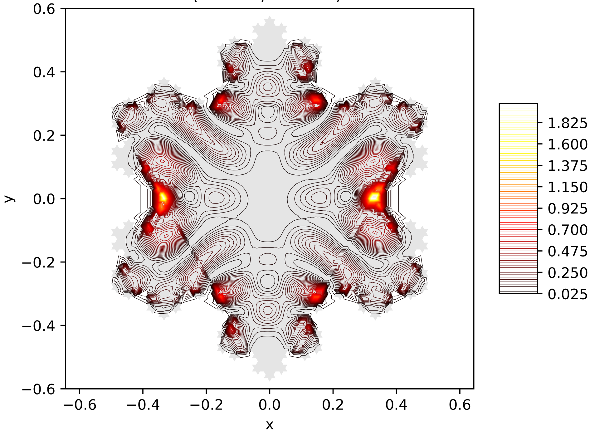
Contour Lines of the Energy Function of the 46. Eigenfunction on the Snowflake (Level 5, Res. 81) with Neumann BC
