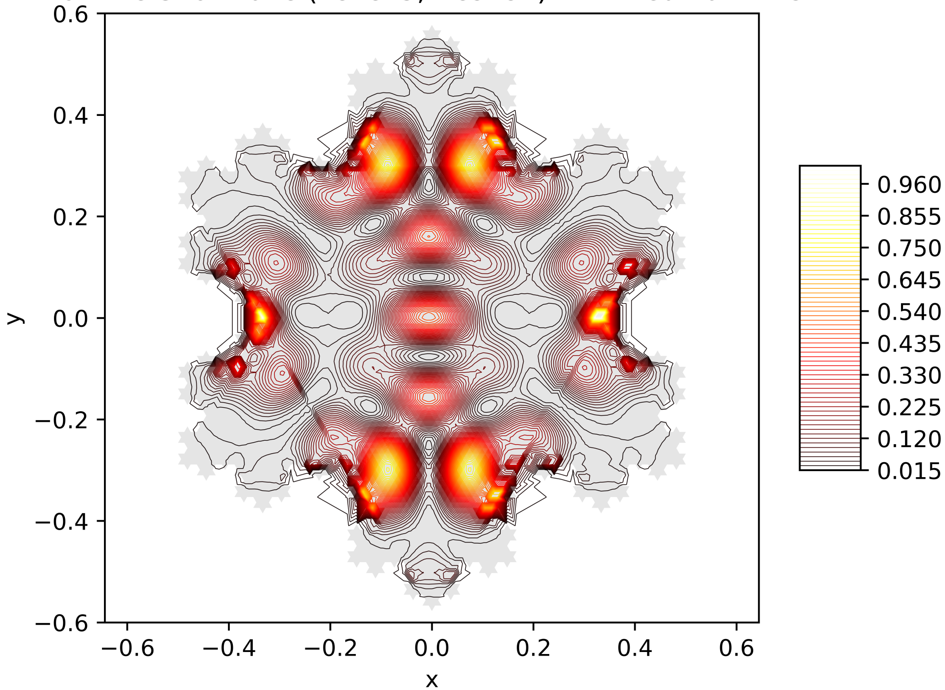
Contour Lines of the Energy Function of the 42. Eigenfunction on the Snowflake (Level 5, Res. 81) with Neumann BC
