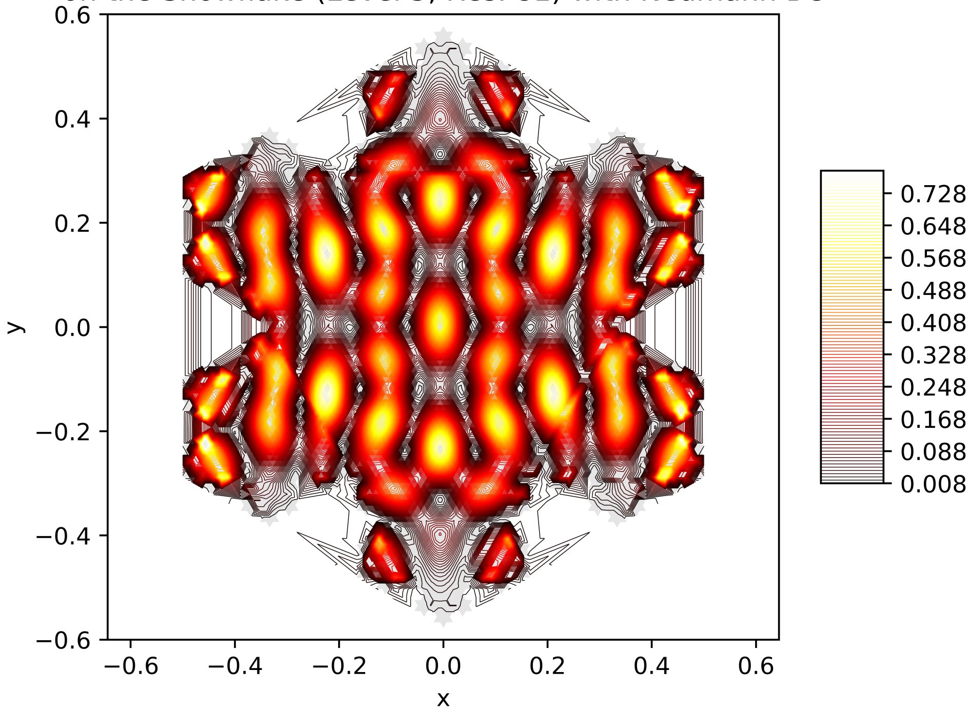
Contour Lines of the Energy Function of the 60. Eigenfunction on the Snowflake (Level 5, Res. 81) with Neumann BC
