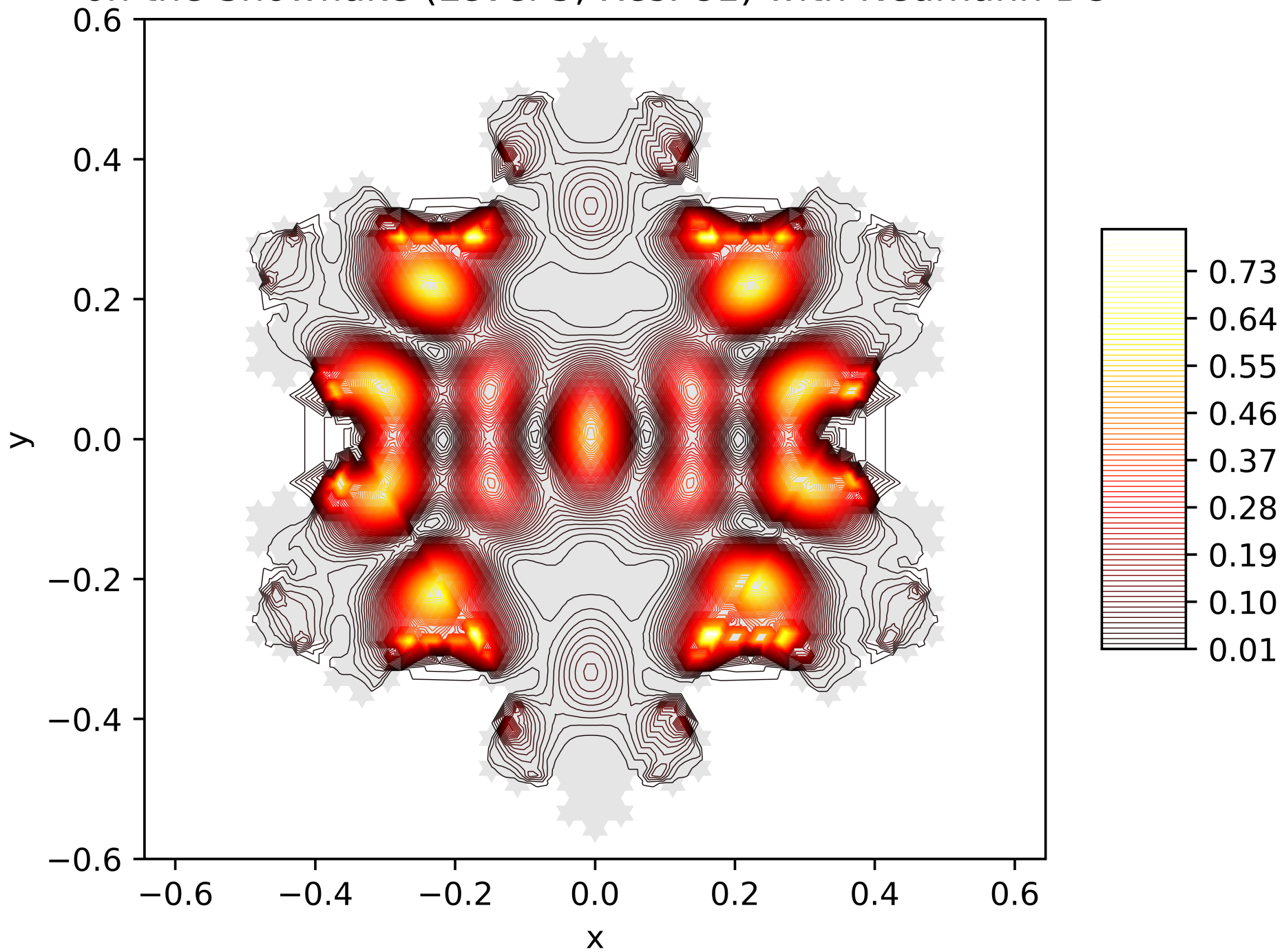
Contour Lines of the Energy Function of the 43. Eigenfunction on the Snowflake (Level 5, Res. 81) with Neumann BC
