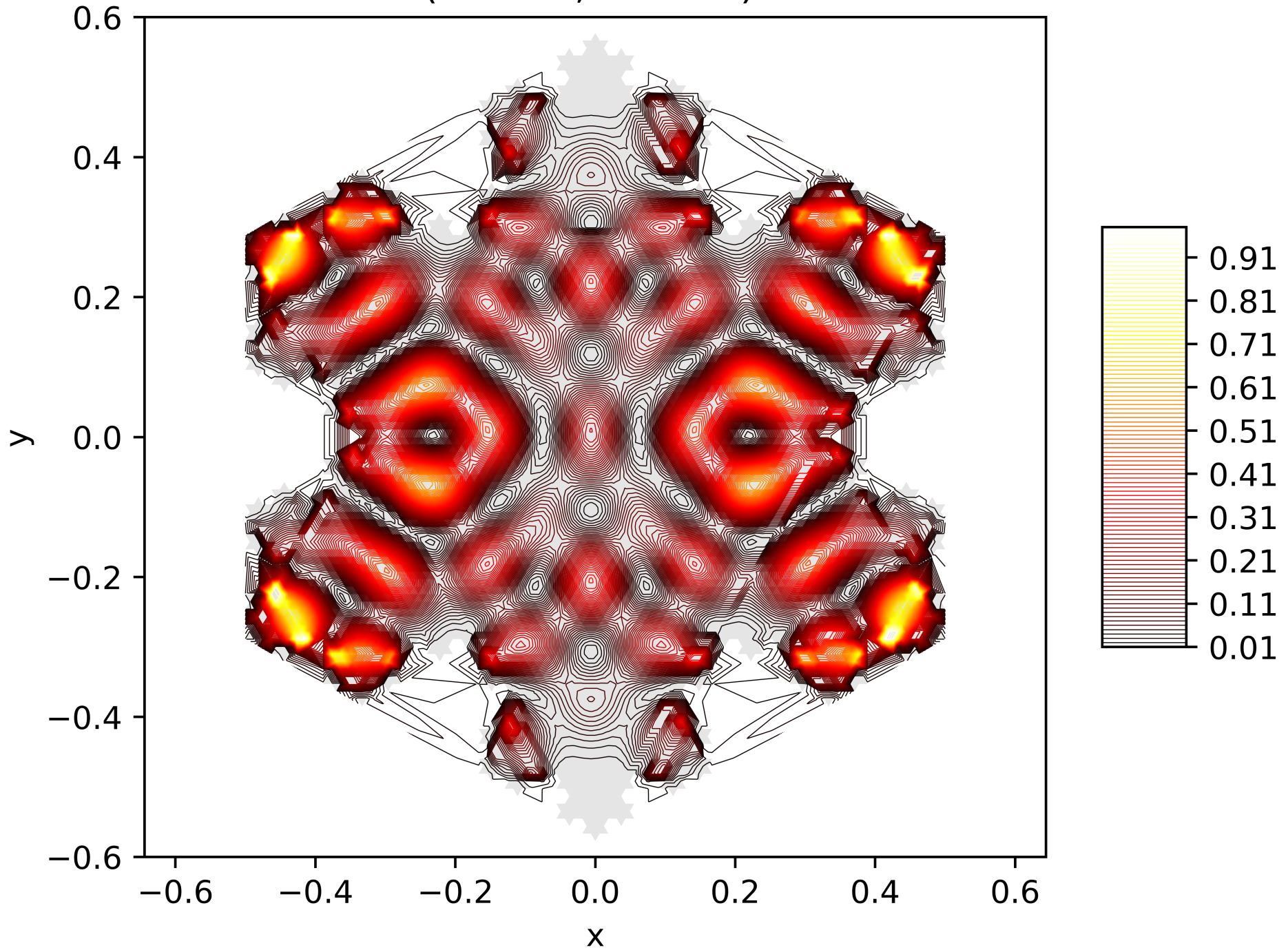
Contour Lines of the Energy Function of the 53. Eigenfunction on the Snowflake (Level 5, Res. 81) with Neumann BC
