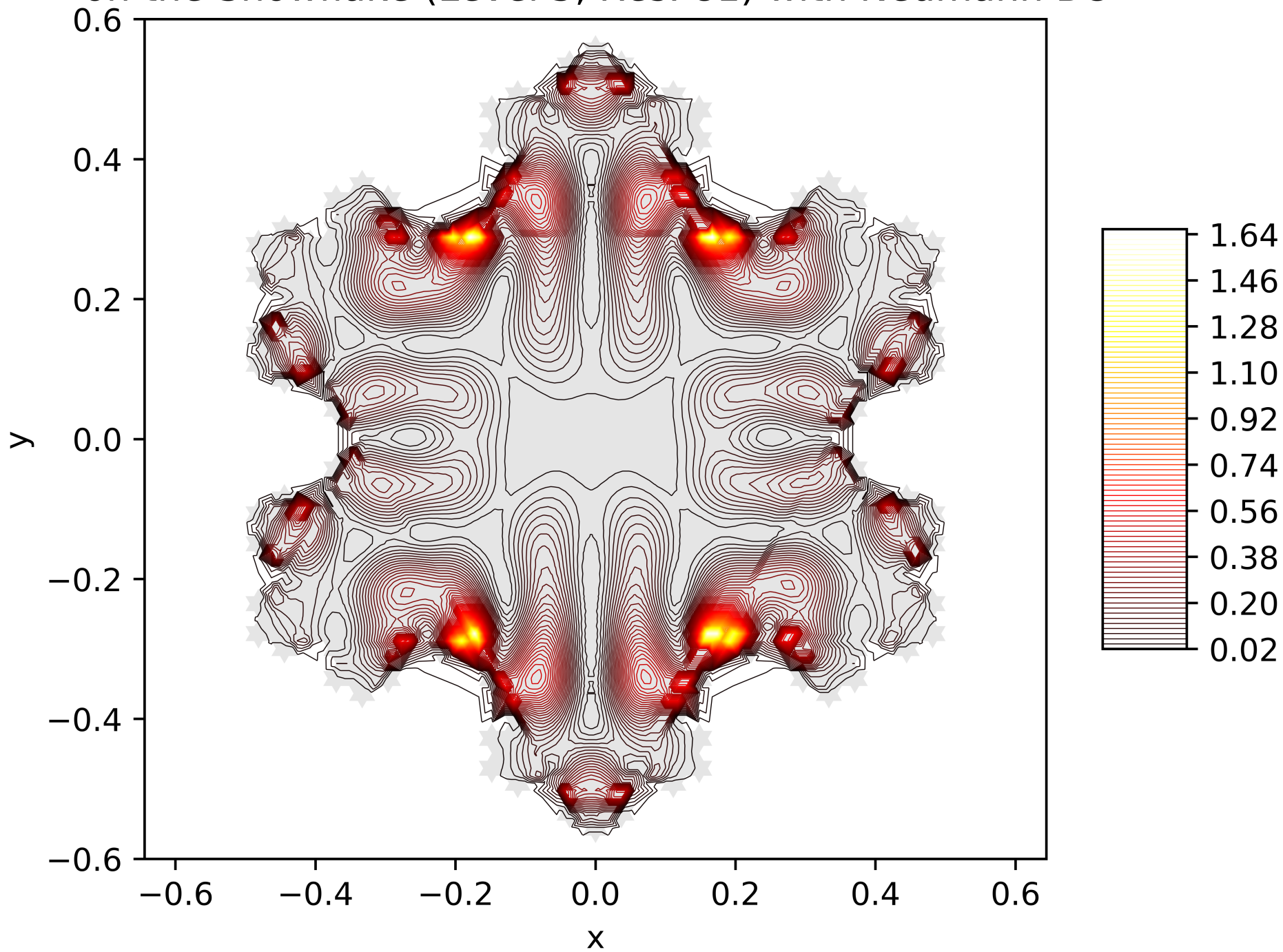
Contour Lines of the Energy Function of the 47. Eigenfunction on the Snowflake (Level 5, Res. 81) with Neumann BC
