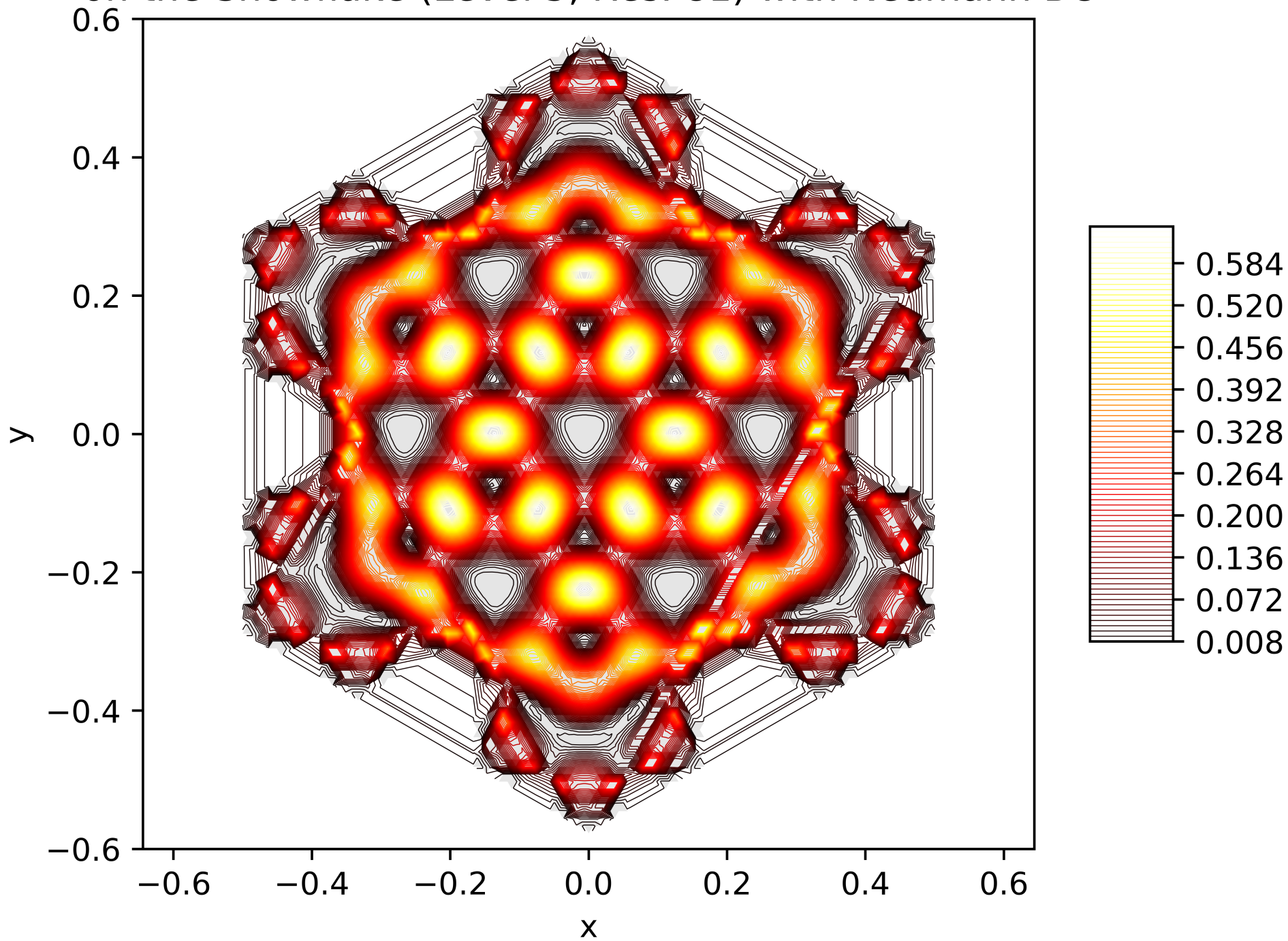
Contour Lines of the Energy Function of the 54. Eigenfunction on the Snowflake (Level 5, Res. 81) with Neumann BC
