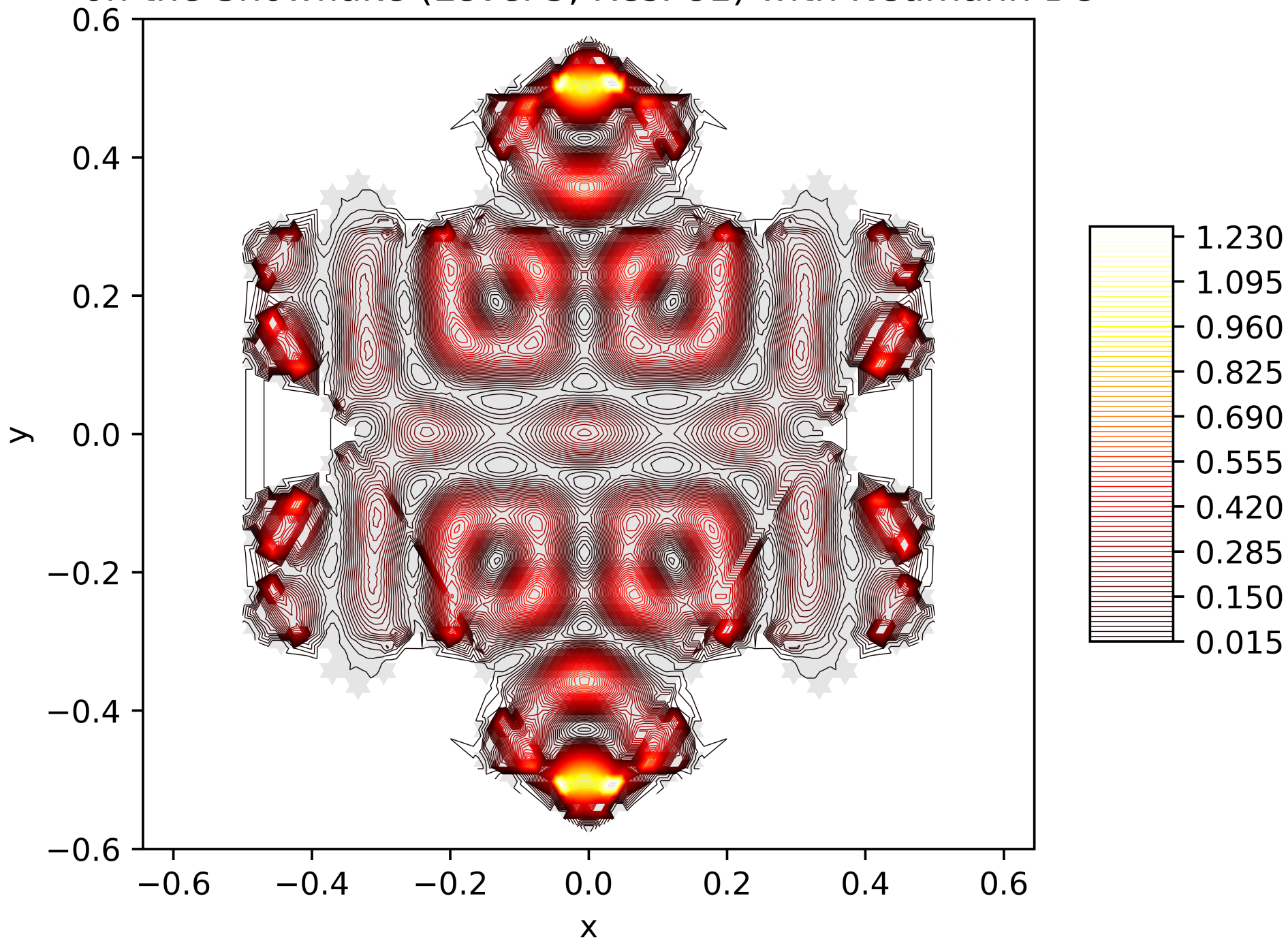
Contour Lines of the Energy Function of the 52. Eigenfunction on the Snowflake (Level 5, Res. 81) with Neumann BC
