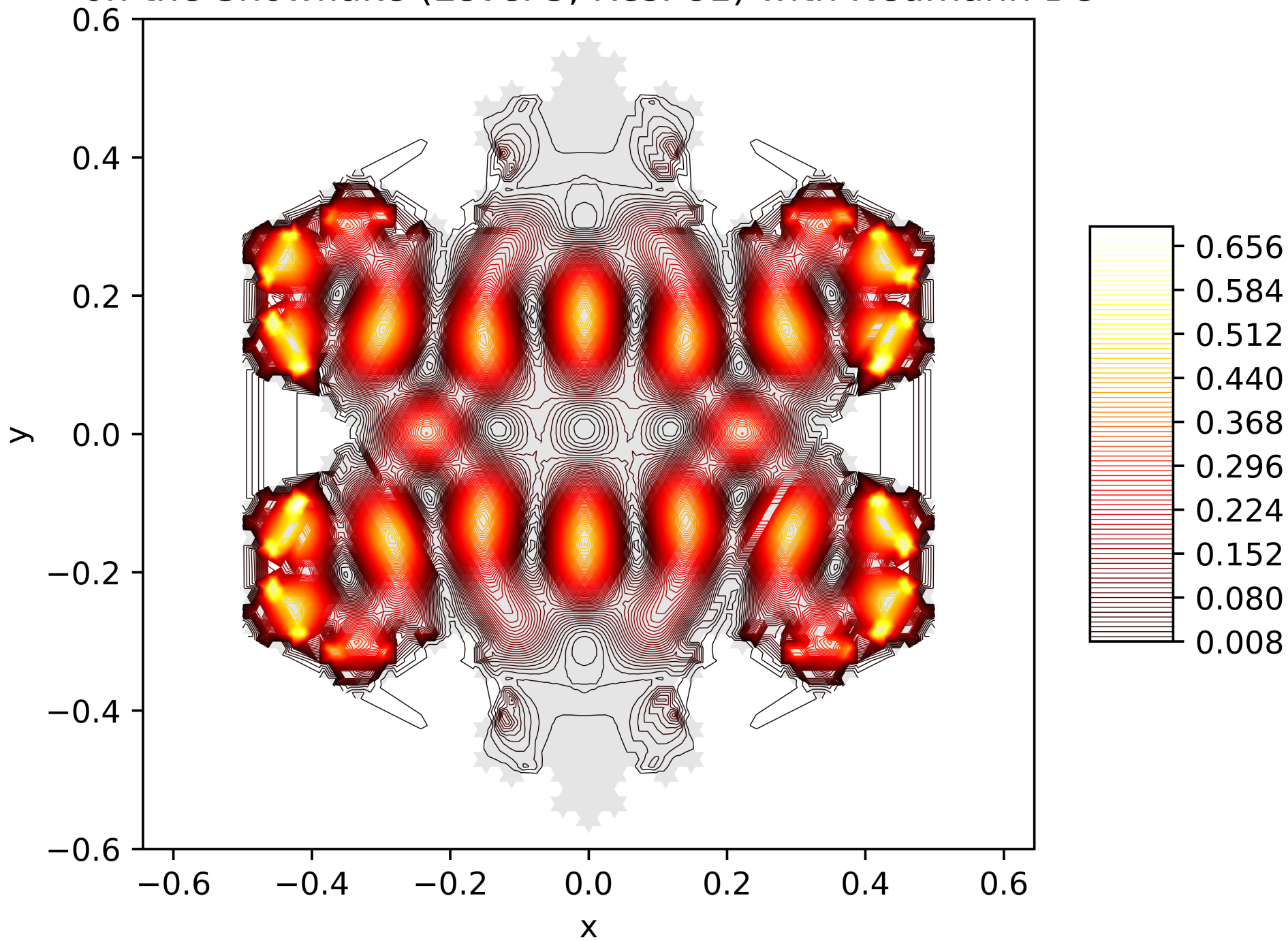
Contour Lines of the Energy Function of the 45. Eigenfunction on the Snowflake (Level 5, Res. 81) with Neumann BC
