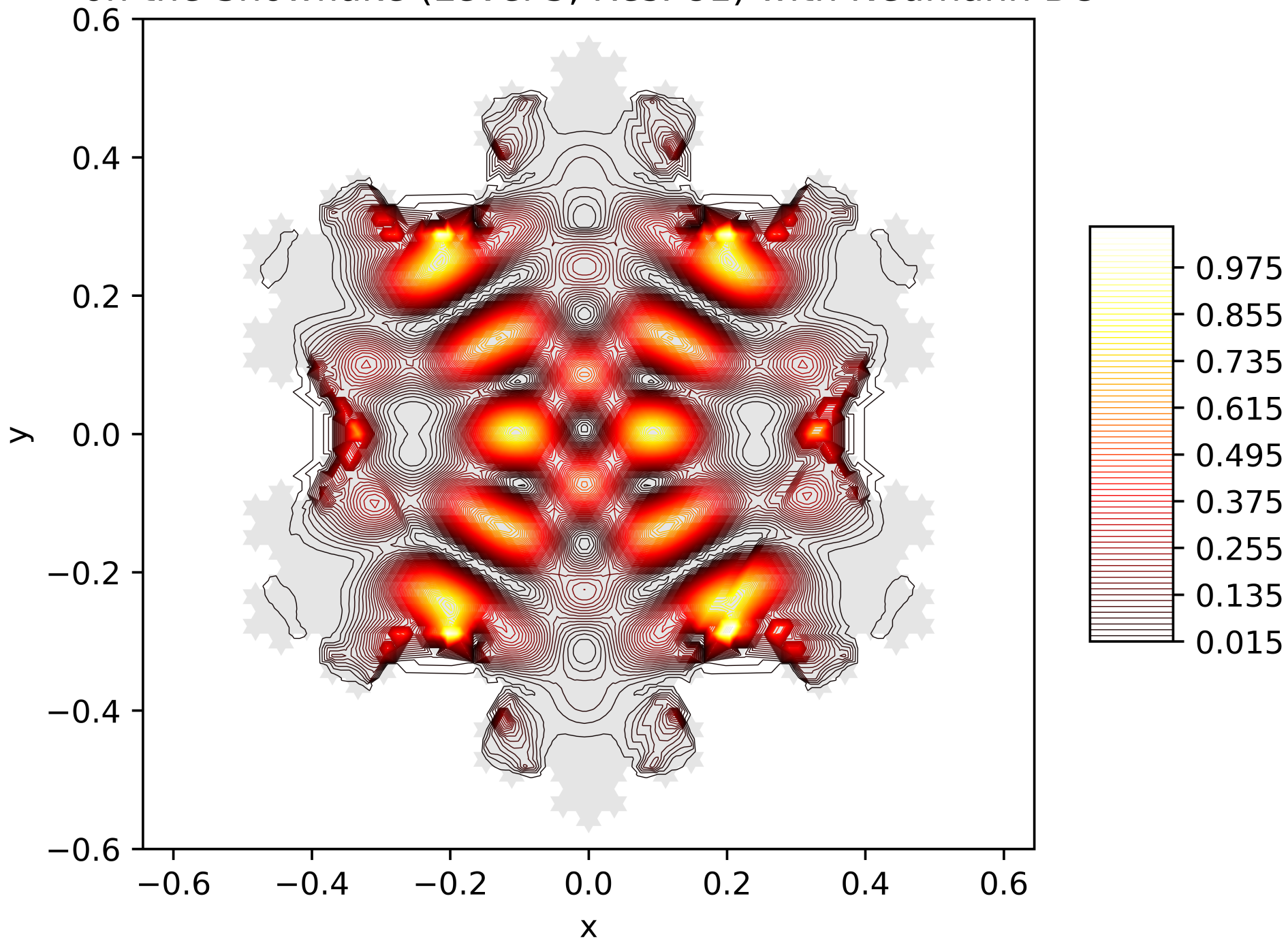
Contour Lines of the Energy Function of the 51. Eigenfunction on the Snowflake (Level 5, Res. 81) with Neumann BC
