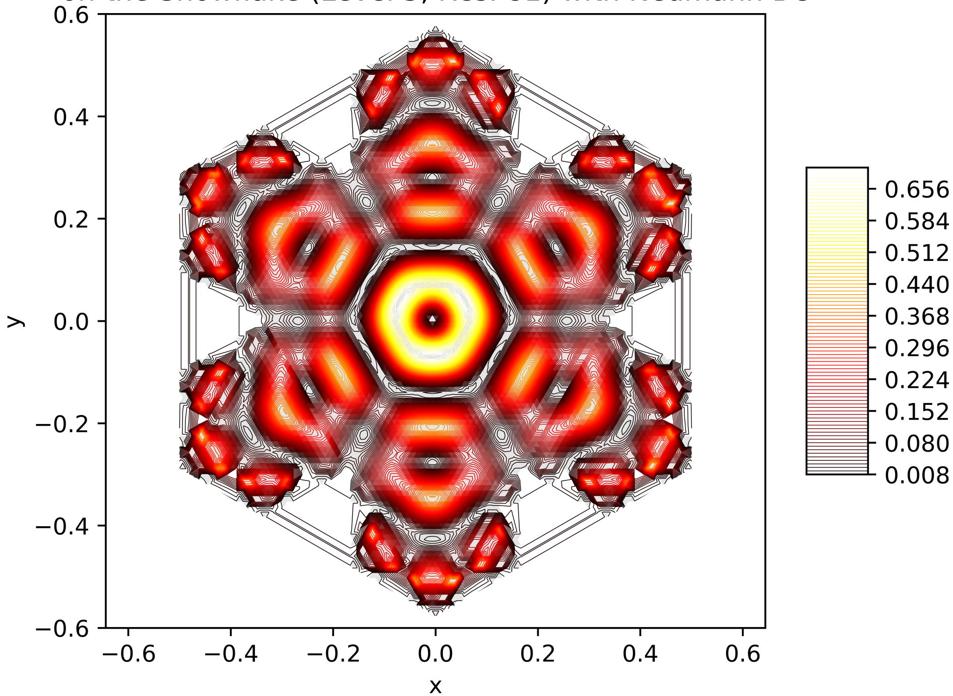
Contour Lines of the Energy Function of the 49. Eigenfunction on the Snowflake (Level 5, Res. 81) with Neumann BC
