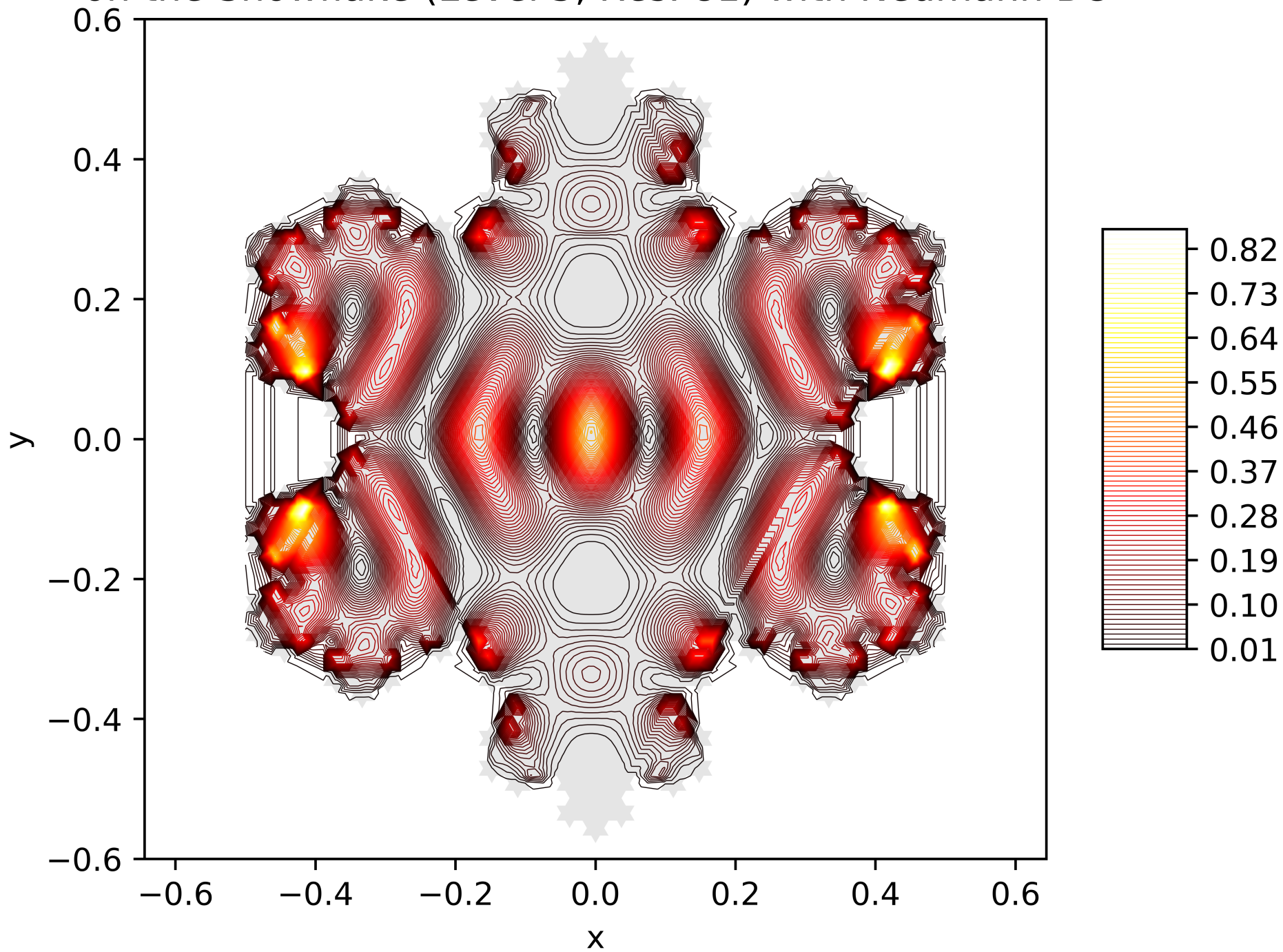
Contour Lines of the Energy Function of the 41. Eigenfunction on the Snowflake (Level 5, Res. 81) with Neumann BC
