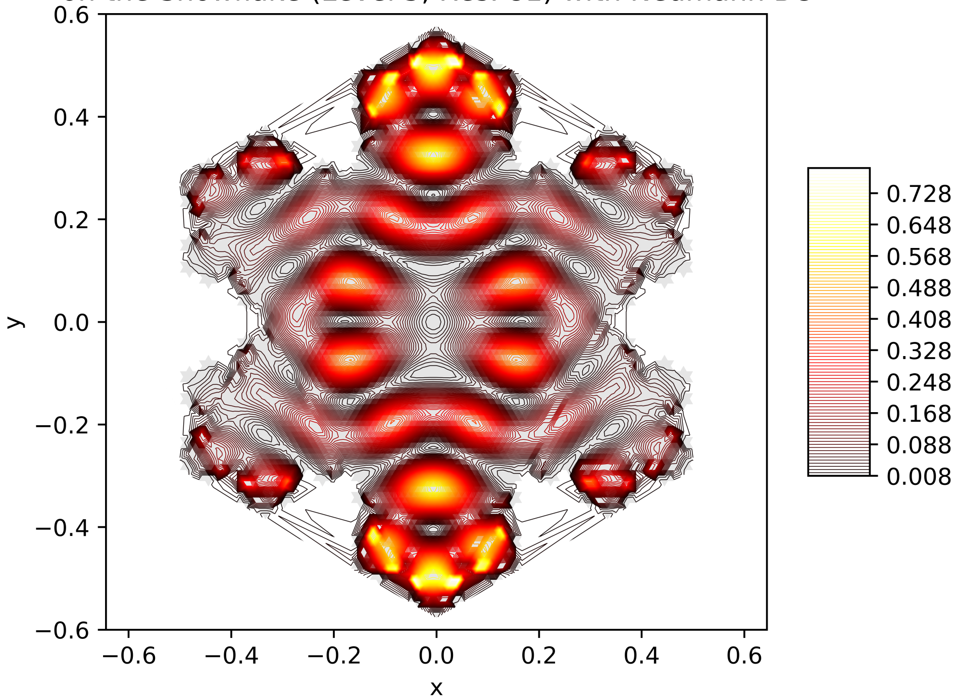
Contour Lines of the Energy Function of the 44. Eigenfunction on the Snowflake (Level 5, Res. 81) with Neumann BC
