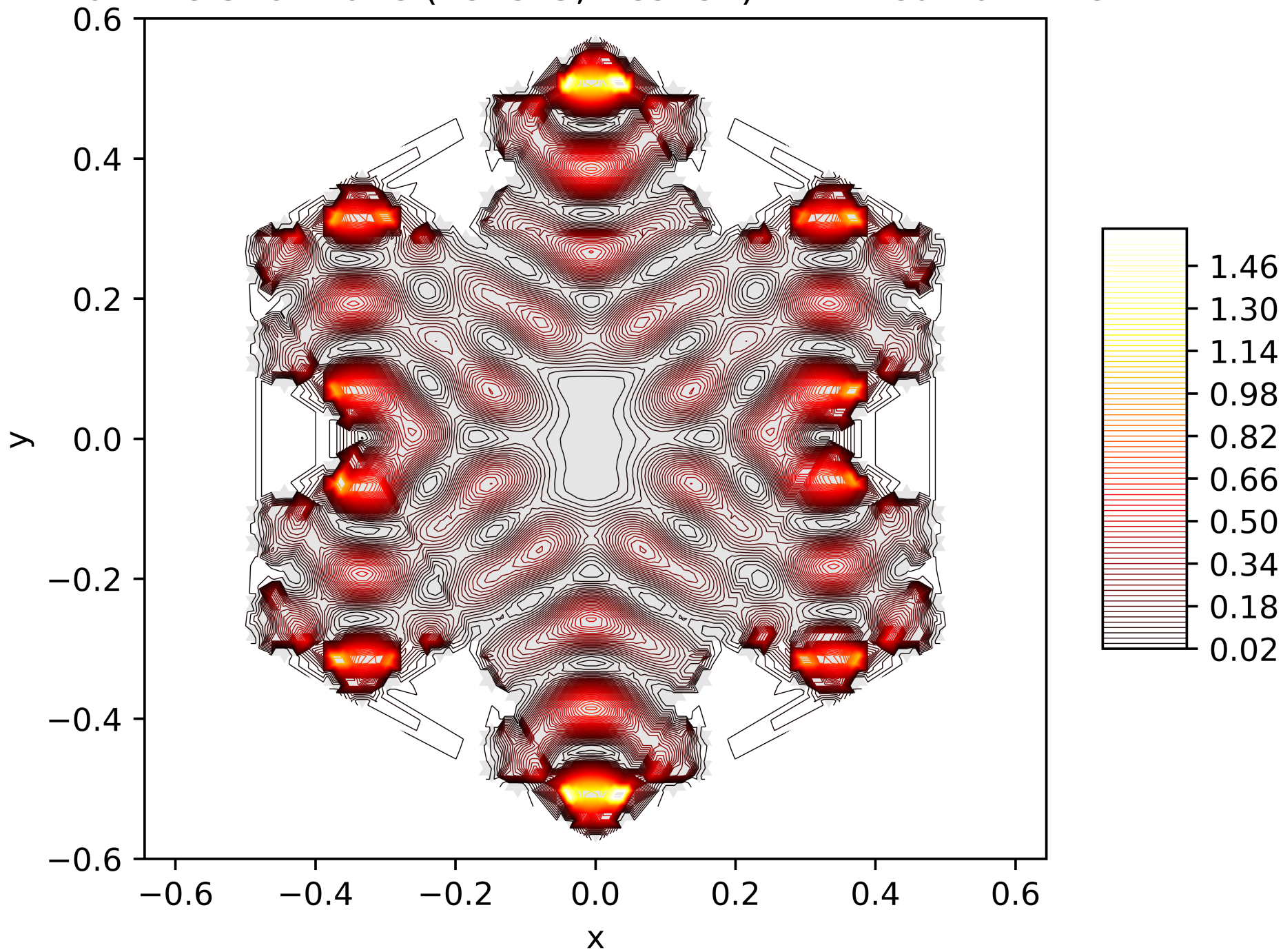
Contour Lines of the Energy Function of the 57. Eigenfunction on the Snowflake (Level 5, Res. 81) with Neumann BC
