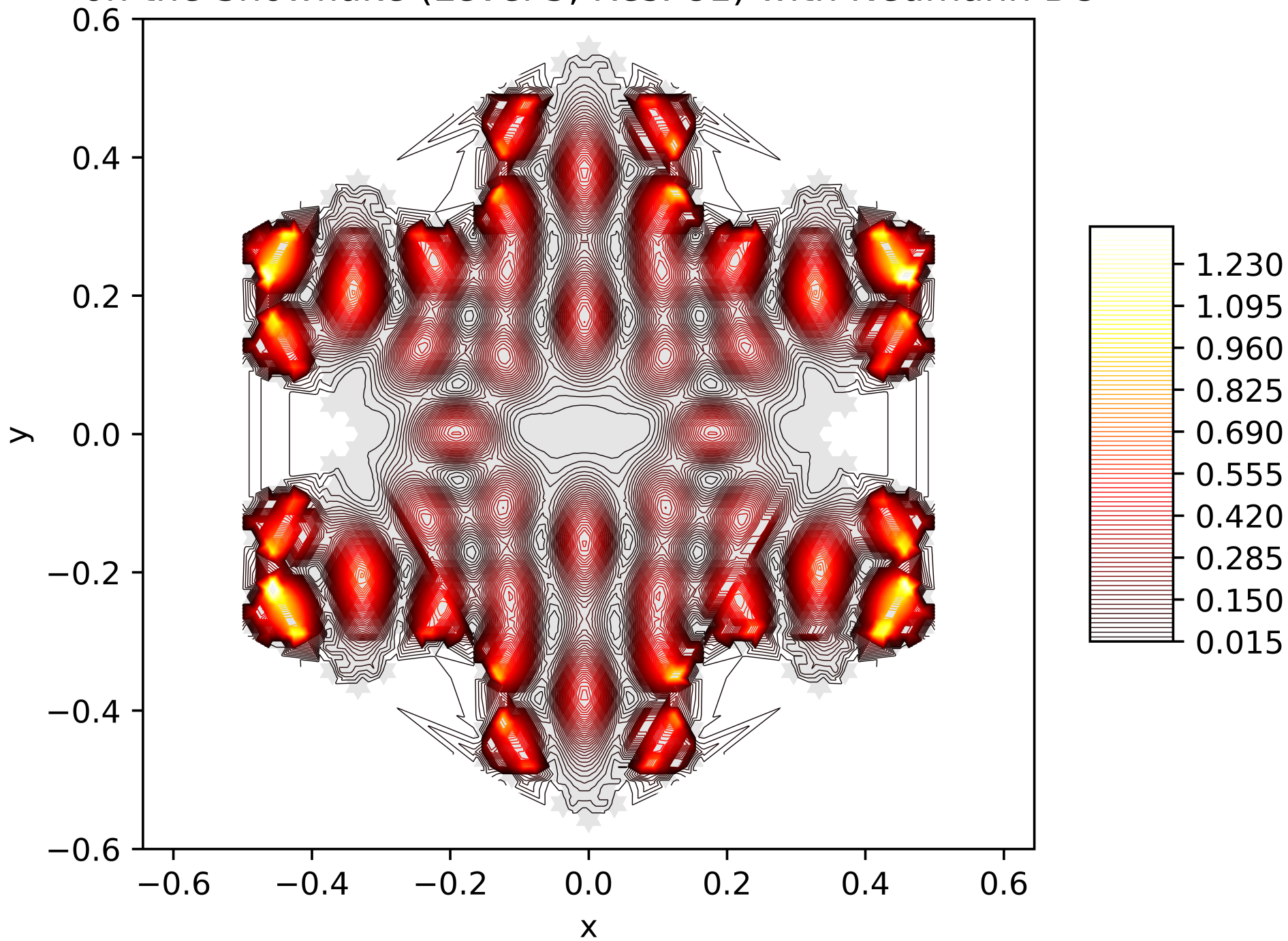
Contour Lines of the Energy Function of the 58. Eigenfunction on the Snowflake (Level 5, Res. 81) with Neumann BC
