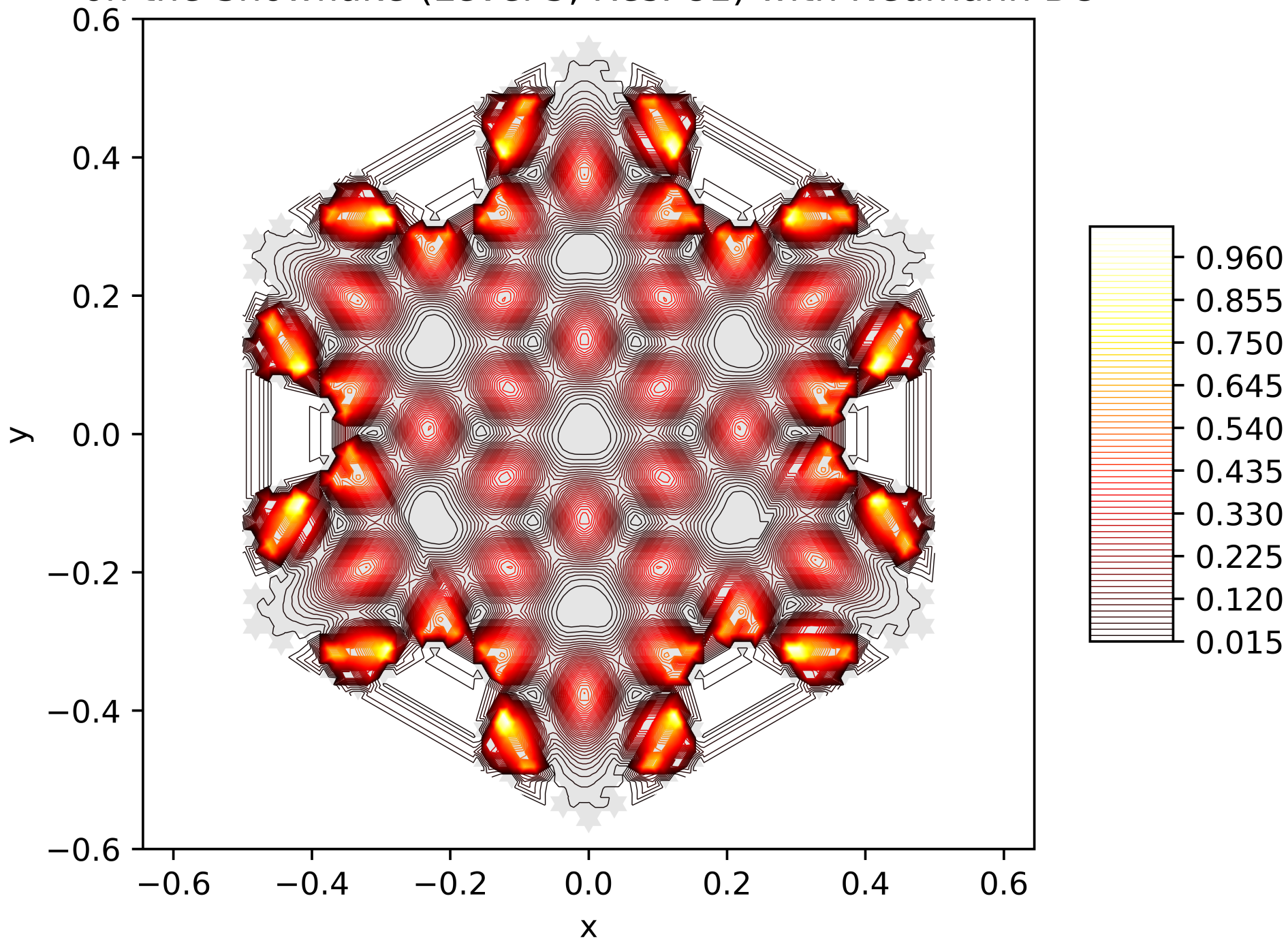
Contour Lines of the Energy Function of the 55. Eigenfunction on the Snowflake (Level 5, Res. 81) with Neumann BC
